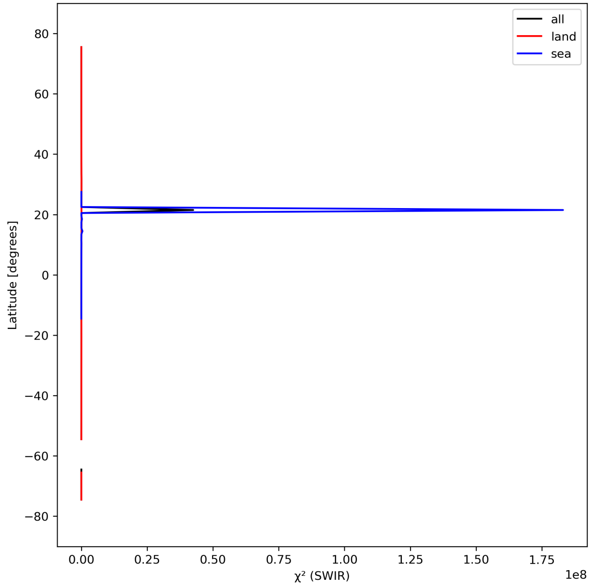
Figure 17: Zonal average of “ \chi^2 (SWIR)” for 2024-03-20 to 2024-03-22.
