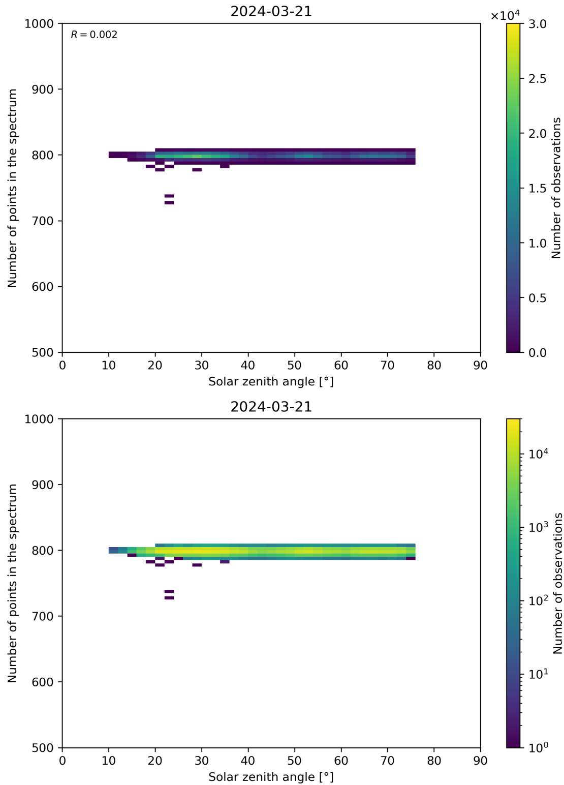
Figure 103: Scatter density plot of “Solar zenith angle” against “Number of points in the spectrum” for 2024-03-20 to 2024-03-22.
