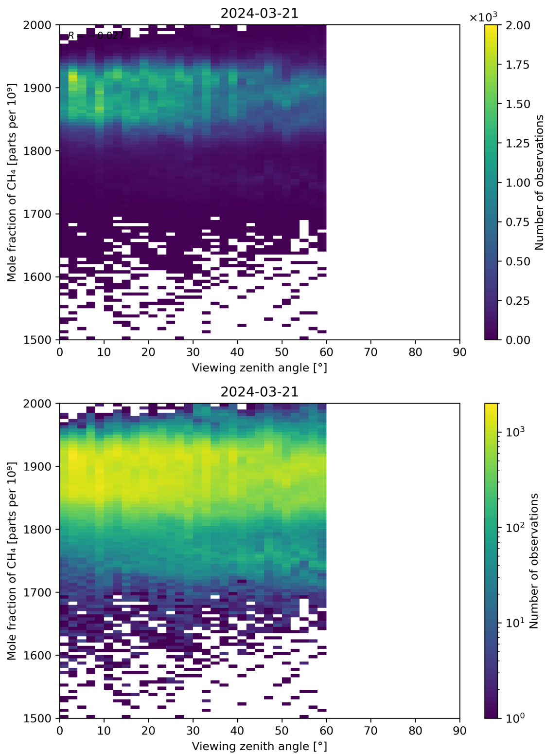
Figure 110: Scatter density plot of “Viewing zenith angle” against “Mole fraction of CH 4 ” for 2024-03-20 to 2024-03-22.
