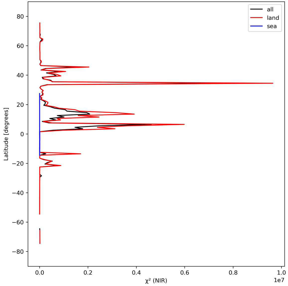
Figure 18: Zonal average of “ \chi^2 (NIR)” for 2024-03-20 to 2024-03-22.
