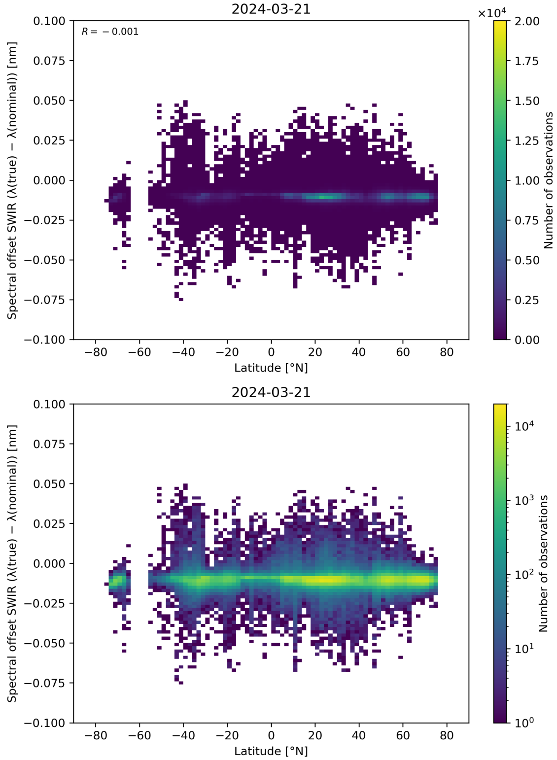
Figure 62: Scatter density plot of “Latitude” against “Spectral offset SWIR ( \lambda(\text{true}) - \lambda(\text{nominal}) )” for 2024-03-20 to 2024-03-22.
