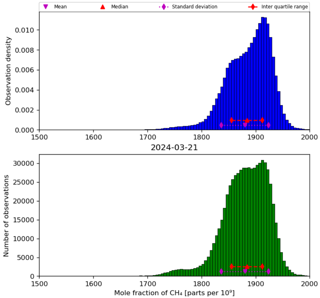
Figure 23: Histogram of “Mole fraction of CH 4 ” for 2024-03-20 to 2024-03-22
