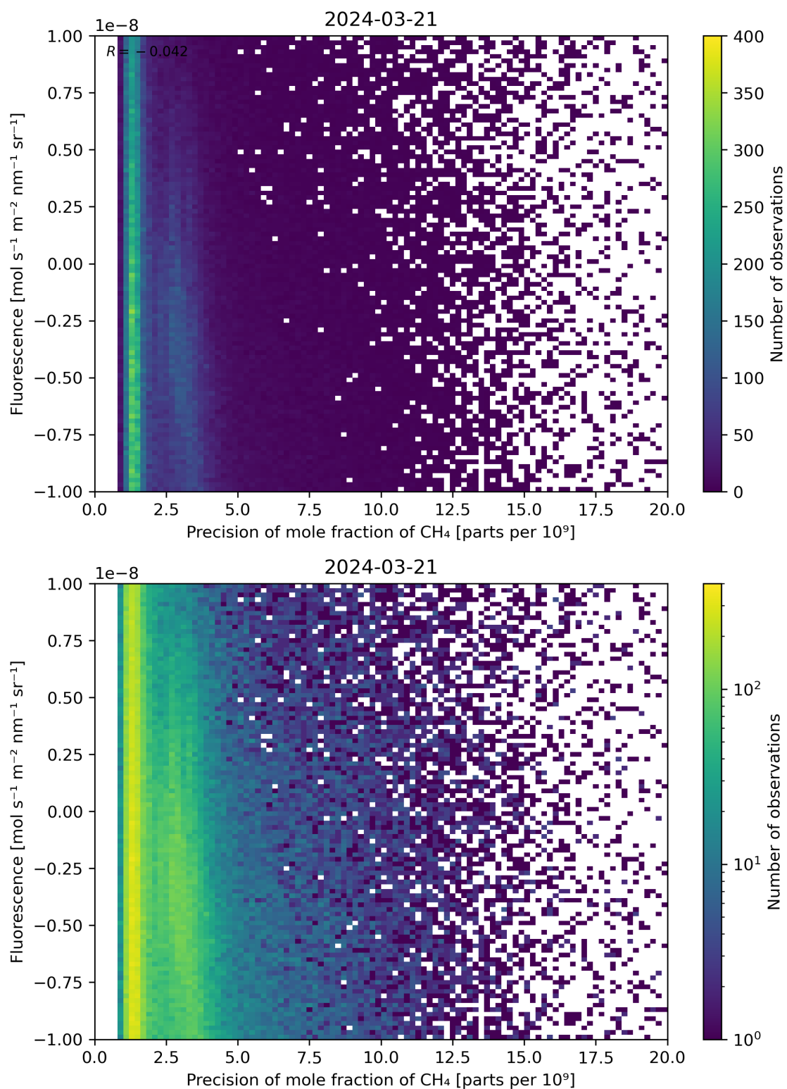
Figure 81: Scatter density plot of “Precision of mole fraction of CH 4 ” against “Fluorescence” for 2024-03-20 to 2024-03-22.
