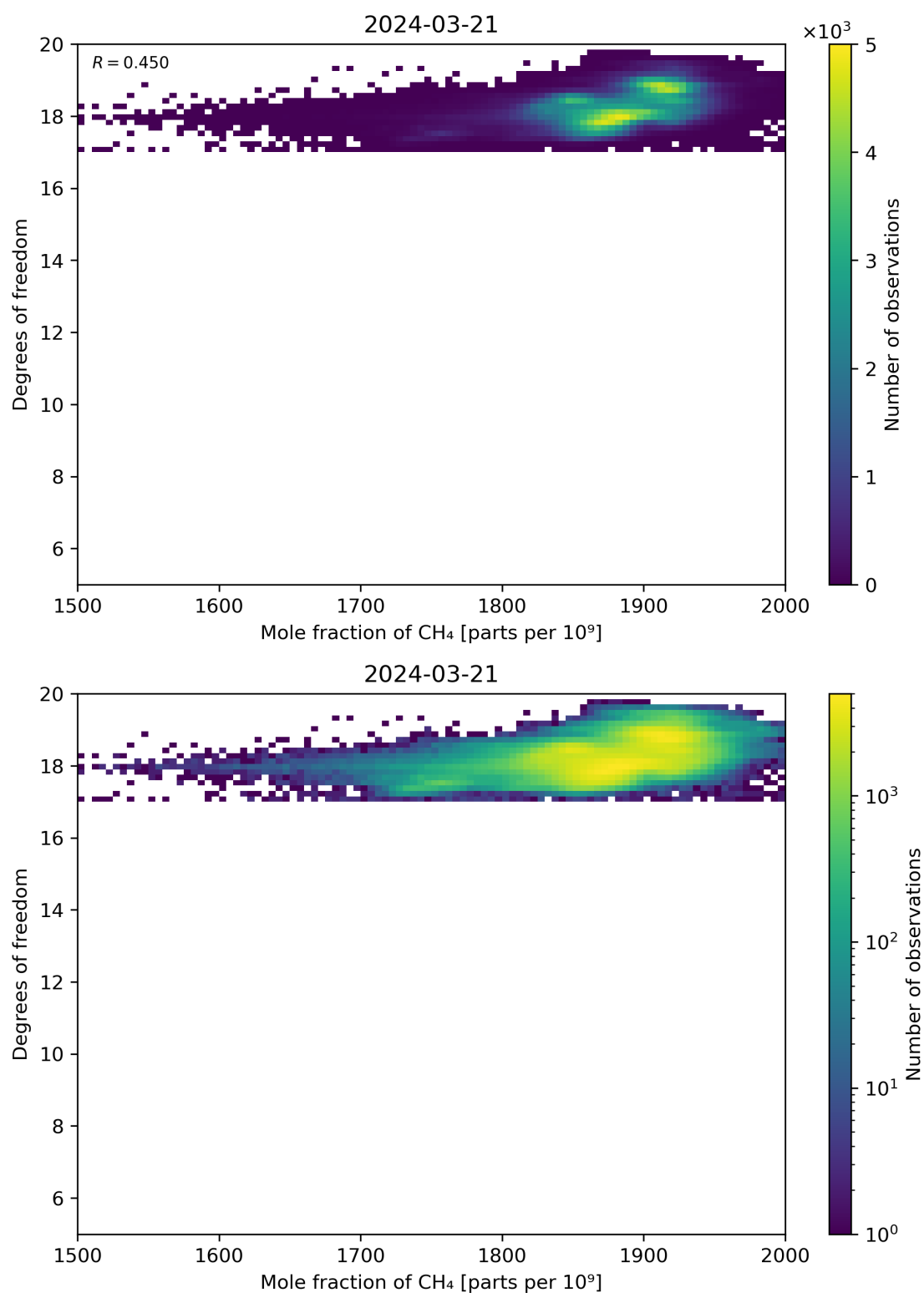
Figure 72: Scatter density plot of “Mole fraction of CH 4 ” against “Degrees of freedom” for 2024-03-20 to 2024-03-22.
