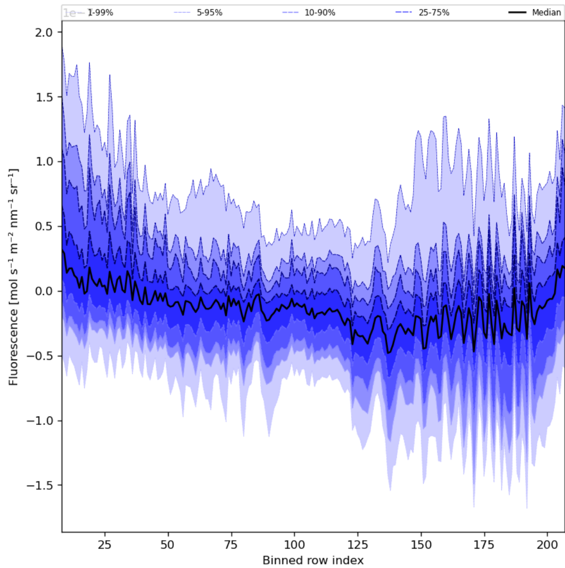
Figure 43: Along track statistics of “Fluorescence” for 2024-03-20 to 2024-03-22
