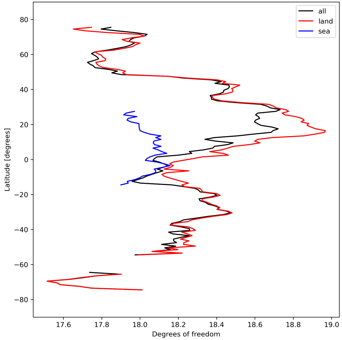
Figure 19: Zonal average of “Degrees of freedom” for 2024-03-20 to 2024-03-22.
