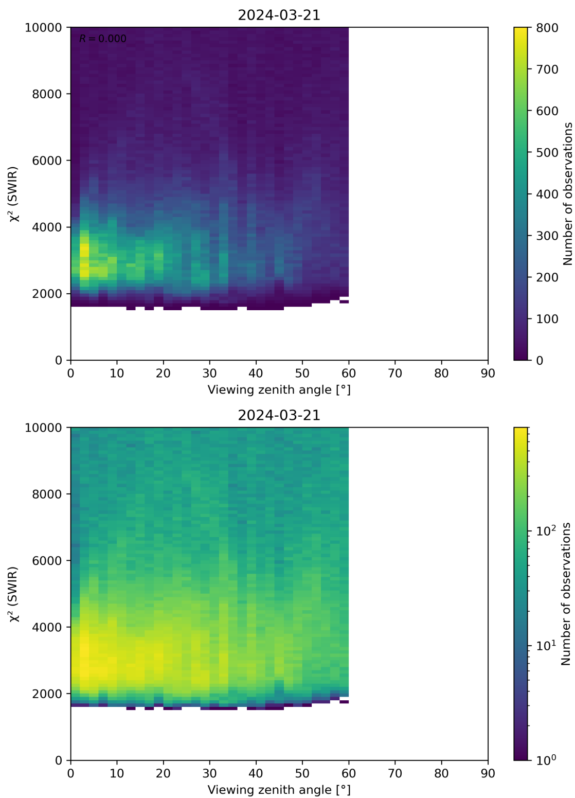
Figure 106: Scatter density plot of “Viewing zenith angle” against “ \chi^2 (SWIR)” for 2024-03-20 to 2024-03-22.
