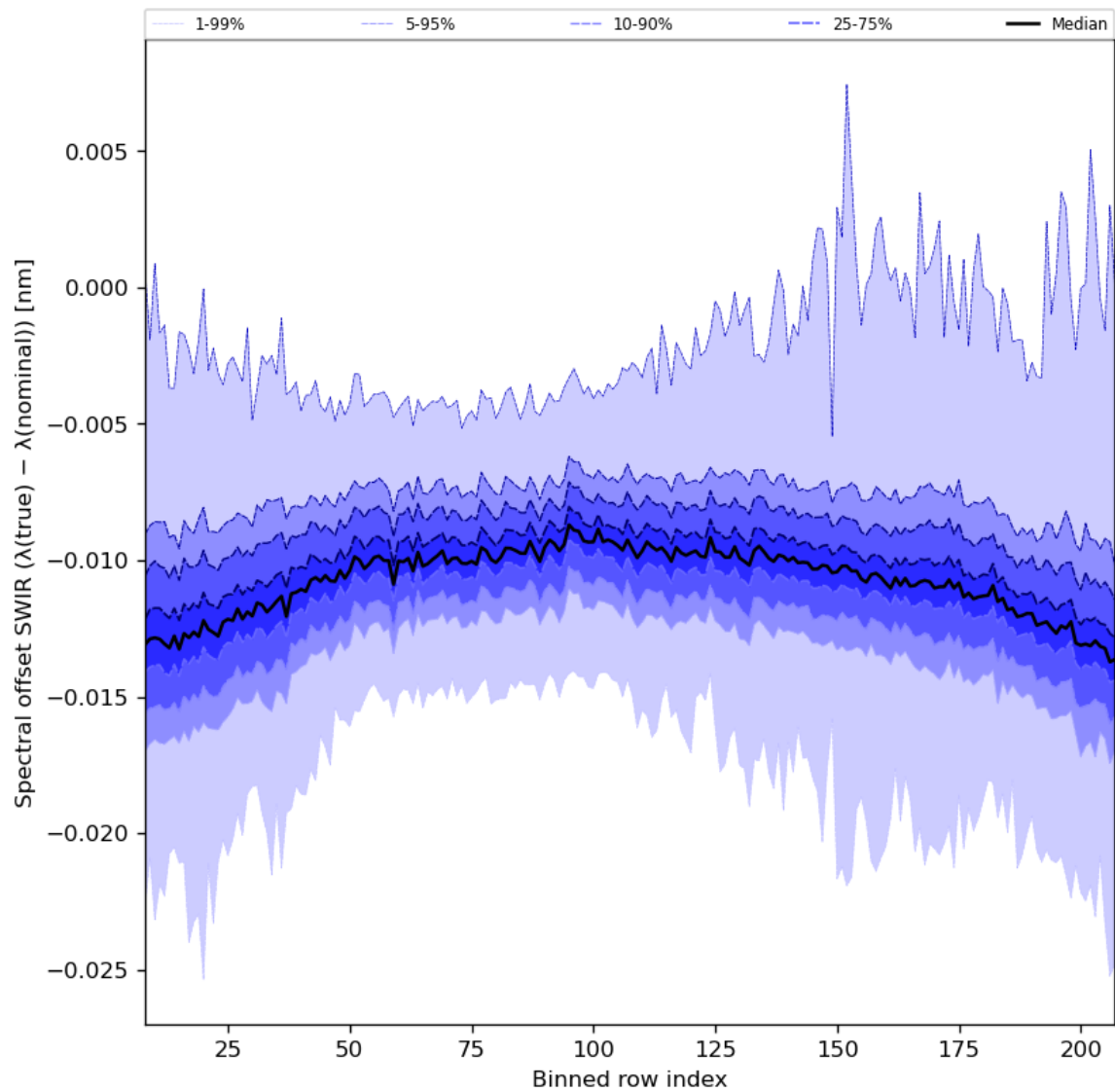
Figure 38: Along track statistics of “Spectral offset SWIR ( \lambda(\text{true}) - \lambda(\text{nominal}) )” for 2024-03-20 to 2024-03-22
