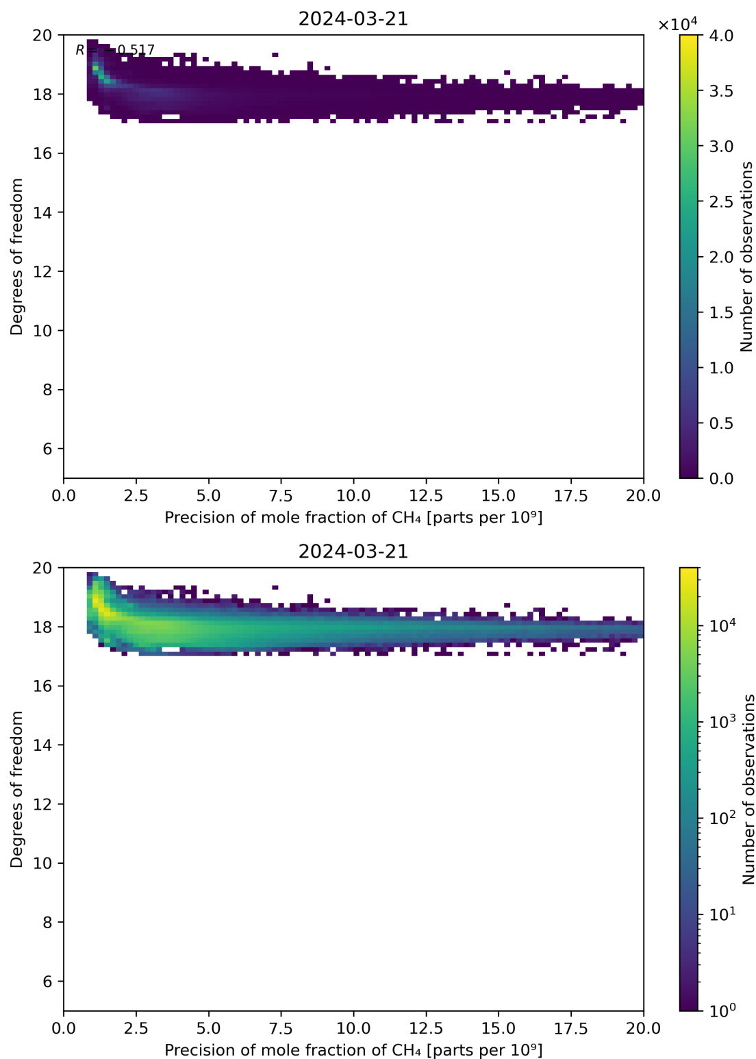
Figure 80: Scatter density plot of “Precision of mole fraction of CH 4 ” against “Degrees of freedom” for 2024-03-20 to 2024-03-22.
