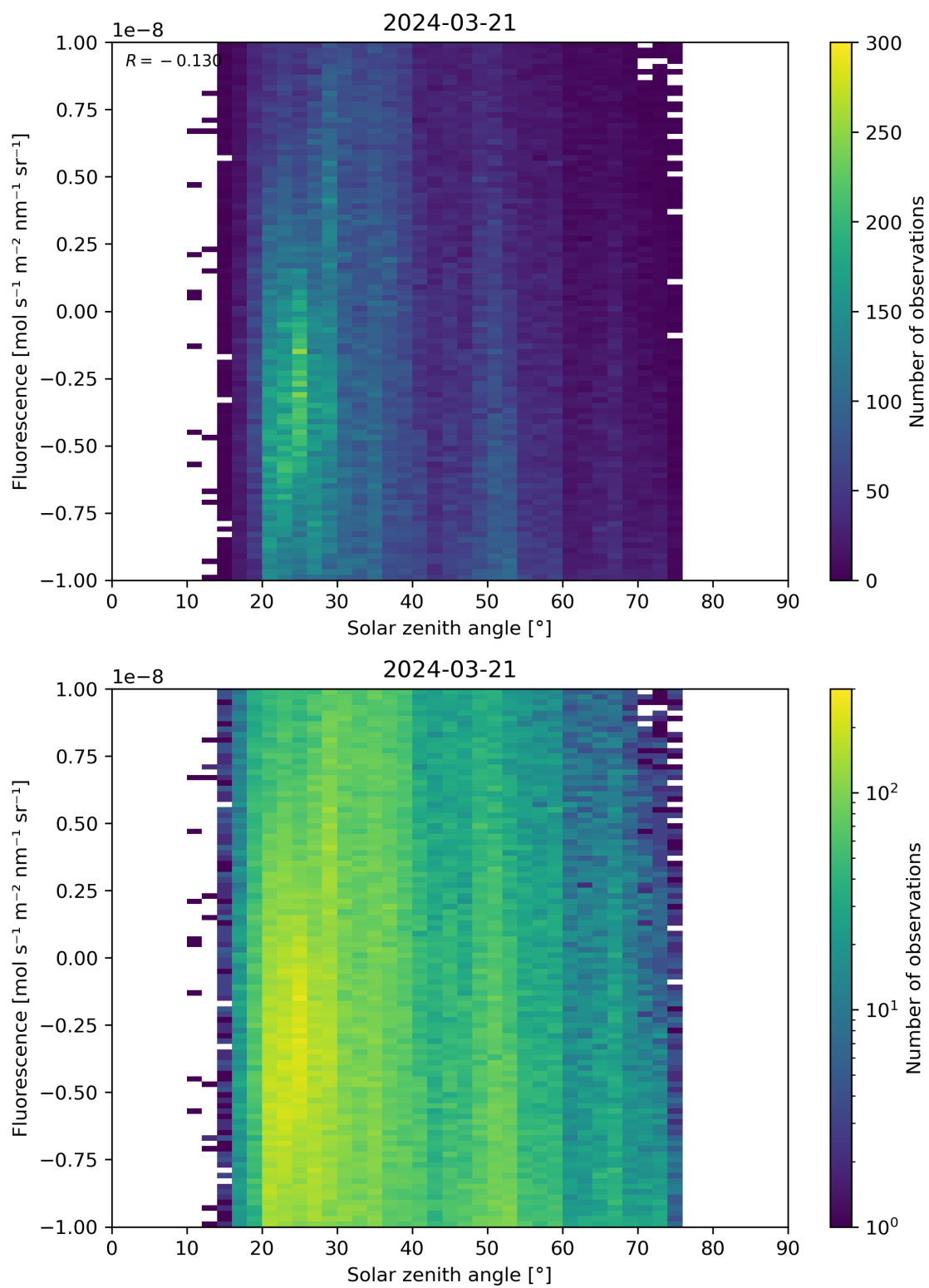
Figure 97: Scatter density plot of “Solar zenith angle” against “Fluorescence” for 2024-03-20 to 2024-03-22.
