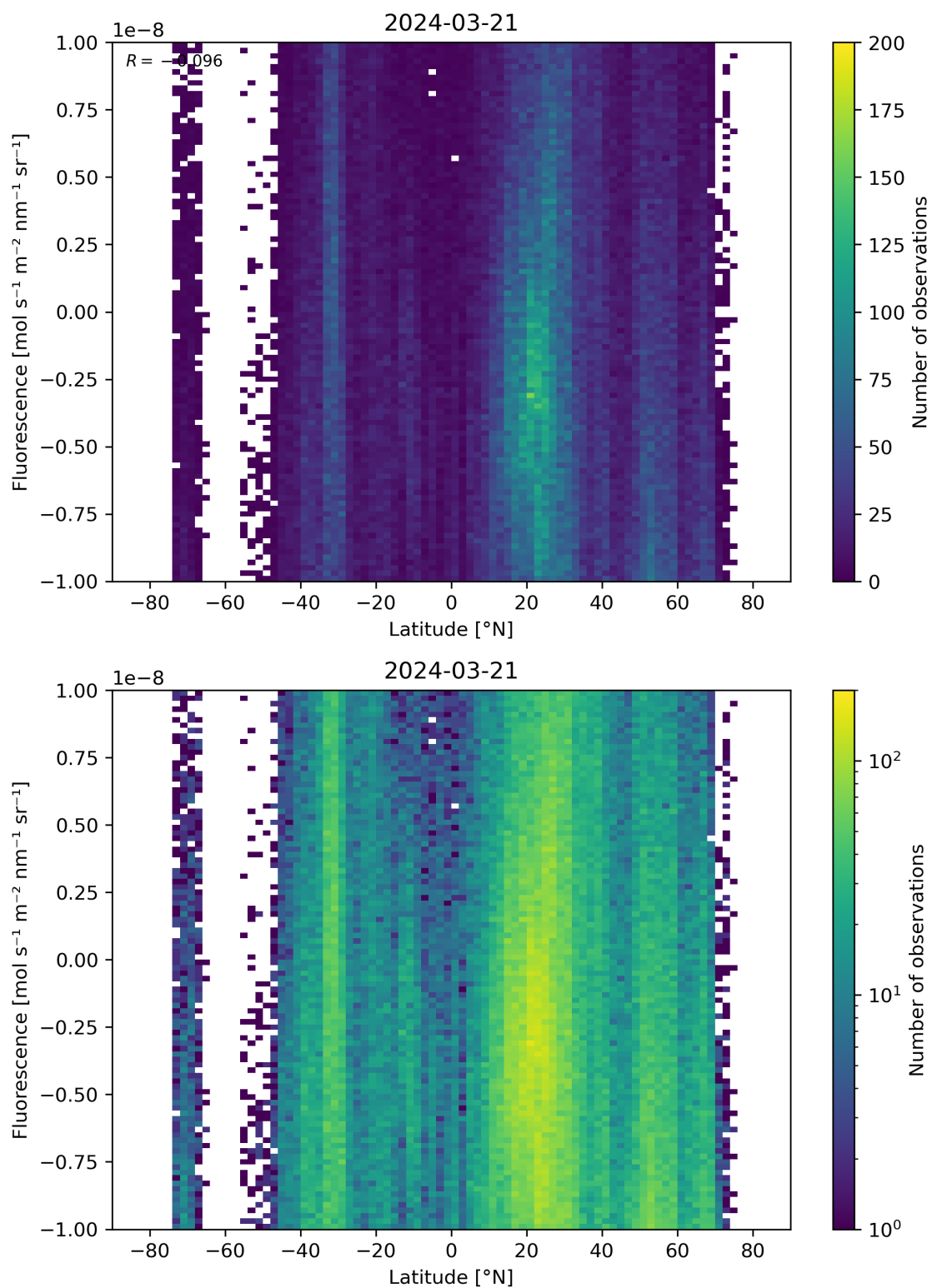
Figure 56: Scatter density plot of “Latitude” against “Fluorescence” for 2024-03-20 to 2024-03-22.
