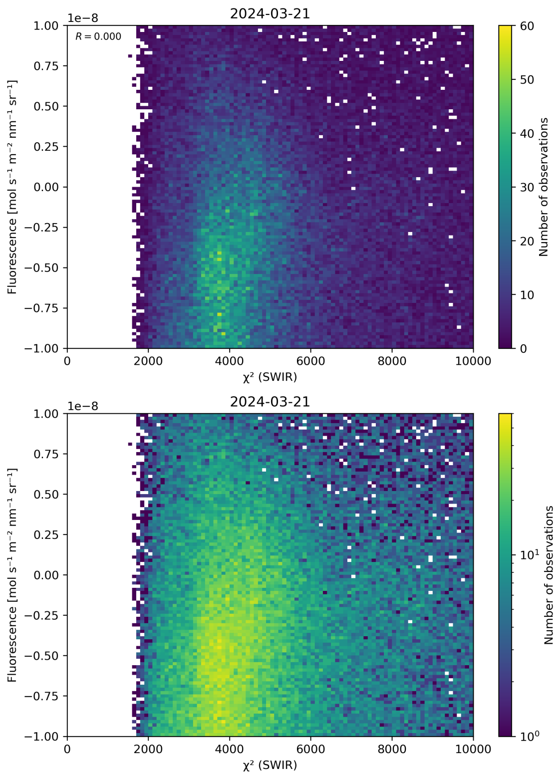
Figure 49: Scatter density plot of “ \chi^2 (SWIR)” against “Fluorescence” for 2024-03-20 to 2024-03-22.
