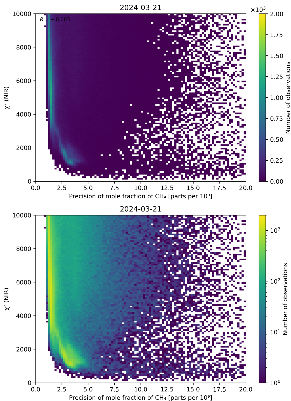
Figure 78: Scatter density plot of “Precision of mole fraction of CH 4 ” against “ \chi^2 (NIR)” for 2024-03-20 to 2024-03-22.
