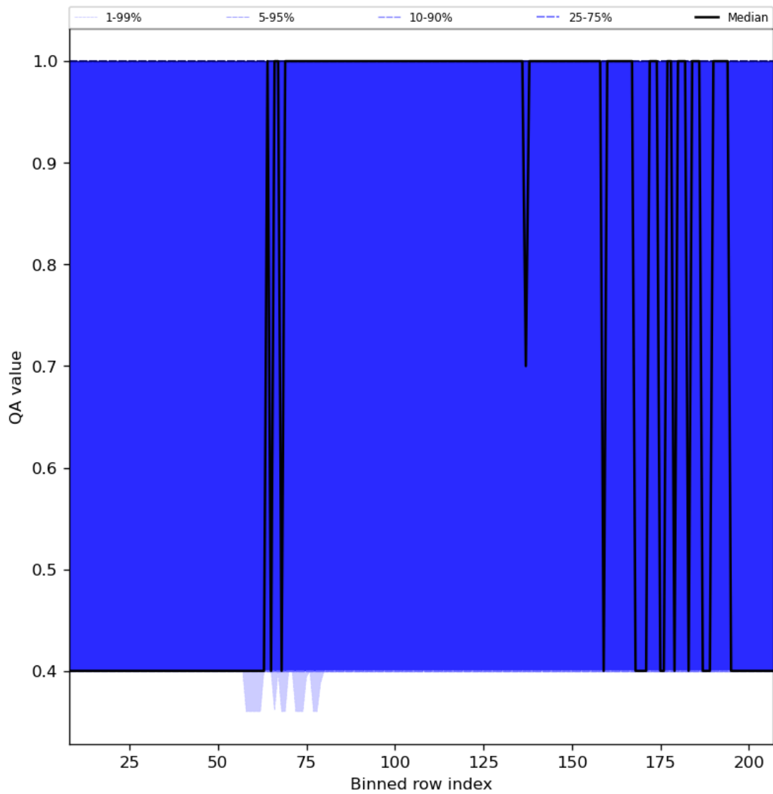
Figure 33: Along track statistics of “QA value” for 2024-03-20 to 2024-03-22
