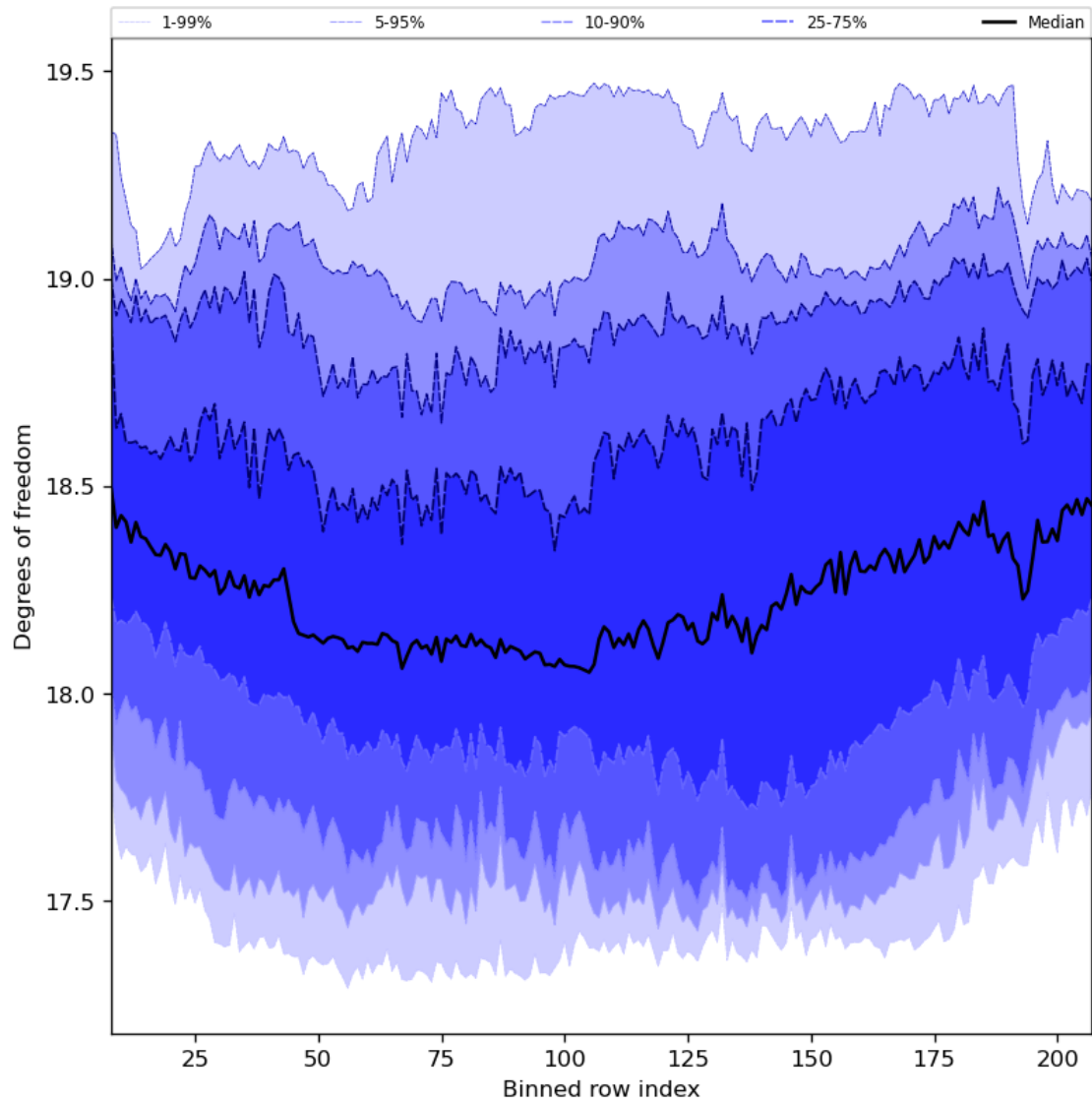
Figure 41: Along track statistics of “Degrees of freedom” for 2024-03-20 to 2024-03-22
