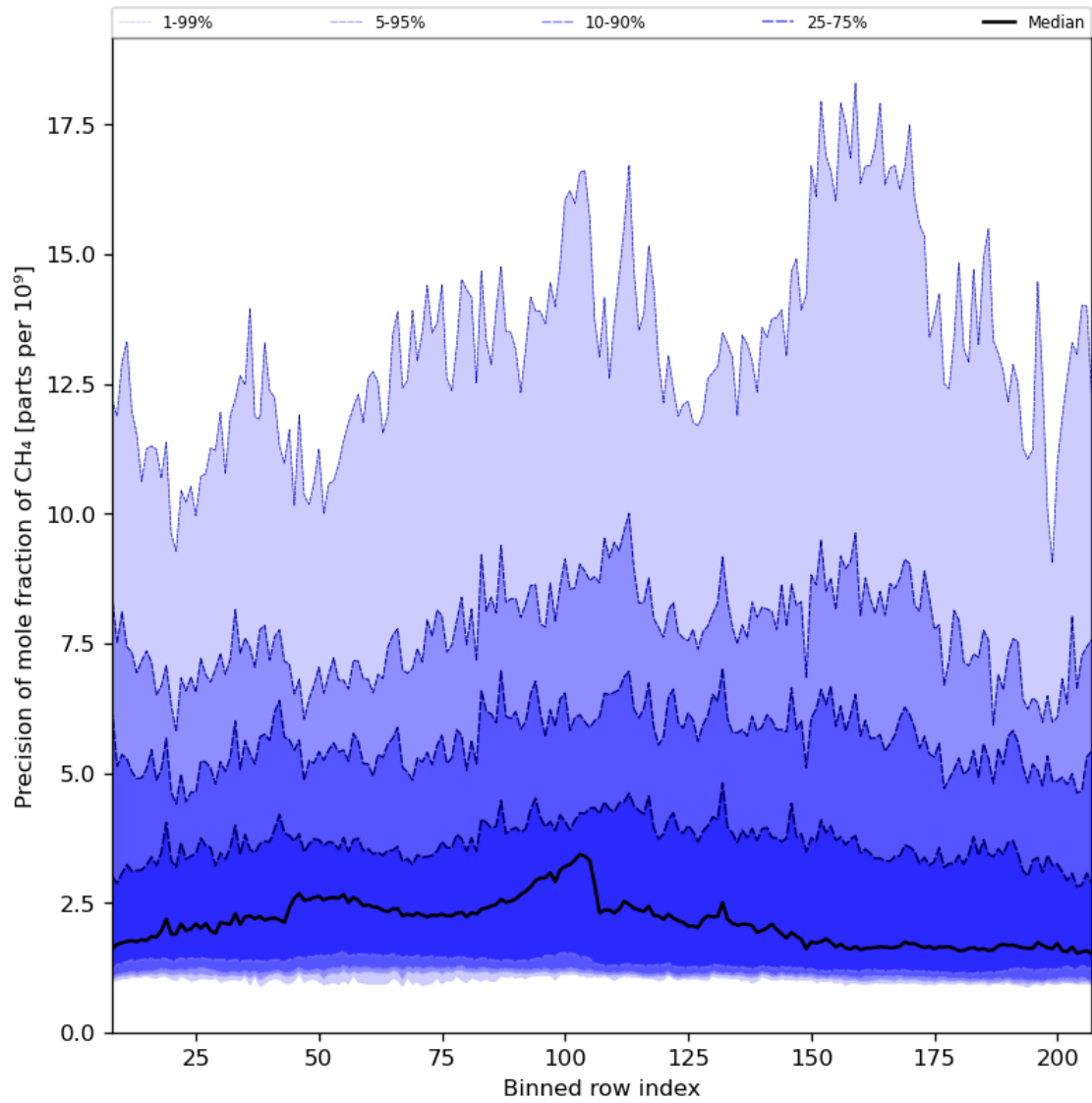
Figure 35: Along track statistics of “Precision of mole fraction of CH 4 ” for 2024-03-20 to 2024-03-22
