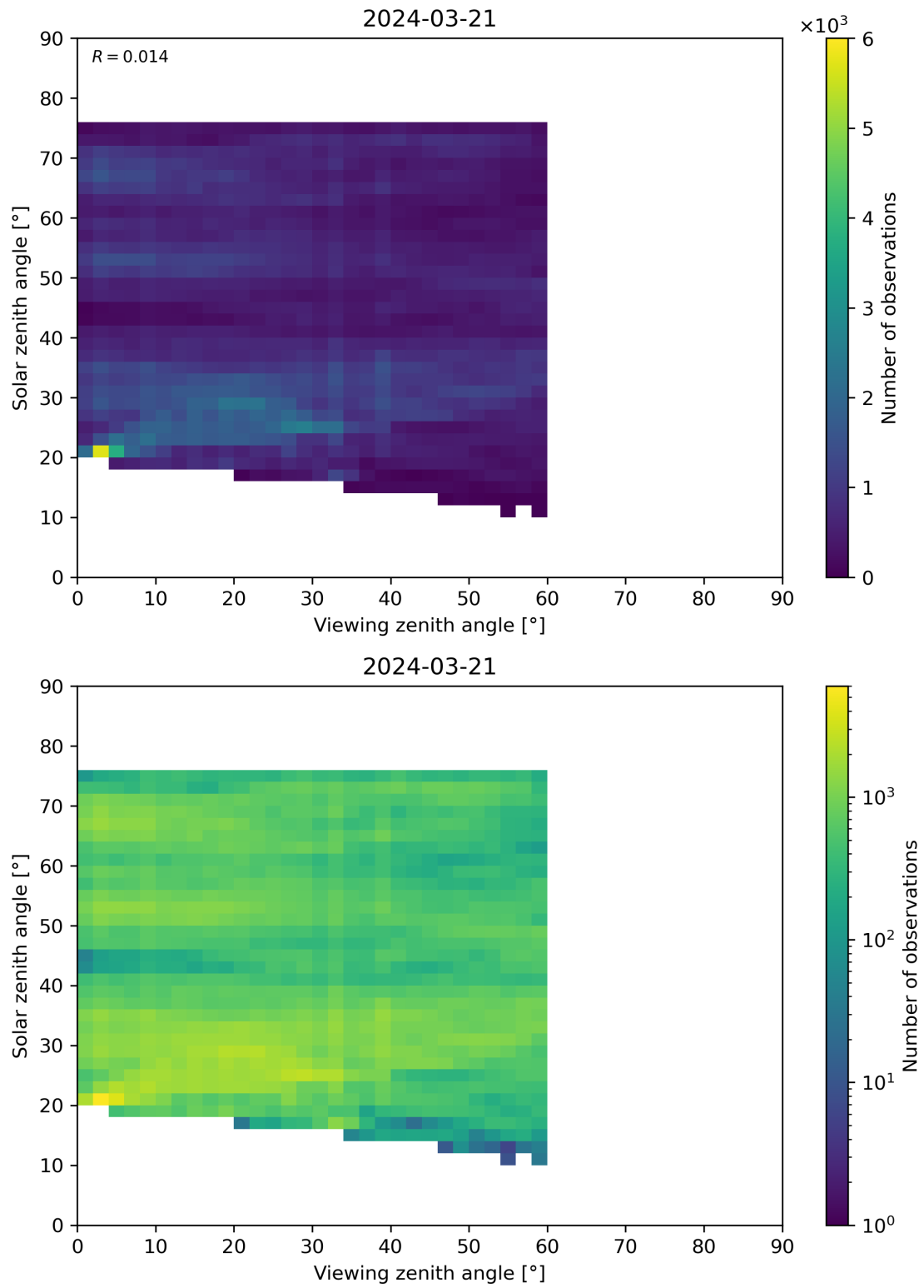
Figure 115: Scatter density plot of “Viewing zenith angle” against “Solar zenith angle” for 2024-03-20 to 2024-03-22.
