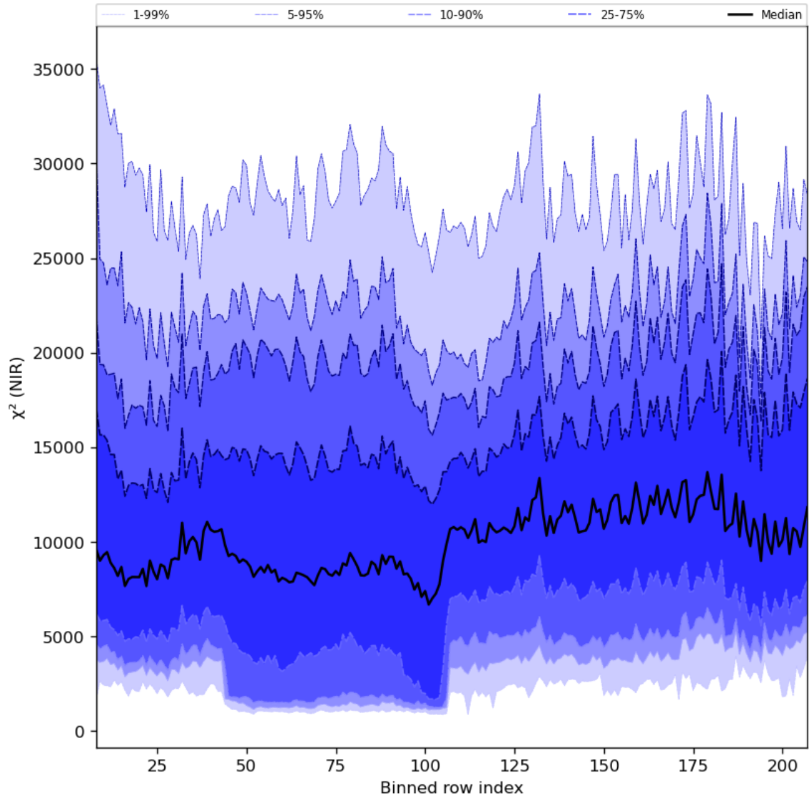
Figure 40: Along track statistics of “ \chi^2 (NIR)” for 2024-03-20 to 2024-03-22
