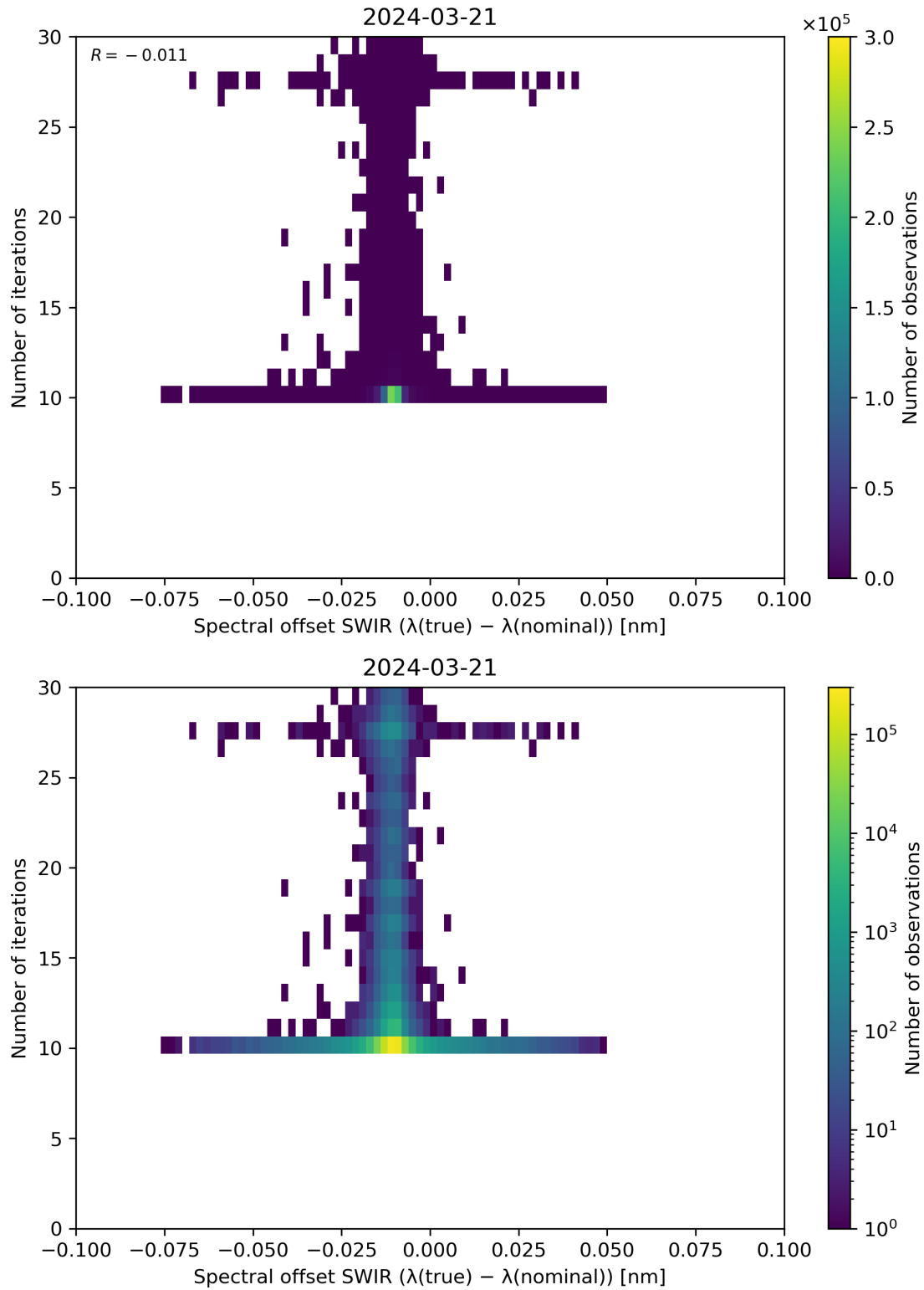
Figure 121: Scatter density plot of “Spectral offset SWIR ( \lambda(\text{true}) - \lambda(\text{nominal}) )” against “Number of iterations” for 2024-03-20 to 2024-03-22.
