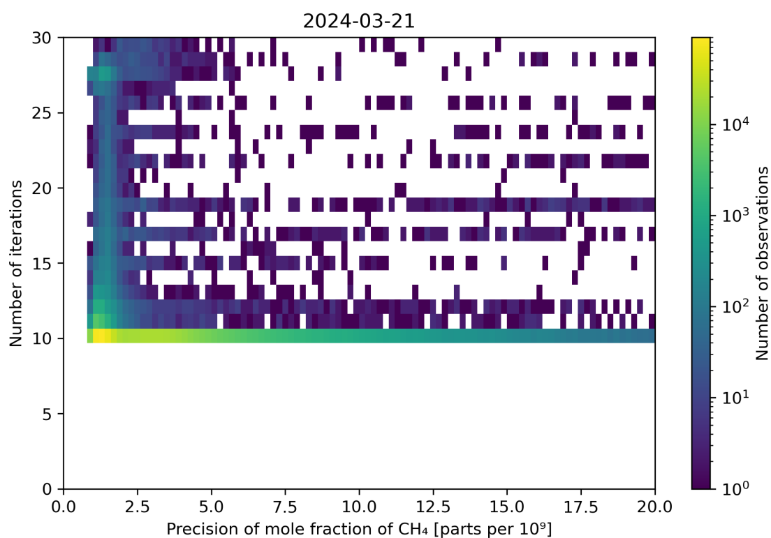
Figure 83: Scatter density plot of “Precision of mole fraction of CH 4 ” against “Number of iterations” for 2024-03-20 to 2024-03-22.
