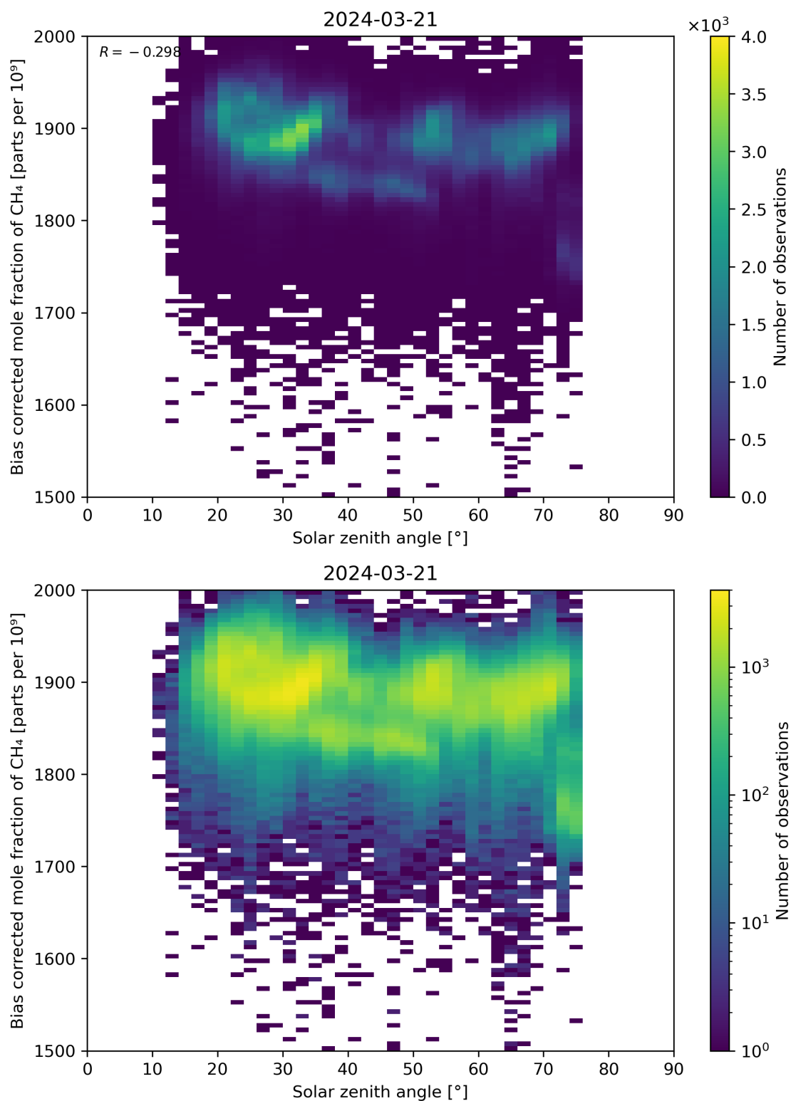
Figure 100: Scatter density plot of “Solar zenith angle” against “Bias corrected mole fraction of \text{CH}_4 ” for 2024-03-20 to 2024-03-22.
