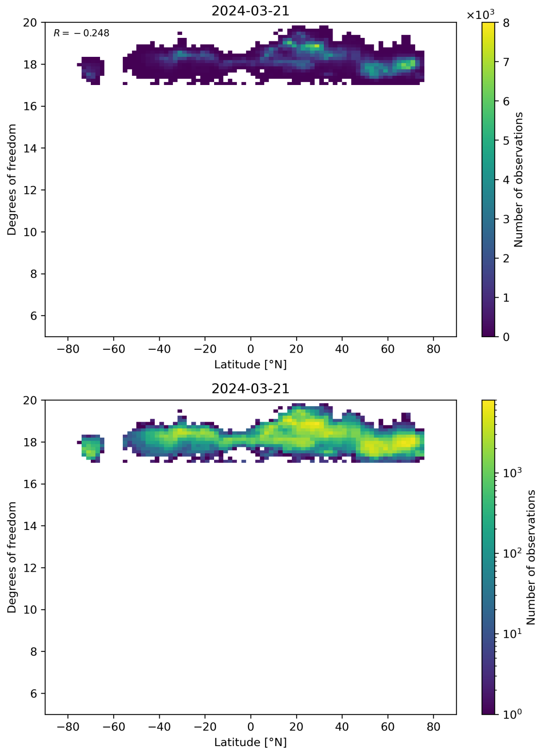
Figure 55: Scatter density plot of “Latitude” against “Degrees of freedom” for 2024-03-20 to 2024-03-22.
