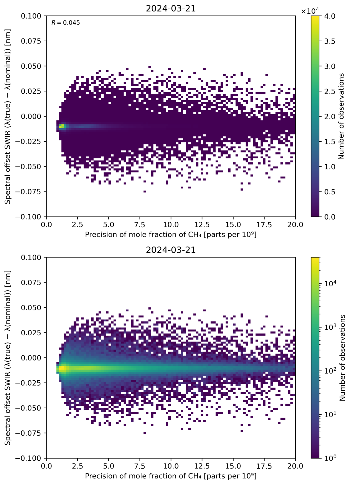
Figure 85: Scatter density plot of “Precision of mole fraction of \text{CH}_4 ” against “Spectral offset SWIR ( \lambda(\text{true}) - \lambda(\text{nominal}) )” for 2024-03-20 to 2024-03-22.
