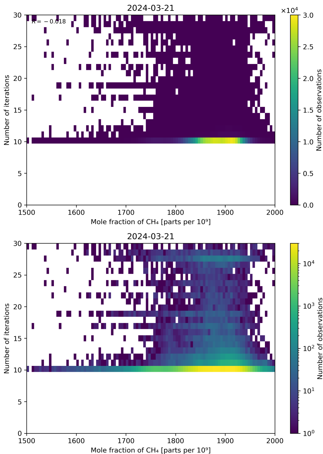
Figure 76: Scatter density plot of “Mole fraction of CH 4 ” against “Number of iterations” for 2024-03-20 to 2024-03-22.
