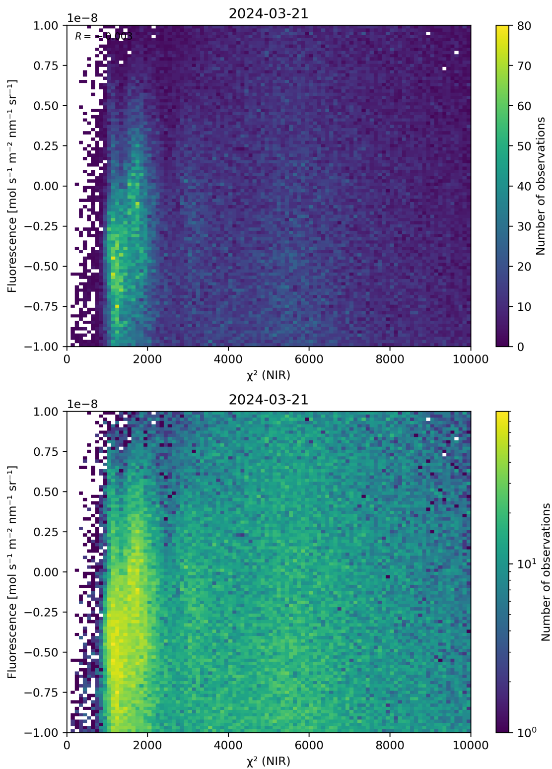
Figure 45: Scatter density plot of “ \chi^2 (NIR)” against “Fluorescence” for 2024-03-20 to 2024-03-22.
