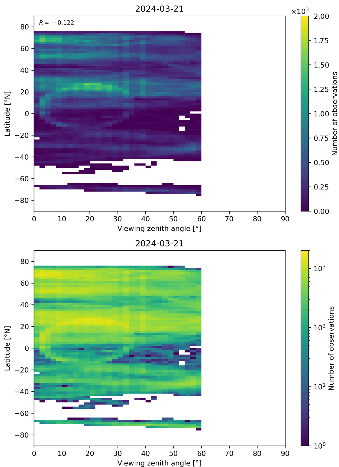
Figure 109: Scatter density plot of “Viewing zenith angle” against “Latitude” for 2024-03-20 to 2024-03-22.
