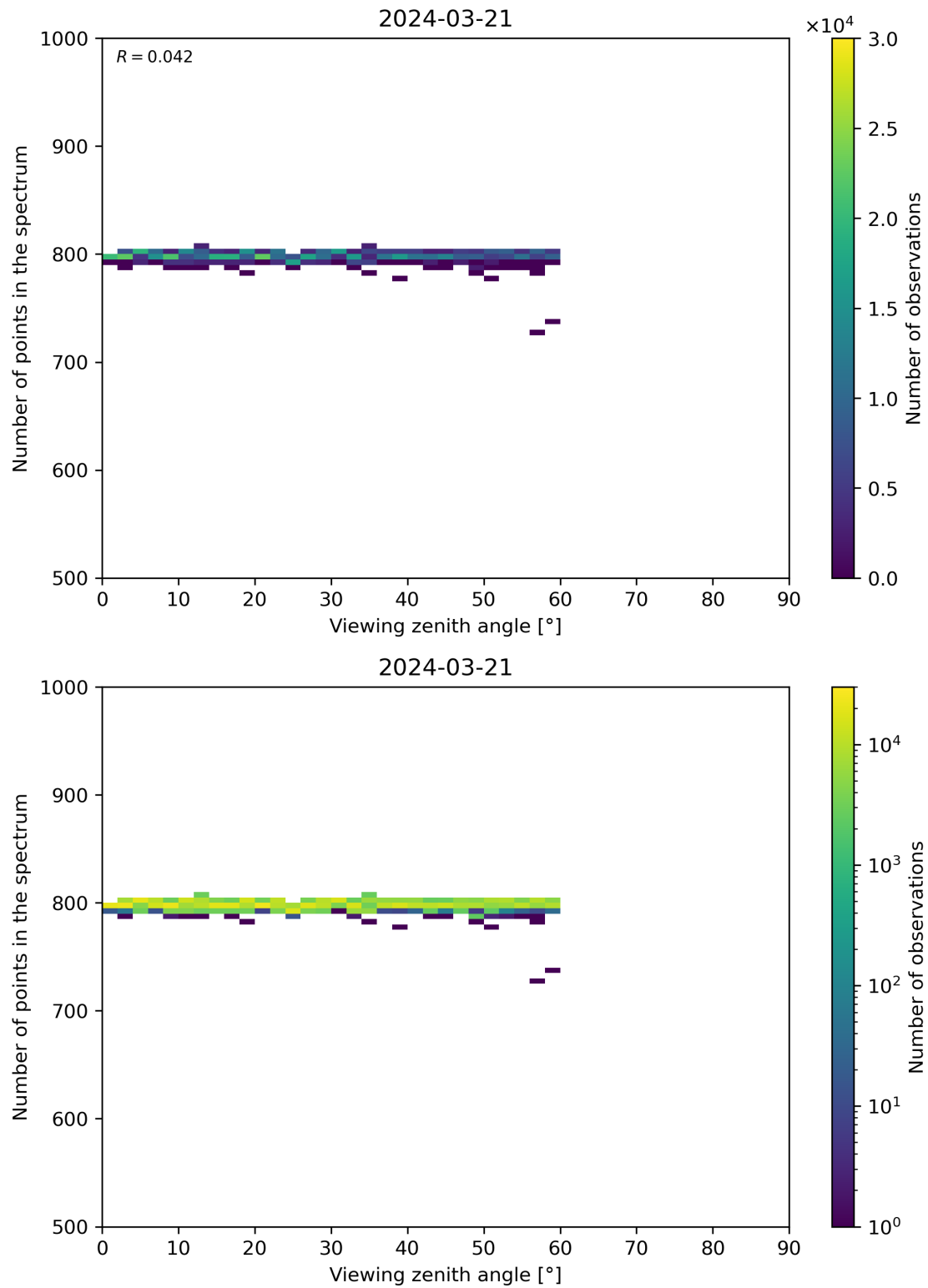
Figure 114: Scatter density plot of “Viewing zenith angle” against “Number of points in the spectrum” for 2024-03-20 to 2024-03-22.
