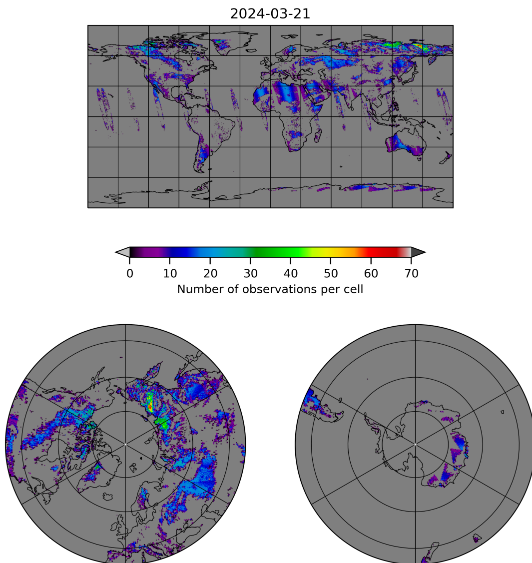
Figure 10: Map of the number of observations for 2024-03-20 to 2024-03-22
