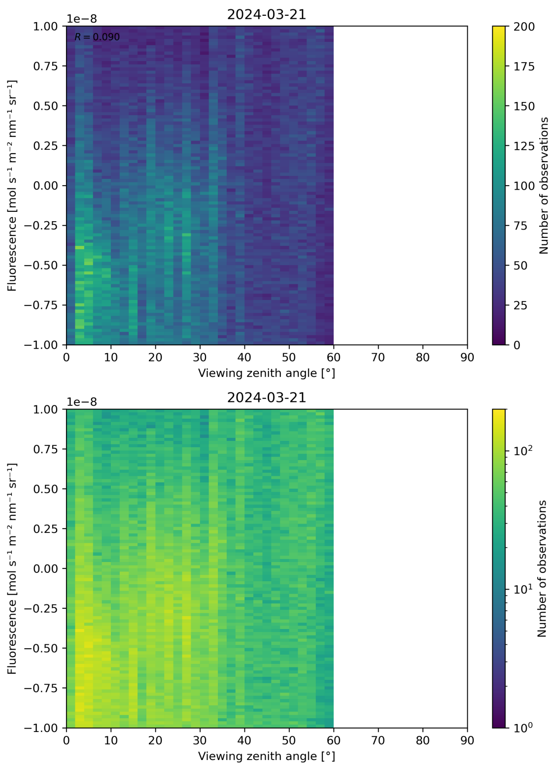
Figure 108: Scatter density plot of “Viewing zenith angle” against “Fluorescence” for 2024-03-20 to 2024-03-22.
