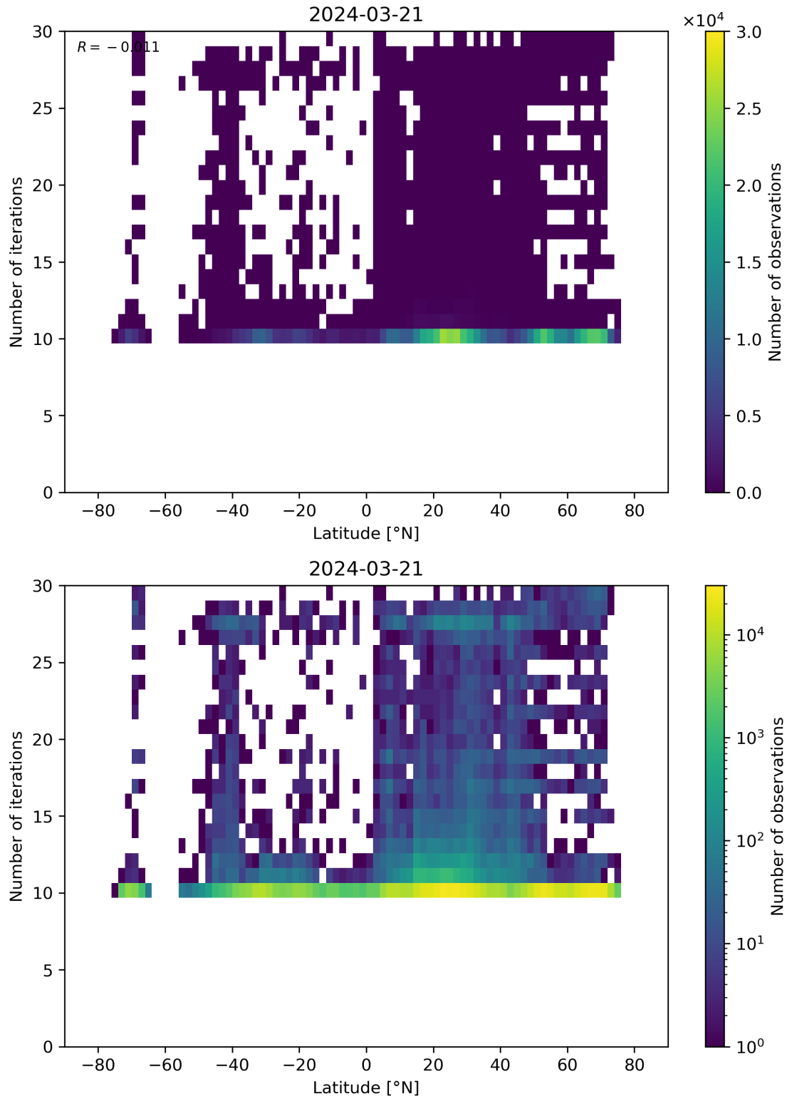
Figure 60: Scatter density plot of “Latitude” against “Number of iterations” for 2024-03-20 to 2024-03-22.
