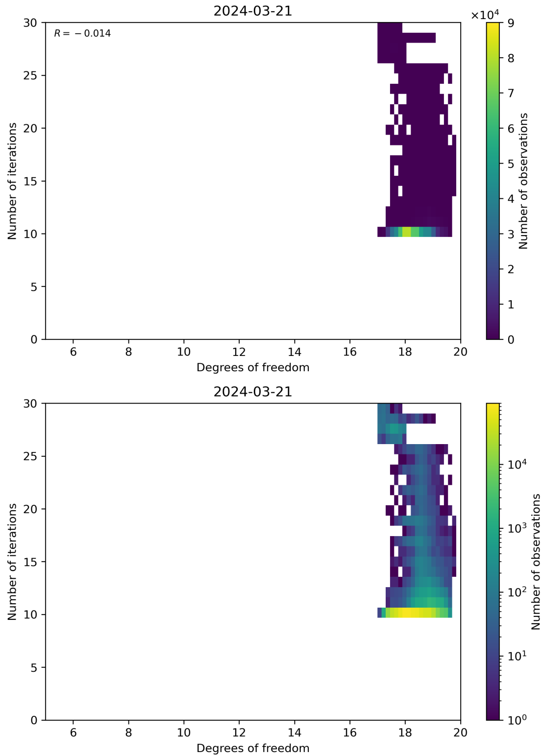
Figure 52: Scatter density plot of “Degrees of freedom” against “Number of iterations” for 2024-03-20 to 2024-03-22.
