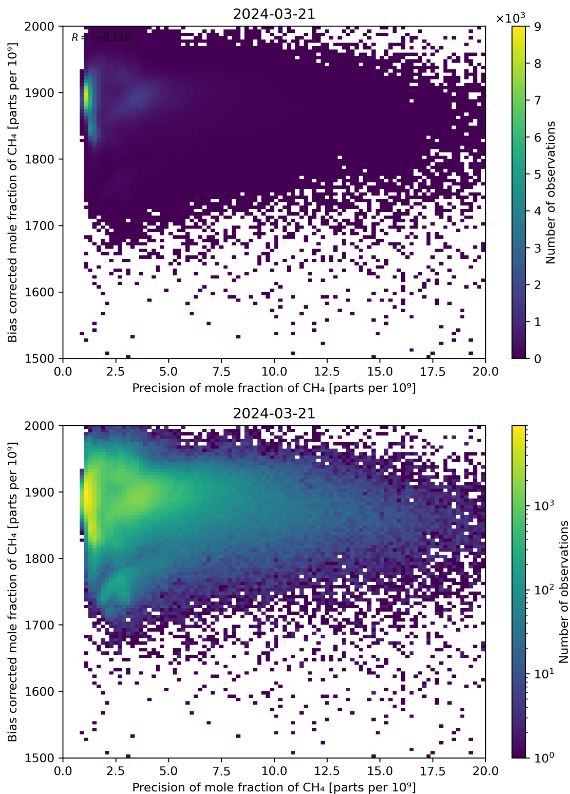
Figure 82: Scatter density plot of “Precision of mole fraction of CH 4 ” against “Bias corrected mole fraction of CH 4 ” for 2024-03-20 to 2024-03-22.
