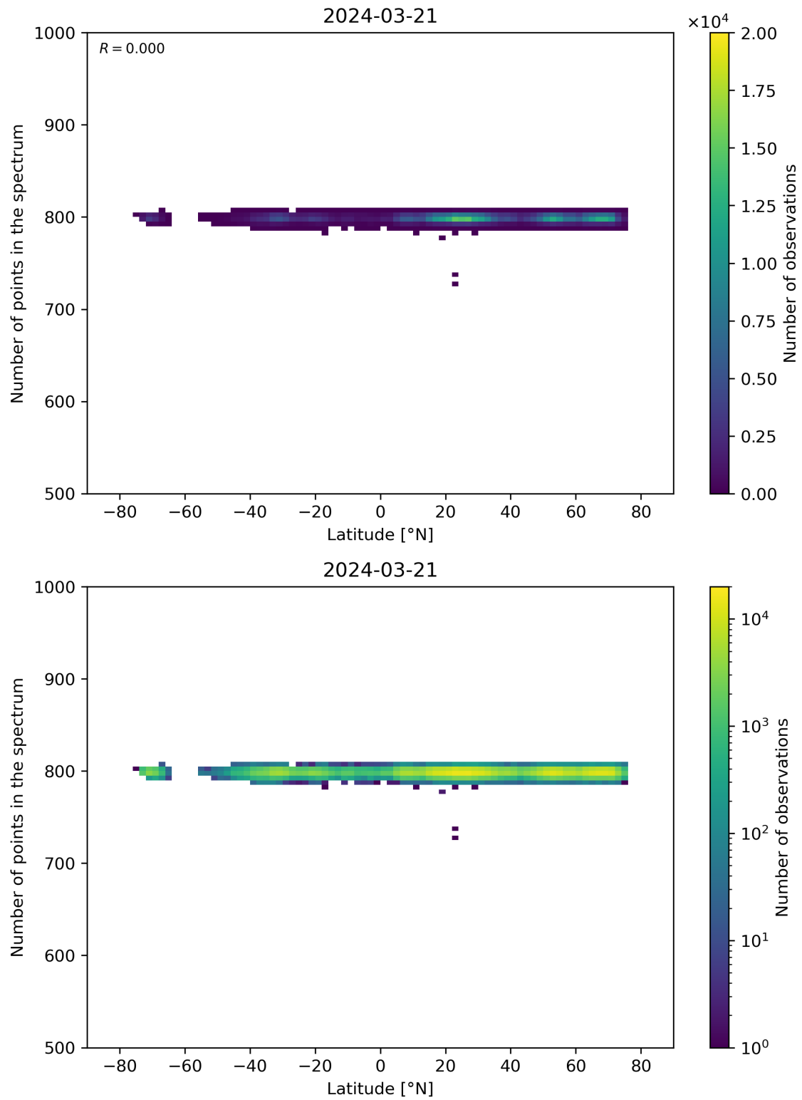
Figure 61: Scatter density plot of “Latitude” against “Number of points in the spectrum” for 2024-03-20 to 2024-03-22.
