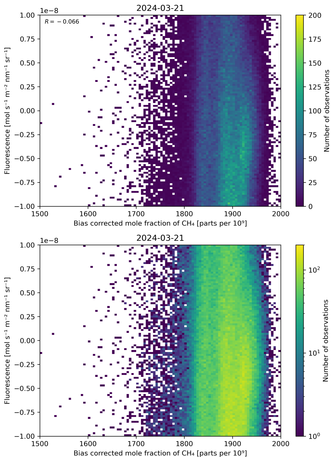
Figure 66: Scatter density plot of “Bias corrected mole fraction of \text{CH}_4 ” against “Fluorescence” for 2024-03-20 to 2024-03-22.
