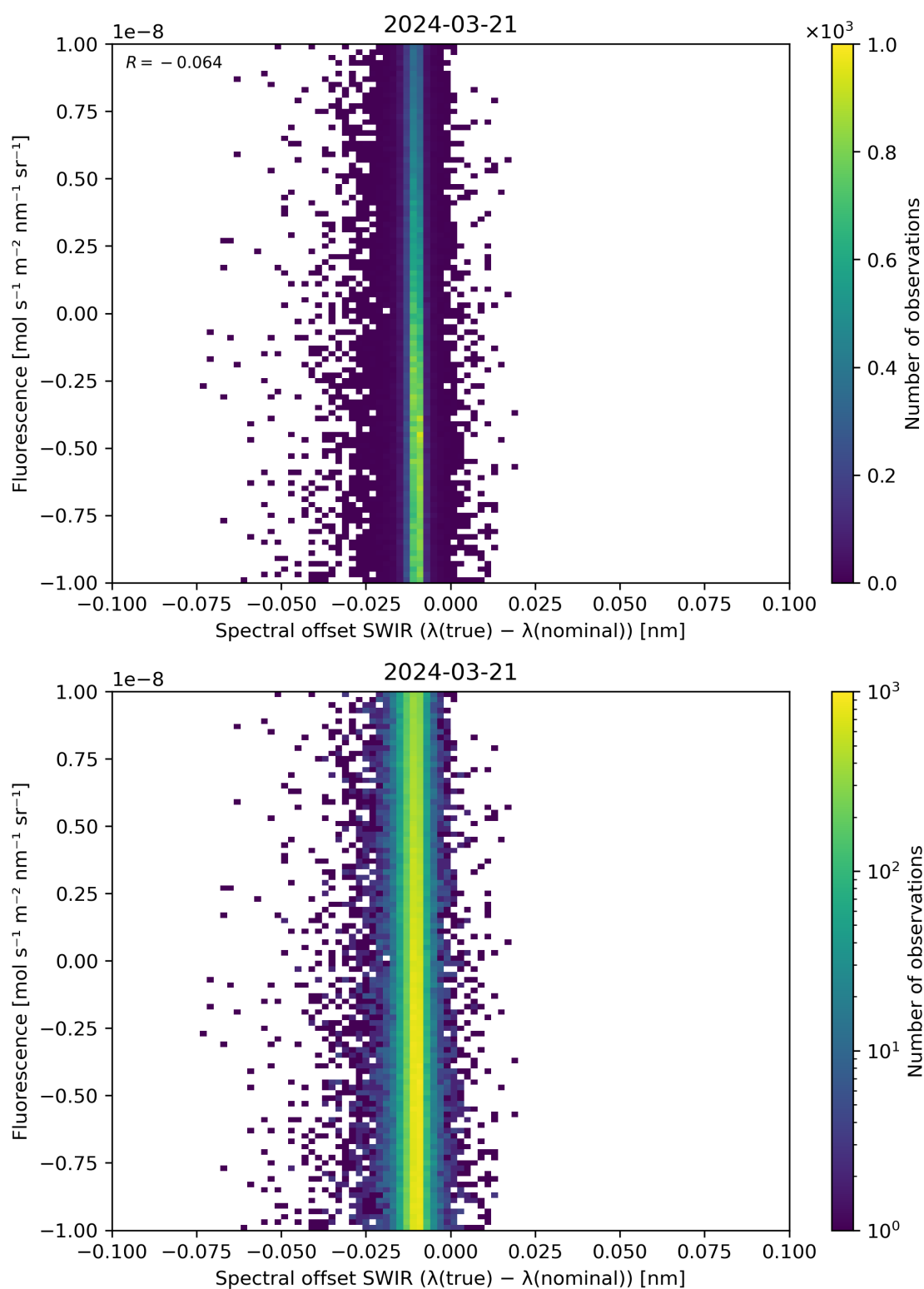
Figure 120: Scatter density plot of “Spectral offset SWIR ( \lambda(\text{true}) - \lambda(\text{nominal}) )” against “Fluorescence” for 2024-03-20 to 2024-03-22.
