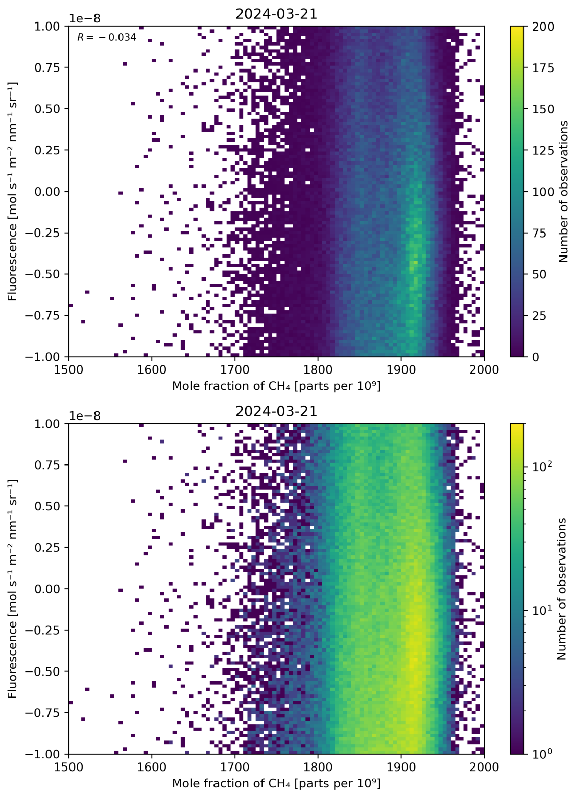
Figure 73: Scatter density plot of “Mole fraction of \text{CH}_4 ” against “Fluorescence” for 2024-03-20 to 2024-03-22.
