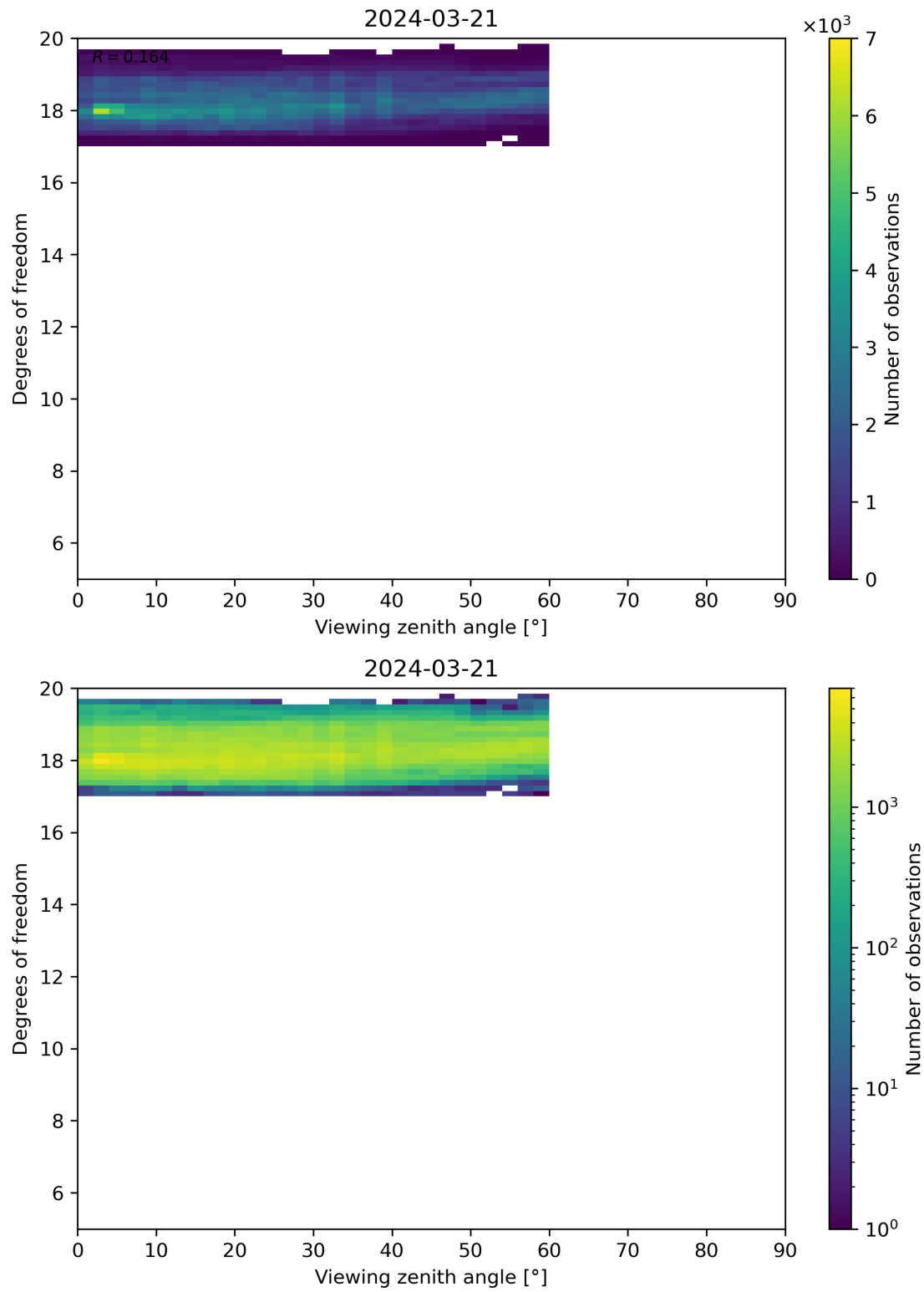
Figure 107: Scatter density plot of “Viewing zenith angle” against “Degrees of freedom” for 2024-03-20 to 2024-03-22.
