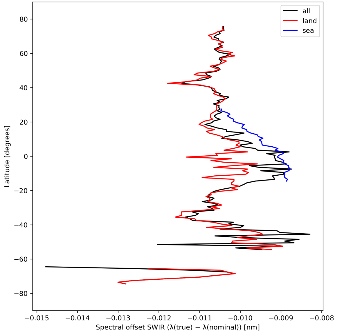
Figure 16: Zonal average of “Spectral offset SWIR ( \lambda(\text{true}) - \lambda(\text{nominal}) )” for 2024-03-20 to 2024-03-22.
