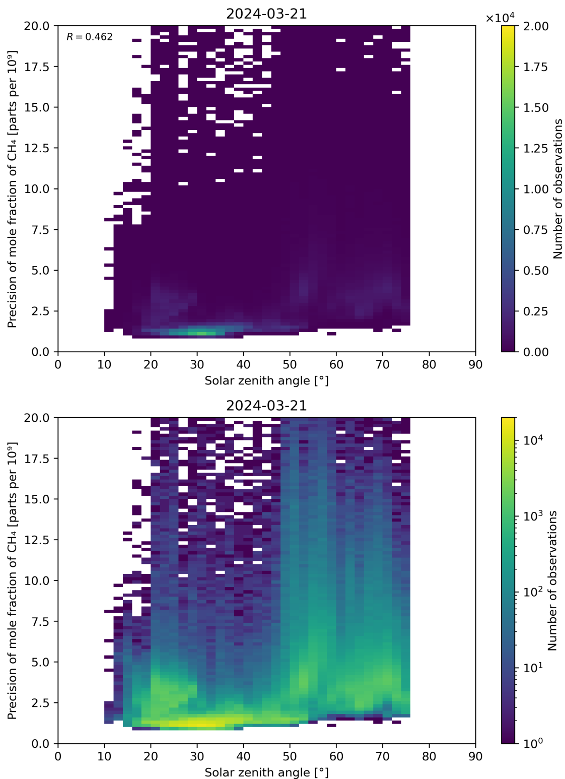
Figure 101: Scatter density plot of “Solar zenith angle” against “Precision of mole fraction of CH 4 ” for 2024-03-20 to 2024-03-22.
