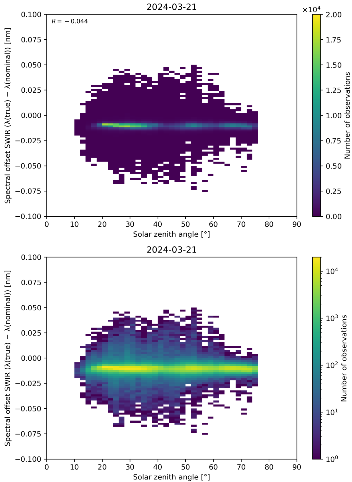
Figure 104: Scatter density plot of “Solar zenith angle” against “Spectral offset SWIR ( \lambda(\text{true}) - \lambda(\text{nominal}) )” for 2024-03-20 to 2024-03-22.
