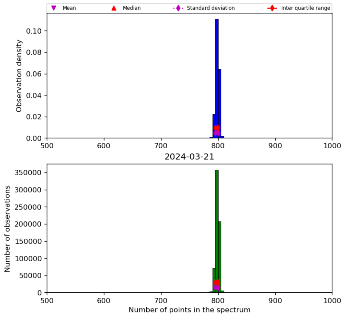
Figure 26: Histogram of “Number of points in the spectrum” for 2024-03-20 to 2024-03-22
