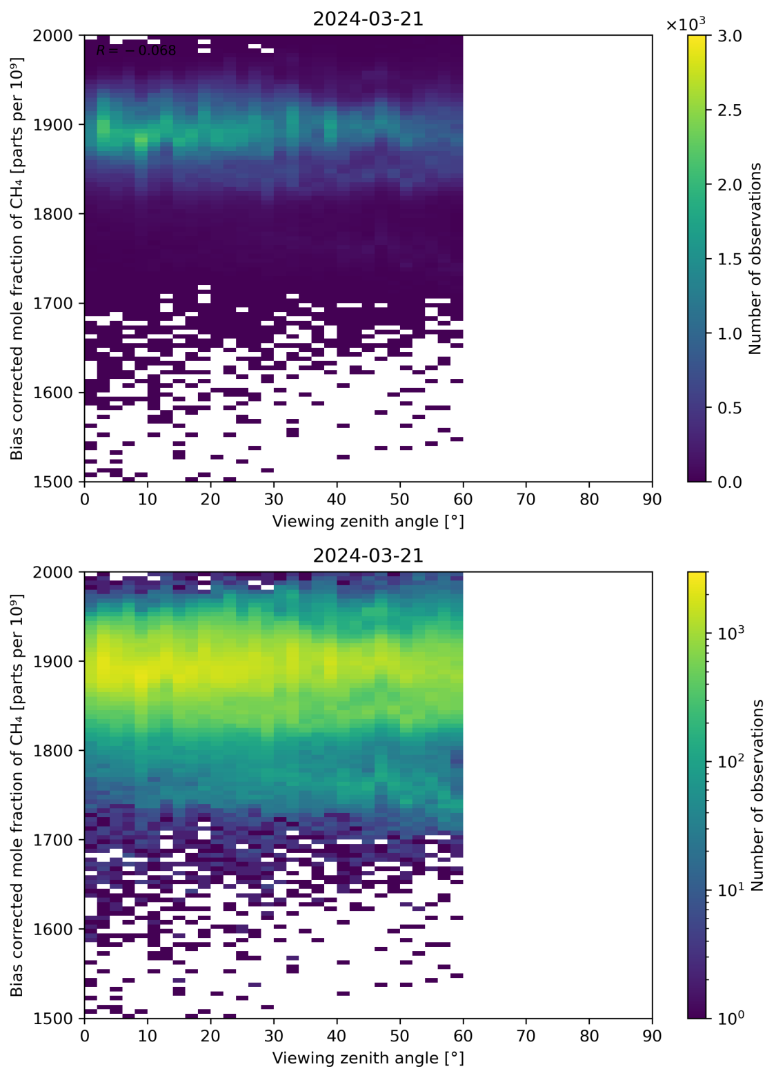
Figure 111: Scatter density plot of “Viewing zenith angle” against “Bias corrected mole fraction of CH 4 ” for 2024-03-20 to 2024-03-22.
