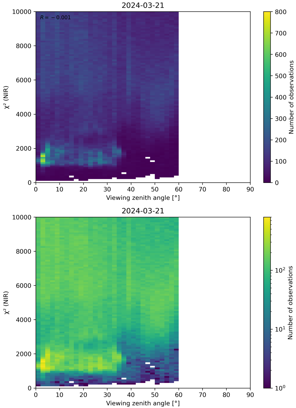
Figure 105: Scatter density plot of “Viewing zenith angle” against “ \chi^2 (NIR)” for 2024-03-20 to 2024-03-22.
