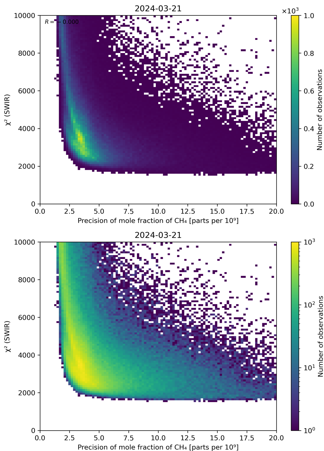
Figure 79: Scatter density plot of “Precision of mole fraction of \text{CH}_4 ” against “ \chi^2 (SWIR)” for 2024-03-20 to 2024-03-22.
