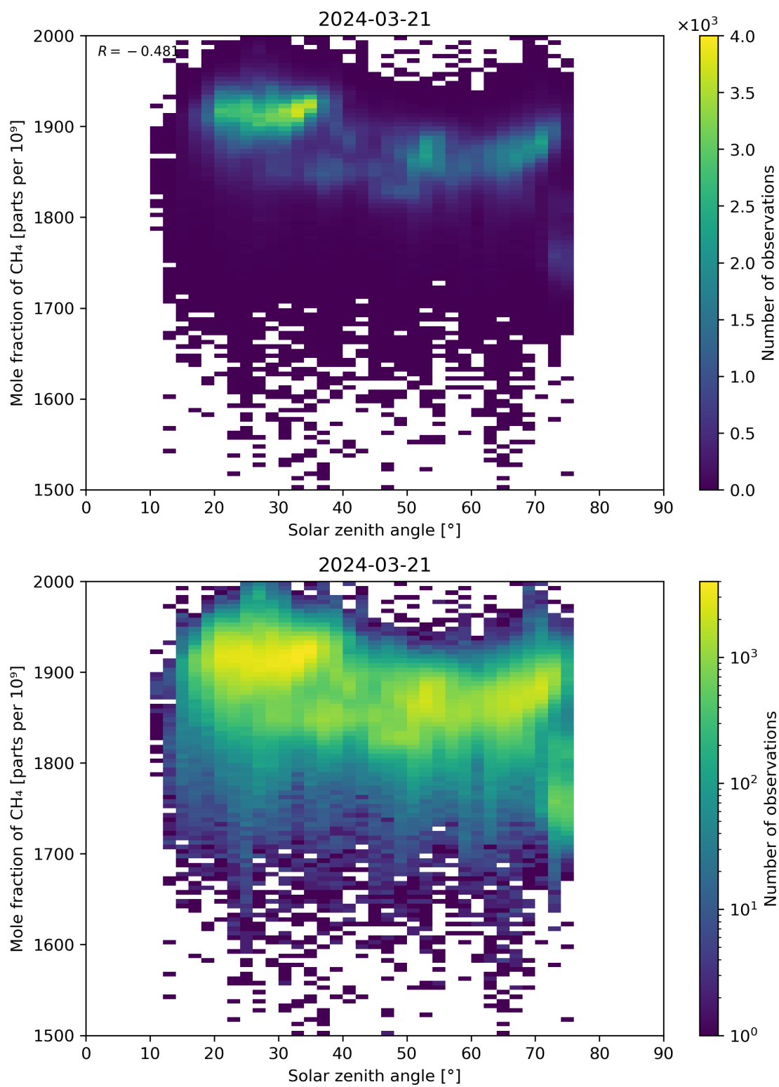
Figure 99: Scatter density plot of “Solar zenith angle” against “Mole fraction of \text{CH}_4 ” for 2024-03-20 to 2024-03-22.
