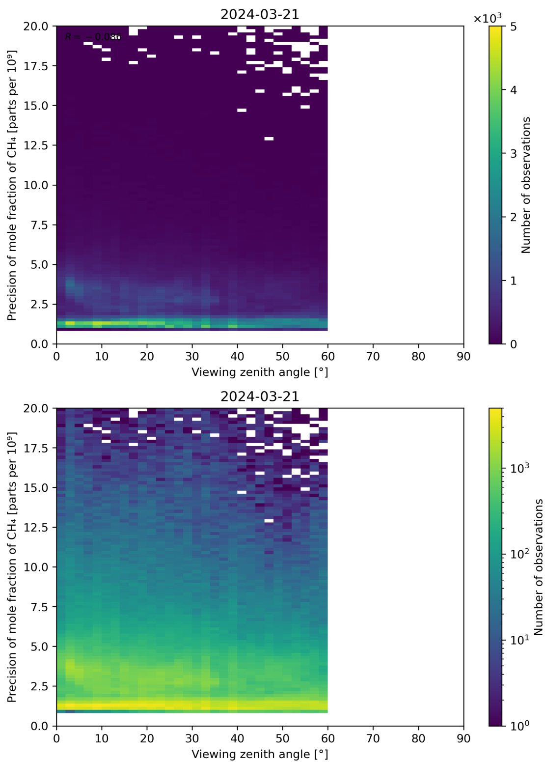
Figure 112: Scatter density plot of “Viewing zenith angle” against “Precision of mole fraction of CH 4 ” for 2024-03-20 to 2024-03-22.
