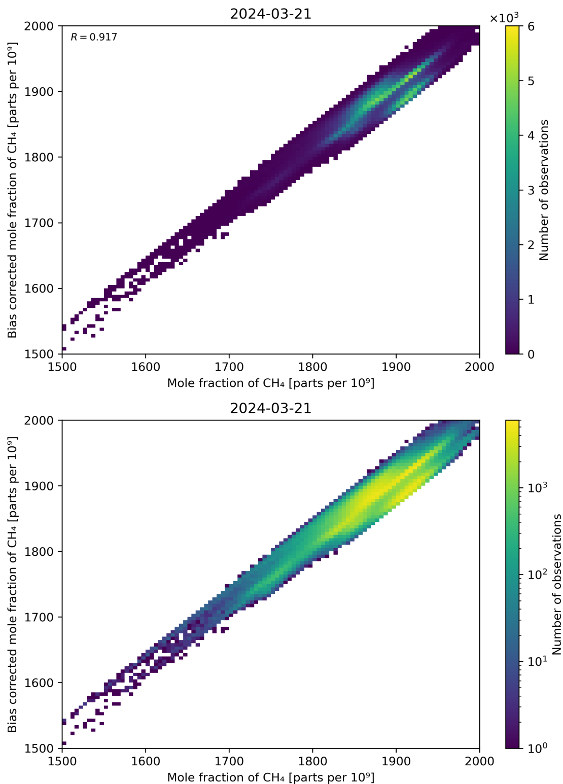
Figure 74: Scatter density plot of “Mole fraction of CH 4 ” against “Bias corrected mole fraction of CH 4 ” for 2024-03-20 to 2024-03-22.
