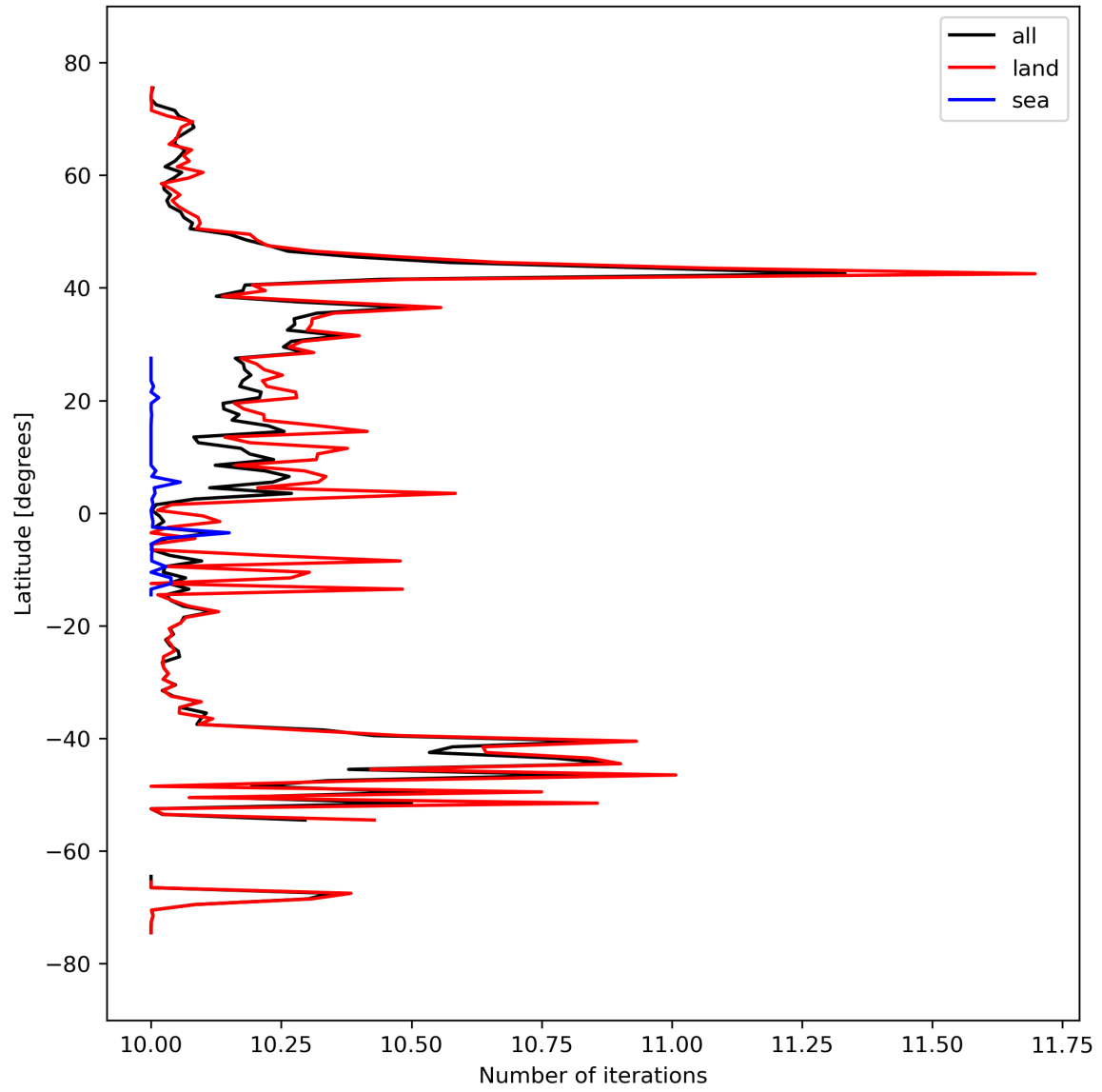
Figure 20: Zonal average of “Number of iterations” for 2024-03-20 to 2024-03-22.
