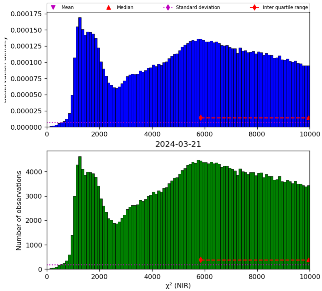
Figure 29: Histogram of “ \chi^2 (NIR)” for 2024-03-20 to 2024-03-22
