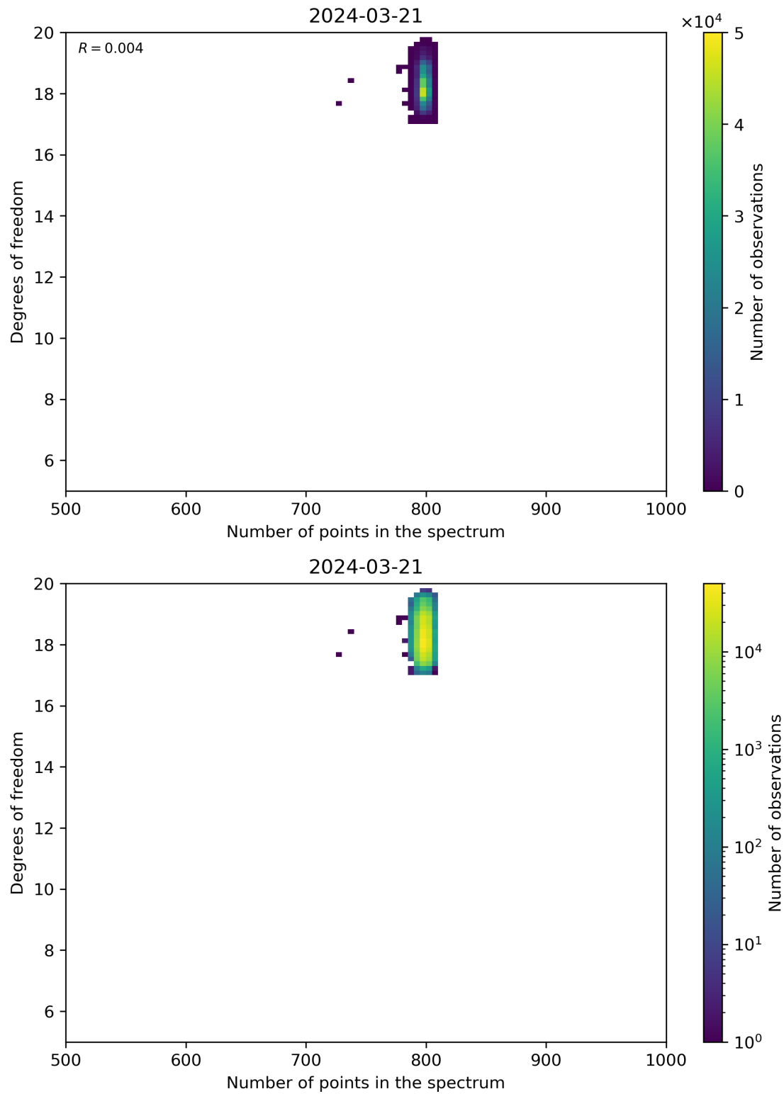
Figure 90: Scatter density plot of “Number of points in the spectrum” against “Degrees of freedom” for 2024-03-20 to 2024-03-22.
