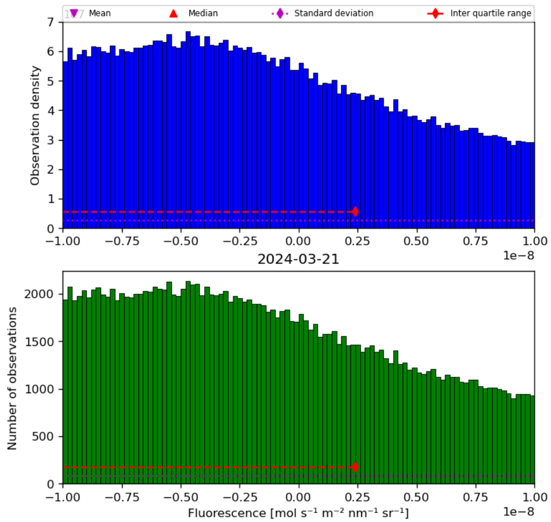
Figure 32: Histogram of “Fluorescence” for 2024-03-20 to 2024-03-22
