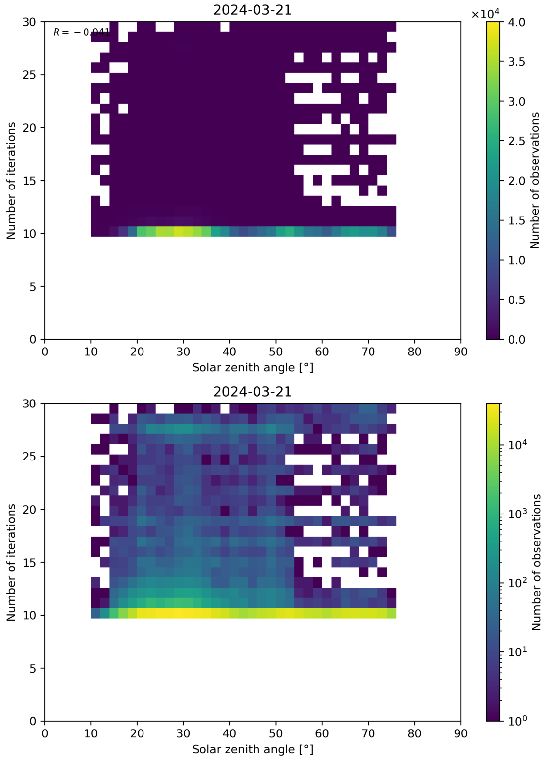
Figure 102: Scatter density plot of “Solar zenith angle” against “Number of iterations” for 2024-03-20 to 2024-03-22.
