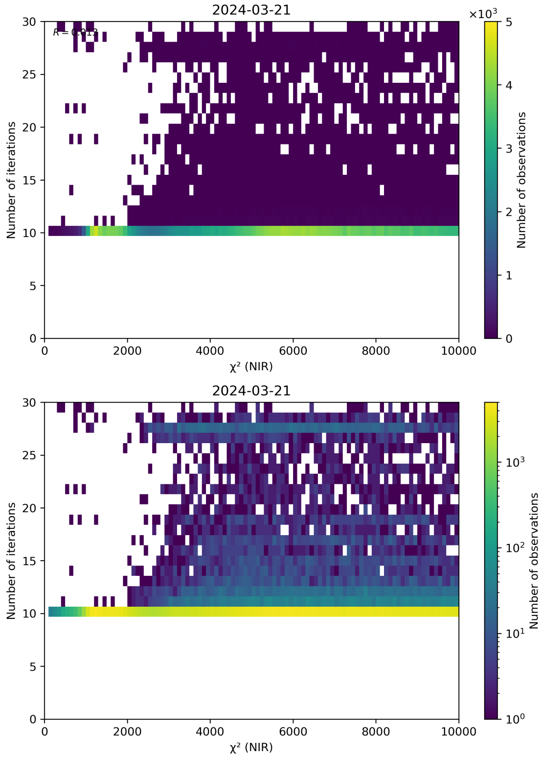
Figure 46: Scatter density plot of “ \chi^2 (NIR)” against “Number of iterations” for 2024-03-20 to 2024-03-22.
