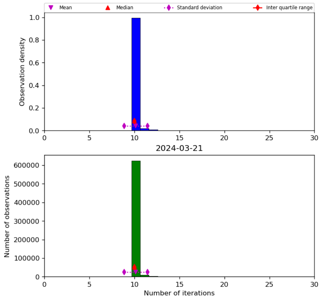
Figure 31: Histogram of “Number of iterations” for 2024-03-20 to 2024-03-22
