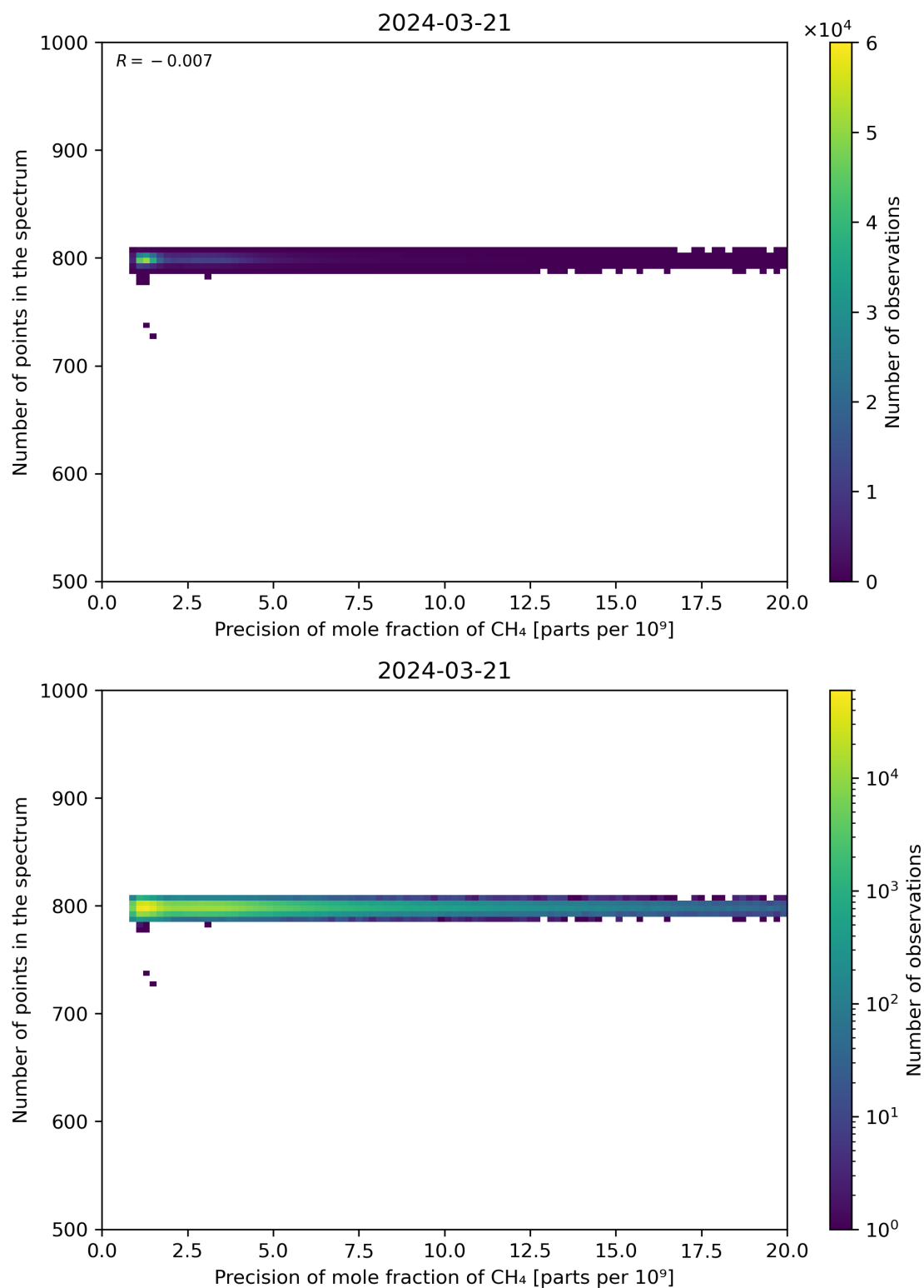
Figure 84: Scatter density plot of “Precision of mole fraction of CH 4 ” against “Number of points in the spectrum” for 2024-03-20 to 2024-03-22.
