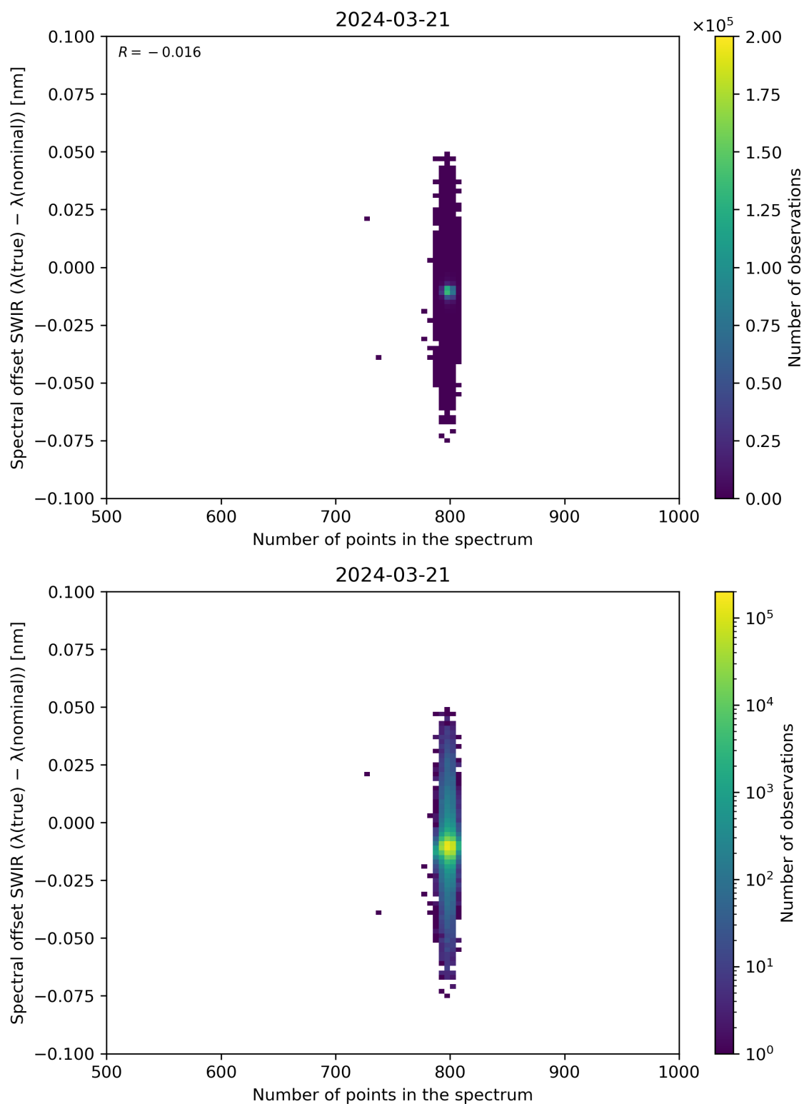
Figure 93: Scatter density plot of “Number of points in the spectrum” against “Spectral offset SWIR ( \lambda(\text{true}) - \lambda(\text{nominal}) )” for 2024-03-20 to 2024-03-22.
