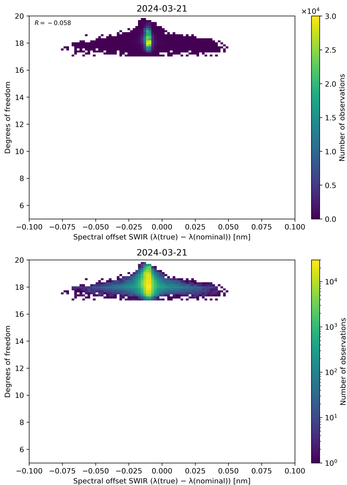
Figure 119: Scatter density plot of “Spectral offset SWIR ( \lambda(\text{true}) - \lambda(\text{nominal}) )” against “Degrees of freedom” for 2024-03-20 to 2024-03-22.
