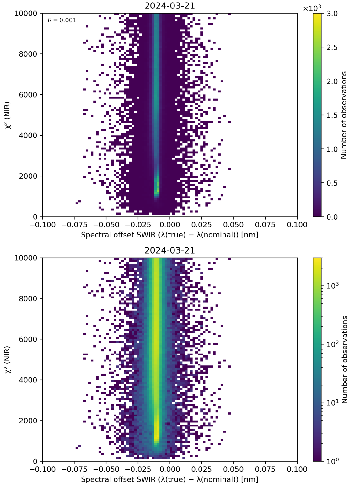
Figure 117: Scatter density plot of “Spectral offset SWIR ( \lambda(\text{true}) - \lambda(\text{nominal}) )” against “ \chi^2 (NIR)” for 2024-03-20 to 2024-03-22.
