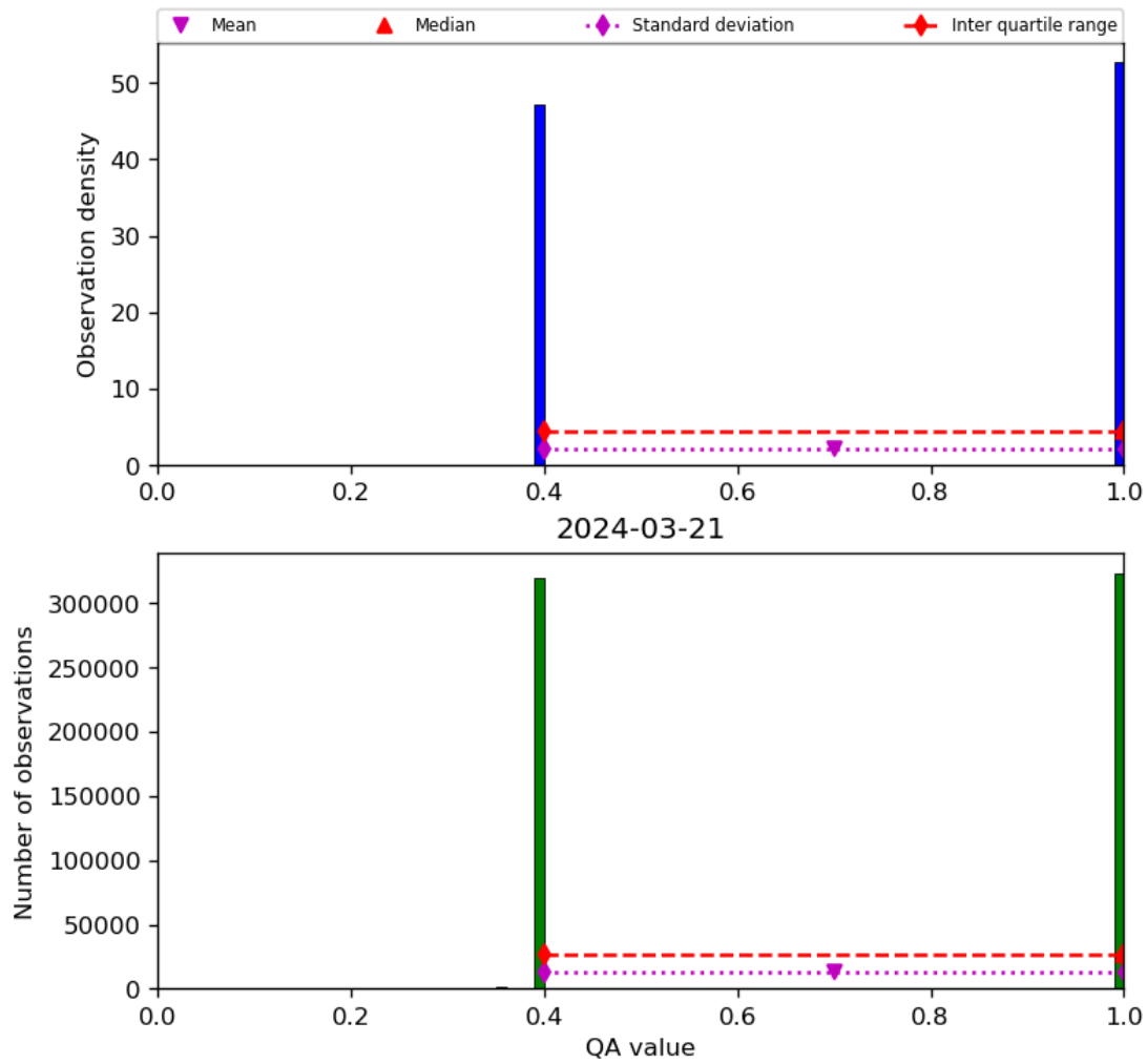
Figure 22: Histogram of “QA value” for 2024-03-20 to 2024-03-22
