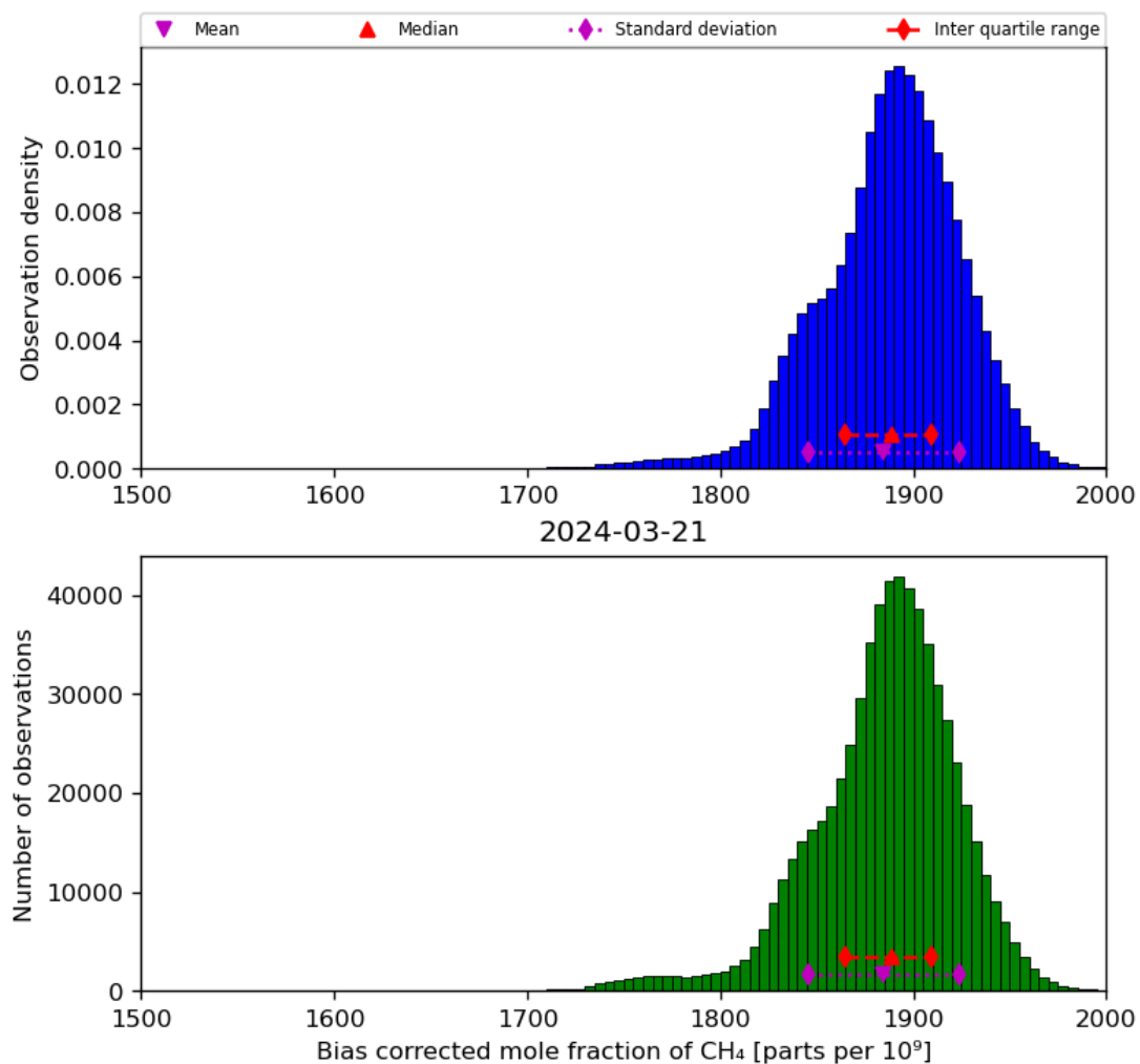
Figure 25: Histogram of “Bias corrected mole fraction of CH 4 ” for 2024-03-20 to 2024-03-22
