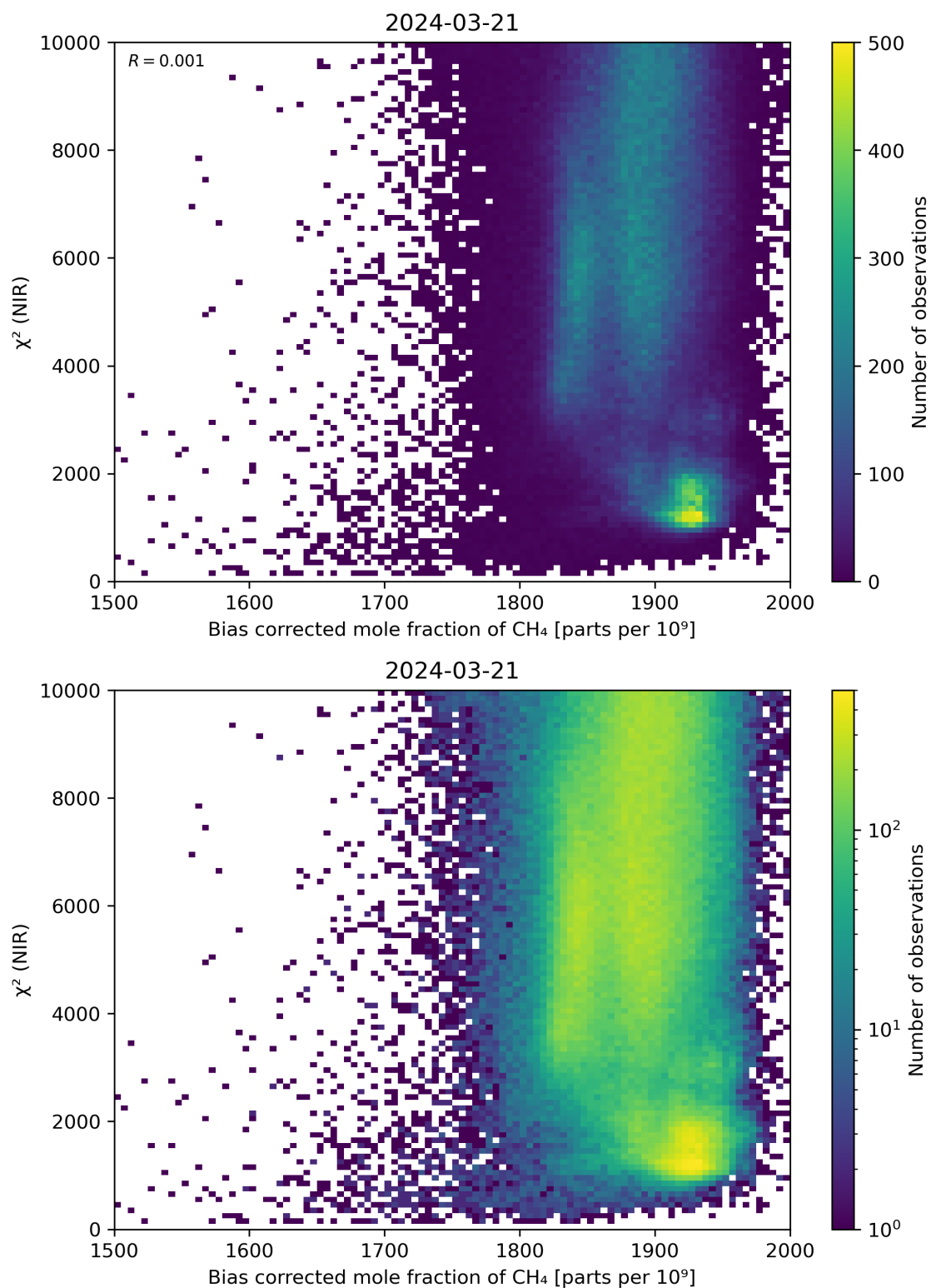
Figure 63: Scatter density plot of “Bias corrected mole fraction of CH 4 ” against “ \chi^2 (NIR)” for 2024-03-20 to 2024-03-22.
