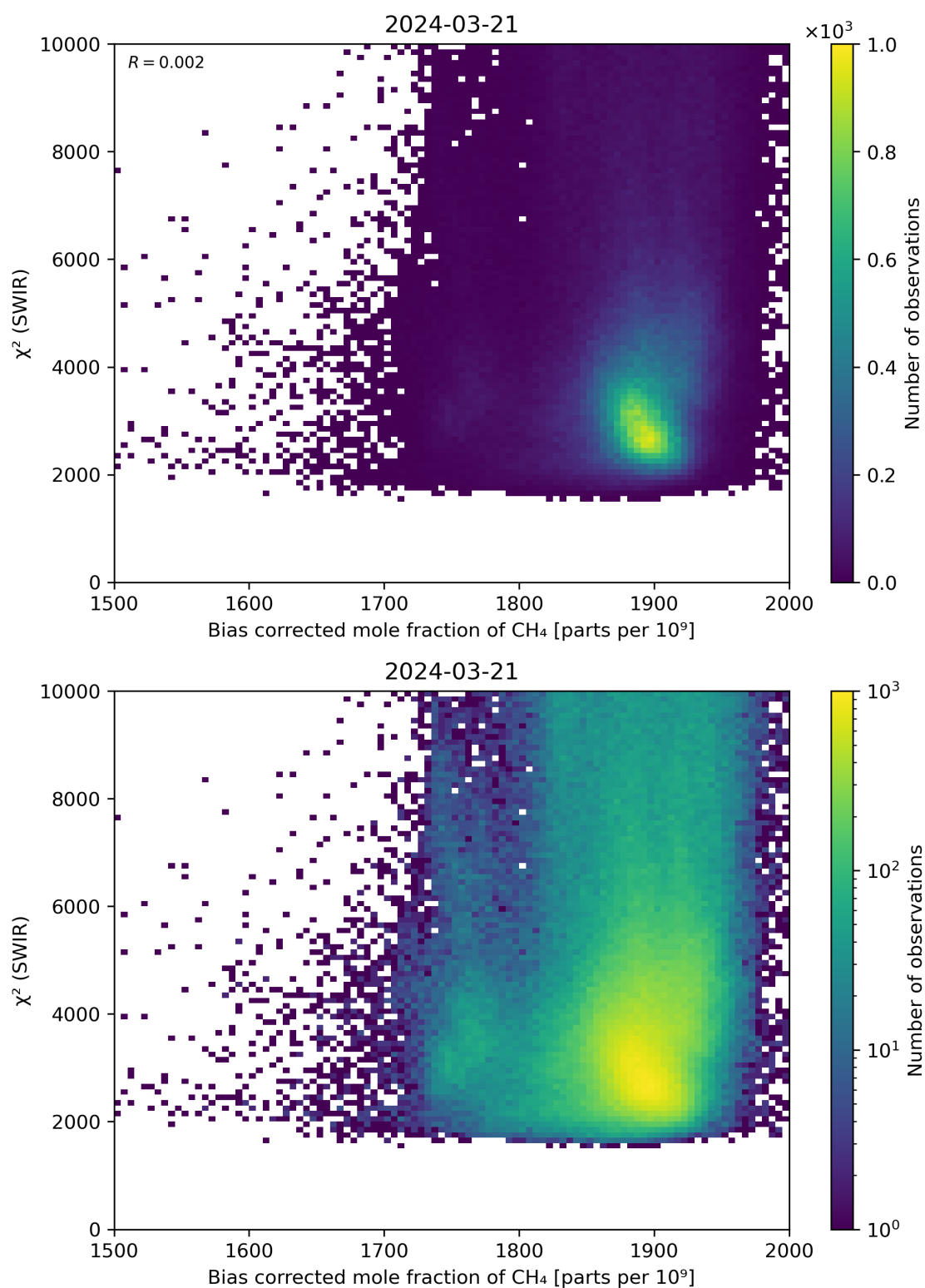
Figure 64: Scatter density plot of “Bias corrected mole fraction of \text{CH}_4 ” against “ \chi^2 (SWIR)” for 2024-03-20 to 2024-03-22.
