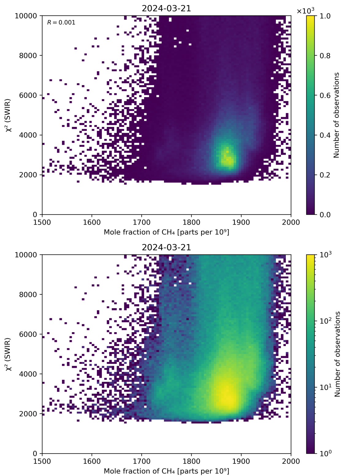
Figure 71: Scatter density plot of “Mole fraction of \text{CH}_4 ” against “ \chi^2 (SWIR)” for 2024-03-20 to 2024-03-22.
