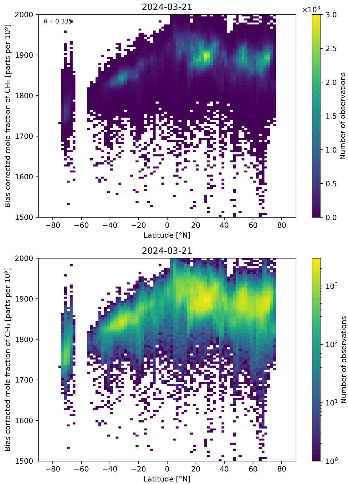
Figure 58: Scatter density plot of “Latitude” against “Bias corrected mole fraction of \text{CH}_4 ” for 2024-03-20 to 2024-03-22.
