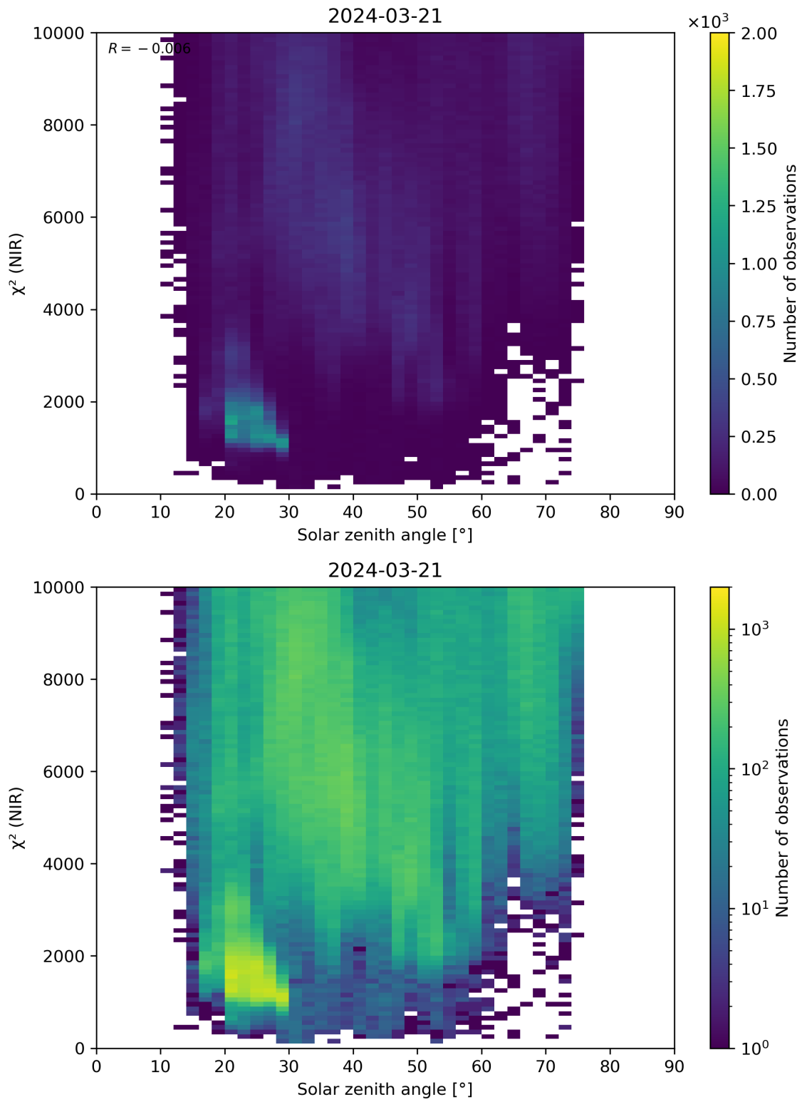
Figure 94: Scatter density plot of “Solar zenith angle” against “ \chi^2 (NIR)” for 2024-03-20 to 2024-03-22.
