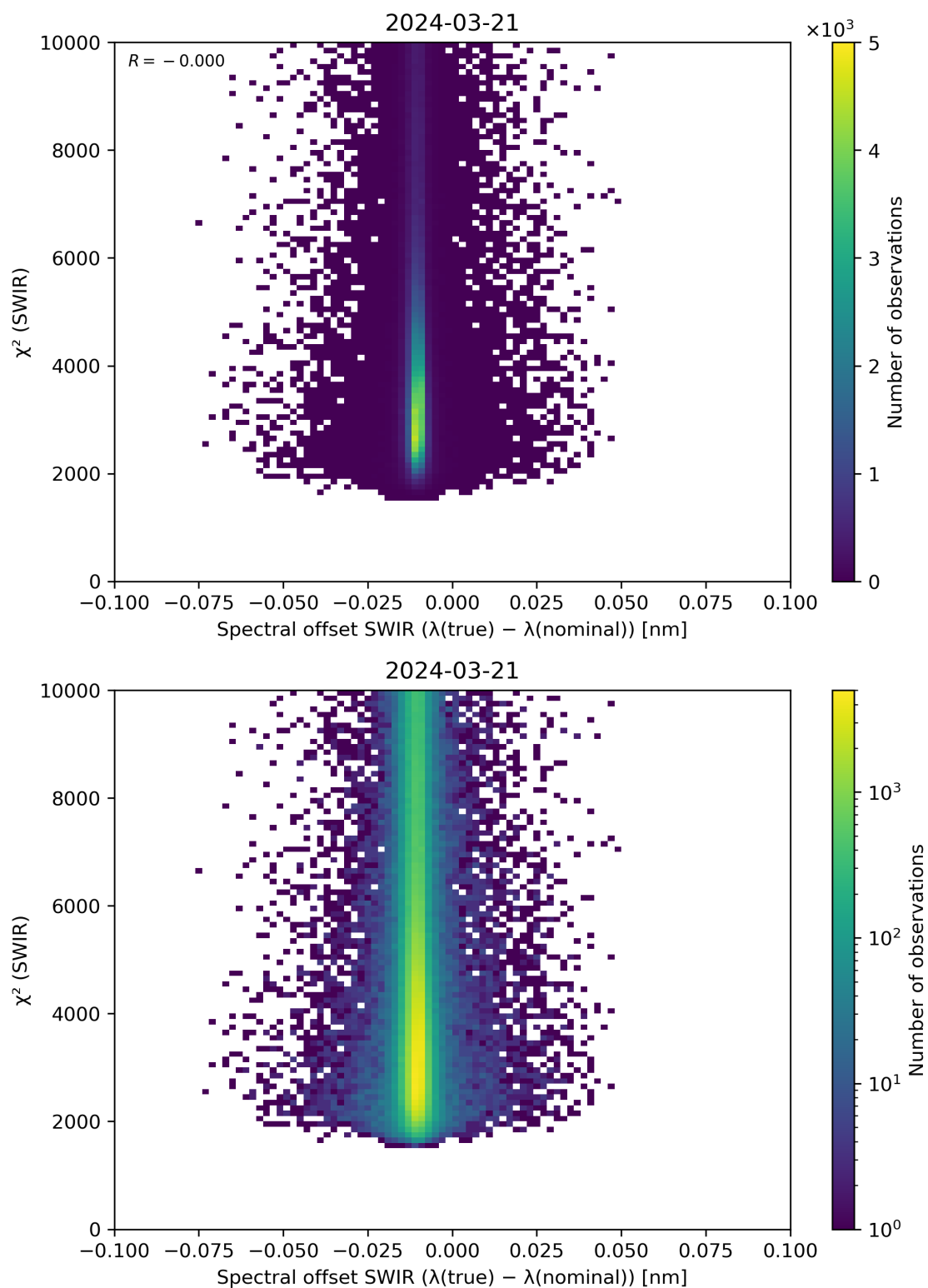
Figure 118: Scatter density plot of “Spectral offset SWIR ( \lambda(\text{true}) - \lambda(\text{nominal}) )” against “ \chi^2 (SWIR)” for 2024-03-20 to 2024-03-22.
