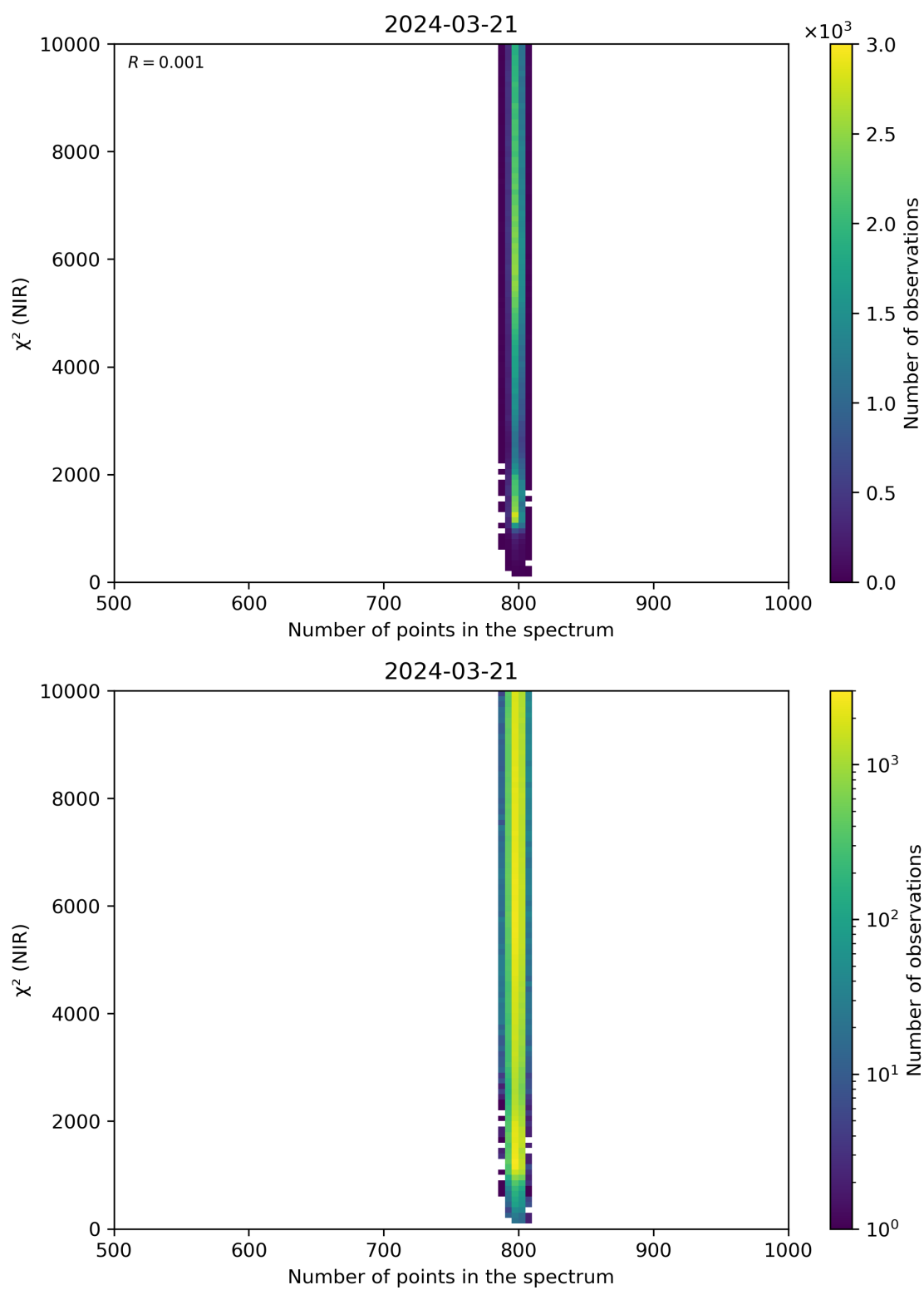
Figure 88: Scatter density plot of “Number of points in the spectrum” against “ \chi^2 (NIR)” for 2024-03-20 to 2024-03-22.
