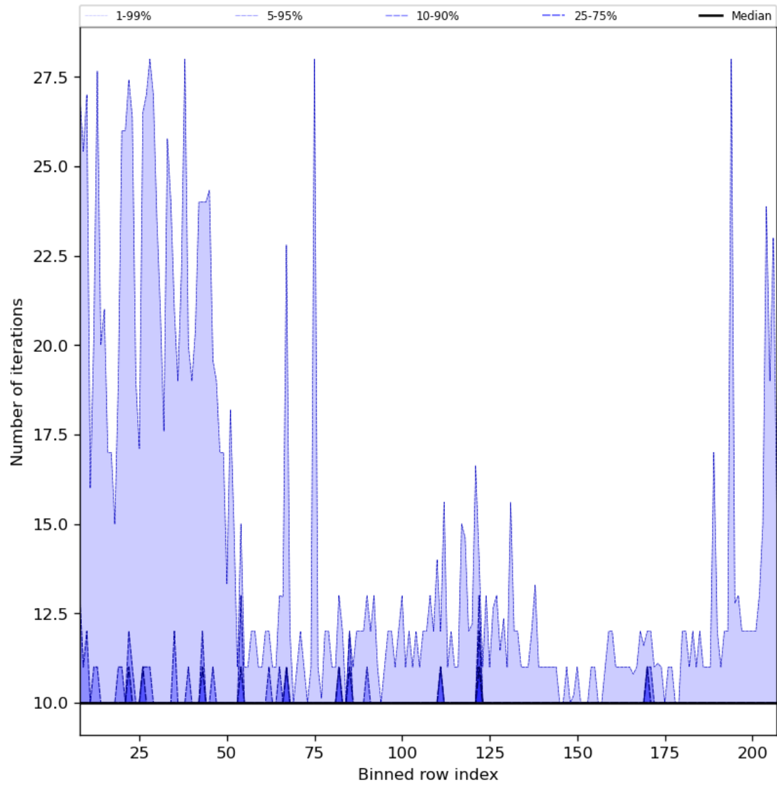
Figure 42: Along track statistics of “Number of iterations” for 2024-03-20 to 2024-03-22
