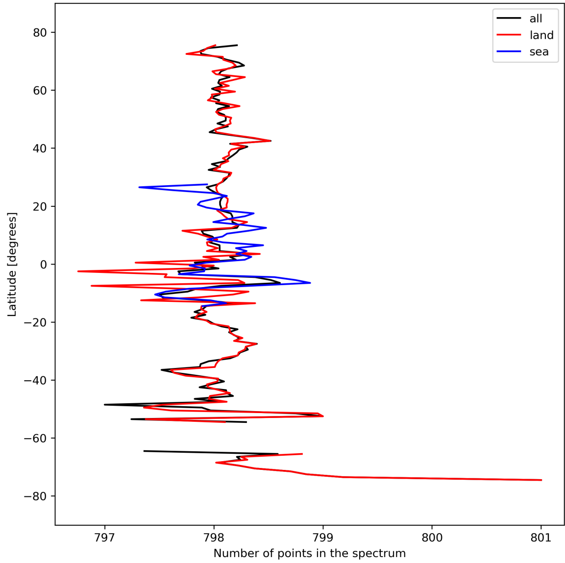
Figure 15: Zonal average of “Number of points in the spectrum” for 2024-03-20 to 2024-03-22.
