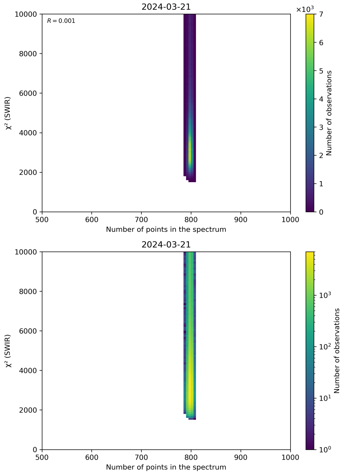
Figure 89: Scatter density plot of “Number of points in the spectrum” against “ \chi^2 (SWIR)” for 2024-03-20 to 2024-03-22.
