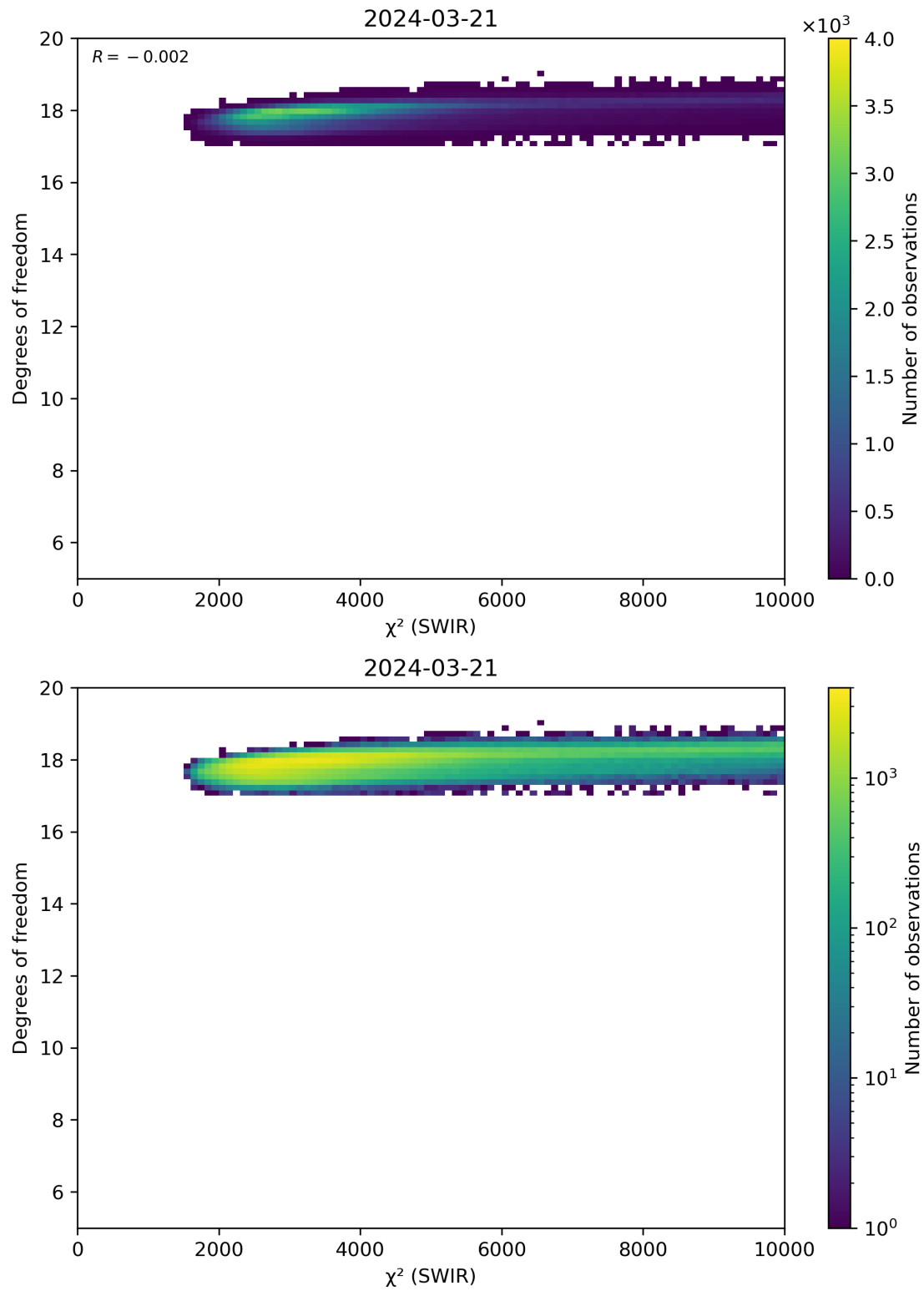
Figure 48: Scatter density plot of “ \chi^2 (SWIR)” against “Degrees of freedom” for 2024-03-20 to 2024-03-22.
