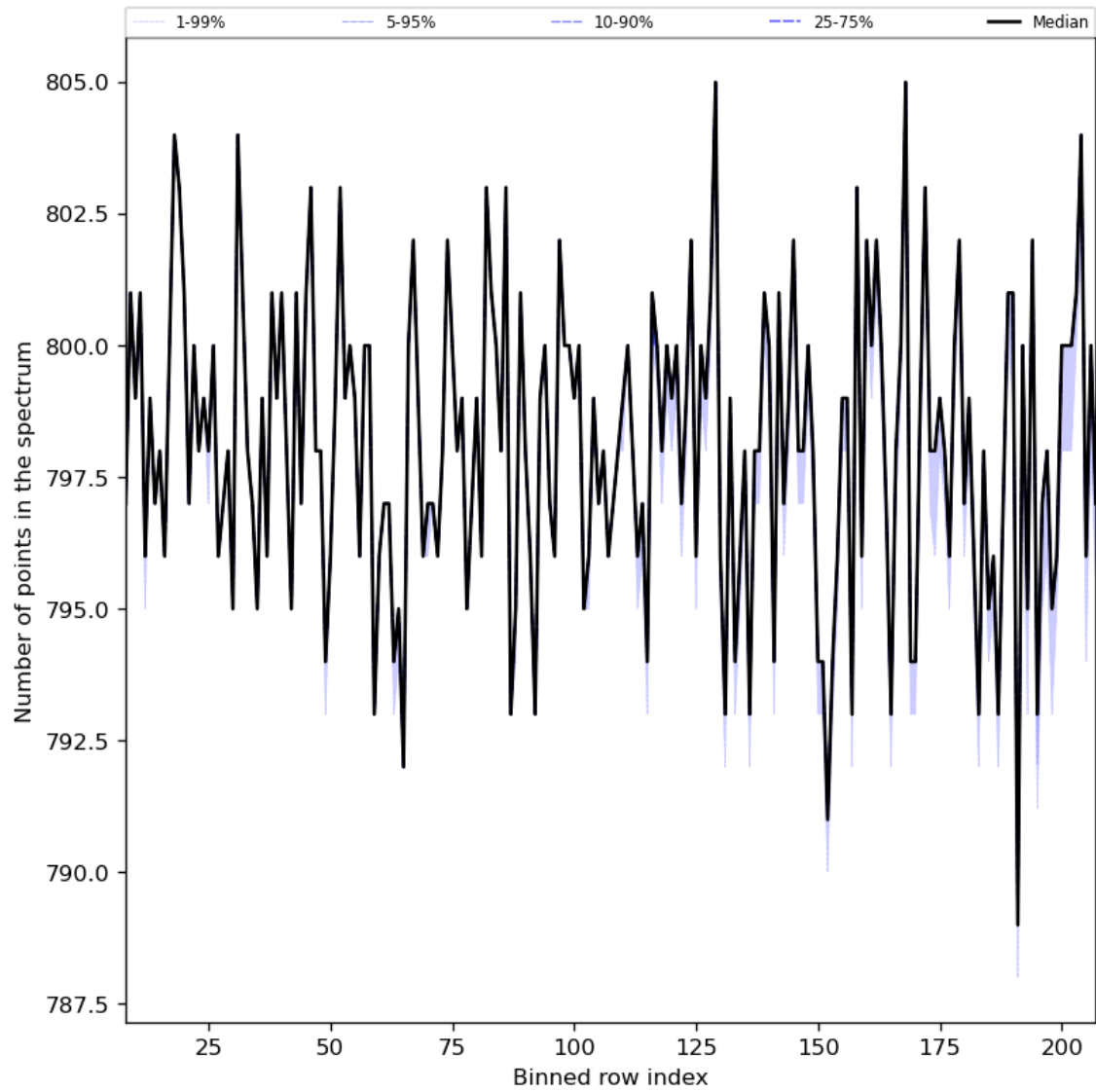
Figure 37: Along track statistics of “Number of points in the spectrum” for 2024-03-20 to 2024-03-22
