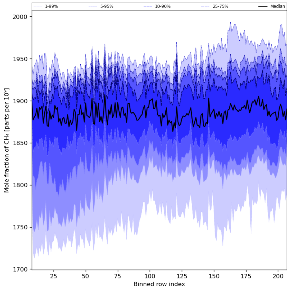
Figure 34: Along track statistics of “Mole fraction of CH 4 ” for 2024-03-20 to 2024-03-22
