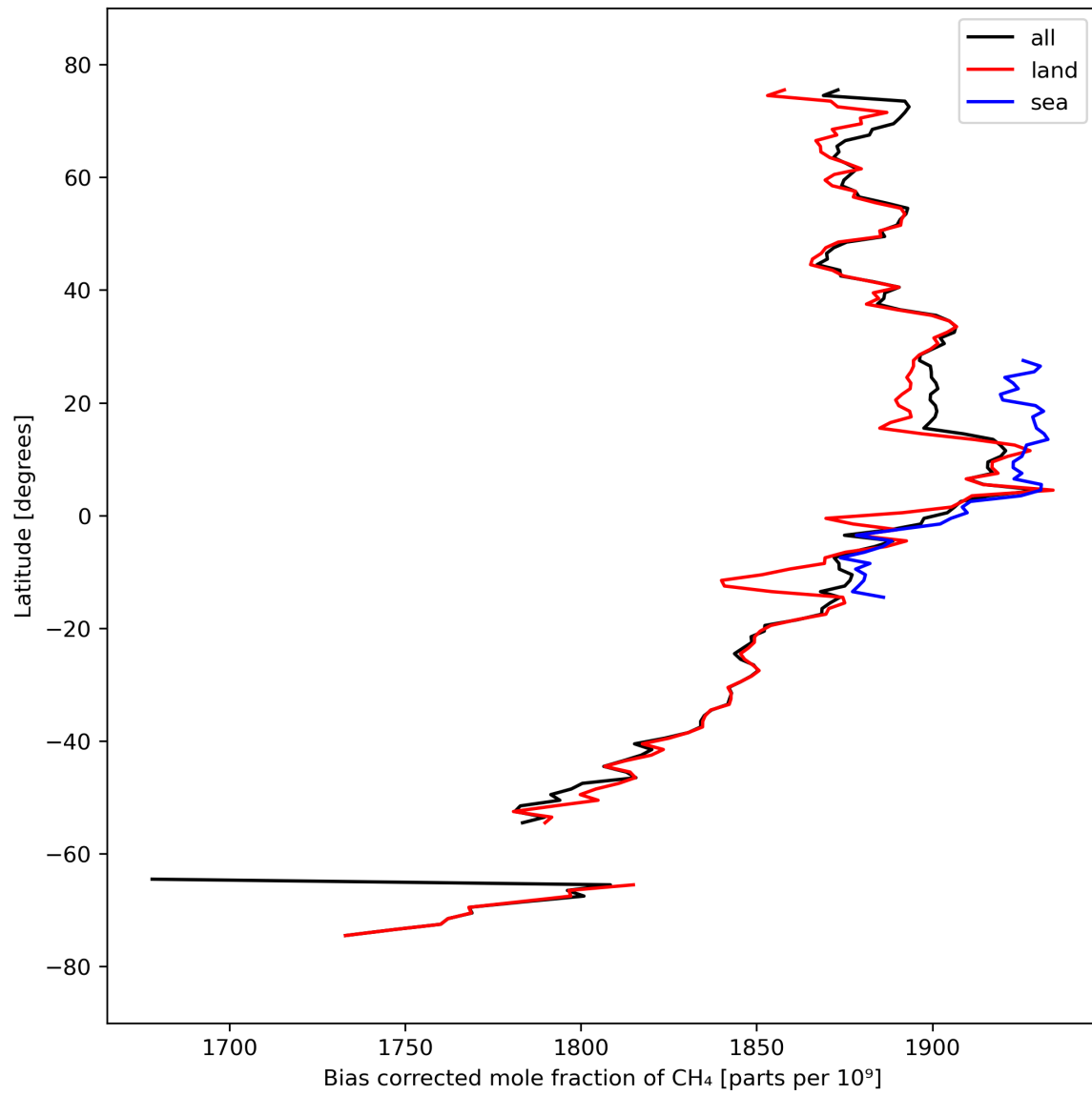
Figure 14: Zonal average of “Bias corrected mole fraction of \text{CH}_4 ” for 2024-03-20 to 2024-03-22.
