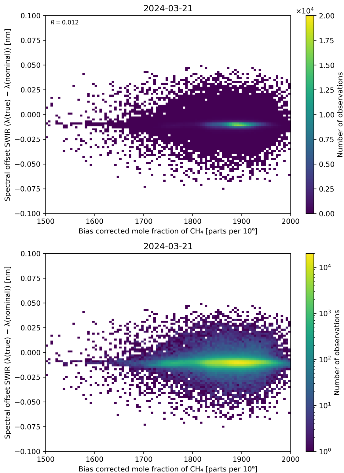
Figure 69: Scatter density plot of “Bias corrected mole fraction of \text{CH}_4 ” against “Spectral offset SWIR ( \lambda(\text{true}) - \lambda(\text{nominal}) )” for 2024-03-20 to 2024-03-22.
