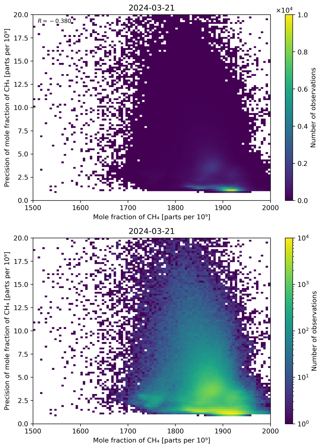
Figure 75: Scatter density plot of “Mole fraction of CH 4 ” against “Precision of mole fraction of CH 4 ” for 2024-03-20 to 2024-03-22.
