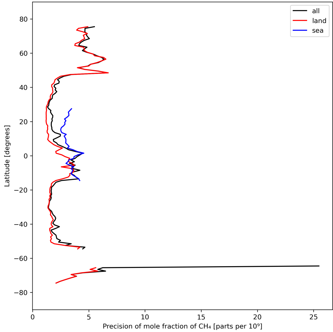
Figure 13: Zonal average of “Precision of mole fraction of CH 4 ” for 2024-03-20 to 2024-03-22.
