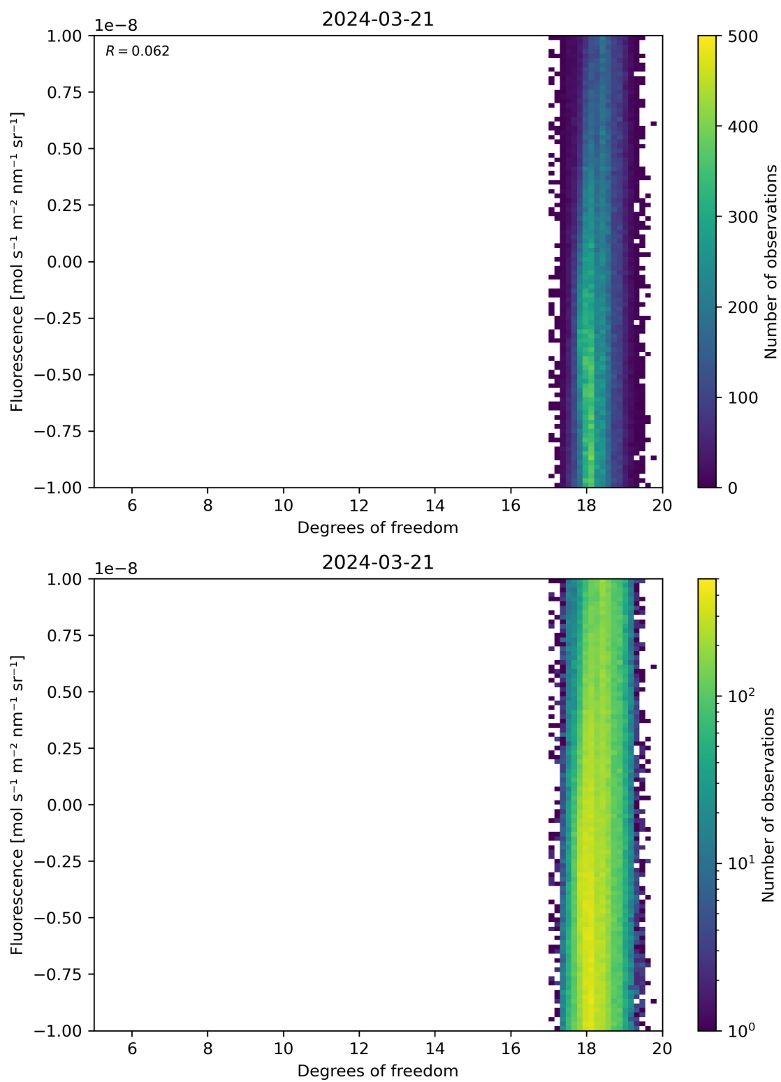
Figure 51: Scatter density plot of “Degrees of freedom” against “Fluorescence” for 2024-03-20 to 2024-03-22.
