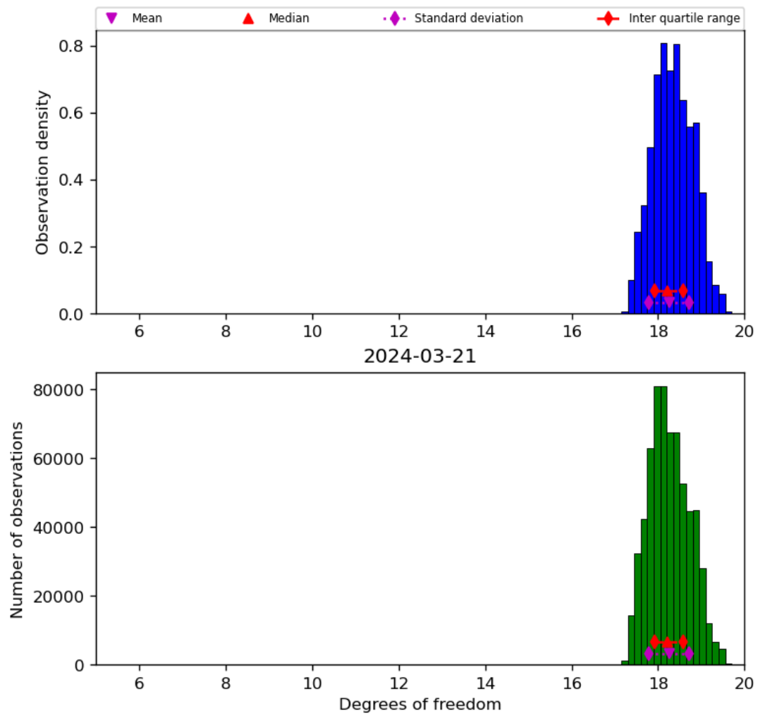
Figure 30: Histogram of “Degrees of freedom” for 2024-03-20 to 2024-03-22
