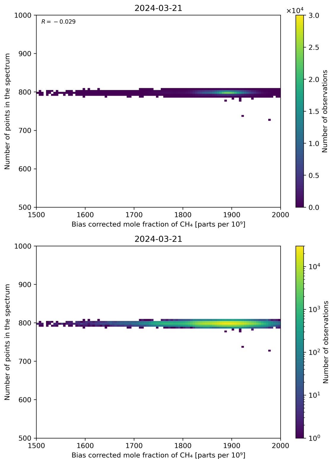
Figure 68: Scatter density plot of “Bias corrected mole fraction of CH 4 ” against “Number of points in the spectrum” for 2024-03-20 to 2024-03-22.
