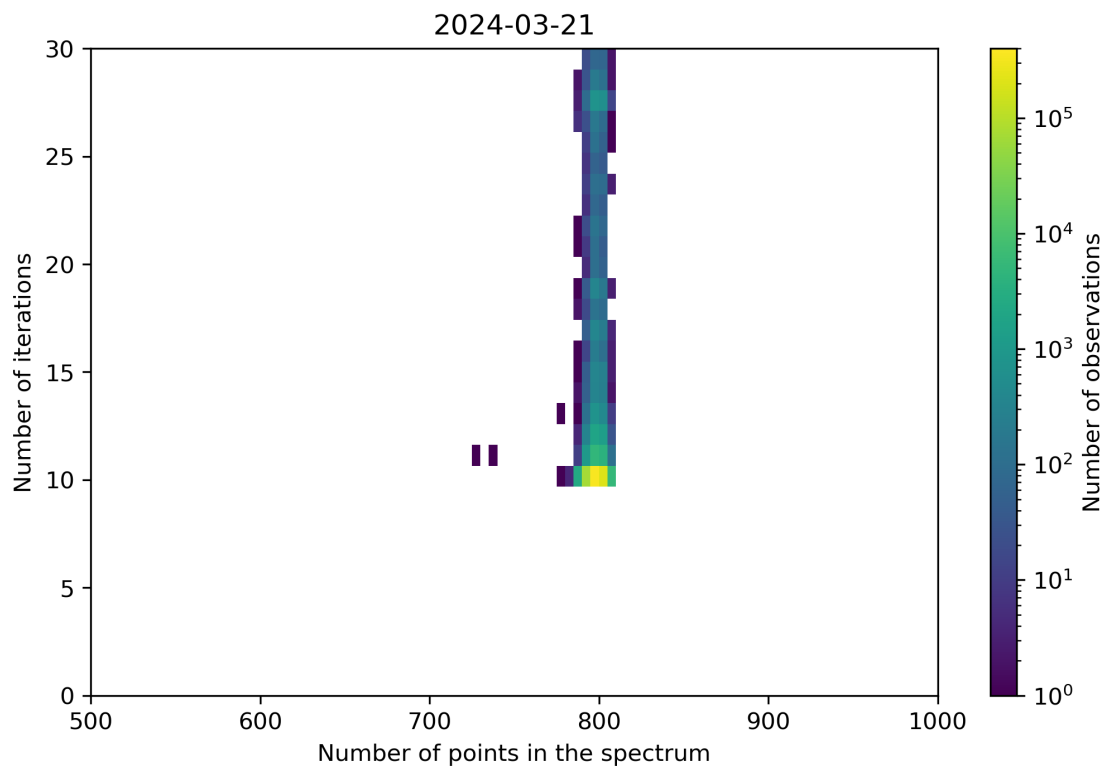
Figure 92: Scatter density plot of “Number of points in the spectrum” against “Number of iterations” for 2024-03-20 to 2024-03-22.
