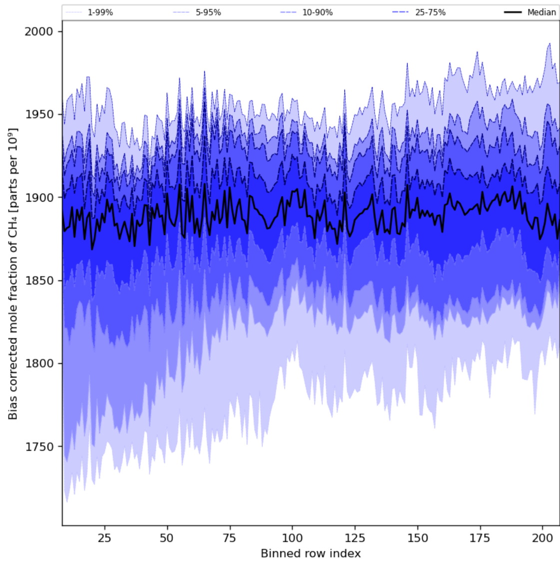
Figure 36: Along track statistics of “Bias corrected mole fraction of CH 4 ” for 2024-03-20 to 2024-03-22
