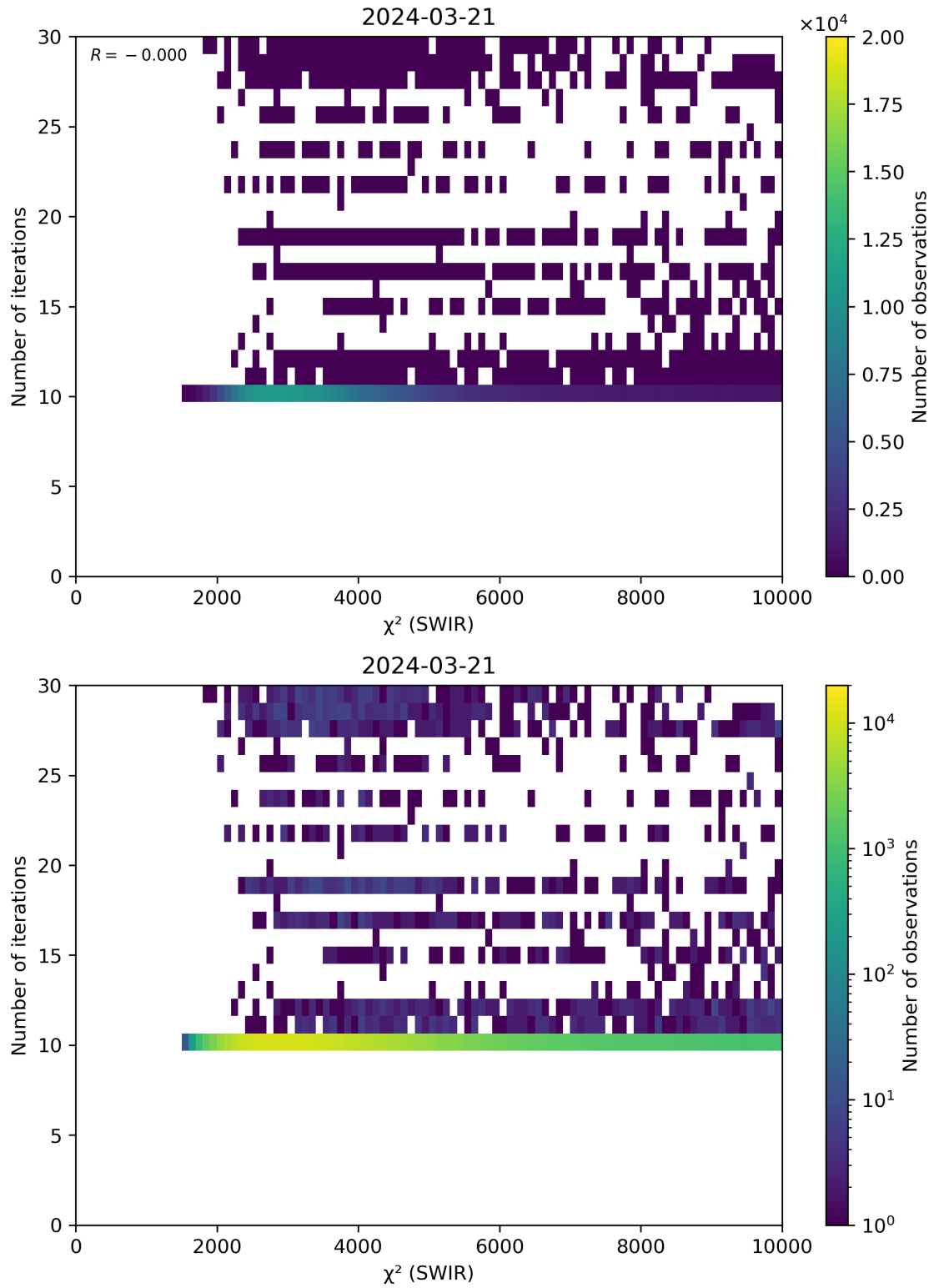
Figure 50: Scatter density plot of “ \chi^2 (SWIR)” against “Number of iterations” for 2024-03-20 to 2024-03-22.
