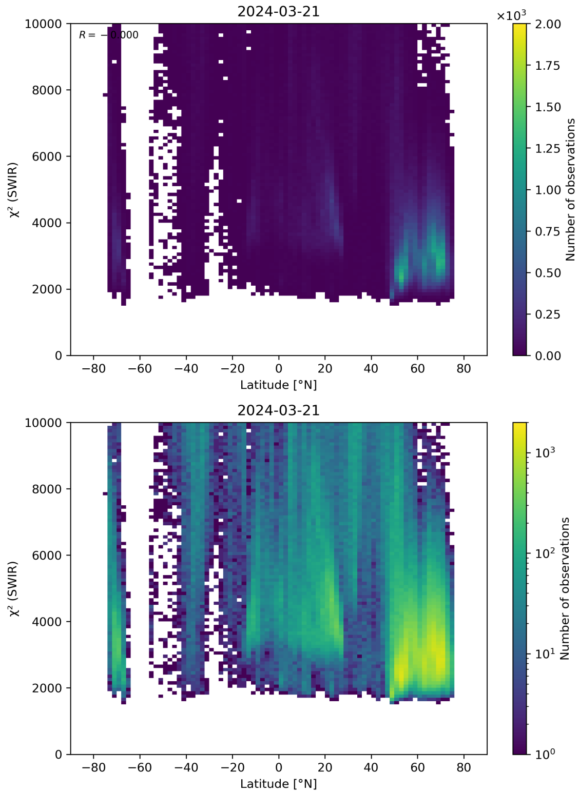
Figure 54: Scatter density plot of “Latitude” against “ \chi^2 (SWIR)” for 2024-03-20 to 2024-03-22.
