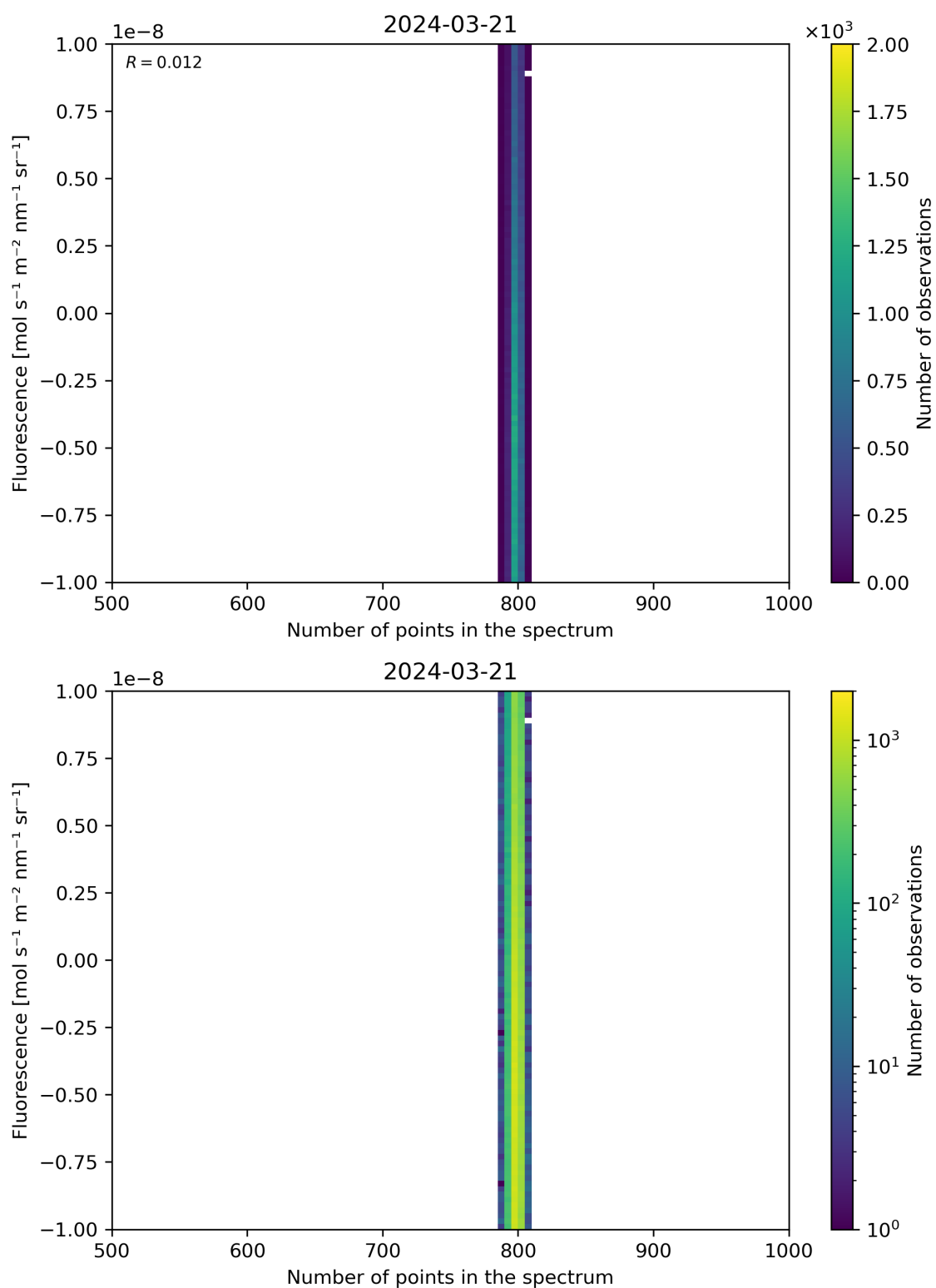
Figure 91: Scatter density plot of “Number of points in the spectrum” against “Fluorescence” for 2024-03-20 to 2024-03-22.
