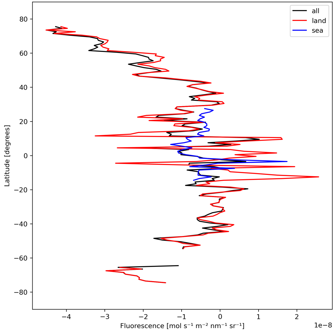
Figure 21: Zonal average of “Fluorescence” for 2024-03-20 to 2024-03-22.
