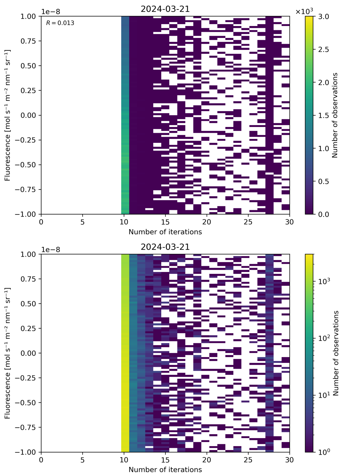
Figure 87: Scatter density plot of “Number of iterations” against “Fluorescence” for 2024-03-20 to 2024-03-22.
