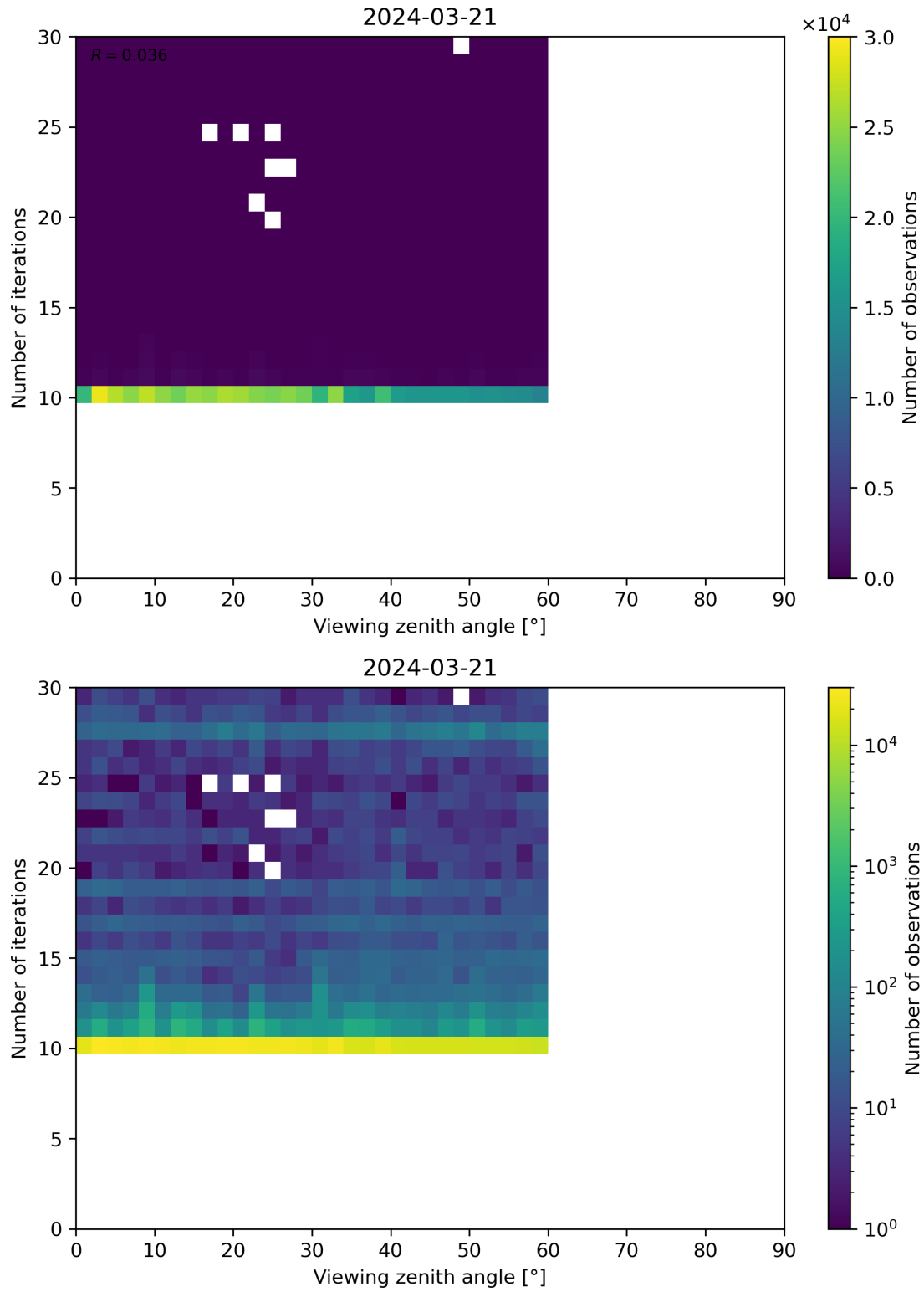
Figure 113: Scatter density plot of “Viewing zenith angle” against “Number of iterations” for 2024-03-20 to 2024-03-22.
