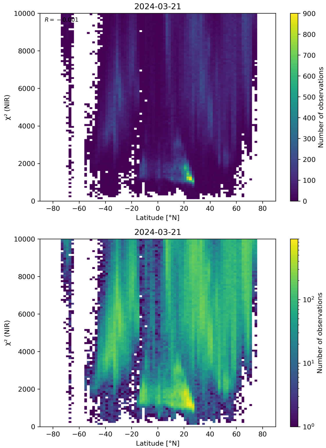
Figure 53: Scatter density plot of “Latitude” against “ \chi^2 (NIR)” for 2024-03-20 to 2024-03-22.
