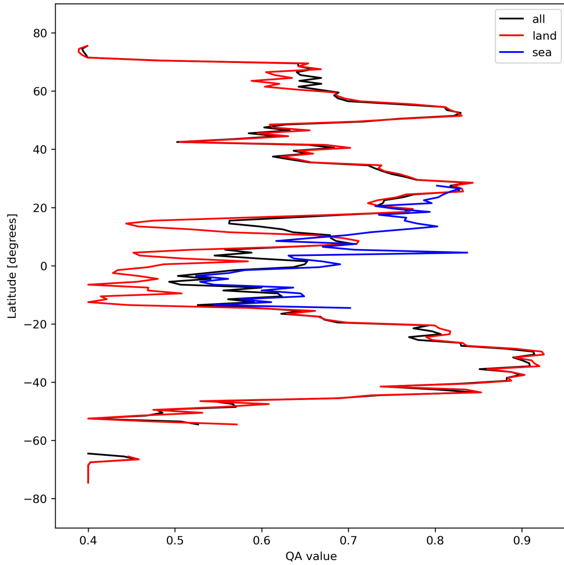
Figure 11: Zonal average of “QA value” for 2024-03-20 to 2024-03-22.
