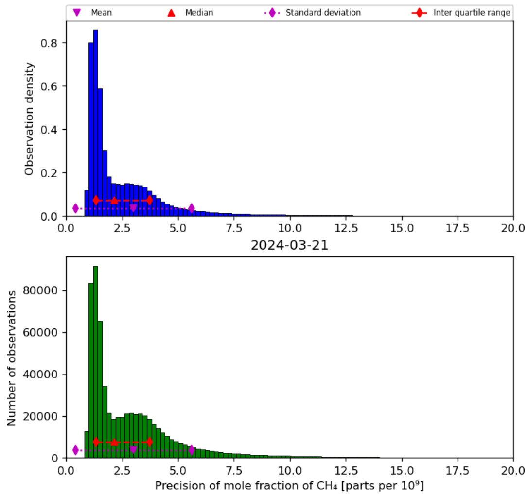
Figure 24: Histogram of “Precision of mole fraction of CH 4 ” for 2024-03-20 to 2024-03-22
