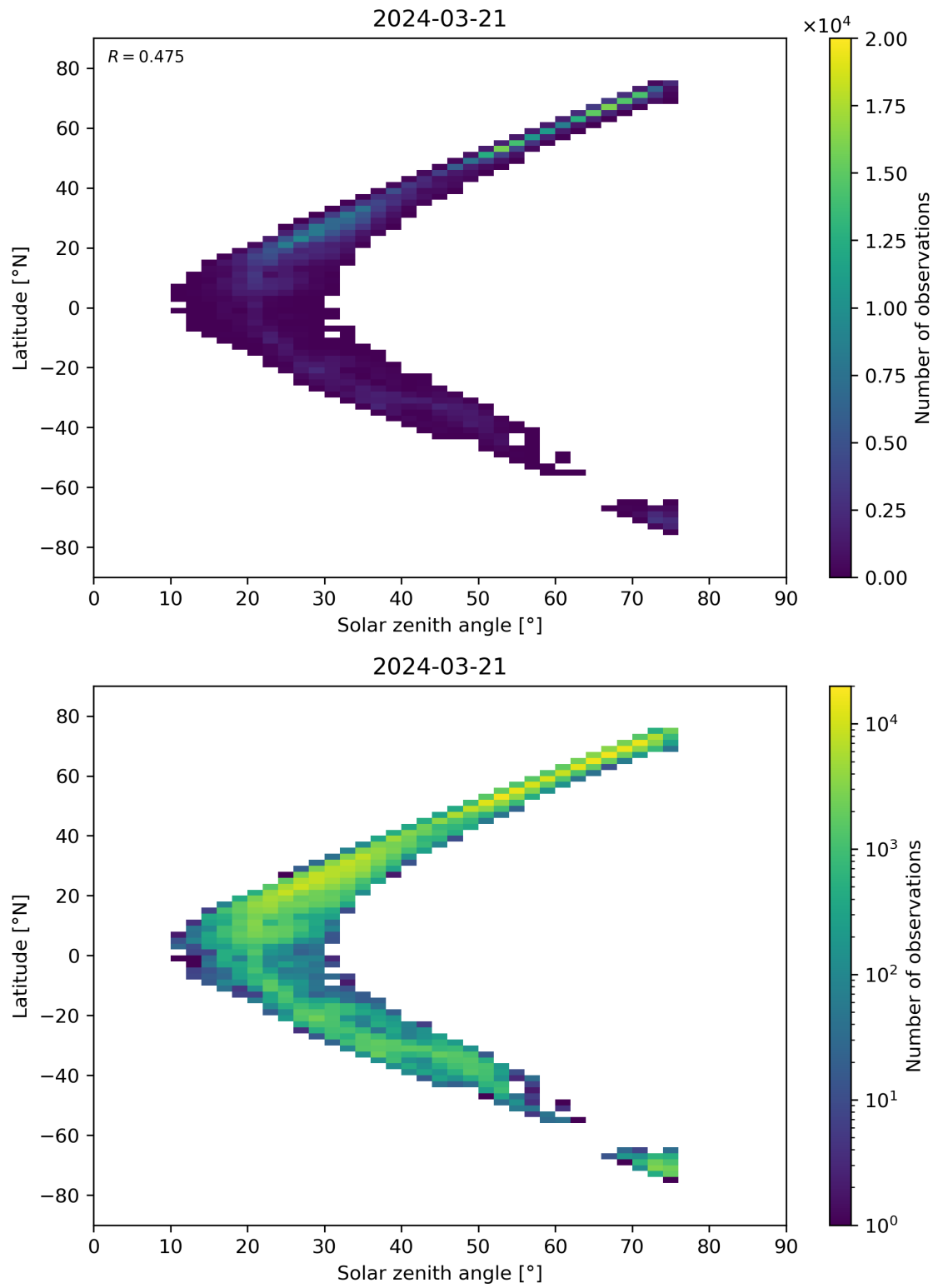
Figure 98: Scatter density plot of “Solar zenith angle” against “Latitude” for 2024-03-20 to 2024-03-22.
