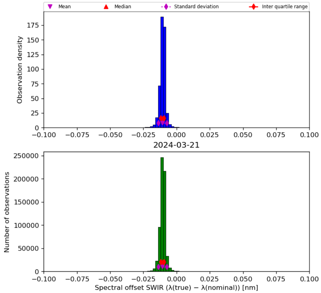
Figure 27: Histogram of “Spectral offset SWIR ( \lambda(\text{true}) - \lambda(\text{nominal}) )” for 2024-03-20 to 2024-03-22
