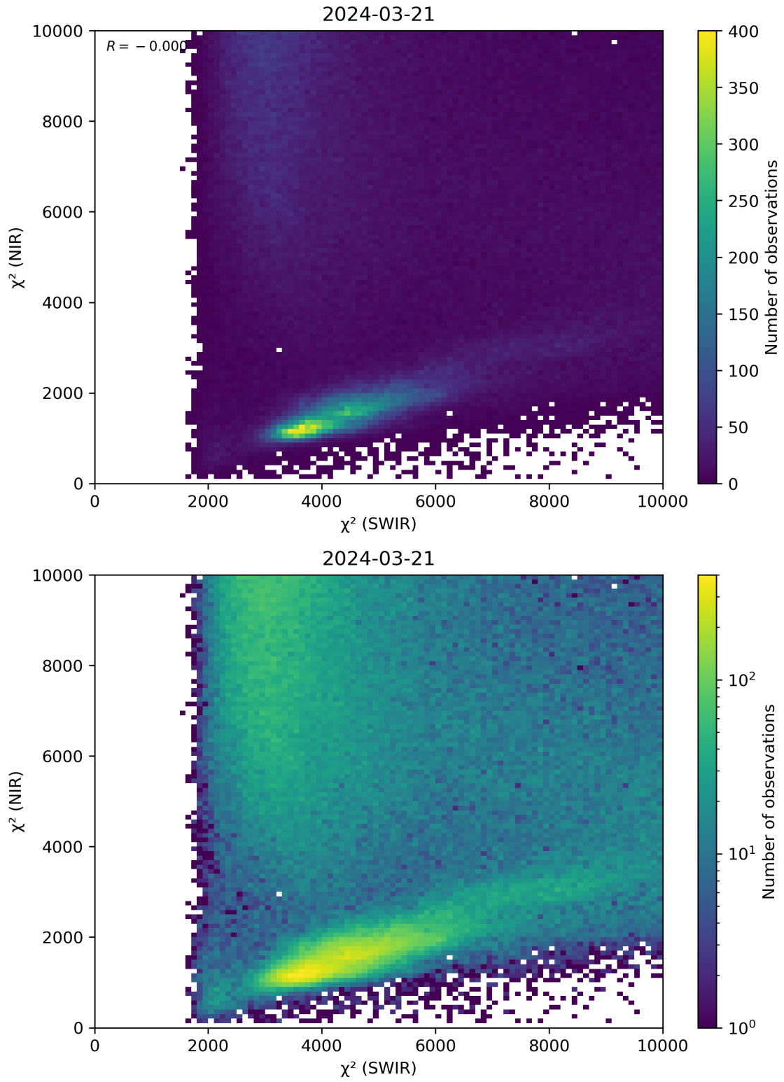
Figure 47: Scatter density plot of “ \chi^2 (SWIR)” against “ \chi^2 (NIR)” for 2024-03-20 to 2024-03-22.
