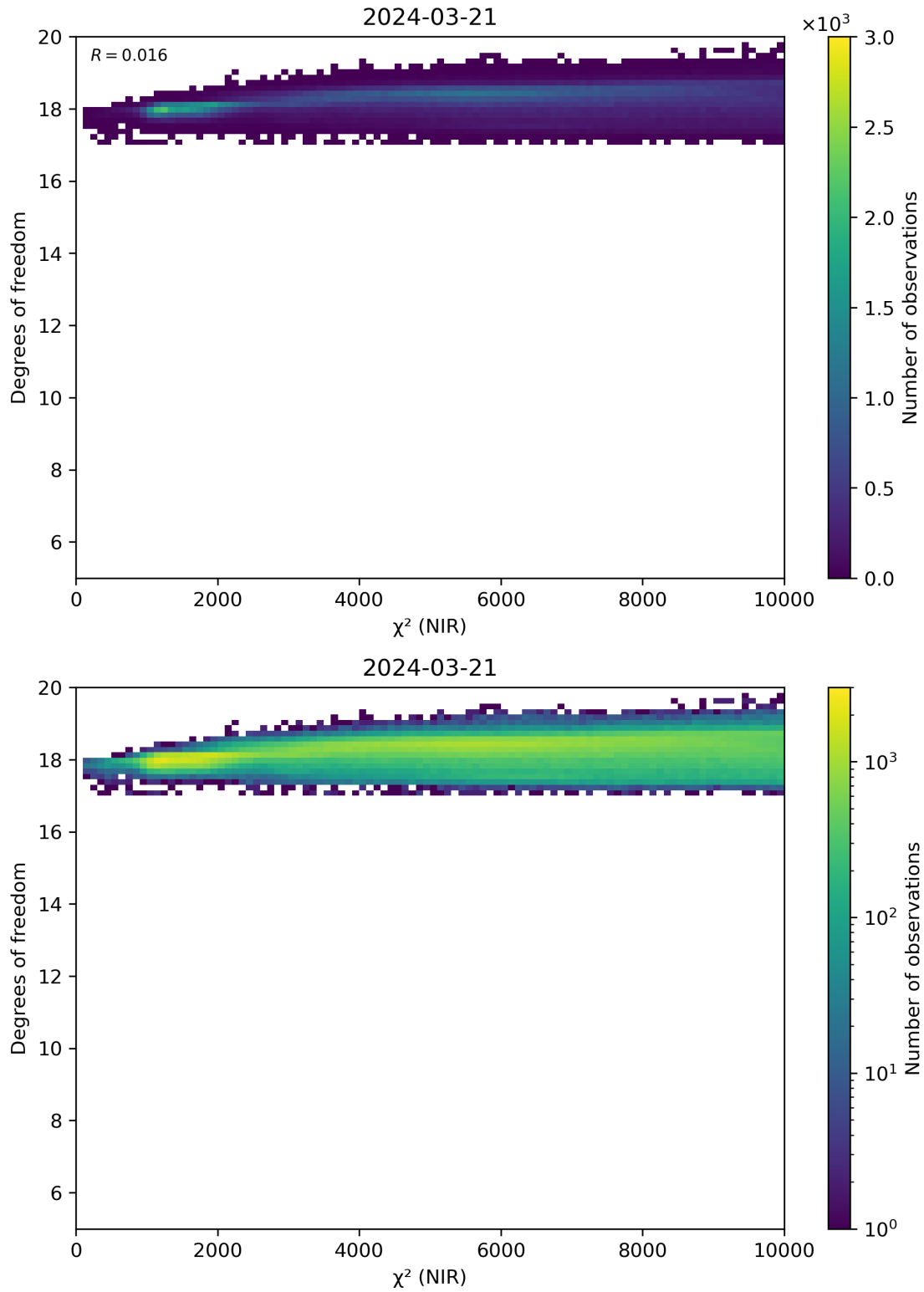
Figure 44: Scatter density plot of “ \chi^2 (NIR)” against “Degrees of freedom” for 2024-03-20 to 2024-03-22.
