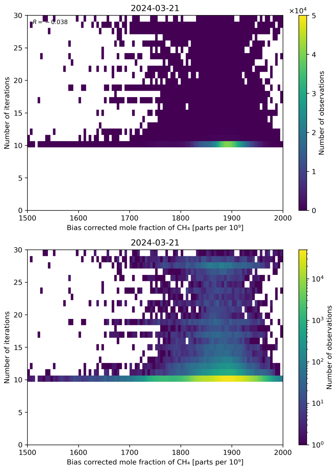
Figure 67: Scatter density plot of “Bias corrected mole fraction of CH 4 ” against “Number of iterations” for 2024-03-20 to 2024-03-22.
