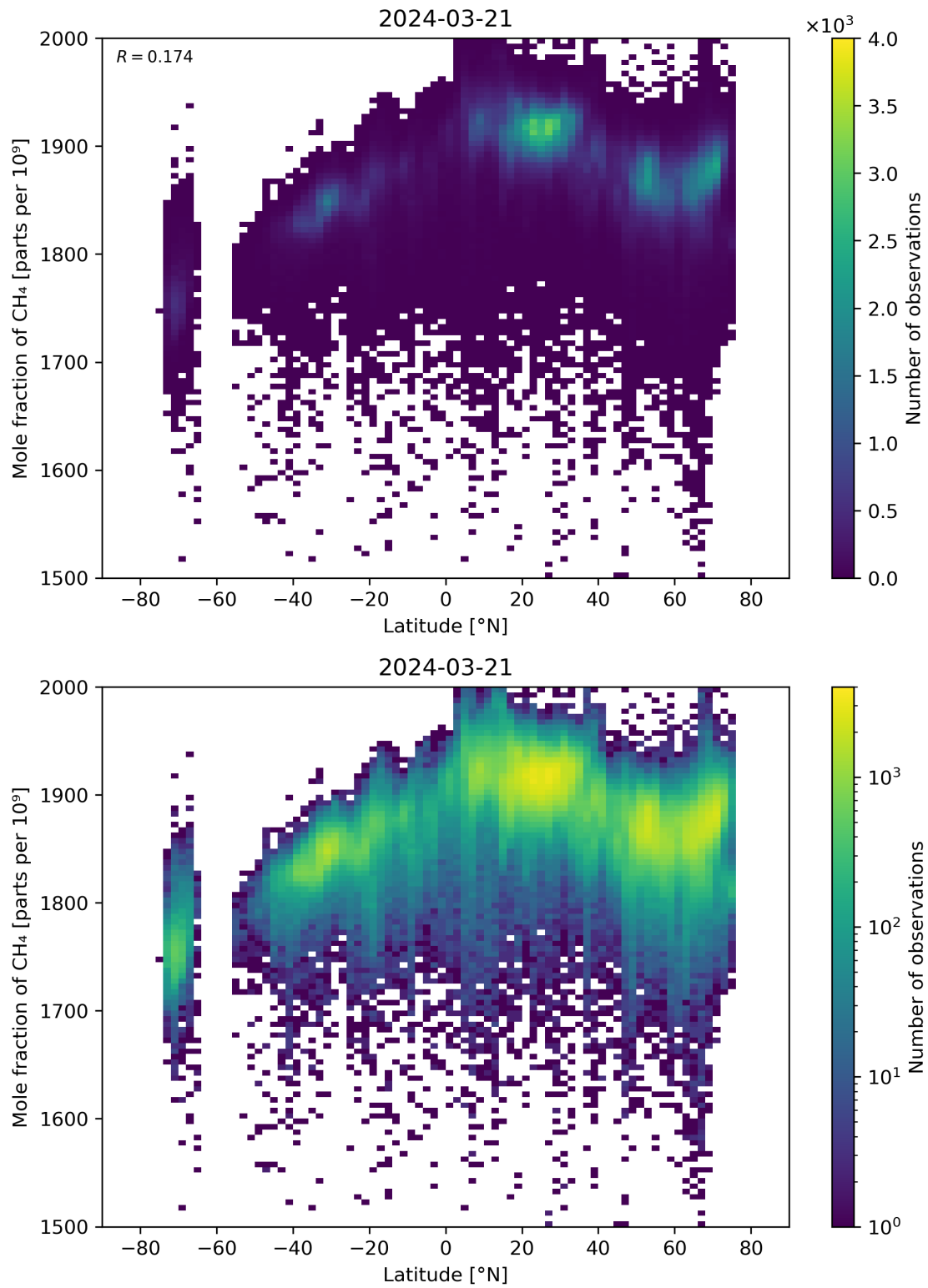
Figure 57: Scatter density plot of “Latitude” against “Mole fraction of \text{CH}_4 ” for 2024-03-20 to 2024-03-22.
