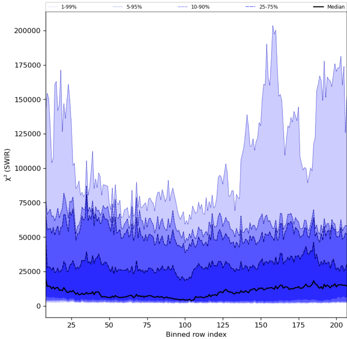
Figure 39: Along track statistics of “ \chi^2 (SWIR)” for 2024-03-20 to 2024-03-22
