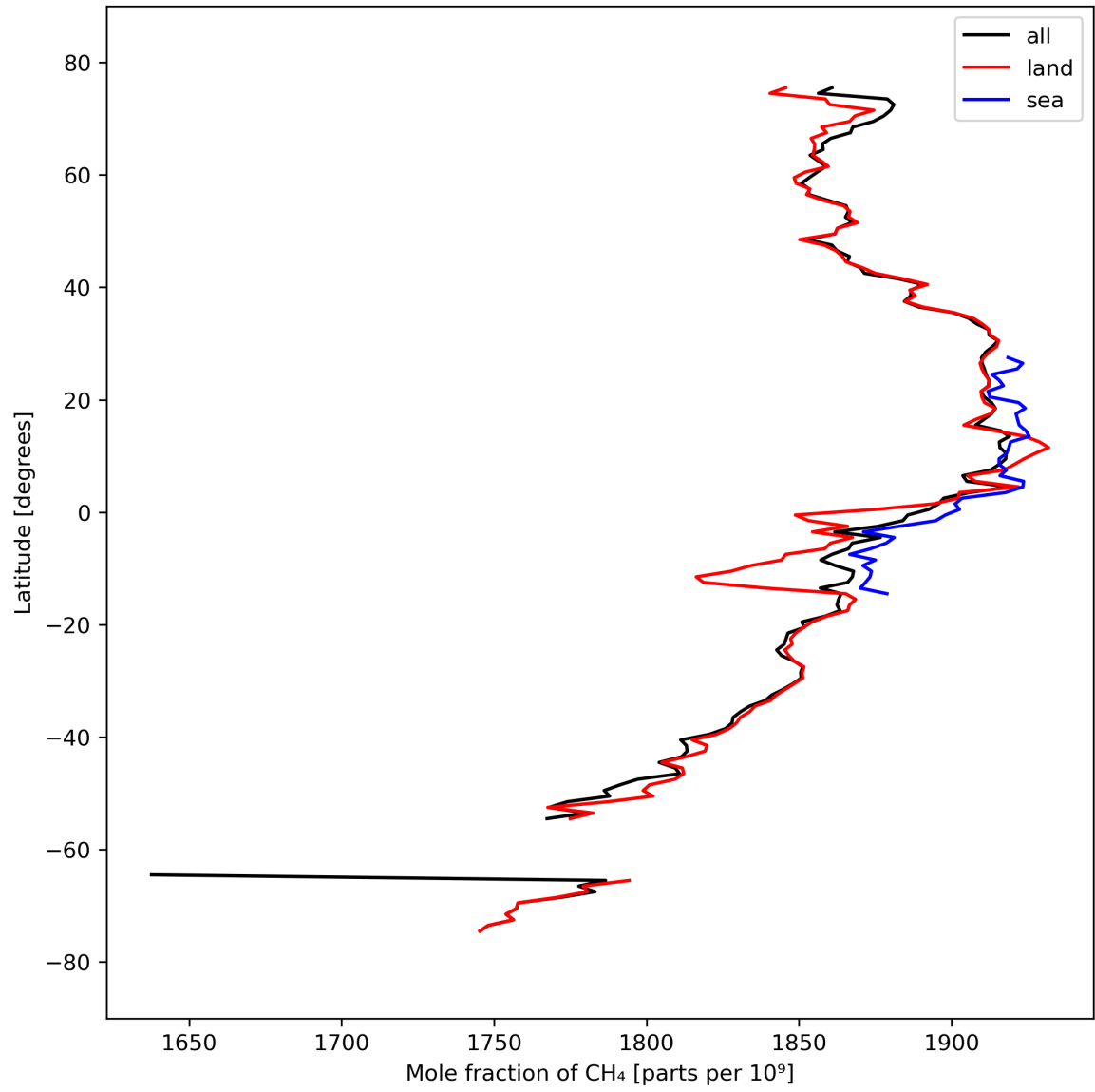
Figure 12: Zonal average of “Mole fraction of CH 4 ” for 2024-03-20 to 2024-03-22.
