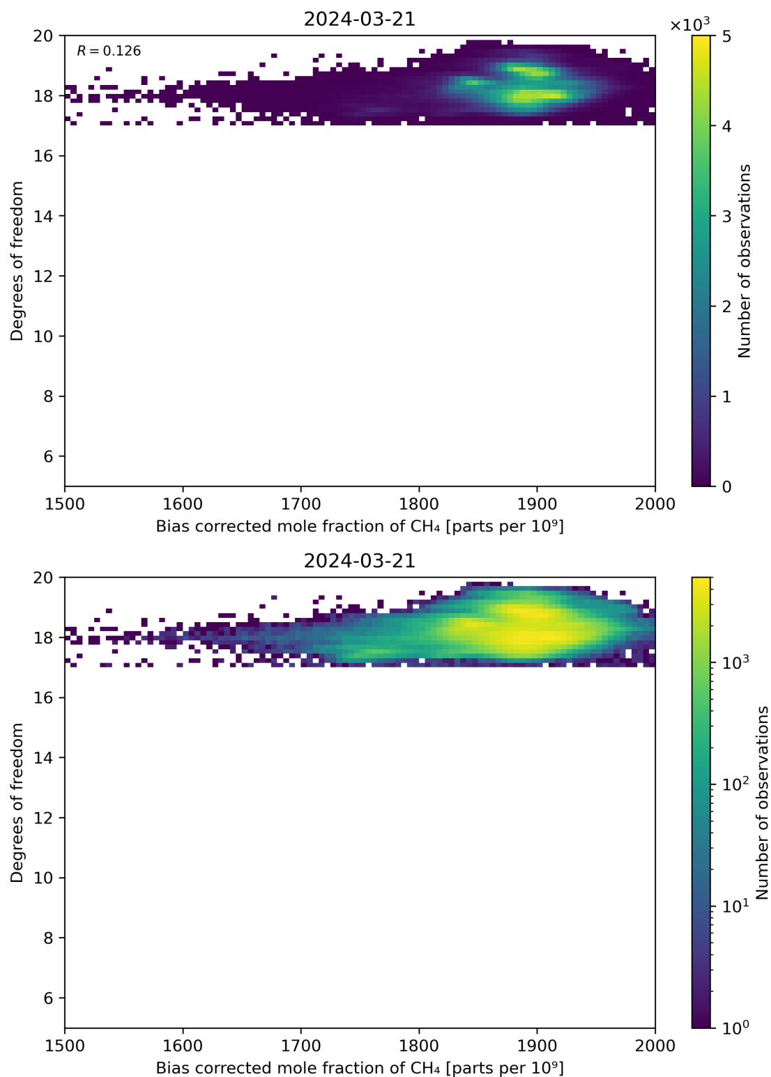
Figure 65: Scatter density plot of “Bias corrected mole fraction of CH 4 ” against “Degrees of freedom” for 2024-03-20 to 2024-03-22.
