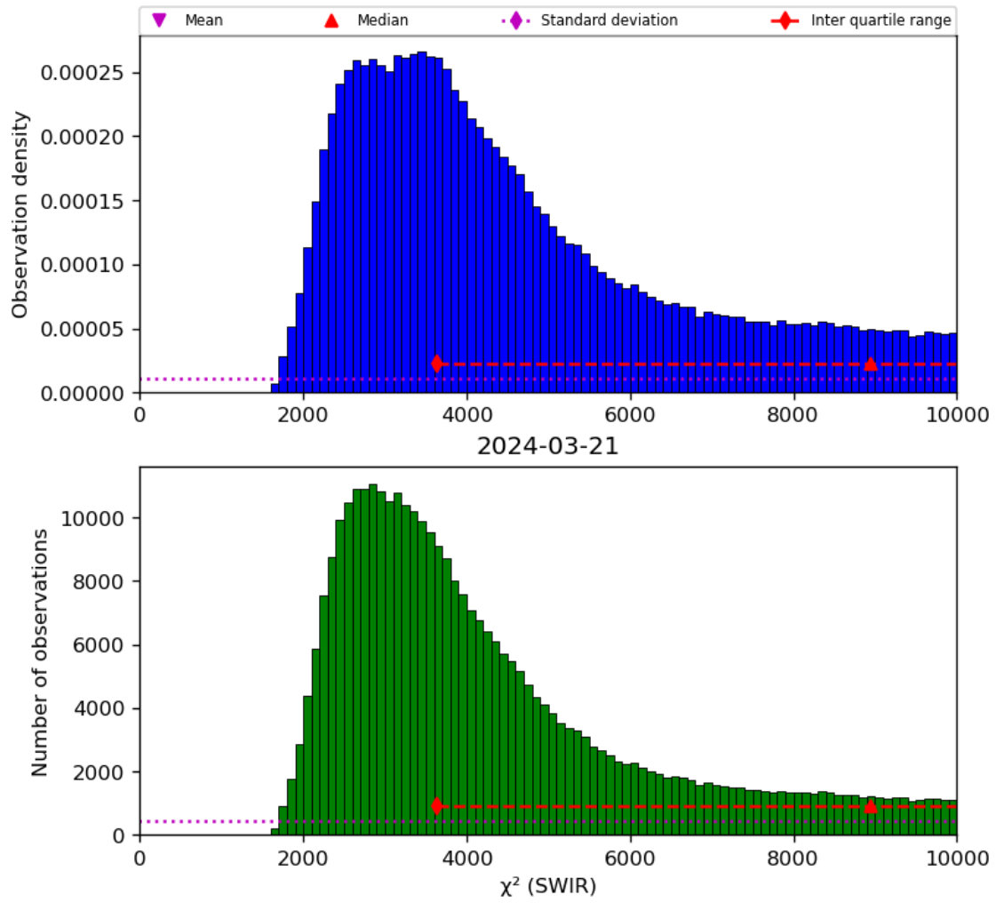
Figure 28: Histogram of “ \chi^2 (SWIR)” for 2024-03-20 to 2024-03-22
