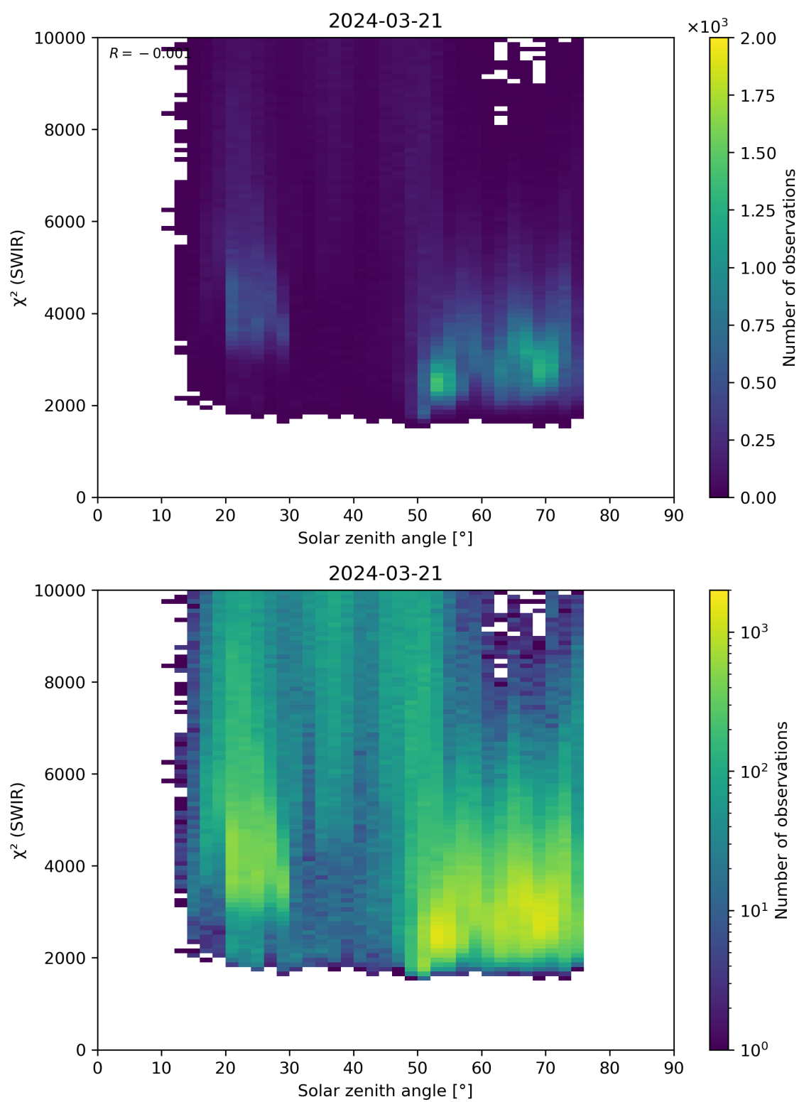
Figure 95: Scatter density plot of “Solar zenith angle” against “ \chi^2 (SWIR)” for 2024-03-20 to 2024-03-22.
