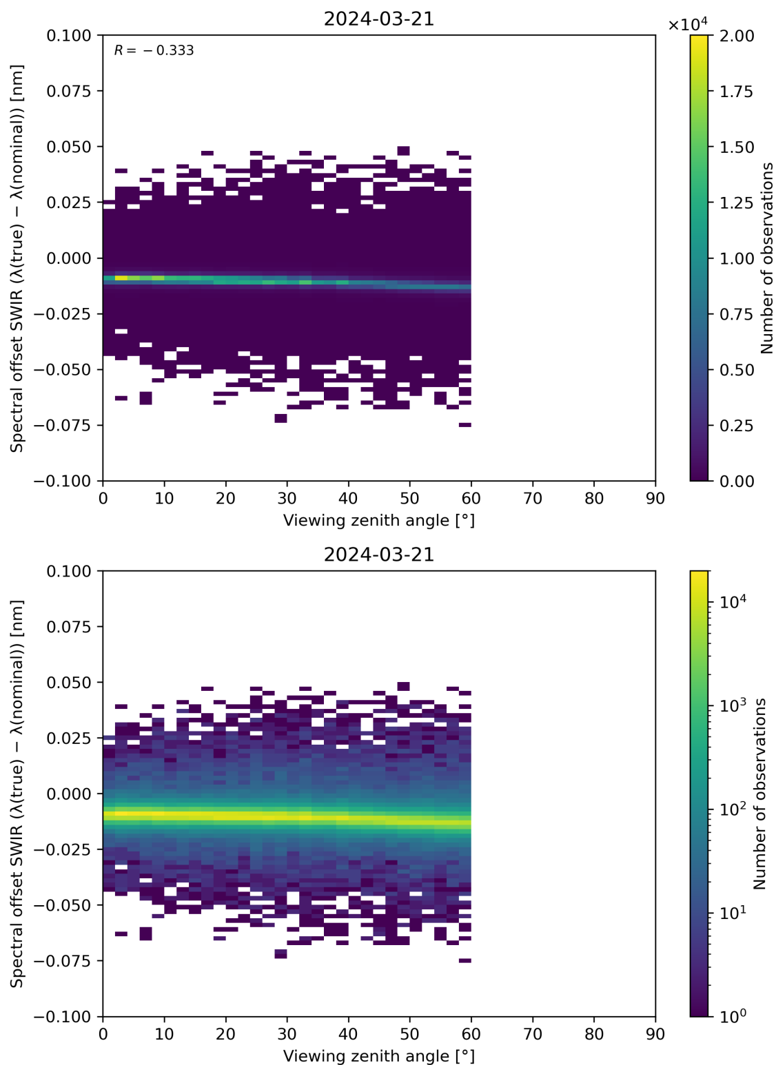
Figure 116: Scatter density plot of “Viewing zenith angle” against “Spectral offset SWIR ( \lambda(\text{true}) - \lambda(\text{nominal}) )” for 2024-03-20 to 2024-03-22.
