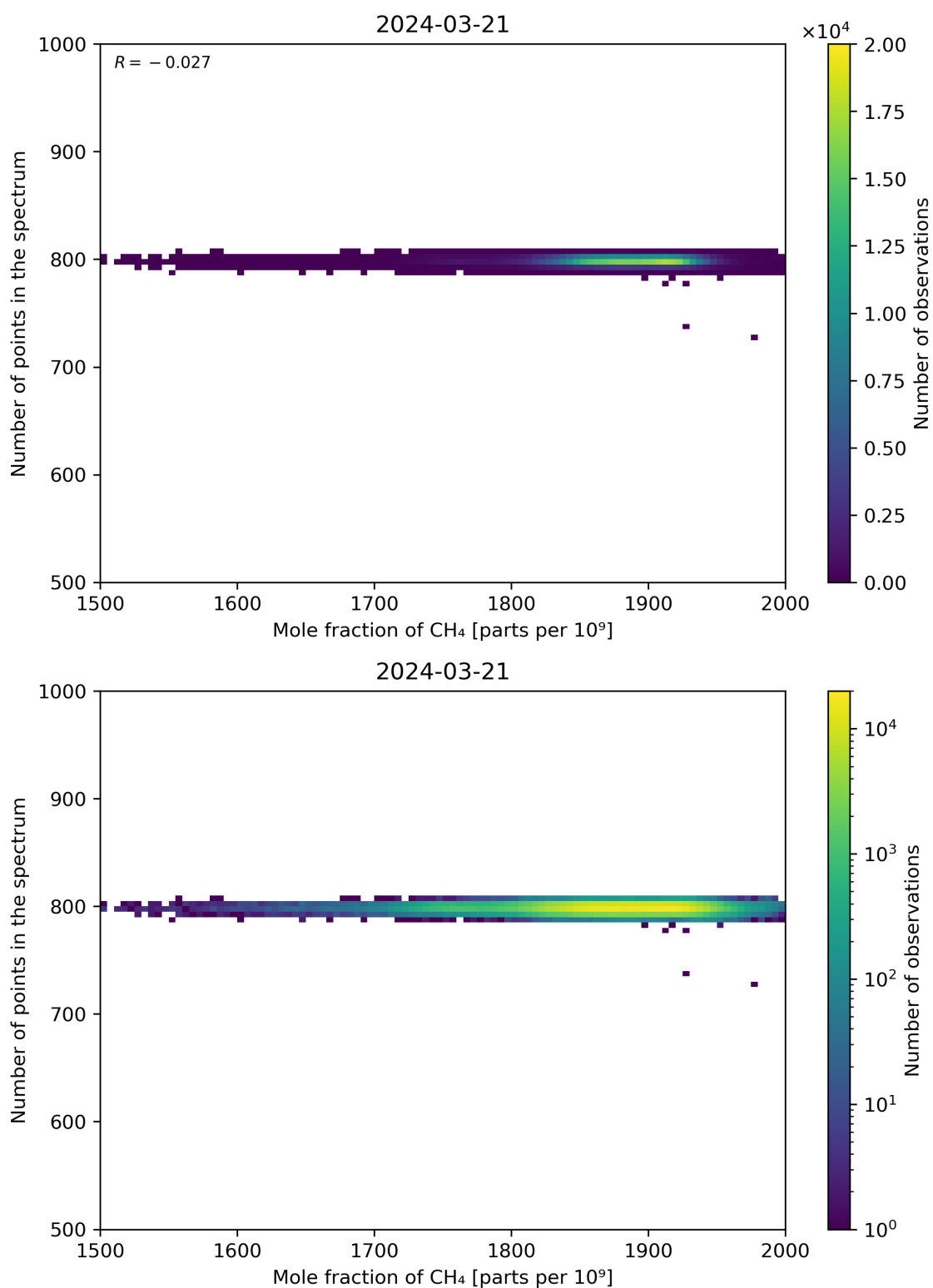
Figure 77: Scatter density plot of “Mole fraction of CH 4 ” against “Number of points in the spectrum” for 2024-03-20 to 2024-03-22.
