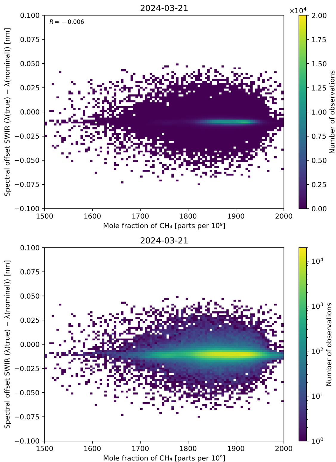
Figure 86: Scatter density plot of “Mole fraction of CH 4 ” against “Spectral offset SWIR ( \lambda(\text{true}) - \lambda(\text{nominal}) )” for 2024-03-20 to 2024-03-22.
