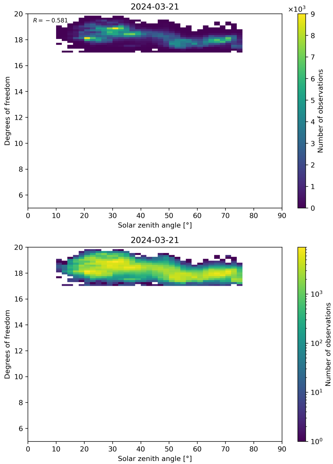
Figure 96: Scatter density plot of “Solar zenith angle” against “Degrees of freedom” for 2024-03-20 to 2024-03-22.
