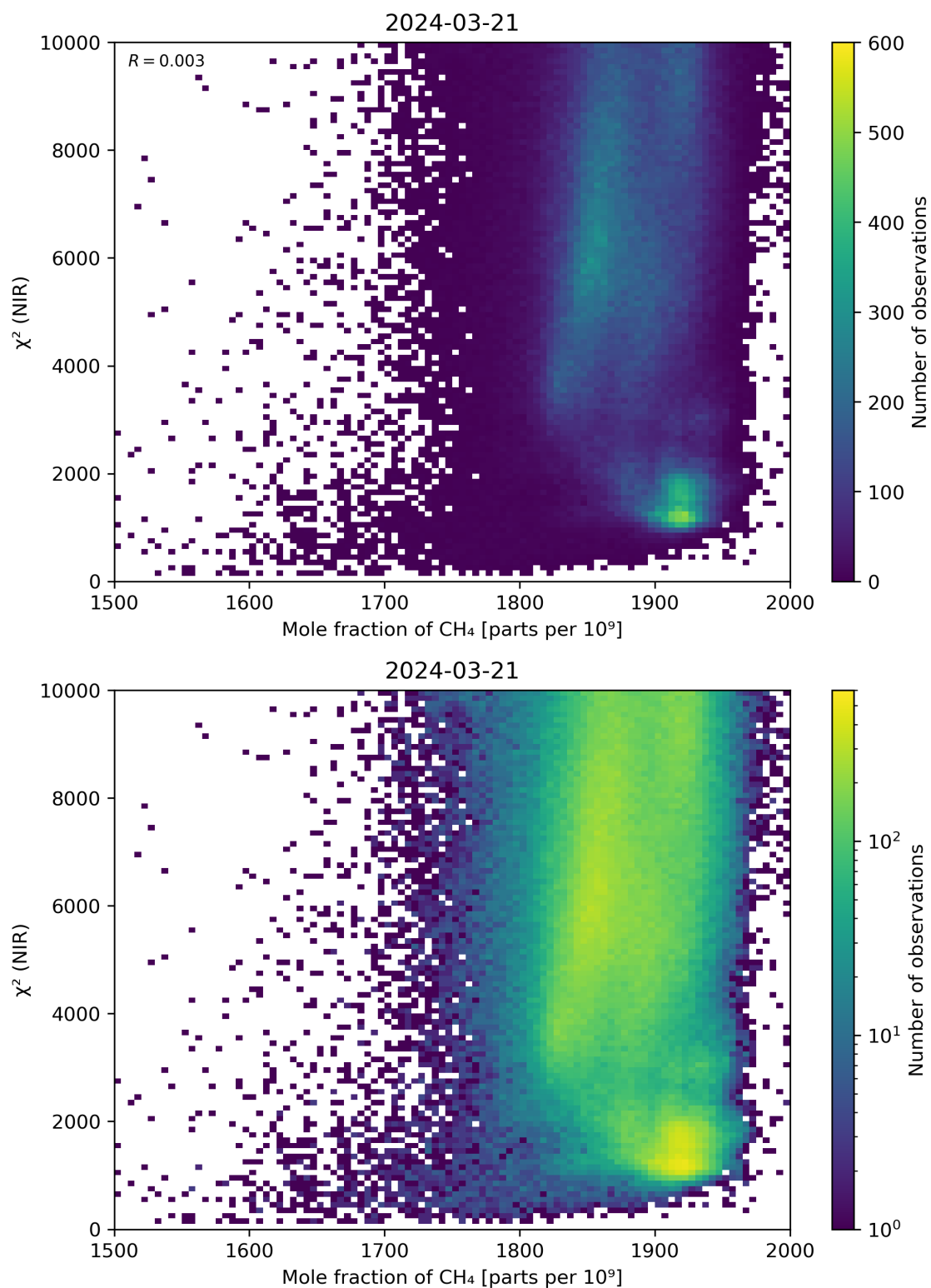
Figure 70: Scatter density plot of “Mole fraction of CH 4 ” against “ \chi^2 (NIR)” for 2024-03-20 to 2024-03-22.
