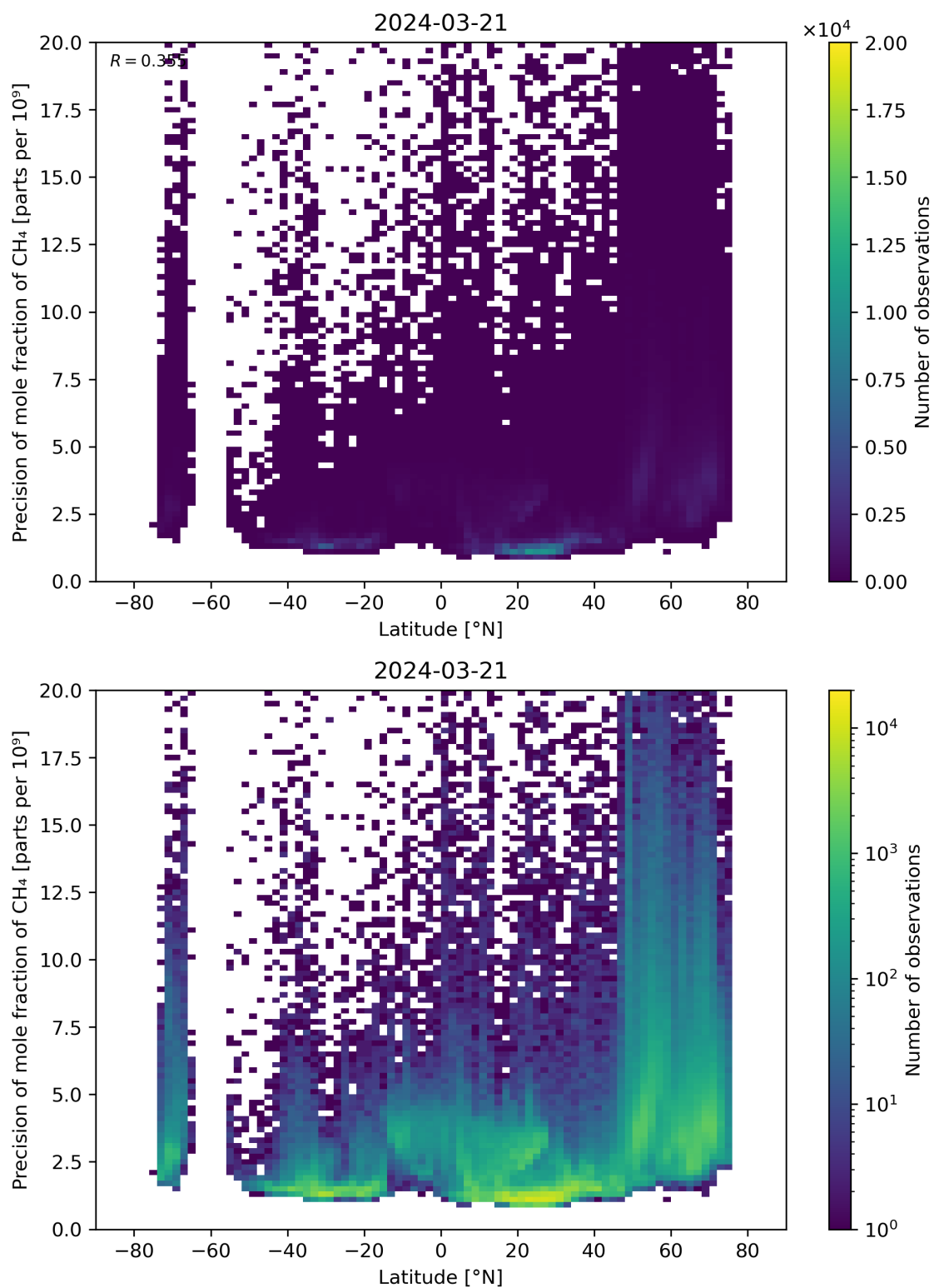
Figure 59: Scatter density plot of “Latitude” against “Precision of mole fraction of \text{CH}_4 ” for 2024-03-20 to 2024-03-22.
