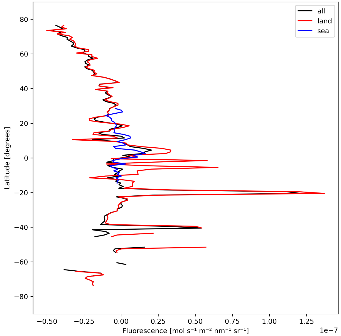
Figure 21: Zonal average of “Fluorescence” for 2024-03-21 to 2024-03-22.
