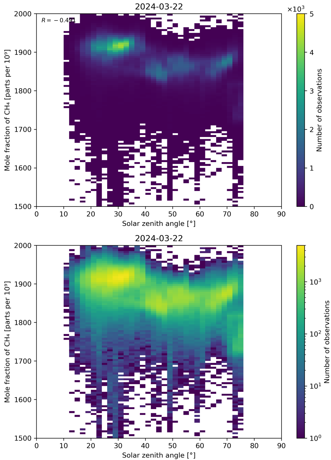
Figure 99: Scatter density plot of “Solar zenith angle” against “Mole fraction of CH 4 ” for 2024-03-21 to 2024-03-22.
