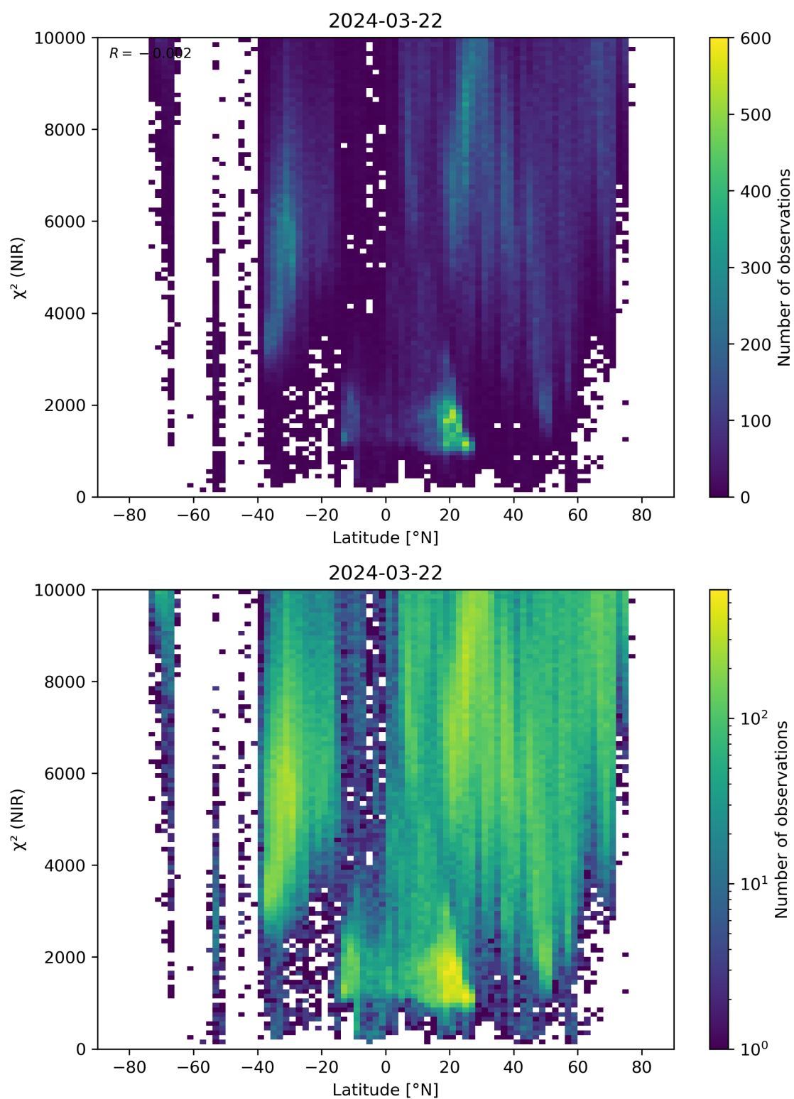
Figure 53: Scatter density plot of “Latitude” against “ \chi^2 (NIR)” for 2024-03-21 to 2024-03-22.
