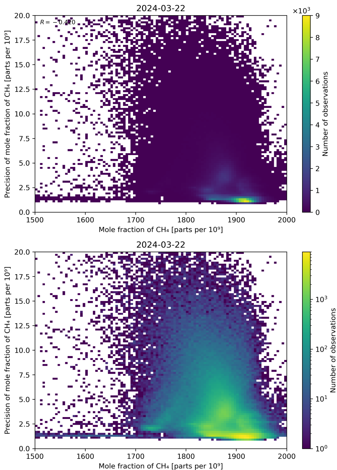
Figure 75: Scatter density plot of “Mole fraction of CH 4 ” against “Precision of mole fraction of CH 4 ” for 2024-03-21 to 2024-03-22.
