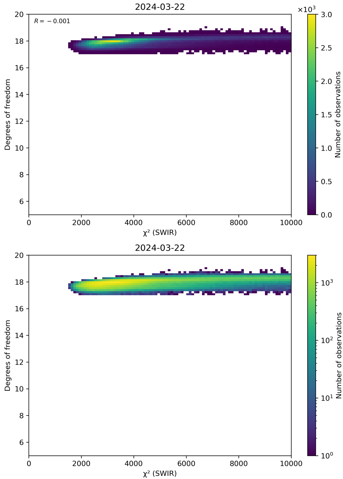
Figure 48: Scatter density plot of “ \chi^2 (SWIR)” against “Degrees of freedom” for 2024-03-21 to 2024-03-22.
