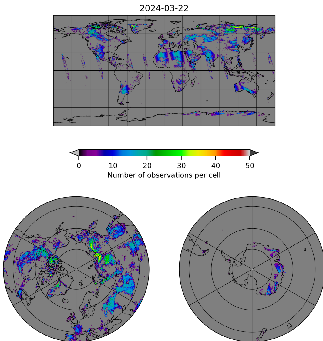
Figure 10: Map of the number of observations for 2024-03-21 to 2024-03-22
