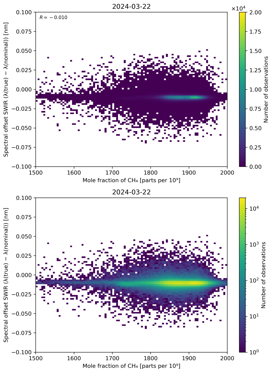
Figure 86: Scatter density plot of “Mole fraction of CH 4 ” against “Spectral offset SWIR ( \lambda(\text{true}) - \lambda(\text{nominal}) )” for 2024-03-21 to 2024-03-22.
