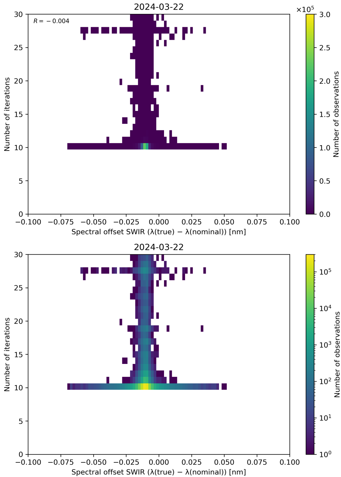
Figure 121: Scatter density plot of “Spectral offset SWIR ( \lambda(\text{true}) - \lambda(\text{nominal}) )” against “Number of iterations” for 2024-03-21 to 2024-03-22.
