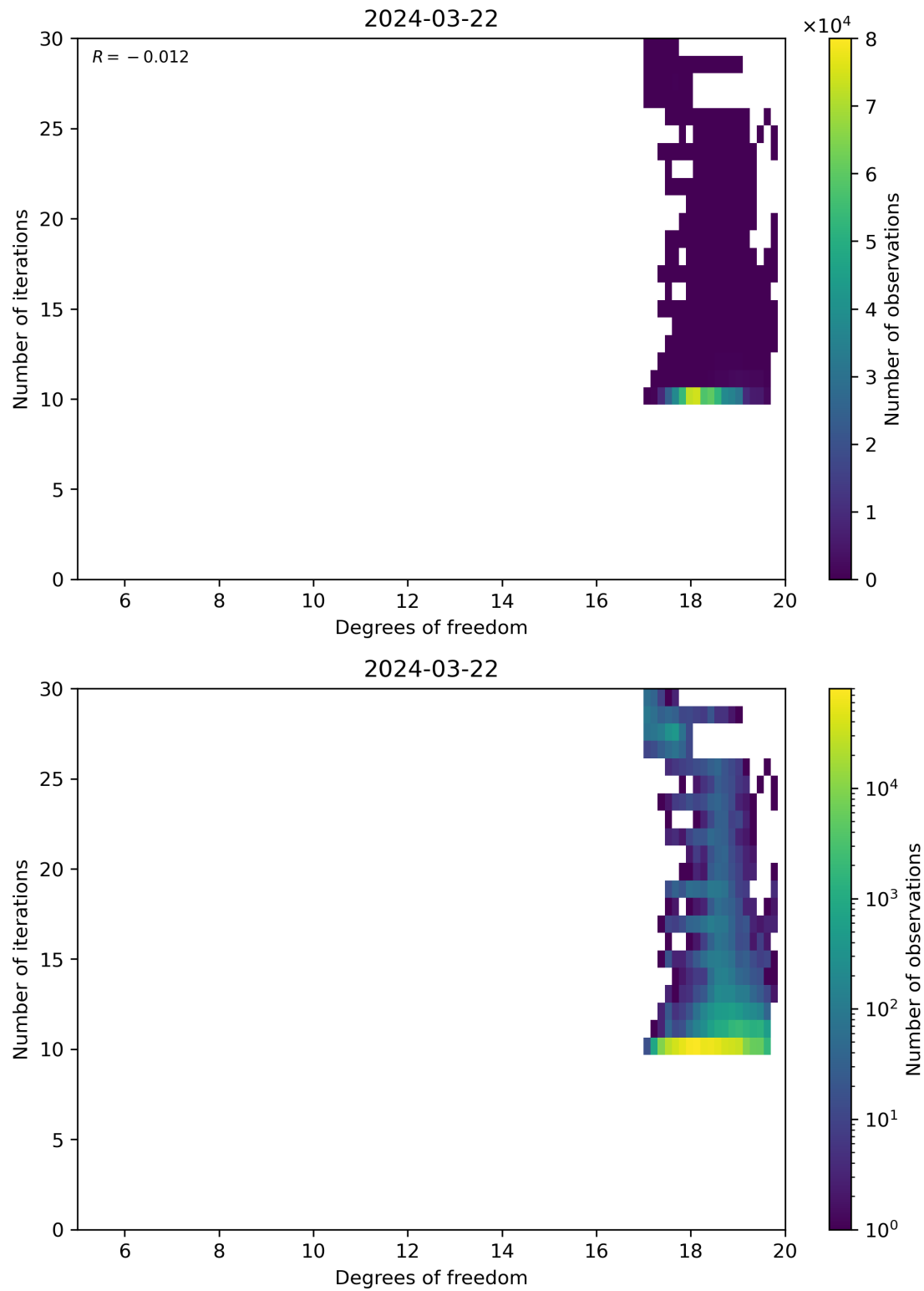
Figure 52: Scatter density plot of “Degrees of freedom” against “Number of iterations” for 2024-03-21 to 2024-03-22.
