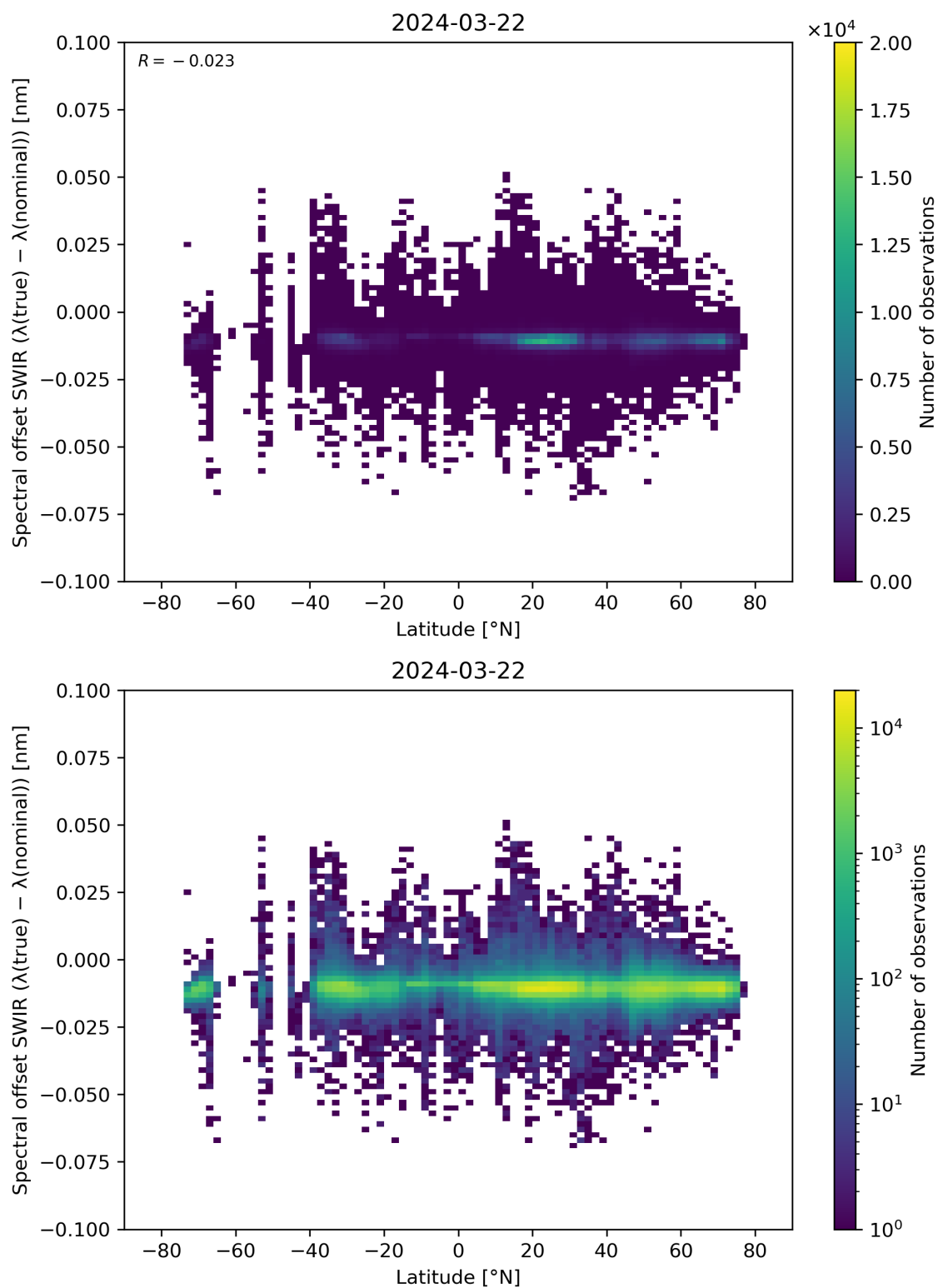
Figure 62: Scatter density plot of “Latitude” against “Spectral offset SWIR ( \lambda(\text{true}) - \lambda(\text{nominal}) )” for 2024-03-21 to 2024-03-22.
