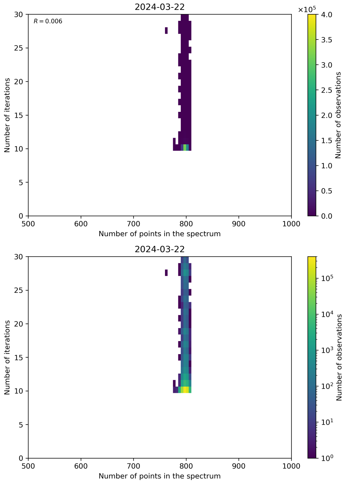
Figure 92: Scatter density plot of “Number of points in the spectrum” against “Number of iterations” for 2024-03-21 to 2024-03-22.
