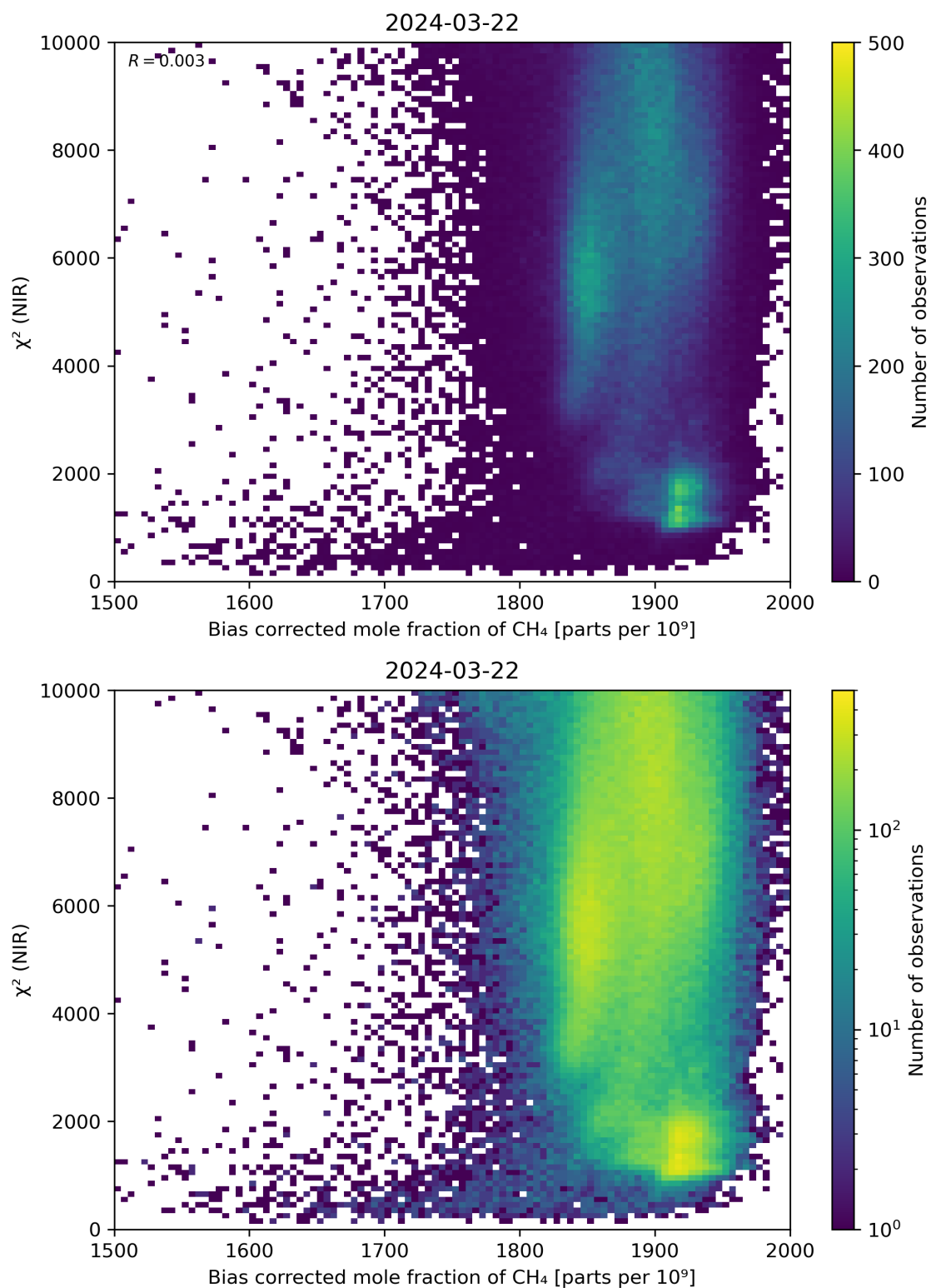
Figure 63: Scatter density plot of “Bias corrected mole fraction of CH 4 ” against “ \chi^2 (NIR)” for 2024-03-21 to 2024-03-22.
