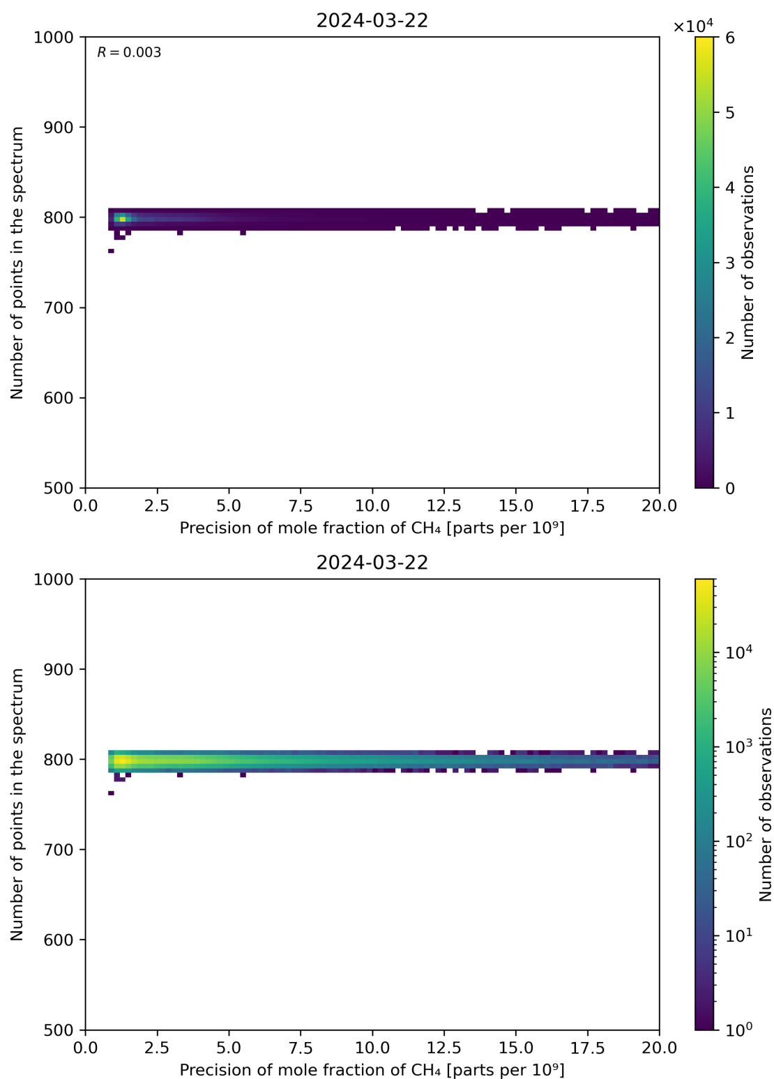
Figure 84: Scatter density plot of “Precision of mole fraction of CH 4 ” against “Number of points in the spectrum” for 2024-03-21 to 2024-03-22.
