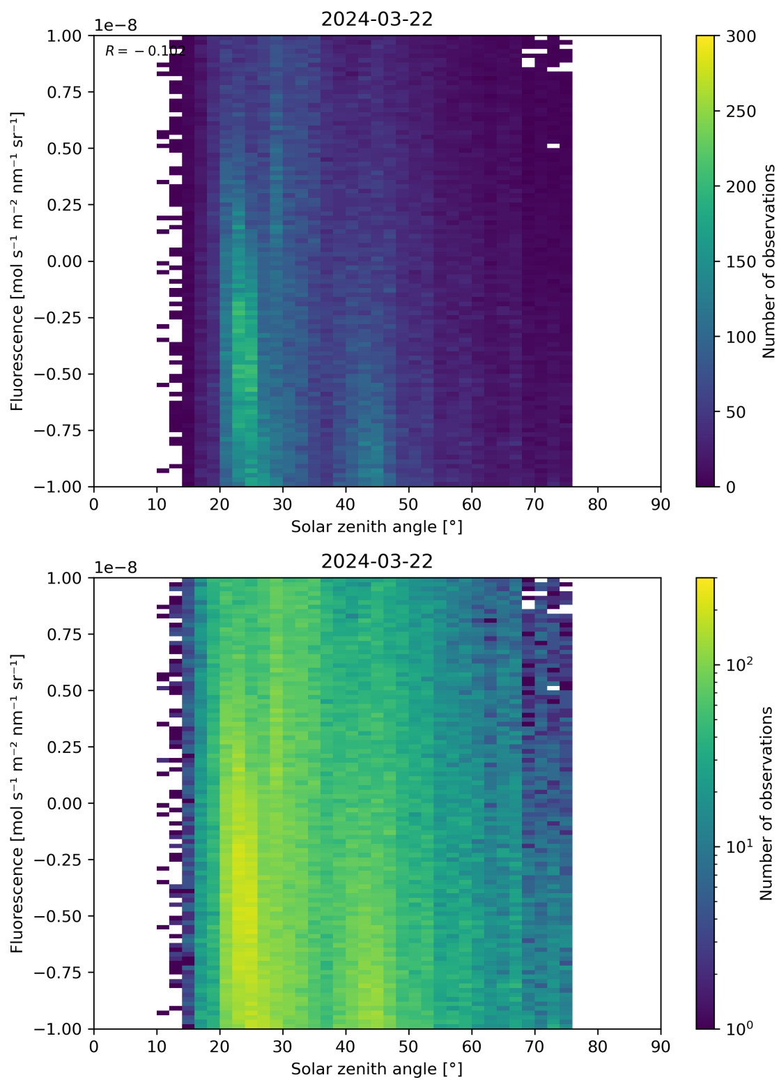
Figure 97: Scatter density plot of “Solar zenith angle” against “Fluorescence” for 2024-03-21 to 2024-03-22.
