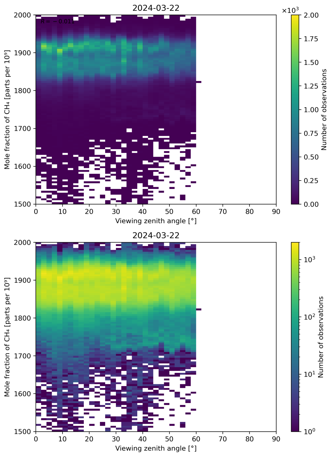
Figure 110: Scatter density plot of “Viewing zenith angle” against “Mole fraction of CH 4 ” for 2024-03-21 to 2024-03-22.
