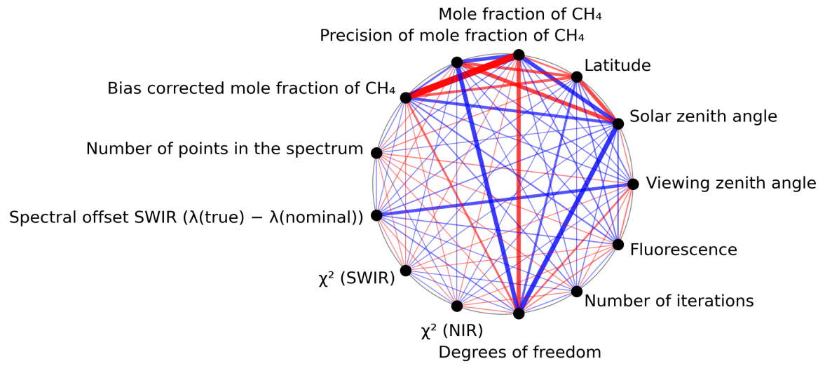
Figure 1: Map of correlation graph for 2024-03-21 to 2024-03-22.
