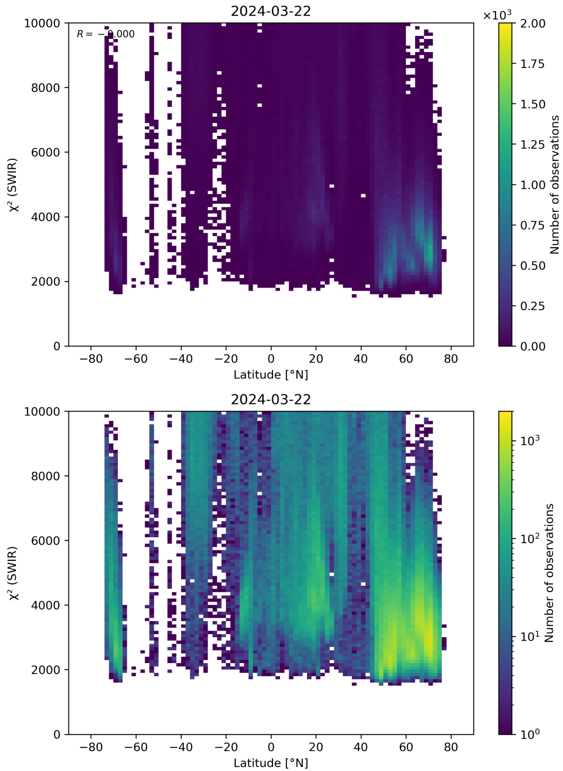
Figure 54: Scatter density plot of “Latitude” against “ \chi^2 (SWIR)” for 2024-03-21 to 2024-03-22.
