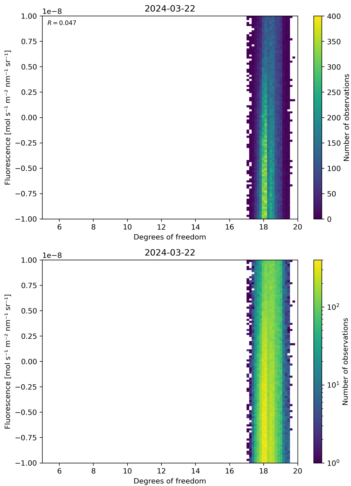
Figure 51: Scatter density plot of “Degrees of freedom” against “Fluorescence” for 2024-03-21 to 2024-03-22.
