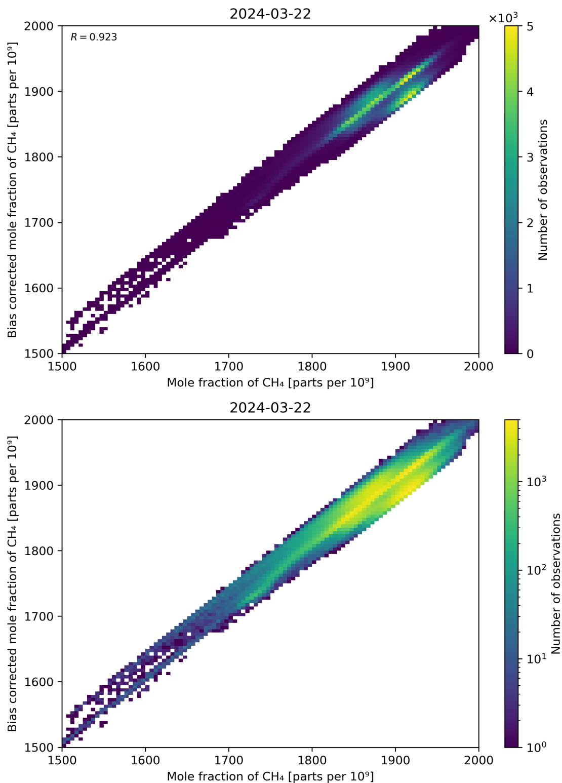
Figure 74: Scatter density plot of “Mole fraction of CH 4 ” against “Bias corrected mole fraction of CH 4 ” for 2024-03-21 to 2024-03-22.
