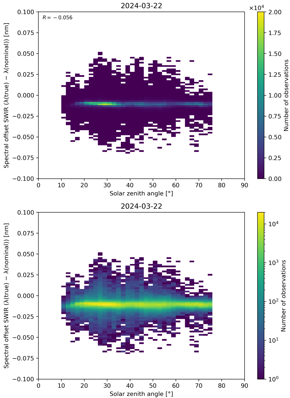
Figure 104: Scatter density plot of “Solar zenith angle” against “Spectral offset SWIR ( \lambda(\text{true}) - \lambda(\text{nominal}) )” for 2024-03-21 to 2024-03-22.
