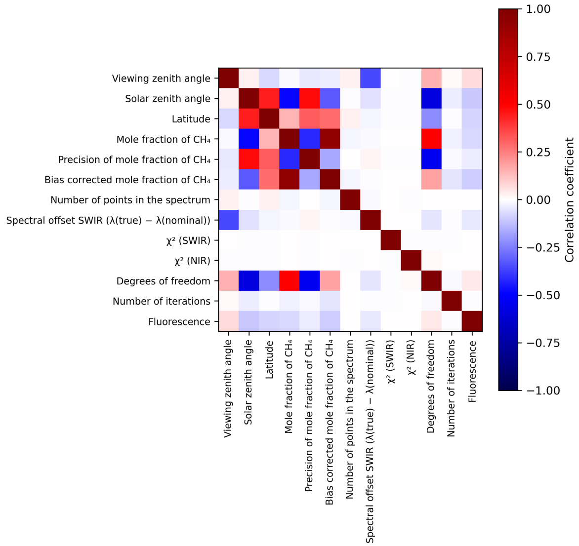
Figure 2: Map of correlation matrix for 2024-03-21 to 2024-03-22.
