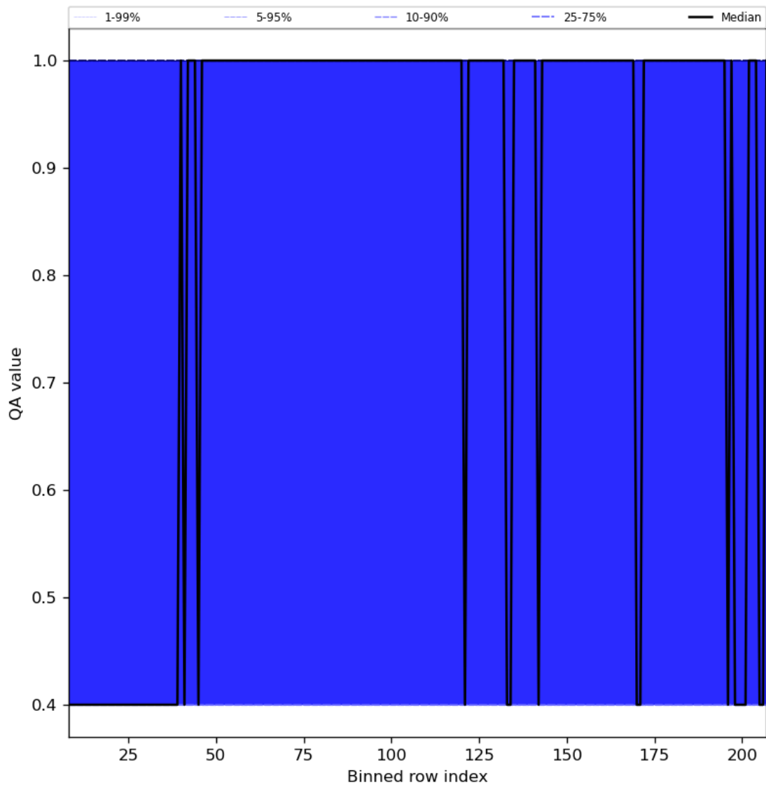
Figure 33: Along track statistics of “QA value” for 2024-03-21 to 2024-03-22
