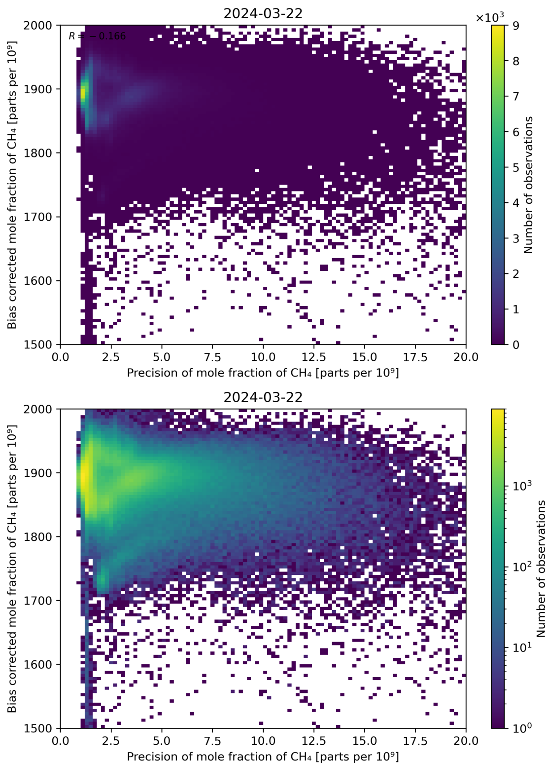
Figure 82: Scatter density plot of “Precision of mole fraction of CH 4 ” against “Bias corrected mole fraction of CH 4 ” for 2024-03-21 to 2024-03-22.
