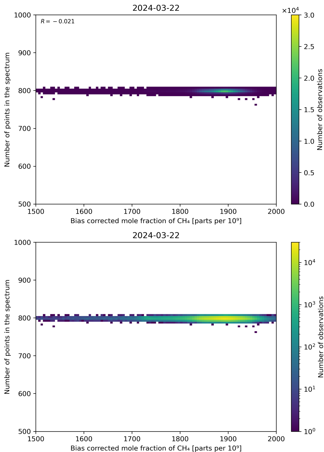
Figure 68: Scatter density plot of “Bias corrected mole fraction of CH 4 ” against “Number of points in the spectrum” for 2024-03-21 to 2024-03-22.
