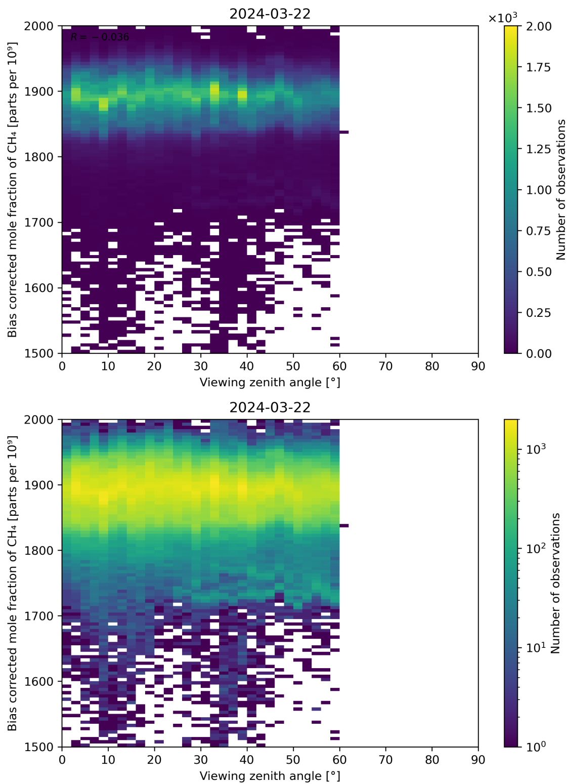
Figure 111: Scatter density plot of “Viewing zenith angle” against “Bias corrected mole fraction of CH 4 ” for 2024-03-21 to 2024-03-22.
