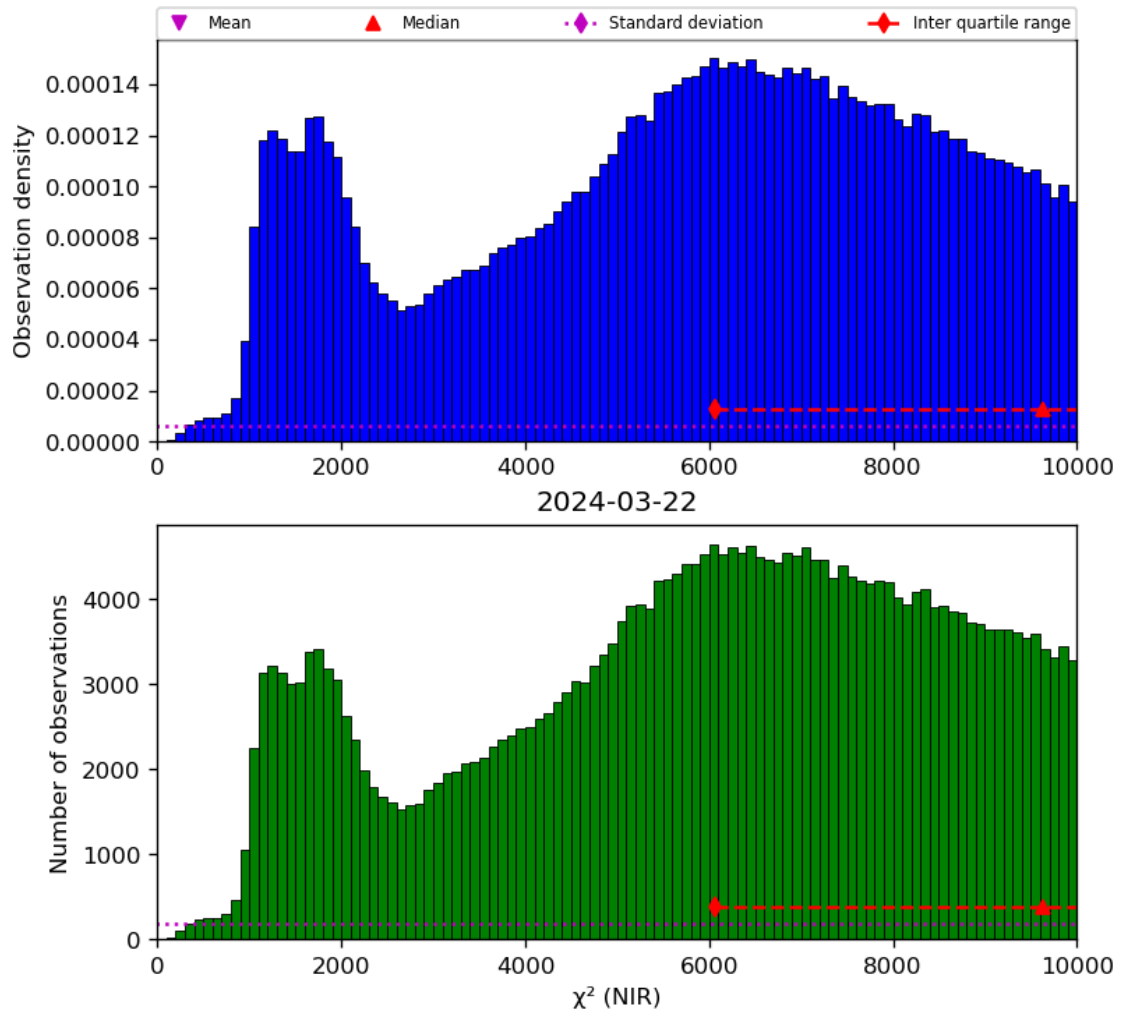
Figure 29: Histogram of “ \chi^2 (NIR)” for 2024-03-21 to 2024-03-22
