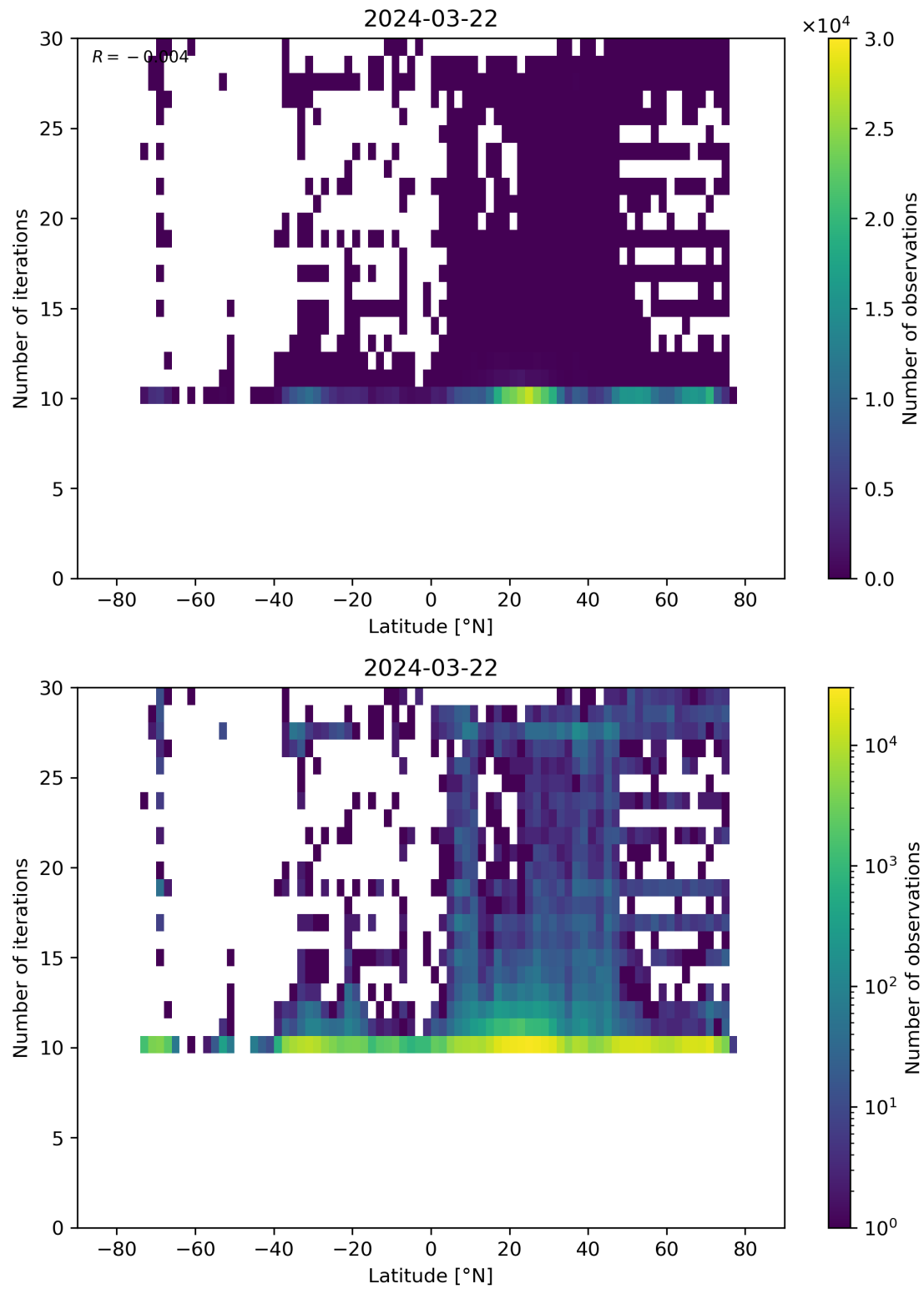
Figure 60: Scatter density plot of “Latitude” against “Number of iterations” for 2024-03-21 to 2024-03-22.
