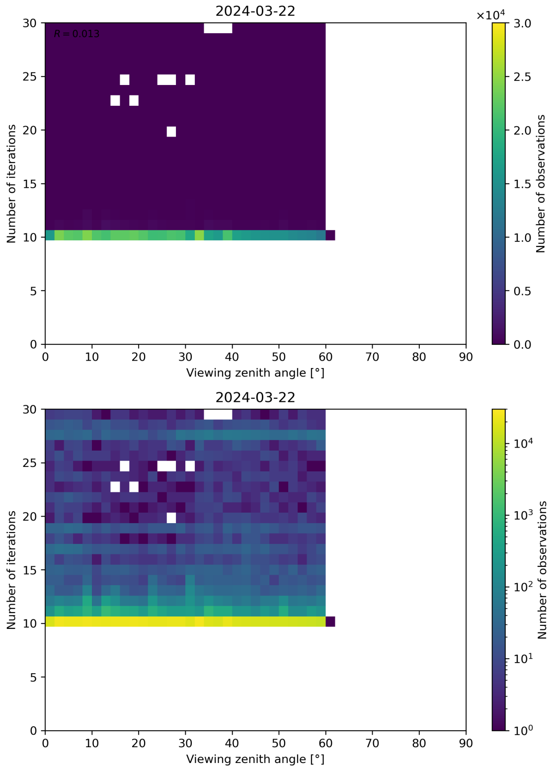
Figure 113: Scatter density plot of “Viewing zenith angle” against “Number of iterations” for 2024-03-21 to 2024-03-22.
