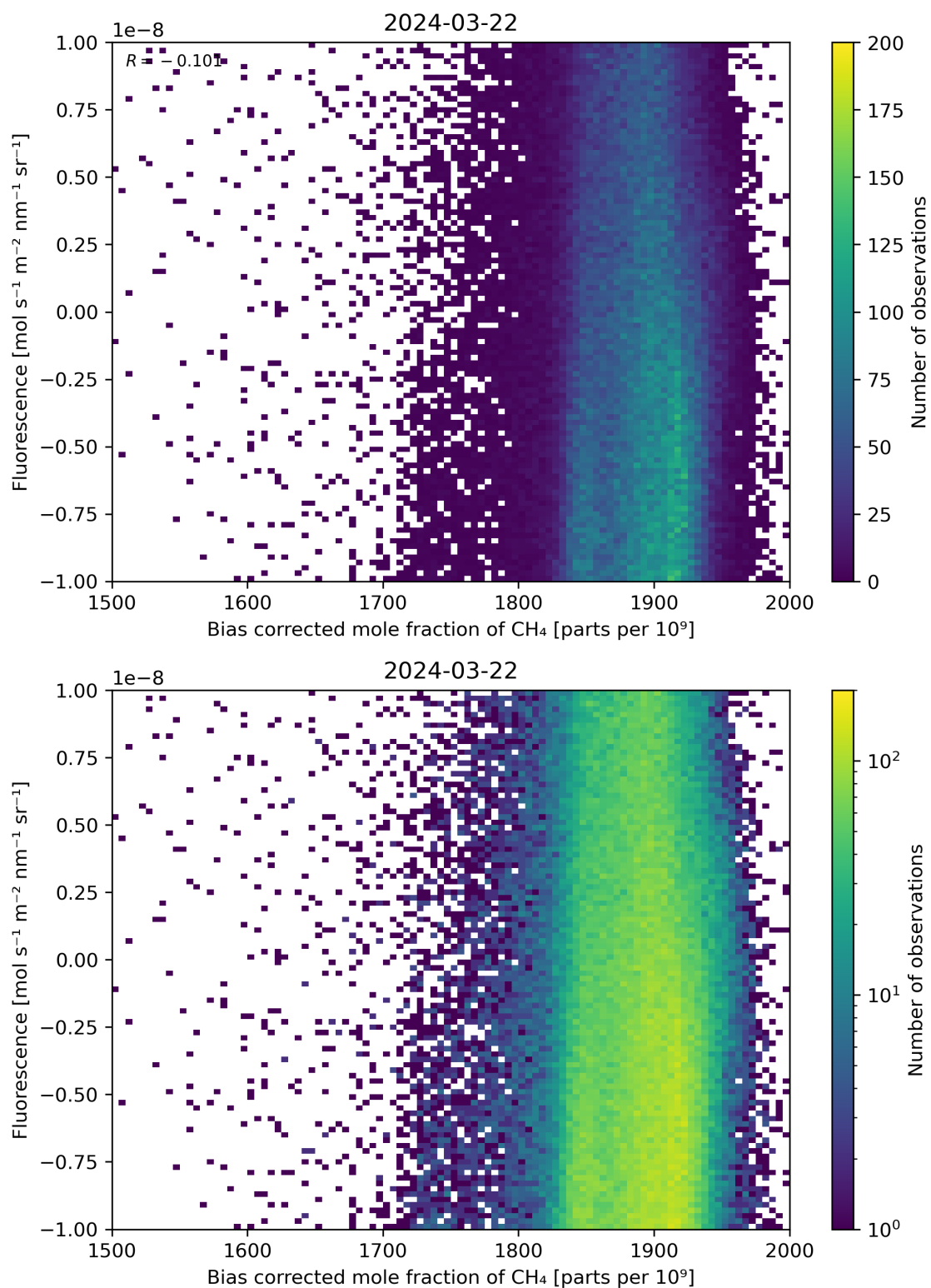
Figure 66: Scatter density plot of “Bias corrected mole fraction of \text{CH}_4 ” against “Fluorescence” for 2024-03-21 to 2024-03-22.
