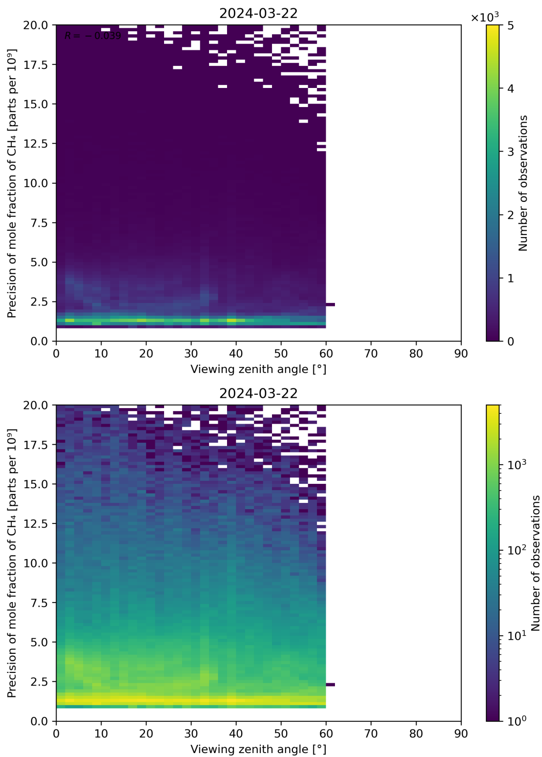
Figure 112: Scatter density plot of “Viewing zenith angle” against “Precision of mole fraction of \text{CH}_4 ” for 2024-03-21 to 2024-03-22.
