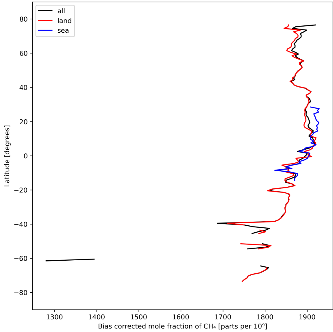
Figure 14: Zonal average of “Bias corrected mole fraction of CH 4 ” for 2024-03-21 to 2024-03-22.
