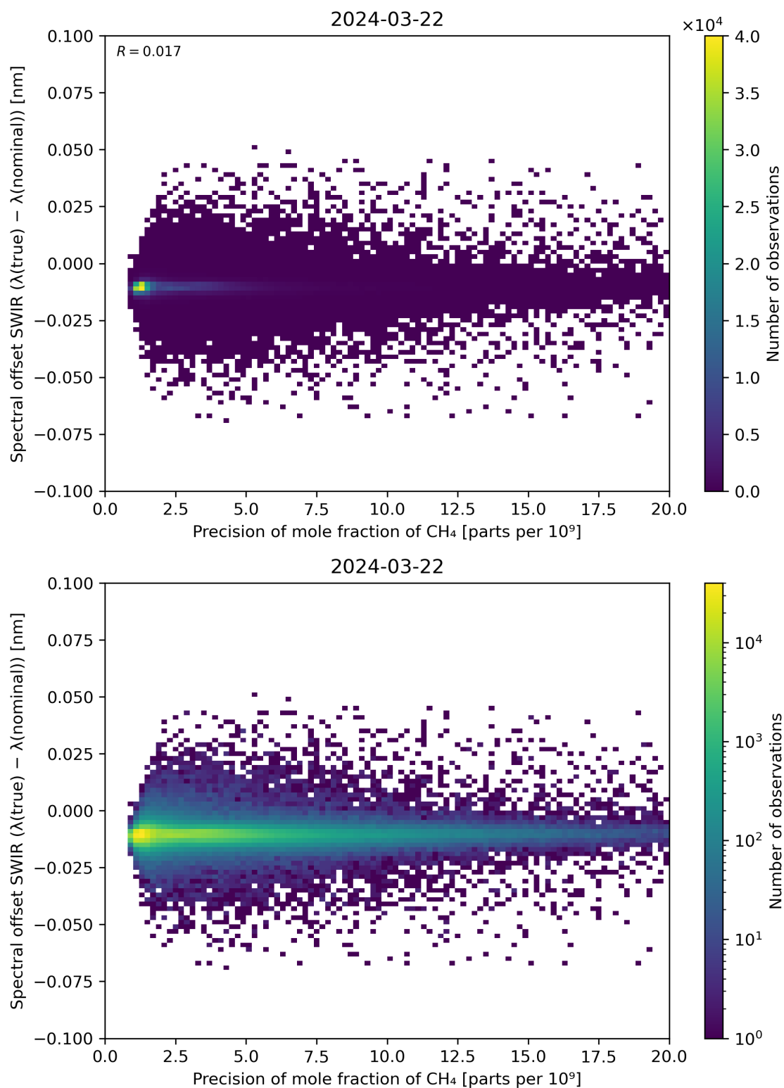
Figure 85: Scatter density plot of “Precision of mole fraction of \text{CH}_4 ” against “Spectral offset SWIR ( \lambda(\text{true}) - \lambda(\text{nominal}) )” for 2024-03-21 to 2024-03-22.
