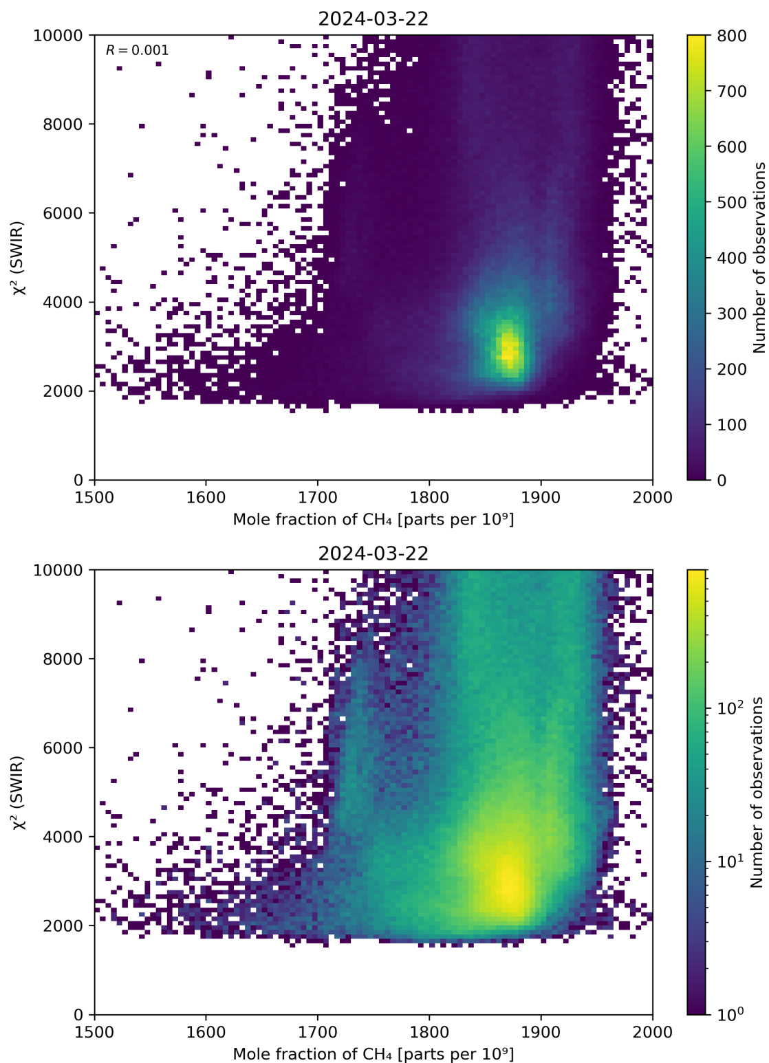
Figure 71: Scatter density plot of “Mole fraction of \text{CH}_4 ” against “ \chi^2 (SWIR)” for 2024-03-21 to 2024-03-22.
