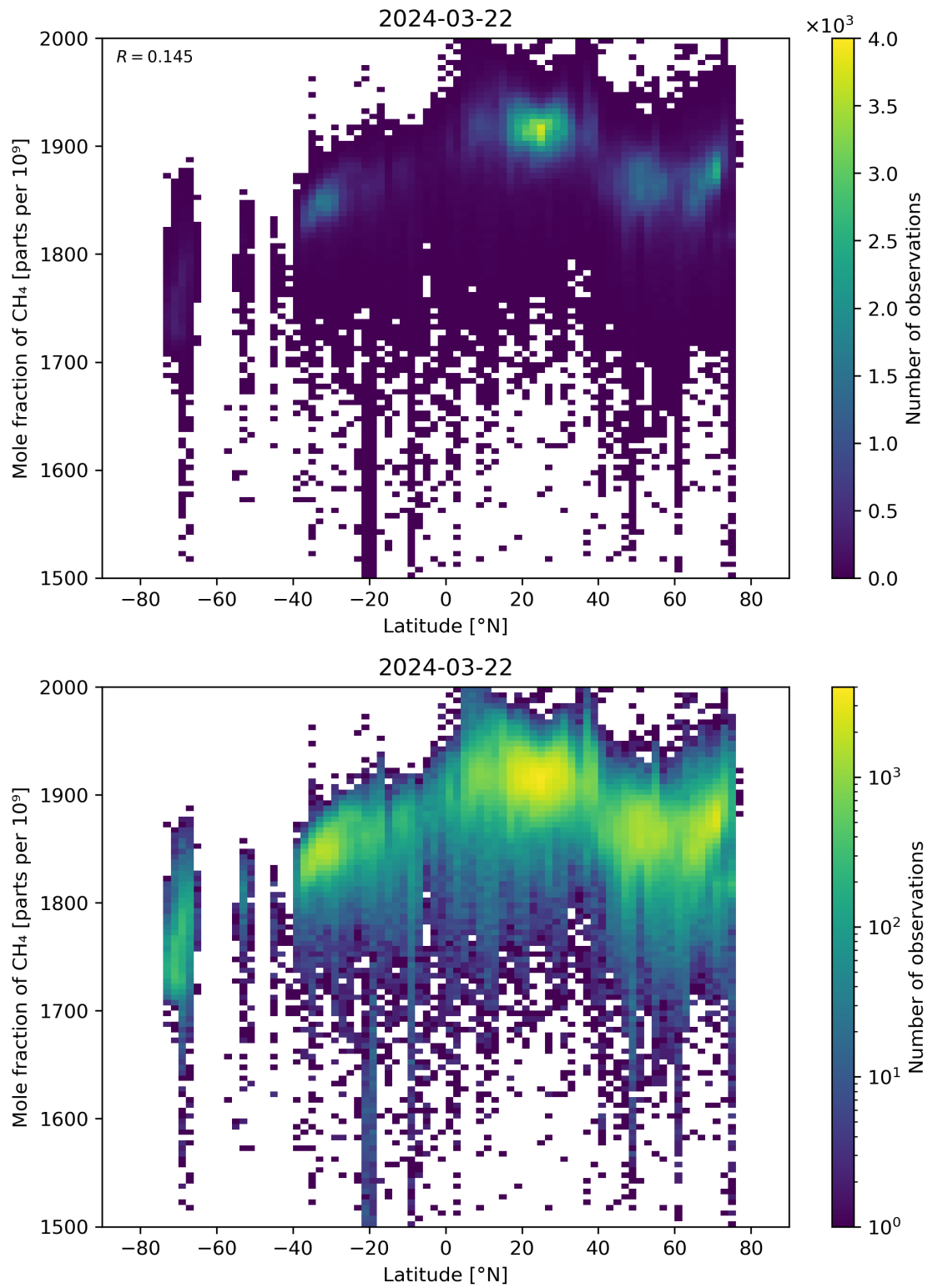
Figure 57: Scatter density plot of “Latitude” against “Mole fraction of CH 4 ” for 2024-03-21 to 2024-03-22.
