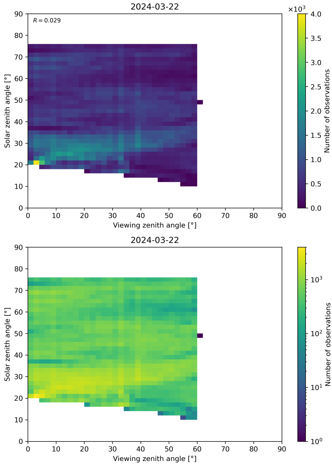
Figure 115: Scatter density plot of “Viewing zenith angle” against “Solar zenith angle” for 2024-03-21 to 2024-03-22.
