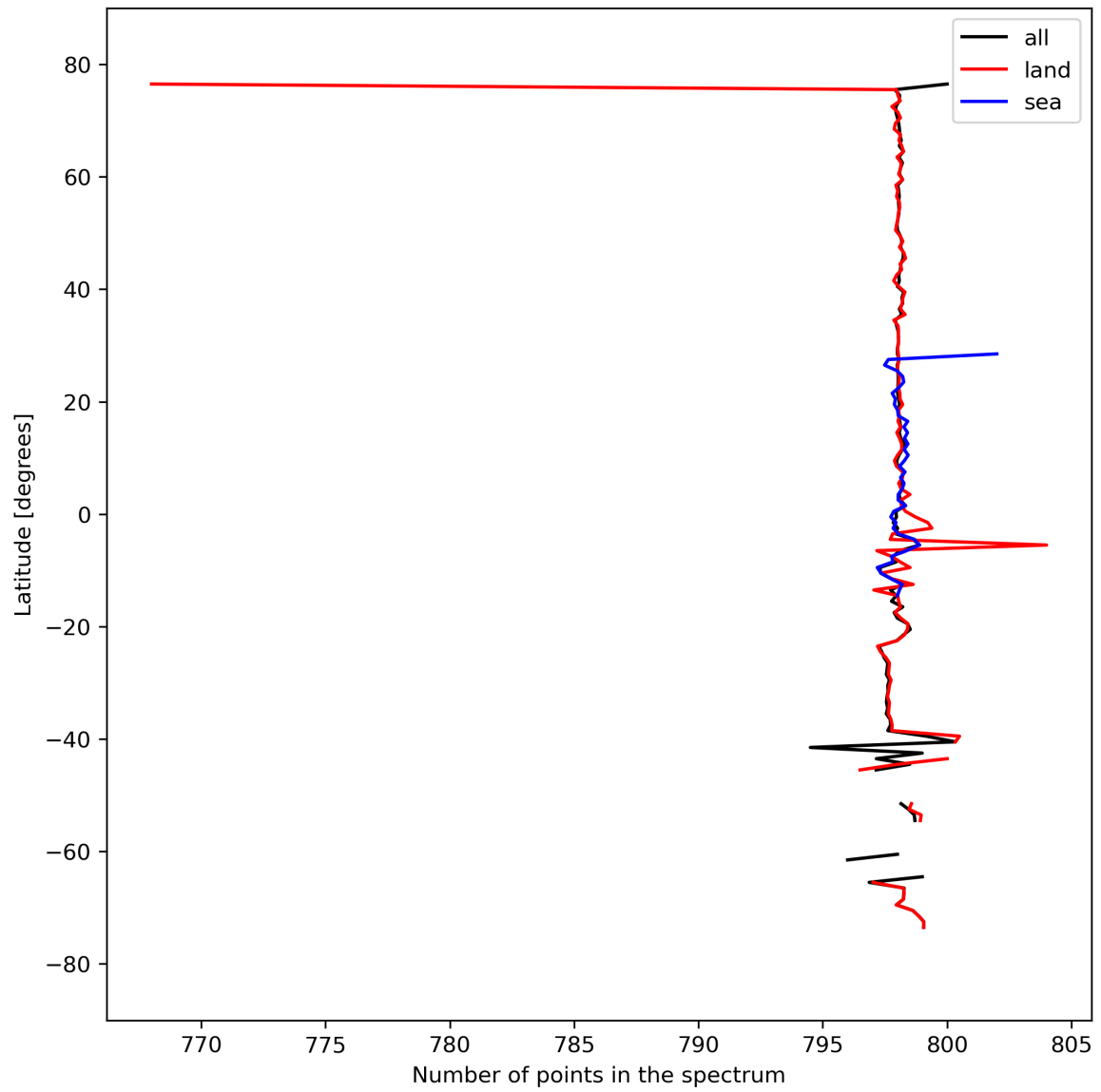
Figure 15: Zonal average of “Number of points in the spectrum” for 2024-03-21 to 2024-03-22.
