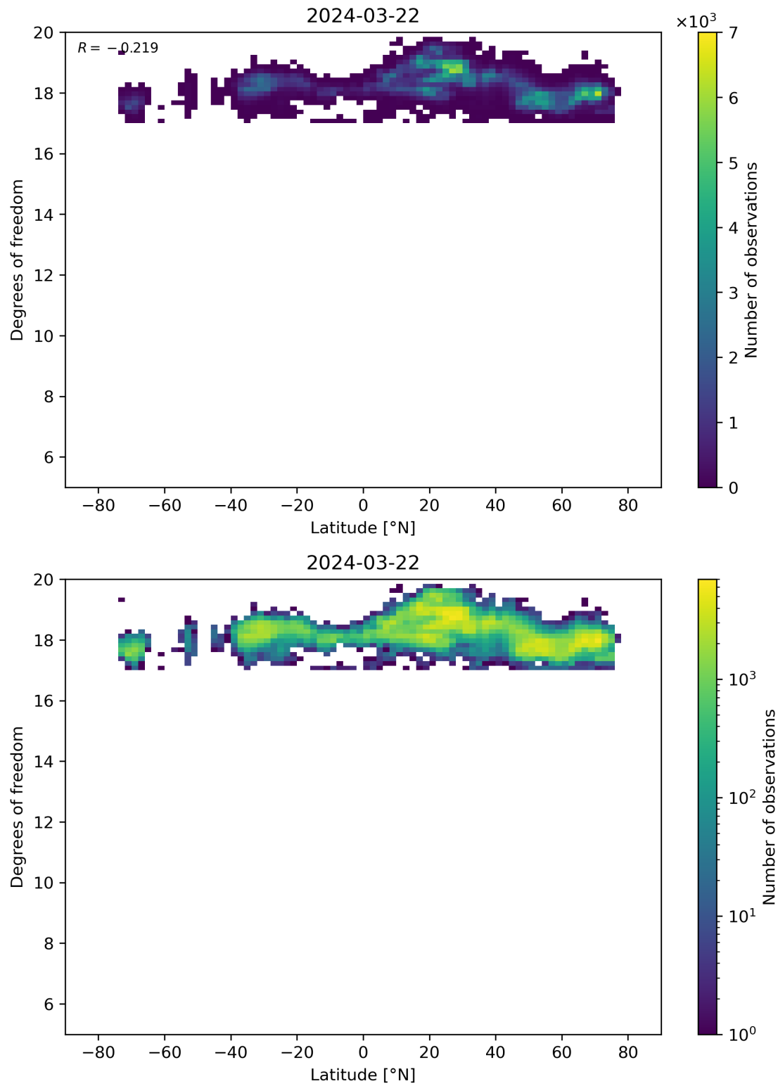
Figure 55: Scatter density plot of “Latitude” against “Degrees of freedom” for 2024-03-21 to 2024-03-22.
