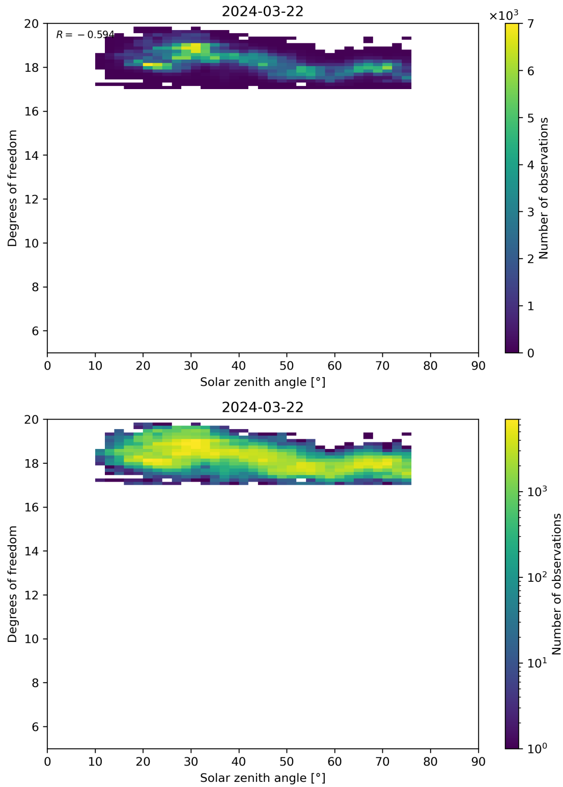
Figure 96: Scatter density plot of “Solar zenith angle” against “Degrees of freedom” for 2024-03-21 to 2024-03-22.
