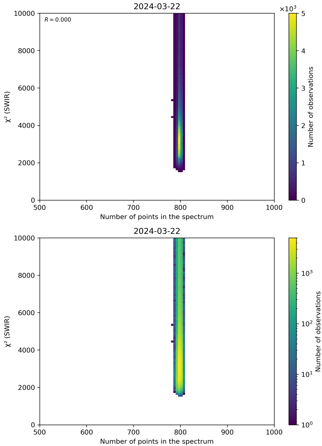
Figure 89: Scatter density plot of “Number of points in the spectrum” against “ \chi^2 (SWIR)” for 2024-03-21 to 2024-03-22.
