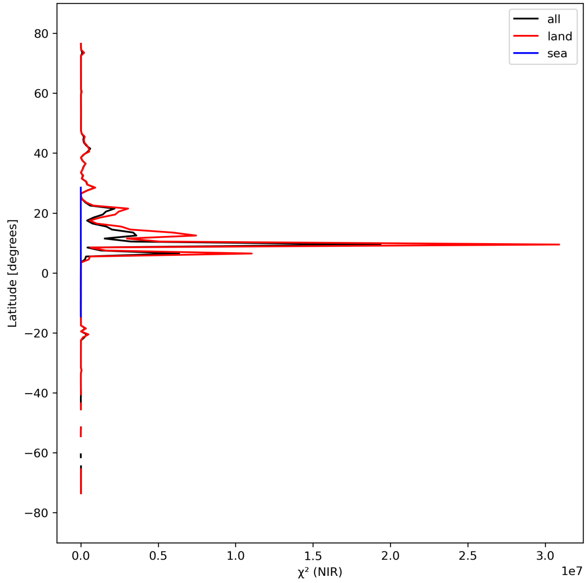
Figure 18: Zonal average of “ \chi^2 (NIR)” for 2024-03-21 to 2024-03-22.
