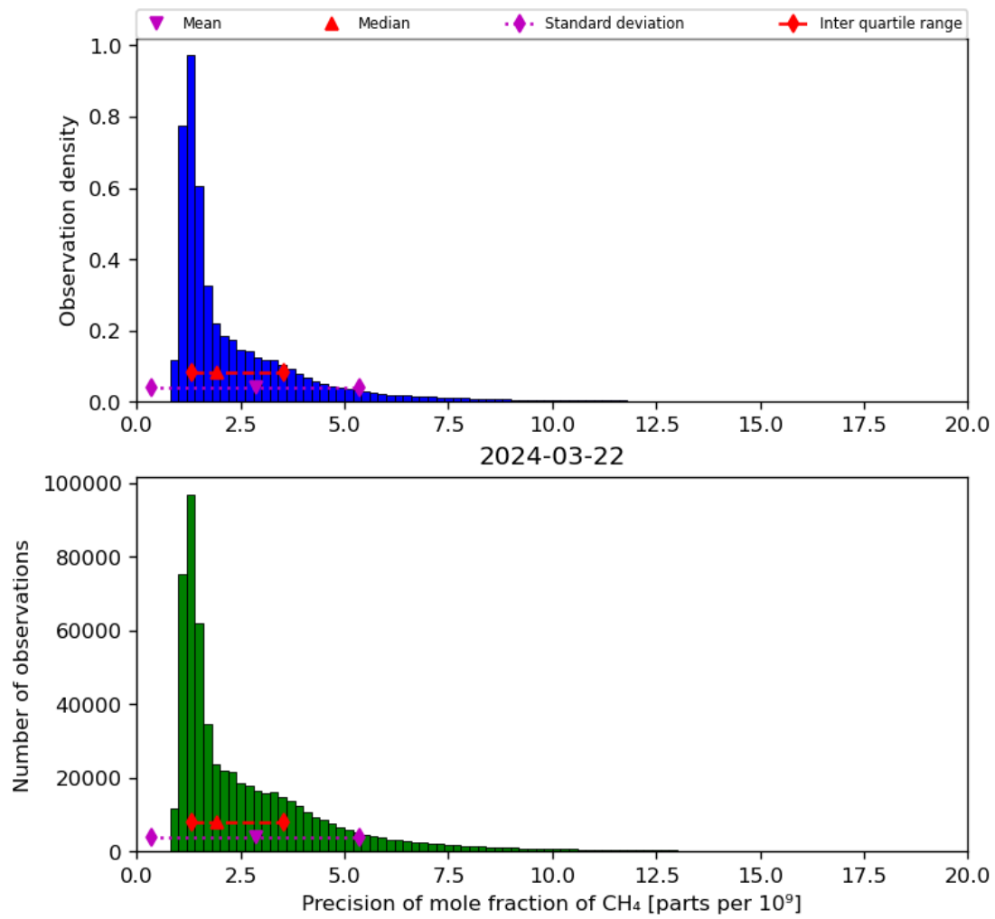
Figure 24: Histogram of “Precision of mole fraction of CH 4 ” for 2024-03-21 to 2024-03-22
