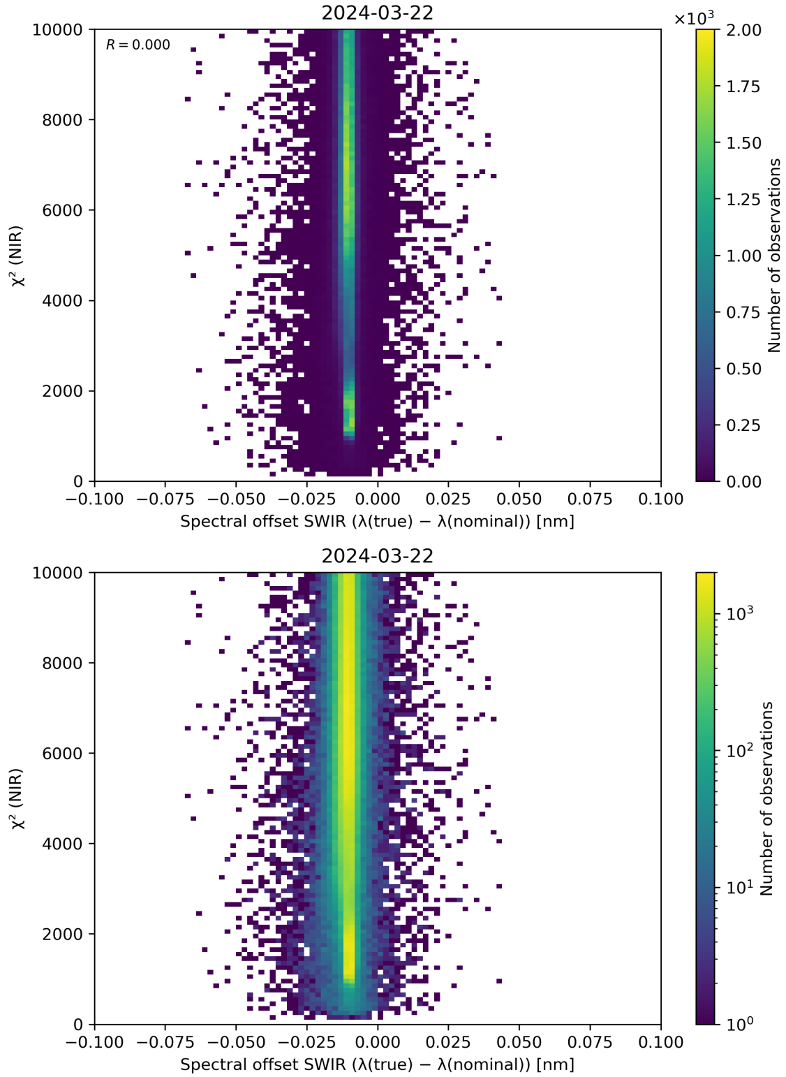
Figure 117: Scatter density plot of “Spectral offset SWIR ( \lambda(\text{true}) - \lambda(\text{nominal}) )” against “ \chi^2 (NIR)” for 2024-03-21 to 2024-03-22.
