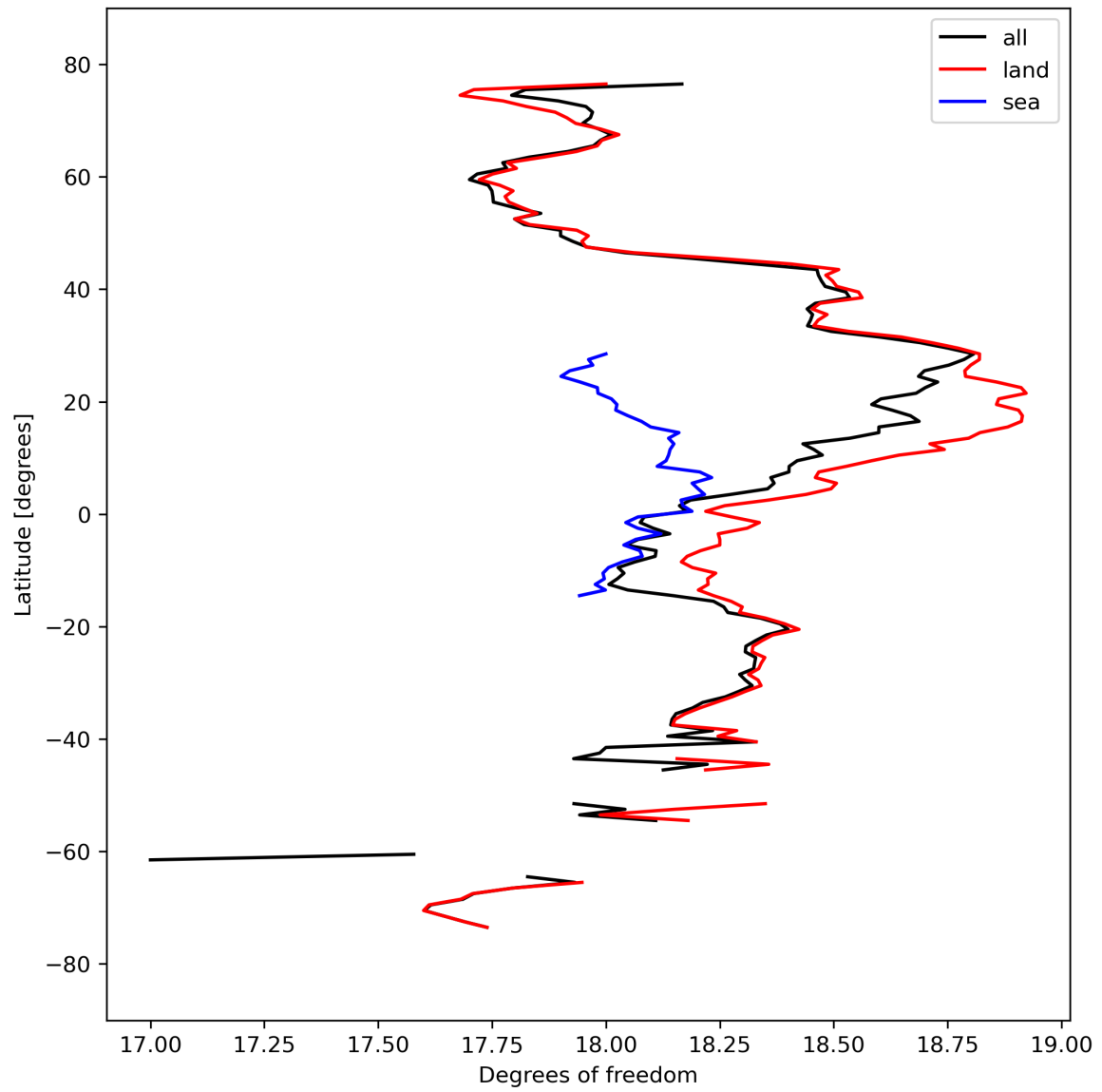
Figure 19: Zonal average of “Degrees of freedom” for 2024-03-21 to 2024-03-22.
