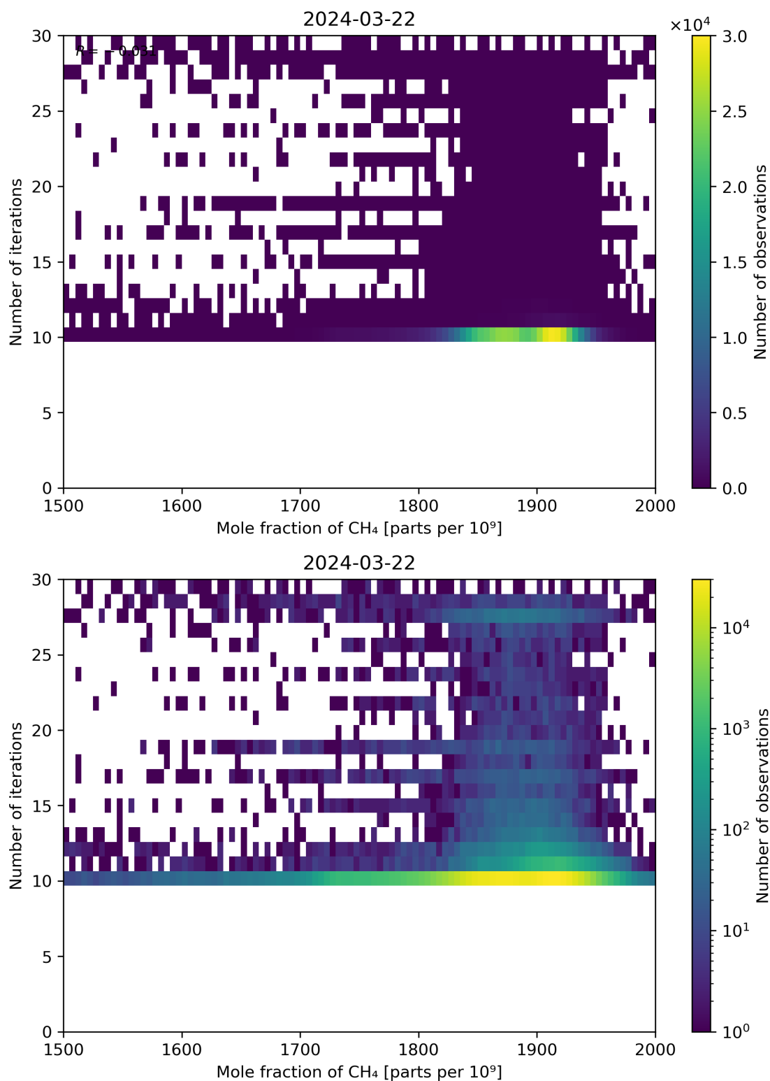
Figure 76: Scatter density plot of “Mole fraction of CH 4 ” against “Number of iterations” for 2024-03-21 to 2024-03-22.
