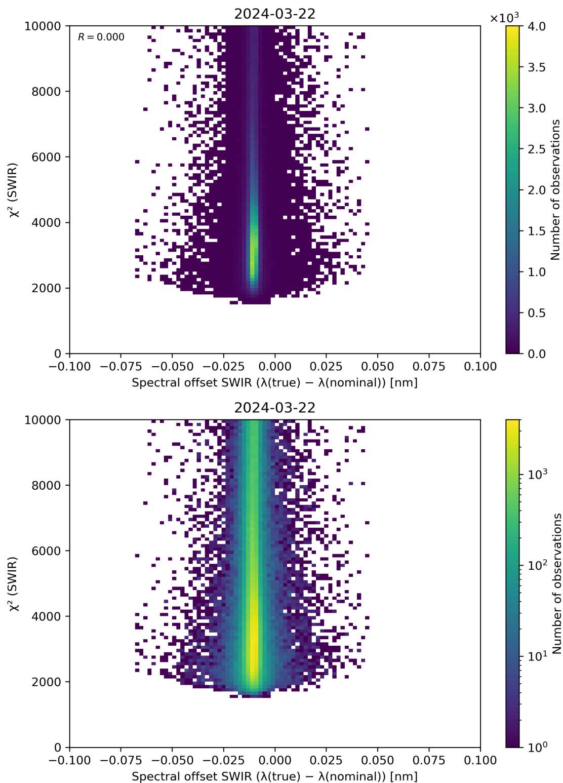
Figure 118: Scatter density plot of “Spectral offset SWIR ( \lambda(\text{true}) - \lambda(\text{nominal}) )” against “ \chi^2 (SWIR)” for 2024-03-21 to 2024-03-22.
