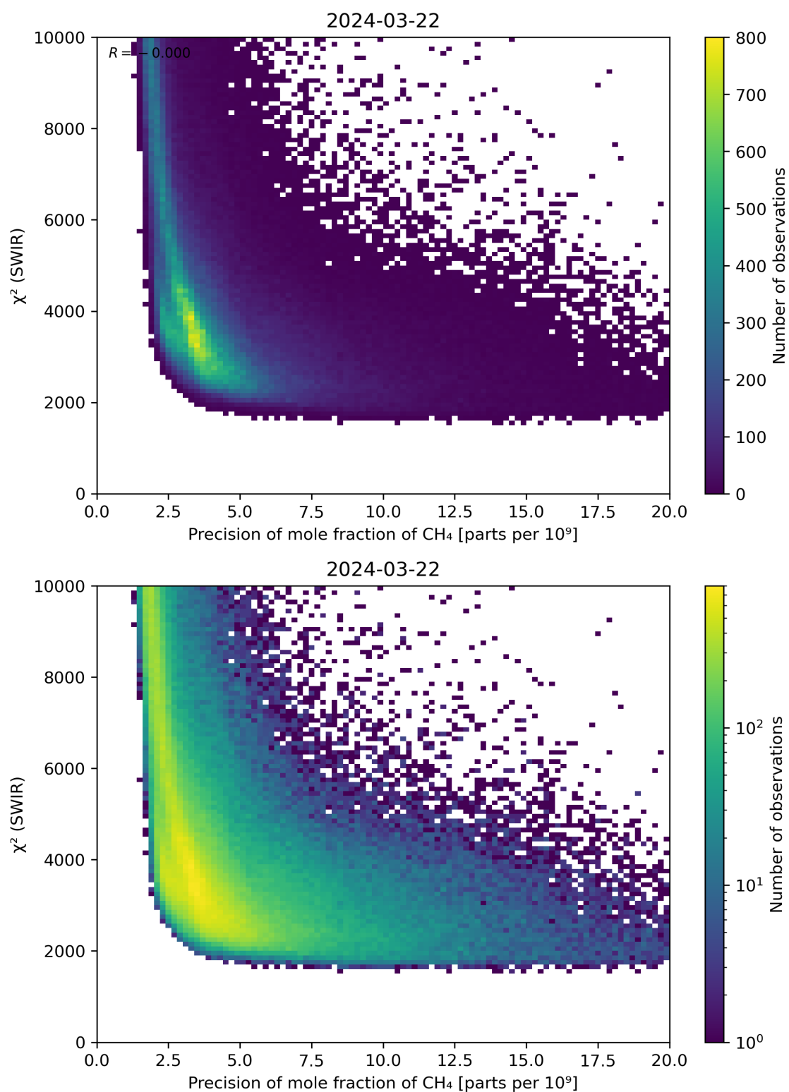
Figure 79: Scatter density plot of “Precision of mole fraction of CH 4 ” against “ \chi^2 (SWIR)” for 2024-03-21 to 2024-03-22.
