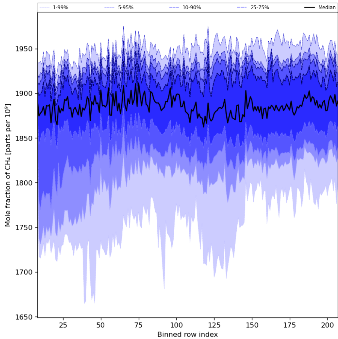
Figure 34: Along track statistics of “Mole fraction of CH 4 ” for 2024-03-21 to 2024-03-22
