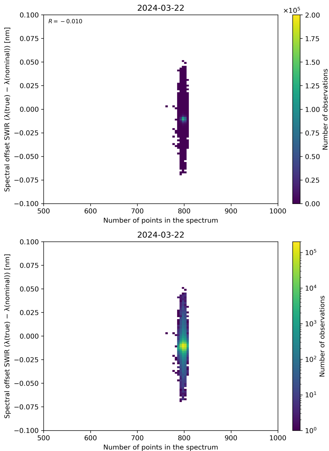
Figure 93: Scatter density plot of “Number of points in the spectrum” against “Spectral offset SWIR ( \lambda(\text{true}) - \lambda(\text{nominal}) )” for 2024-03-21 to 2024-03-22.
