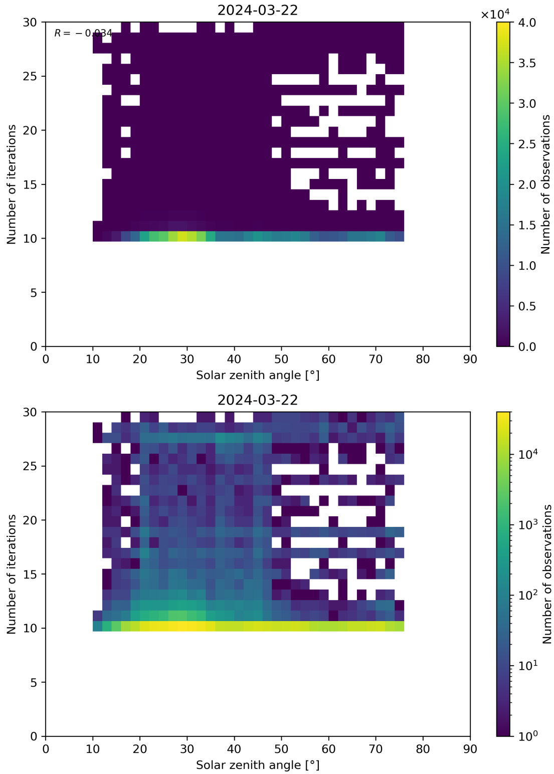
Figure 102: Scatter density plot of “Solar zenith angle” against “Number of iterations” for 2024-03-21 to 2024-03-22.
