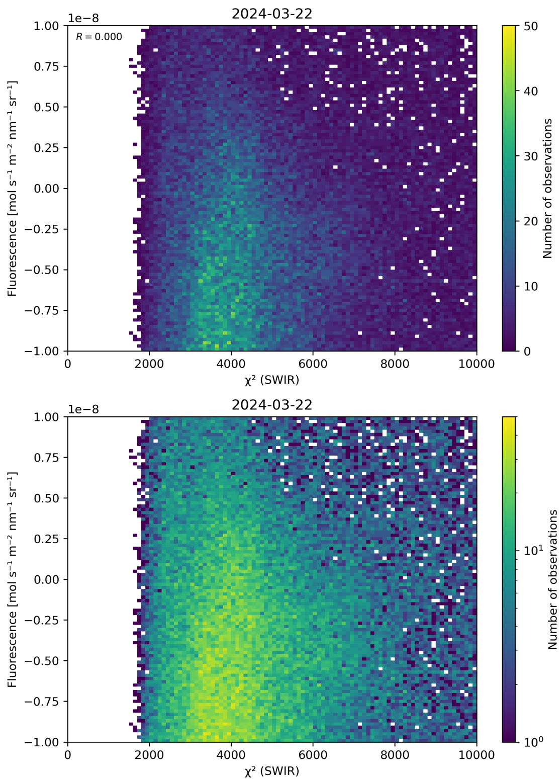
Figure 49: Scatter density plot of “ \chi^2 (SWIR)” against “Fluorescence” for 2024-03-21 to 2024-03-22.
