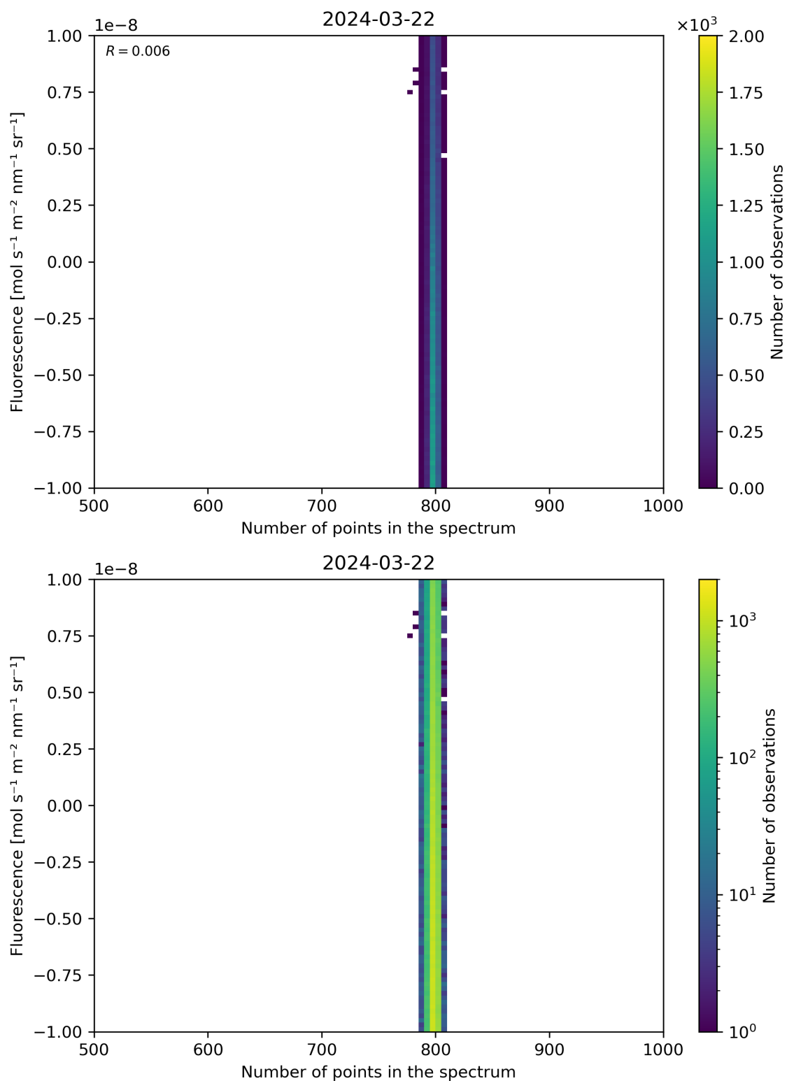
Figure 91: Scatter density plot of “Number of points in the spectrum” against “Fluorescence” for 2024-03-21 to 2024-03-22.
