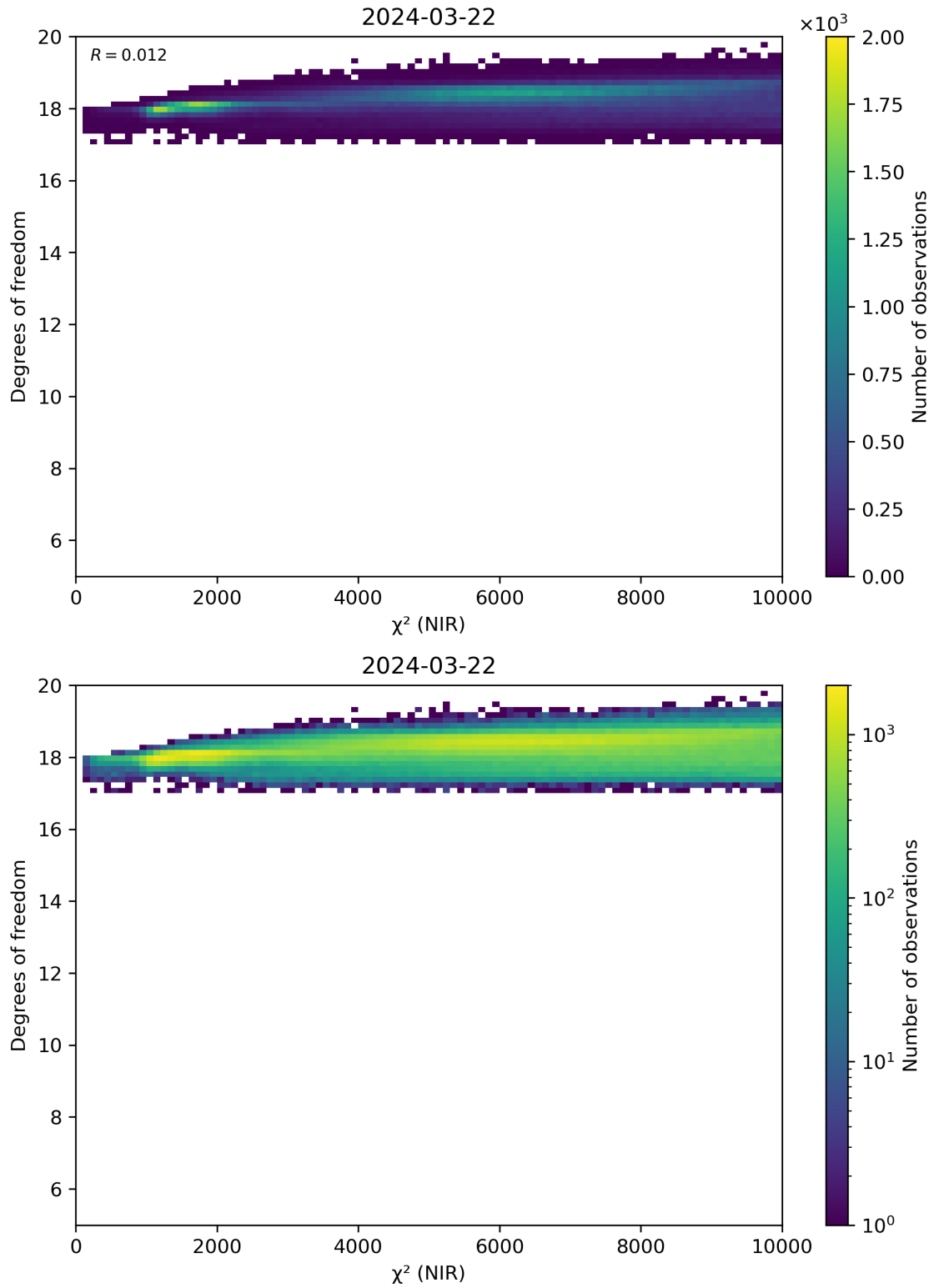
Figure 44: Scatter density plot of “ \chi^2 (NIR)” against “Degrees of freedom” for 2024-03-21 to 2024-03-22.
