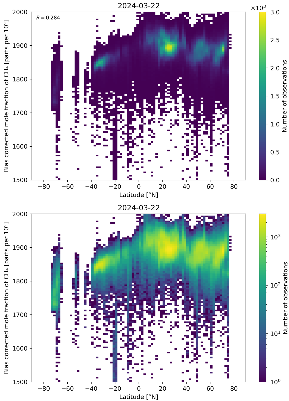
Figure 58: Scatter density plot of “Latitude” against “Bias corrected mole fraction of CH 4 ” for 2024-03-21 to 2024-03-22.
