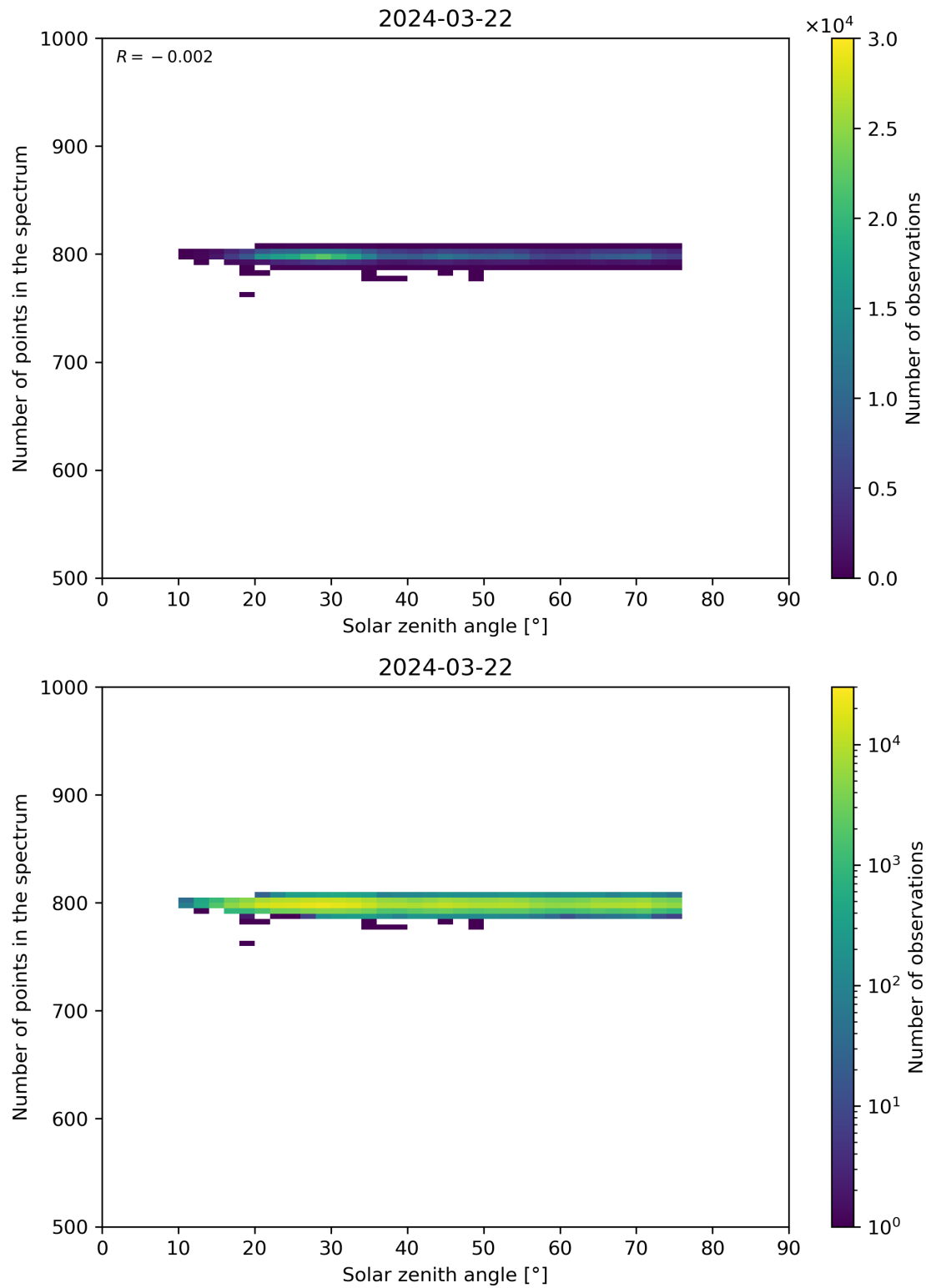
Figure 103: Scatter density plot of “Solar zenith angle” against “Number of points in the spectrum” for 2024-03-21 to 2024-03-22.
