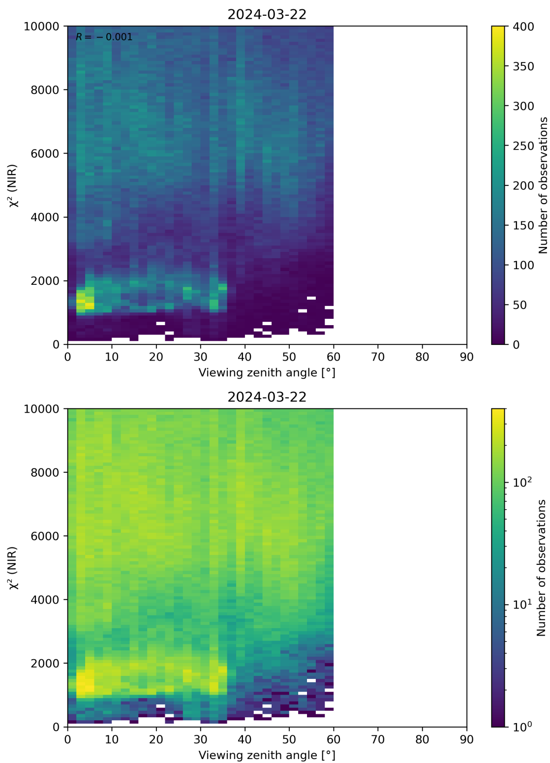
Figure 105: Scatter density plot of “Viewing zenith angle” against “ \chi^2 (NIR)” for 2024-03-21 to 2024-03-22.
