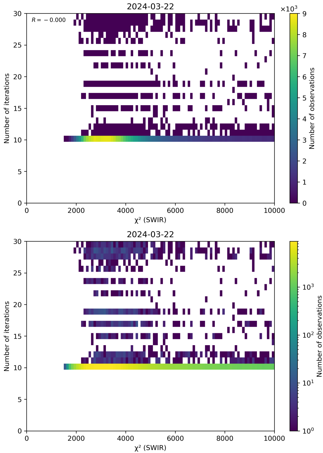
Figure 50: Scatter density plot of “ \chi^2 (SWIR)” against “Number of iterations” for 2024-03-21 to 2024-03-22.
