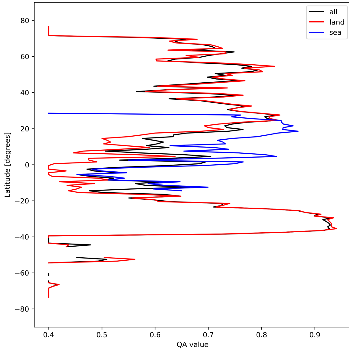
Figure 11: Zonal average of “QA value” for 2024-03-21 to 2024-03-22.
