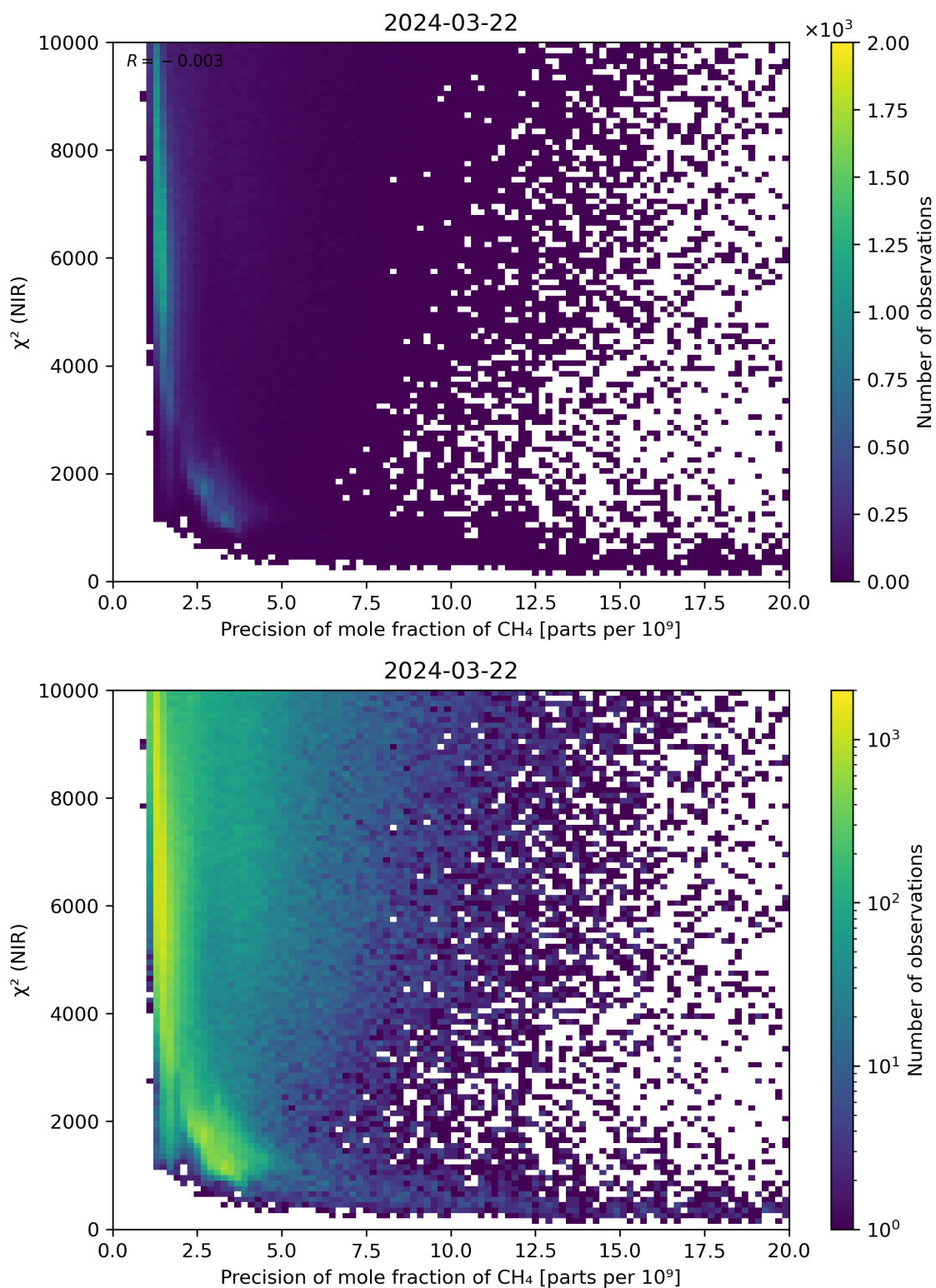
Figure 78: Scatter density plot of “Precision of mole fraction of CH 4 ” against “ \chi^2 (NIR)” for 2024-03-21 to 2024-03-22.
