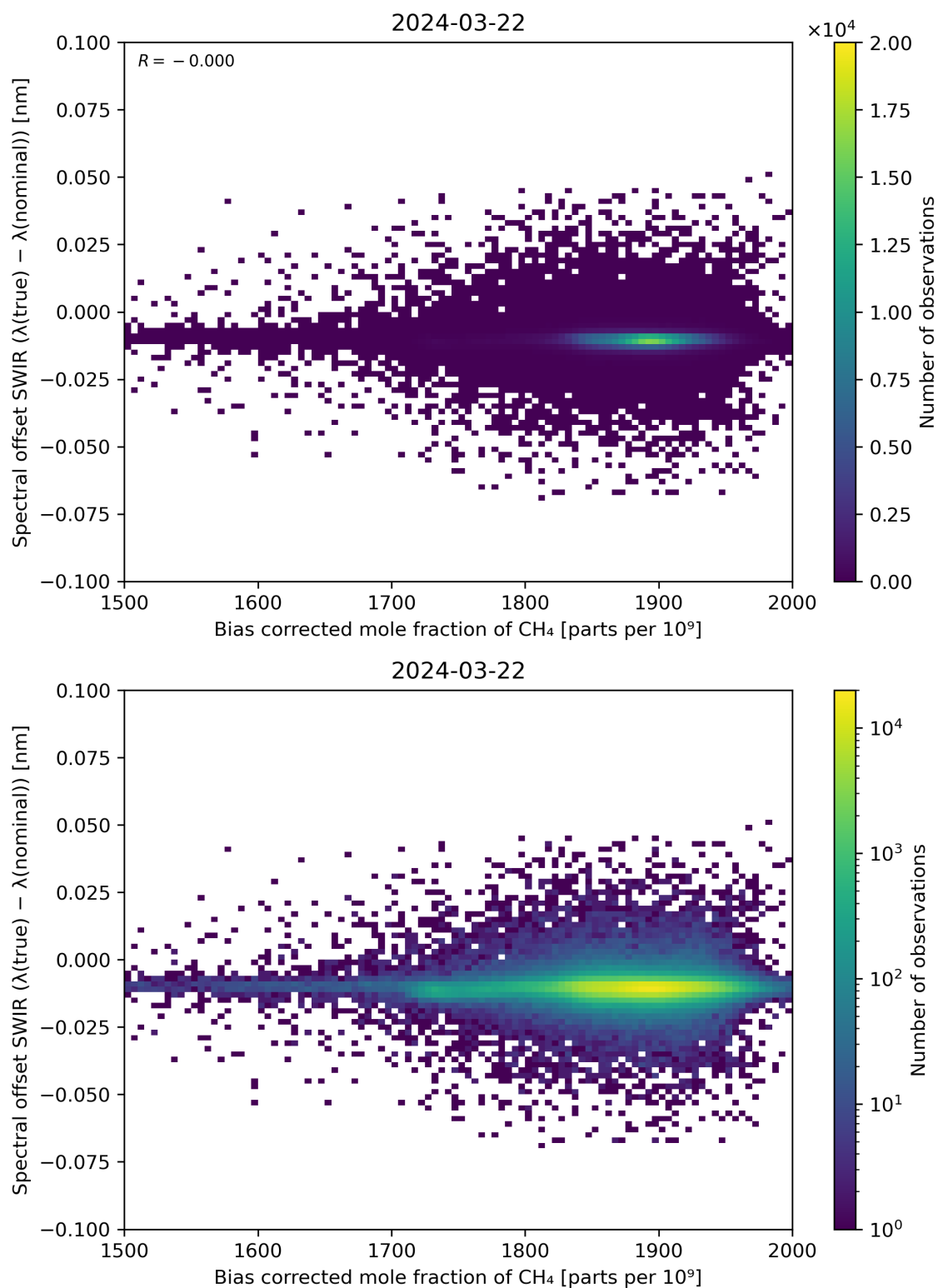
Figure 69: Scatter density plot of “Bias corrected mole fraction of \text{CH}_4 ” against “Spectral offset SWIR ( \lambda(\text{true}) - \lambda(\text{nominal}) )” for 2024-03-21 to 2024-03-22.
