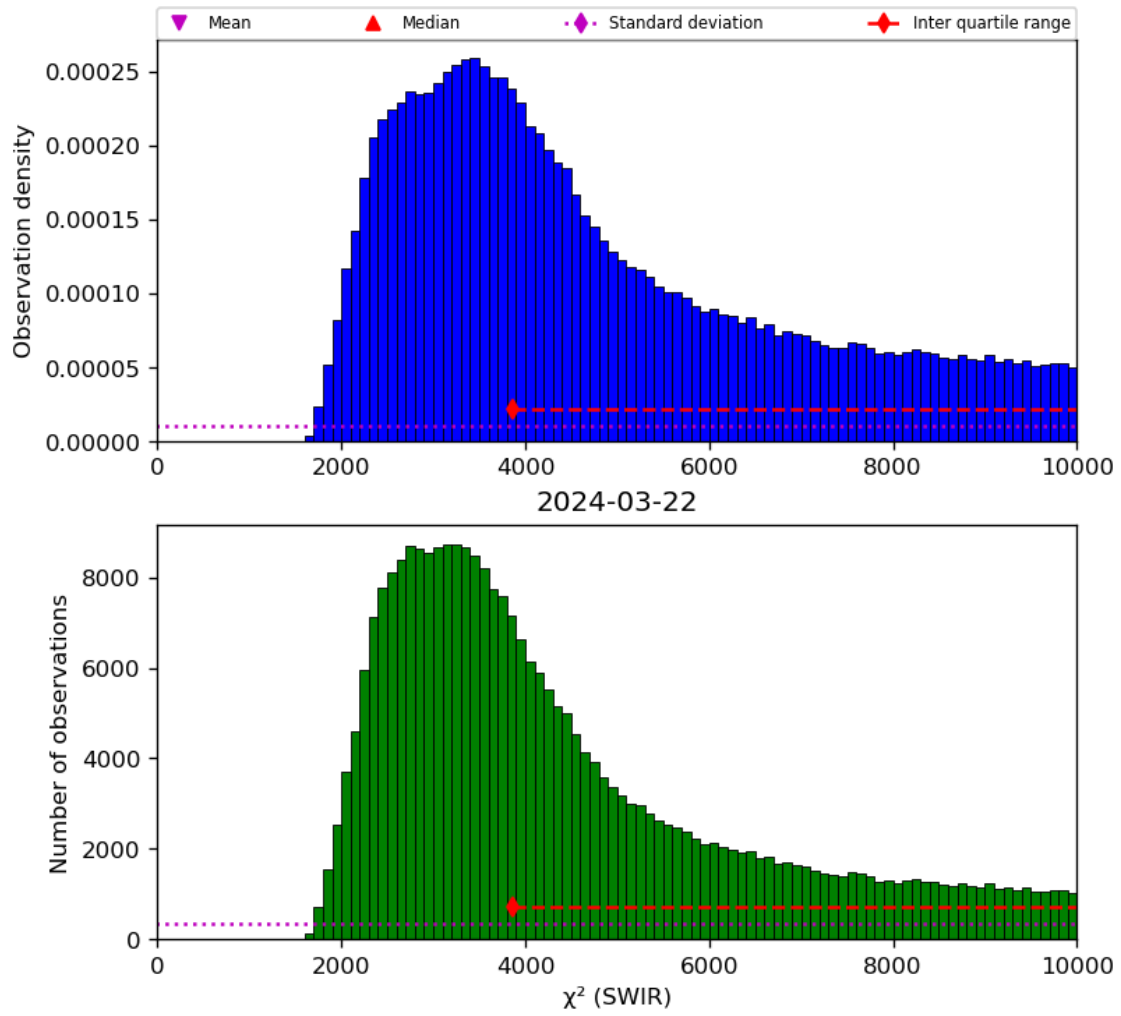
Figure 28: Histogram of " \chi^2 (SWIR)" for 2024-03-21 to 2024-03-22
