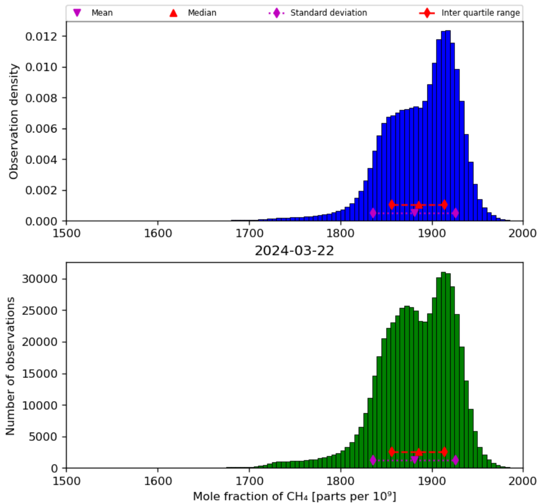
Figure 23: Histogram of “Mole fraction of CH 4 ” for 2024-03-21 to 2024-03-22
