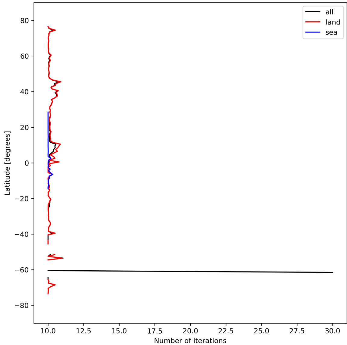
Figure 20: Zonal average of “Number of iterations” for 2024-03-21 to 2024-03-22.
