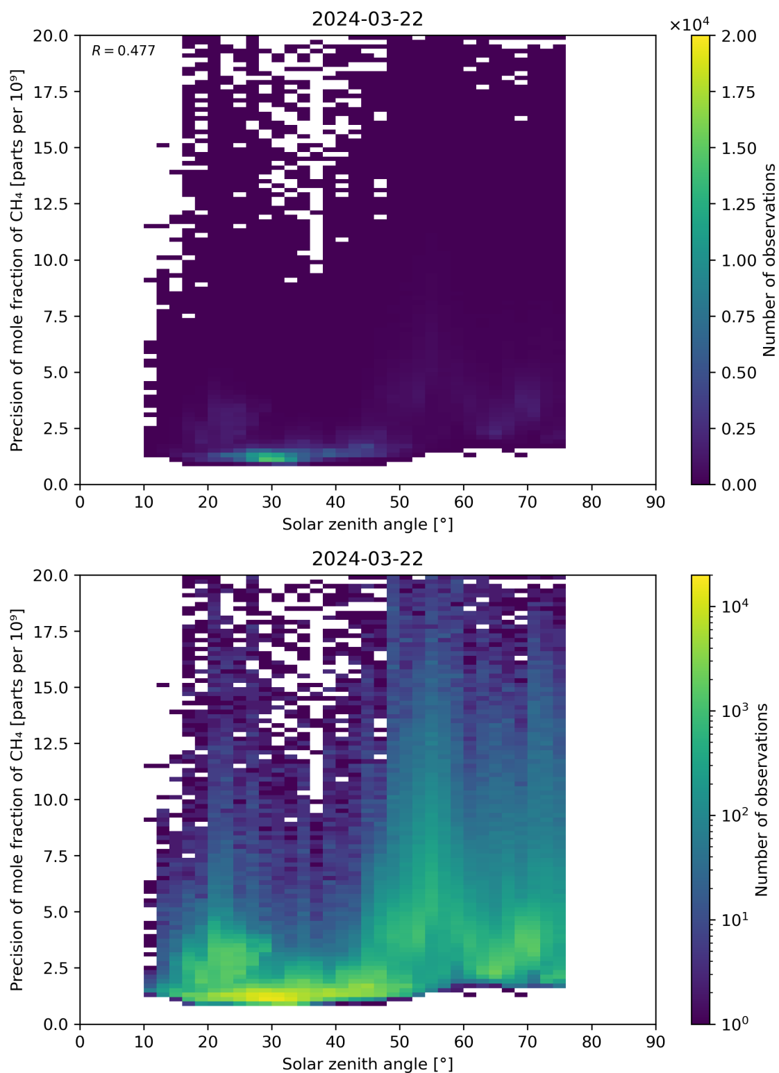
Figure 101: Scatter density plot of “Solar zenith angle” against “Precision of mole fraction of CH 4 ” for 2024-03-21 to 2024-03-22.
