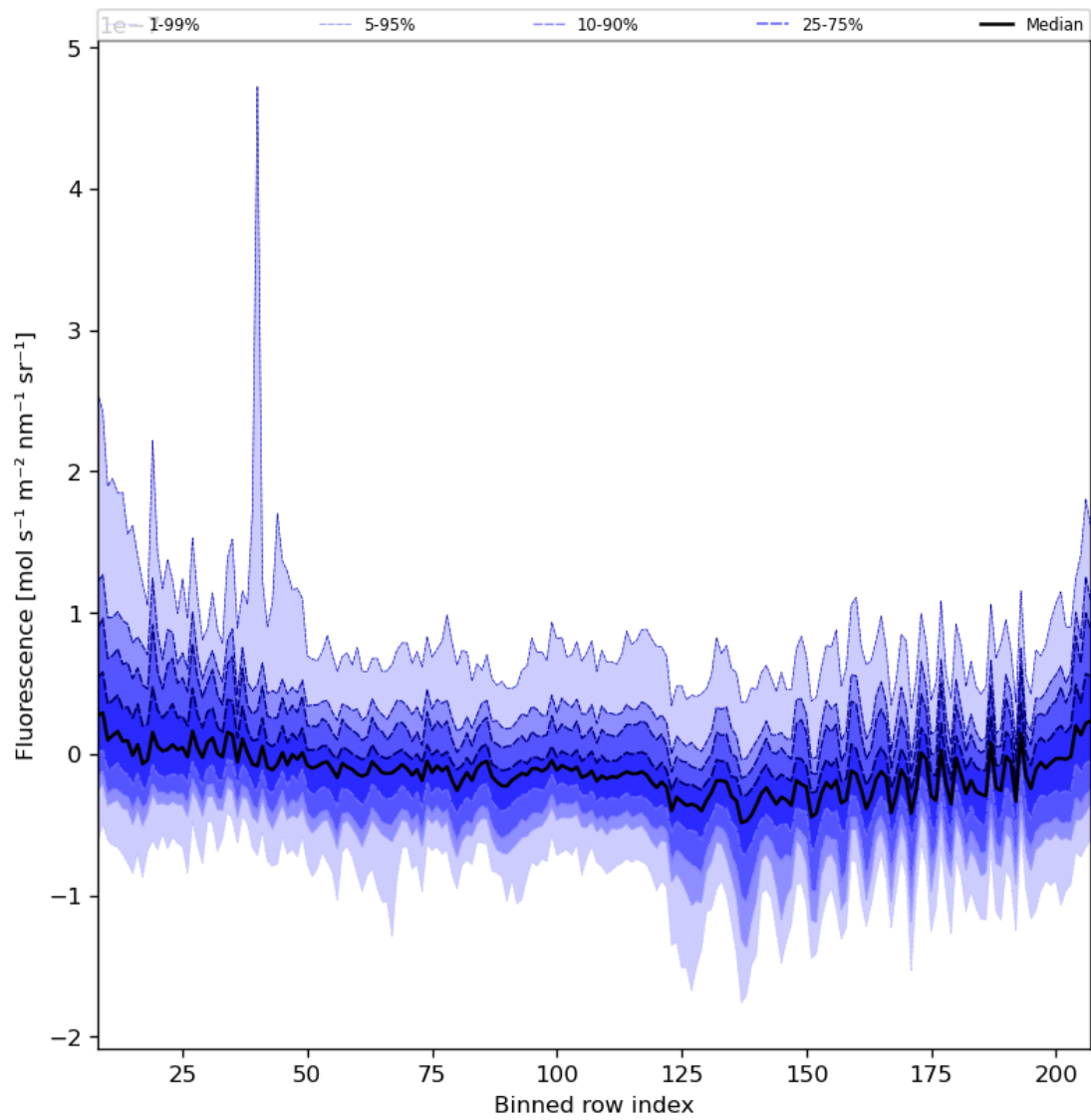
Figure 43: Along track statistics of “Fluorescence” for 2024-03-21 to 2024-03-22
