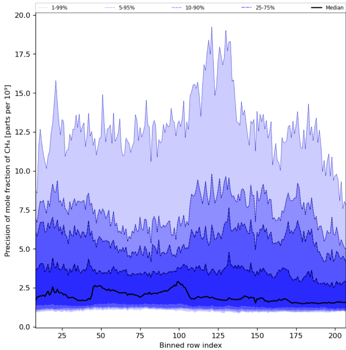
Figure 35: Along track statistics of “Precision of mole fraction of CH 4 ” for 2024-03-21 to 2024-03-22
