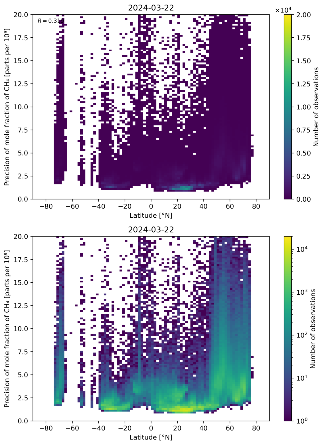
Figure 59: Scatter density plot of “Latitude” against “Precision of mole fraction of CH 4 ” for 2024-03-21 to 2024-03-22.
