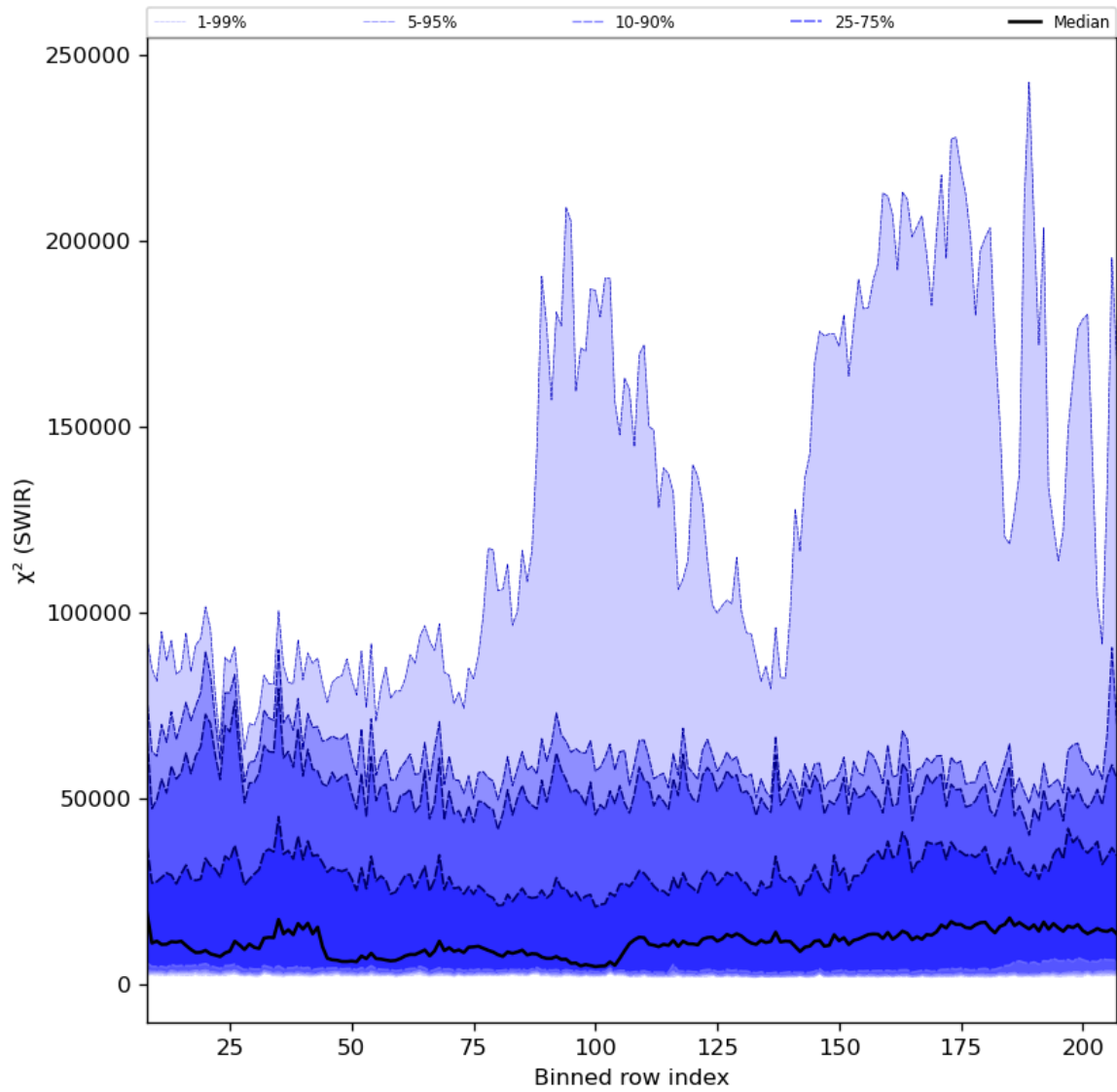
Figure 39: Along track statistics of “ \chi^2 (SWIR)” for 2024-03-21 to 2024-03-22
