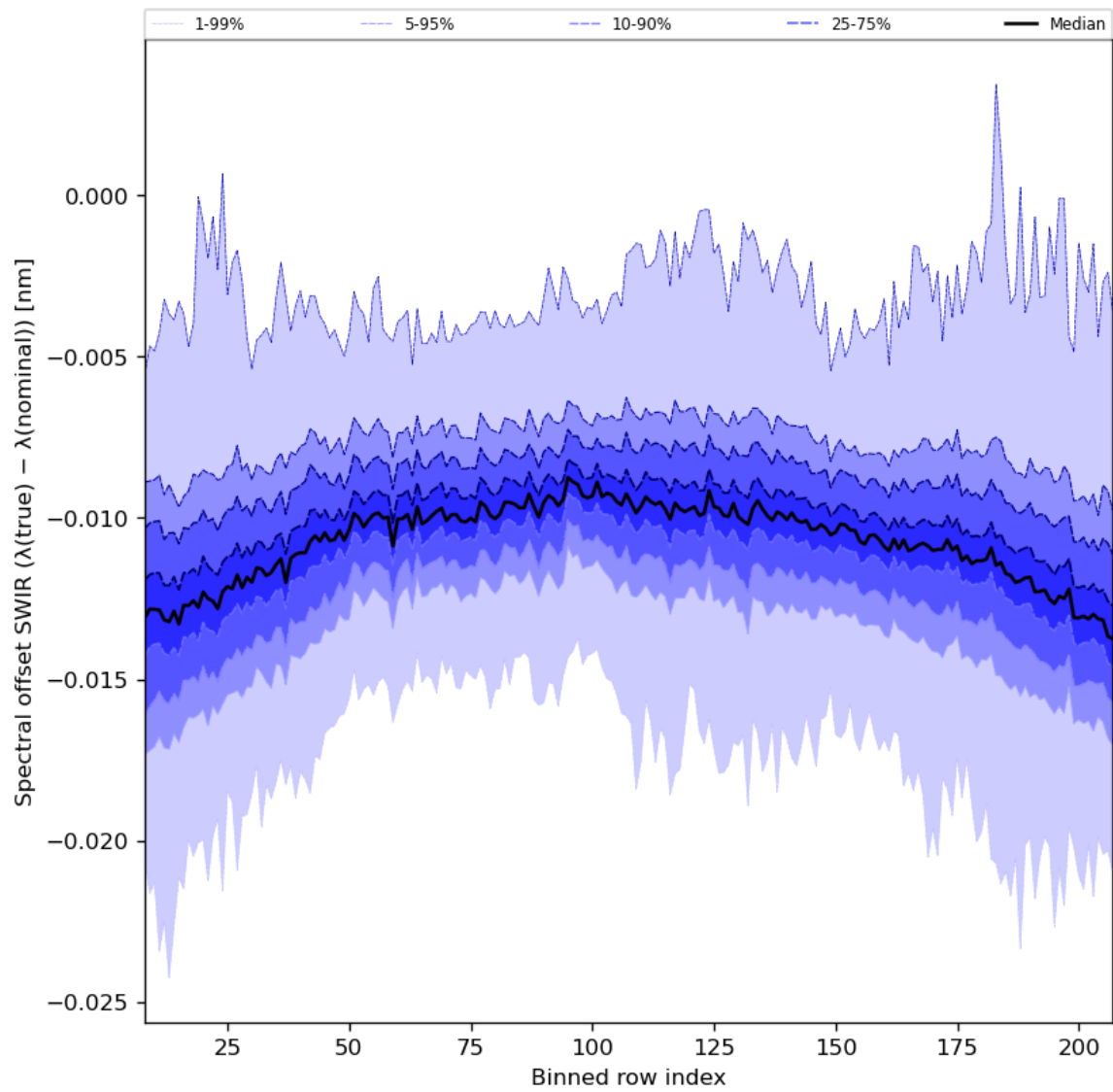
Figure 38: Along track statistics of “Spectral offset SWIR ( \lambda(\text{true}) - \lambda(\text{nominal}) )” for 2024-03-21 to 2024-03-22
