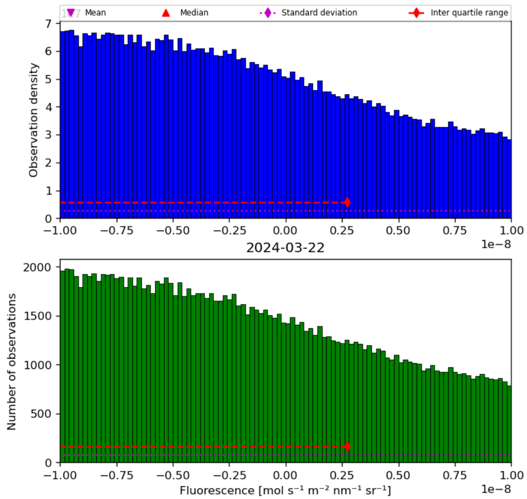
Figure 32: Histogram of “Fluorescence” for 2024-03-21 to 2024-03-22
