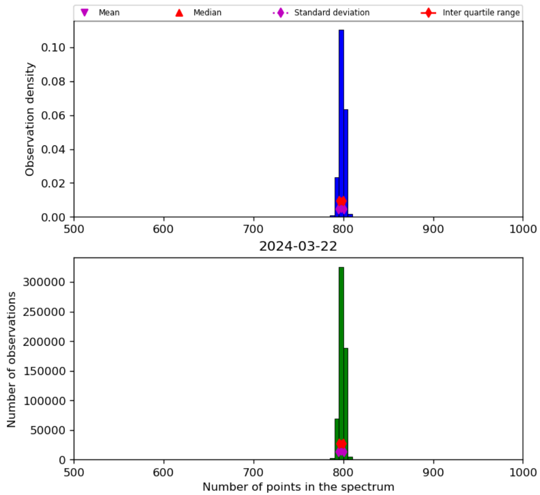
Figure 26: Histogram of “Number of points in the spectrum” for 2024-03-21 to 2024-03-22
