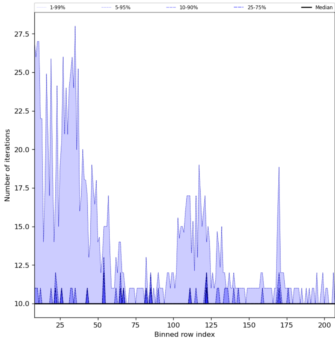
Figure 42: Along track statistics of “Number of iterations” for 2024-03-21 to 2024-03-22
