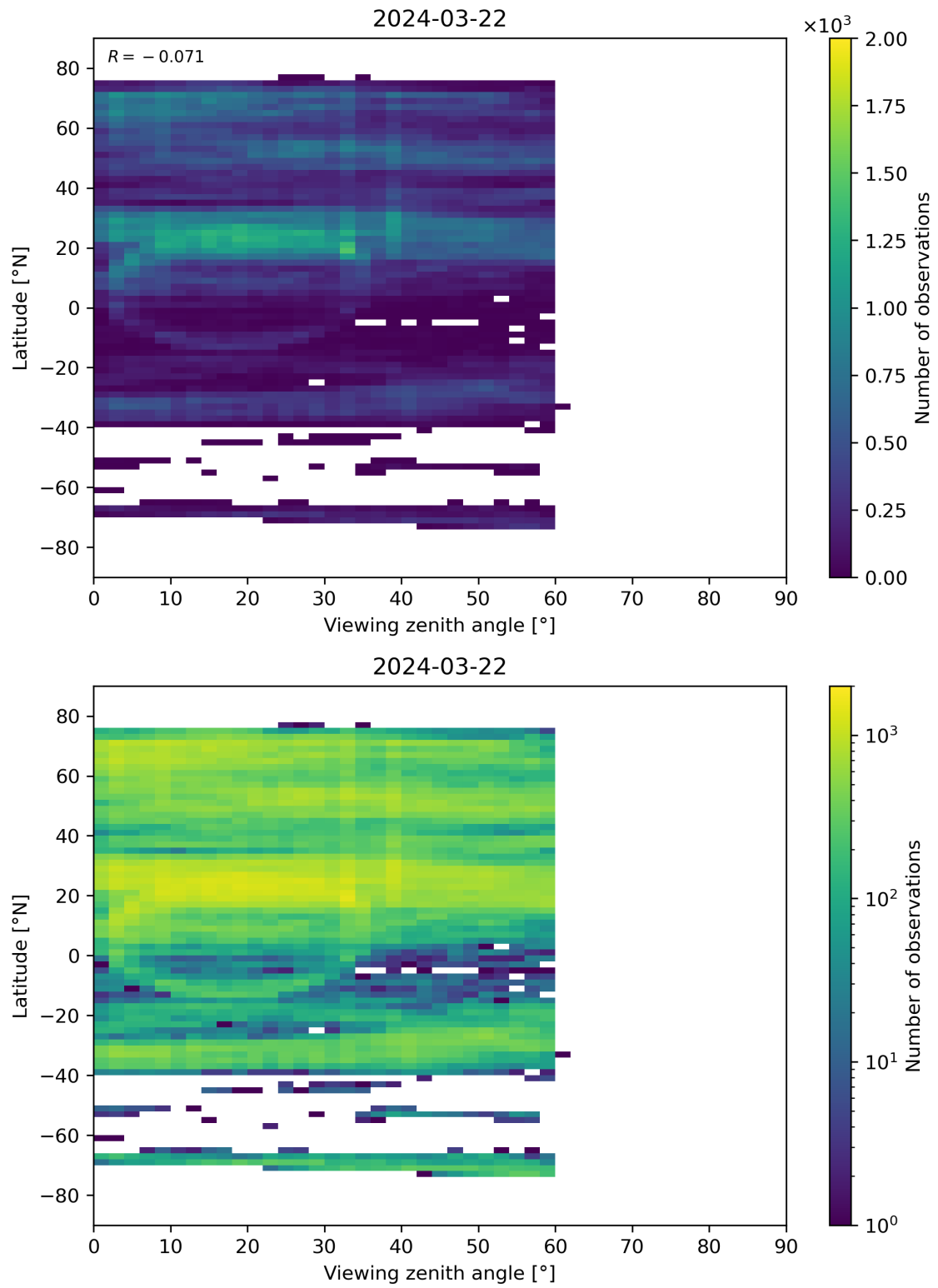
Figure 109: Scatter density plot of “Viewing zenith angle” against “Latitude” for 2024-03-21 to 2024-03-22.
