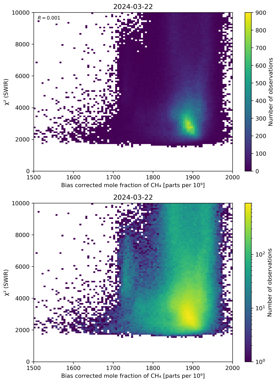
Figure 64: Scatter density plot of “Bias corrected mole fraction of \text{CH}_4 ” against “ \chi^2 (SWIR)” for 2024-03-21 to 2024-03-22.
