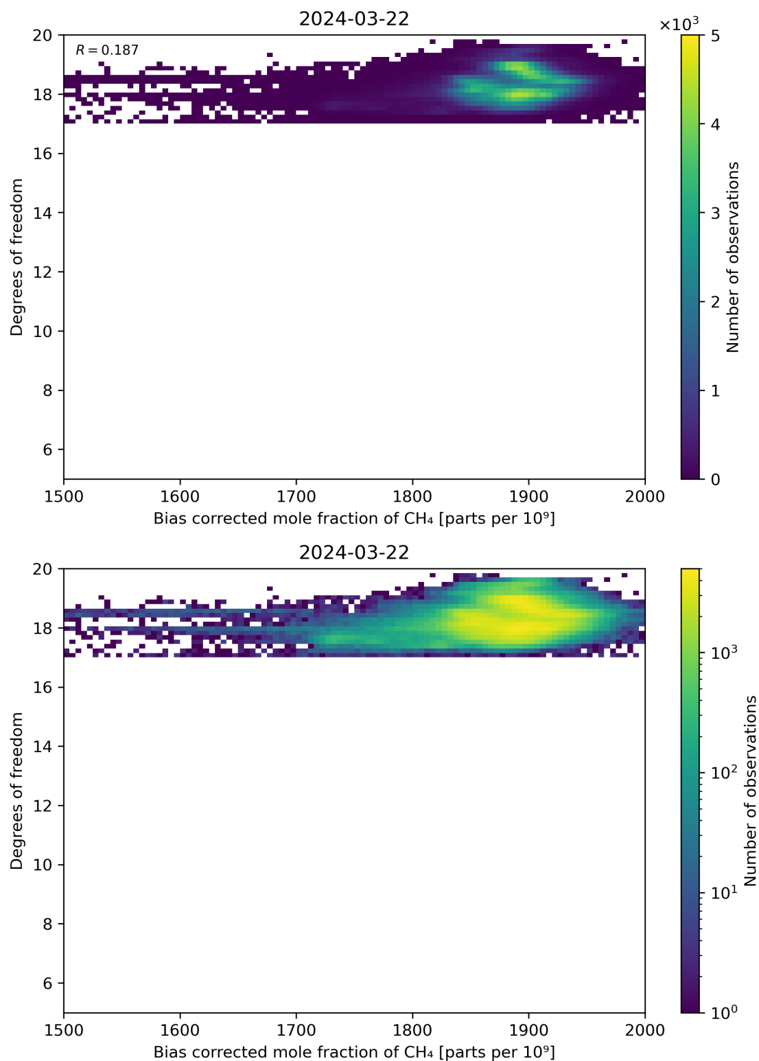
Figure 65: Scatter density plot of “Bias corrected mole fraction of CH 4 ” against “Degrees of freedom” for 2024-03-21 to 2024-03-22.
