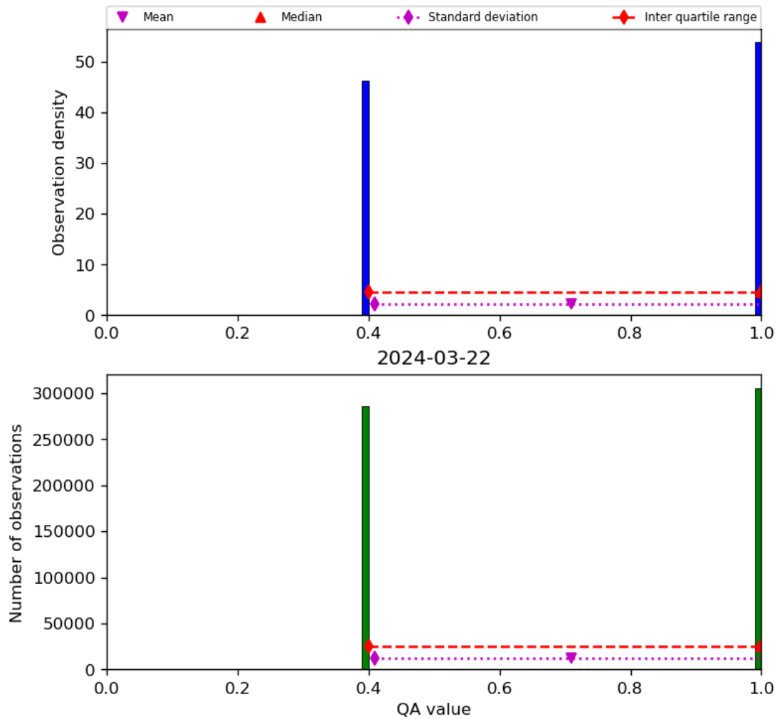
Figure 22: Histogram of “QA value” for 2024-03-21 to 2024-03-22
