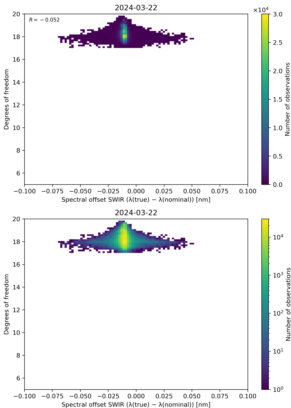
Figure 119: Scatter density plot of “Spectral offset SWIR ( \lambda(\text{true}) - \lambda(\text{nominal}) )” against “Degrees of freedom” for 2024-03-21 to 2024-03-22.
