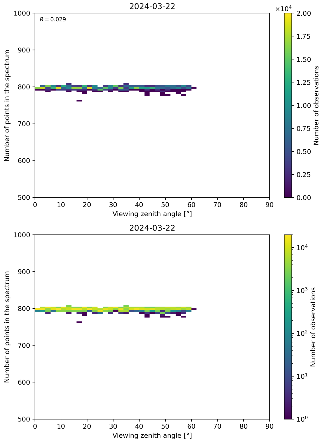
Figure 114: Scatter density plot of “Viewing zenith angle” against “Number of points in the spectrum” for 2024-03-21 to 2024-03-22.
