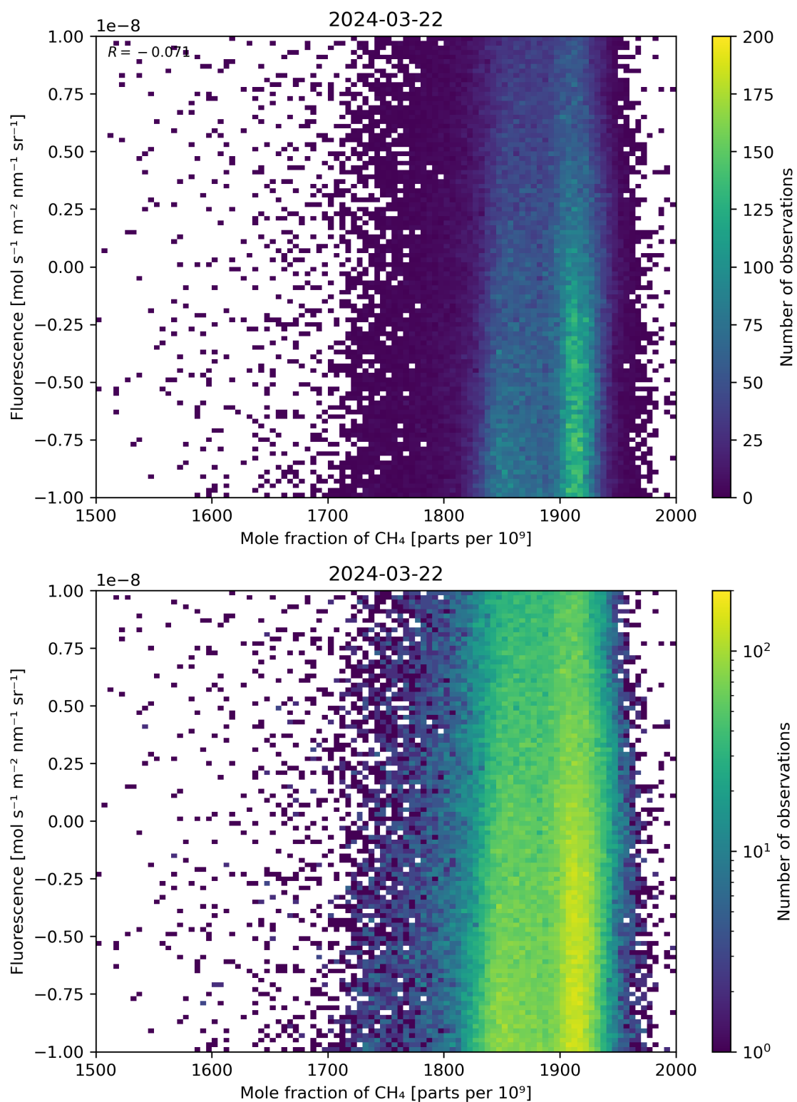
Figure 73: Scatter density plot of “Mole fraction of \text{CH}_4 ” against “Fluorescence” for 2024-03-21 to 2024-03-22.
