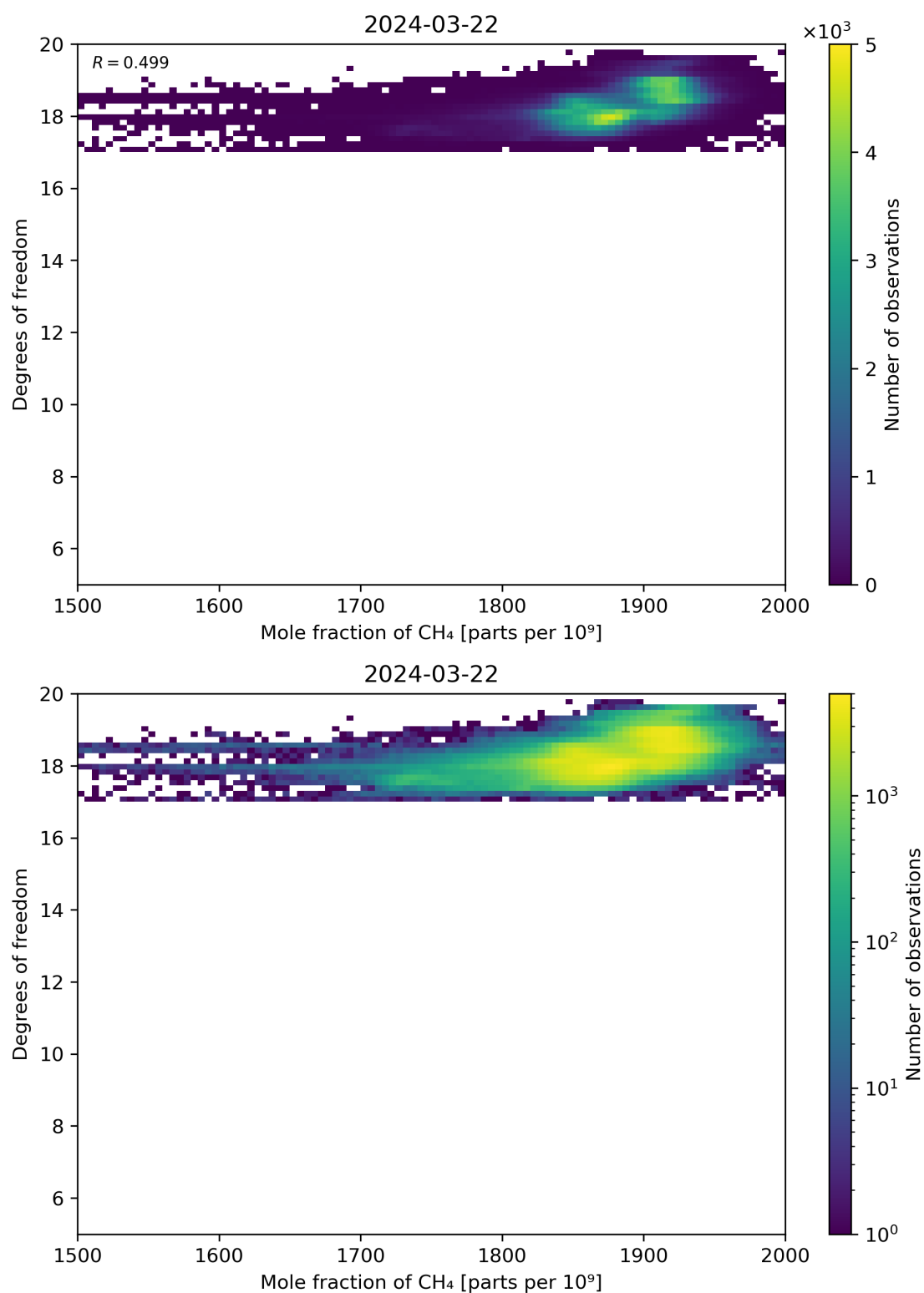
Figure 72: Scatter density plot of “Mole fraction of CH 4 ” against “Degrees of freedom” for 2024-03-21 to 2024-03-22.
