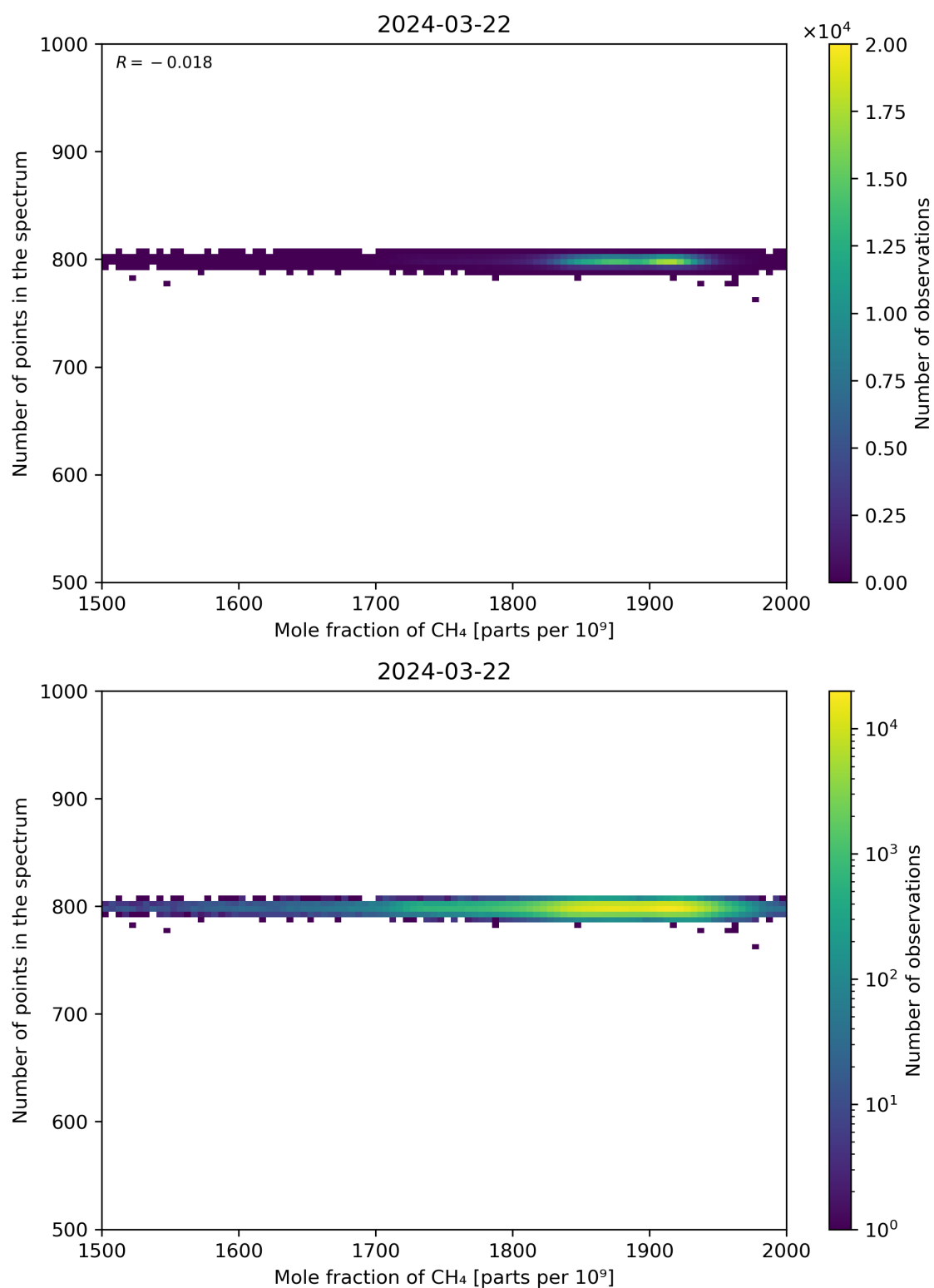
Figure 77: Scatter density plot of “Mole fraction of CH 4 ” against “Number of points in the spectrum” for 2024-03-21 to 2024-03-22.
