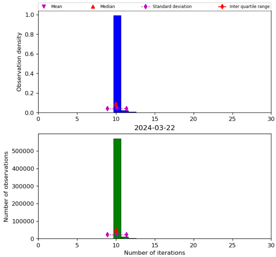
Figure 31: Histogram of “Number of iterations” for 2024-03-21 to 2024-03-22
