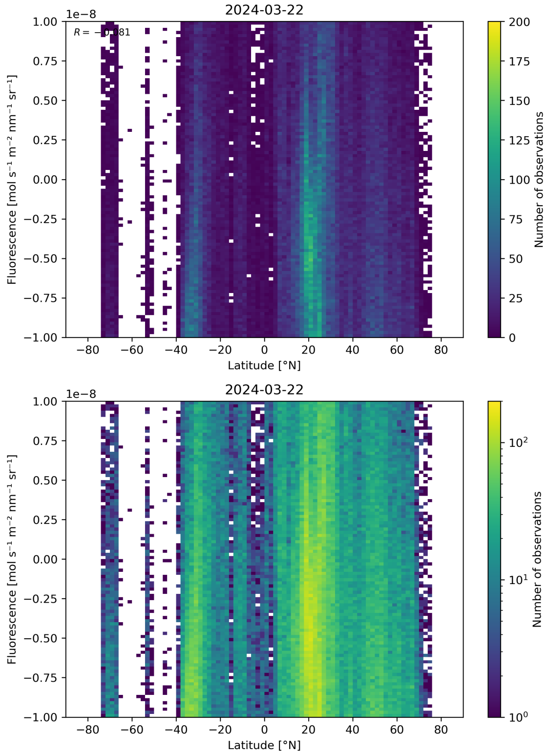
Figure 56: Scatter density plot of “Latitude” against “Fluorescence” for 2024-03-21 to 2024-03-22.
