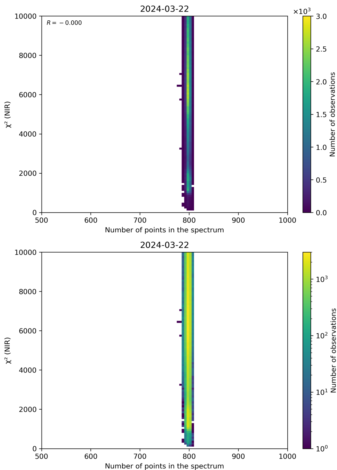
Figure 88: Scatter density plot of “Number of points in the spectrum” against “ \chi^2 (NIR)” for 2024-03-21 to 2024-03-22.
