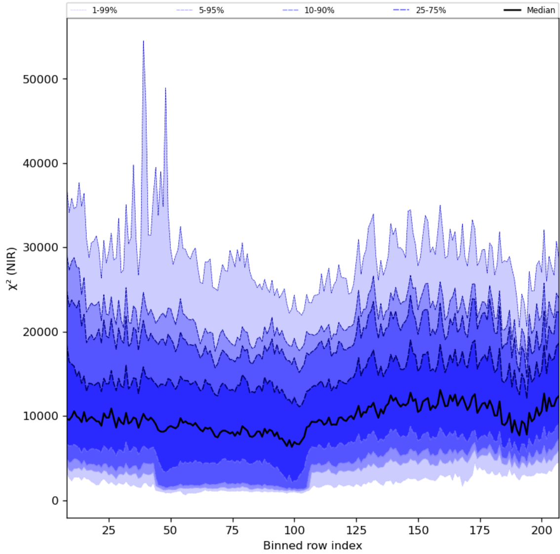
Figure 40: Along track statistics of “ \chi^2 (NIR)” for 2024-03-21 to 2024-03-22
