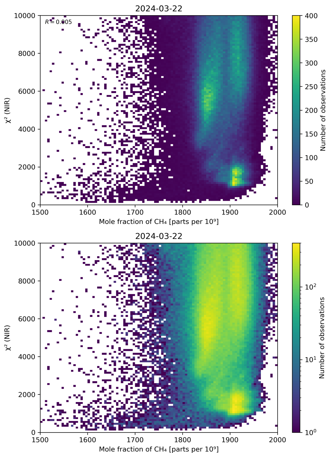
Figure 70: Scatter density plot of “Mole fraction of CH 4 ” against “ \chi^2 (NIR)” for 2024-03-21 to 2024-03-22.
