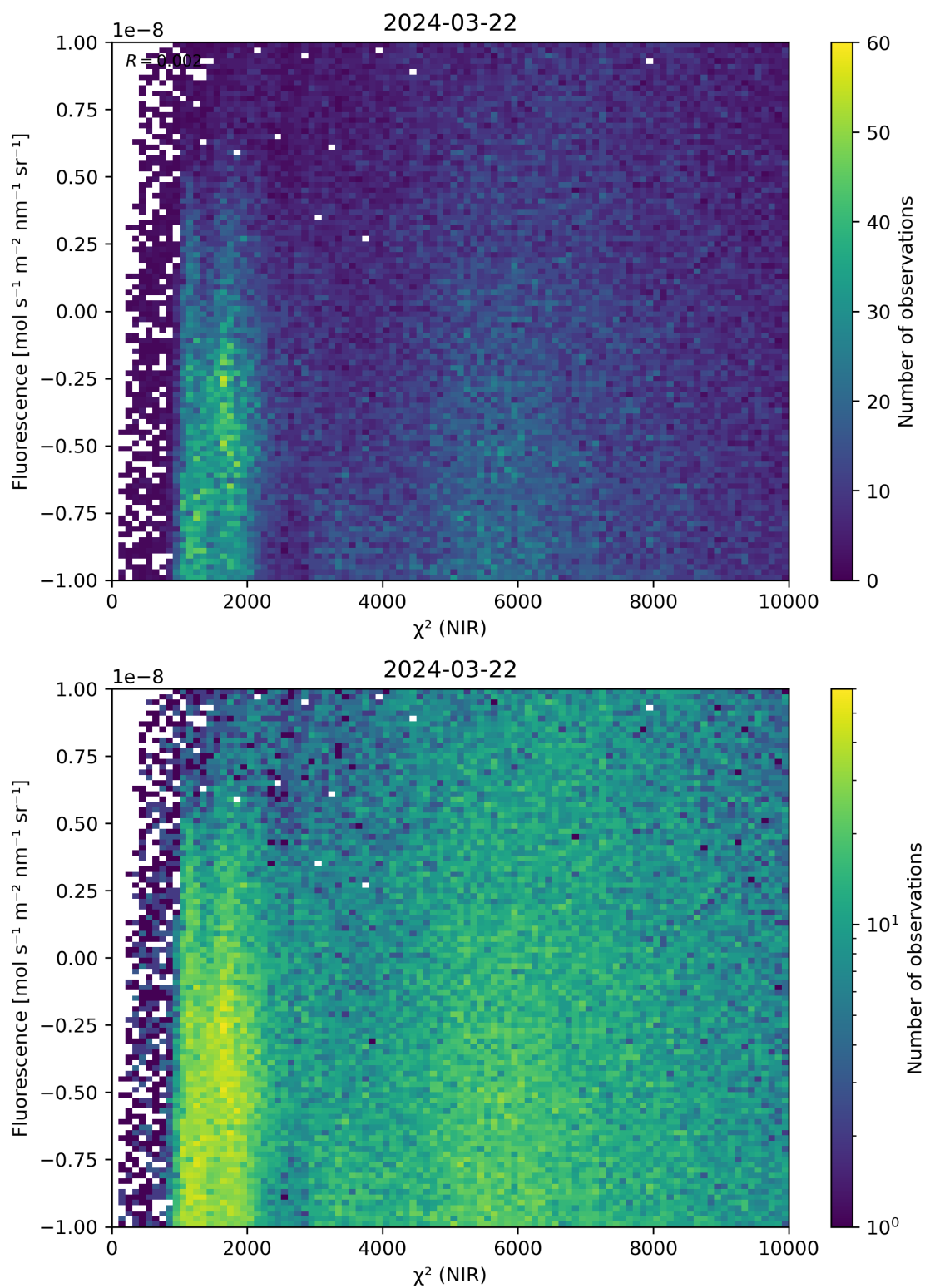
Figure 45: Scatter density plot of “ \chi^2 (NIR)” against “Fluorescence” for 2024-03-21 to 2024-03-22.
