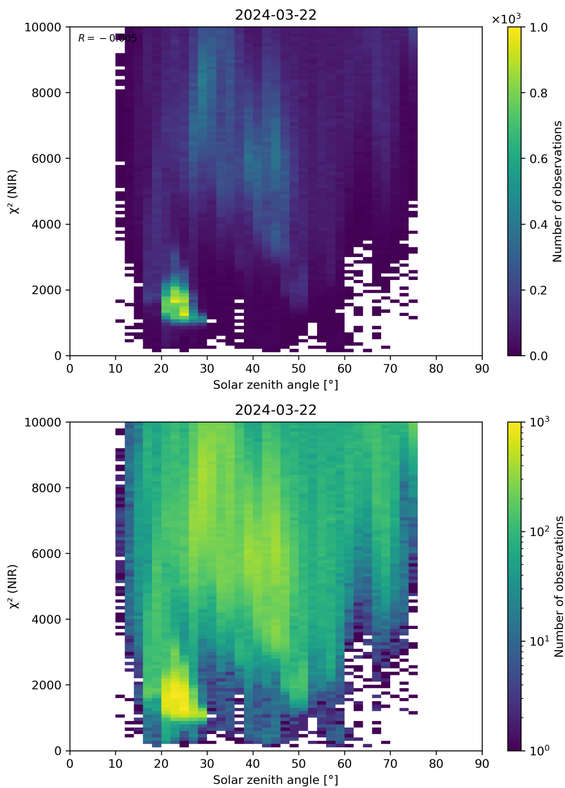
Figure 94: Scatter density plot of “Solar zenith angle” against “ \chi^2 (NIR)” for 2024-03-21 to 2024-03-22.
