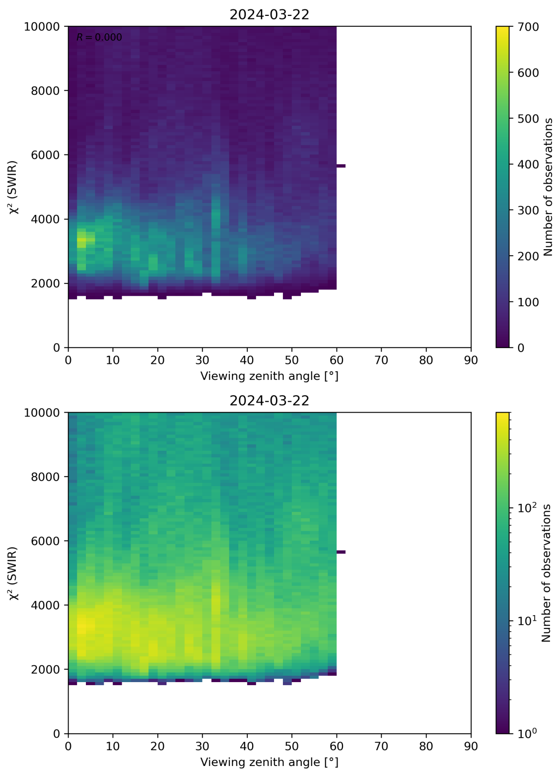
Figure 106: Scatter density plot of “Viewing zenith angle” against “ \chi^2 (SWIR)” for 2024-03-21 to 2024-03-22.
