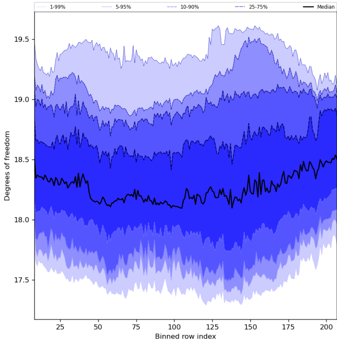
Figure 41: Along track statistics of “Degrees of freedom” for 2024-03-21 to 2024-03-22
