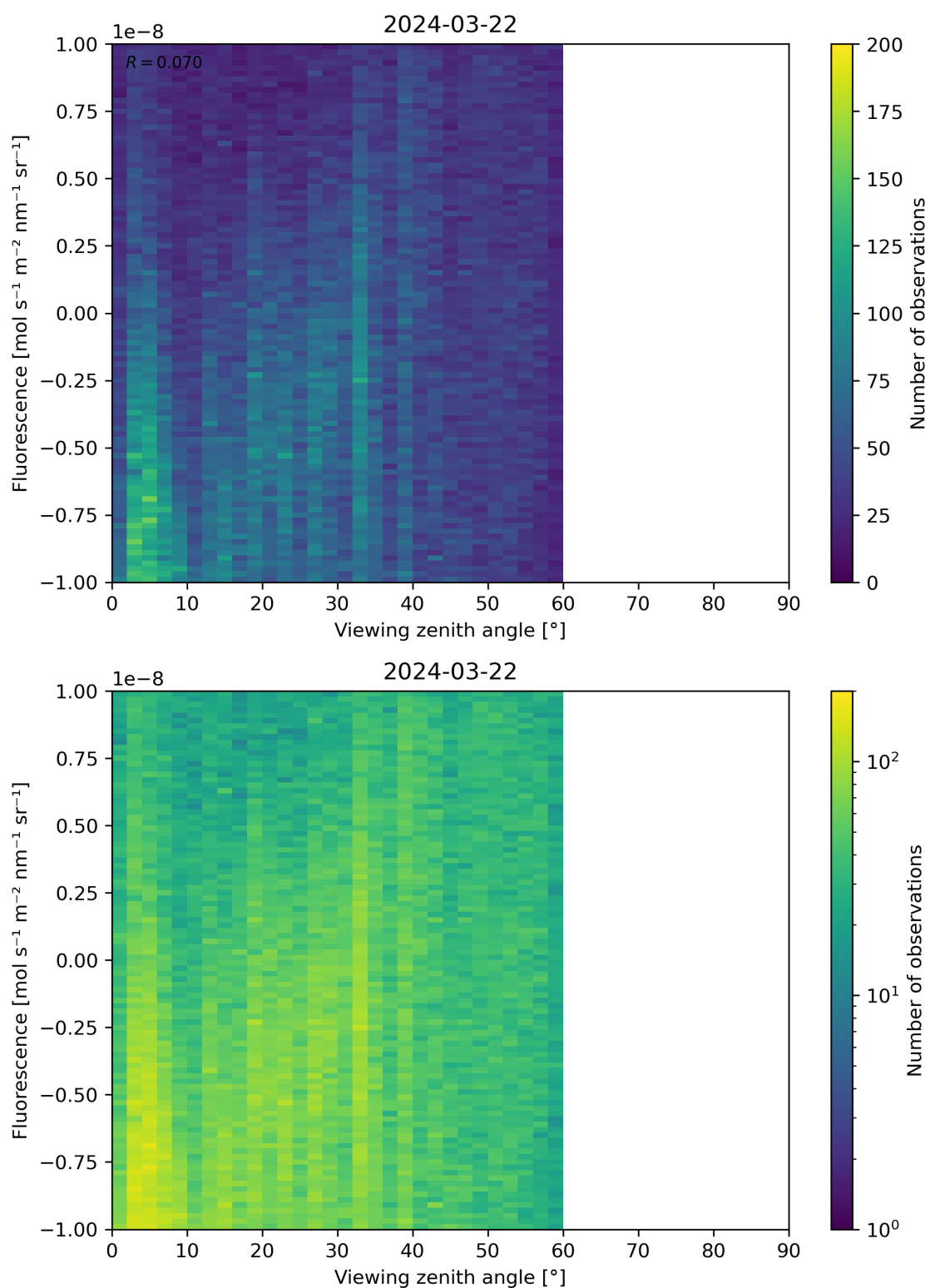
Figure 108: Scatter density plot of “Viewing zenith angle” against “Fluorescence” for 2024-03-21 to 2024-03-22.
