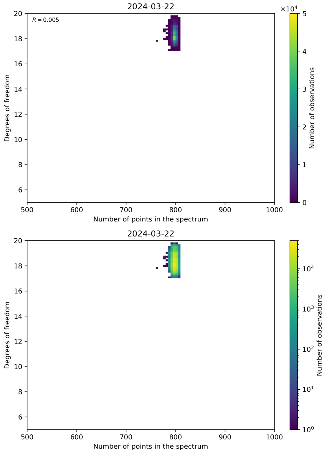
Figure 90: Scatter density plot of “Number of points in the spectrum” against “Degrees of freedom” for 2024-03-21 to 2024-03-22.
