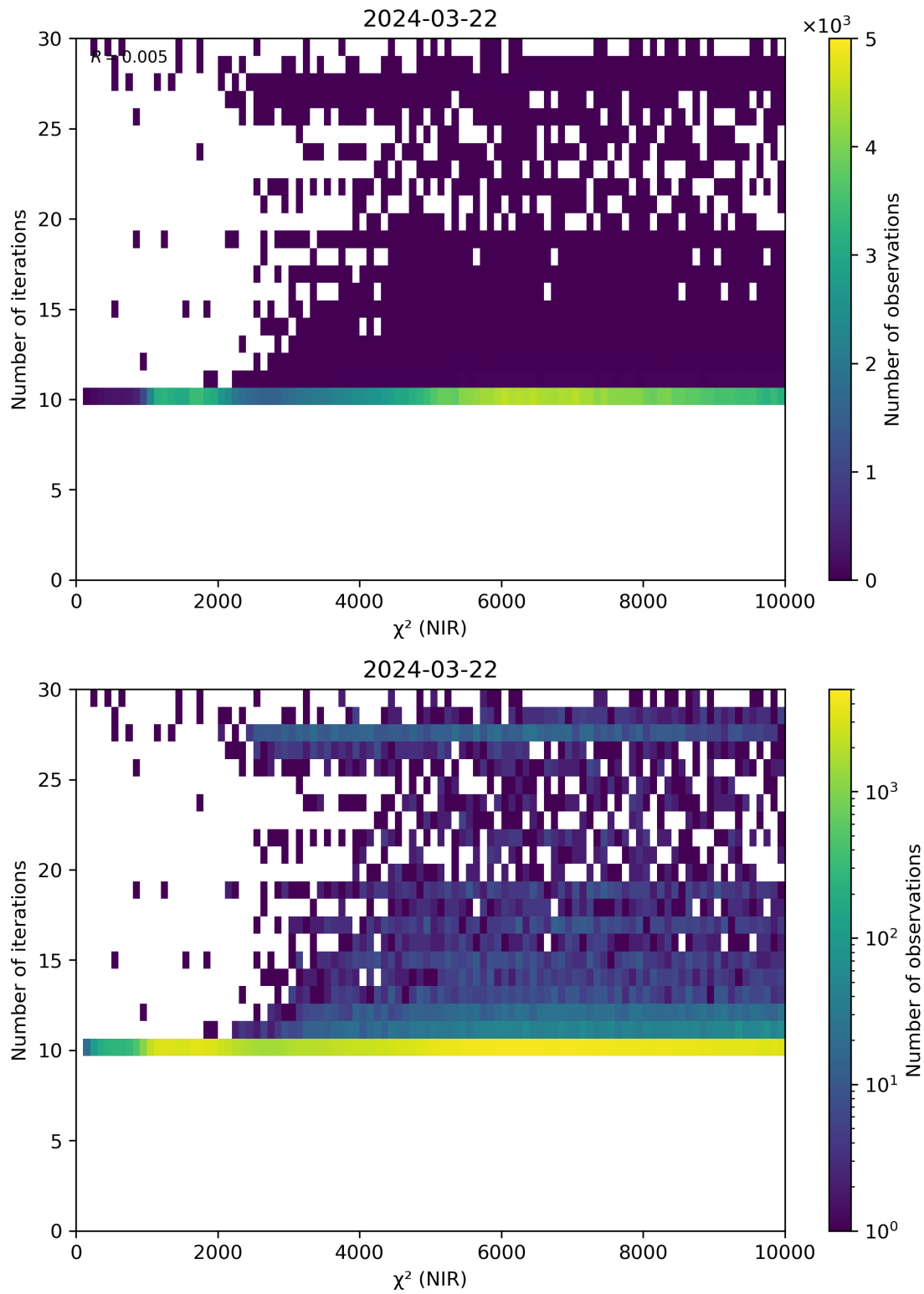
Figure 46: Scatter density plot of “ \chi^2 (NIR)” against “Number of iterations” for 2024-03-21 to 2024-03-22.
