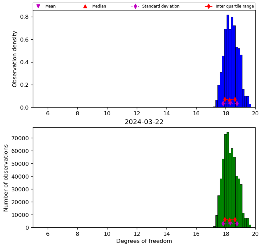
Figure 30: Histogram of “Degrees of freedom” for 2024-03-21 to 2024-03-22
