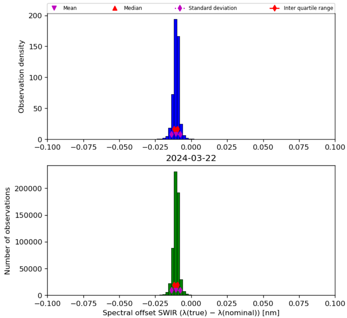
Figure 27: Histogram of “Spectral offset SWIR ( \lambda(\text{true}) - \lambda(\text{nominal}) )” for 2024-03-21 to 2024-03-22
