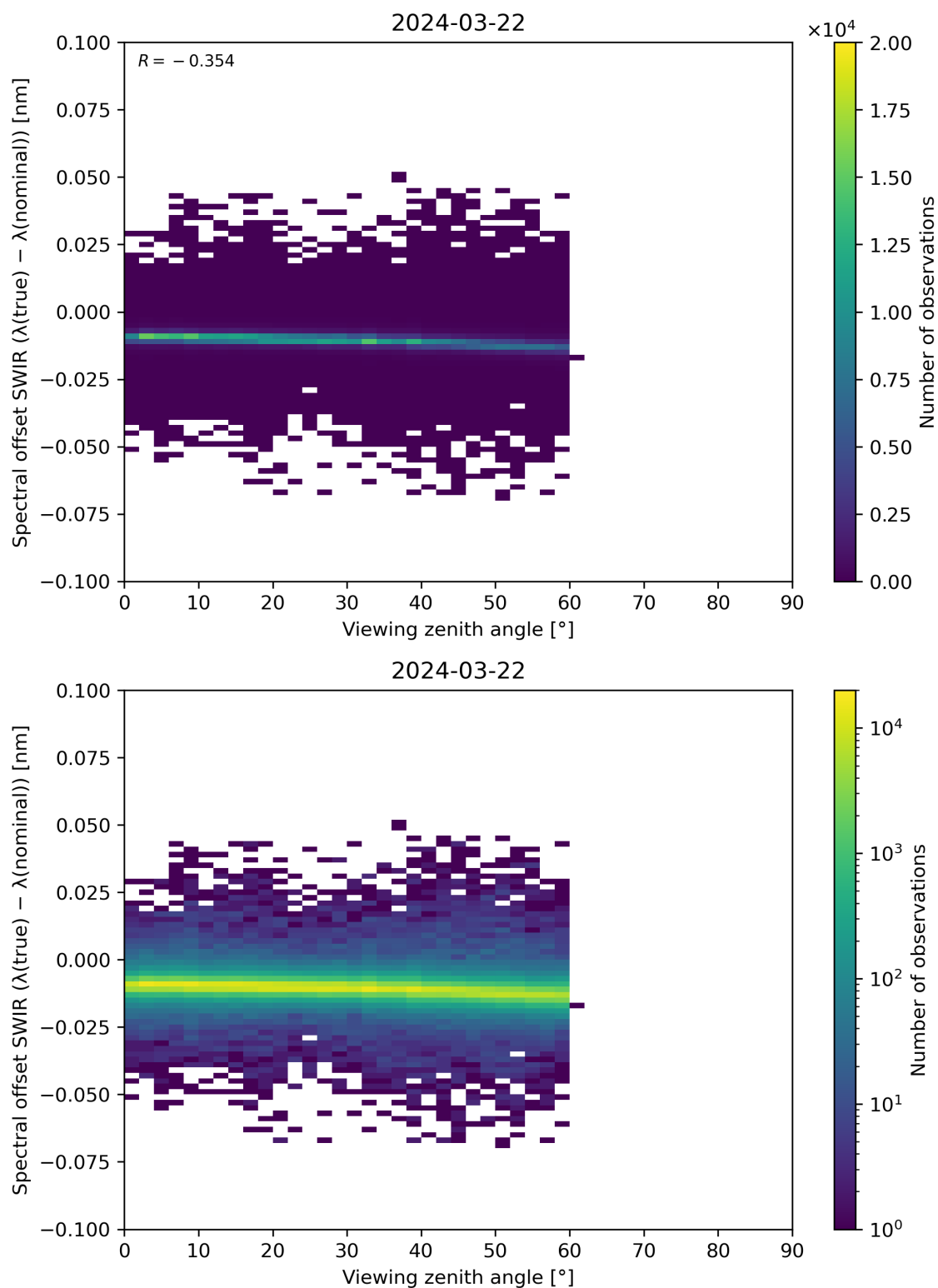
Figure 116: Scatter density plot of “Viewing zenith angle” against “Spectral offset SWIR ( \lambda(\text{true}) - \lambda(\text{nominal}) )” for 2024-03-21 to 2024-03-22.
