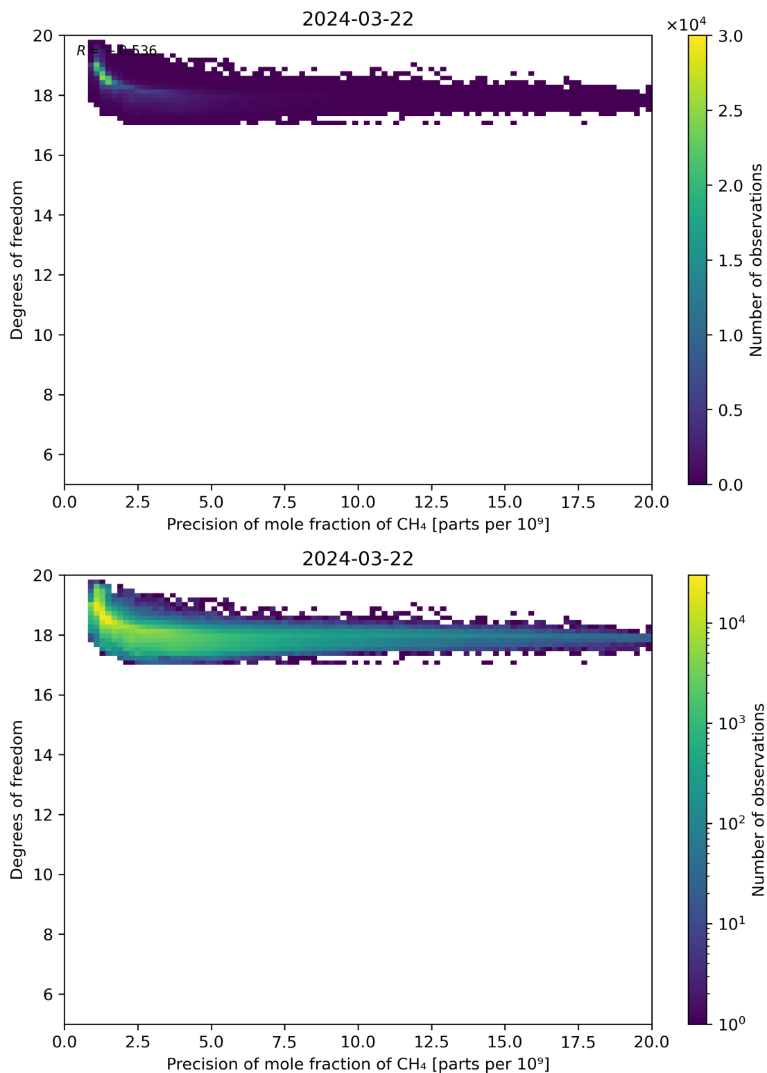
Figure 80: Scatter density plot of “Precision of mole fraction of CH 4 ” against “Degrees of freedom” for 2024-03-21 to 2024-03-22.
