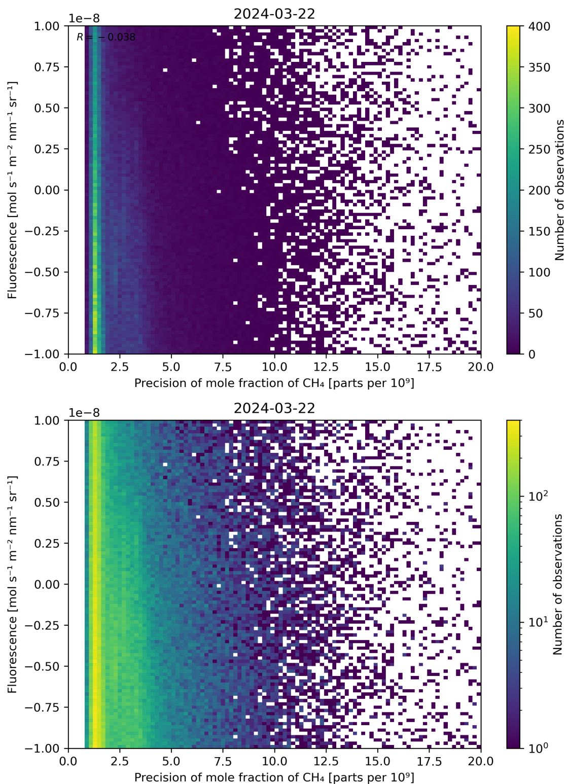
Figure 81: Scatter density plot of “Precision of mole fraction of \text{CH}_4 ” against “Fluorescence” for 2024-03-21 to 2024-03-22.
