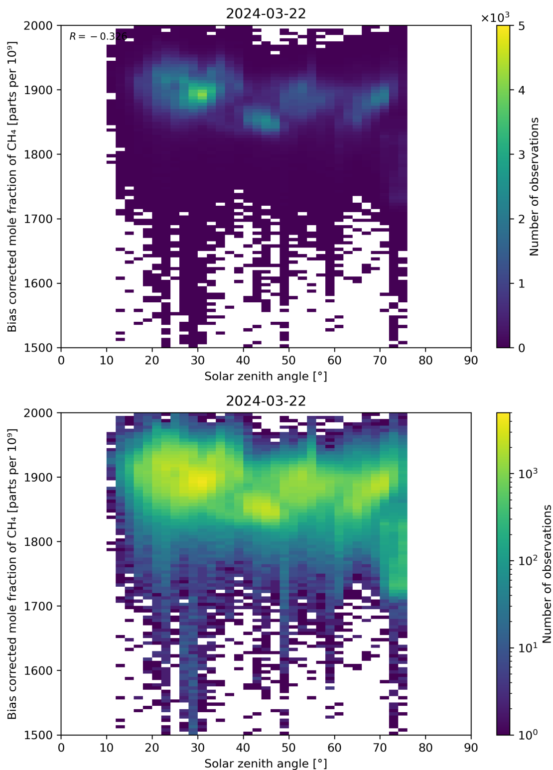
Figure 100: Scatter density plot of “Solar zenith angle” against “Bias corrected mole fraction of CH 4 ” for 2024-03-21 to 2024-03-22.
