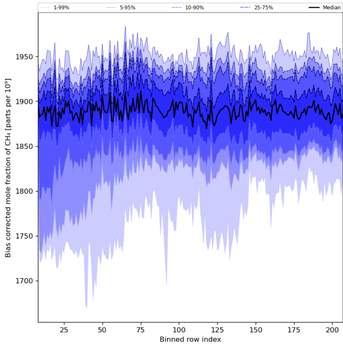
Figure 36: Along track statistics of “Bias corrected mole fraction of CH 4 ” for 2024-03-21 to 2024-03-22
