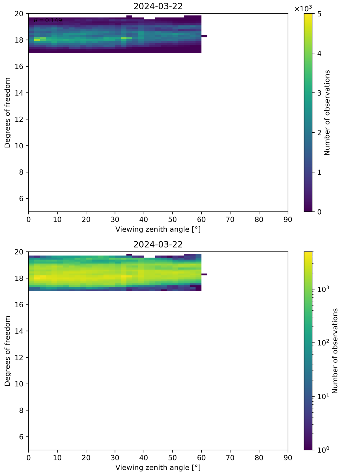
Figure 107: Scatter density plot of “Viewing zenith angle” against “Degrees of freedom” for 2024-03-21 to 2024-03-22.
