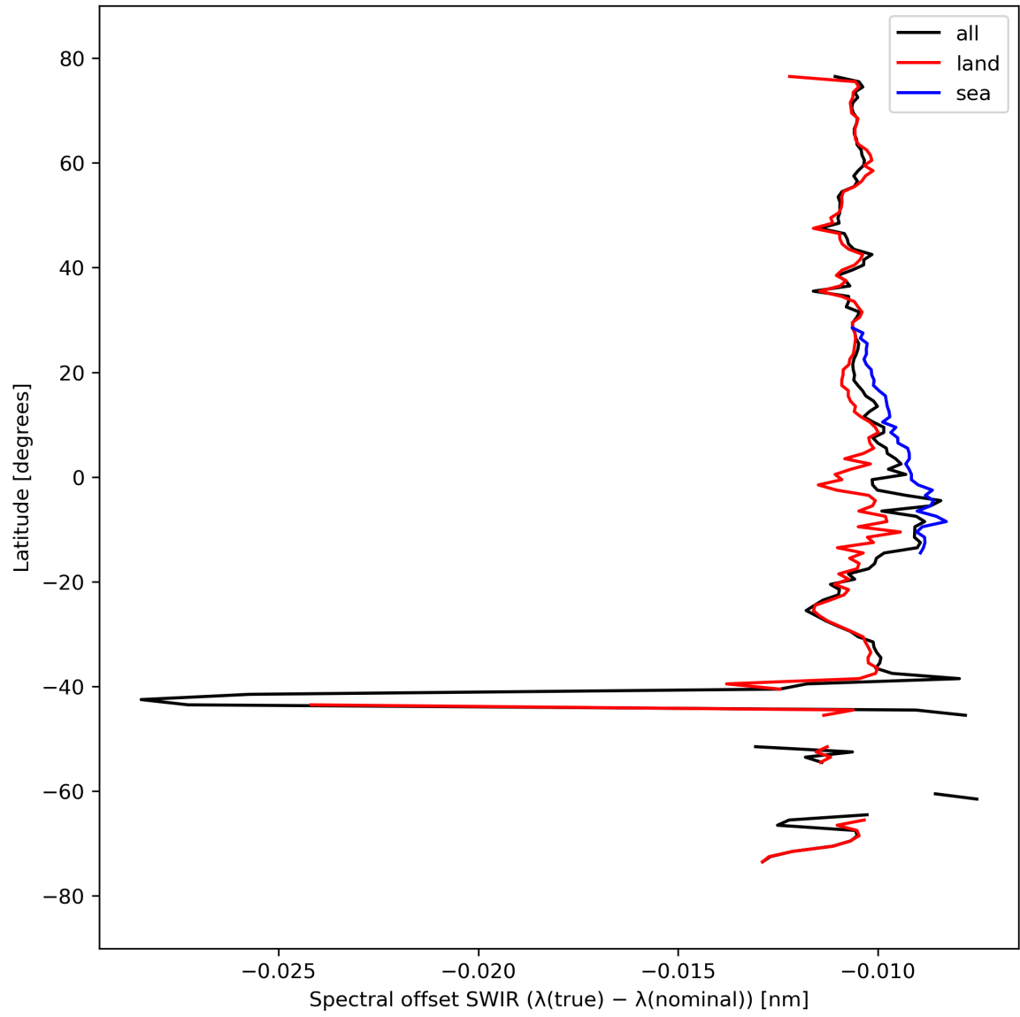
Figure 16: Zonal average of “Spectral offset SWIR ( \lambda(\text{true}) - \lambda(\text{nominal}) )” for 2024-03-21 to 2024-03-22.
