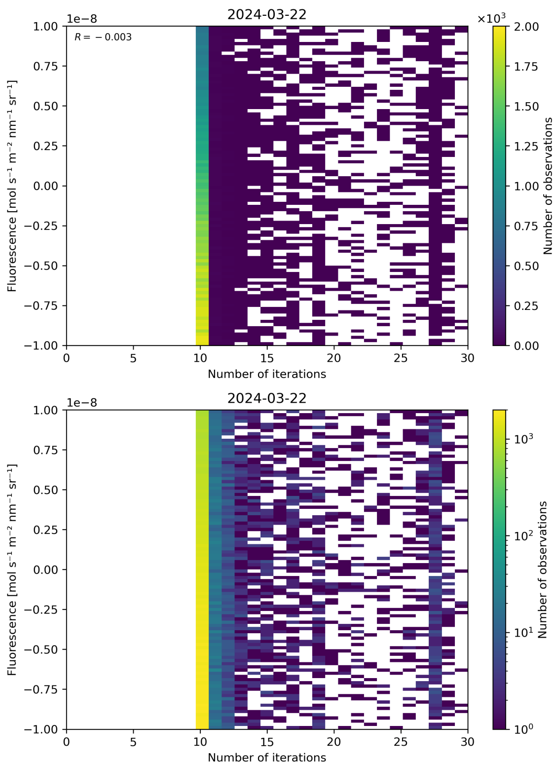
Figure 87: Scatter density plot of “Number of iterations” against “Fluorescence” for 2024-03-21 to 2024-03-22.
