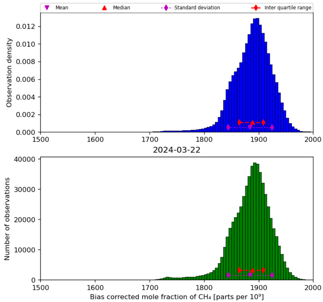
Figure 25: Histogram of “Bias corrected mole fraction of CH 4 ” for 2024-03-21 to 2024-03-22
