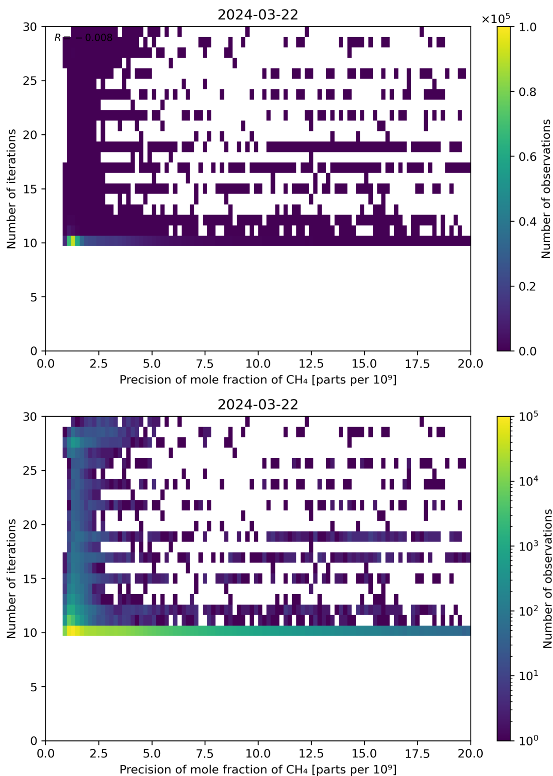
Figure 83: Scatter density plot of “Precision of mole fraction of CH 4 ” against “Number of iterations” for 2024-03-21 to 2024-03-22.
