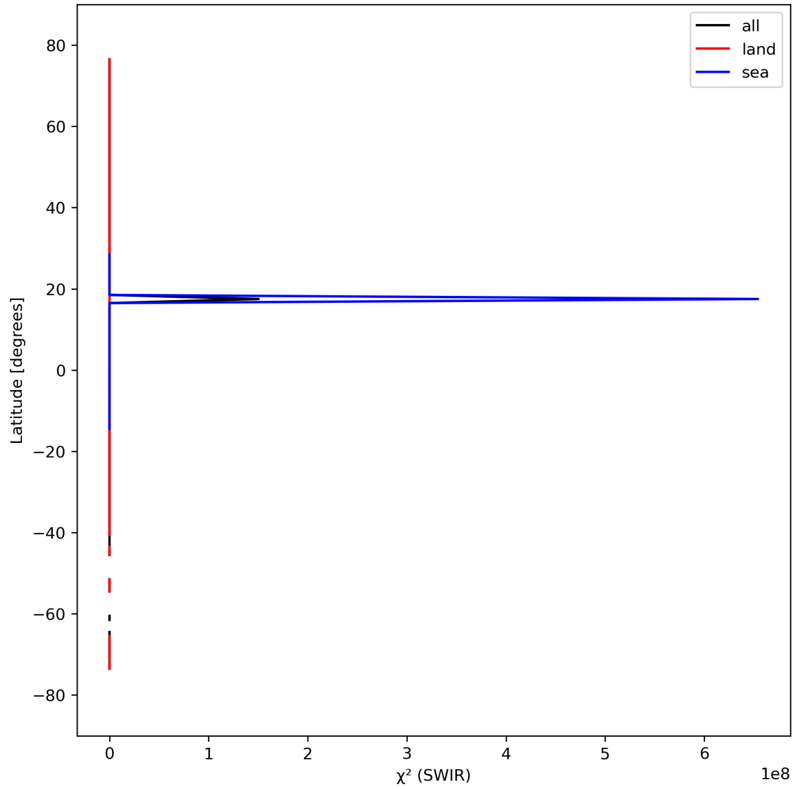
Figure 17: Zonal average of “ \chi^2 (SWIR)” for 2024-03-21 to 2024-03-22.
