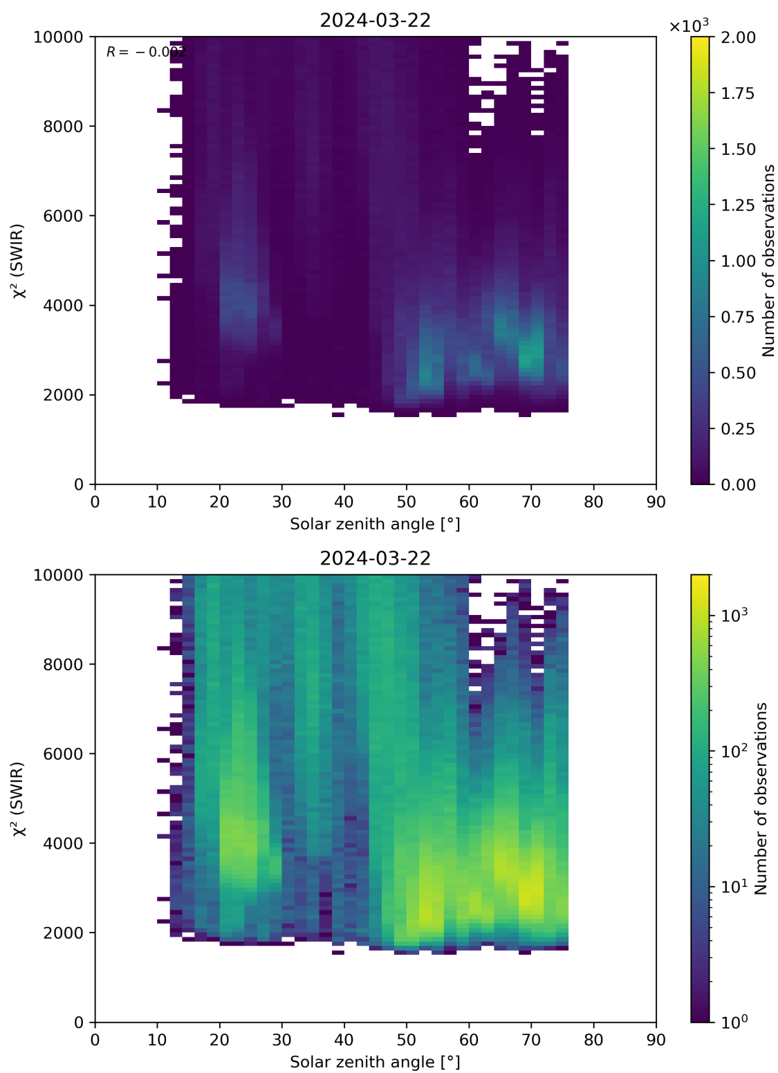
Figure 95: Scatter density plot of “Solar zenith angle” against “ \chi^2 (SWIR)” for 2024-03-21 to 2024-03-22.
