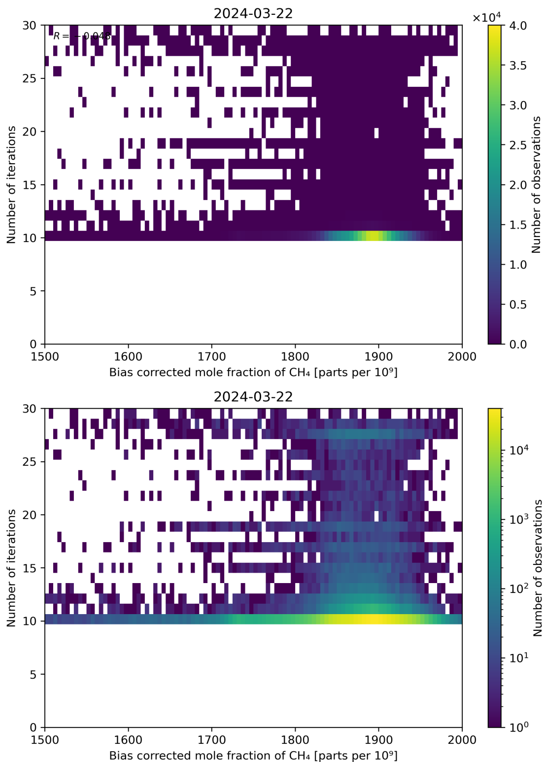
Figure 67: Scatter density plot of “Bias corrected mole fraction of CH 4 ” against “Number of iterations” for 2024-03-21 to 2024-03-22.
