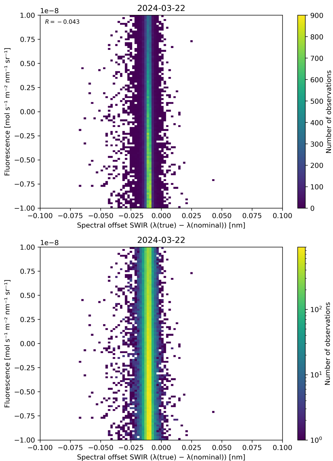
Figure 120: Scatter density plot of “Spectral offset SWIR ( \lambda(\text{true}) - \lambda(\text{nominal}) )” against “Fluorescence” for 2024-03-21 to 2024-03-22.
