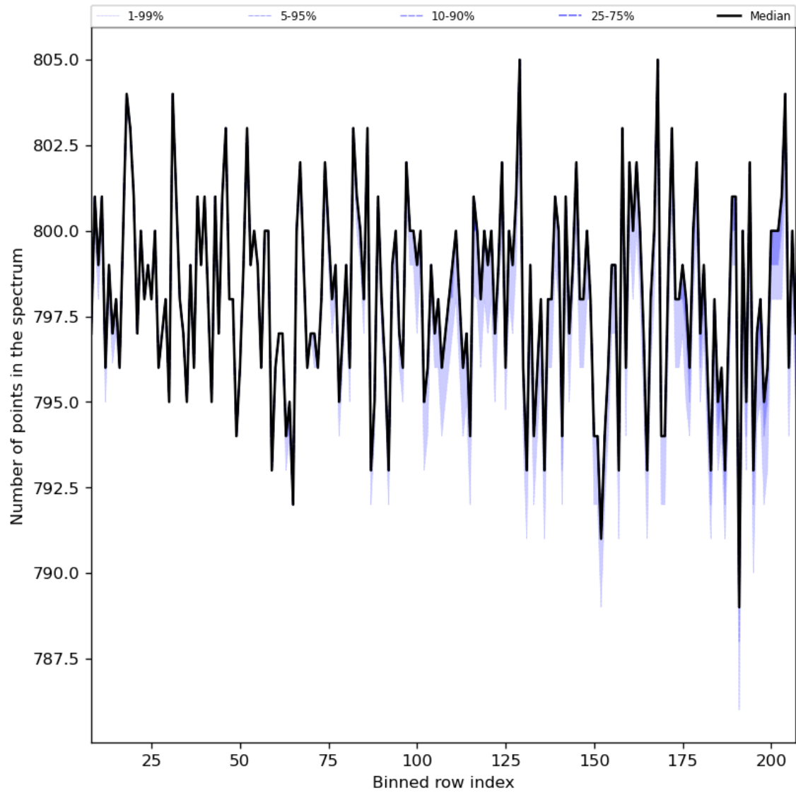
Figure 37: Along track statistics of “Number of points in the spectrum” for 2024-03-21 to 2024-03-22
