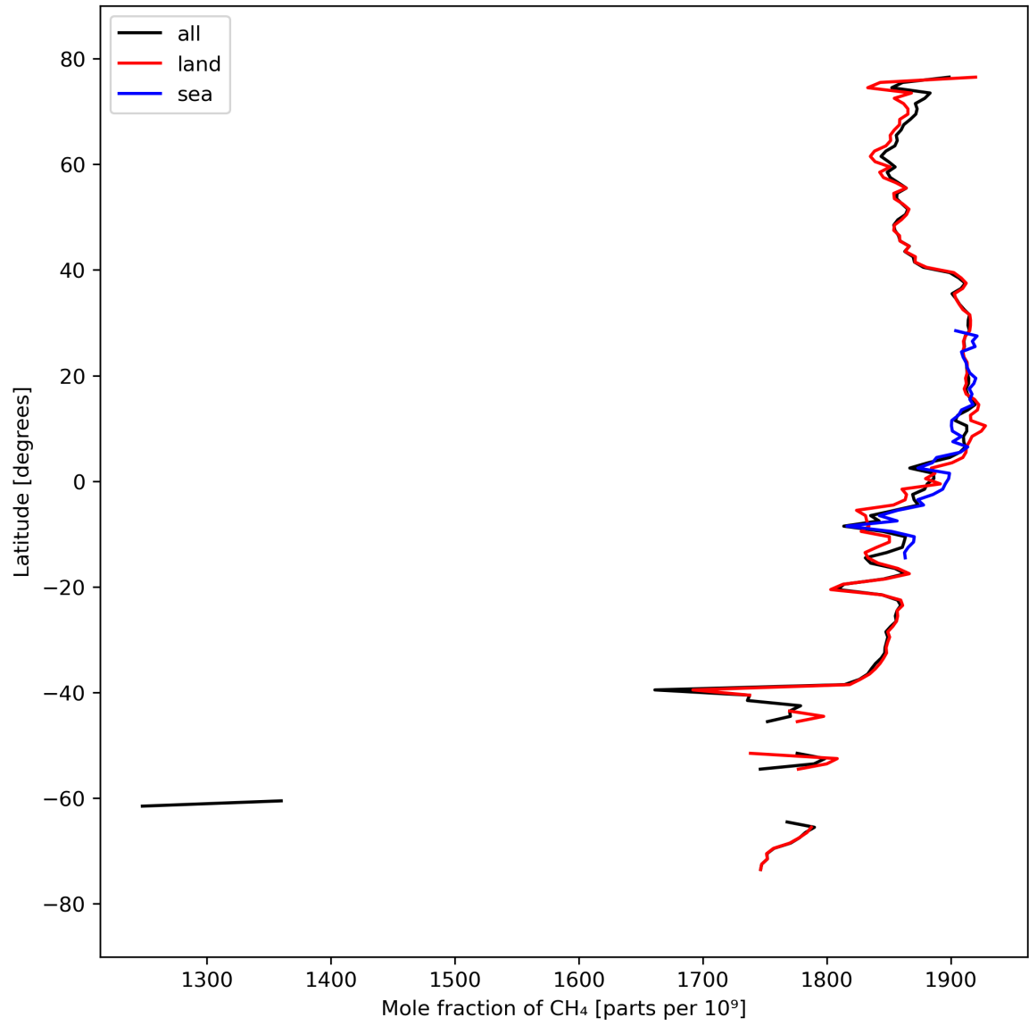
Figure 12: Zonal average of “Mole fraction of CH 4 ” for 2024-03-21 to 2024-03-22.
