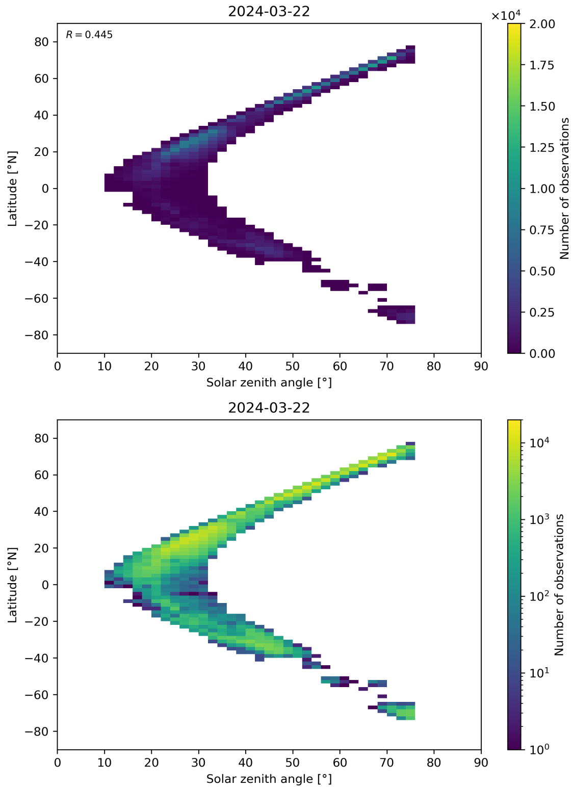
Figure 98: Scatter density plot of “Solar zenith angle” against “Latitude” for 2024-03-21 to 2024-03-22.
