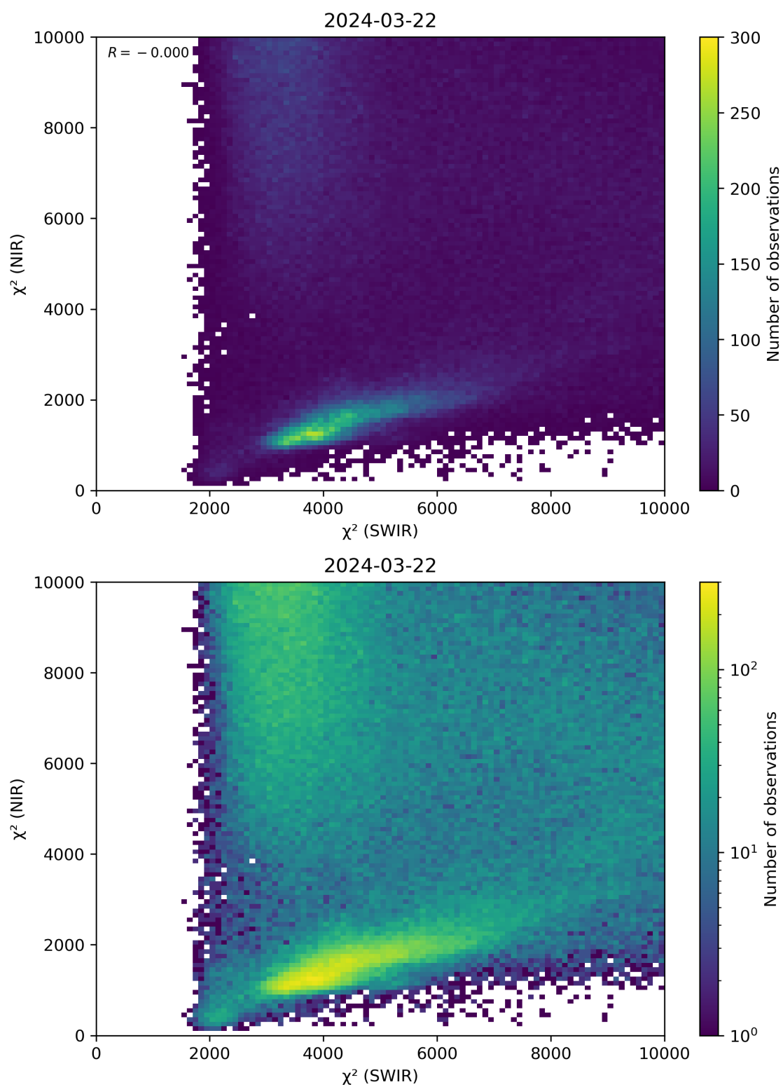
Figure 47: Scatter density plot of “ \chi^2 (SWIR)” against “ \chi^2 (NIR)” for 2024-03-21 to 2024-03-22.
