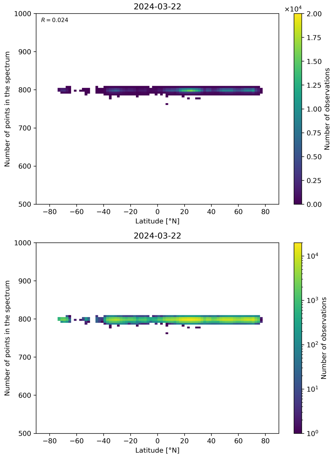
Figure 61: Scatter density plot of “Latitude” against “Number of points in the spectrum” for 2024-03-21 to 2024-03-22.
