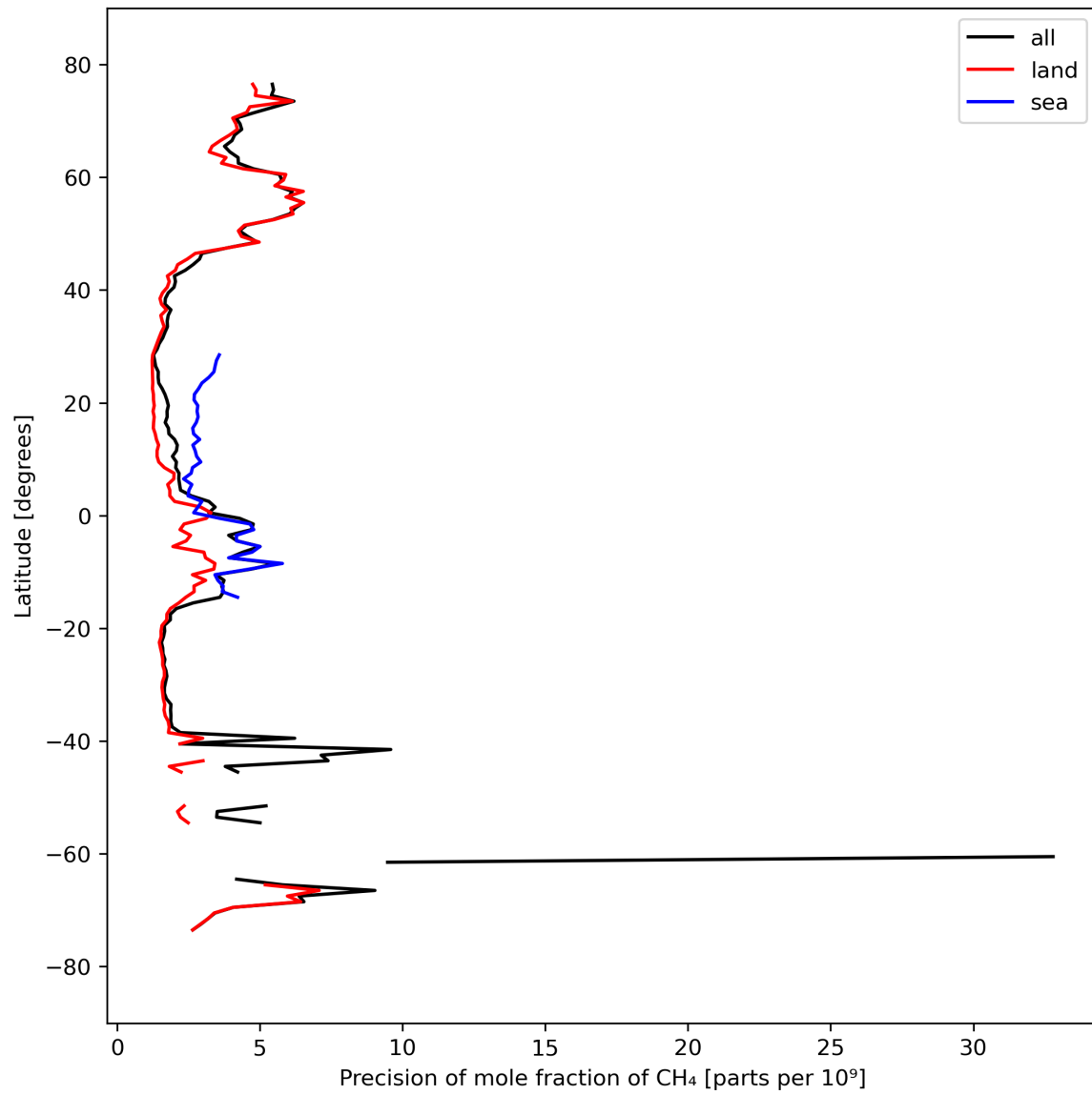
Figure 13: Zonal average of “Precision of mole fraction of \text{CH}_4 ” for 2024-03-21 to 2024-03-22.
