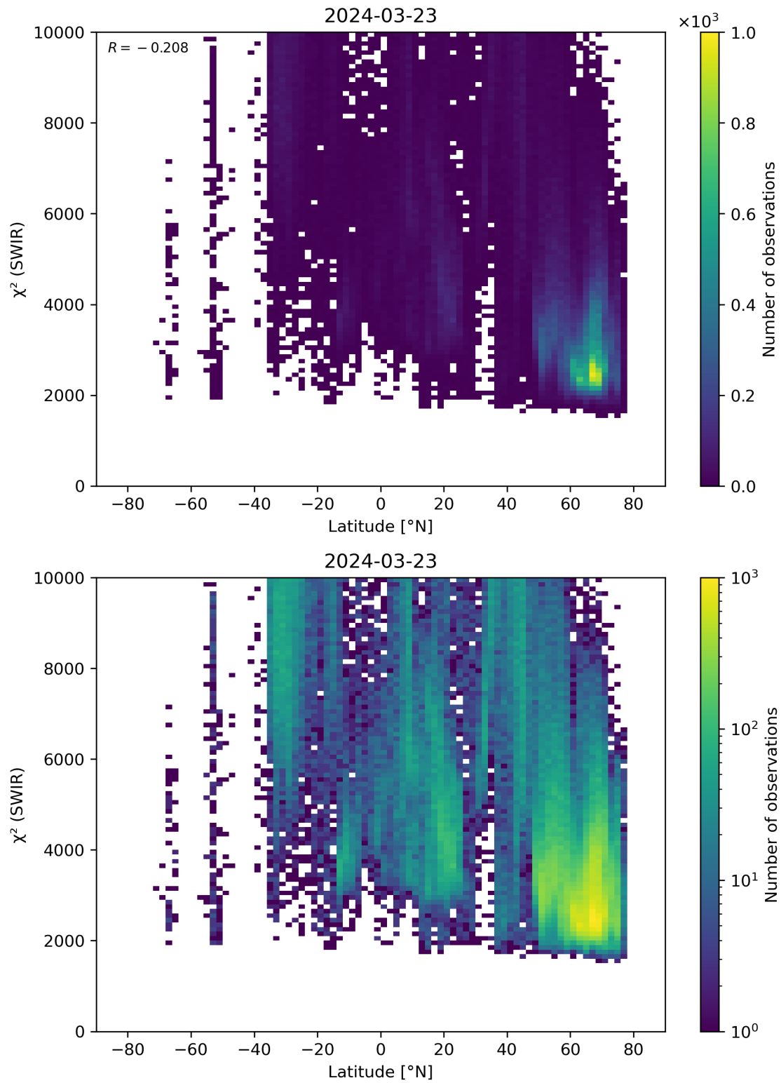
Figure 54: Scatter density plot of “Latitude” against “ \chi^2 (SWIR)” for 2024-03-23 to 2024-03-24.
