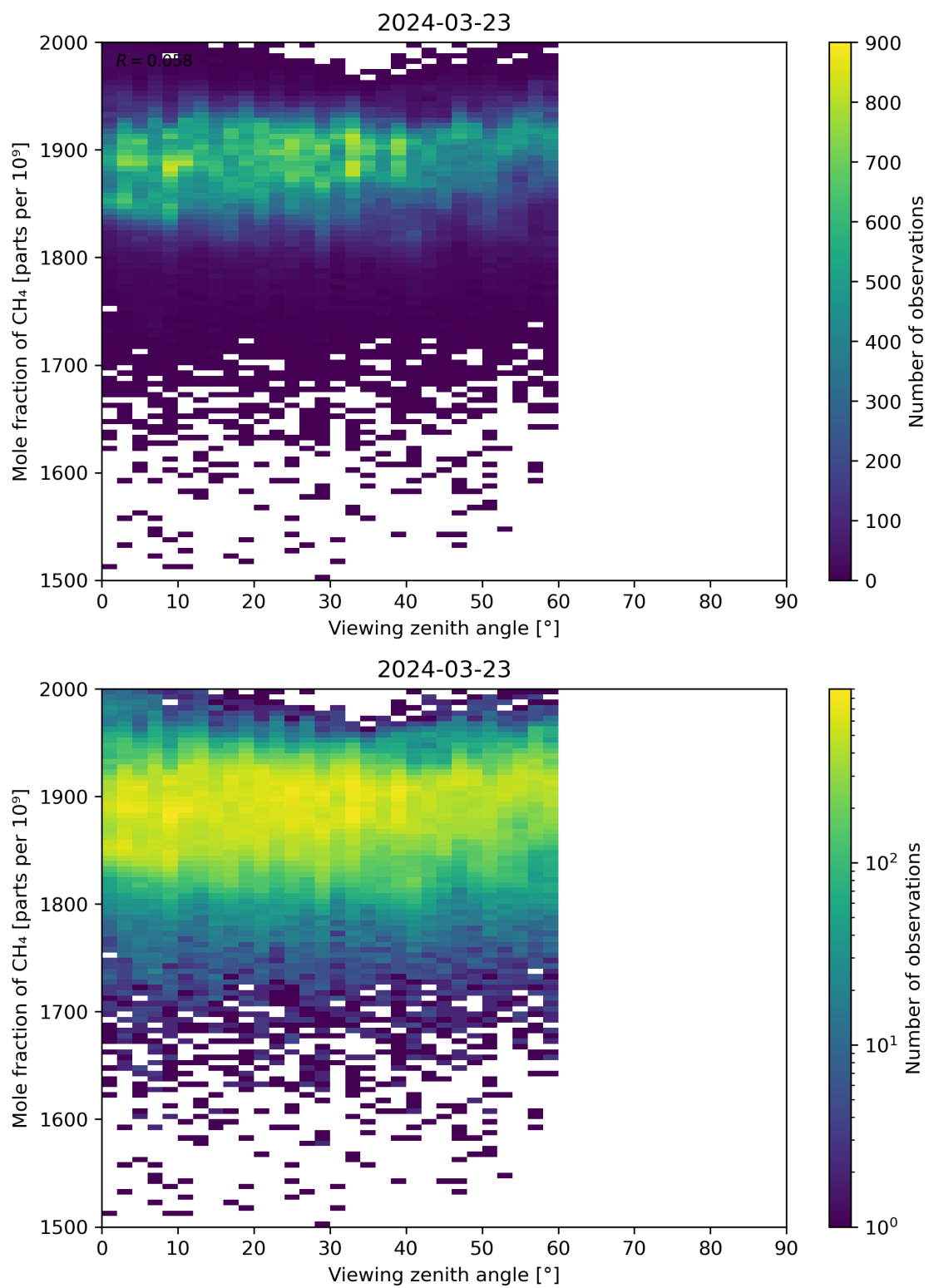
Figure 110: Scatter density plot of “Viewing zenith angle” against “Mole fraction of CH 4 ” for 2024-03-23 to 2024-03-24.
