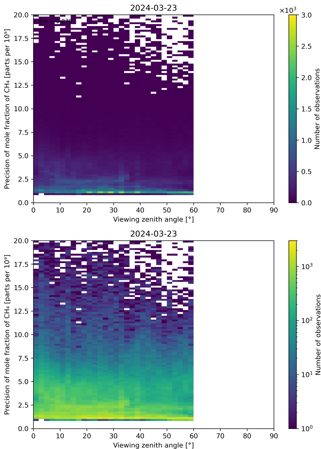
Figure 112: Scatter density plot of “Viewing zenith angle” against “Precision of mole fraction of CH 4 ” for 2024-03-23 to 2024-03-24.
