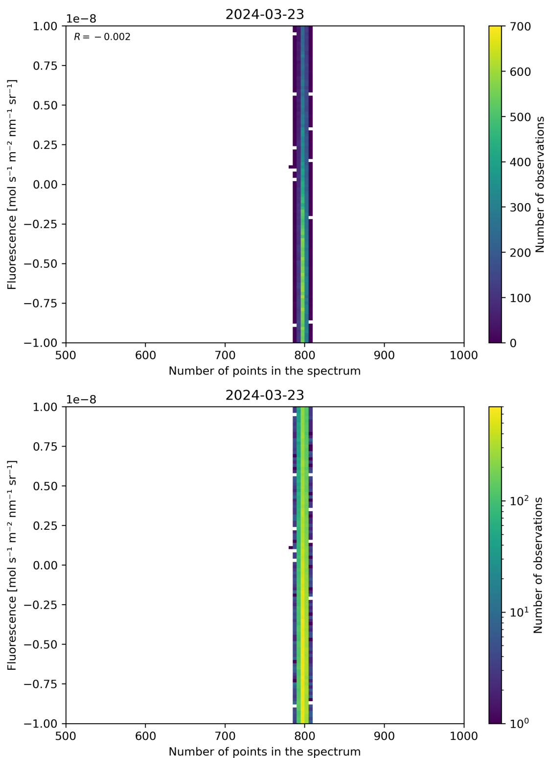
Figure 91: Scatter density plot of “Number of points in the spectrum” against “Fluorescence” for 2024-03-23 to 2024-03-24.
