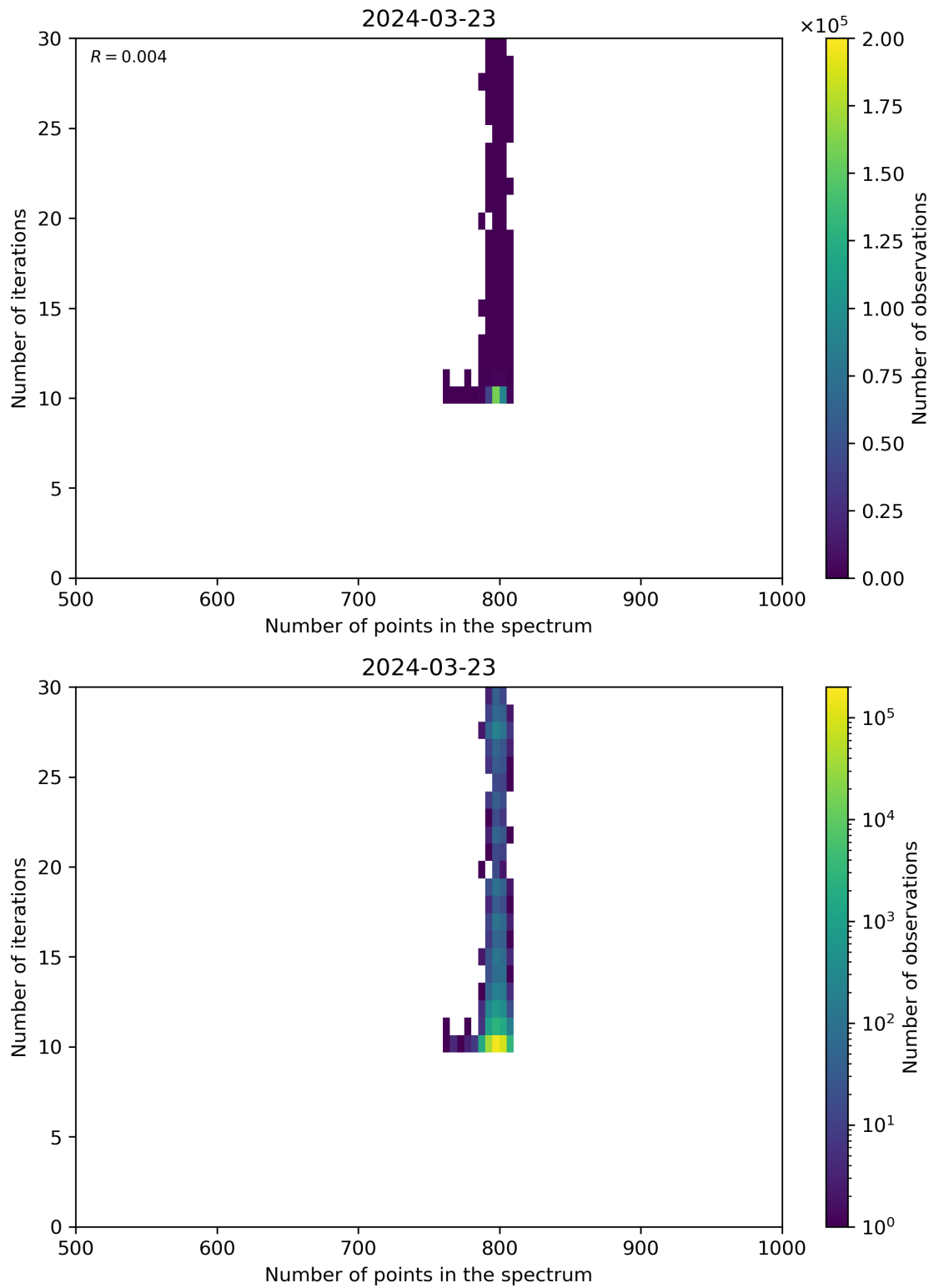
Figure 92: Scatter density plot of “Number of points in the spectrum” against “Number of iterations” for 2024-03-23 to 2024-03-24.
