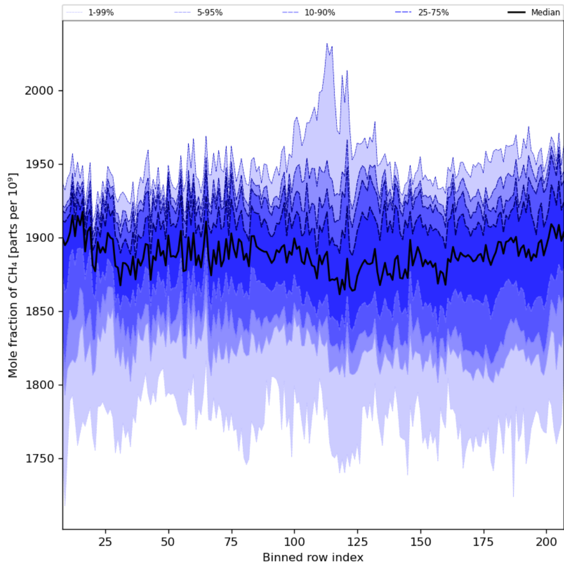
Figure 34: Along track statistics of “Mole fraction of CH 4 ” for 2024-03-23 to 2024-03-24
