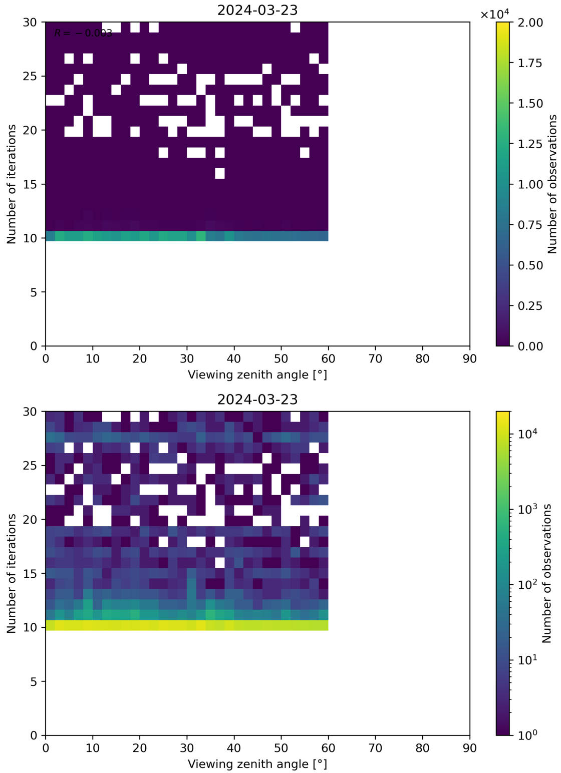
Figure 113: Scatter density plot of “Viewing zenith angle” against “Number of iterations” for 2024-03-23 to 2024-03-24.
