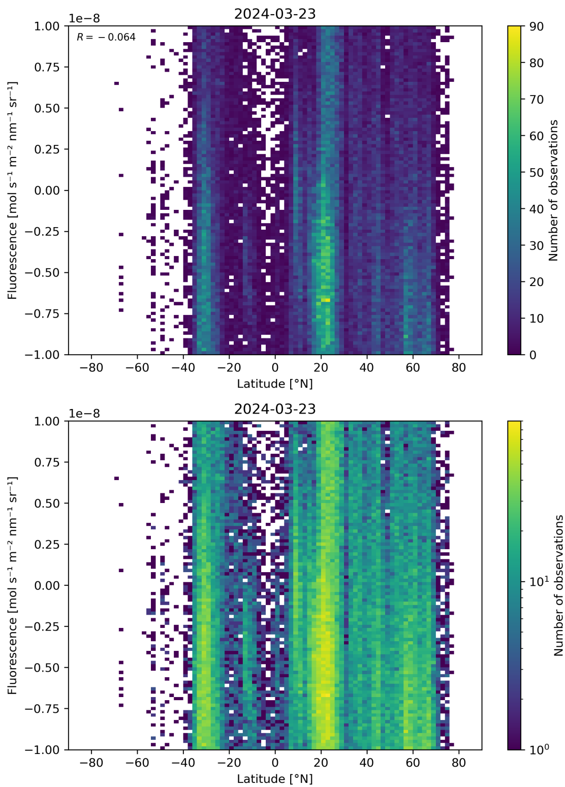
Figure 56: Scatter density plot of “Latitude” against “Fluorescence” for 2024-03-23 to 2024-03-24.
