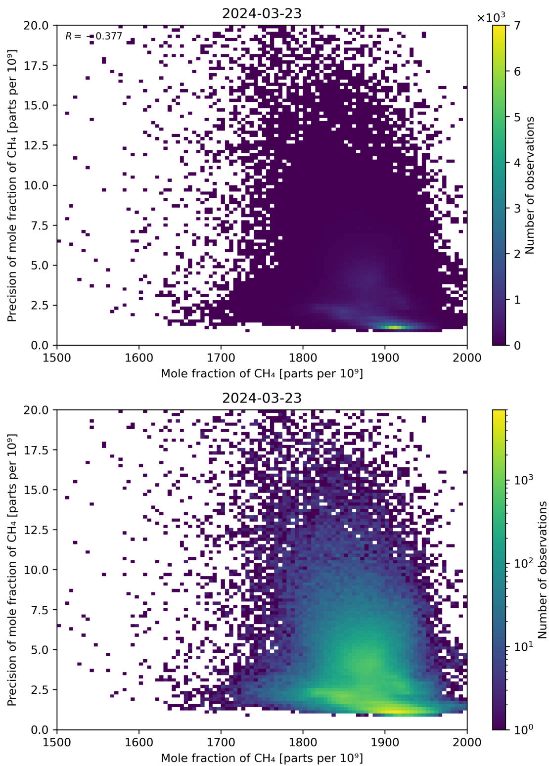
Figure 75: Scatter density plot of “Mole fraction of CH 4 ” against “Precision of mole fraction of CH 4 ” for 2024-03-23 to 2024-03-24.
