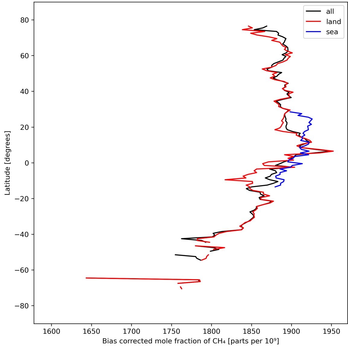
Figure 14: Zonal average of “Bias corrected mole fraction of CH 4 ” for 2024-03-23 to 2024-03-24.
