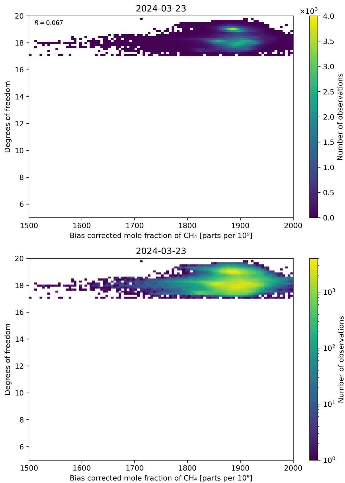
Figure 65: Scatter density plot of “Bias corrected mole fraction of CH 4 ” against “Degrees of freedom” for 2024-03-23 to 2024-03-24.
