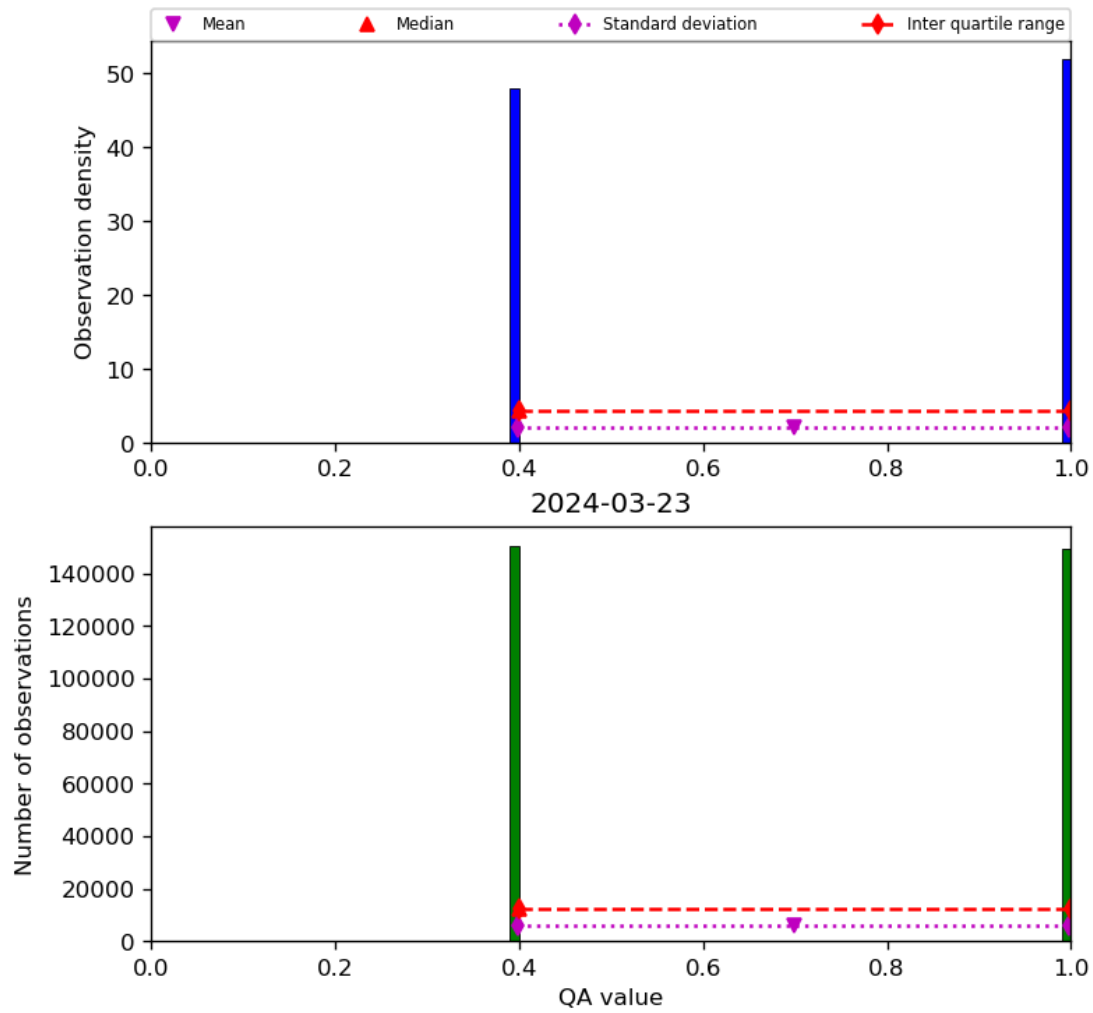
Figure 22: Histogram of “QA value” for 2024-03-23 to 2024-03-24
