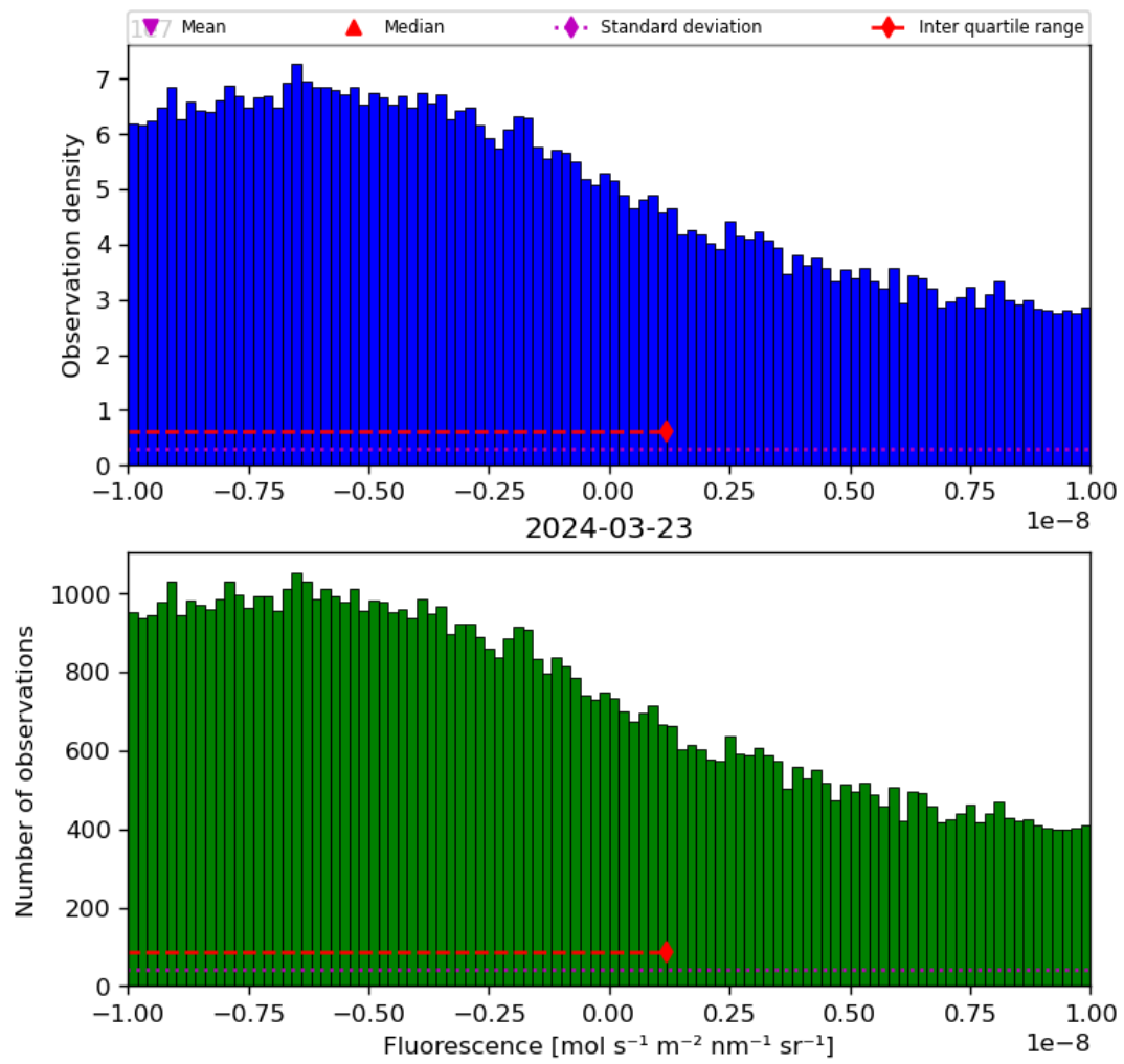
Figure 32: Histogram of “Fluorescence” for 2024-03-23 to 2024-03-24
