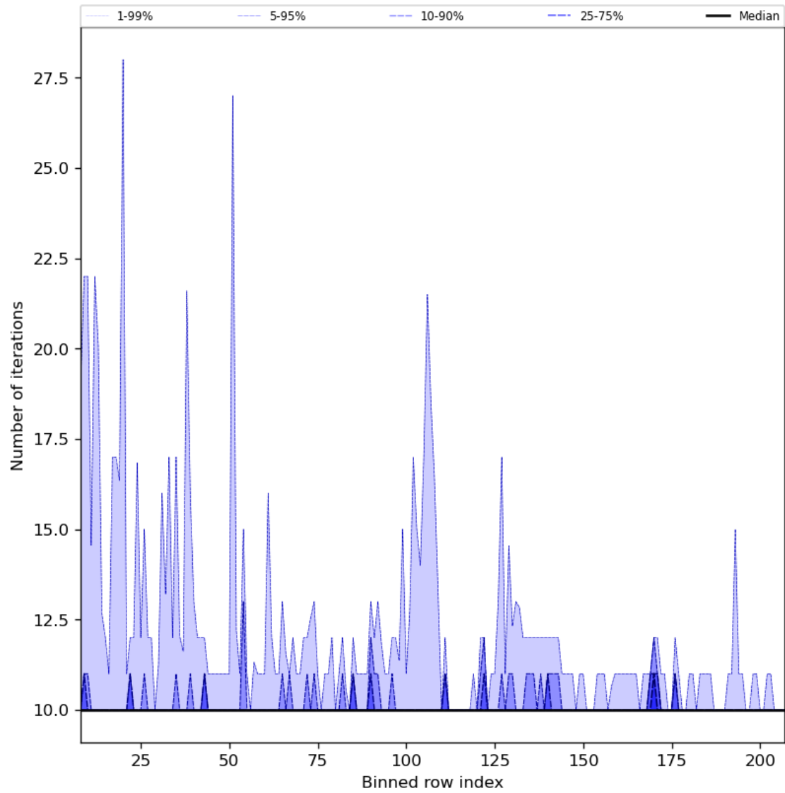
Figure 42: Along track statistics of “Number of iterations” for 2024-03-23 to 2024-03-24
