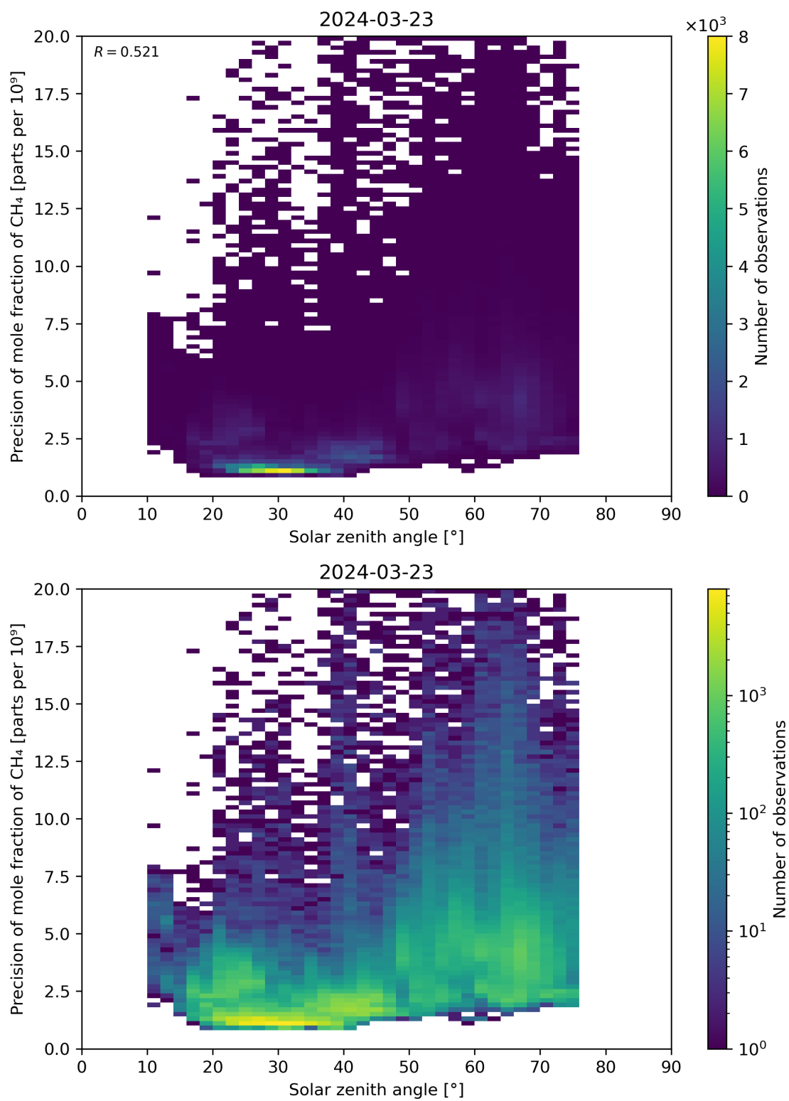
Figure 101: Scatter density plot of “Solar zenith angle” against “Precision of mole fraction of \text{CH}_4 ” for 2024-03-23 to 2024-03-24.
