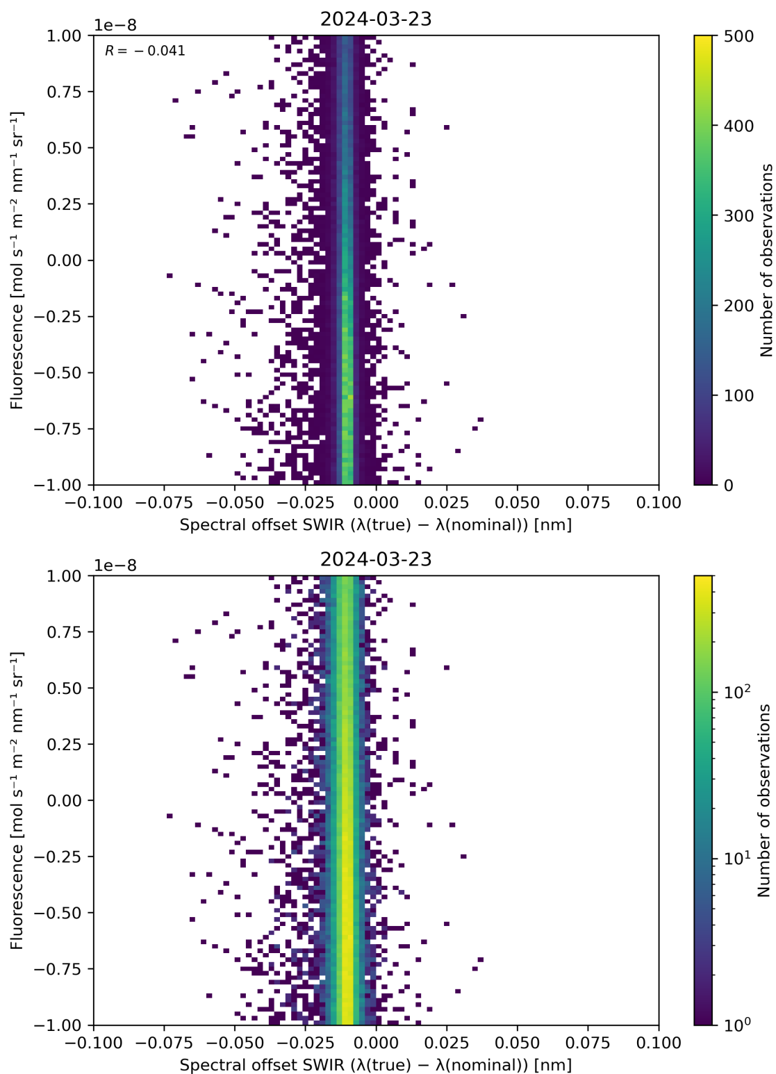
Figure 120: Scatter density plot of “Spectral offset SWIR ( \lambda(\text{true}) - \lambda(\text{nominal}) )” against “Fluorescence” for 2024-03-23 to 2024-03-24.
