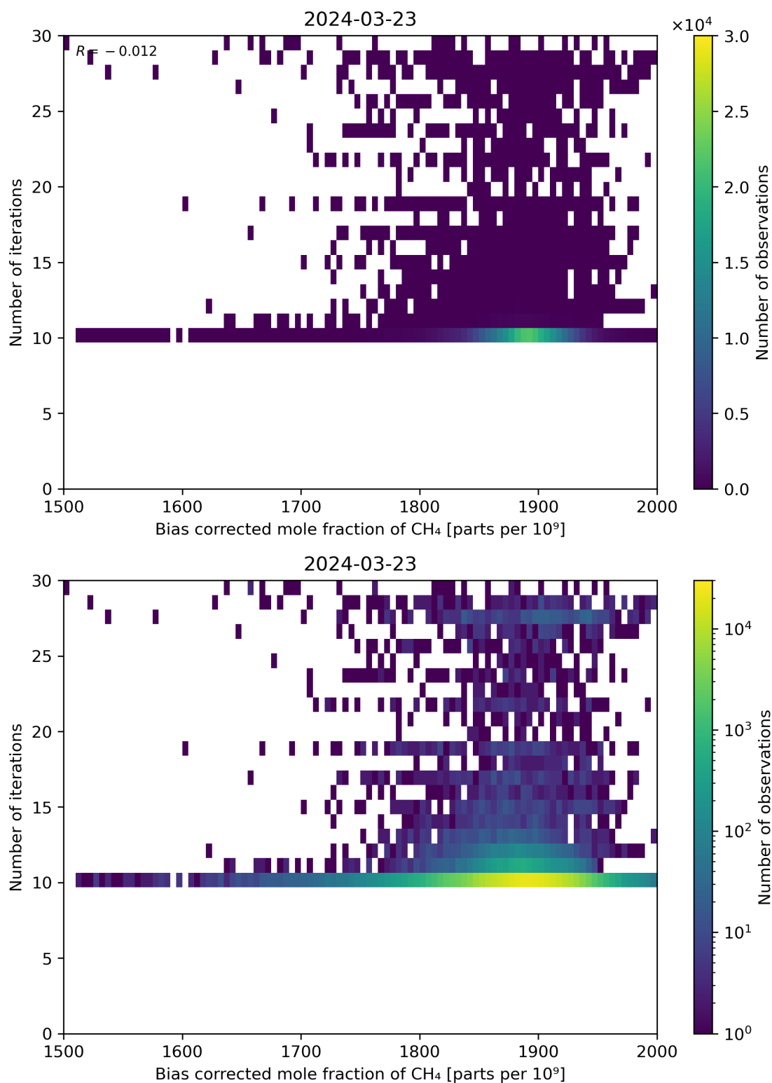
Figure 67: Scatter density plot of “Bias corrected mole fraction of CH 4 ” against “Number of iterations” for 2024-03-23 to 2024-03-24.
