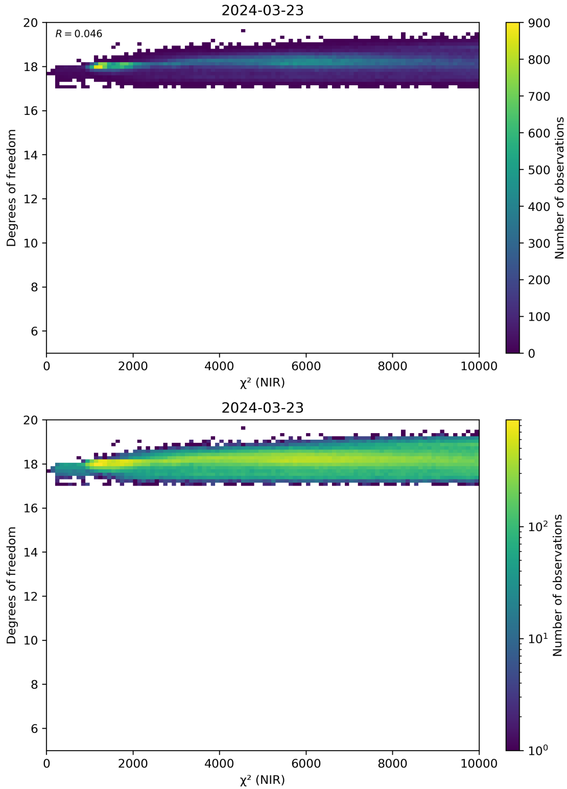
Figure 44: Scatter density plot of “ \chi^2 (NIR)” against “Degrees of freedom” for 2024-03-23 to 2024-03-24.
