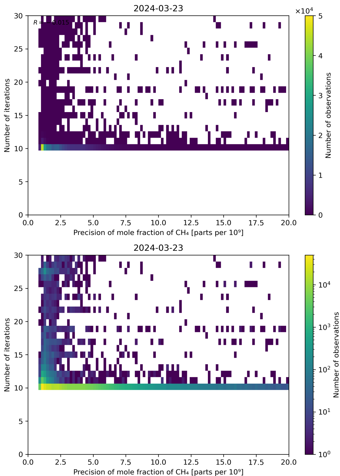
Figure 83: Scatter density plot of “Precision of mole fraction of CH 4 ” against “Number of iterations” for 2024-03-23 to 2024-03-24.
