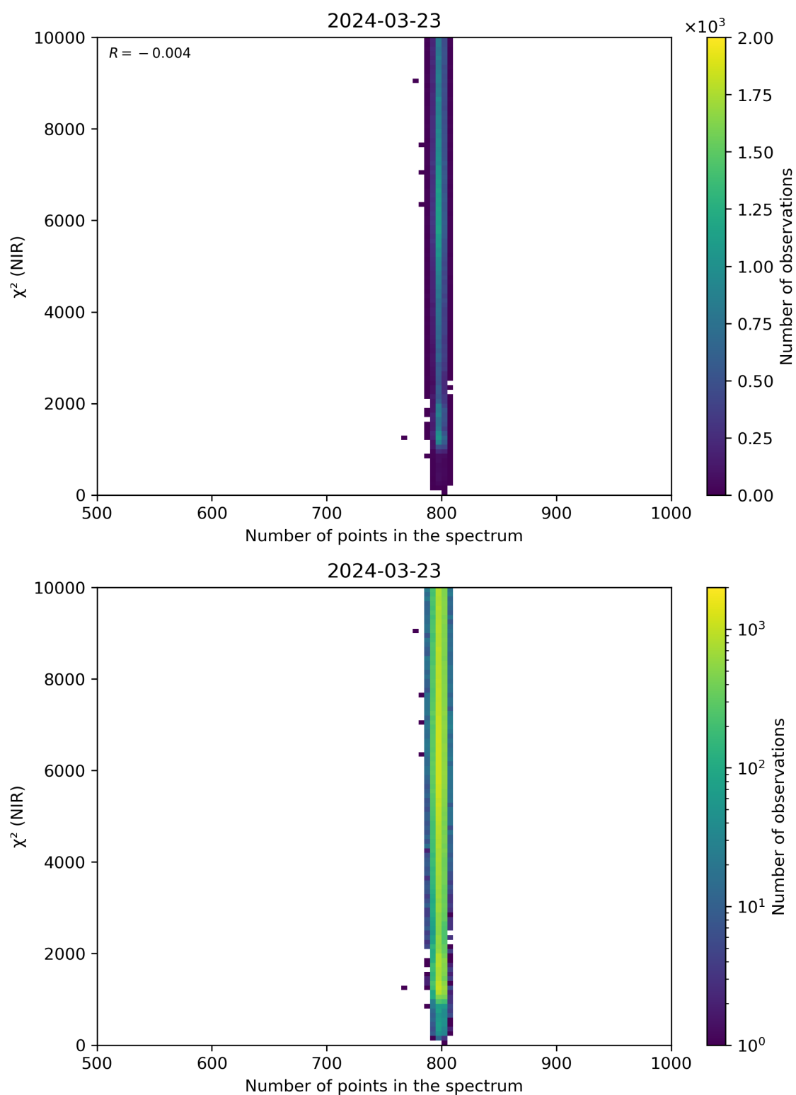
Figure 88: Scatter density plot of “Number of points in the spectrum” against “ \chi^2 (NIR)” for 2024-03-23 to 2024-03-24.
