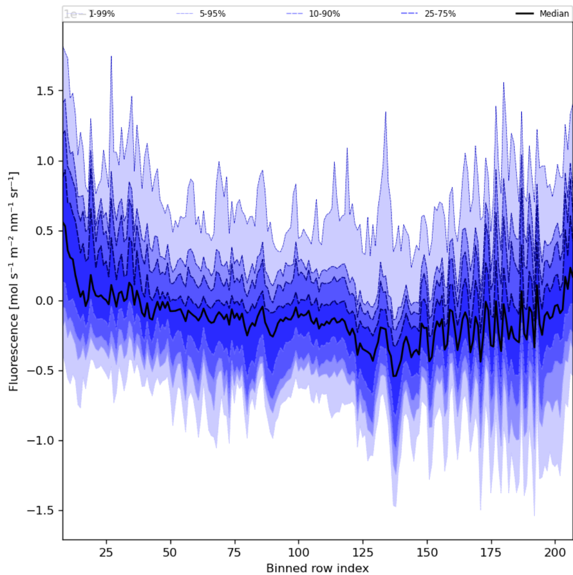
Figure 43: Along track statistics of “Fluorescence” for 2024-03-23 to 2024-03-24
