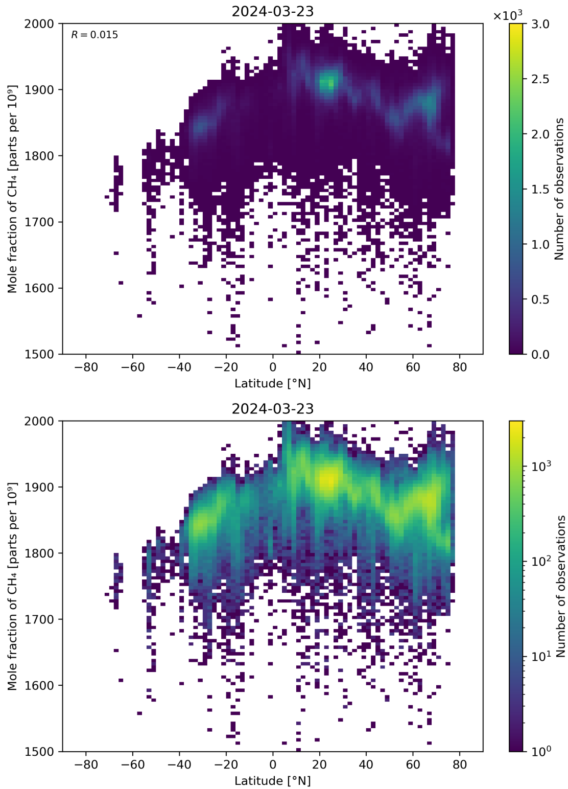
Figure 57: Scatter density plot of “Latitude” against “Mole fraction of \text{CH}_4 ” for 2024-03-23 to 2024-03-24.
