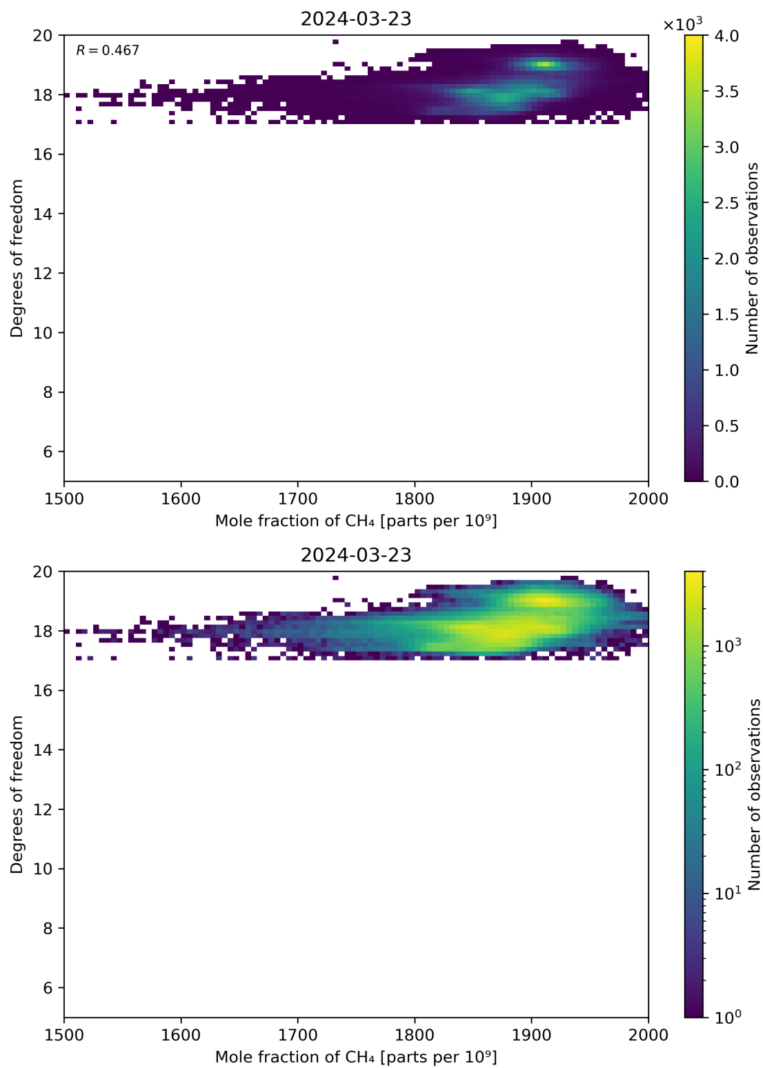
Figure 72: Scatter density plot of “Mole fraction of CH 4 ” against “Degrees of freedom” for 2024-03-23 to 2024-03-24.
