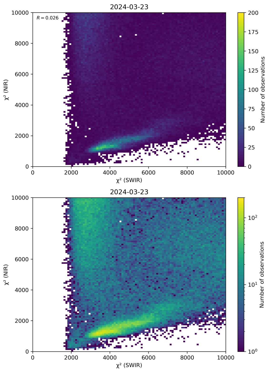
Figure 47: Scatter density plot of “ \chi^2 (SWIR)” against “ \chi^2 (NIR)” for 2024-03-23 to 2024-03-24.
