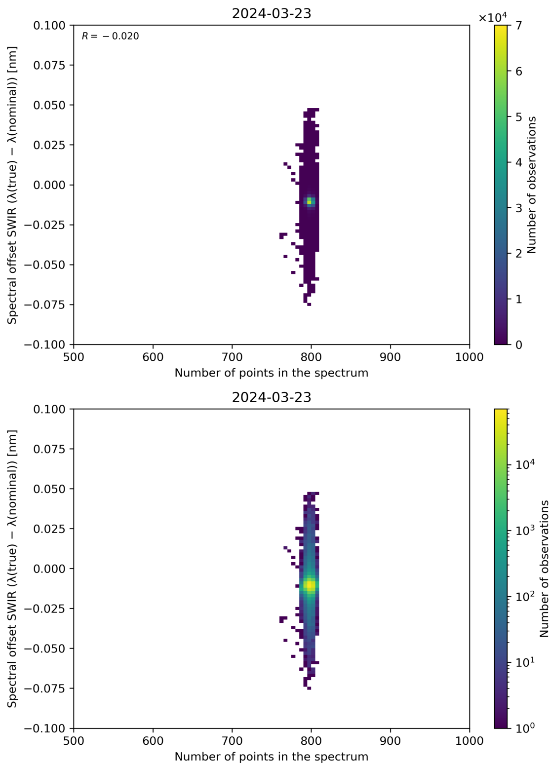
Figure 93: Scatter density plot of “Number of points in the spectrum” against “Spectral offset SWIR ( \lambda(\text{true}) - \lambda(\text{nominal}) )” for 2024-03-23 to 2024-03-24.
