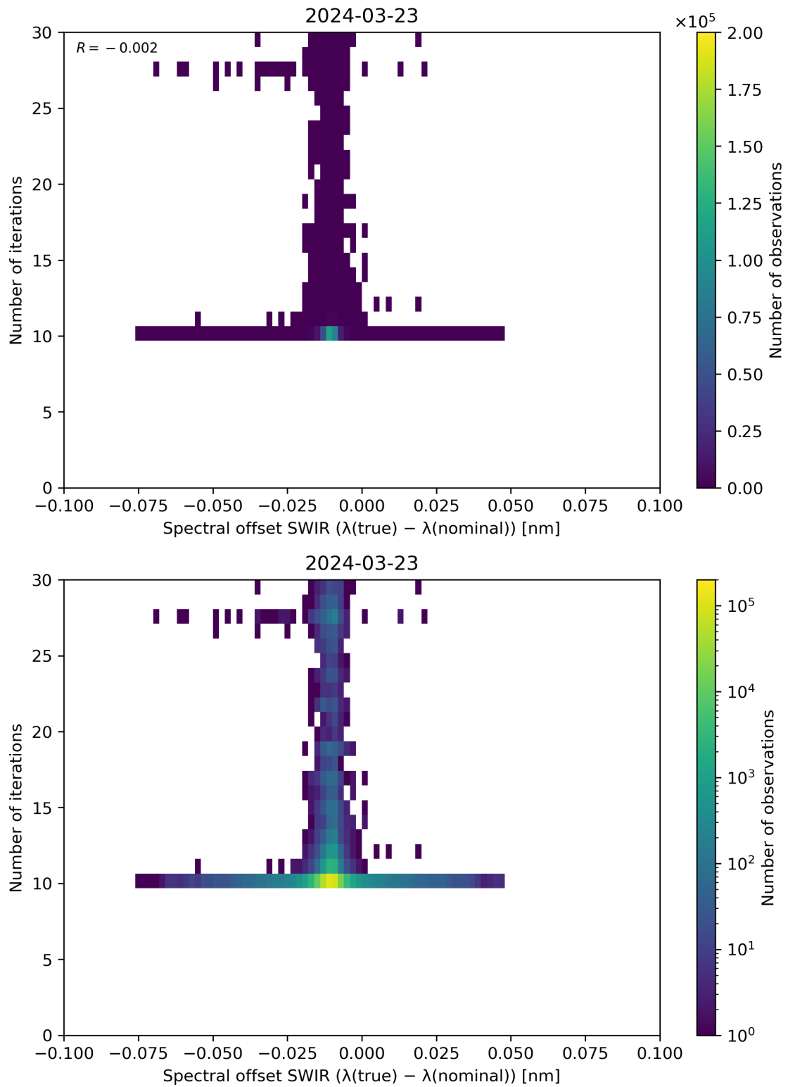
Figure 121: Scatter density plot of “Spectral offset SWIR ( \lambda(\text{true}) - \lambda(\text{nominal}) )” against “Number of iterations” for 2024-03-23 to 2024-03-24.
