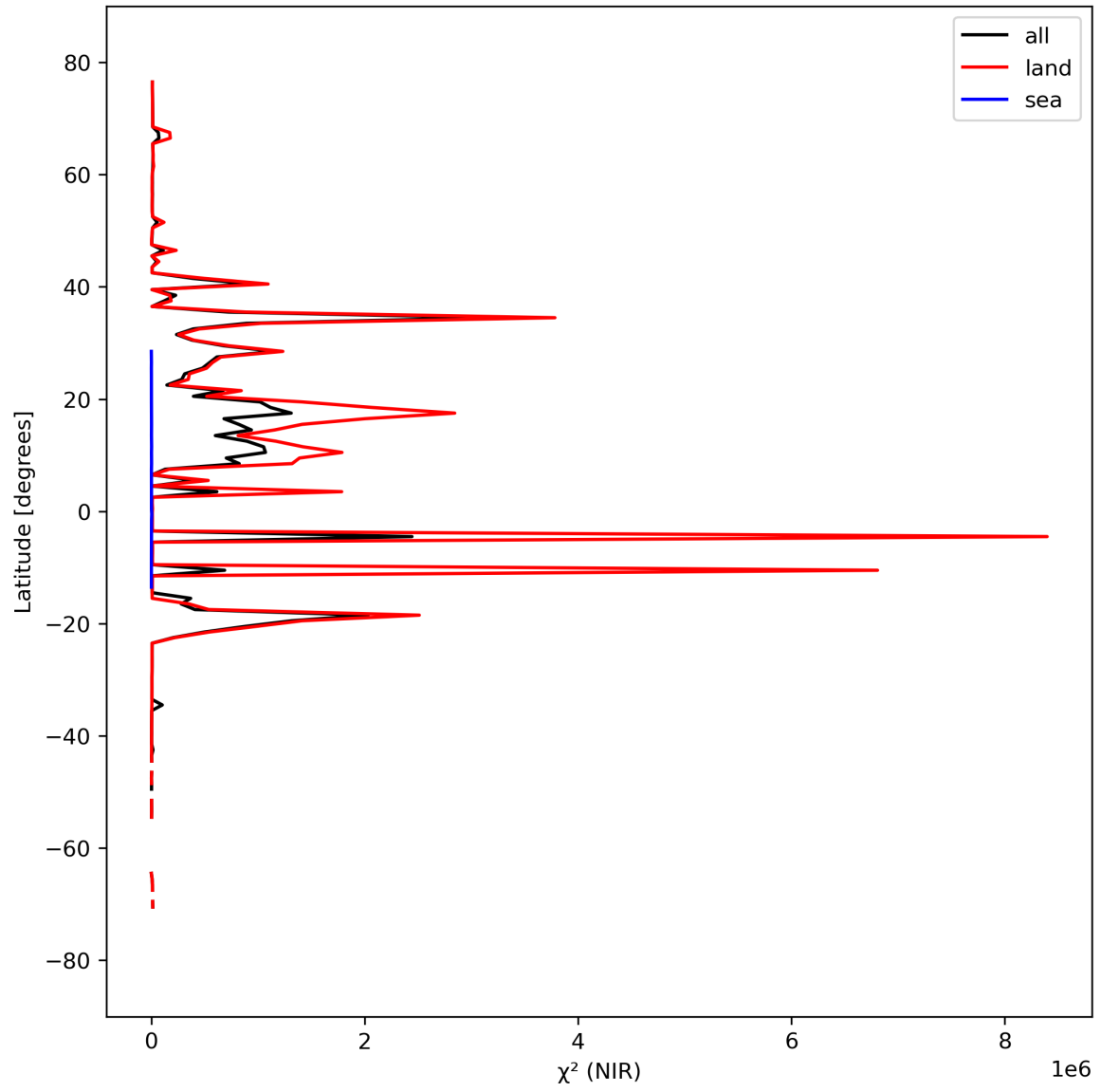
Figure 18: Zonal average of “ \chi^2 (NIR)” for 2024-03-23 to 2024-03-24.
