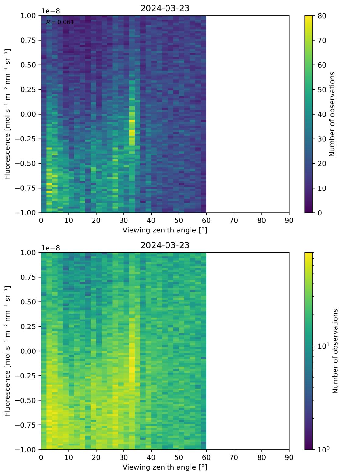
Figure 108: Scatter density plot of “Viewing zenith angle” against “Fluorescence” for 2024-03-23 to 2024-03-24.
