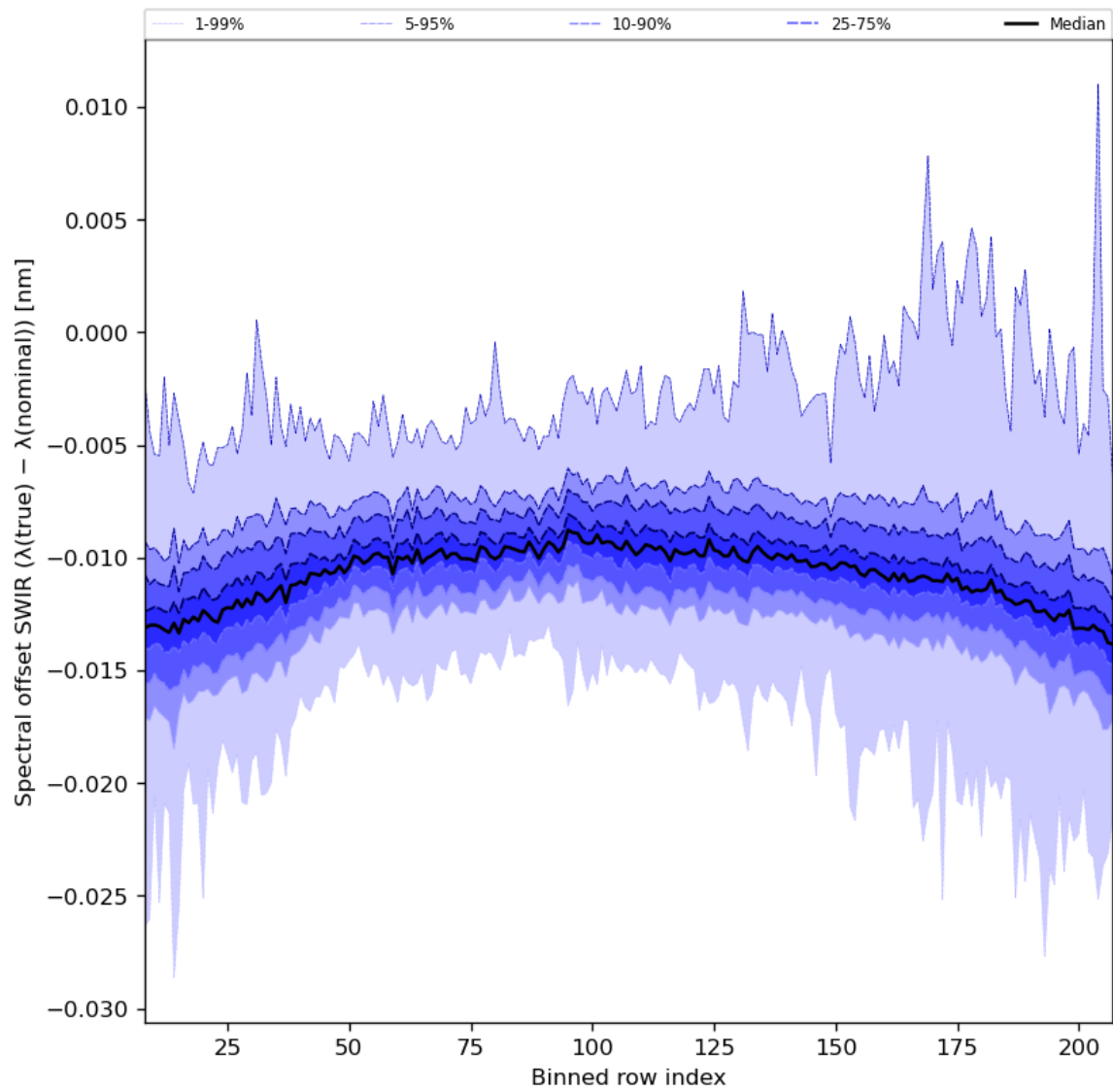
Figure 38: Along track statistics of “Spectral offset SWIR ( \lambda(\text{true}) - \lambda(\text{nominal}) )” for 2024-03-23 to 2024-03-24
