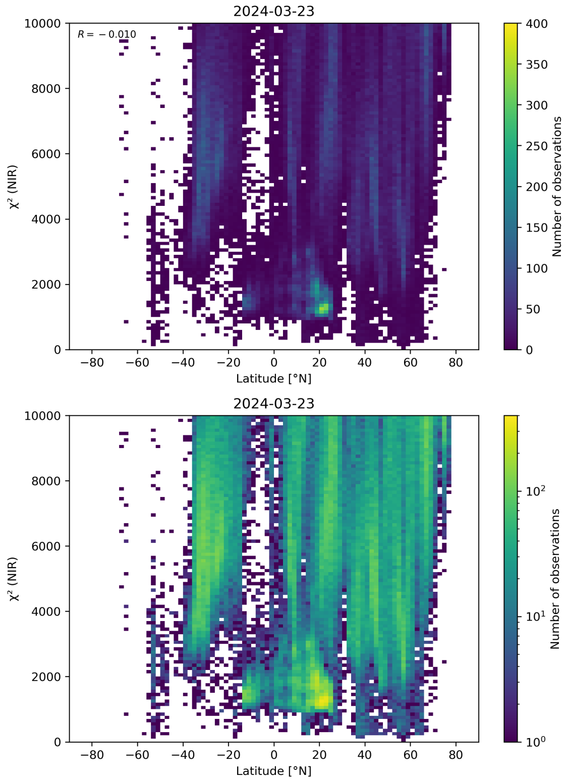
Figure 53: Scatter density plot of “Latitude” against “ \chi^2 (NIR)” for 2024-03-23 to 2024-03-24.
