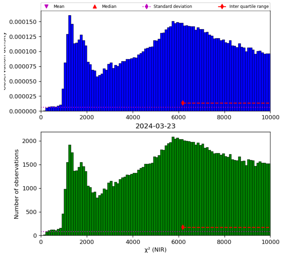
Figure 29: Histogram of “ \chi^2 (NIR)” for 2024-03-23 to 2024-03-24
