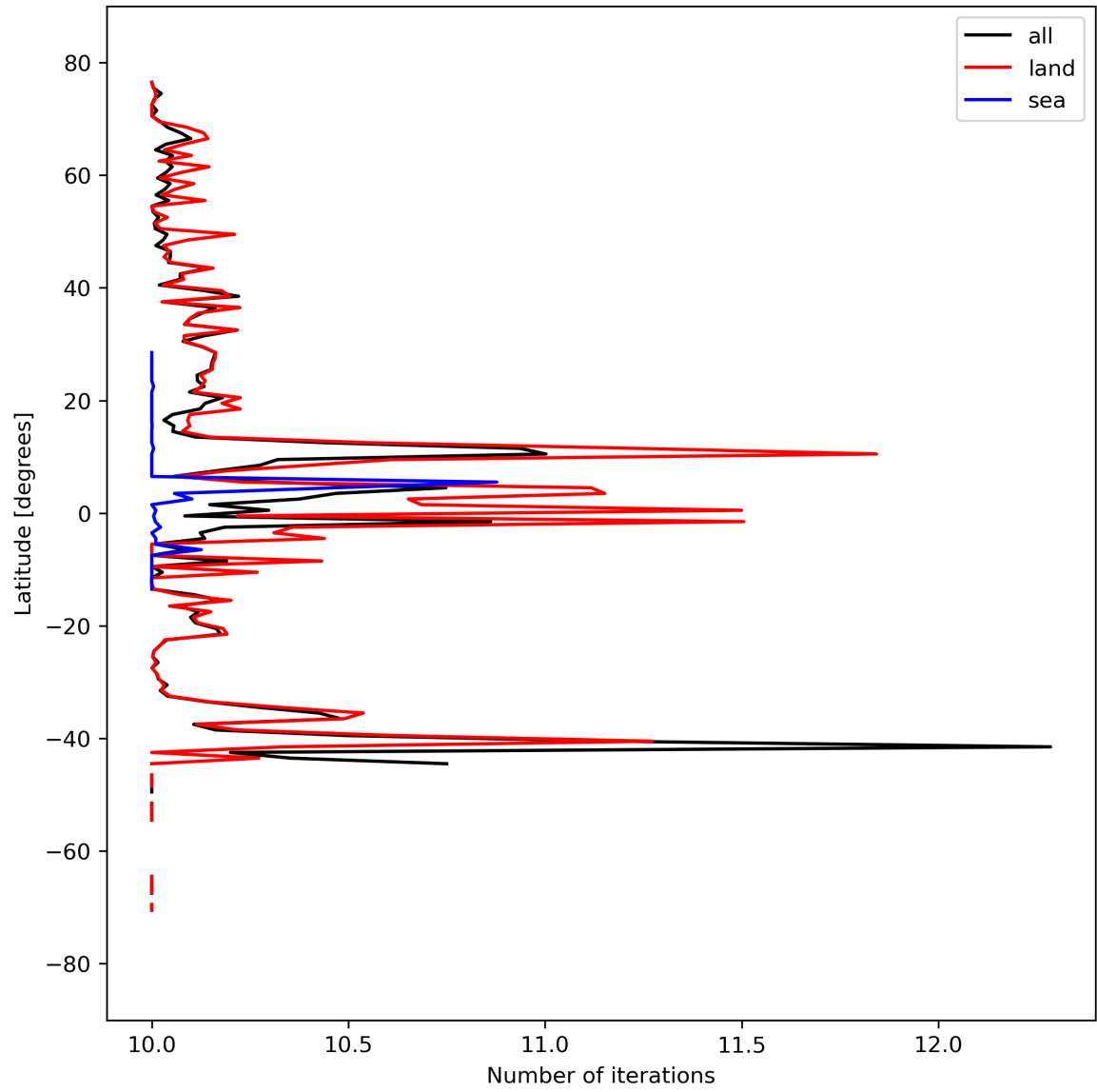
Figure 20: Zonal average of “Number of iterations” for 2024-03-23 to 2024-03-24.
