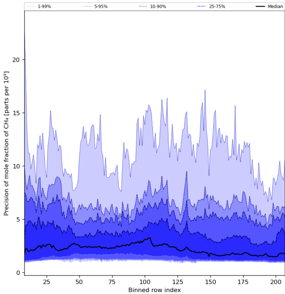
Figure 35: Along track statistics of “Precision of mole fraction of CH 4 ” for 2024-03-23 to 2024-03-24
