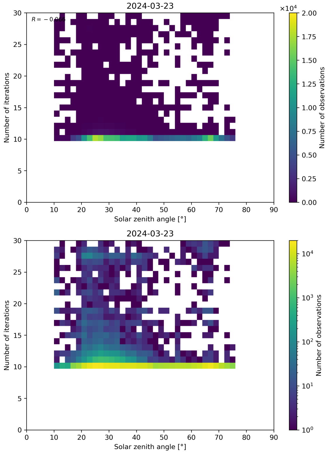
Figure 102: Scatter density plot of “Solar zenith angle” against “Number of iterations” for 2024-03-23 to 2024-03-24.
