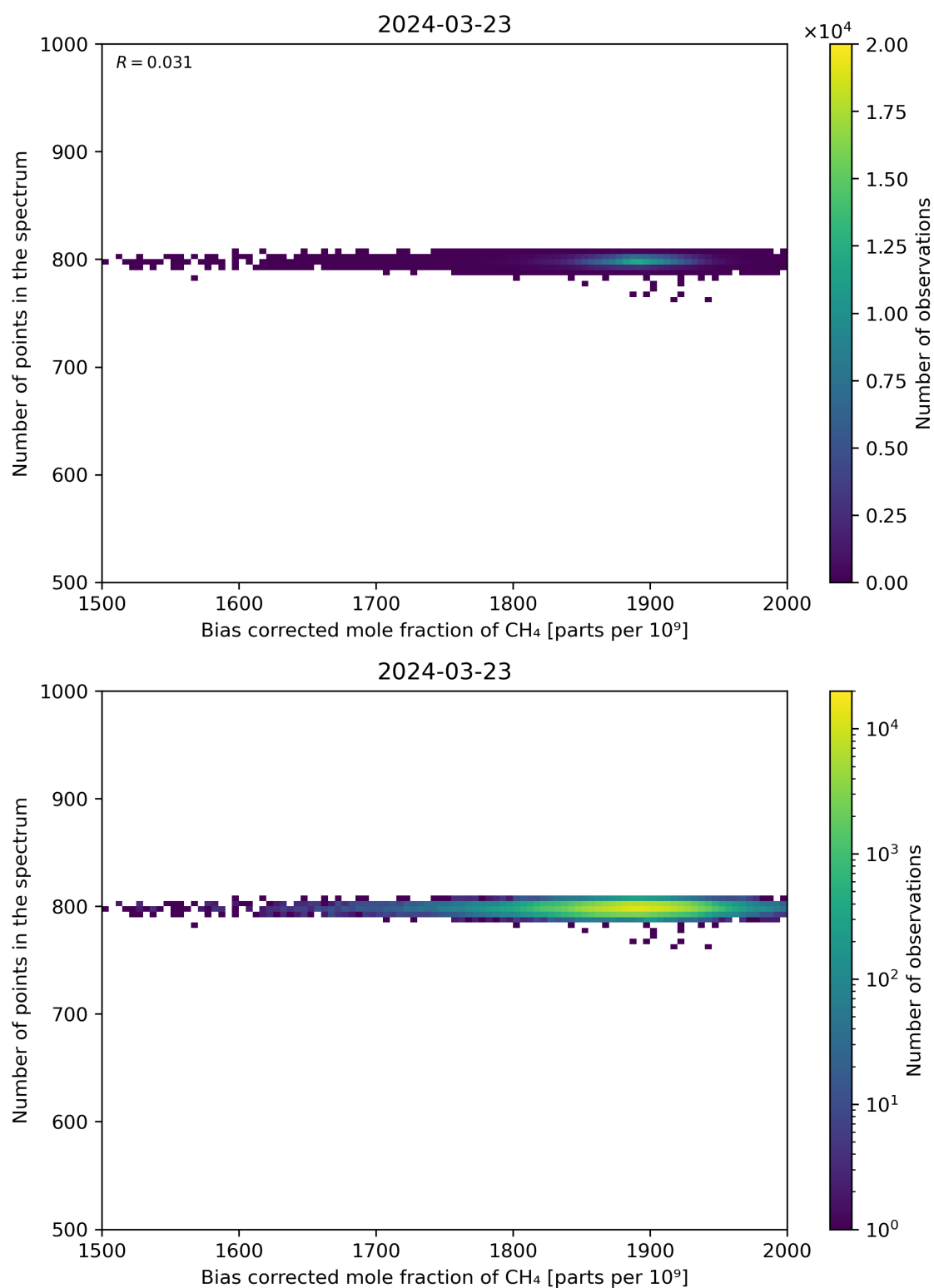
Figure 68: Scatter density plot of “Bias corrected mole fraction of CH 4 ” against “Number of points in the spectrum” for 2024-03-23 to 2024-03-24.
