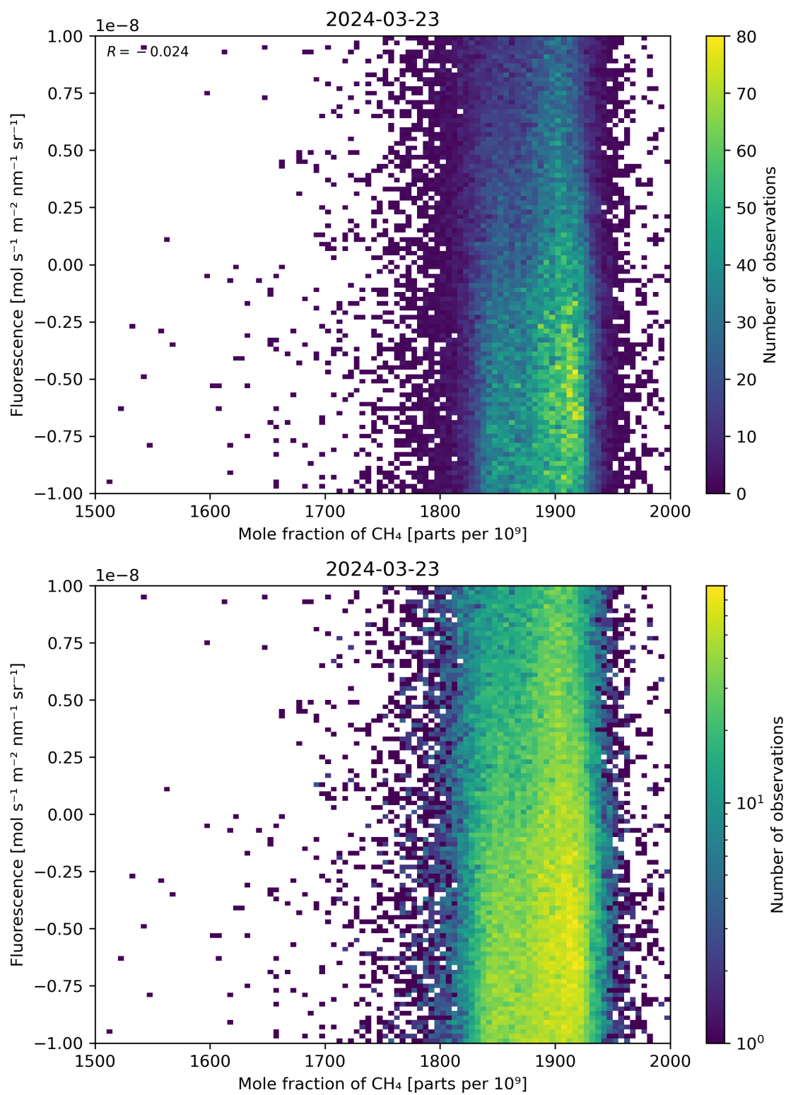
Figure 73: Scatter density plot of “Mole fraction of \text{CH}_4 ” against “Fluorescence” for 2024-03-23 to 2024-03-24.
