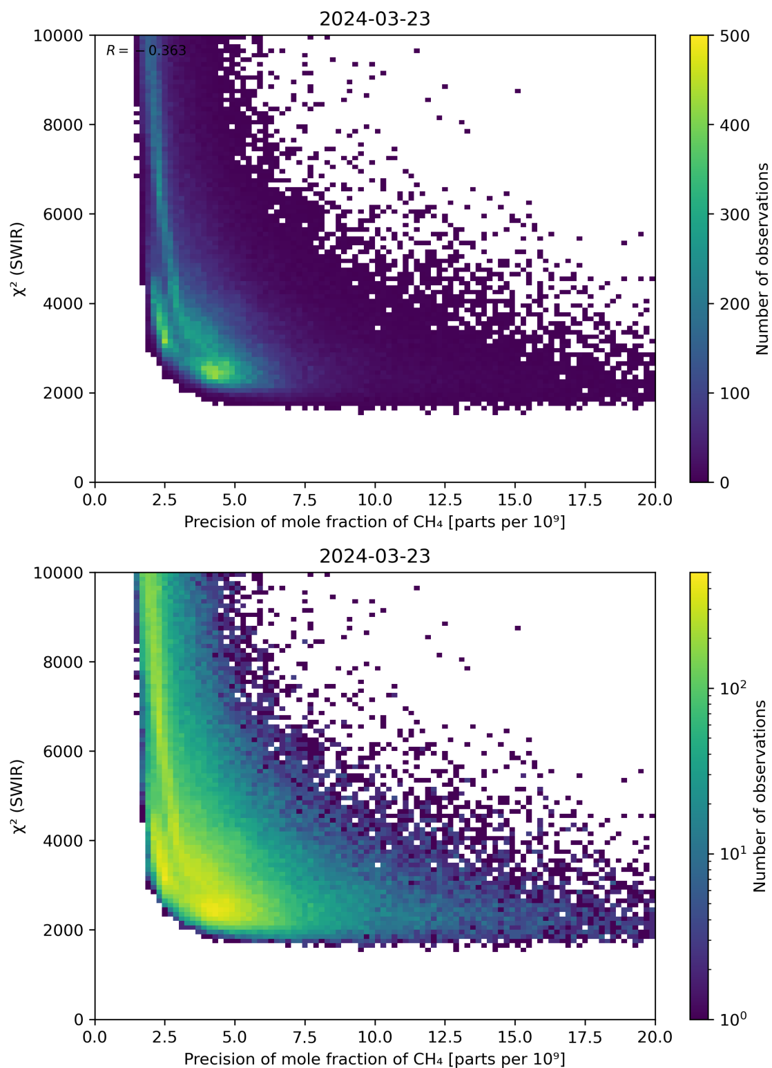
Figure 79: Scatter density plot of “Precision of mole fraction of CH 4 ” against “ \chi^2 (SWIR)” for 2024-03-23 to 2024-03-24.
