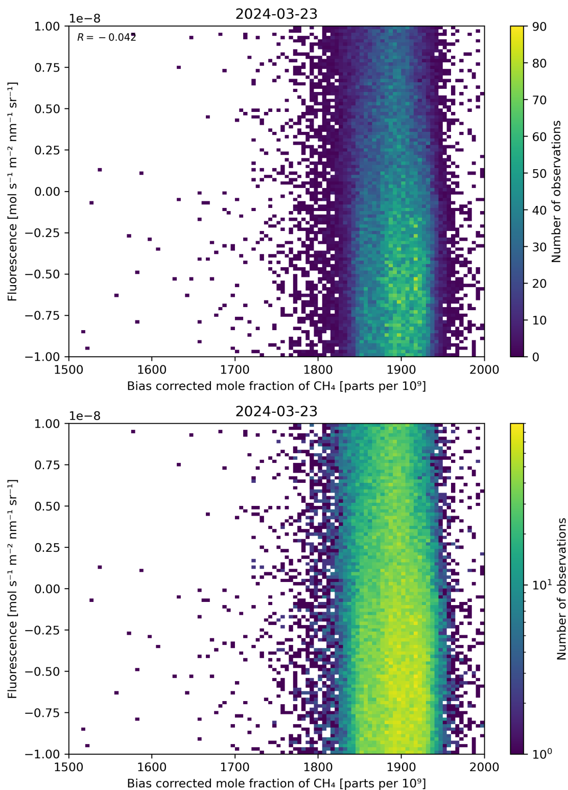
Figure 66: Scatter density plot of “Bias corrected mole fraction of CH 4 ” against “Fluorescence” for 2024-03-23 to 2024-03-24.
