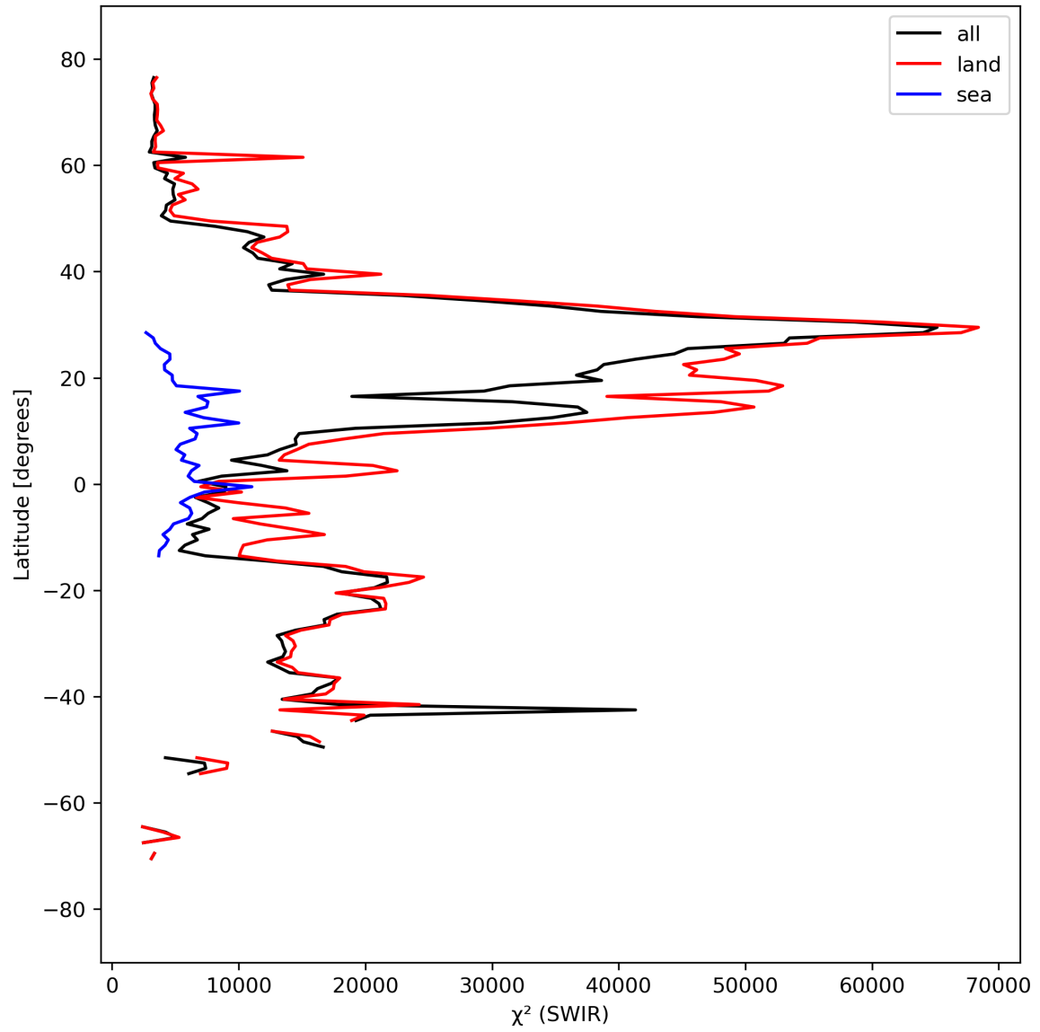
Figure 17: Zonal average of “ \chi^2 (SWIR)” for 2024-03-23 to 2024-03-24.
