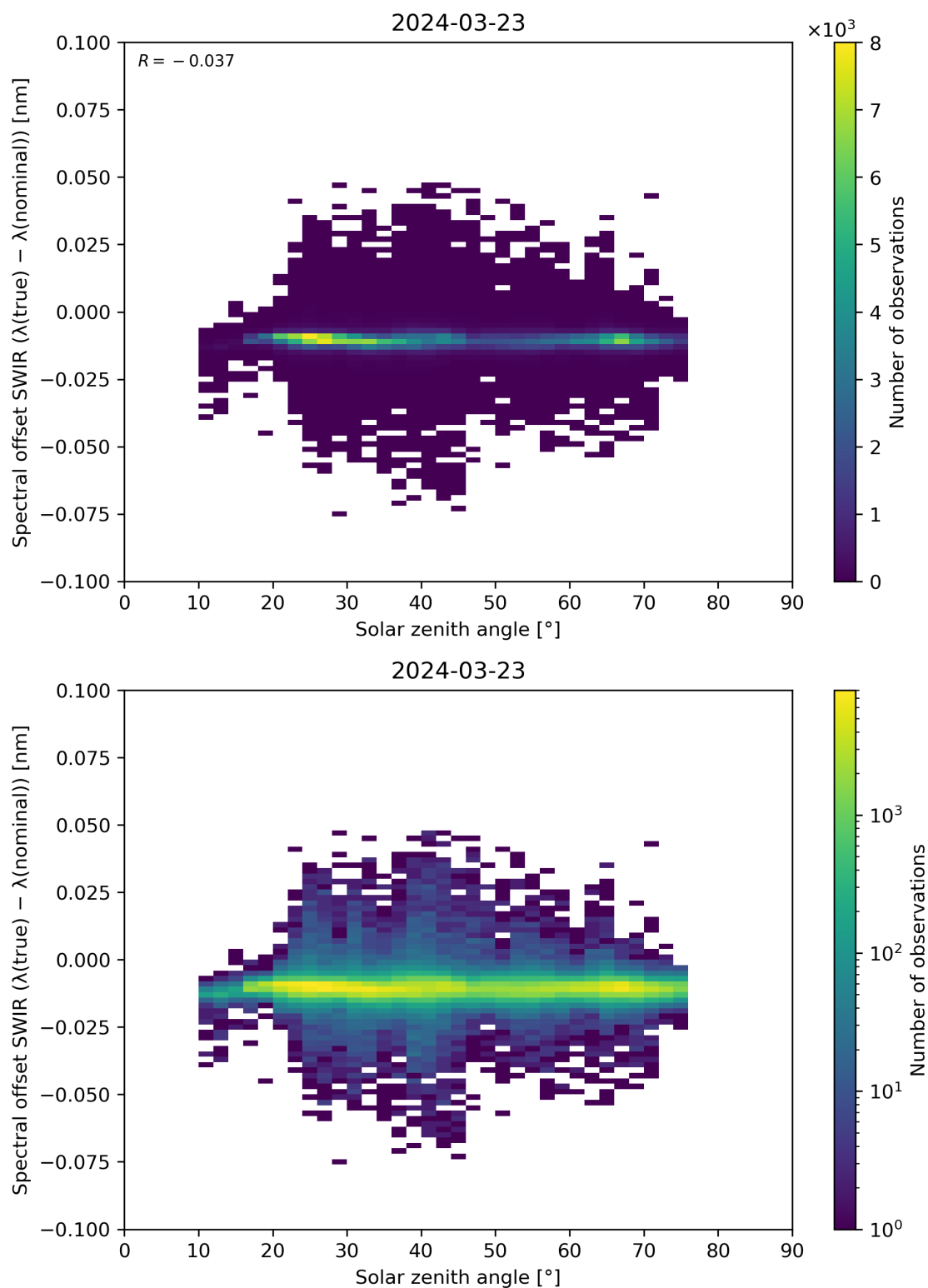
Figure 104: Scatter density plot of “Solar zenith angle” against “Spectral offset SWIR ( \lambda(\text{true}) - \lambda(\text{nominal}) )” for 2024-03-23 to 2024-03-24.
