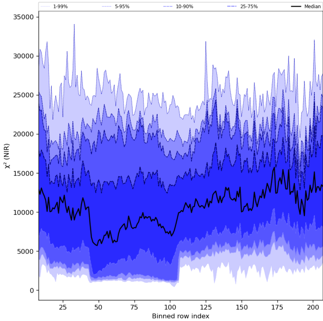
Figure 40: Along track statistics of “ \chi^2 (NIR)” for 2024-03-23 to 2024-03-24
