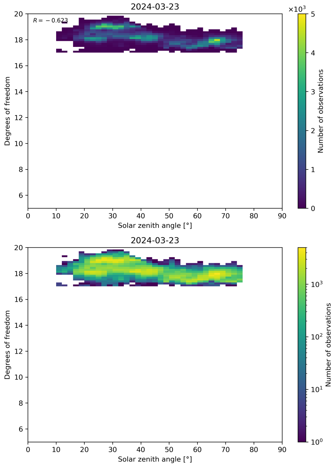
Figure 96: Scatter density plot of “Solar zenith angle” against “Degrees of freedom” for 2024-03-23 to 2024-03-24.
