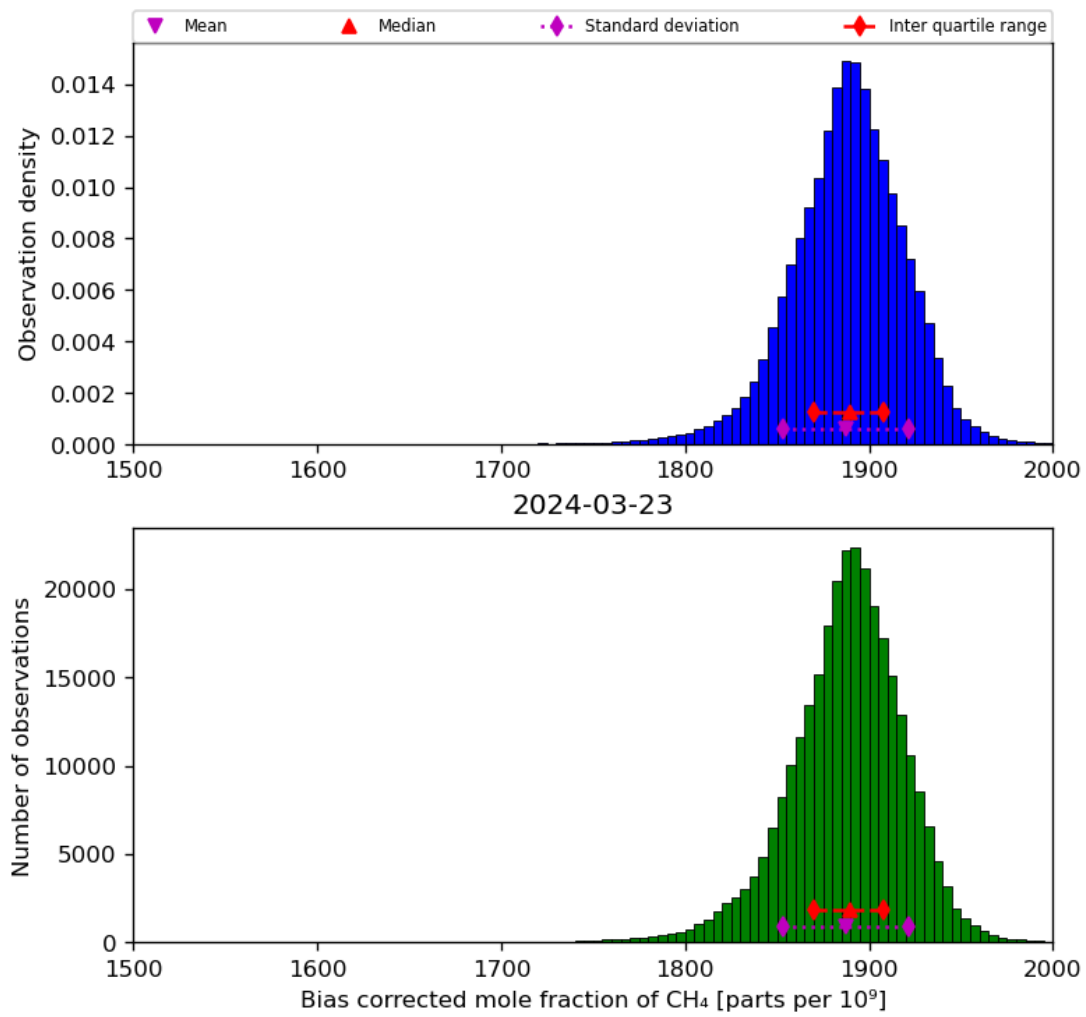
Figure 25: Histogram of “Bias corrected mole fraction of CH 4 ” for 2024-03-23 to 2024-03-24
