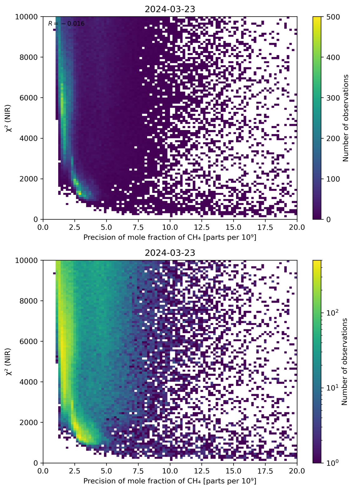
Figure 78: Scatter density plot of “Precision of mole fraction of CH 4 ” against “ \chi^2 (NIR)” for 2024-03-23 to 2024-03-24.
