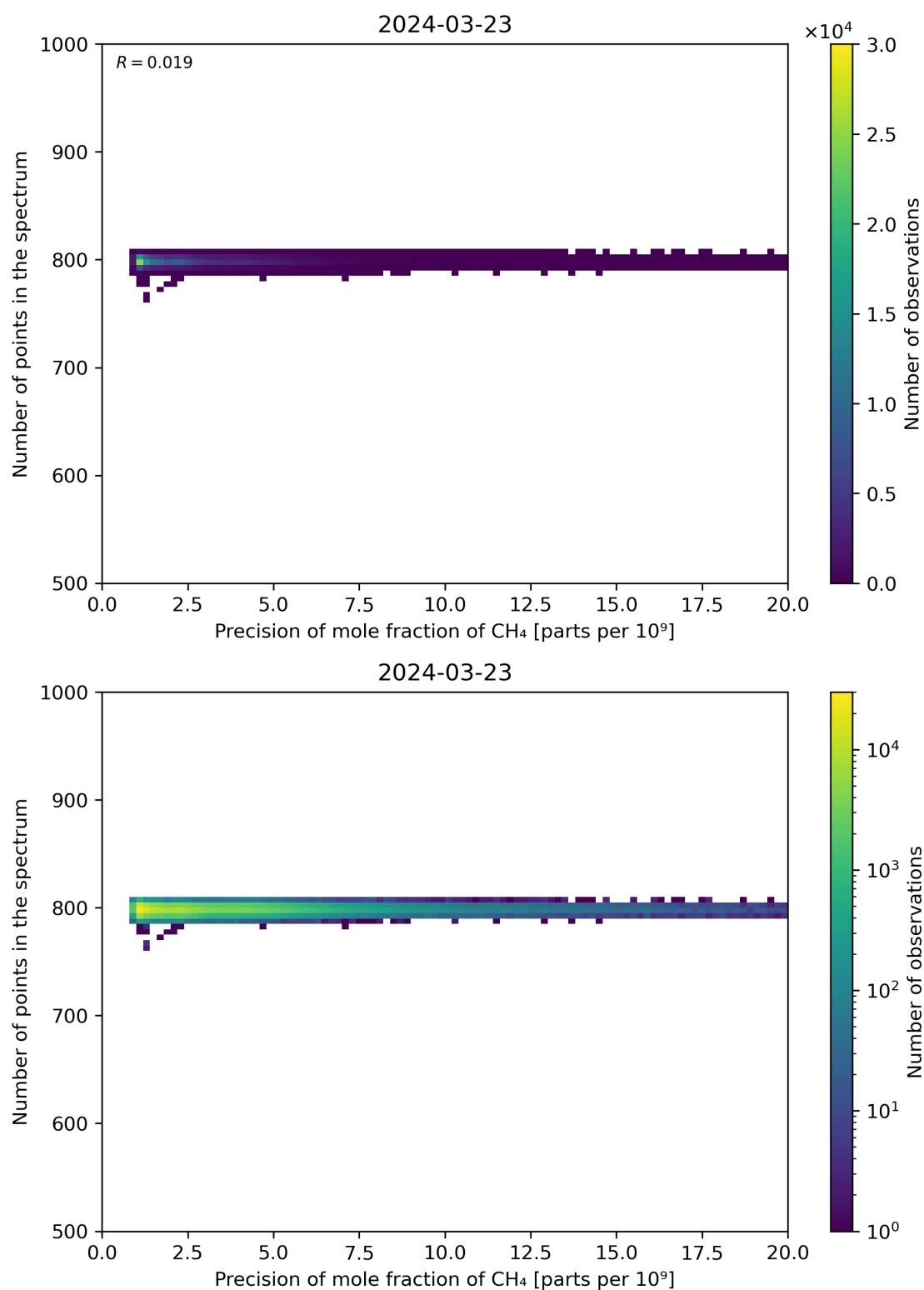
Figure 84: Scatter density plot of “Precision of mole fraction of \text{CH}_4 ” against “Number of points in the spectrum” for 2024-03-23 to 2024-03-24.
