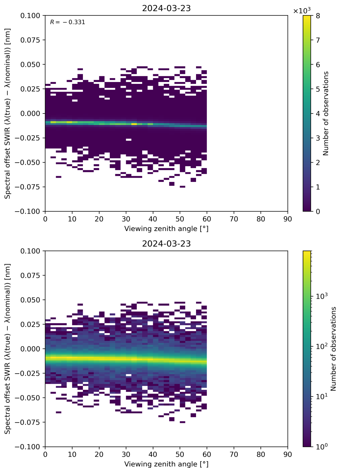
Figure 116: Scatter density plot of “Viewing zenith angle” against “Spectral offset SWIR ( \lambda(\text{true}) - \lambda(\text{nominal}) )” for 2024-03-23 to 2024-03-24.
