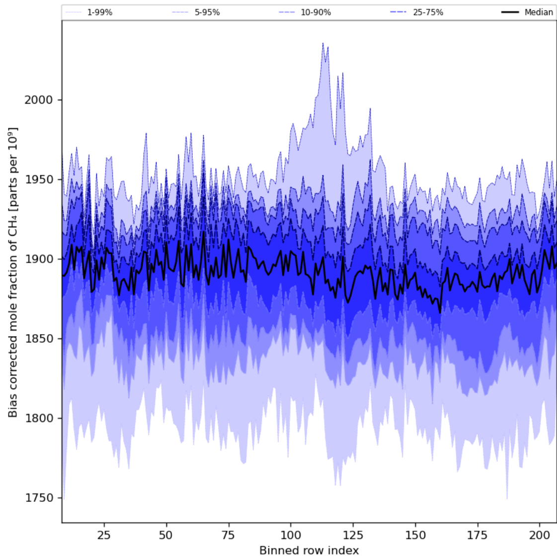
Figure 36: Along track statistics of “Bias corrected mole fraction of CH 4 ” for 2024-03-23 to 2024-03-24
