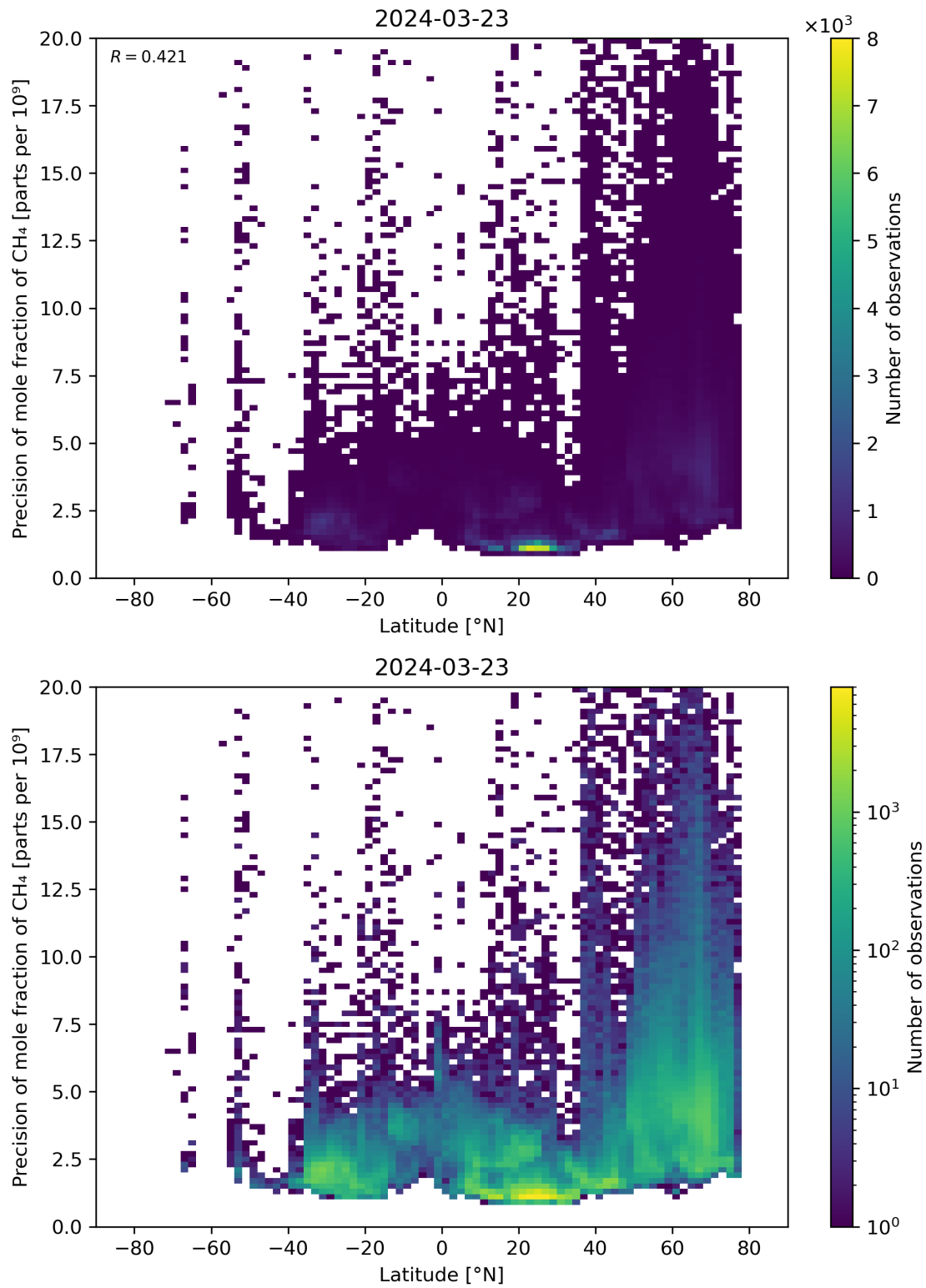
Figure 59: Scatter density plot of “Latitude” against “Precision of mole fraction of CH 4 ” for 2024-03-23 to 2024-03-24.
