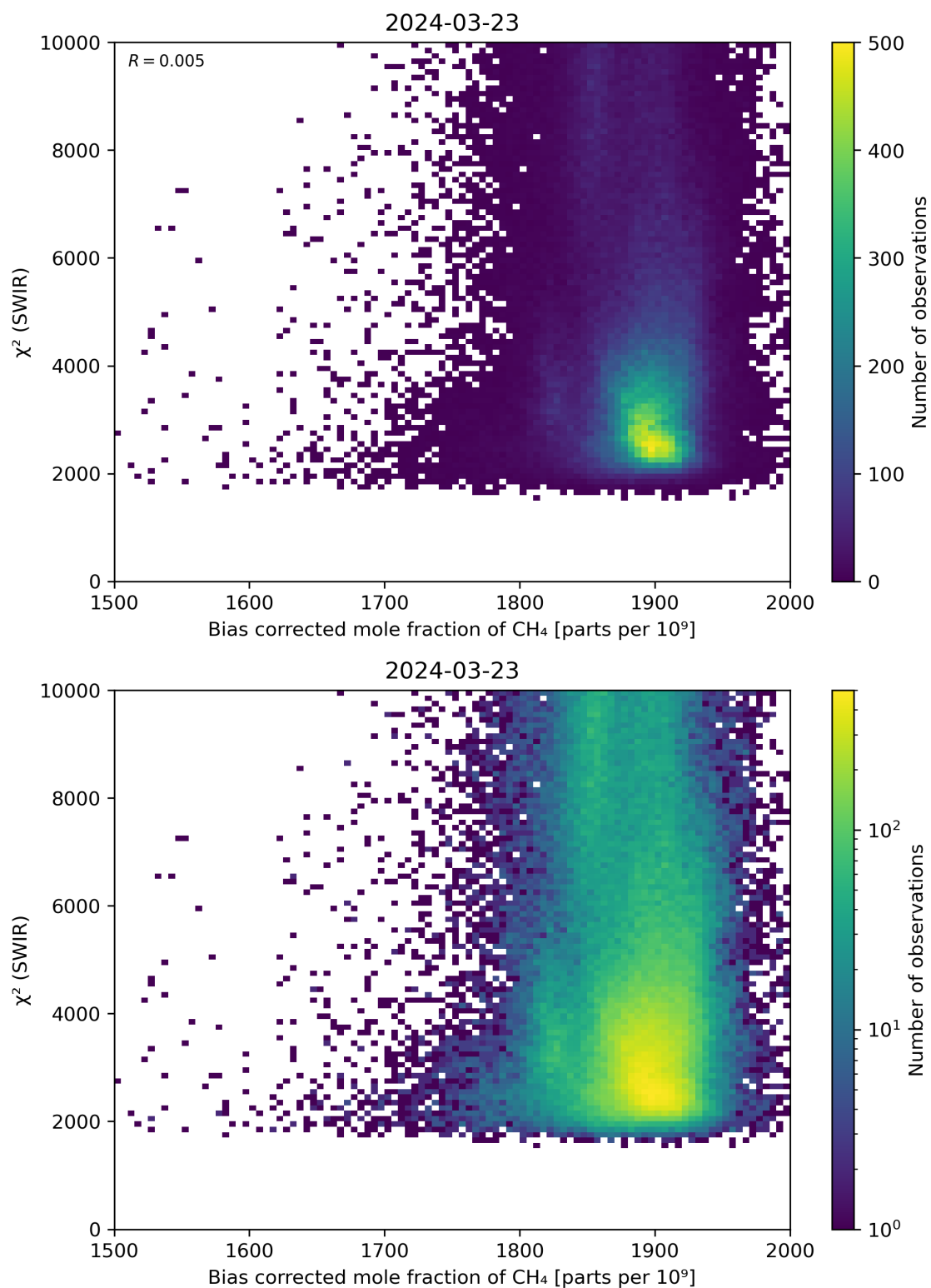
Figure 64: Scatter density plot of “Bias corrected mole fraction of \text{CH}_4 ” against “ \chi^2 (SWIR)” for 2024-03-23 to 2024-03-24.
