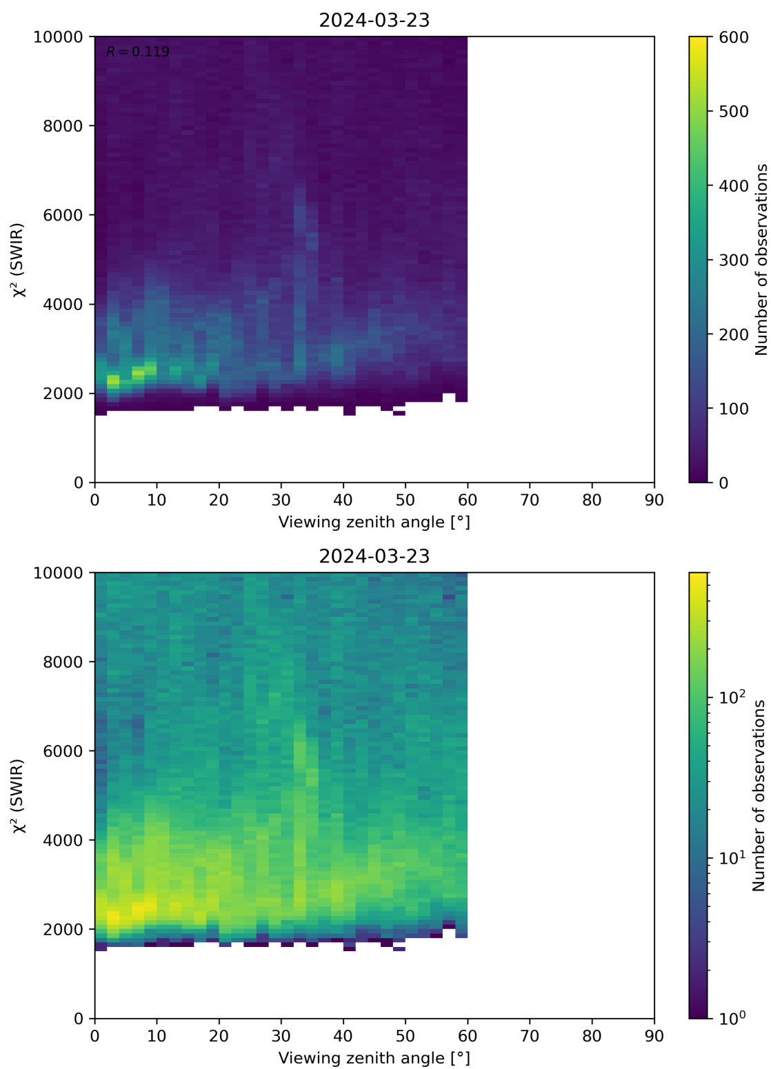
Figure 106: Scatter density plot of “Viewing zenith angle” against “ \chi^2 (SWIR)” for 2024-03-23 to 2024-03-24.
