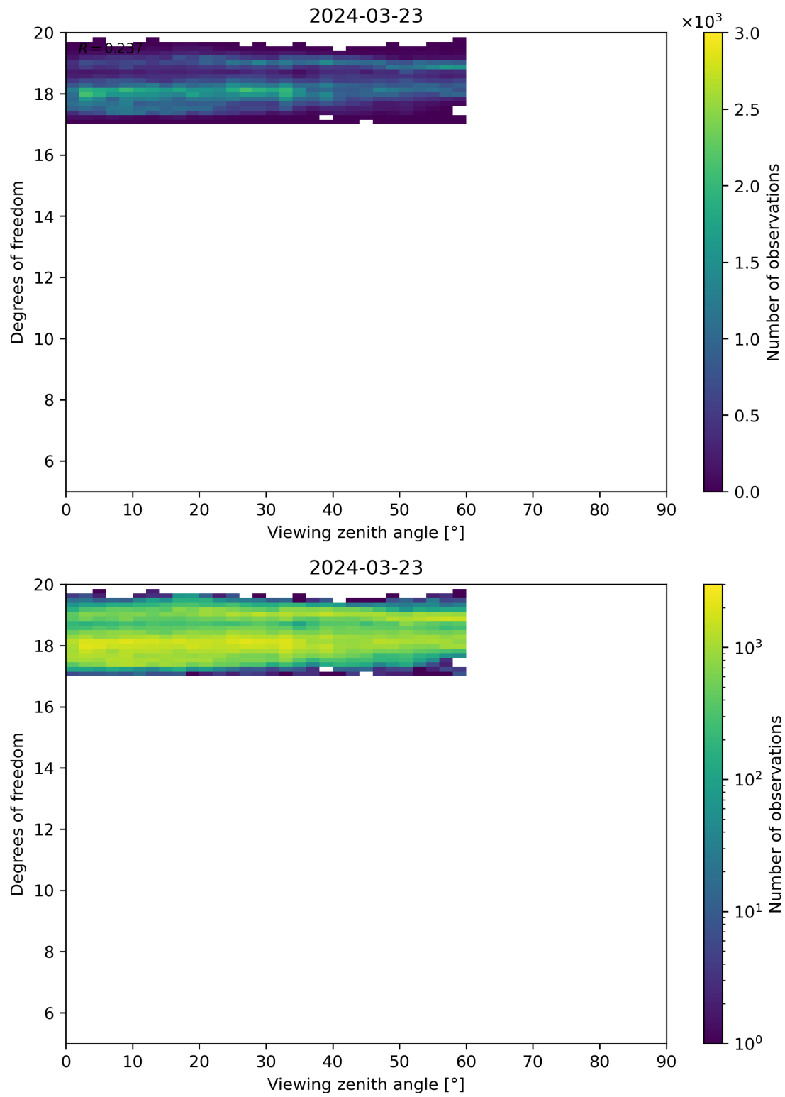
Figure 107: Scatter density plot of “Viewing zenith angle” against “Degrees of freedom” for 2024-03-23 to 2024-03-24.
