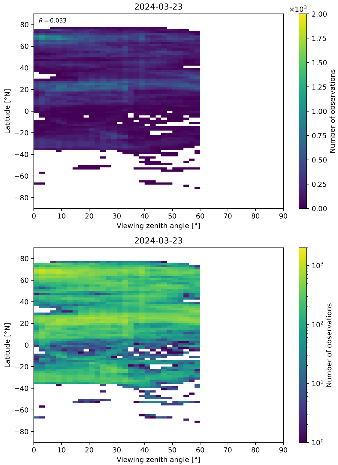
Figure 109: Scatter density plot of “Viewing zenith angle” against “Latitude” for 2024-03-23 to 2024-03-24.
