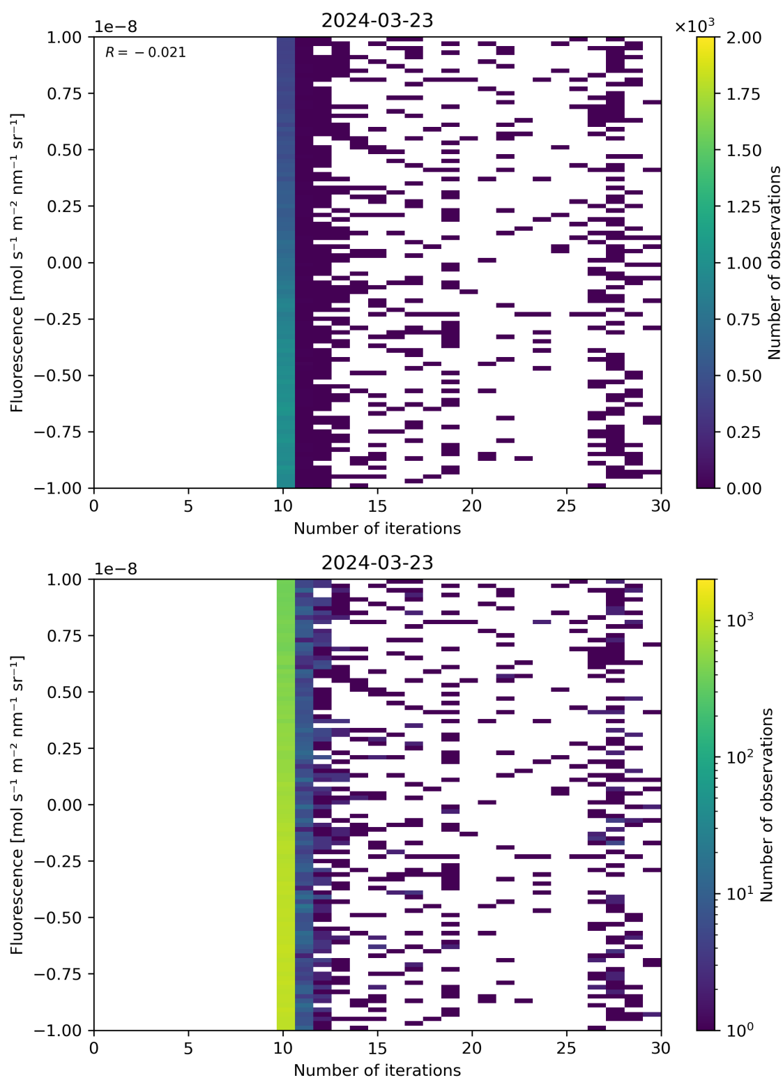
Figure 87: Scatter density plot of “Number of iterations” against “Fluorescence” for 2024-03-23 to 2024-03-24.
