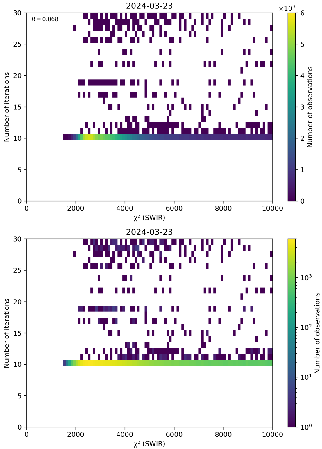
Figure 50: Scatter density plot of “ \chi^2 (SWIR)” against “Number of iterations” for 2024-03-23 to 2024-03-24.
