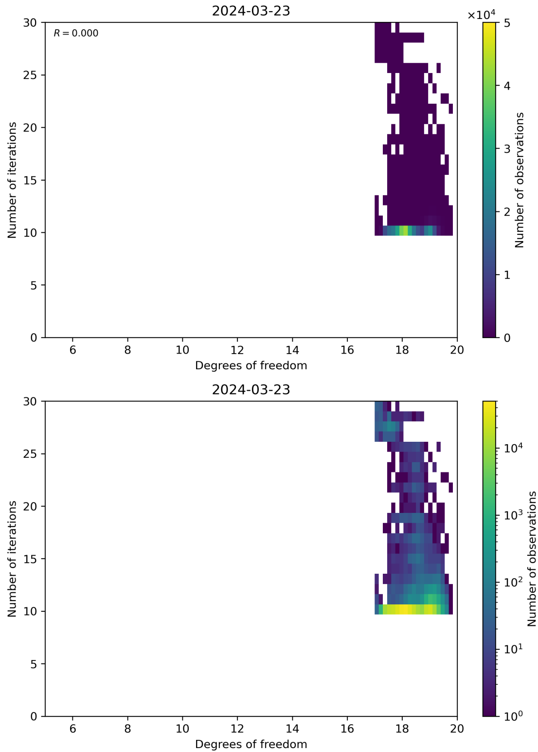
Figure 52: Scatter density plot of “Degrees of freedom” against “Number of iterations” for 2024-03-23 to 2024-03-24.
