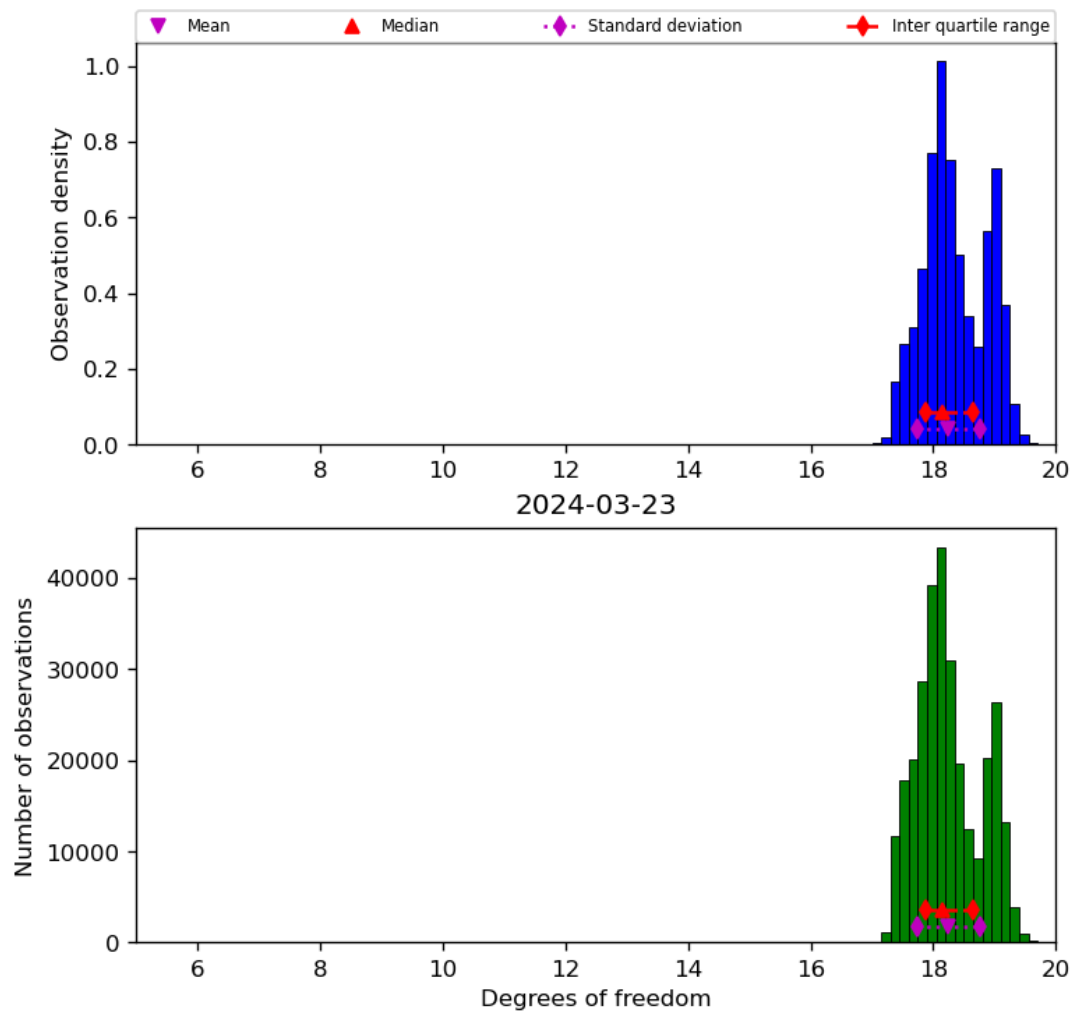
Figure 30: Histogram of “Degrees of freedom” for 2024-03-23 to 2024-03-24
