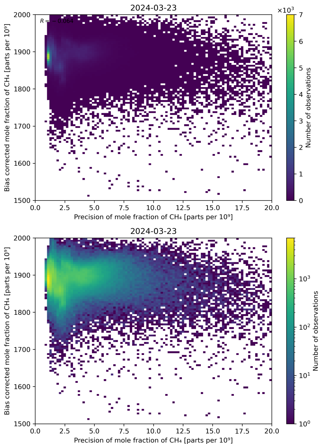
Figure 82: Scatter density plot of “Precision of mole fraction of CH 4 ” against “Bias corrected mole fraction of CH 4 ” for 2024-03-23 to 2024-03-24.
