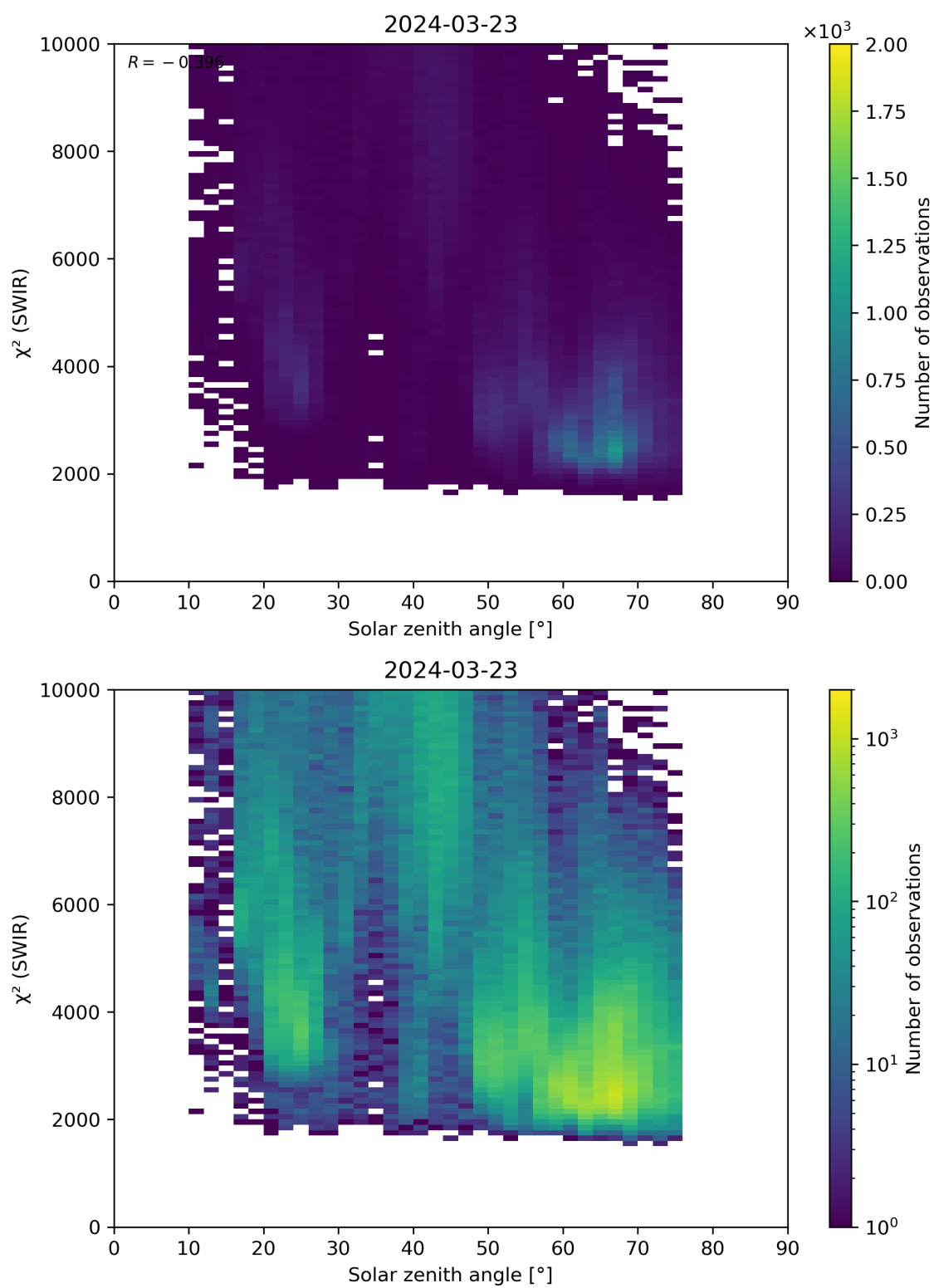
Figure 95: Scatter density plot of “Solar zenith angle” against “ \chi^2 (SWIR)” for 2024-03-23 to 2024-03-24.
