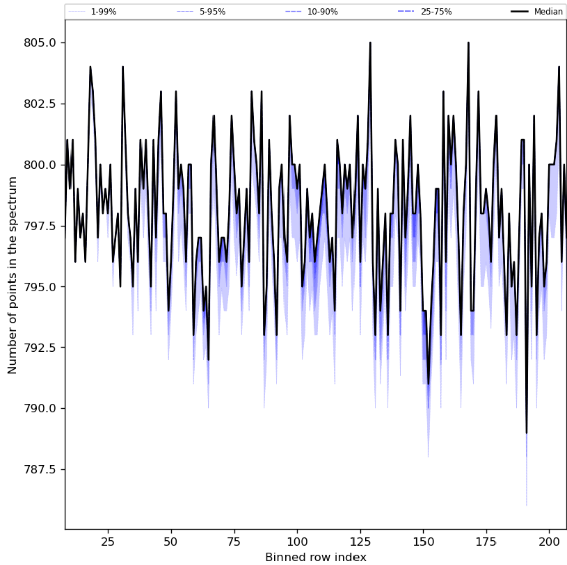
Figure 37: Along track statistics of “Number of points in the spectrum” for 2024-03-23 to 2024-03-24
