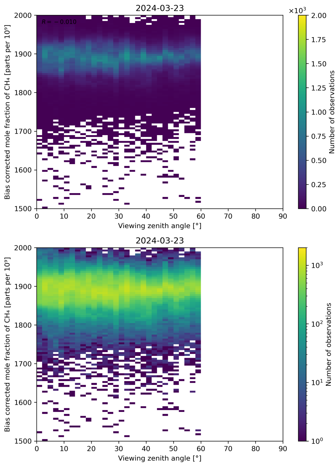
Figure 111: Scatter density plot of “Viewing zenith angle” against “Bias corrected mole fraction of CH 4 ” for 2024-03-23 to 2024-03-24.
