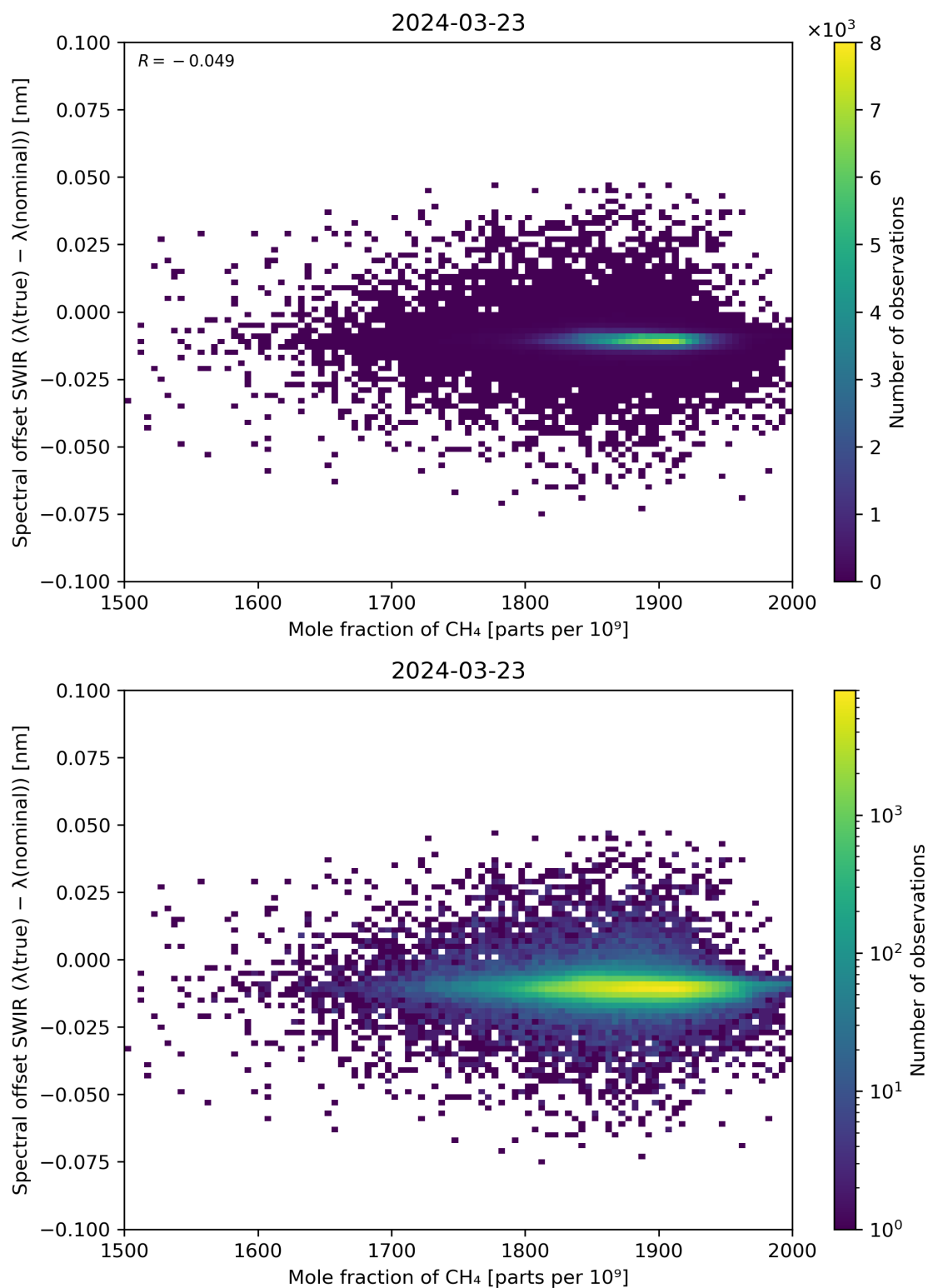
Figure 86: Scatter density plot of “Mole fraction of CH 4 ” against “Spectral offset SWIR ( \lambda(\text{true}) - \lambda(\text{nominal}) )” for 2024-03-23 to 2024-03-24.
