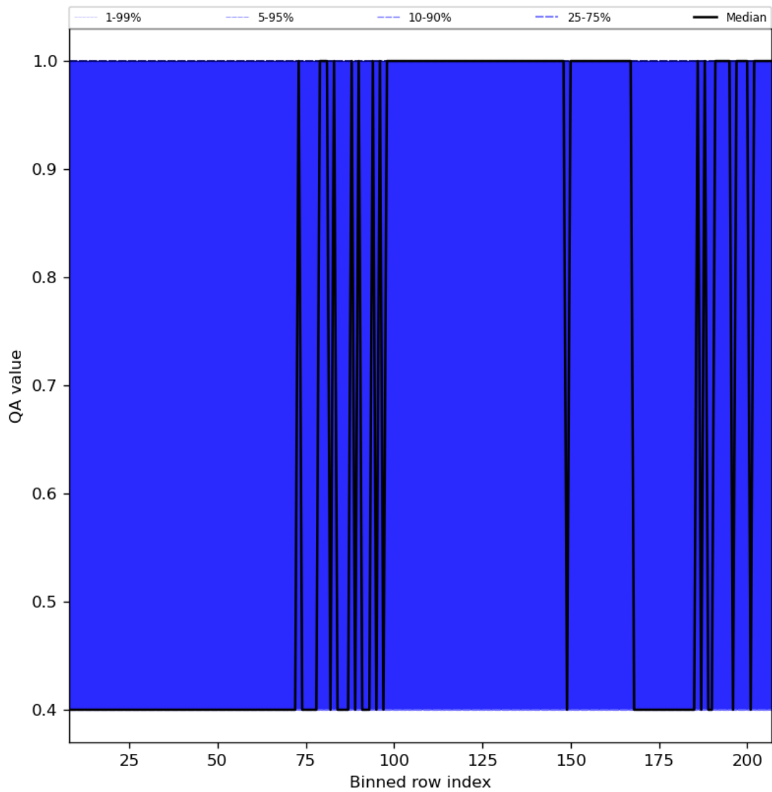
Figure 33: Along track statistics of “QA value” for 2024-03-23 to 2024-03-24
