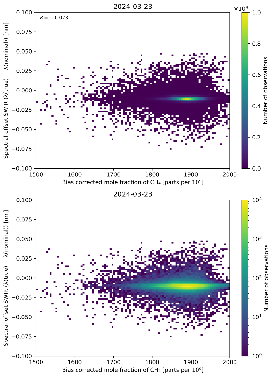
Figure 69: Scatter density plot of “Bias corrected mole fraction of \text{CH}_4 ” against “Spectral offset SWIR ( \lambda(\text{true}) - \lambda(\text{nominal}) )” for 2024-03-23 to 2024-03-24.
