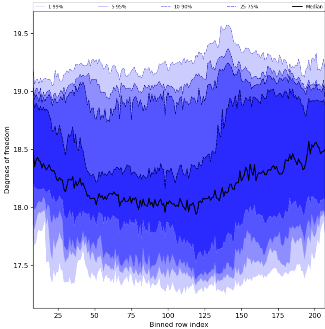
Figure 41: Along track statistics of “Degrees of freedom” for 2024-03-23 to 2024-03-24
