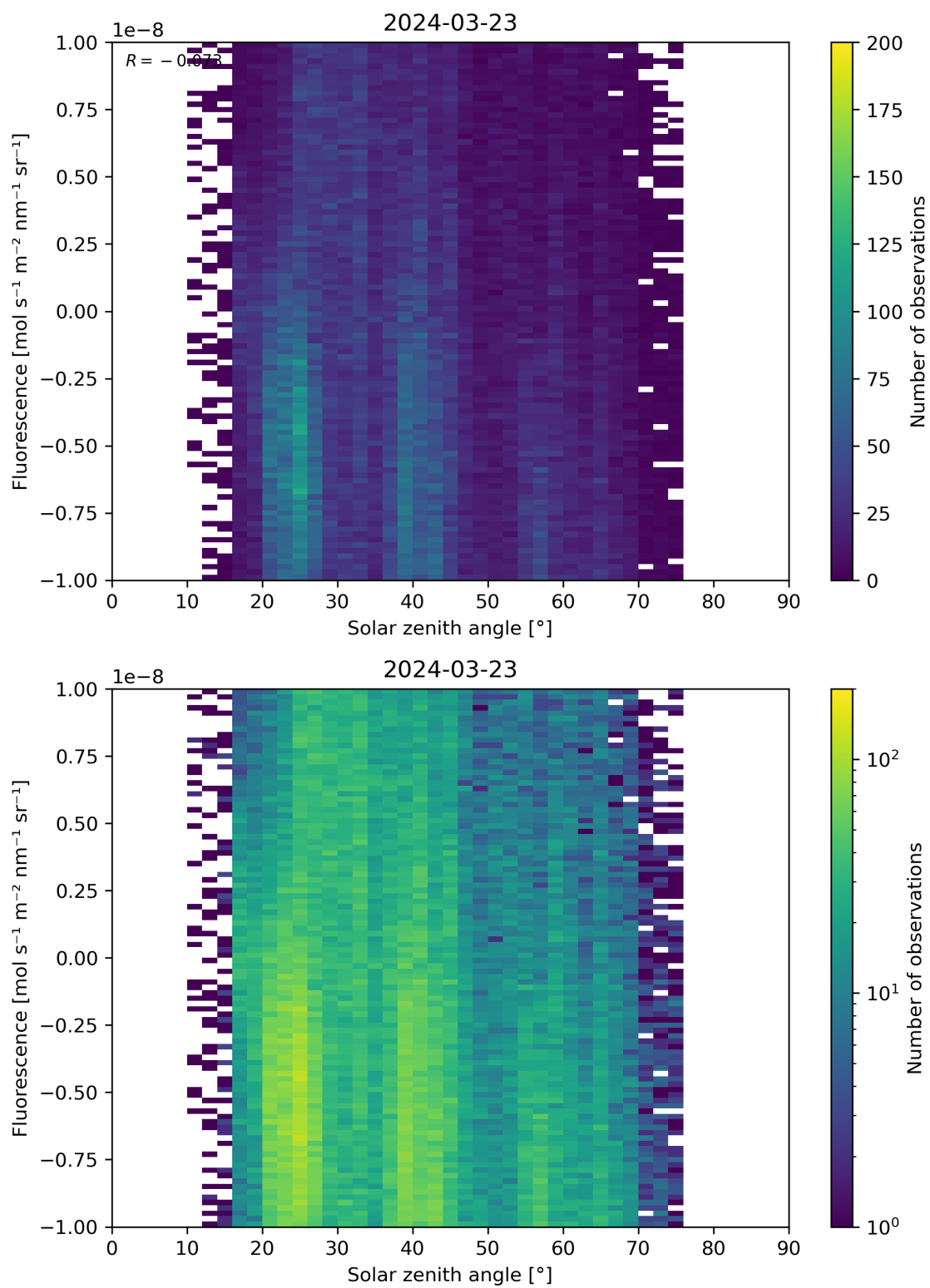
Figure 97: Scatter density plot of “Solar zenith angle” against “Fluorescence” for 2024-03-23 to 2024-03-24.
