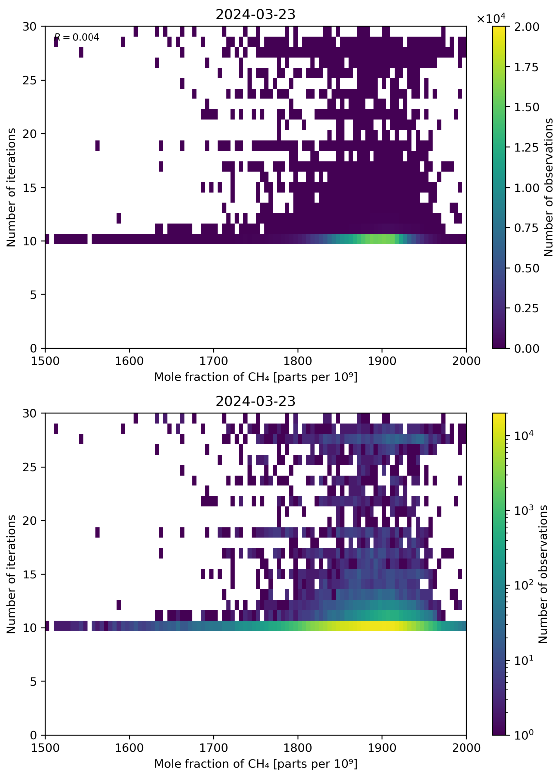
Figure 76: Scatter density plot of “Mole fraction of CH 4 ” against “Number of iterations” for 2024-03-23 to 2024-03-24.
