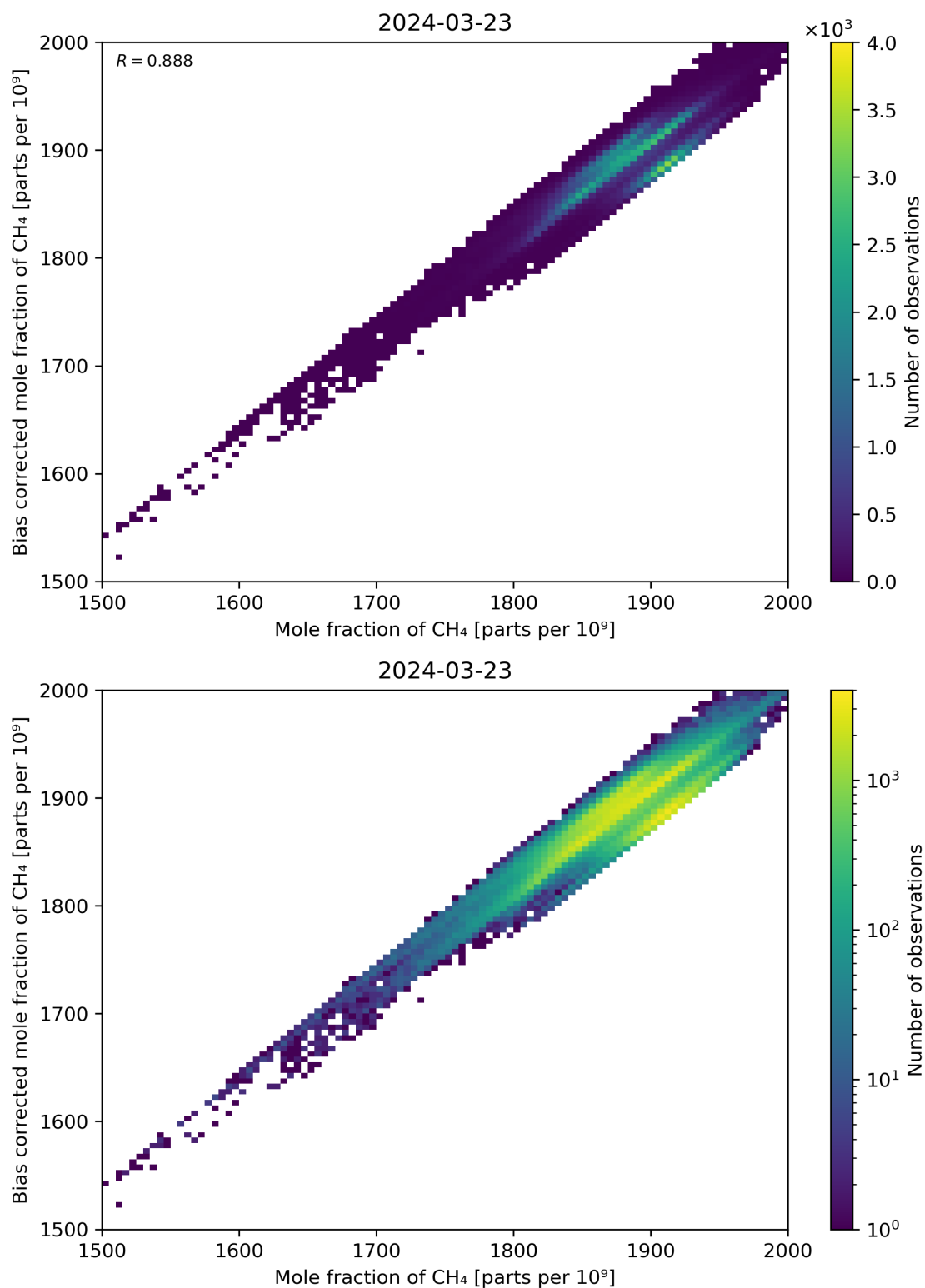
Figure 74: Scatter density plot of “Mole fraction of CH 4 ” against “Bias corrected mole fraction of CH 4 ” for 2024-03-23 to 2024-03-24.
