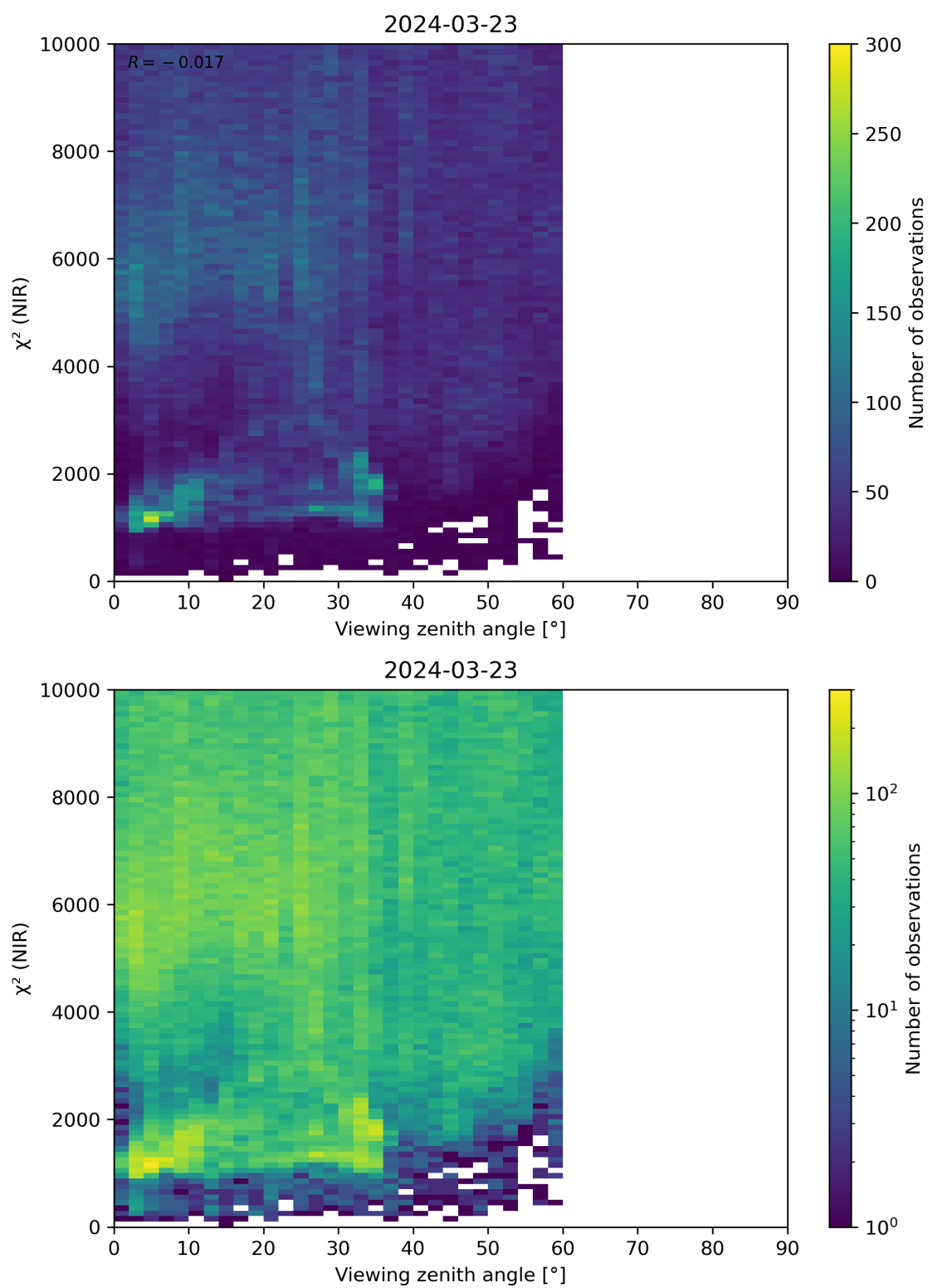
Figure 105: Scatter density plot of “Viewing zenith angle” against “ \chi^2 (NIR)” for 2024-03-23 to 2024-03-24.
