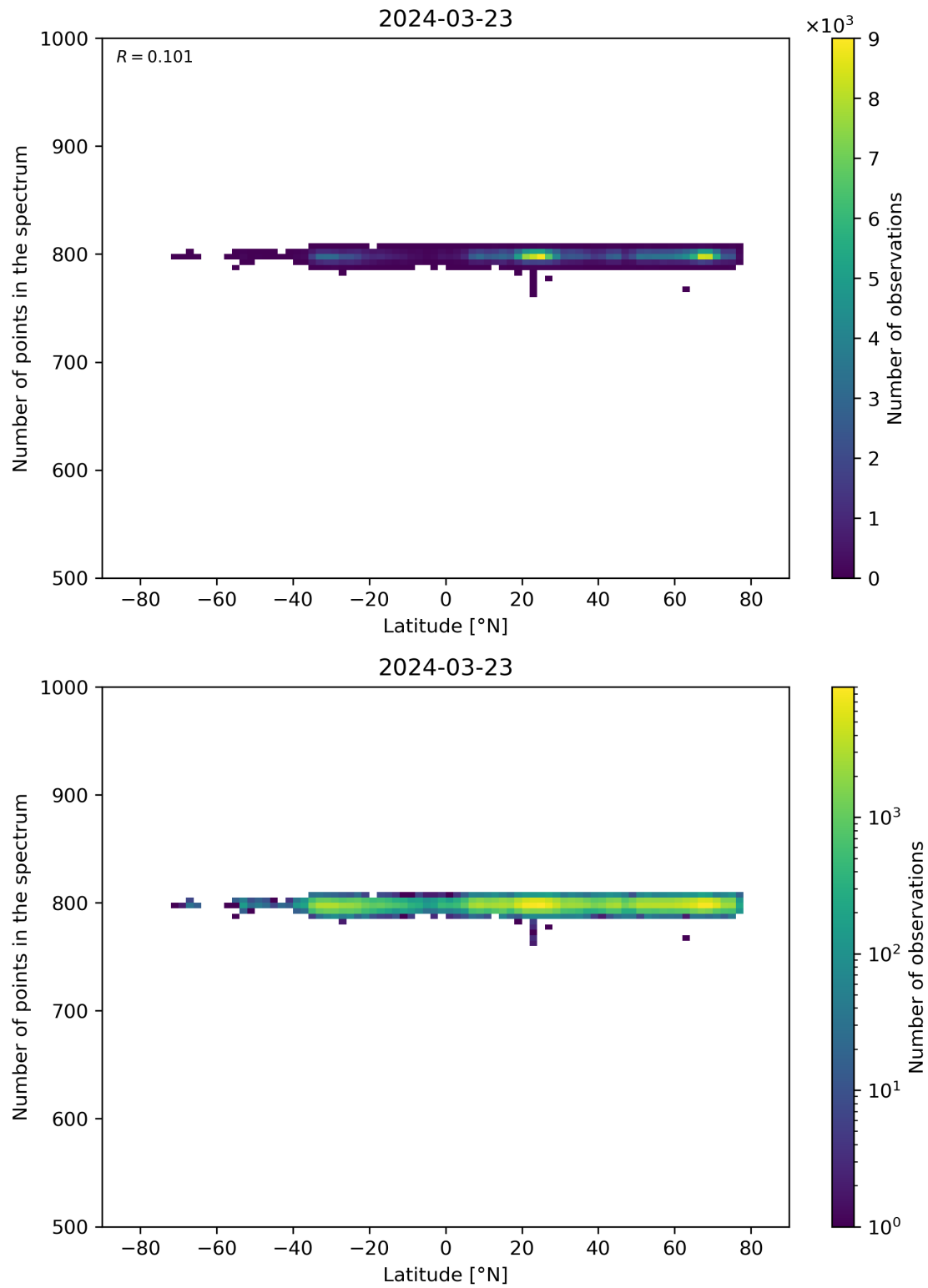
Figure 61: Scatter density plot of “Latitude” against “Number of points in the spectrum” for 2024-03-23 to 2024-03-24.
