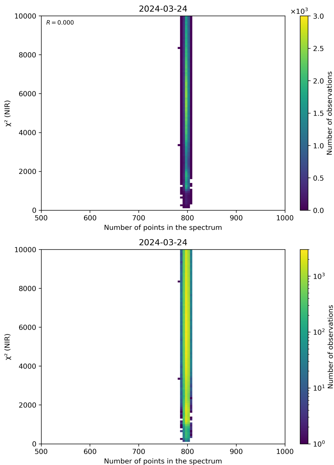
Figure 88: Scatter density plot of “Number of points in the spectrum” against “ \chi^2 (NIR)” for 2024-03-23 to 2024-03-25.
