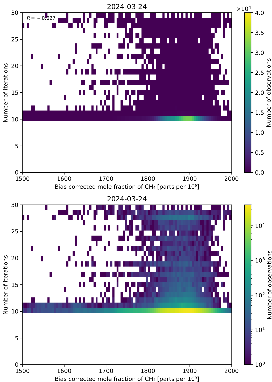
Figure 67: Scatter density plot of “Bias corrected mole fraction of CH 4 ” against “Number of iterations” for 2024-03-23 to 2024-03-25.
