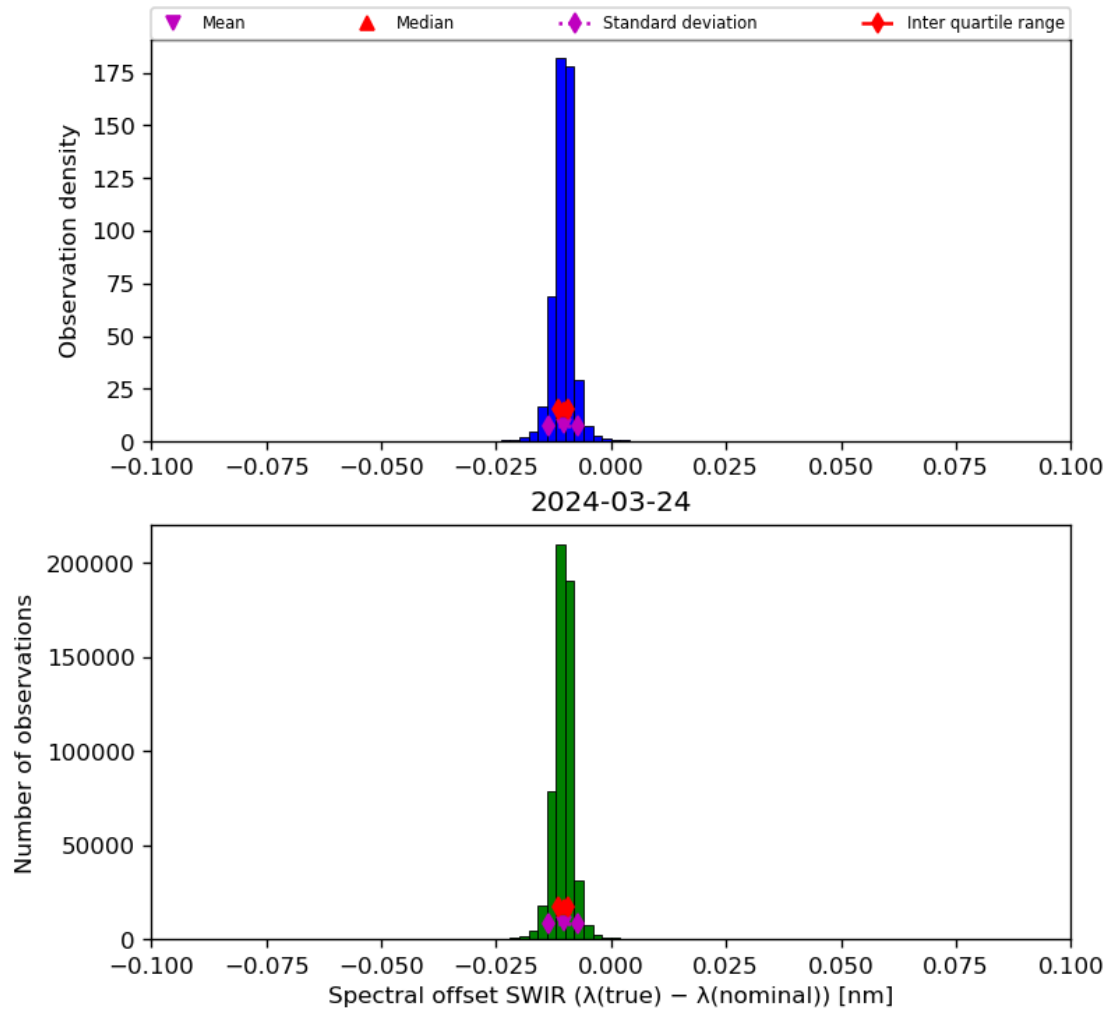
Figure 27: Histogram of “Spectral offset SWIR ( \lambda(\text{true}) - \lambda(\text{nominal}) )” for 2024-03-23 to 2024-03-25
