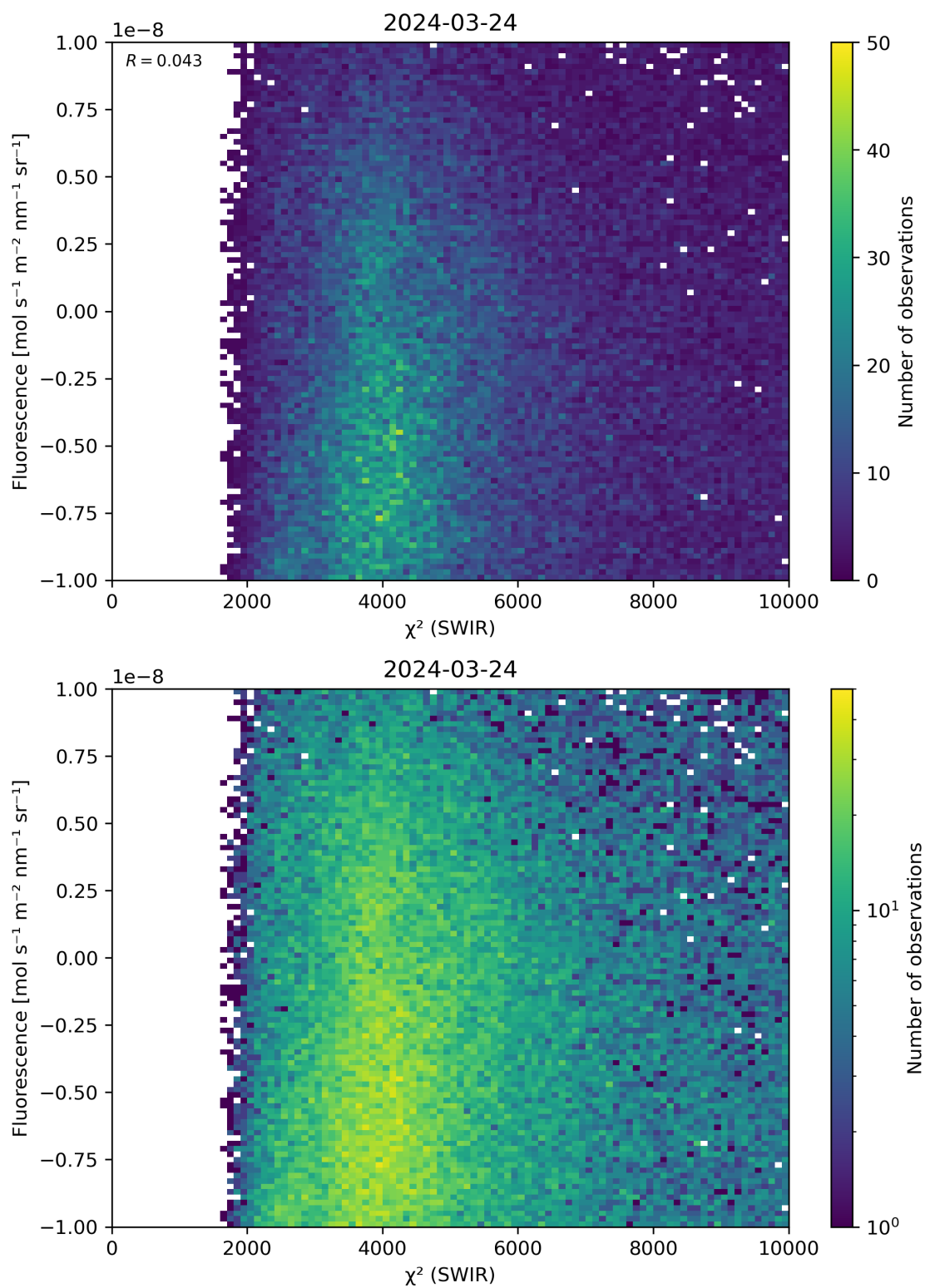
Figure 49: Scatter density plot of “ \chi^2 (SWIR)” against “Fluorescence” for 2024-03-23 to 2024-03-25.
