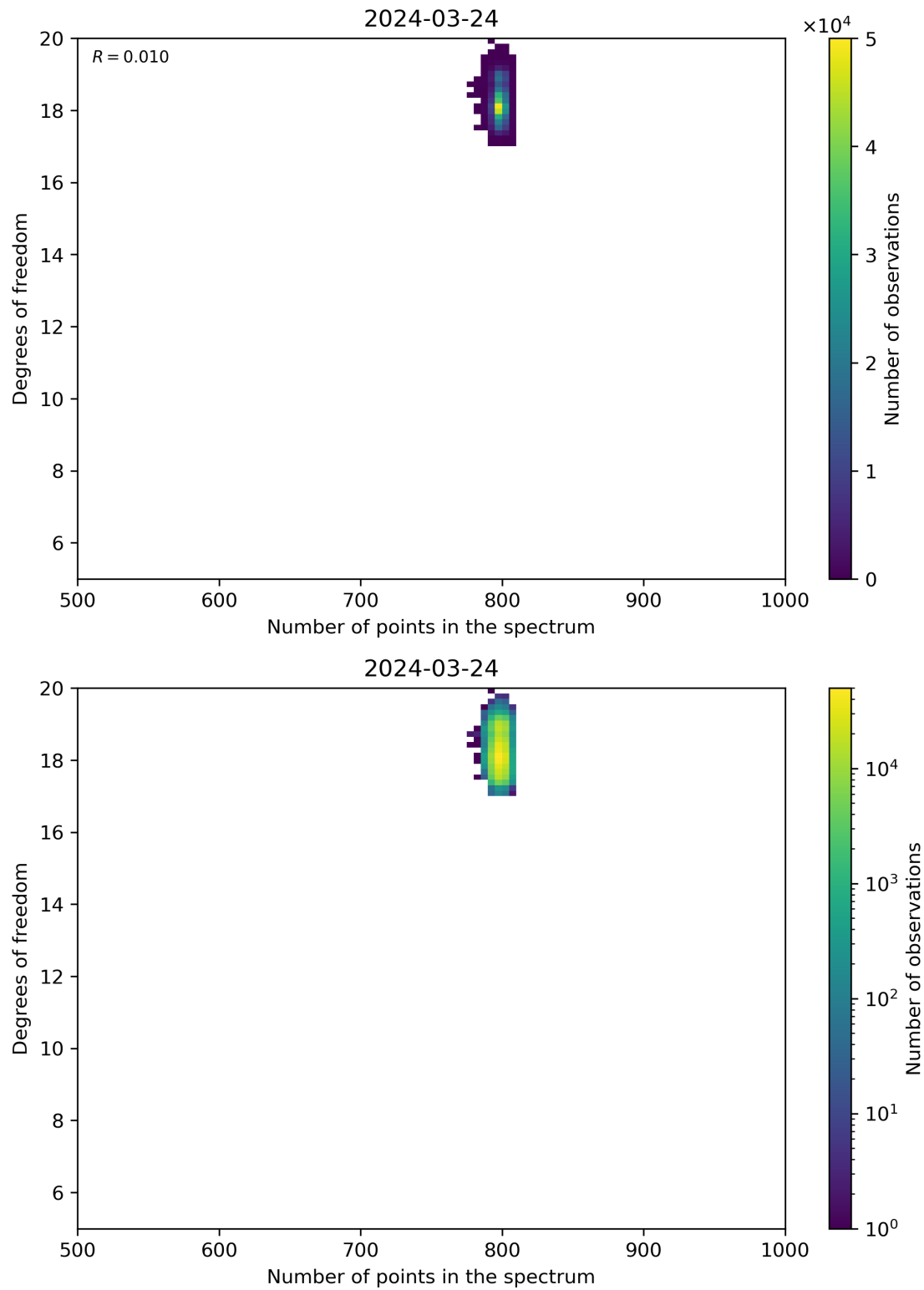
Figure 90: Scatter density plot of “Number of points in the spectrum” against “Degrees of freedom” for 2024-03-23 to 2024-03-25.
