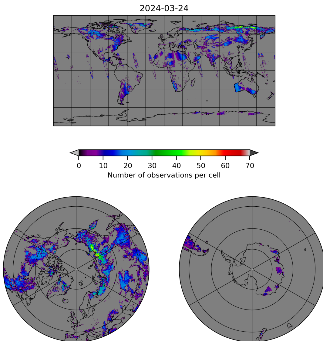
Figure 10: Map of the number of observations for 2024-03-23 to 2024-03-25
