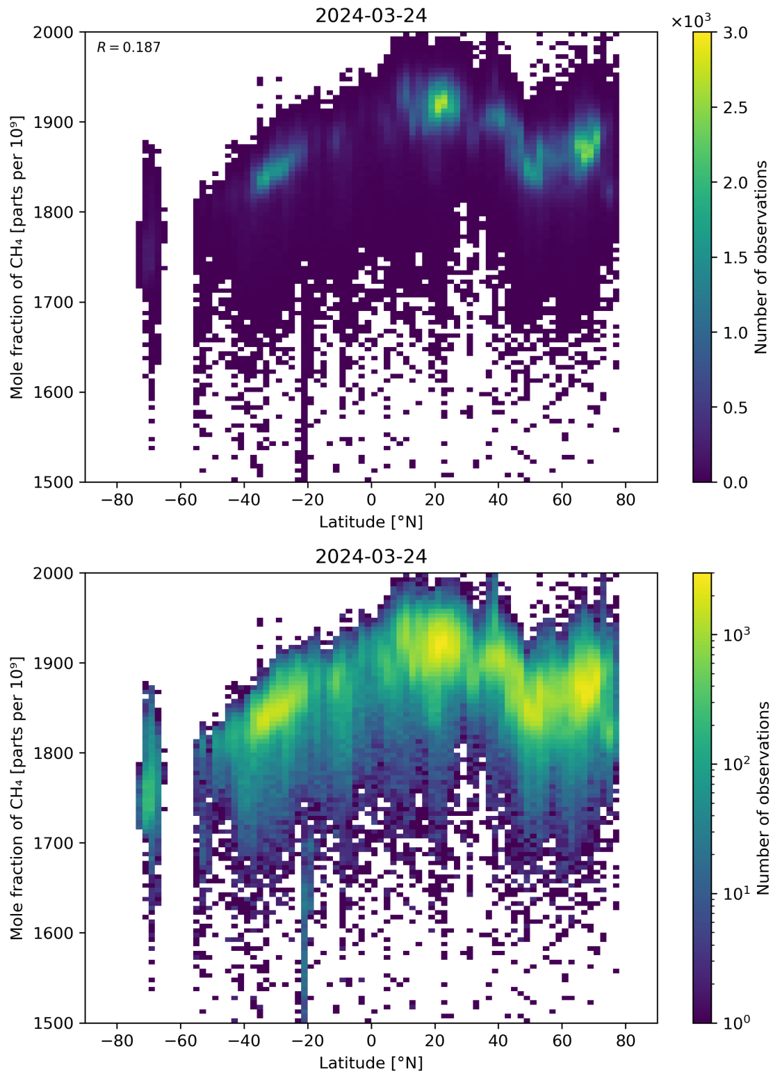
Figure 57: Scatter density plot of “Latitude” against “Mole fraction of CH 4 ” for 2024-03-23 to 2024-03-25.
