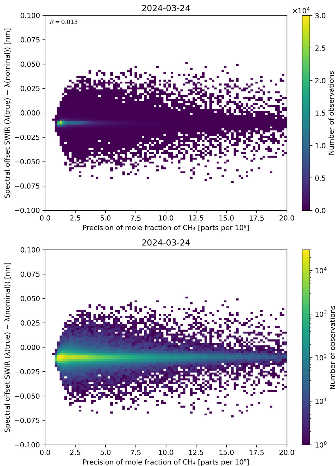
Figure 85: Scatter density plot of “Precision of mole fraction of \text{CH}_4 ” against “Spectral offset SWIR ( \lambda(\text{true}) - \lambda(\text{nominal}) )” for 2024-03-23 to 2024-03-25.
