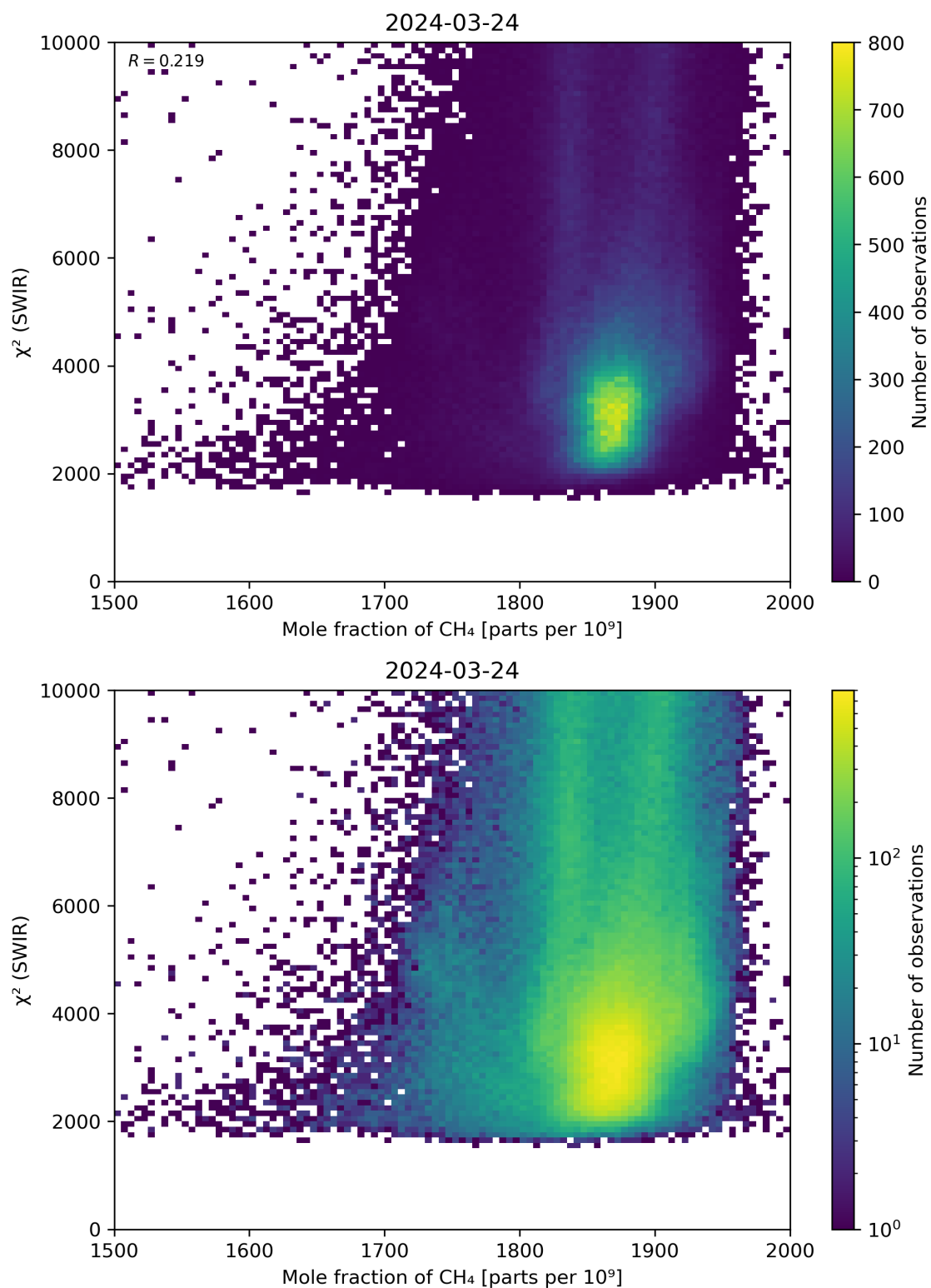
Figure 71: Scatter density plot of “Mole fraction of \text{CH}_4 ” against “ \chi^2 (SWIR)” for 2024-03-23 to 2024-03-25.
