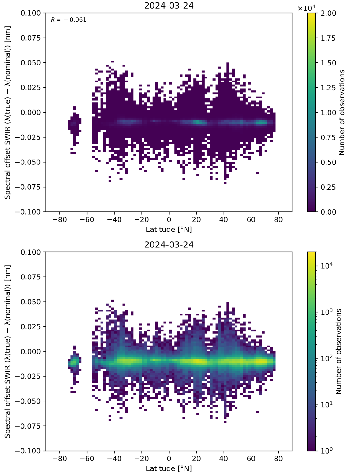
Figure 62: Scatter density plot of “Latitude” against “Spectral offset SWIR ( \lambda(\text{true}) - \lambda(\text{nominal}) )” for 2024-03-23 to 2024-03-25.
