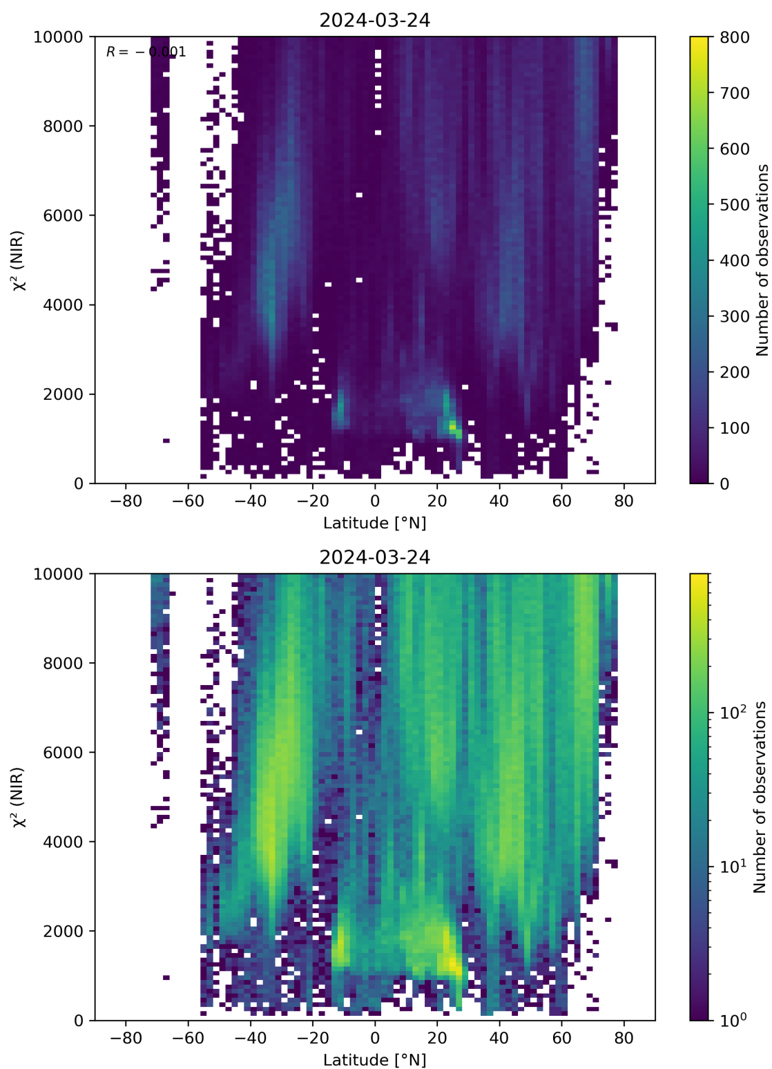
Figure 53: Scatter density plot of “Latitude” against “ \chi^2 (NIR)” for 2024-03-23 to 2024-03-25.
