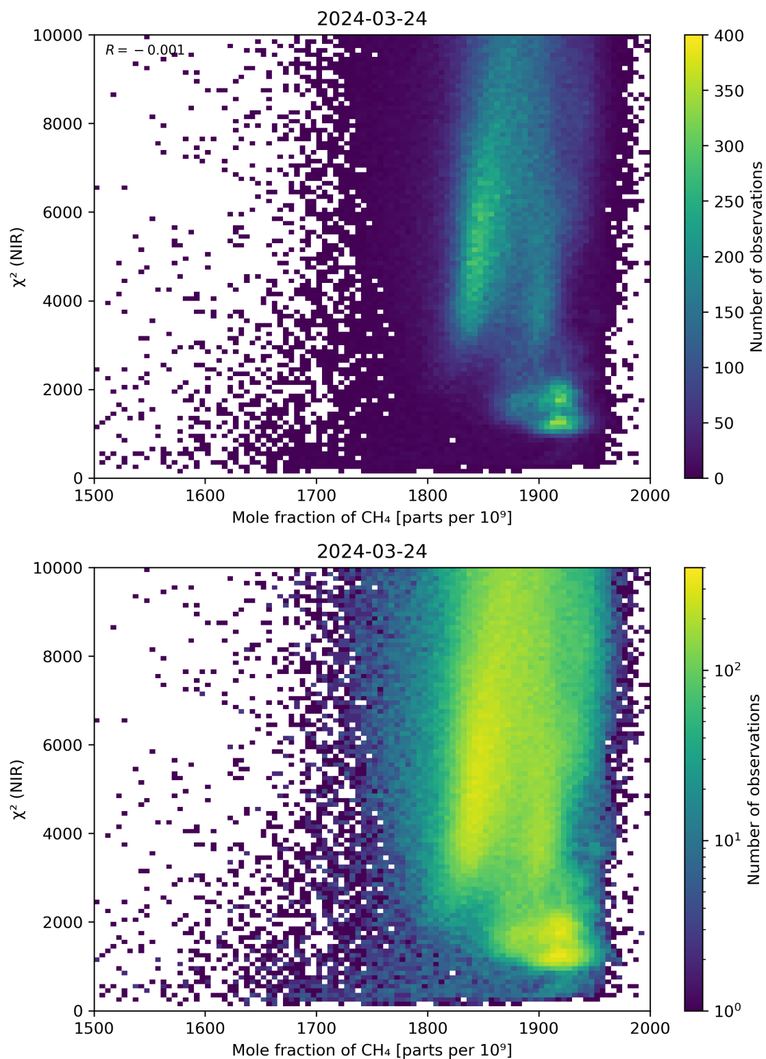
Figure 70: Scatter density plot of “Mole fraction of CH 4 ” against “ \chi^2 (NIR)” for 2024-03-23 to 2024-03-25.
