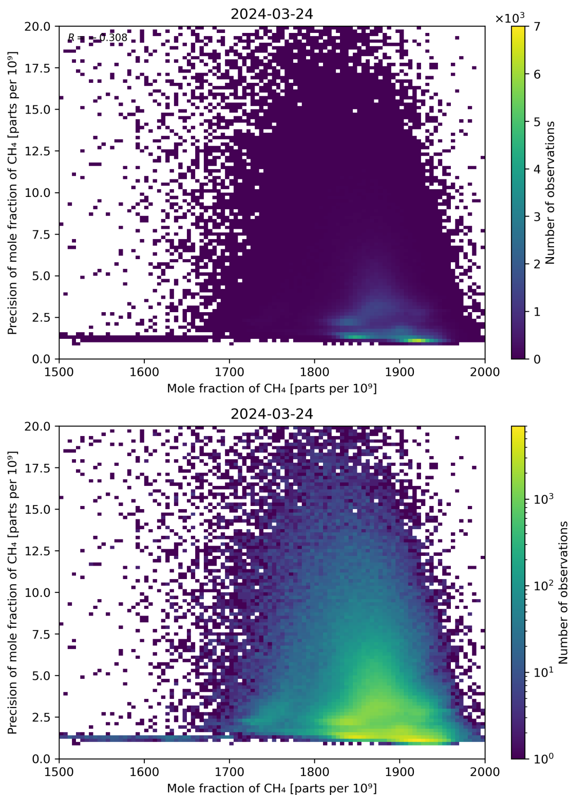
Figure 75: Scatter density plot of “Mole fraction of CH 4 ” against “Precision of mole fraction of CH 4 ” for 2024-03-23 to 2024-03-25.
