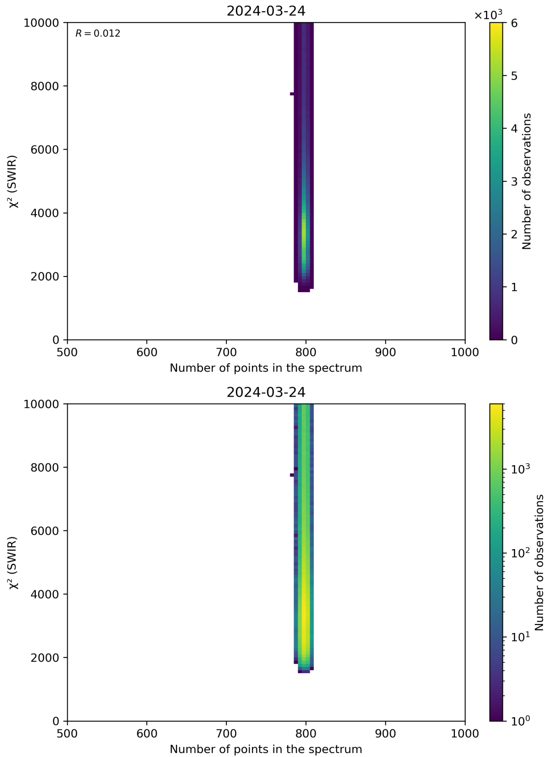
Figure 89: Scatter density plot of “Number of points in the spectrum” against “ \chi^2 (SWIR)” for 2024-03-23 to 2024-03-25.
