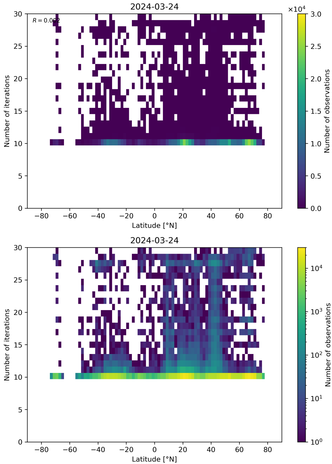
Figure 60: Scatter density plot of “Latitude” against “Number of iterations” for 2024-03-23 to 2024-03-25.
