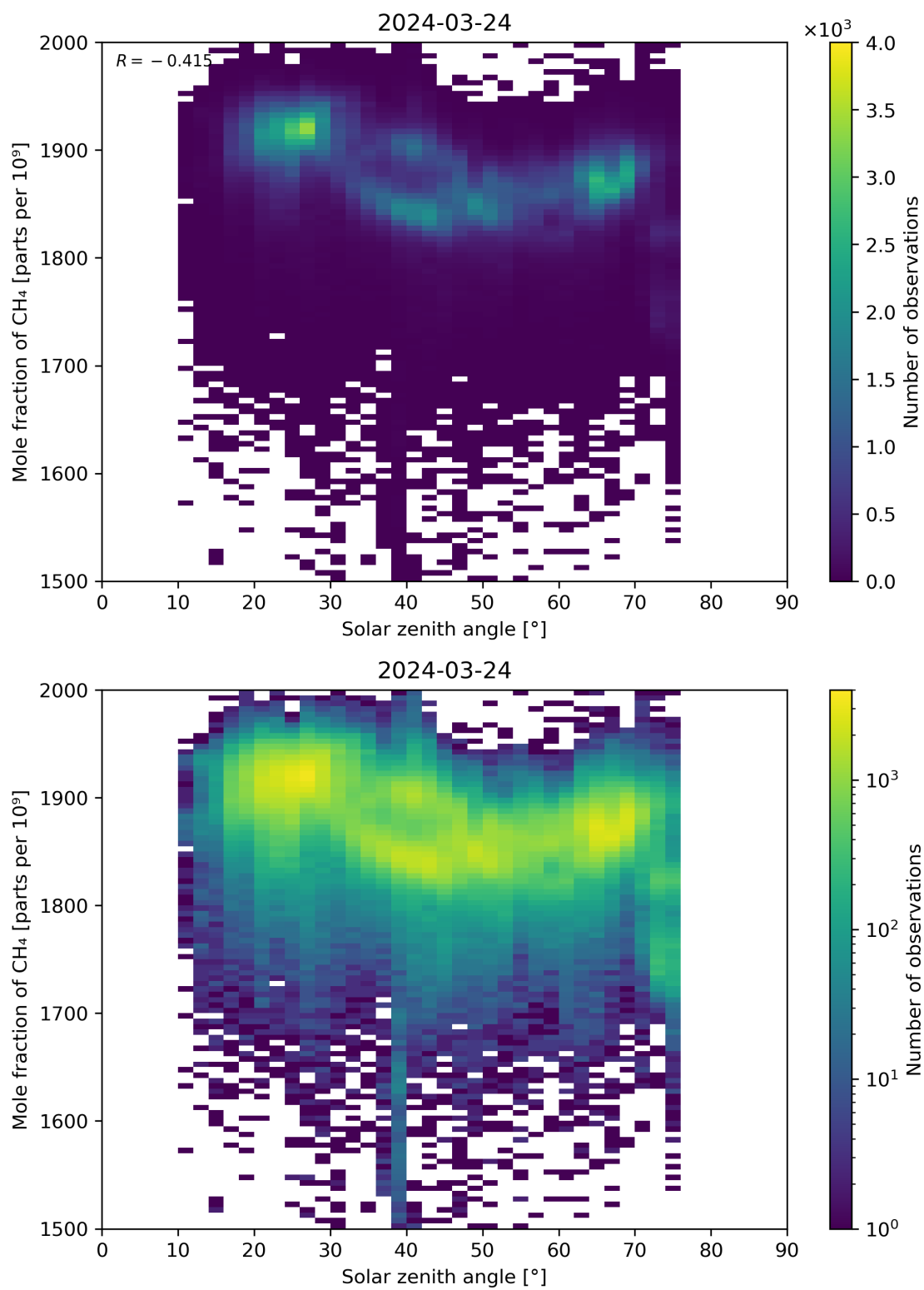
Figure 99: Scatter density plot of “Solar zenith angle” against “Mole fraction of CH 4 ” for 2024-03-23 to 2024-03-25.
