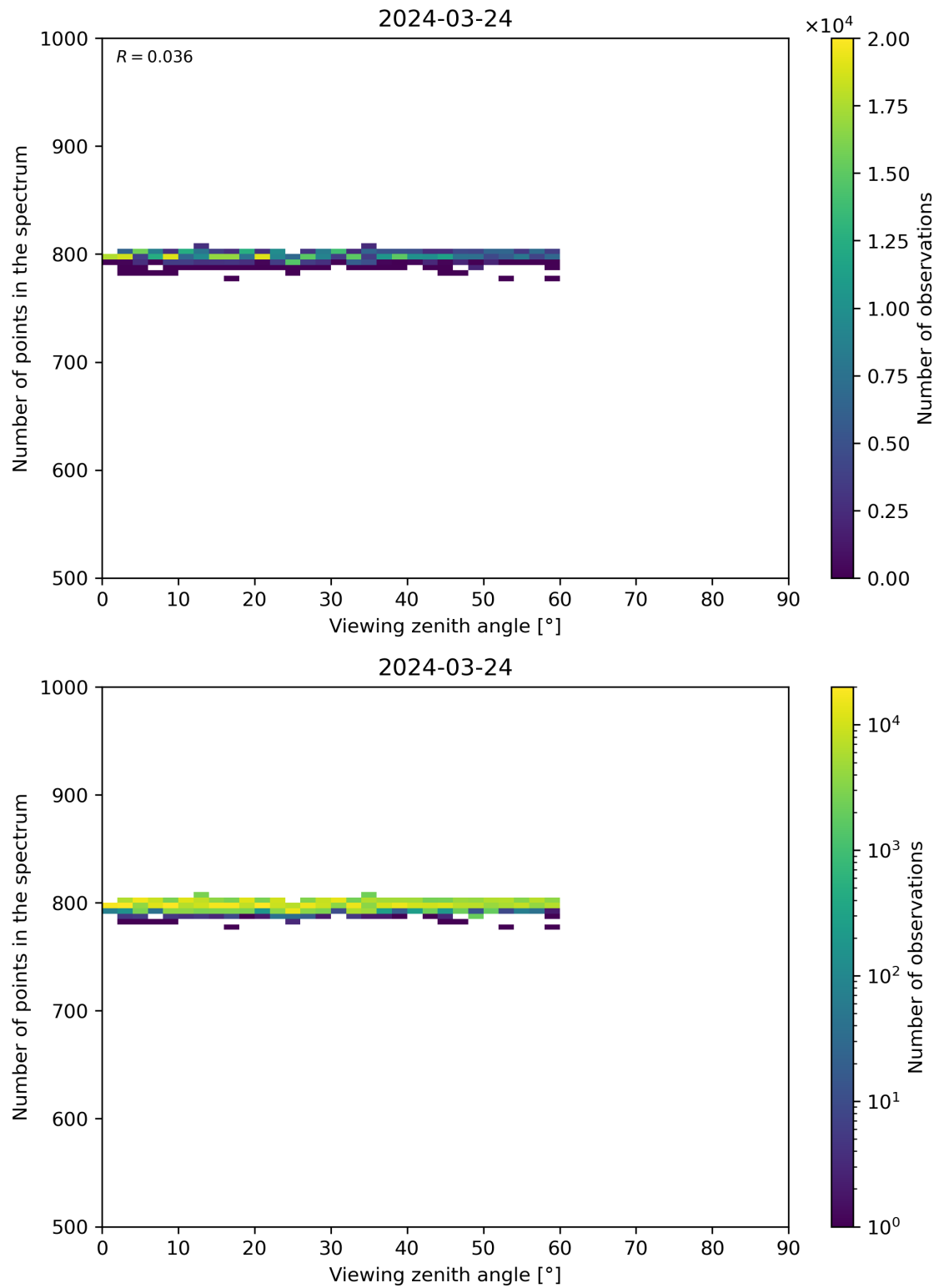
Figure 114: Scatter density plot of “Viewing zenith angle” against “Number of points in the spectrum” for 2024-03-23 to 2024-03-25.
