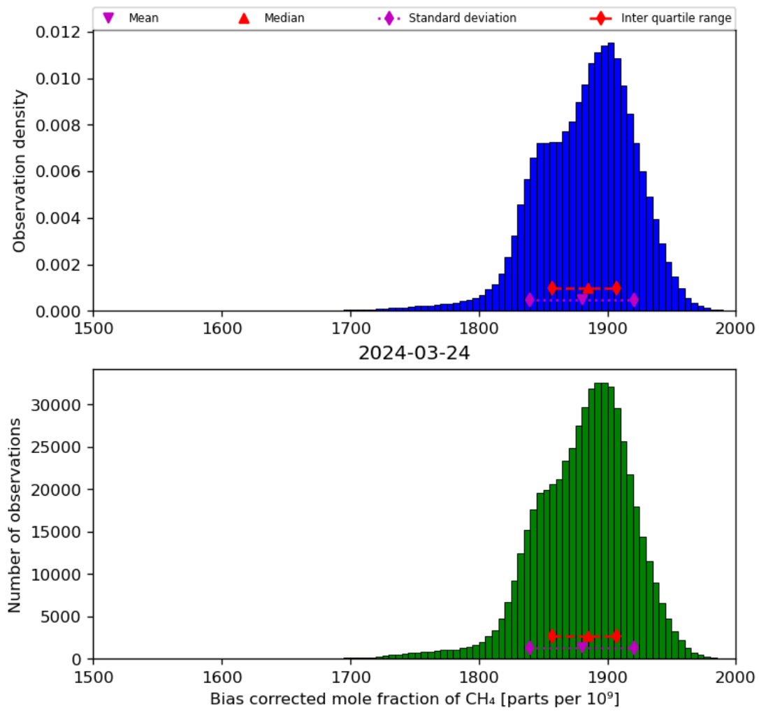
Figure 25: Histogram of “Bias corrected mole fraction of CH 4 ” for 2024-03-23 to 2024-03-25
