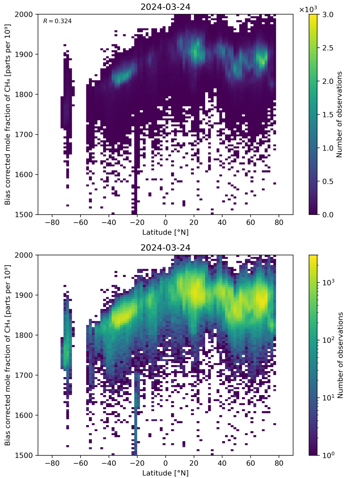
Figure 58: Scatter density plot of “Latitude” against “Bias corrected mole fraction of CH 4 ” for 2024-03-23 to 2024-03-25.
