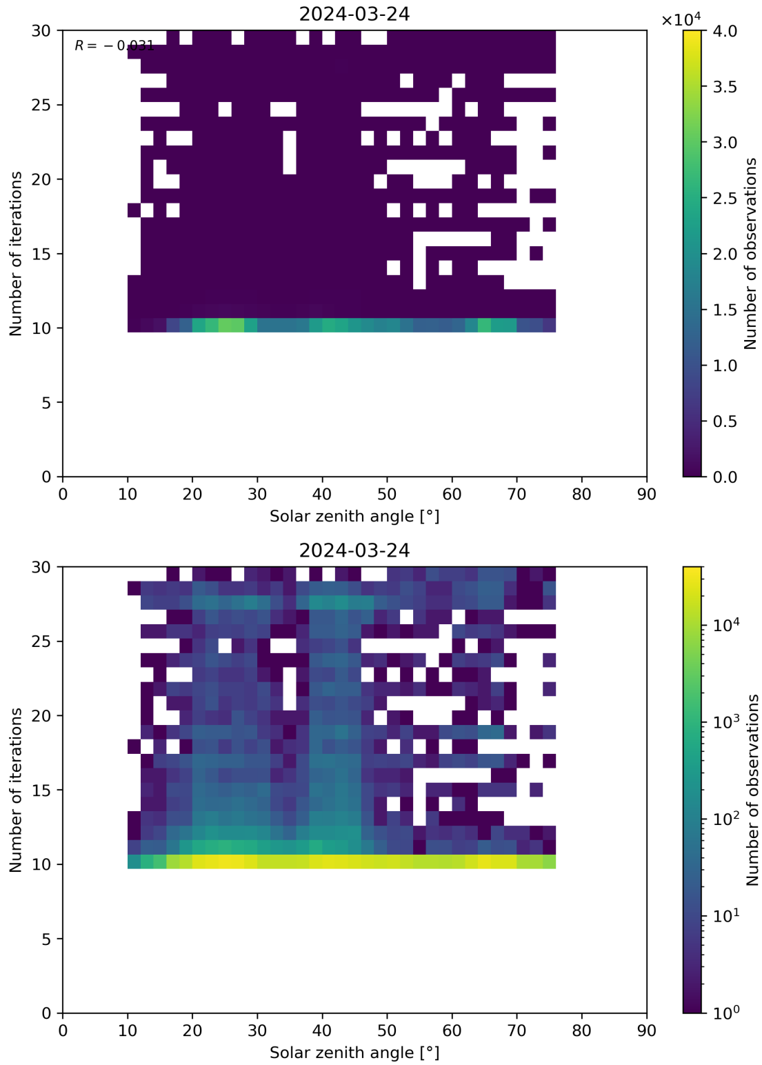
Figure 102: Scatter density plot of “Solar zenith angle” against “Number of iterations” for 2024-03-23 to 2024-03-25.
