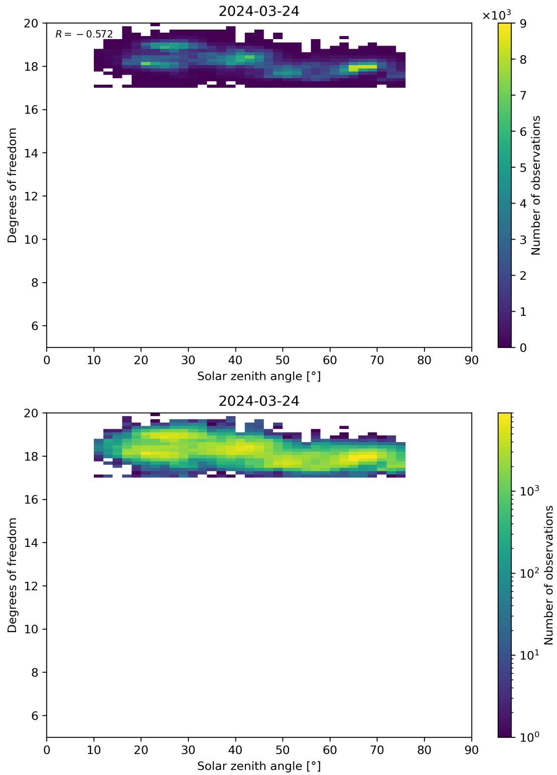
Figure 96: Scatter density plot of “Solar zenith angle” against “Degrees of freedom” for 2024-03-23 to 2024-03-25.
