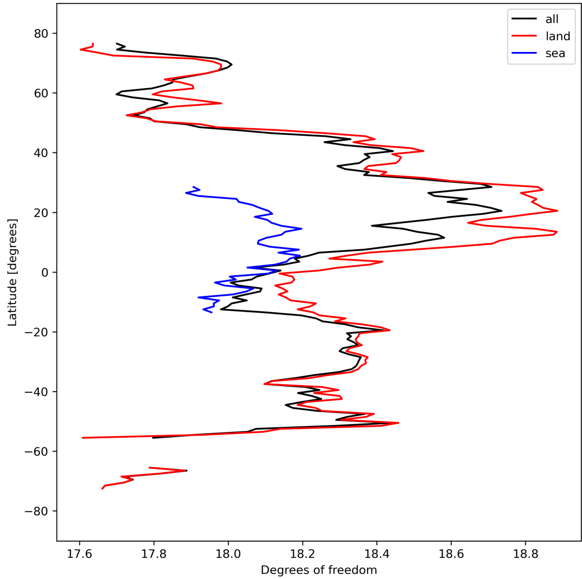
Figure 19: Zonal average of “Degrees of freedom” for 2024-03-23 to 2024-03-25.
