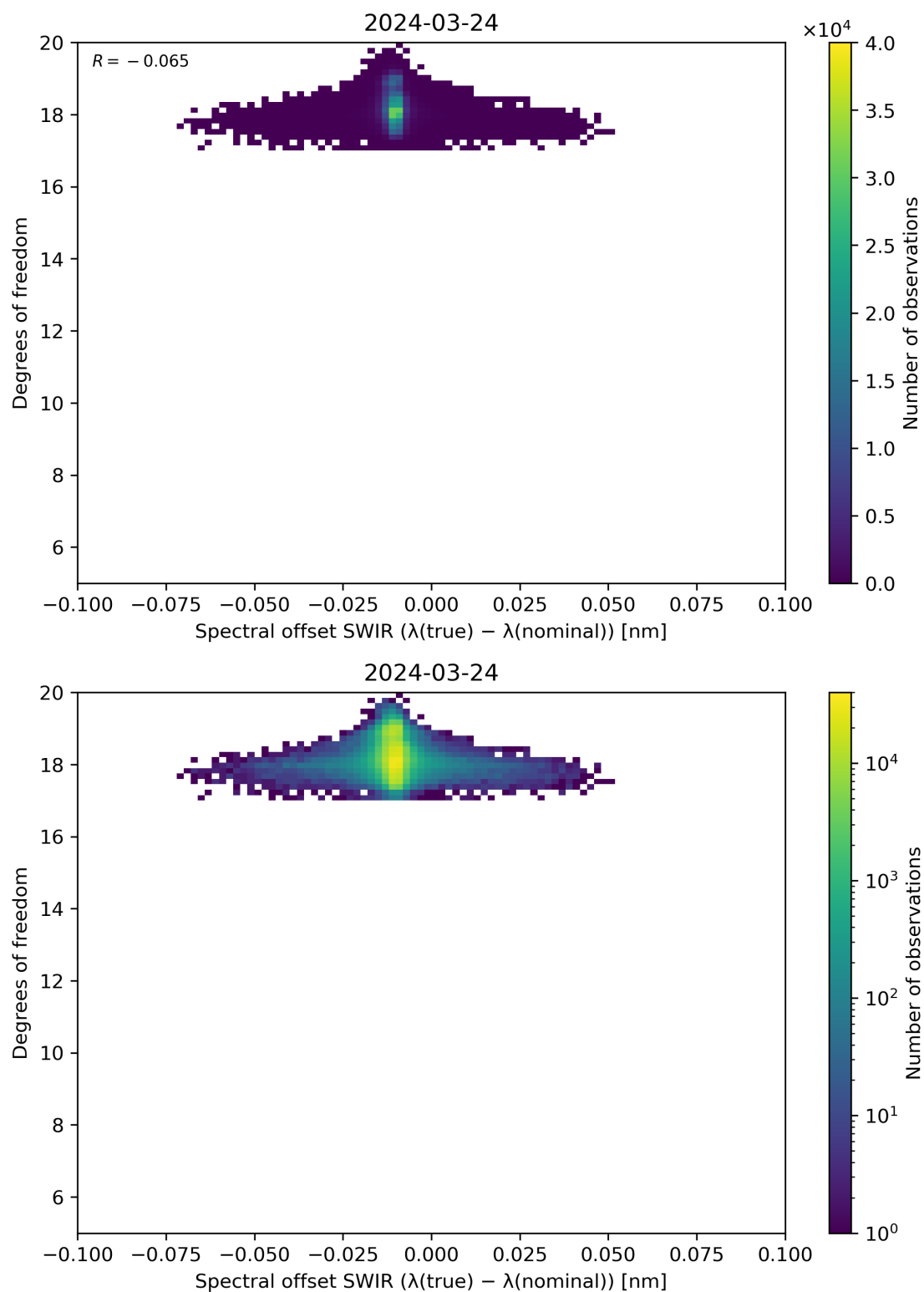
Figure 119: Scatter density plot of “Spectral offset SWIR ( \lambda(\text{true}) - \lambda(\text{nominal}) )” against “Degrees of freedom” for 2024-03-23 to 2024-03-25.
