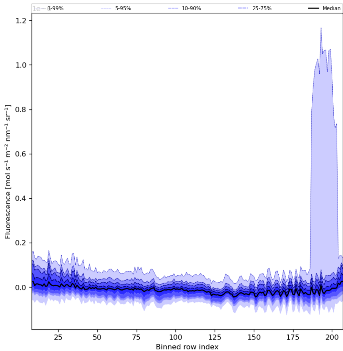
Figure 43: Along track statistics of “Fluorescence” for 2024-03-23 to 2024-03-25
