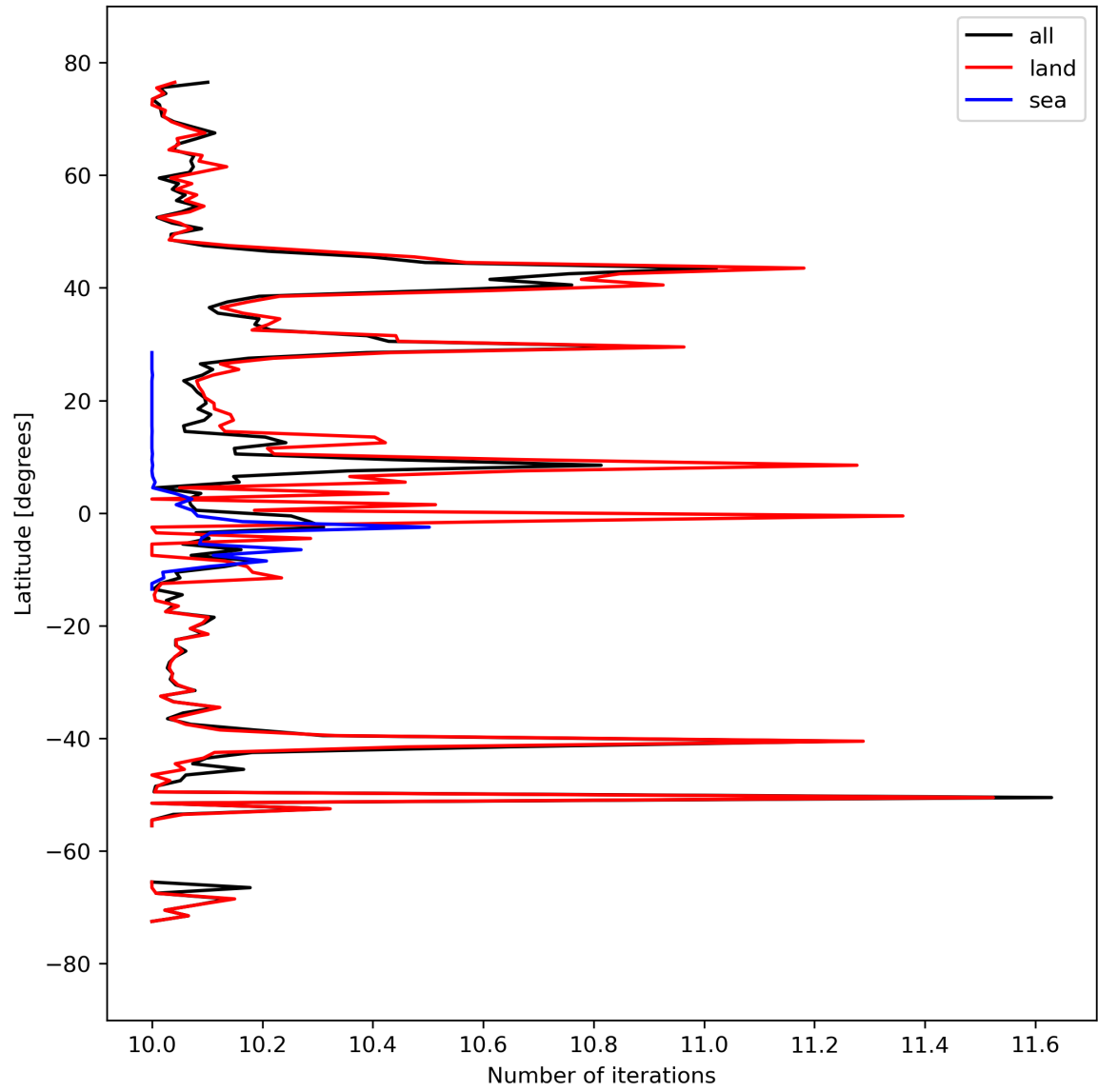
Figure 20: Zonal average of “Number of iterations” for 2024-03-23 to 2024-03-25.
