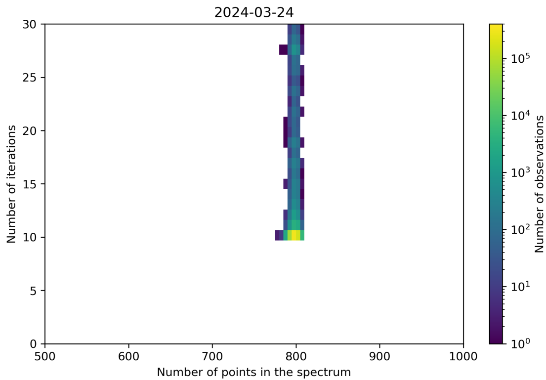
Figure 92: Scatter density plot of “Number of points in the spectrum” against “Number of iterations” for 2024-03-23 to 2024-03-25.
