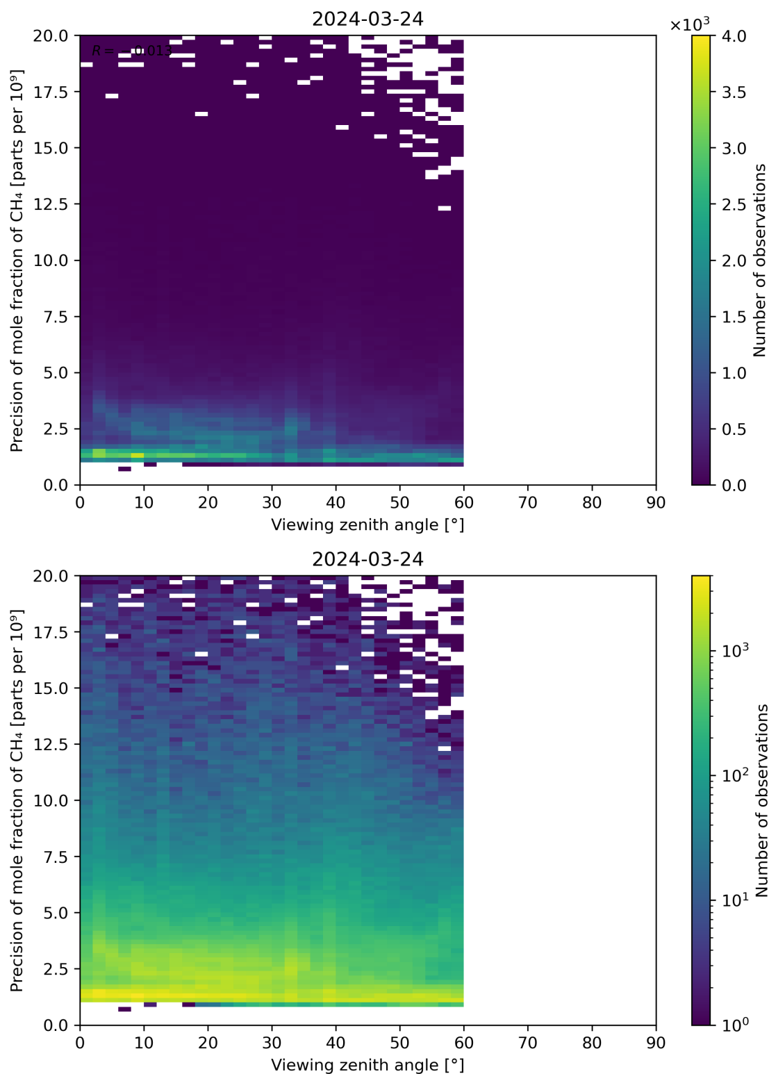
Figure 112: Scatter density plot of “Viewing zenith angle” against “Precision of mole fraction of CH 4 ” for 2024-03-23 to 2024-03-25.
