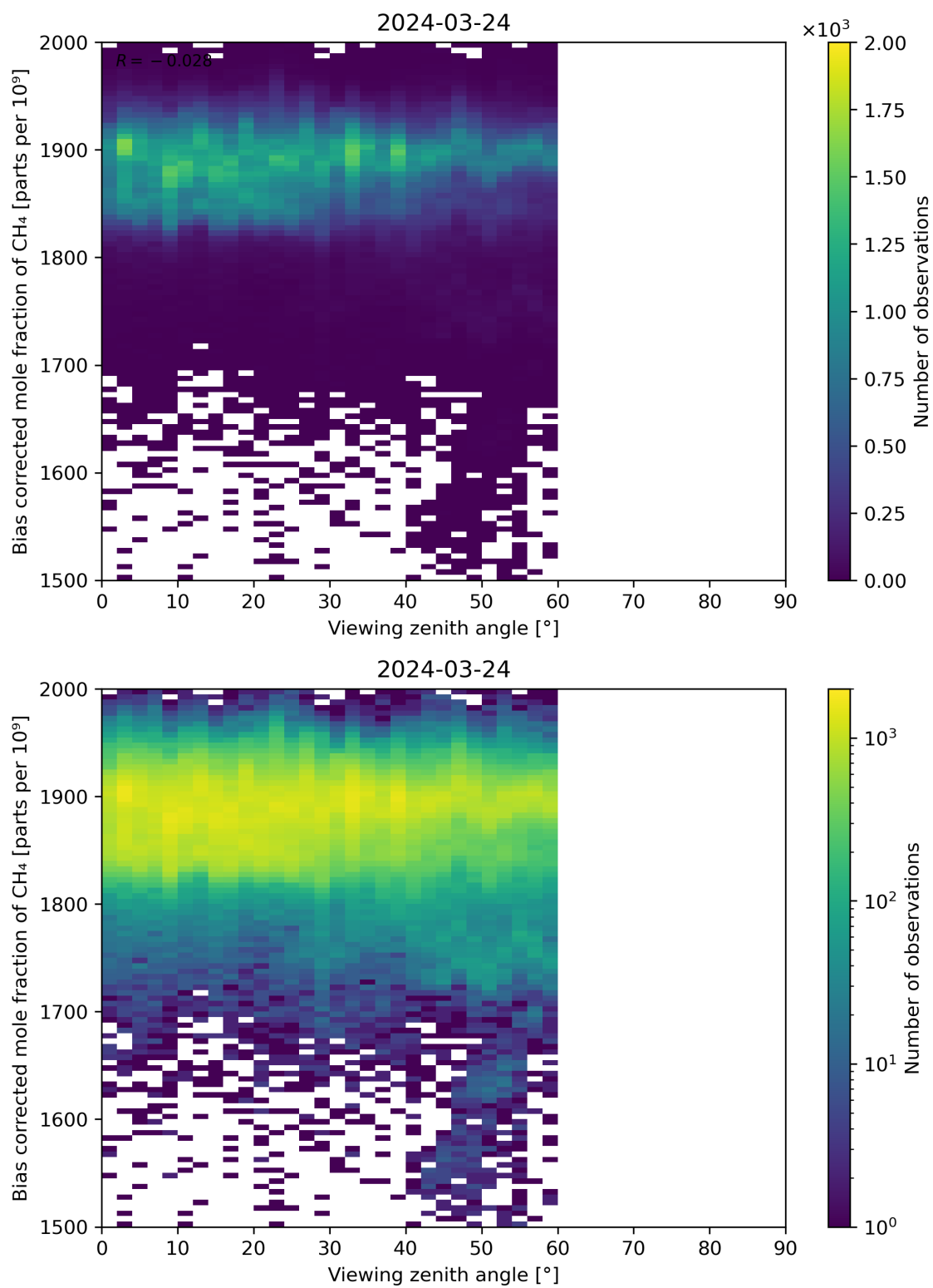
Figure 111: Scatter density plot of “Viewing zenith angle” against “Bias corrected mole fraction of CH 4 ” for 2024-03-23 to 2024-03-25.
