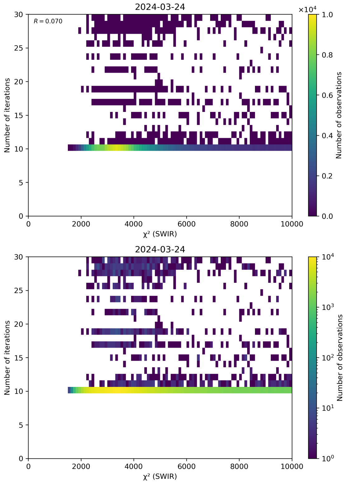
Figure 50: Scatter density plot of “ \chi^2 (SWIR)” against “Number of iterations” for 2024-03-23 to 2024-03-25.
