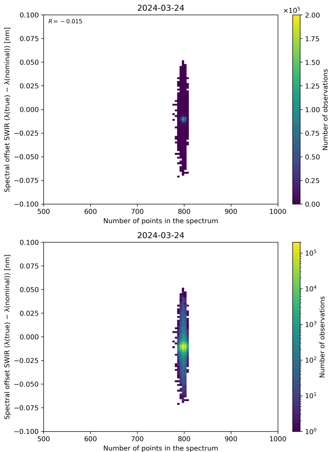
Figure 93: Scatter density plot of “Number of points in the spectrum” against “Spectral offset SWIR ( \lambda(\text{true}) - \lambda(\text{nominal}) )” for 2024-03-23 to 2024-03-25.
