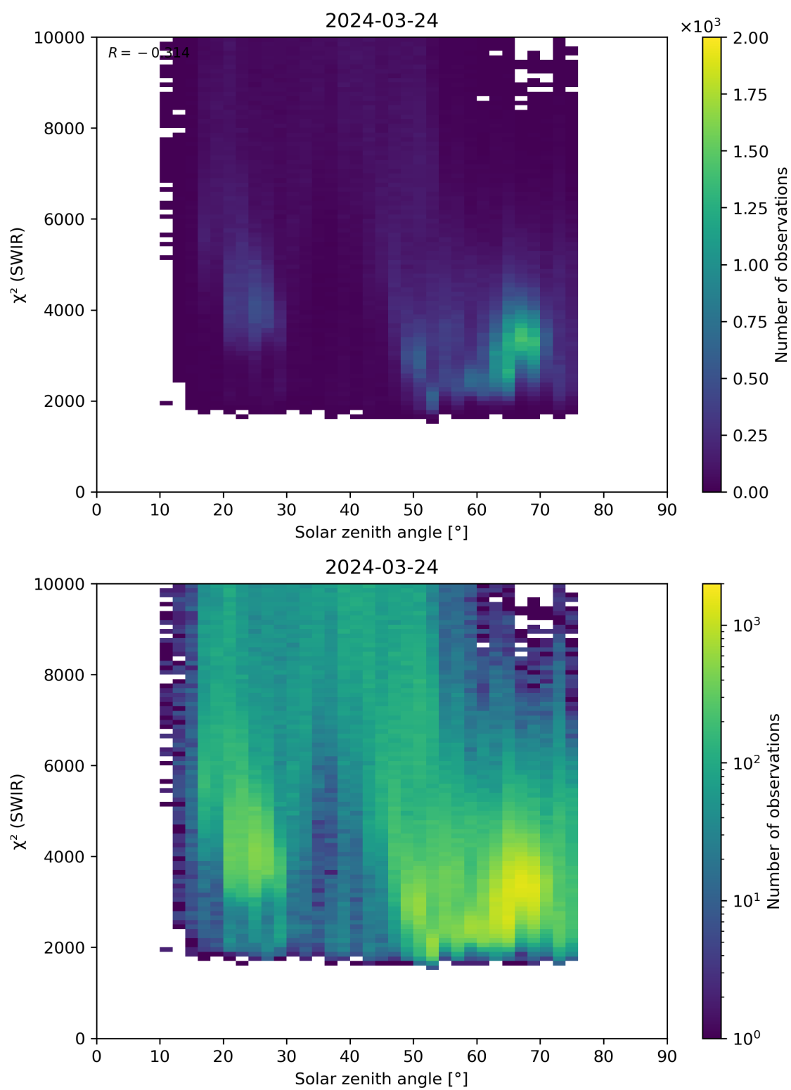
Figure 95: Scatter density plot of “Solar zenith angle” against “ \chi^2 (SWIR)” for 2024-03-23 to 2024-03-25.
