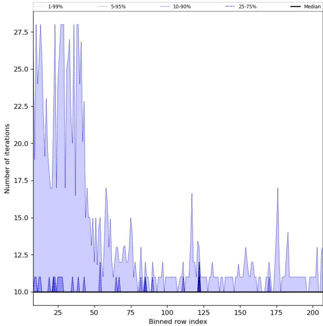
Figure 42: Along track statistics of “Number of iterations” for 2024-03-23 to 2024-03-25
