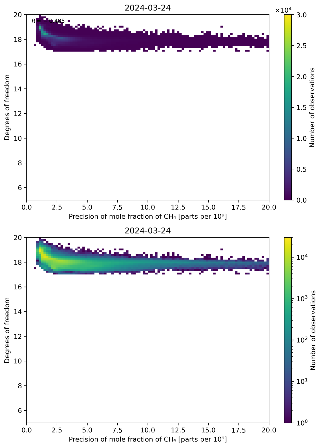
Figure 80: Scatter density plot of “Precision of mole fraction of CH 4 ” against “Degrees of freedom” for 2024-03-23 to 2024-03-25.
