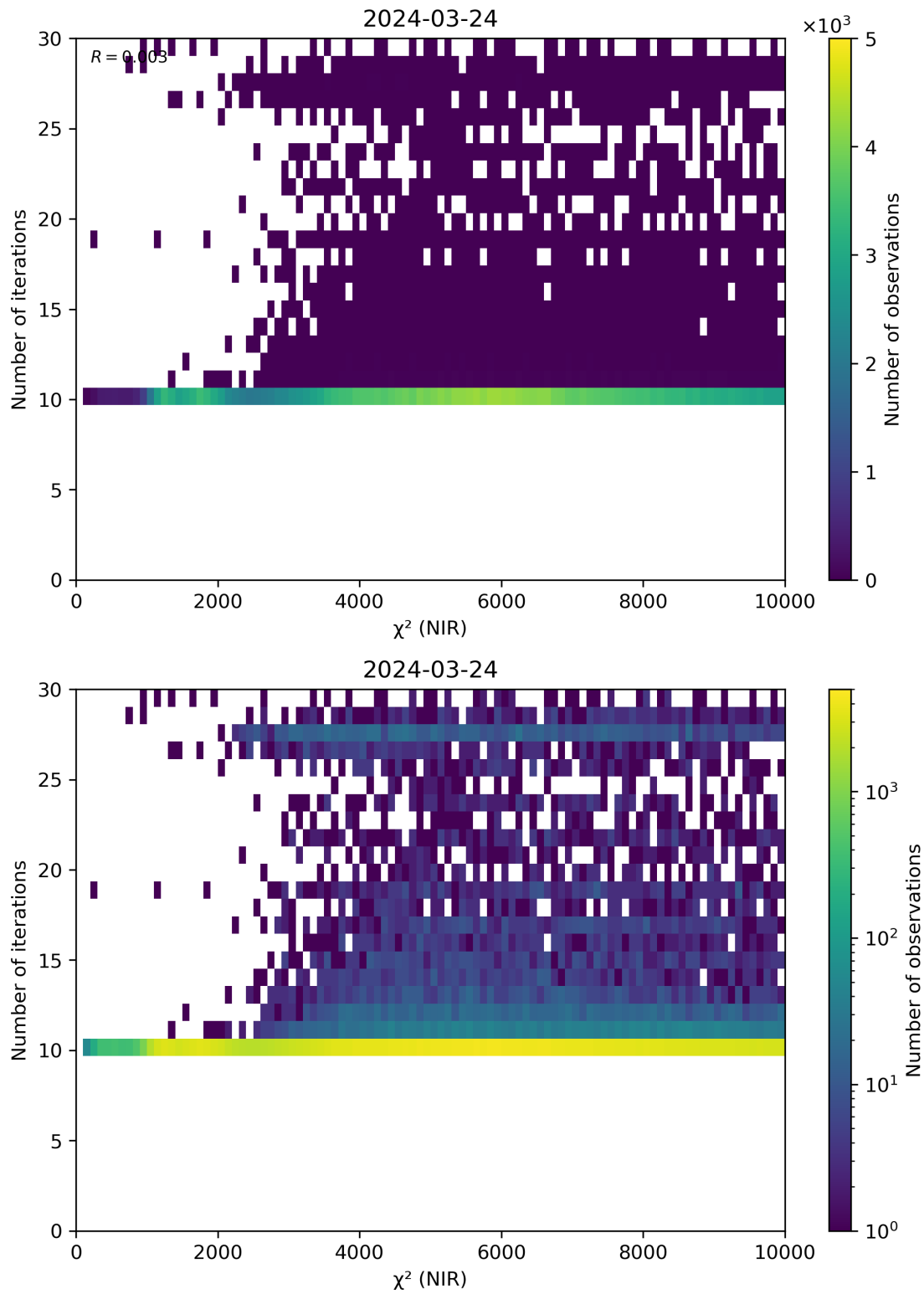
Figure 46: Scatter density plot of “ \chi^2 (NIR)” against “Number of iterations” for 2024-03-23 to 2024-03-25.
