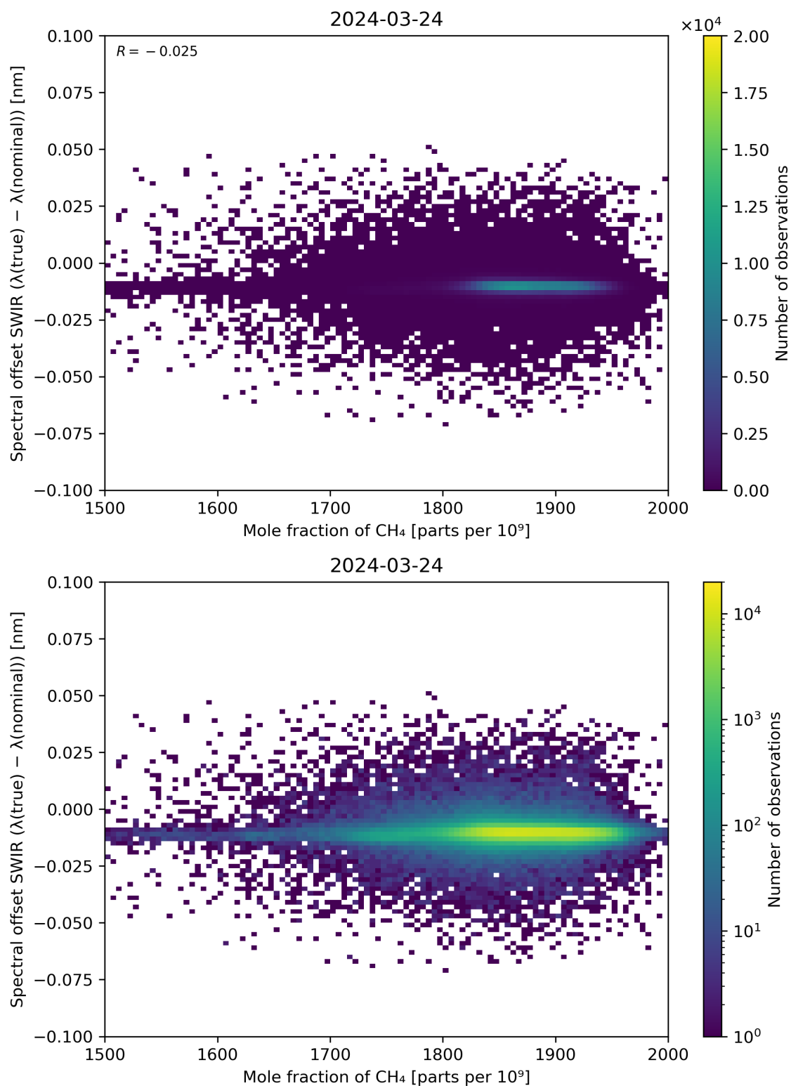
Figure 86: Scatter density plot of “Mole fraction of \text{CH}_4 ” against “Spectral offset SWIR ( \lambda(\text{true}) - \lambda(\text{nominal}) )” for 2024-03-23 to 2024-03-25.
