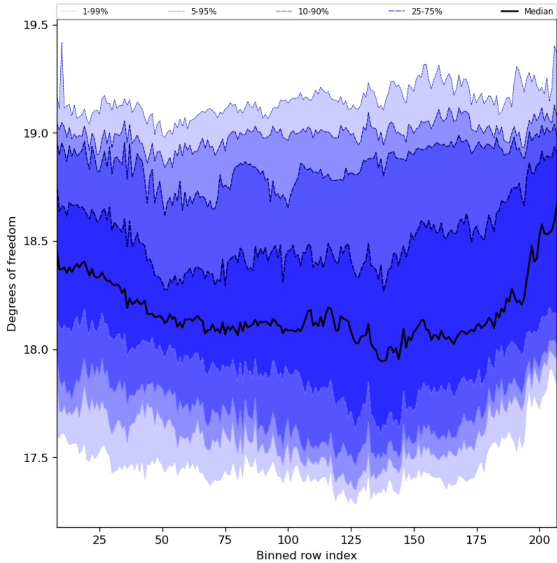
Figure 41: Along track statistics of “Degrees of freedom” for 2024-03-23 to 2024-03-25
