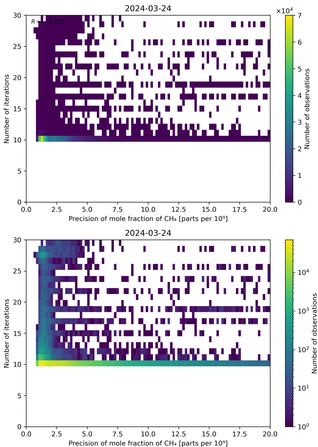
Figure 83: Scatter density plot of “Precision of mole fraction of CH 4 ” against “Number of iterations” for 2024-03-23 to 2024-03-25.
