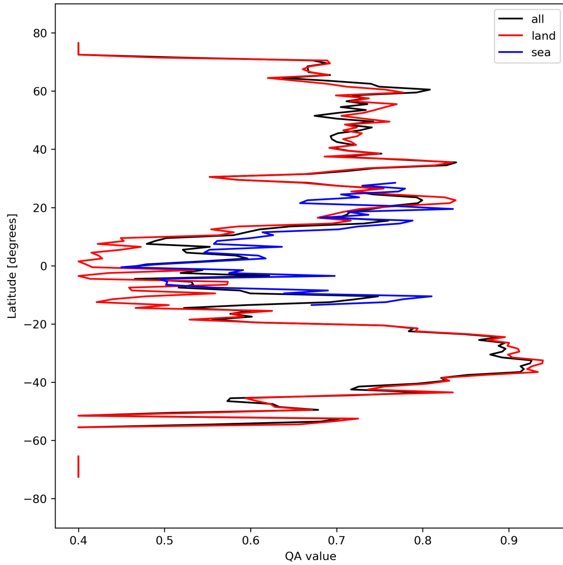
Figure 11: Zonal average of “QA value” for 2024-03-23 to 2024-03-25.
