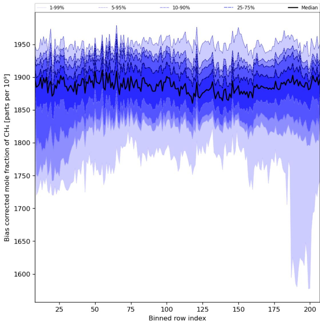
Figure 36: Along track statistics of “Bias corrected mole fraction of CH 4 ” for 2024-03-23 to 2024-03-25
