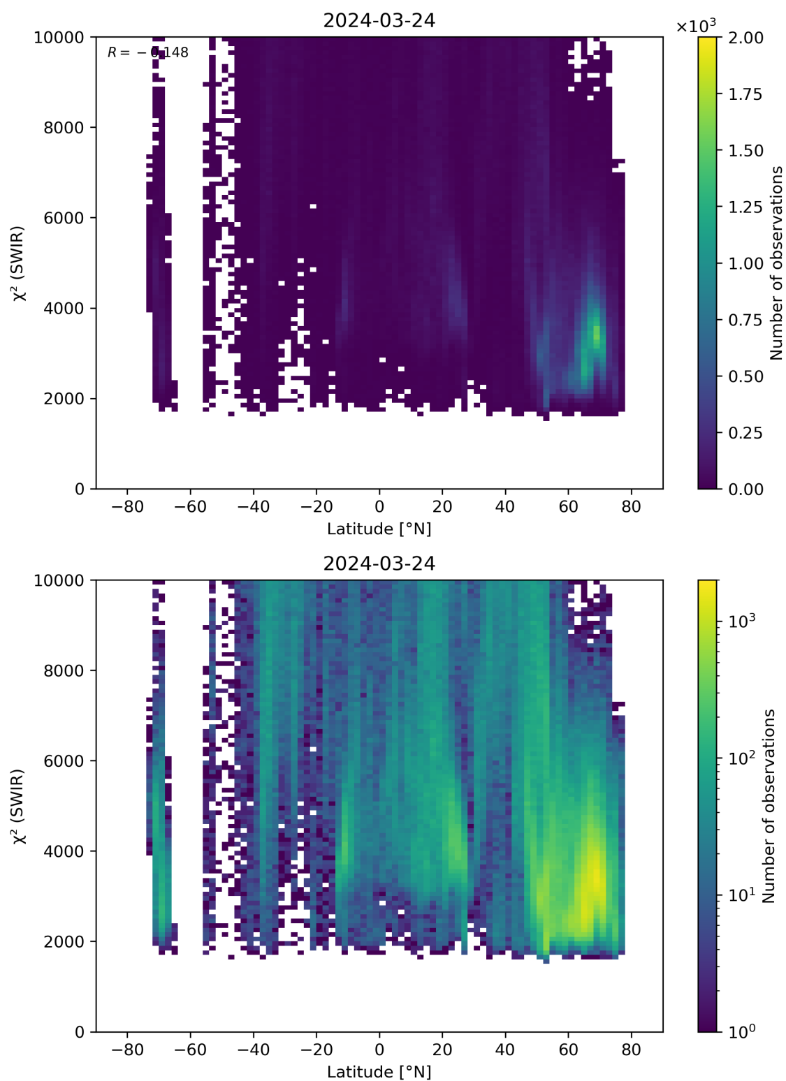
Figure 54: Scatter density plot of “Latitude” against “ \chi^2 (SWIR)” for 2024-03-23 to 2024-03-25.
