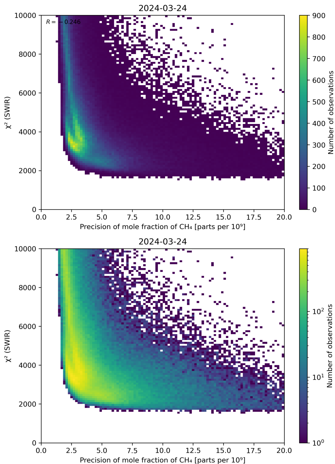
Figure 79: Scatter density plot of “Precision of mole fraction of \text{CH}_4 ” against “ \chi^2 (SWIR)” for 2024-03-23 to 2024-03-25.
