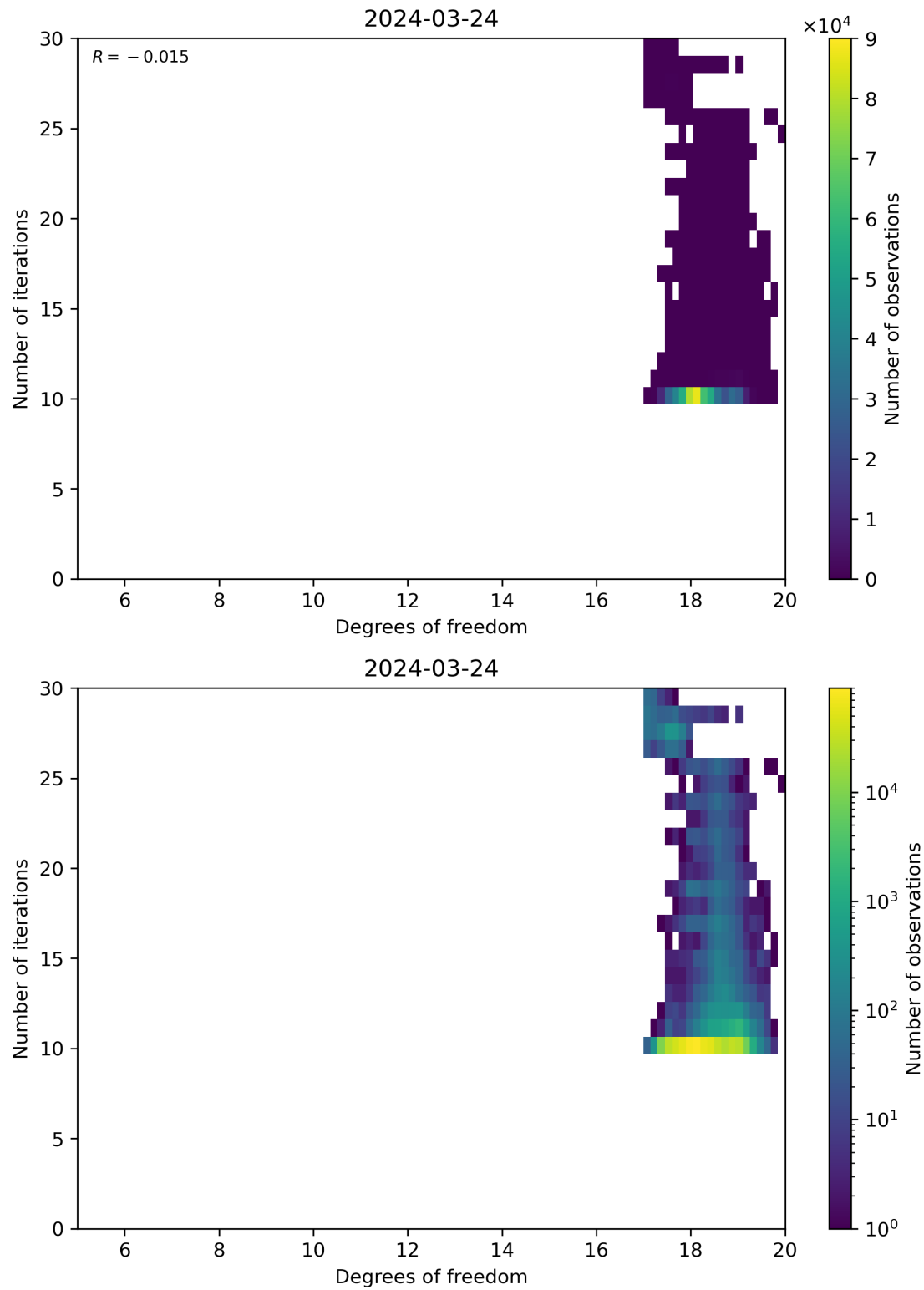
Figure 52: Scatter density plot of “Degrees of freedom” against “Number of iterations” for 2024-03-23 to 2024-03-25.
