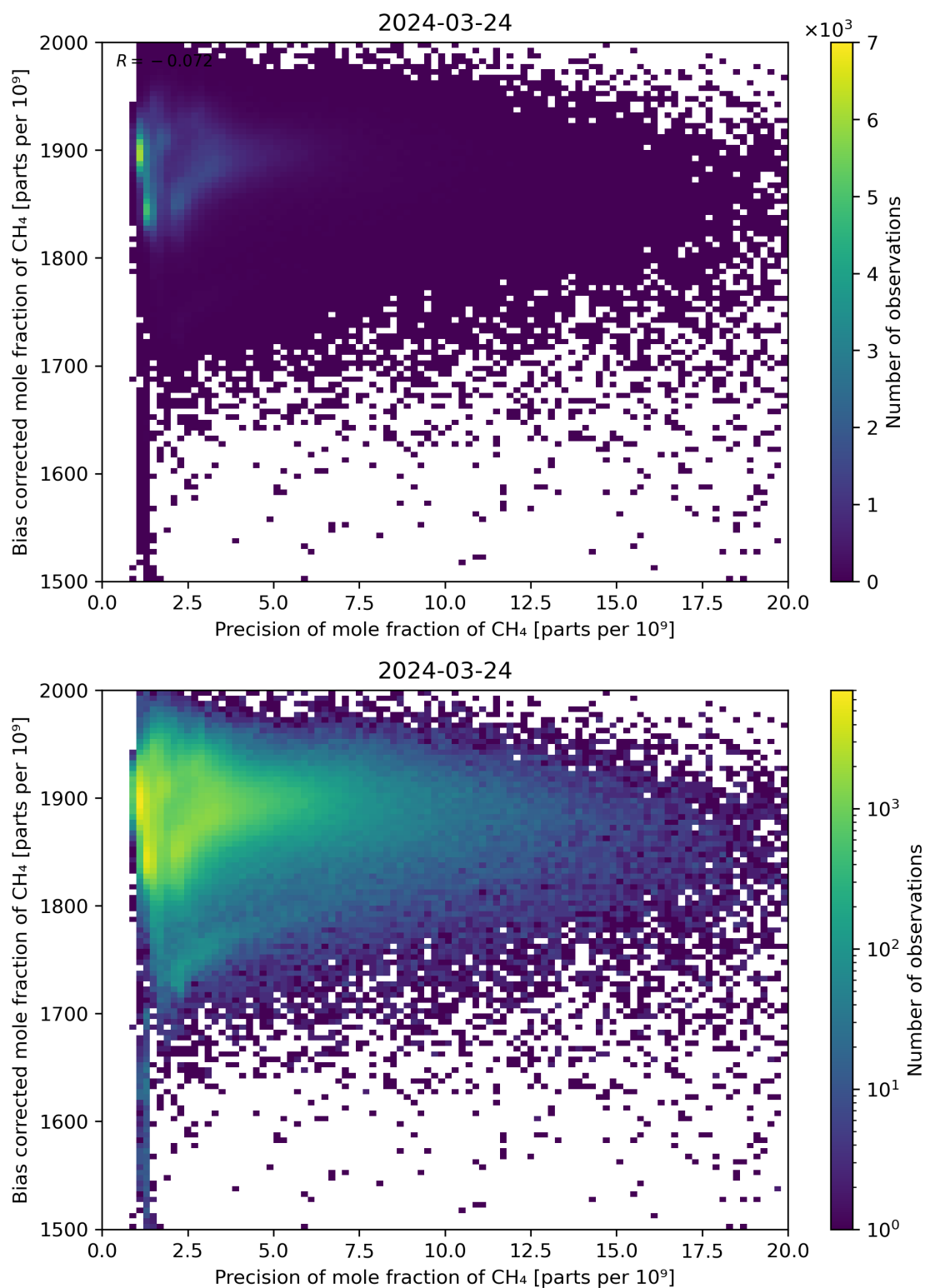
Figure 82: Scatter density plot of “Precision of mole fraction of CH 4 ” against “Bias corrected mole fraction of CH 4 ” for 2024-03-23 to 2024-03-25.
