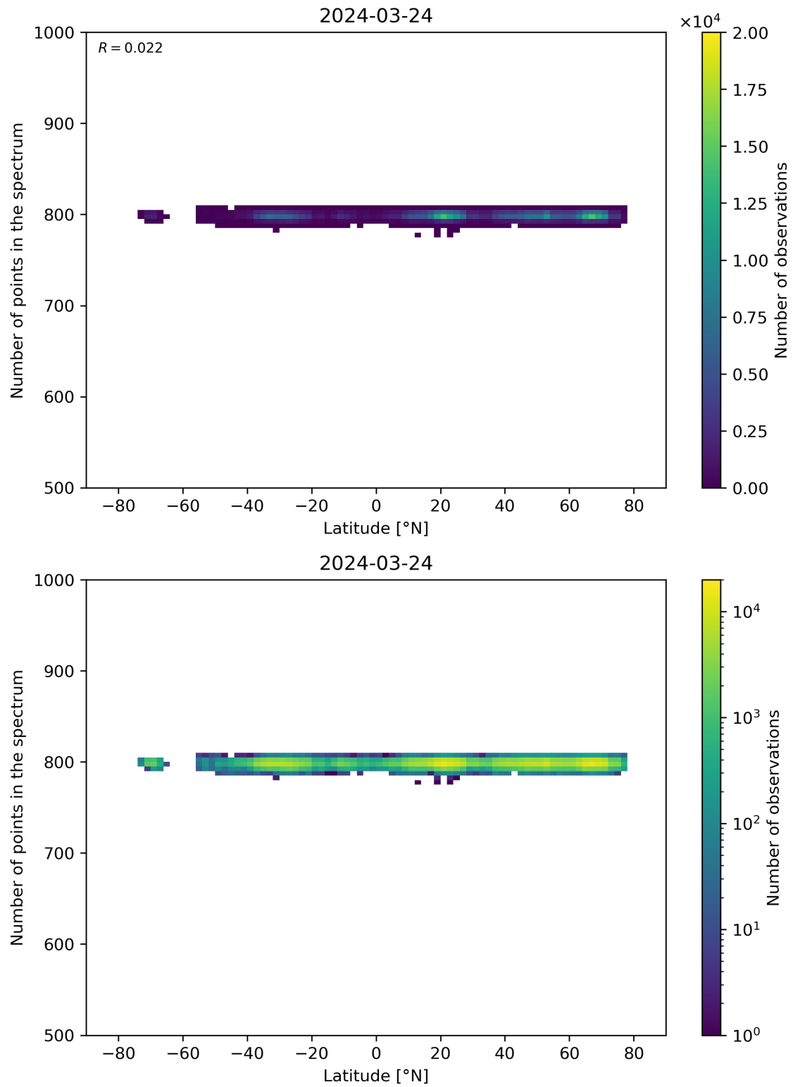
Figure 61: Scatter density plot of “Latitude” against “Number of points in the spectrum” for 2024-03-23 to 2024-03-25.
