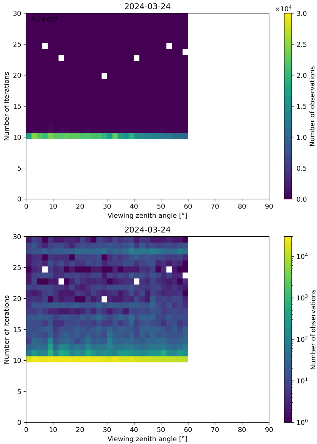
Figure 113: Scatter density plot of “Viewing zenith angle” against “Number of iterations” for 2024-03-23 to 2024-03-25.
