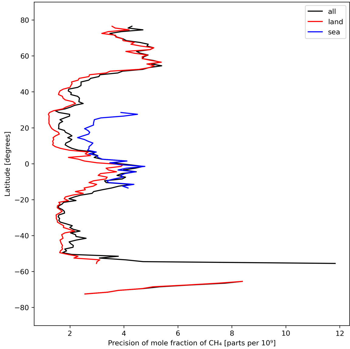
Figure 13: Zonal average of “Precision of mole fraction of CH 4 ” for 2024-03-23 to 2024-03-25.
