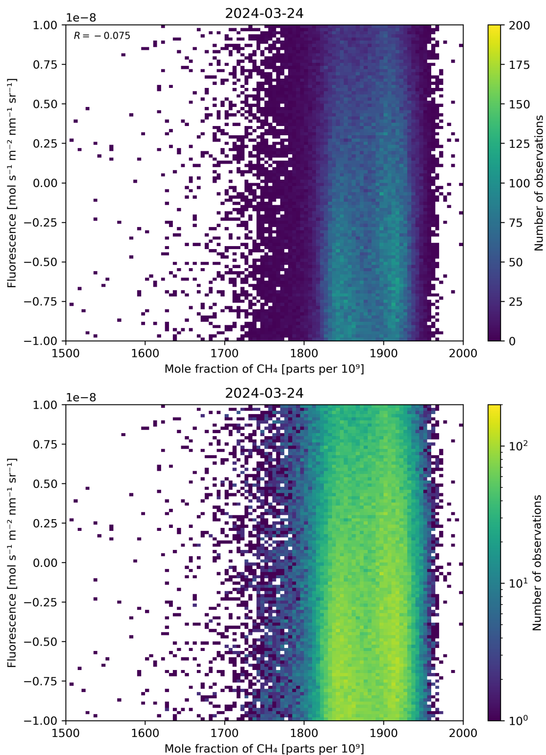
Figure 73: Scatter density plot of “Mole fraction of \text{CH}_4 ” against “Fluorescence” for 2024-03-23 to 2024-03-25.
