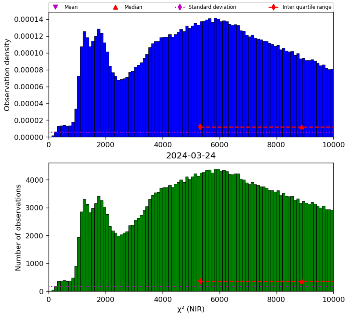
Figure 29: Histogram of “ \chi^2 (NIR)” for 2024-03-23 to 2024-03-25
