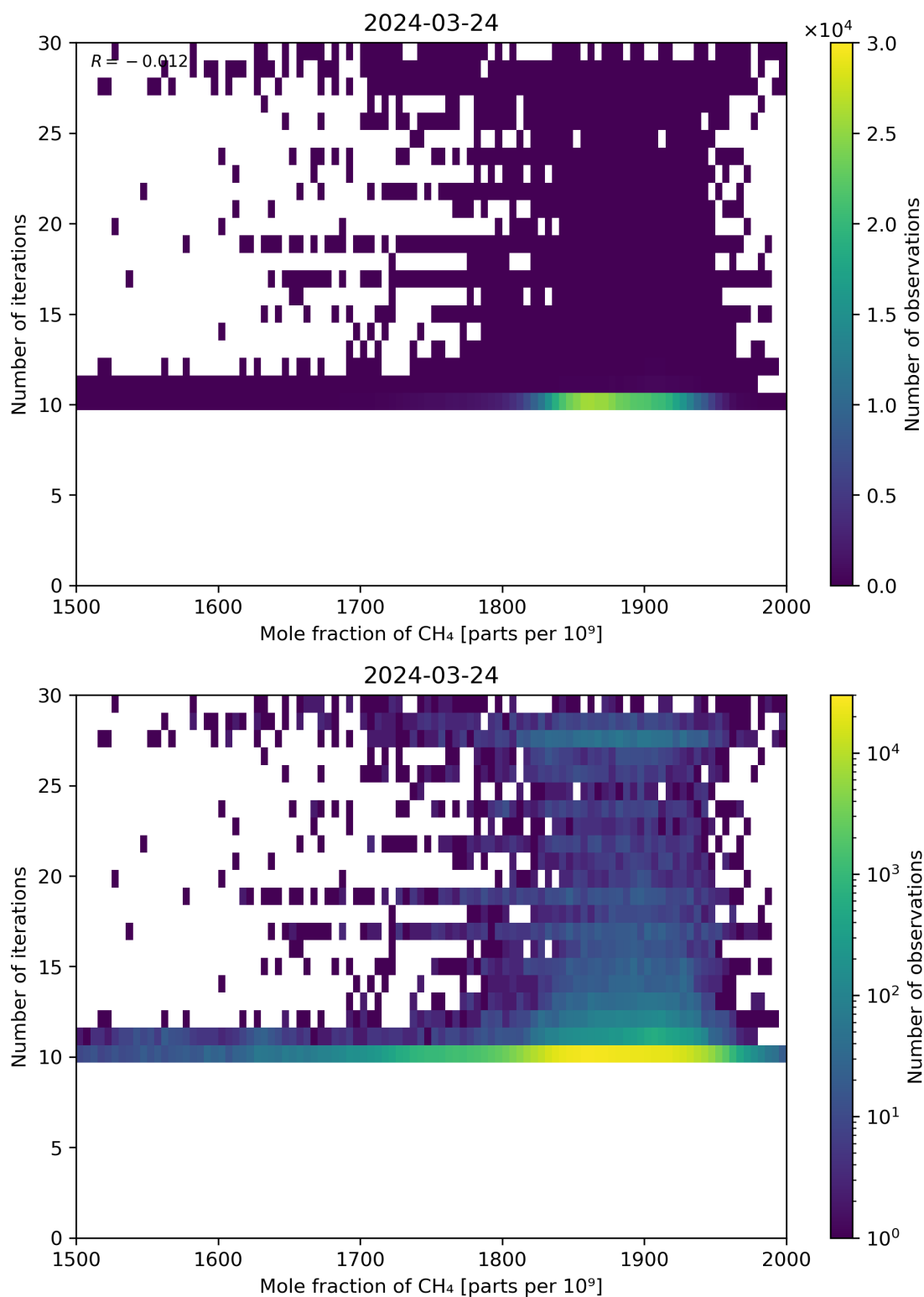
Figure 76: Scatter density plot of “Mole fraction of CH 4 ” against “Number of iterations” for 2024-03-23 to 2024-03-25.
