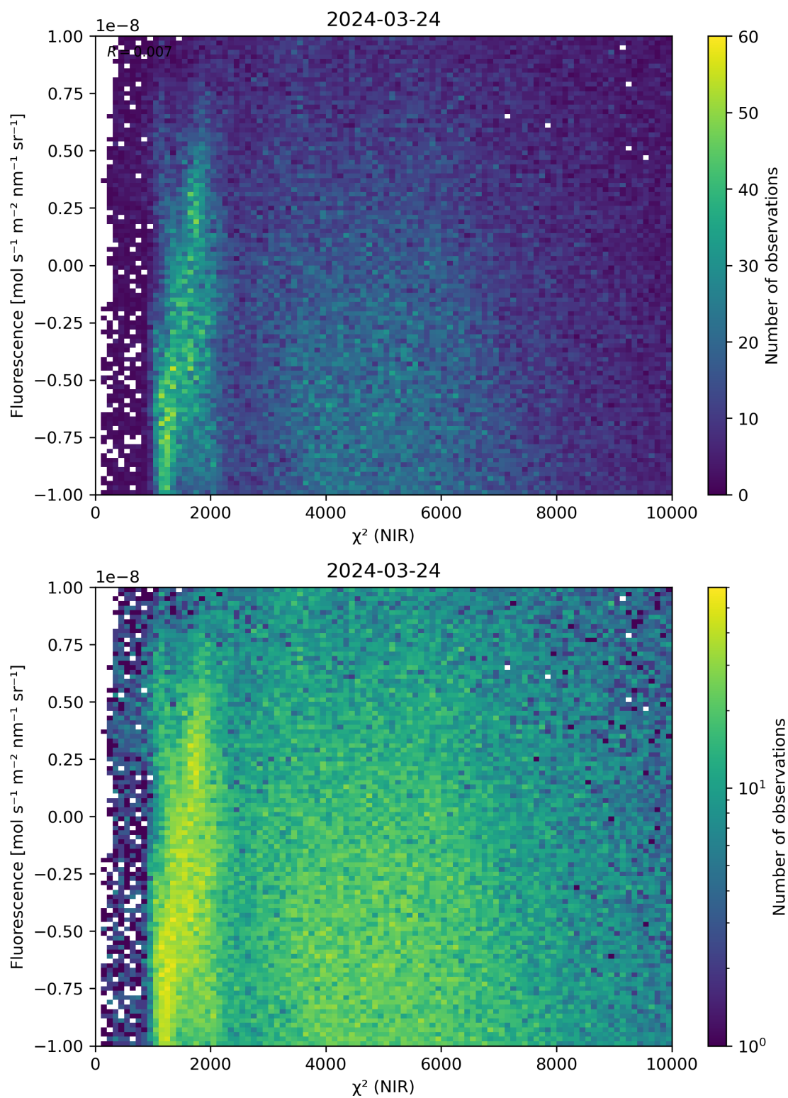
Figure 45: Scatter density plot of “ \chi^2 (NIR)” against “Fluorescence” for 2024-03-23 to 2024-03-25.
