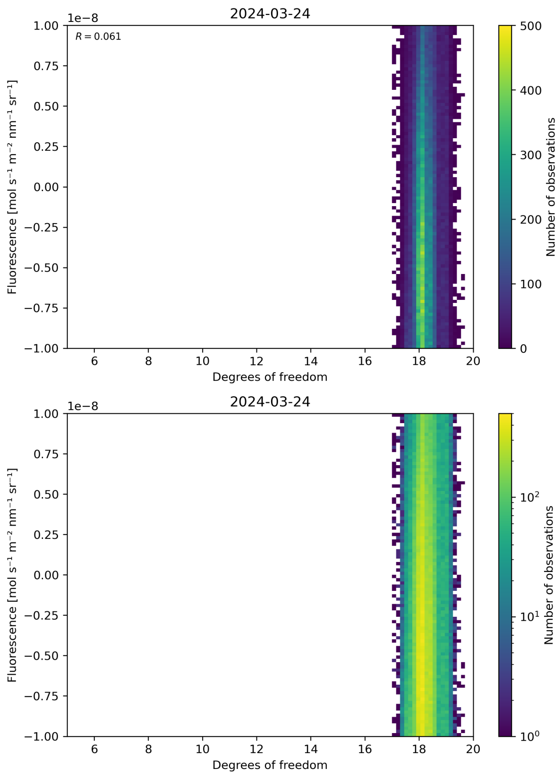
Figure 51: Scatter density plot of “Degrees of freedom” against “Fluorescence” for 2024-03-23 to 2024-03-25.
