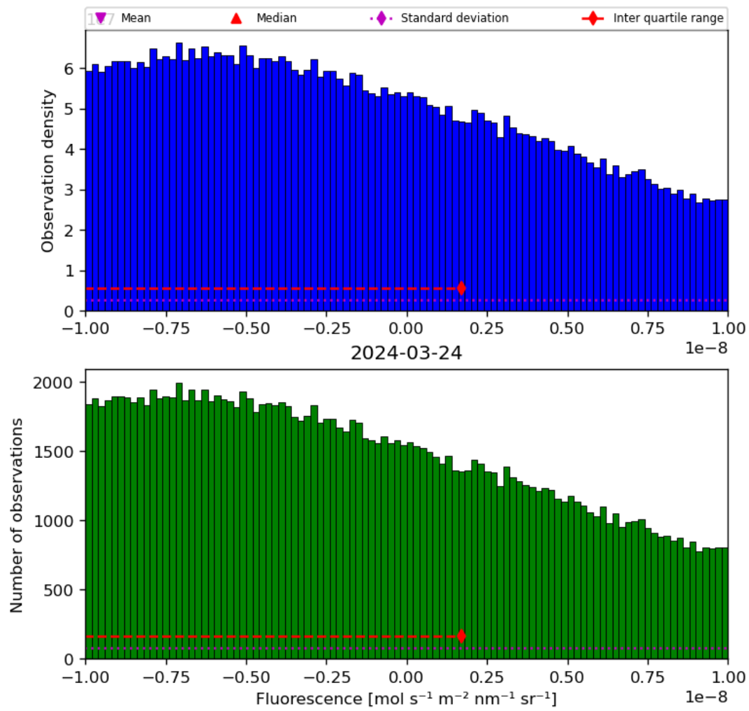
Figure 32: Histogram of “Fluorescence” for 2024-03-23 to 2024-03-25
