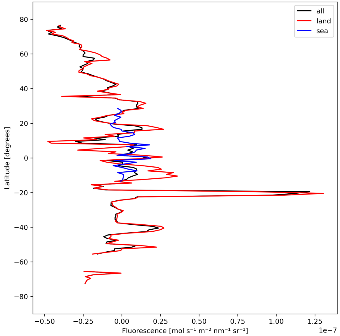
Figure 21: Zonal average of “Fluorescence” for 2024-03-23 to 2024-03-25.
