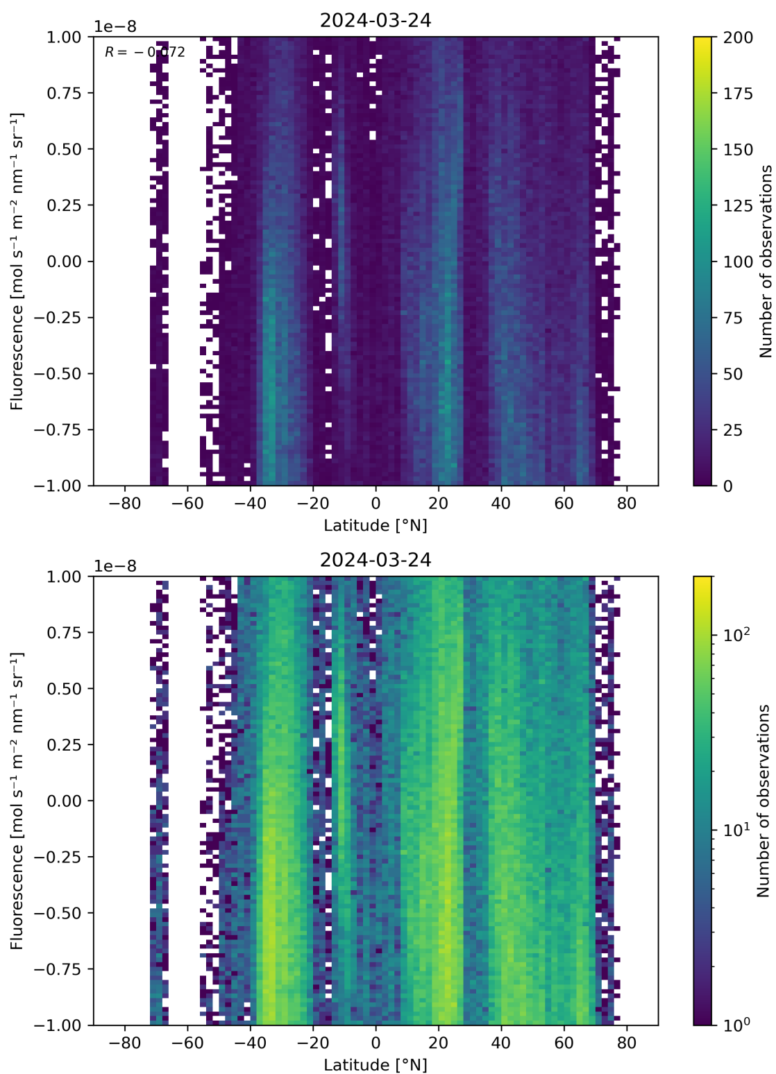
Figure 56: Scatter density plot of “Latitude” against “Fluorescence” for 2024-03-23 to 2024-03-25.
