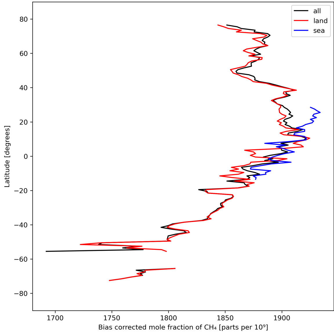
Figure 14: Zonal average of “Bias corrected mole fraction of \text{CH}_4 ” for 2024-03-23 to 2024-03-25.
