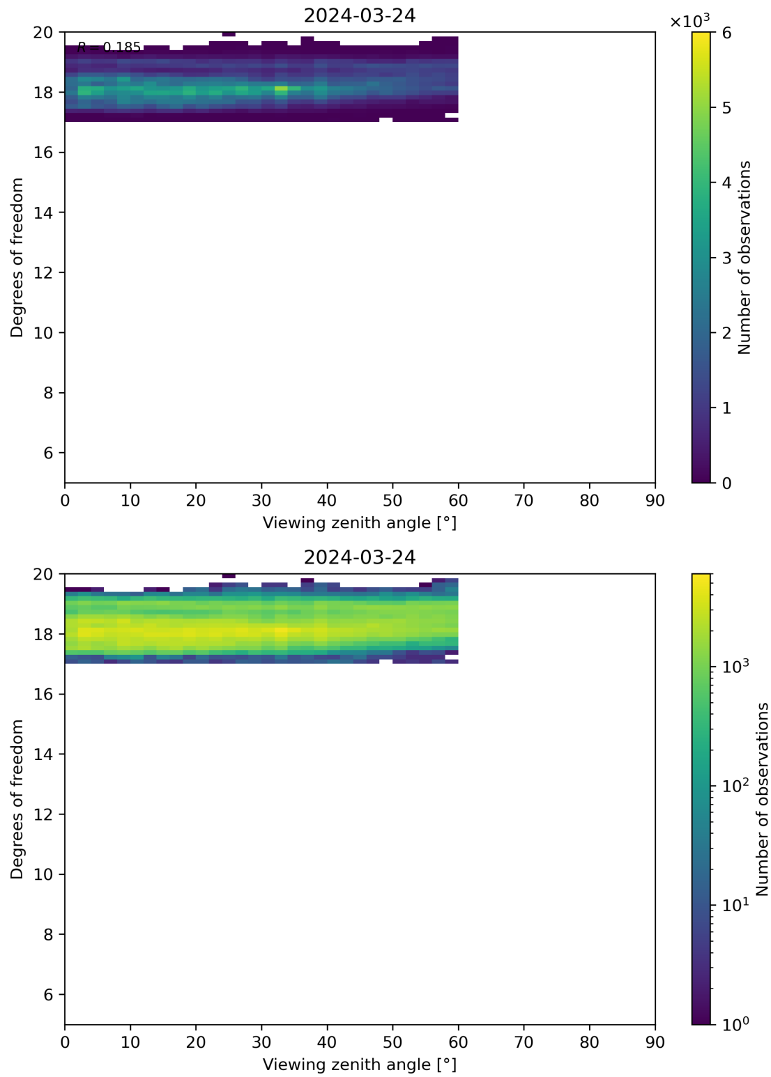
Figure 107: Scatter density plot of “Viewing zenith angle” against “Degrees of freedom” for 2024-03-23 to 2024-03-25.
