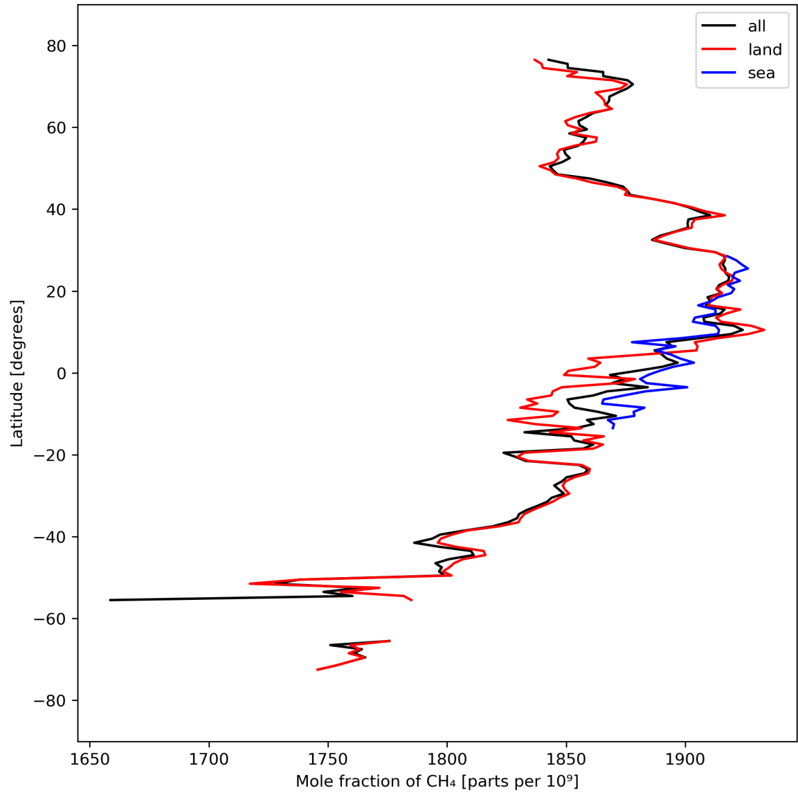
Figure 12: Zonal average of “Mole fraction of CH 4 ” for 2024-03-23 to 2024-03-25.
