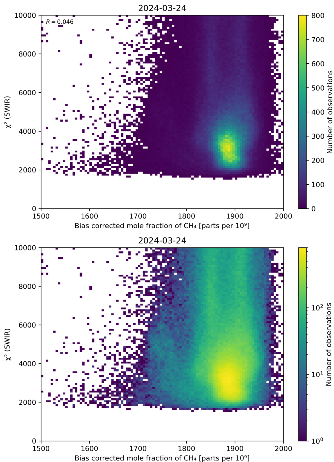
Figure 64: Scatter density plot of “Bias corrected mole fraction of CH 4 ” against “ \chi^2 (SWIR)” for 2024-03-23 to 2024-03-25.
