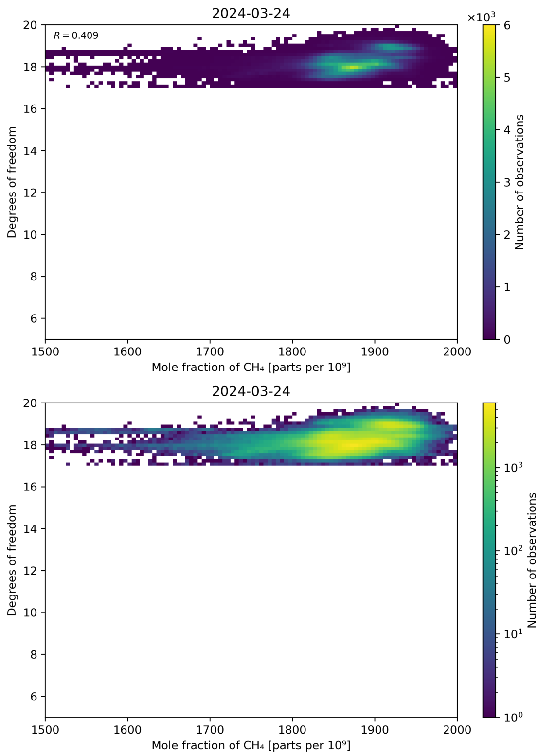
Figure 72: Scatter density plot of “Mole fraction of CH 4 ” against “Degrees of freedom” for 2024-03-23 to 2024-03-25.
