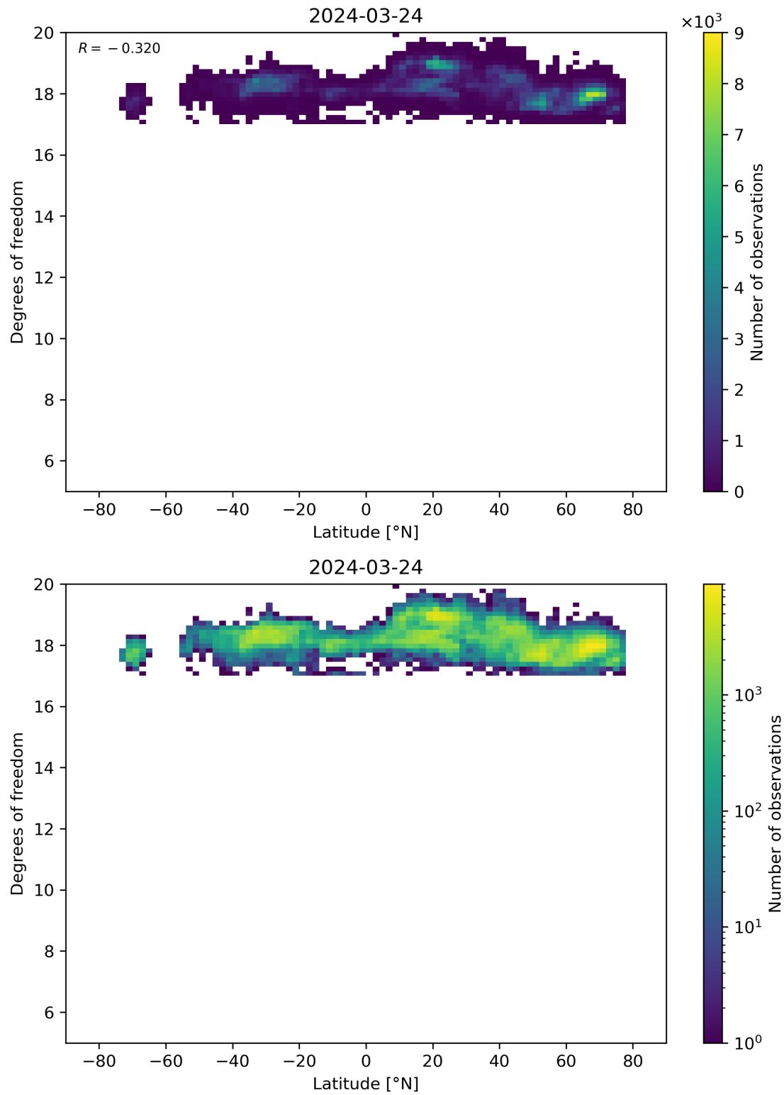
Figure 55: Scatter density plot of “Latitude” against “Degrees of freedom” for 2024-03-23 to 2024-03-25.
