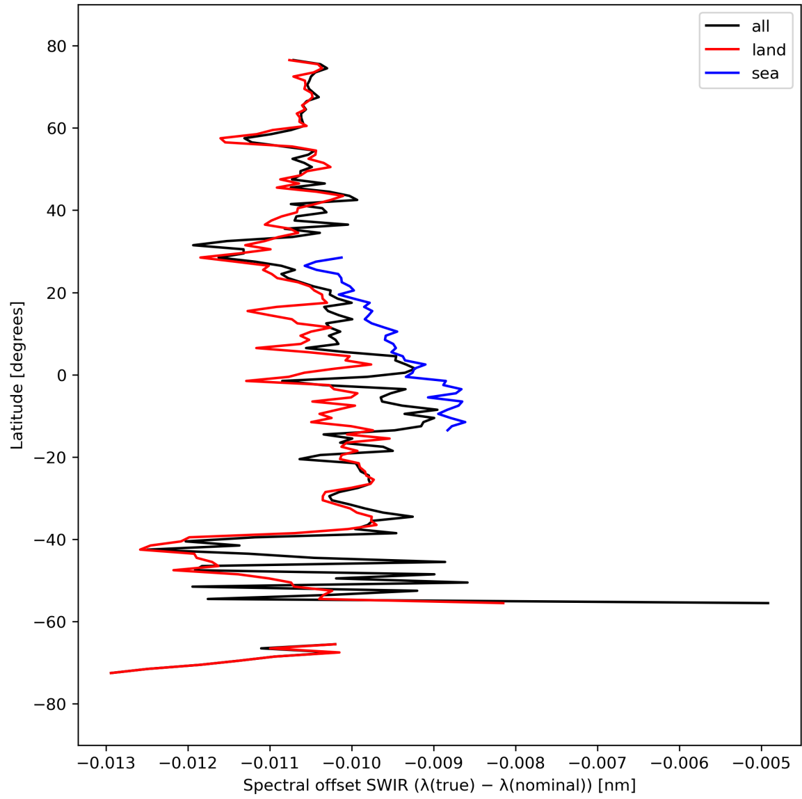
Figure 16: Zonal average of “Spectral offset SWIR ( \lambda(\text{true}) - \lambda(\text{nominal}) )” for 2024-03-23 to 2024-03-25.
