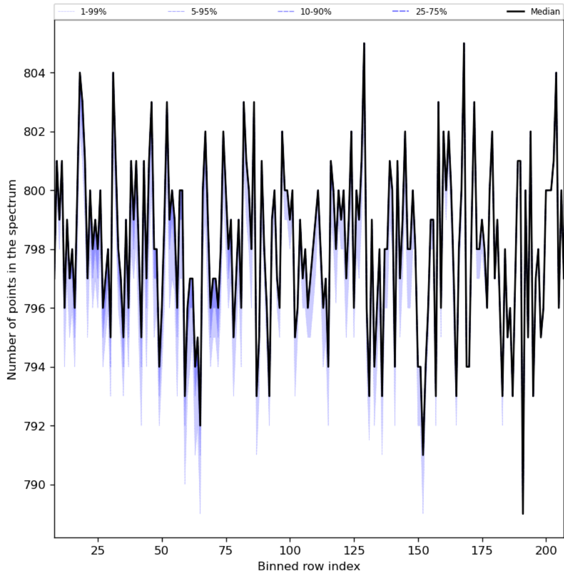
Figure 37: Along track statistics of “Number of points in the spectrum” for 2024-03-23 to 2024-03-25
