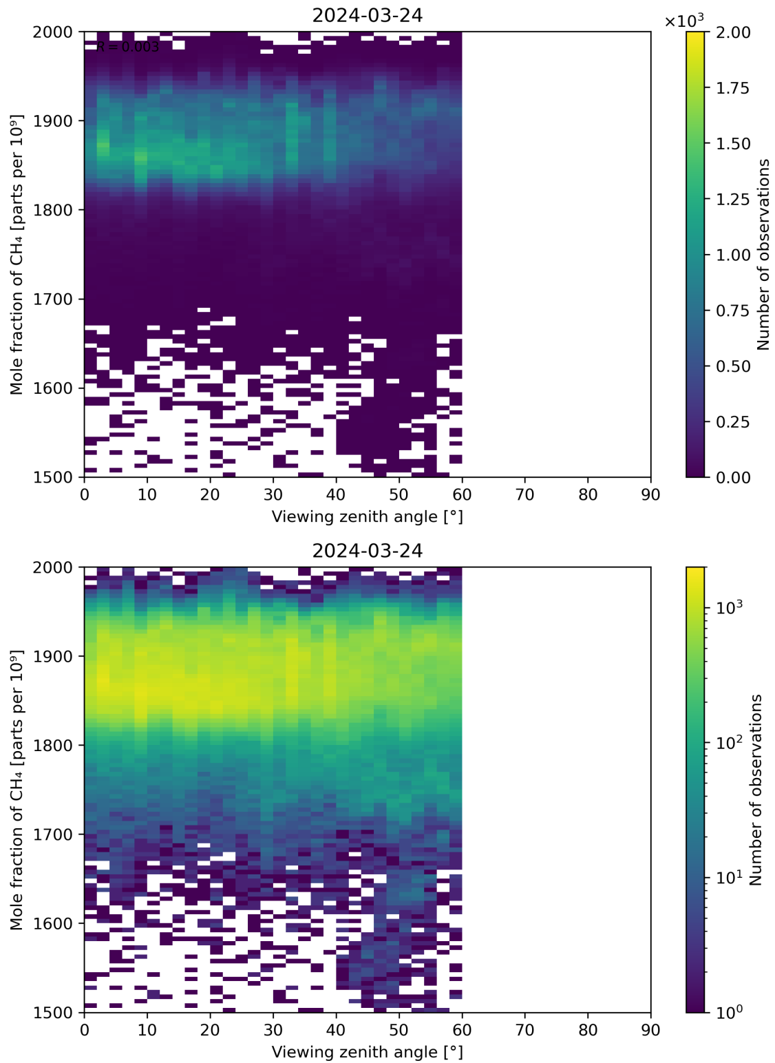
Figure 110: Scatter density plot of “Viewing zenith angle” against “Mole fraction of CH 4 ” for 2024-03-23 to 2024-03-25.
