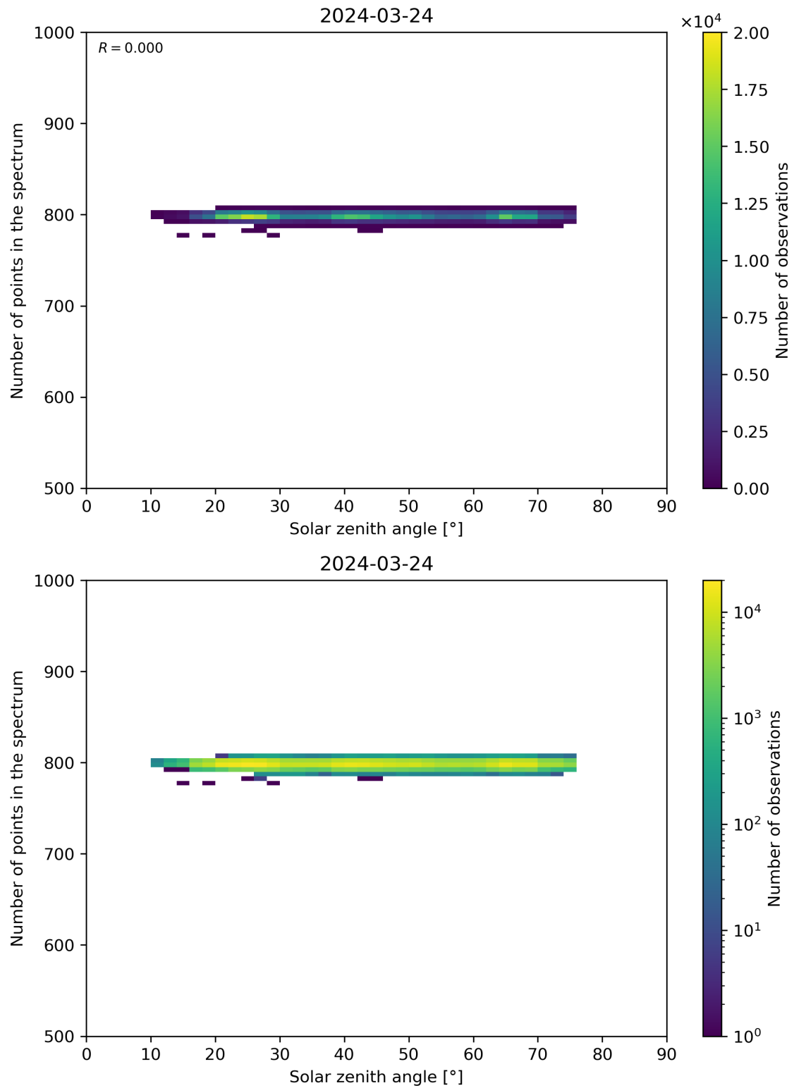
Figure 103: Scatter density plot of “Solar zenith angle” against “Number of points in the spectrum” for 2024-03-23 to 2024-03-25.
