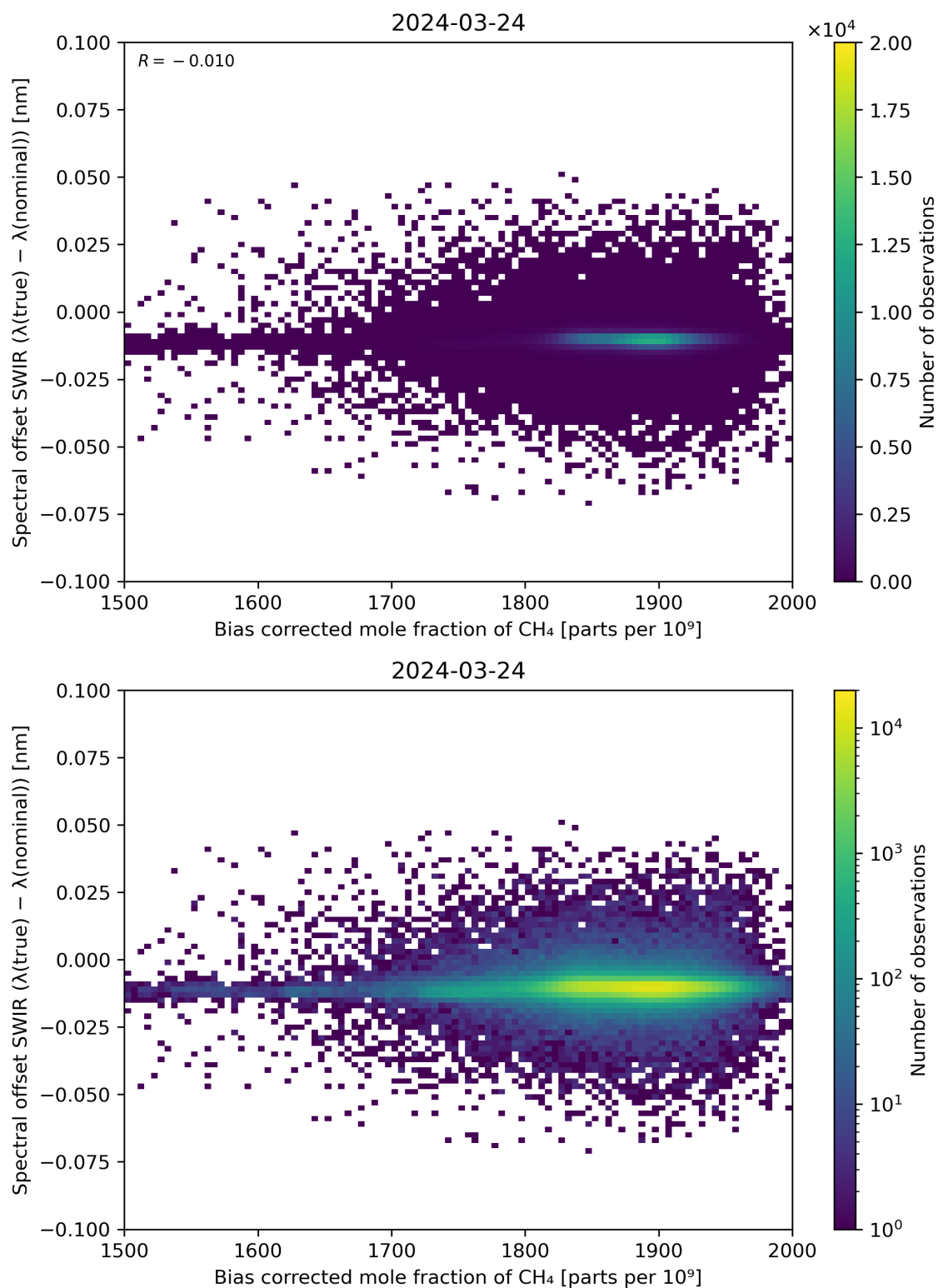
Figure 69: Scatter density plot of “Bias corrected mole fraction of \text{CH}_4 ” against “Spectral offset SWIR ( \lambda(\text{true}) - \lambda(\text{nominal}) )” for 2024-03-23 to 2024-03-25.
