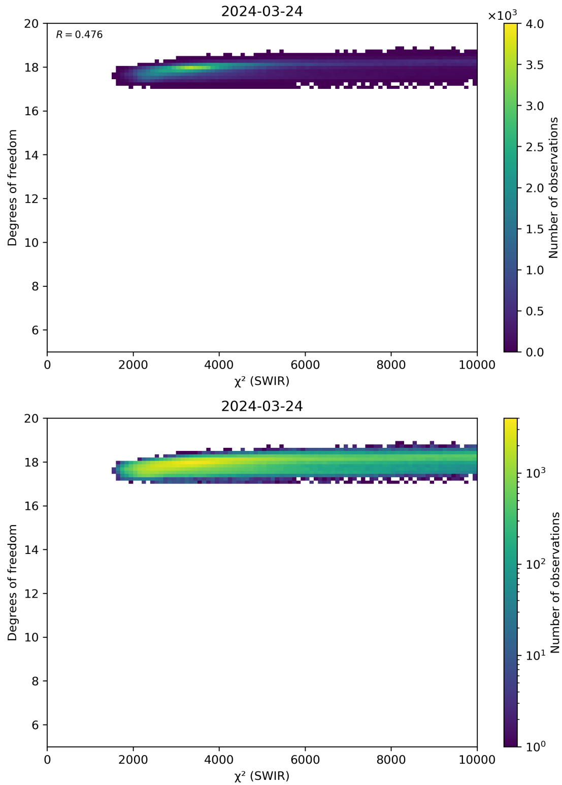
Figure 48: Scatter density plot of “ \chi^2 (SWIR)” against “Degrees of freedom” for 2024-03-23 to 2024-03-25.
