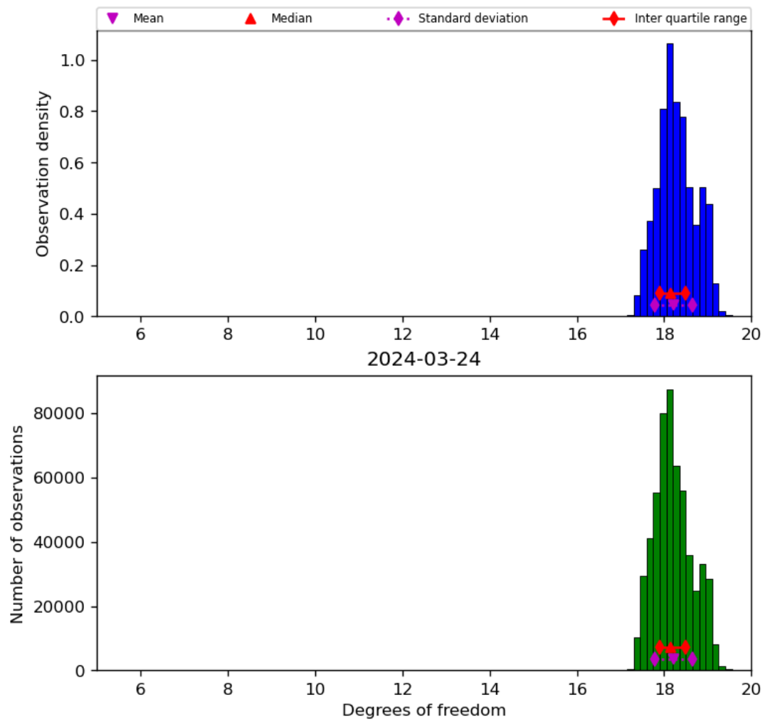
Figure 30: Histogram of “Degrees of freedom” for 2024-03-23 to 2024-03-25
