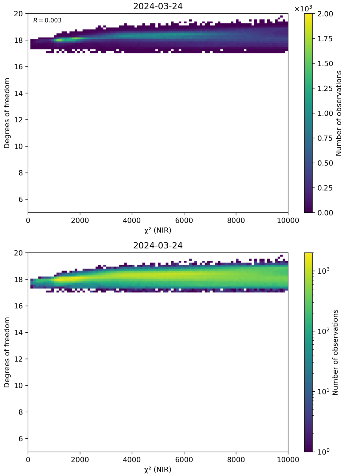
Figure 44: Scatter density plot of “ \chi^2 (NIR)” against “Degrees of freedom” for 2024-03-23 to 2024-03-25.
