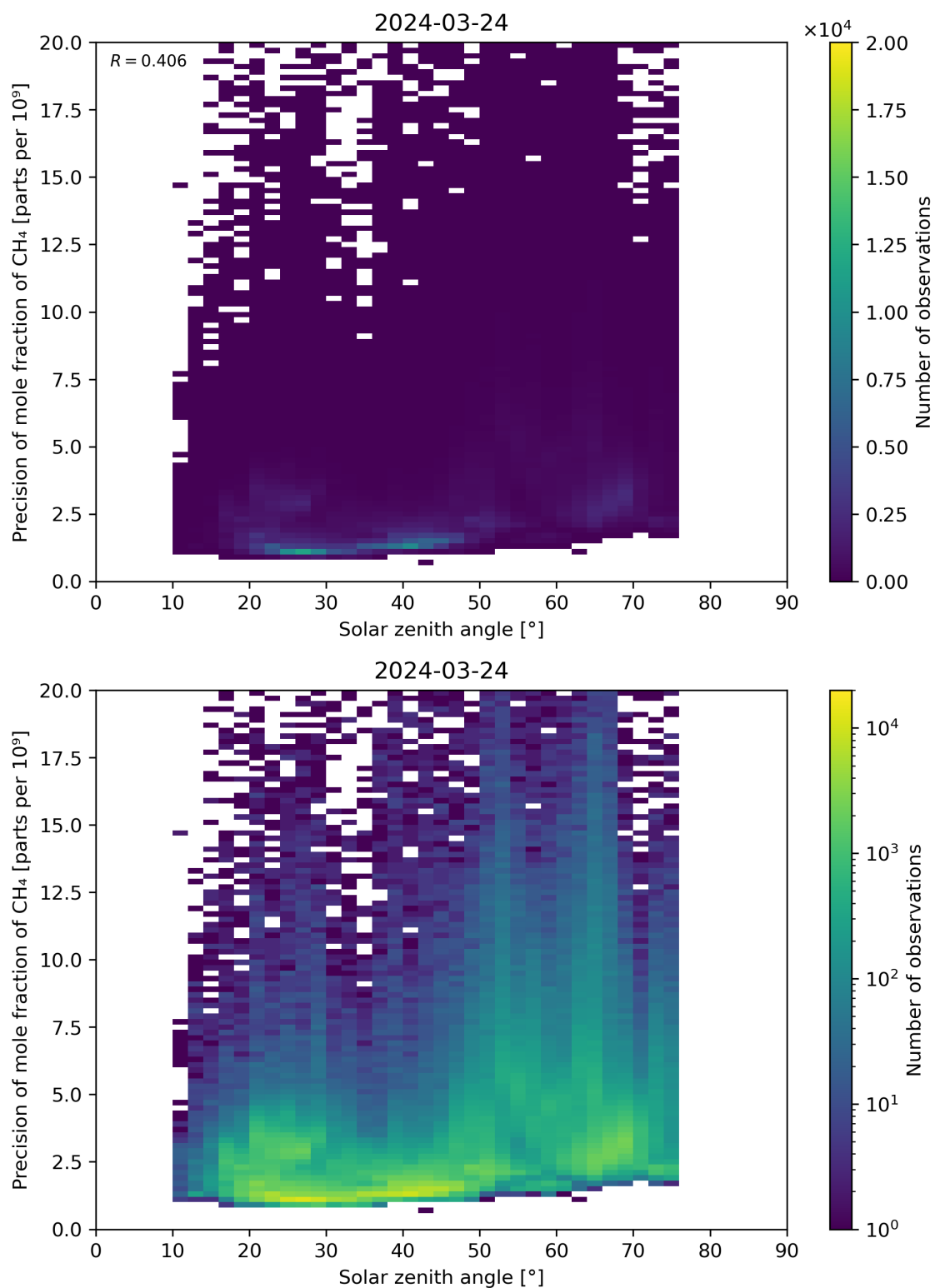
Figure 101: Scatter density plot of “Solar zenith angle” against “Precision of mole fraction of CH 4 ” for 2024-03-23 to 2024-03-25.
