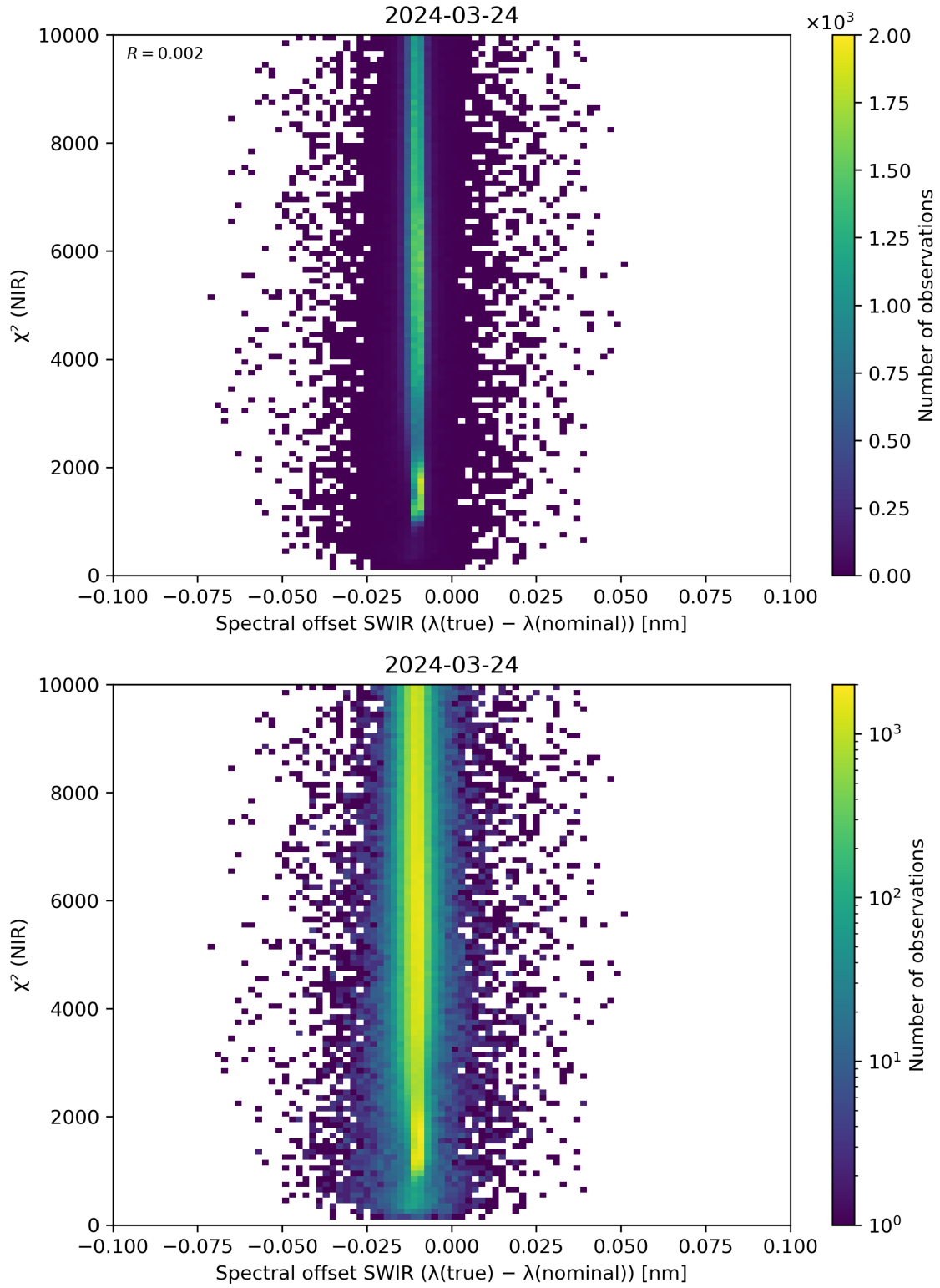
Figure 117: Scatter density plot of “Spectral offset SWIR ( \lambda(\text{true}) - \lambda(\text{nominal}) )” against “ \chi^2 (NIR)” for 2024-03-23 to 2024-03-25.
