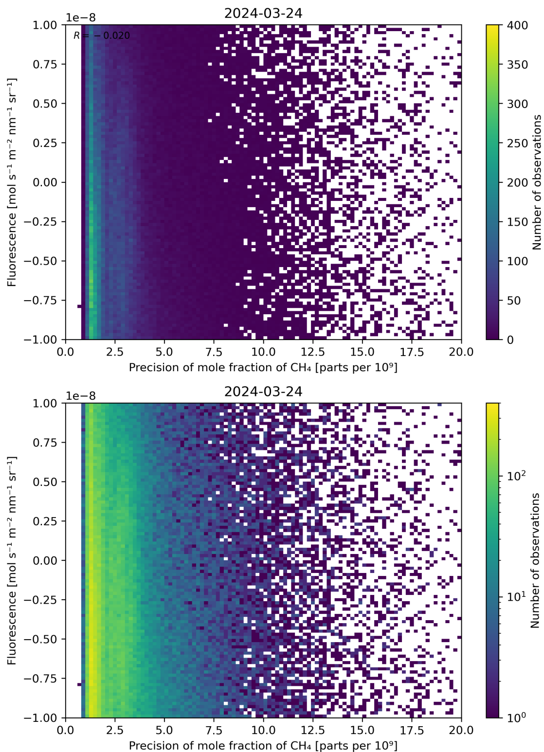
Figure 81: Scatter density plot of “Precision of mole fraction of \text{CH}_4 ” against “Fluorescence” for 2024-03-23 to 2024-03-25.
