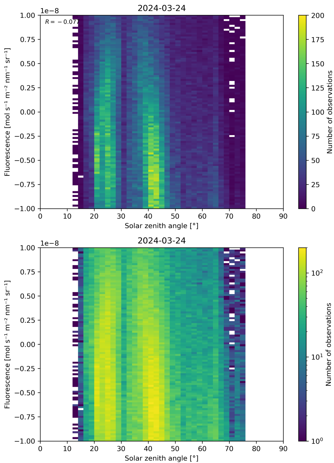
Figure 97: Scatter density plot of “Solar zenith angle” against “Fluorescence” for 2024-03-23 to 2024-03-25.
