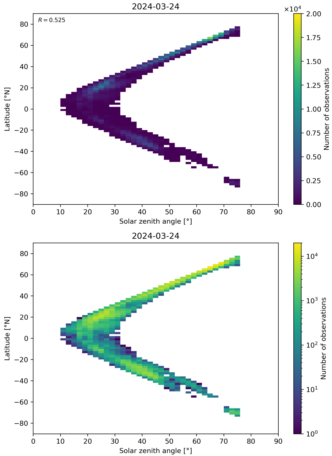
Figure 98: Scatter density plot of “Solar zenith angle” against “Latitude” for 2024-03-23 to 2024-03-25.
