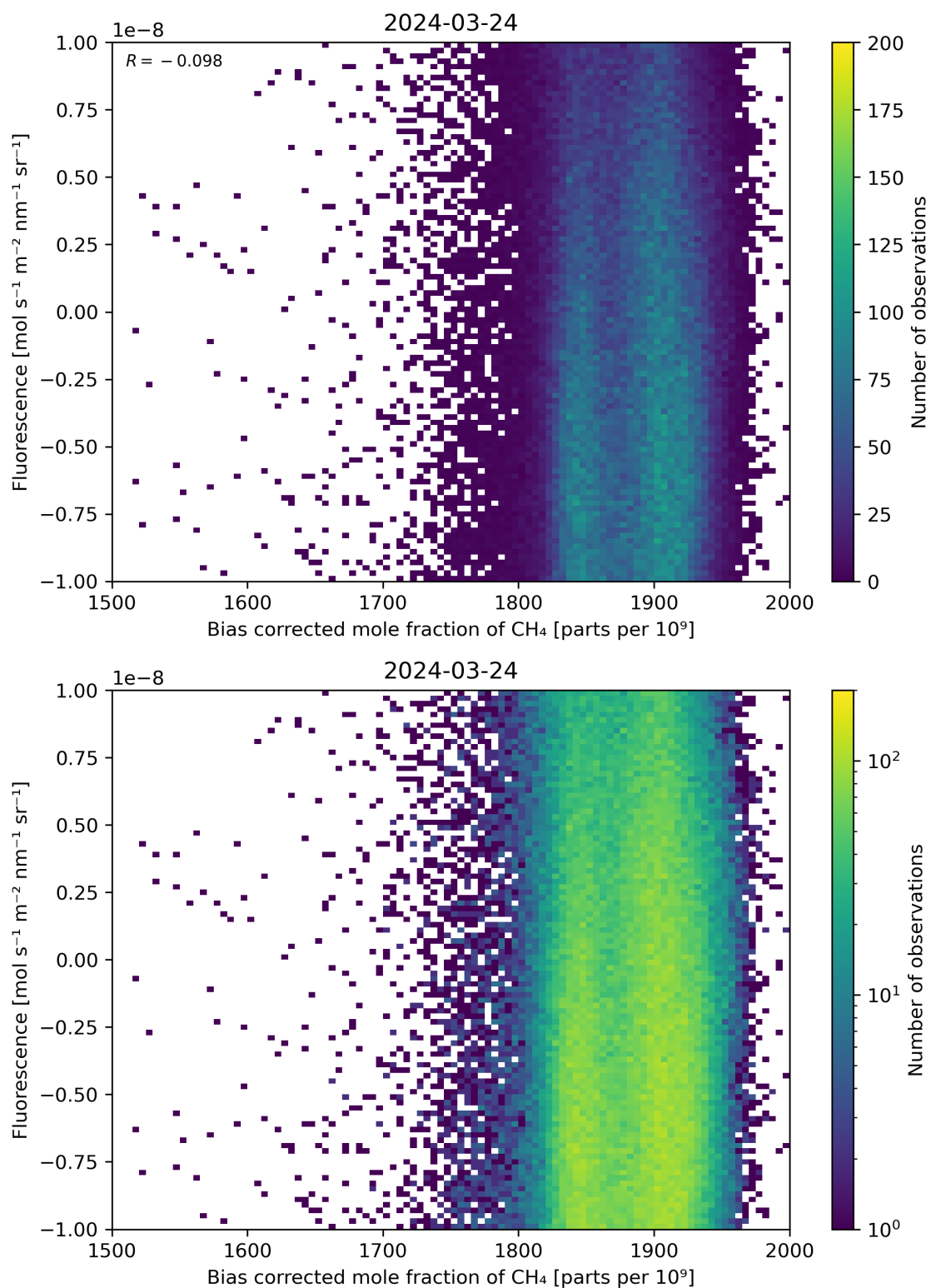
Figure 66: Scatter density plot of “Bias corrected mole fraction of \text{CH}_4 ” against “Fluorescence” for 2024-03-23 to 2024-03-25.
