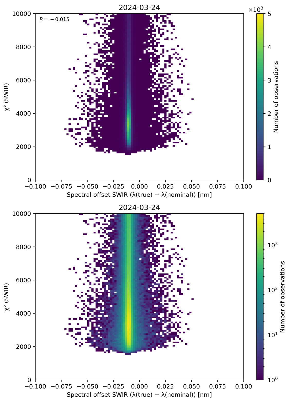
Figure 118: Scatter density plot of “Spectral offset SWIR ( \lambda(\text{true}) - \lambda(\text{nominal}) )” against “ \chi^2 (SWIR)” for 2024-03-23 to 2024-03-25.
