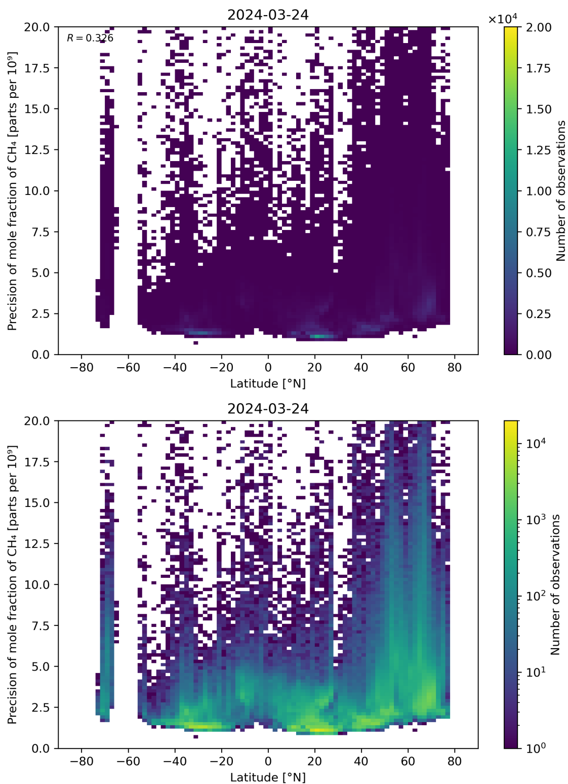
Figure 59: Scatter density plot of “Latitude” against “Precision of mole fraction of CH 4 ” for 2024-03-23 to 2024-03-25.
