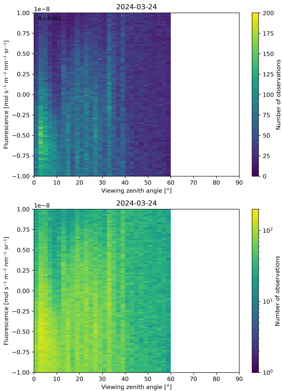
Figure 108: Scatter density plot of “Viewing zenith angle” against “Fluorescence” for 2024-03-23 to 2024-03-25.
