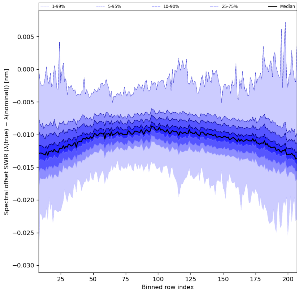
Figure 38: Along track statistics of “Spectral offset SWIR ( \lambda(\text{true}) - \lambda(\text{nominal}) )” for 2024-03-23 to 2024-03-25
