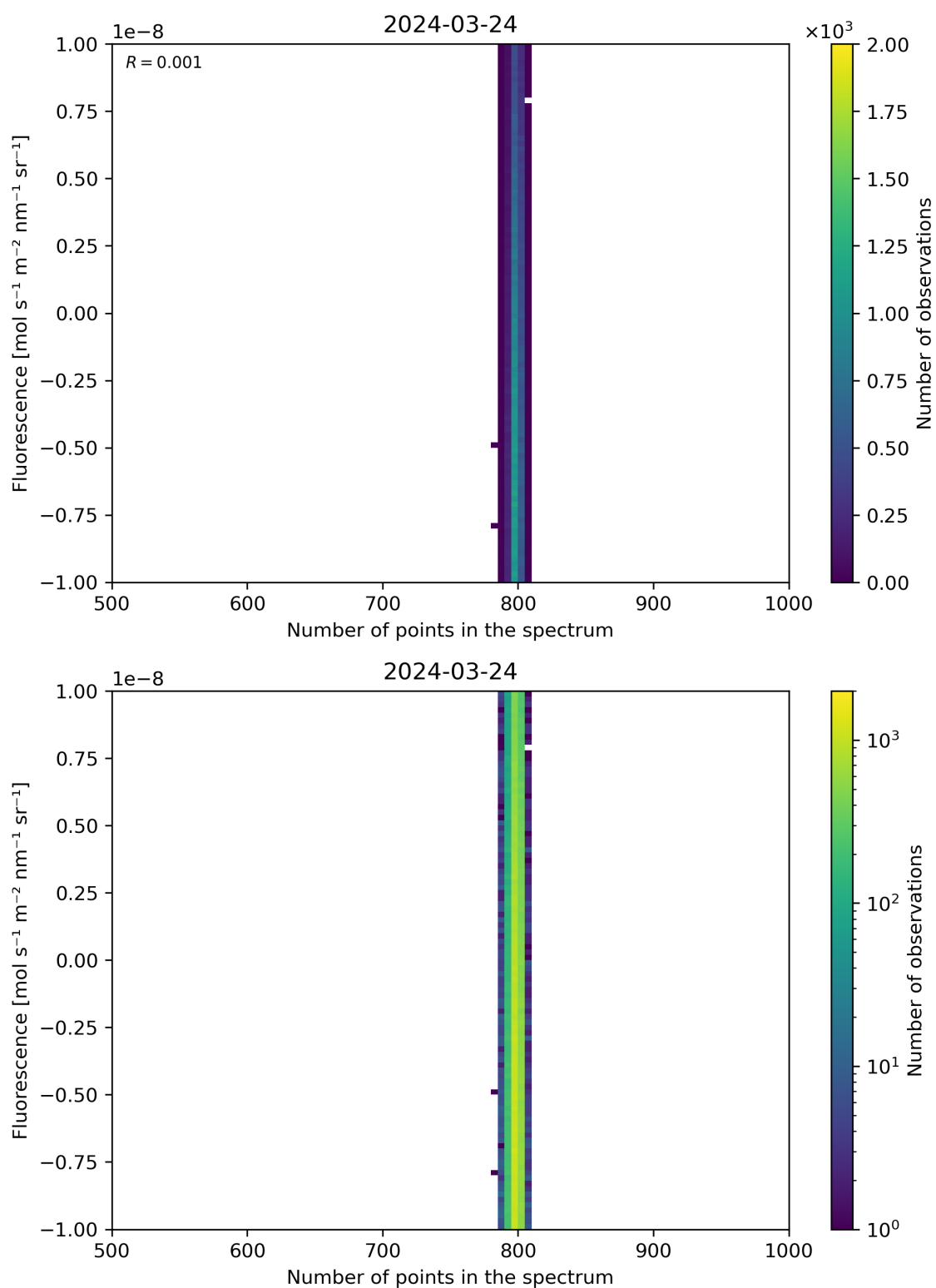
Figure 91: Scatter density plot of “Number of points in the spectrum” against “Fluorescence” for 2024-03-23 to 2024-03-25.
