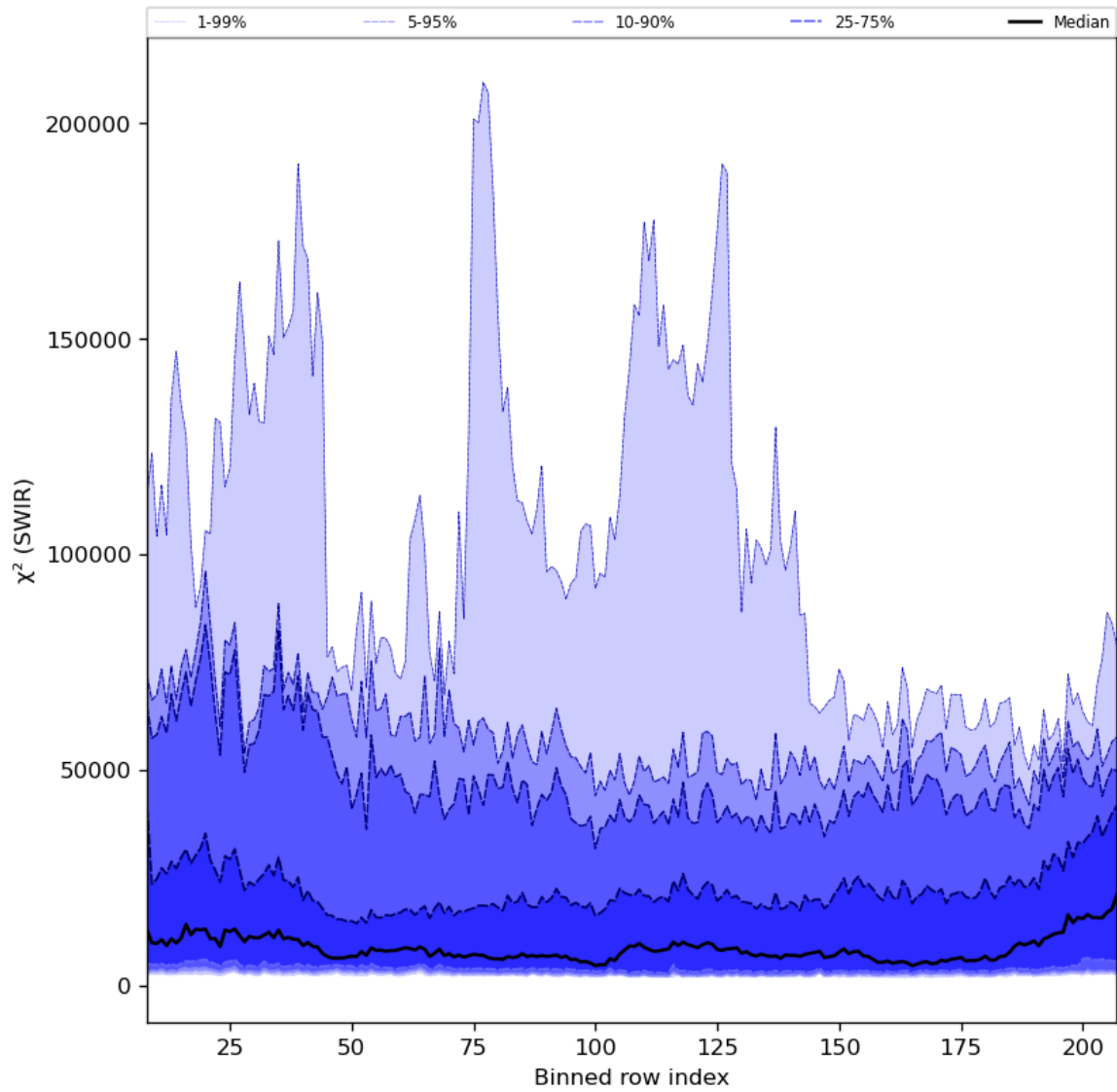
Figure 39: Along track statistics of " \chi^2 (SWIR)" for 2024-03-23 to 2024-03-25
