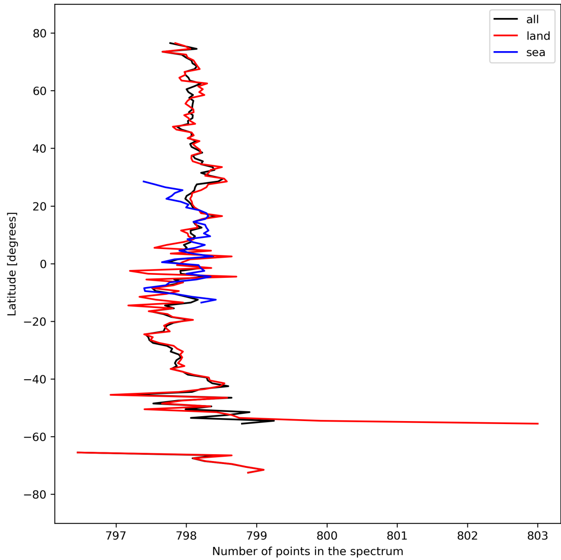
Figure 15: Zonal average of “Number of points in the spectrum” for 2024-03-23 to 2024-03-25.
