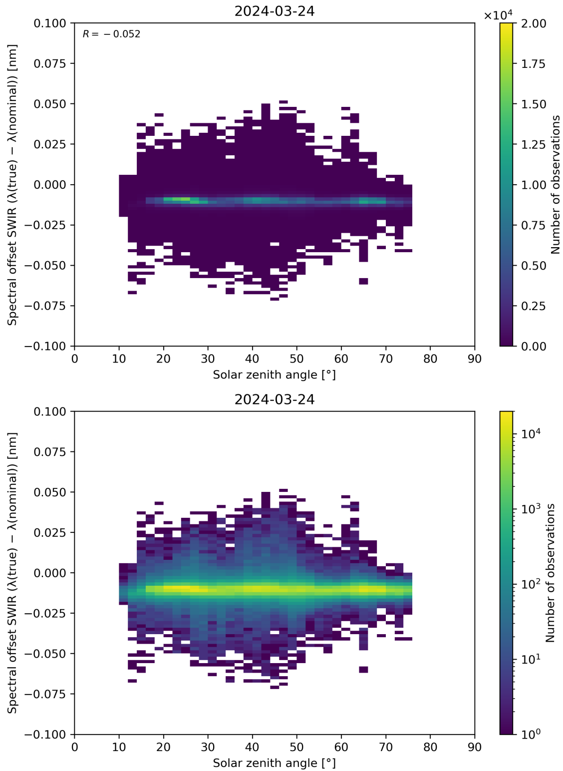
Figure 104: Scatter density plot of “Solar zenith angle” against “Spectral offset SWIR ( \lambda(\text{true}) - \lambda(\text{nominal}) )” for 2024-03-23 to 2024-03-25.
