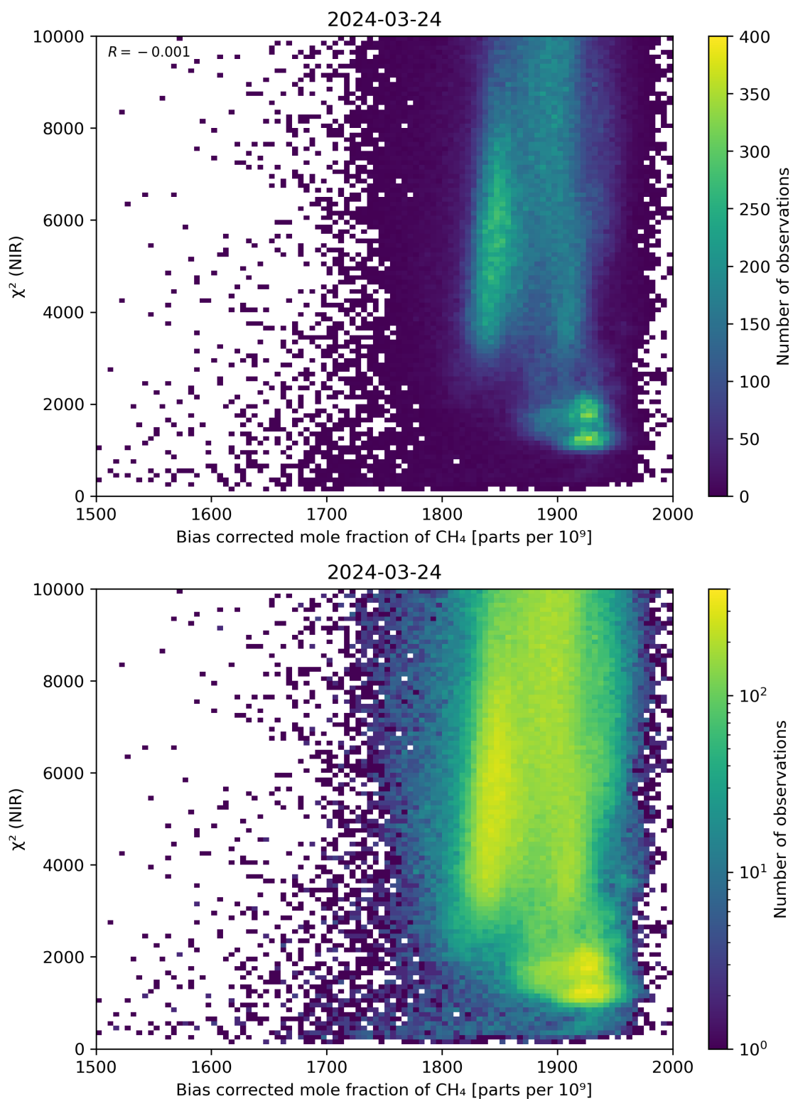
Figure 63: Scatter density plot of “Bias corrected mole fraction of CH 4 ” against “ \chi^2 (NIR)” for 2024-03-23 to 2024-03-25.
