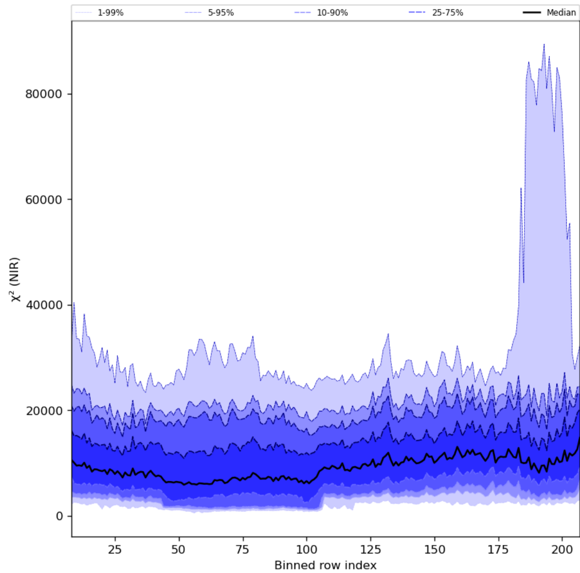
Figure 40: Along track statistics of “ \chi^2 (NIR)” for 2024-03-23 to 2024-03-25
