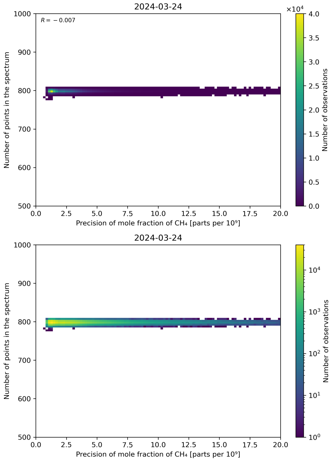
Figure 84: Scatter density plot of “Precision of mole fraction of CH 4 ” against “Number of points in the spectrum” for 2024-03-23 to 2024-03-25.
