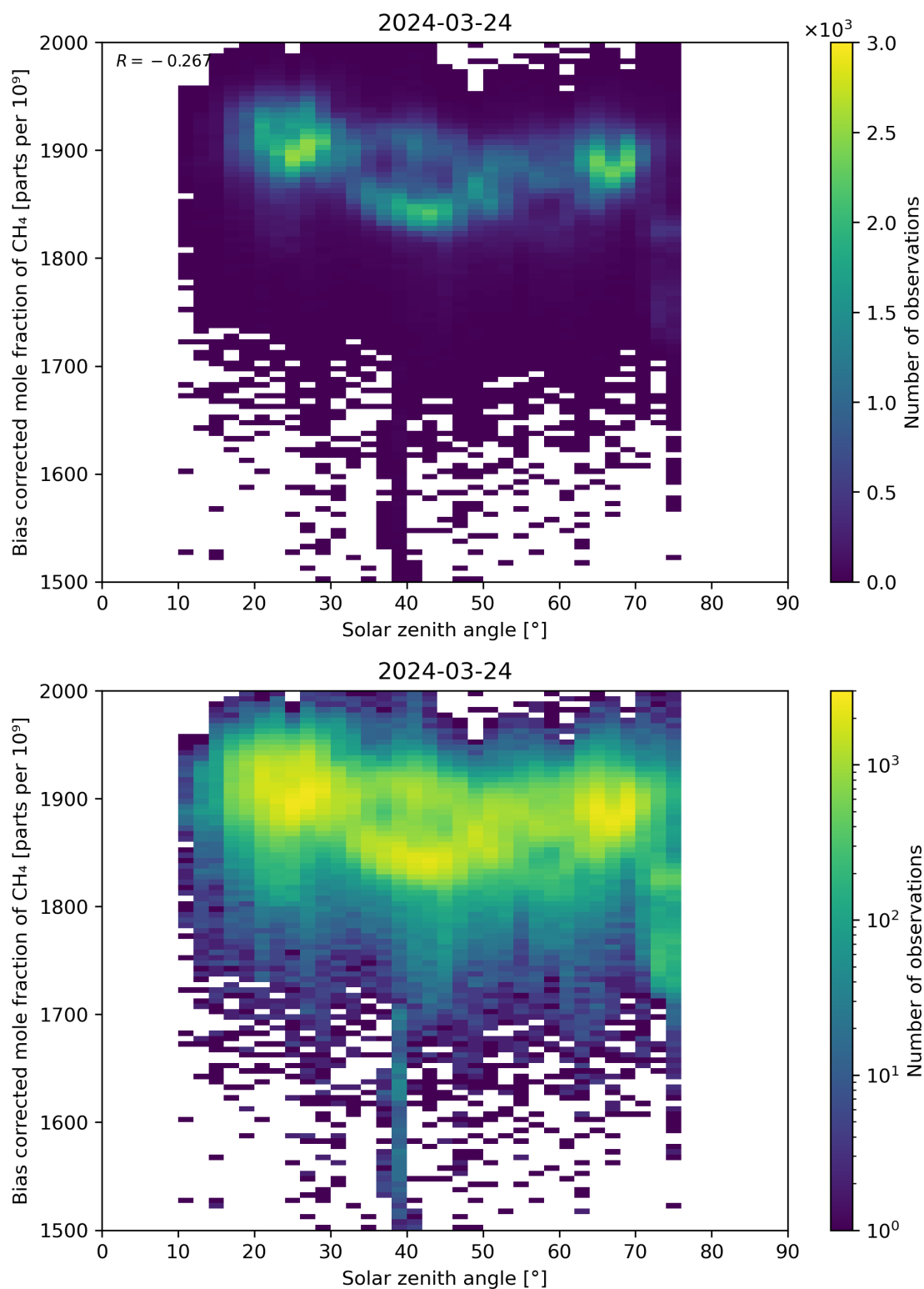
Figure 100: Scatter density plot of “Solar zenith angle” against “Bias corrected mole fraction of CH 4 ” for 2024-03-23 to 2024-03-25.
