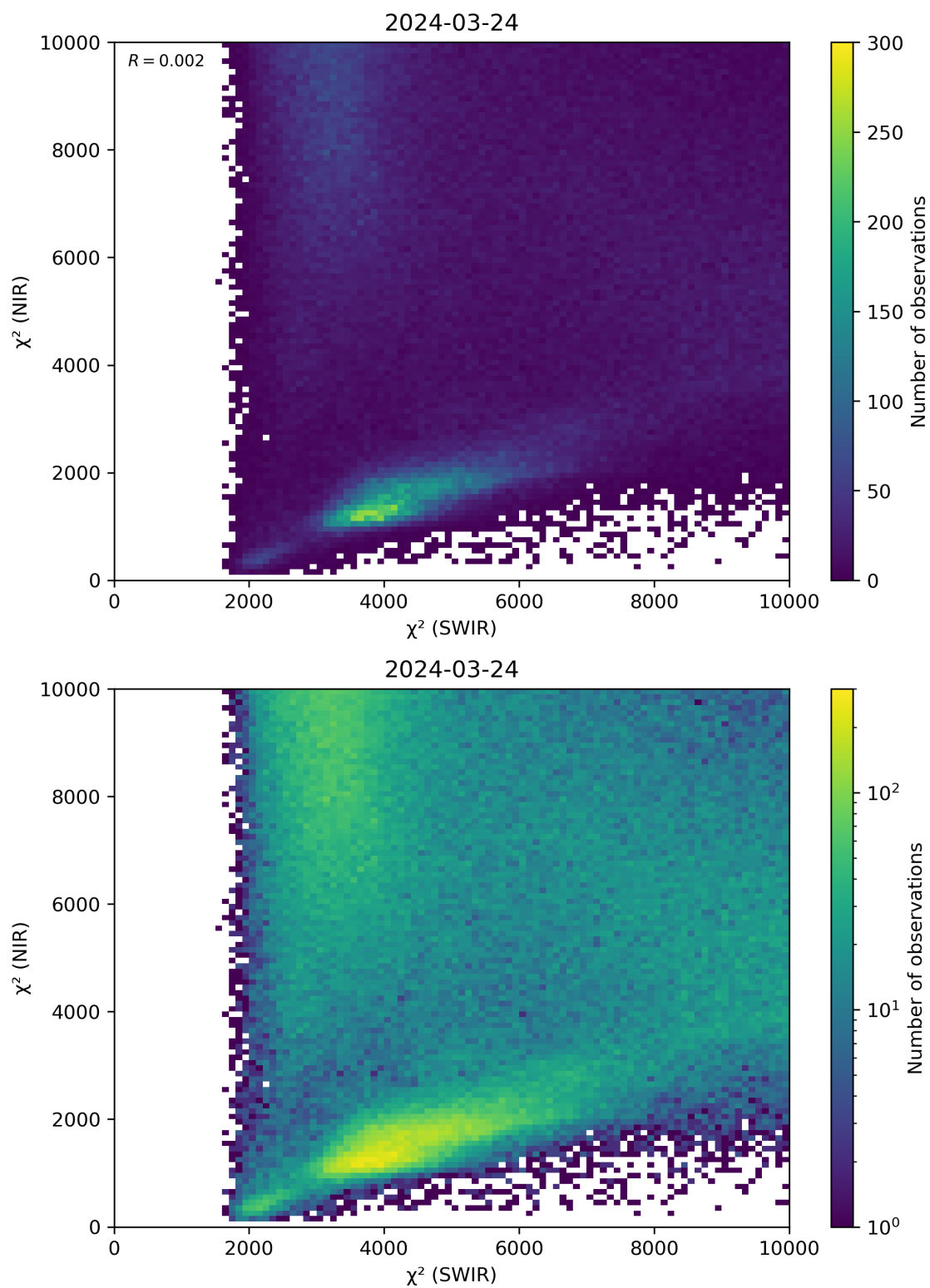
Figure 47: Scatter density plot of “ \chi^2 (SWIR)” against “ \chi^2 (NIR)” for 2024-03-23 to 2024-03-25.
