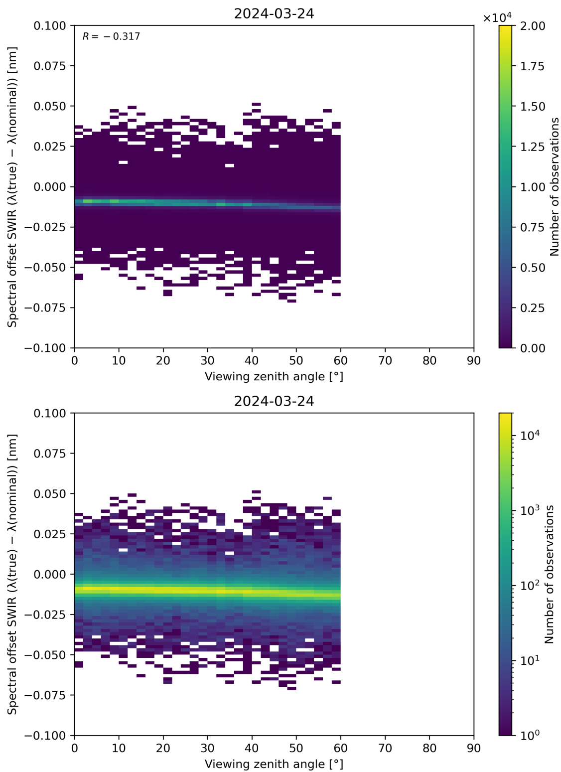
Figure 116: Scatter density plot of “Viewing zenith angle” against “Spectral offset SWIR ( \lambda(\text{true}) - \lambda(\text{nominal}) )” for 2024-03-23 to 2024-03-25.
