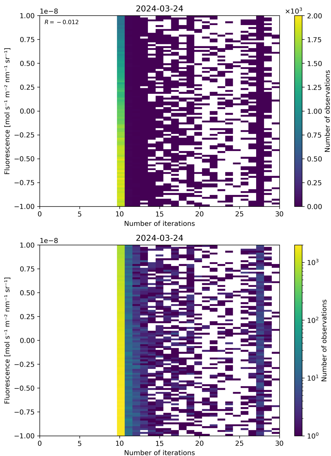
Figure 87: Scatter density plot of “Number of iterations” against “Fluorescence” for 2024-03-23 to 2024-03-25.
