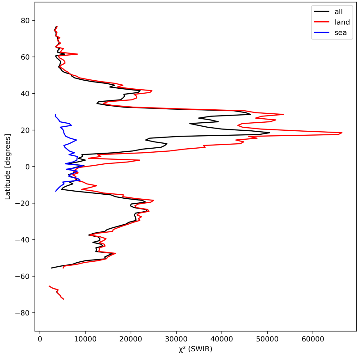
Figure 17: Zonal average of “ \chi^2 (SWIR)” for 2024-03-23 to 2024-03-25.
