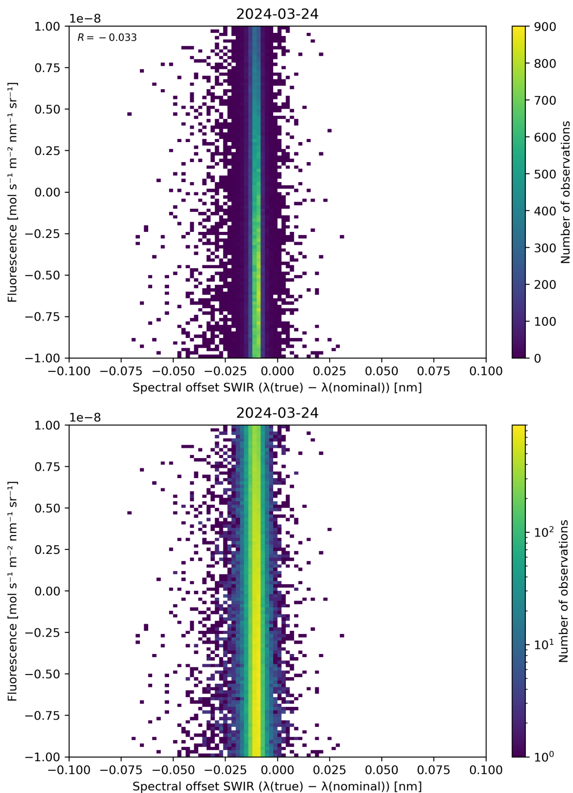
Figure 120: Scatter density plot of “Spectral offset SWIR ( \lambda(\text{true}) - \lambda(\text{nominal}) )” against “Fluorescence” for 2024-03-23 to 2024-03-25.
