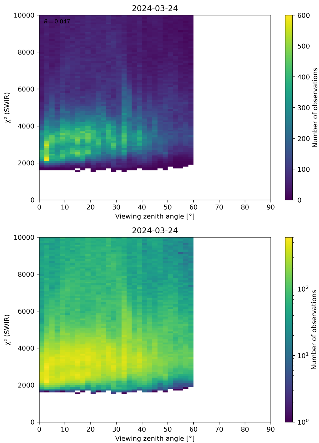
Figure 106: Scatter density plot of “Viewing zenith angle” against “ \chi^2 (SWIR)” for 2024-03-23 to 2024-03-25.
