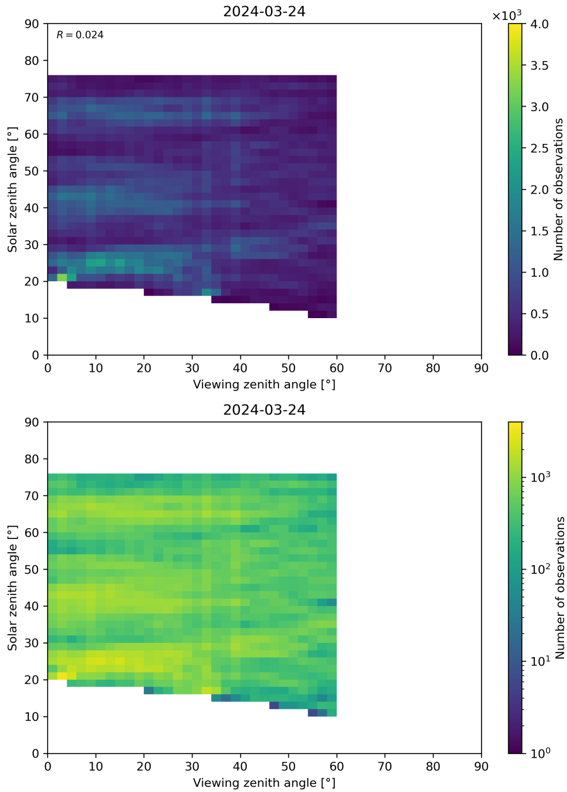
Figure 115: Scatter density plot of “Viewing zenith angle” against “Solar zenith angle” for 2024-03-23 to 2024-03-25.
