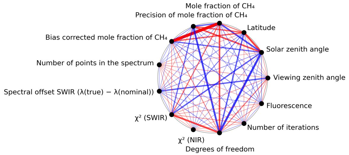
Figure 1: Map of correlation graph for 2024-03-23 to 2024-03-25.
