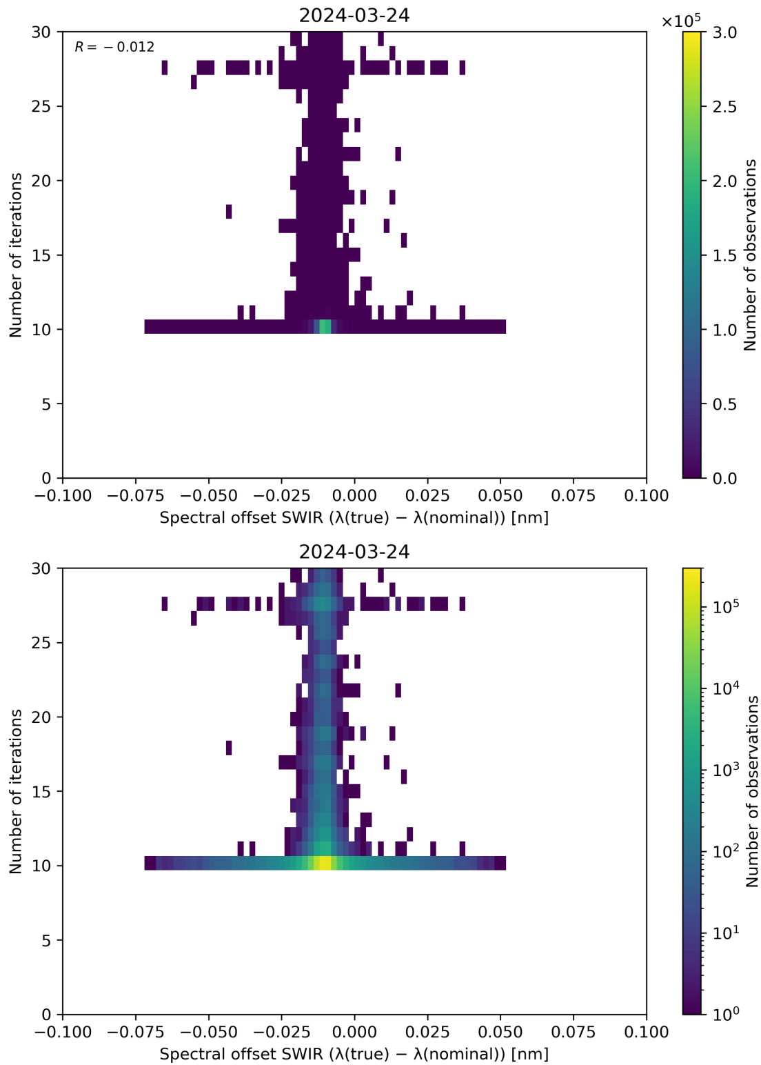
Figure 121: Scatter density plot of “Spectral offset SWIR ( \lambda(\text{true}) - \lambda(\text{nominal}) )” against “Number of iterations” for 2024-03-23 to 2024-03-25.
