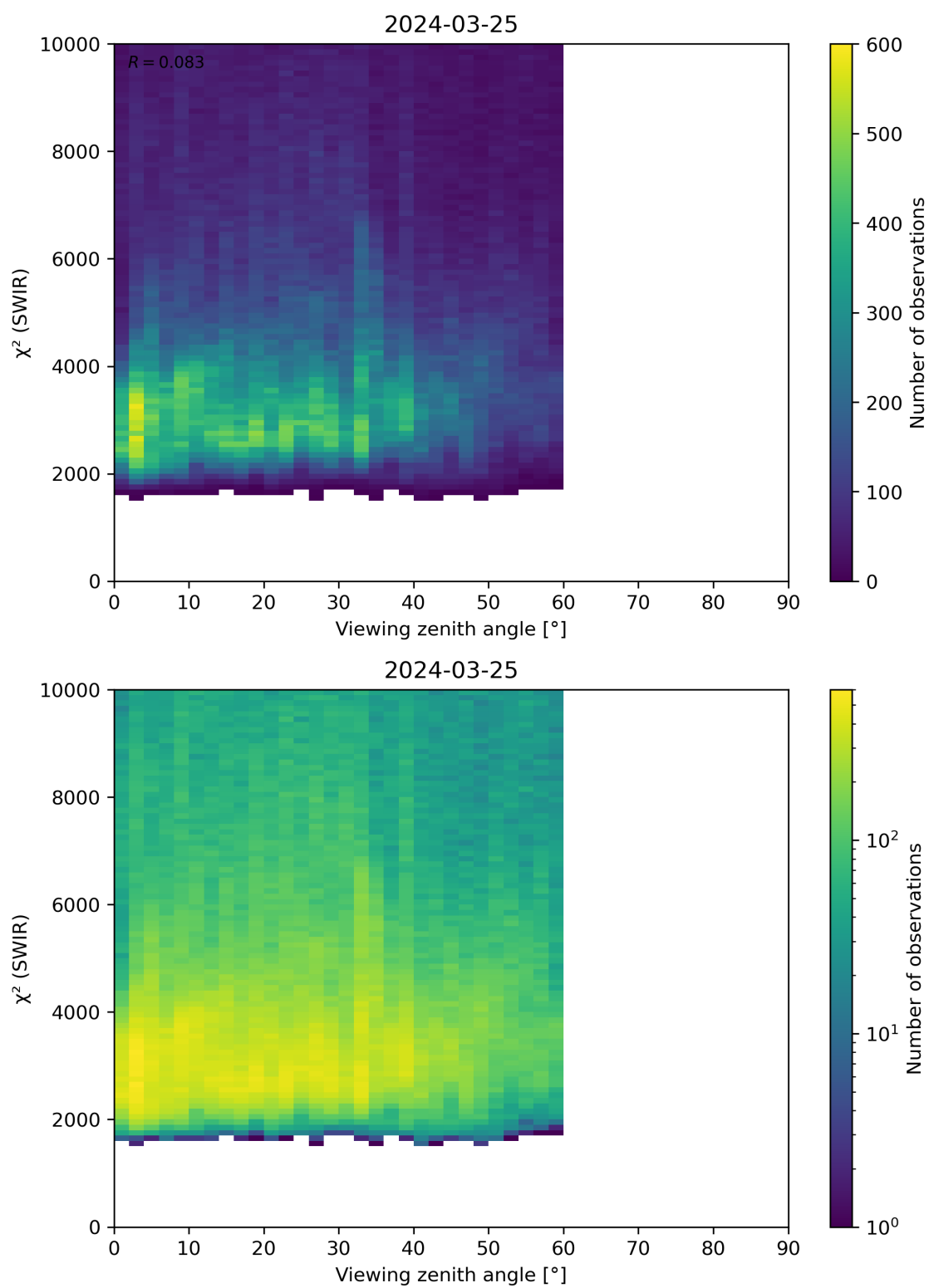
Figure 106: Scatter density plot of “Viewing zenith angle” against “ \chi^2 (SWIR)” for 2024-03-25 to 2024-03-26.
