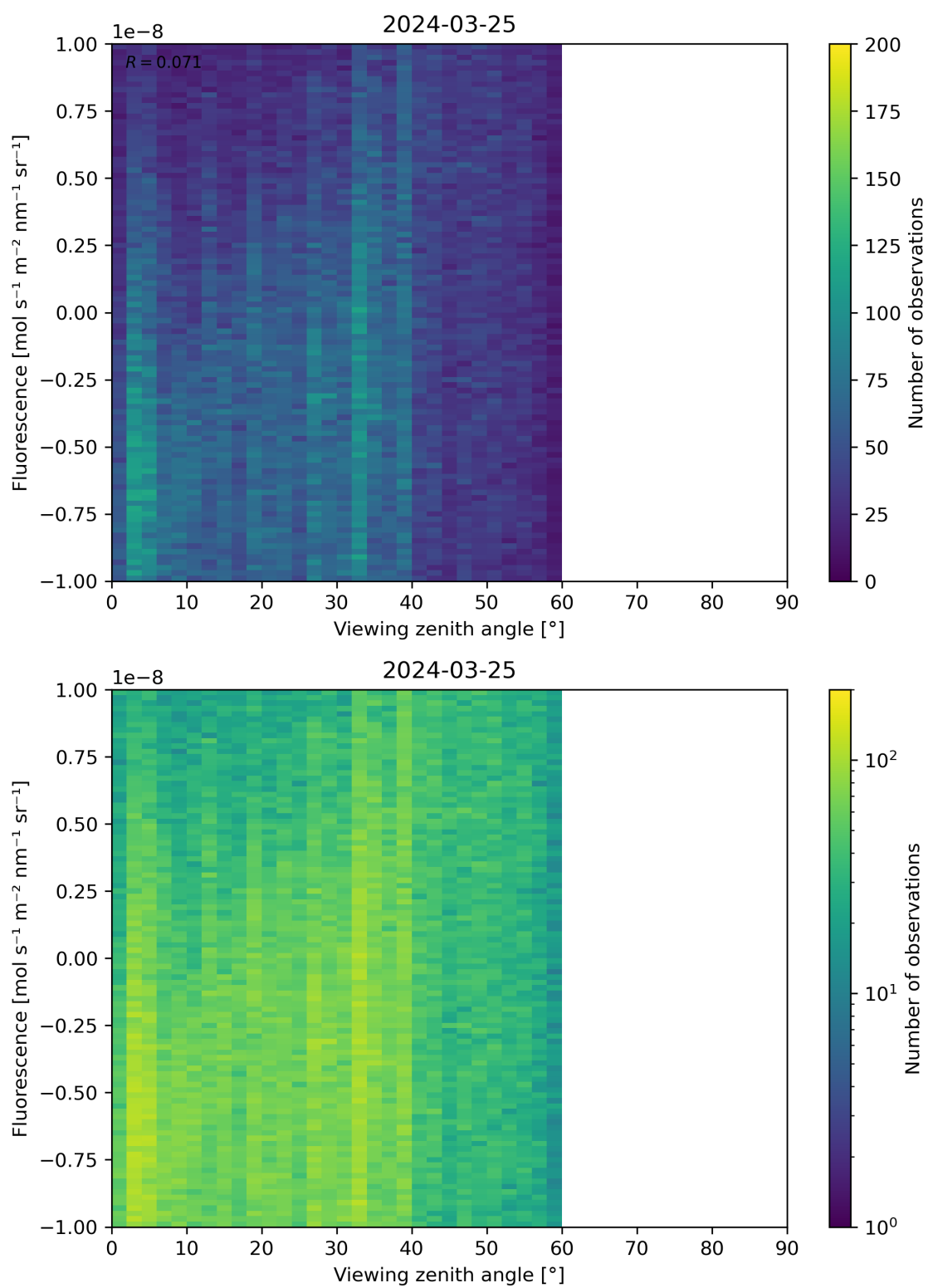
Figure 108: Scatter density plot of “Viewing zenith angle” against “Fluorescence” for 2024-03-25 to 2024-03-26.
