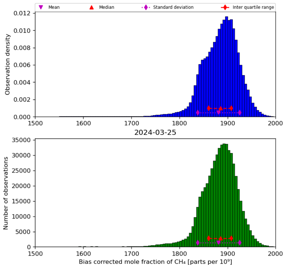
Figure 25: Histogram of “Bias corrected mole fraction of CH 4 ” for 2024-03-25 to 2024-03-26
