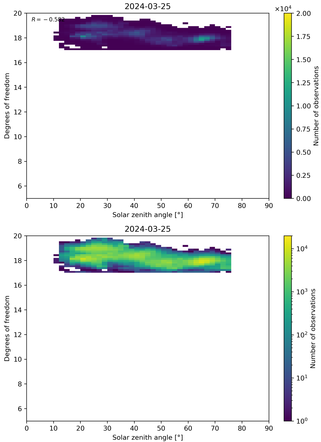
Figure 96: Scatter density plot of “Solar zenith angle” against “Degrees of freedom” for 2024-03-25 to 2024-03-26.
