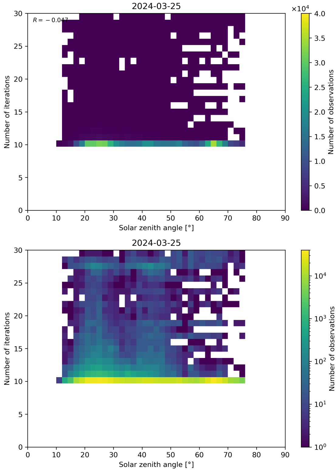
Figure 102: Scatter density plot of “Solar zenith angle” against “Number of iterations” for 2024-03-25 to 2024-03-26.
