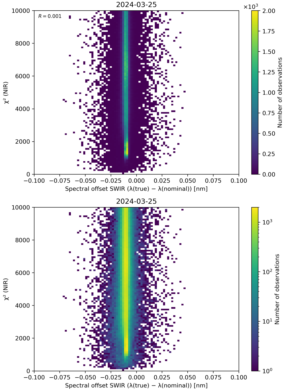
Figure 117: Scatter density plot of “Spectral offset SWIR ( \lambda(\text{true}) - \lambda(\text{nominal}) )” against “ \chi^2 (NIR)” for 2024-03-25 to 2024-03-26.
