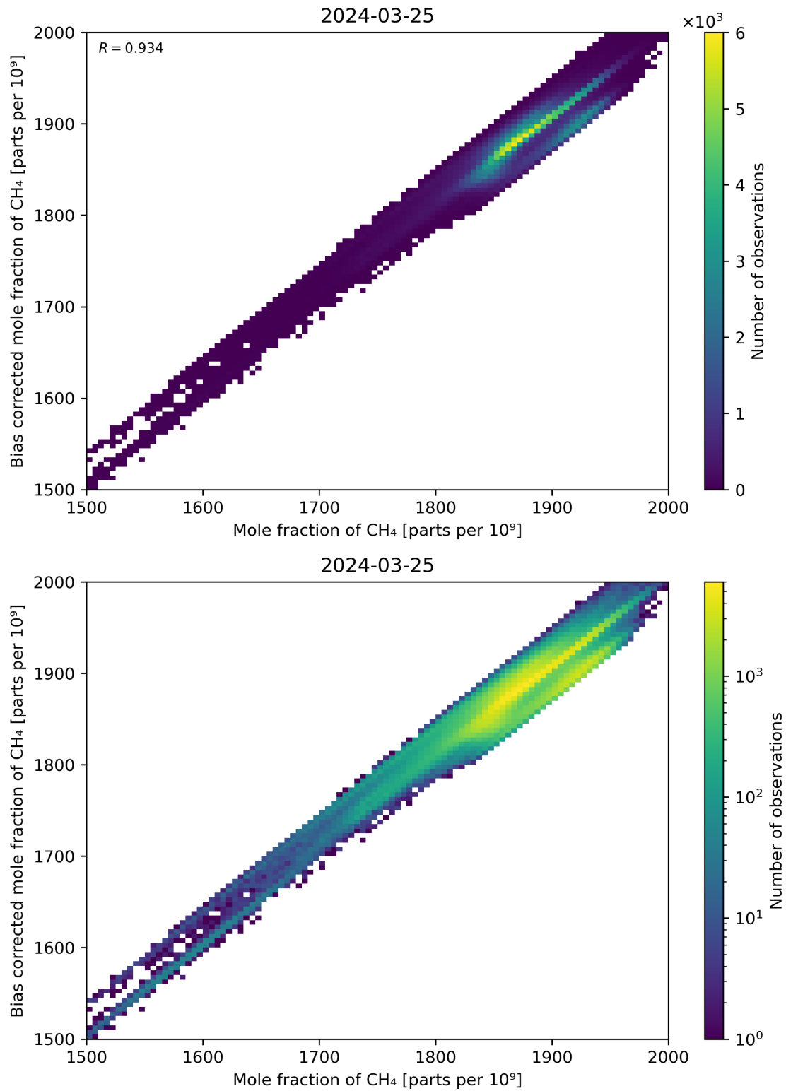
Figure 74: Scatter density plot of “Mole fraction of CH 4 ” against “Bias corrected mole fraction of CH 4 ” for 2024-03-25 to 2024-03-26.
