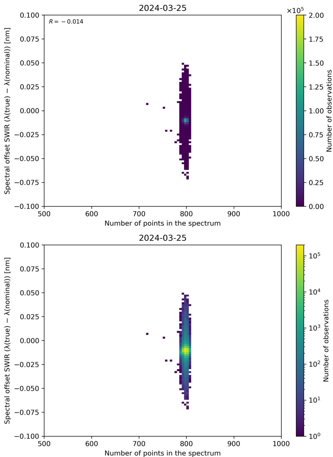
Figure 93: Scatter density plot of “Number of points in the spectrum” against “Spectral offset SWIR ( \lambda(\text{true}) - \lambda(\text{nominal}) )” for 2024-03-25 to 2024-03-26.
