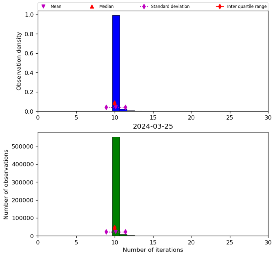
Figure 31: Histogram of “Number of iterations” for 2024-03-25 to 2024-03-26
