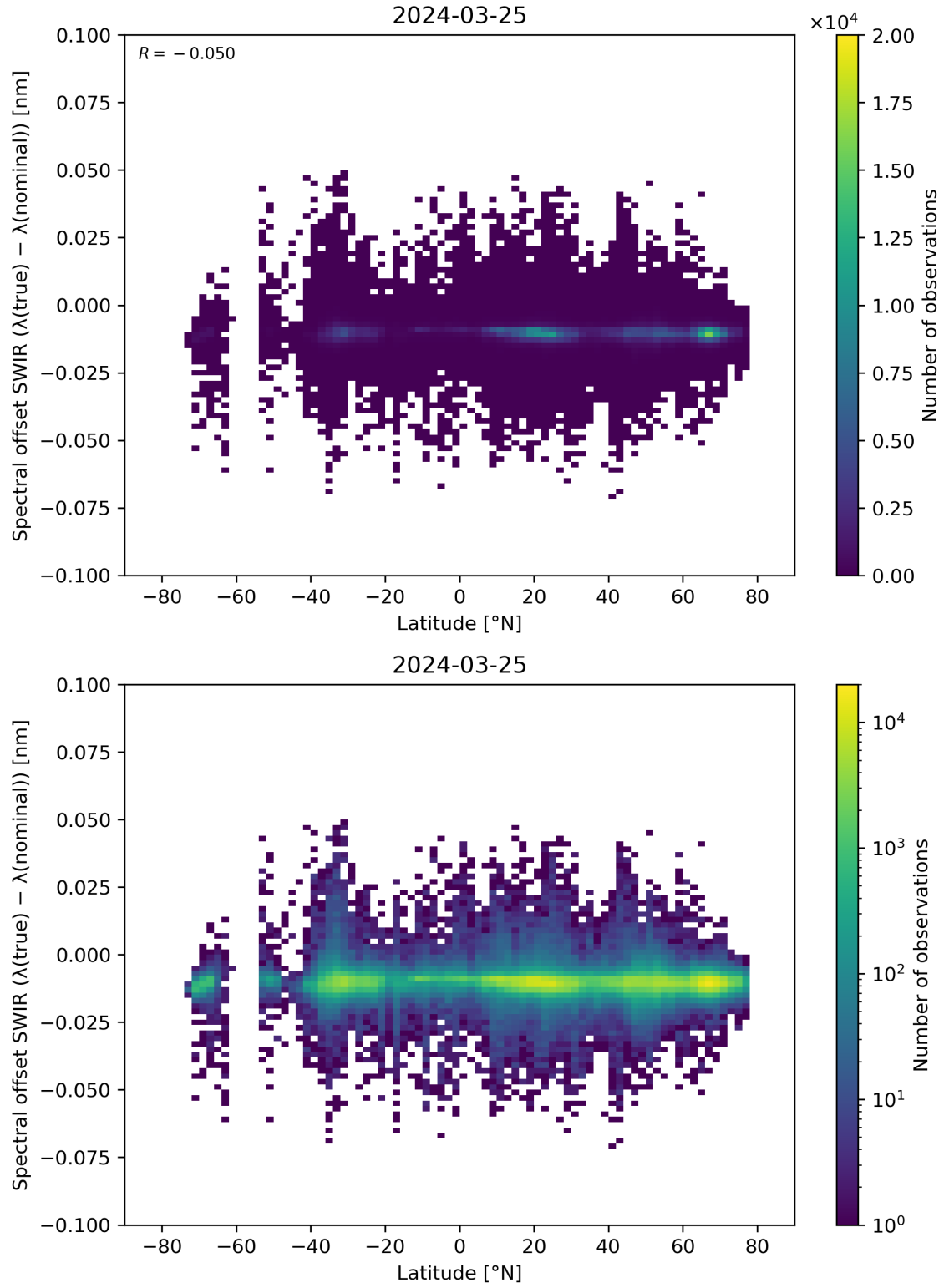
Figure 62: Scatter density plot of “Latitude” against “Spectral offset SWIR ( \lambda(\text{true}) - \lambda(\text{nominal}) )” for 2024-03-25 to 2024-03-26.
