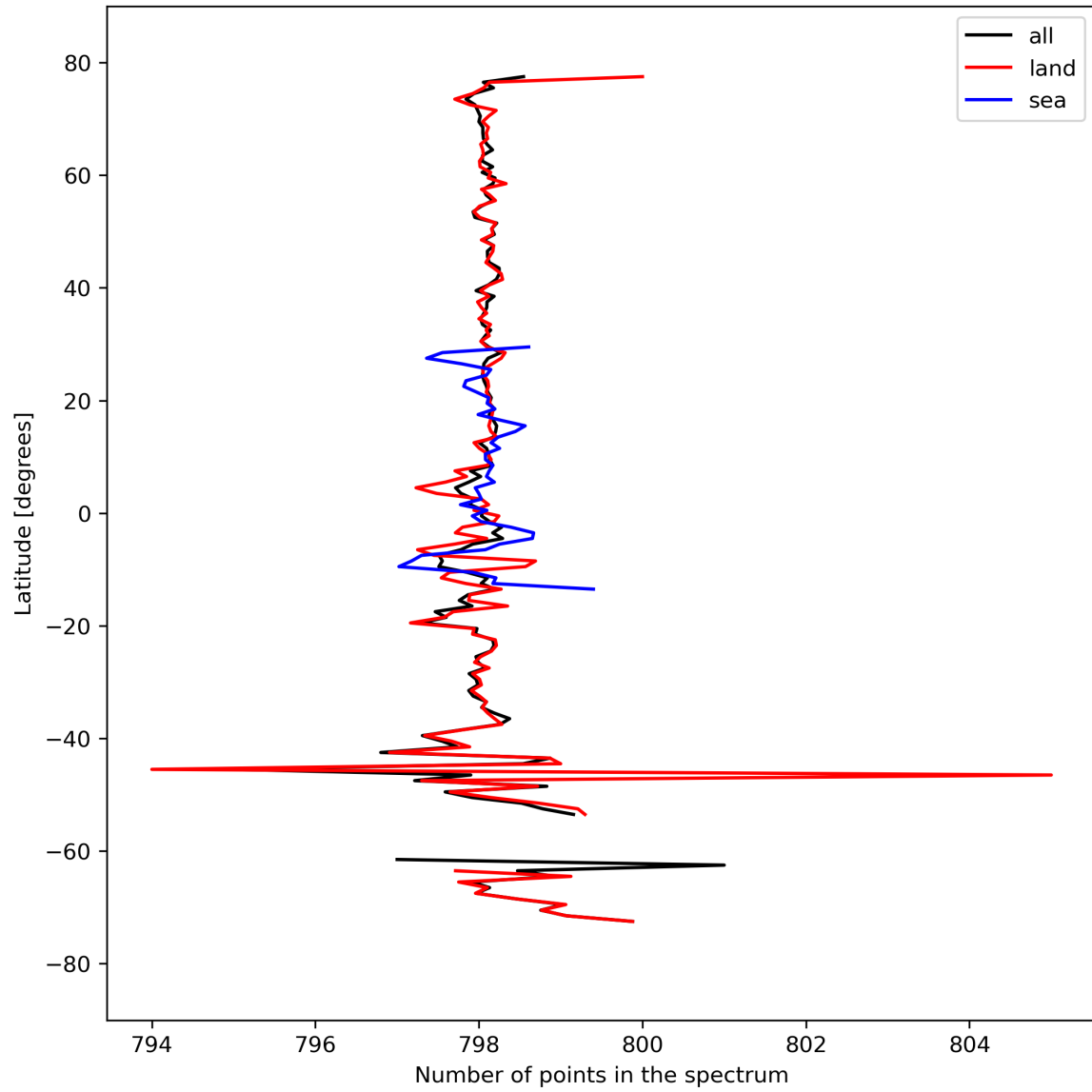
Figure 15: Zonal average of “Number of points in the spectrum” for 2024-03-25 to 2024-03-26.
