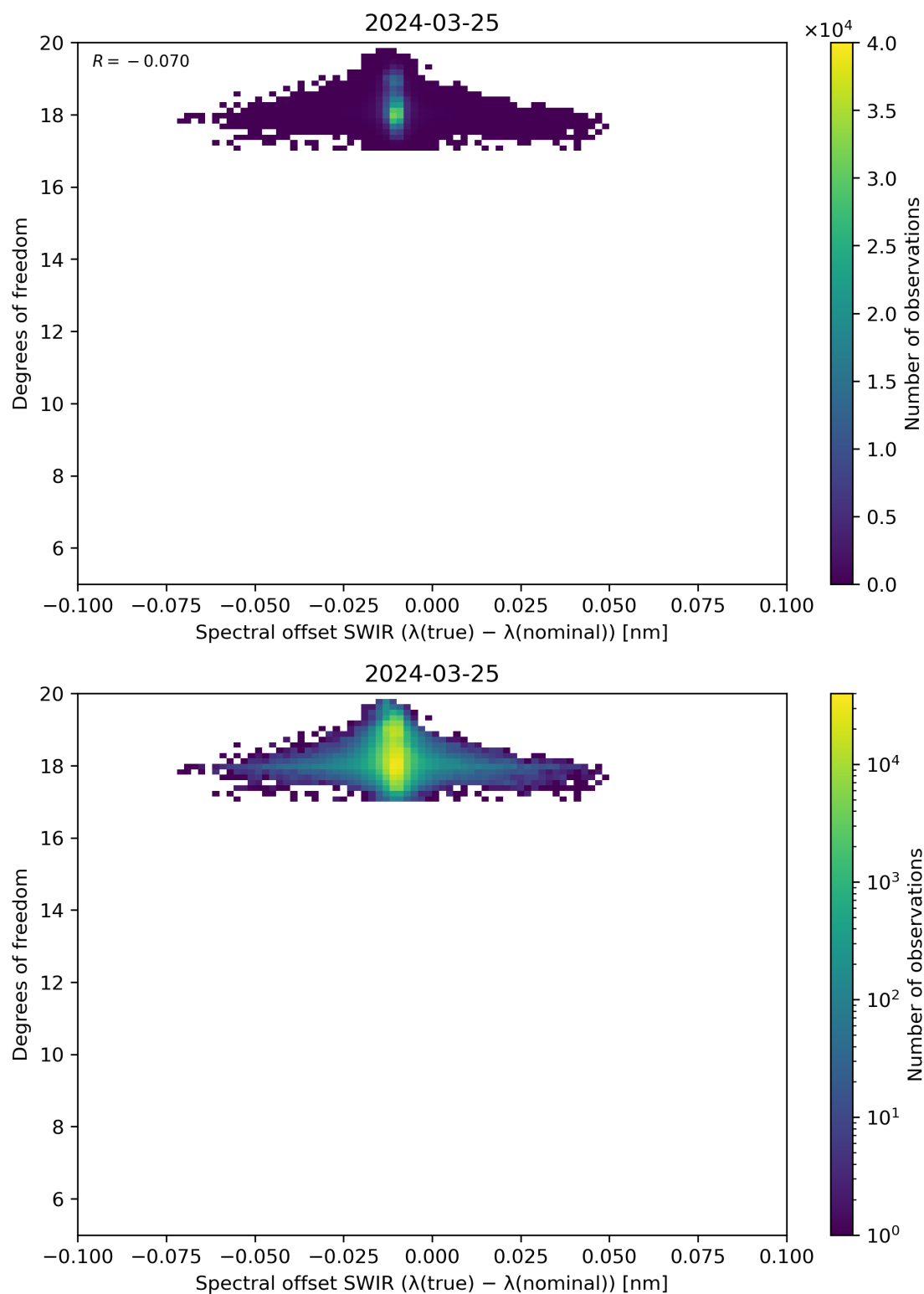
Figure 119: Scatter density plot of “Spectral offset SWIR ( \lambda(\text{true}) - \lambda(\text{nominal}) )” against “Degrees of freedom” for 2024-03-25 to 2024-03-26.
