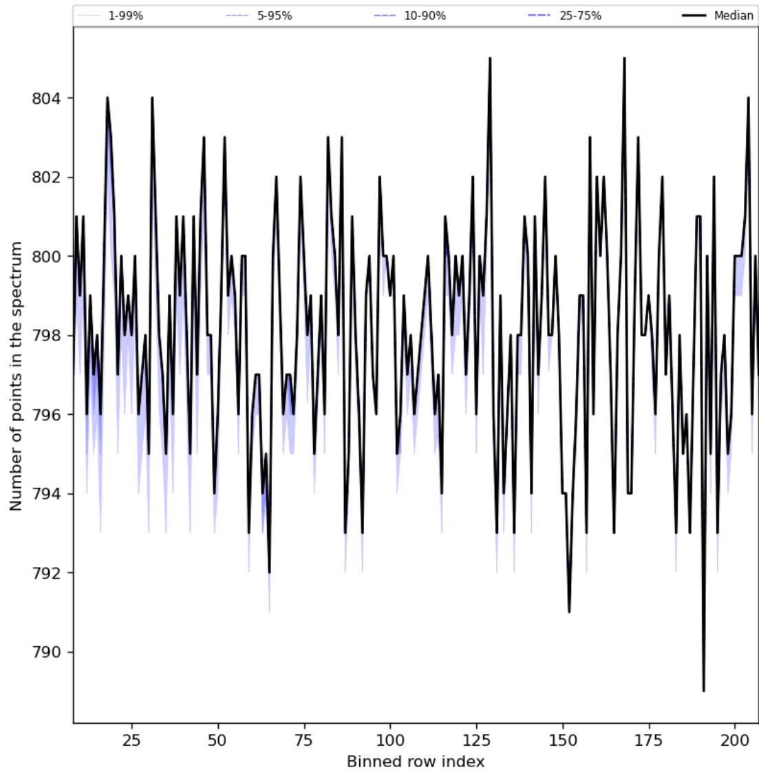
Figure 37: Along track statistics of “Number of points in the spectrum” for 2024-03-25 to 2024-03-26
