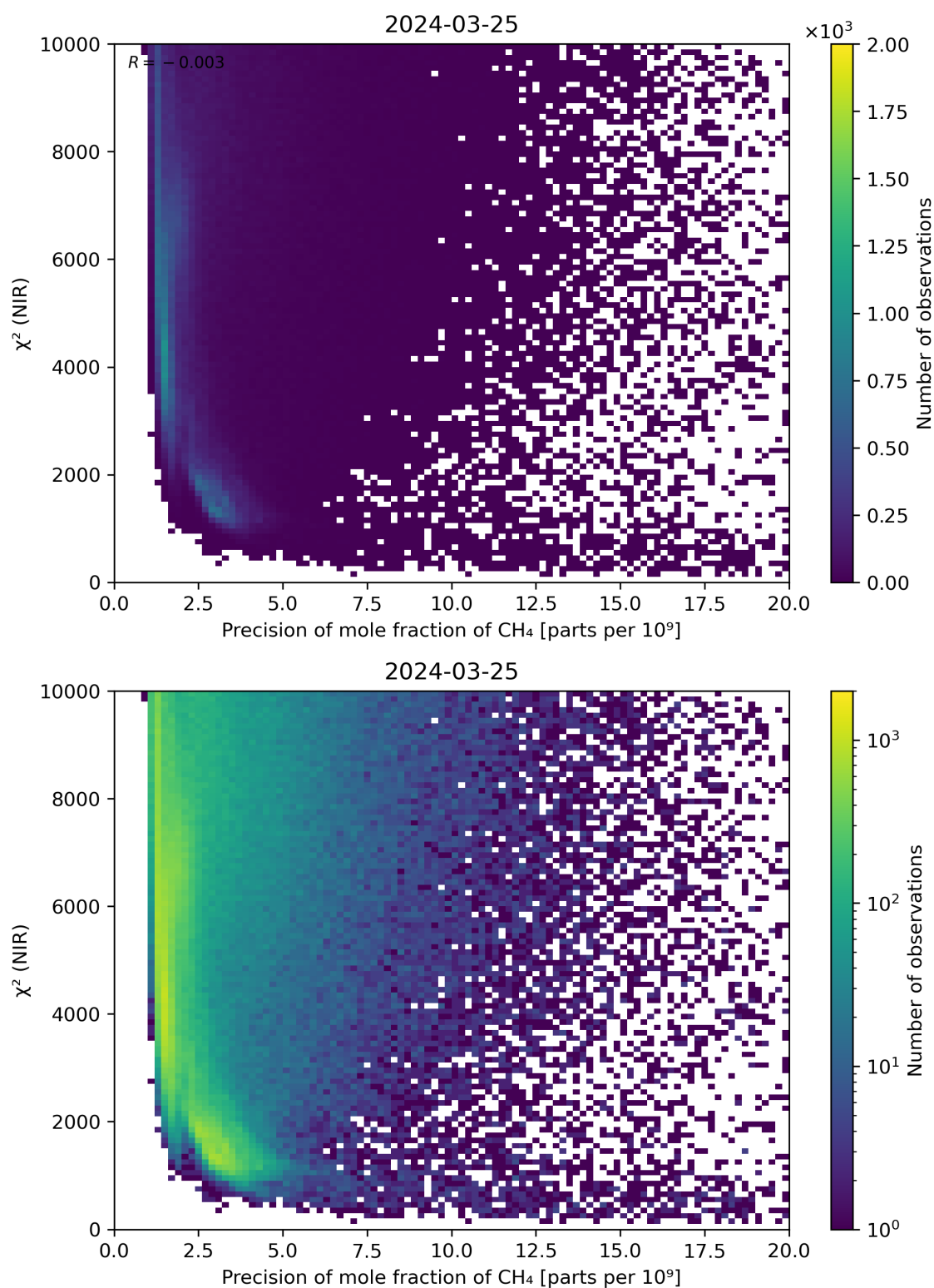
Figure 78: Scatter density plot of “Precision of mole fraction of CH 4 ” against “ \chi^2 (NIR)” for 2024-03-25 to 2024-03-26.
