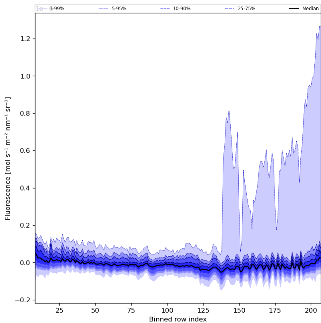
Figure 43: Along track statistics of “Fluorescence” for 2024-03-25 to 2024-03-26
