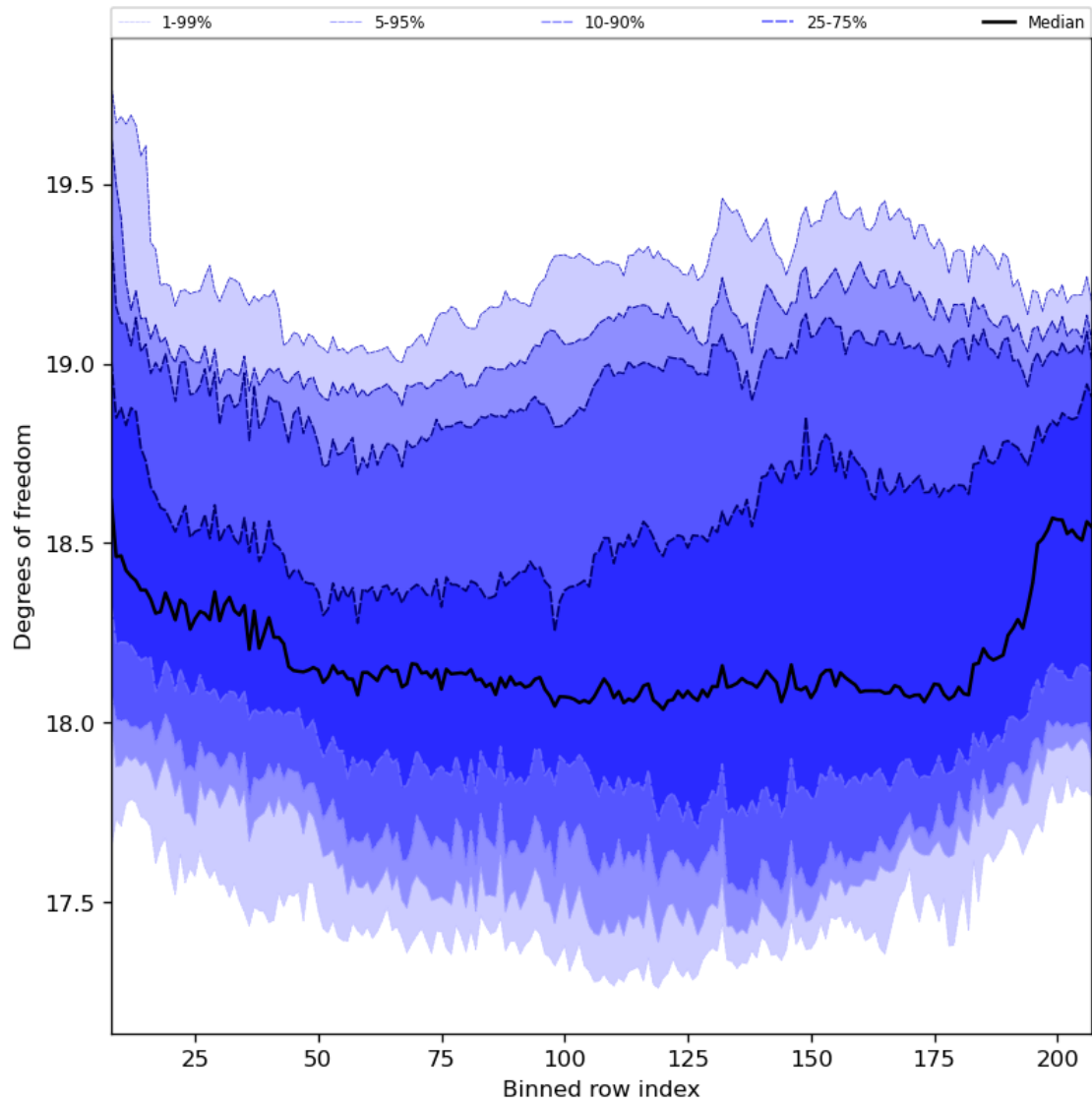
Figure 41: Along track statistics of “Degrees of freedom” for 2024-03-25 to 2024-03-26
