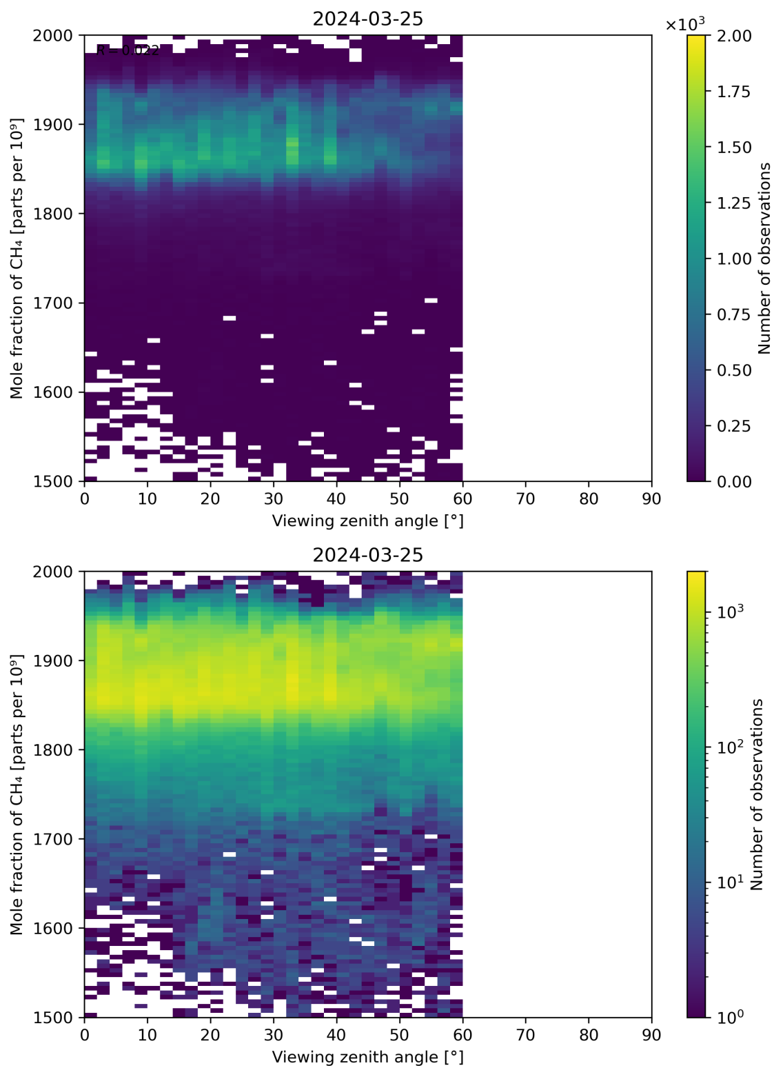
Figure 110: Scatter density plot of “Viewing zenith angle” against “Mole fraction of CH 4 ” for 2024-03-25 to 2024-03-26.
