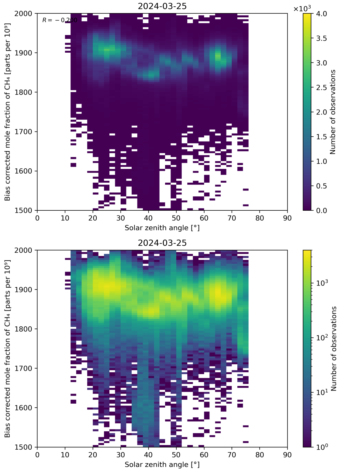
Figure 100: Scatter density plot of “Solar zenith angle” against “Bias corrected mole fraction of \text{CH}_4 ” for 2024-03-25 to 2024-03-26.
