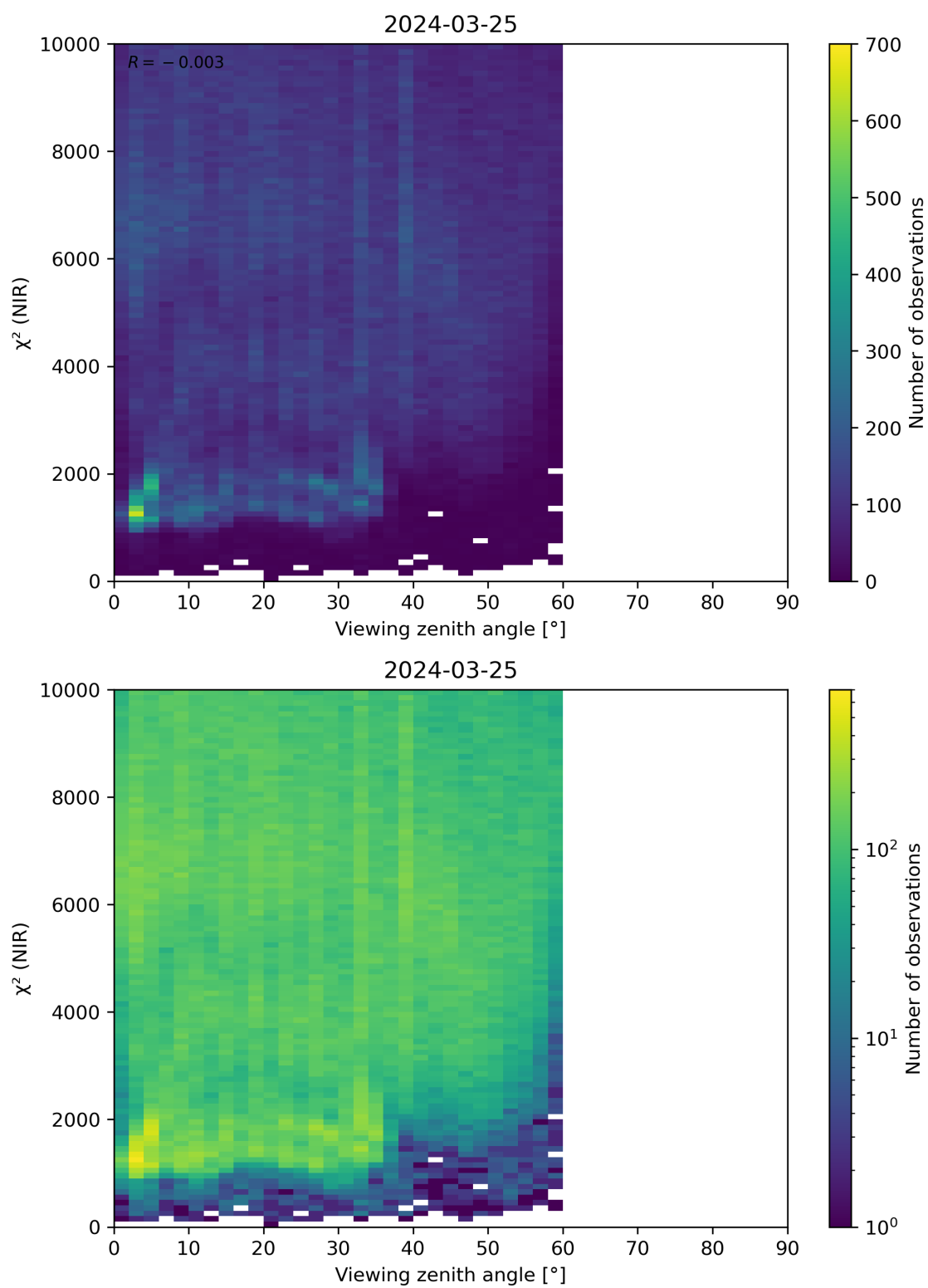
Figure 105: Scatter density plot of “Viewing zenith angle” against “ \chi^2 (NIR)” for 2024-03-25 to 2024-03-26.
