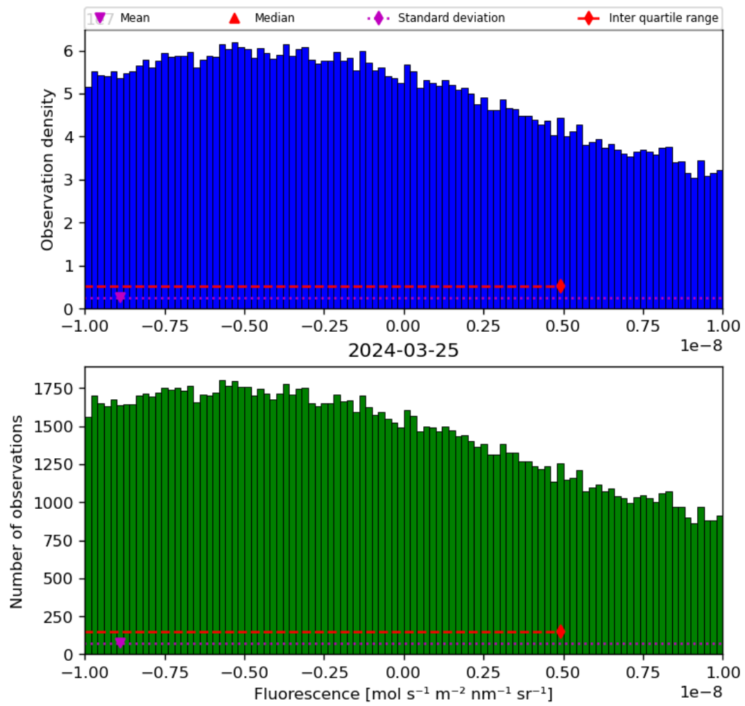
Figure 32: Histogram of “Fluorescence” for 2024-03-25 to 2024-03-26
