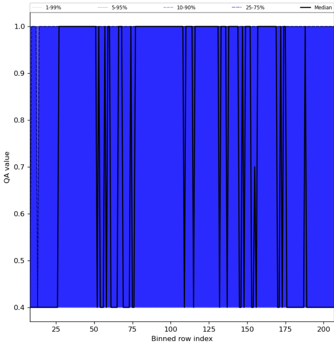
Figure 33: Along track statistics of “QA value” for 2024-03-25 to 2024-03-26
