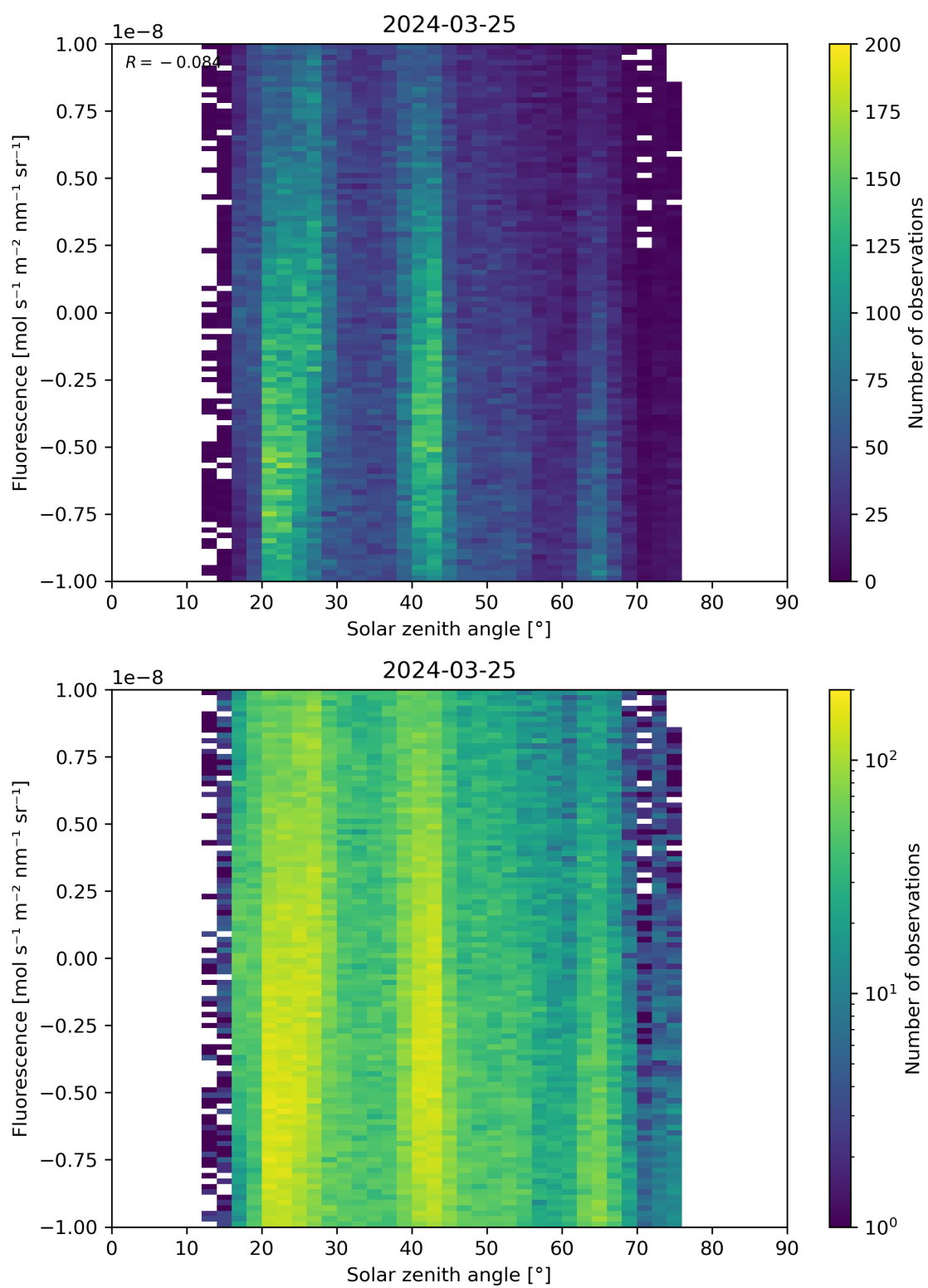
Figure 97: Scatter density plot of “Solar zenith angle” against “Fluorescence” for 2024-03-25 to 2024-03-26.
