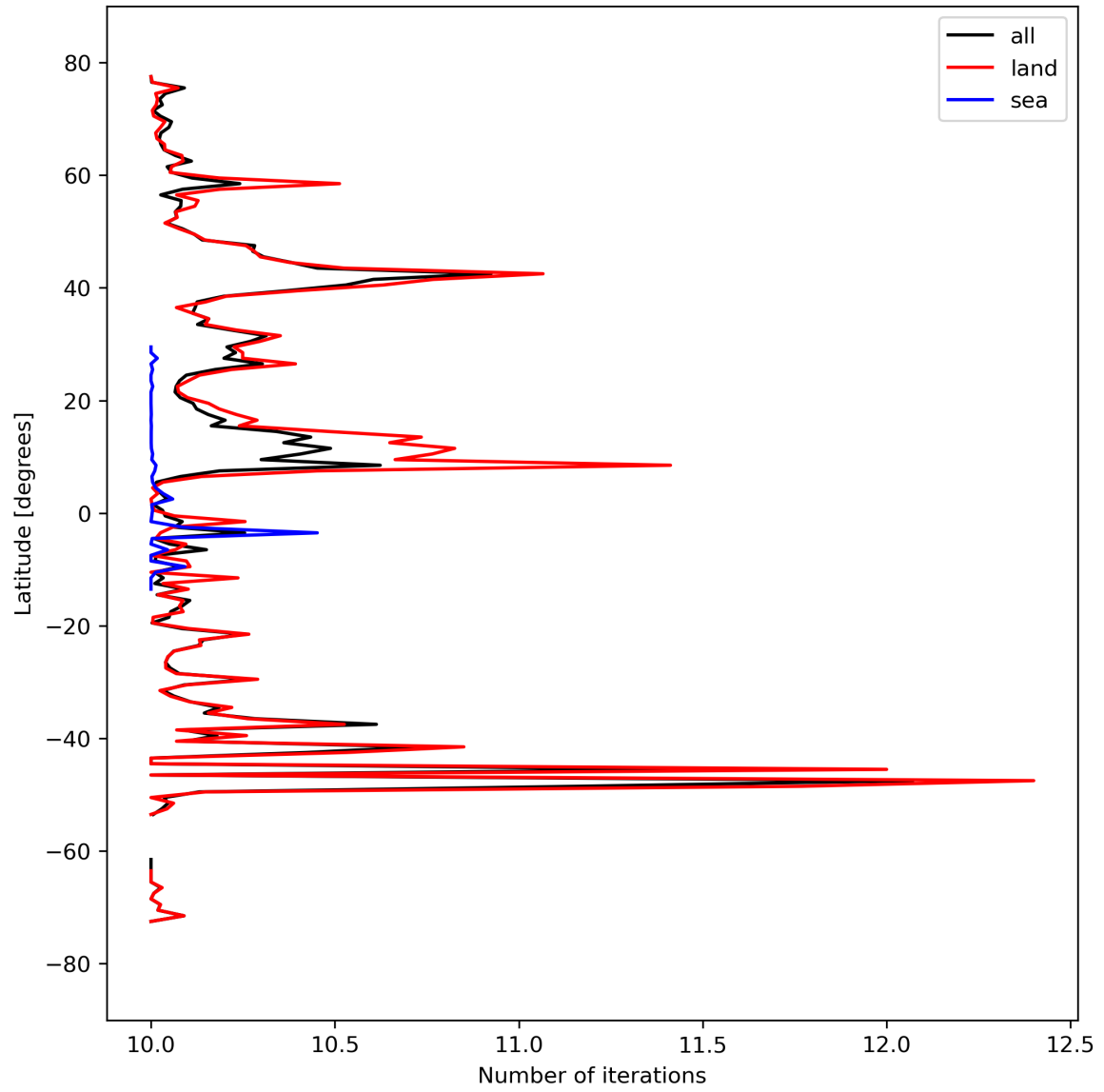
Figure 20: Zonal average of “Number of iterations” for 2024-03-25 to 2024-03-26.
