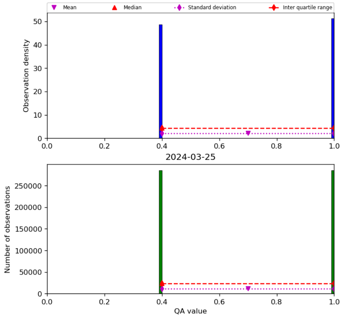
Figure 22: Histogram of “QA value” for 2024-03-25 to 2024-03-26
