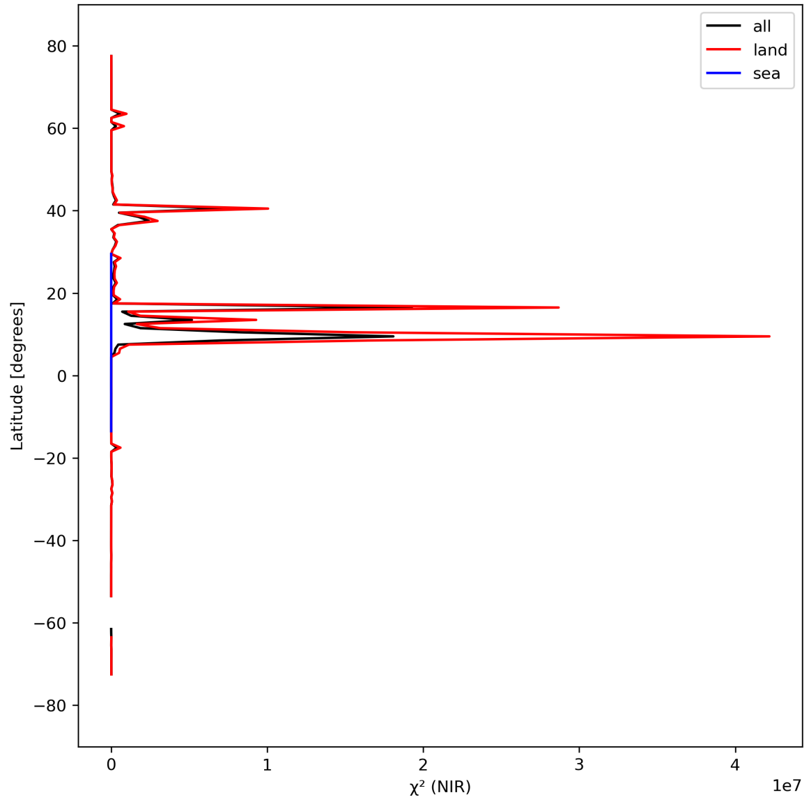
Figure 18: Zonal average of “ \chi^2 (NIR)” for 2024-03-25 to 2024-03-26.
