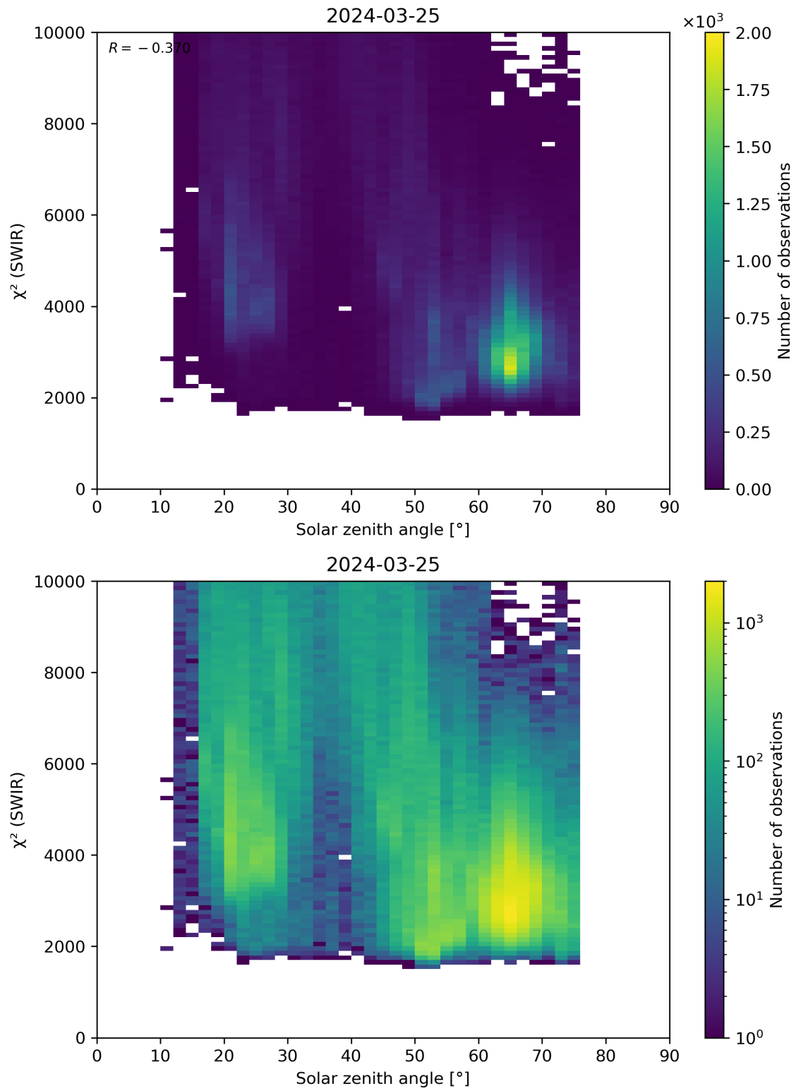
Figure 95: Scatter density plot of “Solar zenith angle” against “ \chi^2 (SWIR)” for 2024-03-25 to 2024-03-26.
