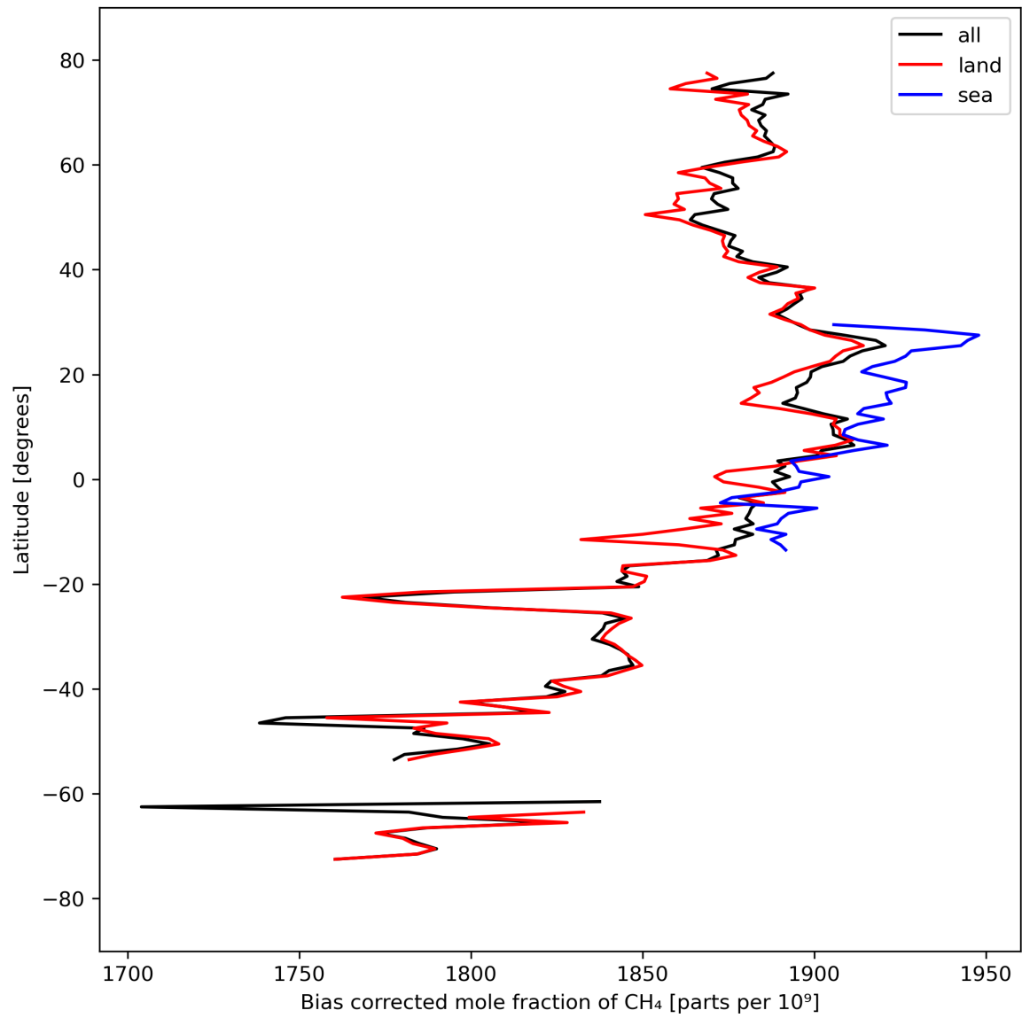
Figure 14: Zonal average of “Bias corrected mole fraction of CH 4 ” for 2024-03-25 to 2024-03-26.
