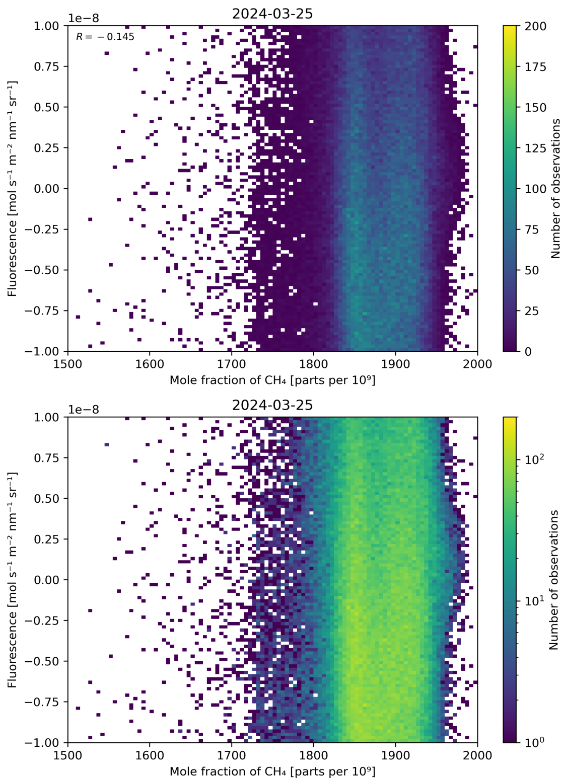
Figure 73: Scatter density plot of “Mole fraction of \text{CH}_4 ” against “Fluorescence” for 2024-03-25 to 2024-03-26.
