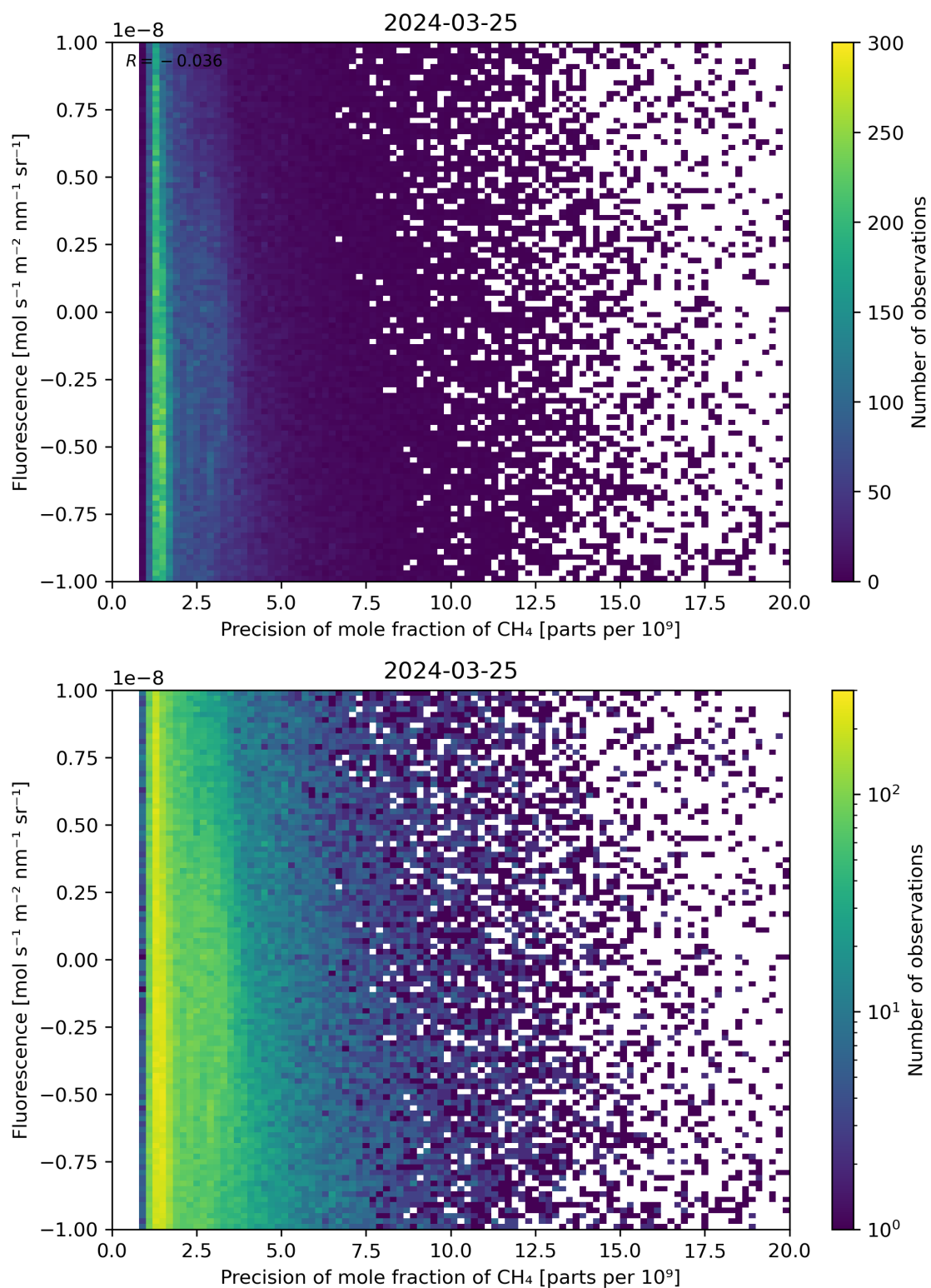
Figure 81: Scatter density plot of “Precision of mole fraction of \text{CH}_4 ” against “Fluorescence” for 2024-03-25 to 2024-03-26.
