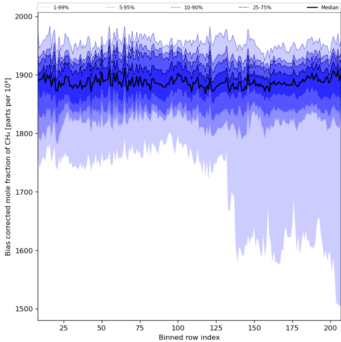
Figure 36: Along track statistics of “Bias corrected mole fraction of CH 4 ” for 2024-03-25 to 2024-03-26
