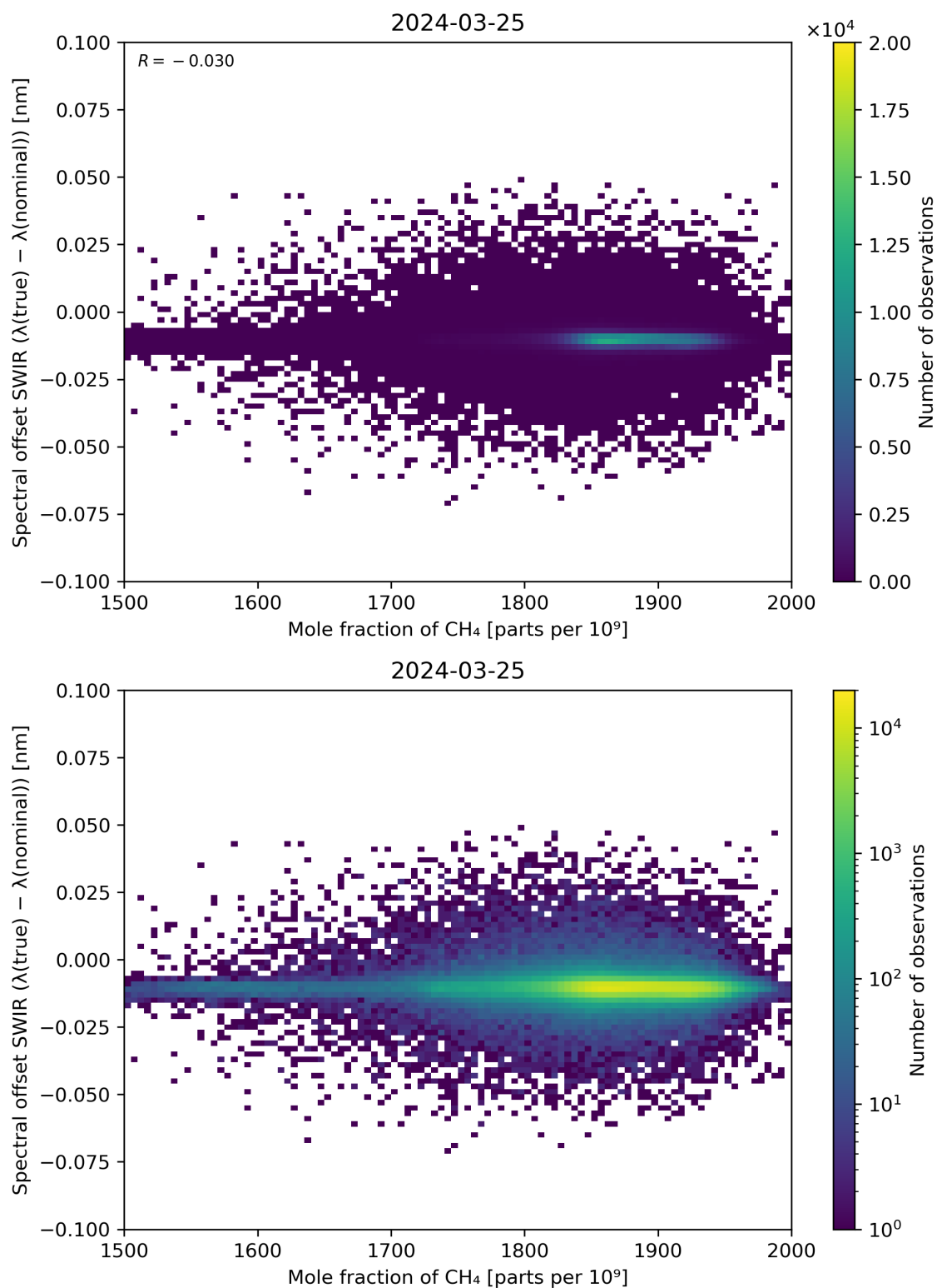
Figure 86: Scatter density plot of “Mole fraction of CH 4 ” against “Spectral offset SWIR ( \lambda(\text{true}) - \lambda(\text{nominal}) )” for 2024-03-25 to 2024-03-26.
