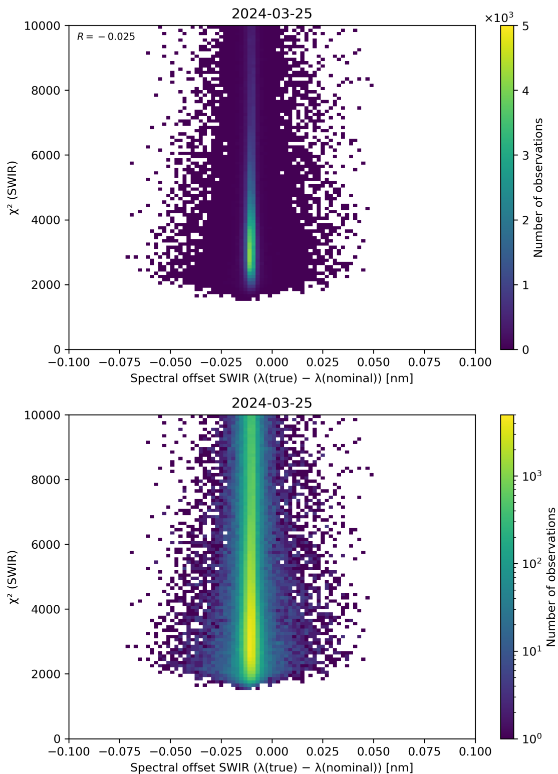
Figure 118: Scatter density plot of “Spectral offset SWIR ( \lambda(\text{true}) - \lambda(\text{nominal}) )” against “ \chi^2 (SWIR)” for 2024-03-25 to 2024-03-26.
