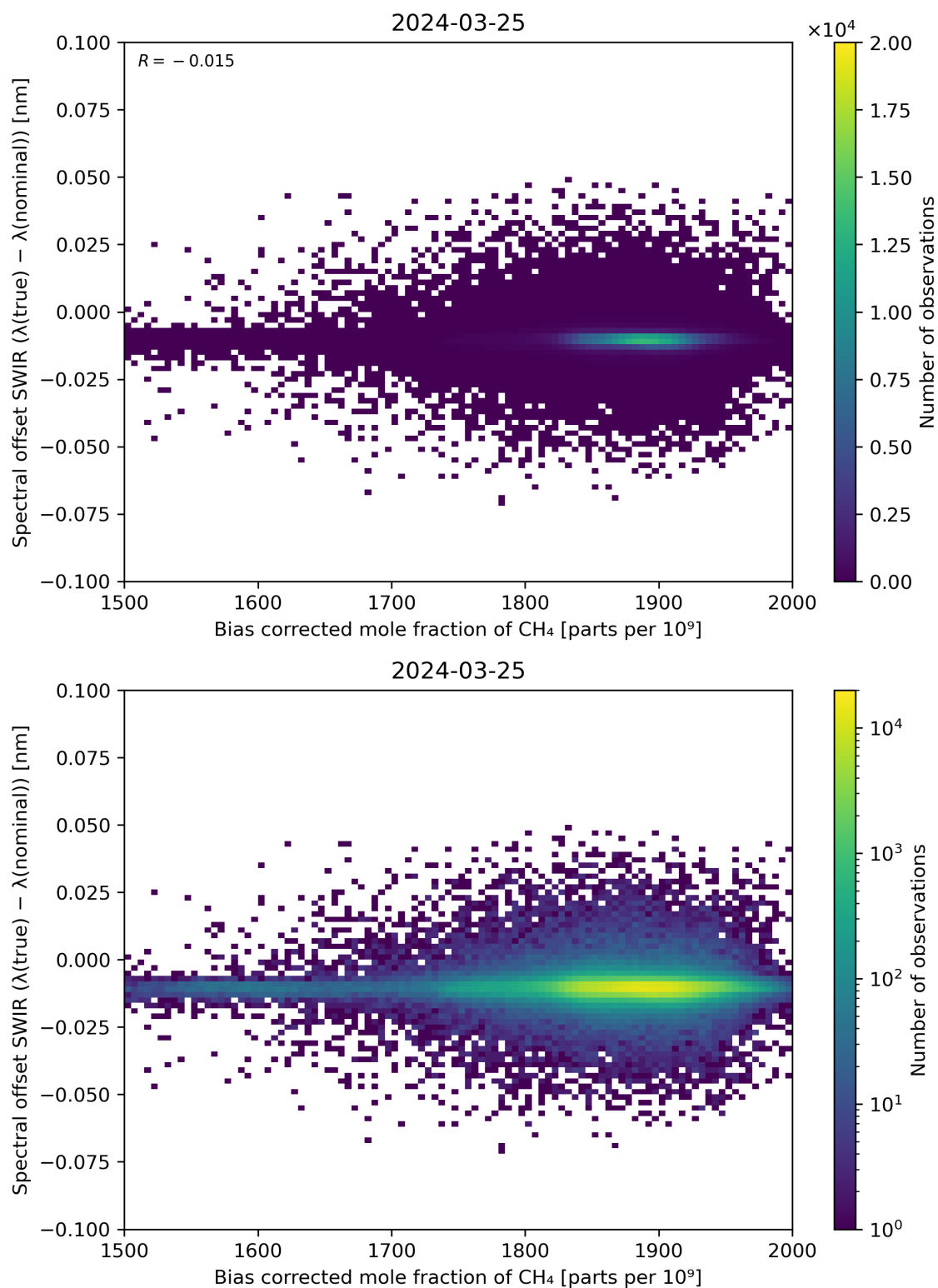
Figure 69: Scatter density plot of “Bias corrected mole fraction of \text{CH}_4 ” against “Spectral offset SWIR ( \lambda(\text{true}) - \lambda(\text{nominal}) )” for 2024-03-25 to 2024-03-26.
