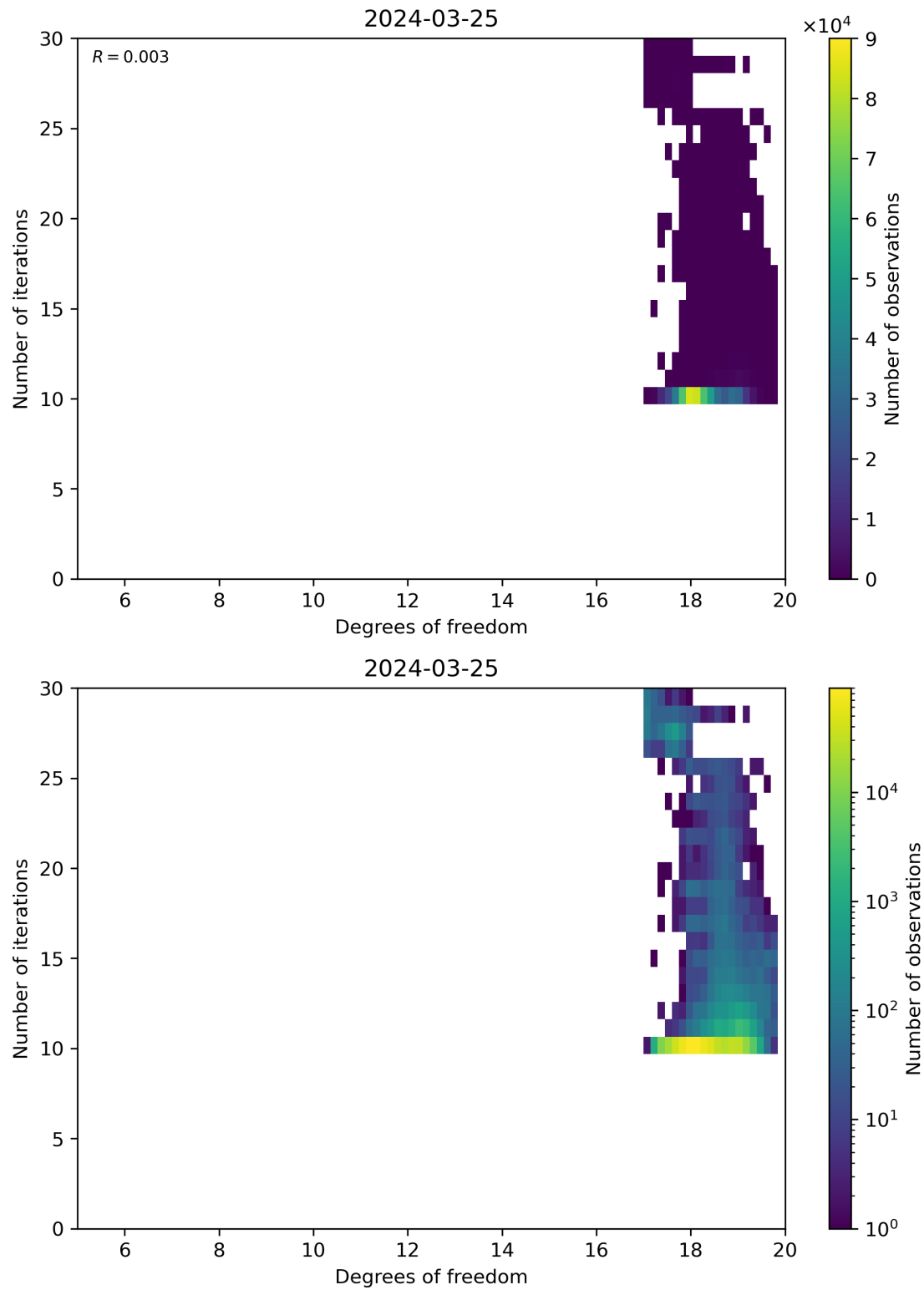
Figure 52: Scatter density plot of “Degrees of freedom” against “Number of iterations” for 2024-03-25 to 2024-03-26.
