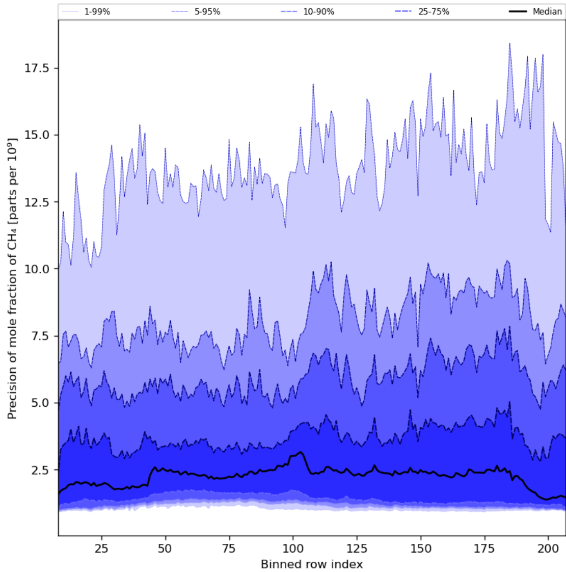
Figure 35: Along track statistics of “Precision of mole fraction of CH 4 ” for 2024-03-25 to 2024-03-26
