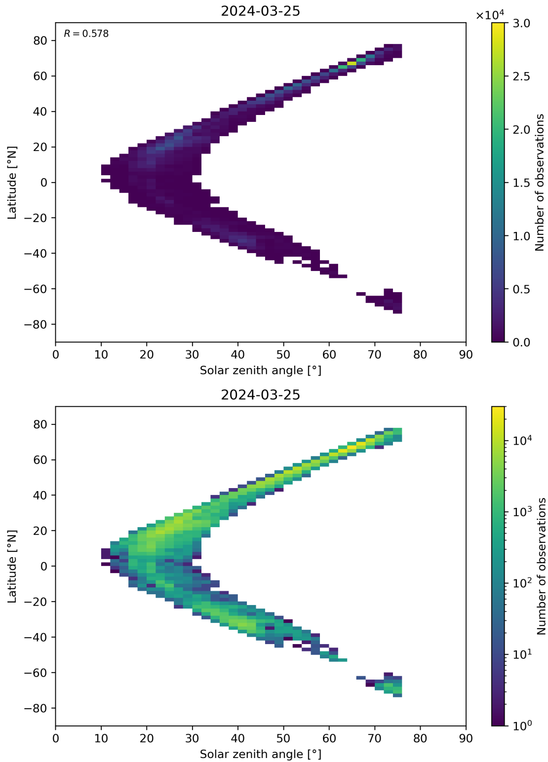
Figure 98: Scatter density plot of “Solar zenith angle” against “Latitude” for 2024-03-25 to 2024-03-26.
