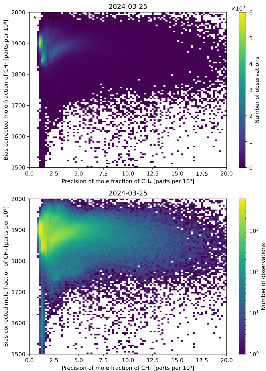
Figure 82: Scatter density plot of “Precision of mole fraction of CH 4 ” against “Bias corrected mole fraction of CH 4 ” for 2024-03-25 to 2024-03-26.
