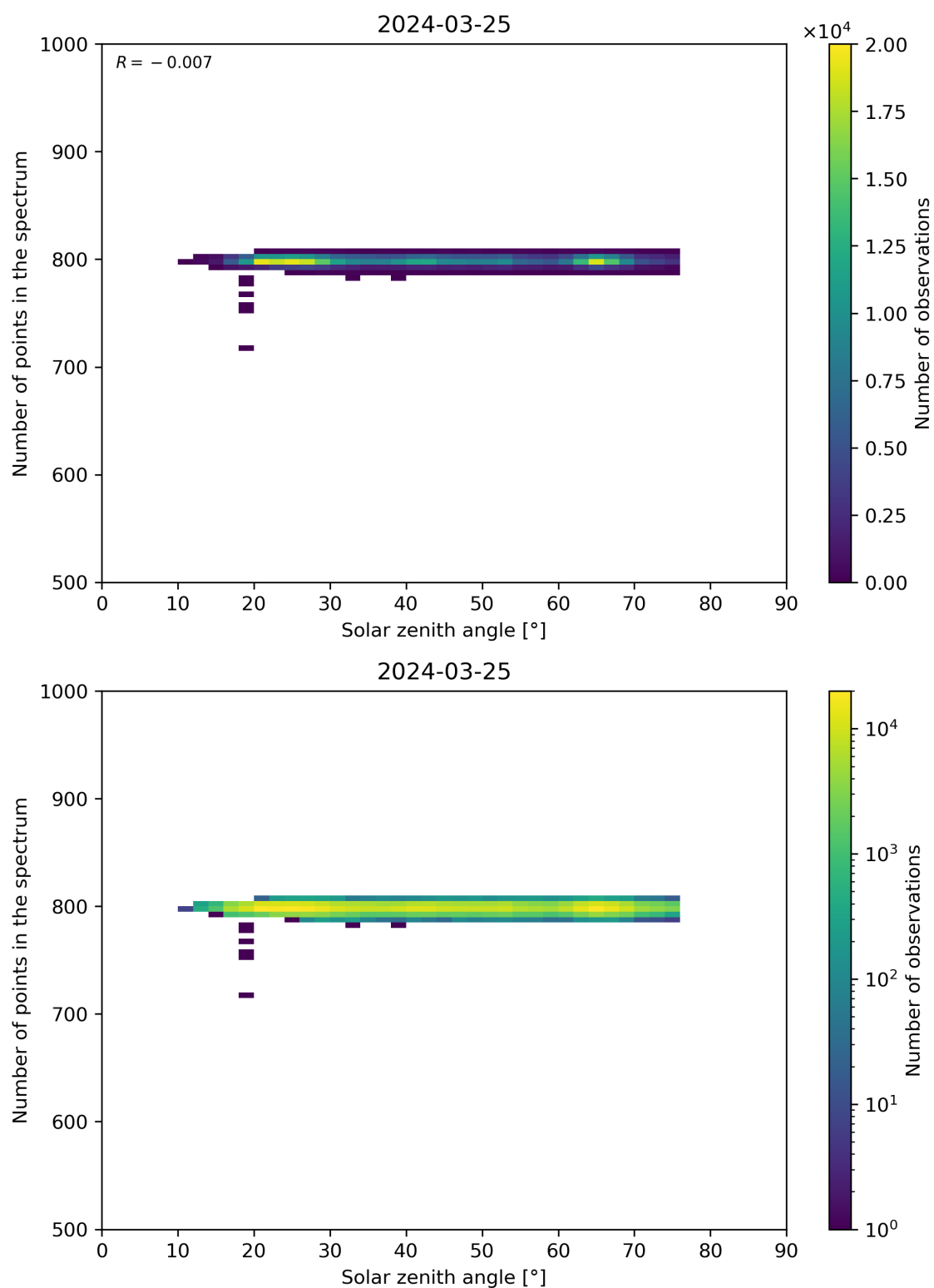
Figure 103: Scatter density plot of “Solar zenith angle” against “Number of points in the spectrum” for 2024-03-25 to 2024-03-26.
