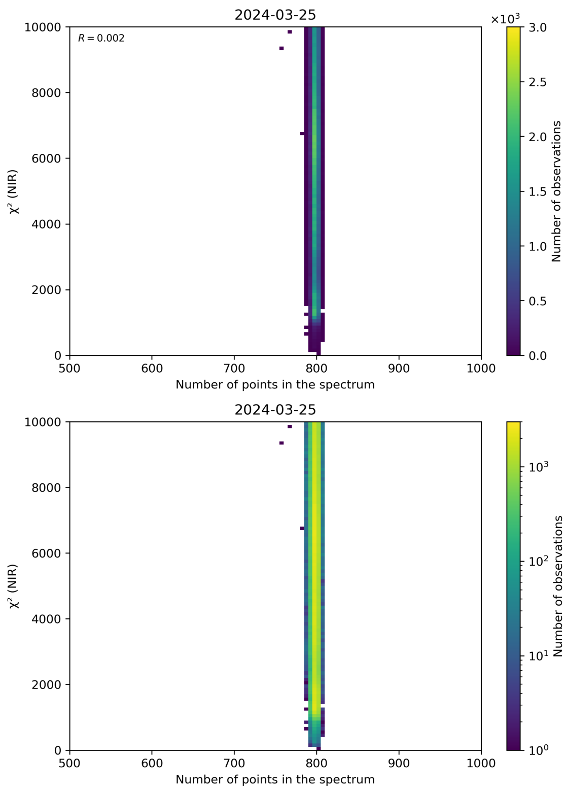
Figure 88: Scatter density plot of “Number of points in the spectrum” against “ \chi^2 (NIR)” for 2024-03-25 to 2024-03-26.
