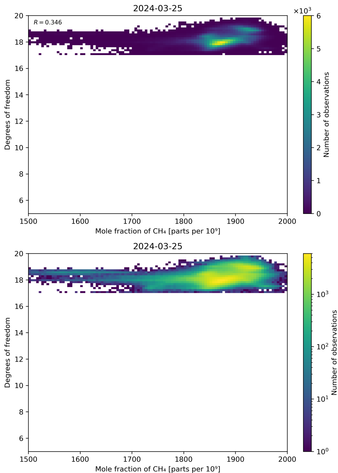
Figure 72: Scatter density plot of “Mole fraction of CH 4 ” against “Degrees of freedom” for 2024-03-25 to 2024-03-26.
