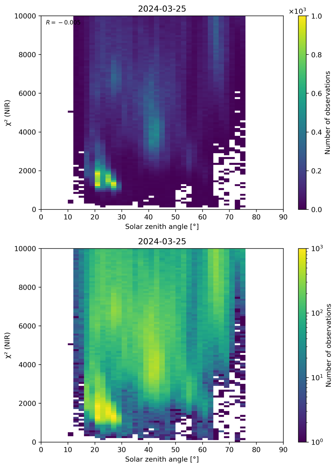
Figure 94: Scatter density plot of “Solar zenith angle” against “ \chi^2 (NIR)” for 2024-03-25 to 2024-03-26.
