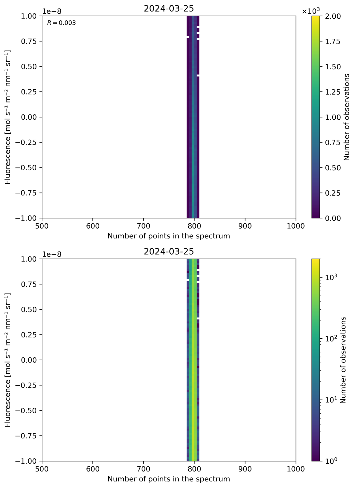
Figure 91: Scatter density plot of “Number of points in the spectrum” against “Fluorescence” for 2024-03-25 to 2024-03-26.
