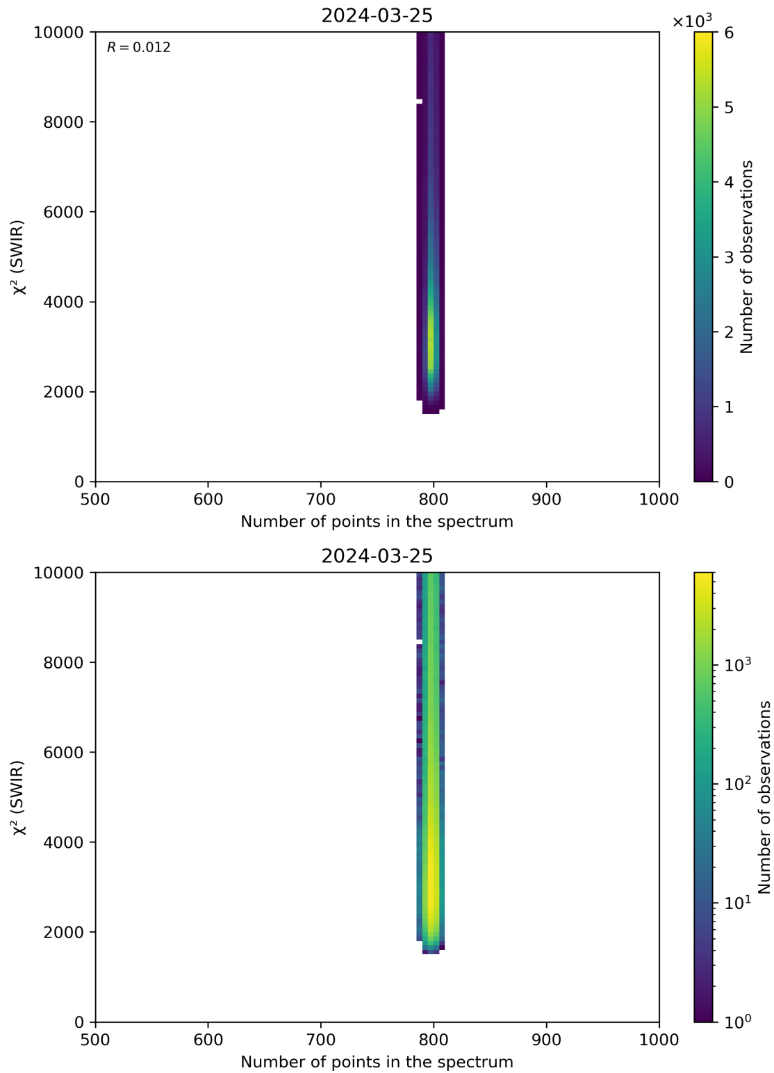
Figure 89: Scatter density plot of “Number of points in the spectrum” against “ \chi^2 (SWIR)” for 2024-03-25 to 2024-03-26.
