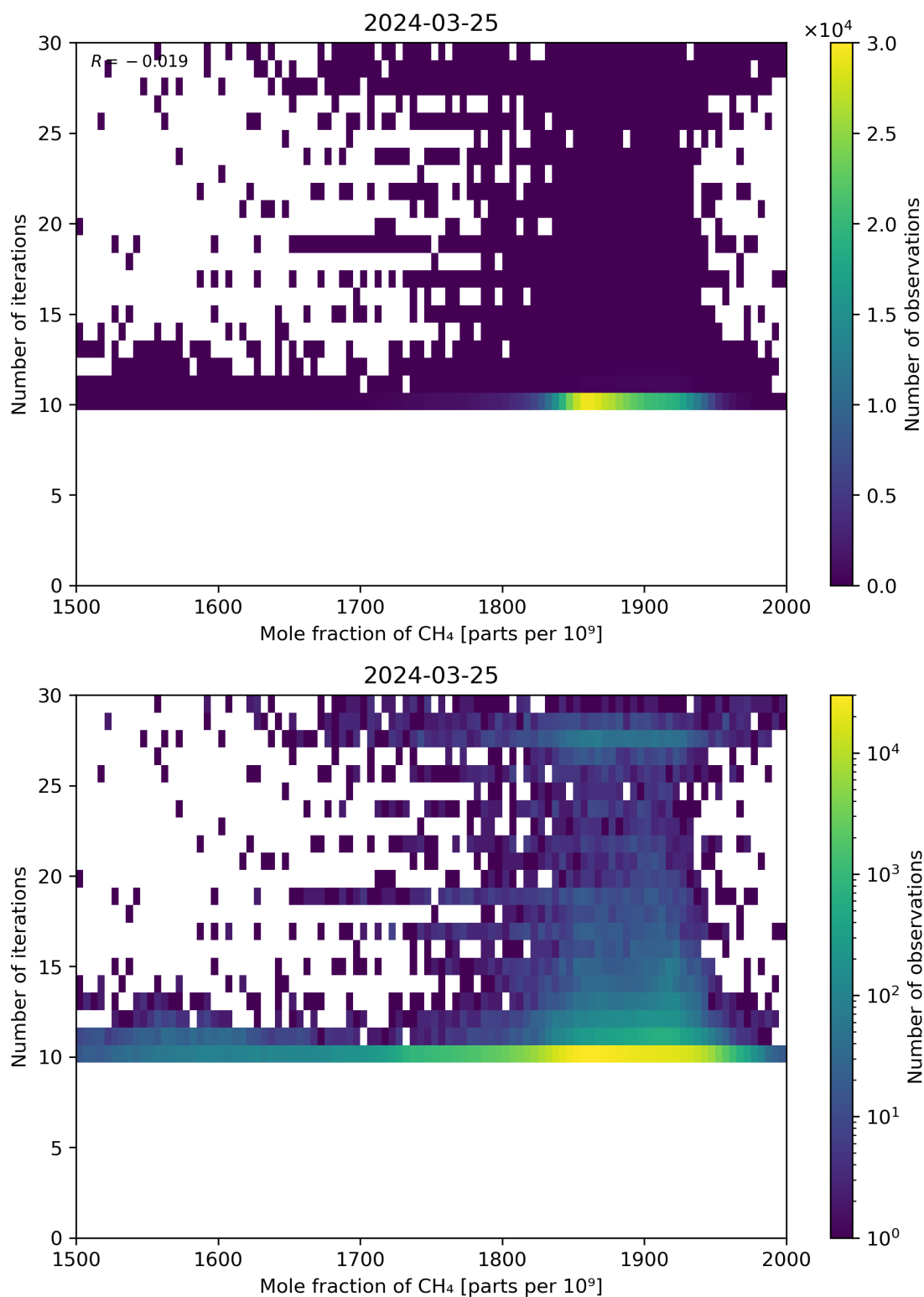
Figure 76: Scatter density plot of “Mole fraction of CH 4 ” against “Number of iterations” for 2024-03-25 to 2024-03-26.
