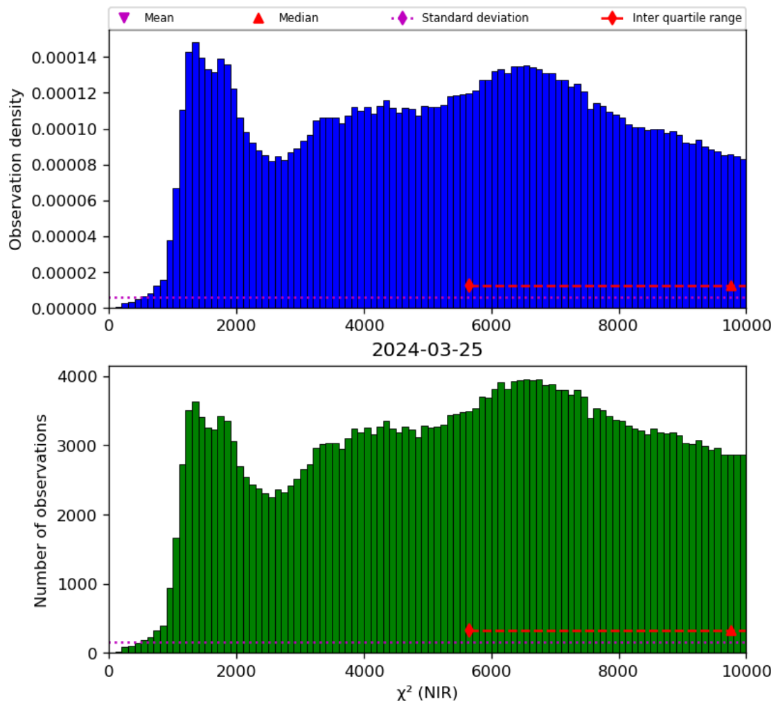
Figure 29: Histogram of “ \chi^2 (NIR)” for 2024-03-25 to 2024-03-26
