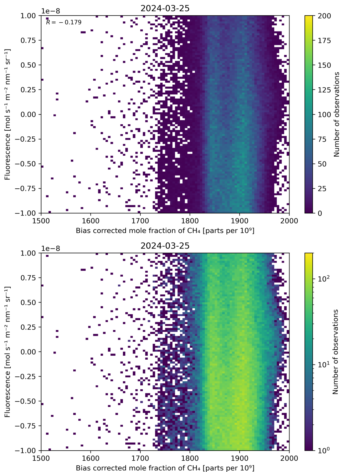
Figure 66: Scatter density plot of “Bias corrected mole fraction of \text{CH}_4 ” against “Fluorescence” for 2024-03-25 to 2024-03-26.
