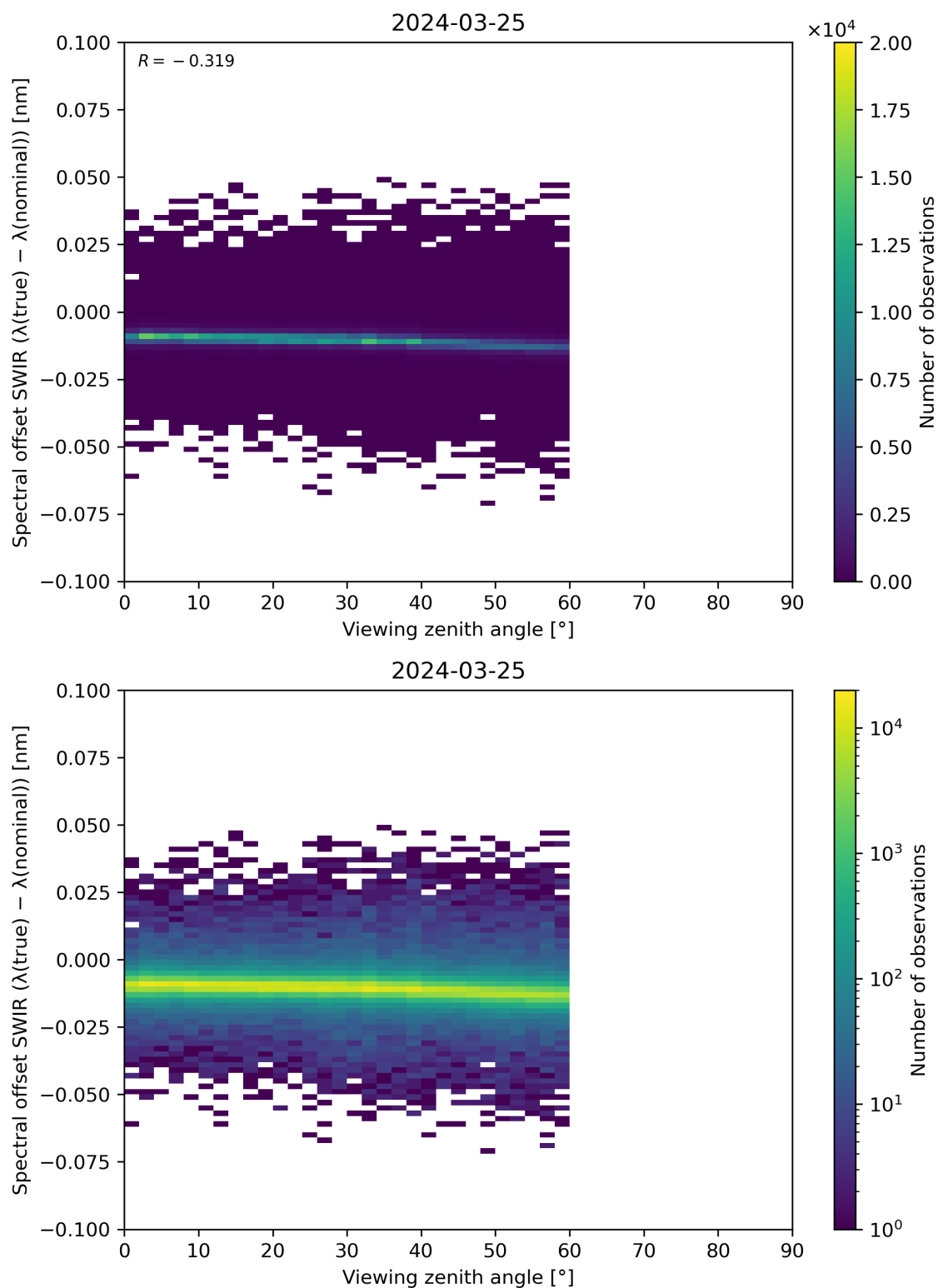
Figure 116: Scatter density plot of “Viewing zenith angle” against “Spectral offset SWIR ( \lambda(\text{true}) - \lambda(\text{nominal}) )” for 2024-03-25 to 2024-03-26.
