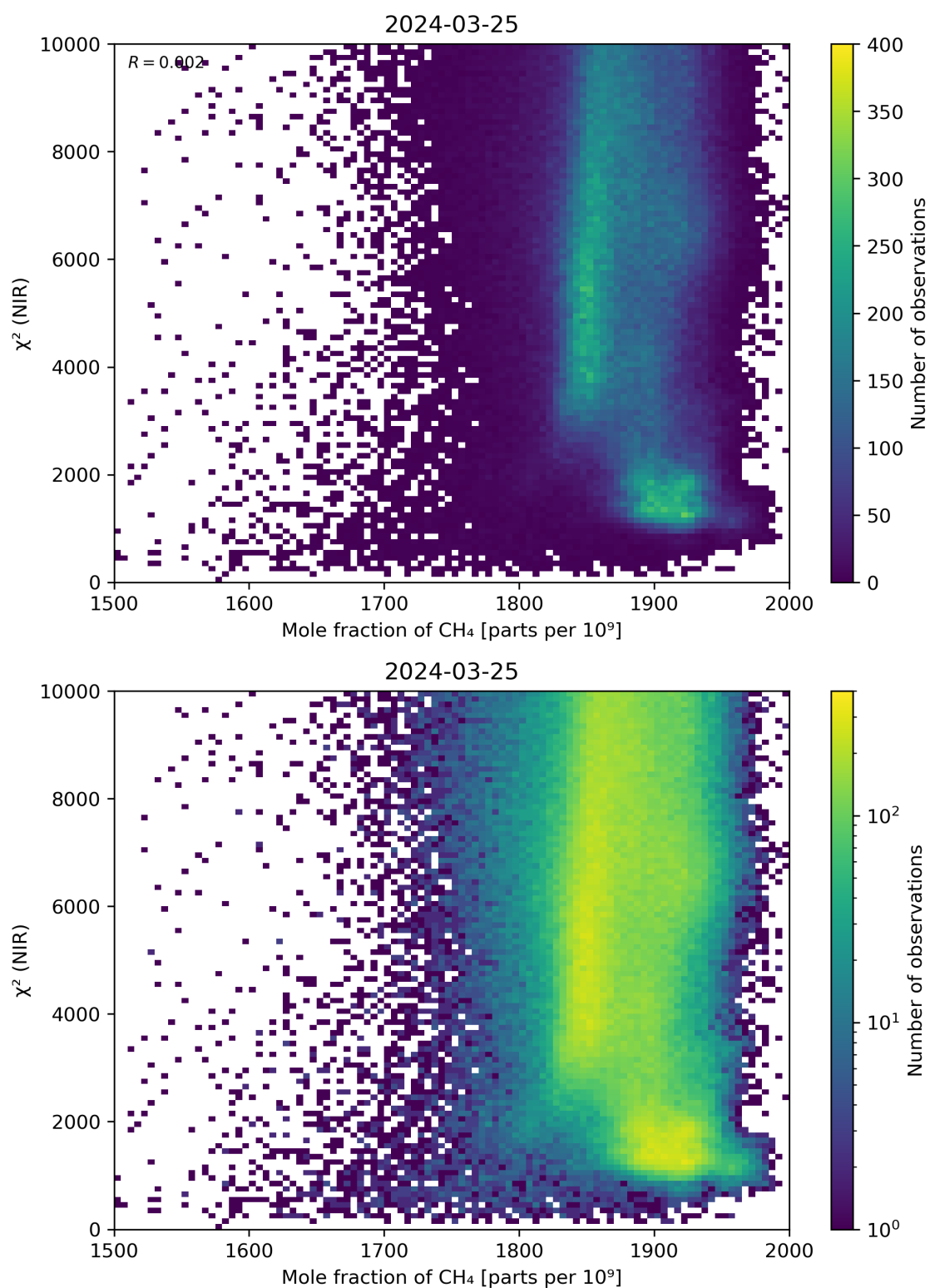
Figure 70: Scatter density plot of “Mole fraction of \text{CH}_4 ” against “ \chi^2 (NIR)” for 2024-03-25 to 2024-03-26.
