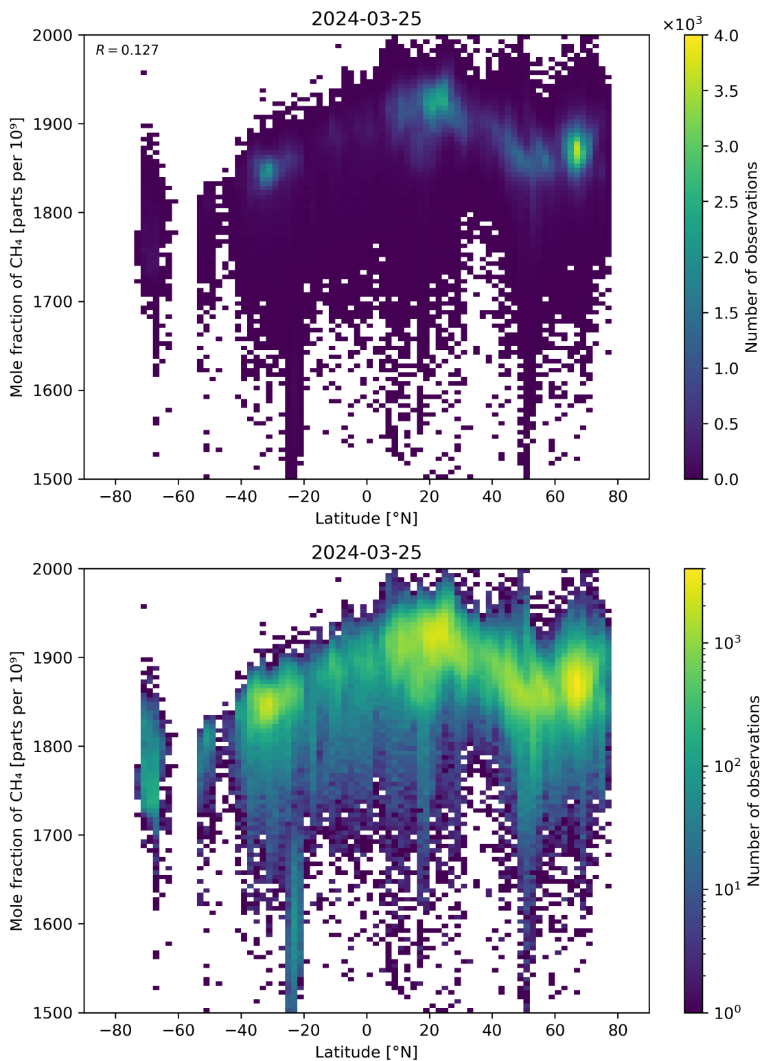
Figure 57: Scatter density plot of “Latitude” against “Mole fraction of CH 4 ” for 2024-03-25 to 2024-03-26.
