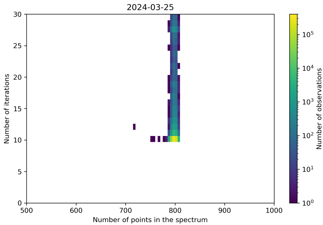
Figure 92: Scatter density plot of “Number of points in the spectrum” against “Number of iterations” for 2024-03-25 to 2024-03-26.
