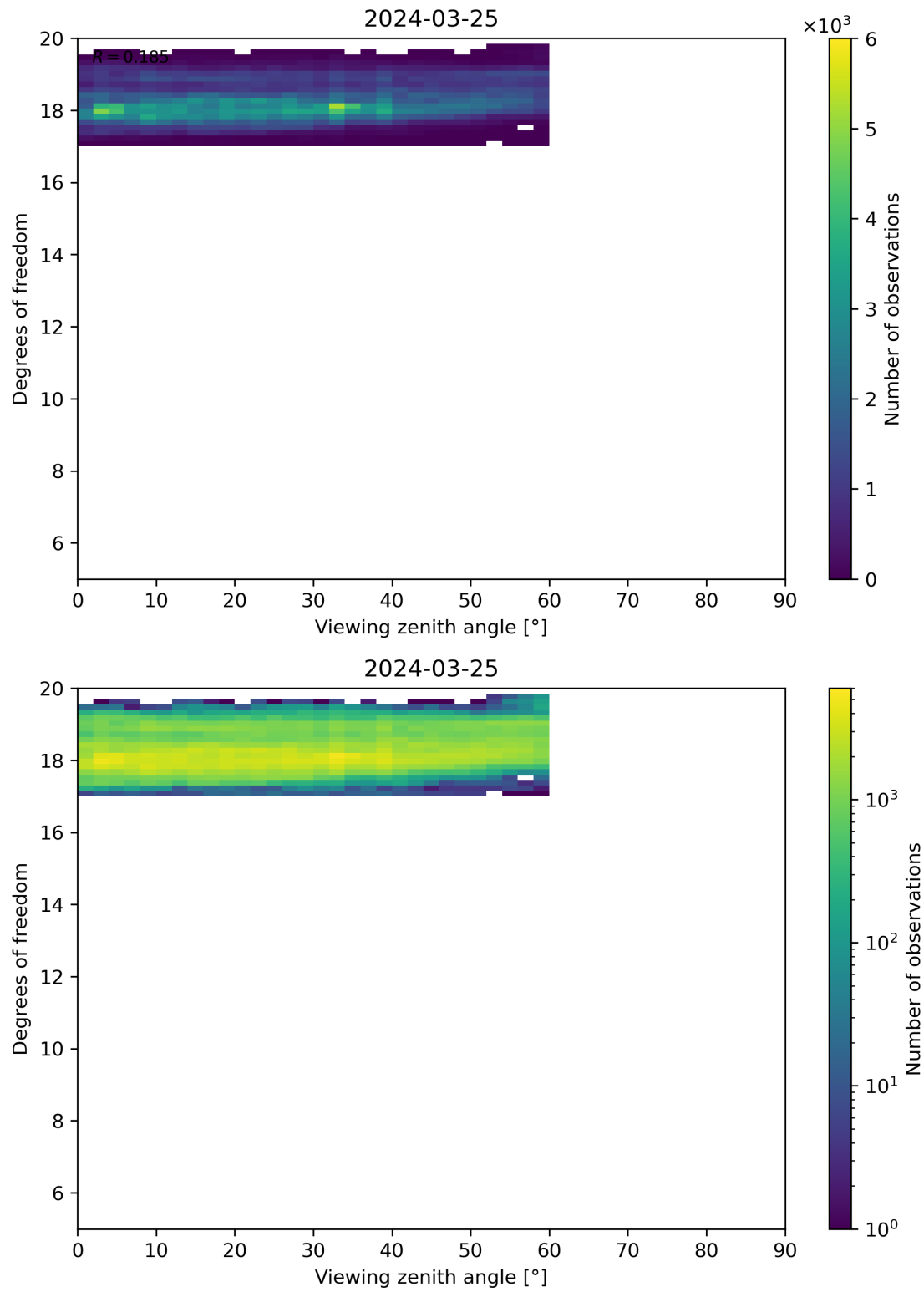
Figure 107: Scatter density plot of “Viewing zenith angle” against “Degrees of freedom” for 2024-03-25 to 2024-03-26.
