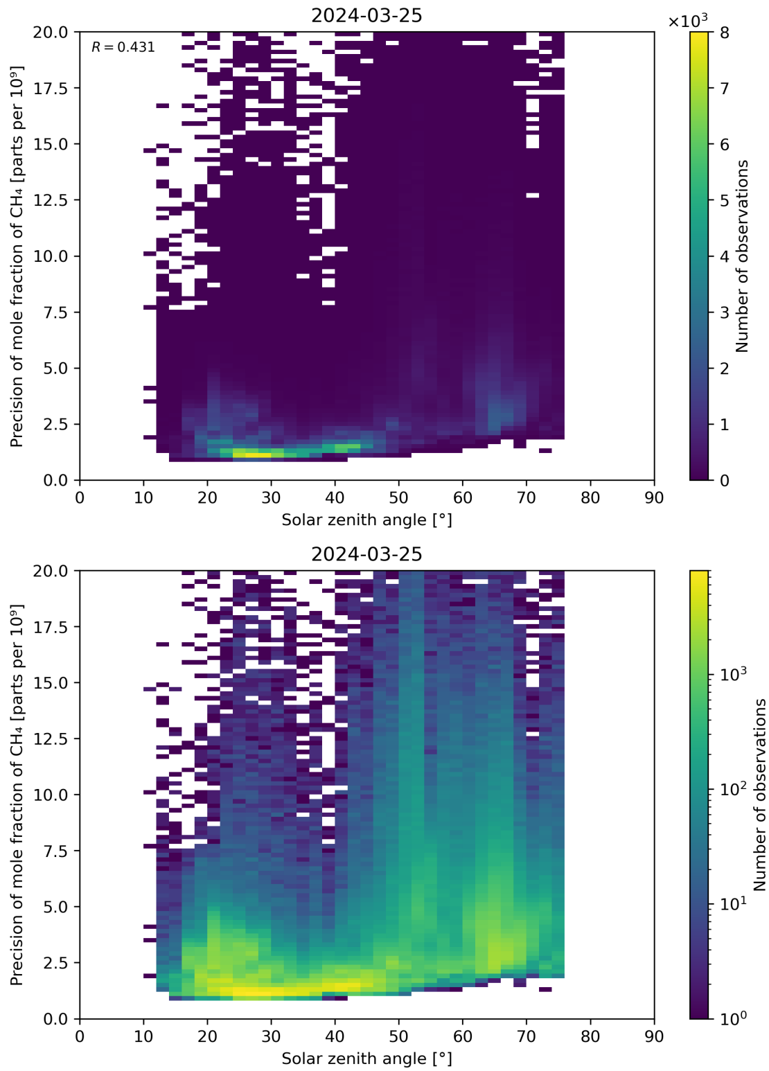
Figure 101: Scatter density plot of “Solar zenith angle” against “Precision of mole fraction of CH 4 ” for 2024-03-25 to 2024-03-26.
