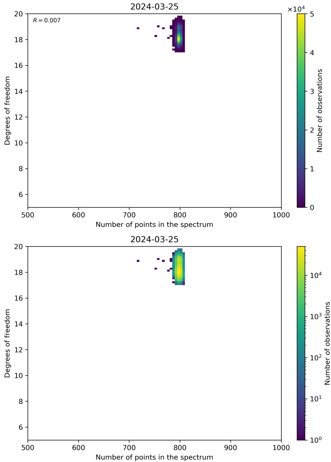
Figure 90: Scatter density plot of “Number of points in the spectrum” against “Degrees of freedom” for 2024-03-25 to 2024-03-26.
