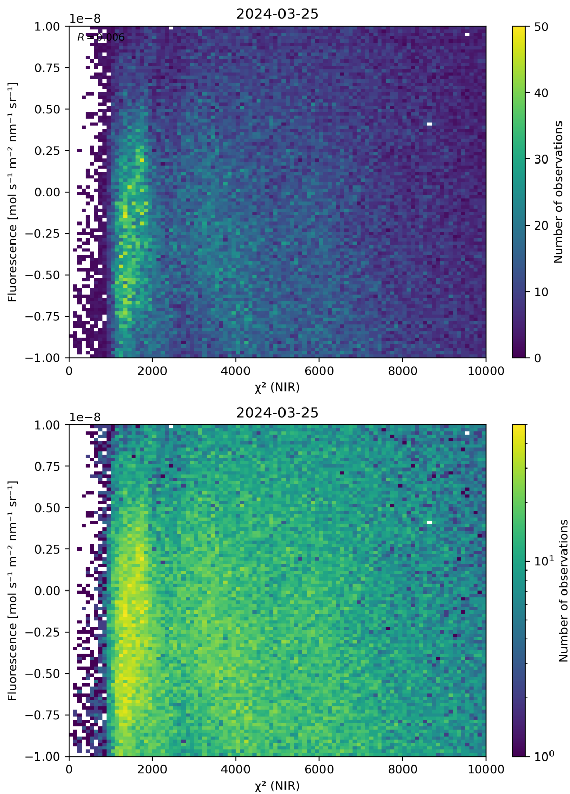
Figure 45: Scatter density plot of “ \chi^2 (NIR)” against “Fluorescence” for 2024-03-25 to 2024-03-26.
