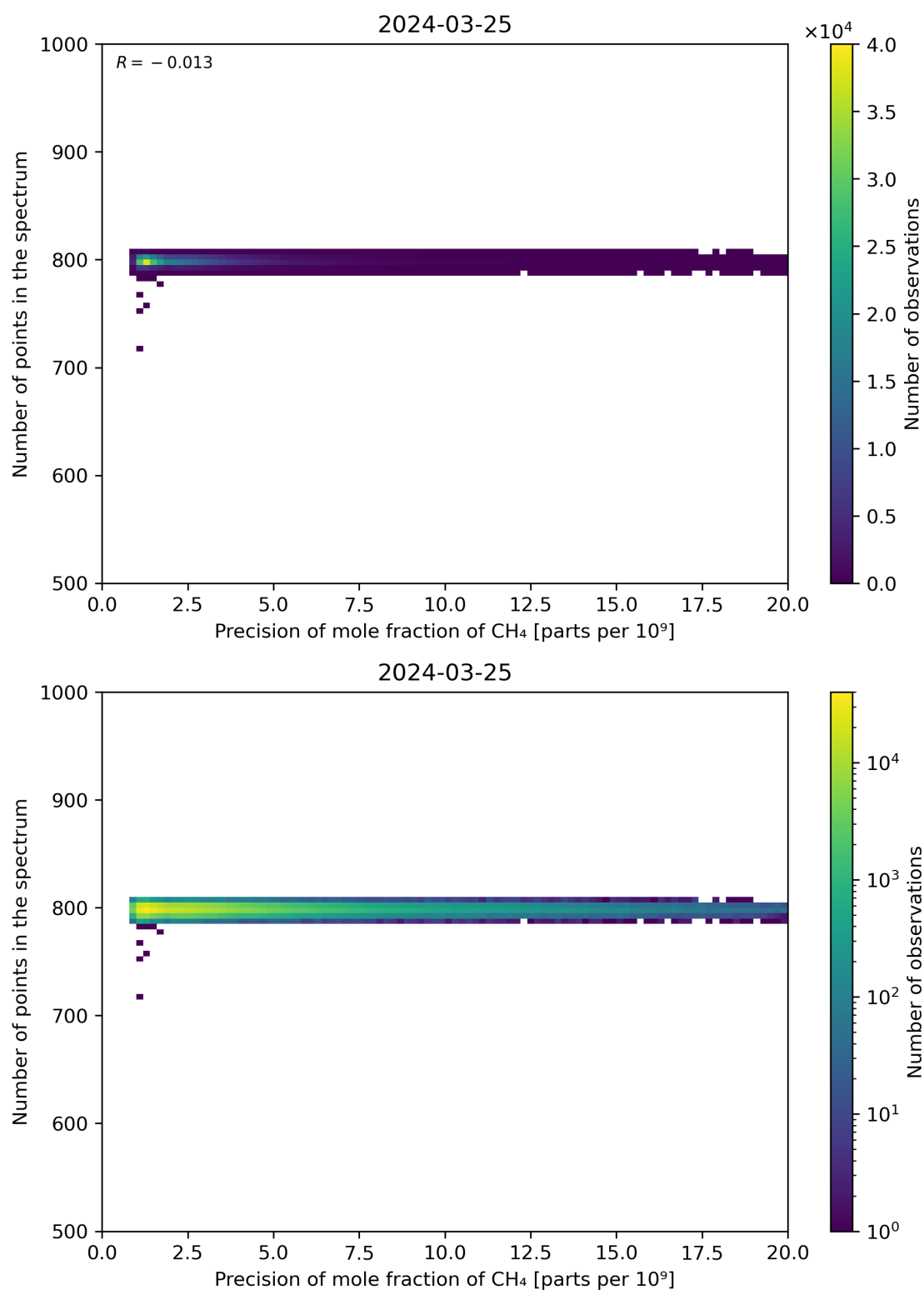
Figure 84: Scatter density plot of “Precision of mole fraction of CH 4 ” against “Number of points in the spectrum” for 2024-03-25 to 2024-03-26.
