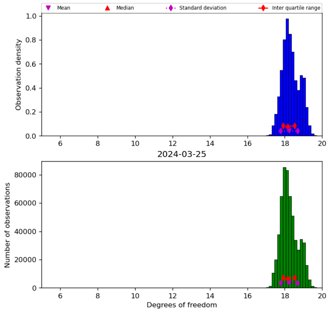
Figure 30: Histogram of “Degrees of freedom” for 2024-03-25 to 2024-03-26
