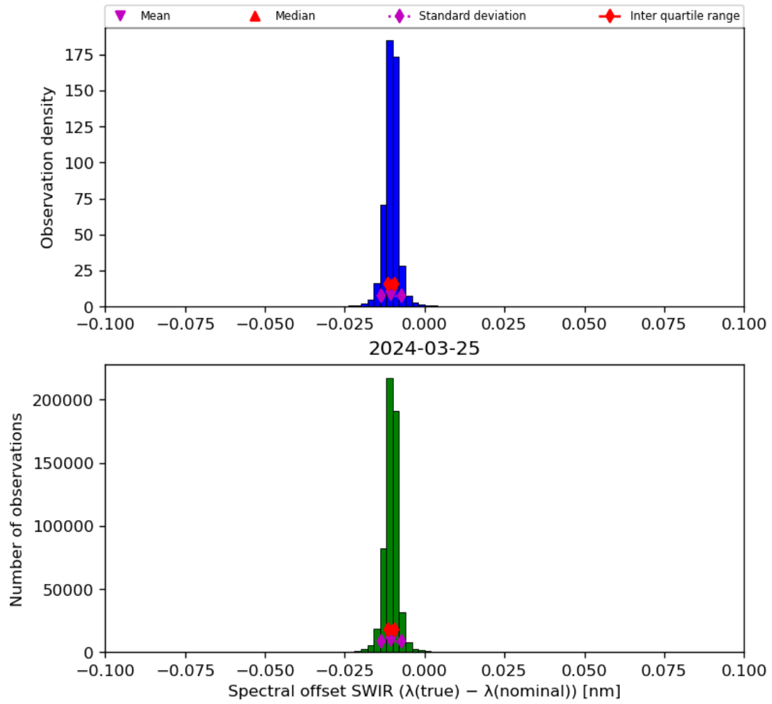
Figure 27: Histogram of “Spectral offset SWIR ( \lambda(\text{true}) - \lambda(\text{nominal}) )” for 2024-03-25 to 2024-03-26
