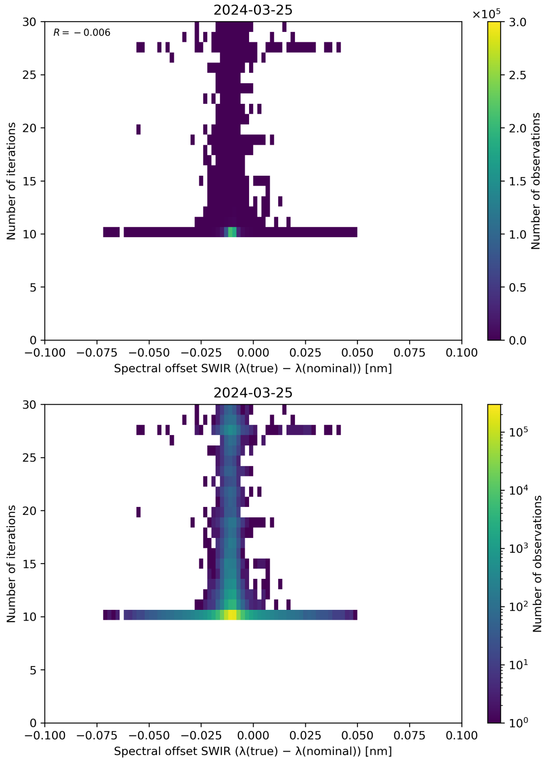
Figure 121: Scatter density plot of “Spectral offset SWIR ( \lambda(\text{true}) - \lambda(\text{nominal}) )” against “Number of iterations” for 2024-03-25 to 2024-03-26.
