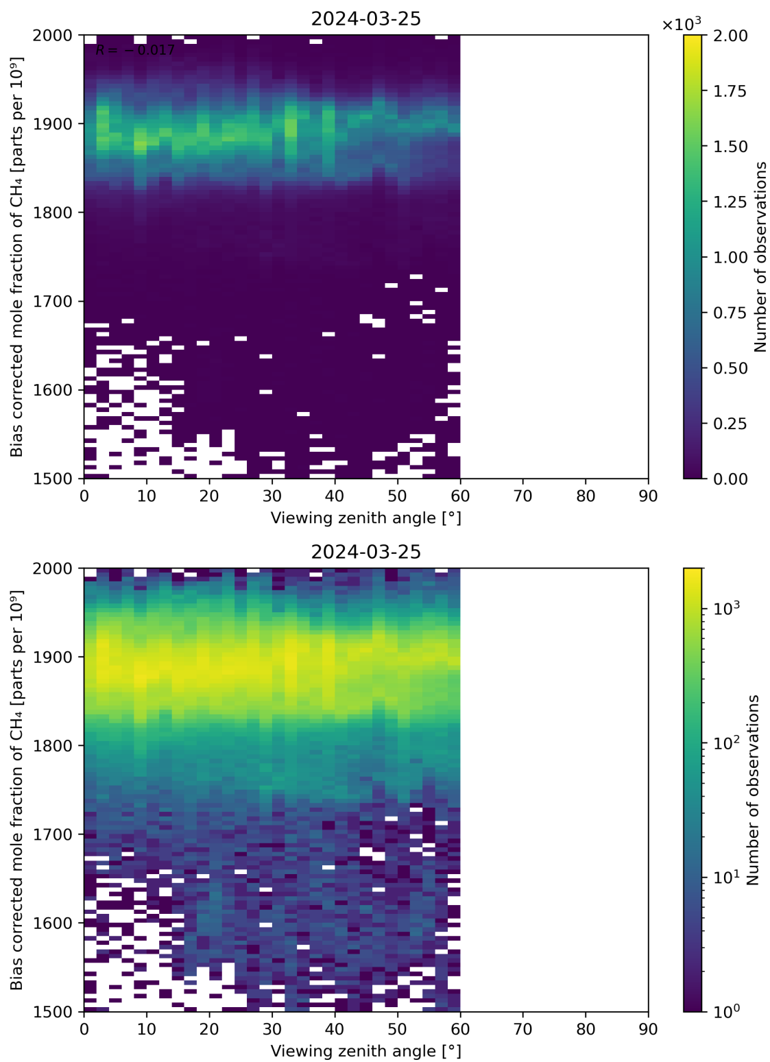
Figure 111: Scatter density plot of “Viewing zenith angle” against “Bias corrected mole fraction of CH 4 ” for 2024-03-25 to 2024-03-26.
