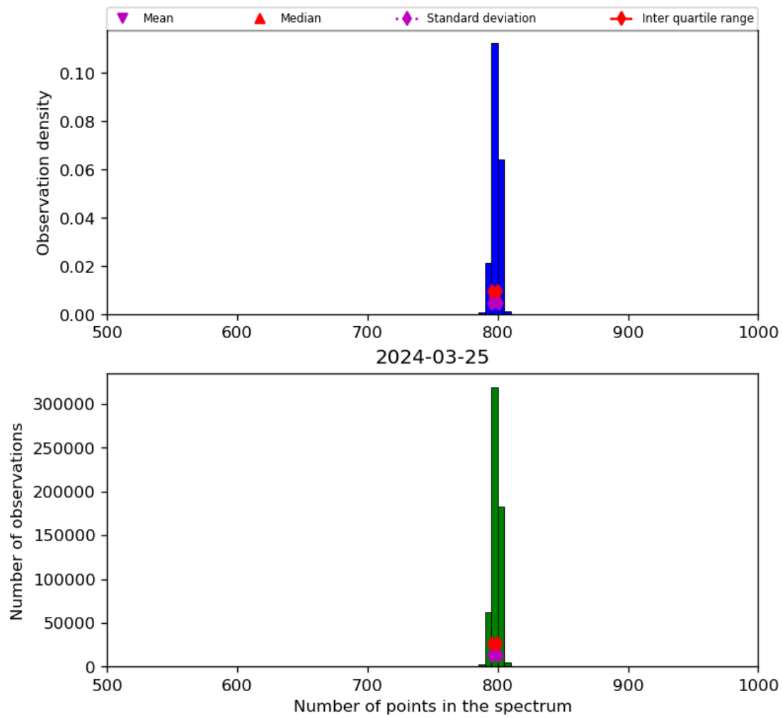
Figure 26: Histogram of “Number of points in the spectrum” for 2024-03-25 to 2024-03-26
