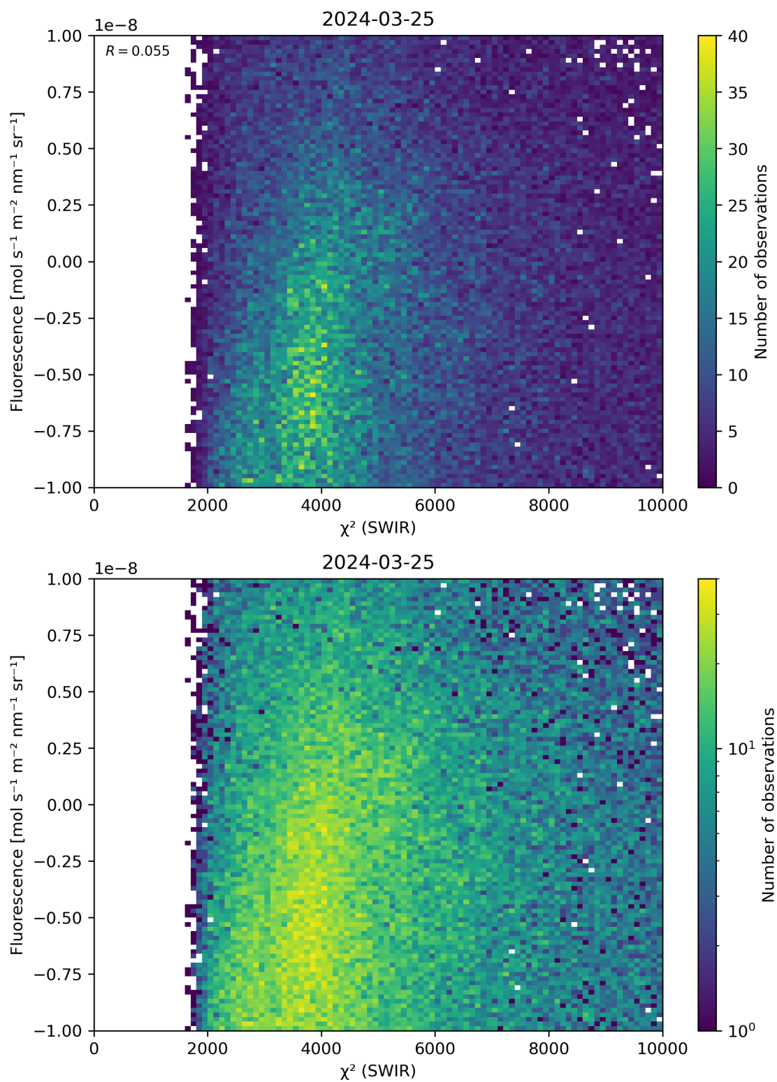
Figure 49: Scatter density plot of “ \chi^2 (SWIR)” against “Fluorescence” for 2024-03-25 to 2024-03-26.
