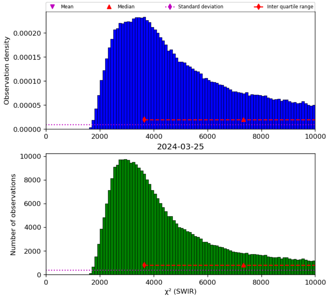
Figure 28: Histogram of “ \chi^2 (SWIR)” for 2024-03-25 to 2024-03-26
