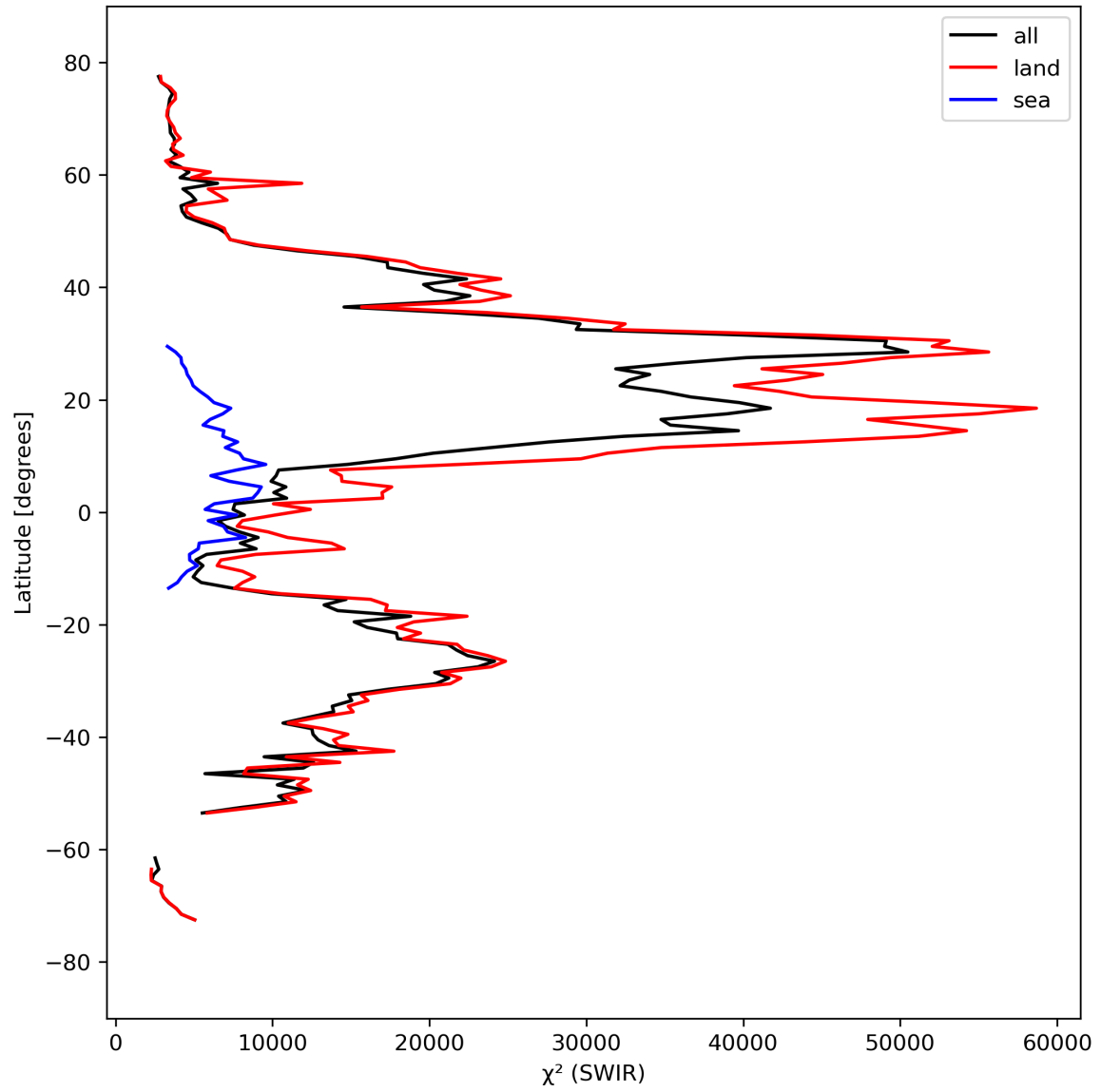
Figure 17: Zonal average of “ \chi^2 (SWIR)” for 2024-03-25 to 2024-03-26.
