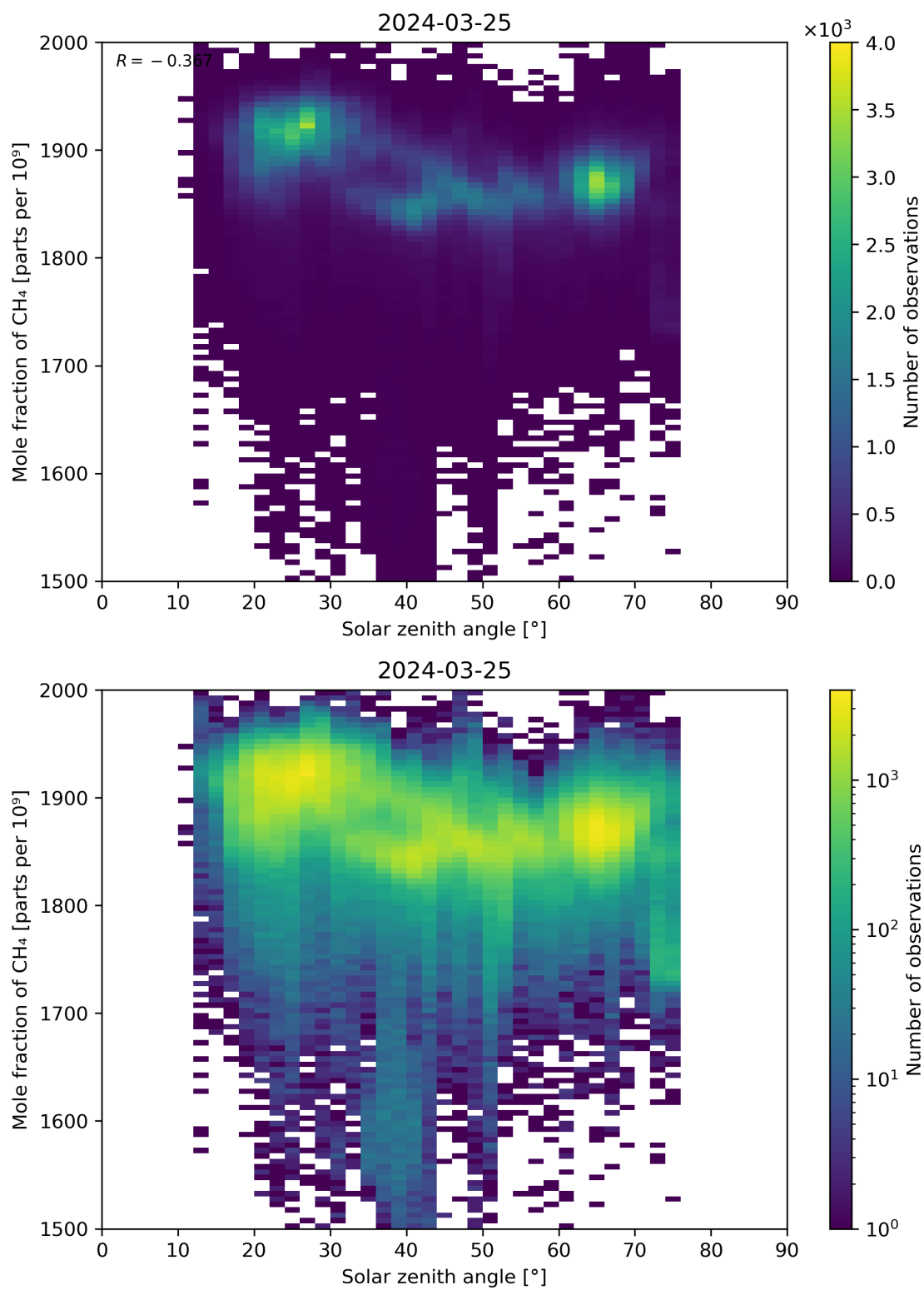
Figure 99: Scatter density plot of “Solar zenith angle” against “Mole fraction of CH 4 ” for 2024-03-25 to 2024-03-26.
