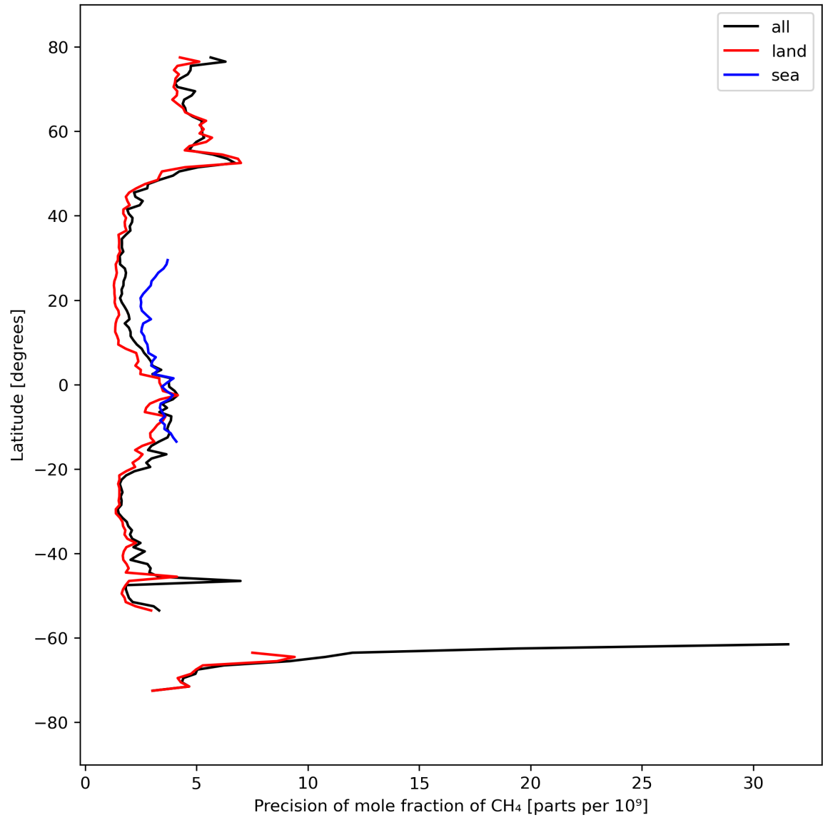
Figure 13: Zonal average of “Precision of mole fraction of CH 4 ” for 2024-03-25 to 2024-03-26.
