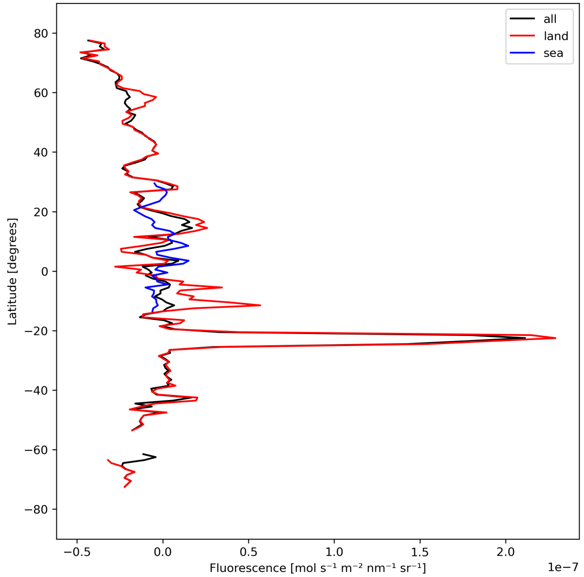
Figure 21: Zonal average of “Fluorescence” for 2024-03-25 to 2024-03-26.
