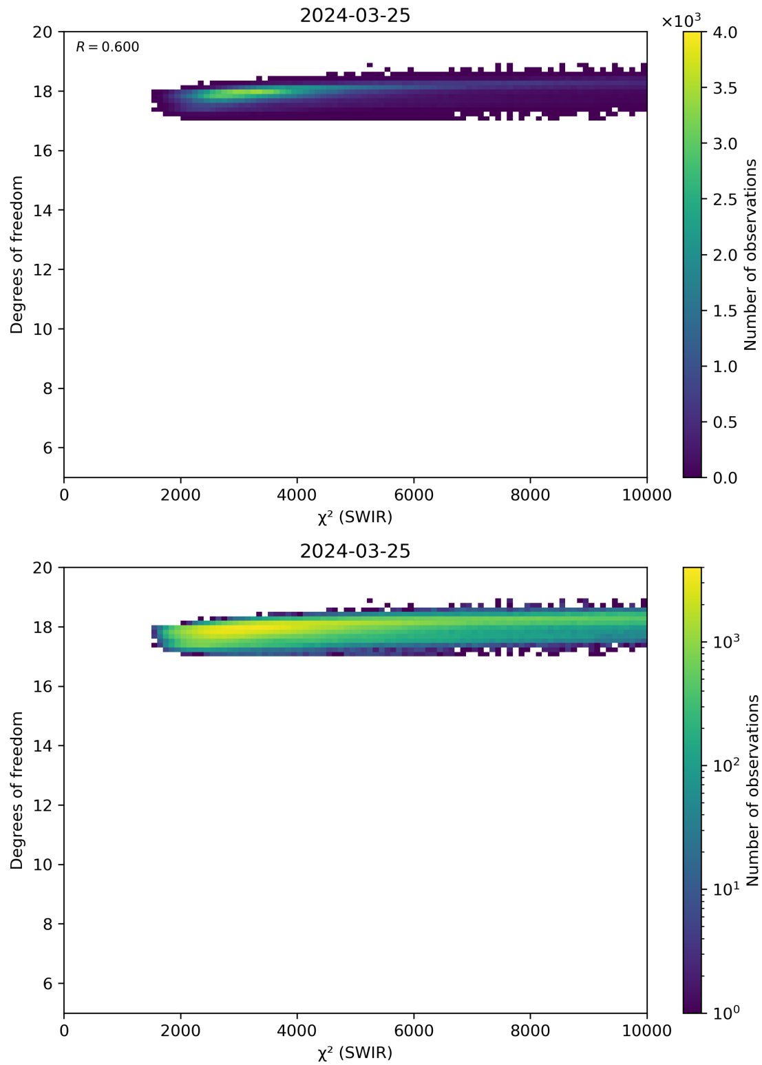
Figure 48: Scatter density plot of “ \chi^2 (SWIR)” against “Degrees of freedom” for 2024-03-25 to 2024-03-26.
