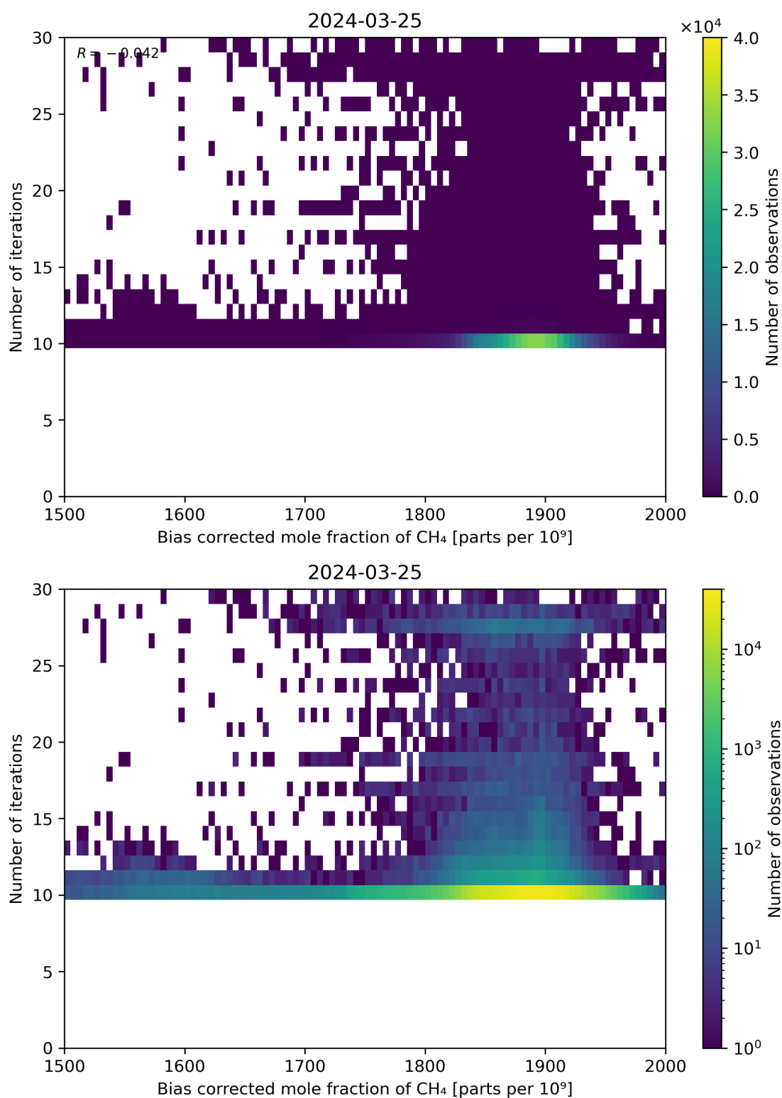
Figure 67: Scatter density plot of “Bias corrected mole fraction of CH 4 ” against “Number of iterations” for 2024-03-25 to 2024-03-26.
