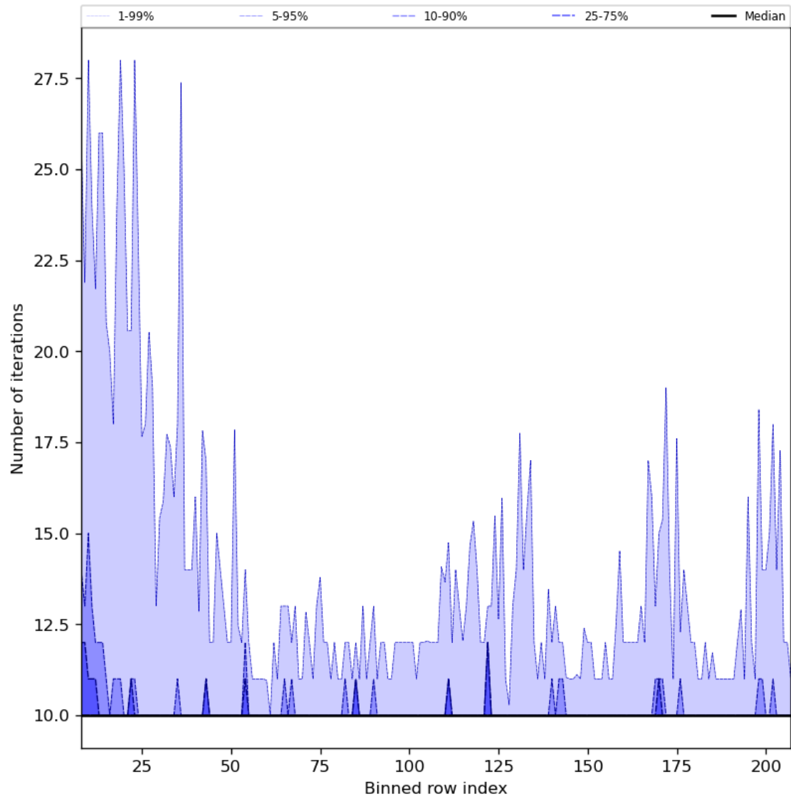
Figure 42: Along track statistics of “Number of iterations” for 2024-03-25 to 2024-03-26
