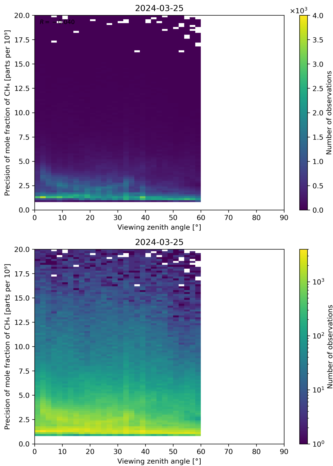
Figure 112: Scatter density plot of “Viewing zenith angle” against “Precision of mole fraction of CH 4 ” for 2024-03-25 to 2024-03-26.
