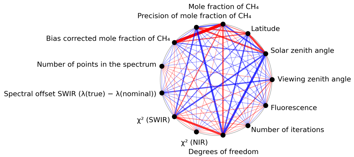
Figure 1: Map of correlation graph for 2024-03-25 to 2024-03-26.
