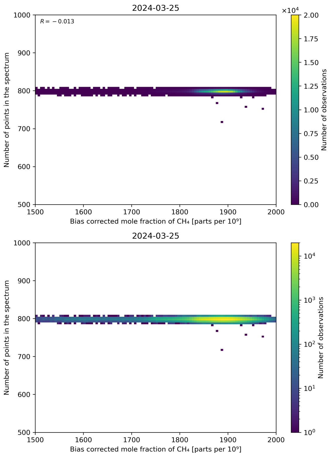
Figure 68: Scatter density plot of “Bias corrected mole fraction of CH 4 ” against “Number of points in the spectrum” for 2024-03-25 to 2024-03-26.
