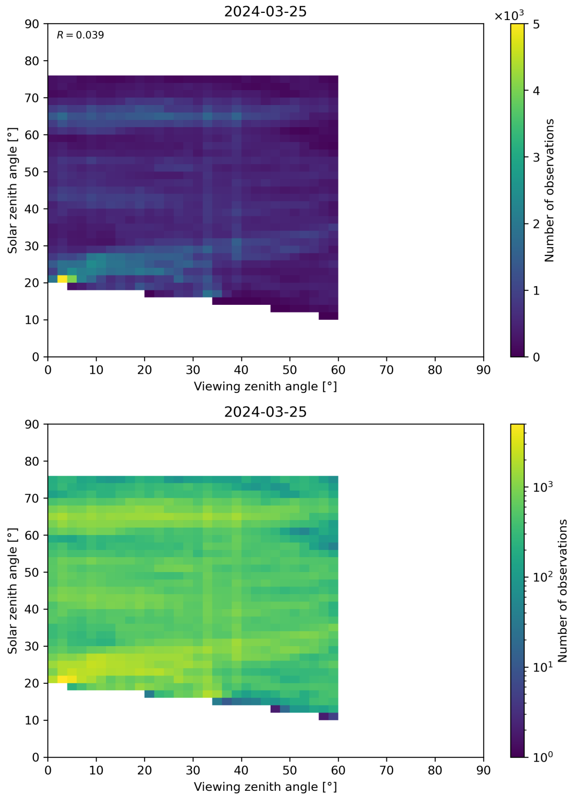
Figure 115: Scatter density plot of “Viewing zenith angle” against “Solar zenith angle” for 2024-03-25 to 2024-03-26.
