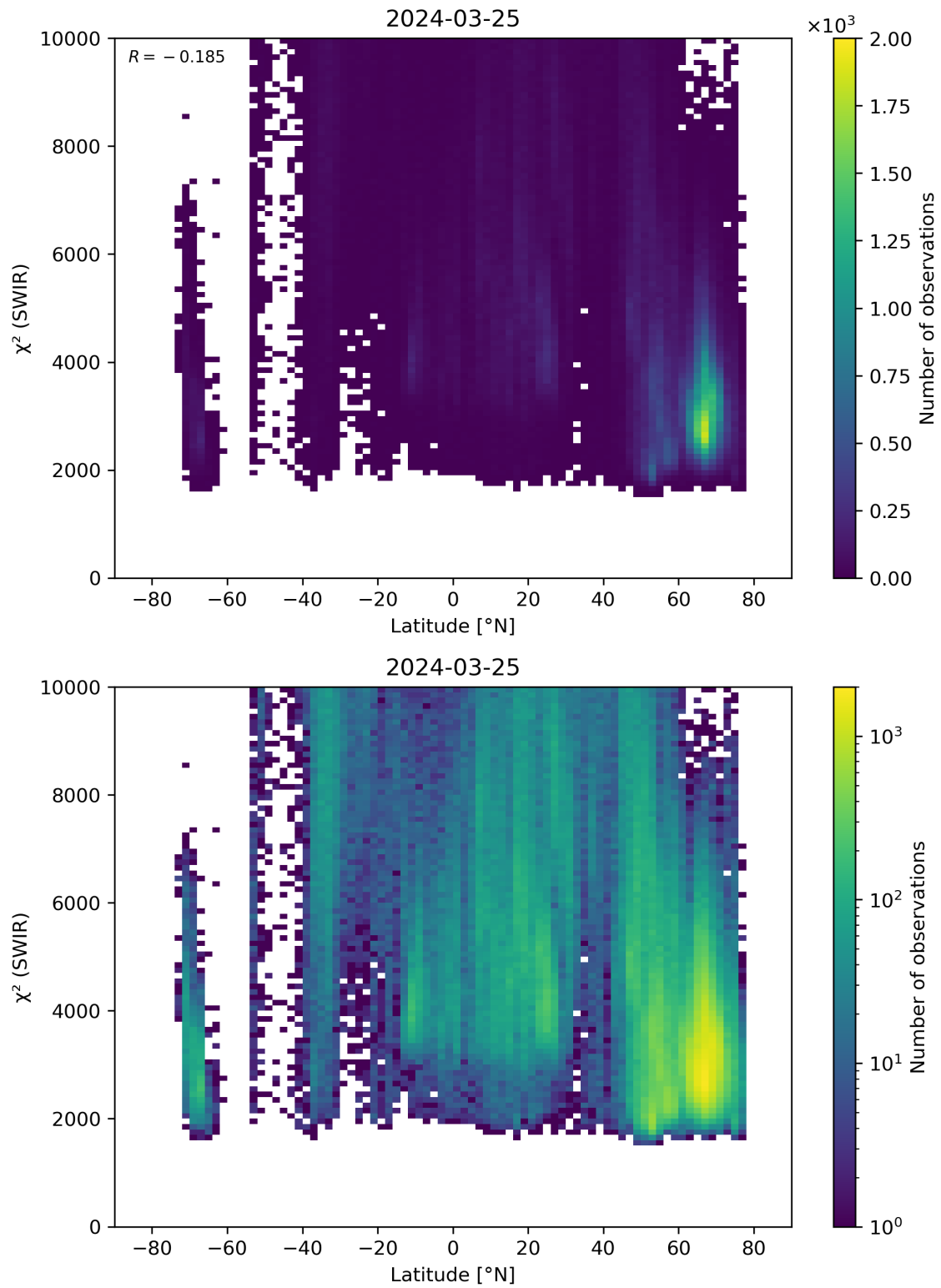
Figure 54: Scatter density plot of “Latitude” against “ \chi^2 (SWIR)” for 2024-03-25 to 2024-03-26.
