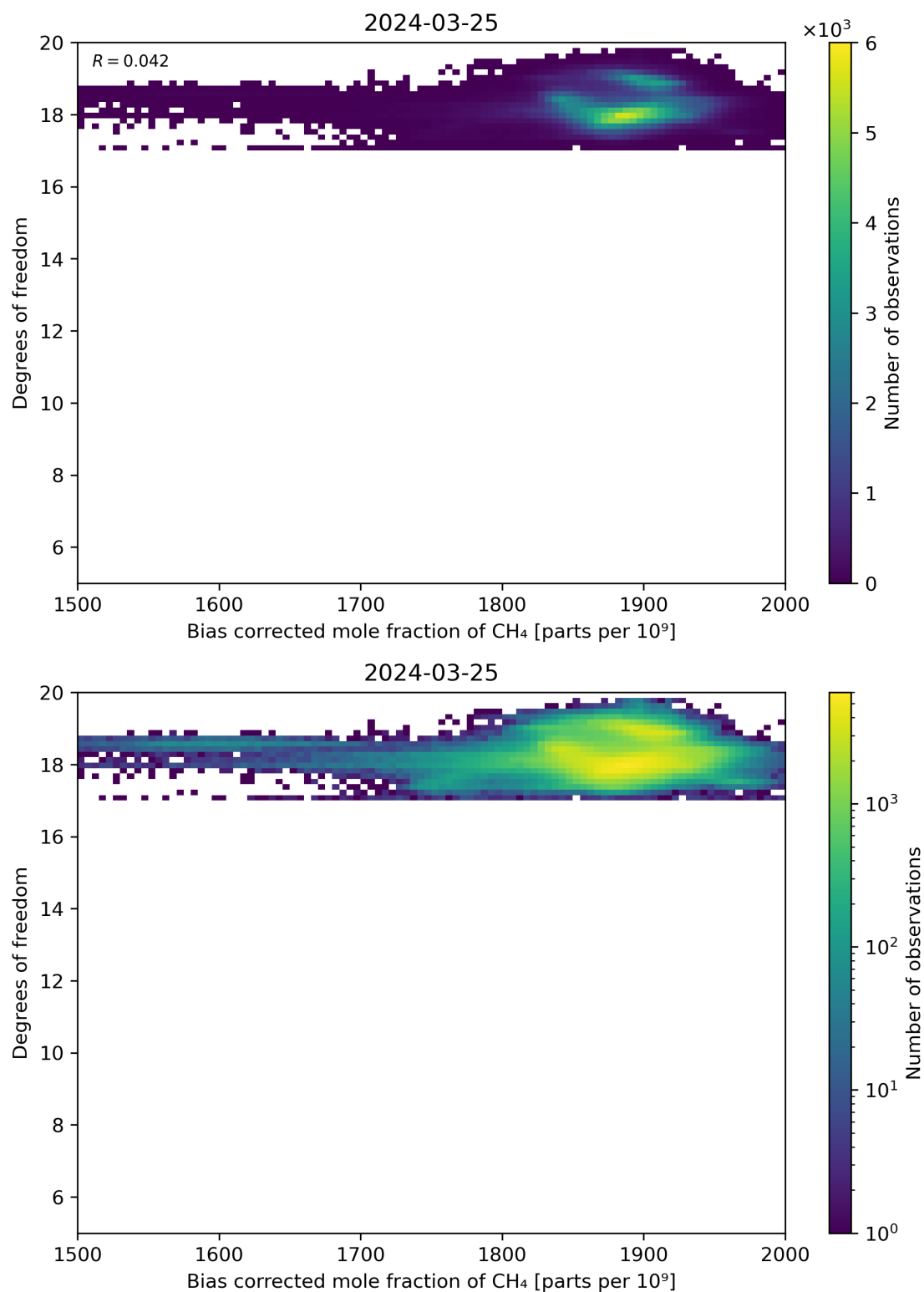
Figure 65: Scatter density plot of “Bias corrected mole fraction of CH 4 ” against “Degrees of freedom” for 2024-03-25 to 2024-03-26.
