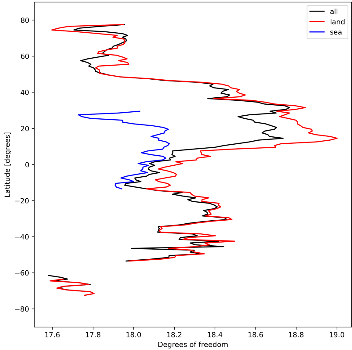
Figure 19: Zonal average of “Degrees of freedom” for 2024-03-25 to 2024-03-26.
