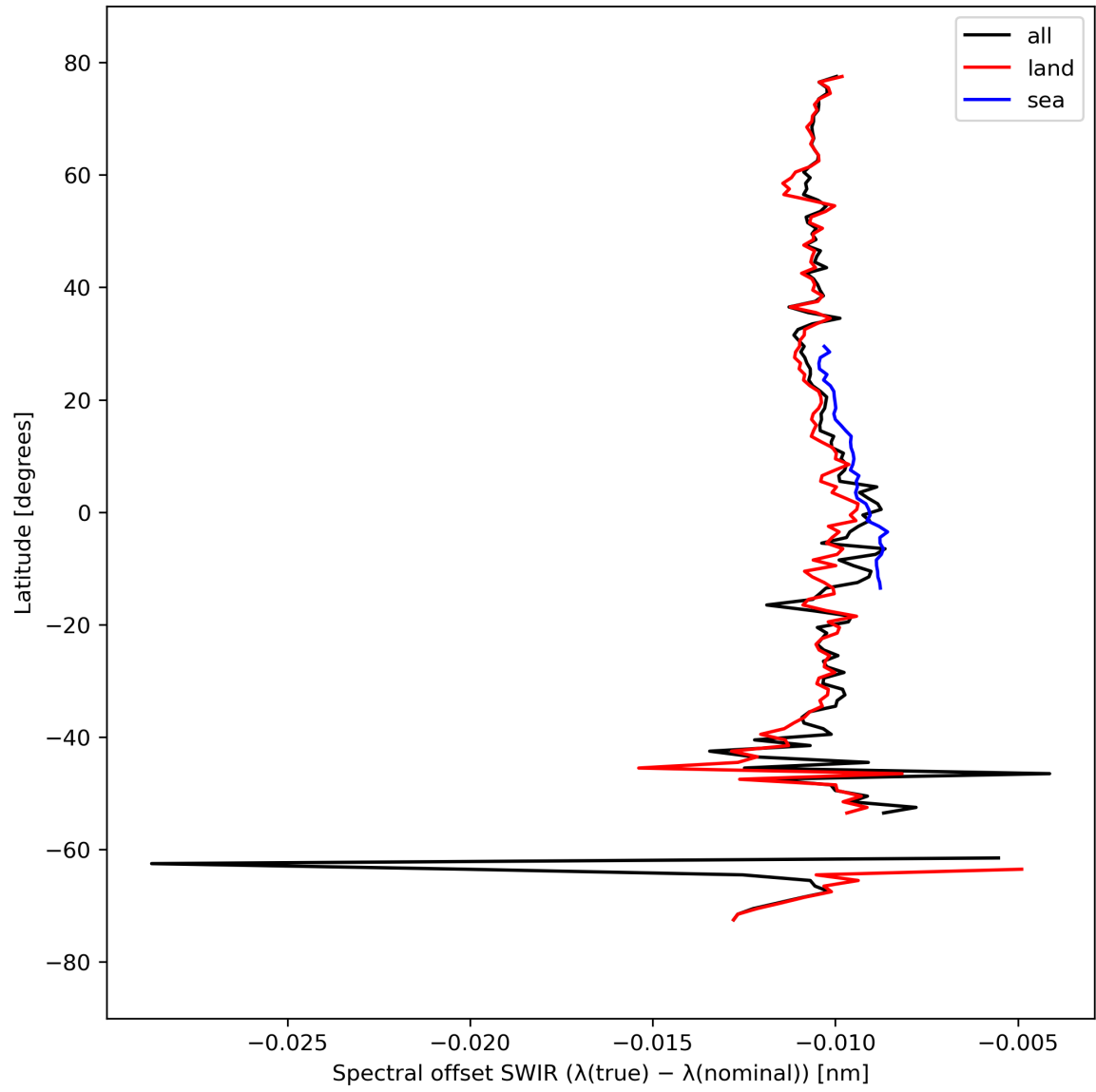
Figure 16: Zonal average of “Spectral offset SWIR ( \lambda(\text{true}) - \lambda(\text{nominal}) )” for 2024-03-25 to 2024-03-26.
