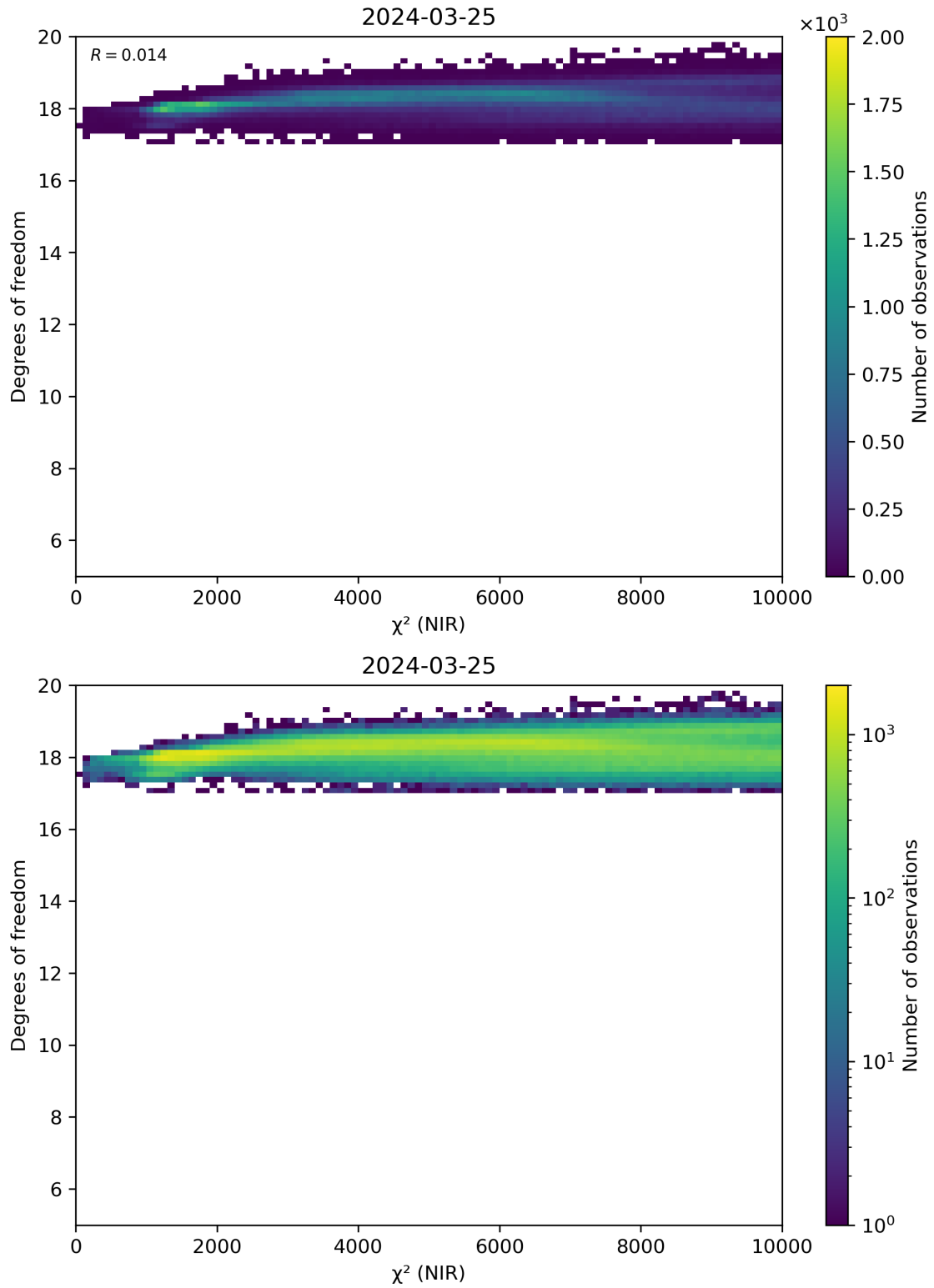
Figure 44: Scatter density plot of “ \chi^2 (NIR)” against “Degrees of freedom” for 2024-03-25 to 2024-03-26.
