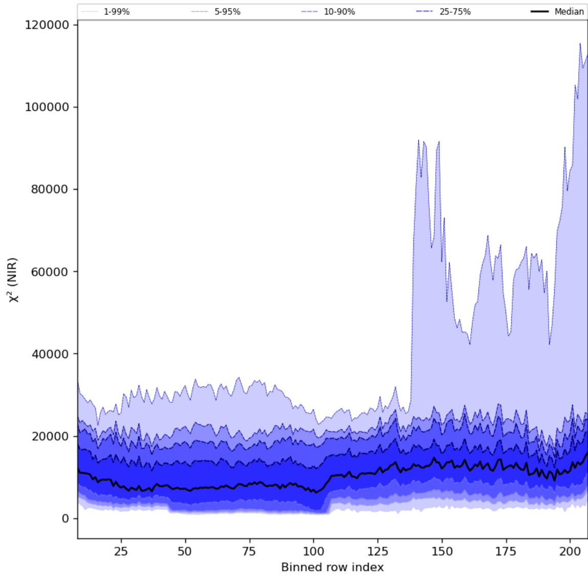
Figure 40: Along track statistics of “ \chi^2 (NIR)” for 2024-03-25 to 2024-03-26
