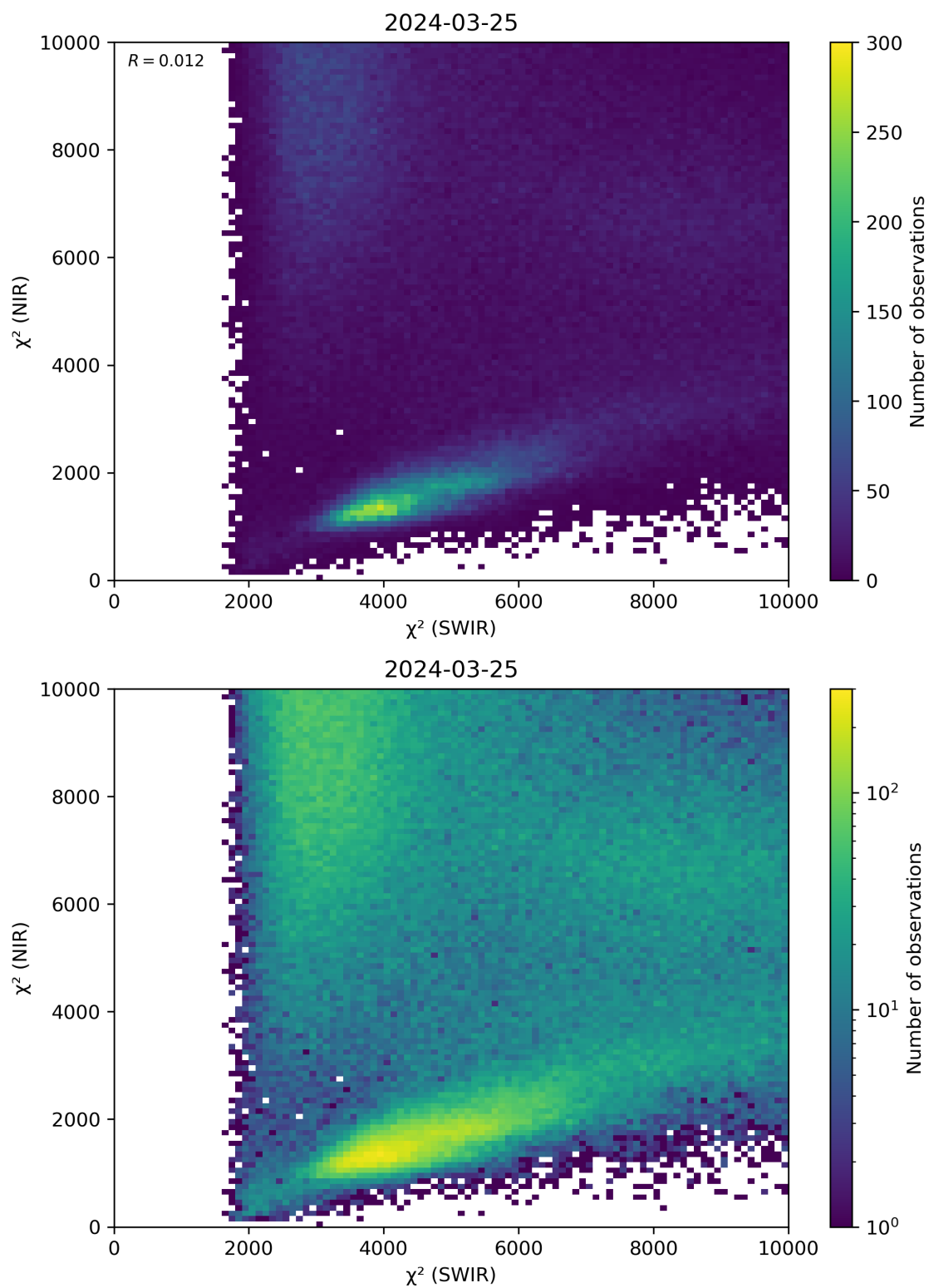
Figure 47: Scatter density plot of “ \chi^2 (SWIR)” against “ \chi^2 (NIR)” for 2024-03-25 to 2024-03-26.
