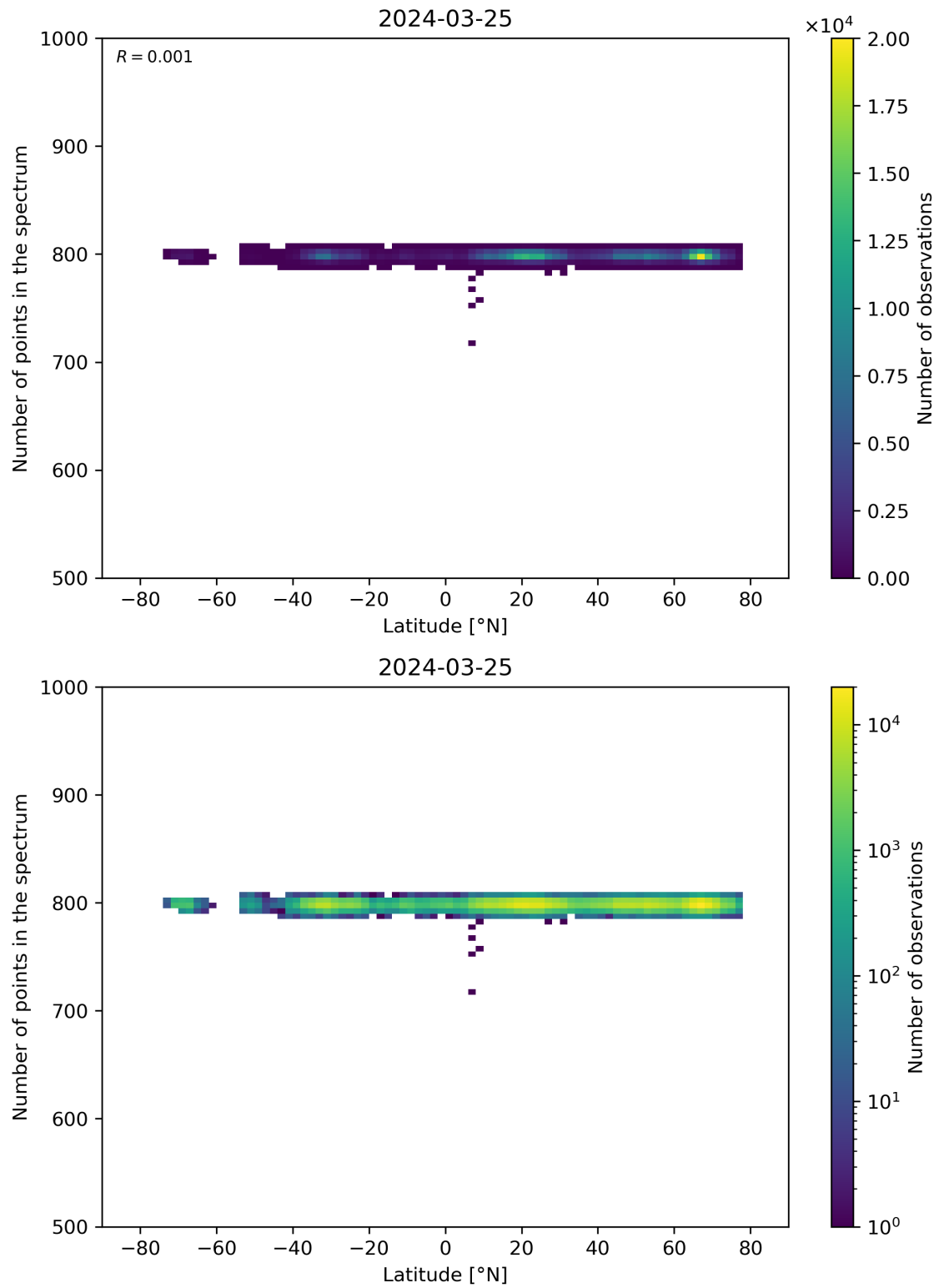
Figure 61: Scatter density plot of “Latitude” against “Number of points in the spectrum” for 2024-03-25 to 2024-03-26.
