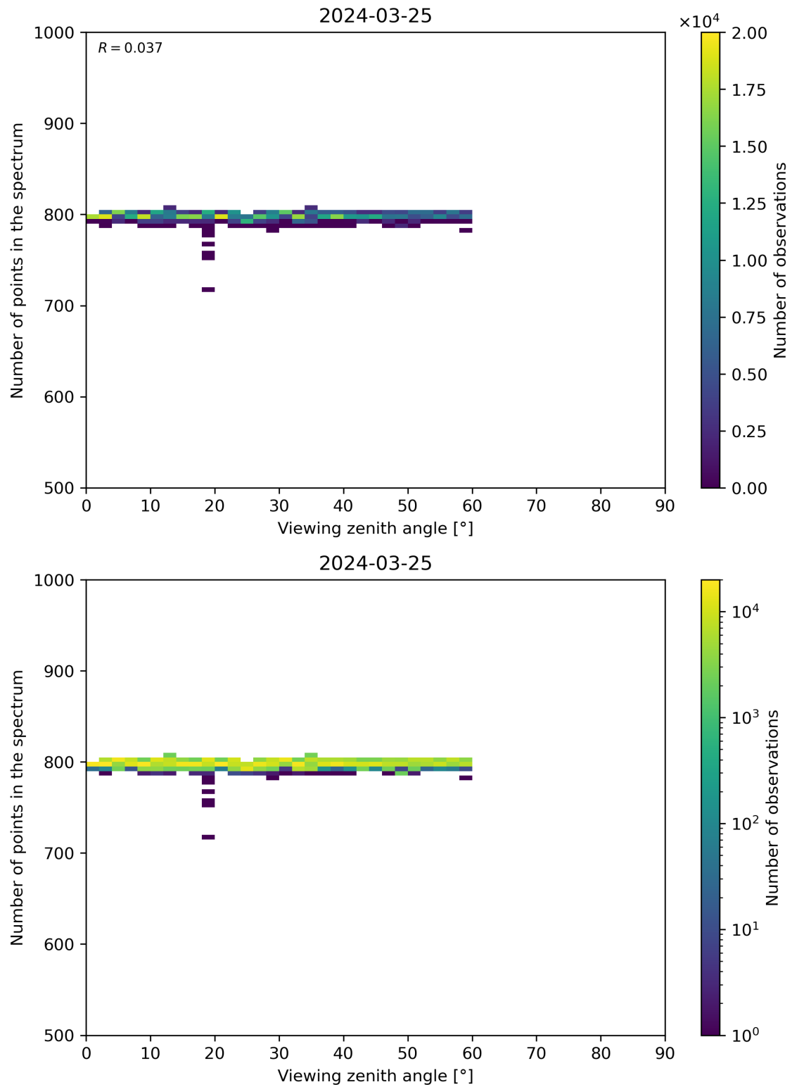
Figure 114: Scatter density plot of “Viewing zenith angle” against “Number of points in the spectrum” for 2024-03-25 to 2024-03-26.
