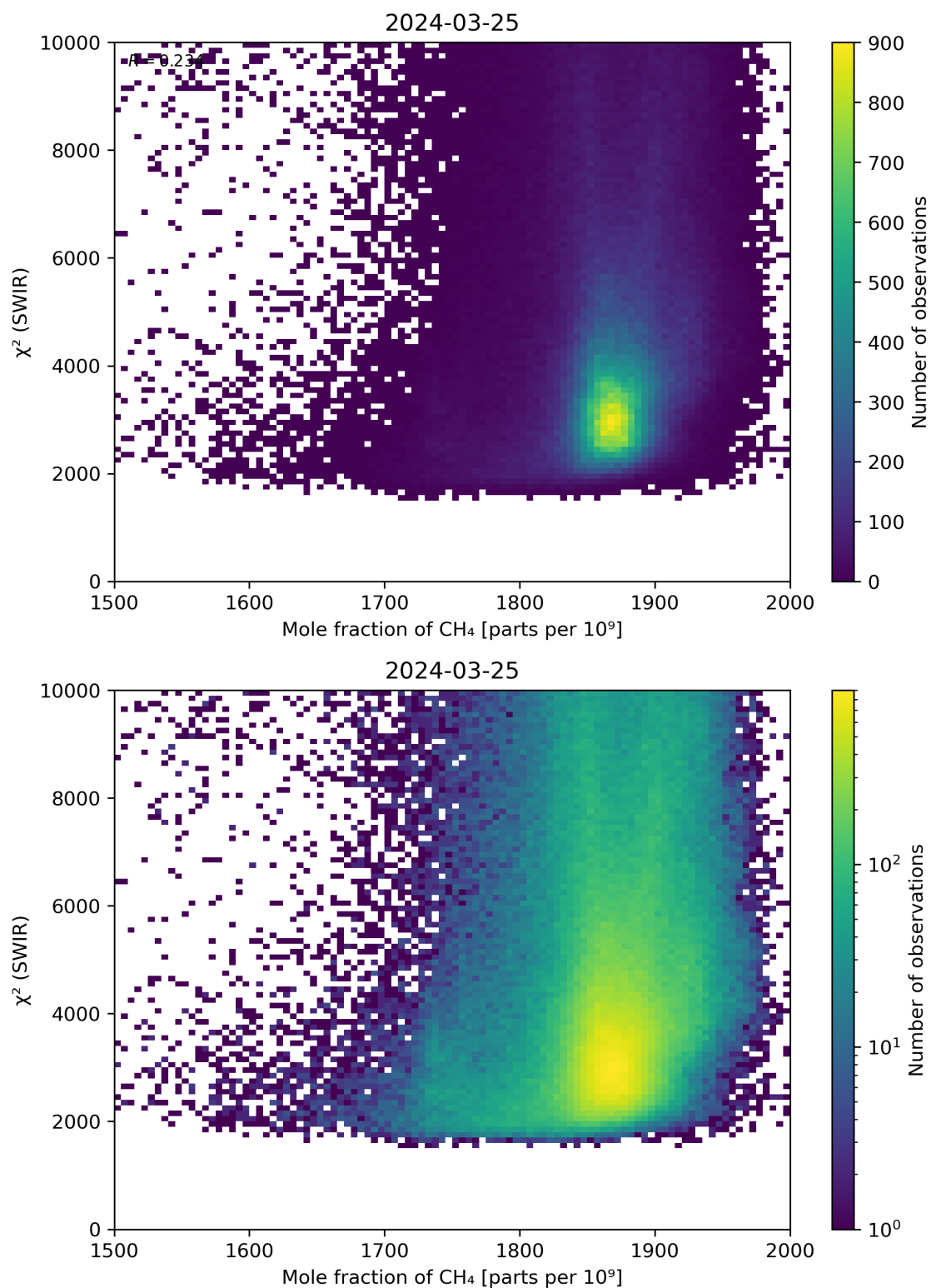
Figure 71: Scatter density plot of “Mole fraction of \text{CH}_4 ” against “ \chi^2 (SWIR)” for 2024-03-25 to 2024-03-26.
