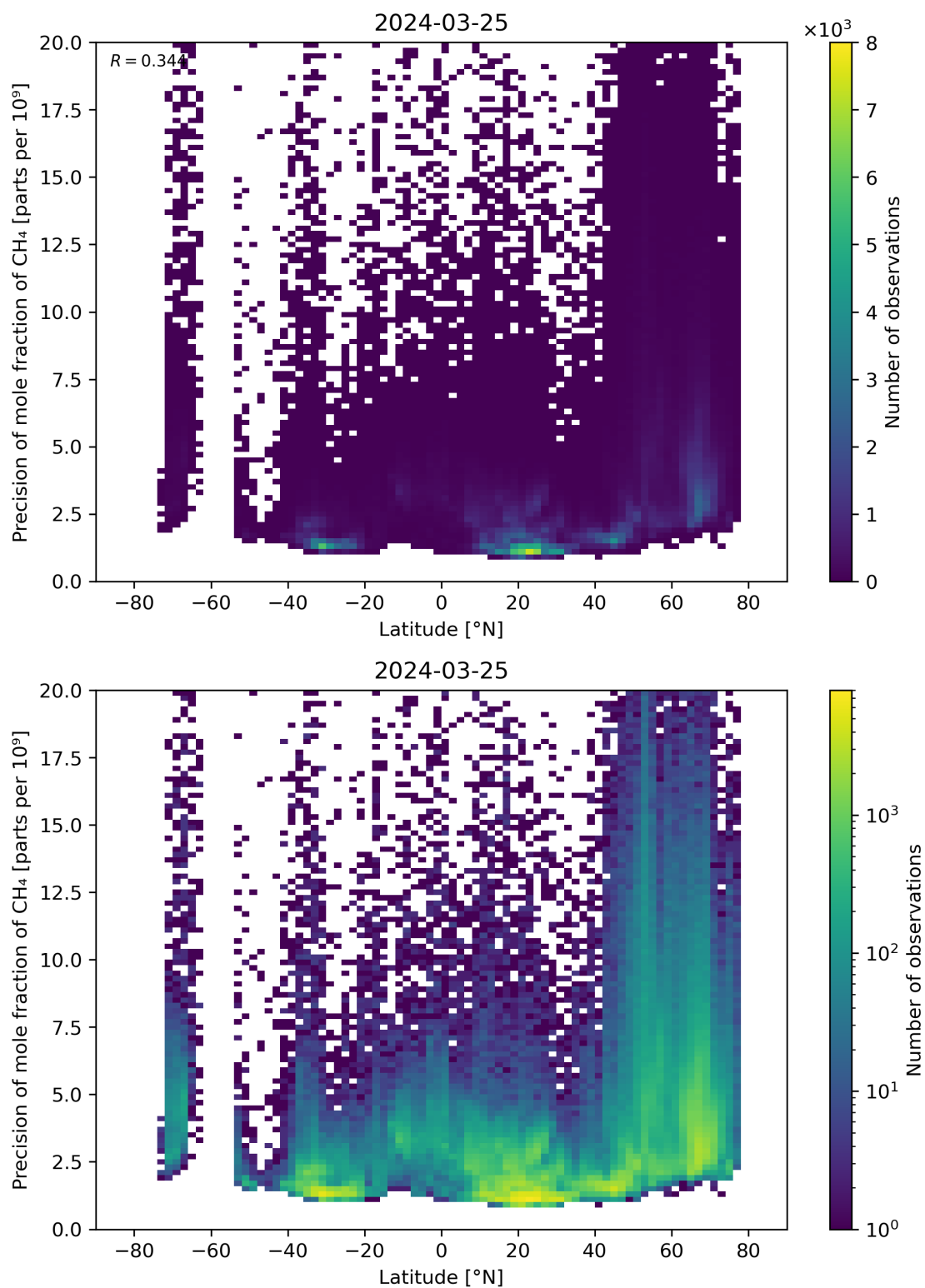
Figure 59: Scatter density plot of “Latitude” against “Precision of mole fraction of CH 4 ” for 2024-03-25 to 2024-03-26.
