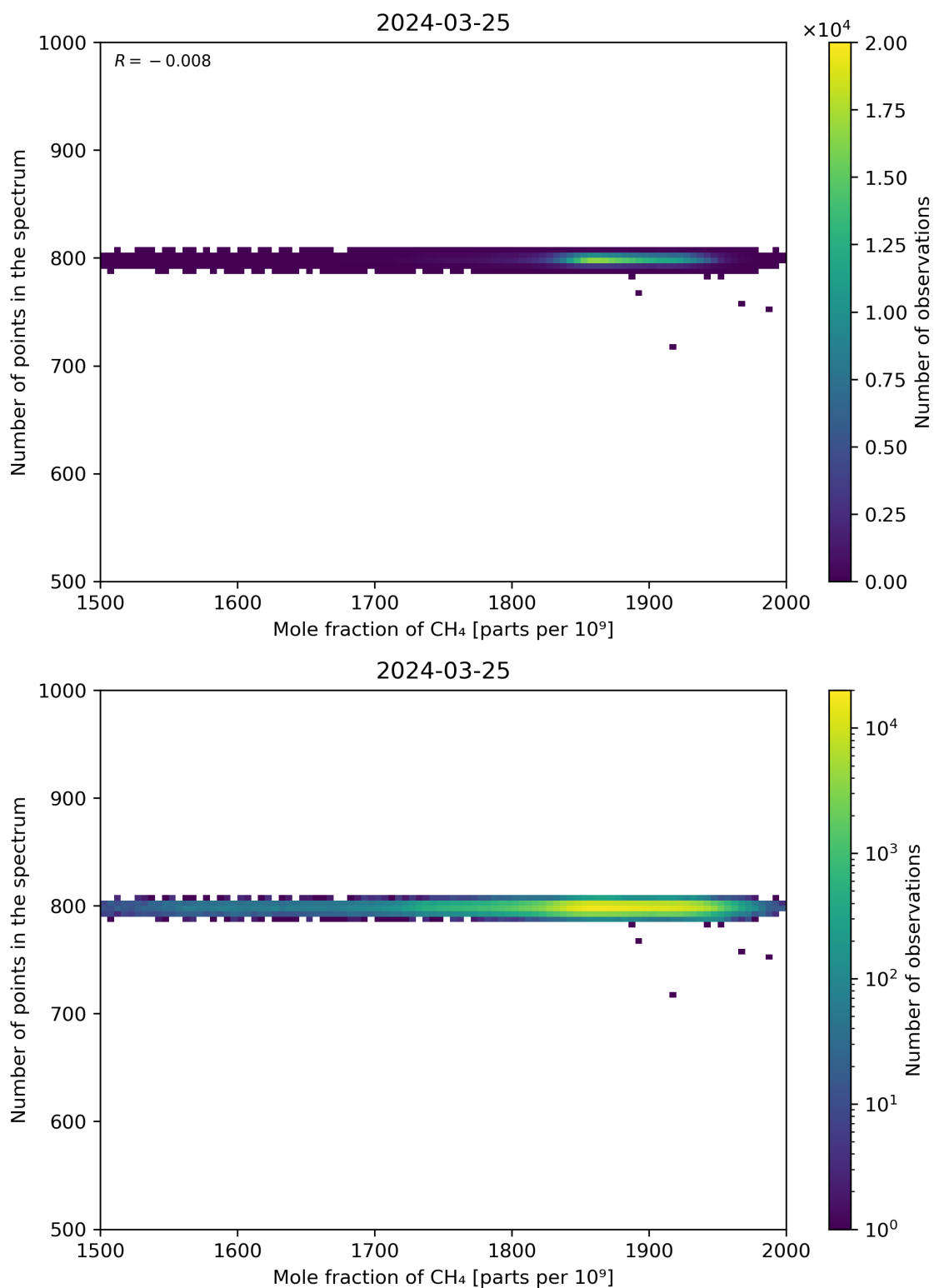
Figure 77: Scatter density plot of “Mole fraction of CH 4 ” against “Number of points in the spectrum” for 2024-03-25 to 2024-03-26.
