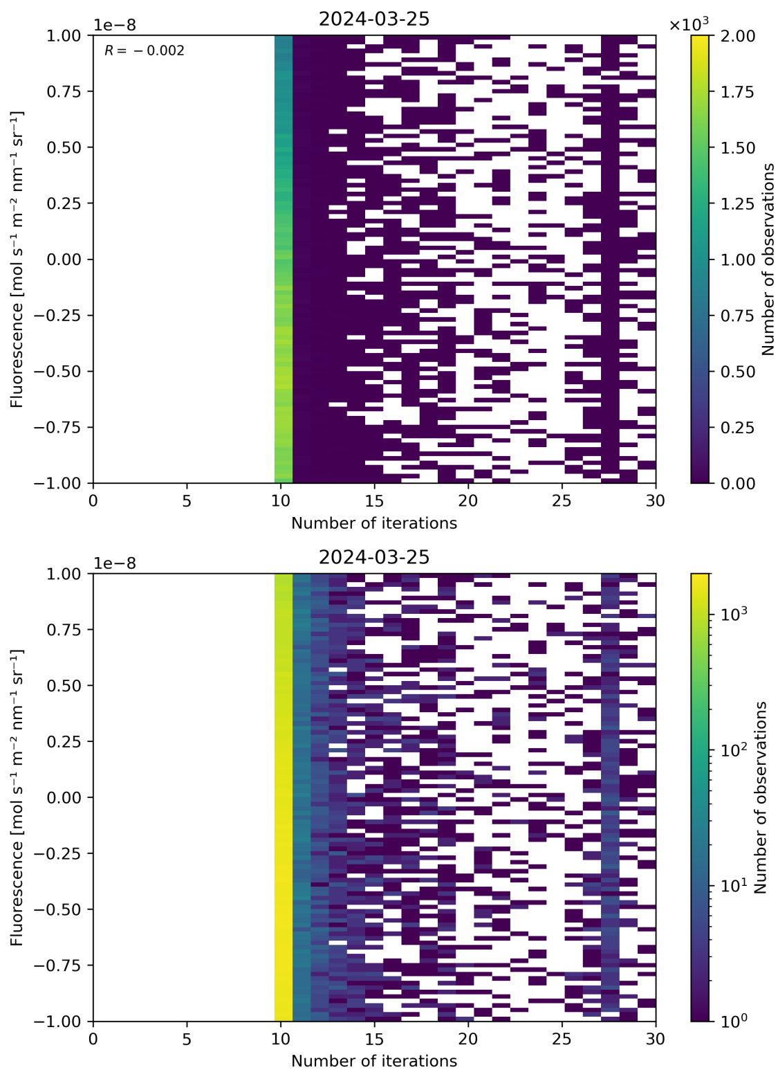
Figure 87: Scatter density plot of “Number of iterations” against “Fluorescence” for 2024-03-25 to 2024-03-26.
