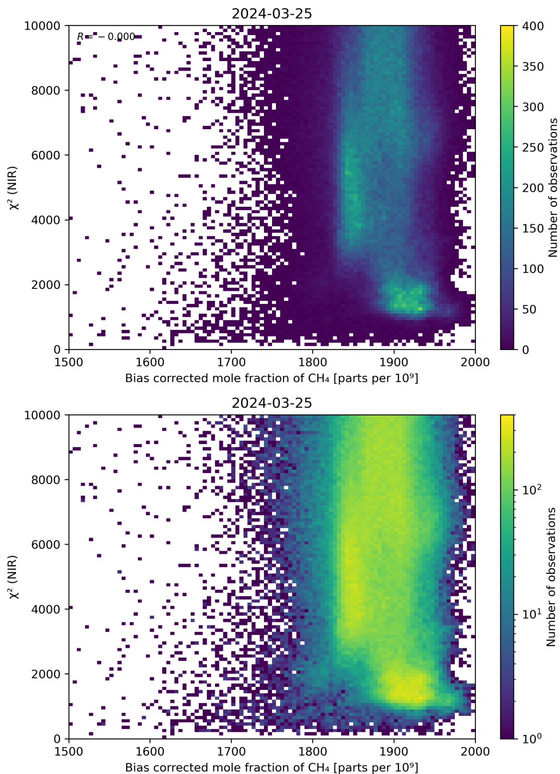
Figure 63: Scatter density plot of “Bias corrected mole fraction of \text{CH}_4 ” against “ \chi^2 (NIR)” for 2024-03-25 to 2024-03-26.
