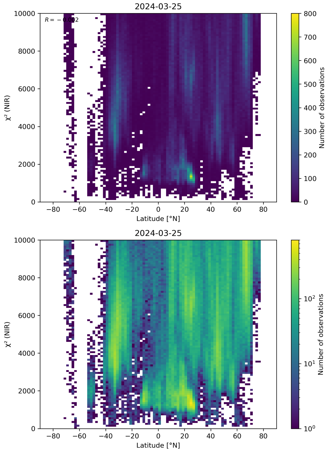
Figure 53: Scatter density plot of “Latitude” against “ \chi^2 (NIR)” for 2024-03-25 to 2024-03-26.
