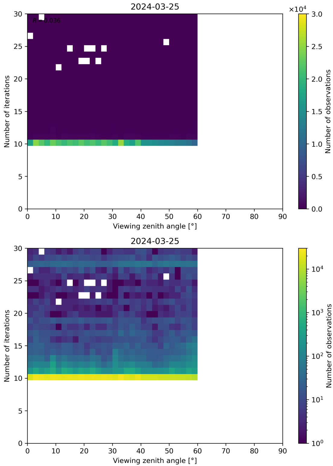
Figure 113: Scatter density plot of “Viewing zenith angle” against “Number of iterations” for 2024-03-25 to 2024-03-26.
