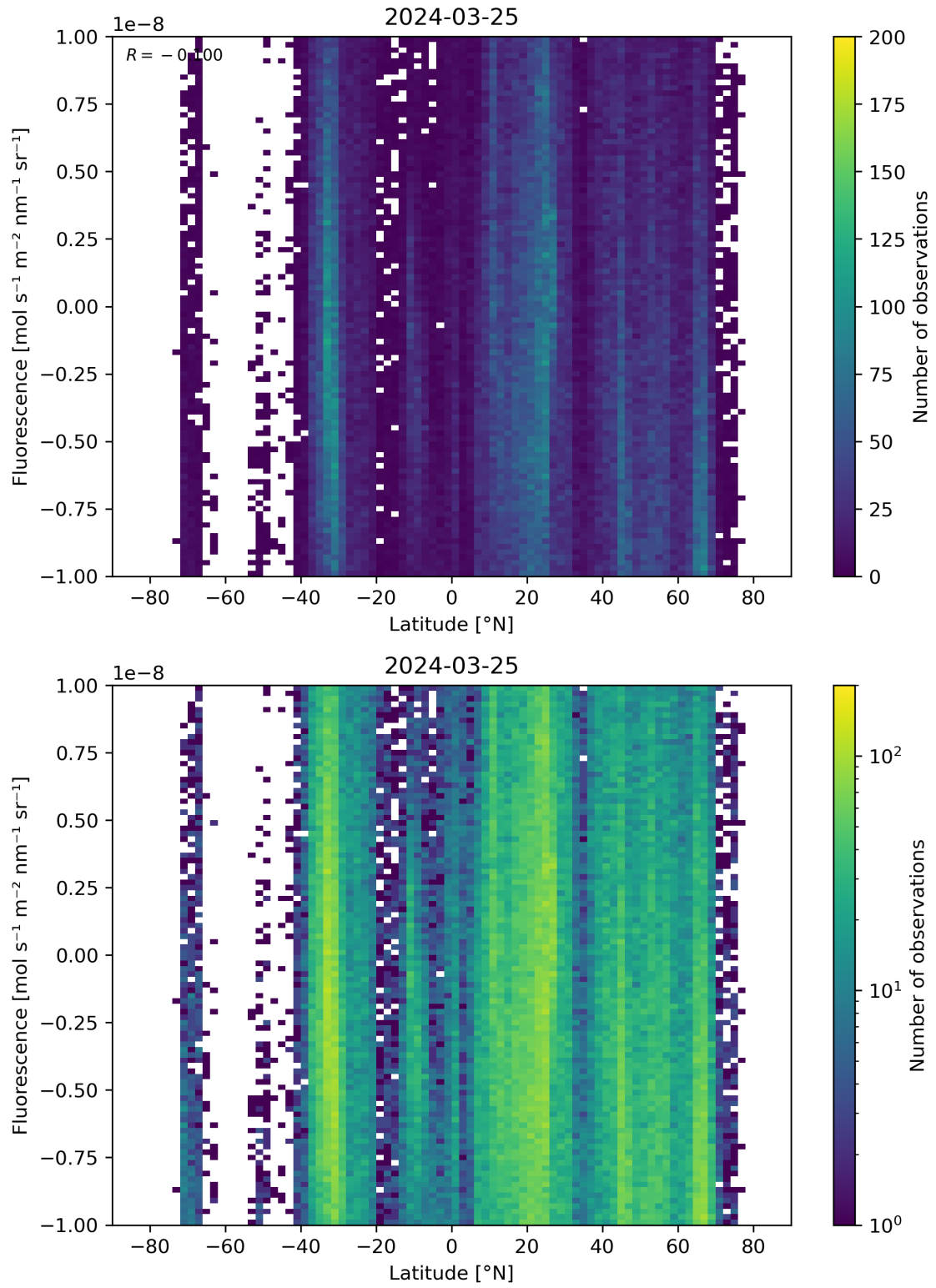
Figure 56: Scatter density plot of “Latitude” against “Fluorescence” for 2024-03-25 to 2024-03-26.
