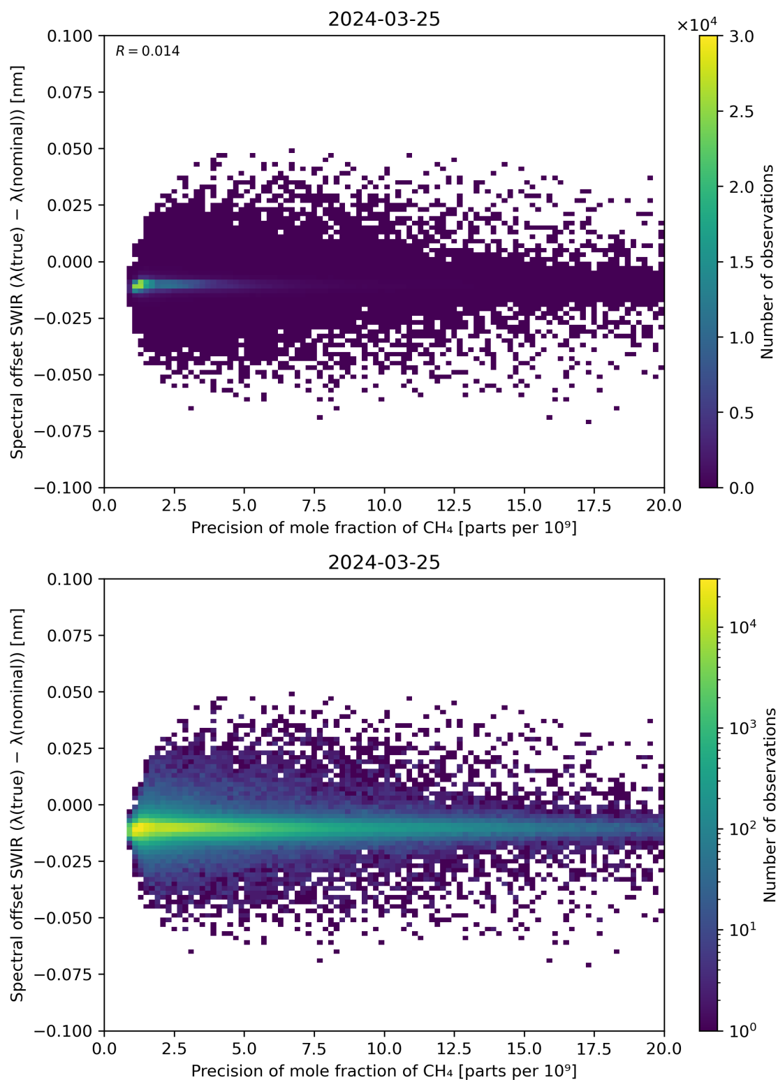
Figure 85: Scatter density plot of “Precision of mole fraction of CH 4 ” against “Spectral offset SWIR ( \lambda(\text{true}) - \lambda(\text{nominal}) )” for 2024-03-25 to 2024-03-26.
