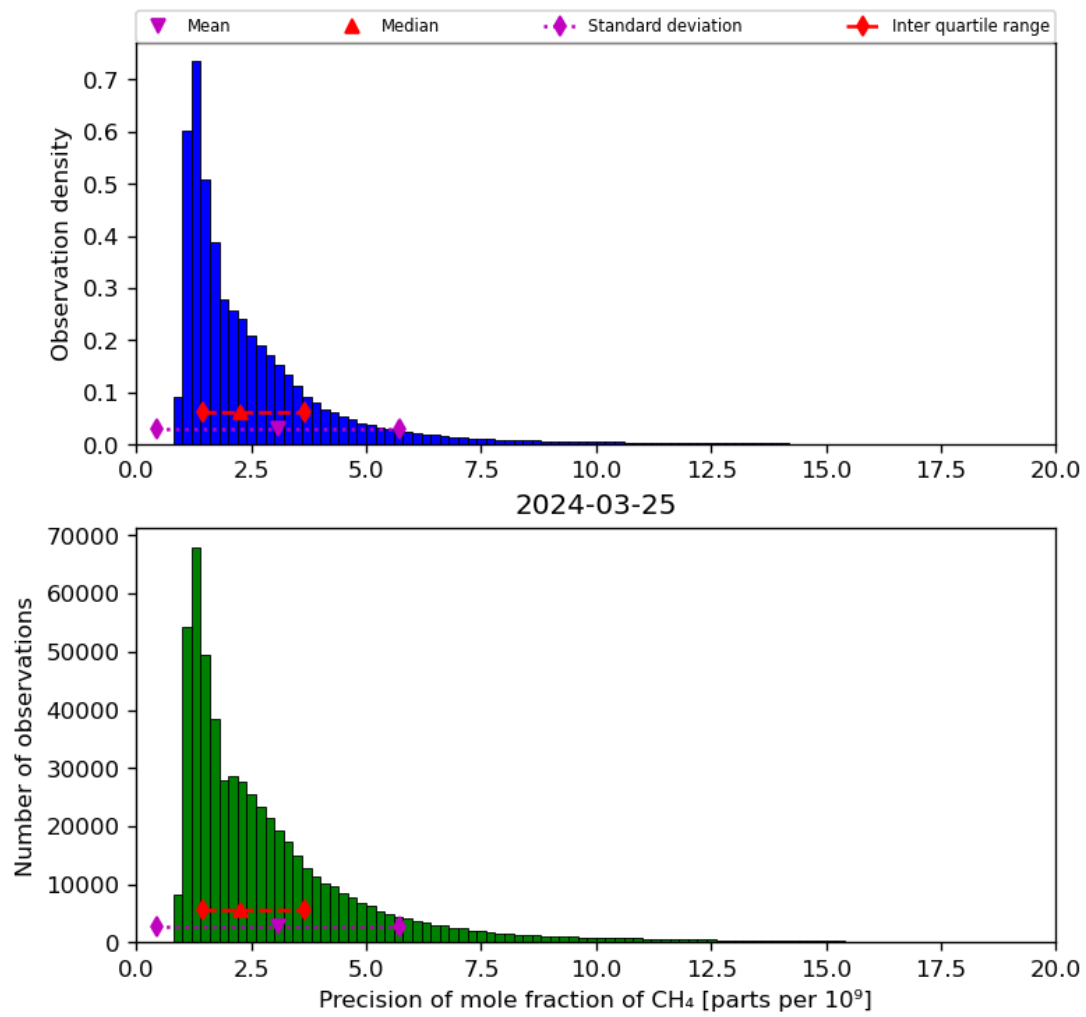
Figure 24: Histogram of “Precision of mole fraction of CH 4 ” for 2024-03-25 to 2024-03-26
