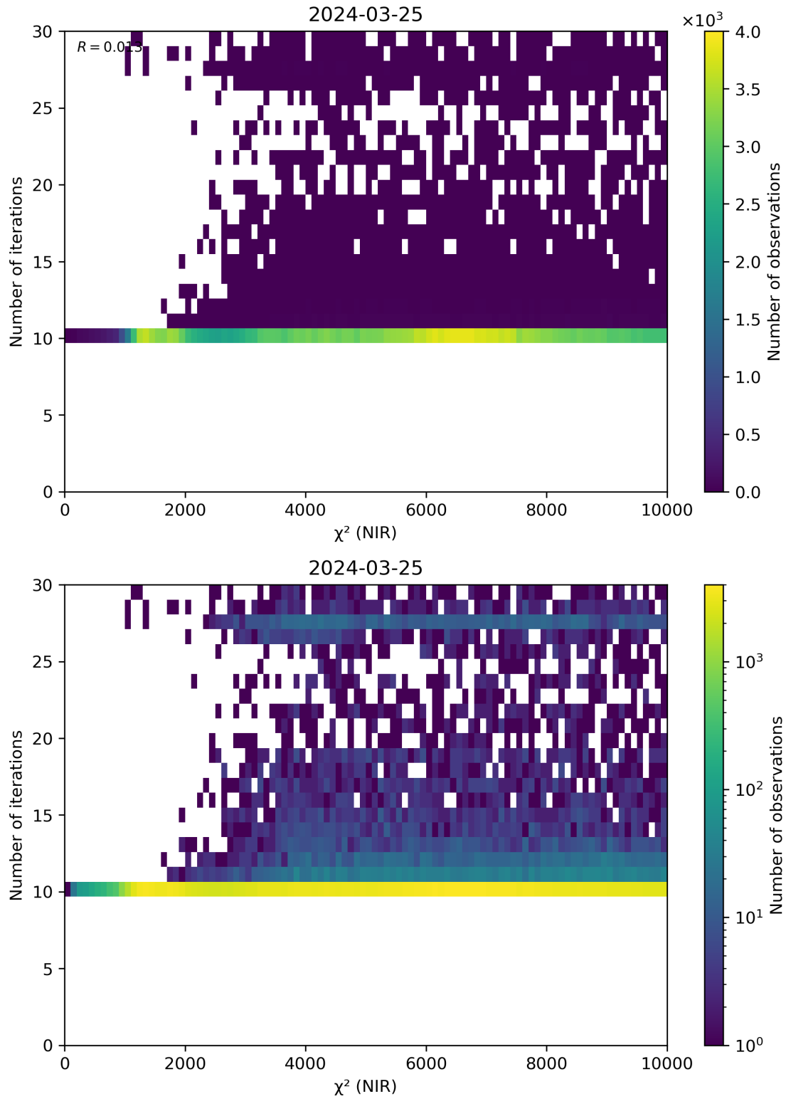
Figure 46: Scatter density plot of “ \chi^2 (NIR)” against “Number of iterations” for 2024-03-25 to 2024-03-26.
