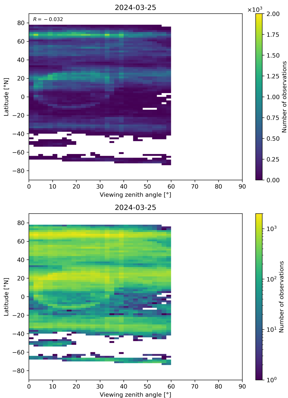
Figure 109: Scatter density plot of “Viewing zenith angle” against “Latitude” for 2024-03-25 to 2024-03-26.
