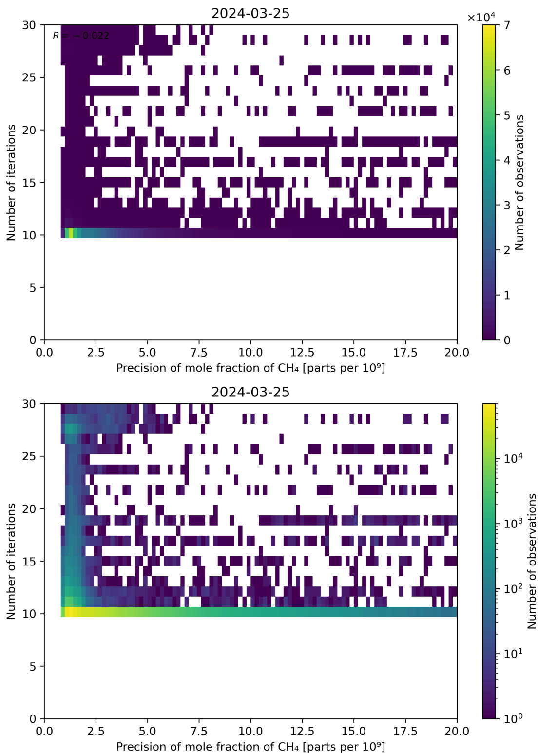
Figure 83: Scatter density plot of “Precision of mole fraction of CH 4 ” against “Number of iterations” for 2024-03-25 to 2024-03-26.
