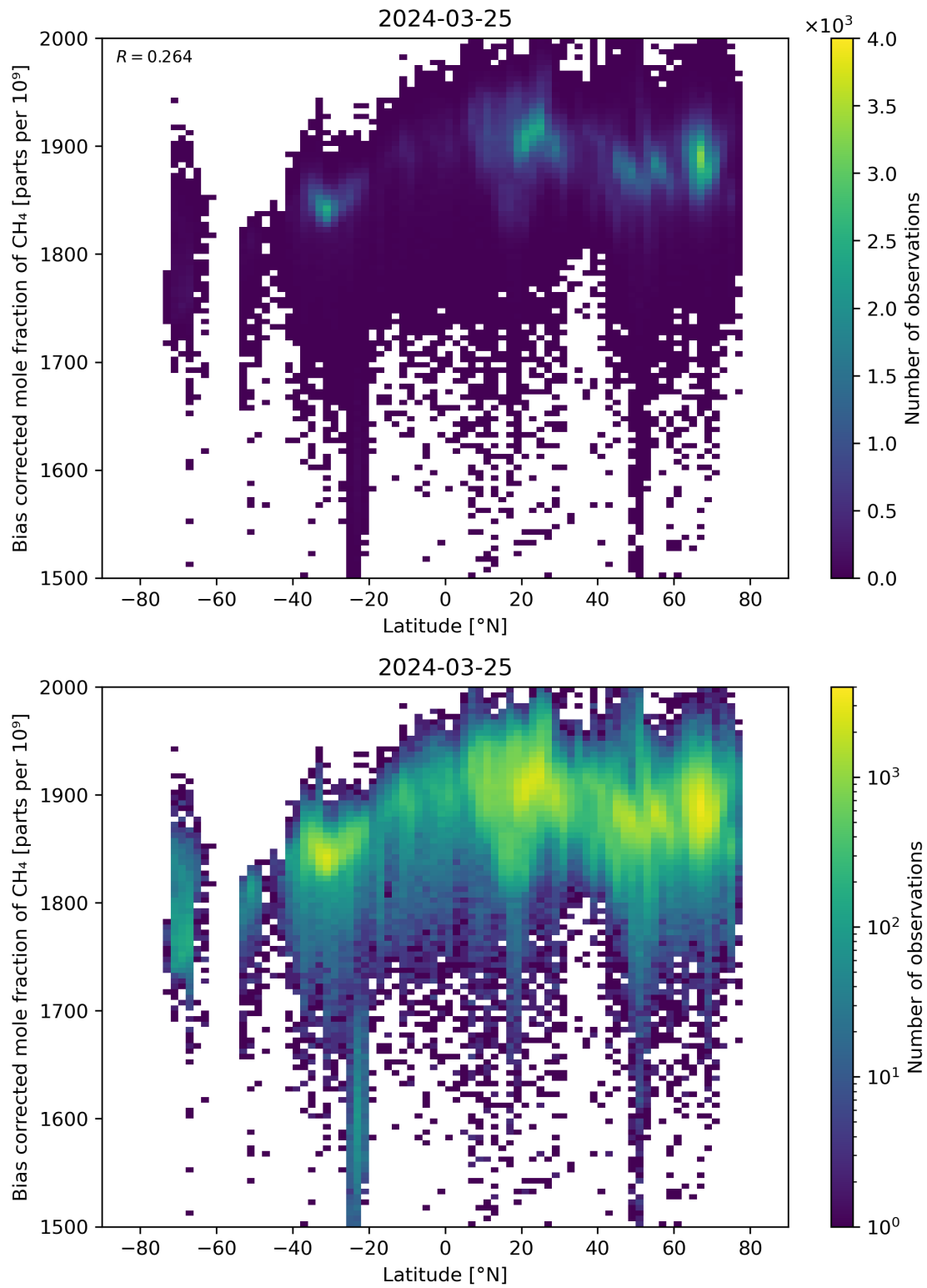
Figure 58: Scatter density plot of “Latitude” against “Bias corrected mole fraction of CH 4 ” for 2024-03-25 to 2024-03-26.
