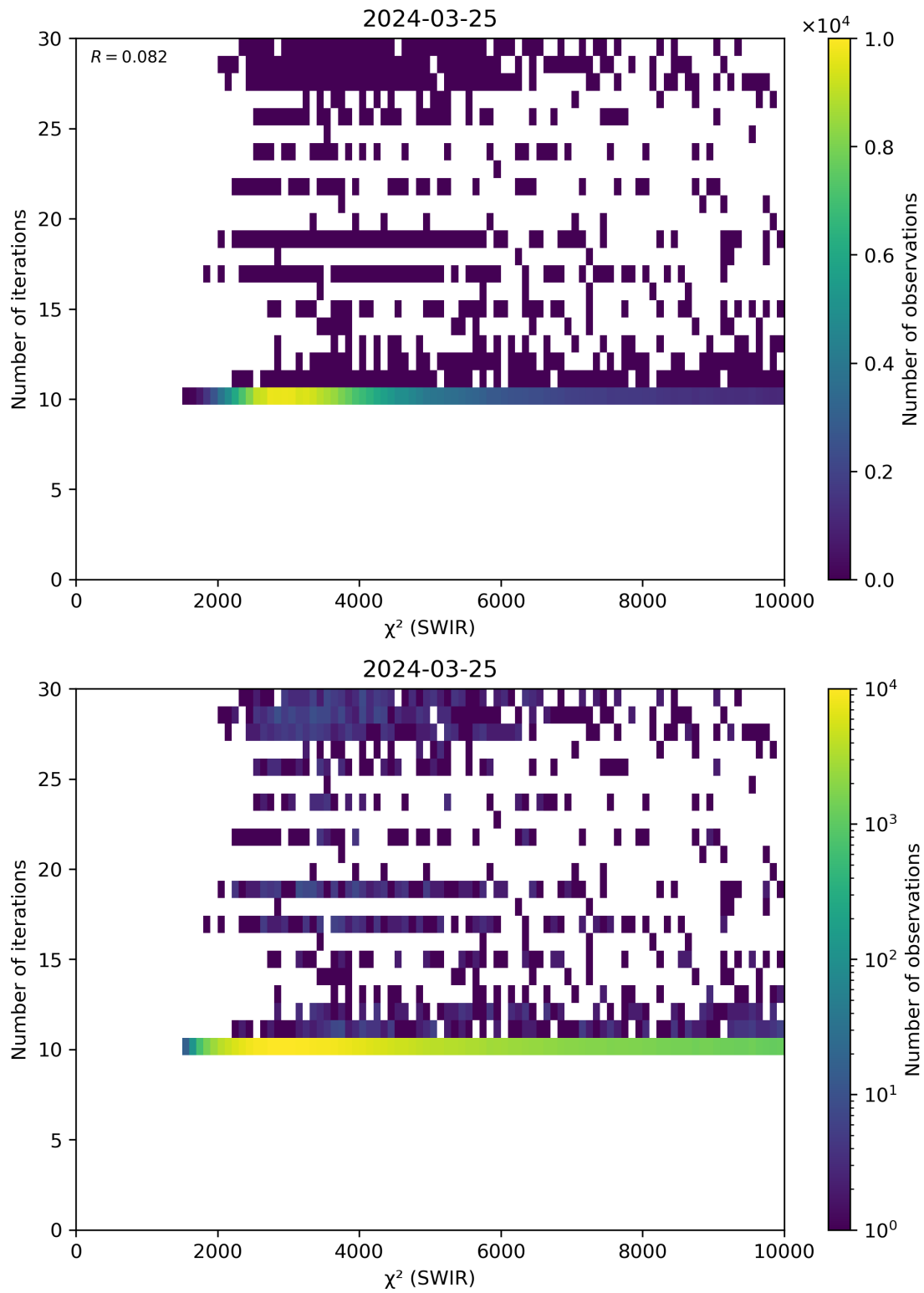
Figure 50: Scatter density plot of “ \chi^2 (SWIR)” against “Number of iterations” for 2024-03-25 to 2024-03-26.
