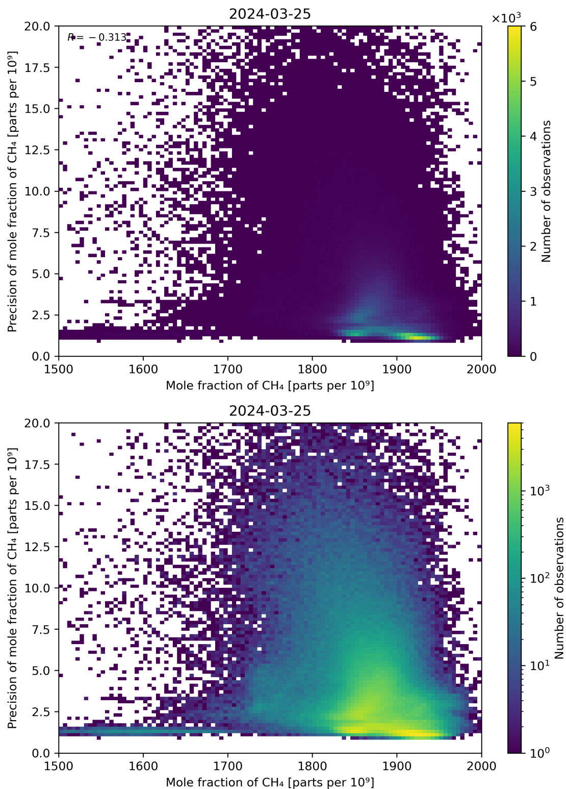
Figure 75: Scatter density plot of “Mole fraction of CH 4 ” against “Precision of mole fraction of CH 4 ” for 2024-03-25 to 2024-03-26.
