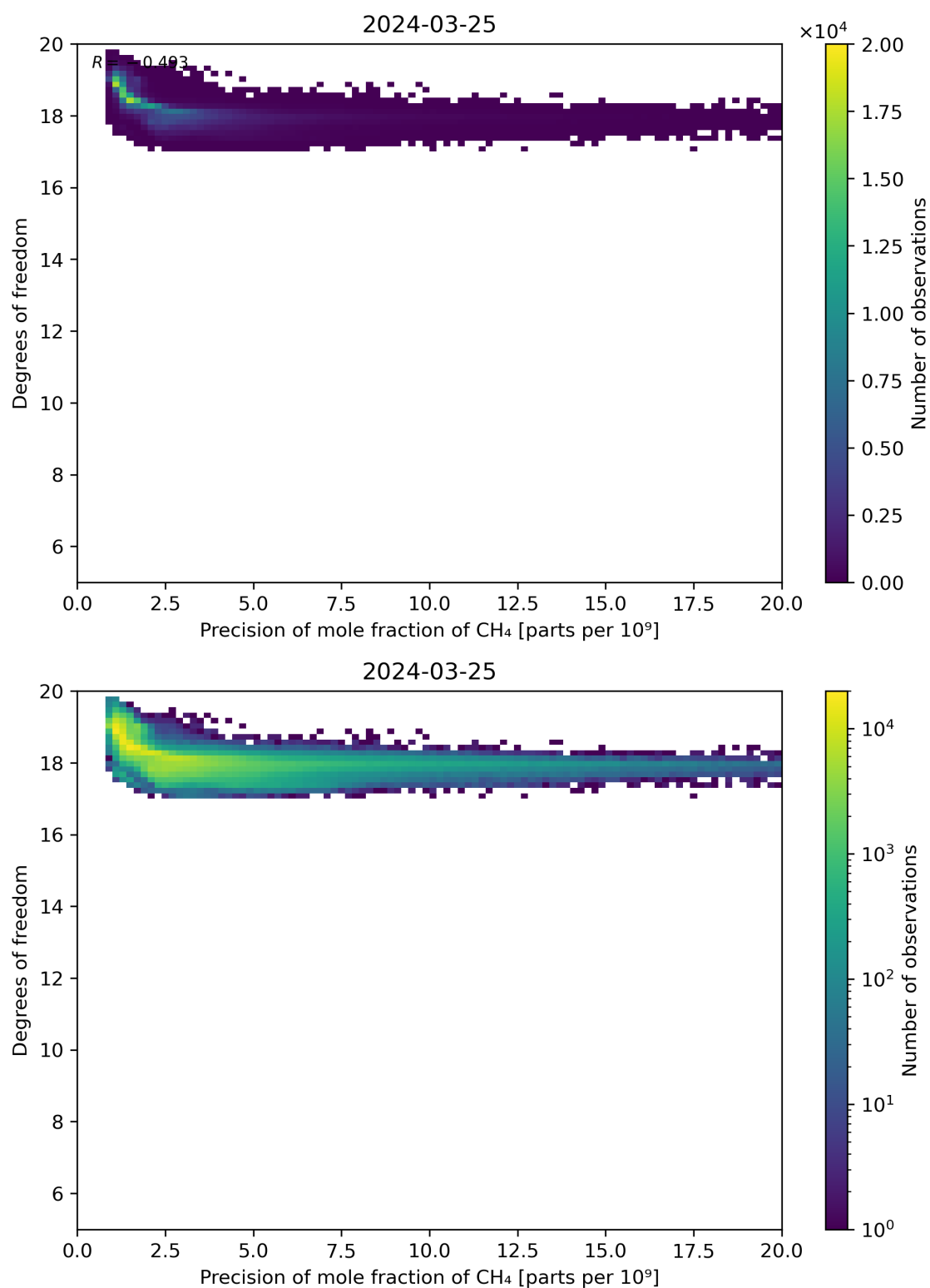
Figure 80: Scatter density plot of “Precision of mole fraction of CH 4 ” against “Degrees of freedom” for 2024-03-25 to 2024-03-26.
