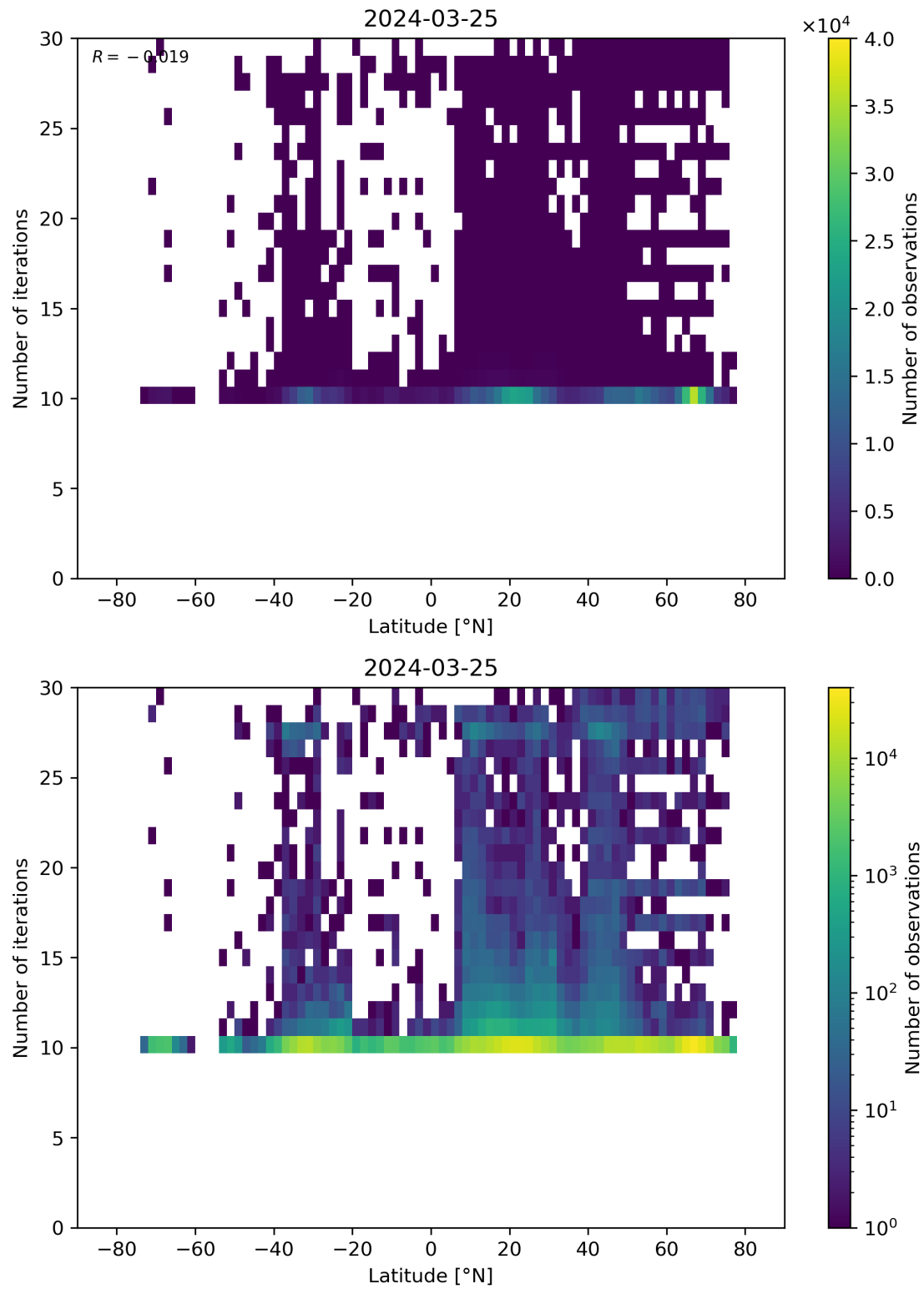
Figure 60: Scatter density plot of “Latitude” against “Number of iterations” for 2024-03-25 to 2024-03-26.
