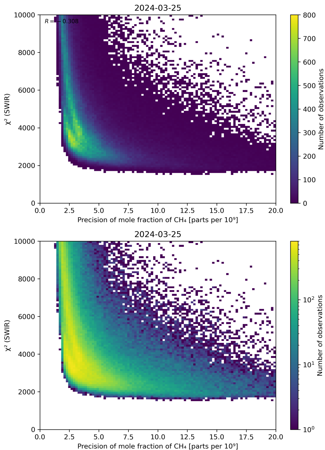
Figure 79: Scatter density plot of “Precision of mole fraction of \text{CH}_4 ” against “ \chi^2 (SWIR)” for 2024-03-25 to 2024-03-26.
