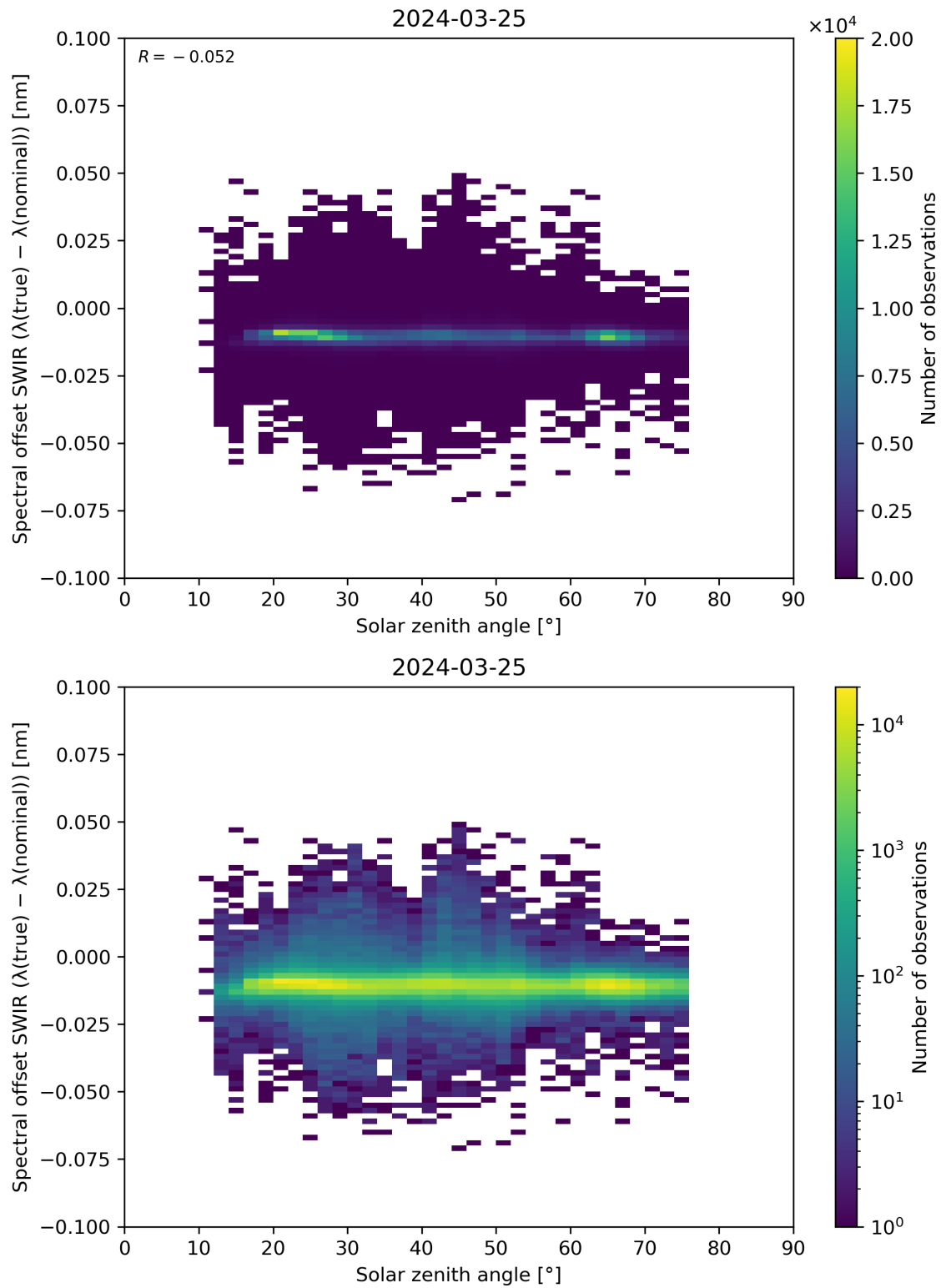
Figure 104: Scatter density plot of “Solar zenith angle” against “Spectral offset SWIR ( \lambda(\text{true}) - \lambda(\text{nominal}) )” for 2024-03-25 to 2024-03-26.
