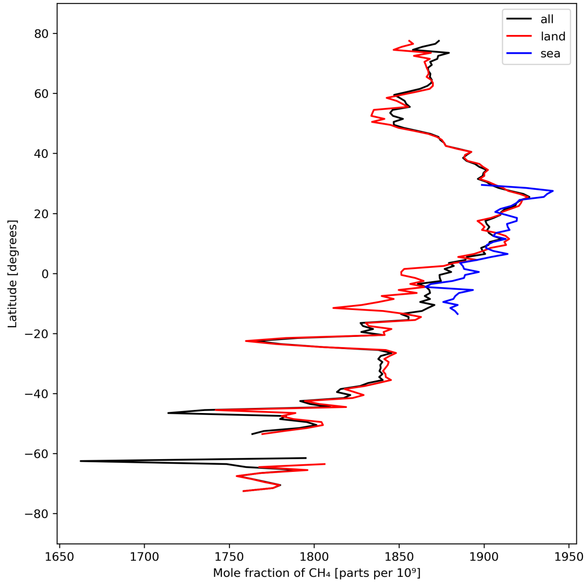
Figure 12: Zonal average of “Mole fraction of CH 4 ” for 2024-03-25 to 2024-03-26.
