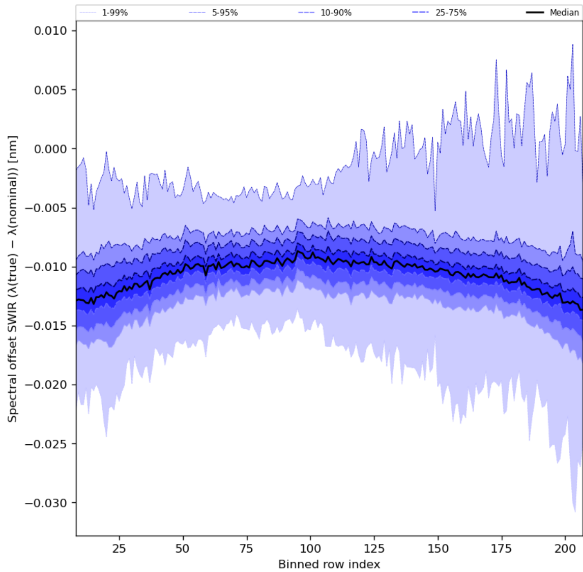
Figure 38: Along track statistics of “Spectral offset SWIR ( \lambda(\text{true}) - \lambda(\text{nominal}) )” for 2024-03-25 to 2024-03-26
