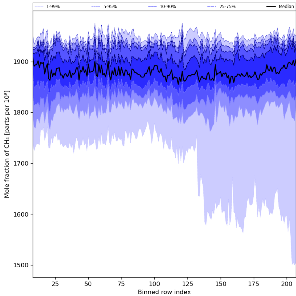
Figure 34: Along track statistics of “Mole fraction of CH 4 ” for 2024-03-25 to 2024-03-26
