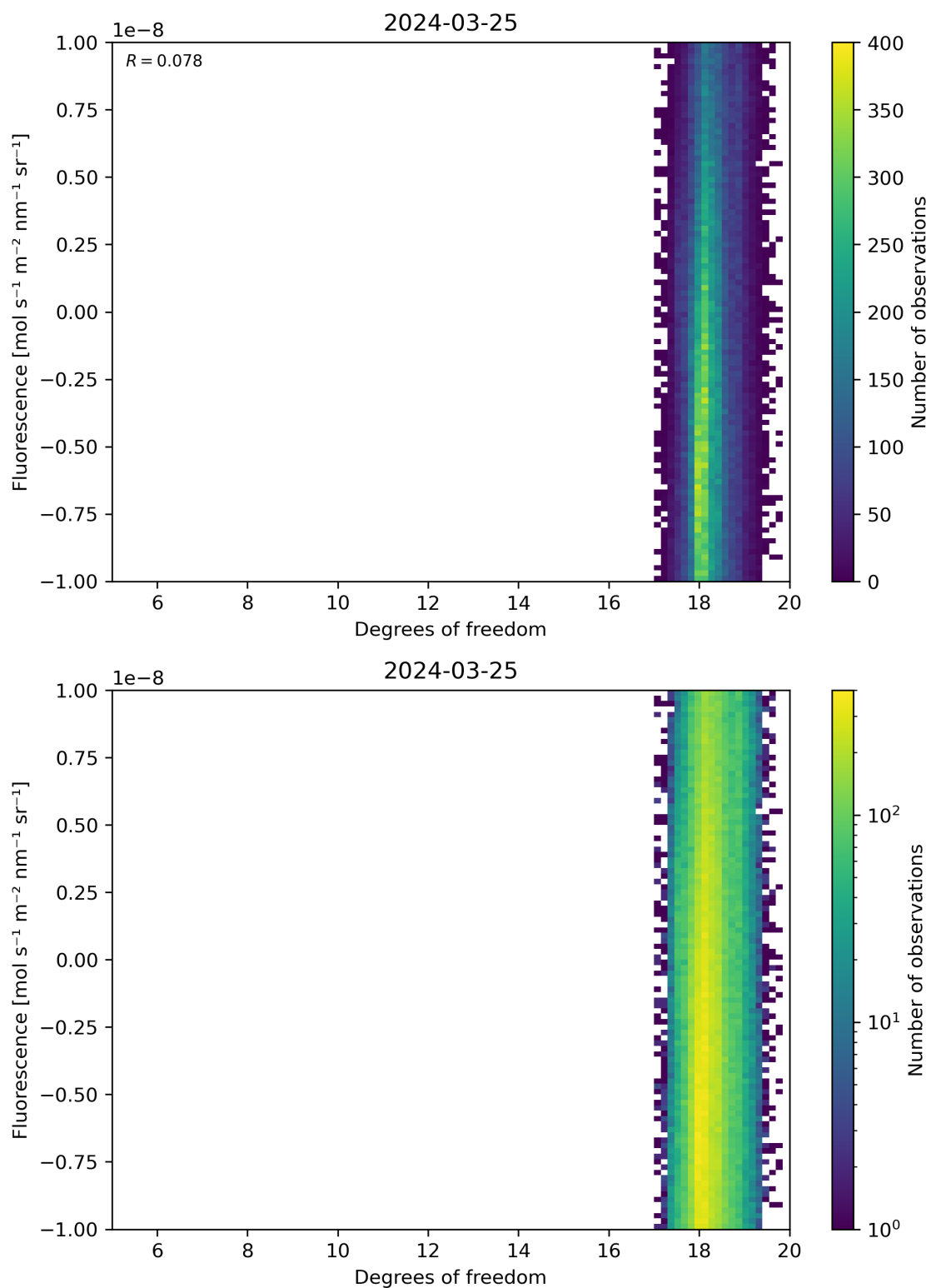
Figure 51: Scatter density plot of “Degrees of freedom” against “Fluorescence” for 2024-03-25 to 2024-03-26.
