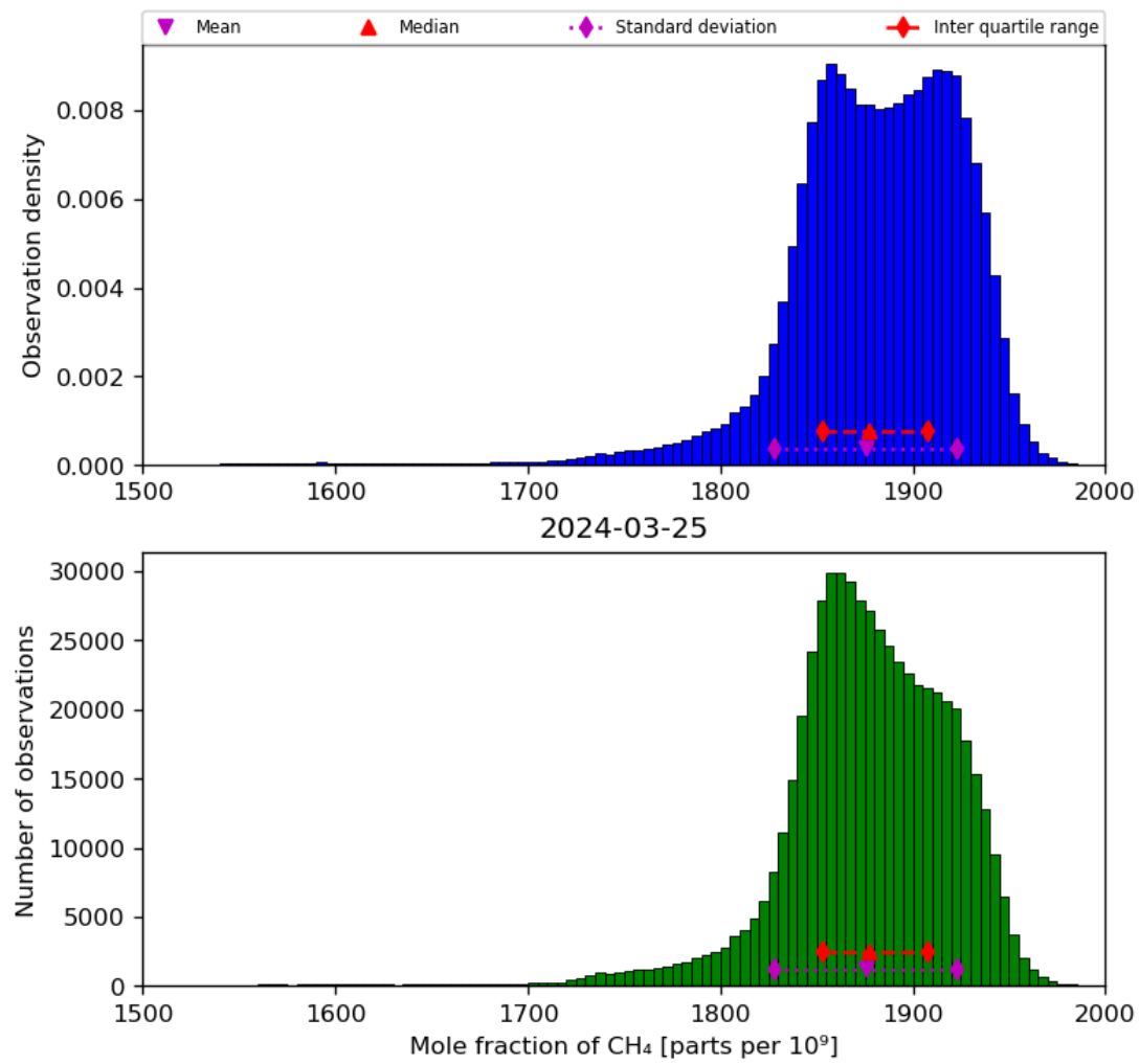
Figure 23: Histogram of “Mole fraction of CH 4 ” for 2024-03-25 to 2024-03-26
