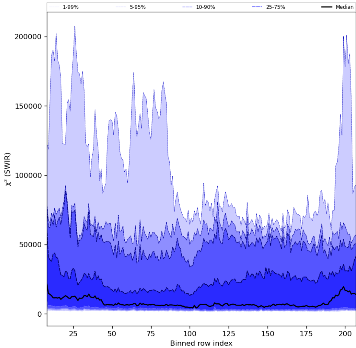
Figure 39: Along track statistics of “ \chi^2 (SWIR)” for 2024-03-25 to 2024-03-26
