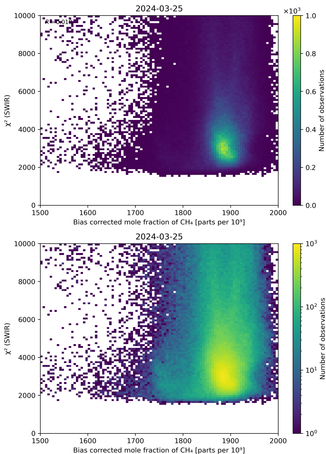
Figure 64: Scatter density plot of “Bias corrected mole fraction of CH 4 ” against “ \chi^2 (SWIR)” for 2024-03-25 to 2024-03-26.
