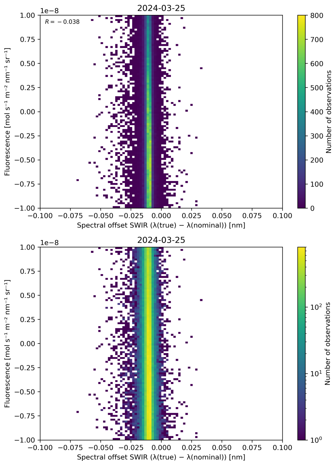
Figure 120: Scatter density plot of “Spectral offset SWIR ( \lambda(\text{true}) - \lambda(\text{nominal}) )” against “Fluorescence” for 2024-03-25 to 2024-03-26.
