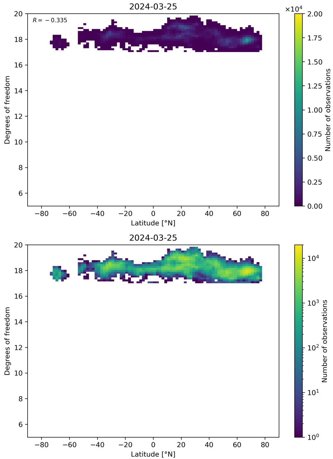
Figure 55: Scatter density plot of “Latitude” against “Degrees of freedom” for 2024-03-25 to 2024-03-26.
