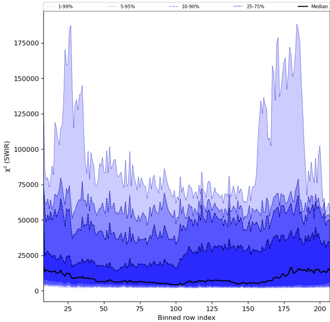
Figure 39: Along track statistics of " \chi^2 (SWIR)" for 2024-03-25 to 2024-03-27
