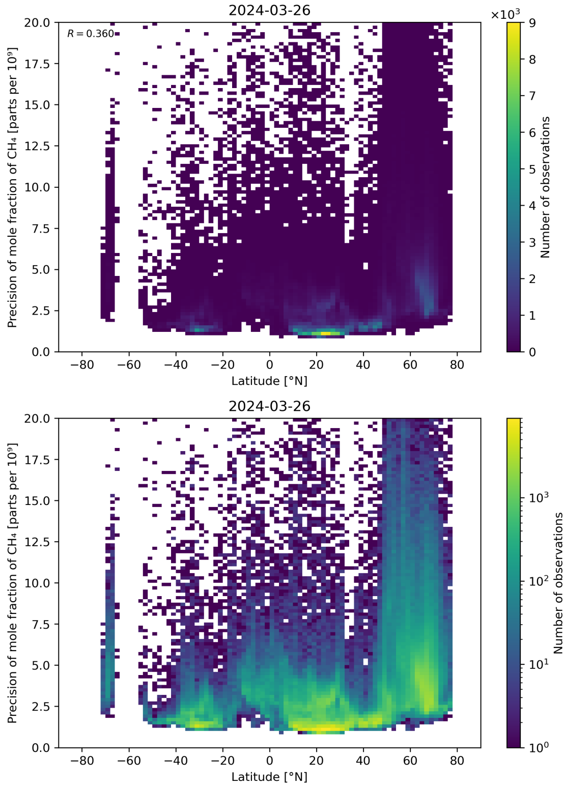
Figure 59: Scatter density plot of “Latitude” against “Precision of mole fraction of \text{CH}_4 ” for 2024-03-25 to 2024-03-27.
