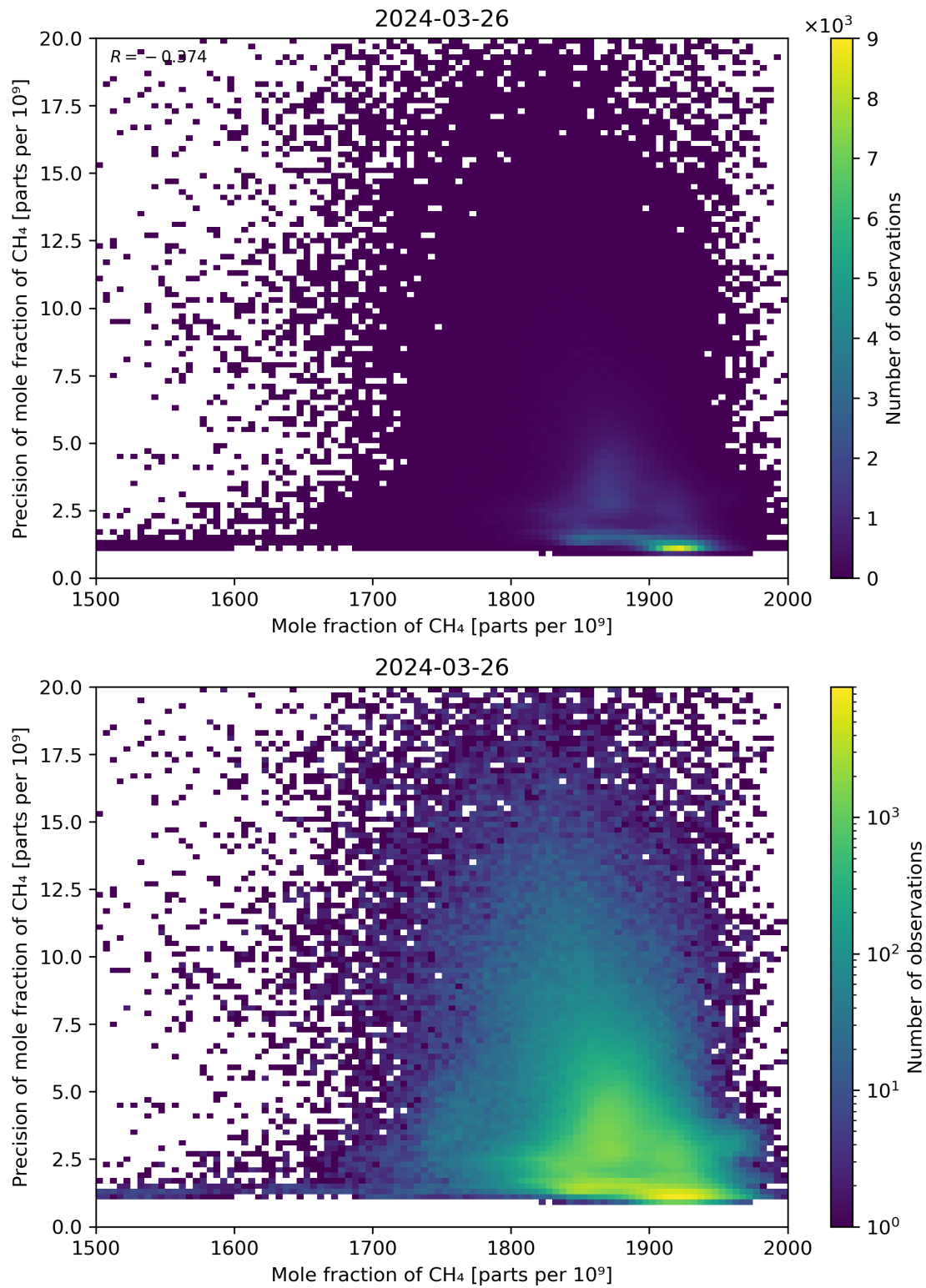
Figure 75: Scatter density plot of “Mole fraction of CH 4 ” against “Precision of mole fraction of CH 4 ” for 2024-03-25 to 2024-03-27.
