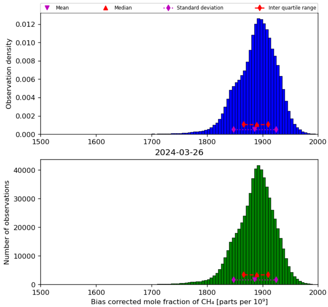
Figure 25: Histogram of “Bias corrected mole fraction of CH 4 ” for 2024-03-25 to 2024-03-27
