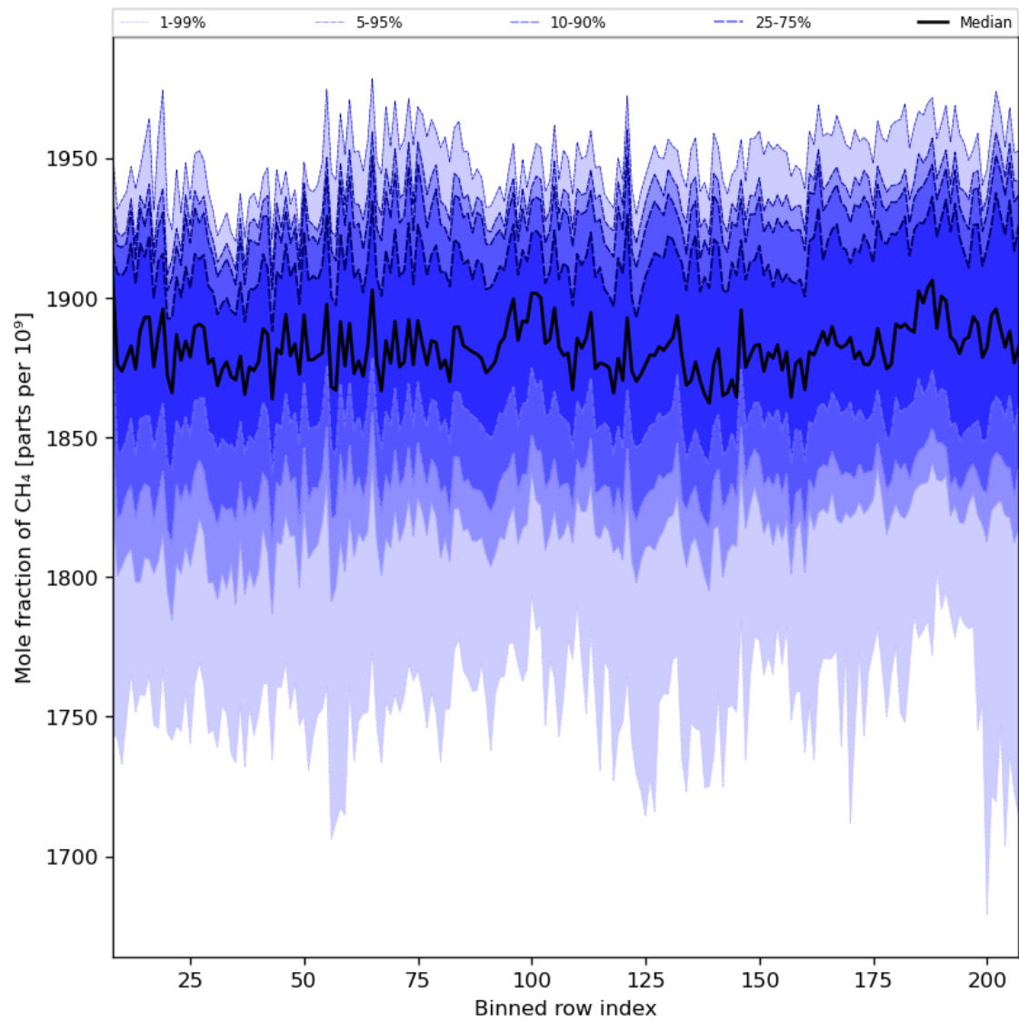
Figure 34: Along track statistics of “Mole fraction of CH 4 ” for 2024-03-25 to 2024-03-27
