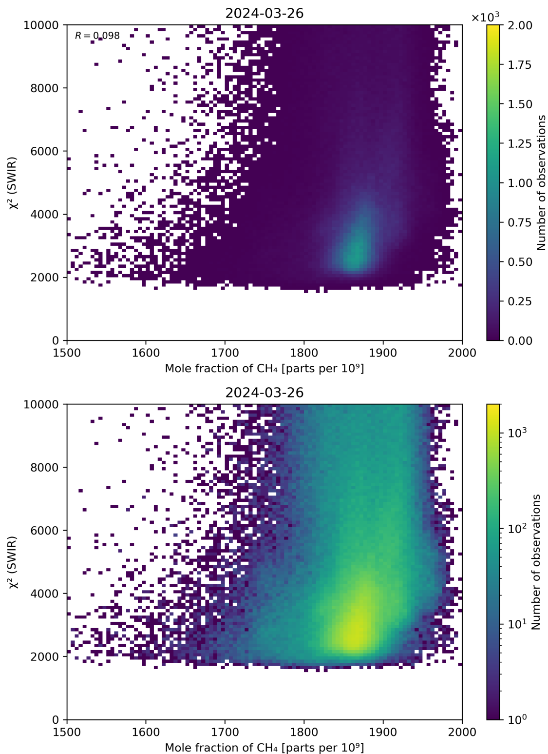
Figure 71: Scatter density plot of “Mole fraction of \text{CH}_4 ” against “ \chi^2 (SWIR)” for 2024-03-25 to 2024-03-27.
