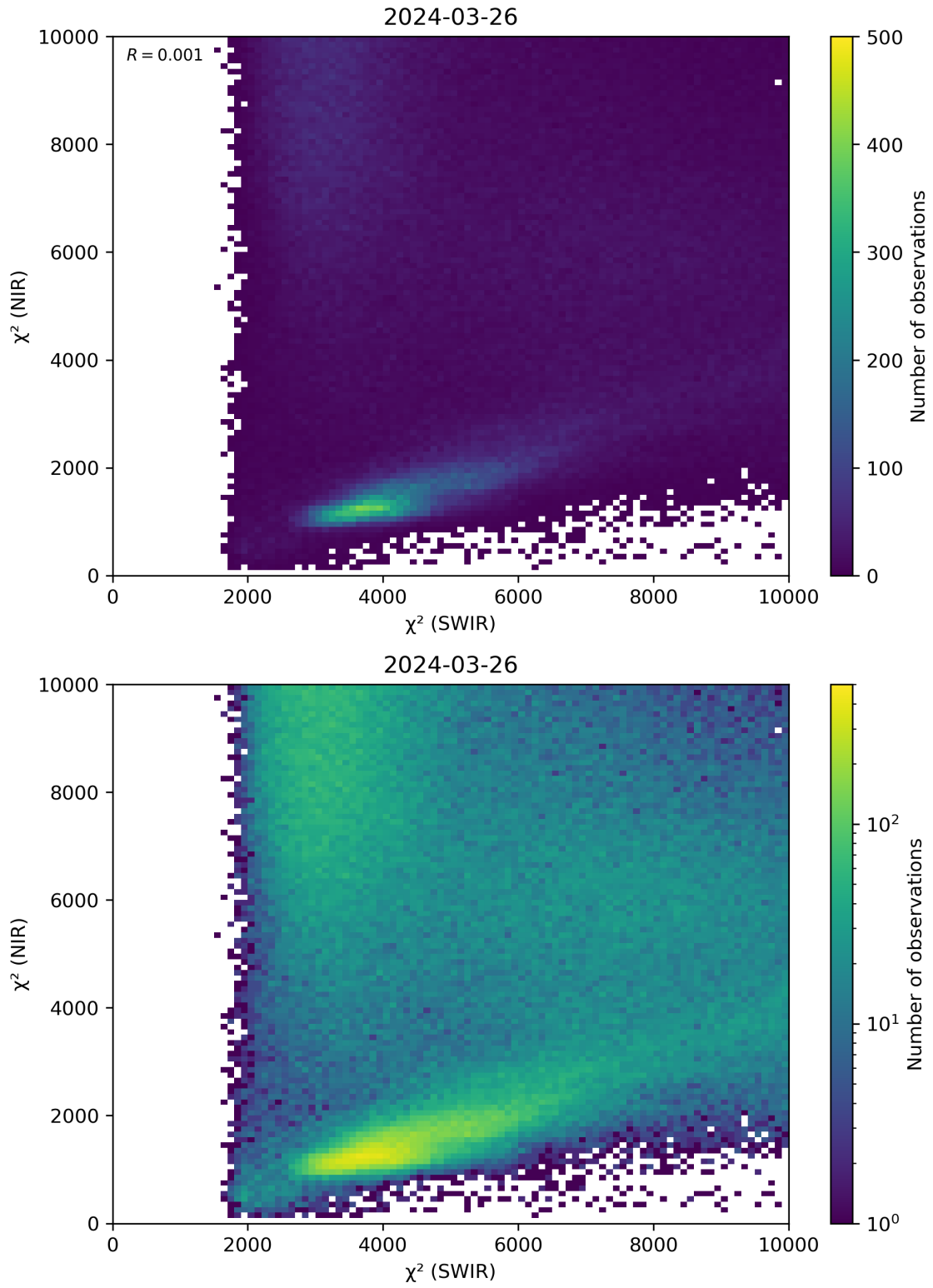
Figure 47: Scatter density plot of “ \chi^2 (SWIR)” against “ \chi^2 (NIR)” for 2024-03-25 to 2024-03-27.
