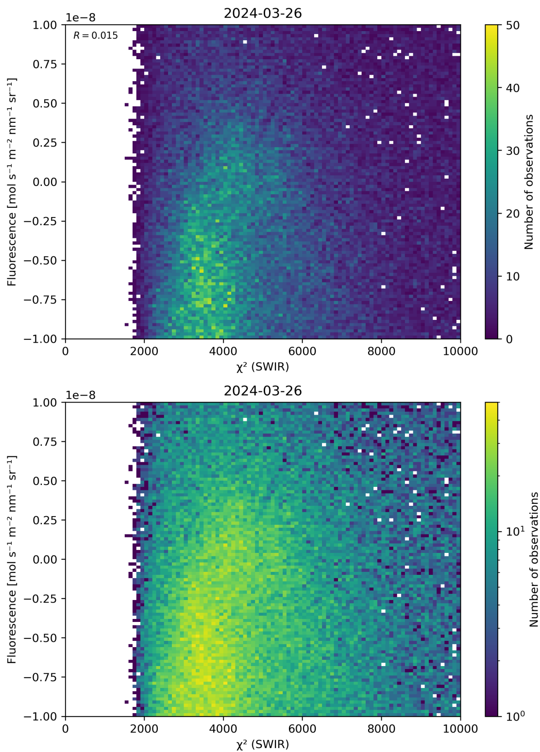
Figure 49: Scatter density plot of “ \chi^2 (SWIR)” against “Fluorescence” for 2024-03-25 to 2024-03-27.
