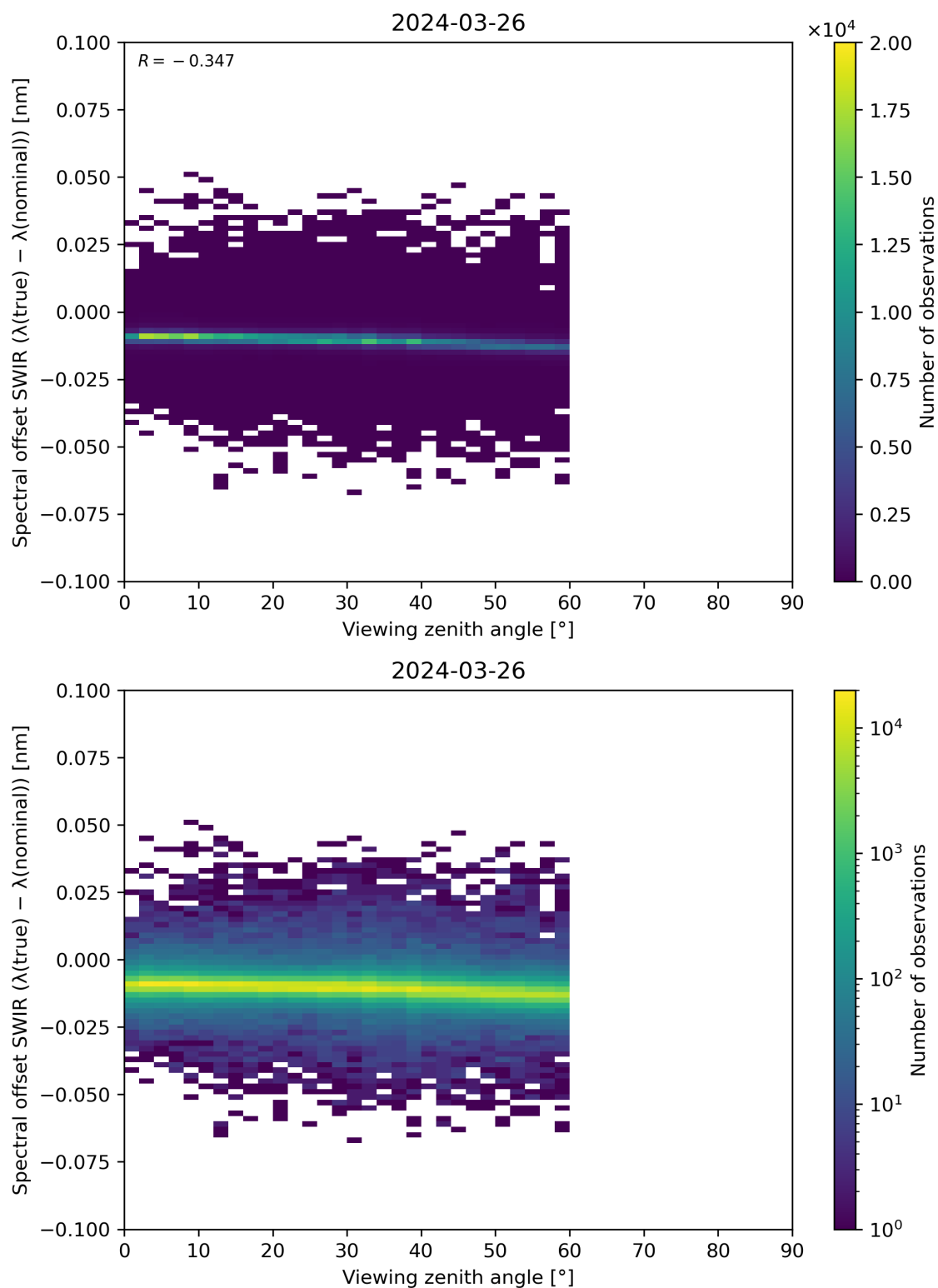
Figure 116: Scatter density plot of “Viewing zenith angle” against “Spectral offset SWIR ( \lambda(\text{true}) - \lambda(\text{nominal}) )” for 2024-03-25 to 2024-03-27.
