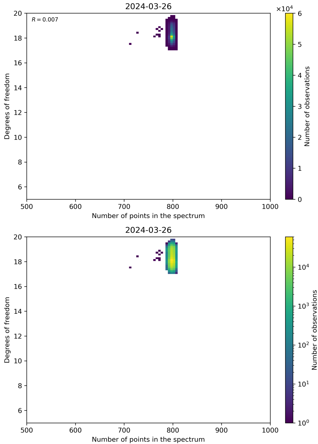
Figure 90: Scatter density plot of “Number of points in the spectrum” against “Degrees of freedom” for 2024-03-25 to 2024-03-27.
