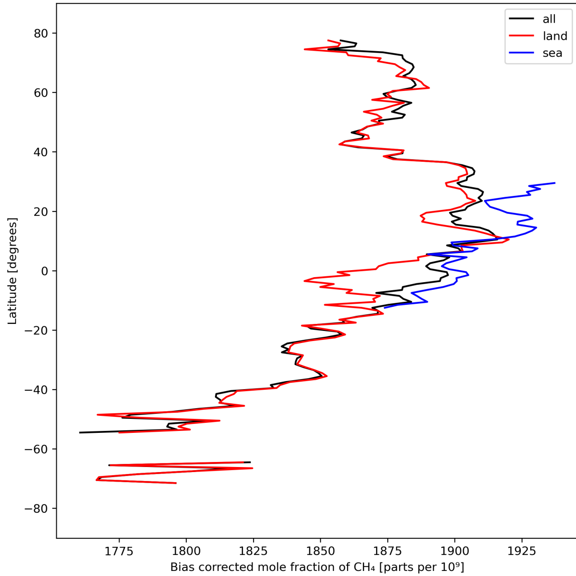
Figure 14: Zonal average of “Bias corrected mole fraction of CH 4 ” for 2024-03-25 to 2024-03-27.
