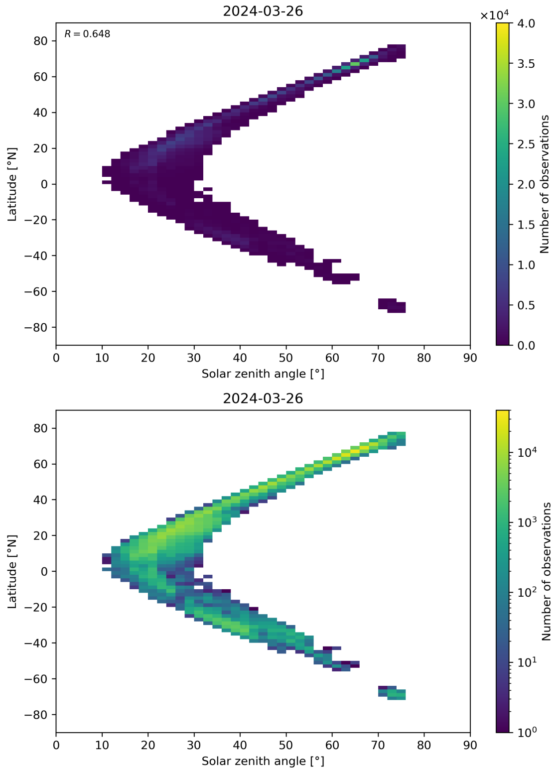
Figure 98: Scatter density plot of “Solar zenith angle” against “Latitude” for 2024-03-25 to 2024-03-27.
