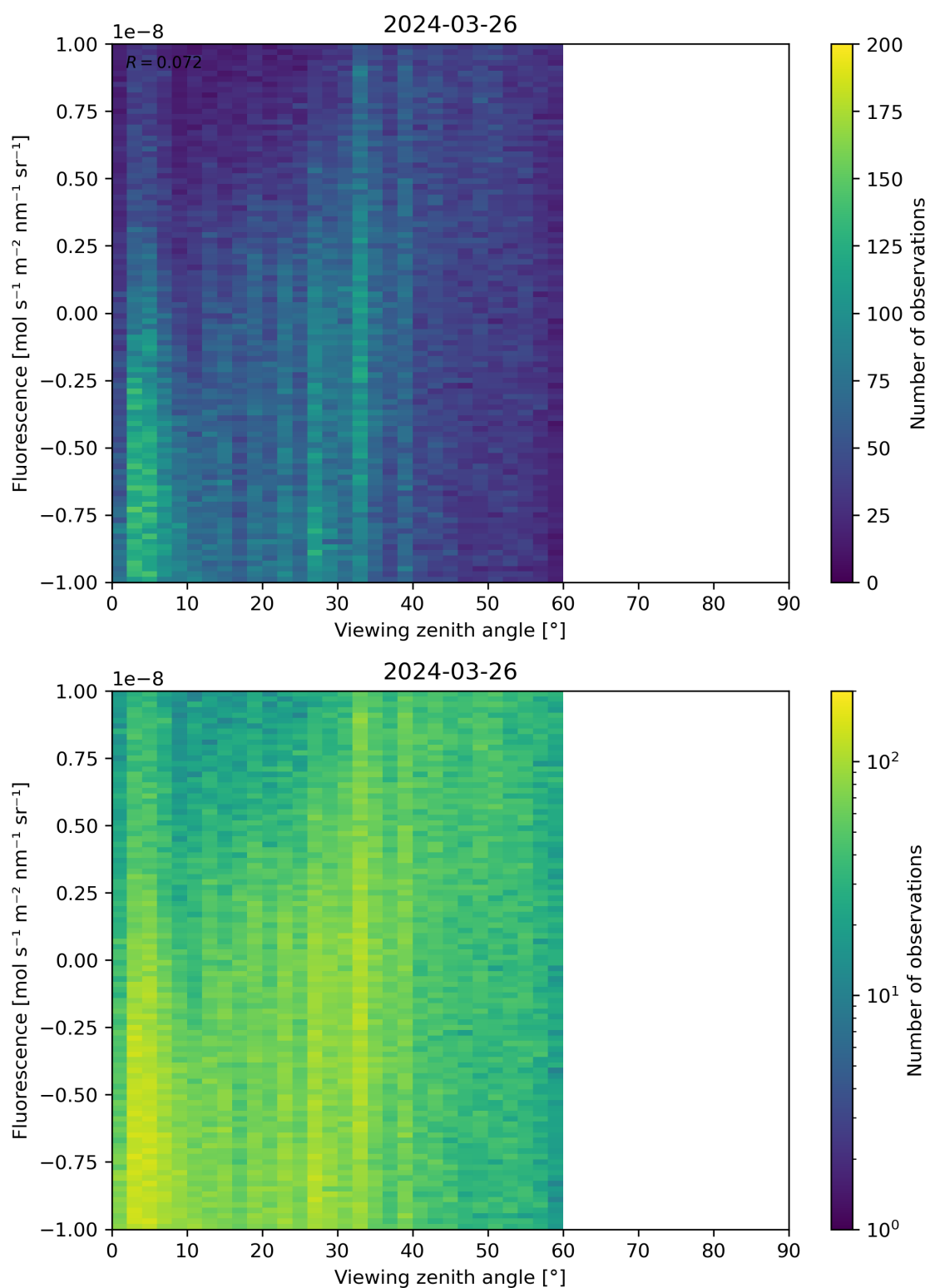
Figure 108: Scatter density plot of “Viewing zenith angle” against “Fluorescence” for 2024-03-25 to 2024-03-27.
