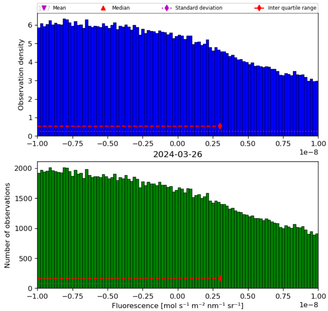
Figure 32: Histogram of “Fluorescence” for 2024-03-25 to 2024-03-27
