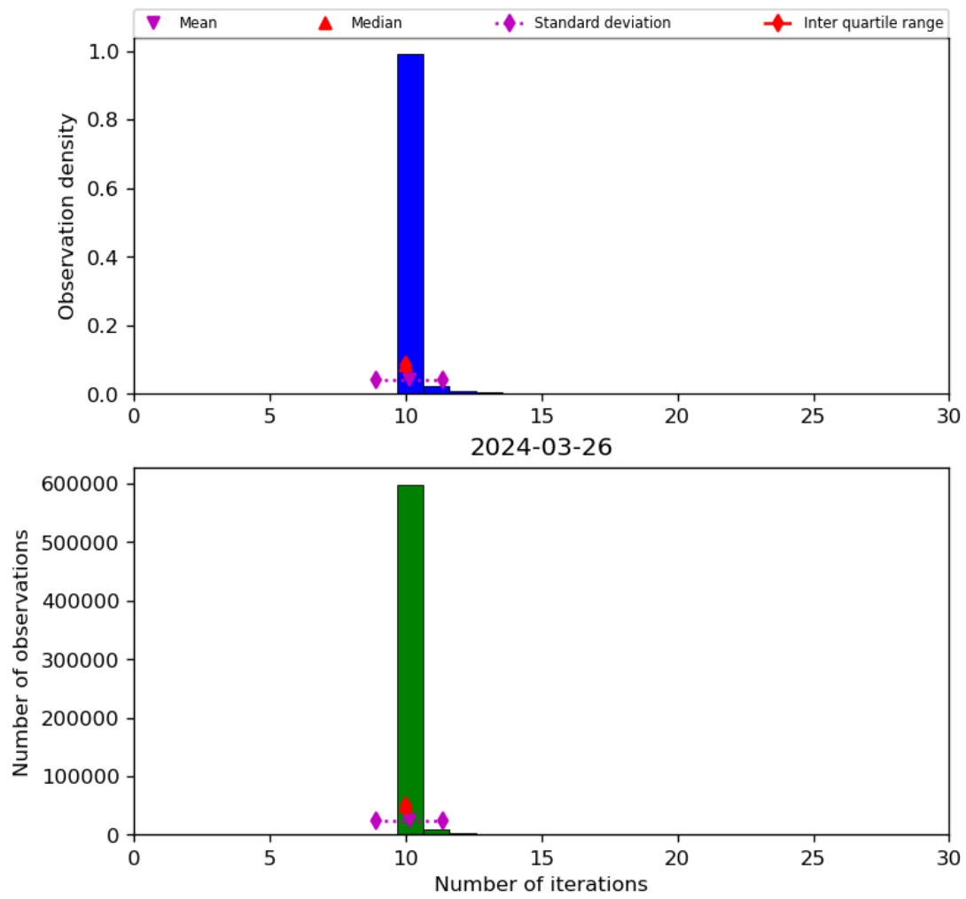
Figure 31: Histogram of “Number of iterations” for 2024-03-25 to 2024-03-27
