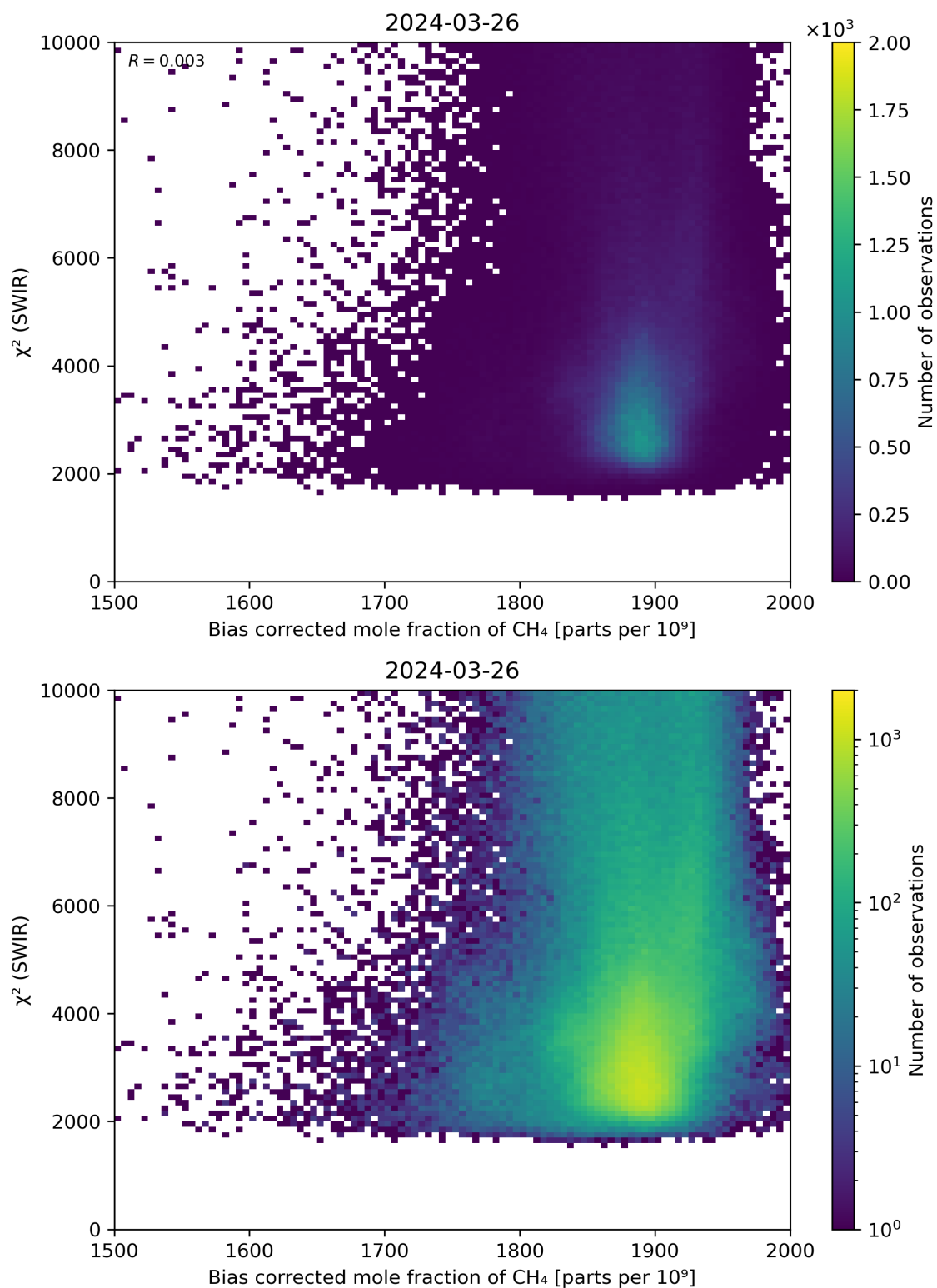
Figure 64: Scatter density plot of “Bias corrected mole fraction of \text{CH}_4 ” against “ \chi^2 (SWIR)” for 2024-03-25 to 2024-03-27.
