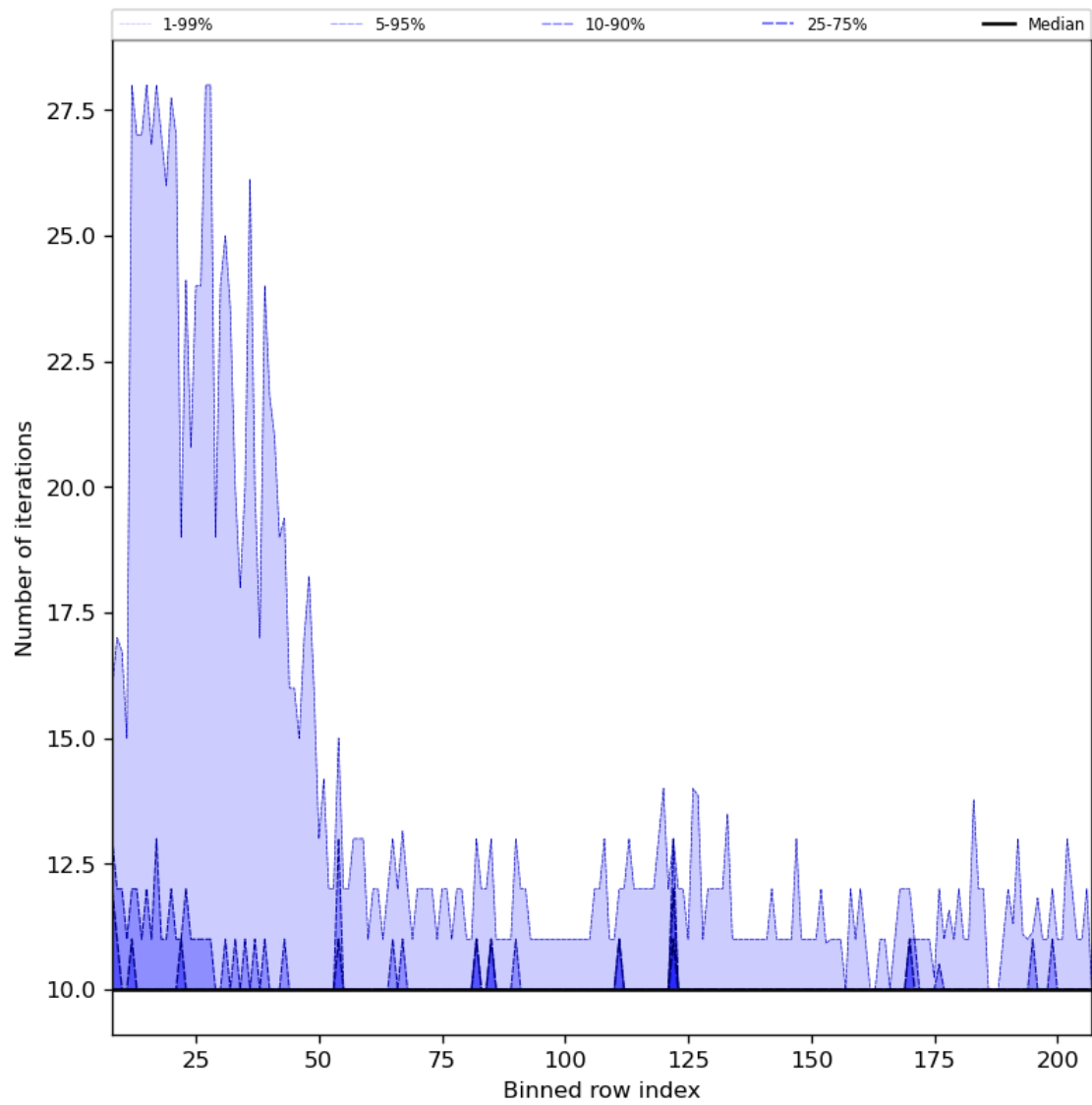
Figure 42: Along track statistics of “Number of iterations” for 2024-03-25 to 2024-03-27
