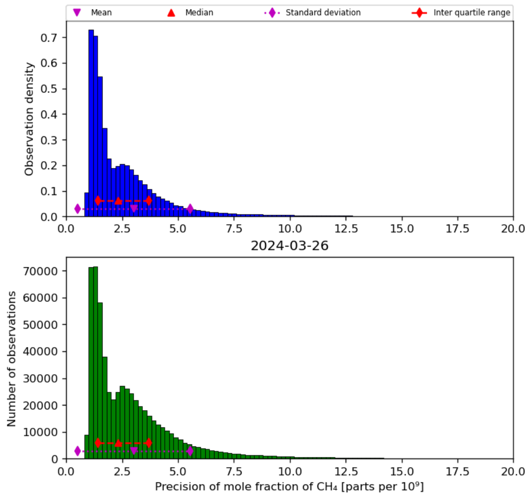
Figure 24: Histogram of “Precision of mole fraction of CH 4 ” for 2024-03-25 to 2024-03-27
