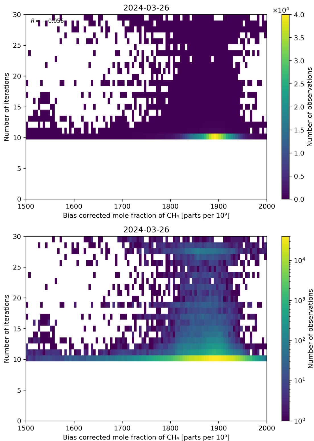
Figure 67: Scatter density plot of “Bias corrected mole fraction of CH 4 ” against “Number of iterations” for 2024-03-25 to 2024-03-27.
