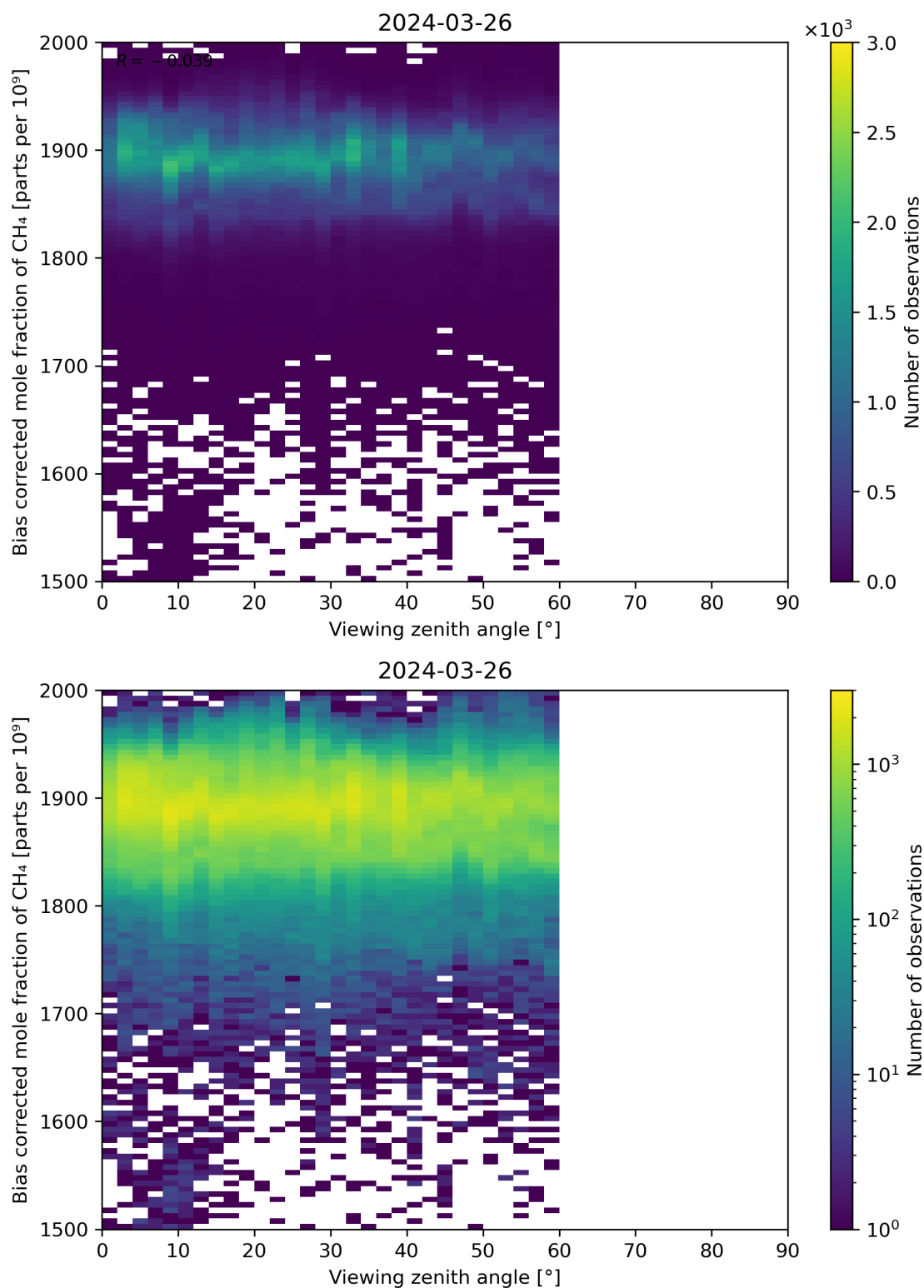
Figure 111: Scatter density plot of “Viewing zenith angle” against “Bias corrected mole fraction of CH 4 ” for 2024-03-25 to 2024-03-27.
