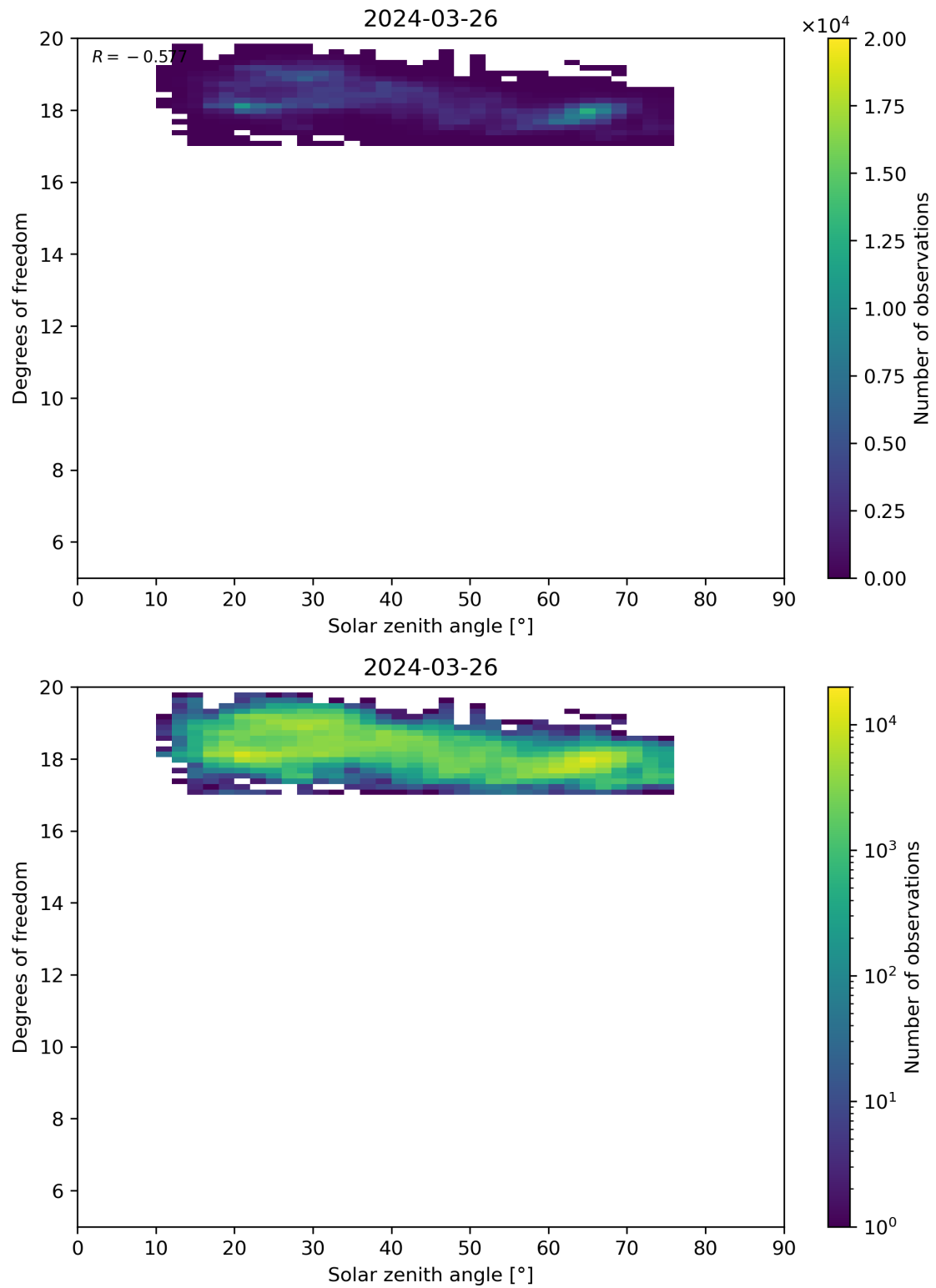
Figure 96: Scatter density plot of “Solar zenith angle” against “Degrees of freedom” for 2024-03-25 to 2024-03-27.
