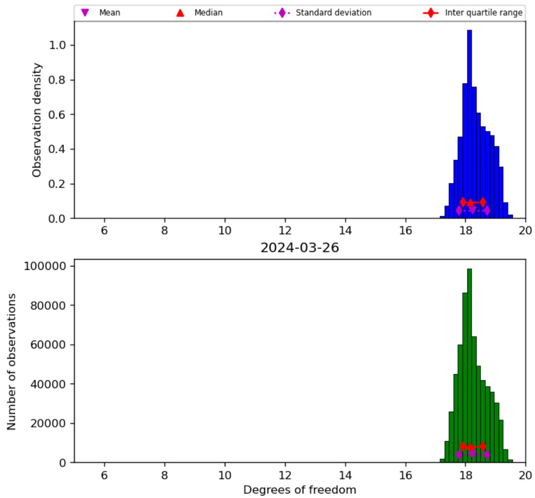
Figure 30: Histogram of “Degrees of freedom” for 2024-03-25 to 2024-03-27
