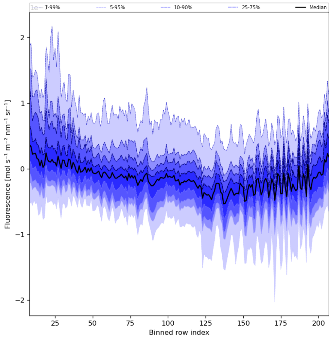
Figure 43: Along track statistics of “Fluorescence” for 2024-03-25 to 2024-03-27
