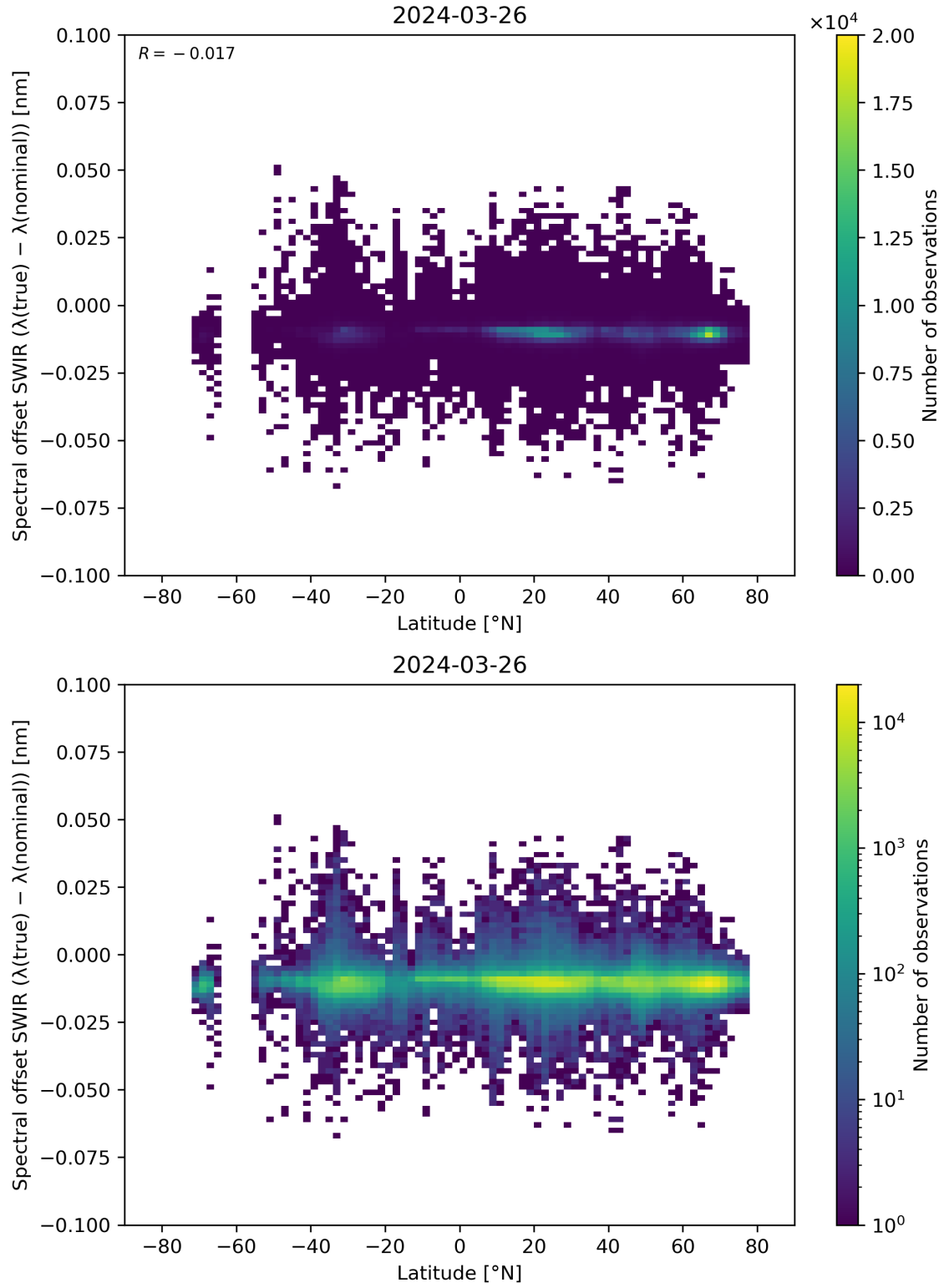
Figure 62: Scatter density plot of “Latitude” against “Spectral offset SWIR ( \lambda(\text{true}) - \lambda(\text{nominal}) )” for 2024-03-25 to 2024-03-27.
