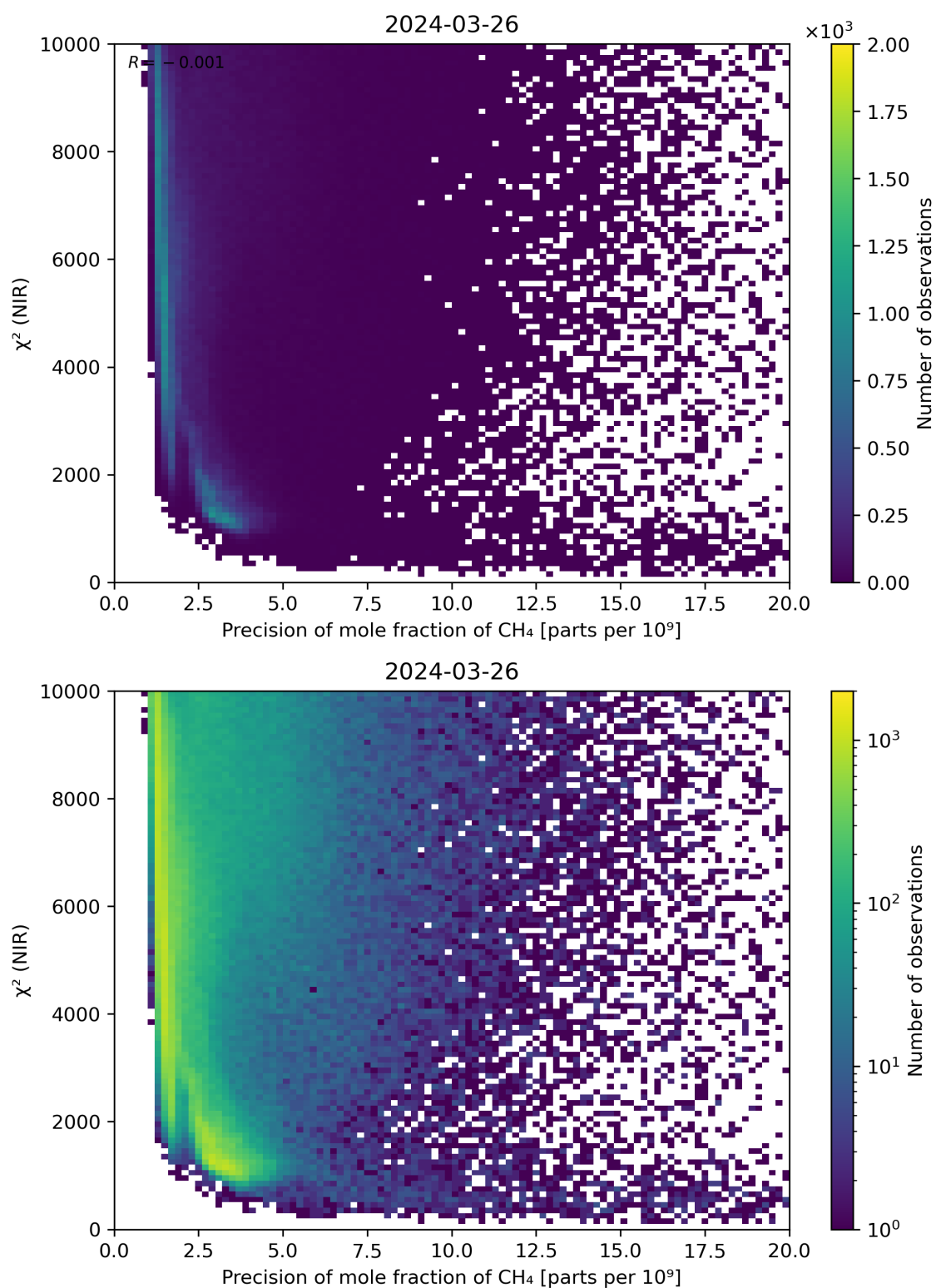
Figure 78: Scatter density plot of “Precision of mole fraction of CH 4 ” against “ \chi^2 (NIR)” for 2024-03-25 to 2024-03-27.
