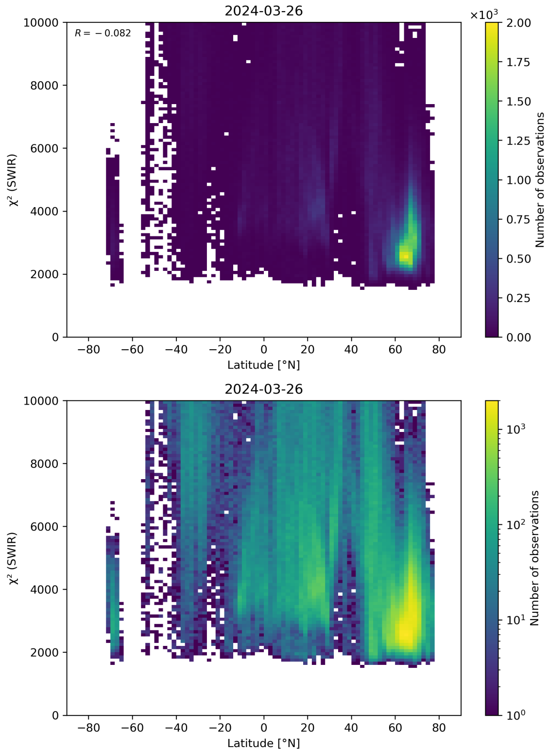
Figure 54: Scatter density plot of “Latitude” against “ \chi^2 (SWIR)” for 2024-03-25 to 2024-03-27.
