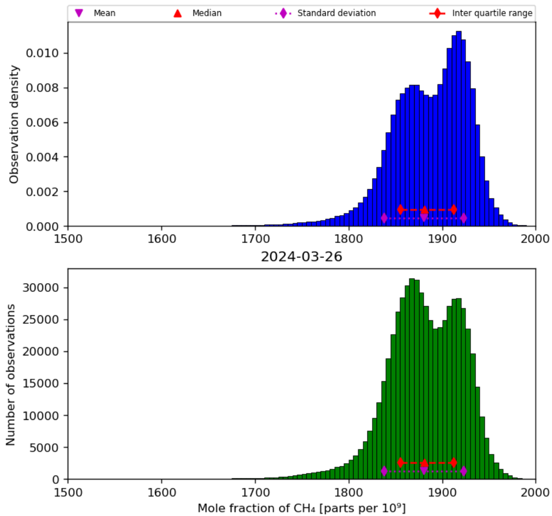
Figure 23: Histogram of “Mole fraction of CH 4 ” for 2024-03-25 to 2024-03-27
