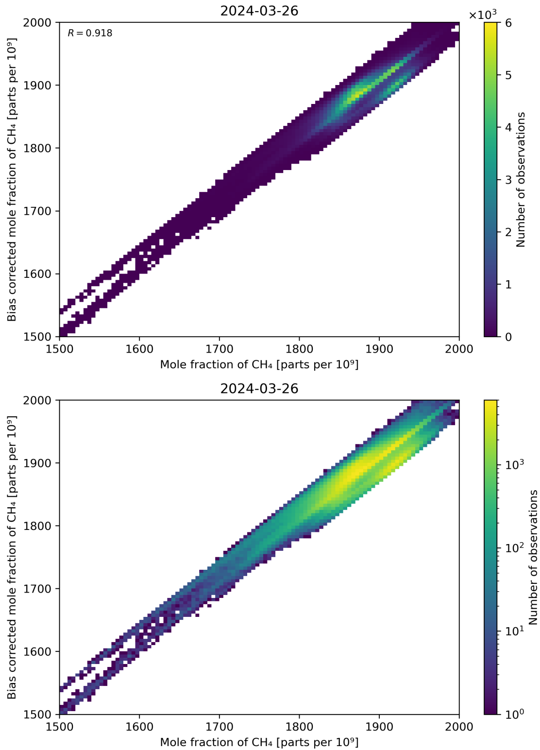
Figure 74: Scatter density plot of “Mole fraction of CH 4 ” against “Bias corrected mole fraction of CH 4 ” for 2024-03-25 to 2024-03-27.
