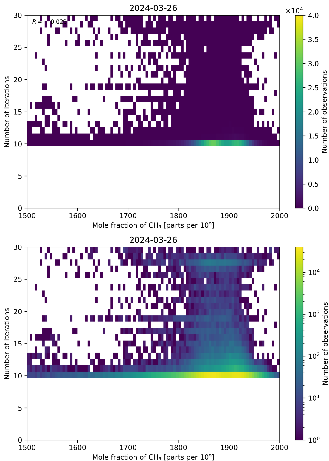
Figure 76: Scatter density plot of “Mole fraction of CH 4 ” against “Number of iterations” for 2024-03-25 to 2024-03-27.
