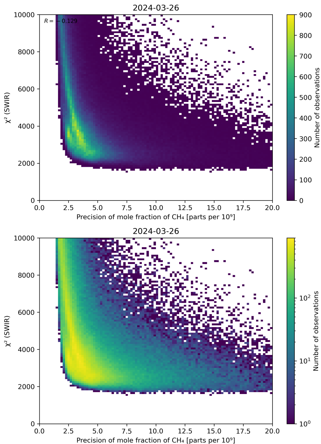
Figure 79: Scatter density plot of “Precision of mole fraction of \text{CH}_4 ” against “ \chi^2 (SWIR)” for 2024-03-25 to 2024-03-27.
