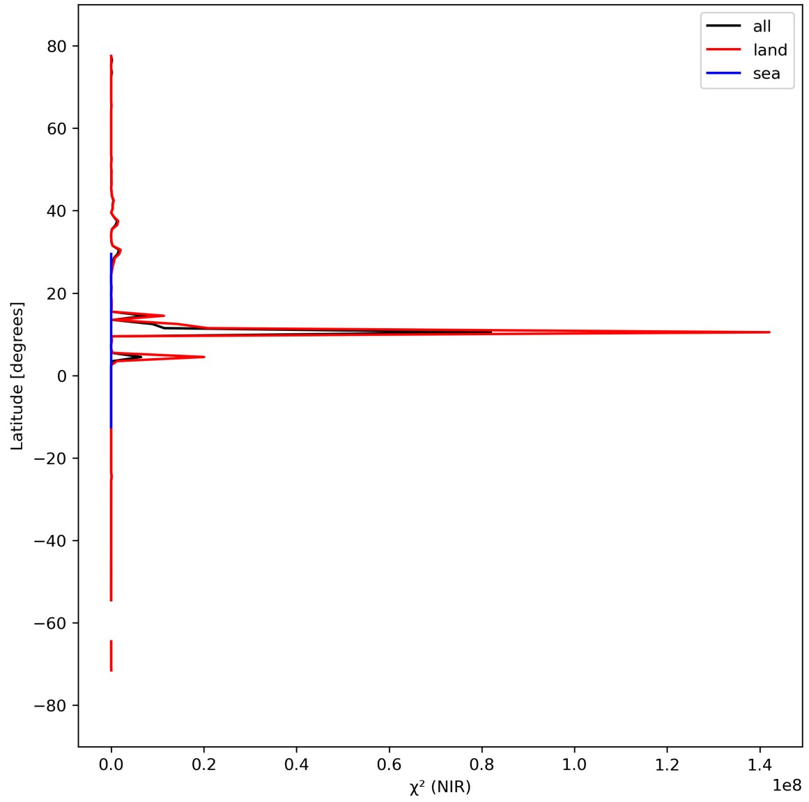
Figure 18: Zonal average of “ \chi^2 (NIR)” for 2024-03-25 to 2024-03-27.
