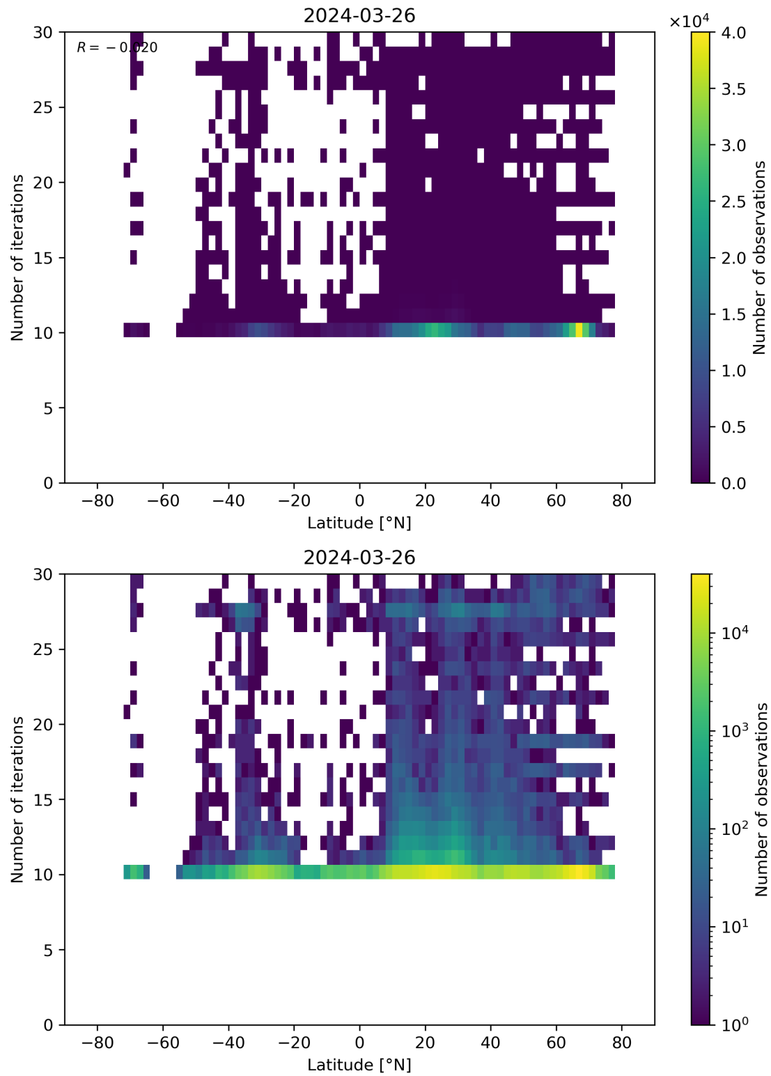
Figure 60: Scatter density plot of “Latitude” against “Number of iterations” for 2024-03-25 to 2024-03-27.
