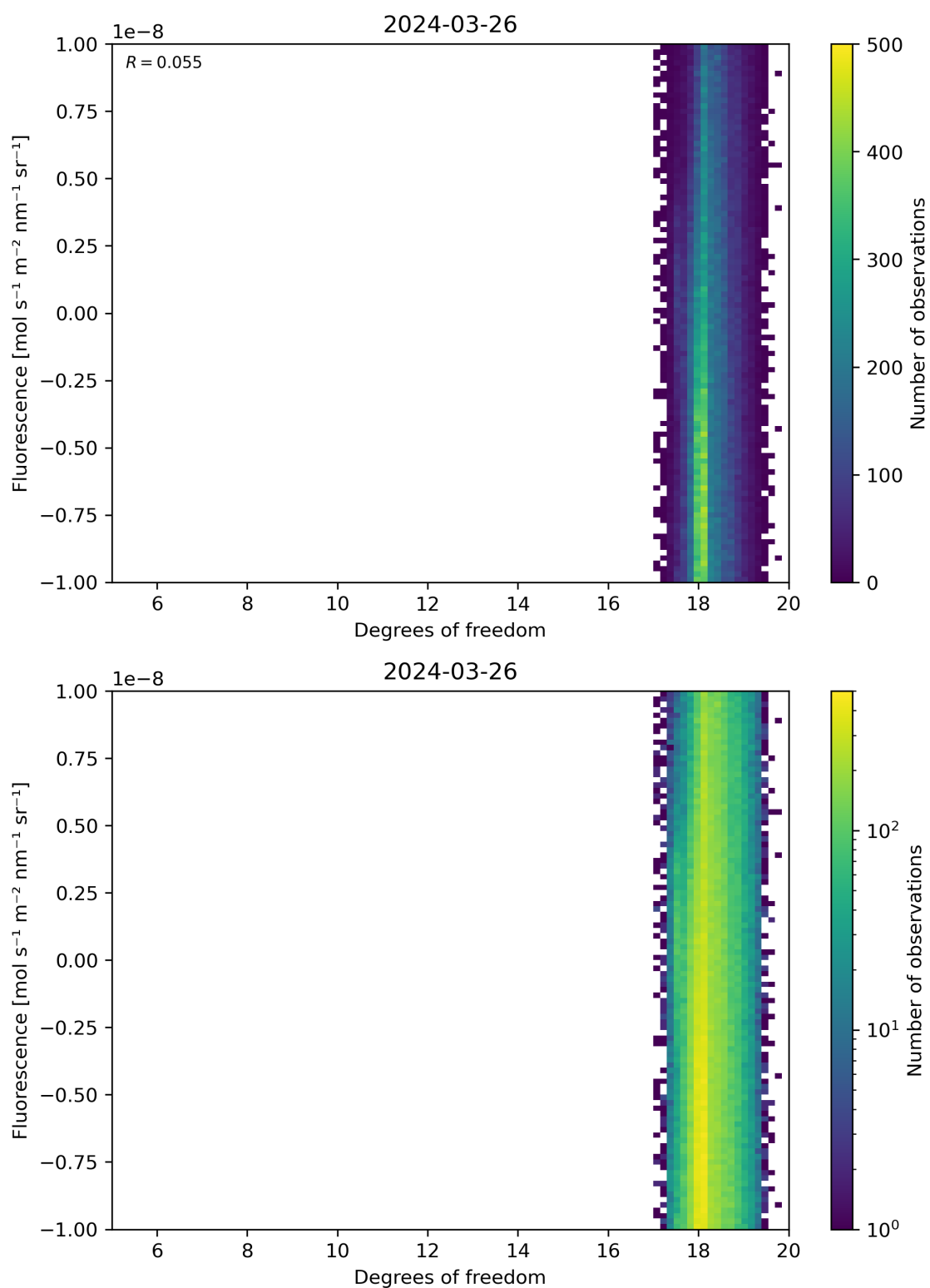
Figure 51: Scatter density plot of “Degrees of freedom” against “Fluorescence” for 2024-03-25 to 2024-03-27.
