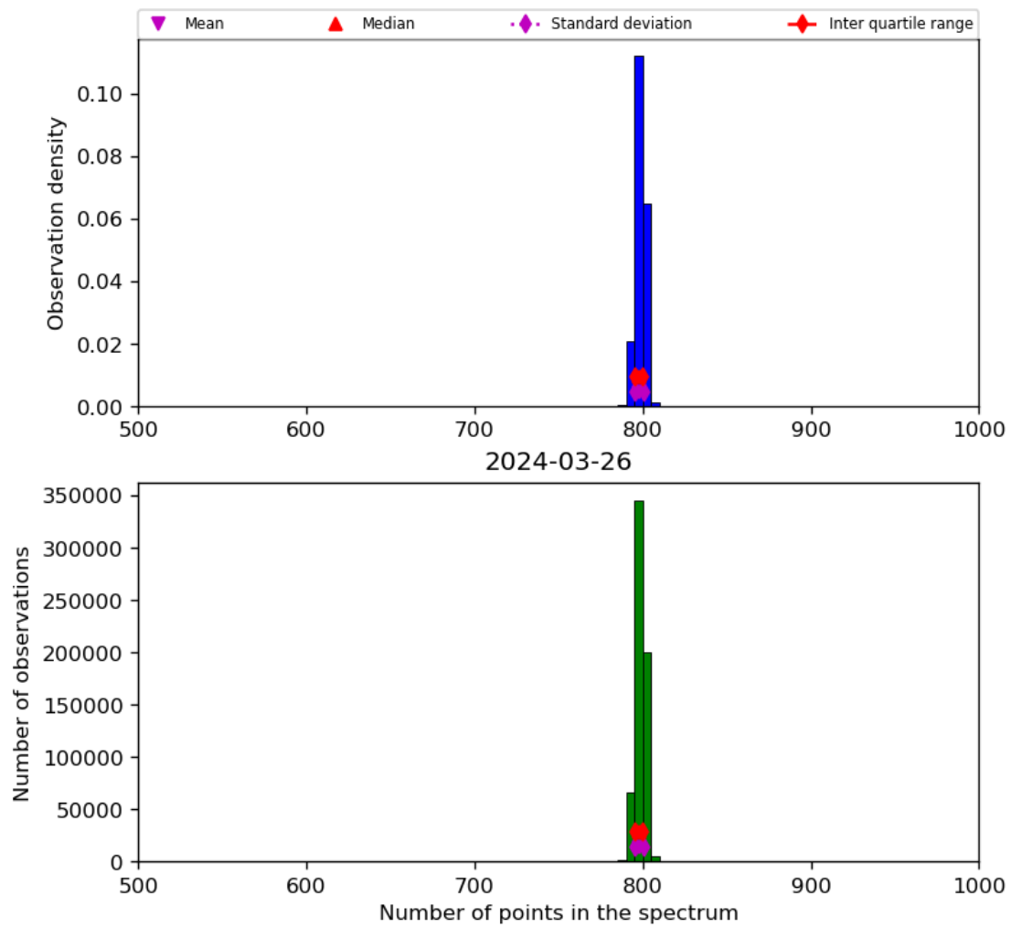
Figure 26: Histogram of “Number of points in the spectrum” for 2024-03-25 to 2024-03-27
