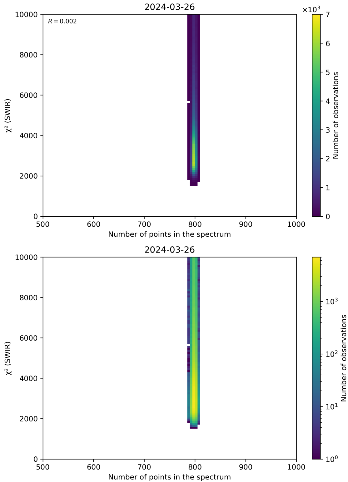
Figure 89: Scatter density plot of “Number of points in the spectrum” against “ \chi^2 (SWIR)” for 2024-03-25 to 2024-03-27.
