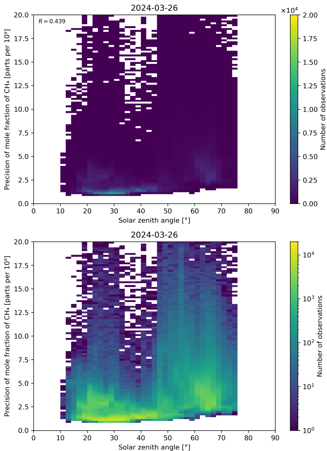
Figure 101: Scatter density plot of “Solar zenith angle” against “Precision of mole fraction of CH 4 ” for 2024-03-25 to 2024-03-27.
