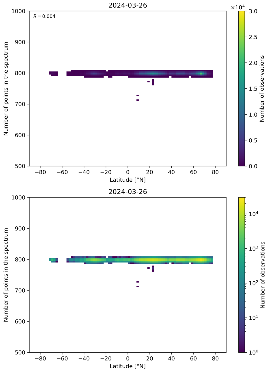
Figure 61: Scatter density plot of “Latitude” against “Number of points in the spectrum” for 2024-03-25 to 2024-03-27.
