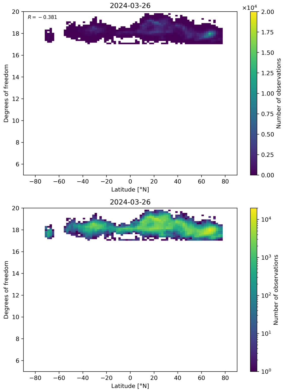
Figure 55: Scatter density plot of “Latitude” against “Degrees of freedom” for 2024-03-25 to 2024-03-27.
