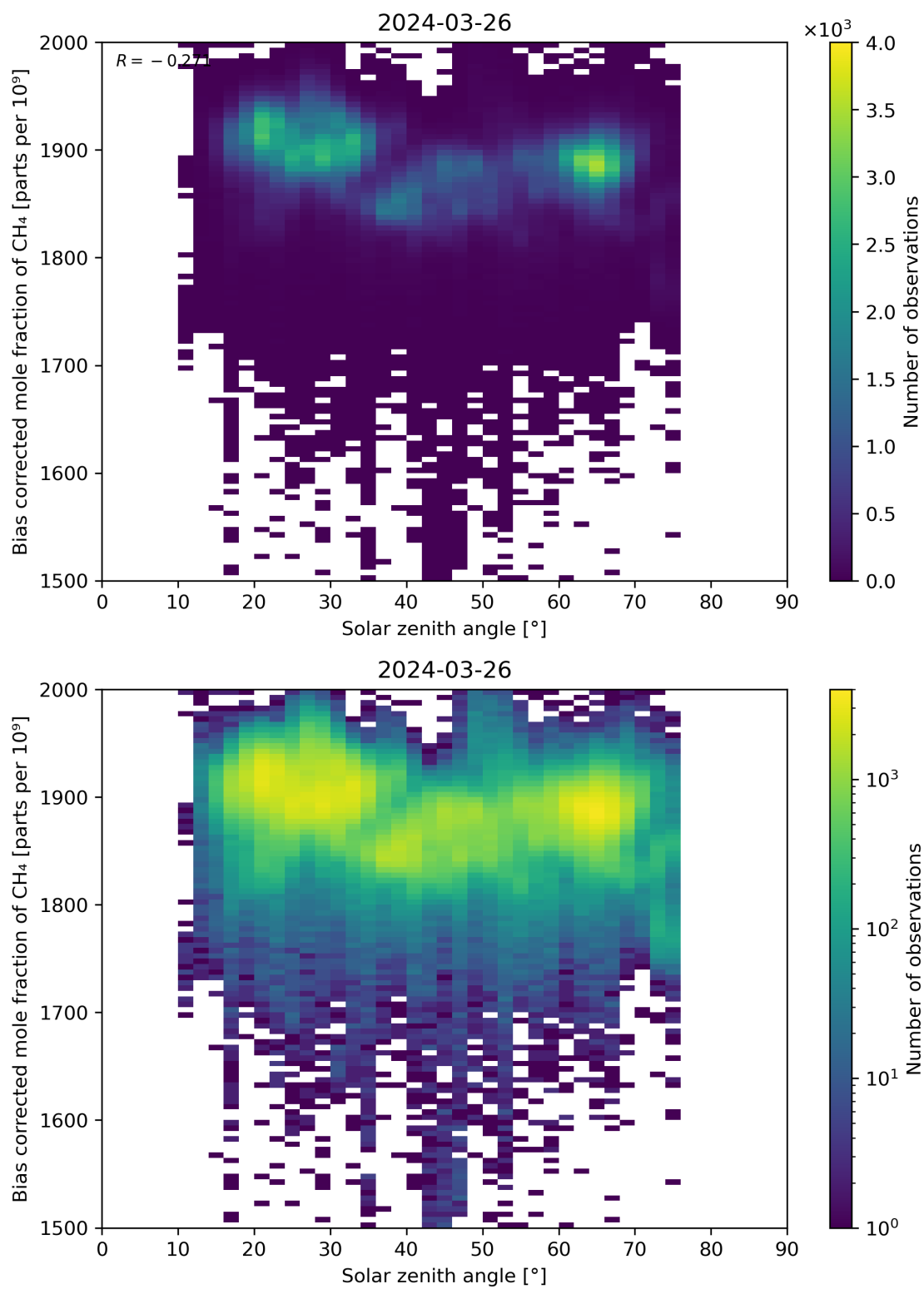
Figure 100: Scatter density plot of “Solar zenith angle” against “Bias corrected mole fraction of CH 4 ” for 2024-03-25 to 2024-03-27.
