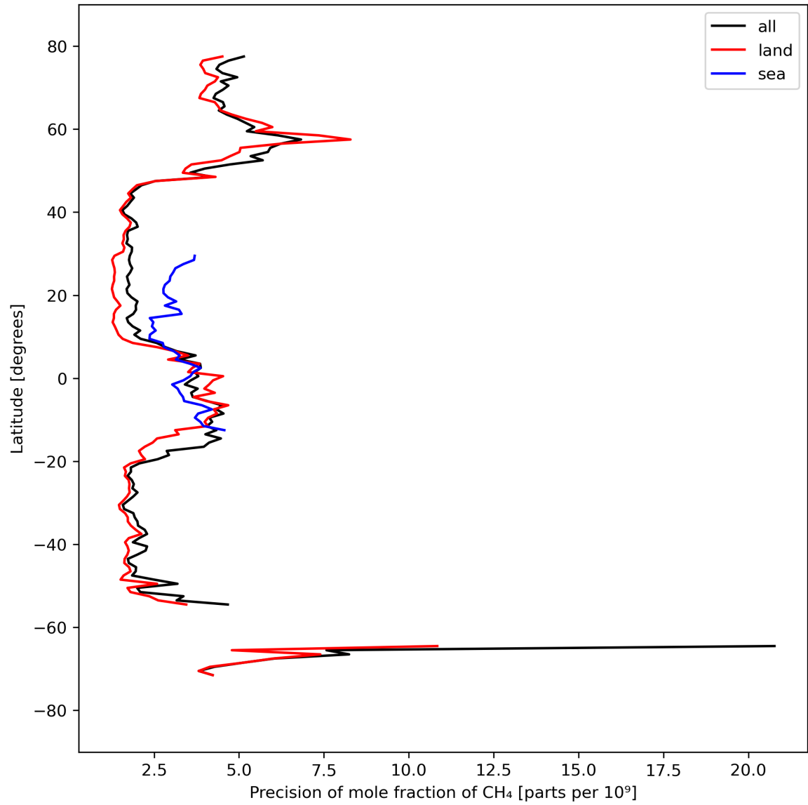
Figure 13: Zonal average of “Precision of mole fraction of CH 4 ” for 2024-03-25 to 2024-03-27.
