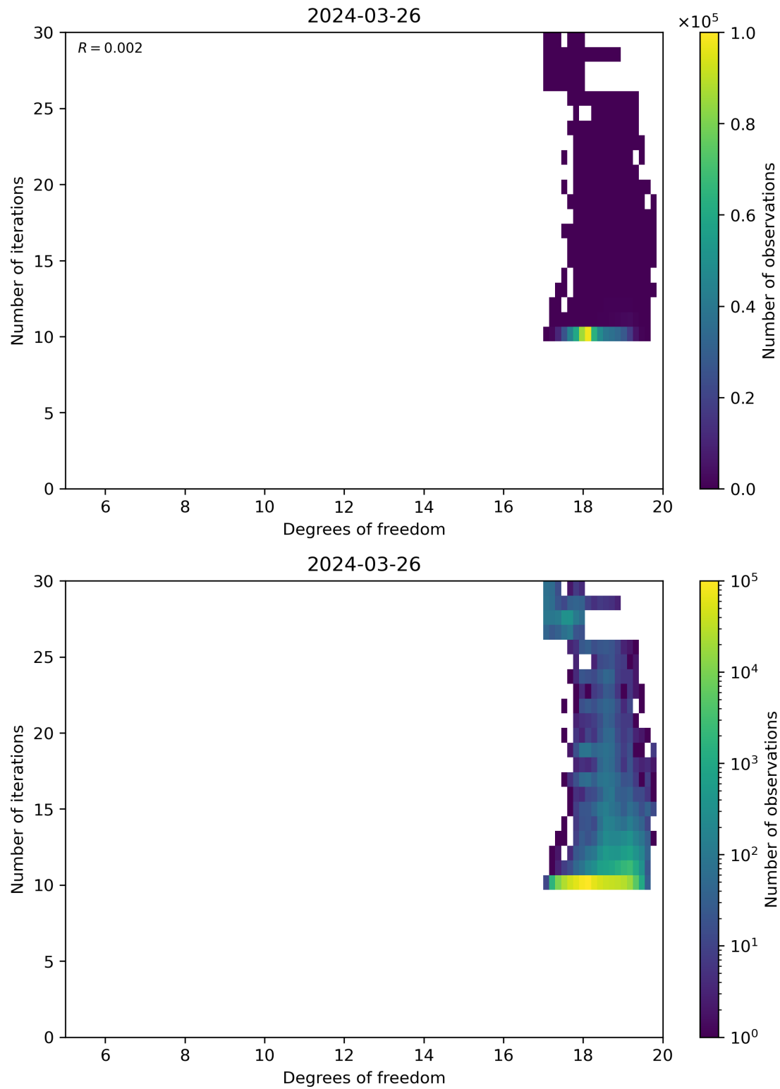
Figure 52: Scatter density plot of “Degrees of freedom” against “Number of iterations” for 2024-03-25 to 2024-03-27.
