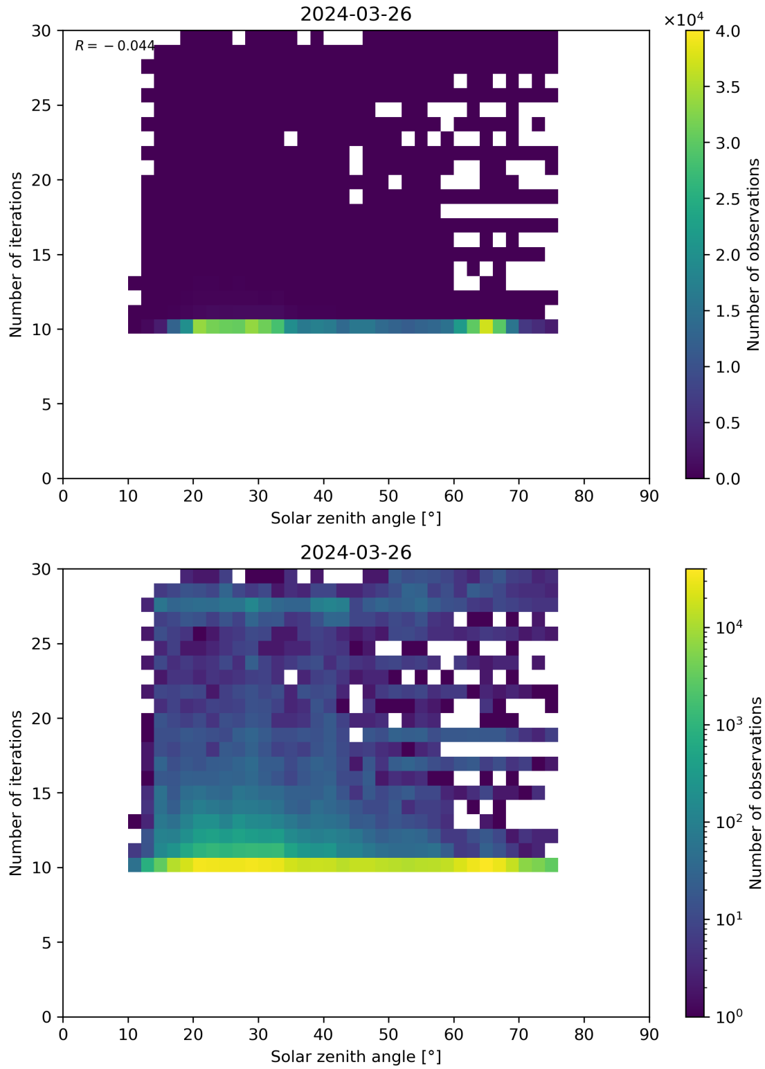
Figure 102: Scatter density plot of “Solar zenith angle” against “Number of iterations” for 2024-03-25 to 2024-03-27.
