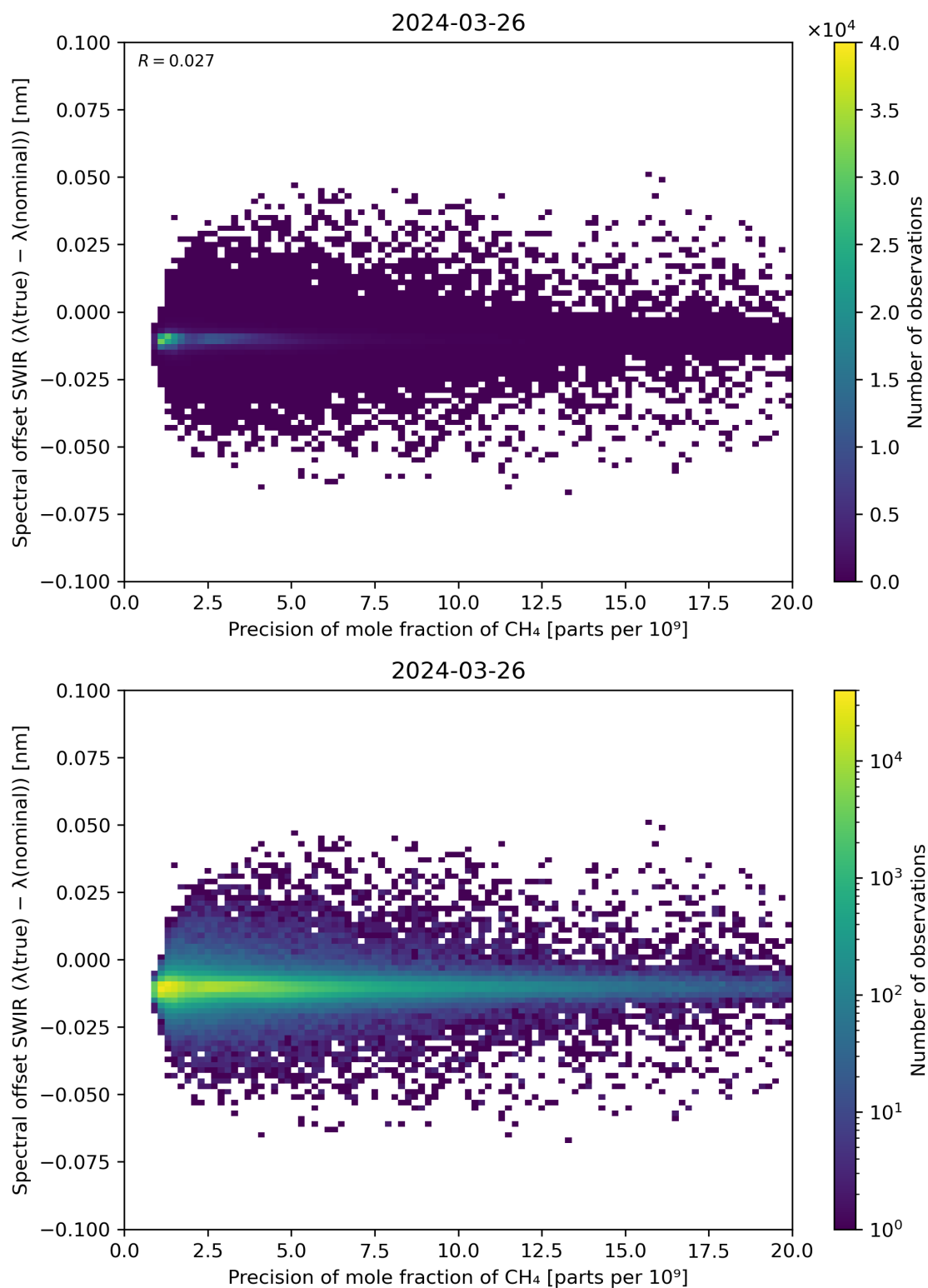
Figure 85: Scatter density plot of “Precision of mole fraction of \text{CH}_4 ” against “Spectral offset SWIR ( \lambda(\text{true}) - \lambda(\text{nominal}) )” for 2024-03-25 to 2024-03-27.
