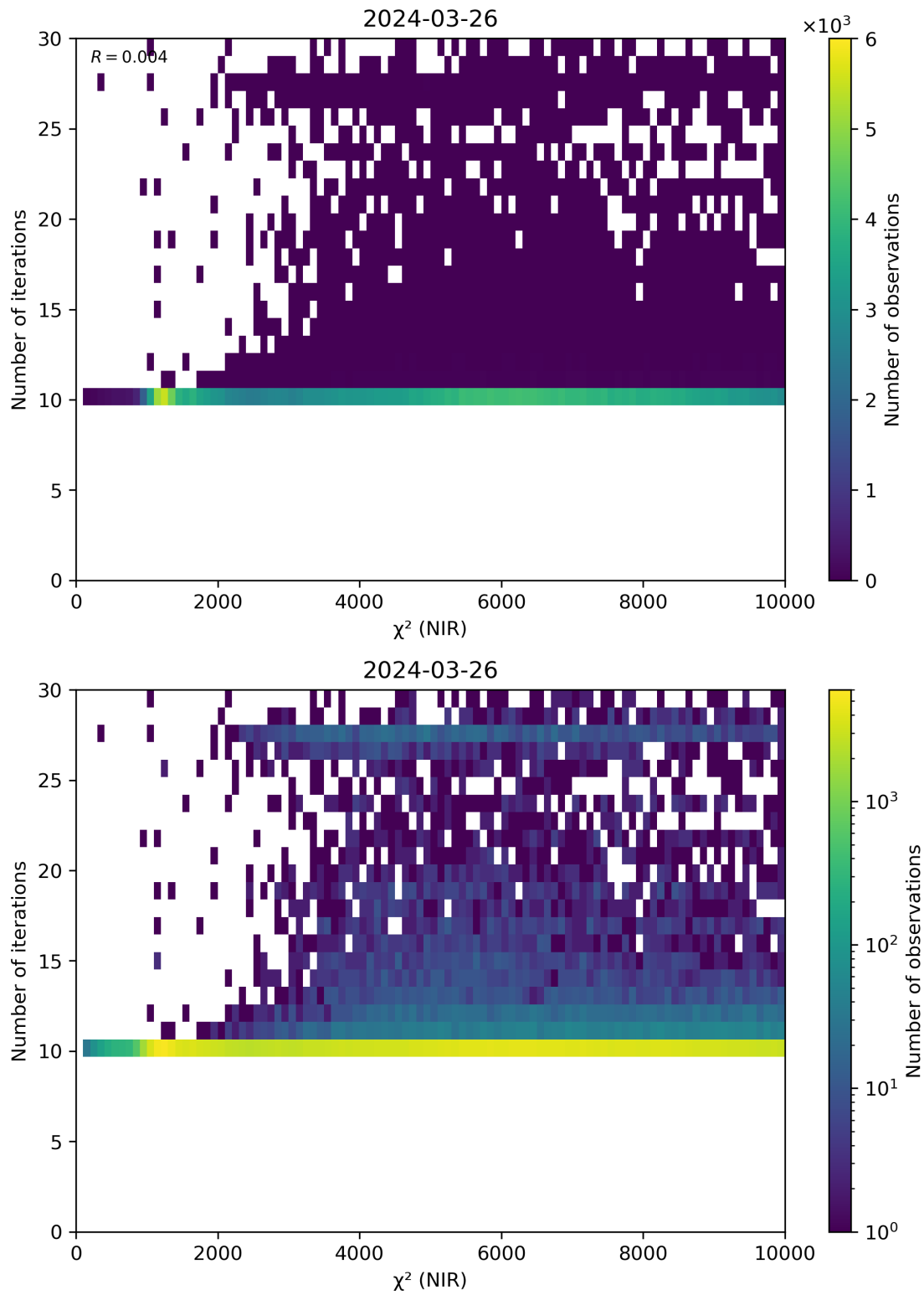
Figure 46: Scatter density plot of “ \chi^2 (NIR)” against “Number of iterations” for 2024-03-25 to 2024-03-27.
