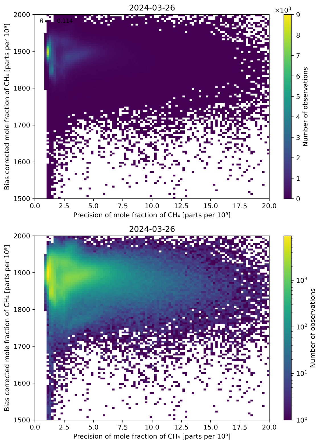
Figure 82: Scatter density plot of “Precision of mole fraction of CH 4 ” against “Bias corrected mole fraction of CH 4 ” for 2024-03-25 to 2024-03-27.
