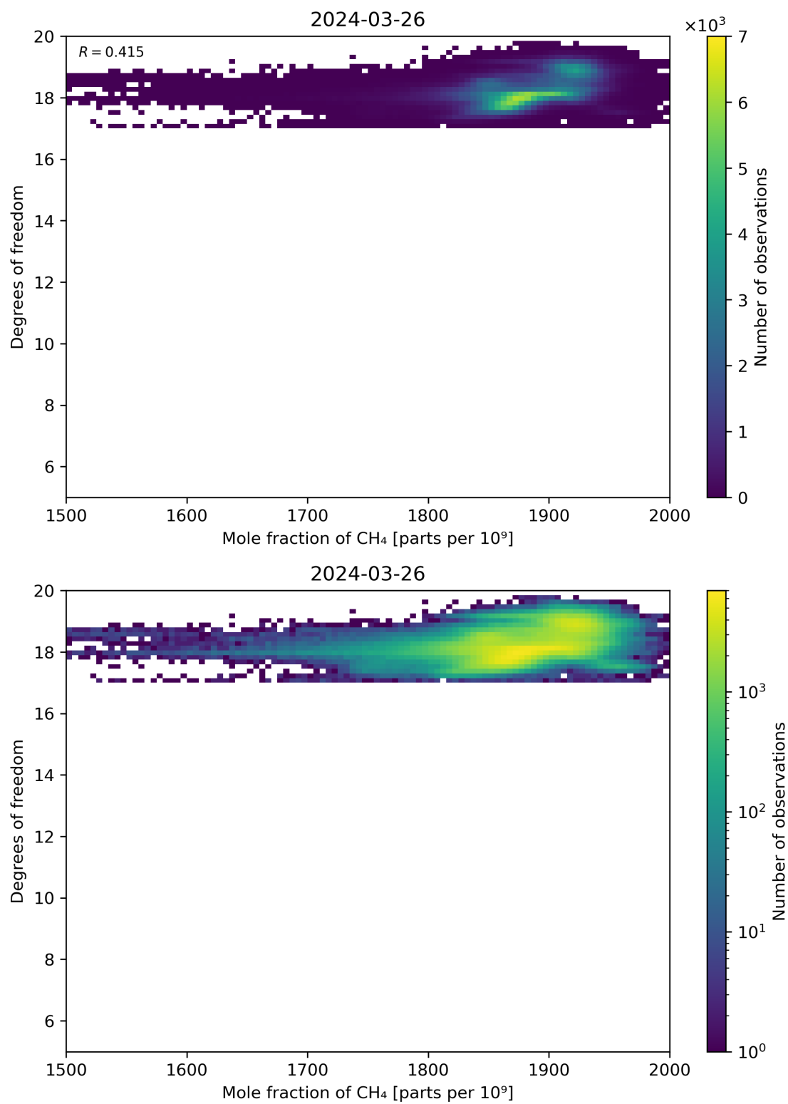
Figure 72: Scatter density plot of “Mole fraction of CH 4 ” against “Degrees of freedom” for 2024-03-25 to 2024-03-27.
