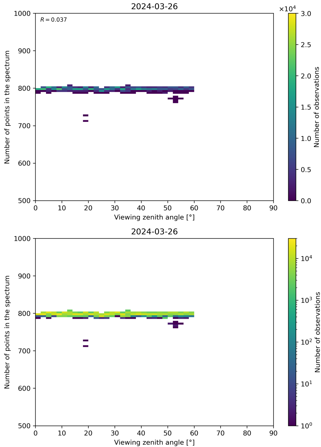
Figure 114: Scatter density plot of “Viewing zenith angle” against “Number of points in the spectrum” for 2024-03-25 to 2024-03-27.
