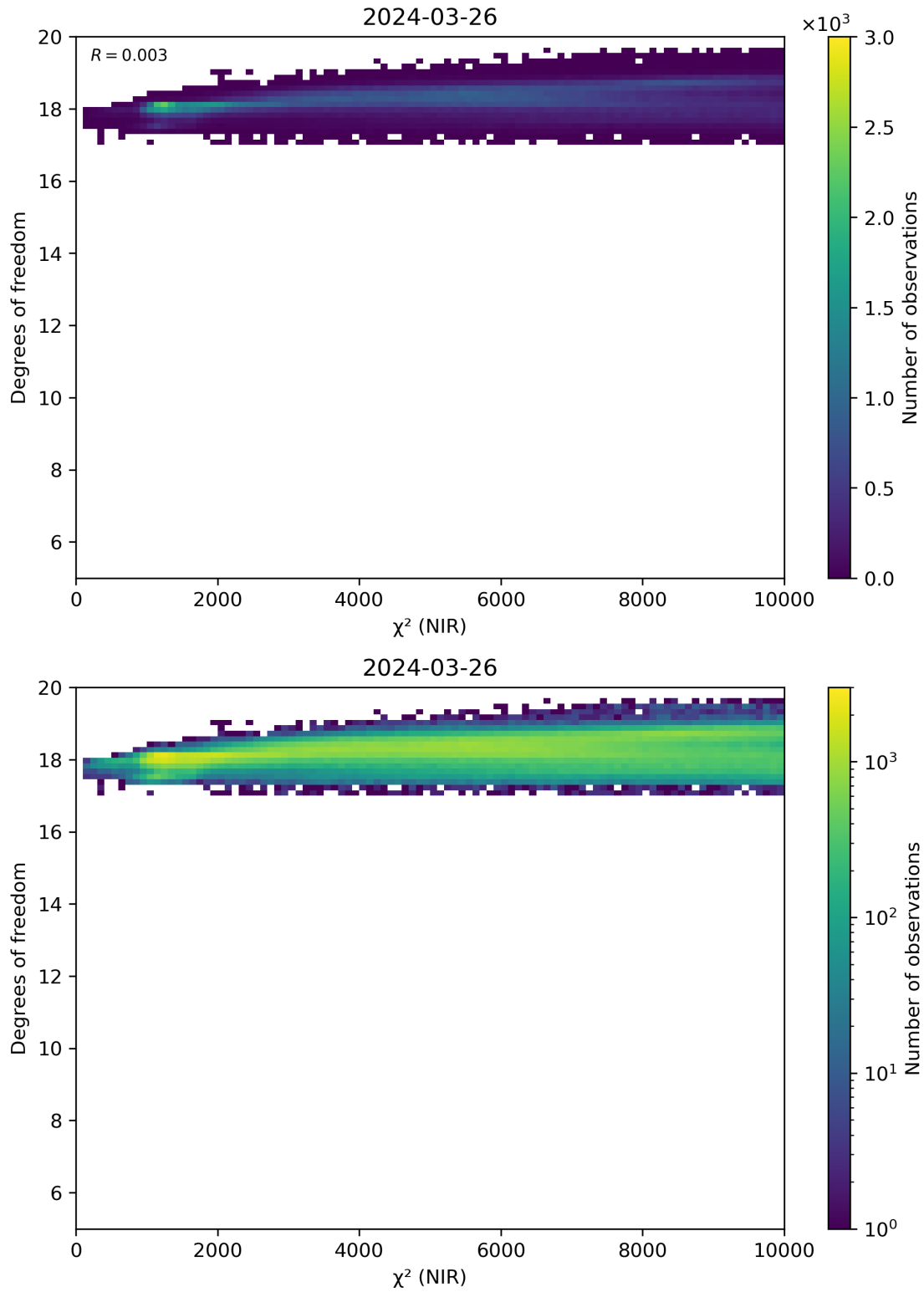
Figure 44: Scatter density plot of “ \chi^2 (NIR)” against “Degrees of freedom” for 2024-03-25 to 2024-03-27.
