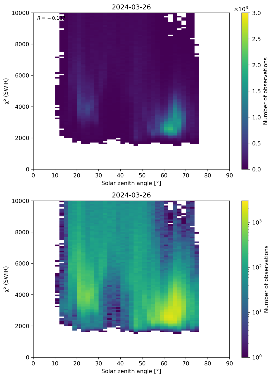
Figure 95: Scatter density plot of “Solar zenith angle” against “ \chi^2 (SWIR)” for 2024-03-25 to 2024-03-27.
