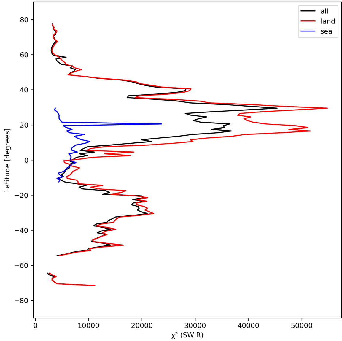
Figure 17: Zonal average of “ \chi^2 (SWIR)” for 2024-03-25 to 2024-03-27.
