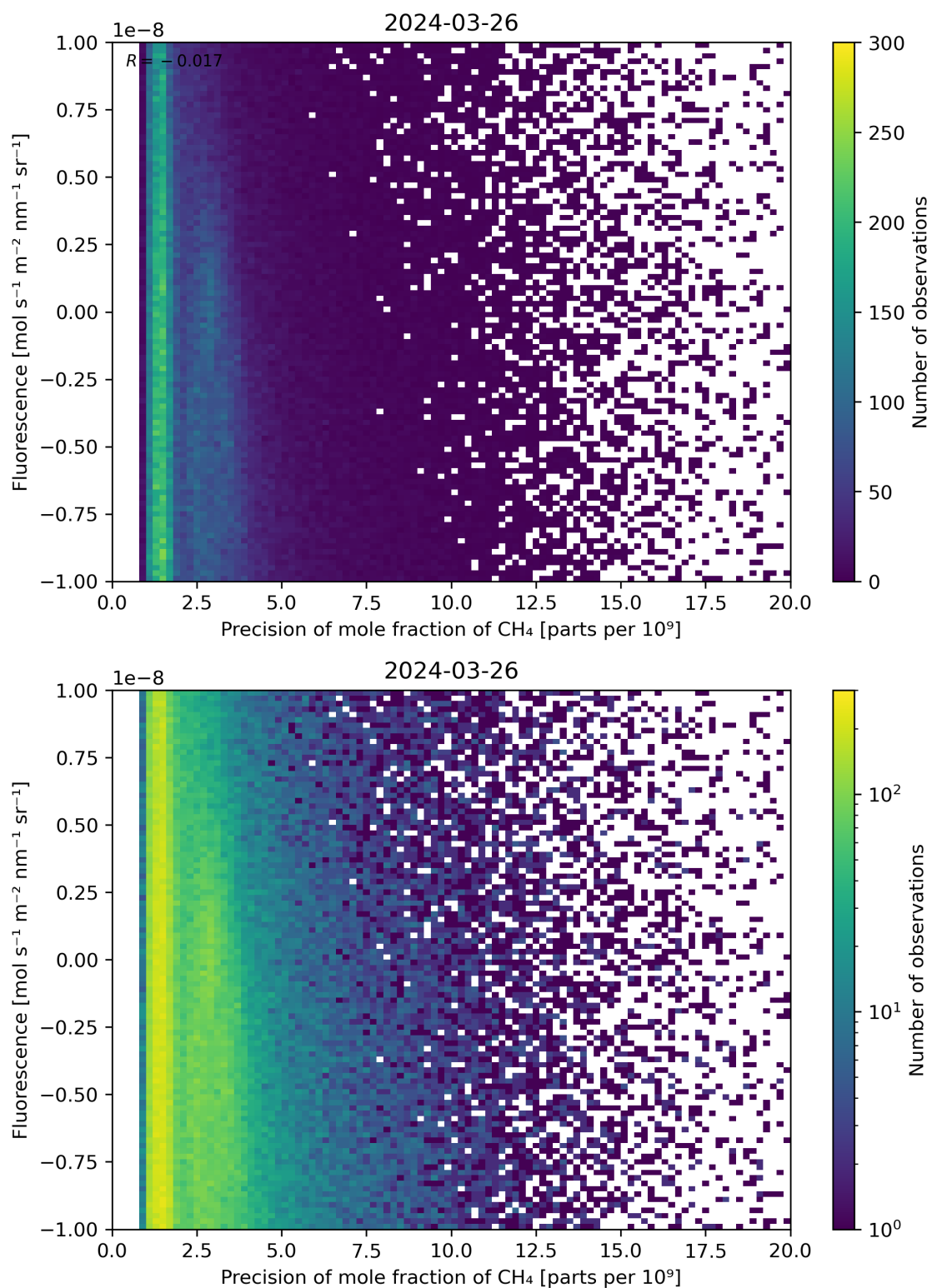
Figure 81: Scatter density plot of “Precision of mole fraction of CH 4 ” against “Fluorescence” for 2024-03-25 to 2024-03-27.
