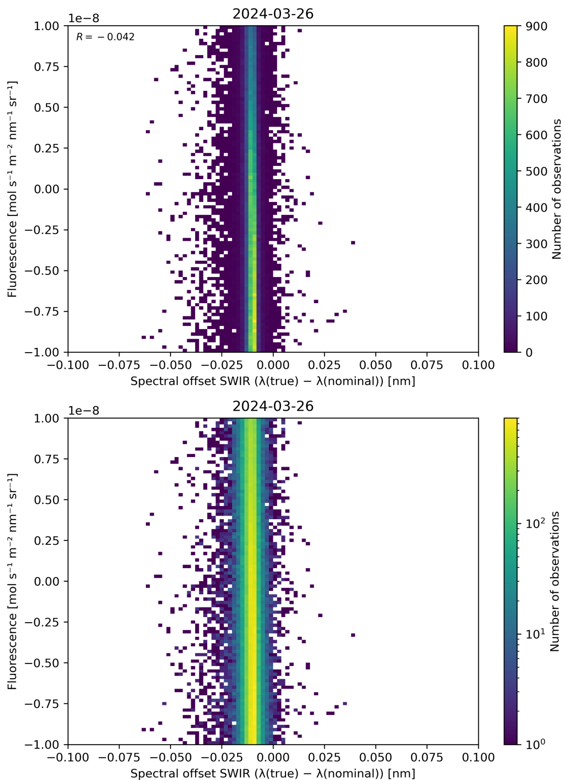
Figure 120: Scatter density plot of “Spectral offset SWIR ( \lambda(\text{true}) - \lambda(\text{nominal}) )” against “Fluorescence” for 2024-03-25 to 2024-03-27.
