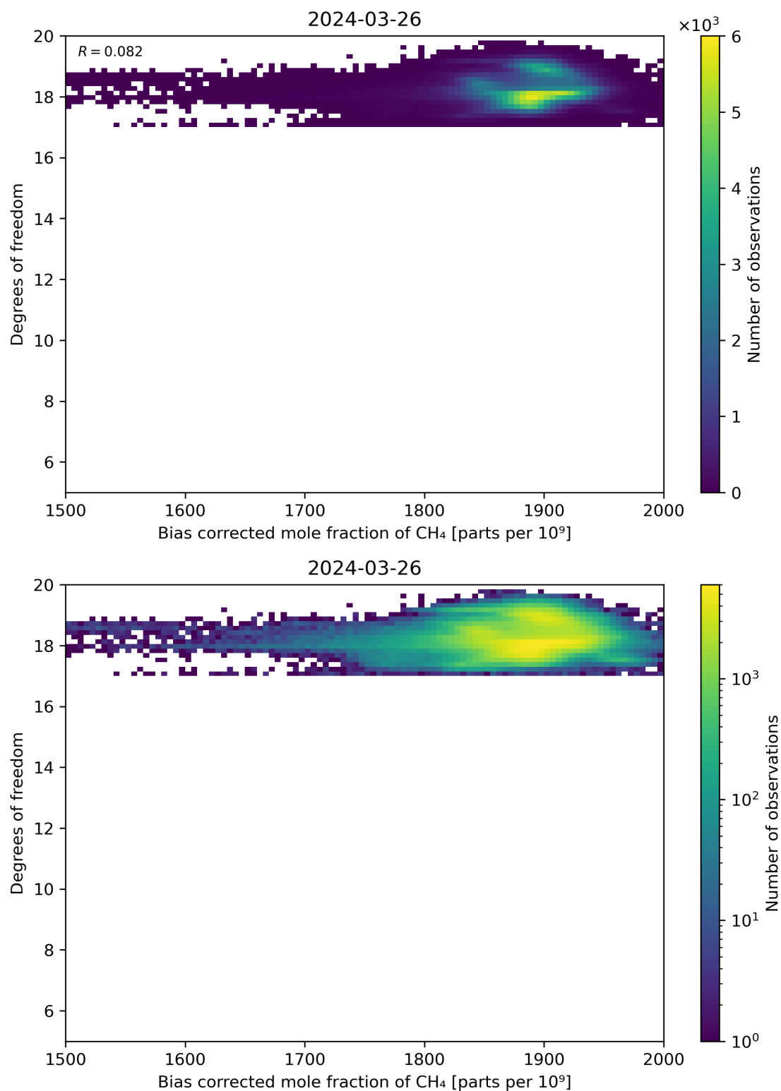
Figure 65: Scatter density plot of “Bias corrected mole fraction of CH 4 ” against “Degrees of freedom” for 2024-03-25 to 2024-03-27.
