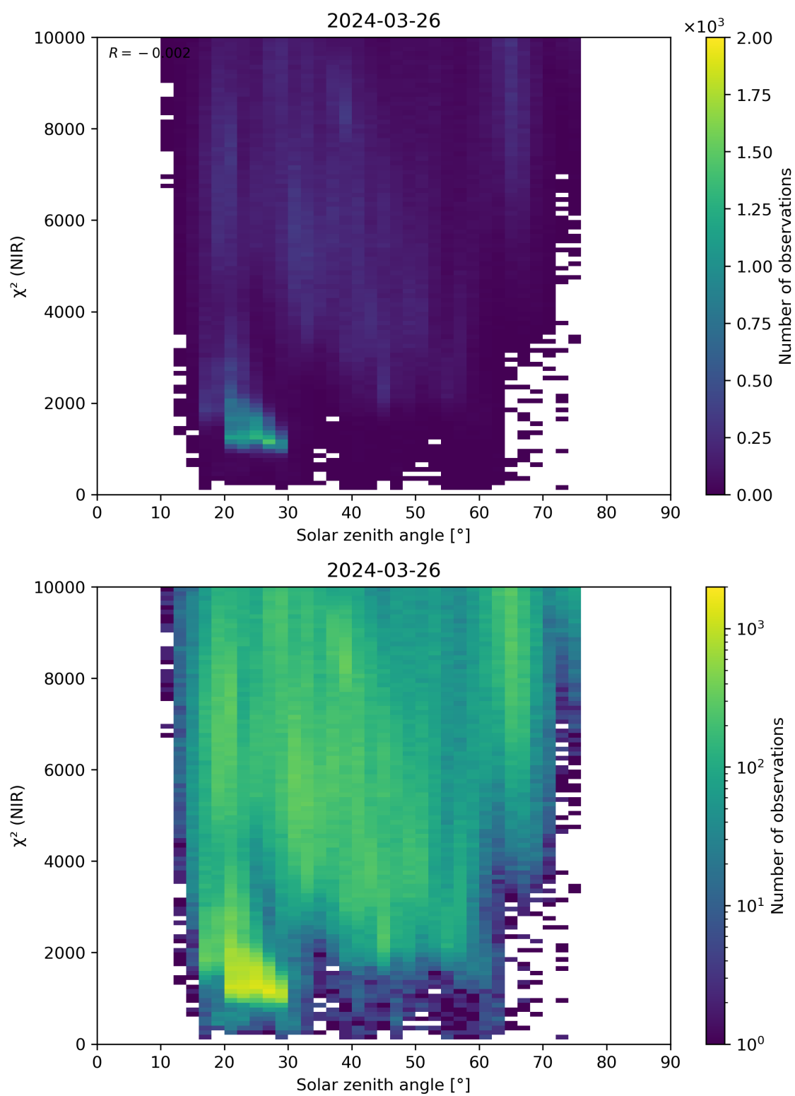
Figure 94: Scatter density plot of “Solar zenith angle” against “ \chi^2 (NIR)” for 2024-03-25 to 2024-03-27.
