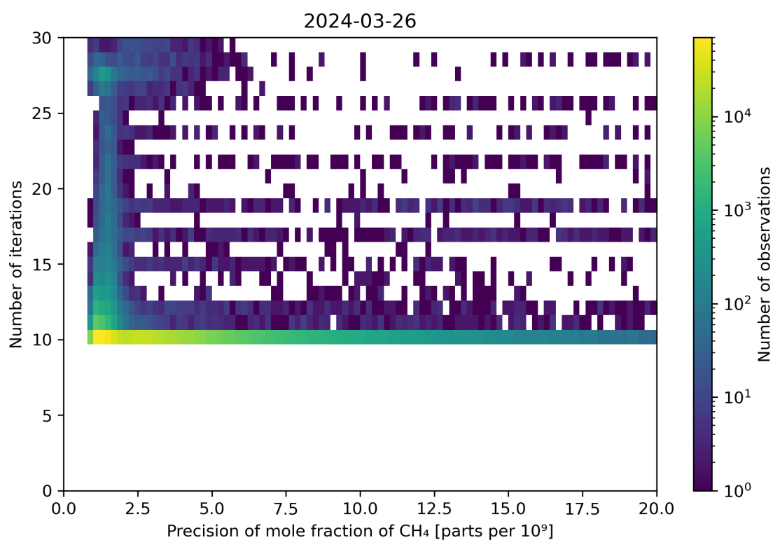
Figure 83: Scatter density plot of “Precision of mole fraction of CH 4 ” against “Number of iterations” for 2024-03-25 to 2024-03-27.
