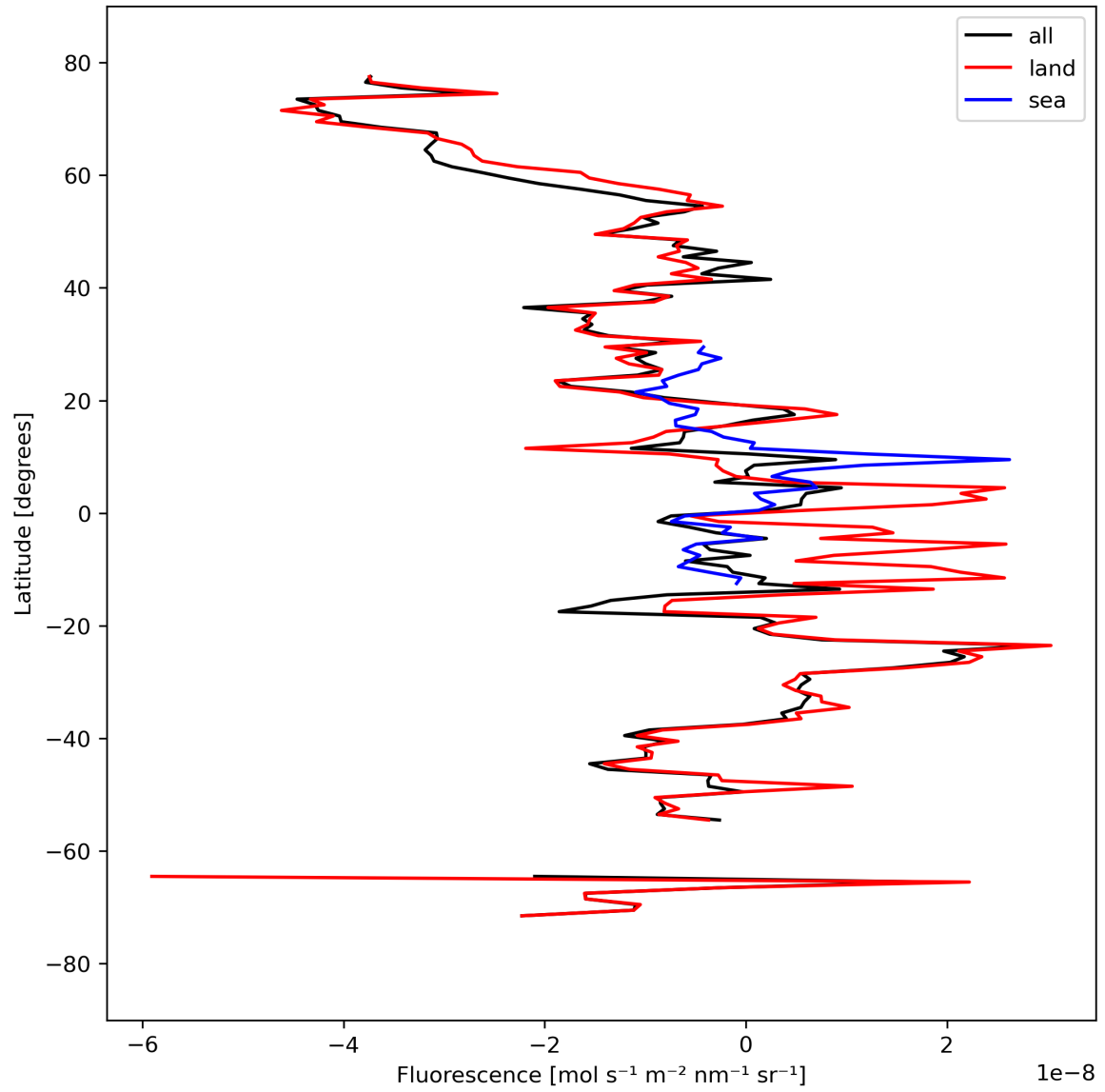
Figure 21: Zonal average of “Fluorescence” for 2024-03-25 to 2024-03-27.
