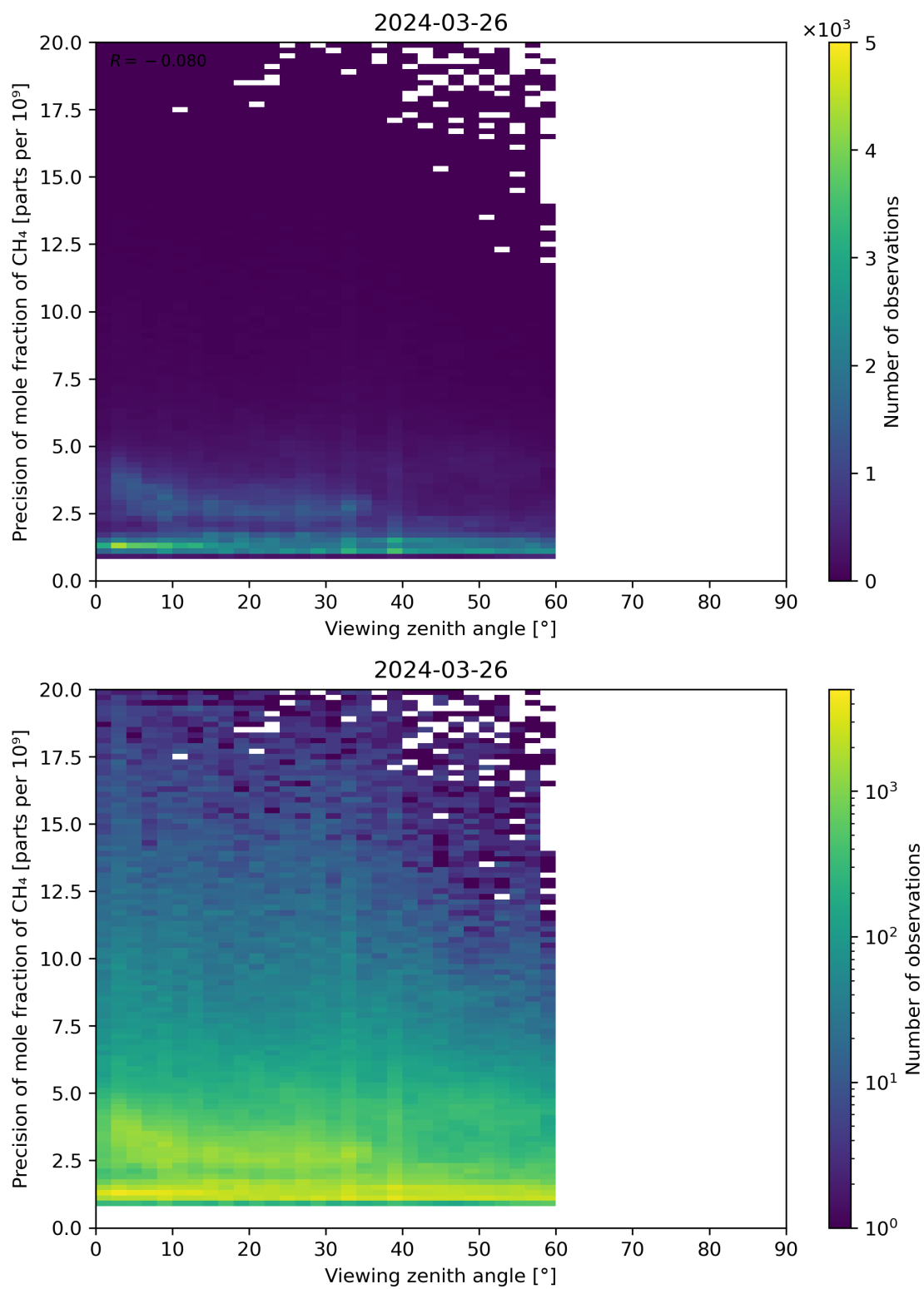
Figure 112: Scatter density plot of “Viewing zenith angle” against “Precision of mole fraction of CH 4 ” for 2024-03-25 to 2024-03-27.
