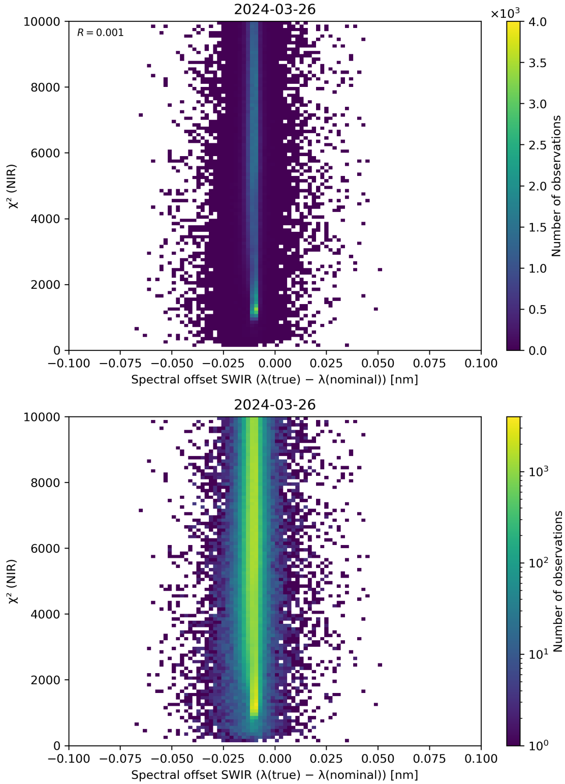
Figure 117: Scatter density plot of “Spectral offset SWIR ( \lambda(\text{true}) - \lambda(\text{nominal}) )” against “ \chi^2 (NIR)” for 2024-03-25 to 2024-03-27.
