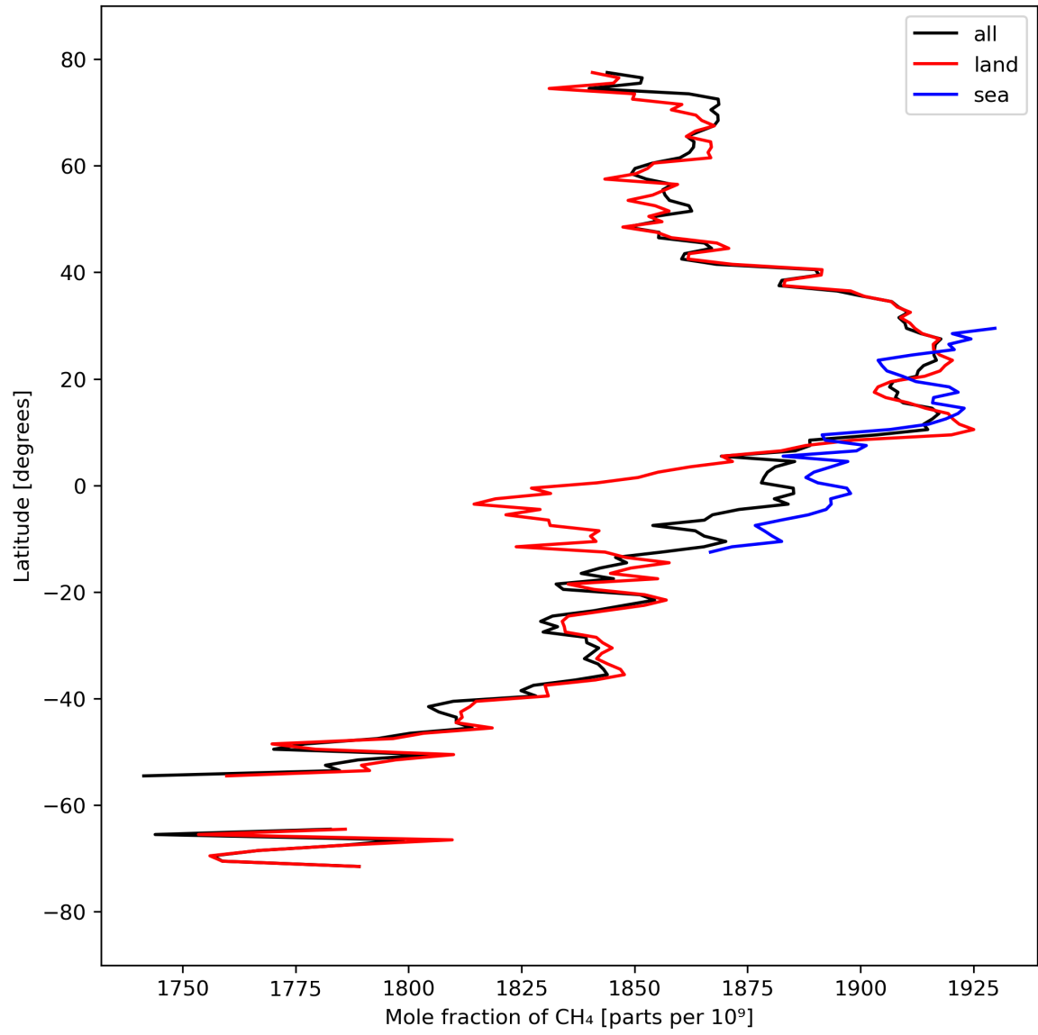
Figure 12: Zonal average of “Mole fraction of CH 4 ” for 2024-03-25 to 2024-03-27.
