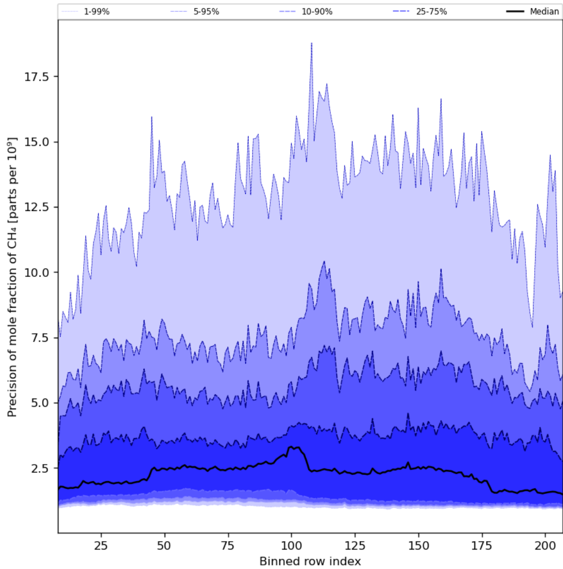
Figure 35: Along track statistics of “Precision of mole fraction of CH 4 ” for 2024-03-25 to 2024-03-27
