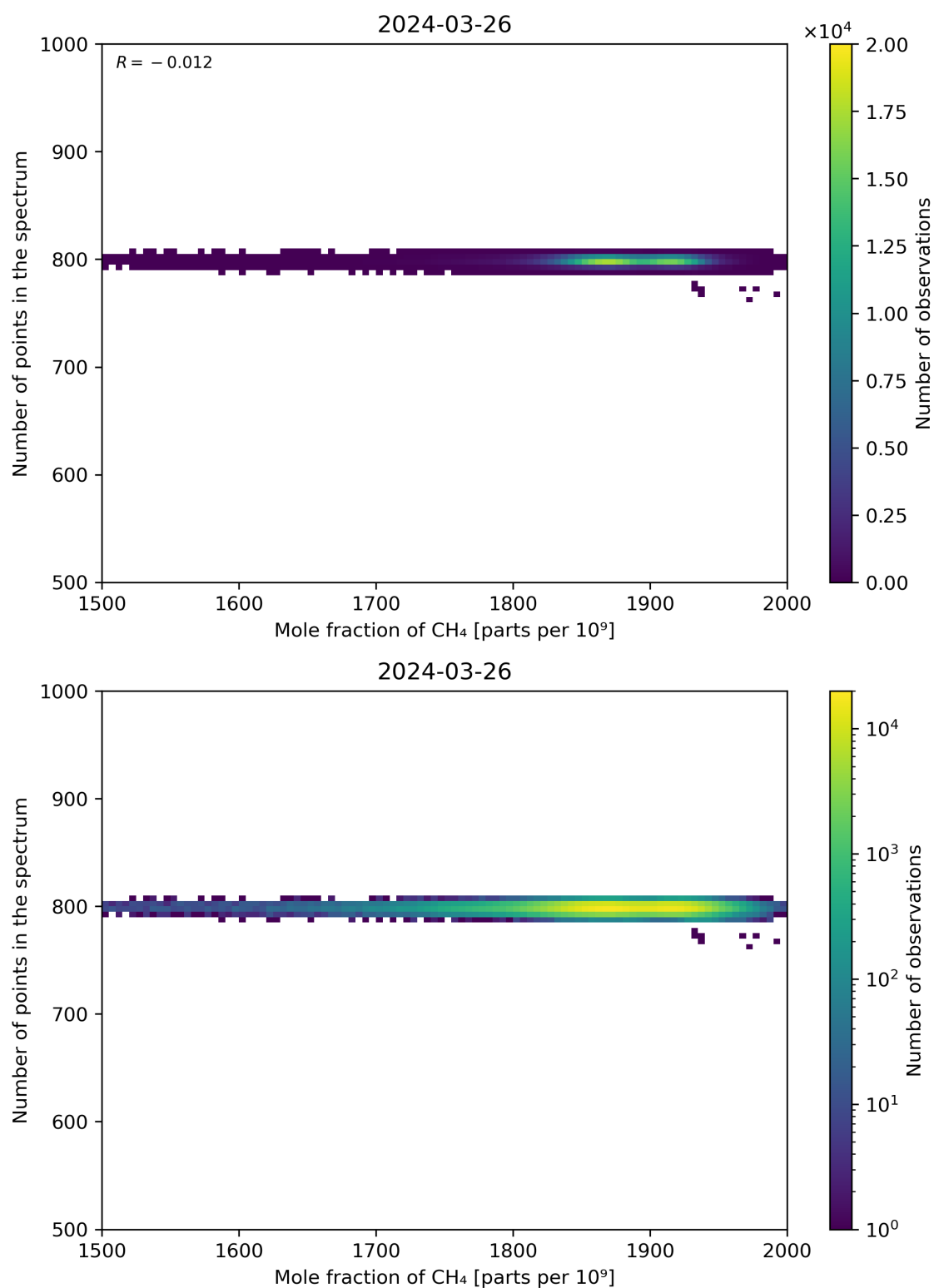
Figure 77: Scatter density plot of “Mole fraction of CH 4 ” against “Number of points in the spectrum” for 2024-03-25 to 2024-03-27.
