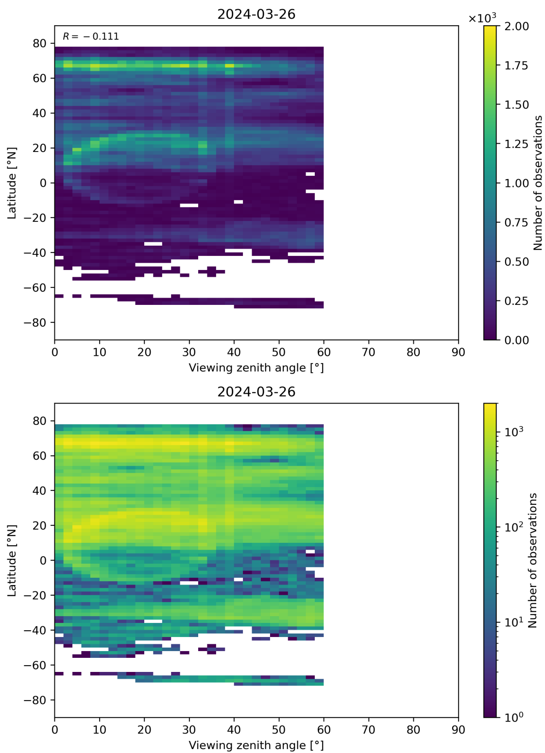
Figure 109: Scatter density plot of “Viewing zenith angle” against “Latitude” for 2024-03-25 to 2024-03-27.
