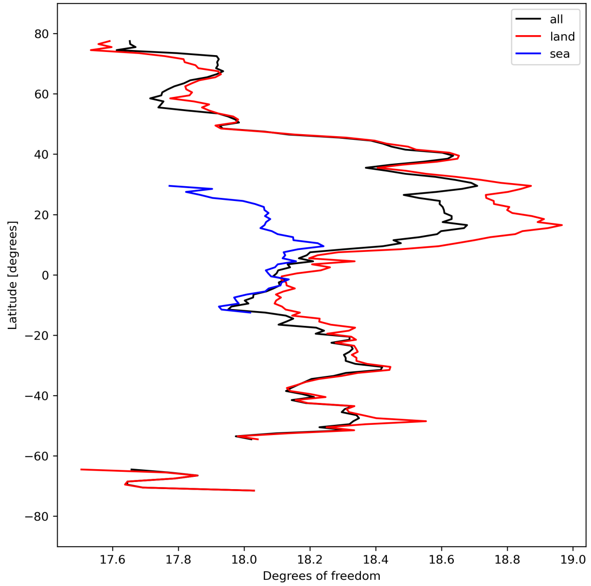
Figure 19: Zonal average of “Degrees of freedom” for 2024-03-25 to 2024-03-27.
