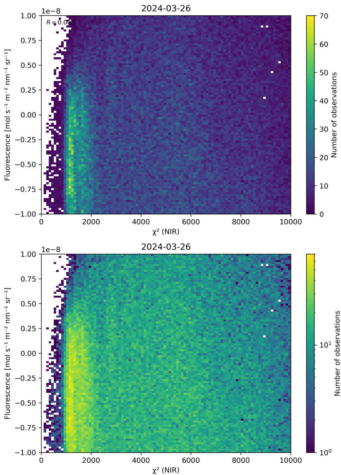
Figure 45: Scatter density plot of “ \chi^2 (NIR)” against “Fluorescence” for 2024-03-25 to 2024-03-27.
