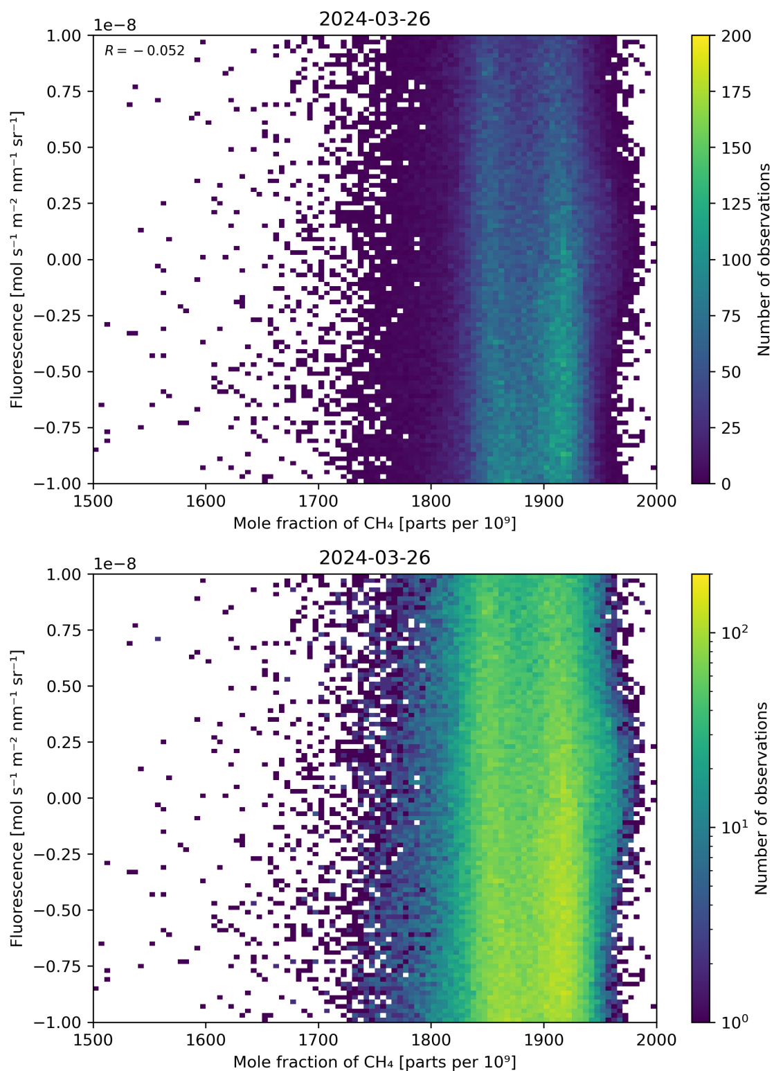
Figure 73: Scatter density plot of “Mole fraction of \text{CH}_4 ” against “Fluorescence” for 2024-03-25 to 2024-03-27.
