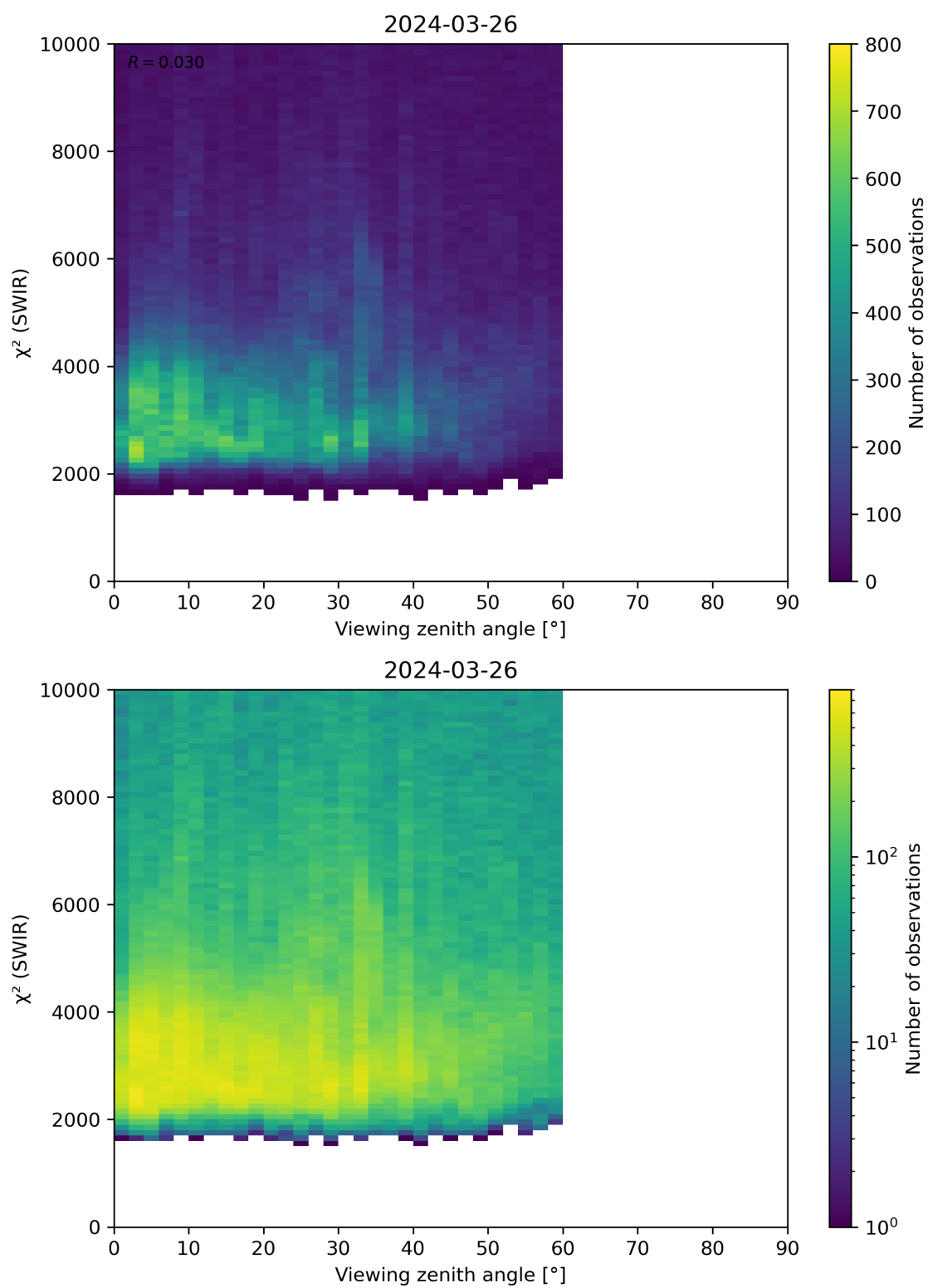
Figure 106: Scatter density plot of “Viewing zenith angle” against “ \chi^2 (SWIR)” for 2024-03-25 to 2024-03-27.
