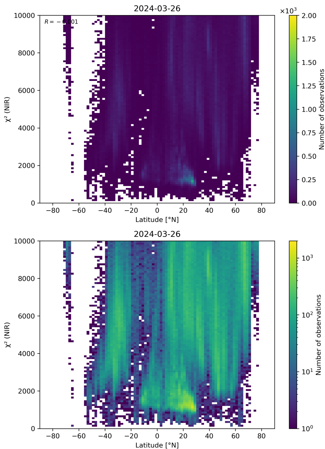
Figure 53: Scatter density plot of “Latitude” against “ \chi^2 (NIR)” for 2024-03-25 to 2024-03-27.
