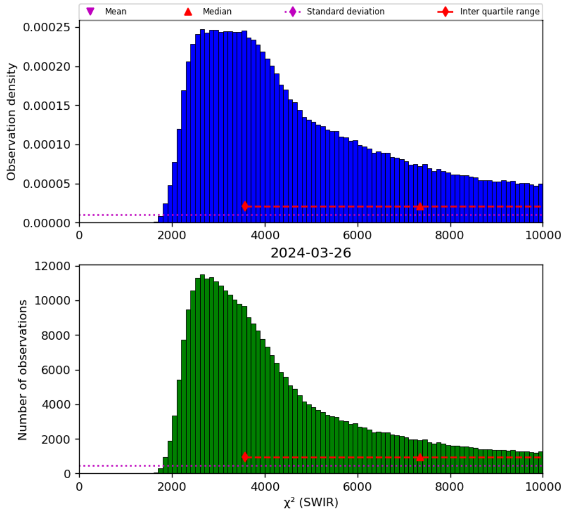
Figure 28: Histogram of “ \chi^2 (SWIR)” for 2024-03-25 to 2024-03-27
