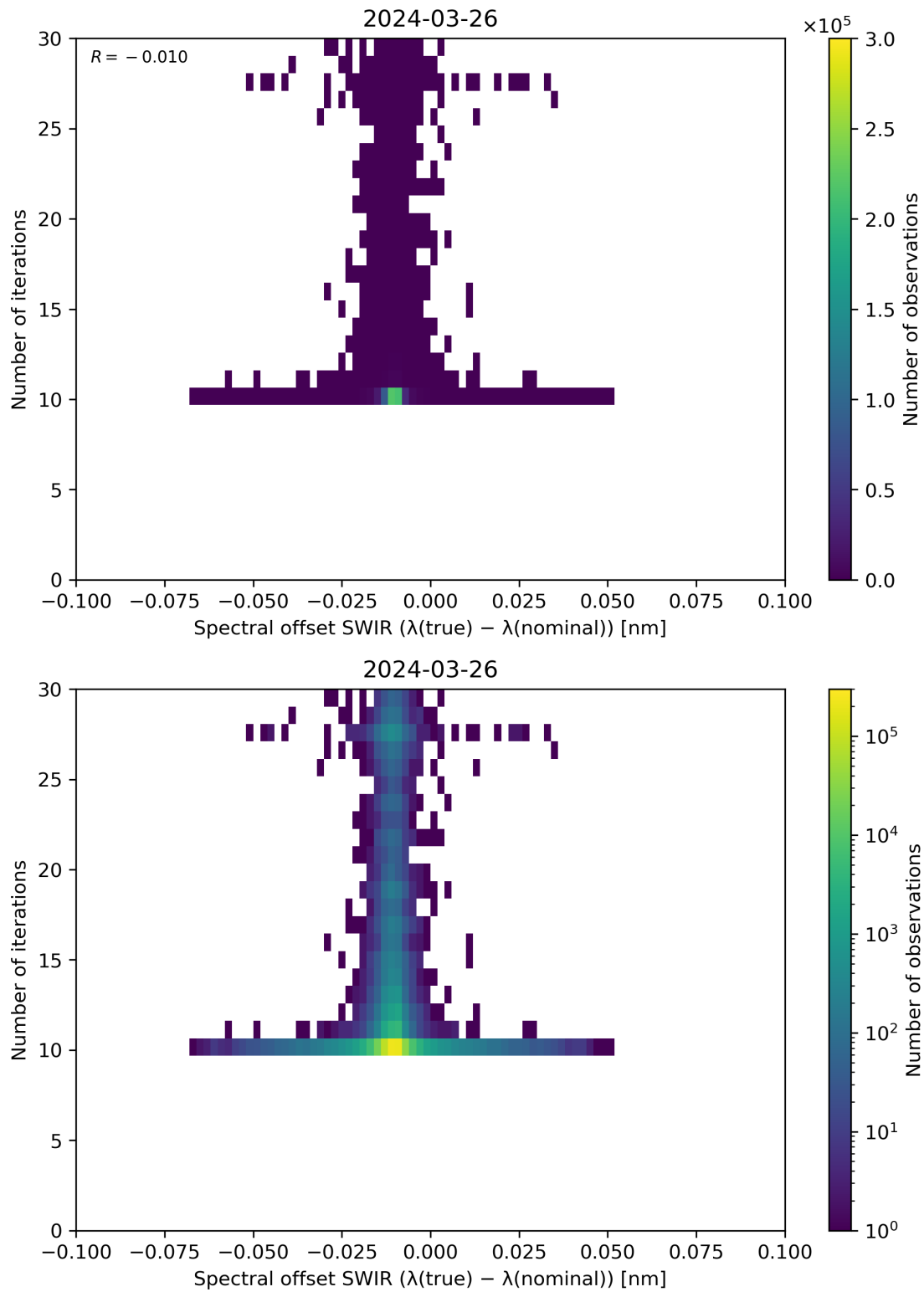
Figure 121: Scatter density plot of “Spectral offset SWIR ( \lambda(\text{true}) - \lambda(\text{nominal}) )” against “Number of iterations” for 2024-03-25 to 2024-03-27.
