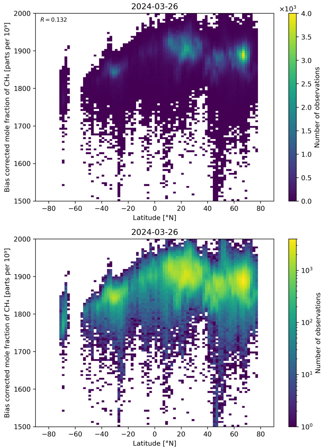
Figure 58: Scatter density plot of “Latitude” against “Bias corrected mole fraction of CH 4 ” for 2024-03-25 to 2024-03-27.
