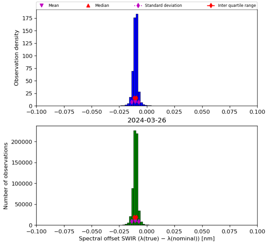
Figure 27: Histogram of “Spectral offset SWIR ( \lambda(\text{true}) - \lambda(\text{nominal}) )” for 2024-03-25 to 2024-03-27
