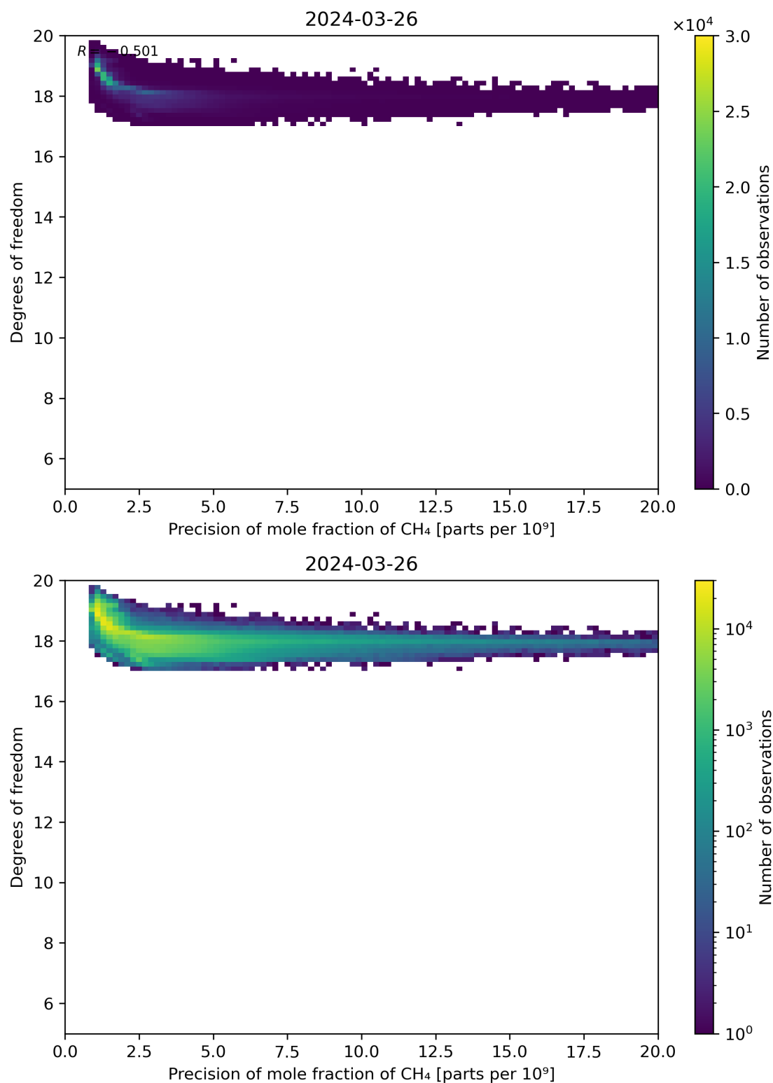
Figure 80: Scatter density plot of “Precision of mole fraction of CH 4 ” against “Degrees of freedom” for 2024-03-25 to 2024-03-27.
