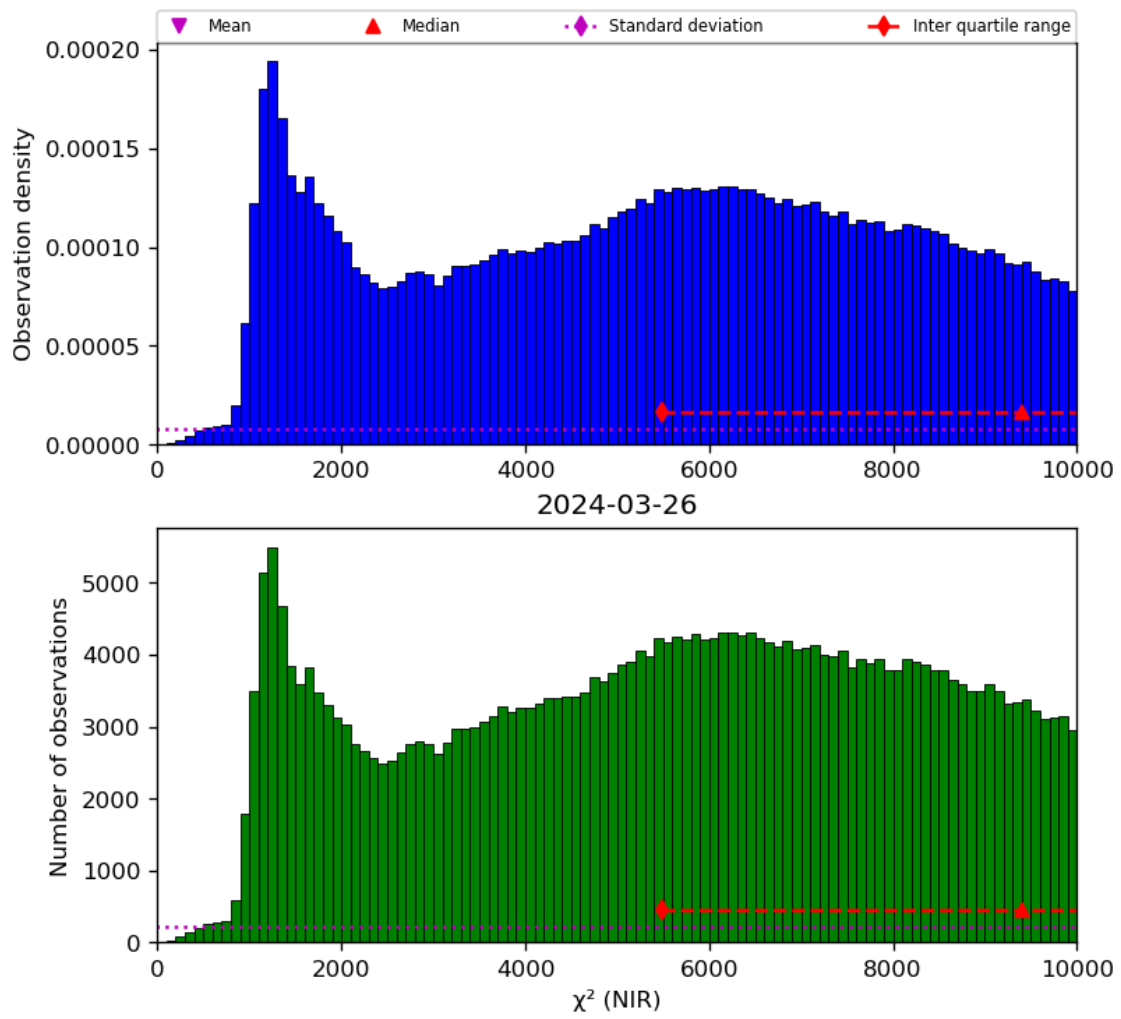
Figure 29: Histogram of “ \chi^2 (NIR)” for 2024-03-25 to 2024-03-27
