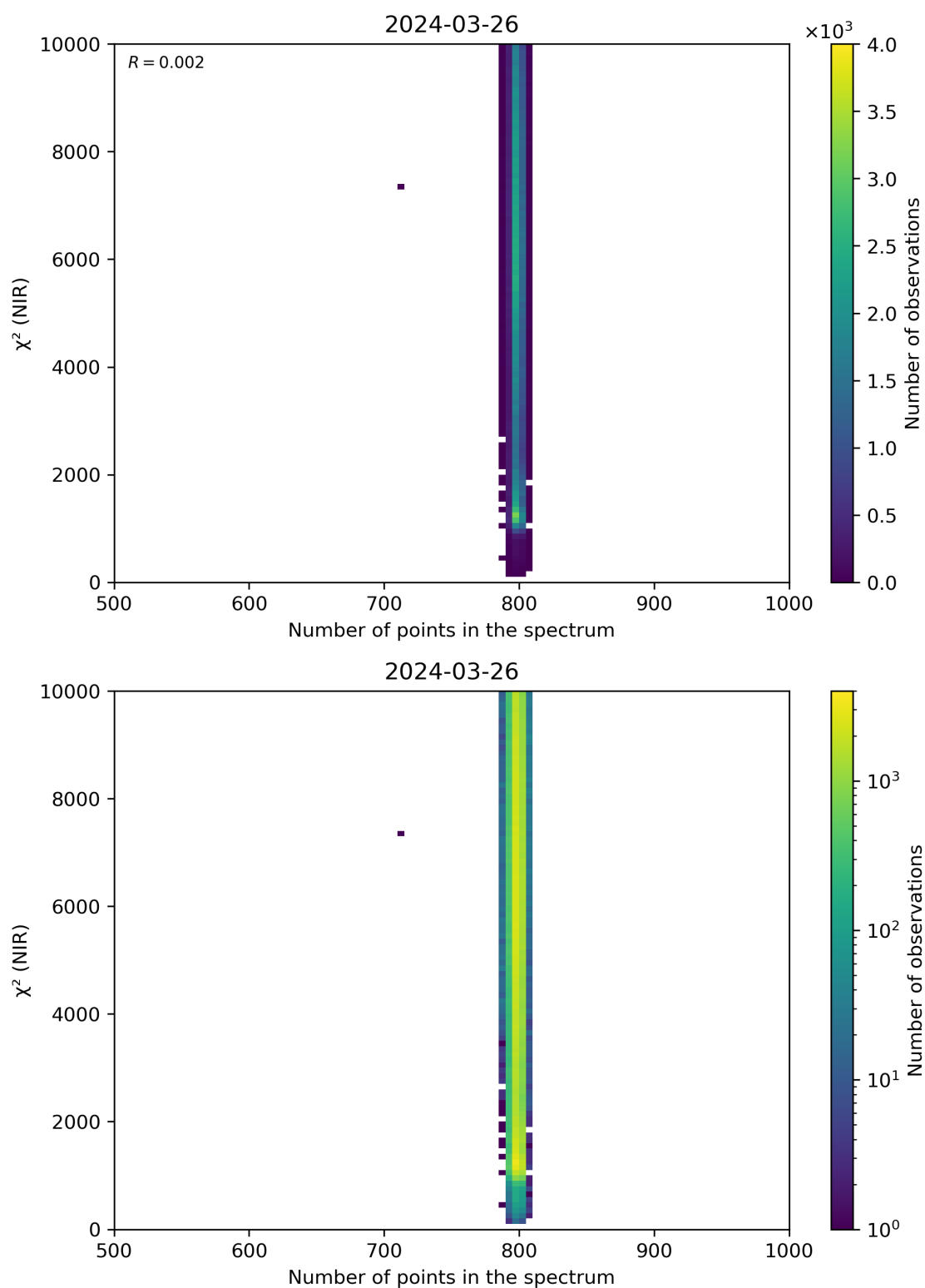
Figure 88: Scatter density plot of “Number of points in the spectrum” against “ \chi^2 (NIR)” for 2024-03-25 to 2024-03-27.
