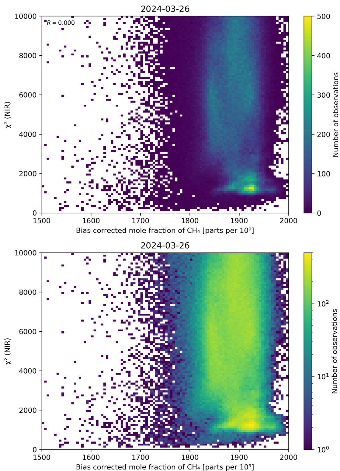
Figure 63: Scatter density plot of “Bias corrected mole fraction of CH 4 ” against “ \chi^2 (NIR)” for 2024-03-25 to 2024-03-27.
