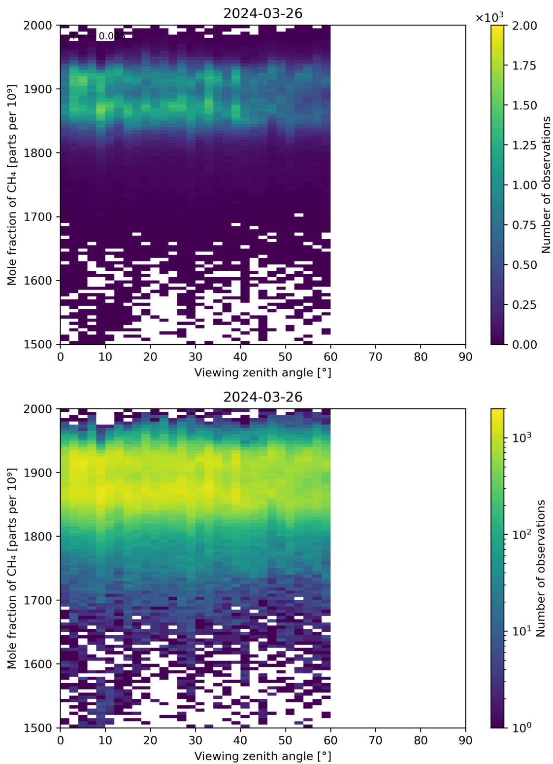
Figure 110: Scatter density plot of “Viewing zenith angle” against “Mole fraction of CH 4 ” for 2024-03-25 to 2024-03-27.
