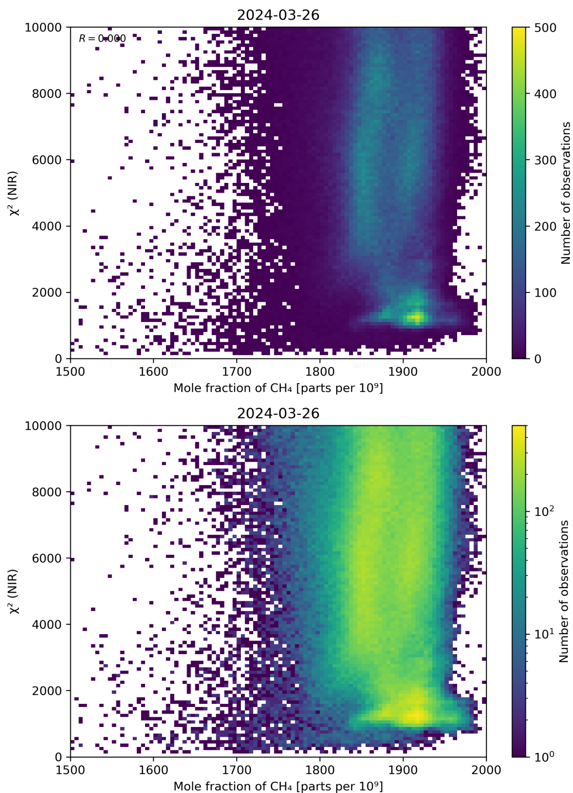
Figure 70: Scatter density plot of “Mole fraction of \text{CH}_4 ” against “ \chi^2 (NIR)” for 2024-03-25 to 2024-03-27.
