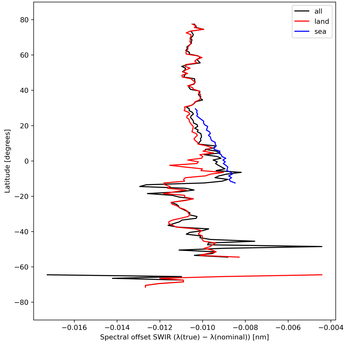
Figure 16: Zonal average of “Spectral offset SWIR ( \lambda(\text{true}) - \lambda(\text{nominal}) )” for 2024-03-25 to 2024-03-27.
