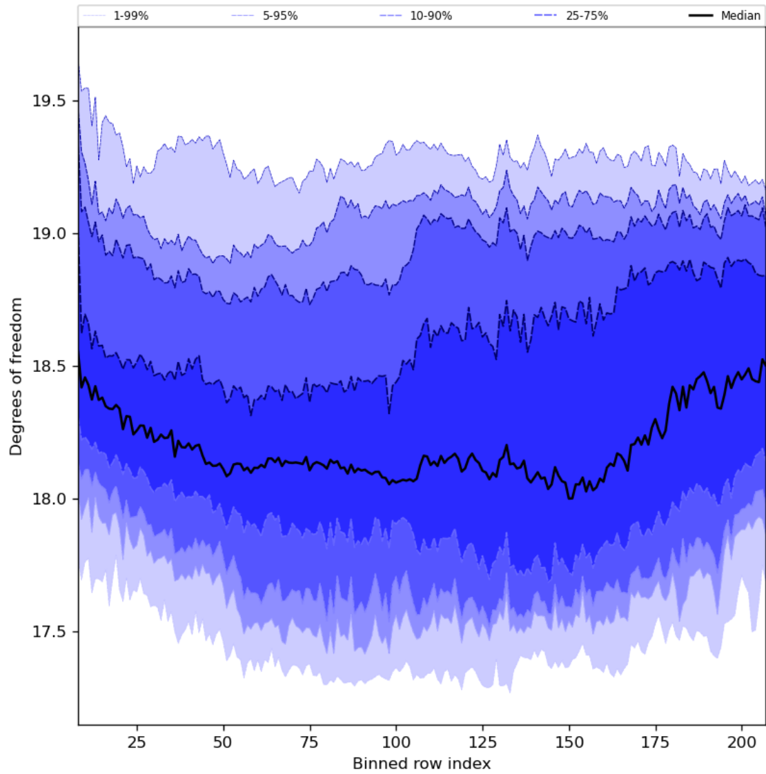
Figure 41: Along track statistics of “Degrees of freedom” for 2024-03-25 to 2024-03-27
