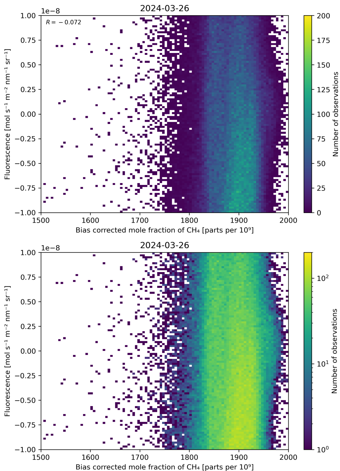
Figure 66: Scatter density plot of “Bias corrected mole fraction of \text{CH}_4 ” against “Fluorescence” for 2024-03-25 to 2024-03-27.
