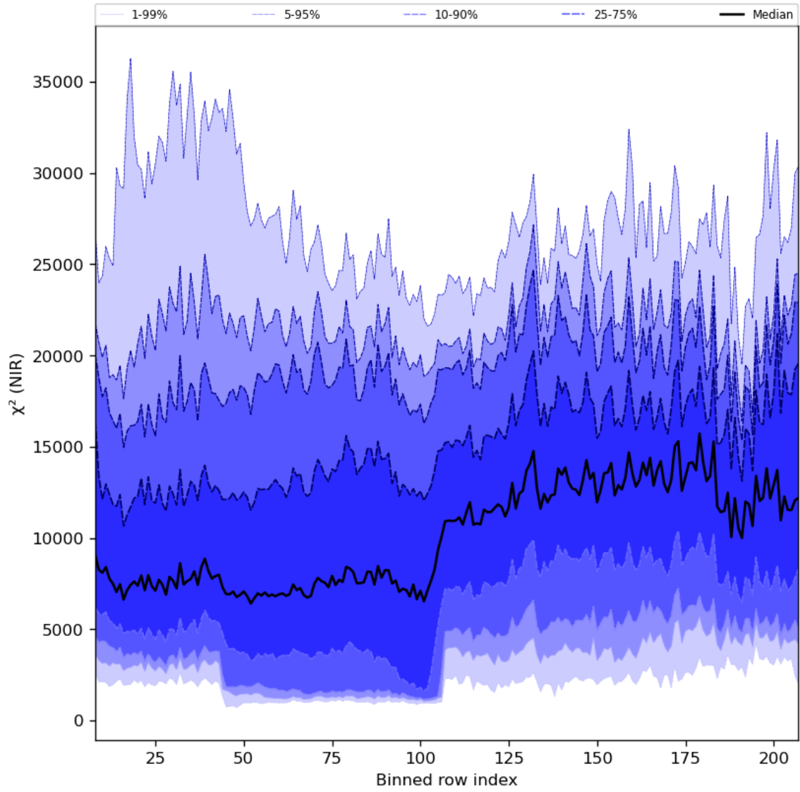
Figure 40: Along track statistics of “ \chi^2 (NIR)” for 2024-03-25 to 2024-03-27
