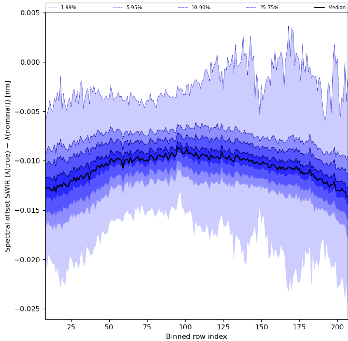
Figure 38: Along track statistics of “Spectral offset SWIR ( \lambda(\text{true}) - \lambda(\text{nominal}) )” for 2024-03-25 to 2024-03-27
