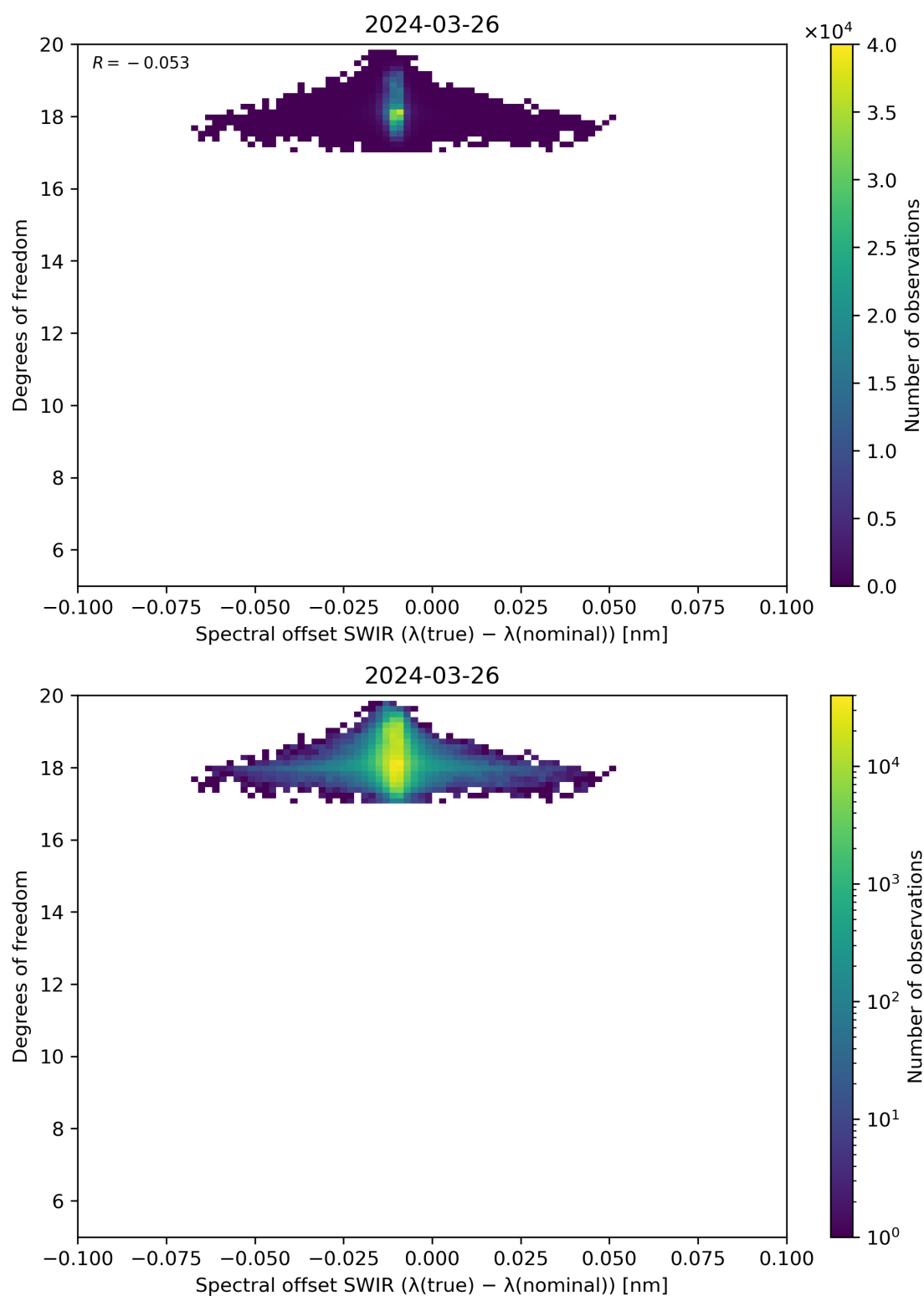
Figure 119: Scatter density plot of “Spectral offset SWIR ( \lambda(\text{true}) - \lambda(\text{nominal}) )” against “Degrees of freedom” for 2024-03-25 to 2024-03-27.
