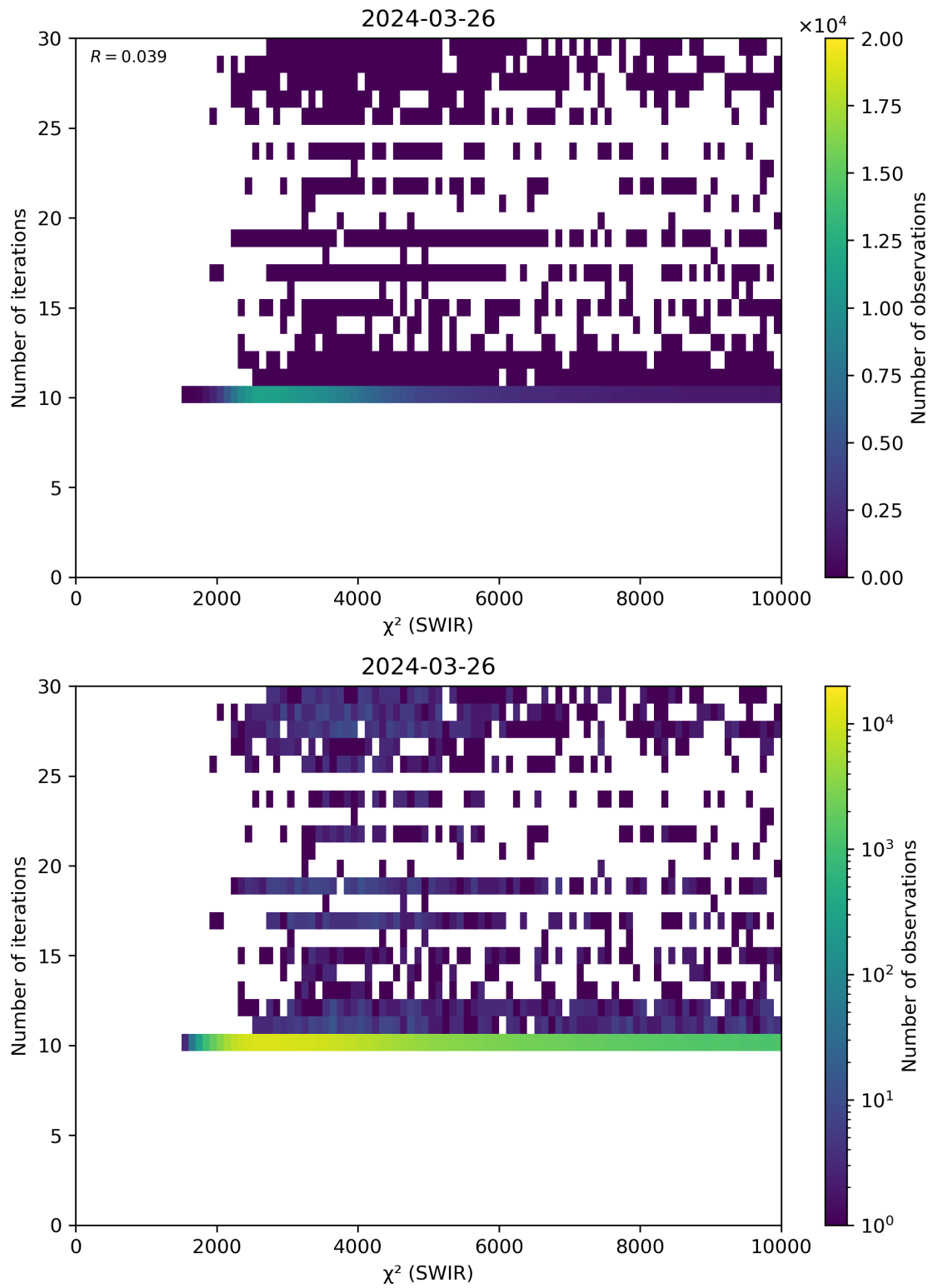
Figure 50: Scatter density plot of “ \chi^2 (SWIR)” against “Number of iterations” for 2024-03-25 to 2024-03-27.
