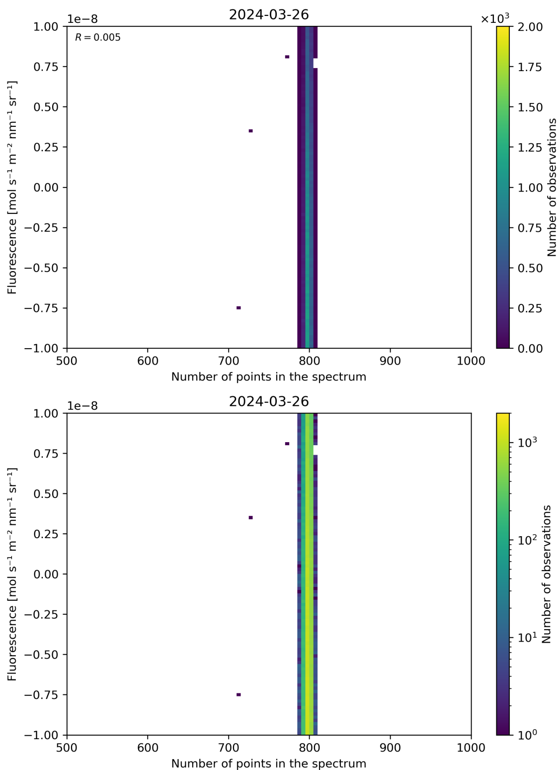
Figure 91: Scatter density plot of “Number of points in the spectrum” against “Fluorescence” for 2024-03-25 to 2024-03-27.
