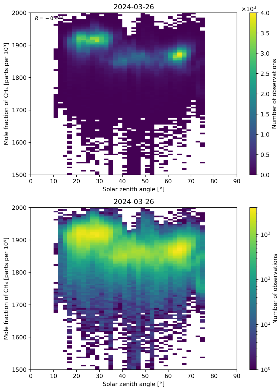
Figure 99: Scatter density plot of “Solar zenith angle” against “Mole fraction of CH 4 ” for 2024-03-25 to 2024-03-27.
