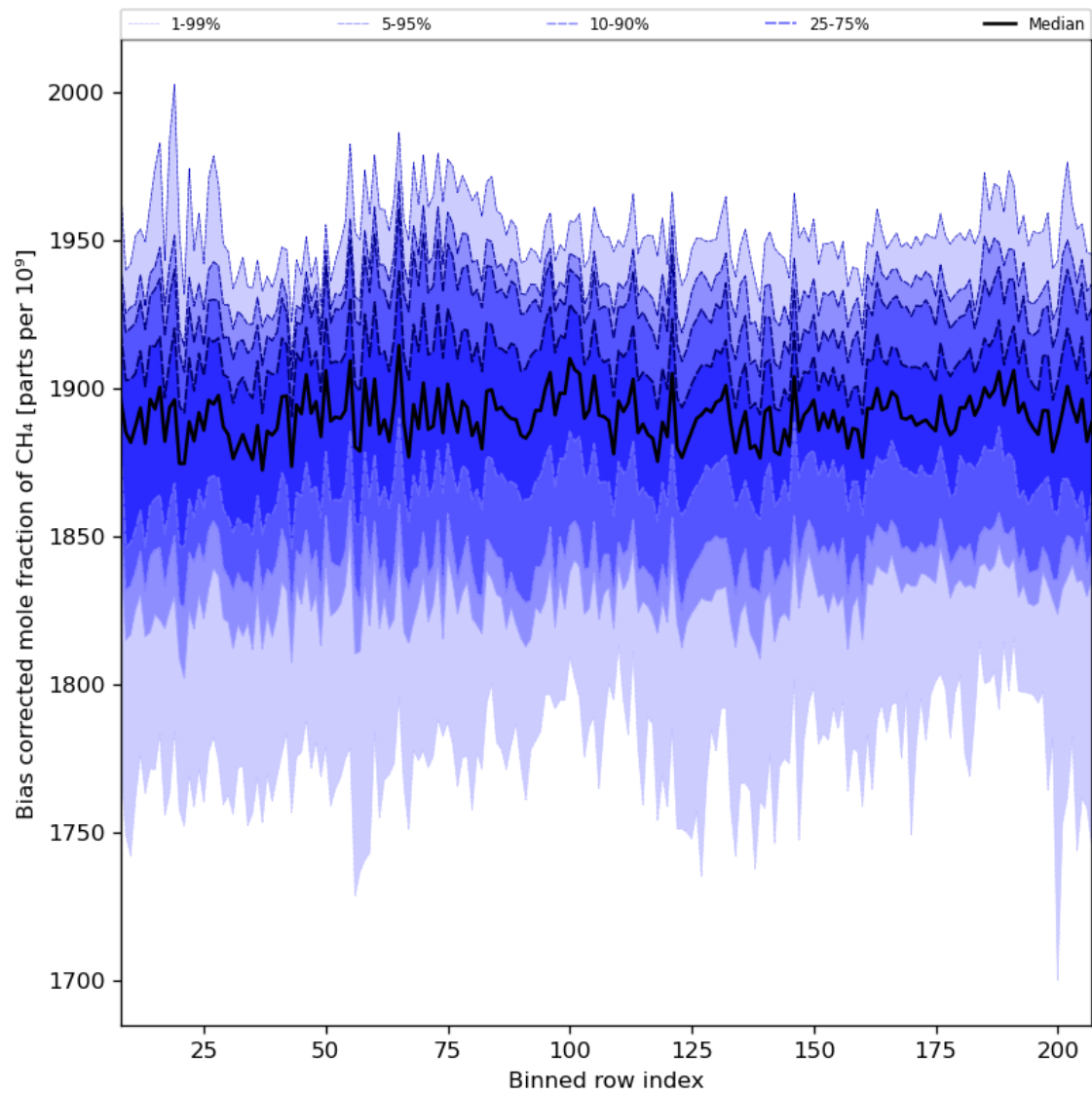
Figure 36: Along track statistics of “Bias corrected mole fraction of CH 4 ” for 2024-03-25 to 2024-03-27
