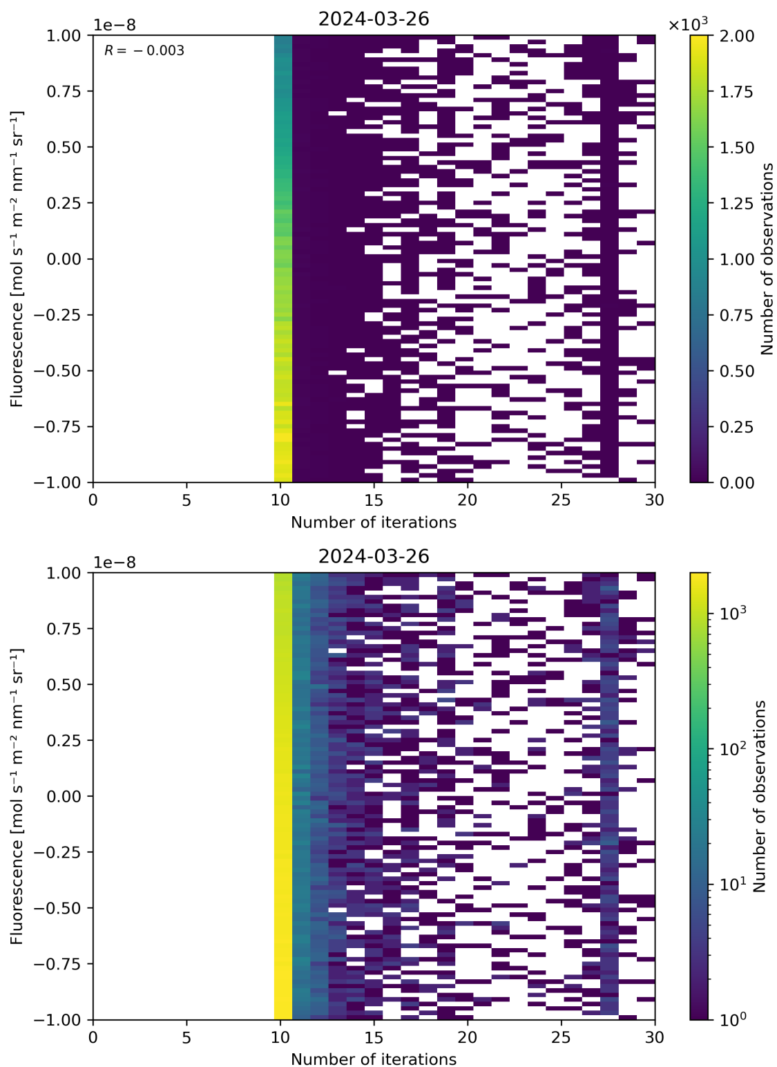
Figure 87: Scatter density plot of “Number of iterations” against “Fluorescence” for 2024-03-25 to 2024-03-27.
