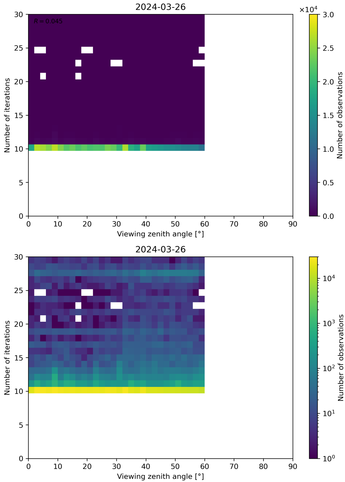
Figure 113: Scatter density plot of “Viewing zenith angle” against “Number of iterations” for 2024-03-25 to 2024-03-27.
