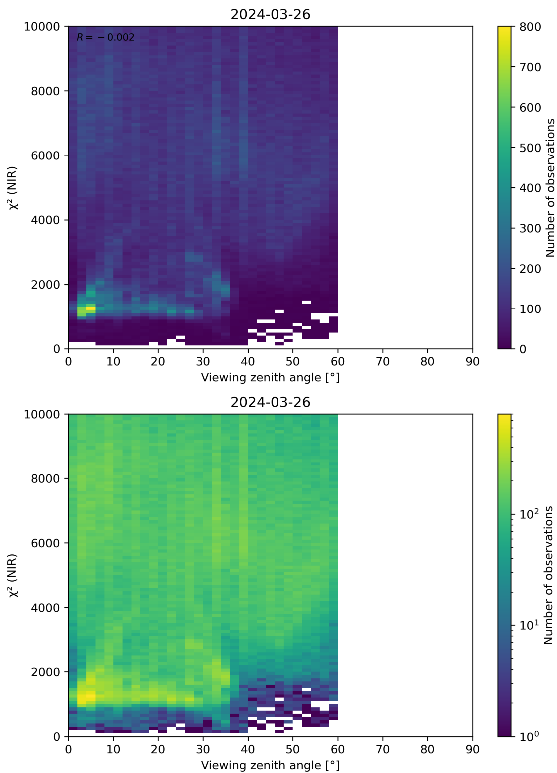
Figure 105: Scatter density plot of “Viewing zenith angle” against “ \chi^2 (NIR)” for 2024-03-25 to 2024-03-27.
