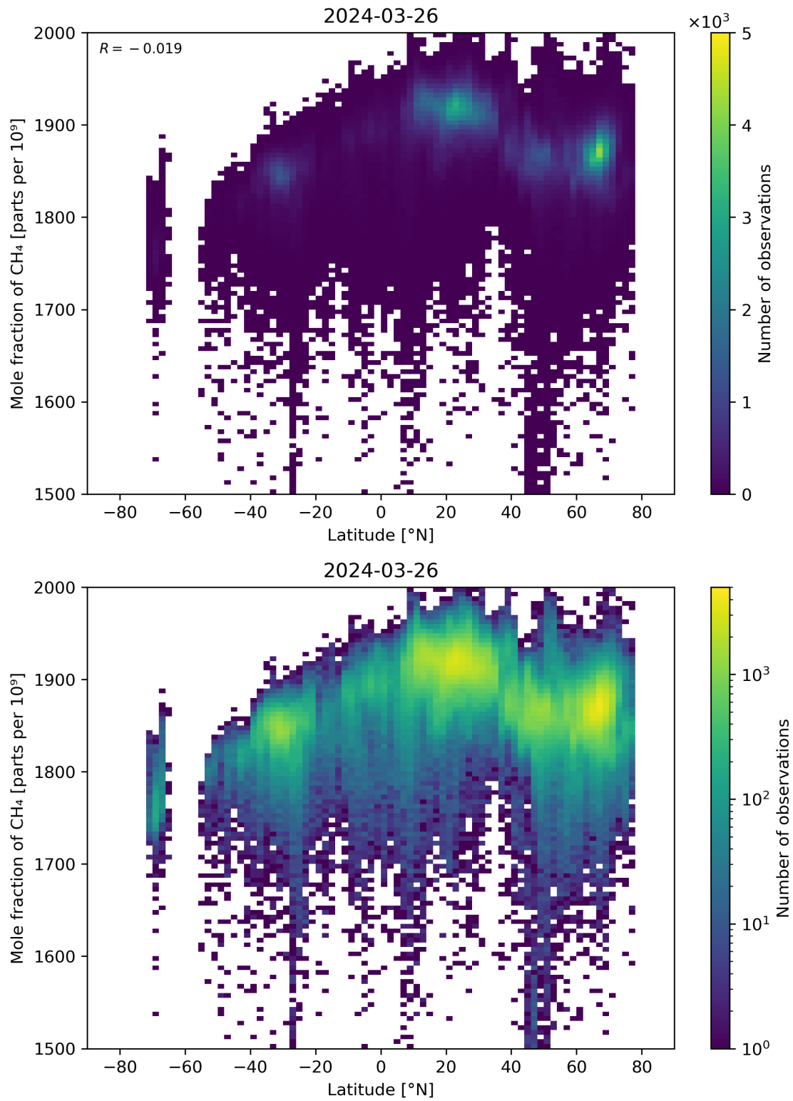
Figure 57: Scatter density plot of “Latitude” against “Mole fraction of CH 4 ” for 2024-03-25 to 2024-03-27.
