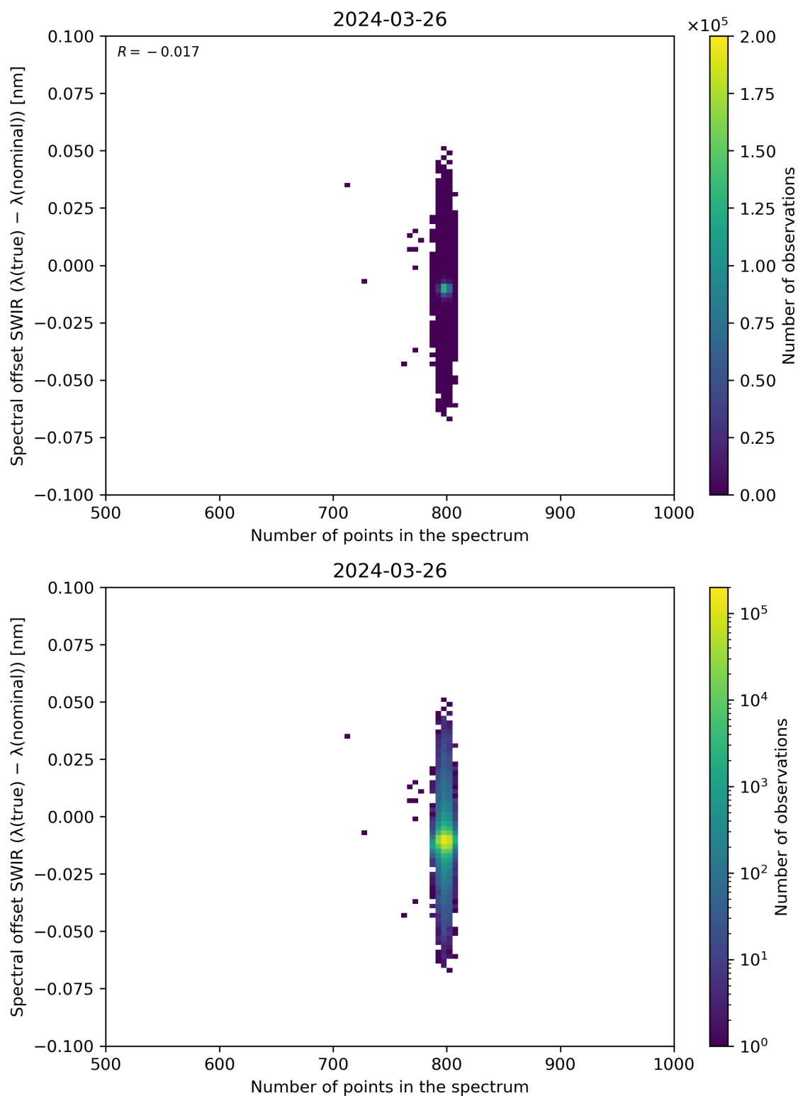
Figure 93: Scatter density plot of “Number of points in the spectrum” against “Spectral offset SWIR ( \lambda(\text{true}) - \lambda(\text{nominal}) )” for 2024-03-25 to 2024-03-27.
