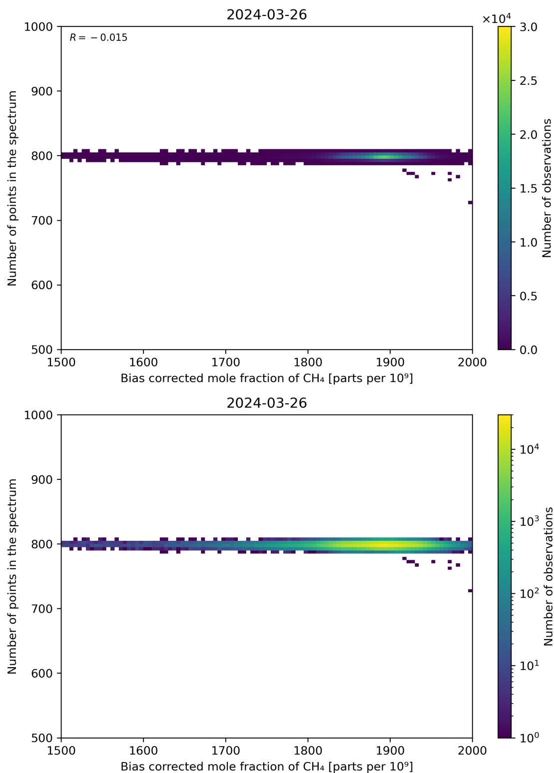
Figure 68: Scatter density plot of “Bias corrected mole fraction of CH 4 ” against “Number of points in the spectrum” for 2024-03-25 to 2024-03-27.
