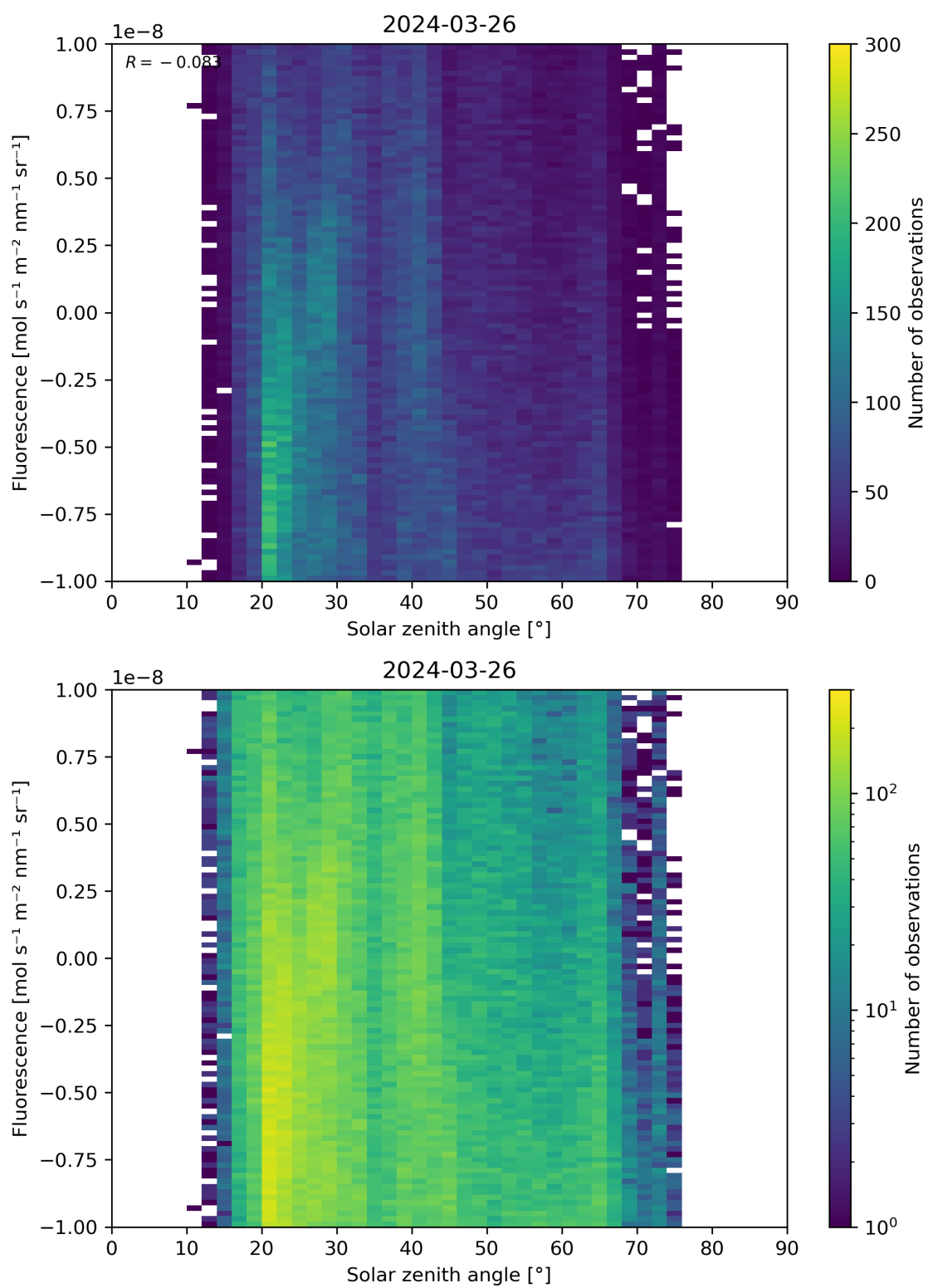
Figure 97: Scatter density plot of “Solar zenith angle” against “Fluorescence” for 2024-03-25 to 2024-03-27.
