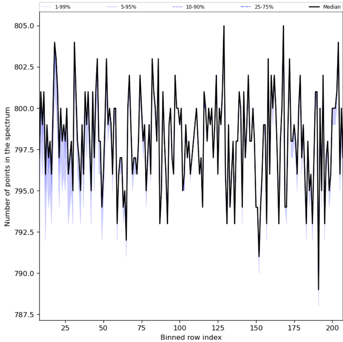
Figure 37: Along track statistics of “Number of points in the spectrum” for 2024-03-25 to 2024-03-27
