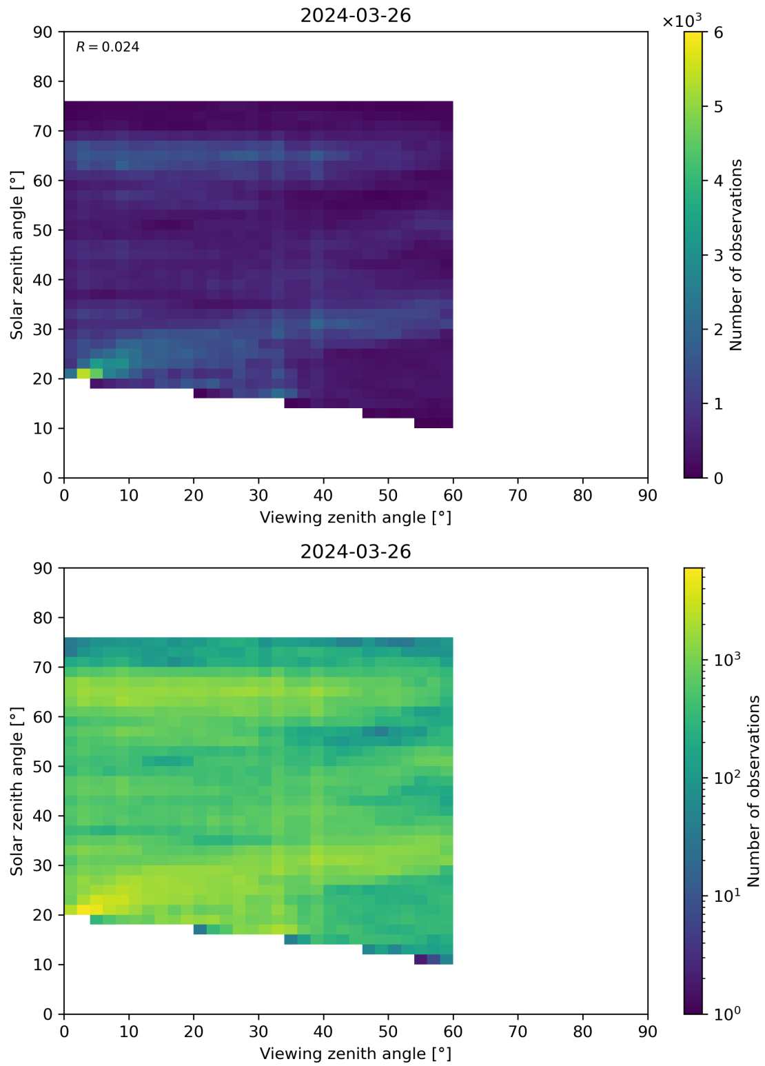
Figure 115: Scatter density plot of “Viewing zenith angle” against “Solar zenith angle” for 2024-03-25 to 2024-03-27.
