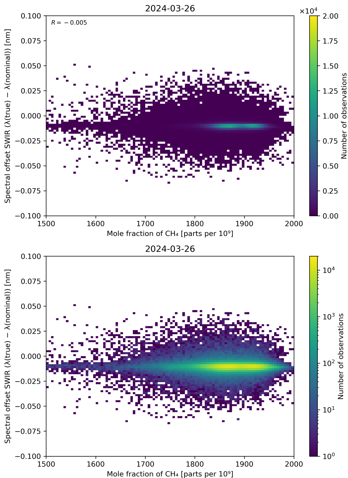
Figure 86: Scatter density plot of “Mole fraction of CH 4 ” against “Spectral offset SWIR ( \lambda(\text{true}) - \lambda(\text{nominal}) )” for 2024-03-25 to 2024-03-27.
