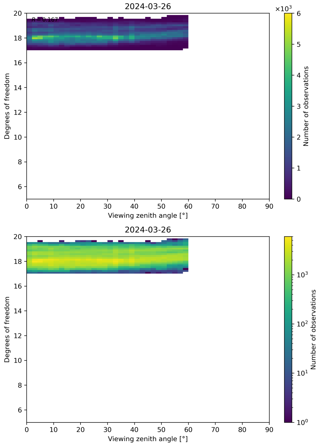
Figure 107: Scatter density plot of “Viewing zenith angle” against “Degrees of freedom” for 2024-03-25 to 2024-03-27.
