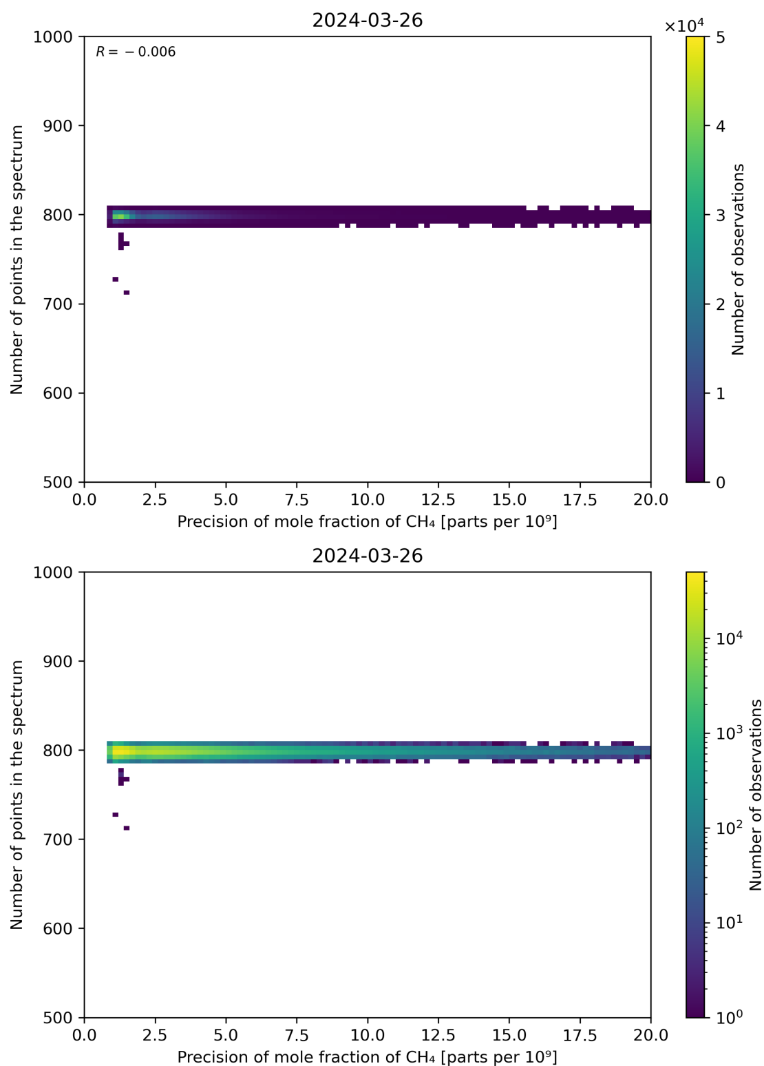
Figure 84: Scatter density plot of “Precision of mole fraction of CH 4 ” against “Number of points in the spectrum” for 2024-03-25 to 2024-03-27.
