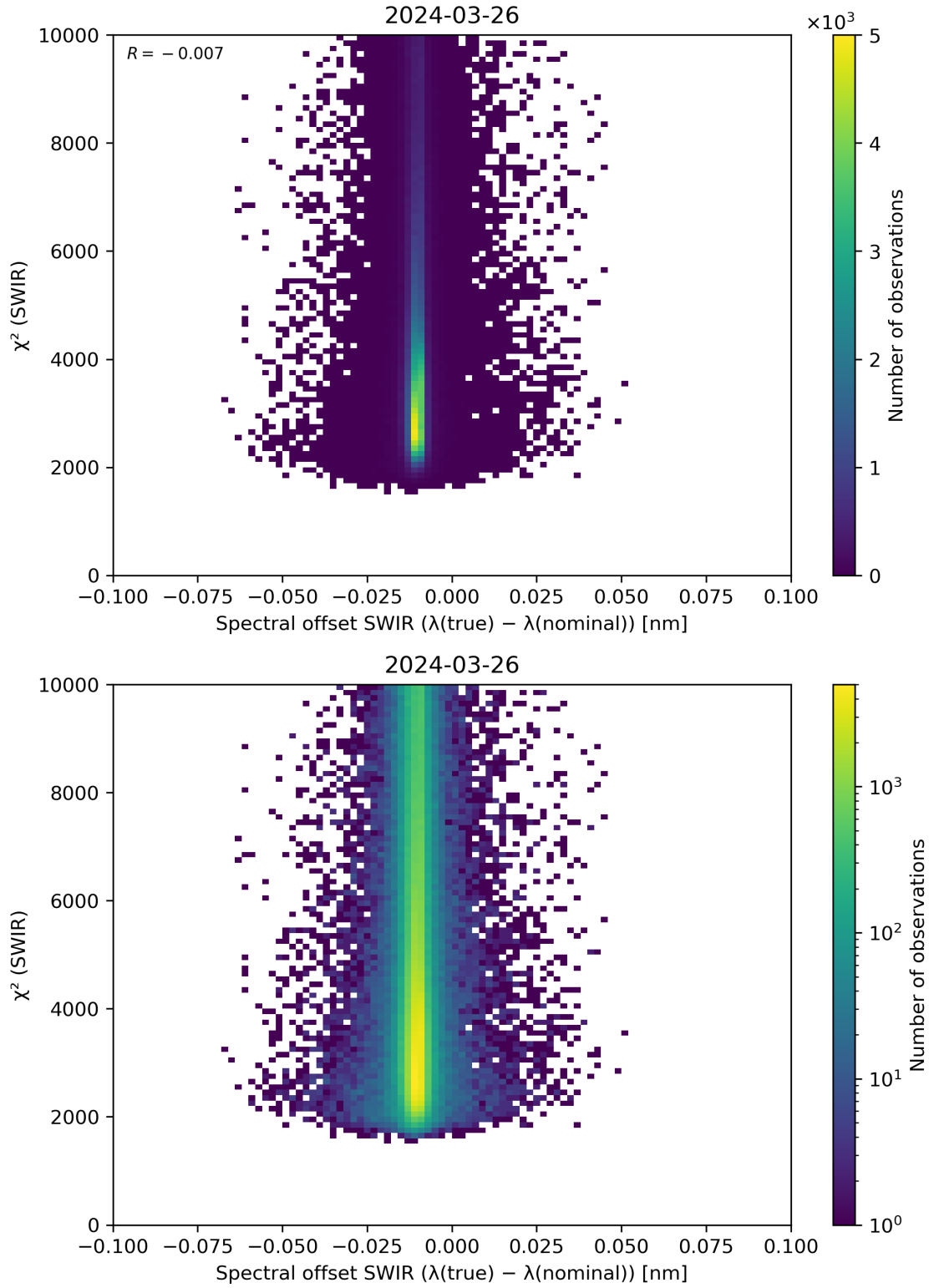
Figure 118: Scatter density plot of “Spectral offset SWIR ( \lambda(\text{true}) - \lambda(\text{nominal}) )” against “ \chi^2 (SWIR)” for 2024-03-25 to 2024-03-27.
