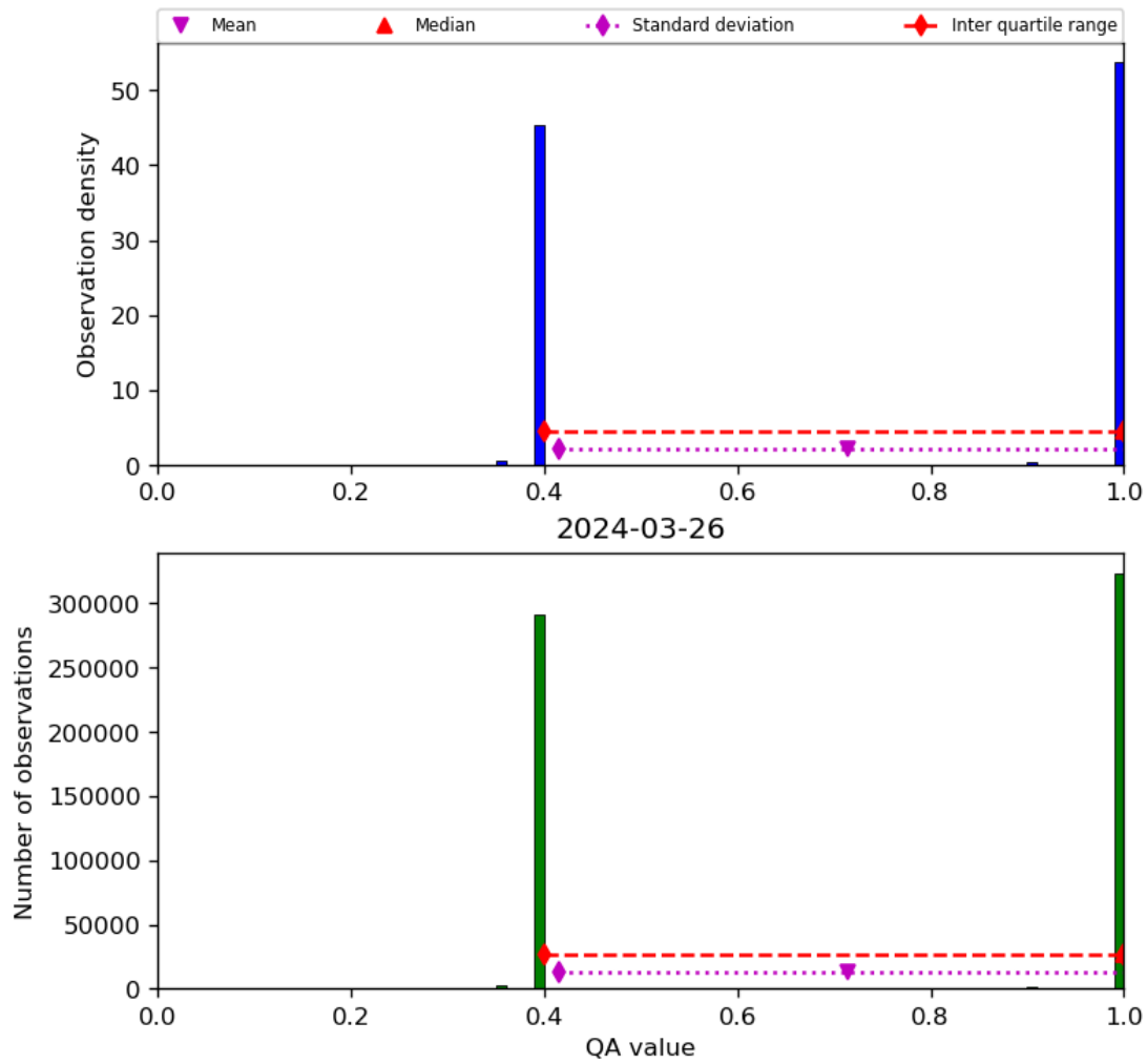
Figure 22: Histogram of “QA value” for 2024-03-25 to 2024-03-27
