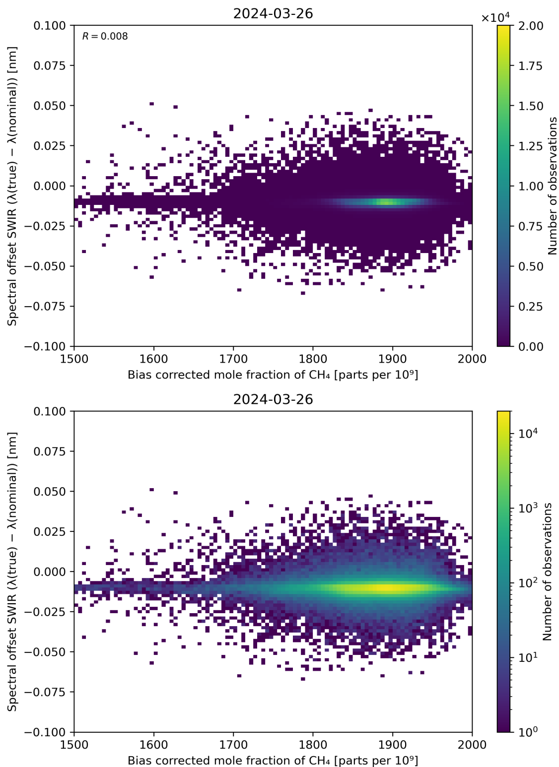
Figure 69: Scatter density plot of “Bias corrected mole fraction of \text{CH}_4 ” against “Spectral offset SWIR ( \lambda(\text{true}) - \lambda(\text{nominal}) )” for 2024-03-25 to 2024-03-27.
