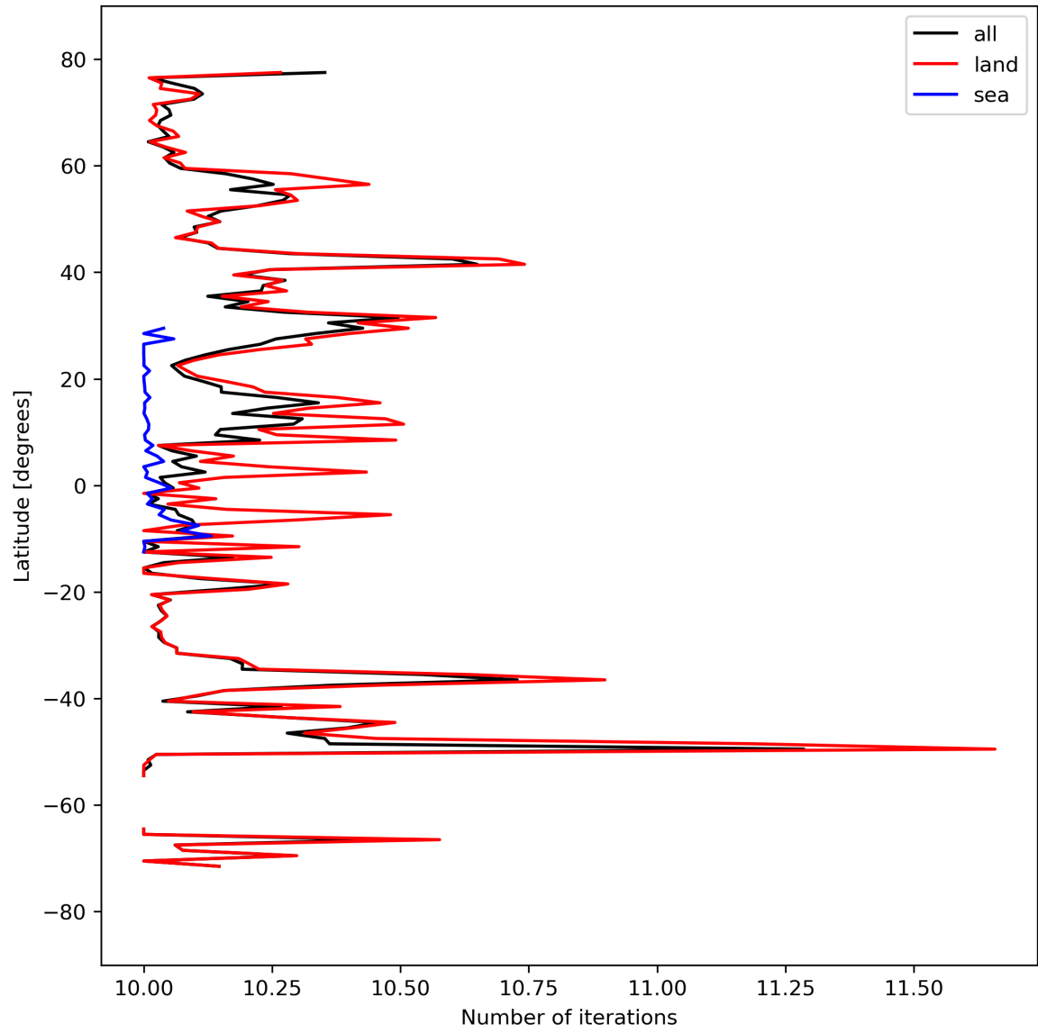
Figure 20: Zonal average of “Number of iterations” for 2024-03-25 to 2024-03-27.
