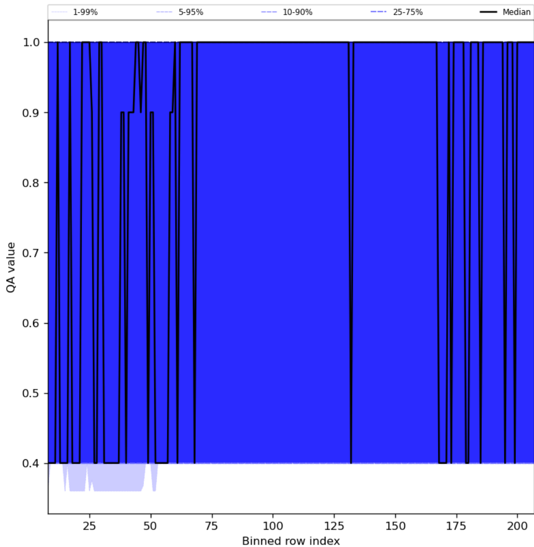
Figure 33: Along track statistics of “QA value” for 2024-03-25 to 2024-03-27
