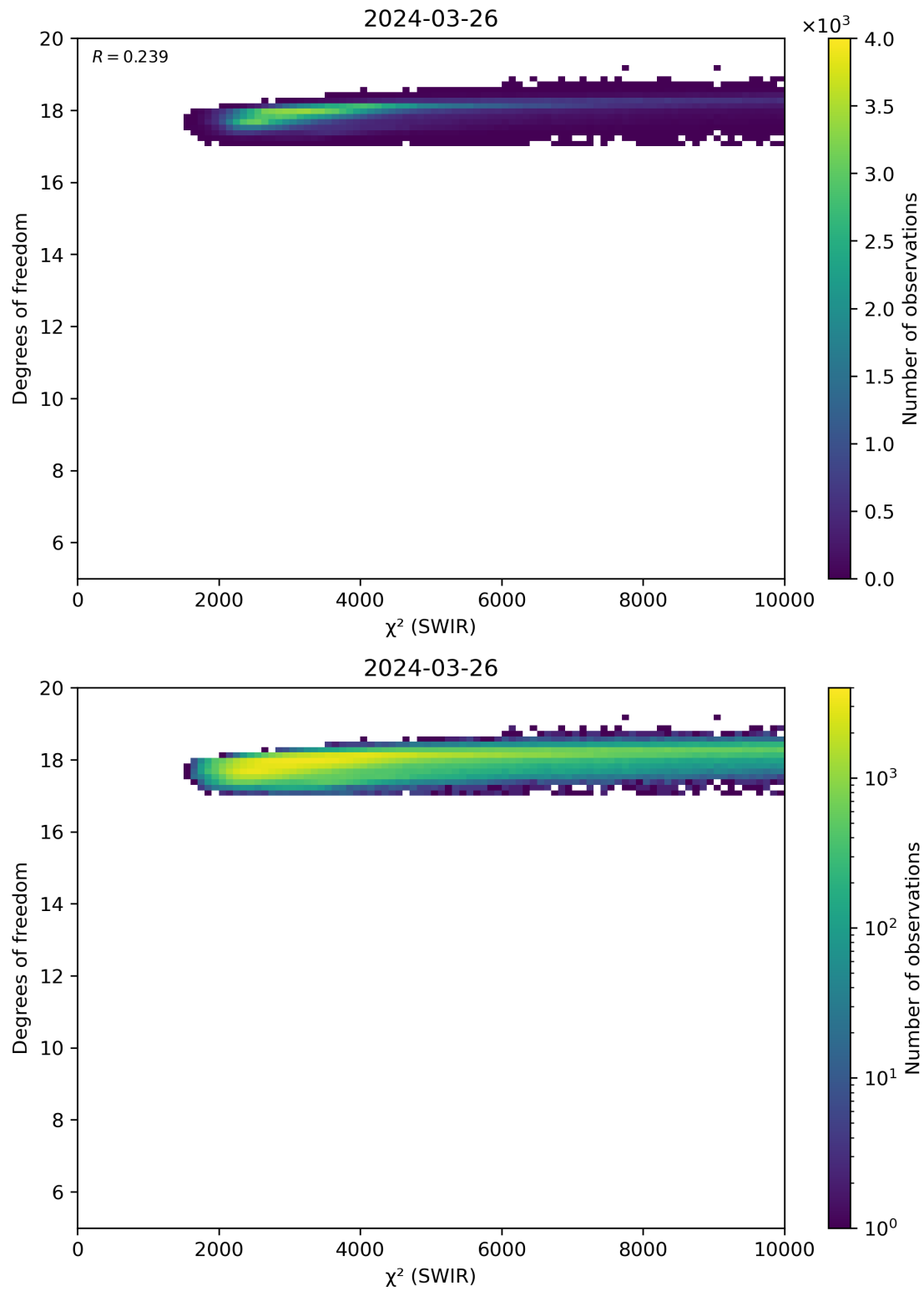
Figure 48: Scatter density plot of “ \chi^2 (SWIR)” against “Degrees of freedom” for 2024-03-25 to 2024-03-27.
