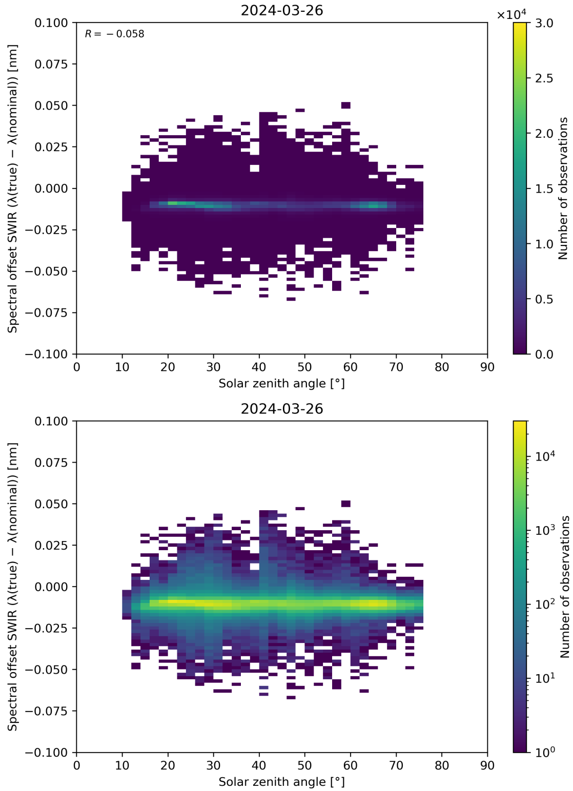
Figure 104: Scatter density plot of “Solar zenith angle” against “Spectral offset SWIR ( \lambda(\text{true}) - \lambda(\text{nominal}) )” for 2024-03-25 to 2024-03-27.
