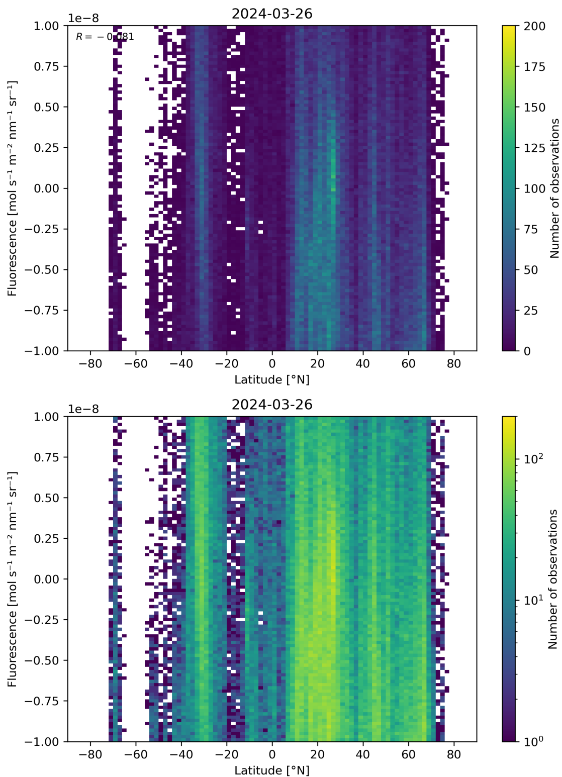
Figure 56: Scatter density plot of “Latitude” against “Fluorescence” for 2024-03-25 to 2024-03-27.
