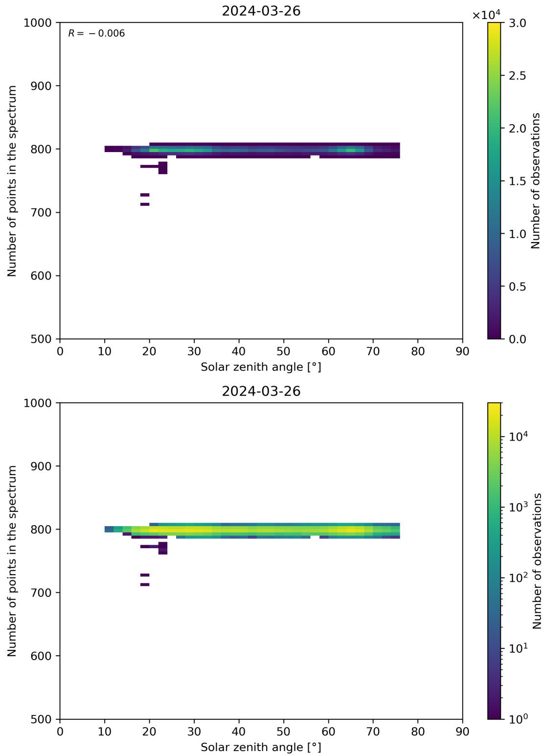
Figure 103: Scatter density plot of “Solar zenith angle” against “Number of points in the spectrum” for 2024-03-25 to 2024-03-27.
