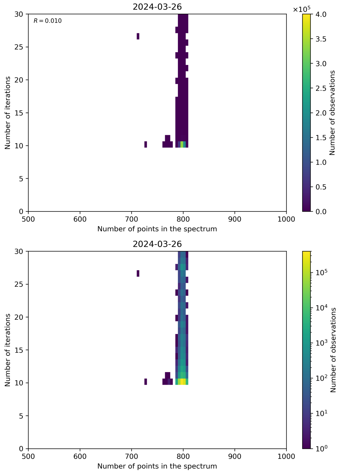
Figure 92: Scatter density plot of “Number of points in the spectrum” against “Number of iterations” for 2024-03-25 to 2024-03-27.
