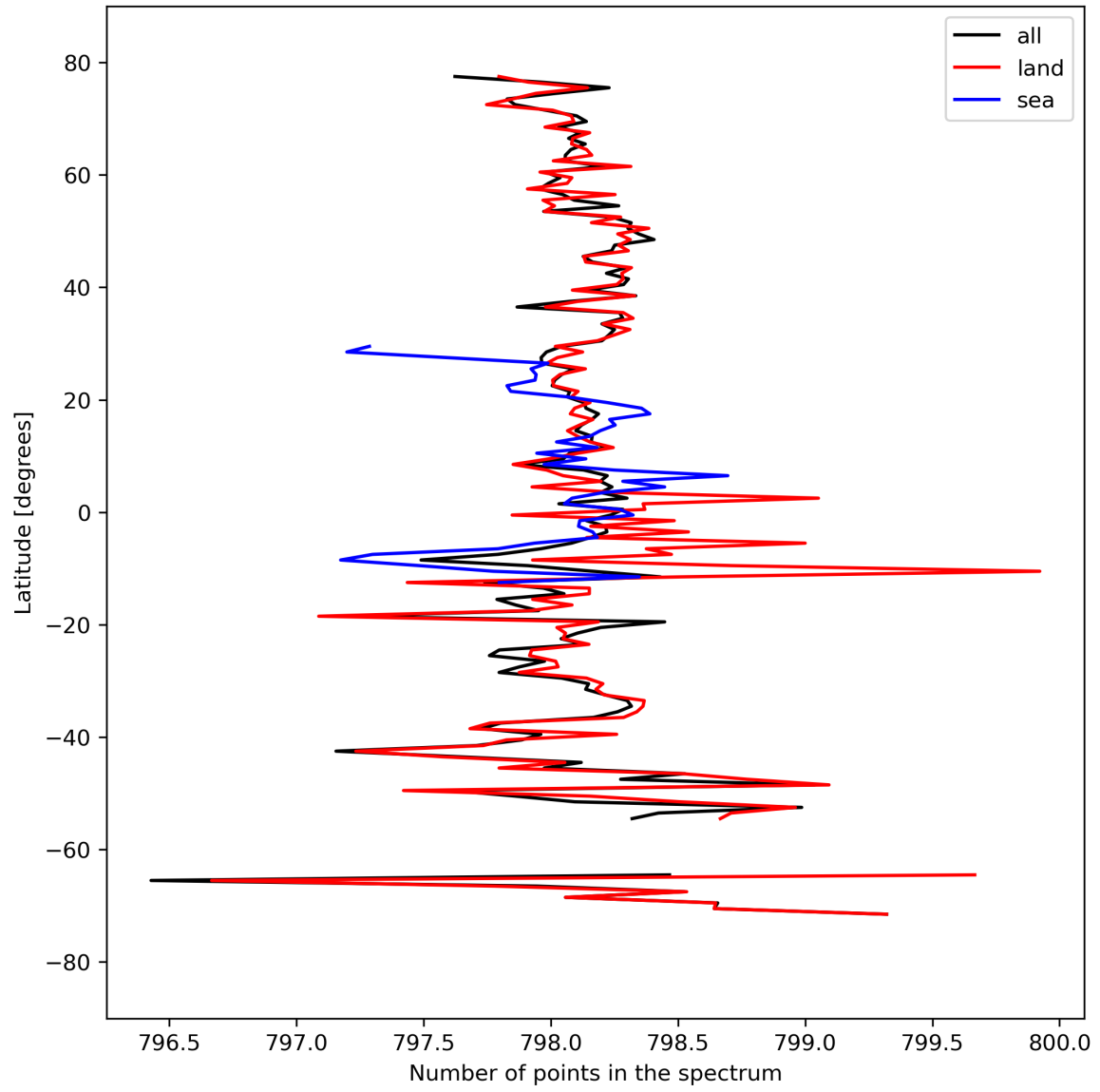
Figure 15: Zonal average of “Number of points in the spectrum” for 2024-03-25 to 2024-03-27.
