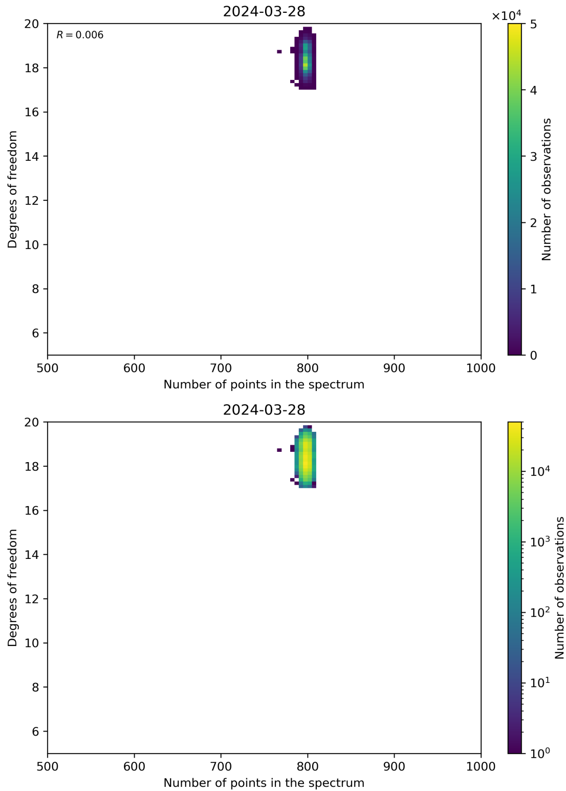
Figure 90: Scatter density plot of “Number of points in the spectrum” against “Degrees of freedom” for 2024-03-27 to 2024-03-29.
