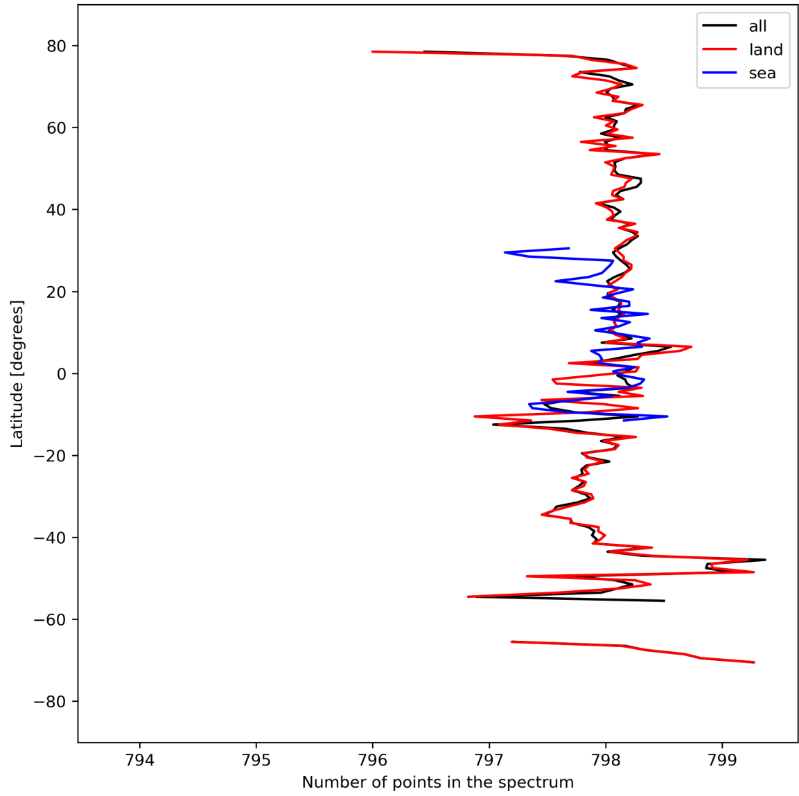
Figure 15: Zonal average of “Number of points in the spectrum” for 2024-03-27 to 2024-03-29.
