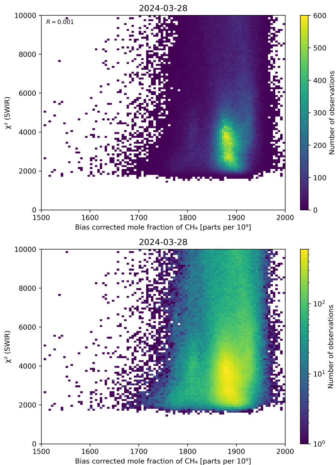
Figure 64: Scatter density plot of “Bias corrected mole fraction of CH 4 ” against “ \chi^2 (SWIR)” for 2024-03-27 to 2024-03-29.
