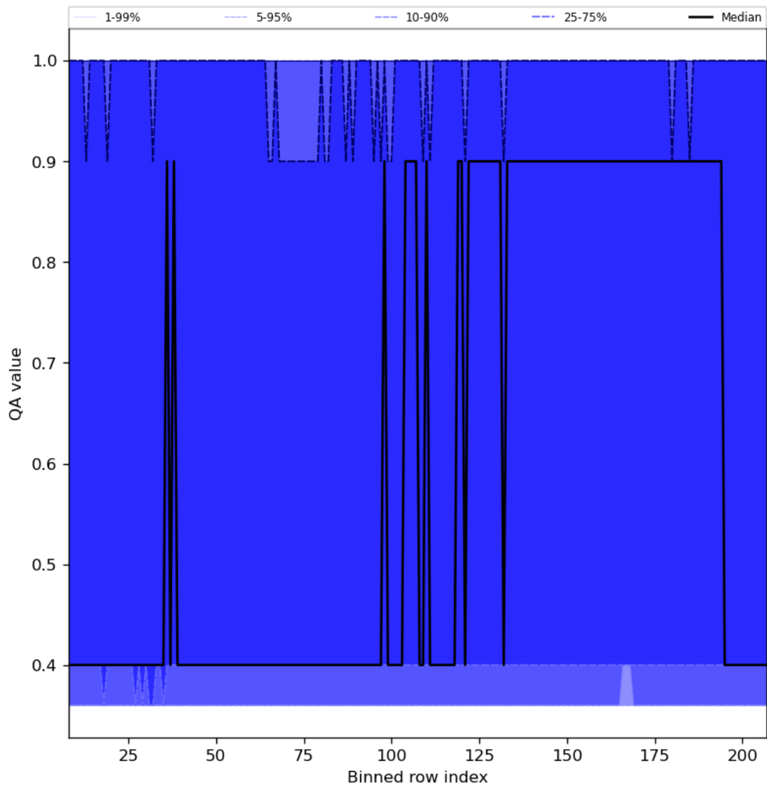
Figure 33: Along track statistics of “QA value” for 2024-03-27 to 2024-03-29
