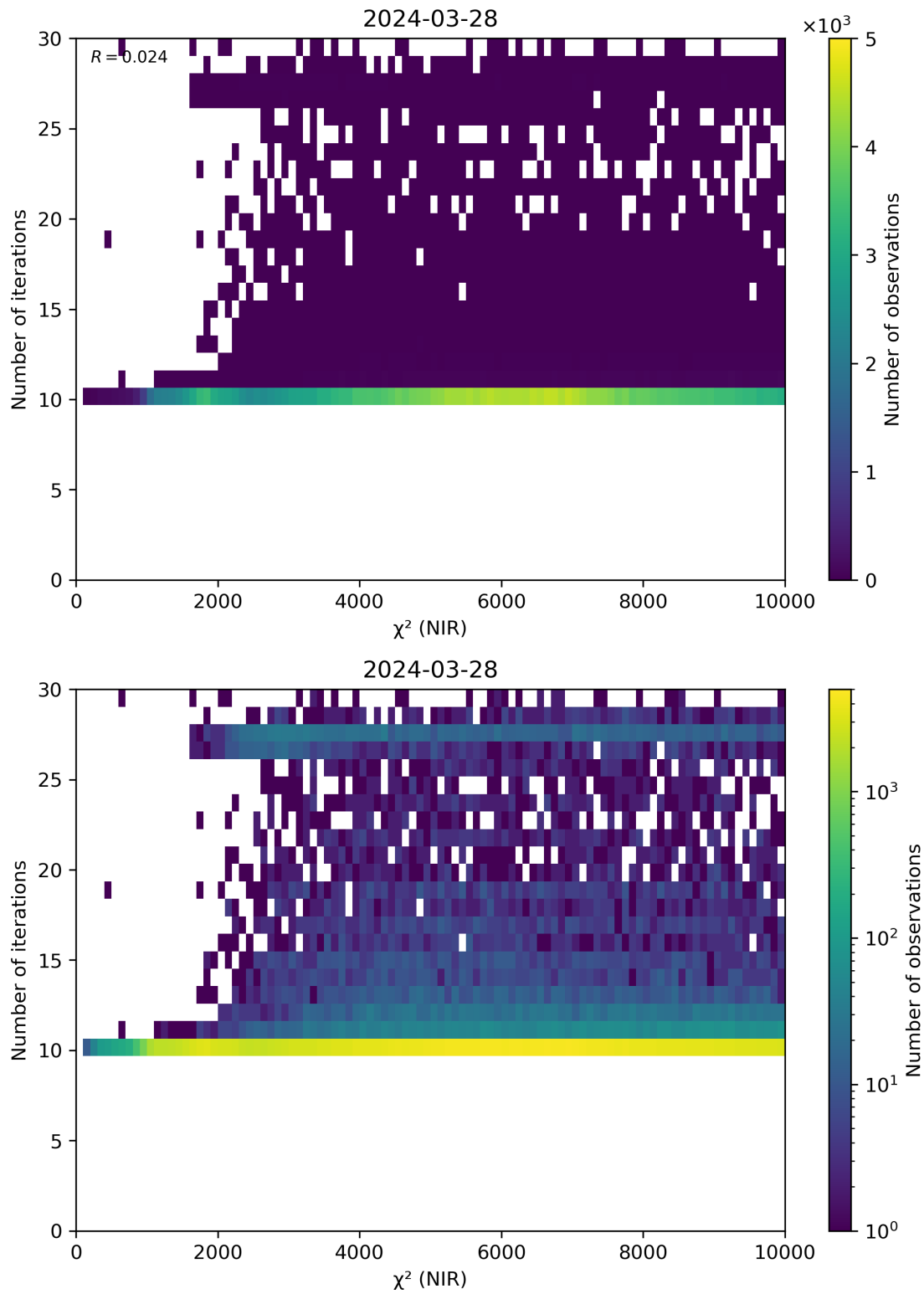
Figure 46: Scatter density plot of “ \chi^2 (NIR)” against “Number of iterations” for 2024-03-27 to 2024-03-29.
