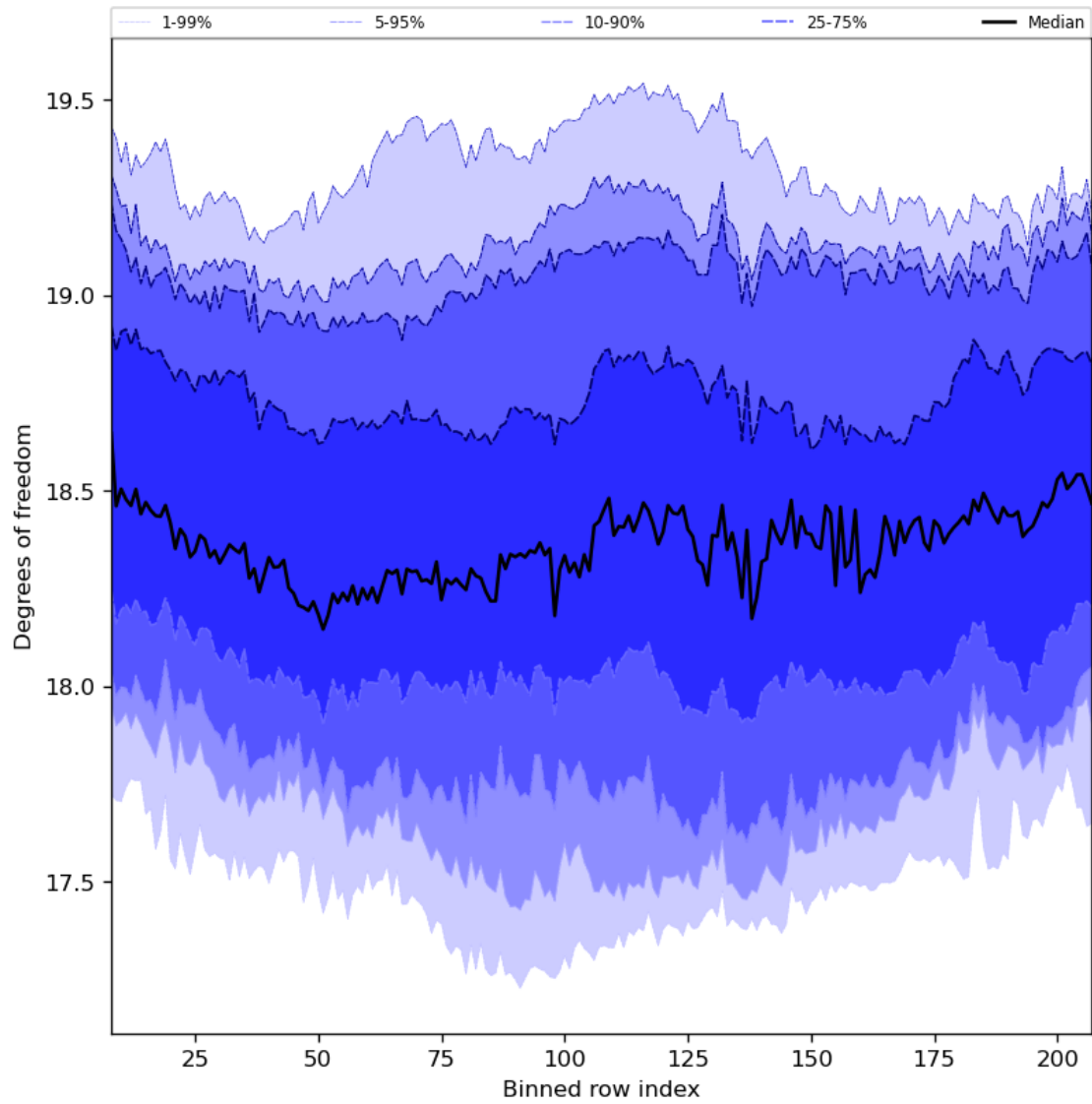
Figure 41: Along track statistics of “Degrees of freedom” for 2024-03-27 to 2024-03-29
