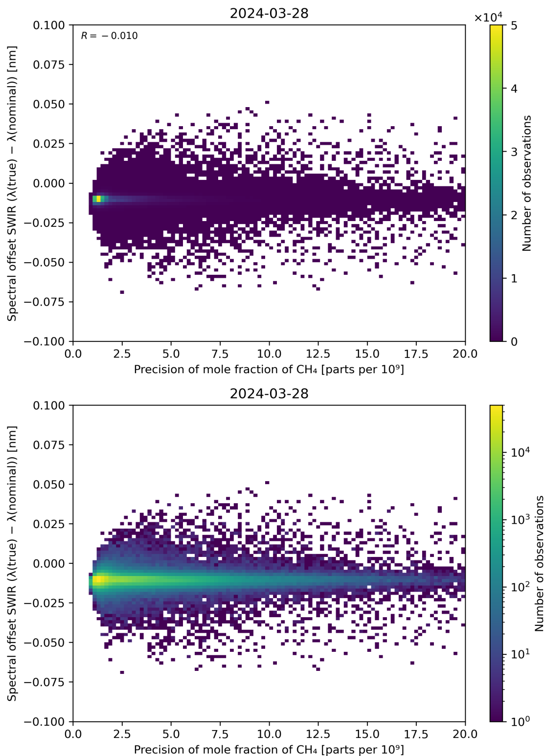
Figure 85: Scatter density plot of “Precision of mole fraction of \text{CH}_4 ” against “Spectral offset SWIR ( \lambda(\text{true}) - \lambda(\text{nominal}) )” for 2024-03-27 to 2024-03-29.
