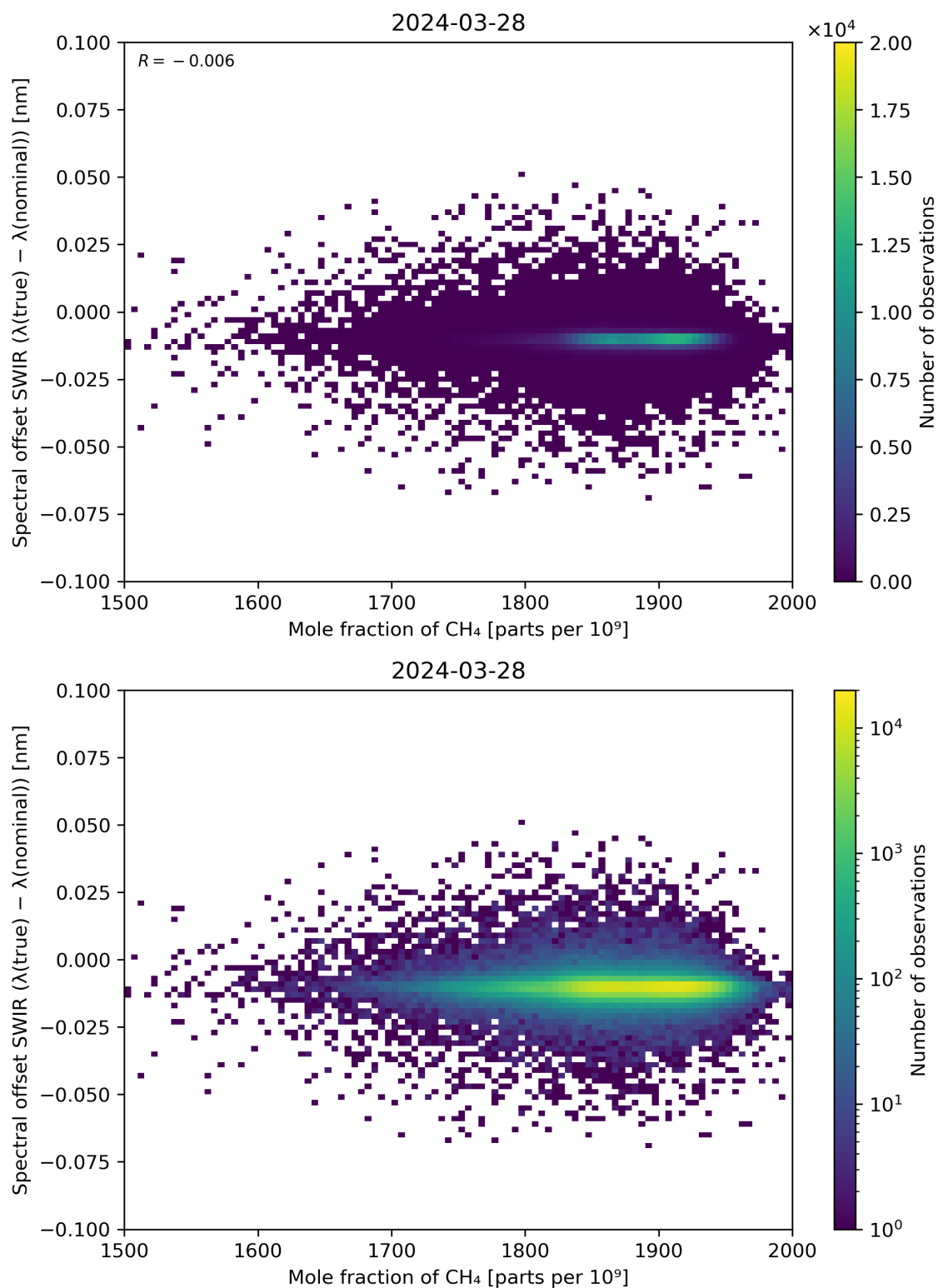
Figure 86: Scatter density plot of “Mole fraction of CH 4 ” against “Spectral offset SWIR ( \lambda(\text{true}) - \lambda(\text{nominal}) )” for 2024-03-27 to 2024-03-29.
