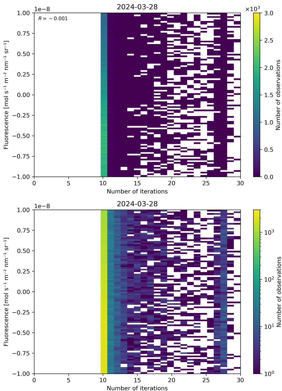
Figure 87: Scatter density plot of “Number of iterations” against “Fluorescence” for 2024-03-27 to 2024-03-29.
