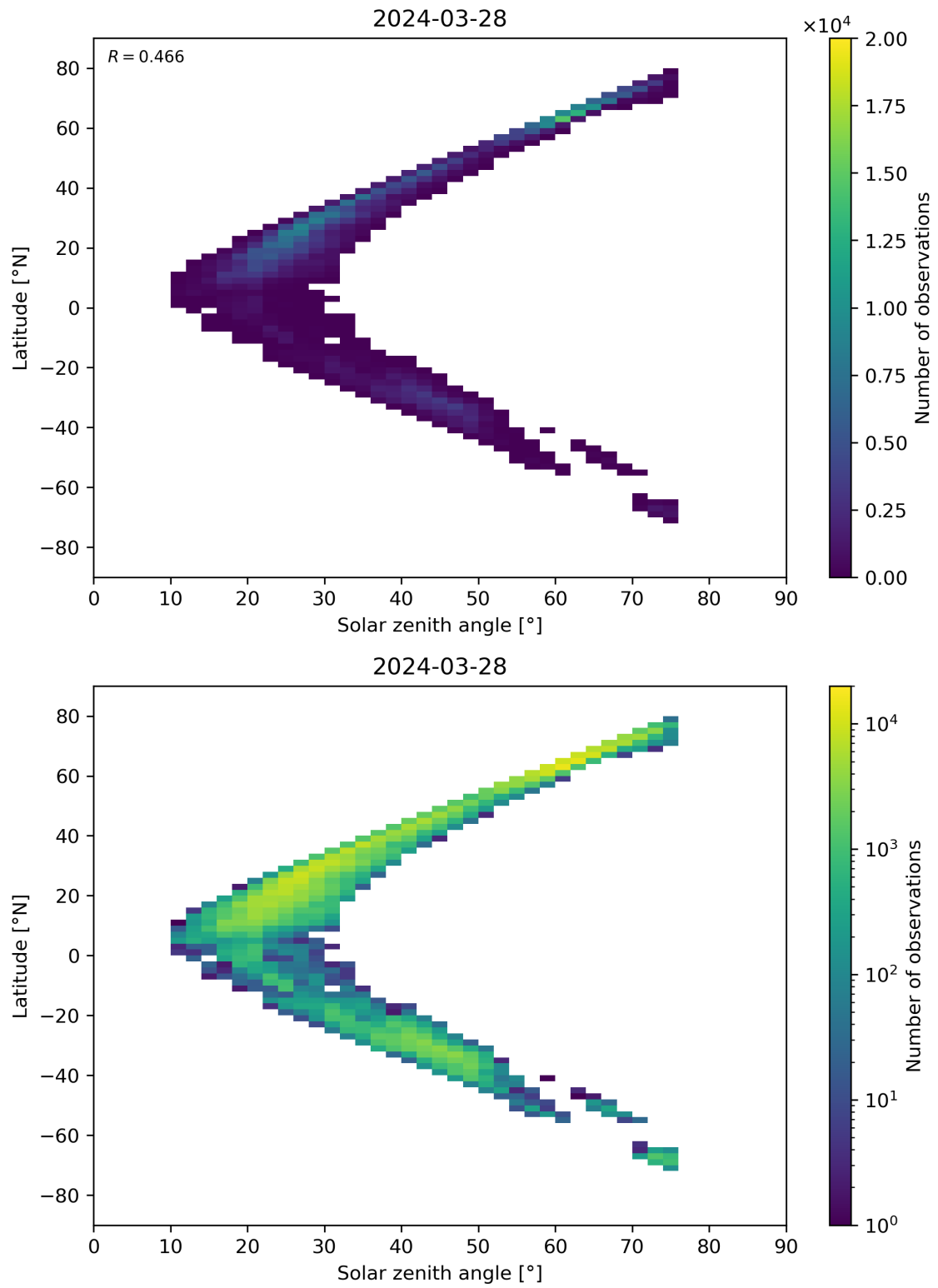
Figure 98: Scatter density plot of “Solar zenith angle” against “Latitude” for 2024-03-27 to 2024-03-29.
