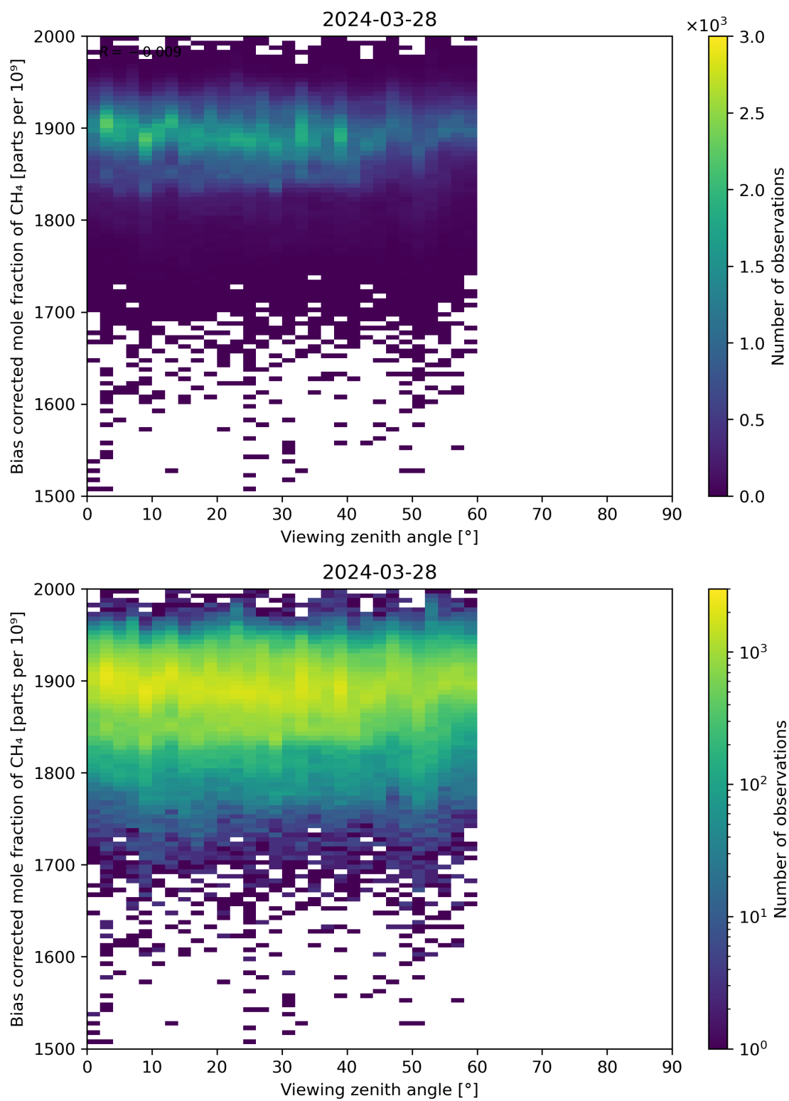
Figure 111: Scatter density plot of “Viewing zenith angle” against “Bias corrected mole fraction of CH 4 ” for 2024-03-27 to 2024-03-29.
