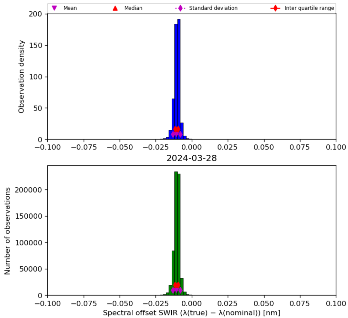
Figure 27: Histogram of “Spectral offset SWIR ( \lambda(\text{true}) - \lambda(\text{nominal}) )” for 2024-03-27 to 2024-03-29
