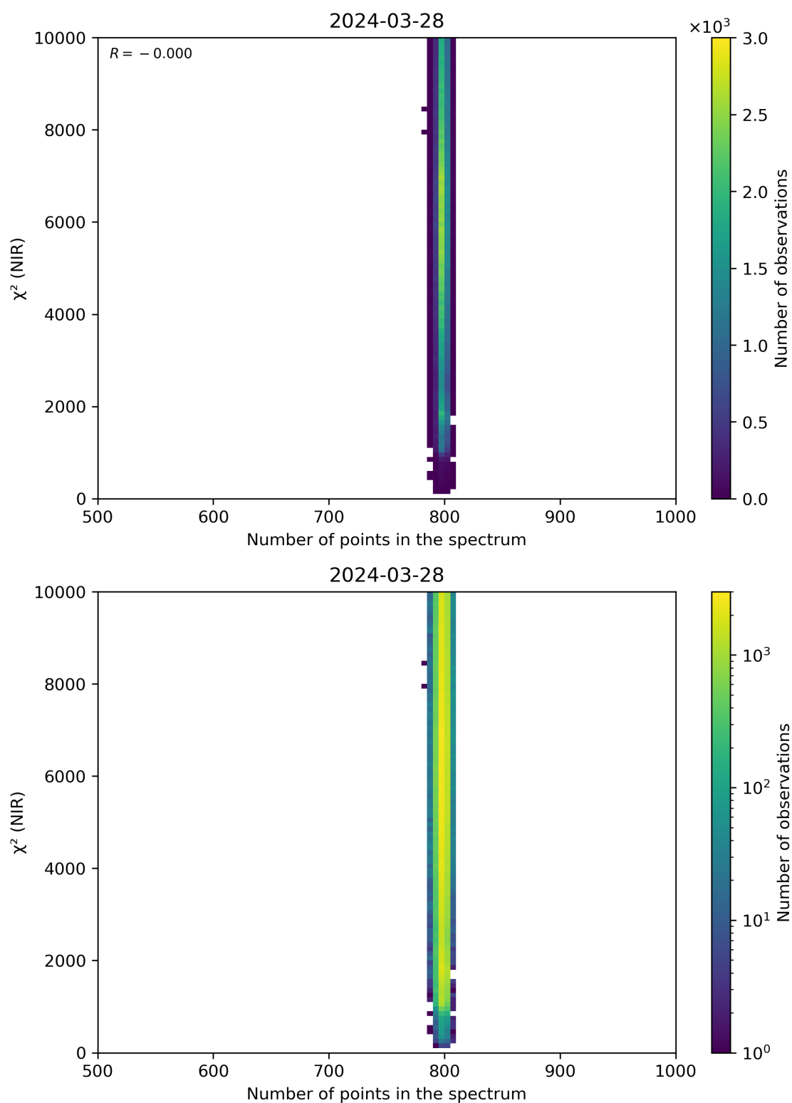
Figure 88: Scatter density plot of “Number of points in the spectrum” against “ \chi^2 (NIR)” for 2024-03-27 to 2024-03-29.
