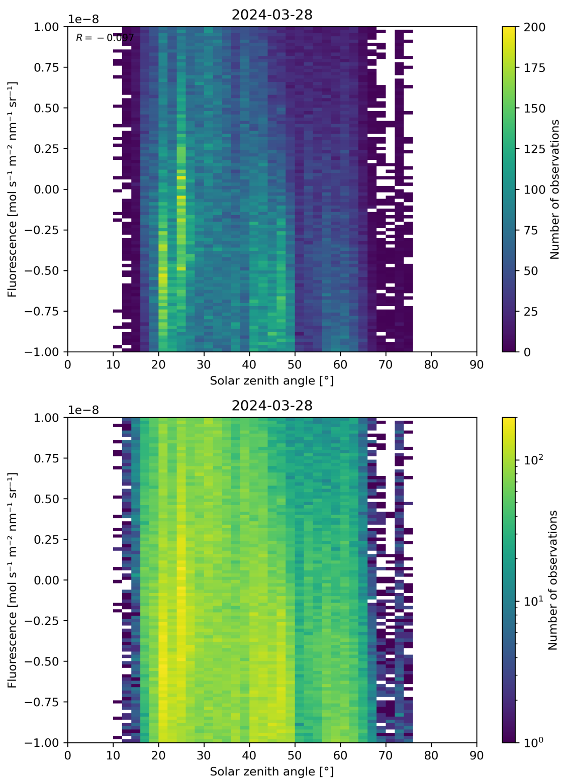
Figure 97: Scatter density plot of “Solar zenith angle” against “Fluorescence” for 2024-03-27 to 2024-03-29.
