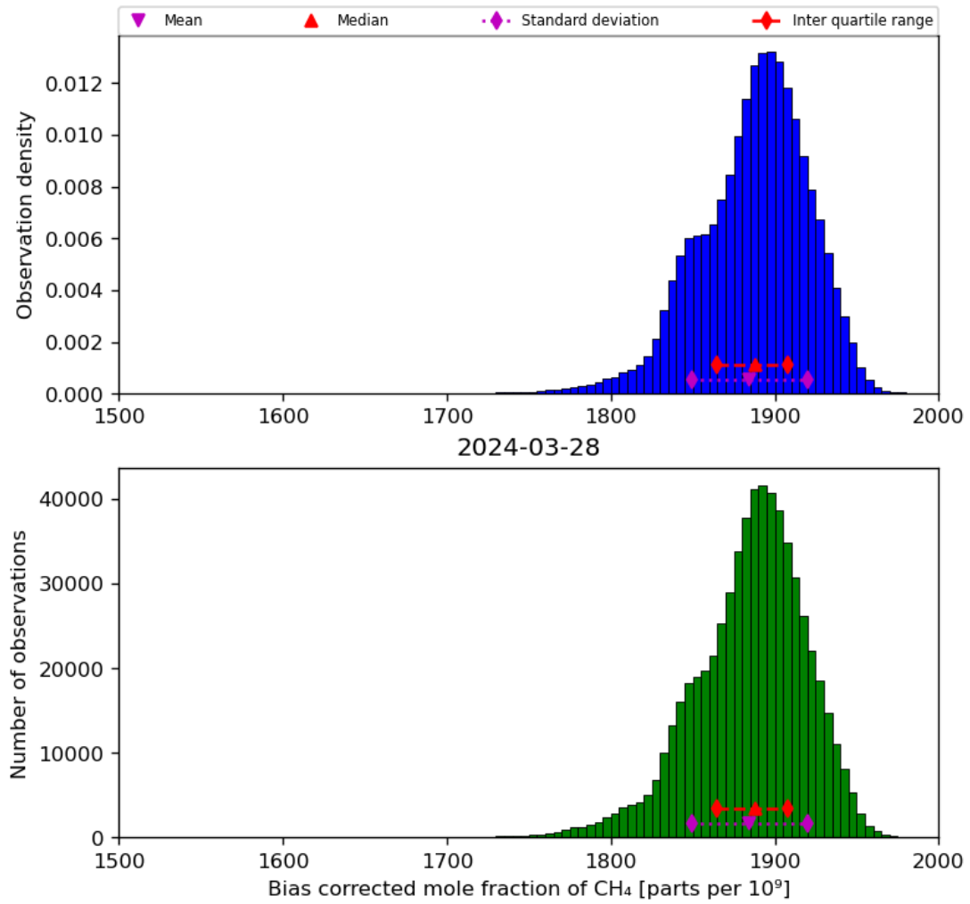
Figure 25: Histogram of “Bias corrected mole fraction of CH 4 ” for 2024-03-27 to 2024-03-29
