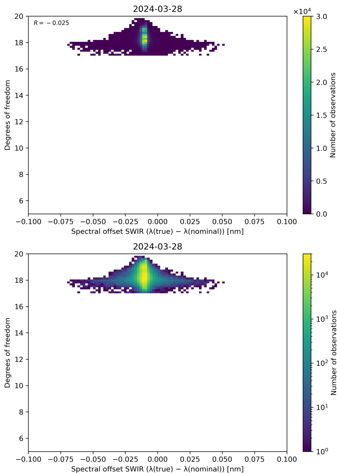
Figure 119: Scatter density plot of “Spectral offset SWIR ( \lambda(\text{true}) - \lambda(\text{nominal}) )” against “Degrees of freedom” for 2024-03-27 to 2024-03-29.
