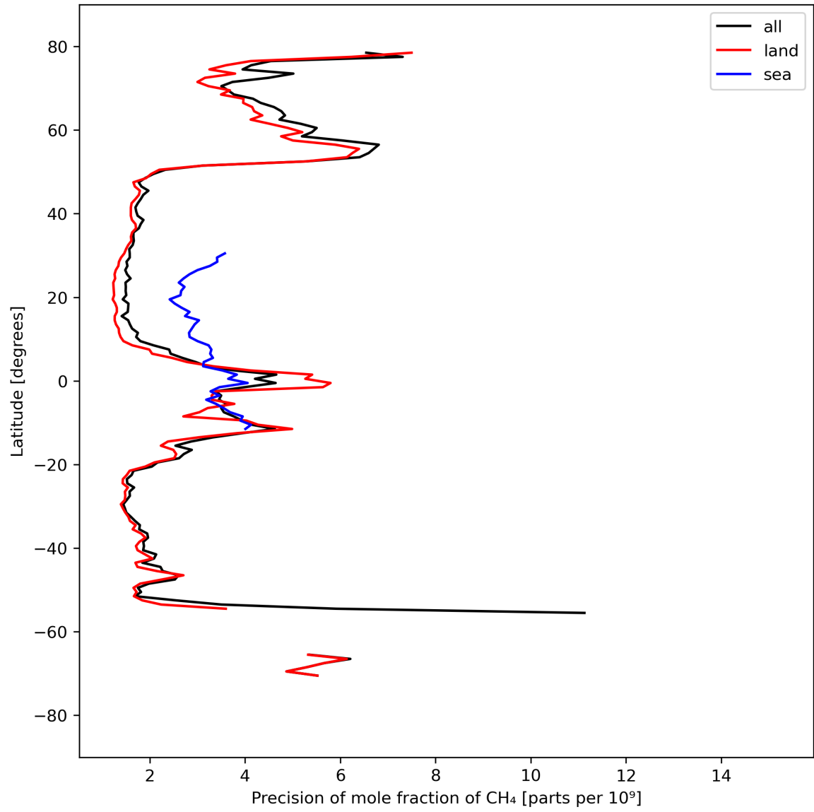
Figure 13: Zonal average of “Precision of mole fraction of CH 4 ” for 2024-03-27 to 2024-03-29.
