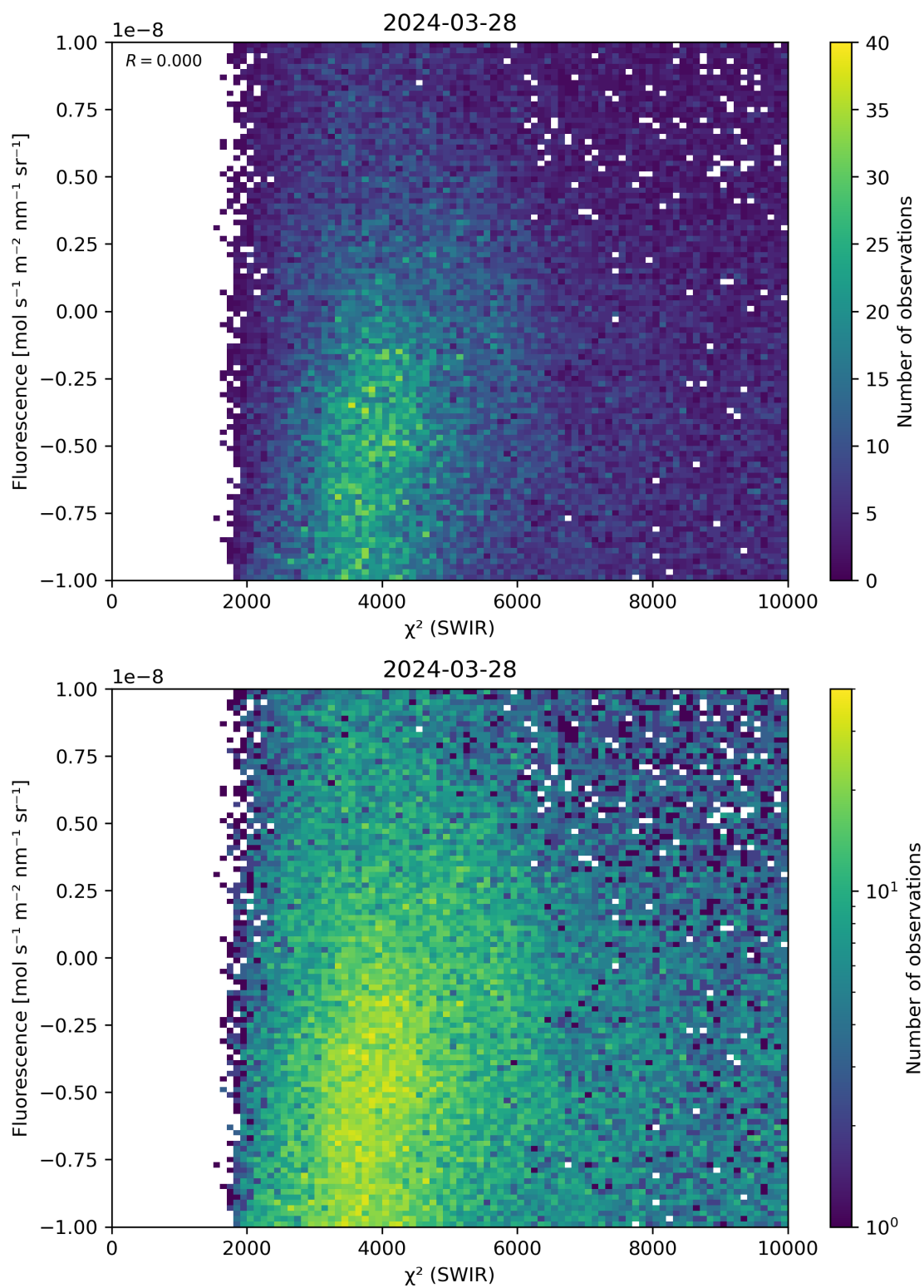
Figure 49: Scatter density plot of “ \chi^2 (SWIR)” against “Fluorescence” for 2024-03-27 to 2024-03-29.
