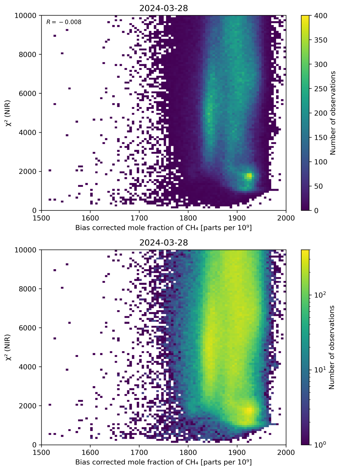
Figure 63: Scatter density plot of “Bias corrected mole fraction of CH 4 ” against “ \chi^2 (NIR)” for 2024-03-27 to 2024-03-29.
