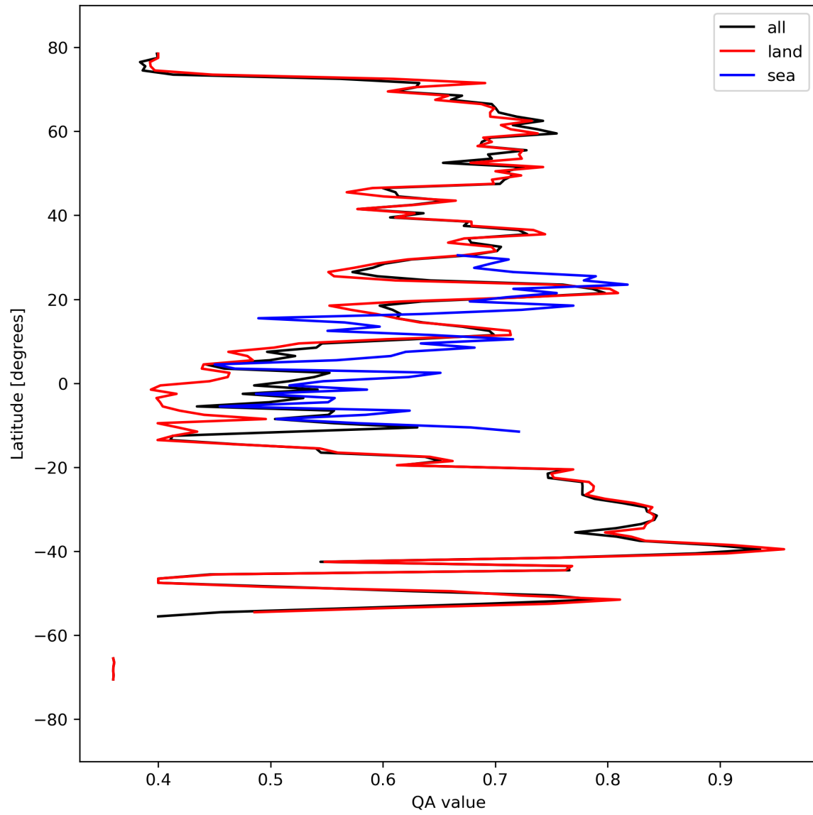
Figure 11: Zonal average of “QA value” for 2024-03-27 to 2024-03-29.
