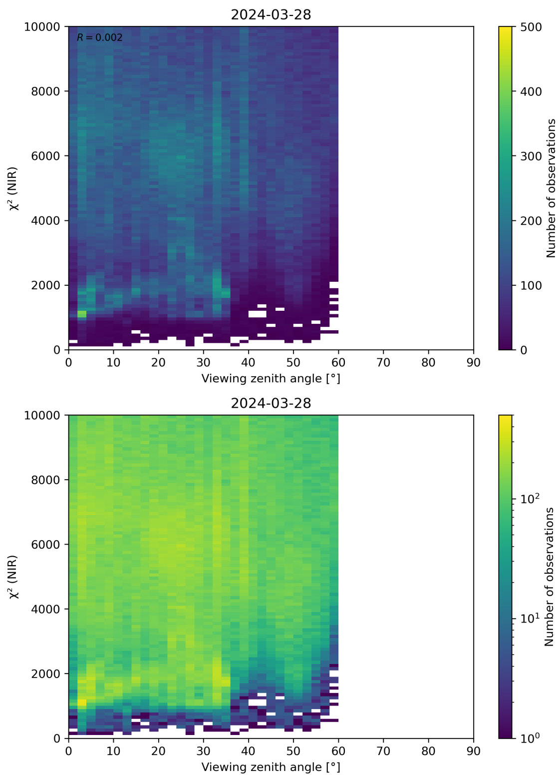
Figure 105: Scatter density plot of “Viewing zenith angle” against “ \chi^2 (NIR)” for 2024-03-27 to 2024-03-29.
