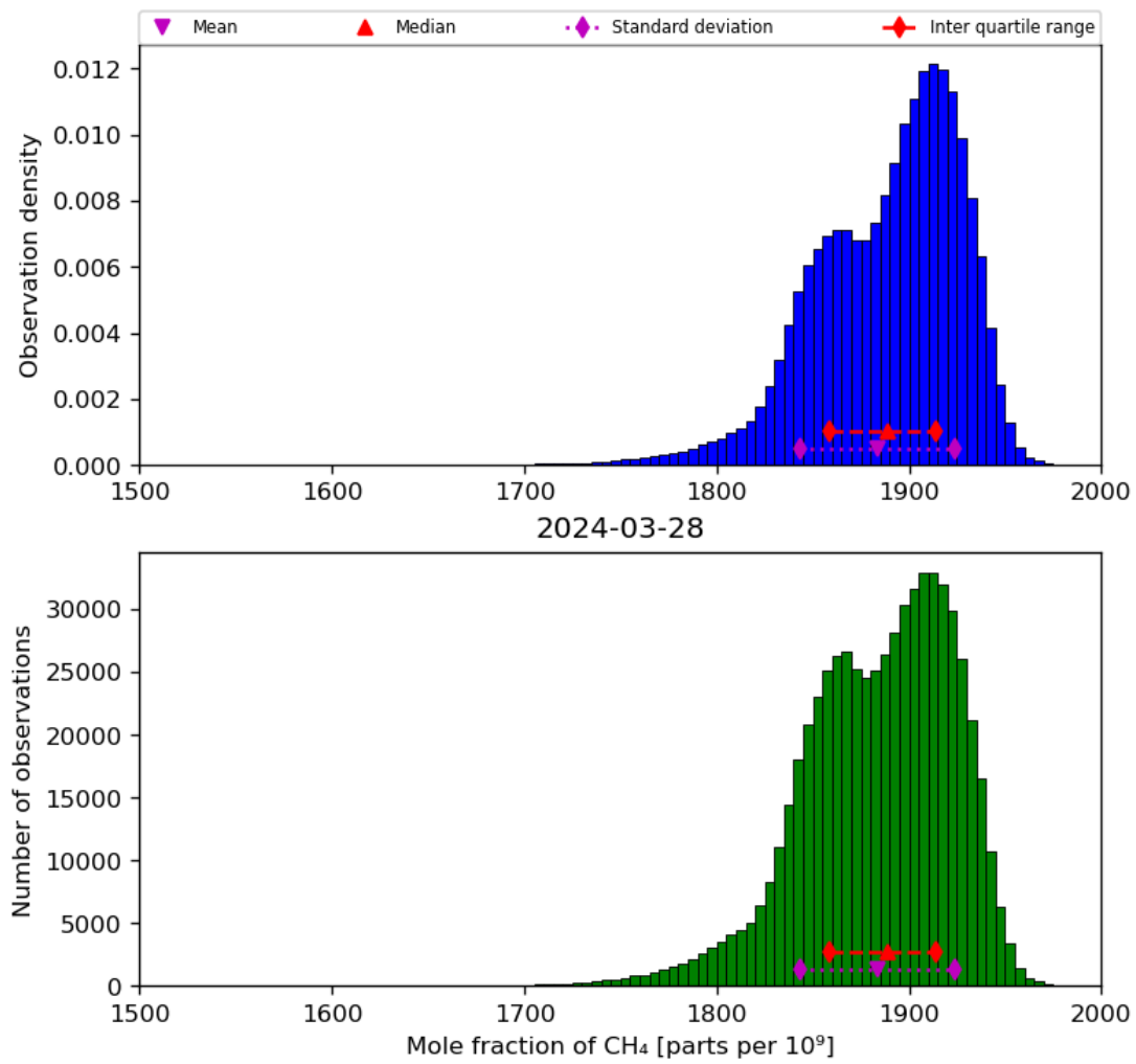
Figure 23: Histogram of “Mole fraction of CH 4 ” for 2024-03-27 to 2024-03-29
