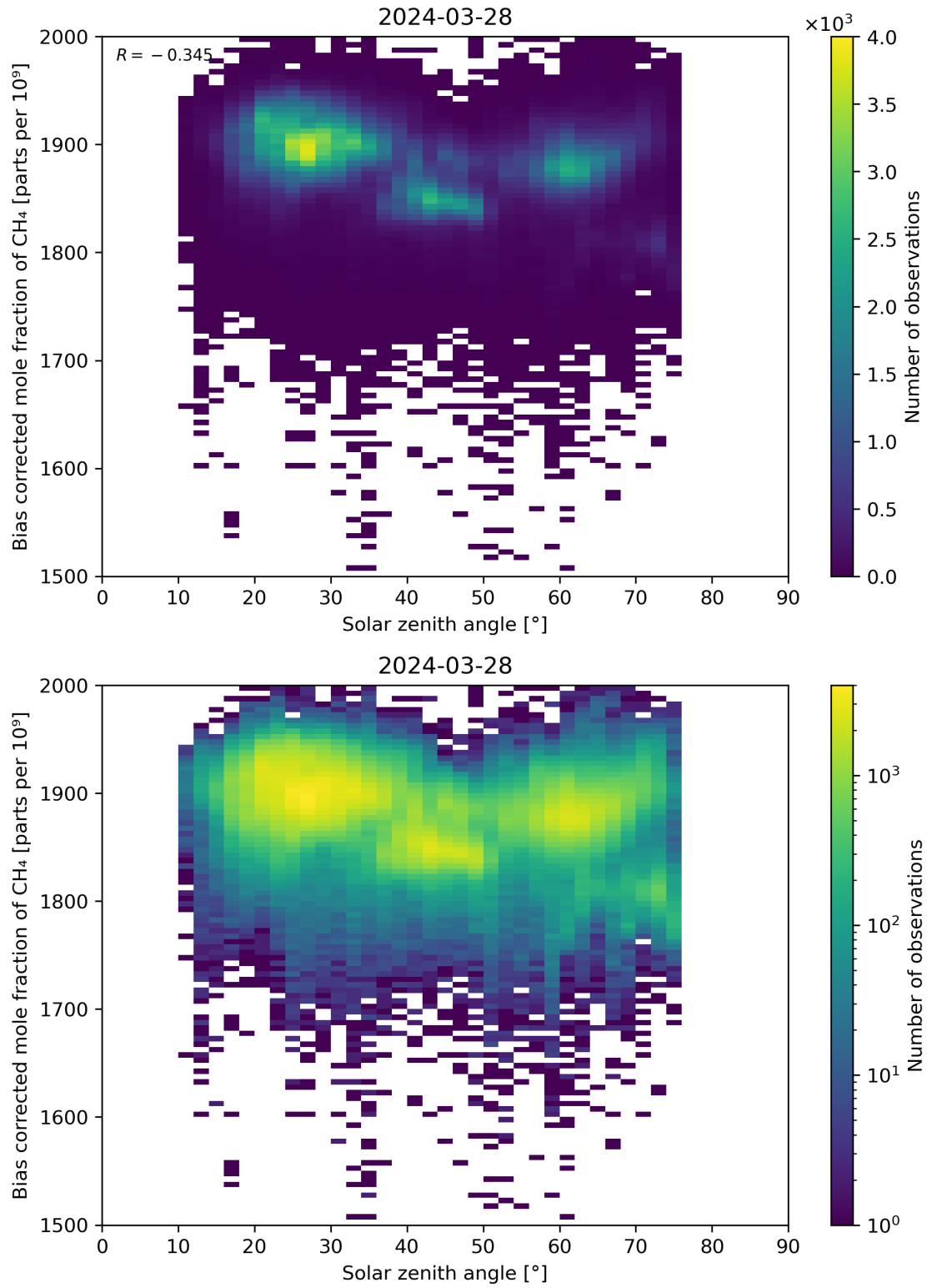
Figure 100: Scatter density plot of “Solar zenith angle” against “Bias corrected mole fraction of CH 4 ” for 2024-03-27 to 2024-03-29.
