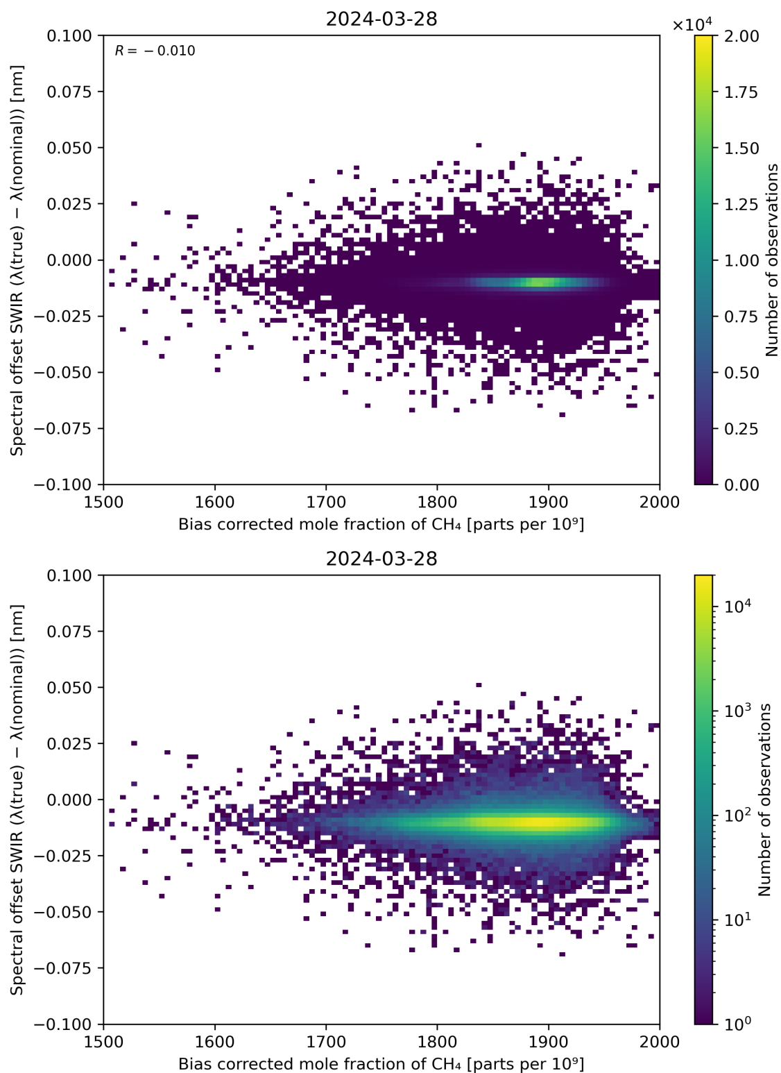
Figure 69: Scatter density plot of “Bias corrected mole fraction of \text{CH}_4 ” against “Spectral offset SWIR ( \lambda(\text{true}) - \lambda(\text{nominal}) )” for 2024-03-27 to 2024-03-29.
