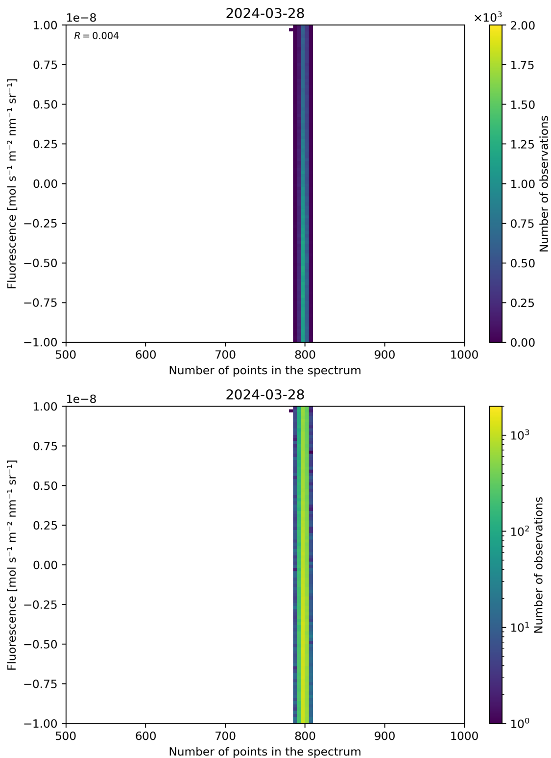
Figure 91: Scatter density plot of “Number of points in the spectrum” against “Fluorescence” for 2024-03-27 to 2024-03-29.
