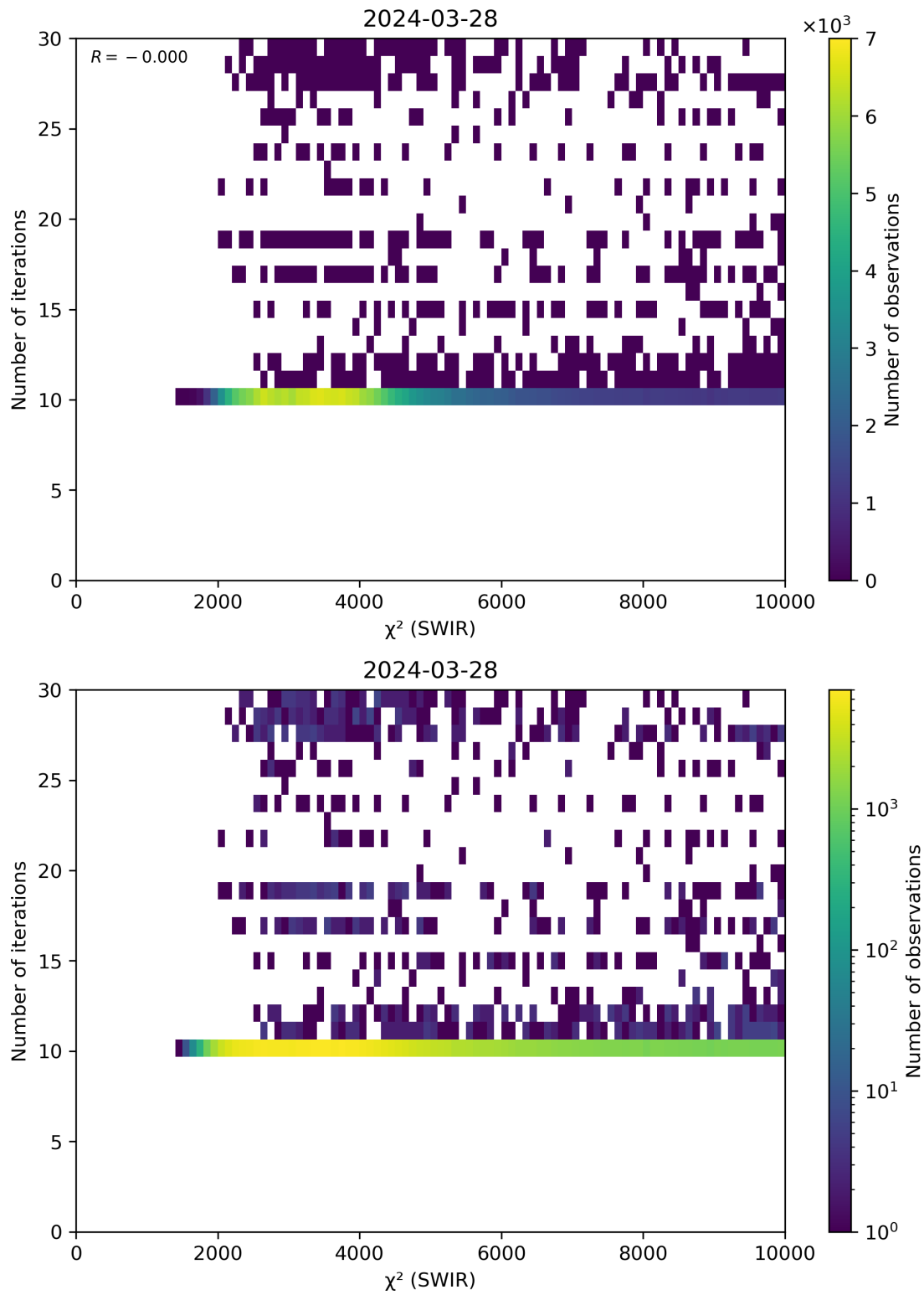
Figure 50: Scatter density plot of “ \chi^2 (SWIR)” against “Number of iterations” for 2024-03-27 to 2024-03-29.
