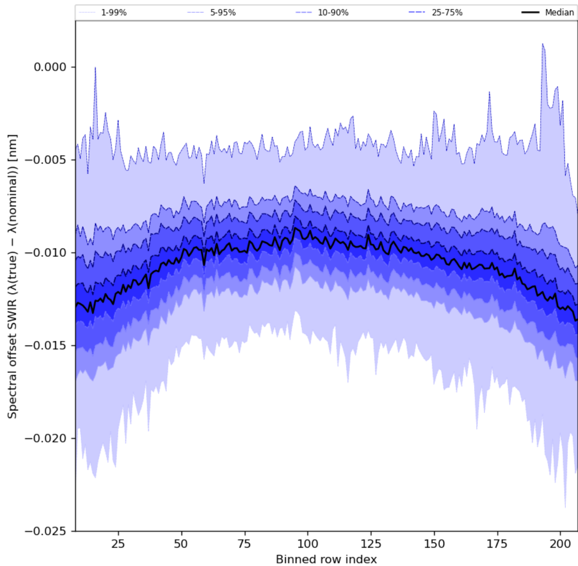
Figure 38: Along track statistics of “Spectral offset SWIR ( \lambda(\text{true}) - \lambda(\text{nominal}) )” for 2024-03-27 to 2024-03-29
