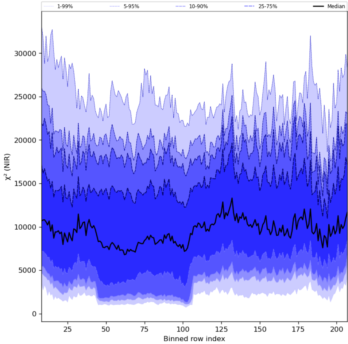
Figure 40: Along track statistics of “ \chi^2 (NIR)” for 2024-03-27 to 2024-03-29
