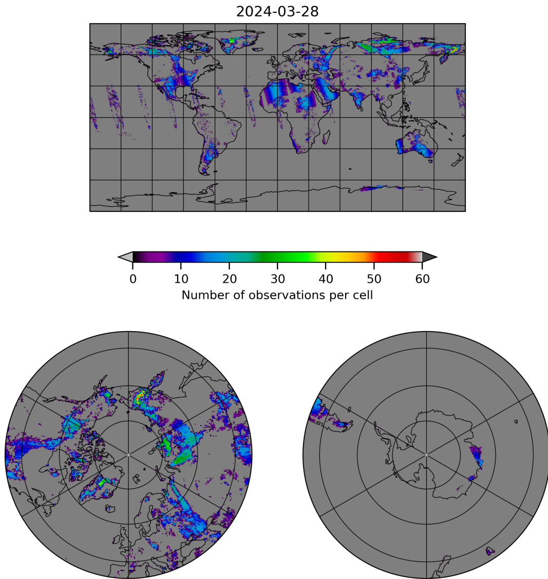
Figure 10: Map of the number of observations for 2024-03-27 to 2024-03-29
