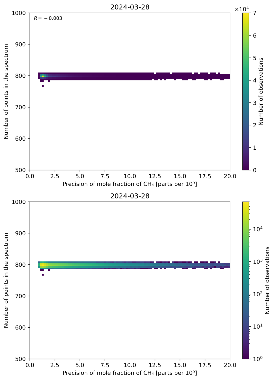
Figure 84: Scatter density plot of “Precision of mole fraction of CH 4 ” against “Number of points in the spectrum” for 2024-03-27 to 2024-03-29.
