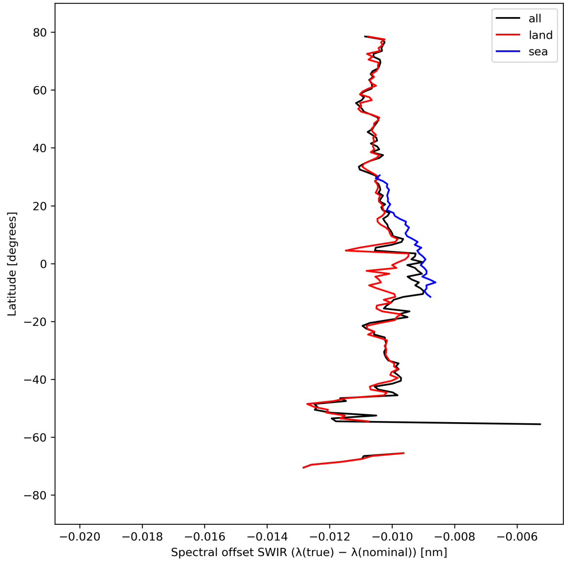
Figure 16: Zonal average of “Spectral offset SWIR ( \lambda(\text{true}) - \lambda(\text{nominal}) )” for 2024-03-27 to 2024-03-29.
