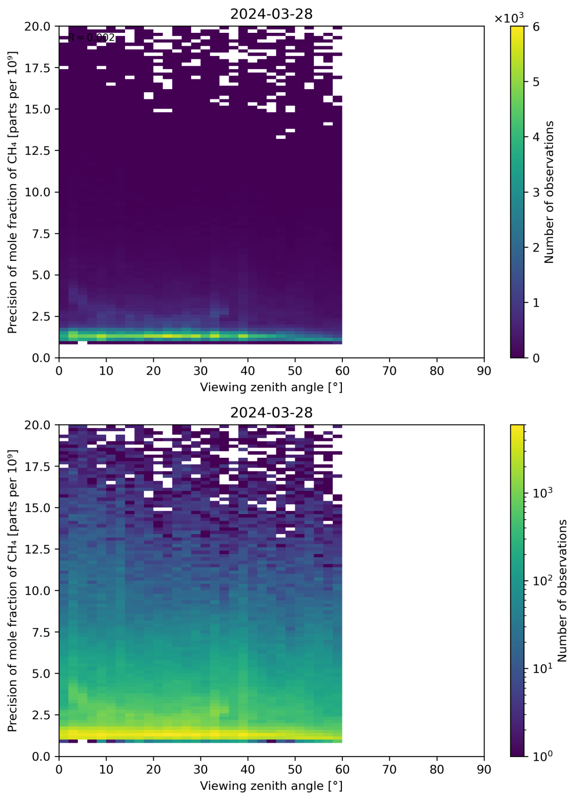
Figure 112: Scatter density plot of “Viewing zenith angle” against “Precision of mole fraction of CH 4 ” for 2024-03-27 to 2024-03-29.
