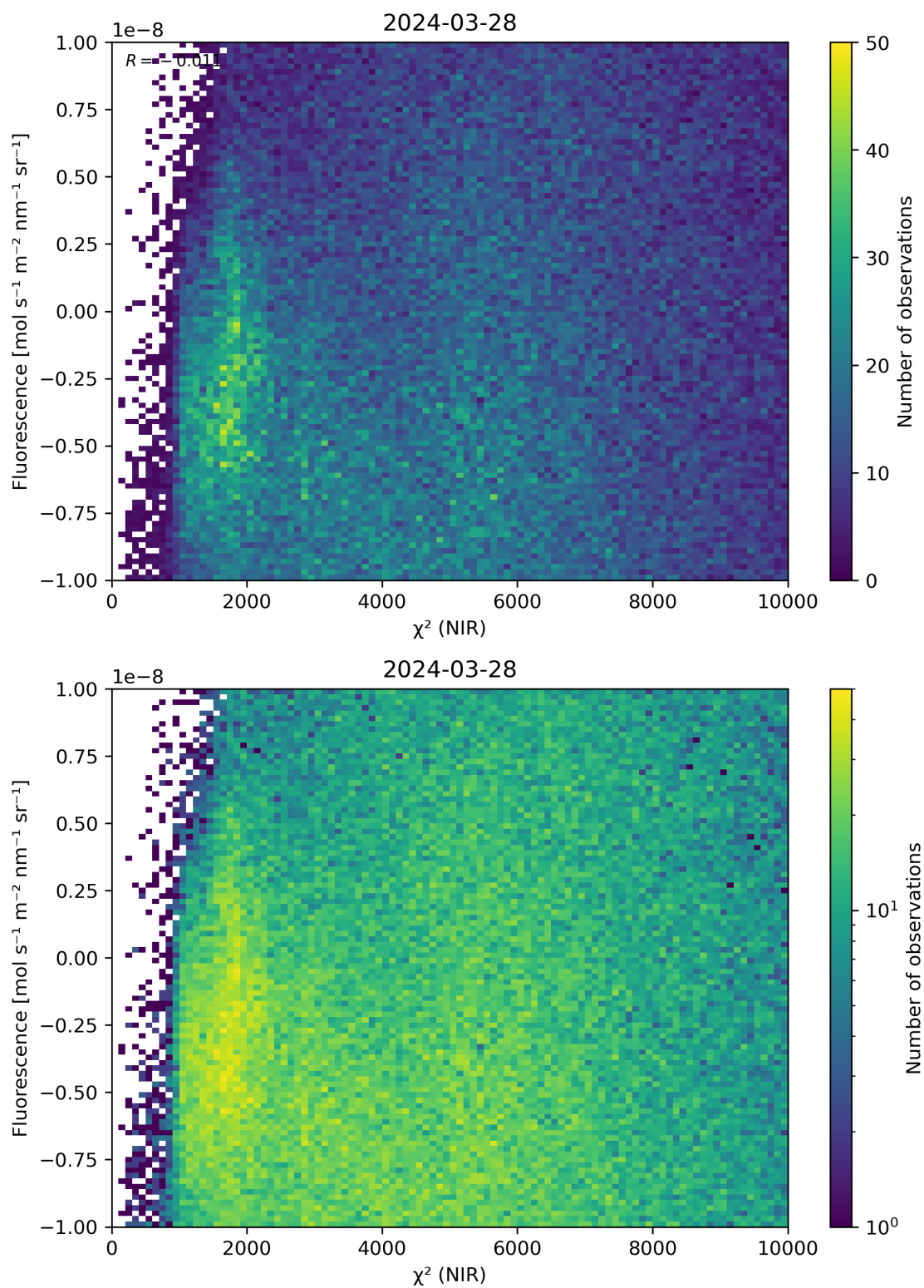
Figure 45: Scatter density plot of “ \chi^2 (NIR)” against “Fluorescence” for 2024-03-27 to 2024-03-29.
