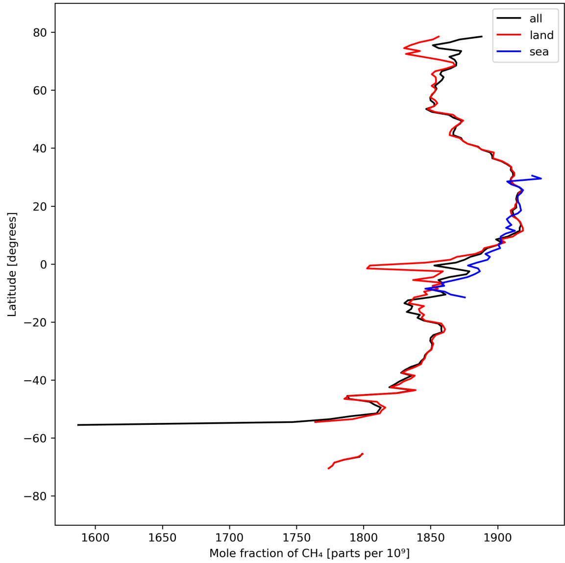
Figure 12: Zonal average of “Mole fraction of CH 4 ” for 2024-03-27 to 2024-03-29.
