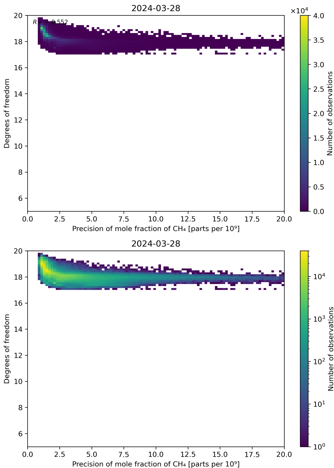
Figure 80: Scatter density plot of “Precision of mole fraction of CH 4 ” against “Degrees of freedom” for 2024-03-27 to 2024-03-29.
