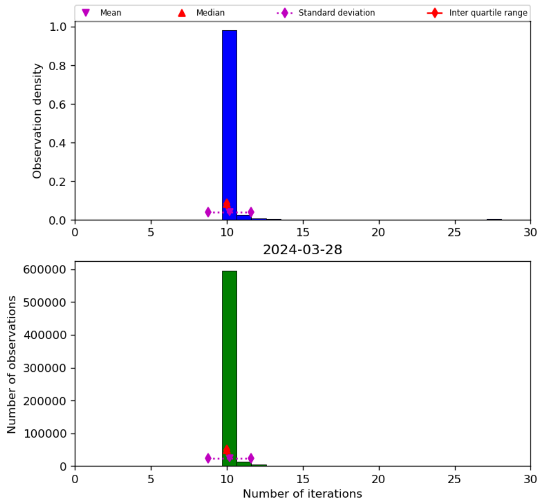
Figure 31: Histogram of “Number of iterations” for 2024-03-27 to 2024-03-29
