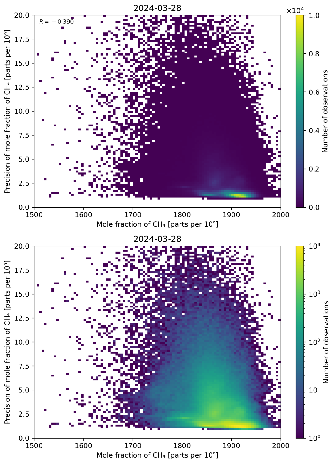
Figure 75: Scatter density plot of “Mole fraction of CH 4 ” against “Precision of mole fraction of CH 4 ” for 2024-03-27 to 2024-03-29.
