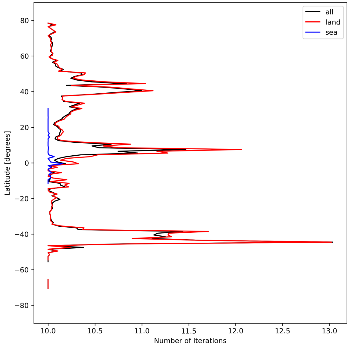
Figure 20: Zonal average of “Number of iterations” for 2024-03-27 to 2024-03-29.
