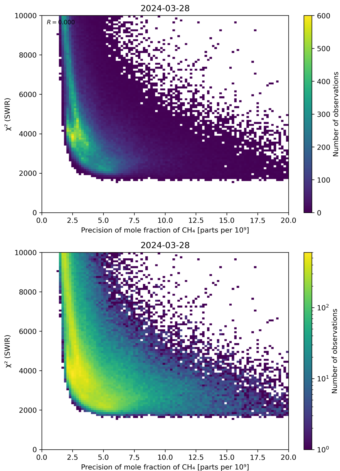
Figure 79: Scatter density plot of “Precision of mole fraction of \text{CH}_4 ” against “ \chi^2 (SWIR)” for 2024-03-27 to 2024-03-29.
