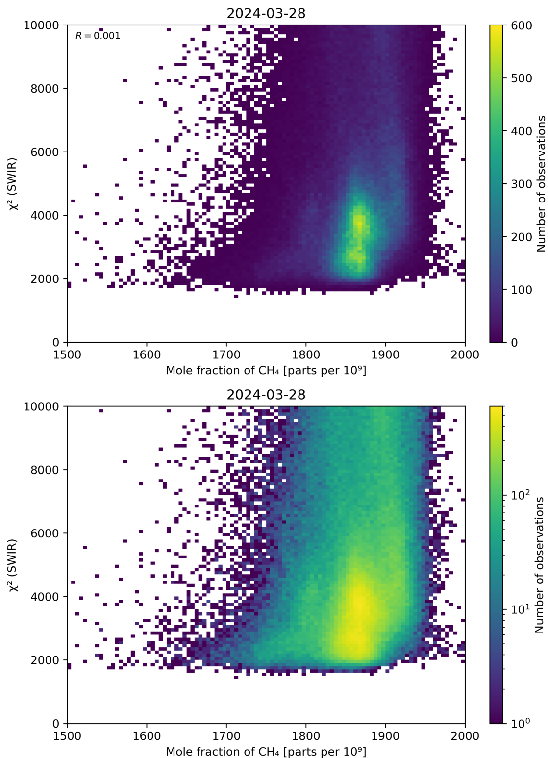
Figure 71: Scatter density plot of “Mole fraction of \text{CH}_4 ” against “ \chi^2 (SWIR)” for 2024-03-27 to 2024-03-29.
