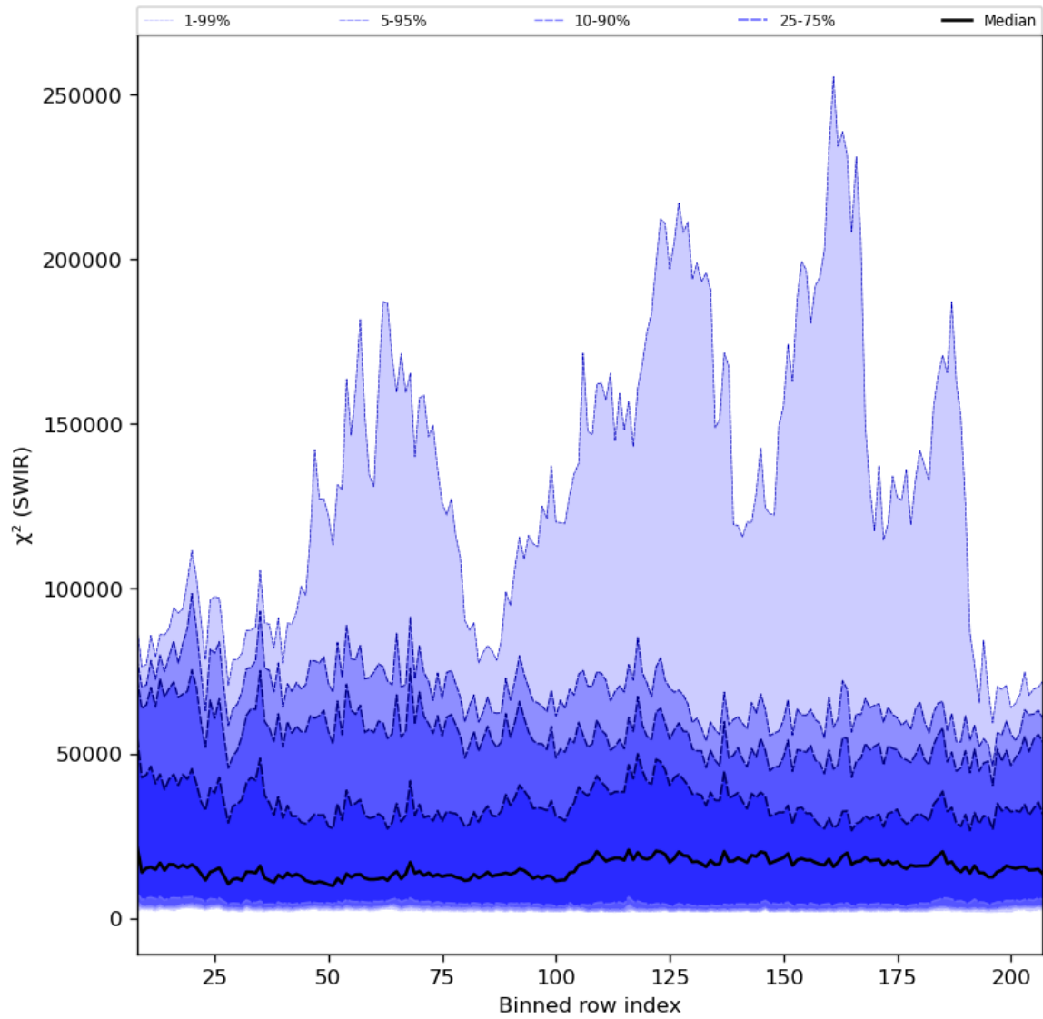
Figure 39: Along track statistics of " \chi^2 (SWIR)" for 2024-03-27 to 2024-03-29
