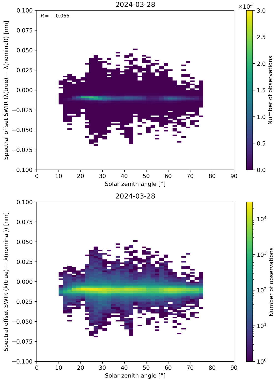
Figure 104: Scatter density plot of “Solar zenith angle” against “Spectral offset SWIR ( \lambda(\text{true}) - \lambda(\text{nominal}) )” for 2024-03-27 to 2024-03-29.
