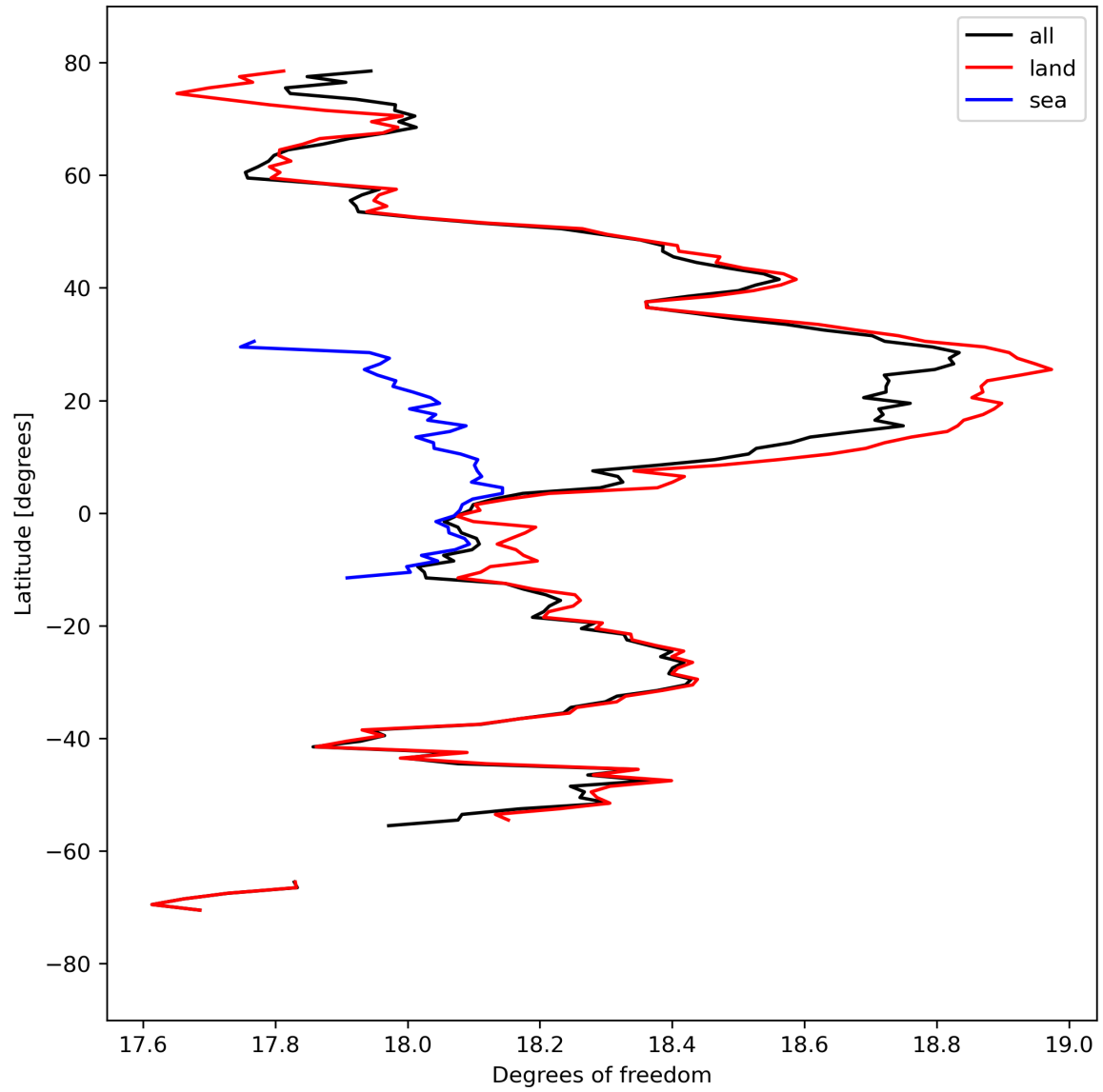
Figure 19: Zonal average of “Degrees of freedom” for 2024-03-27 to 2024-03-29.
