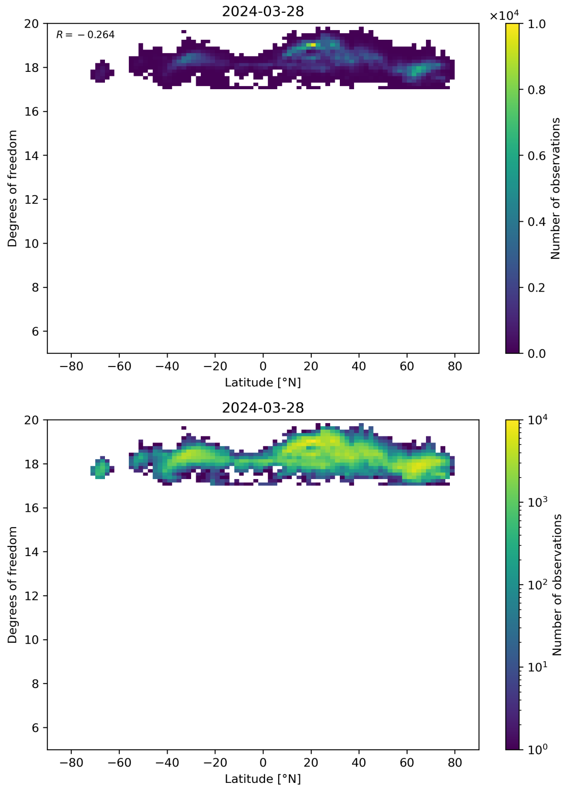
Figure 55: Scatter density plot of “Latitude” against “Degrees of freedom” for 2024-03-27 to 2024-03-29.
