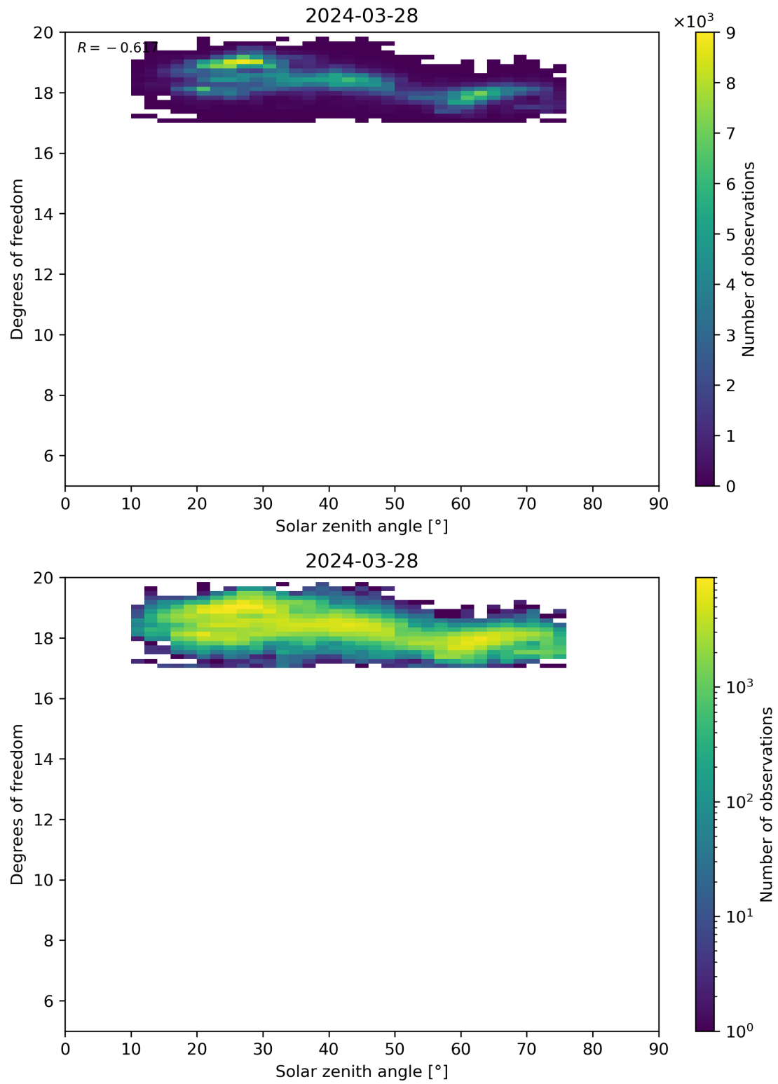
Figure 96: Scatter density plot of “Solar zenith angle” against “Degrees of freedom” for 2024-03-27 to 2024-03-29.
