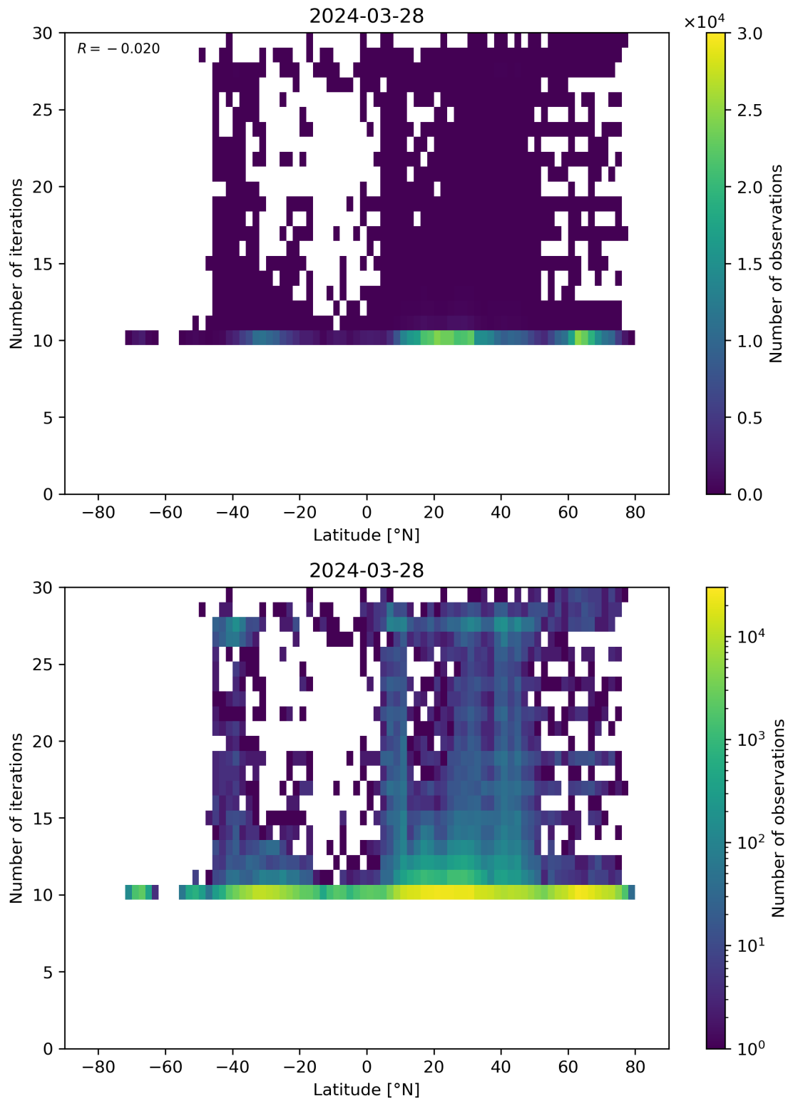
Figure 60: Scatter density plot of “Latitude” against “Number of iterations” for 2024-03-27 to 2024-03-29.
