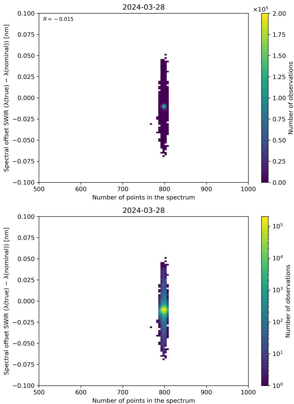
Figure 93: Scatter density plot of “Number of points in the spectrum” against “Spectral offset SWIR ( \lambda(\text{true}) - \lambda(\text{nominal}) )” for 2024-03-27 to 2024-03-29.
