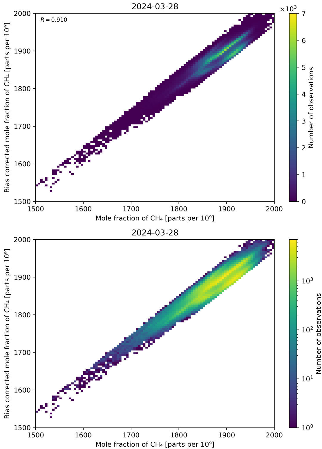
Figure 74: Scatter density plot of “Mole fraction of CH 4 ” against “Bias corrected mole fraction of CH 4 ” for 2024-03-27 to 2024-03-29.
