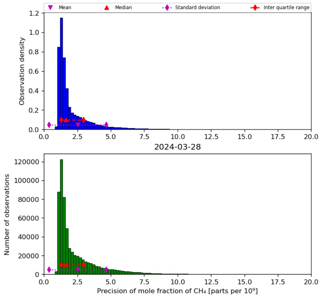
Figure 24: Histogram of “Precision of mole fraction of CH 4 ” for 2024-03-27 to 2024-03-29
