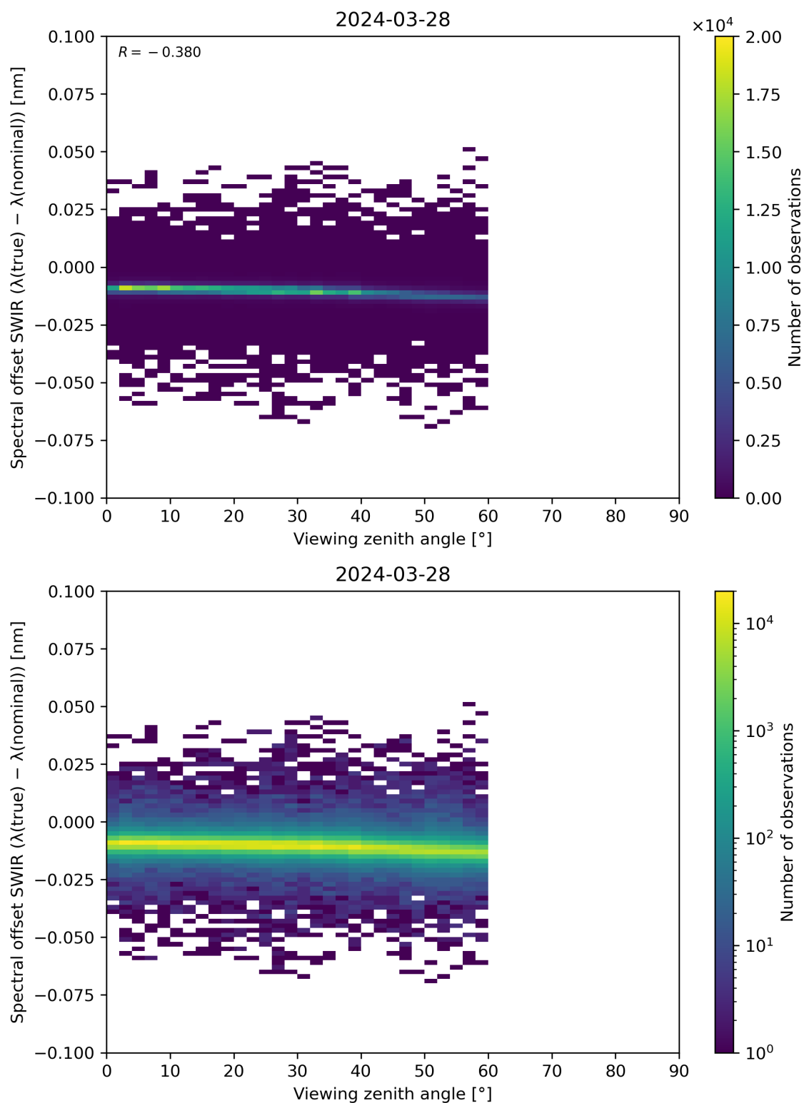
Figure 116: Scatter density plot of “Viewing zenith angle” against “Spectral offset SWIR ( \lambda(\text{true}) - \lambda(\text{nominal}) )” for 2024-03-27 to 2024-03-29.
