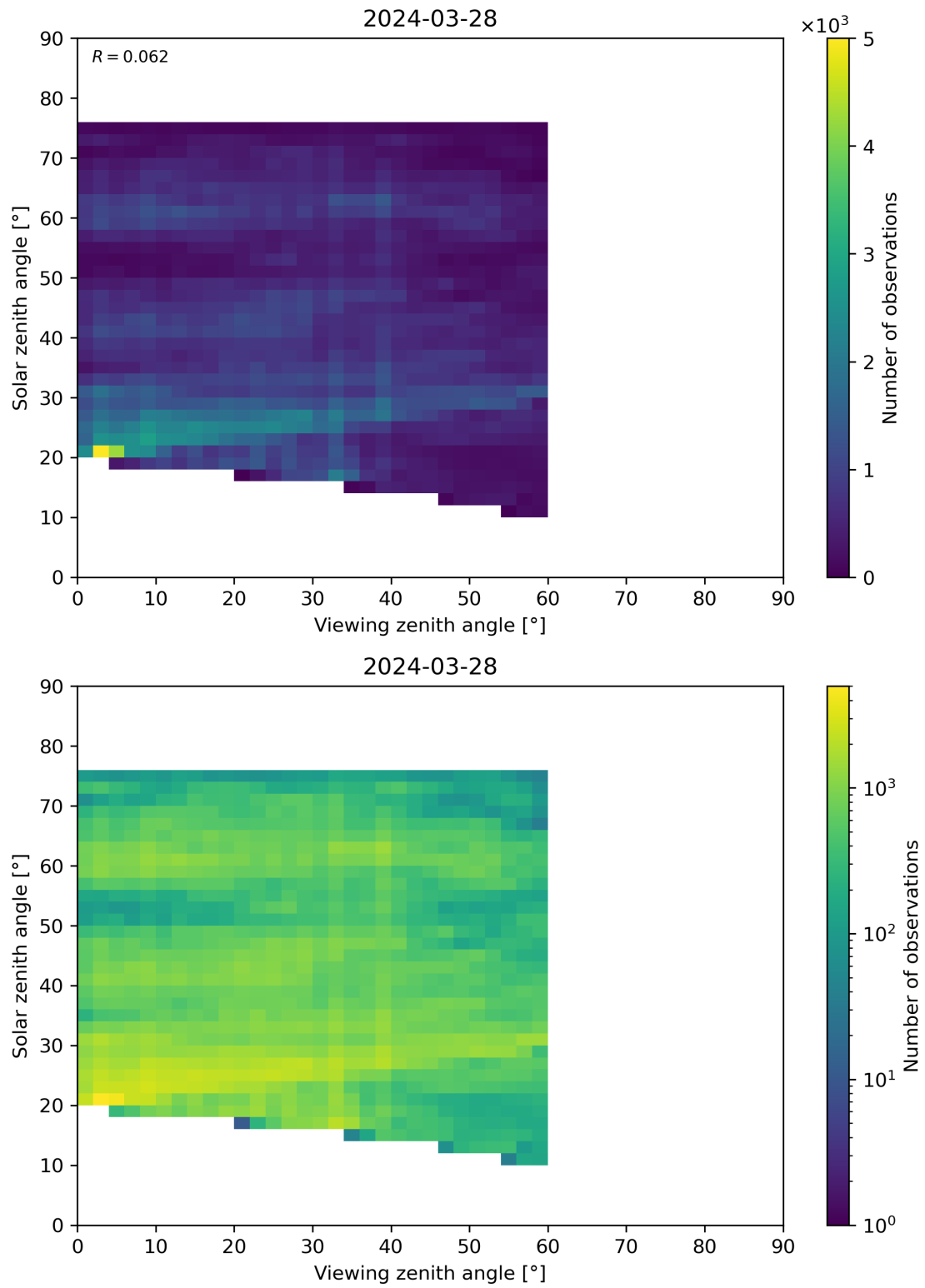
Figure 115: Scatter density plot of “Viewing zenith angle” against “Solar zenith angle” for 2024-03-27 to 2024-03-29.
