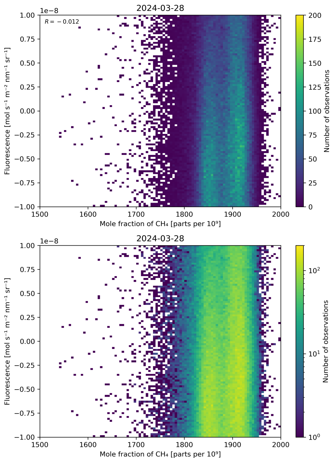
Figure 73: Scatter density plot of “Mole fraction of \text{CH}_4 ” against “Fluorescence” for 2024-03-27 to 2024-03-29.
