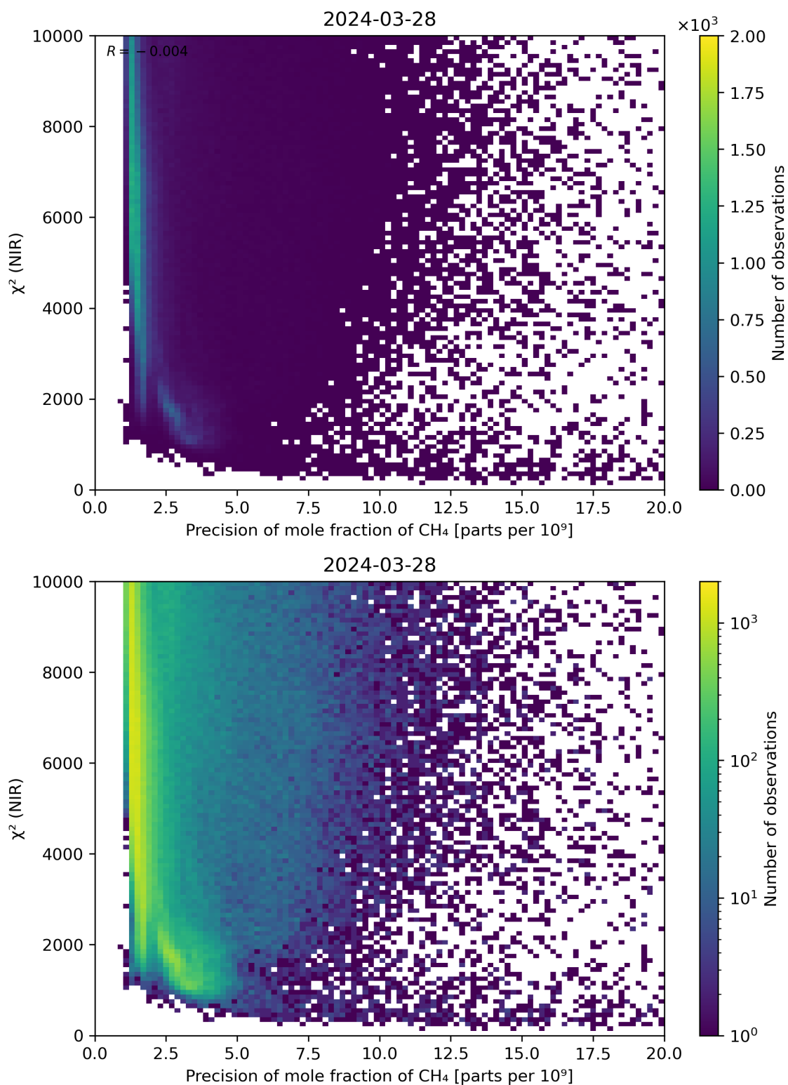
Figure 78: Scatter density plot of “Precision of mole fraction of CH 4 ” against “ \chi^2 (NIR)” for 2024-03-27 to 2024-03-29.
