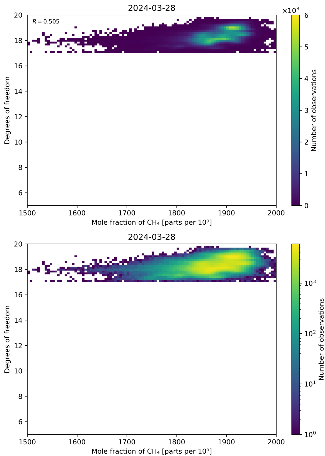
Figure 72: Scatter density plot of “Mole fraction of CH 4 ” against “Degrees of freedom” for 2024-03-27 to 2024-03-29.
