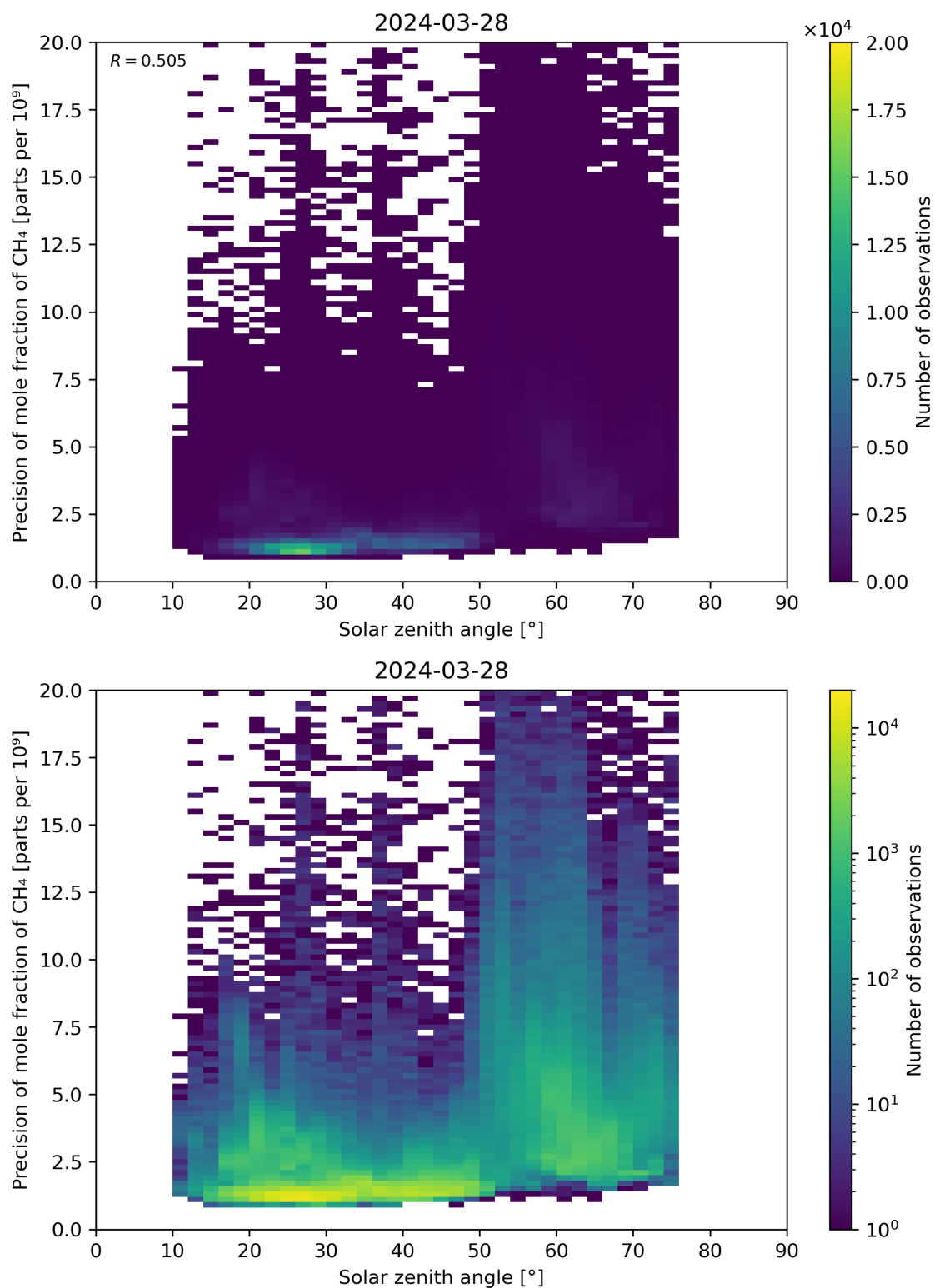
Figure 101: Scatter density plot of “Solar zenith angle” against “Precision of mole fraction of CH 4 ” for 2024-03-27 to 2024-03-29.
