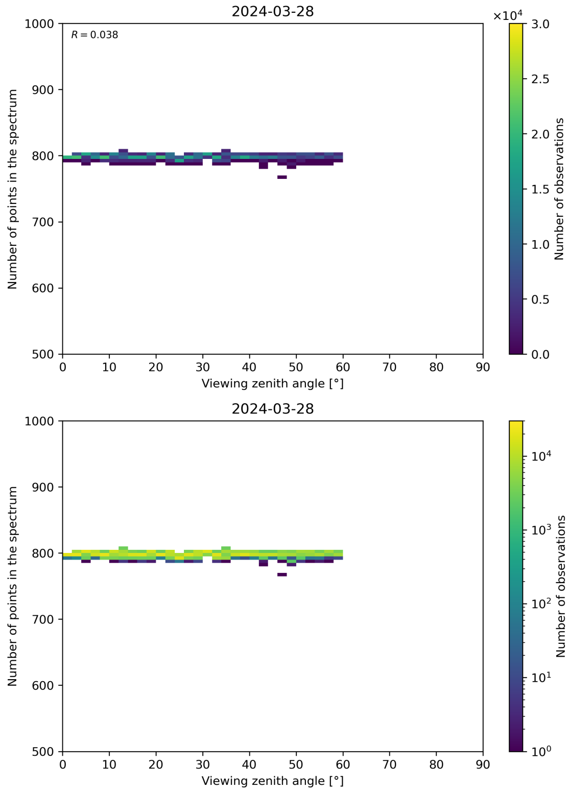
Figure 114: Scatter density plot of “Viewing zenith angle” against “Number of points in the spectrum” for 2024-03-27 to 2024-03-29.
