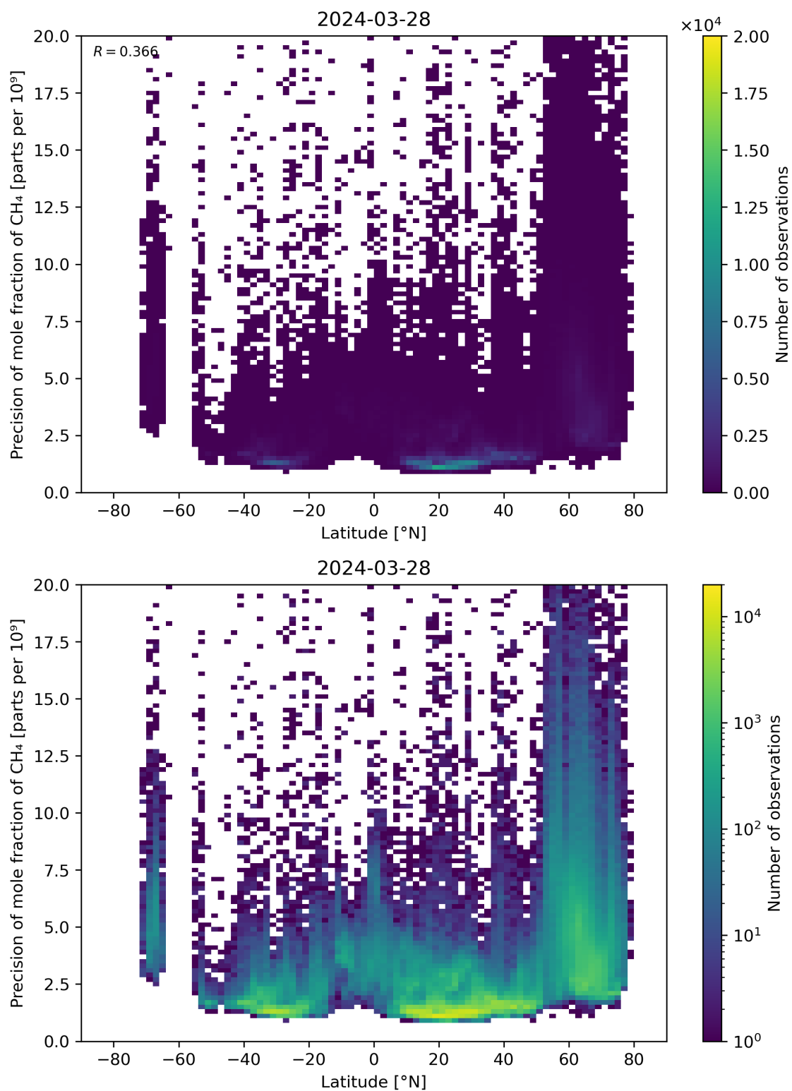
Figure 59: Scatter density plot of “Latitude” against “Precision of mole fraction of \text{CH}_4 ” for 2024-03-27 to 2024-03-29.
