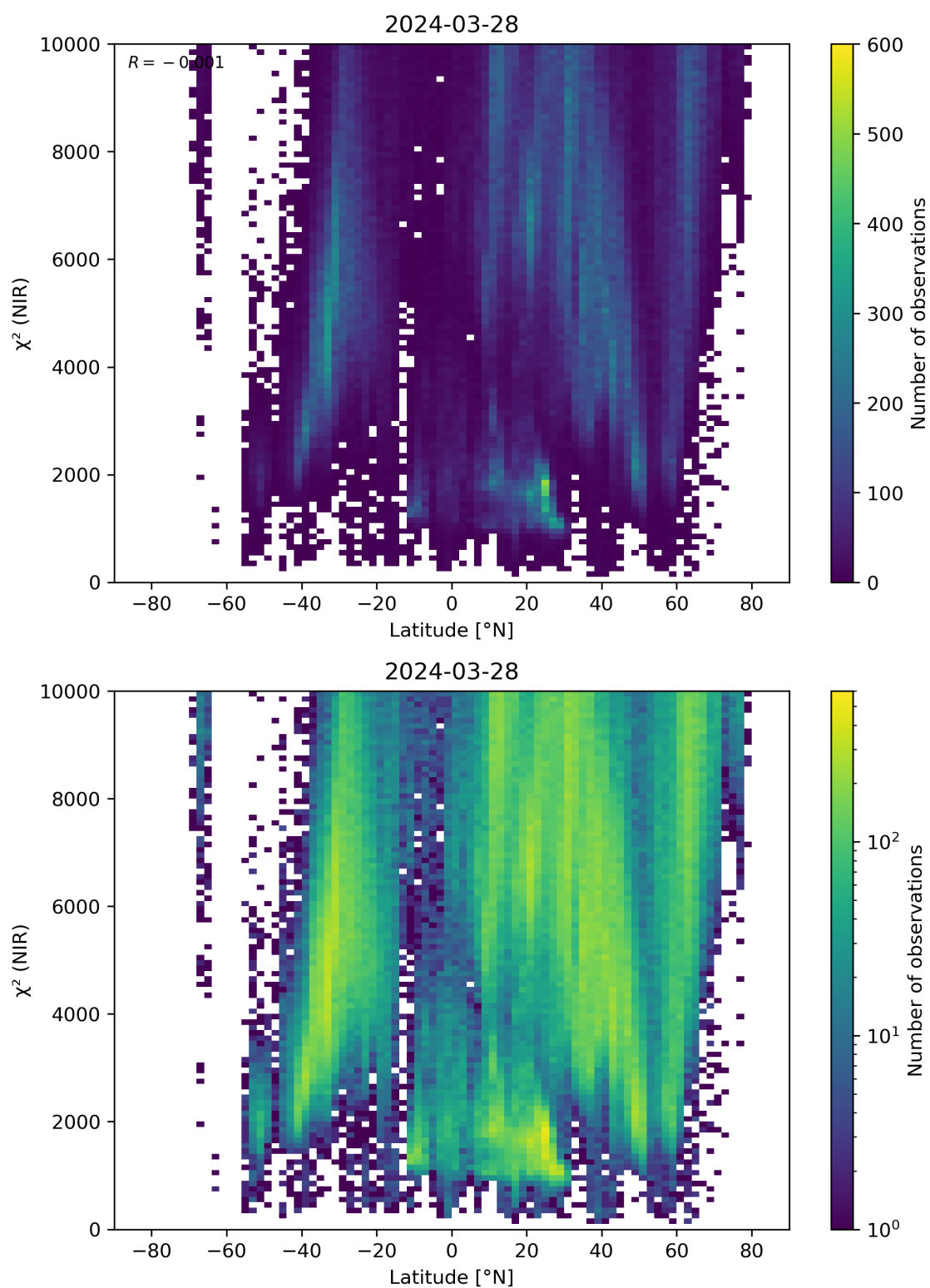
Figure 53: Scatter density plot of “Latitude” against “ \chi^2 (NIR)” for 2024-03-27 to 2024-03-29.
