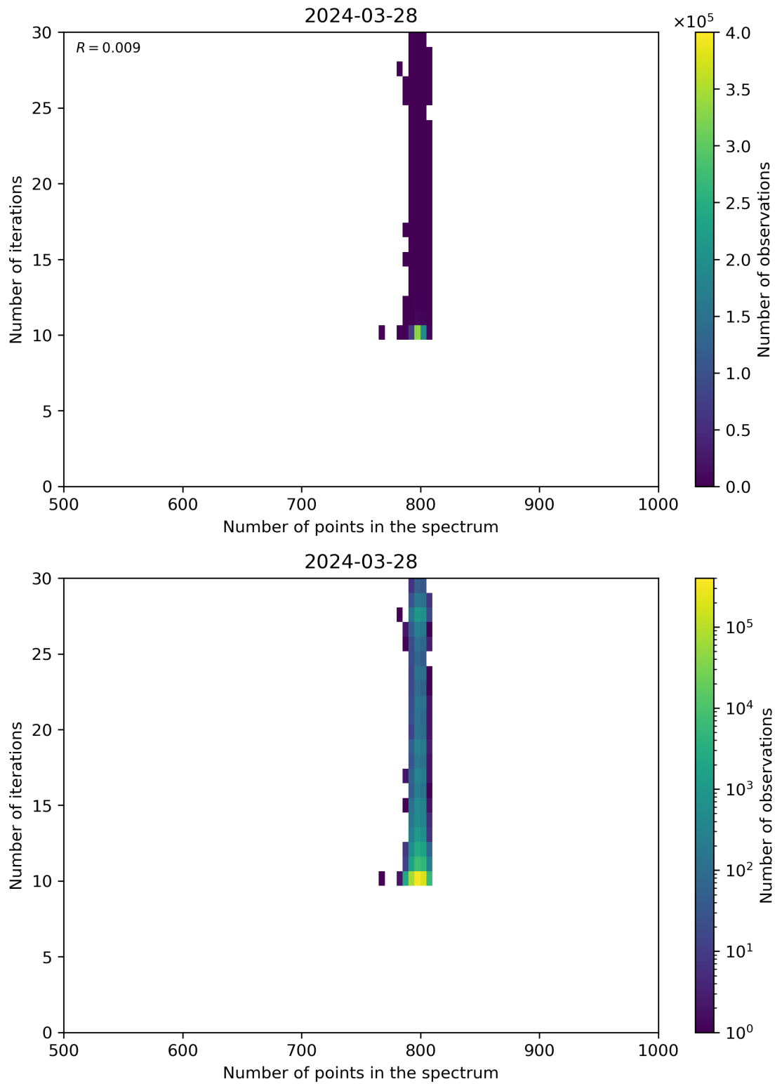
Figure 92: Scatter density plot of “Number of points in the spectrum” against “Number of iterations” for 2024-03-27 to 2024-03-29.
