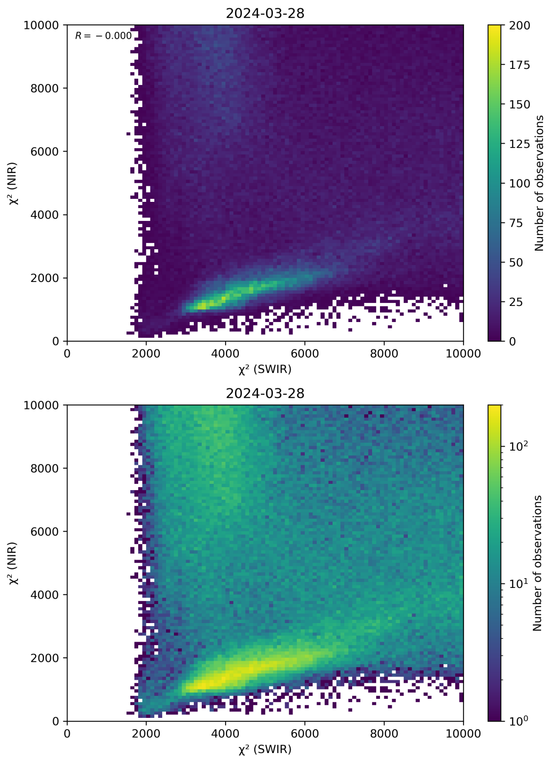
Figure 47: Scatter density plot of “ \chi^2 (SWIR)” against “ \chi^2 (NIR)” for 2024-03-27 to 2024-03-29.
