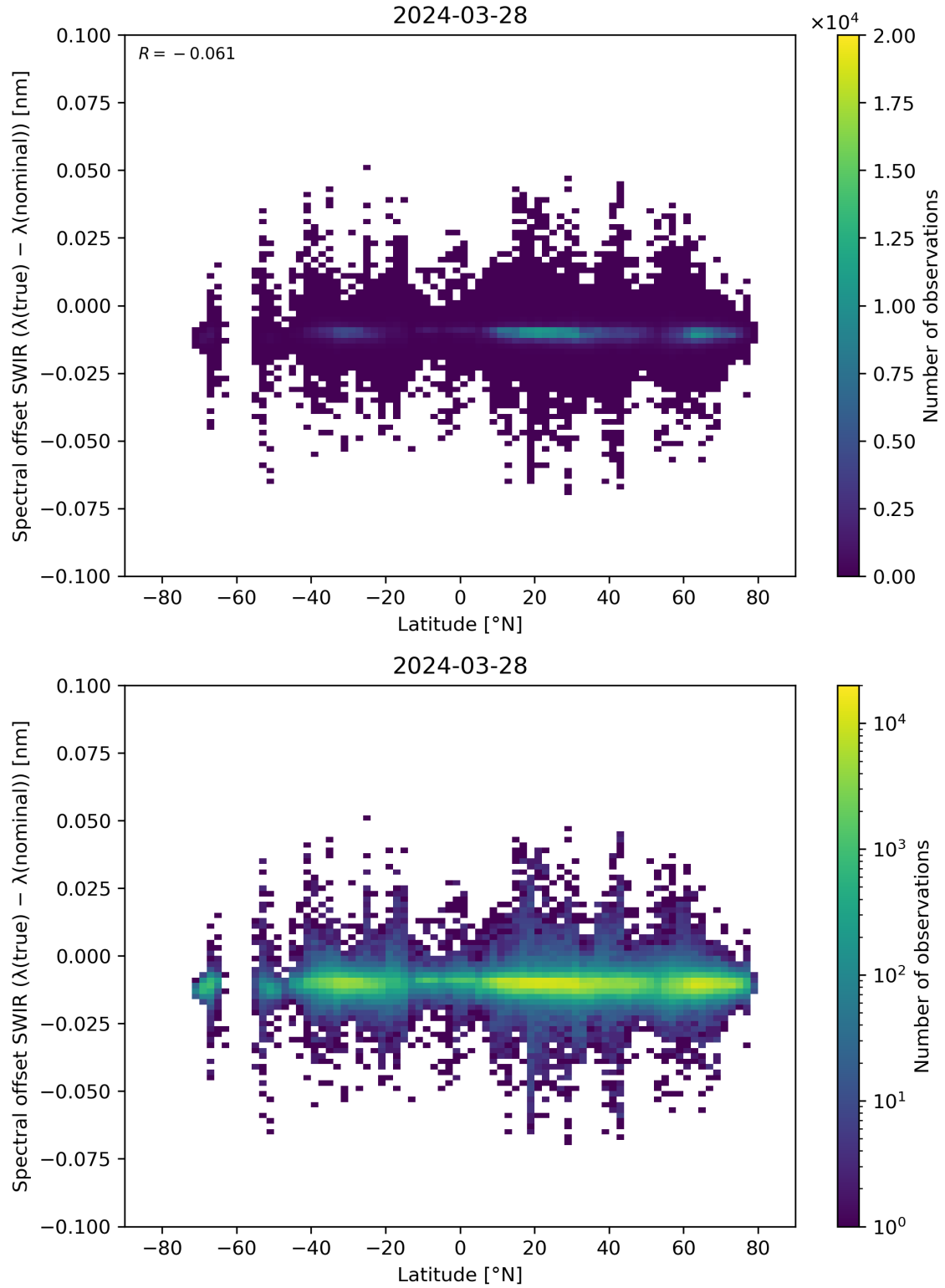
Figure 62: Scatter density plot of “Latitude” against “Spectral offset SWIR ( \lambda(\text{true}) - \lambda(\text{nominal}) )” for 2024-03-27 to 2024-03-29.
