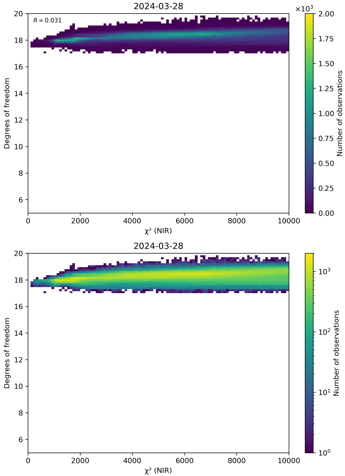
Figure 44: Scatter density plot of “ \chi^2 (NIR)” against “Degrees of freedom” for 2024-03-27 to 2024-03-29.
