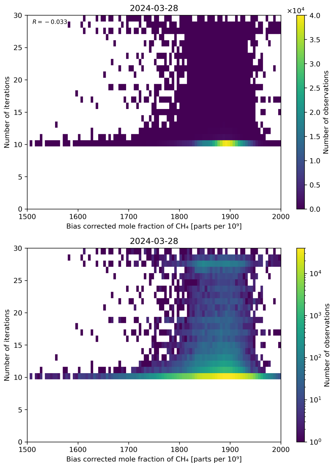
Figure 67: Scatter density plot of “Bias corrected mole fraction of \text{CH}_4 ” against “Number of iterations” for 2024-03-27 to 2024-03-29.
