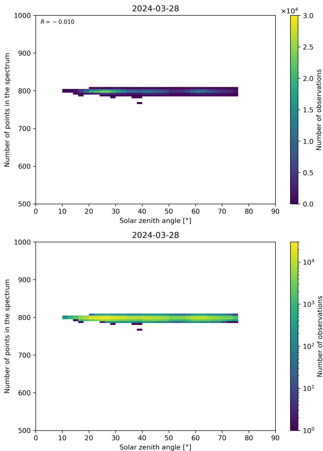
Figure 103: Scatter density plot of “Solar zenith angle” against “Number of points in the spectrum” for 2024-03-27 to 2024-03-29.
