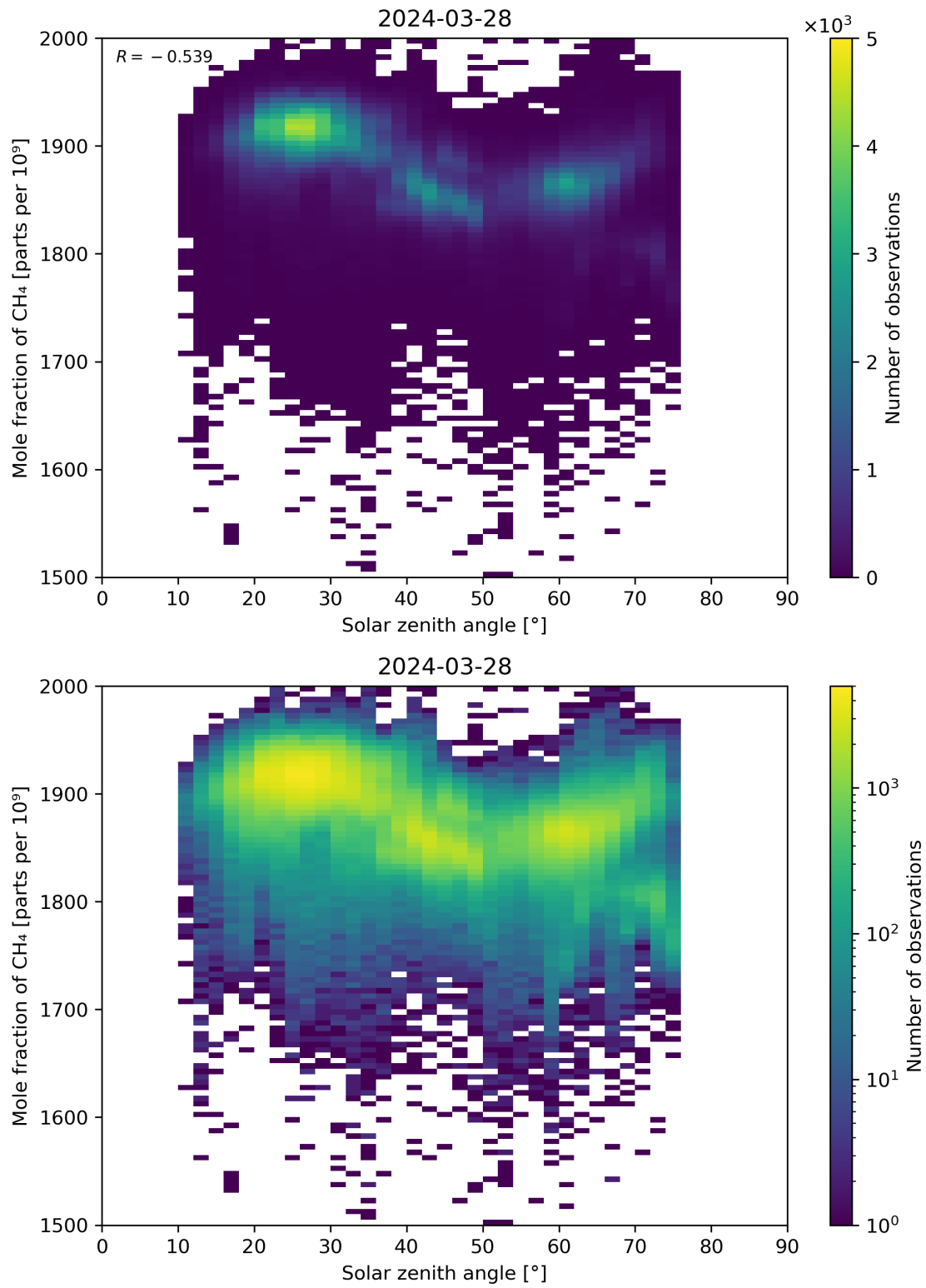
Figure 99: Scatter density plot of “Solar zenith angle” against “Mole fraction of CH 4 ” for 2024-03-27 to 2024-03-29.
