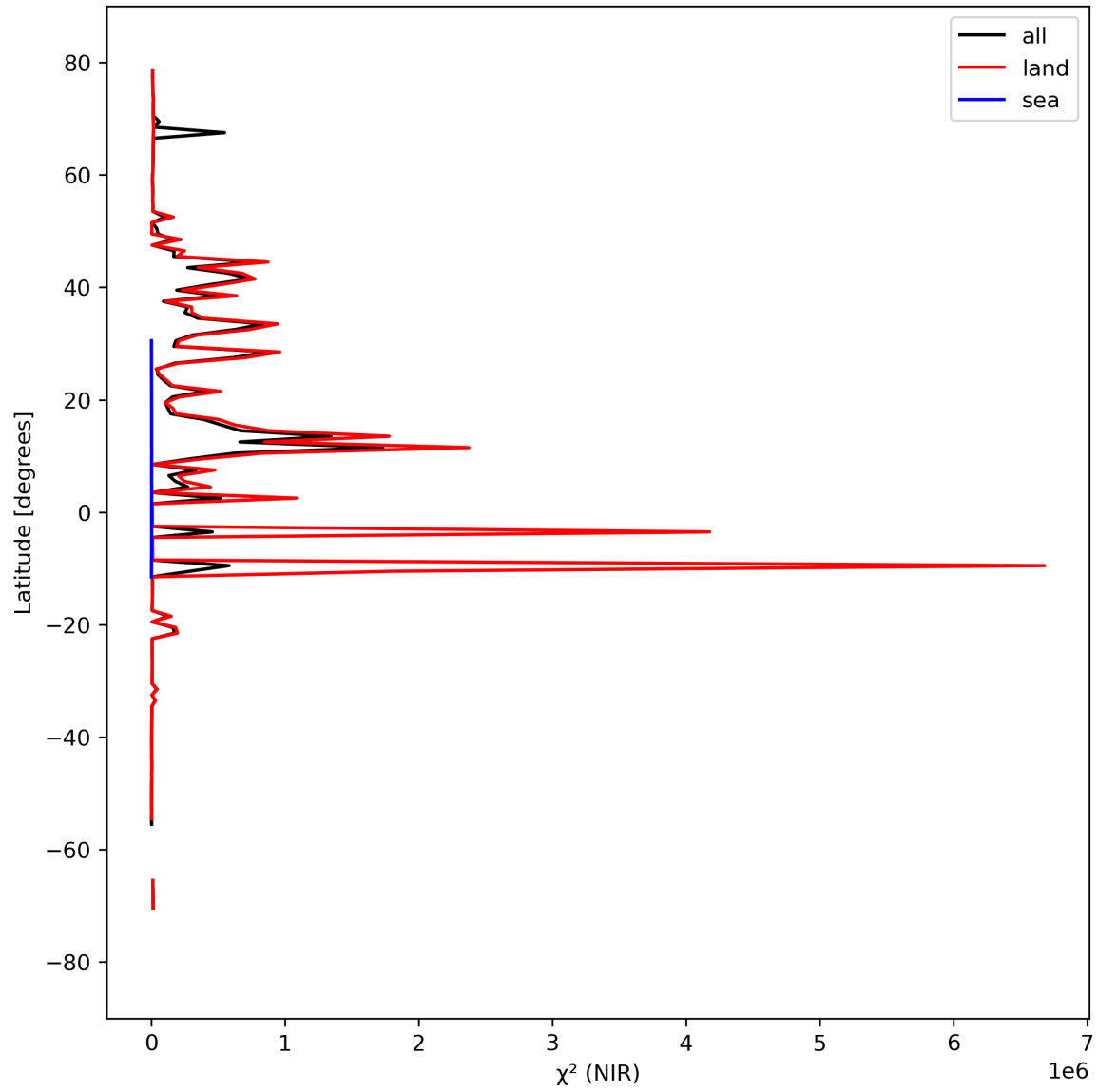
Figure 18: Zonal average of “ \chi^2 (NIR)” for 2024-03-27 to 2024-03-29.
