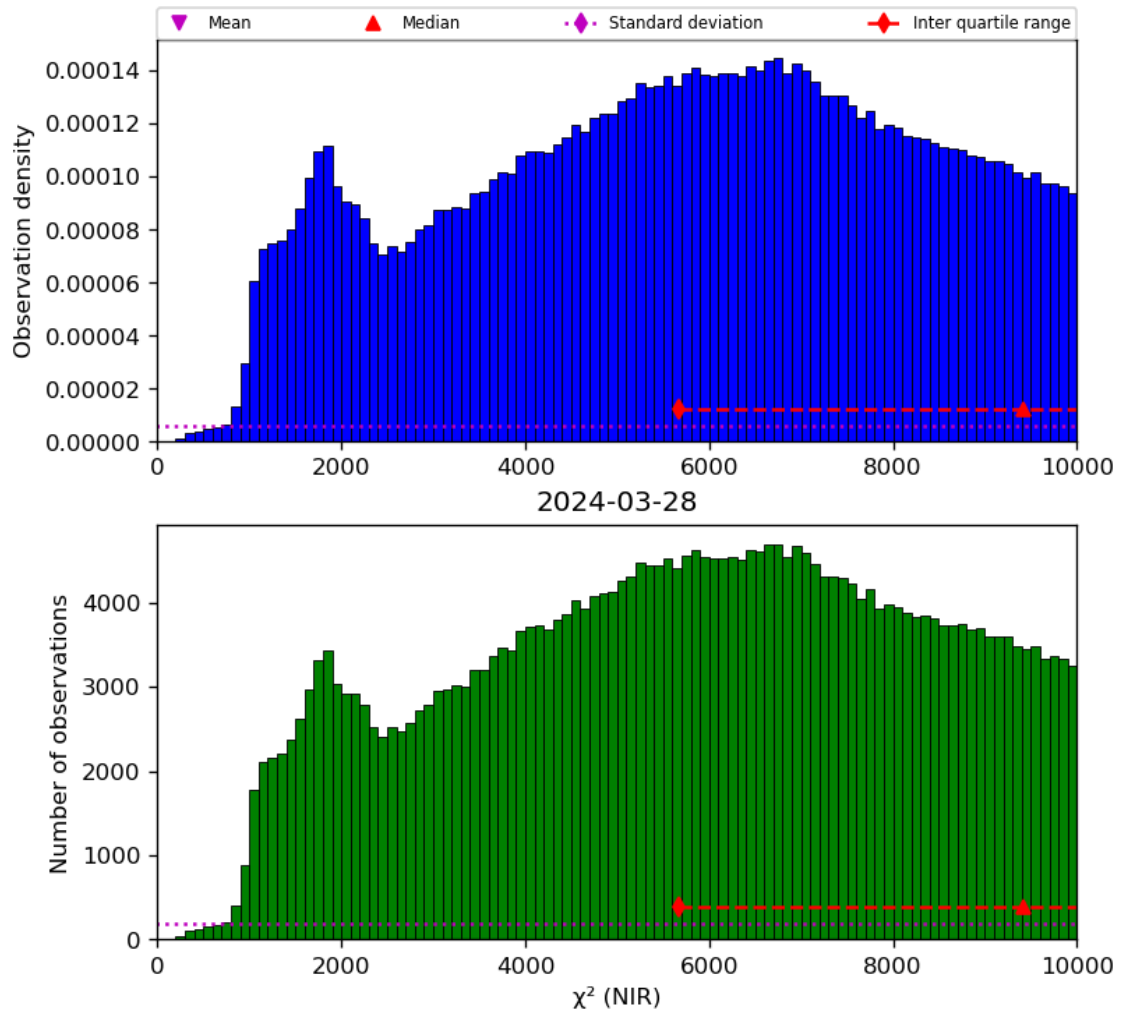
Figure 29: Histogram of “ \chi^2 (NIR)” for 2024-03-27 to 2024-03-29
