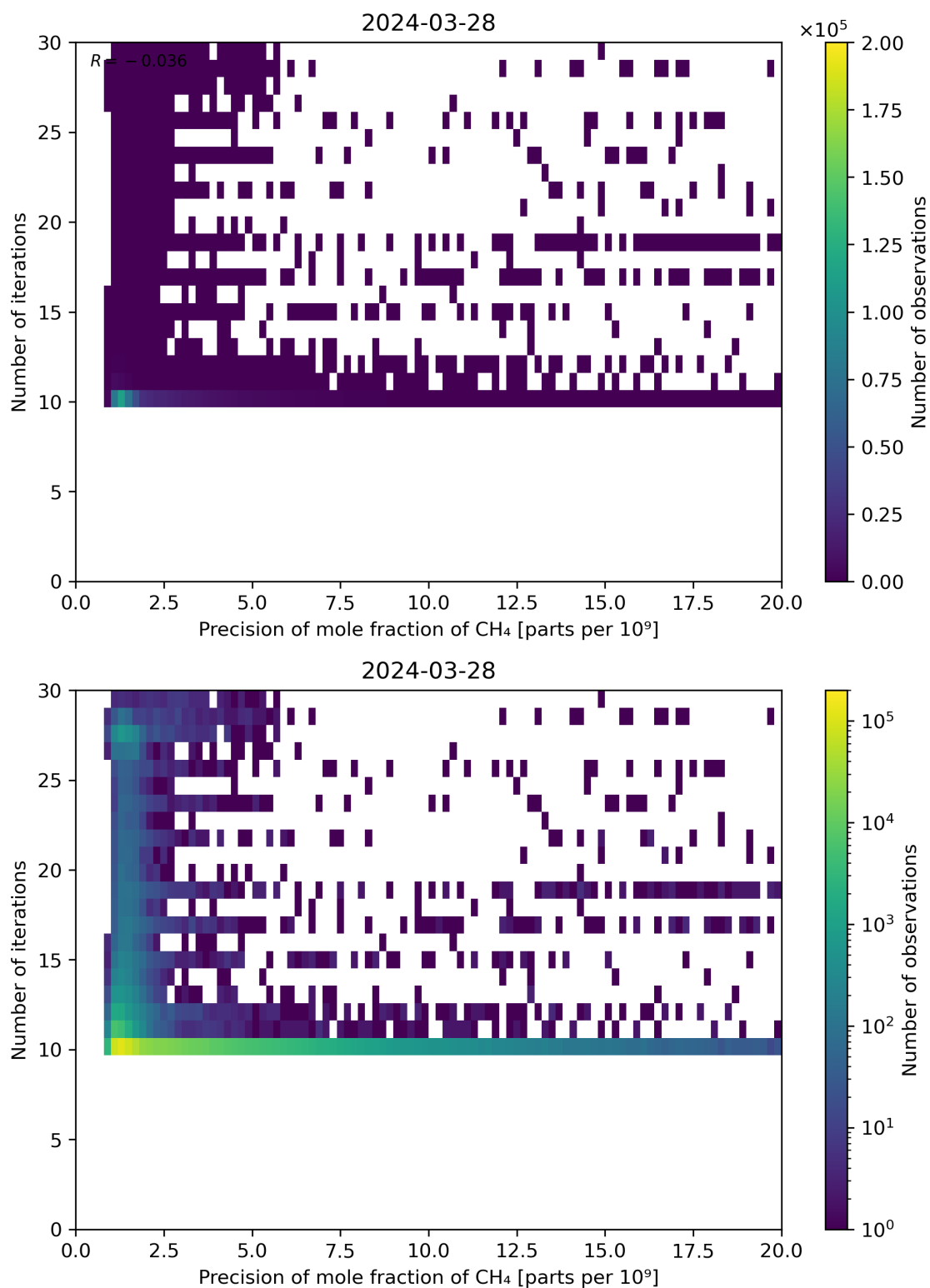
Figure 83: Scatter density plot of “Precision of mole fraction of CH 4 ” against “Number of iterations” for 2024-03-27 to 2024-03-29.
