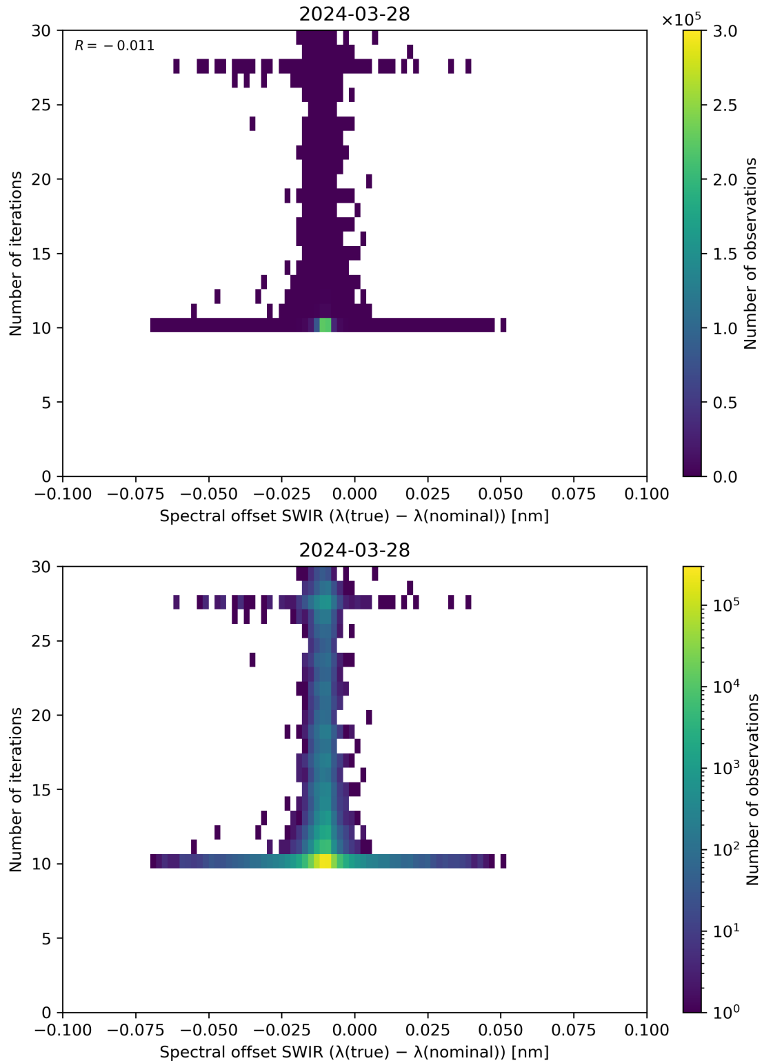
Figure 121: Scatter density plot of “Spectral offset SWIR ( \lambda(\text{true}) - \lambda(\text{nominal}) )” against “Number of iterations” for 2024-03-27 to 2024-03-29.
