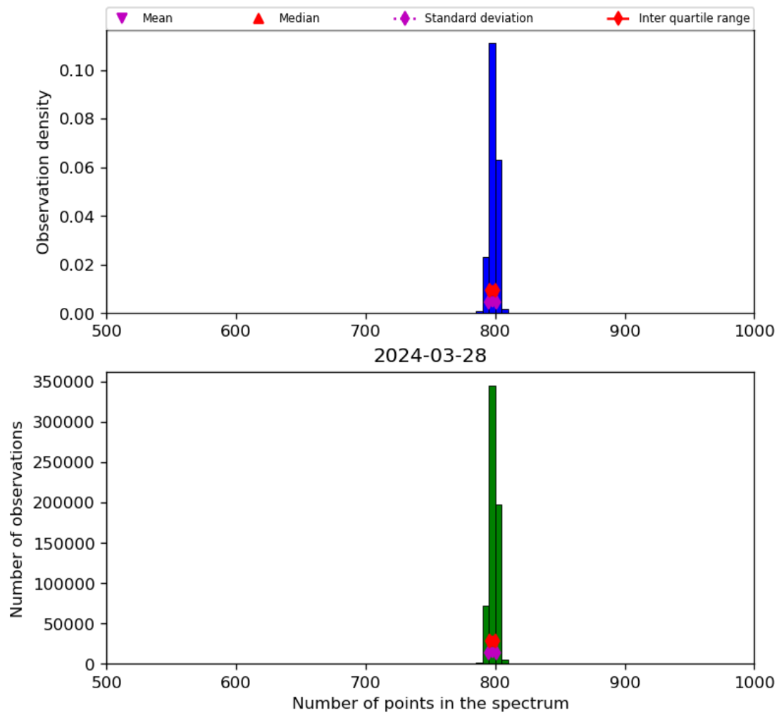
Figure 26: Histogram of “Number of points in the spectrum” for 2024-03-27 to 2024-03-29
