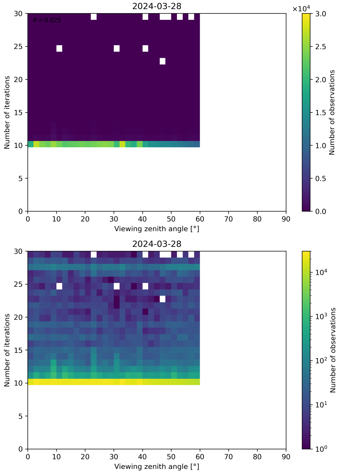
Figure 113: Scatter density plot of “Viewing zenith angle” against “Number of iterations” for 2024-03-27 to 2024-03-29.
