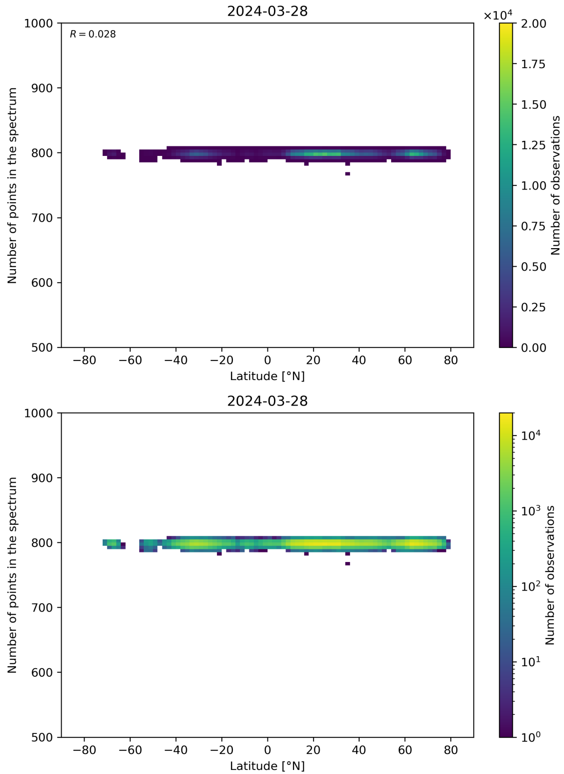
Figure 61: Scatter density plot of “Latitude” against “Number of points in the spectrum” for 2024-03-27 to 2024-03-29.
