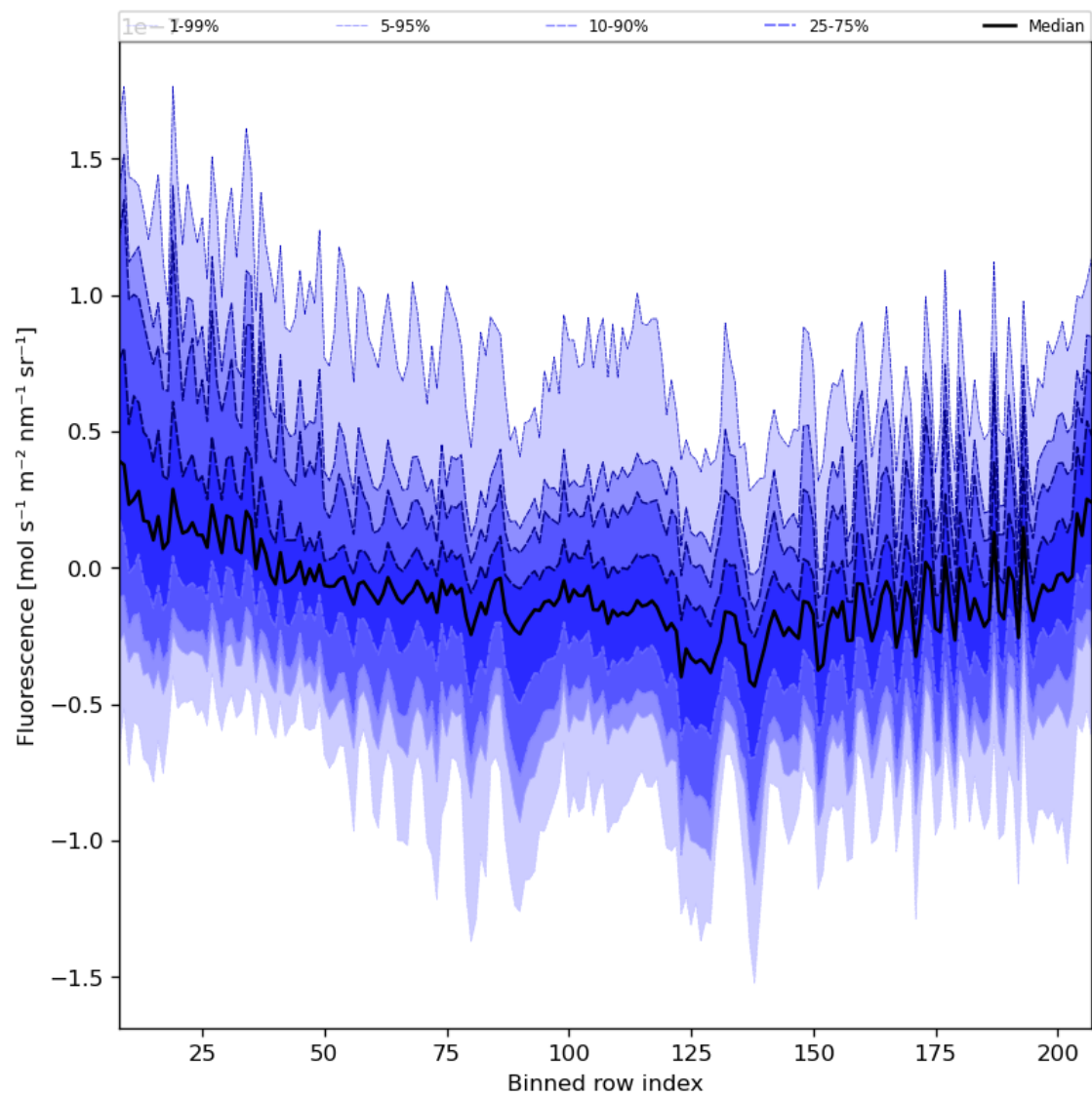
Figure 43: Along track statistics of “Fluorescence” for 2024-03-27 to 2024-03-29
