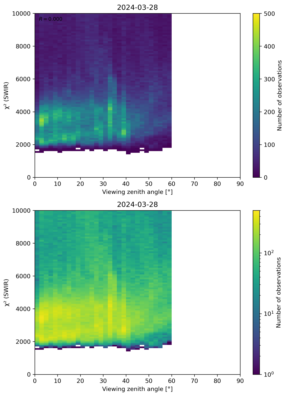
Figure 106: Scatter density plot of “Viewing zenith angle” against “ \chi^2 (SWIR)” for 2024-03-27 to 2024-03-29.
