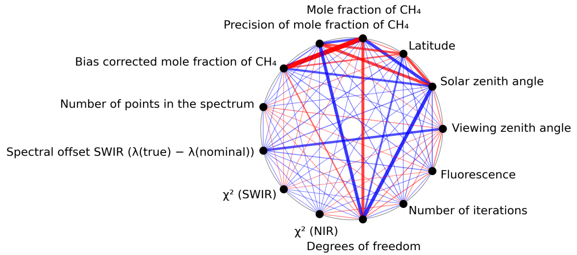
Figure 1: Map of correlation graph for 2024-03-27 to 2024-03-29.
