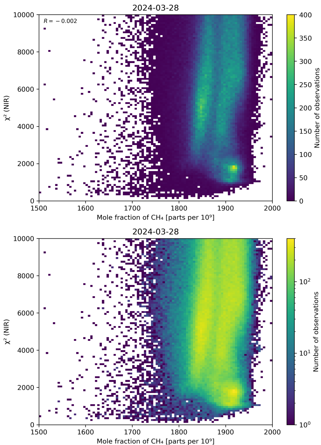
Figure 70: Scatter density plot of “Mole fraction of CH 4 ” against “ \chi^2 (NIR)” for 2024-03-27 to 2024-03-29.
