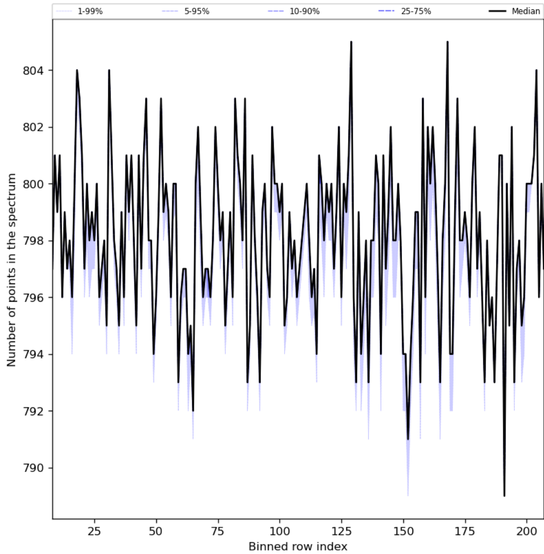
Figure 37: Along track statistics of “Number of points in the spectrum” for 2024-03-27 to 2024-03-29
