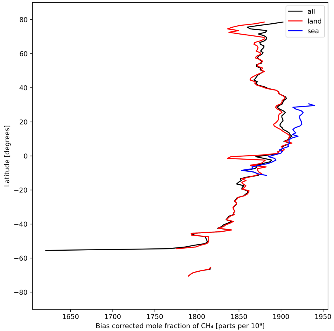
Figure 14: Zonal average of “Bias corrected mole fraction of CH 4 ” for 2024-03-27 to 2024-03-29.
