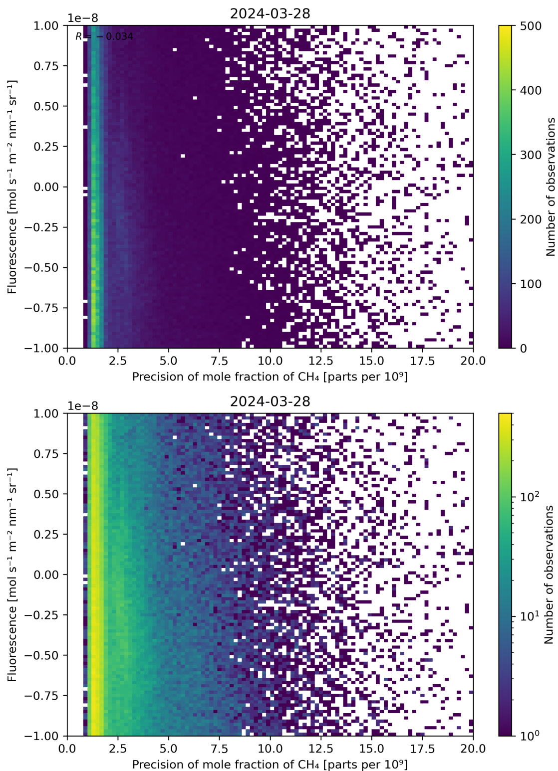
Figure 81: Scatter density plot of “Precision of mole fraction of \text{CH}_4 ” against “Fluorescence” for 2024-03-27 to 2024-03-29.
