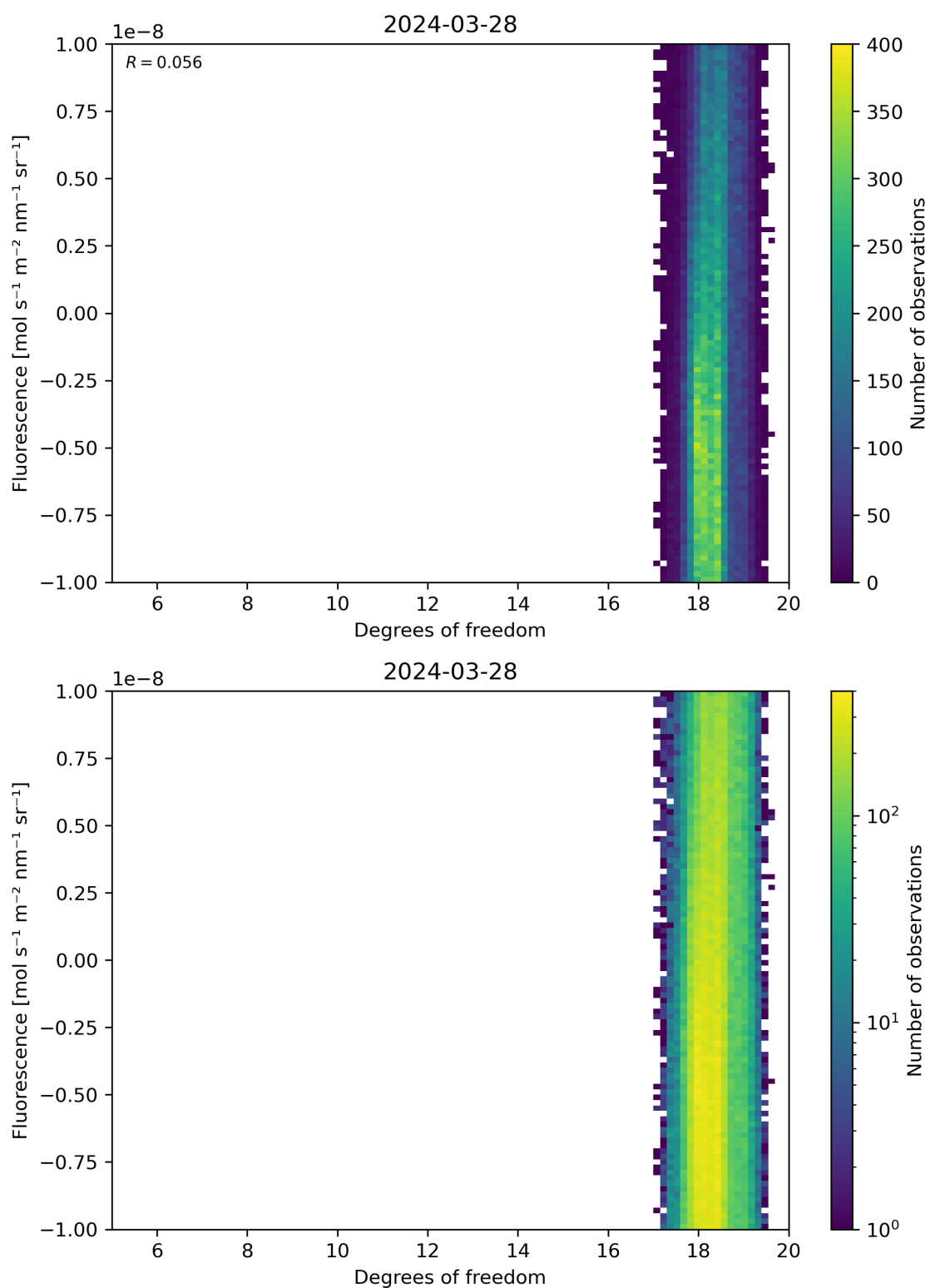
Figure 51: Scatter density plot of “Degrees of freedom” against “Fluorescence” for 2024-03-27 to 2024-03-29.
