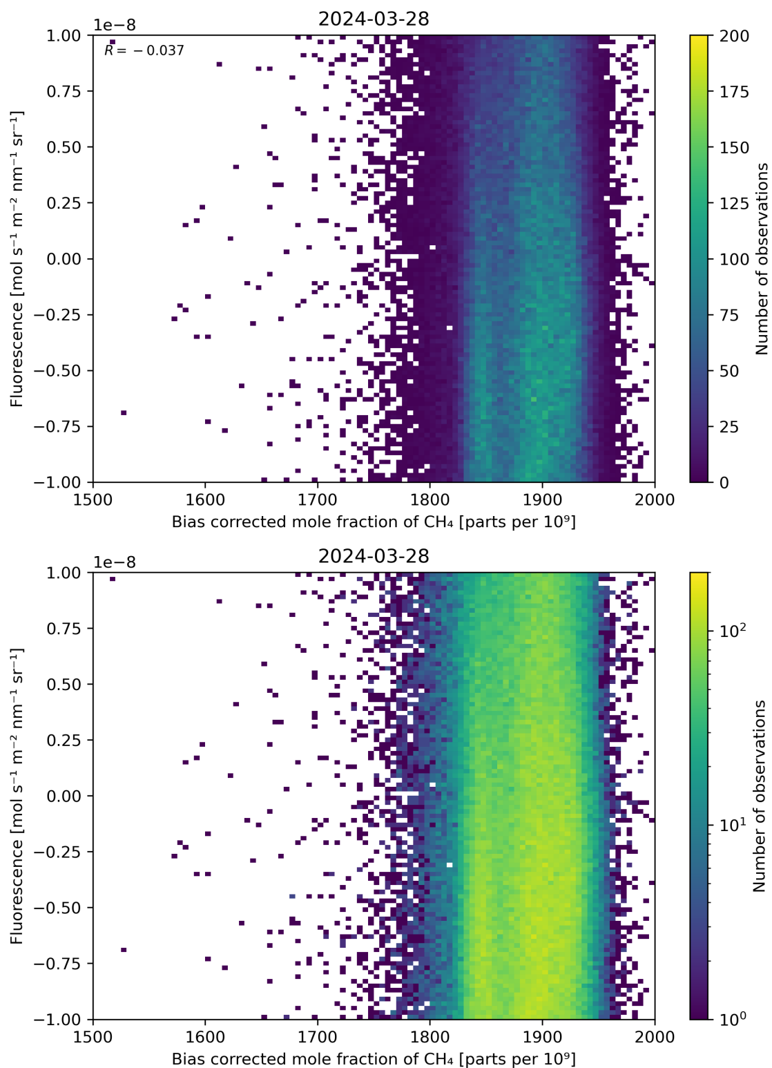
Figure 66: Scatter density plot of “Bias corrected mole fraction of \text{CH}_4 ” against “Fluorescence” for 2024-03-27 to 2024-03-29.
