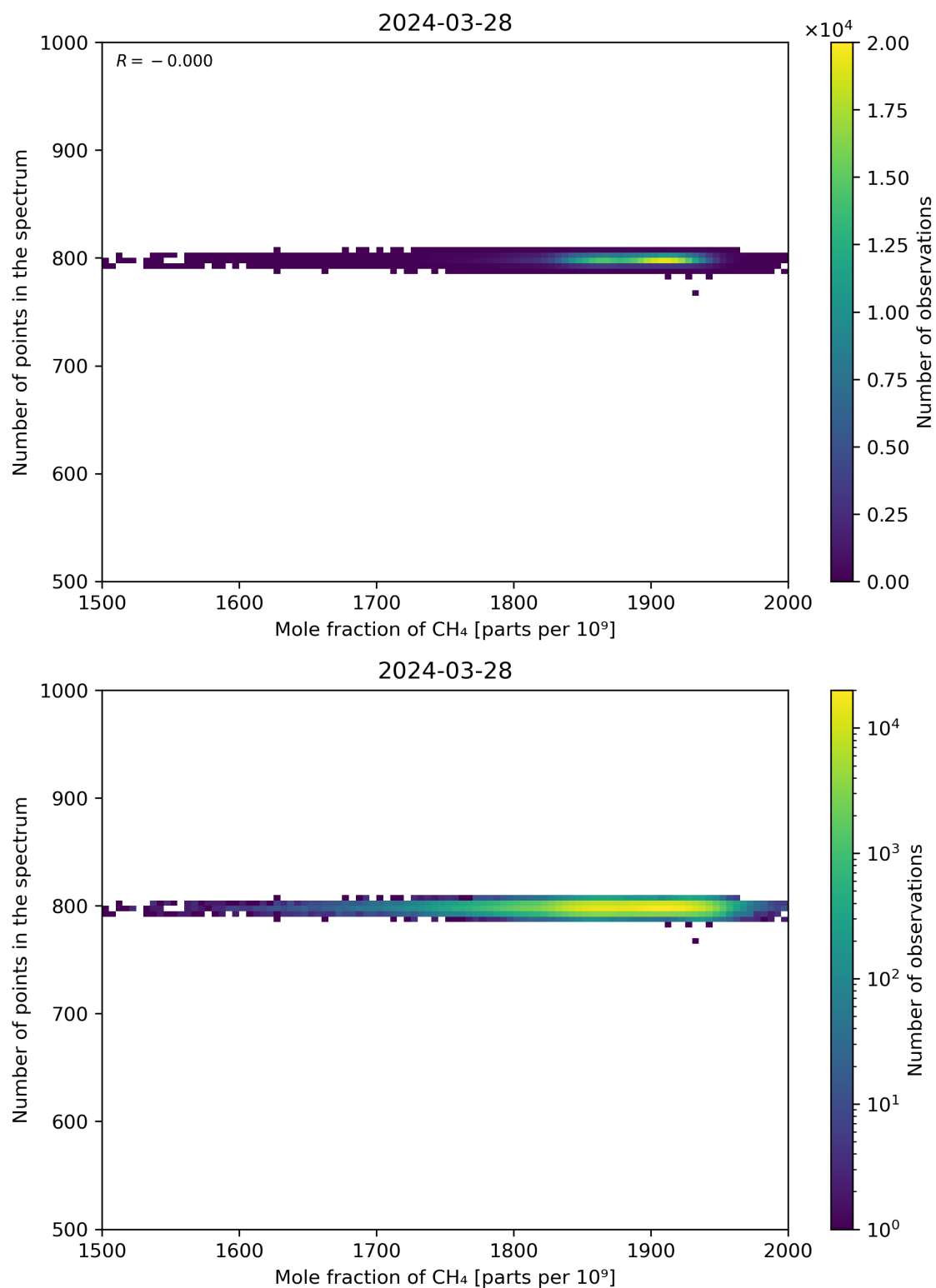
Figure 77: Scatter density plot of “Mole fraction of CH 4 ” against “Number of points in the spectrum” for 2024-03-27 to 2024-03-29.
