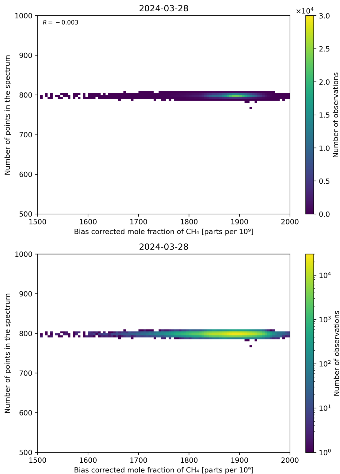
Figure 68: Scatter density plot of “Bias corrected mole fraction of CH 4 ” against “Number of points in the spectrum” for 2024-03-27 to 2024-03-29.
