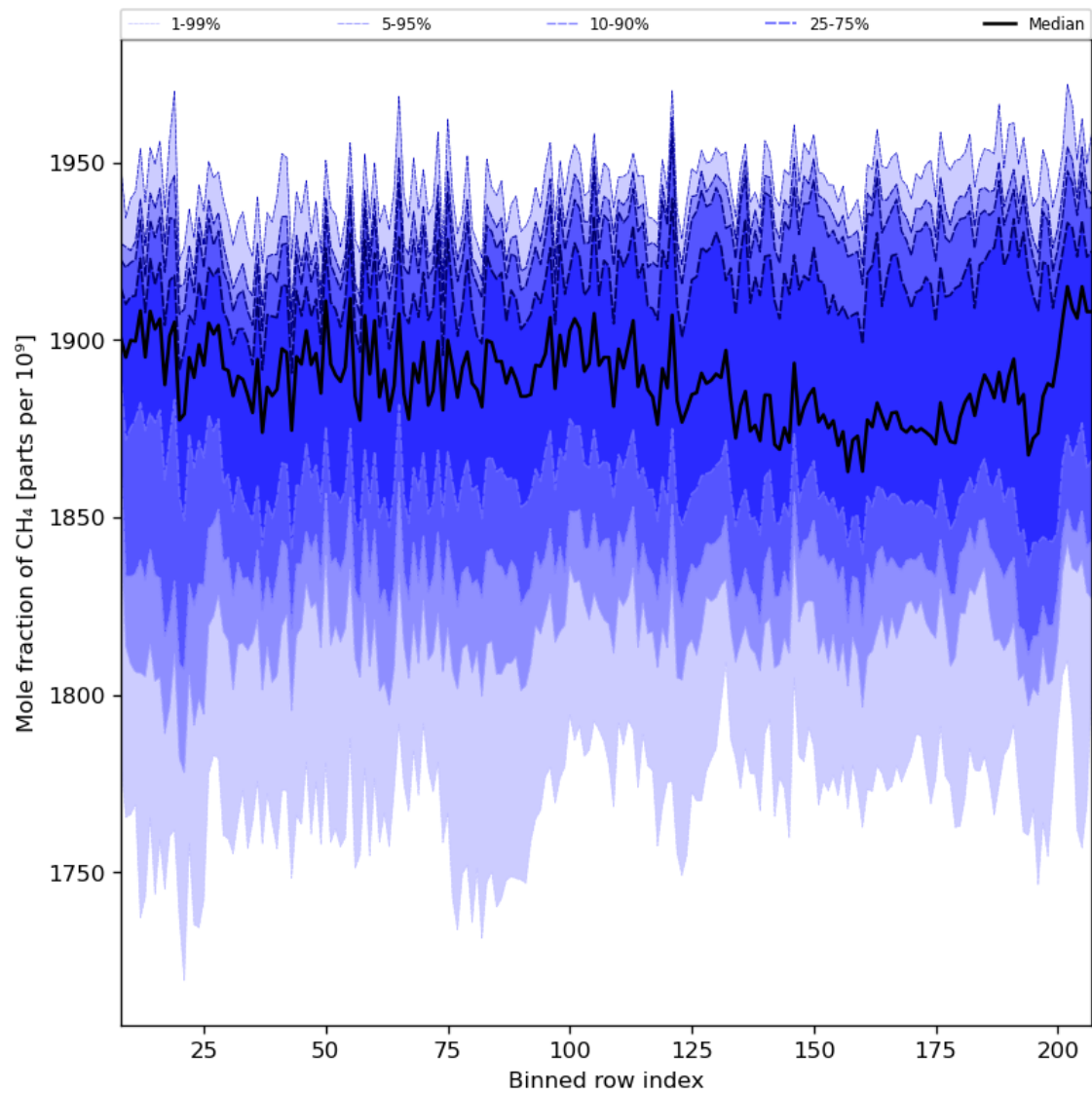
Figure 34: Along track statistics of “Mole fraction of CH 4 ” for 2024-03-27 to 2024-03-29
