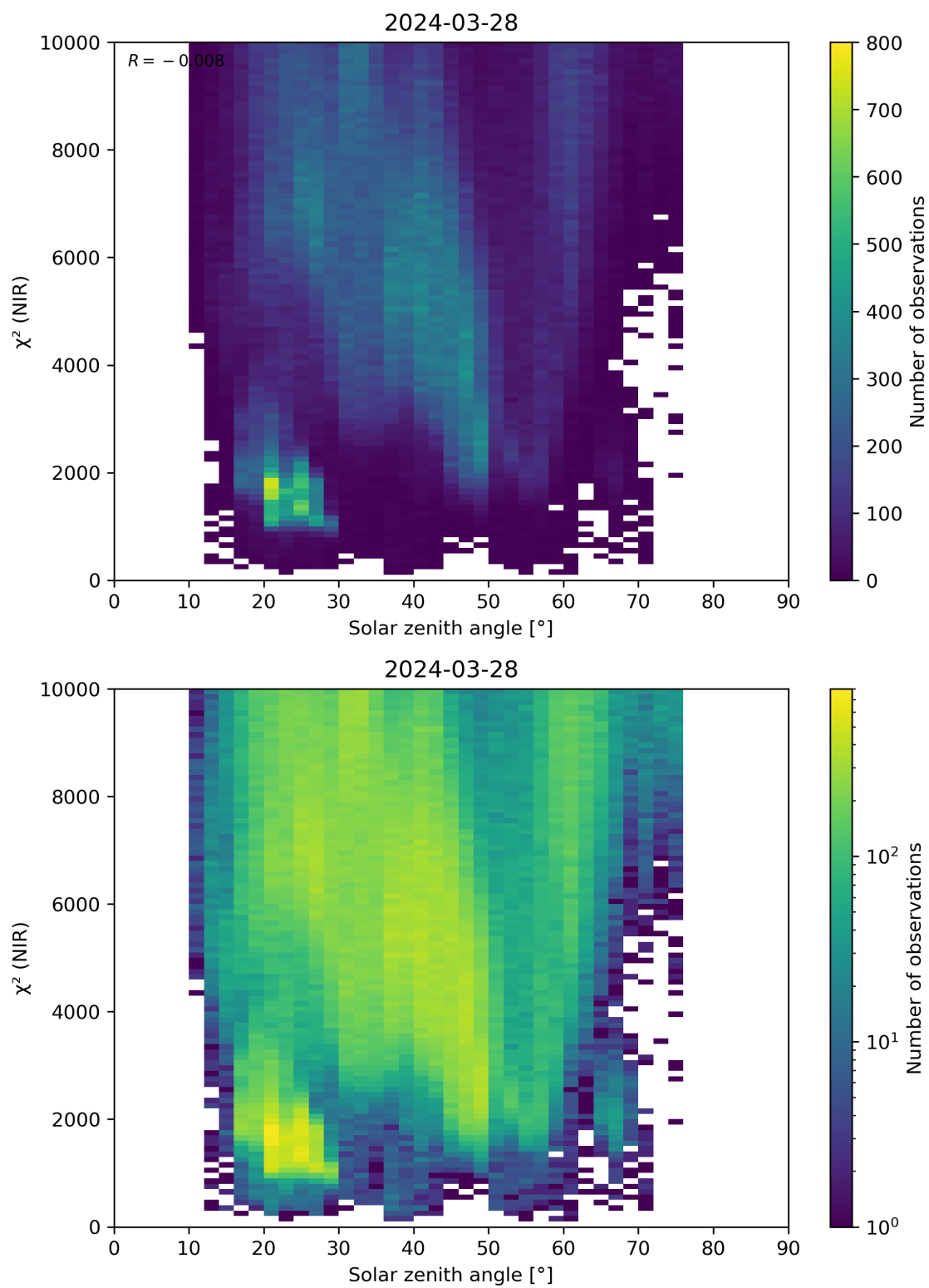
Figure 94: Scatter density plot of “Solar zenith angle” against “ \chi^2 (NIR)” for 2024-03-27 to 2024-03-29.
