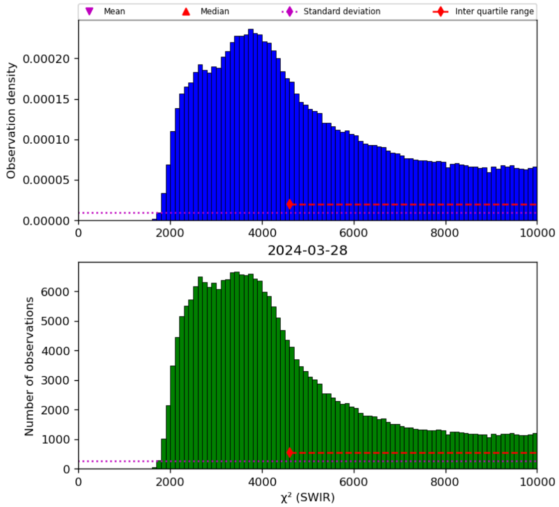
Figure 28: Histogram of “ \chi^2 (SWIR)” for 2024-03-27 to 2024-03-29
