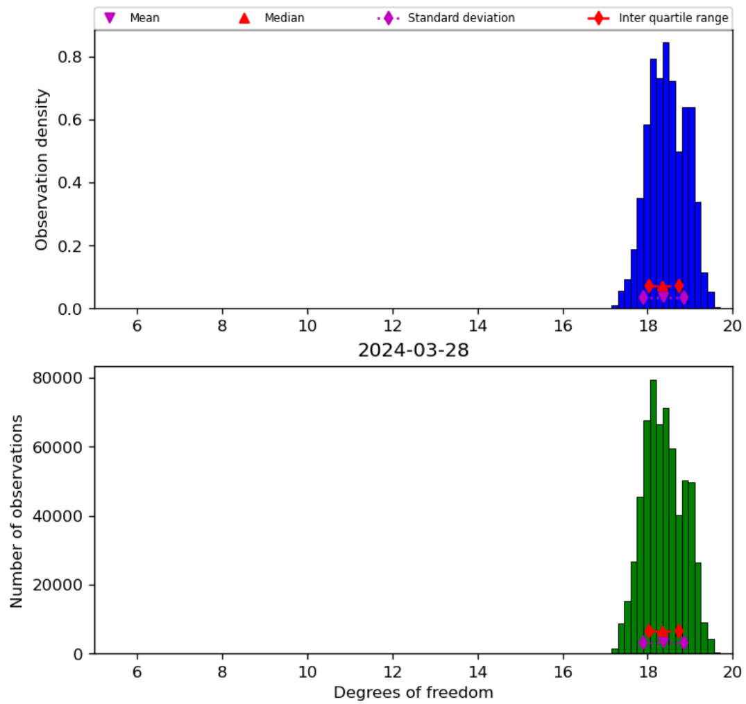
Figure 30: Histogram of “Degrees of freedom” for 2024-03-27 to 2024-03-29
