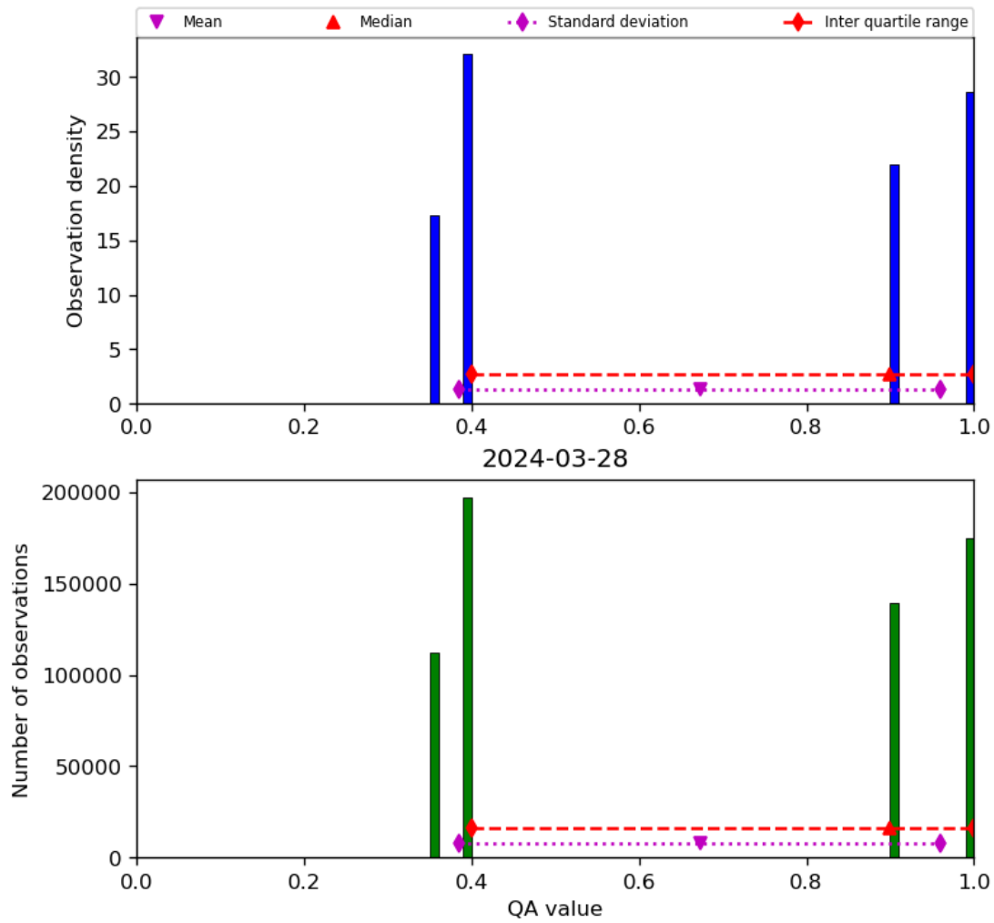
Figure 22: Histogram of “QA value” for 2024-03-27 to 2024-03-29
