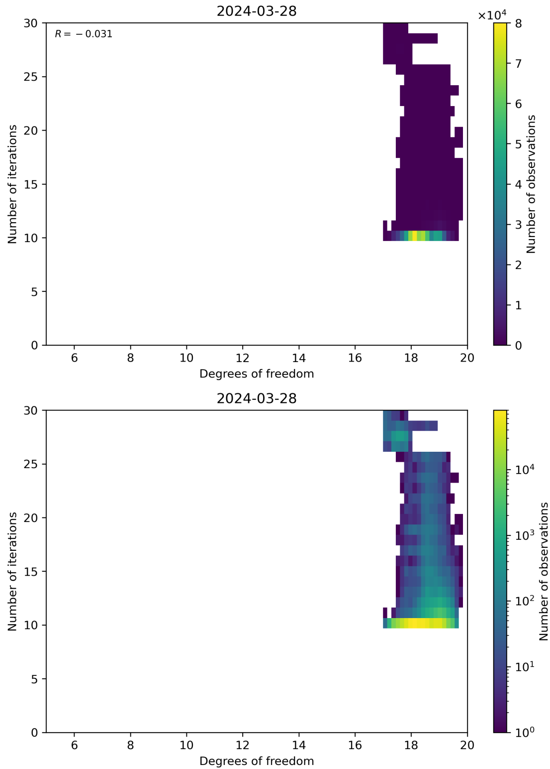
Figure 52: Scatter density plot of “Degrees of freedom” against “Number of iterations” for 2024-03-27 to 2024-03-29.
