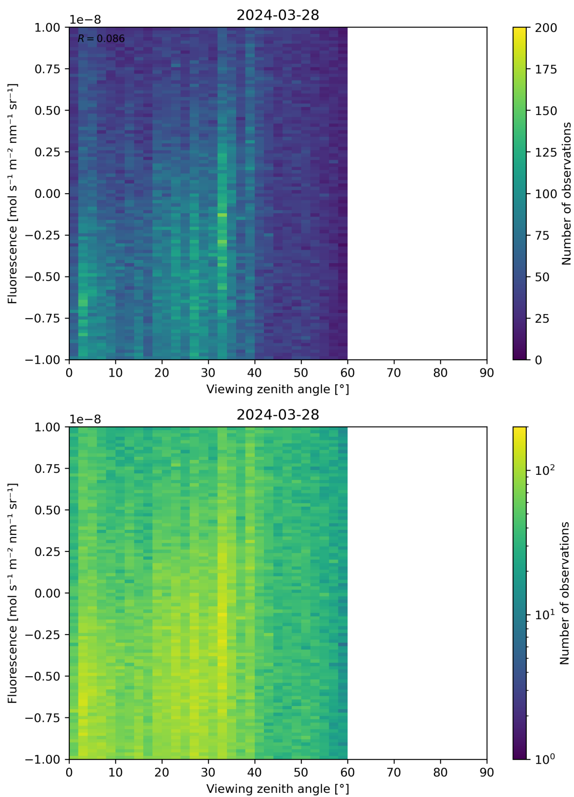
Figure 108: Scatter density plot of “Viewing zenith angle” against “Fluorescence” for 2024-03-27 to 2024-03-29.
