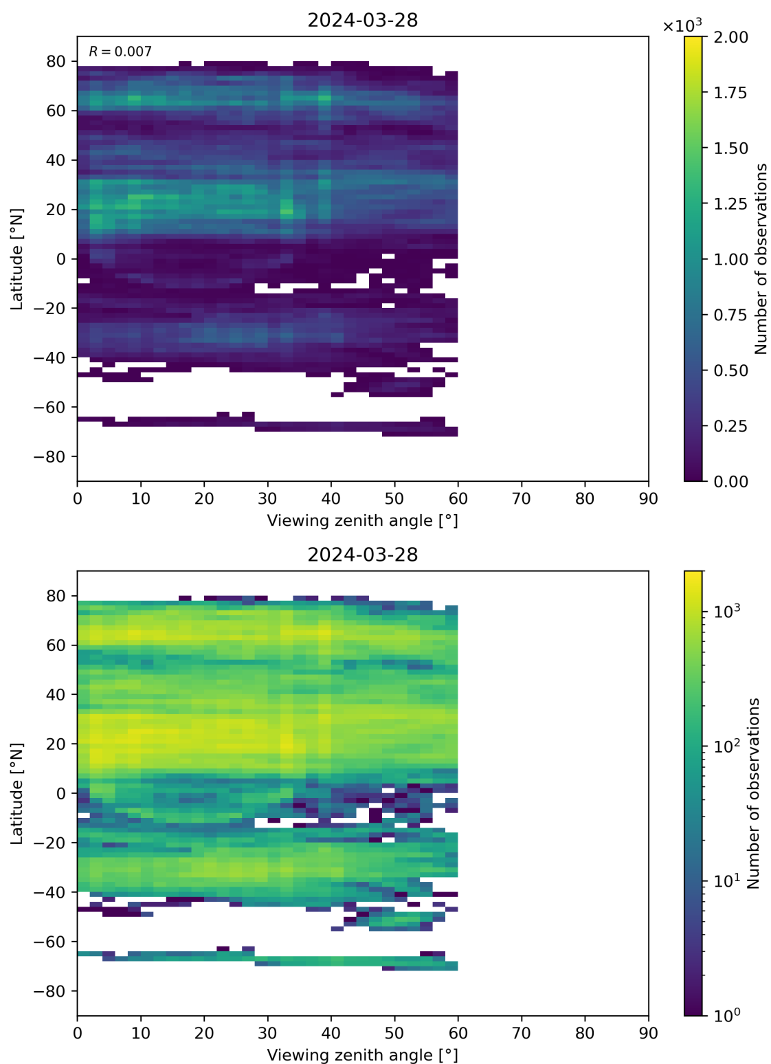
Figure 109: Scatter density plot of “Viewing zenith angle” against “Latitude” for 2024-03-27 to 2024-03-29.
