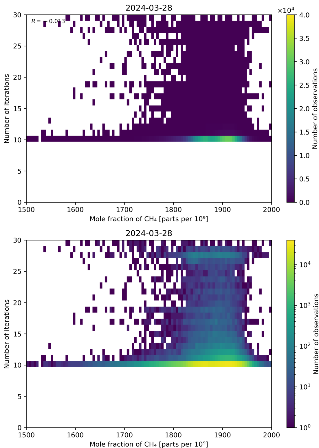
Figure 76: Scatter density plot of “Mole fraction of CH 4 ” against “Number of iterations” for 2024-03-27 to 2024-03-29.
