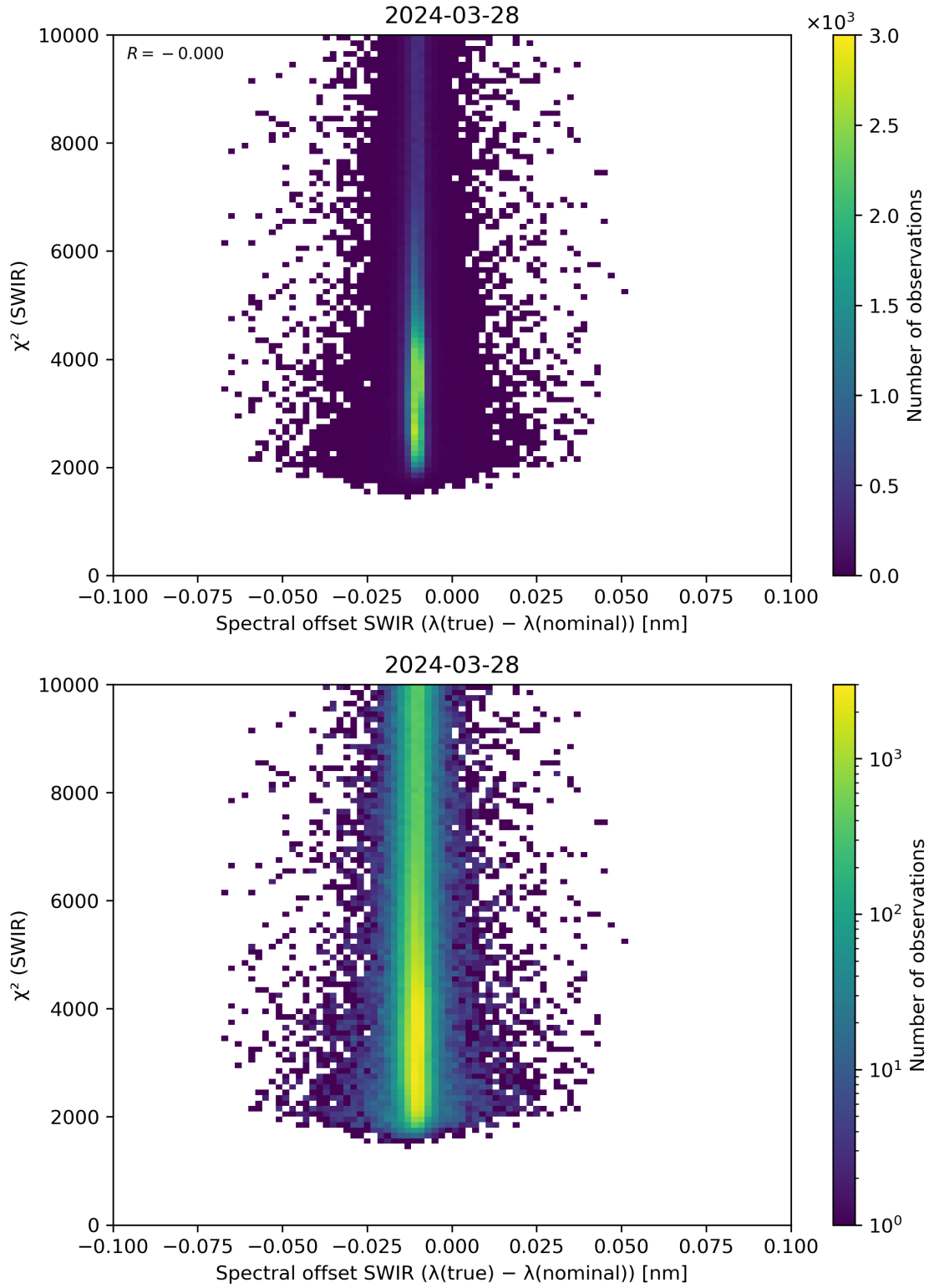
Figure 118: Scatter density plot of “Spectral offset SWIR ( \lambda(\text{true}) - \lambda(\text{nominal}) )” against “ \chi^2 (SWIR)” for 2024-03-27 to 2024-03-29.
