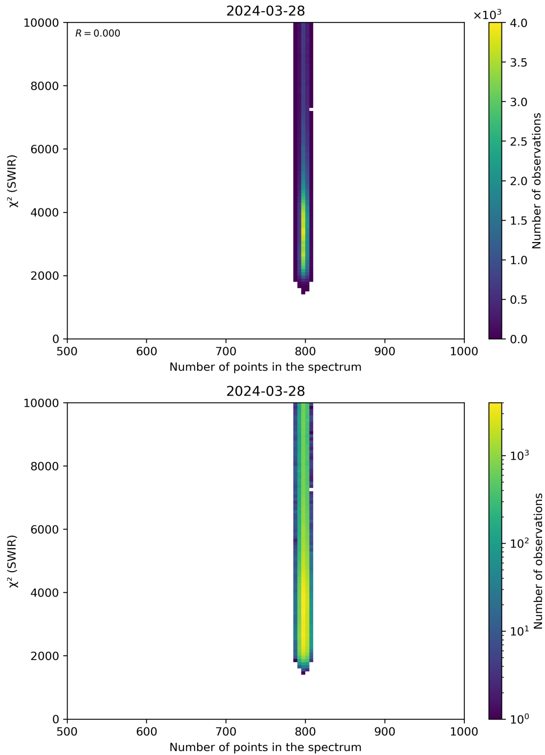
Figure 89: Scatter density plot of “Number of points in the spectrum” against “ \chi^2 (SWIR)” for 2024-03-27 to 2024-03-29.
