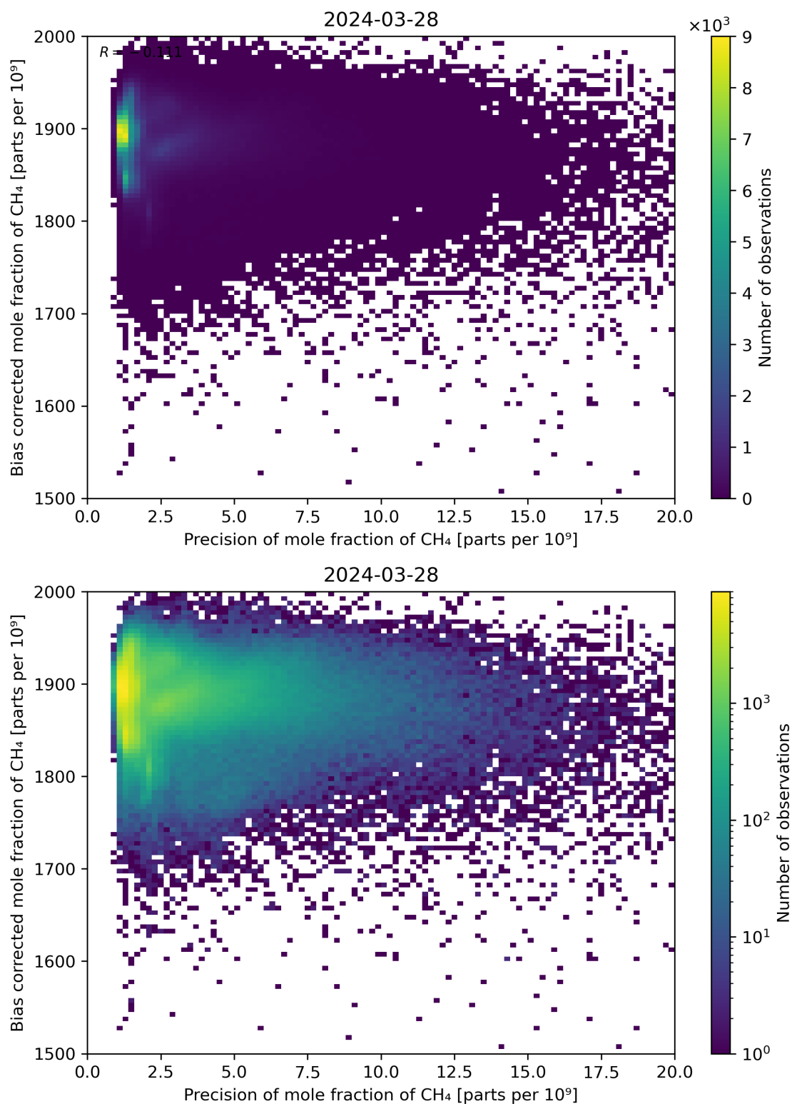
Figure 82: Scatter density plot of “Precision of mole fraction of CH 4 ” against “Bias corrected mole fraction of CH 4 ” for 2024-03-27 to 2024-03-29.
