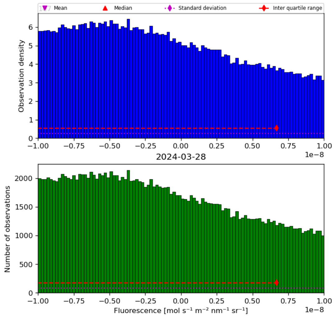
Figure 32: Histogram of “Fluorescence” for 2024-03-27 to 2024-03-29
