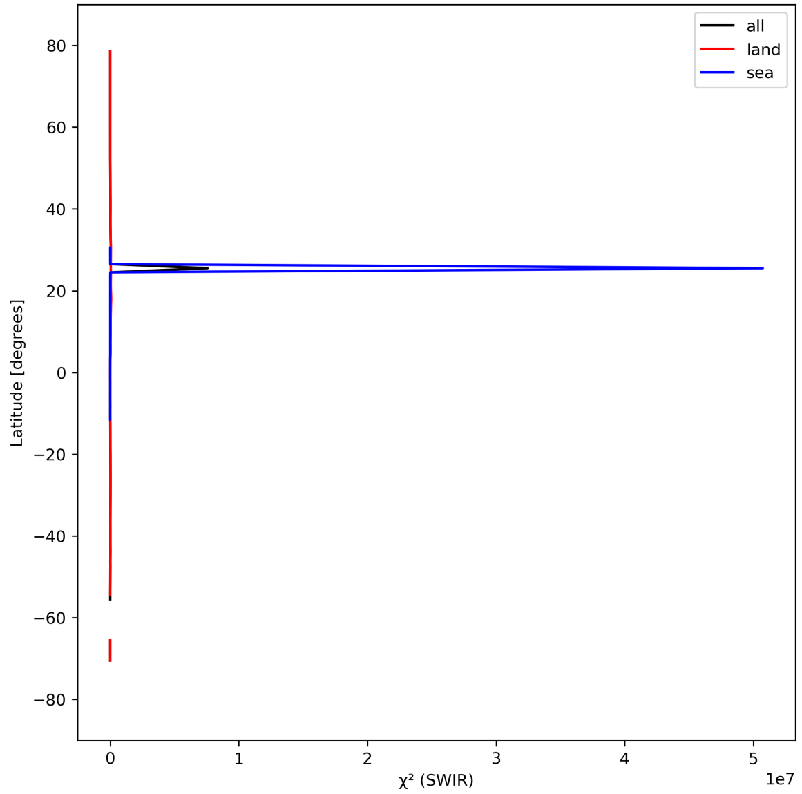
Figure 17: Zonal average of “ \chi^2 (SWIR)” for 2024-03-27 to 2024-03-29.
