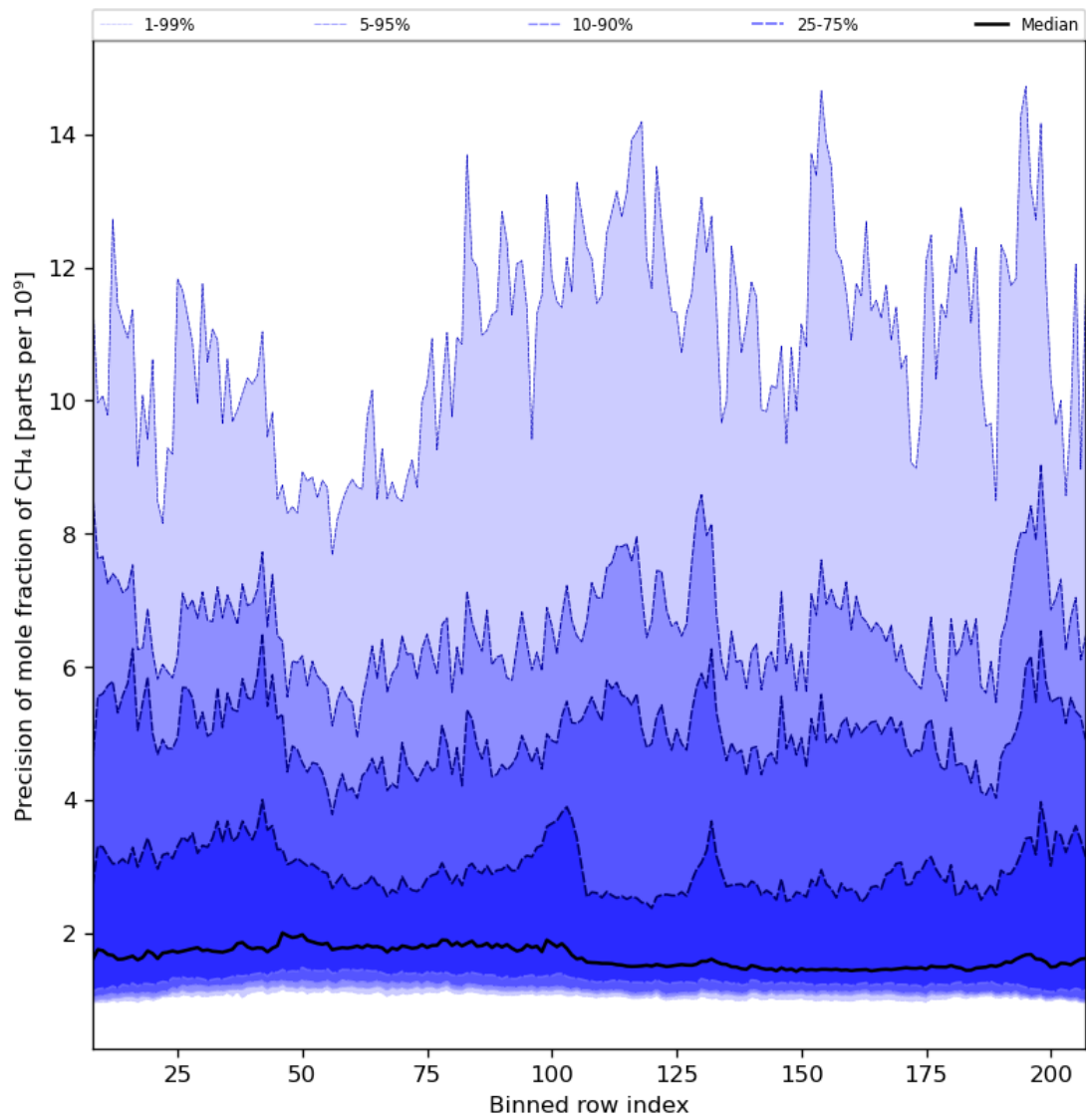
Figure 35: Along track statistics of “Precision of mole fraction of CH 4 ” for 2024-03-27 to 2024-03-29
