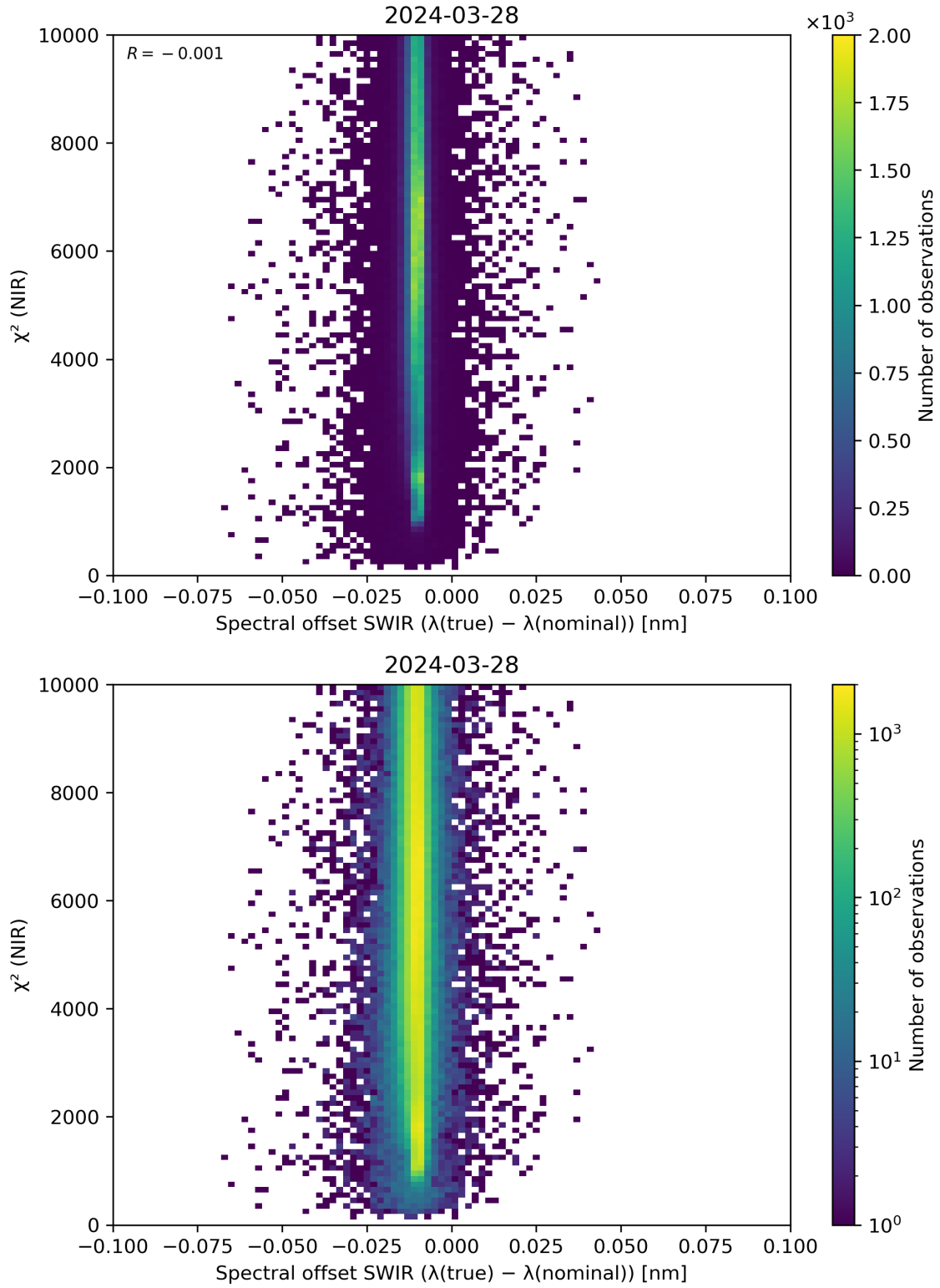
Figure 117: Scatter density plot of “Spectral offset SWIR ( \lambda(\text{true}) - \lambda(\text{nominal}) )” against “ \chi^2 (NIR)” for 2024-03-27 to 2024-03-29.
