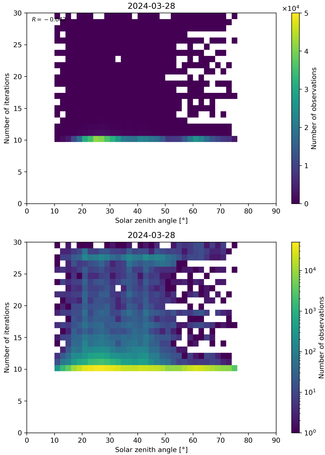
Figure 102: Scatter density plot of “Solar zenith angle” against “Number of iterations” for 2024-03-27 to 2024-03-29.
