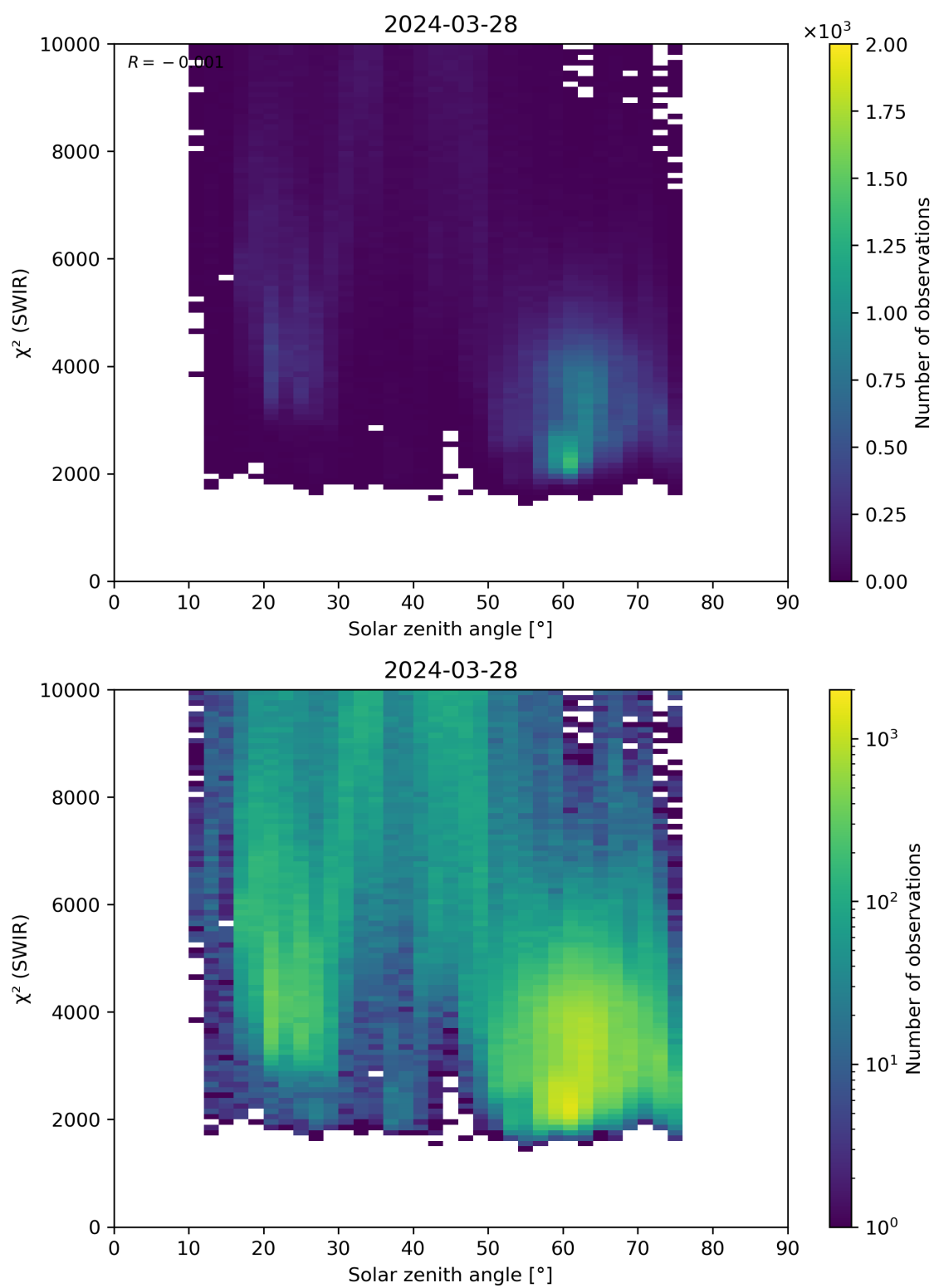
Figure 95: Scatter density plot of “Solar zenith angle” against “ \chi^2 (SWIR)” for 2024-03-27 to 2024-03-29.
