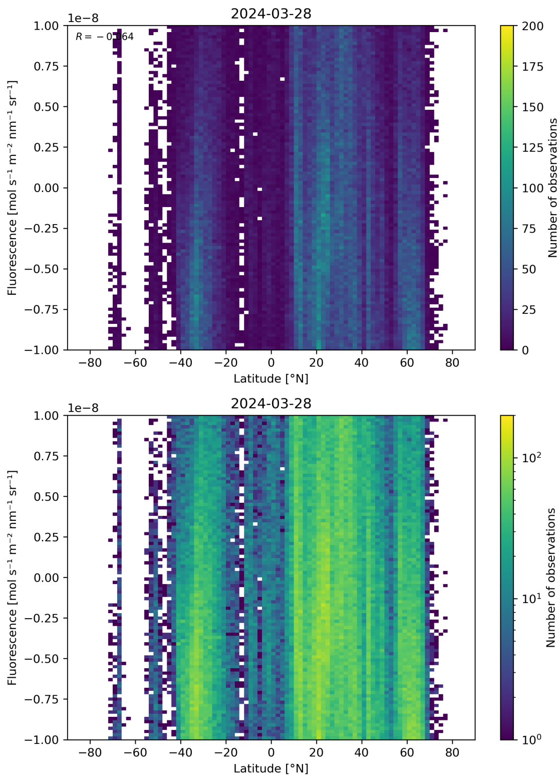
Figure 56: Scatter density plot of “Latitude” against “Fluorescence” for 2024-03-27 to 2024-03-29.
