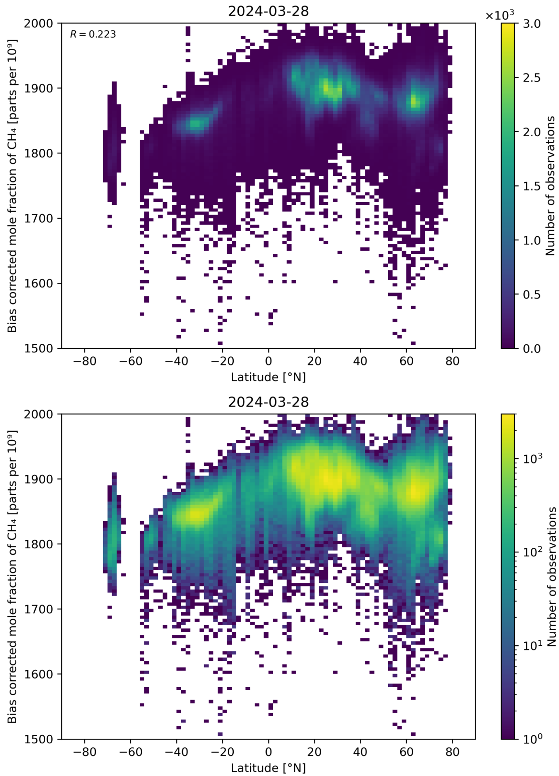
Figure 58: Scatter density plot of “Latitude” against “Bias corrected mole fraction of CH 4 ” for 2024-03-27 to 2024-03-29.
