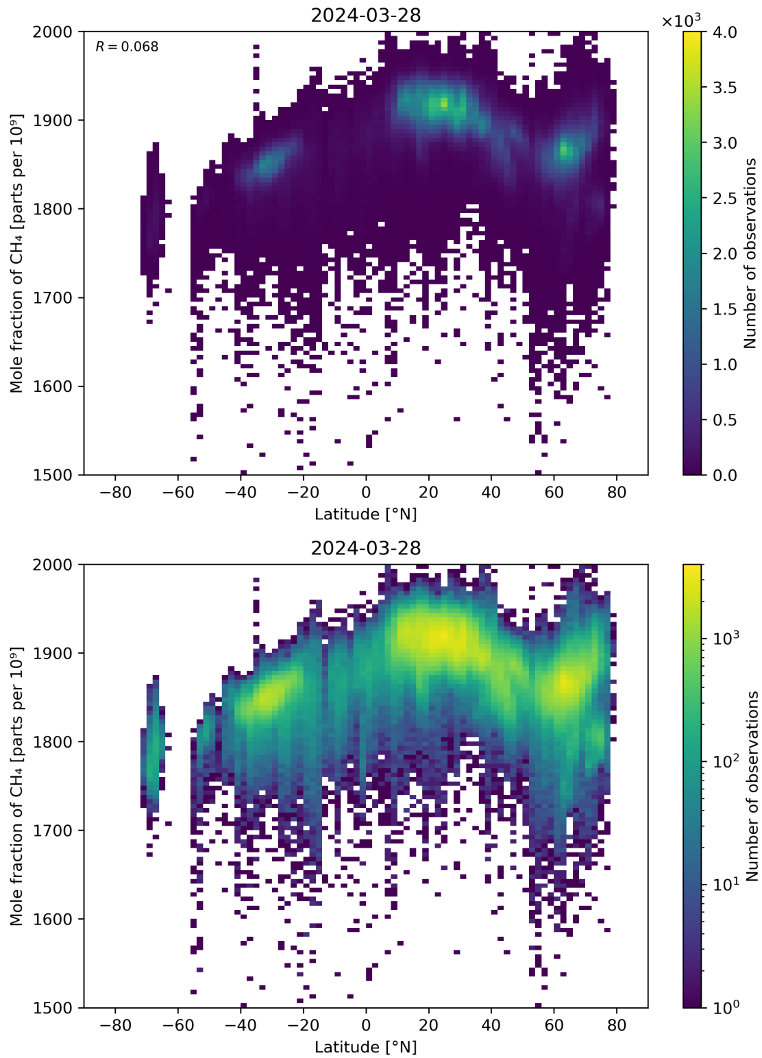
Figure 57: Scatter density plot of “Latitude” against “Mole fraction of \text{CH}_4 ” for 2024-03-27 to 2024-03-29.
