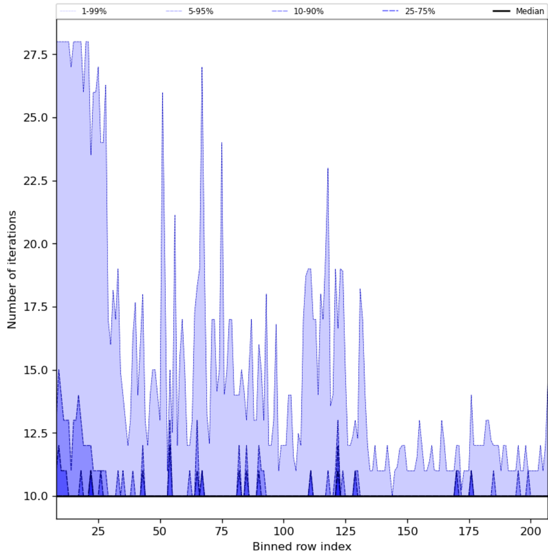
Figure 42: Along track statistics of “Number of iterations” for 2024-03-27 to 2024-03-29
