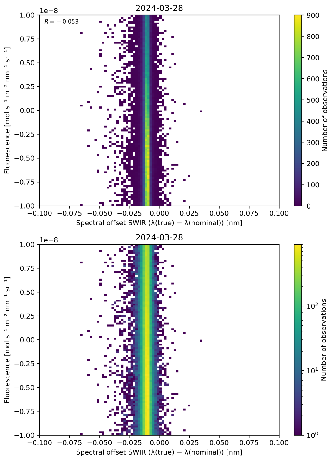
Figure 120: Scatter density plot of “Spectral offset SWIR ( \lambda(\text{true}) - \lambda(\text{nominal}) )” against “Fluorescence” for 2024-03-27 to 2024-03-29.
