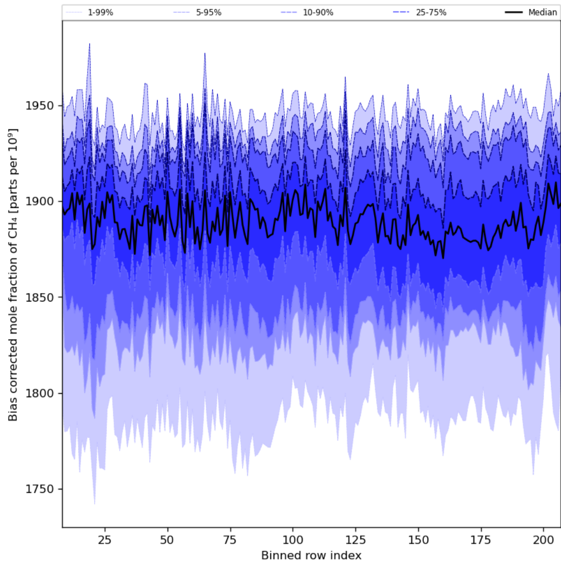
Figure 36: Along track statistics of “Bias corrected mole fraction of CH 4 ” for 2024-03-27 to 2024-03-29
