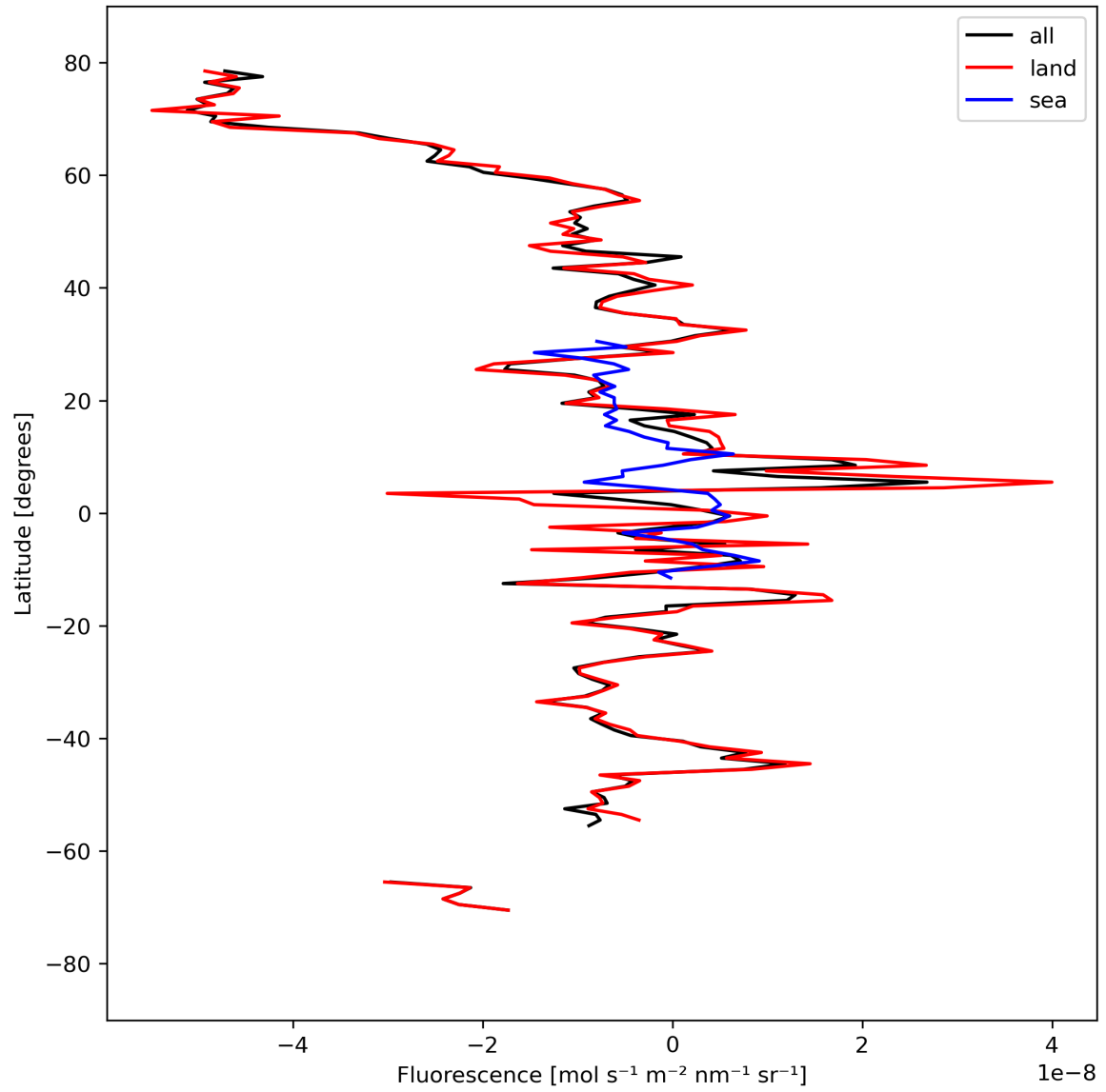
Figure 21: Zonal average of “Fluorescence” for 2024-03-27 to 2024-03-29.
