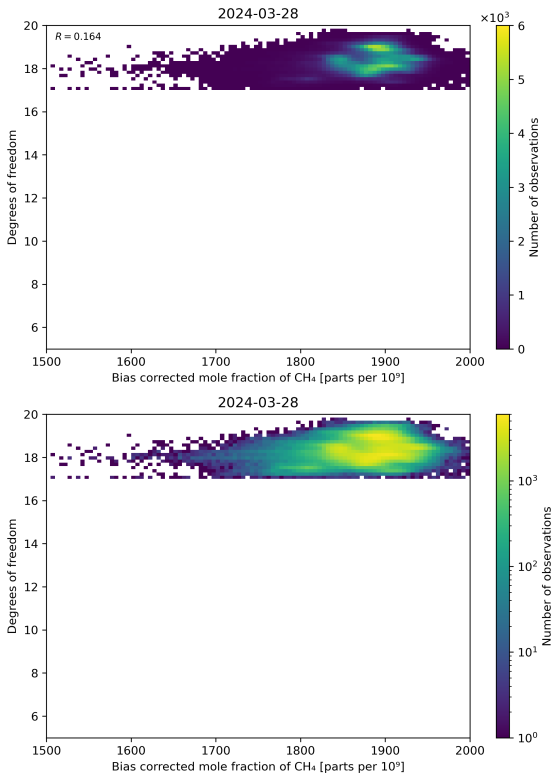
Figure 65: Scatter density plot of “Bias corrected mole fraction of CH 4 ” against “Degrees of freedom” for 2024-03-27 to 2024-03-29.
