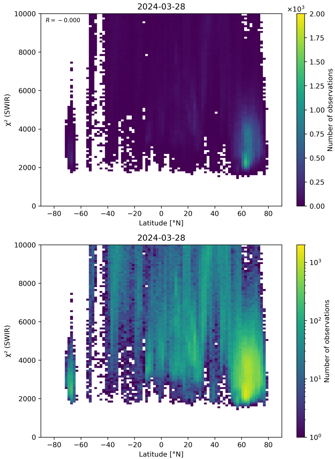
Figure 54: Scatter density plot of “Latitude” against “ \chi^2 (SWIR)” for 2024-03-27 to 2024-03-29.
