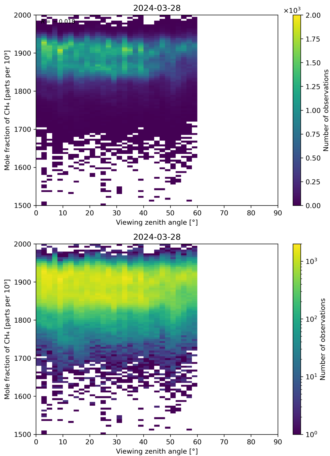
Figure 110: Scatter density plot of “Viewing zenith angle” against “Mole fraction of CH 4 ” for 2024-03-27 to 2024-03-29.
