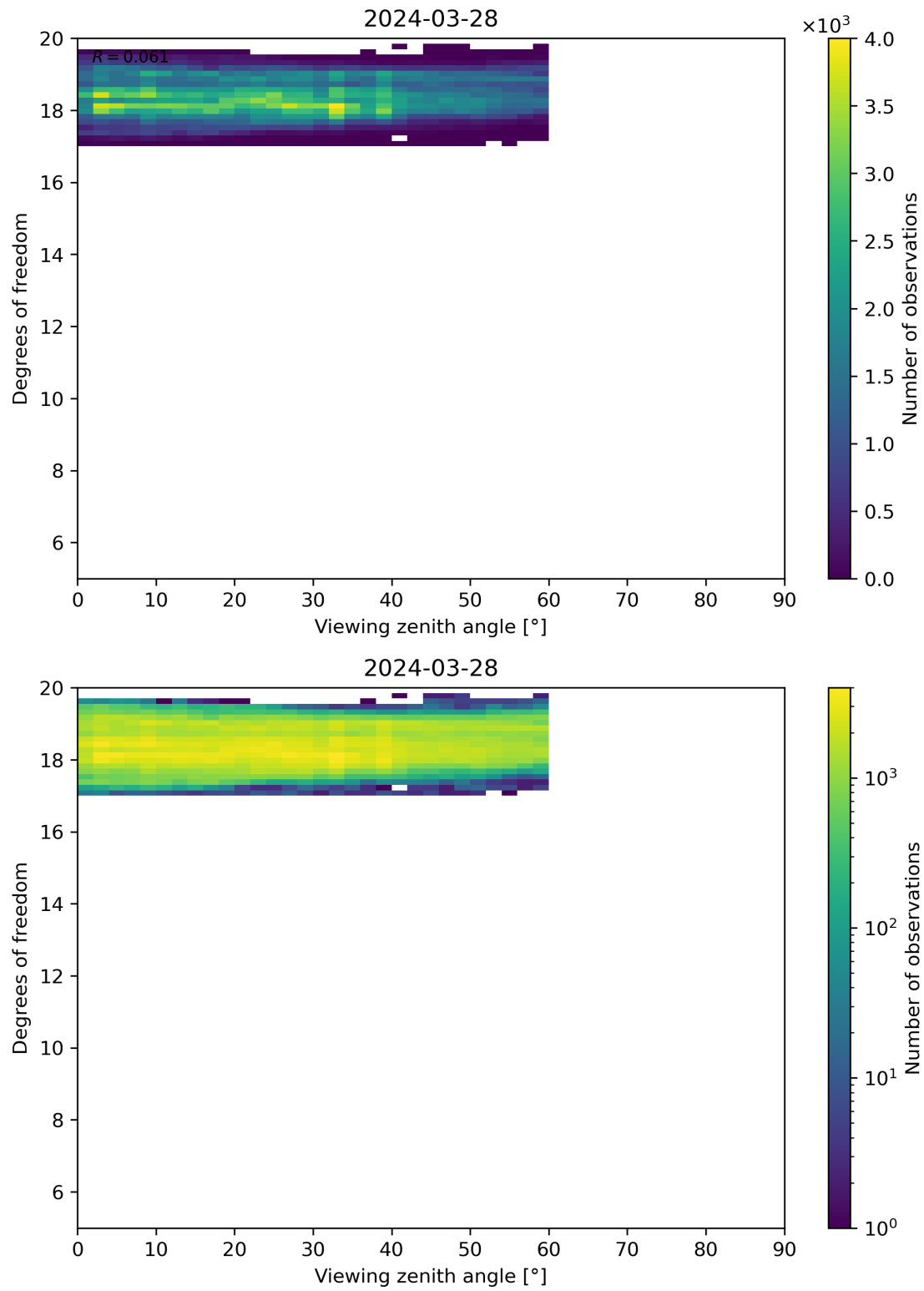
Figure 107: Scatter density plot of “Viewing zenith angle” against “Degrees of freedom” for 2024-03-27 to 2024-03-29.
