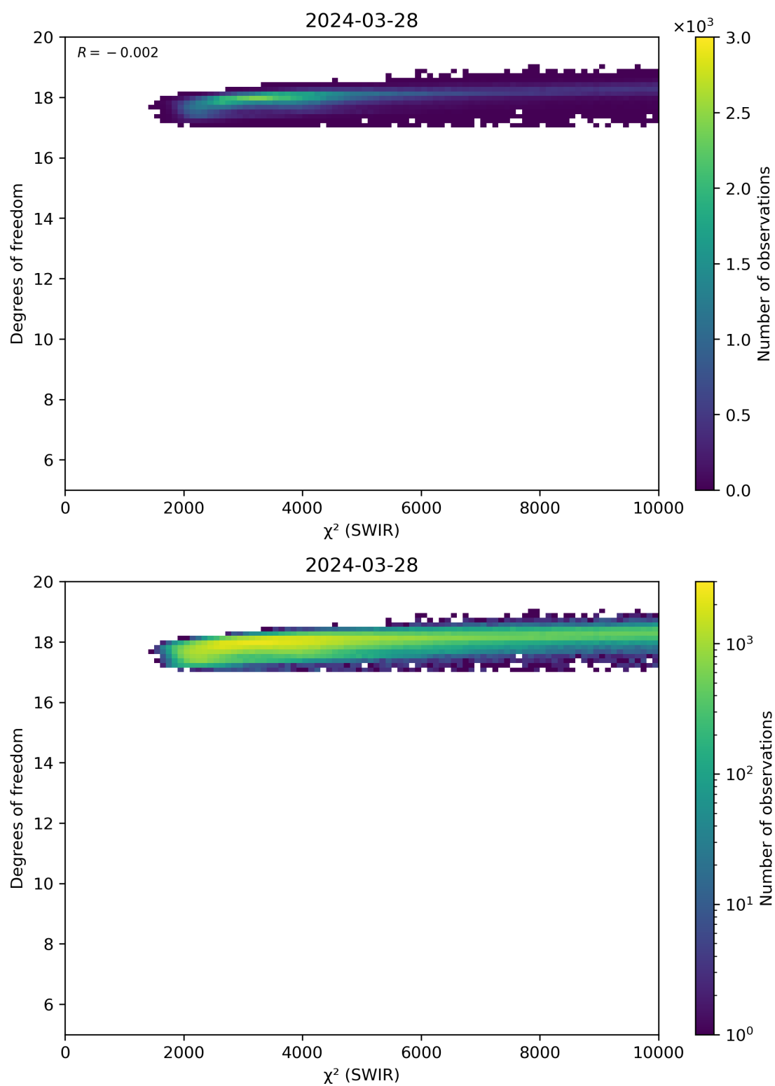
Figure 48: Scatter density plot of “ \chi^2 (SWIR)” against “Degrees of freedom” for 2024-03-27 to 2024-03-29.
