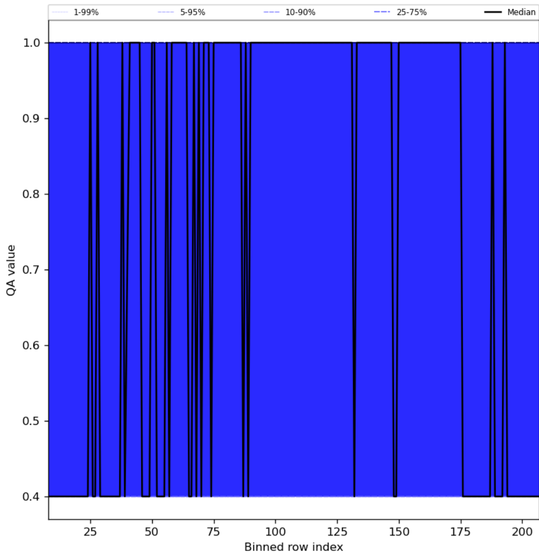
Figure 33: Along track statistics of “QA value” for 2024-03-28 to 2024-03-30
