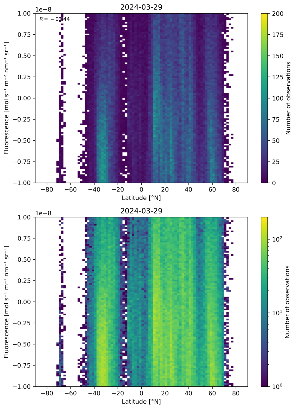
Figure 56: Scatter density plot of “Latitude” against “Fluorescence” for 2024-03-28 to 2024-03-30.
