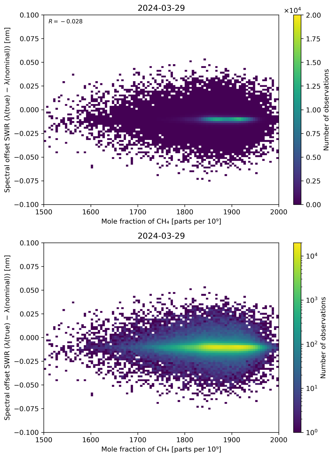
Figure 86: Scatter density plot of “Mole fraction of CH 4 ” against “Spectral offset SWIR ( \lambda(\text{true}) - \lambda(\text{nominal}) )” for 2024-03-28 to 2024-03-30.
