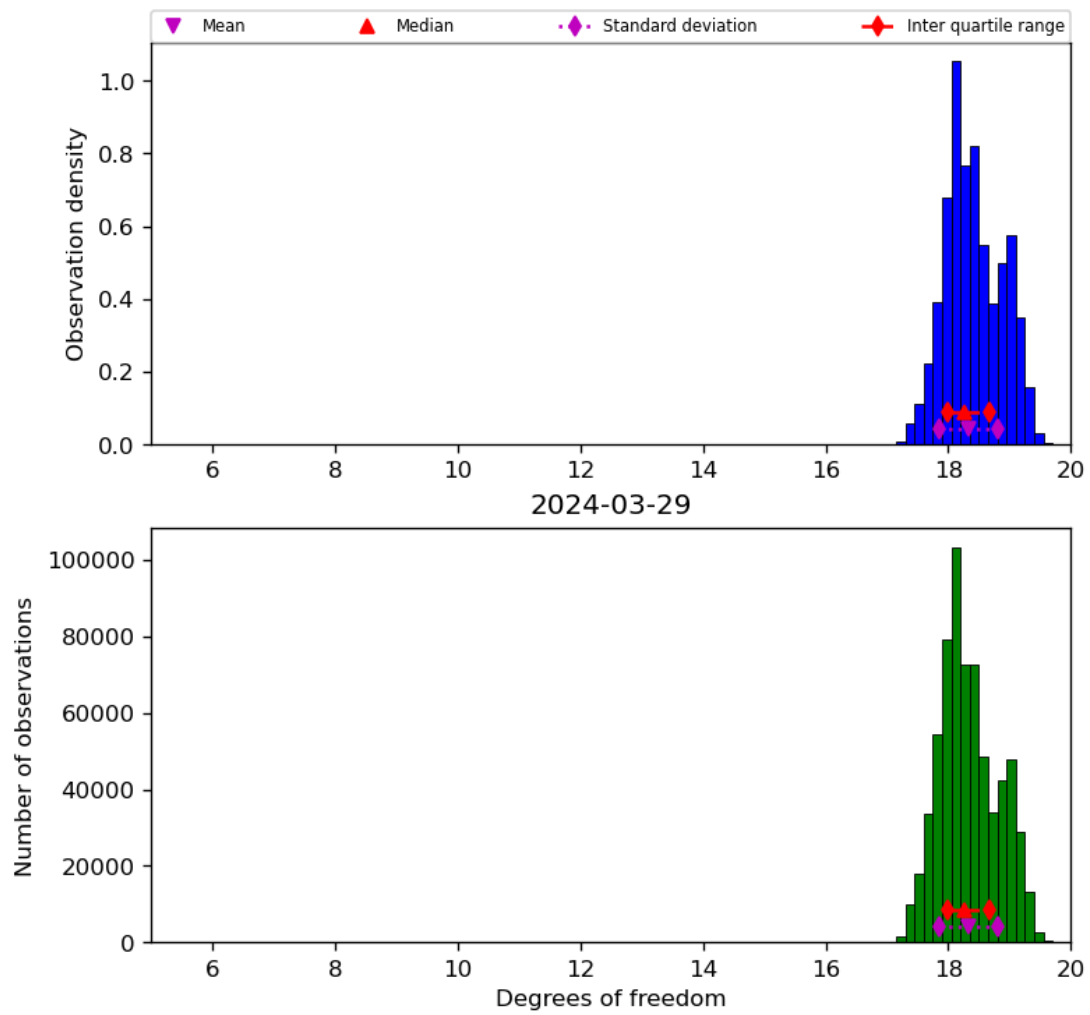
Figure 30: Histogram of “Degrees of freedom” for 2024-03-28 to 2024-03-30
