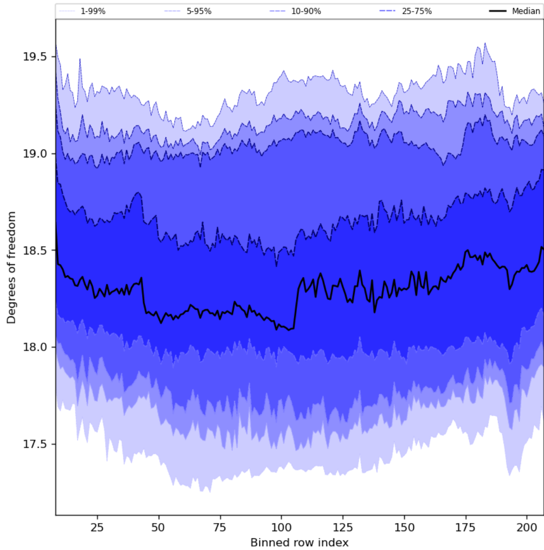
Figure 41: Along track statistics of “Degrees of freedom” for 2024-03-28 to 2024-03-30
