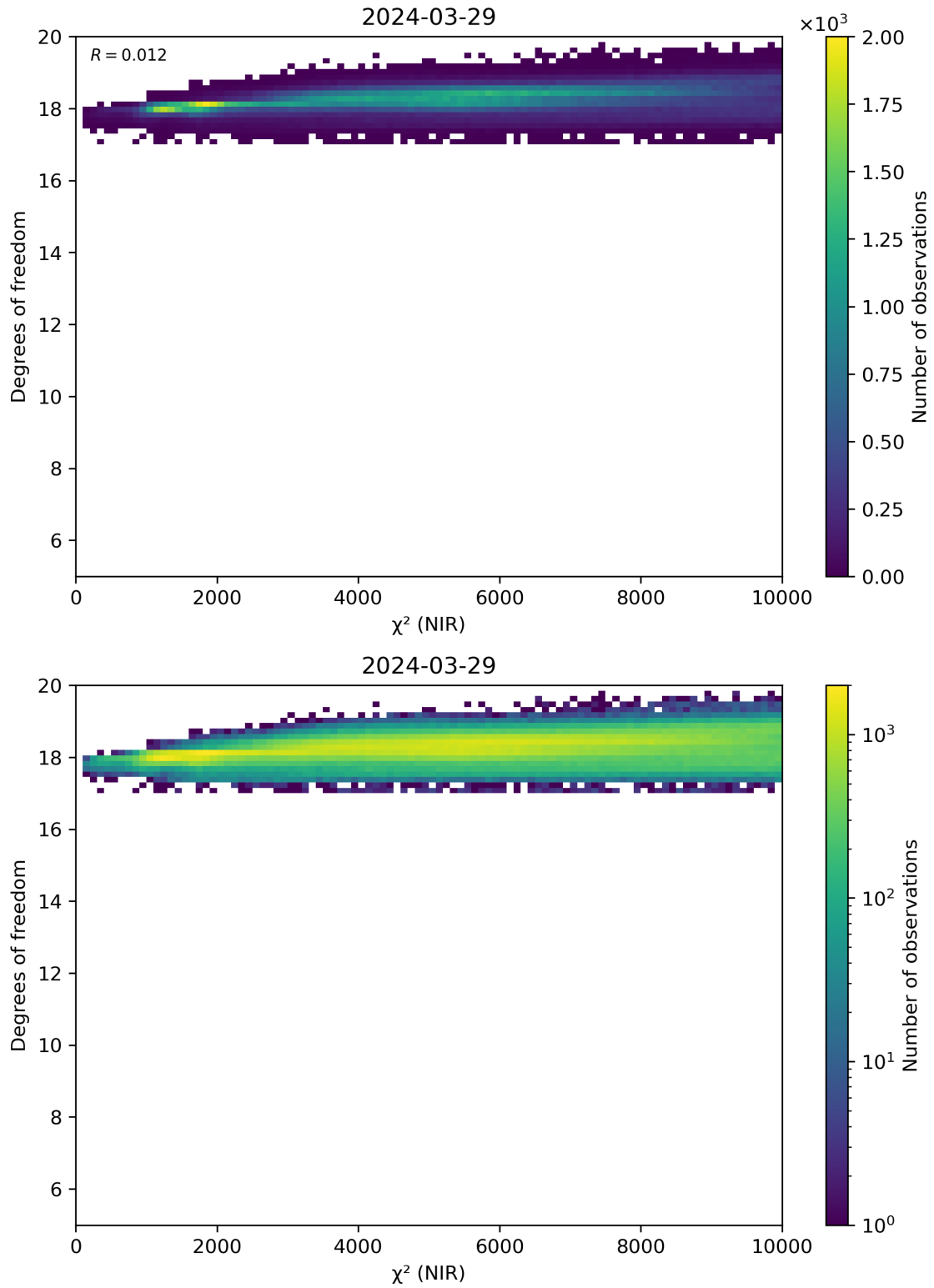
Figure 44: Scatter density plot of “ \chi^2 (NIR)” against “Degrees of freedom” for 2024-03-28 to 2024-03-30.
