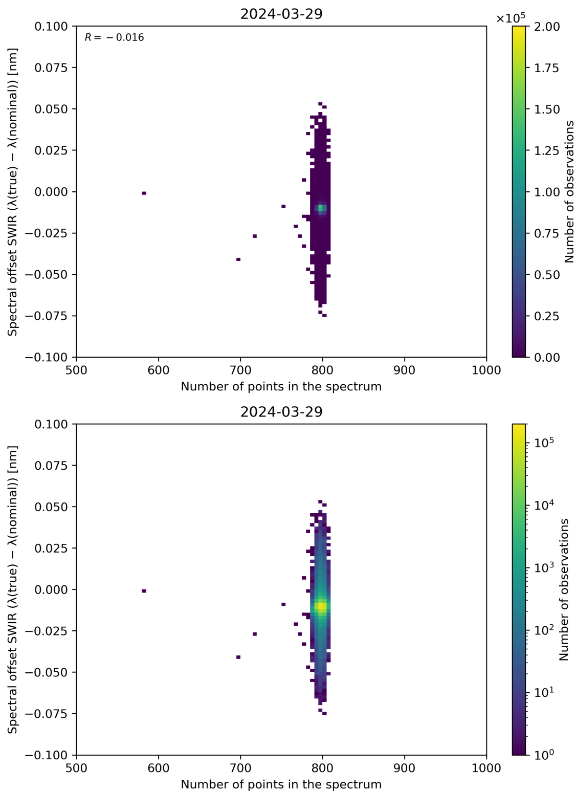
Figure 93: Scatter density plot of “Number of points in the spectrum” against “Spectral offset SWIR ( \lambda(\text{true}) - \lambda(\text{nominal}) )” for 2024-03-28 to 2024-03-30.
