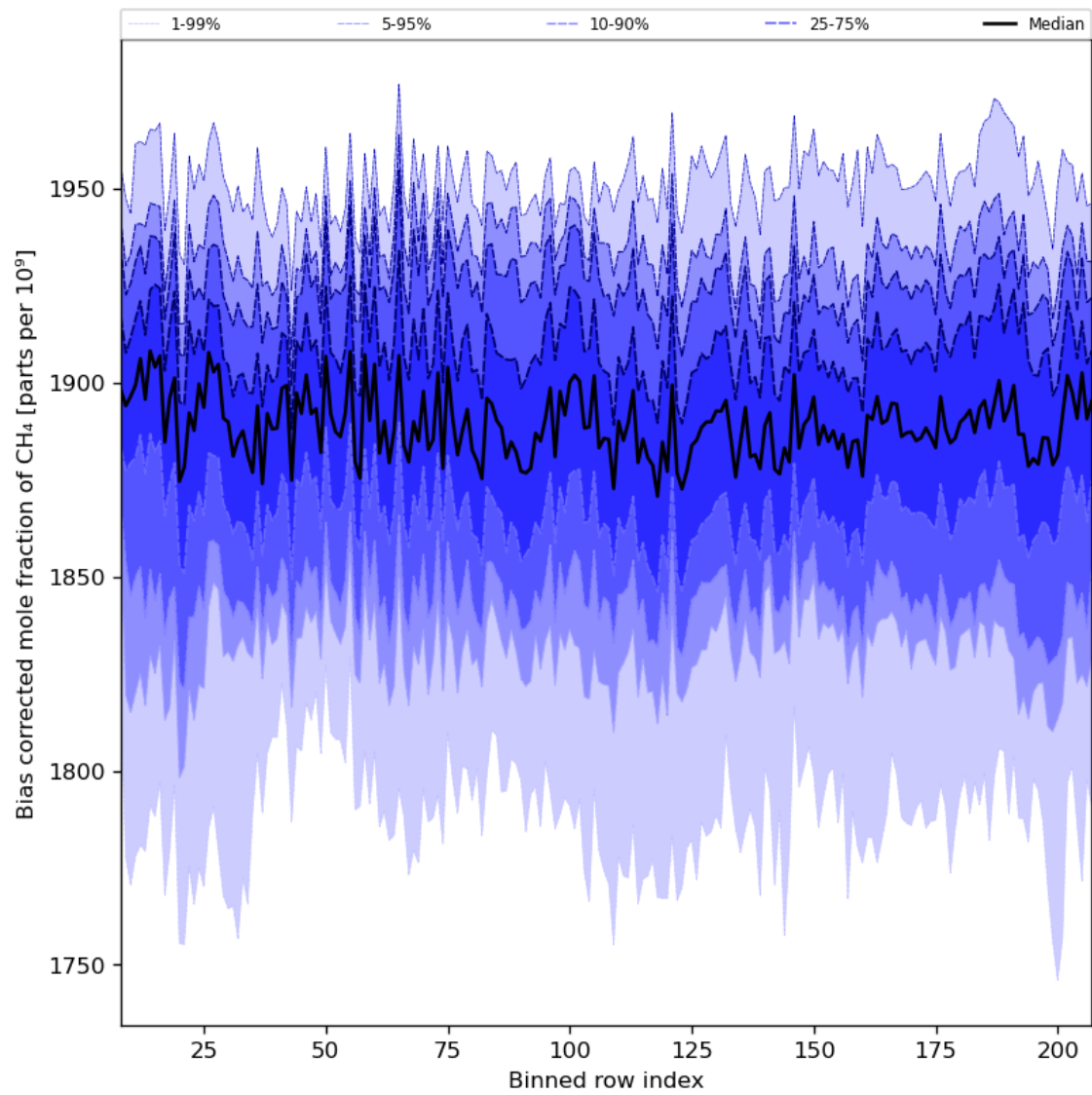
Figure 36: Along track statistics of “Bias corrected mole fraction of CH 4 ” for 2024-03-28 to 2024-03-30
