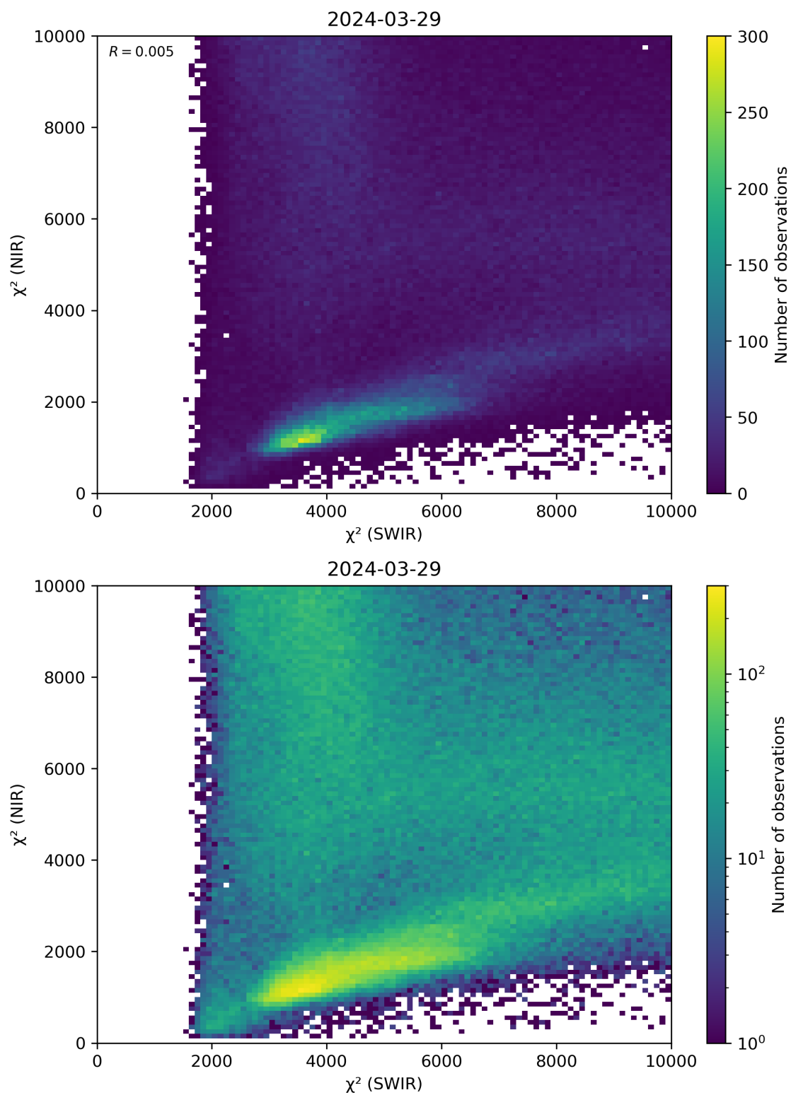
Figure 47: Scatter density plot of “ \chi^2 (SWIR)” against “ \chi^2 (NIR)” for 2024-03-28 to 2024-03-30.
