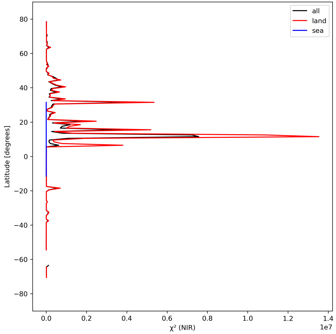
Figure 18: Zonal average of “ \chi^2 (NIR)” for 2024-03-28 to 2024-03-30.
