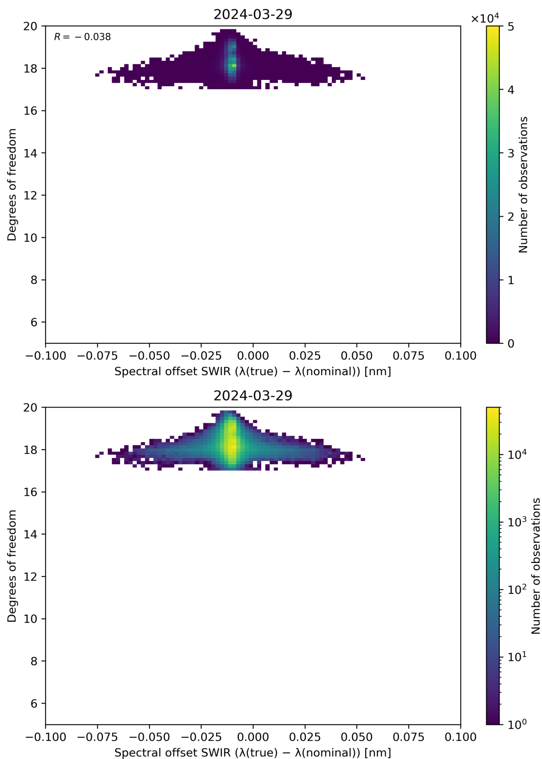
Figure 119: Scatter density plot of “Spectral offset SWIR ( \lambda(\text{true}) - \lambda(\text{nominal}) )” against “Degrees of freedom” for 2024-03-28 to 2024-03-30.
