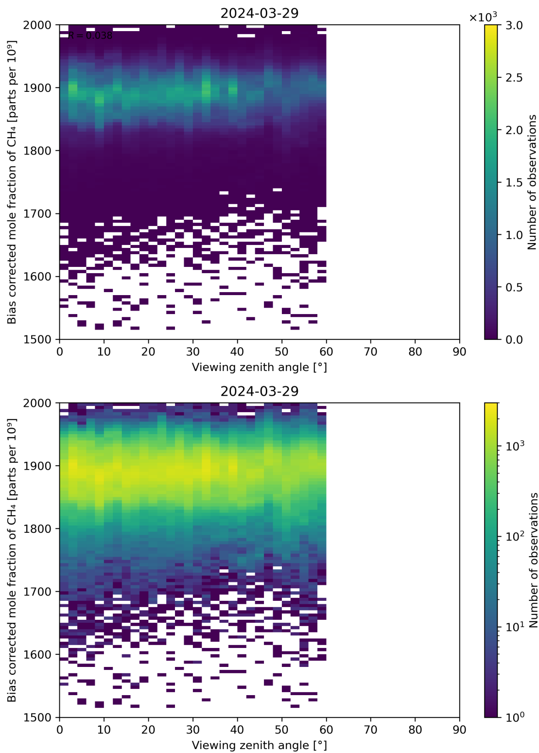
Figure 111: Scatter density plot of “Viewing zenith angle” against “Bias corrected mole fraction of CH 4 ” for 2024-03-28 to 2024-03-30.
