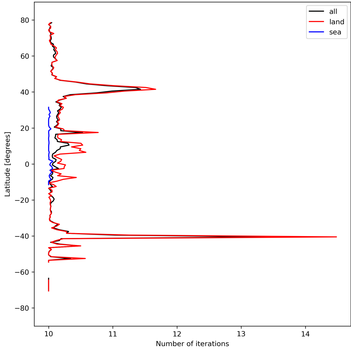
Figure 20: Zonal average of “Number of iterations” for 2024-03-28 to 2024-03-30.
