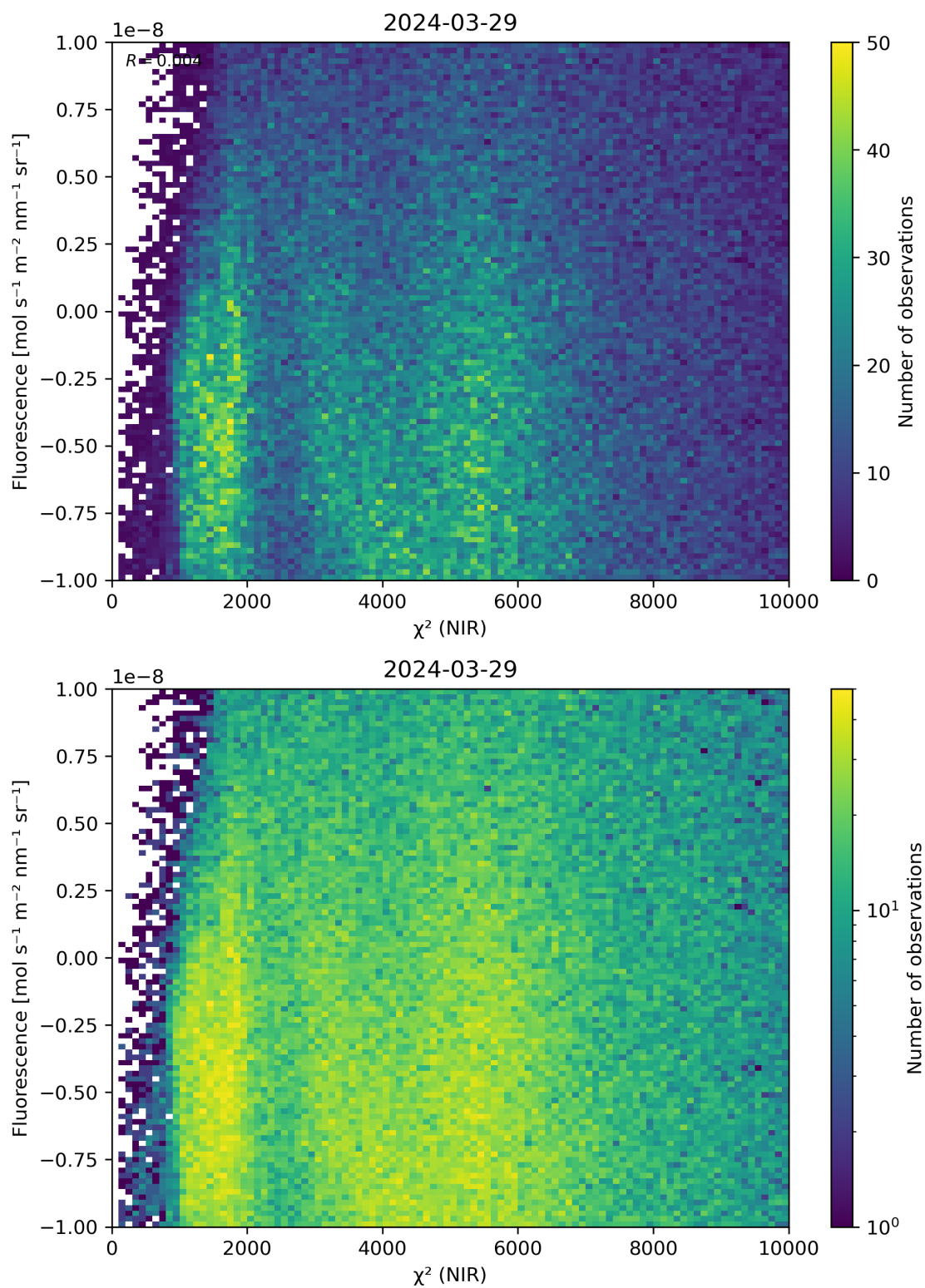
Figure 45: Scatter density plot of “ \chi^2 (NIR)” against “Fluorescence” for 2024-03-28 to 2024-03-30.
