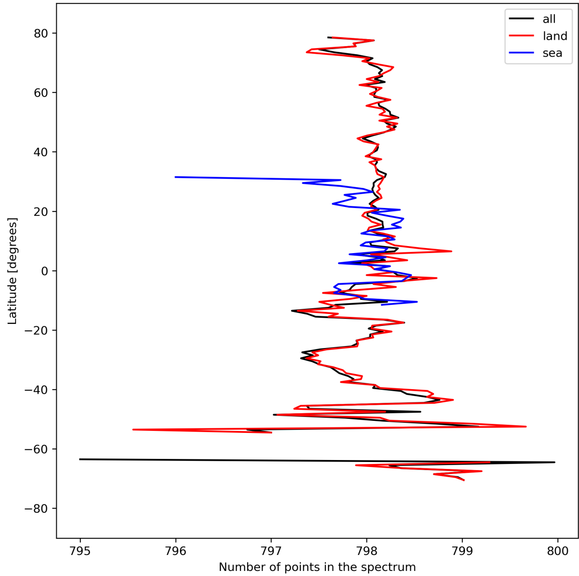
Figure 15: Zonal average of “Number of points in the spectrum” for 2024-03-28 to 2024-03-30.
