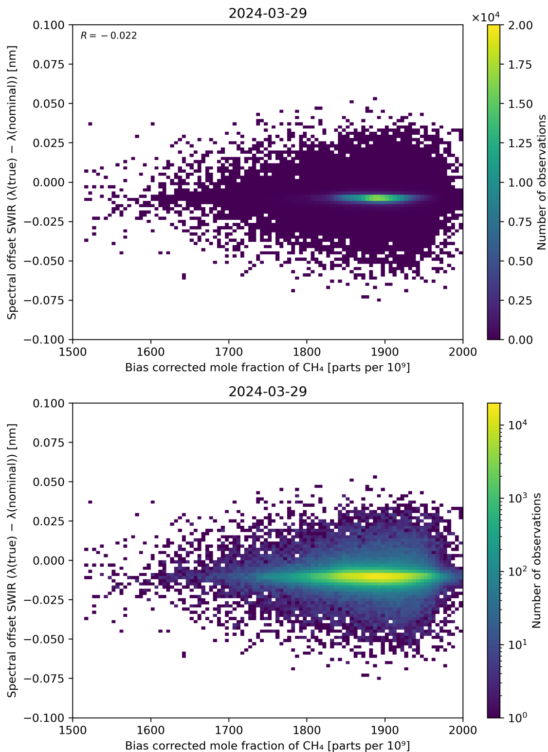
Figure 69: Scatter density plot of “Bias corrected mole fraction of \text{CH}_4 ” against “Spectral offset SWIR ( \lambda(\text{true}) - \lambda(\text{nominal}) )” for 2024-03-28 to 2024-03-30.
