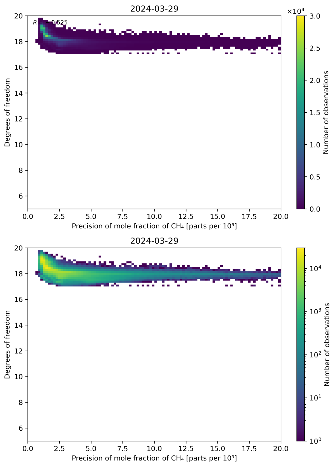
Figure 80: Scatter density plot of “Precision of mole fraction of CH 4 ” against “Degrees of freedom” for 2024-03-28 to 2024-03-30.
