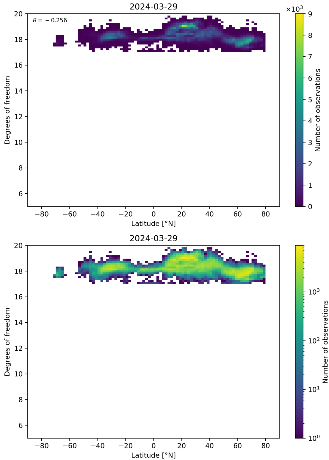
Figure 55: Scatter density plot of “Latitude” against “Degrees of freedom” for 2024-03-28 to 2024-03-30.
