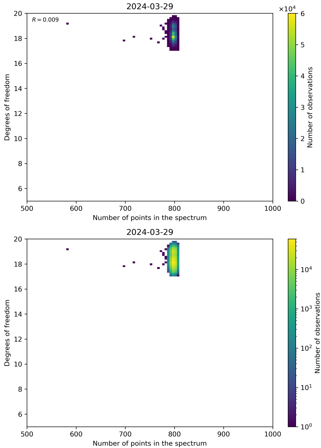
Figure 90: Scatter density plot of “Number of points in the spectrum” against “Degrees of freedom” for 2024-03-28 to 2024-03-30.
