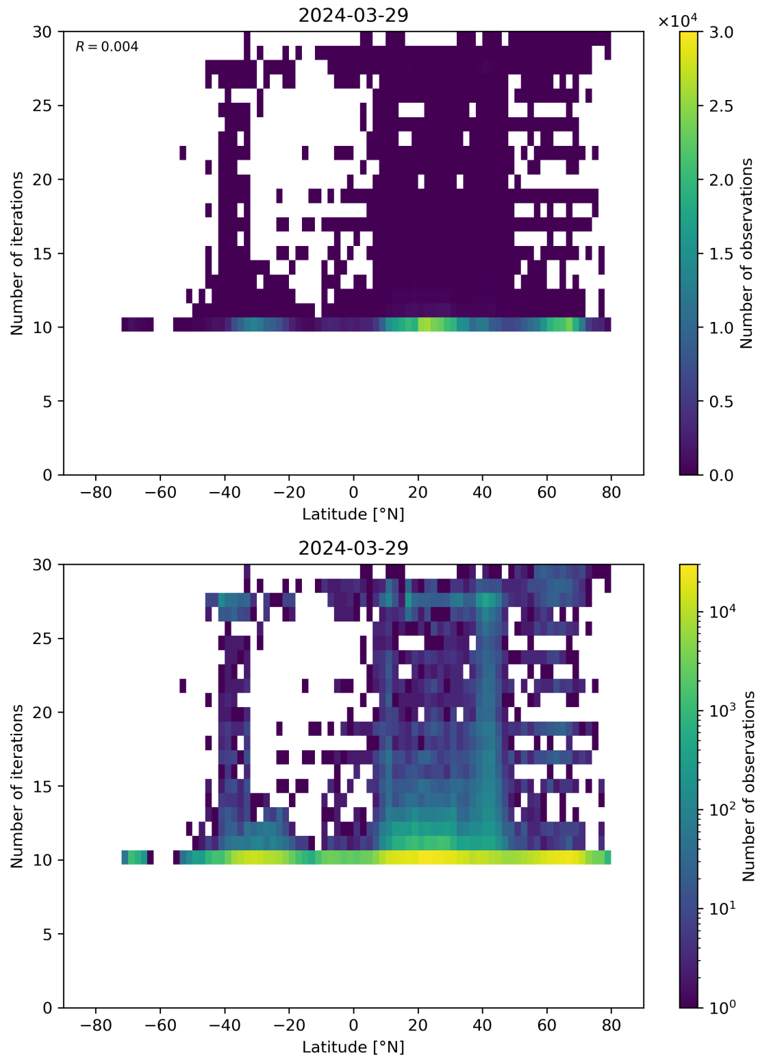
Figure 60: Scatter density plot of “Latitude” against “Number of iterations” for 2024-03-28 to 2024-03-30.
