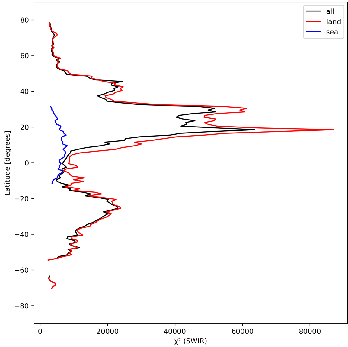
Figure 17: Zonal average of “ \chi^2 (SWIR)” for 2024-03-28 to 2024-03-30.
