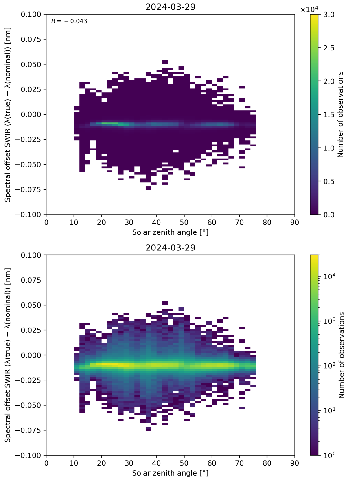
Figure 104: Scatter density plot of “Solar zenith angle” against “Spectral offset SWIR ( \lambda(\text{true}) - \lambda(\text{nominal}) )” for 2024-03-28 to 2024-03-30.
