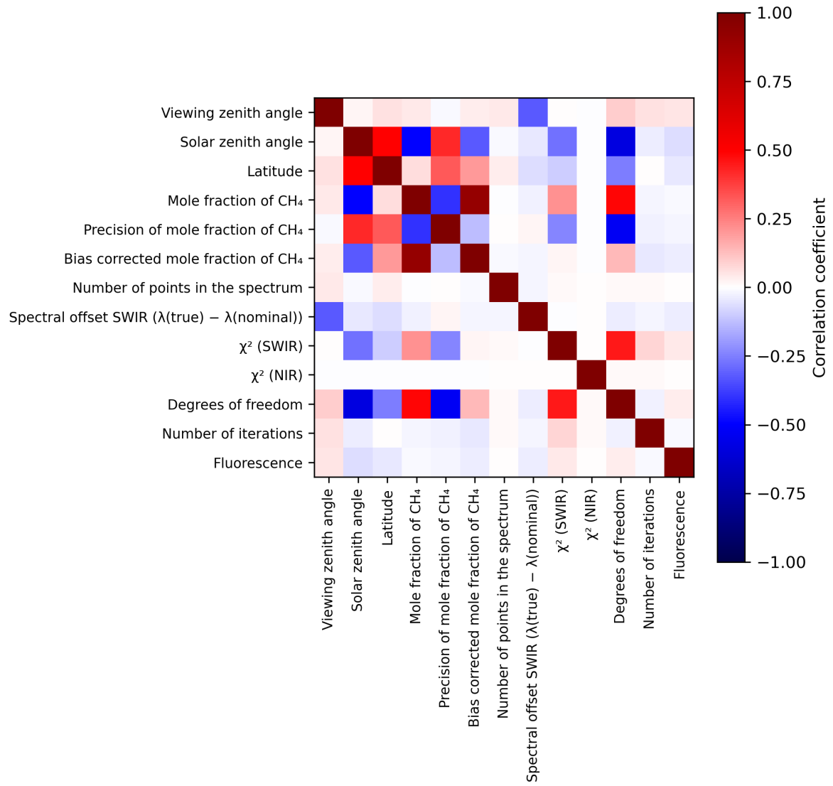
Figure 2: Map of correlation matrix for 2024-03-28 to 2024-03-30.
