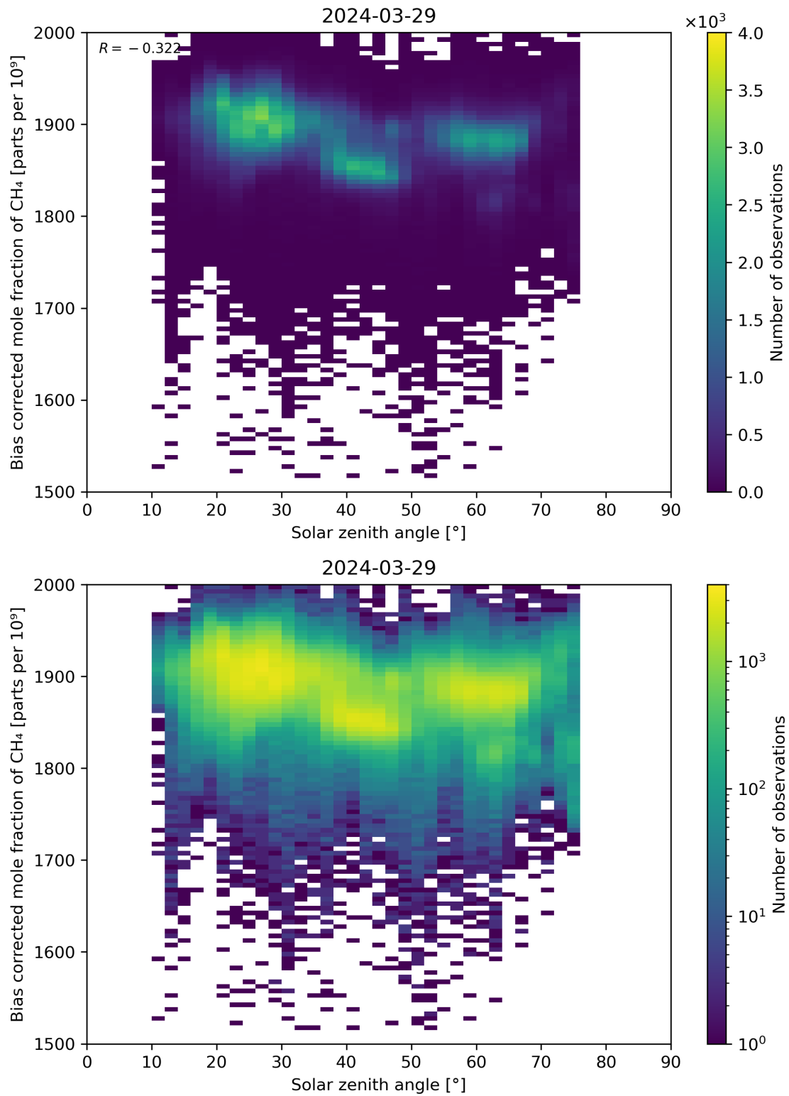
Figure 100: Scatter density plot of “Solar zenith angle” against “Bias corrected mole fraction of \text{CH}_4 ” for 2024-03-28 to 2024-03-30.
