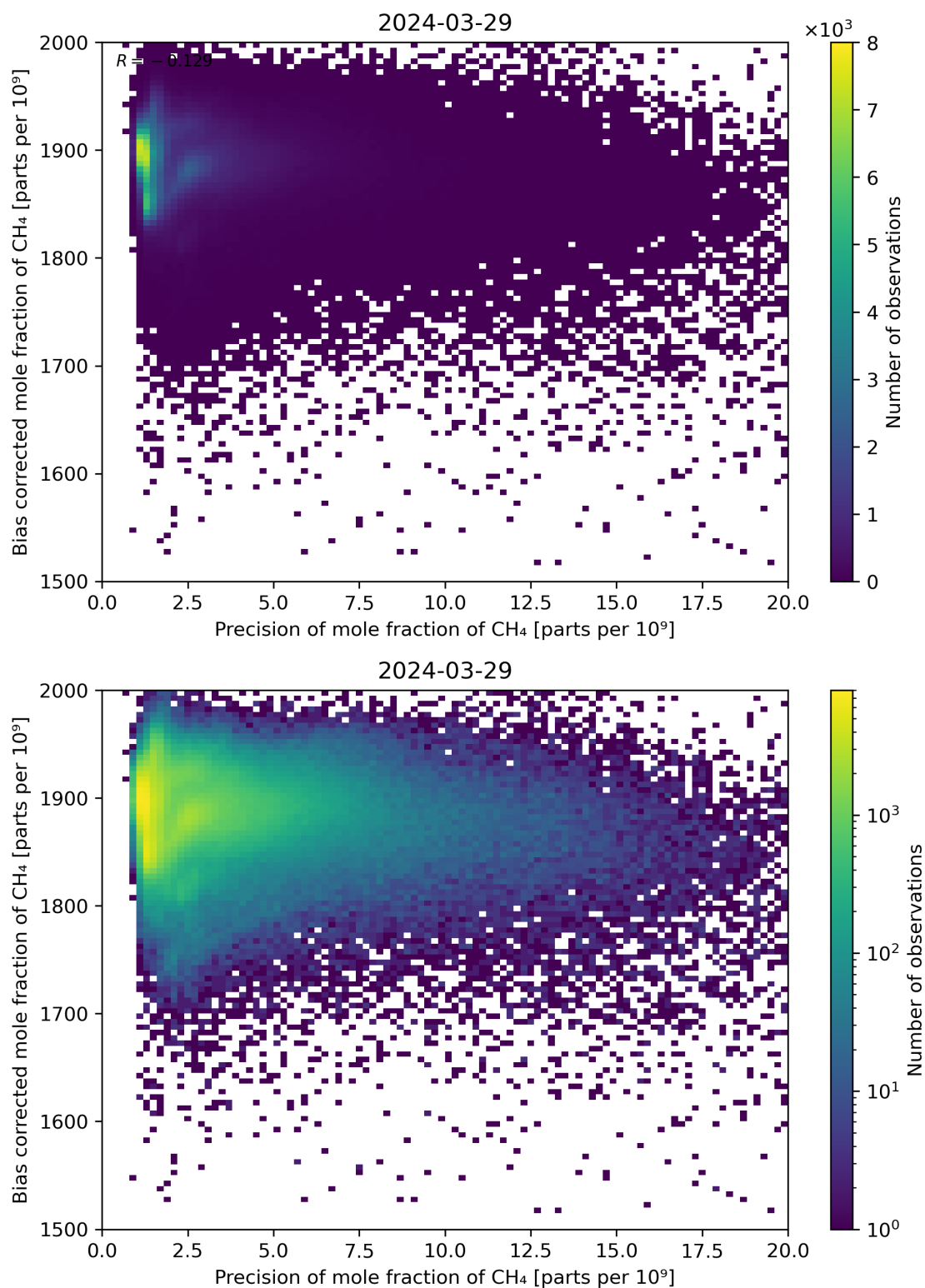
Figure 82: Scatter density plot of “Precision of mole fraction of CH 4 ” against “Bias corrected mole fraction of CH 4 ” for 2024-03-28 to 2024-03-30.
