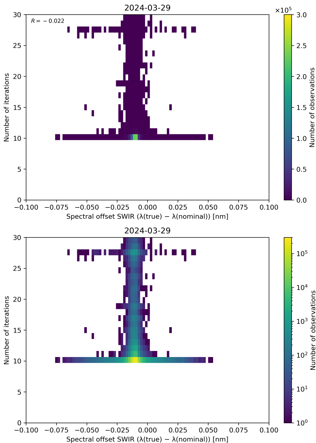
Figure 121: Scatter density plot of “Spectral offset SWIR ( \lambda(\text{true}) - \lambda(\text{nominal}) )” against “Number of iterations” for 2024-03-28 to 2024-03-30.
