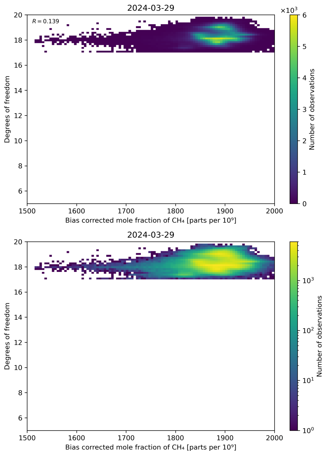
Figure 65: Scatter density plot of “Bias corrected mole fraction of CH 4 ” against “Degrees of freedom” for 2024-03-28 to 2024-03-30.
