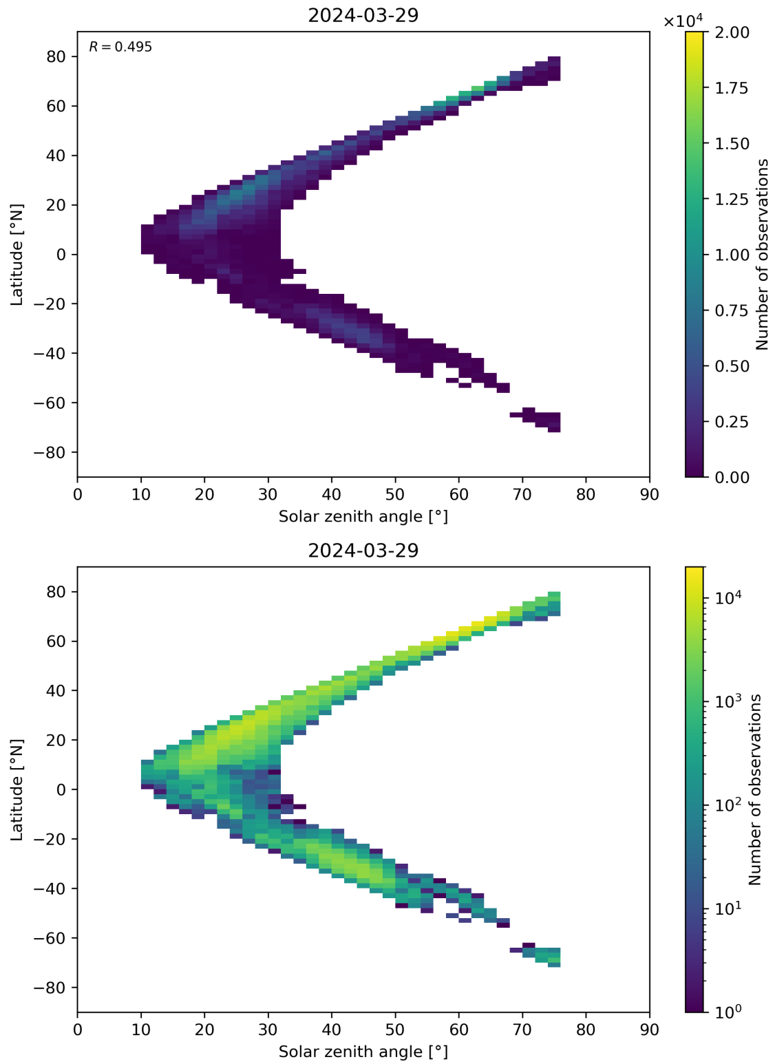
Figure 98: Scatter density plot of “Solar zenith angle” against “Latitude” for 2024-03-28 to 2024-03-30.
