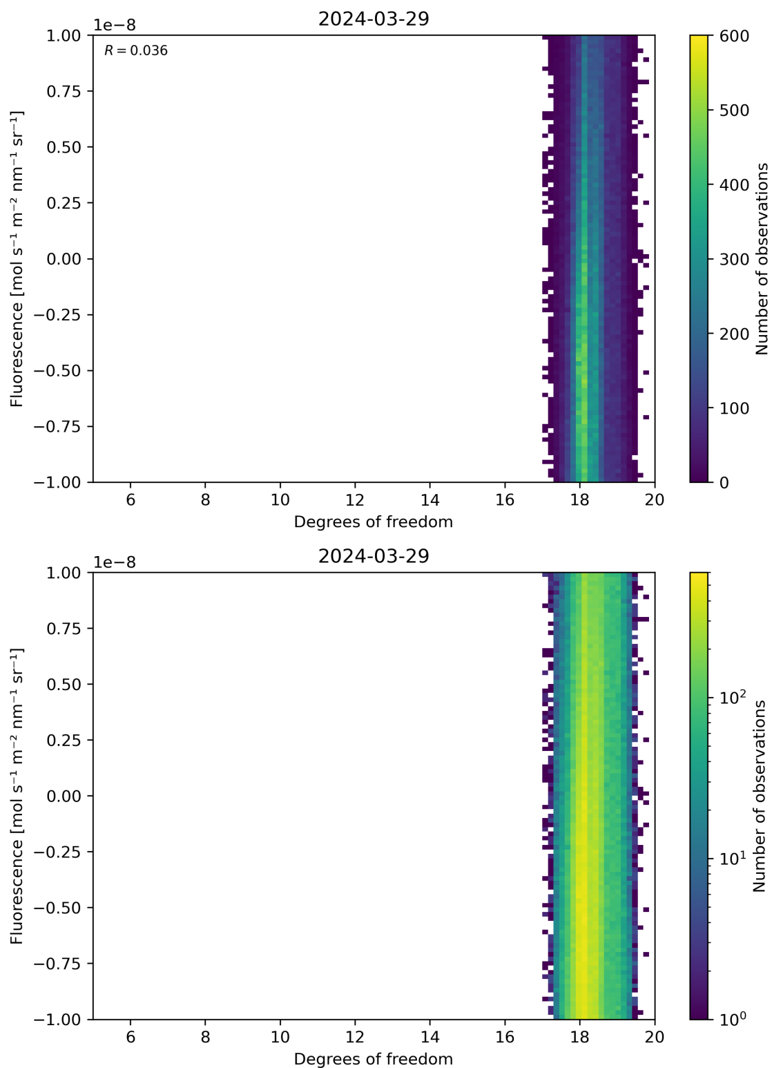
Figure 51: Scatter density plot of “Degrees of freedom” against “Fluorescence” for 2024-03-28 to 2024-03-30.
