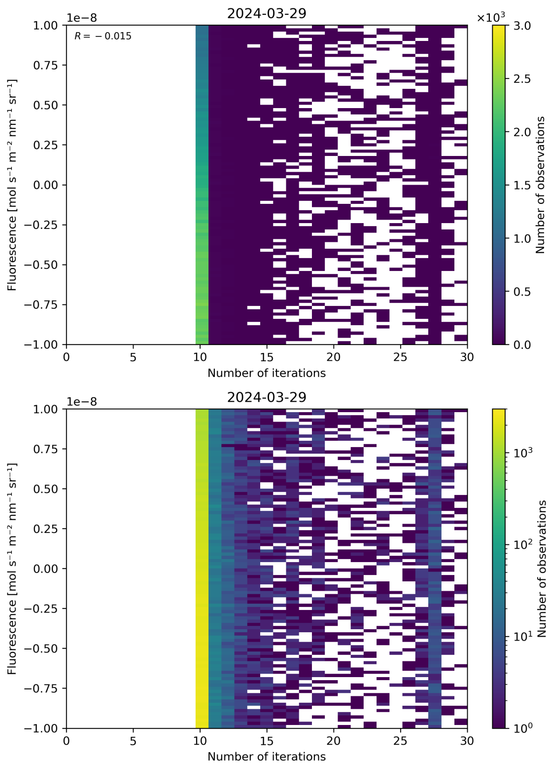
Figure 87: Scatter density plot of “Number of iterations” against “Fluorescence” for 2024-03-28 to 2024-03-30.
