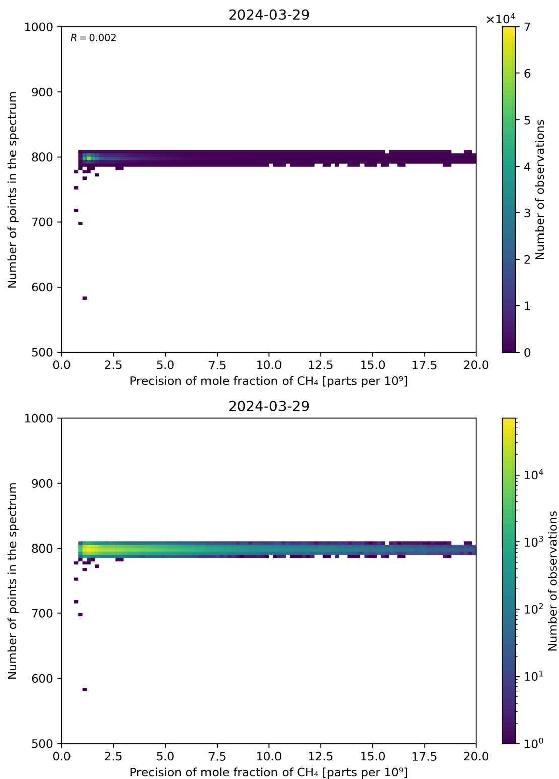
Figure 84: Scatter density plot of “Precision of mole fraction of \text{CH}_4 ” against “Number of points in the spectrum” for 2024-03-28 to 2024-03-30.
