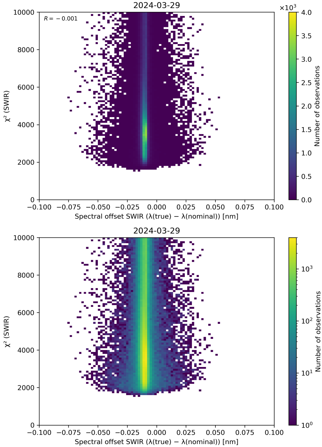
Figure 118: Scatter density plot of “Spectral offset SWIR ( \lambda(\text{true}) - \lambda(\text{nominal}) )” against “ \chi^2 (SWIR)” for 2024-03-28 to 2024-03-30.
