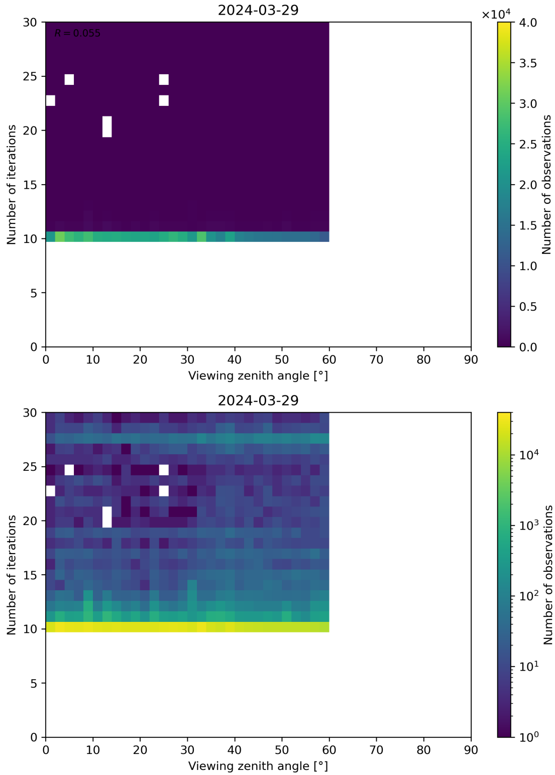
Figure 113: Scatter density plot of “Viewing zenith angle” against “Number of iterations” for 2024-03-28 to 2024-03-30.
