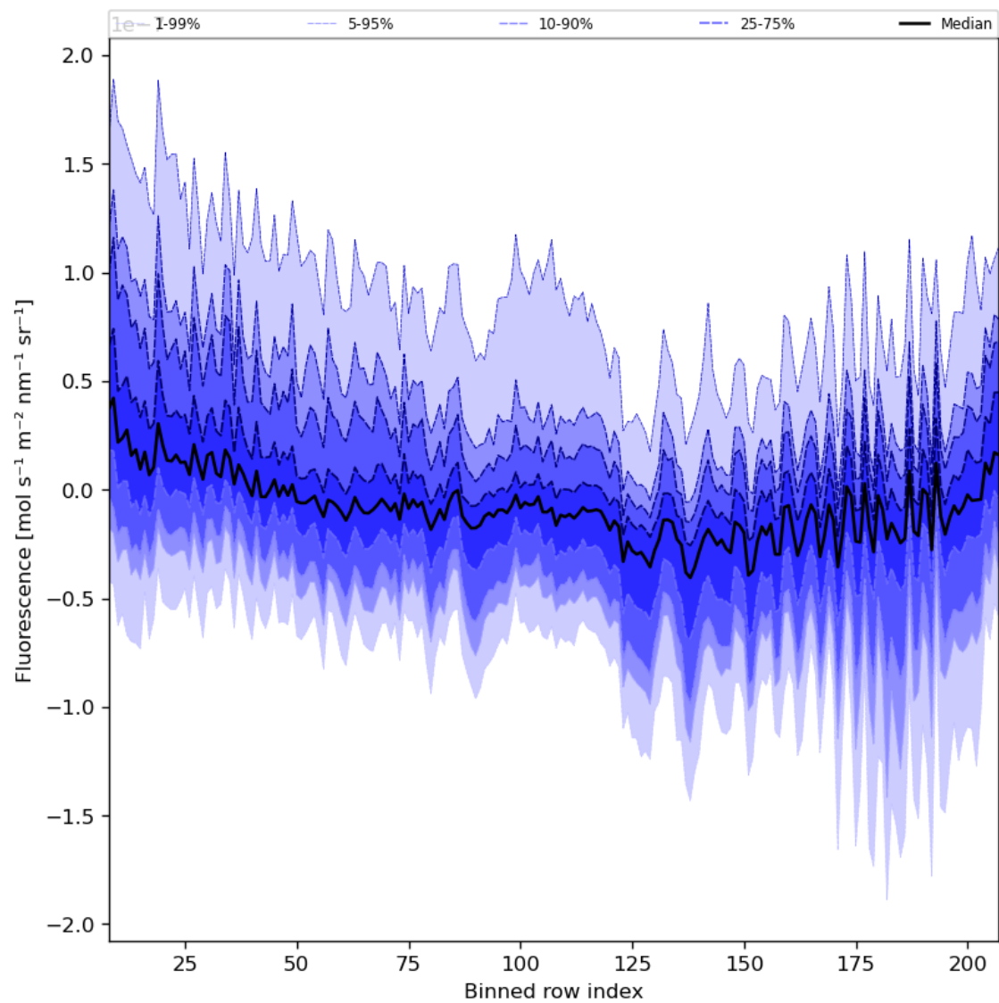
Figure 43: Along track statistics of “Fluorescence” for 2024-03-28 to 2024-03-30
