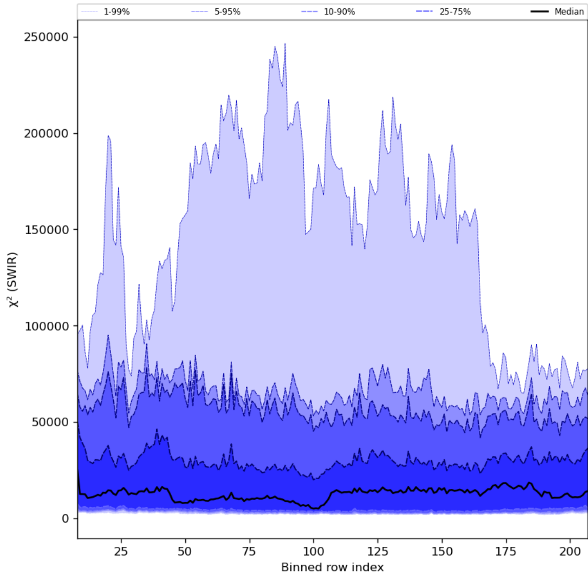
Figure 39: Along track statistics of " \chi^2 (SWIR)" for 2024-03-28 to 2024-03-30
