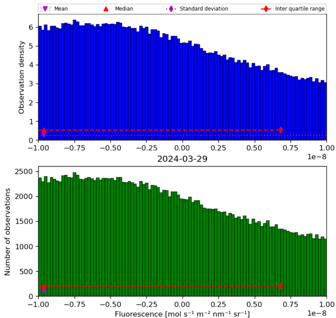
Figure 32: Histogram of “Fluorescence” for 2024-03-28 to 2024-03-30
