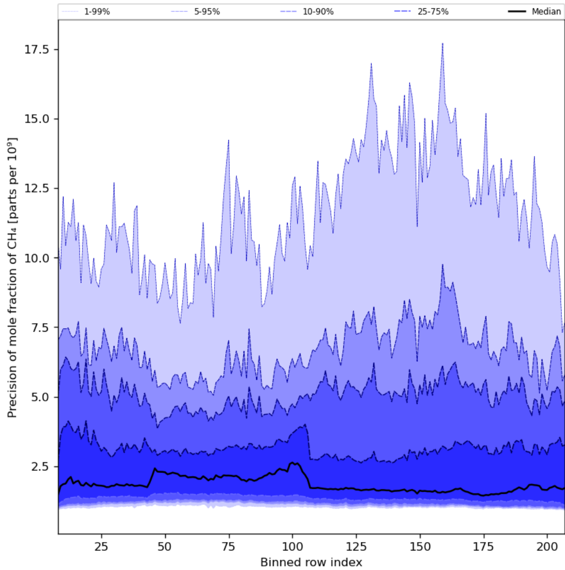
Figure 35: Along track statistics of “Precision of mole fraction of CH 4 ” for 2024-03-28 to 2024-03-30
