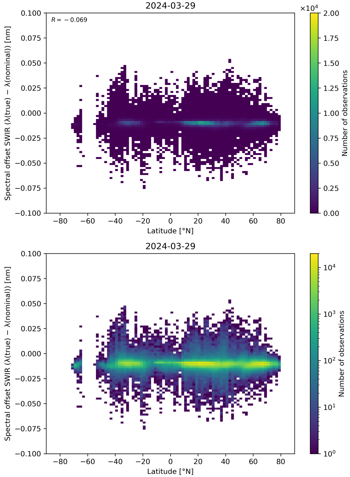
Figure 62: Scatter density plot of “Latitude” against “Spectral offset SWIR ( \lambda(\text{true}) - \lambda(\text{nominal}) )” for 2024-03-28 to 2024-03-30.
