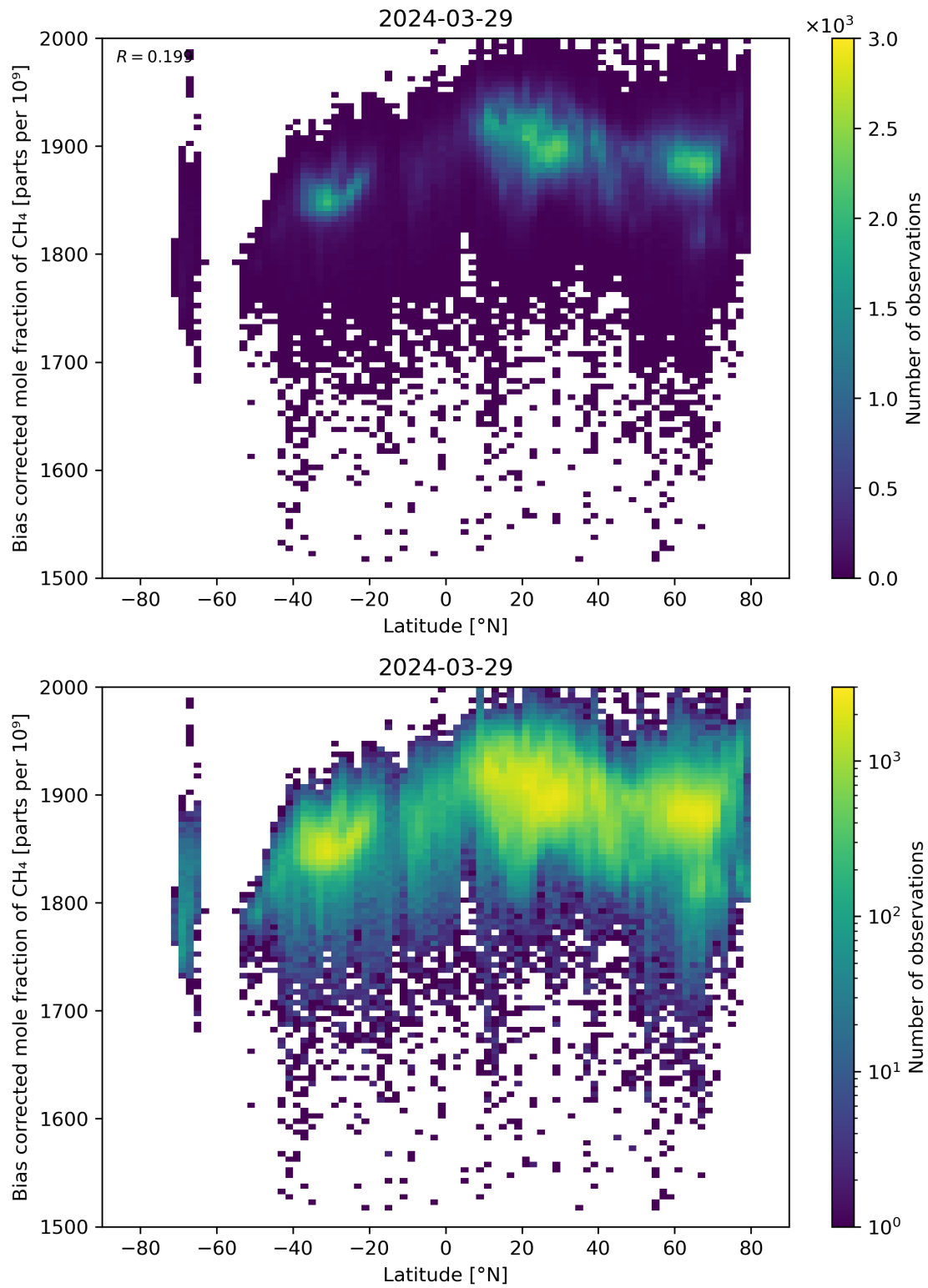
Figure 58: Scatter density plot of “Latitude” against “Bias corrected mole fraction of CH 4 ” for 2024-03-28 to 2024-03-30.
