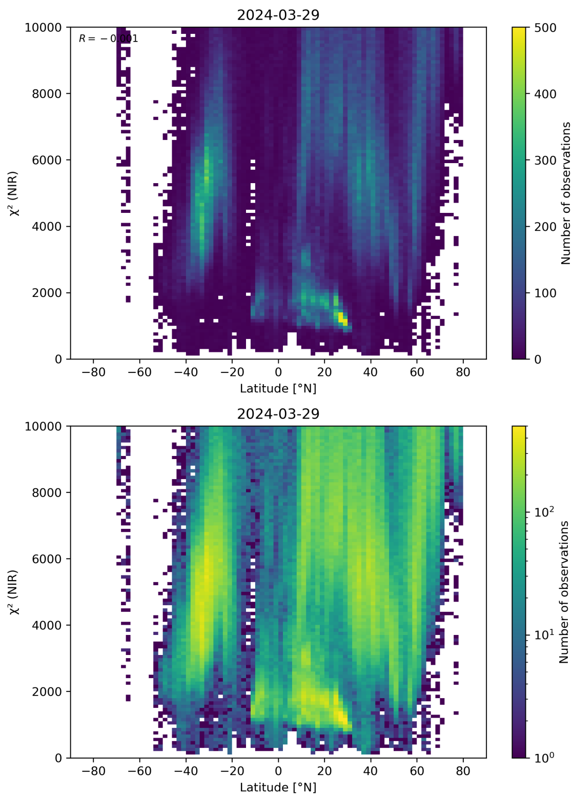
Figure 53: Scatter density plot of “Latitude” against “ \chi^2 (NIR)” for 2024-03-28 to 2024-03-30.
