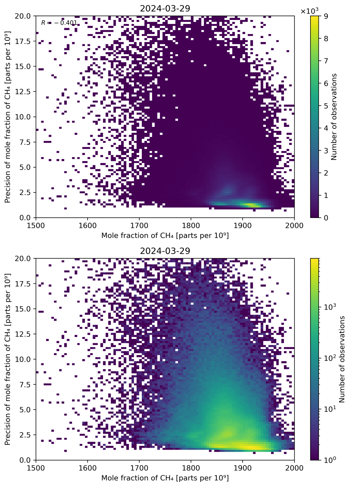
Figure 75: Scatter density plot of “Mole fraction of CH 4 ” against “Precision of mole fraction of CH 4 ” for 2024-03-28 to 2024-03-30.
