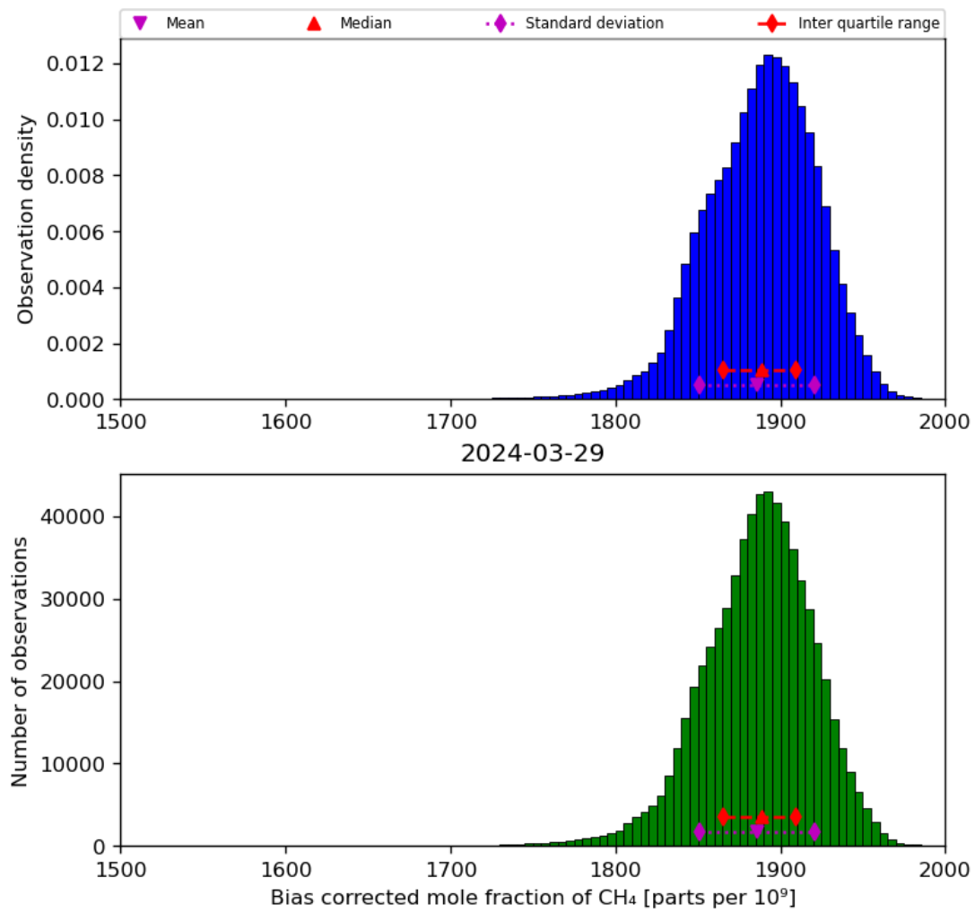
Figure 25: Histogram of “Bias corrected mole fraction of CH 4 ” for 2024-03-28 to 2024-03-30
