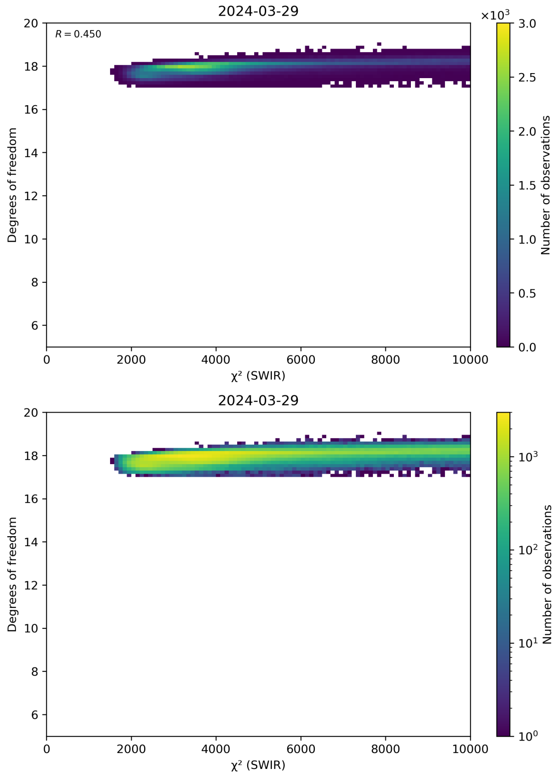
Figure 48: Scatter density plot of “ \chi^2 (SWIR)” against “Degrees of freedom” for 2024-03-28 to 2024-03-30.
