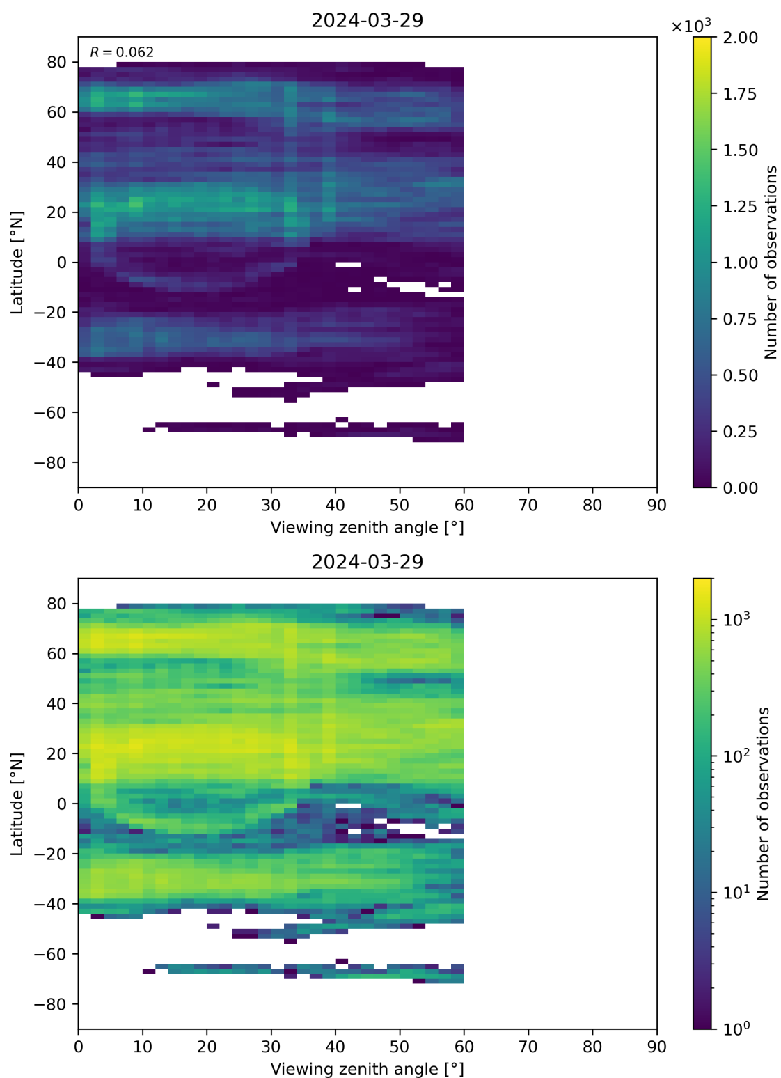
Figure 109: Scatter density plot of “Viewing zenith angle” against “Latitude” for 2024-03-28 to 2024-03-30.
