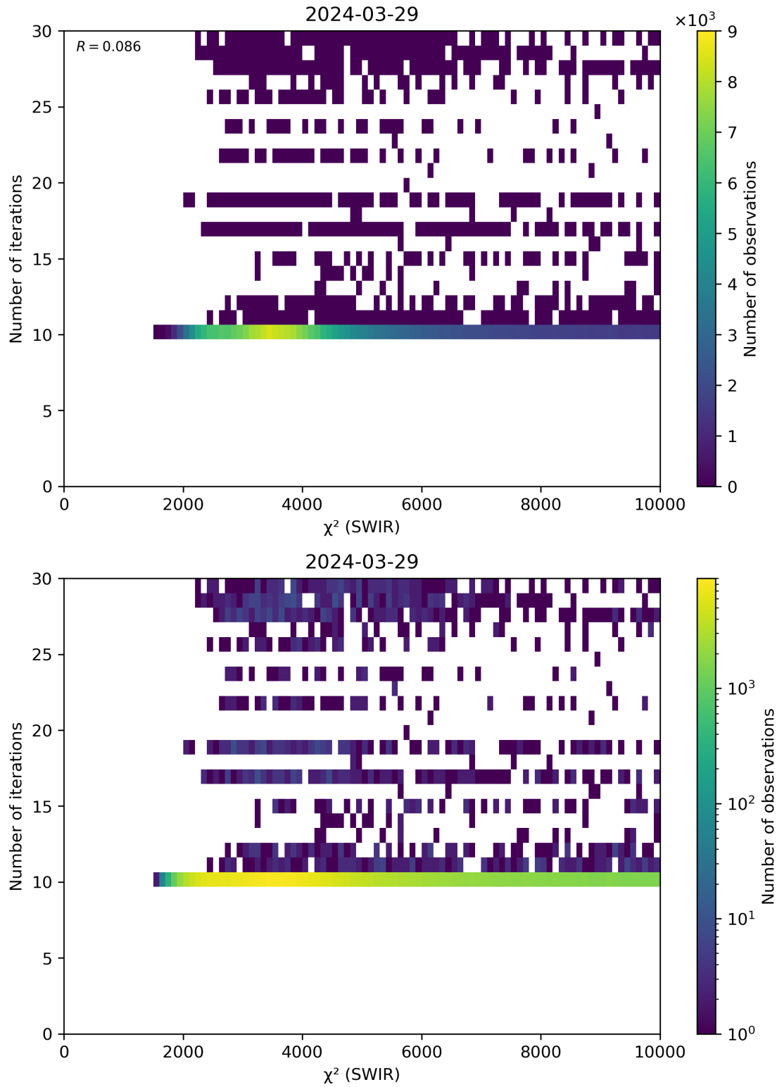
Figure 50: Scatter density plot of “ \chi^2 (SWIR)” against “Number of iterations” for 2024-03-28 to 2024-03-30.
