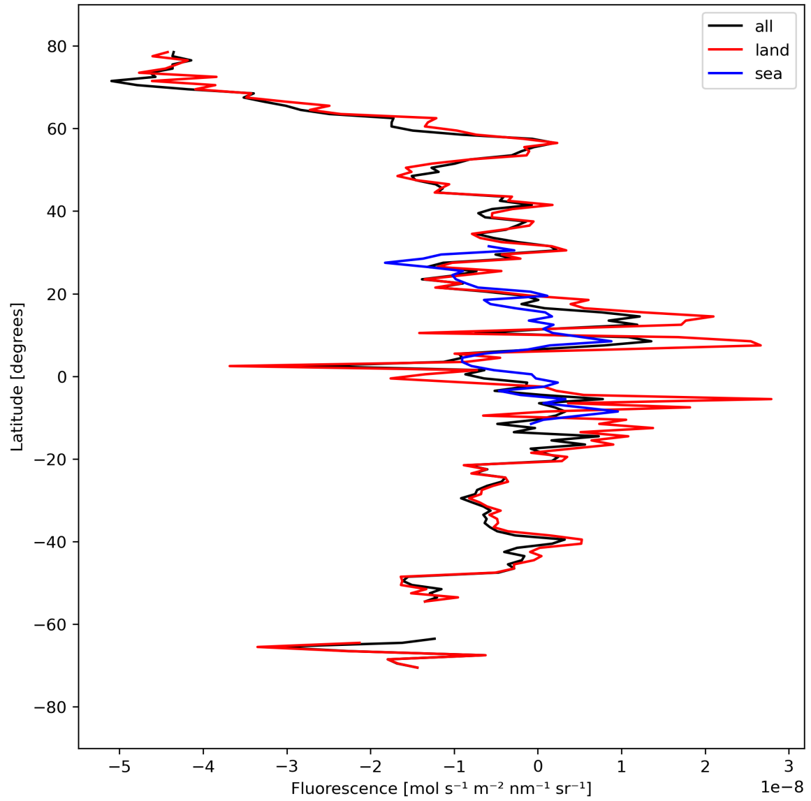
Figure 21: Zonal average of “Fluorescence” for 2024-03-28 to 2024-03-30.
