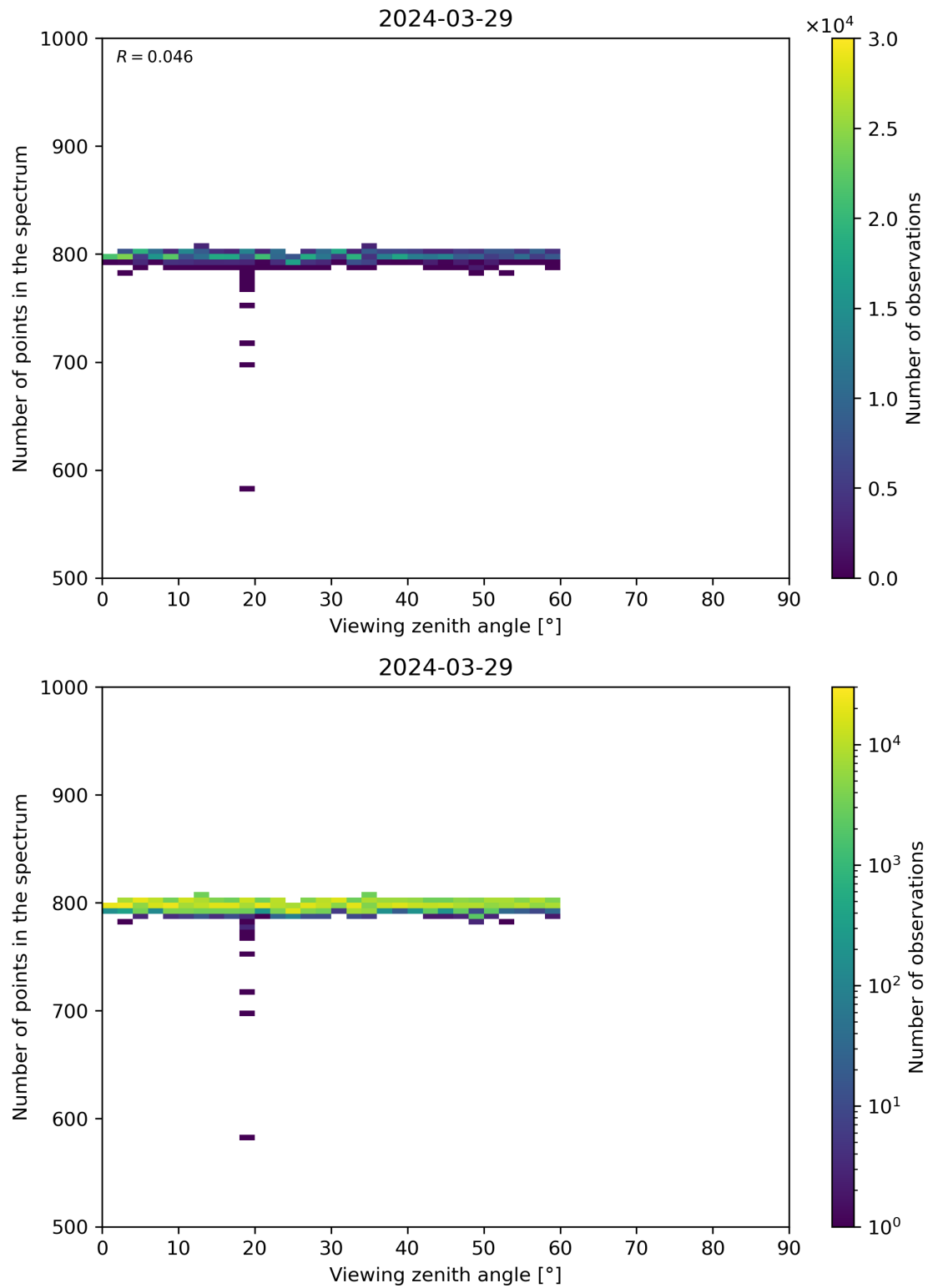
Figure 114: Scatter density plot of “Viewing zenith angle” against “Number of points in the spectrum” for 2024-03-28 to 2024-03-30.
