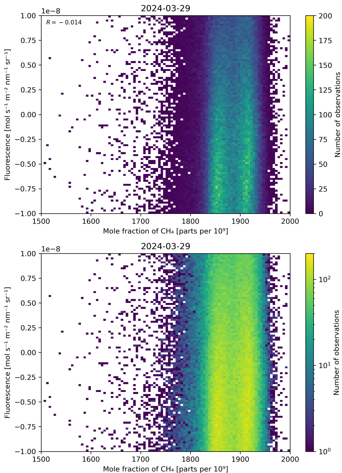
Figure 73: Scatter density plot of “Mole fraction of \text{CH}_4 ” against “Fluorescence” for 2024-03-28 to 2024-03-30.
