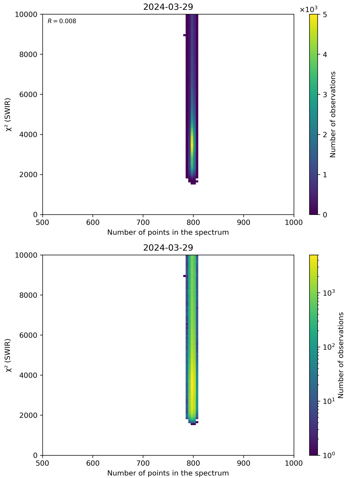
Figure 89: Scatter density plot of “Number of points in the spectrum” against “ \chi^2 (SWIR)” for 2024-03-28 to 2024-03-30.
