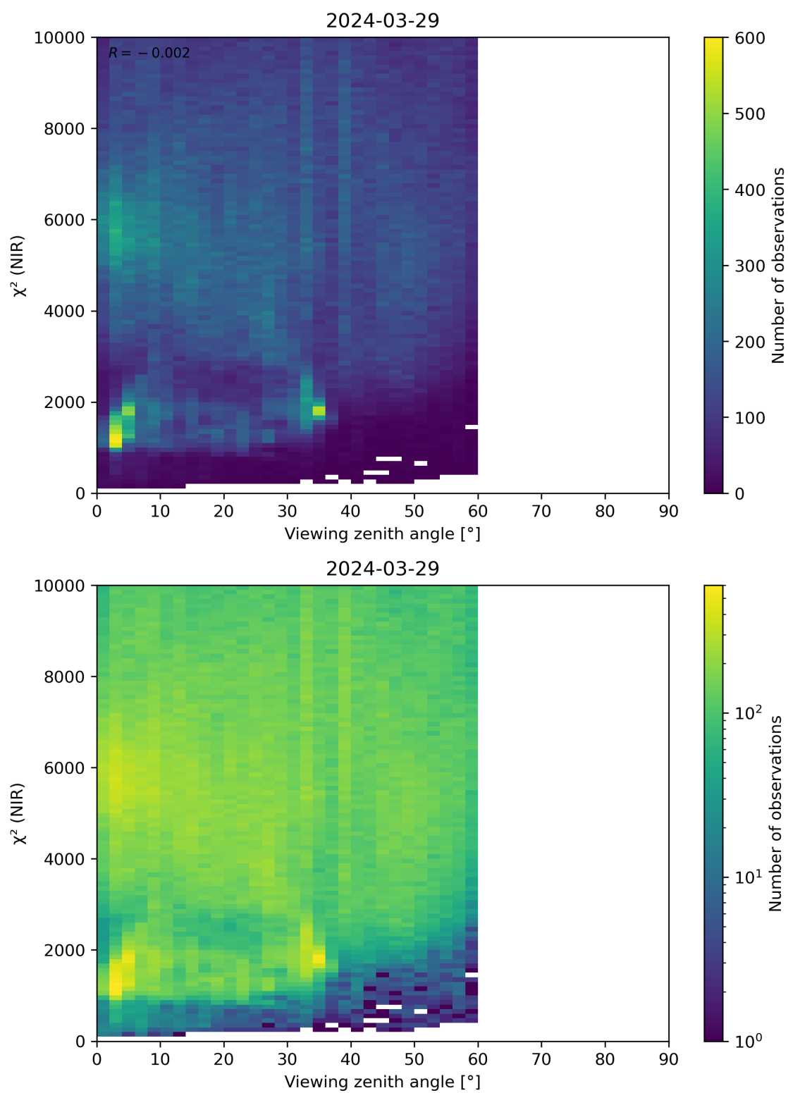
Figure 105: Scatter density plot of “Viewing zenith angle” against “ \chi^2 (NIR)” for 2024-03-28 to 2024-03-30.
