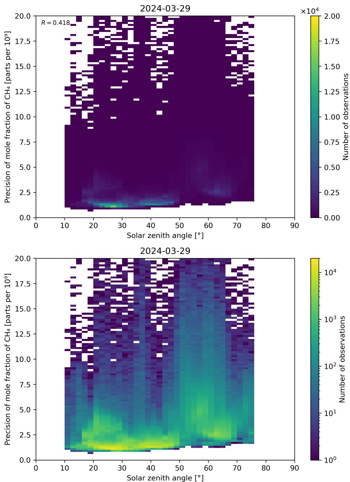
Figure 101: Scatter density plot of “Solar zenith angle” against “Precision of mole fraction of CH 4 ” for 2024-03-28 to 2024-03-30.
