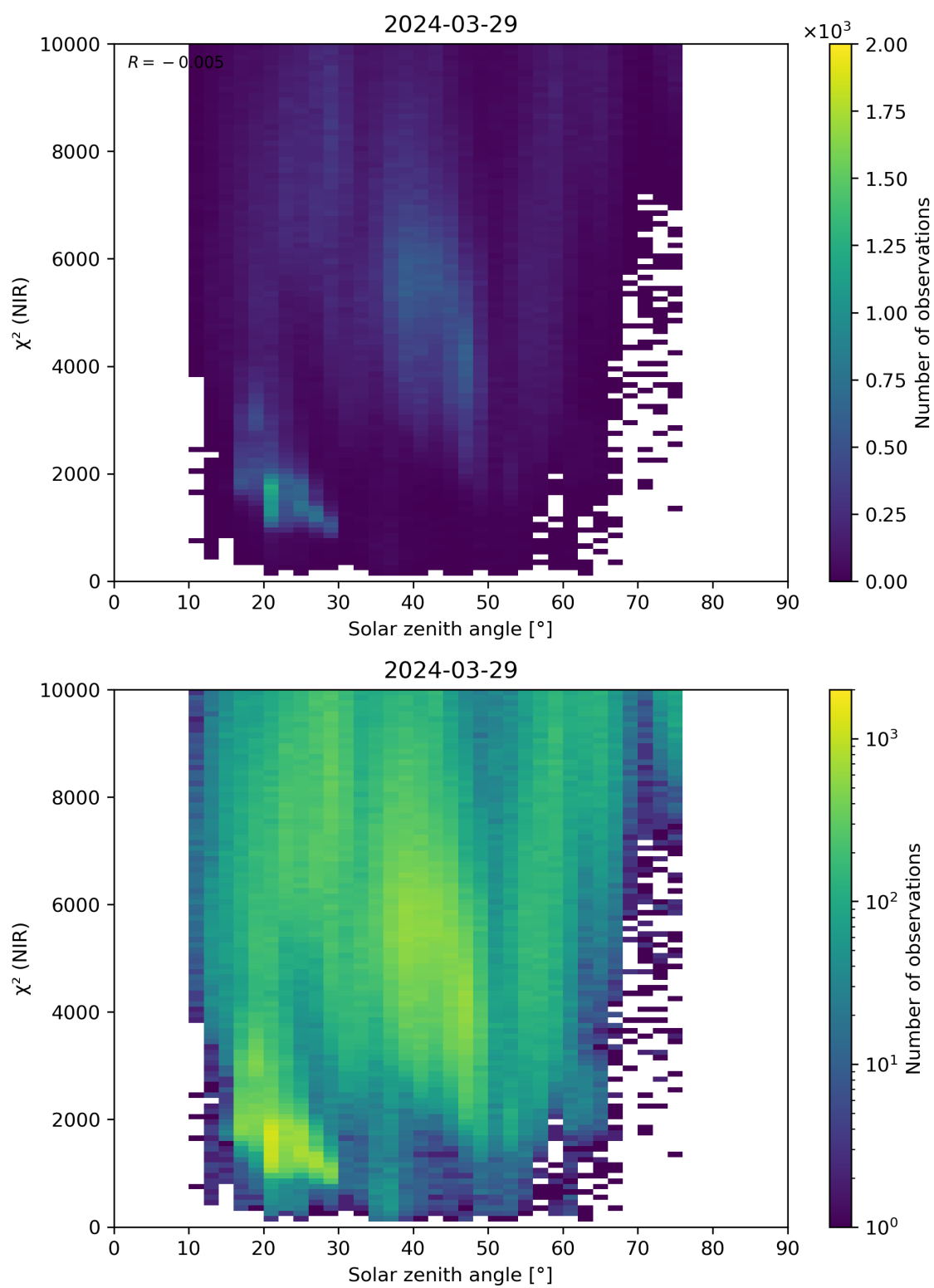
Figure 94: Scatter density plot of “Solar zenith angle” against “ \chi^2 (NIR)” for 2024-03-28 to 2024-03-30.
