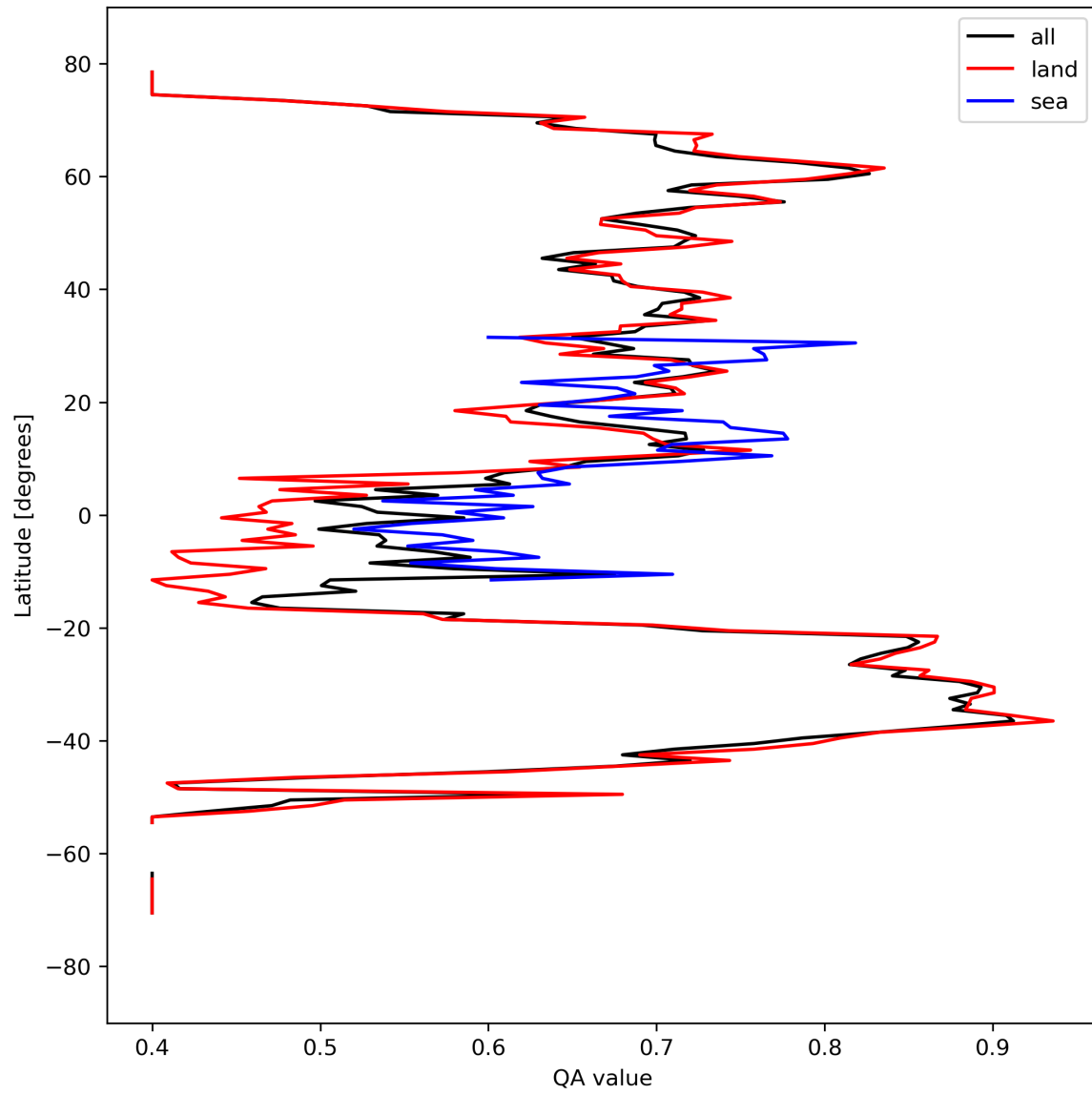
Figure 11: Zonal average of “QA value” for 2024-03-28 to 2024-03-30.
