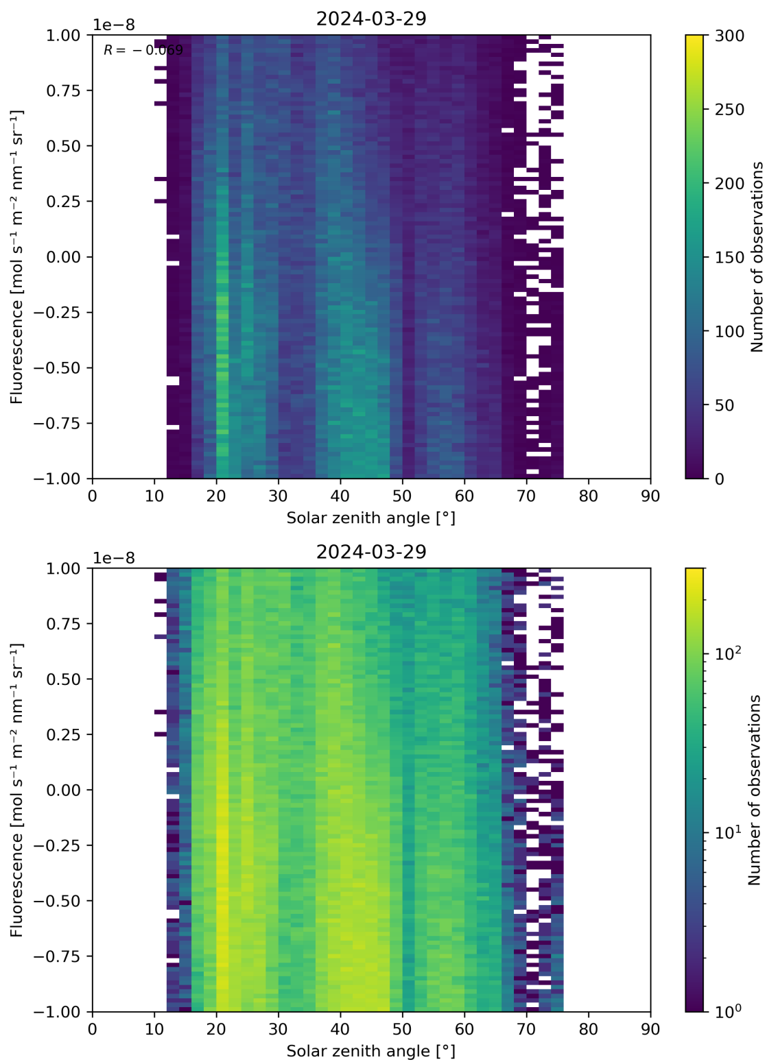
Figure 97: Scatter density plot of “Solar zenith angle” against “Fluorescence” for 2024-03-28 to 2024-03-30.
