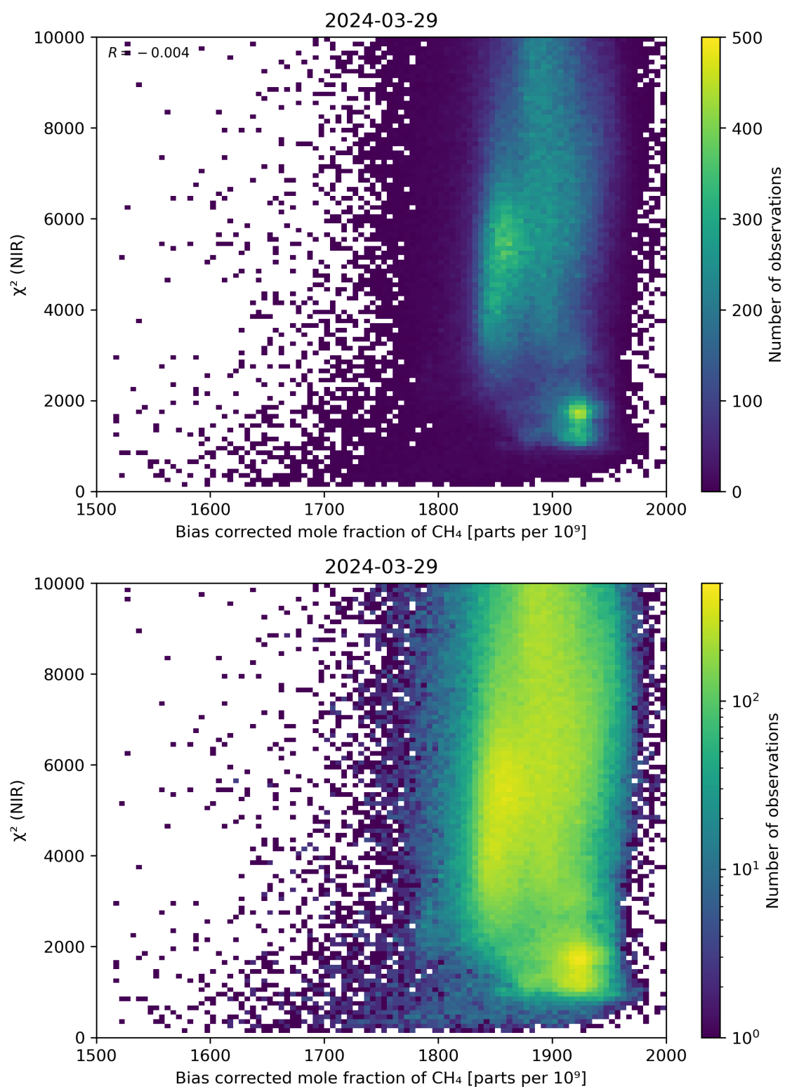
Figure 63: Scatter density plot of “Bias corrected mole fraction of CH 4 ” against “ \chi^2 (NIR)” for 2024-03-28 to 2024-03-30.
