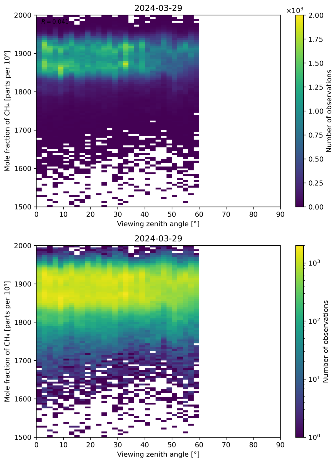
Figure 110: Scatter density plot of “Viewing zenith angle” against “Mole fraction of CH 4 ” for 2024-03-28 to 2024-03-30.
