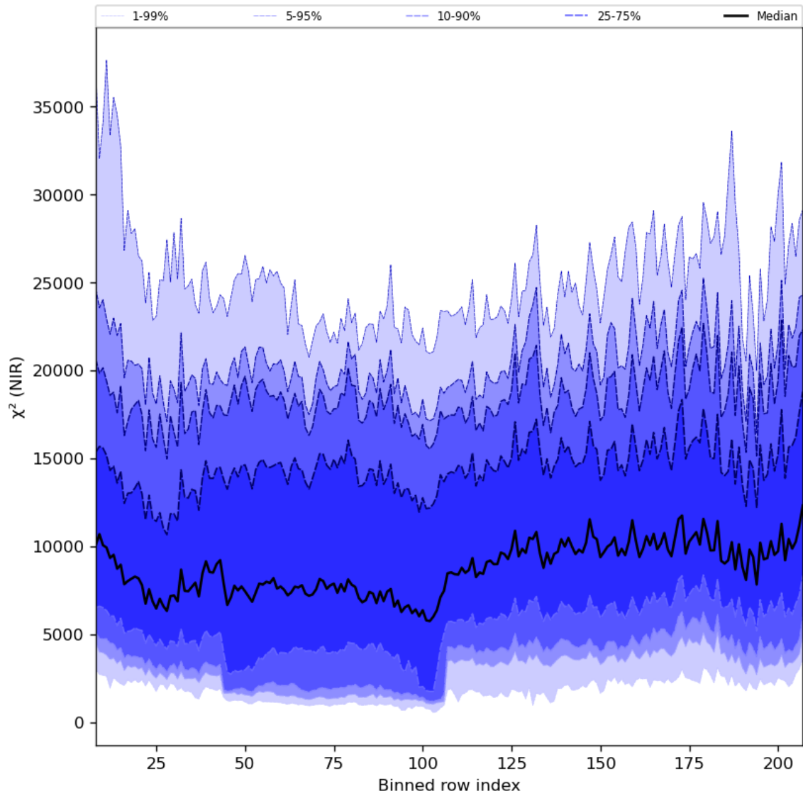
Figure 40: Along track statistics of " \chi^2 (NIR)" for 2024-03-28 to 2024-03-30
