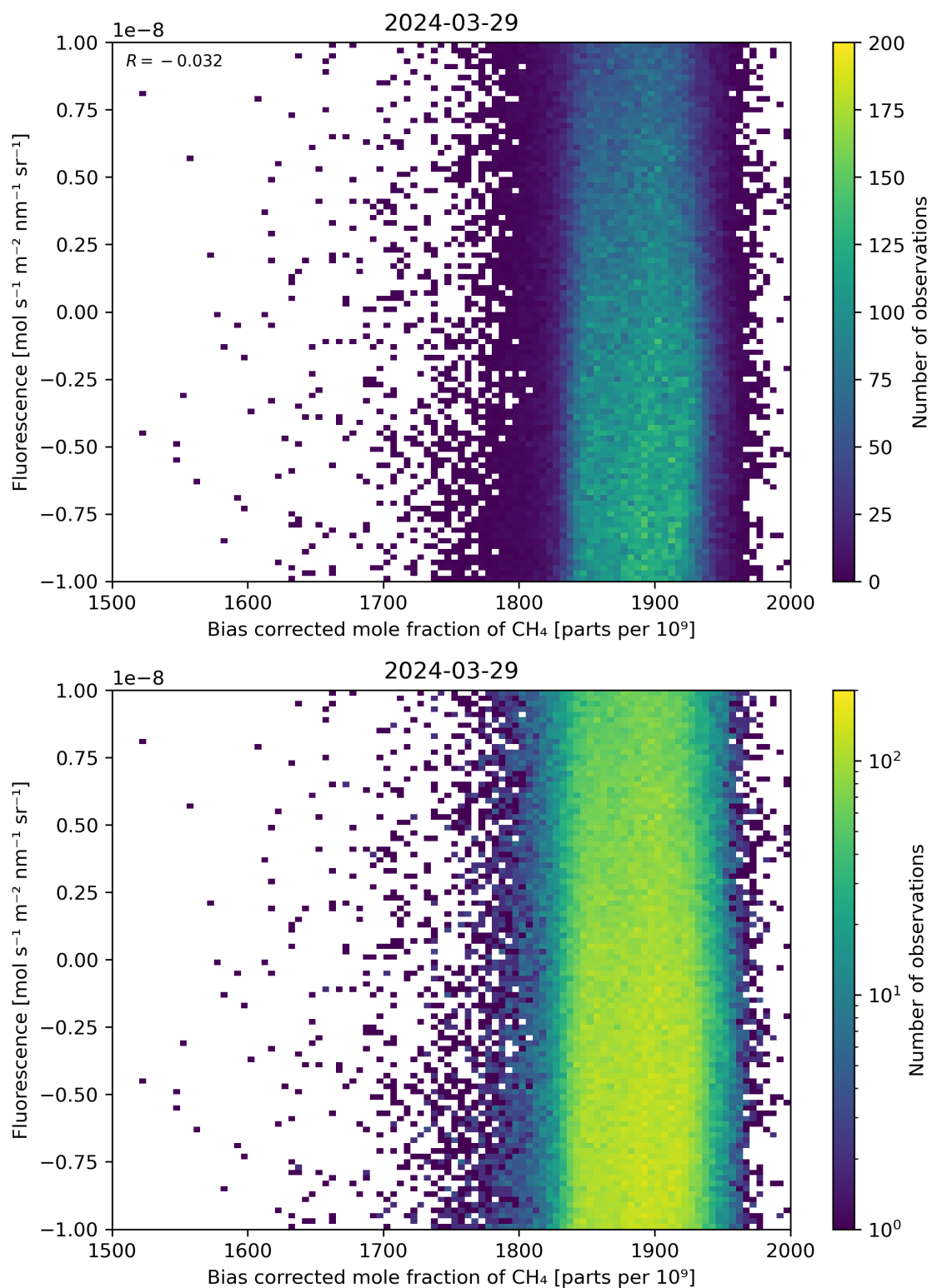
Figure 66: Scatter density plot of “Bias corrected mole fraction of \text{CH}_4 ” against “Fluorescence” for 2024-03-28 to 2024-03-30.
