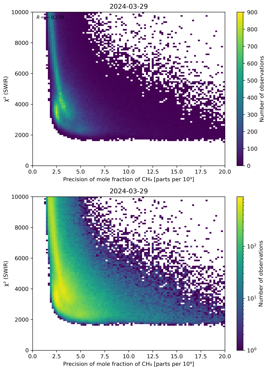
Figure 79: Scatter density plot of “Precision of mole fraction of CH 4 ” against “ \chi^2 (SWIR)” for 2024-03-28 to 2024-03-30.
