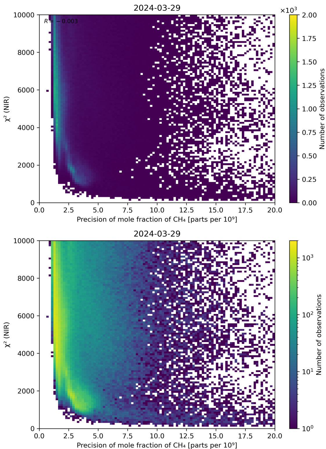
Figure 78: Scatter density plot of “Precision of mole fraction of \text{CH}_4 ” against “ \chi^2 (NIR)” for 2024-03-28 to 2024-03-30.
