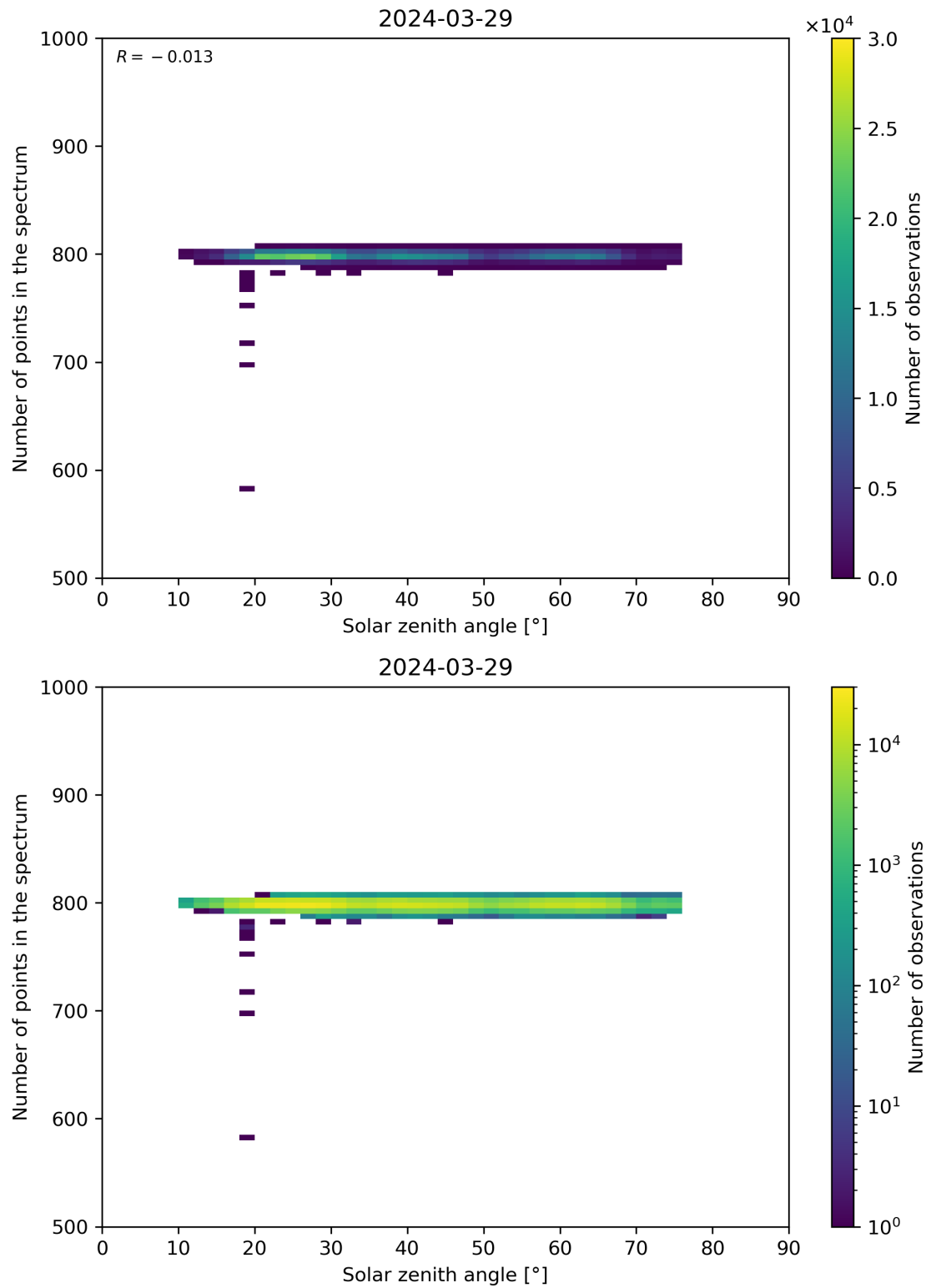
Figure 103: Scatter density plot of “Solar zenith angle” against “Number of points in the spectrum” for 2024-03-28 to 2024-03-30.
