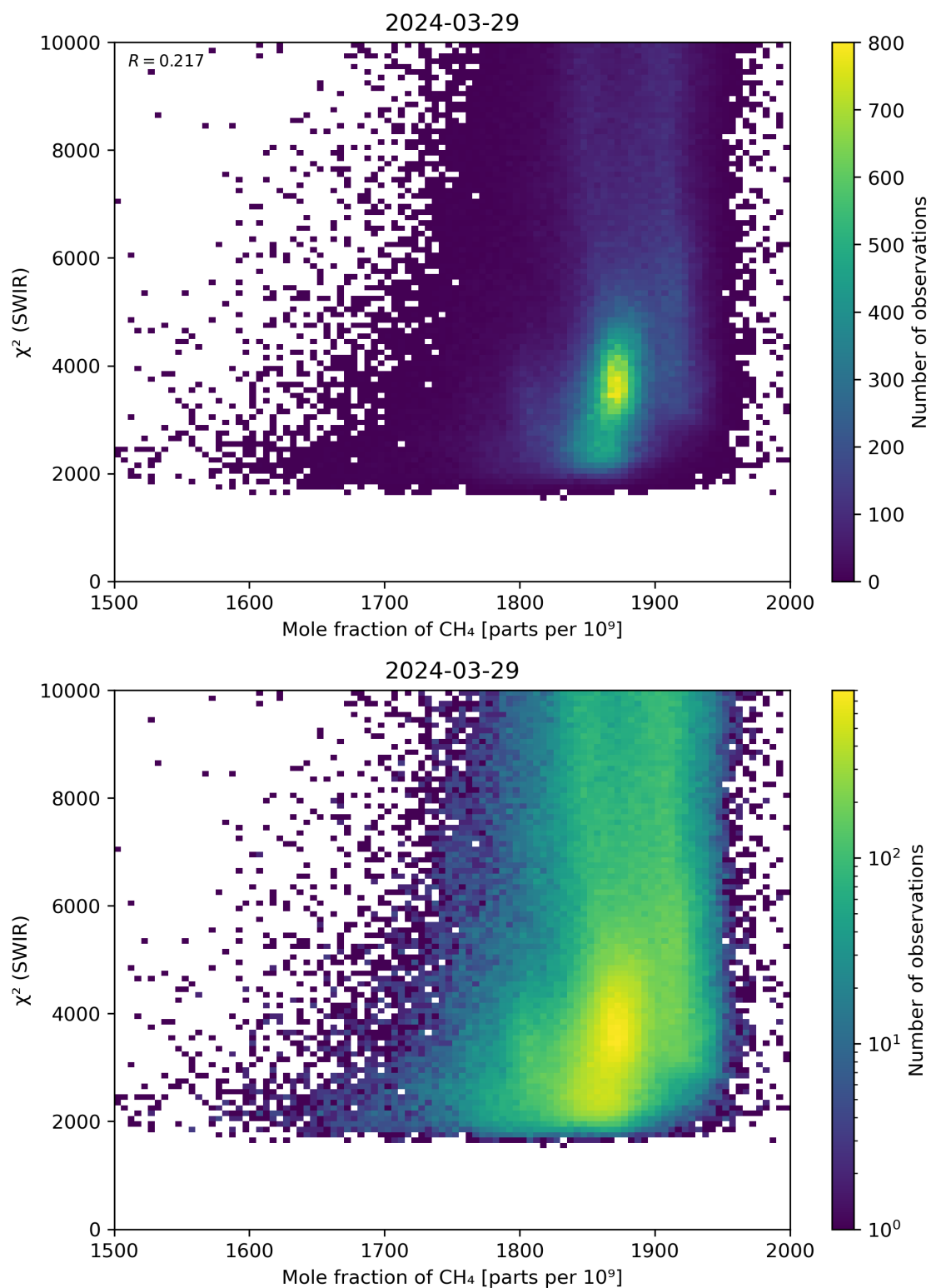
Figure 71: Scatter density plot of “Mole fraction of \text{CH}_4 ” against “ \chi^2 (SWIR)” for 2024-03-28 to 2024-03-30.
