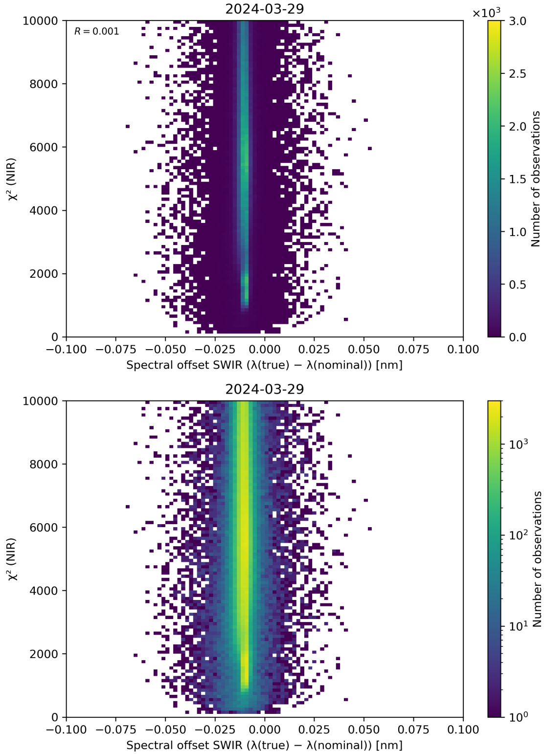
Figure 117: Scatter density plot of “Spectral offset SWIR ( \lambda(\text{true}) - \lambda(\text{nominal}) )” against “ \chi^2 (NIR)” for 2024-03-28 to 2024-03-30.
