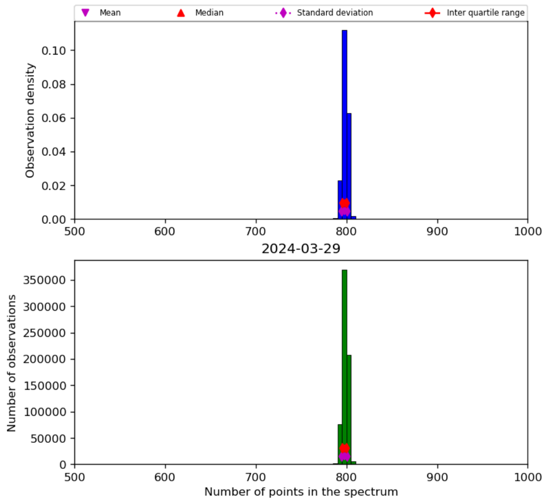
Figure 26: Histogram of “Number of points in the spectrum” for 2024-03-28 to 2024-03-30
