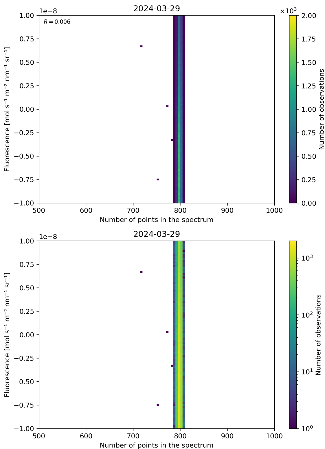
Figure 91: Scatter density plot of “Number of points in the spectrum” against “Fluorescence” for 2024-03-28 to 2024-03-30.
