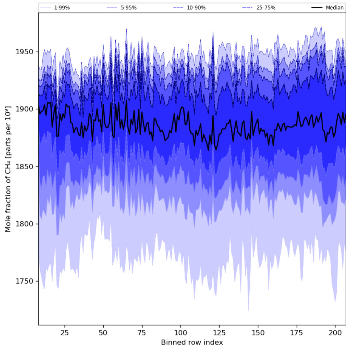
Figure 34: Along track statistics of “Mole fraction of CH 4 ” for 2024-03-28 to 2024-03-30
