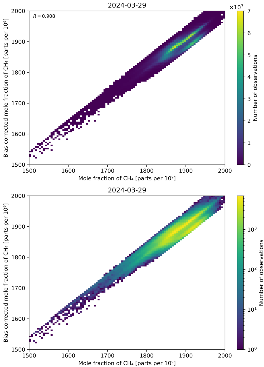
Figure 74: Scatter density plot of “Mole fraction of CH 4 ” against “Bias corrected mole fraction of CH 4 ” for 2024-03-28 to 2024-03-30.
