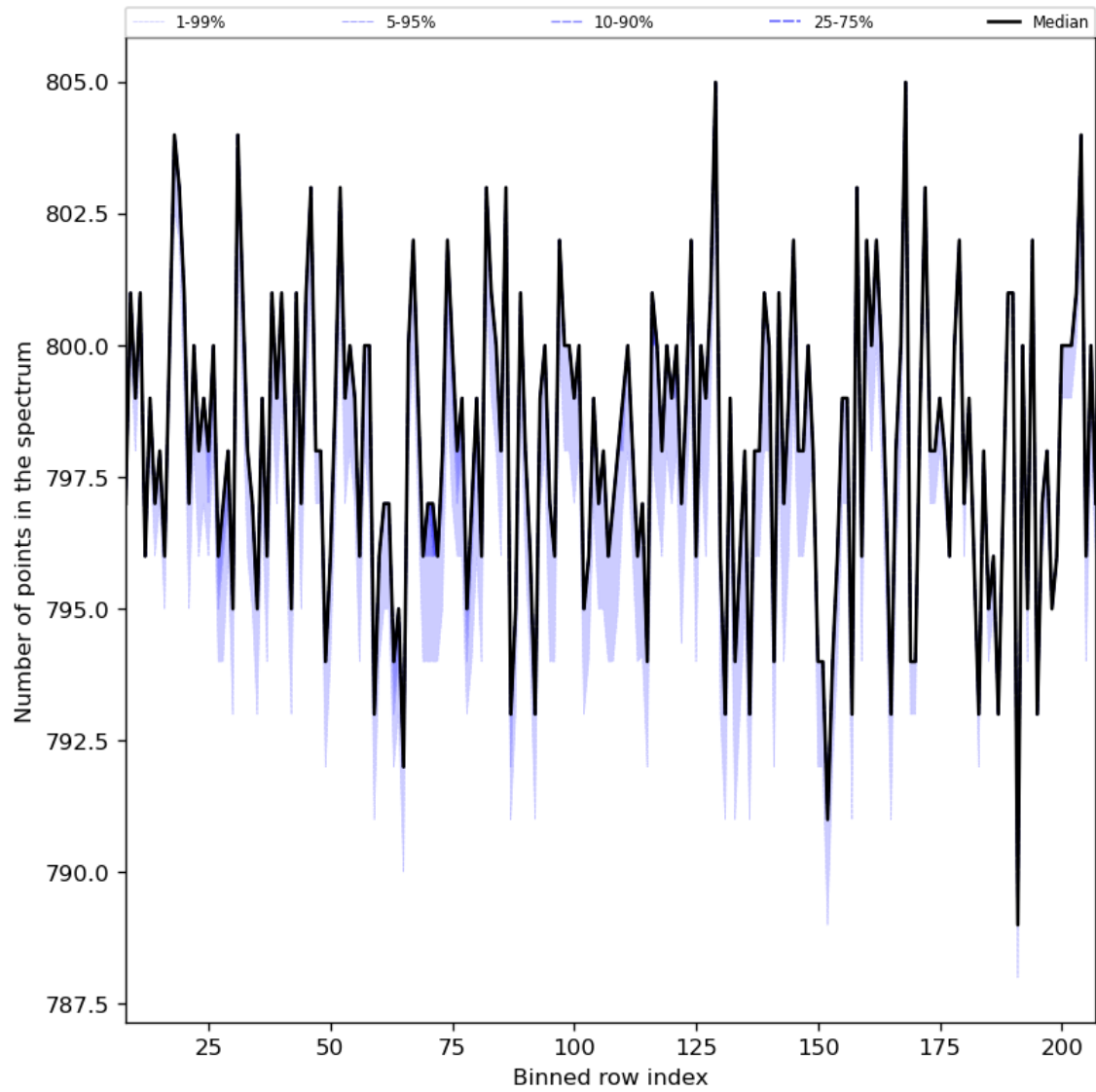
Figure 37: Along track statistics of “Number of points in the spectrum” for 2024-03-28 to 2024-03-30
