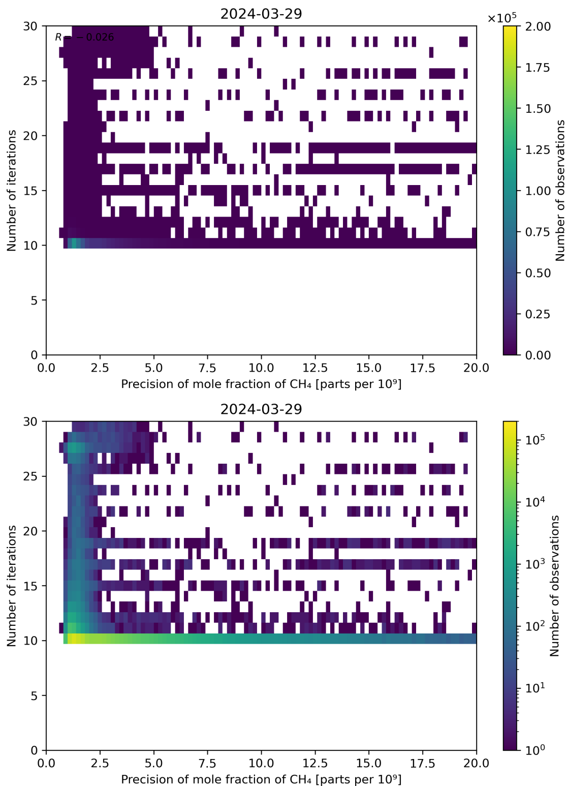
Figure 83: Scatter density plot of “Precision of mole fraction of CH 4 ” against “Number of iterations” for 2024-03-28 to 2024-03-30.
