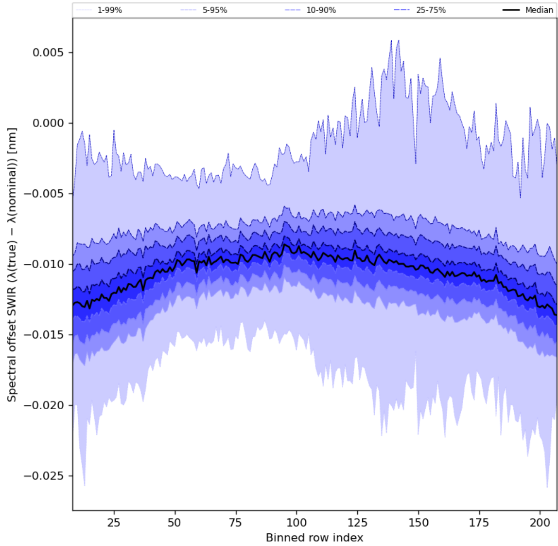
Figure 38: Along track statistics of “Spectral offset SWIR ( \lambda(\text{true}) - \lambda(\text{nominal}) )” for 2024-03-28 to 2024-03-30
