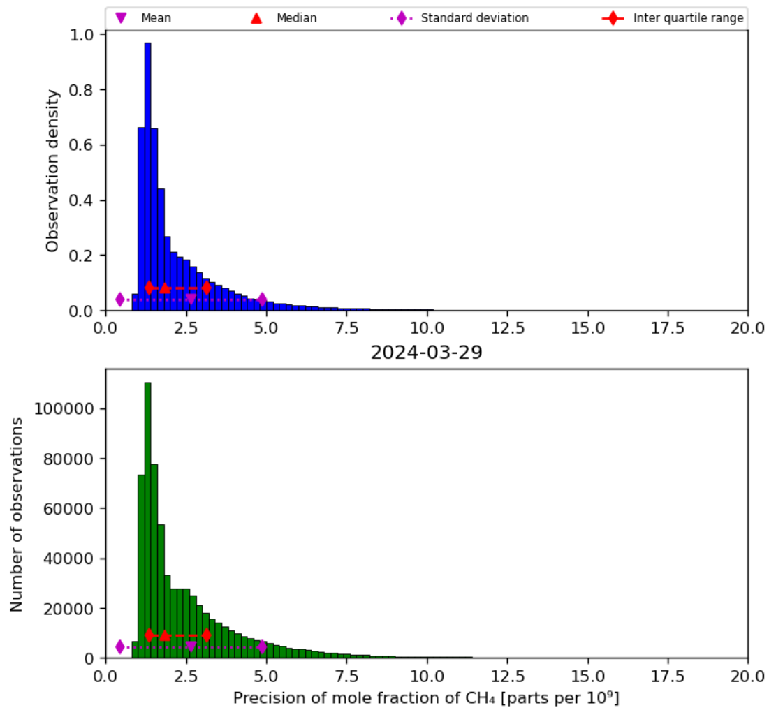
Figure 24: Histogram of “Precision of mole fraction of CH 4 ” for 2024-03-28 to 2024-03-30
