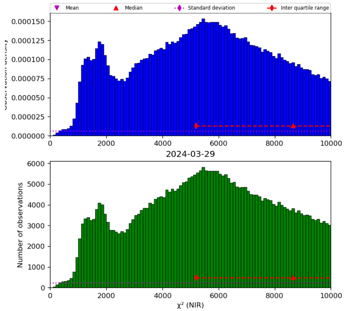
Figure 29: Histogram of “ \chi^2 (NIR)” for 2024-03-28 to 2024-03-30
