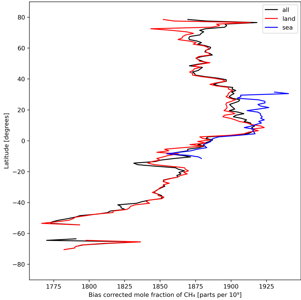
Figure 14: Zonal average of “Bias corrected mole fraction of CH 4 ” for 2024-03-28 to 2024-03-30.
