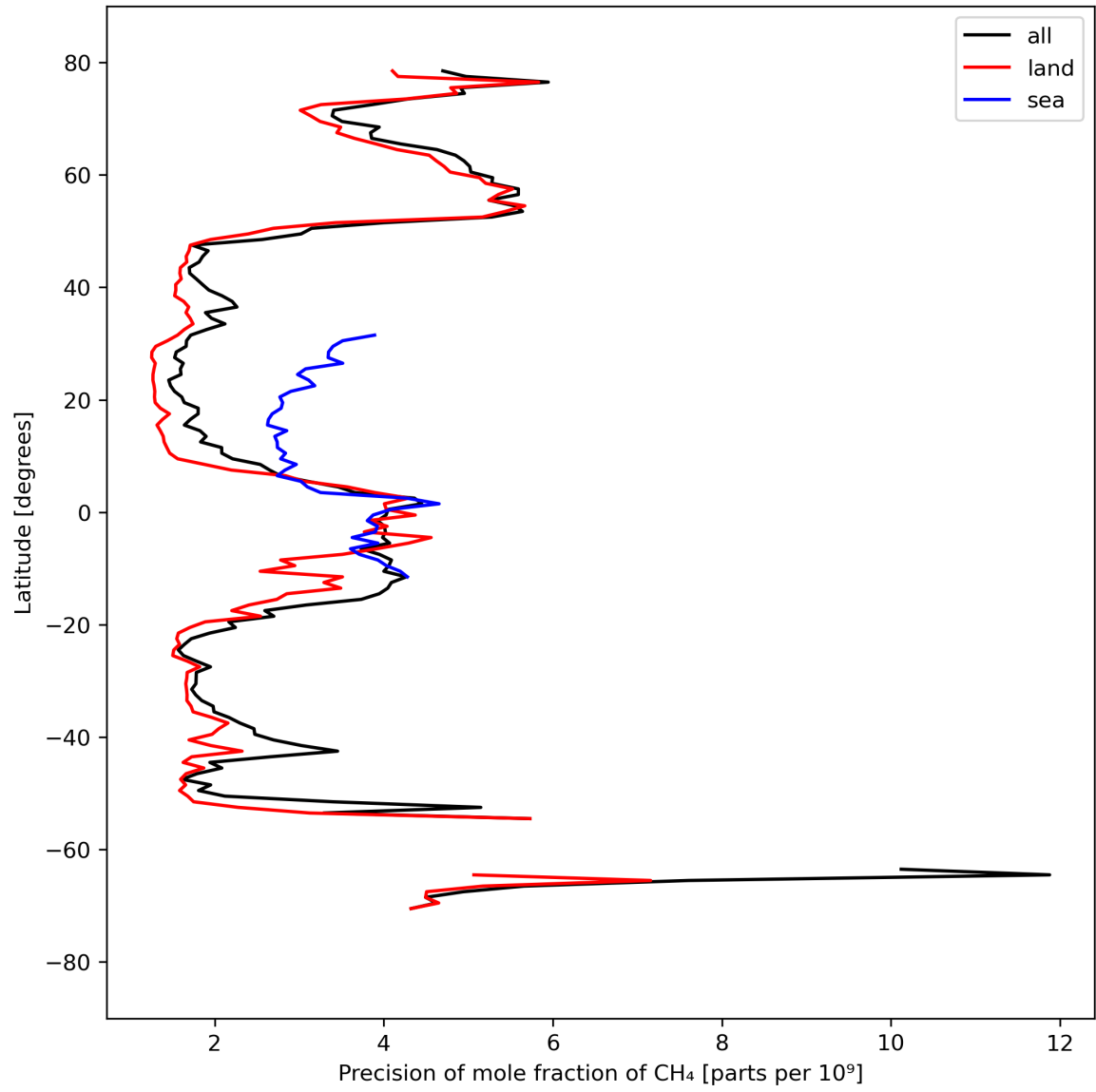
Figure 13: Zonal average of “Precision of mole fraction of CH 4 ” for 2024-03-28 to 2024-03-30.
