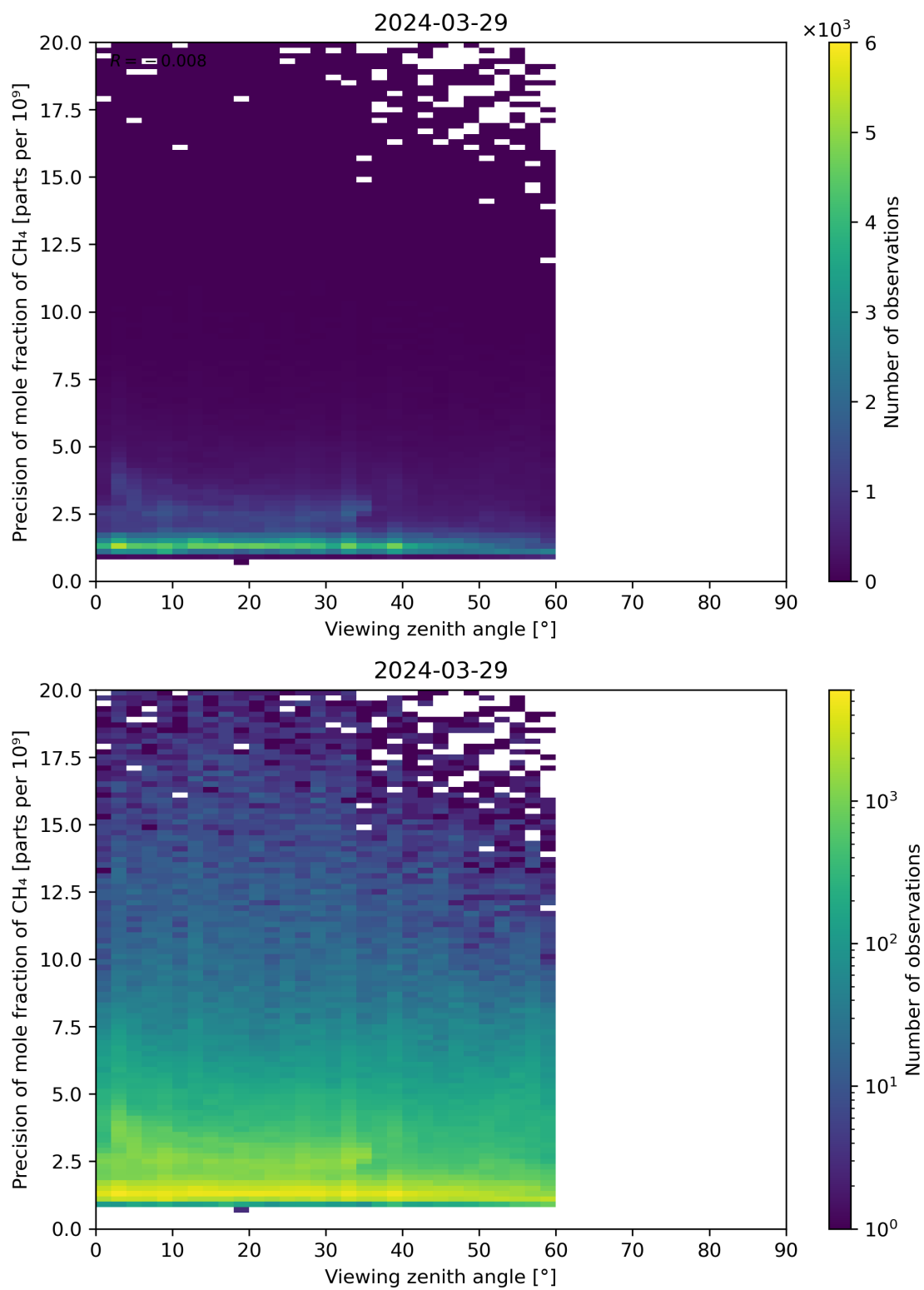
Figure 112: Scatter density plot of “Viewing zenith angle” against “Precision of mole fraction of CH 4 ” for 2024-03-28 to 2024-03-30.
