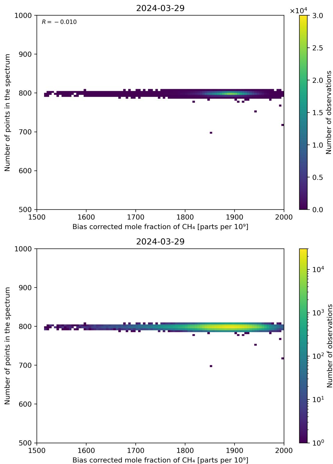
Figure 68: Scatter density plot of “Bias corrected mole fraction of CH 4 ” against “Number of points in the spectrum” for 2024-03-28 to 2024-03-30.
