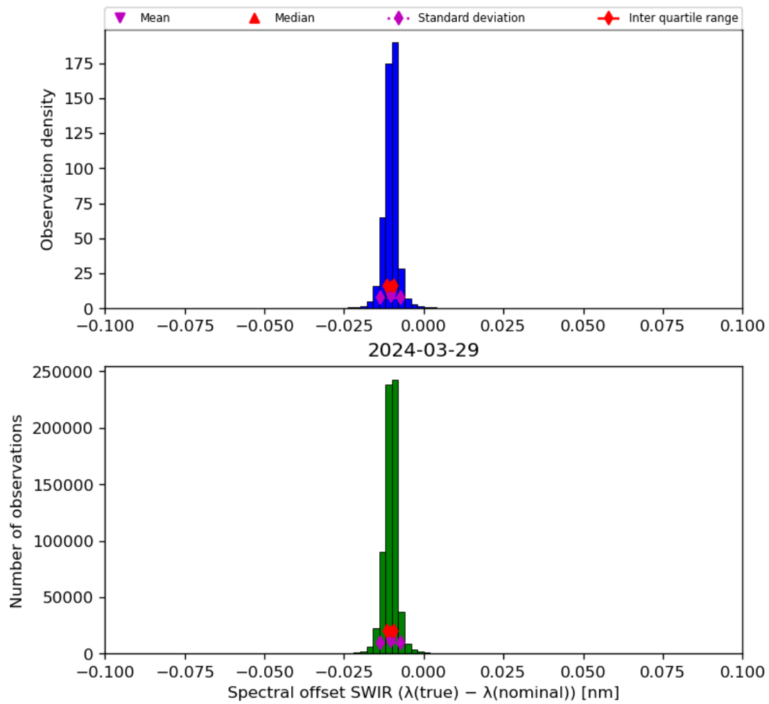
Figure 27: Histogram of “Spectral offset SWIR ( \lambda(\text{true}) - \lambda(\text{nominal}) )” for 2024-03-28 to 2024-03-30
