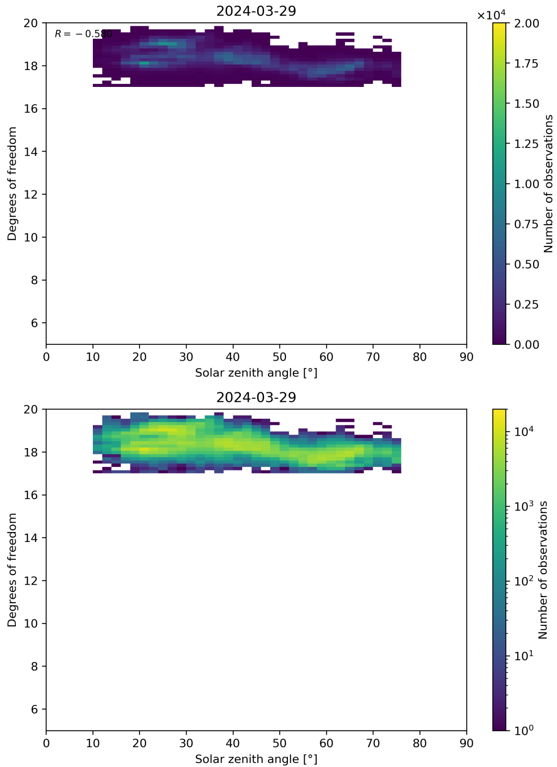
Figure 96: Scatter density plot of “Solar zenith angle” against “Degrees of freedom” for 2024-03-28 to 2024-03-30.
