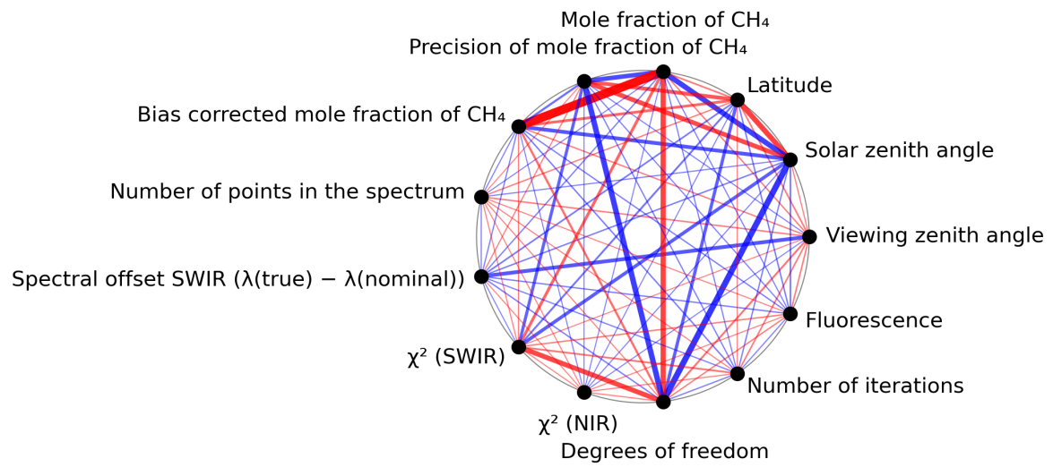
Figure 1: Map of correlation graph for 2024-03-28 to 2024-03-30.
