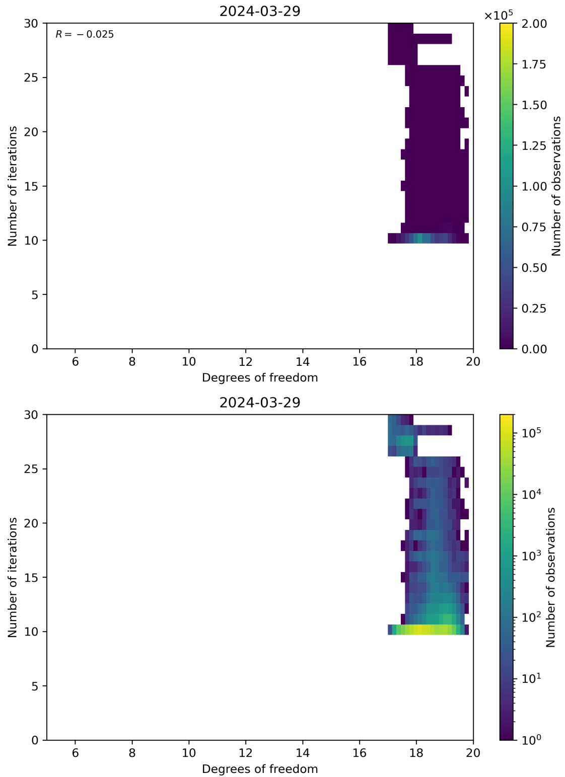
Figure 52: Scatter density plot of “Degrees of freedom” against “Number of iterations” for 2024-03-28 to 2024-03-30.
