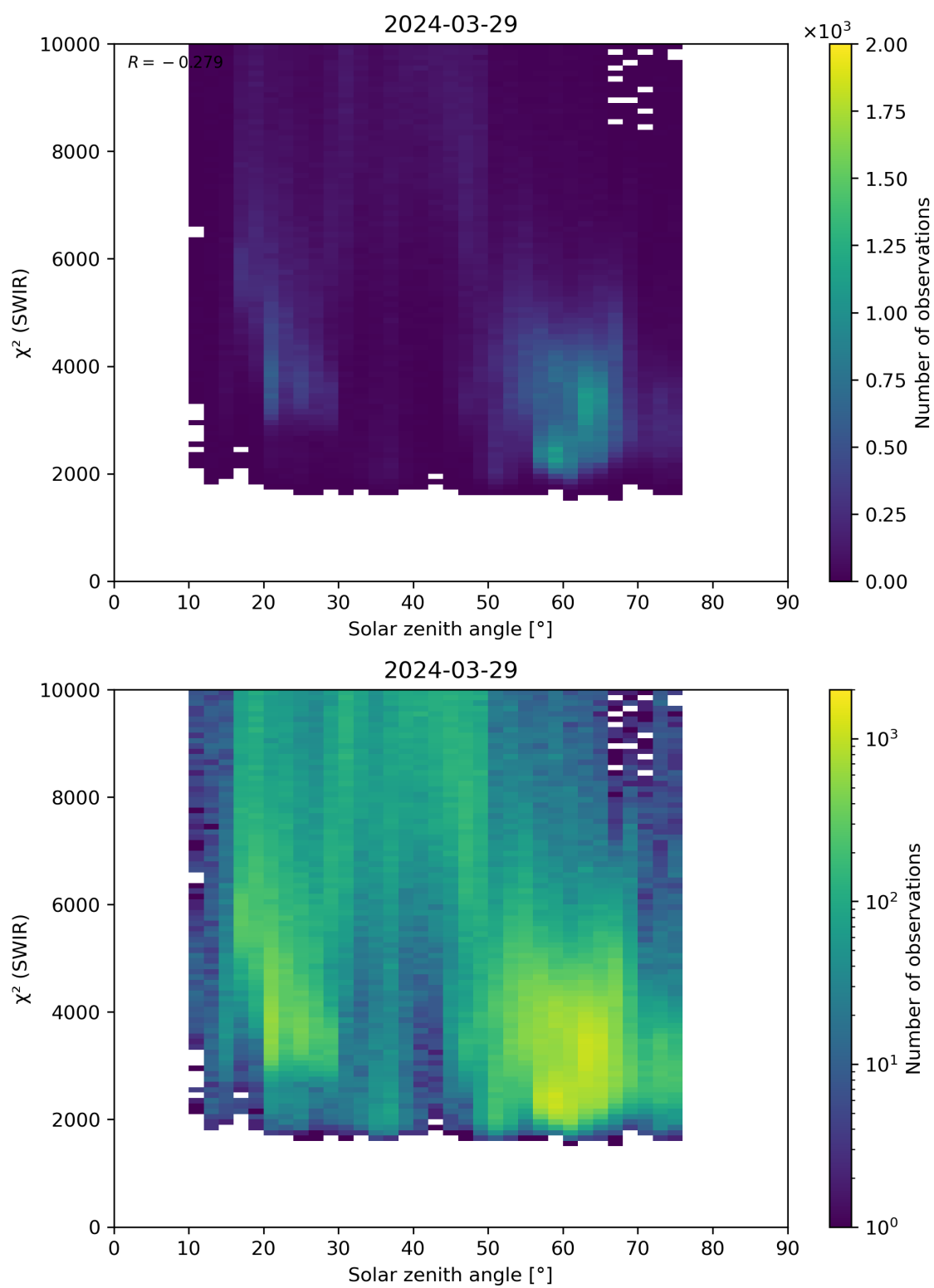
Figure 95: Scatter density plot of “Solar zenith angle” against “ \chi^2 (SWIR)” for 2024-03-28 to 2024-03-30.
