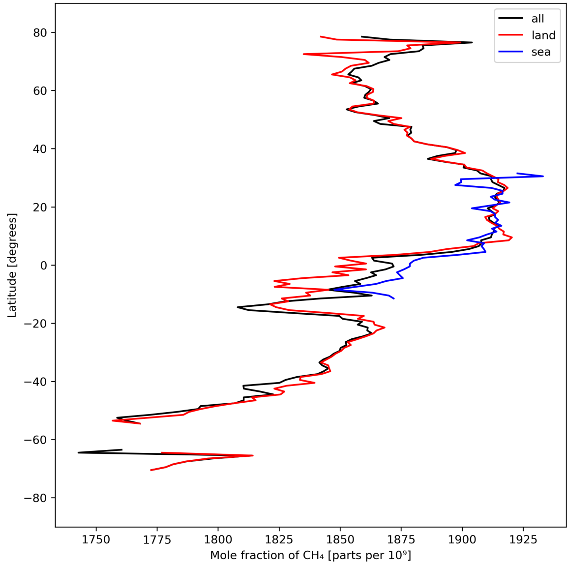
Figure 12: Zonal average of “Mole fraction of \text{CH}_4 ” for 2024-03-28 to 2024-03-30.
