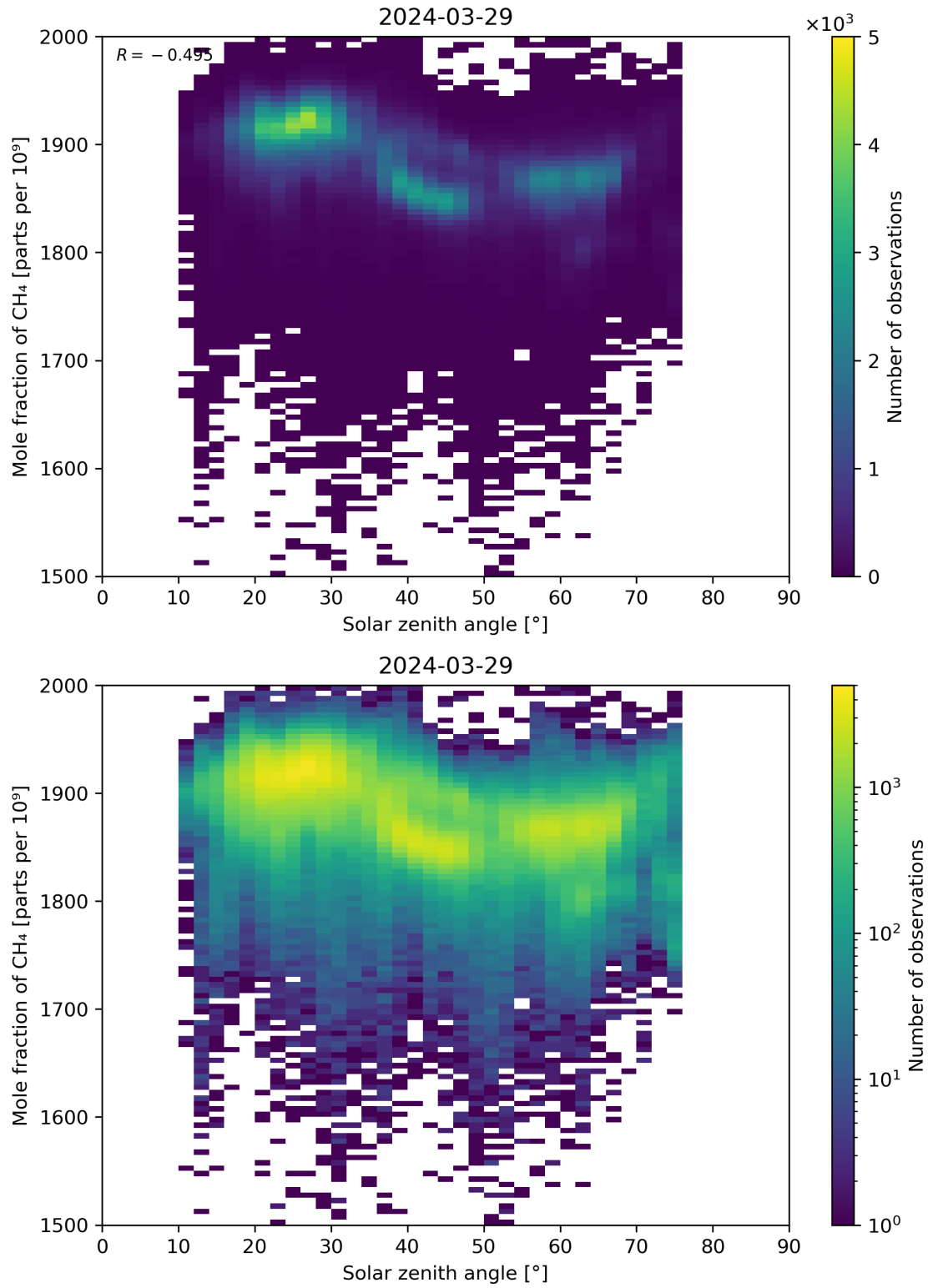
Figure 99: Scatter density plot of “Solar zenith angle” against “Mole fraction of CH 4 ” for 2024-03-28 to 2024-03-30.
