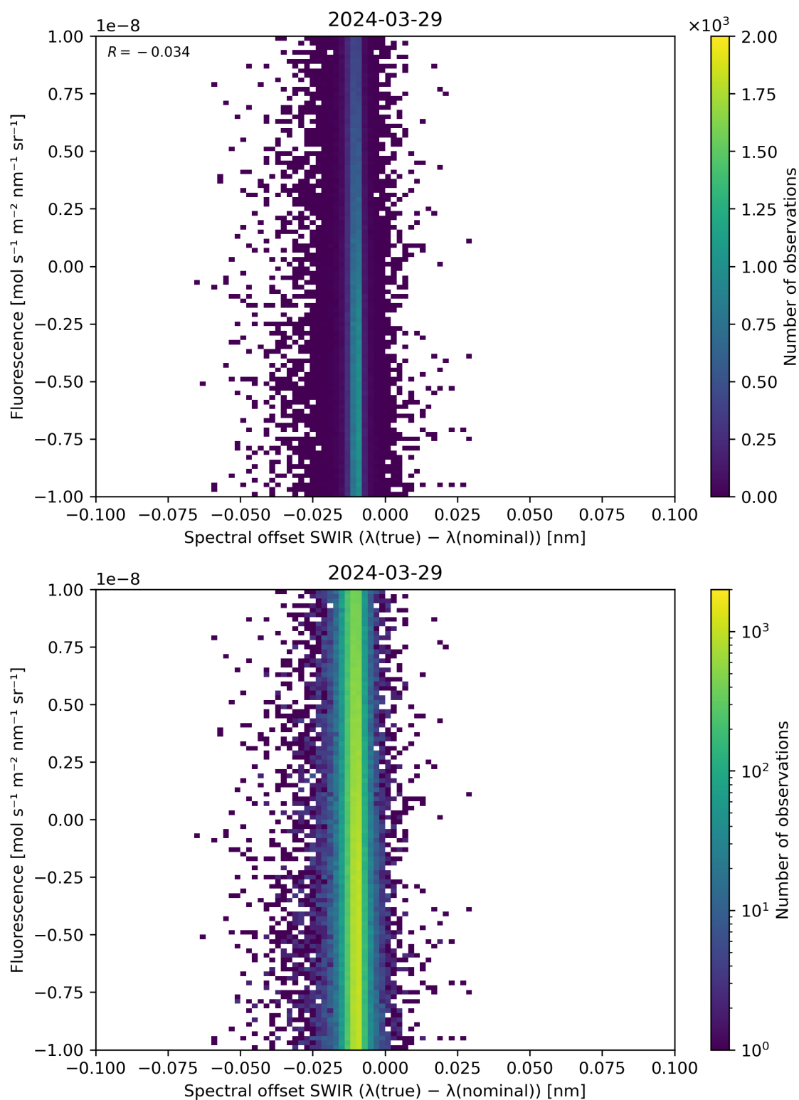
Figure 120: Scatter density plot of “Spectral offset SWIR ( \lambda(\text{true}) - \lambda(\text{nominal}) )” against “Fluorescence” for 2024-03-28 to 2024-03-30.
