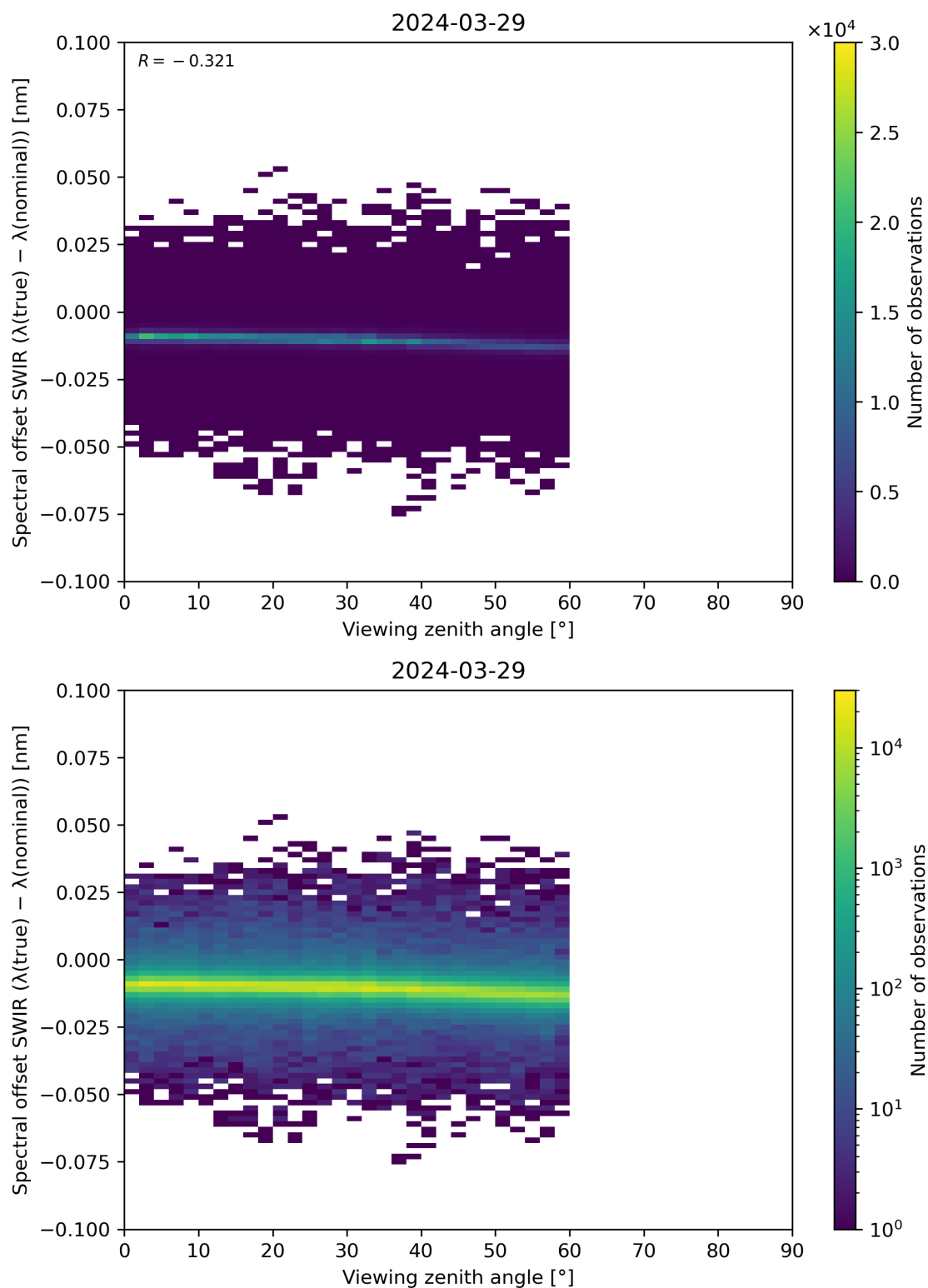
Figure 116: Scatter density plot of “Viewing zenith angle” against “Spectral offset SWIR ( \lambda(\text{true}) - \lambda(\text{nominal}) )” for 2024-03-28 to 2024-03-30.
