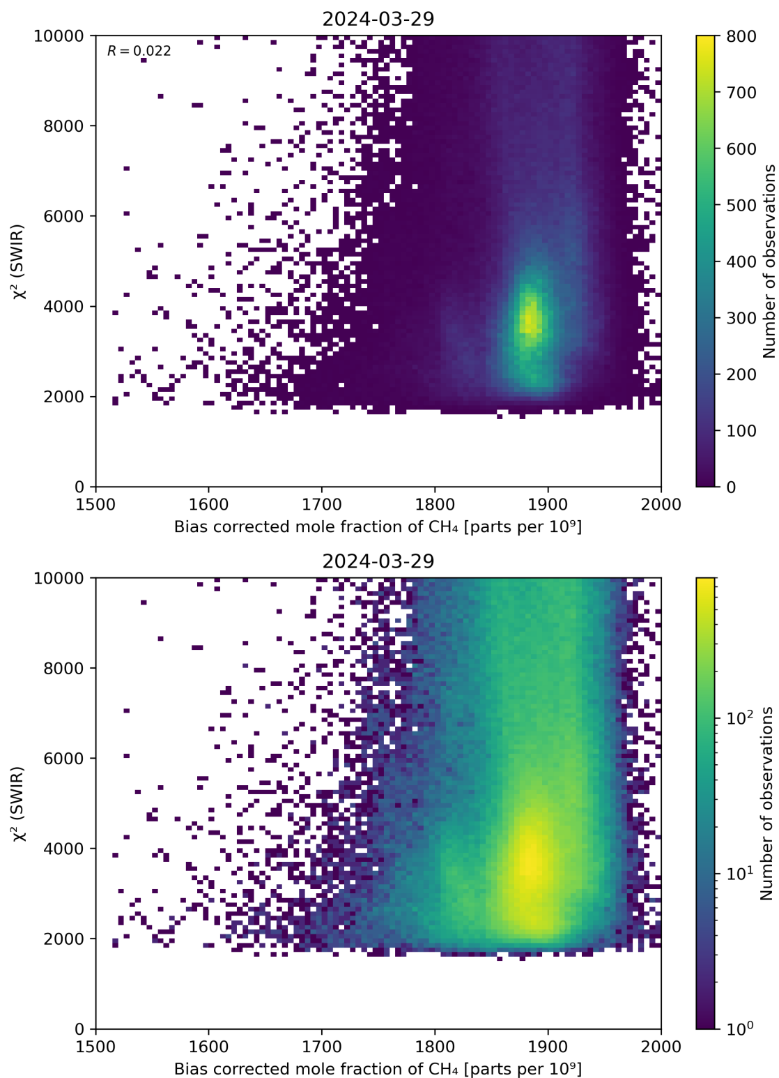
Figure 64: Scatter density plot of “Bias corrected mole fraction of CH 4 ” against “ \chi^2 (SWIR)” for 2024-03-28 to 2024-03-30.
