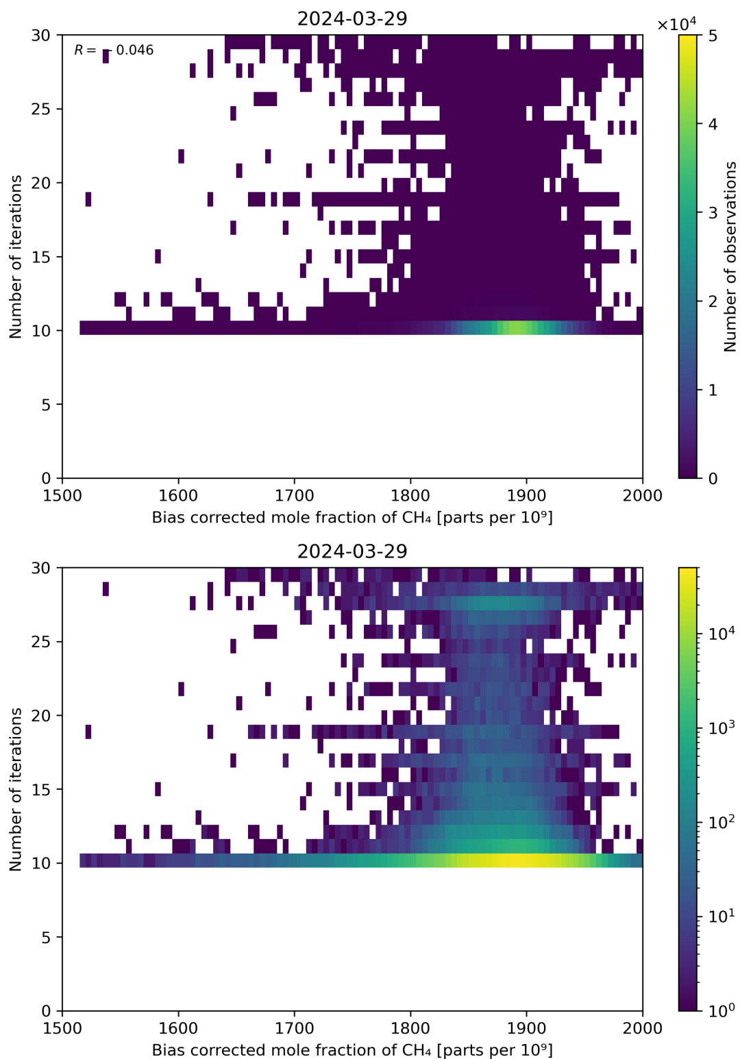
Figure 67: Scatter density plot of “Bias corrected mole fraction of \text{CH}_4 ” against “Number of iterations” for 2024-03-28 to 2024-03-30.
