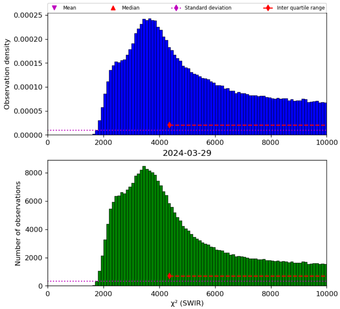
Figure 28: Histogram of “ \chi^2 (SWIR)” for 2024-03-28 to 2024-03-30
