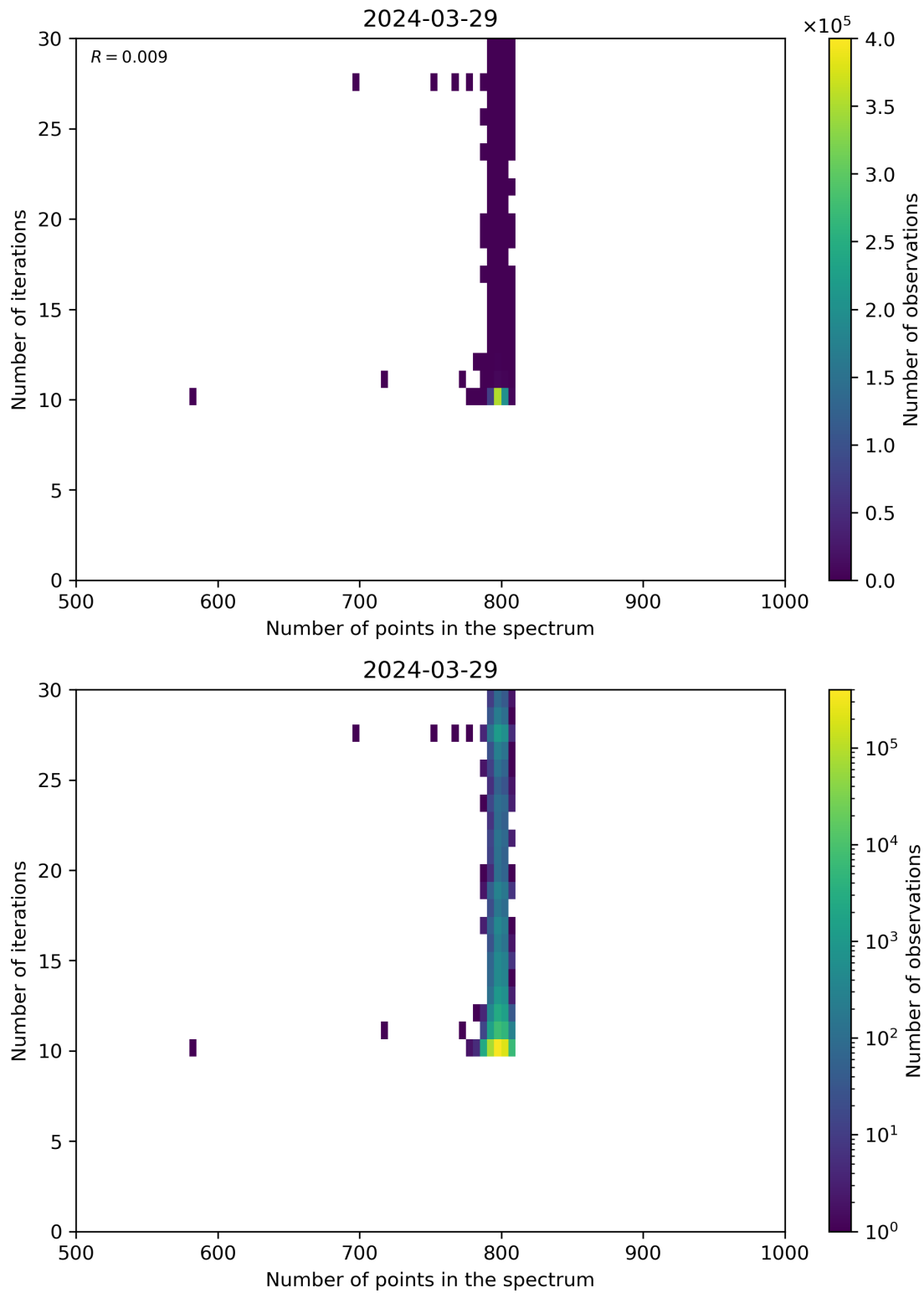
Figure 92: Scatter density plot of “Number of points in the spectrum” against “Number of iterations” for 2024-03-28 to 2024-03-30.
