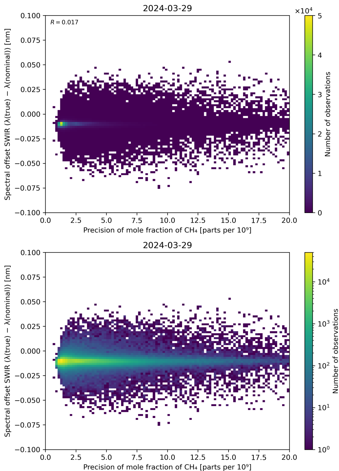
Figure 85: Scatter density plot of “Precision of mole fraction of CH 4 ” against “Spectral offset SWIR ( \lambda(\text{true}) - \lambda(\text{nominal}) )” for 2024-03-28 to 2024-03-30.
