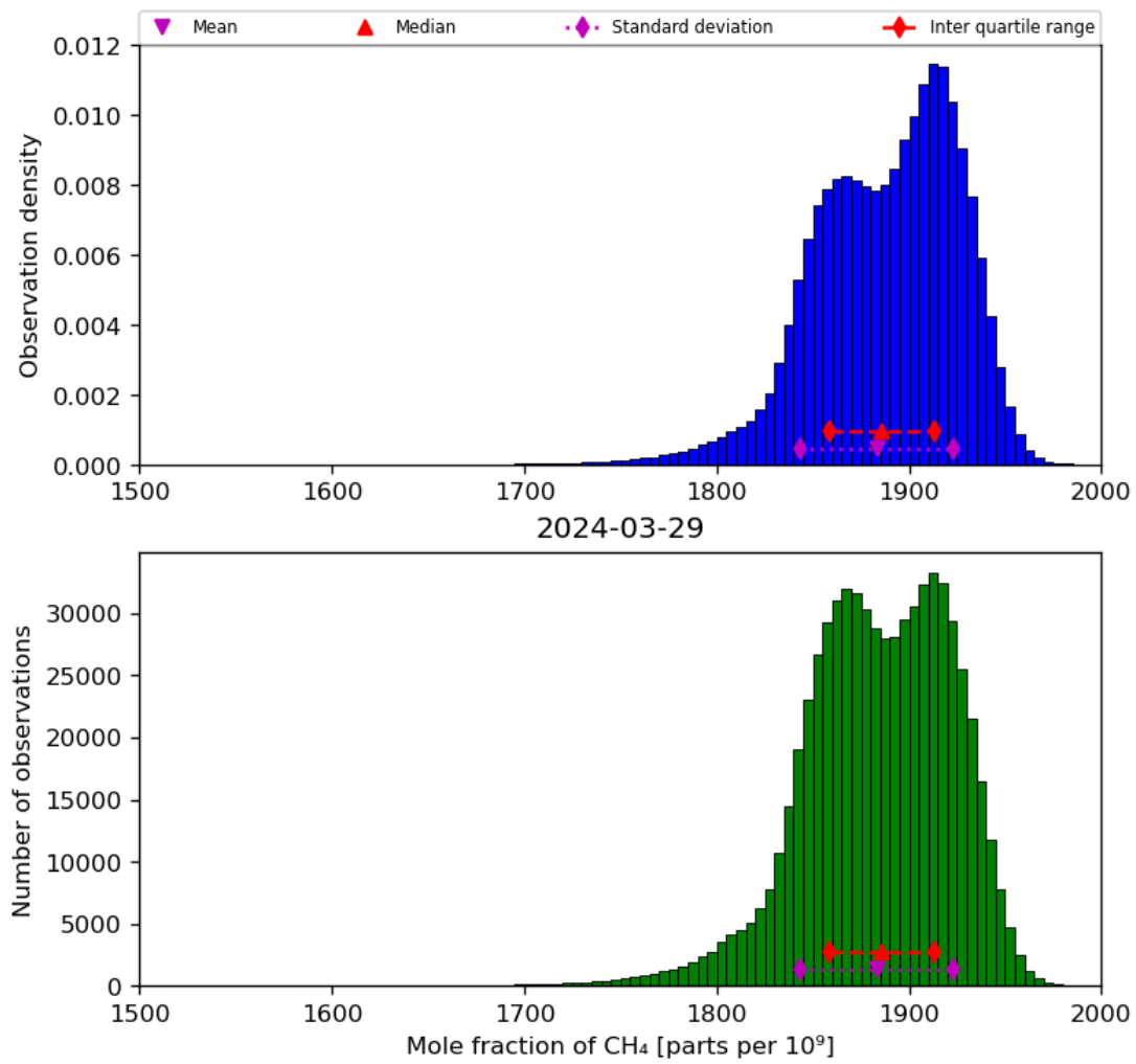
Figure 23: Histogram of “Mole fraction of CH 4 ” for 2024-03-28 to 2024-03-30
