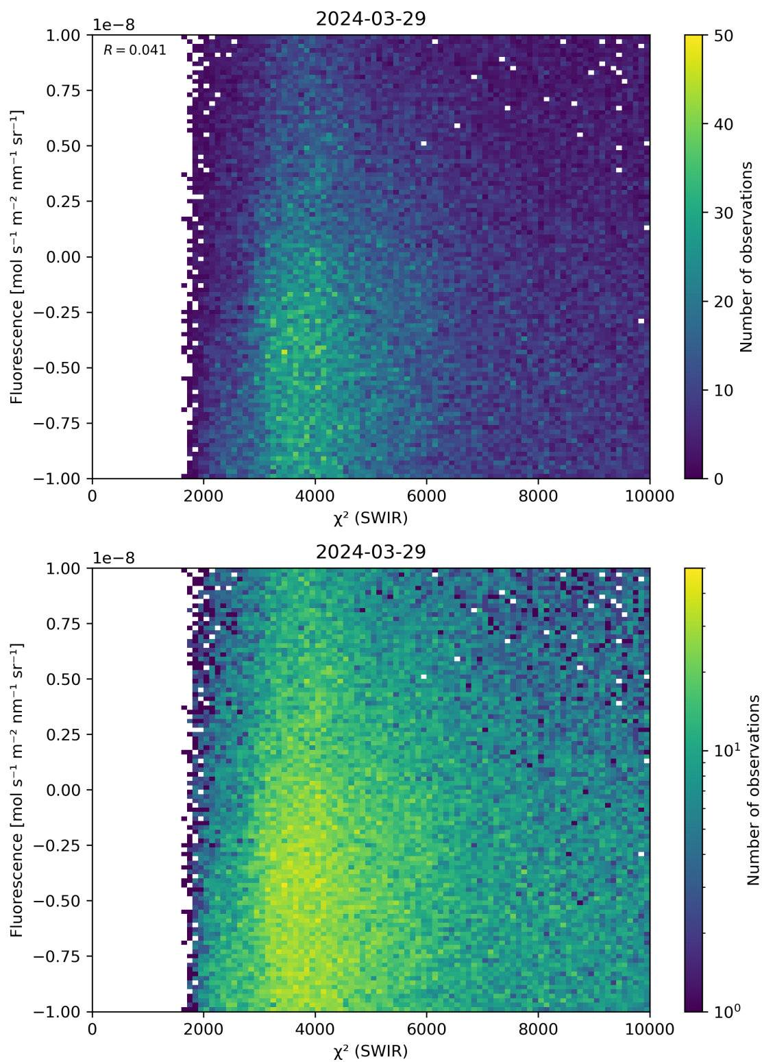
Figure 49: Scatter density plot of “ \chi^2 (SWIR)” against “Fluorescence” for 2024-03-28 to 2024-03-30.
