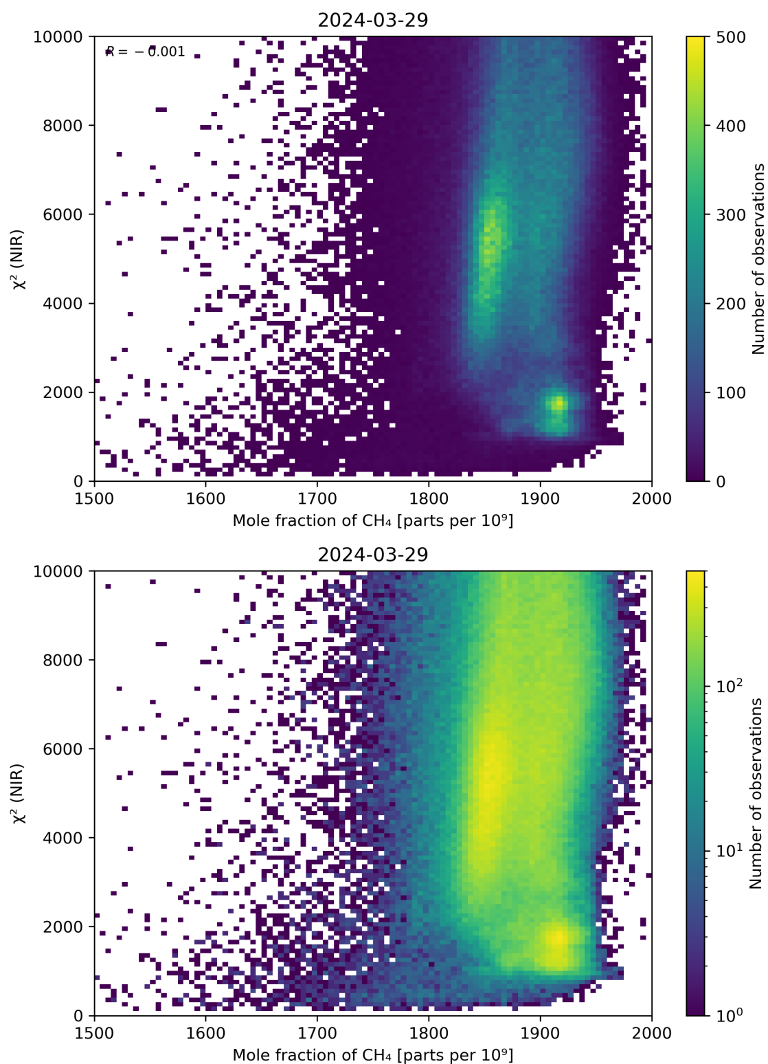
Figure 70: Scatter density plot of “Mole fraction of CH 4 ” against “ \chi^2 (NIR)” for 2024-03-28 to 2024-03-30.
