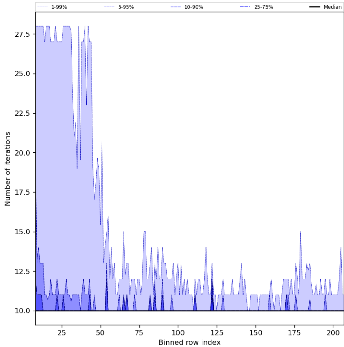
Figure 42: Along track statistics of “Number of iterations” for 2024-03-28 to 2024-03-30
