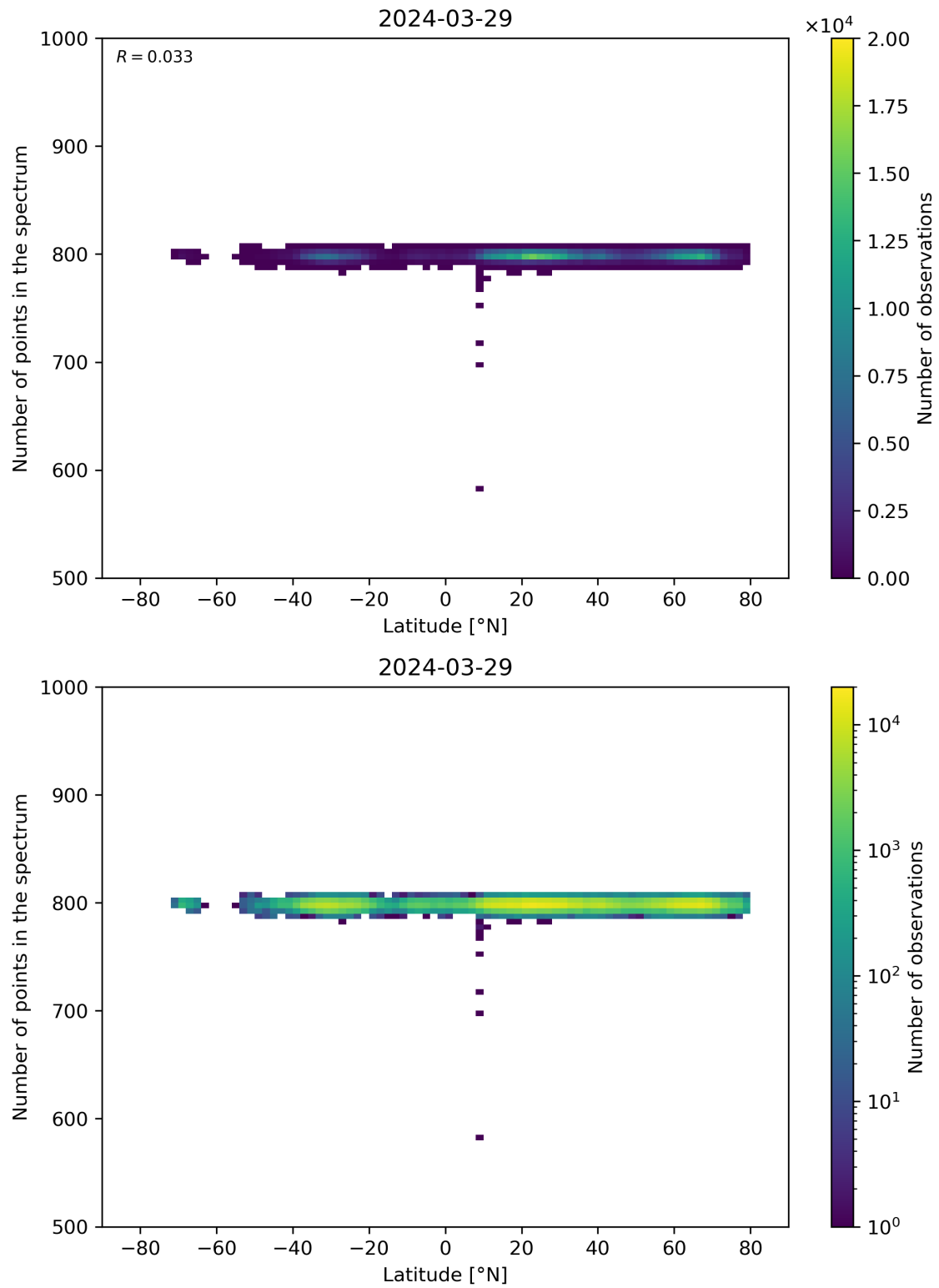
Figure 61: Scatter density plot of “Latitude” against “Number of points in the spectrum” for 2024-03-28 to 2024-03-30.
