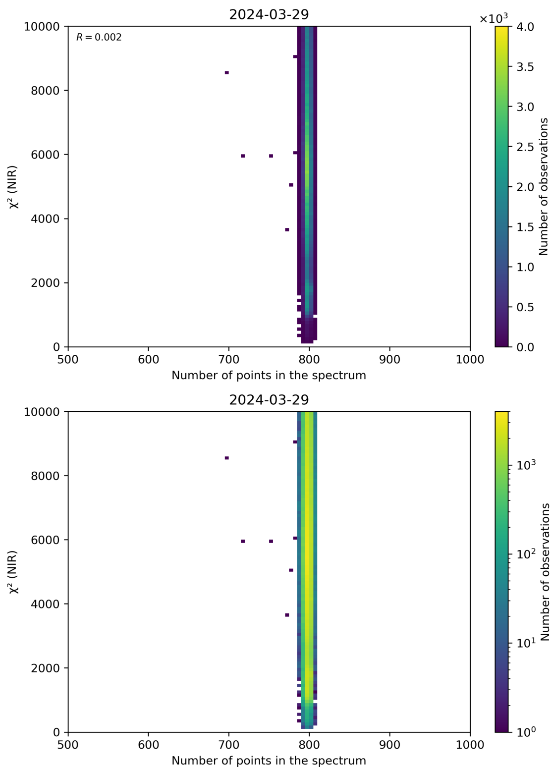
Figure 88: Scatter density plot of “Number of points in the spectrum” against “ \chi^2 (NIR)” for 2024-03-28 to 2024-03-30.
