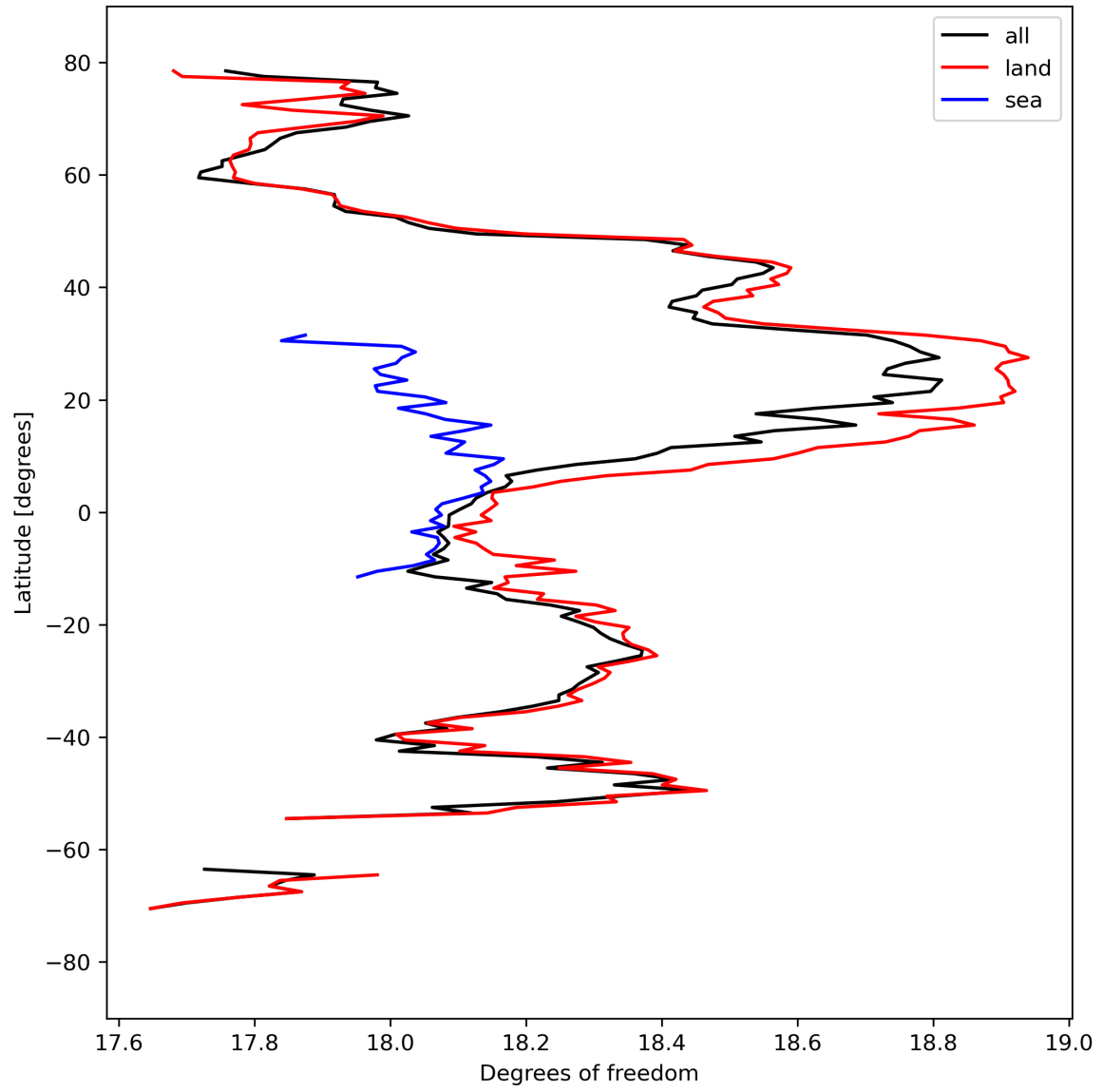
Figure 19: Zonal average of “Degrees of freedom” for 2024-03-28 to 2024-03-30.
