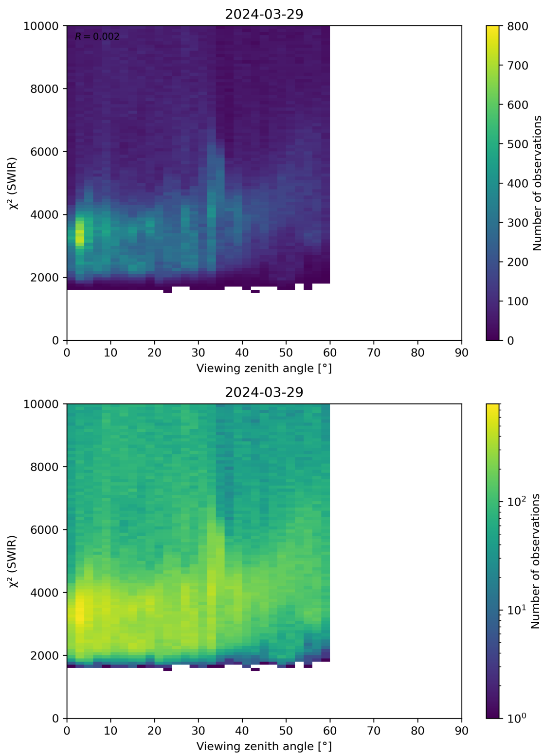
Figure 106: Scatter density plot of “Viewing zenith angle” against “ \chi^2 (SWIR)” for 2024-03-28 to 2024-03-30.
