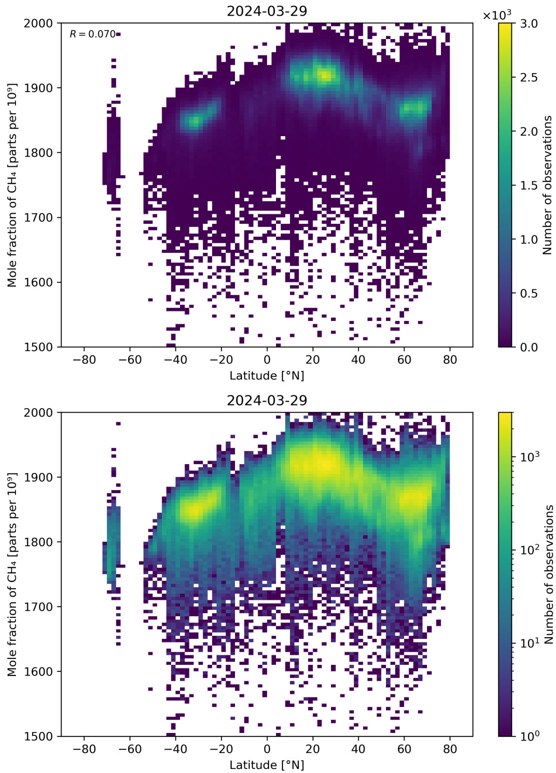
Figure 57: Scatter density plot of “Latitude” against “Mole fraction of \text{CH}_4 ” for 2024-03-28 to 2024-03-30.
