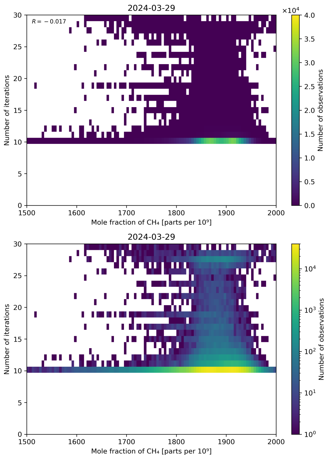
Figure 76: Scatter density plot of “Mole fraction of CH 4 ” against “Number of iterations” for 2024-03-28 to 2024-03-30.
