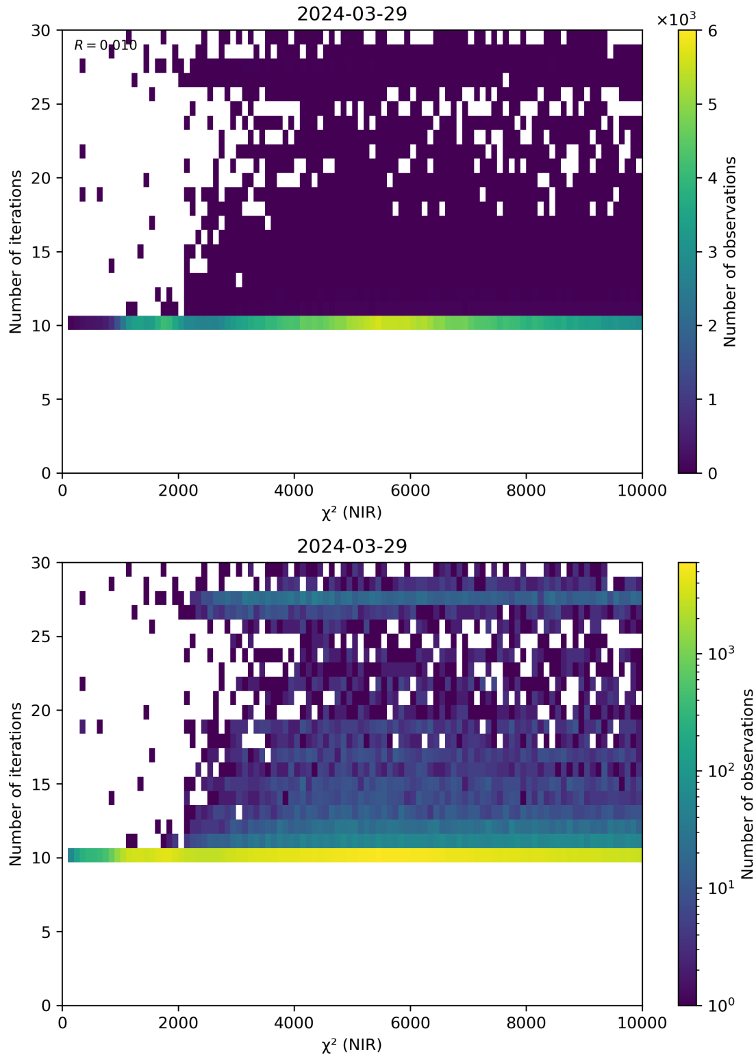
Figure 46: Scatter density plot of “ \chi^2 (NIR)” against “Number of iterations” for 2024-03-28 to 2024-03-30.
