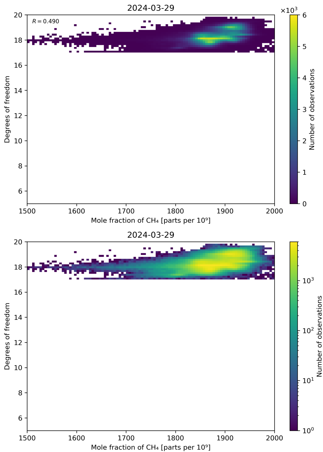
Figure 72: Scatter density plot of “Mole fraction of CH 4 ” against “Degrees of freedom” for 2024-03-28 to 2024-03-30.
