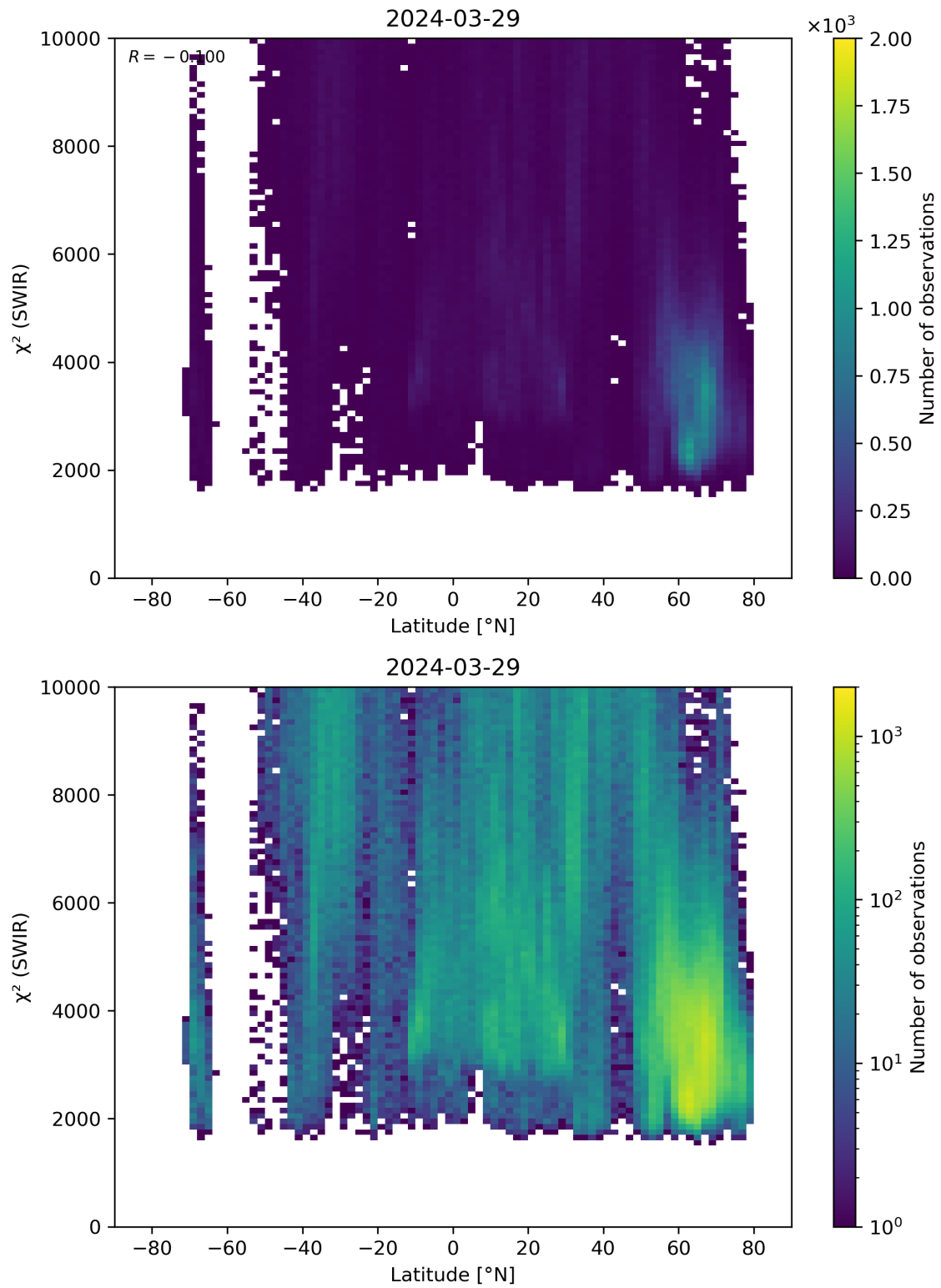
Figure 54: Scatter density plot of “Latitude” against “ \chi^2 (SWIR)” for 2024-03-28 to 2024-03-30.
