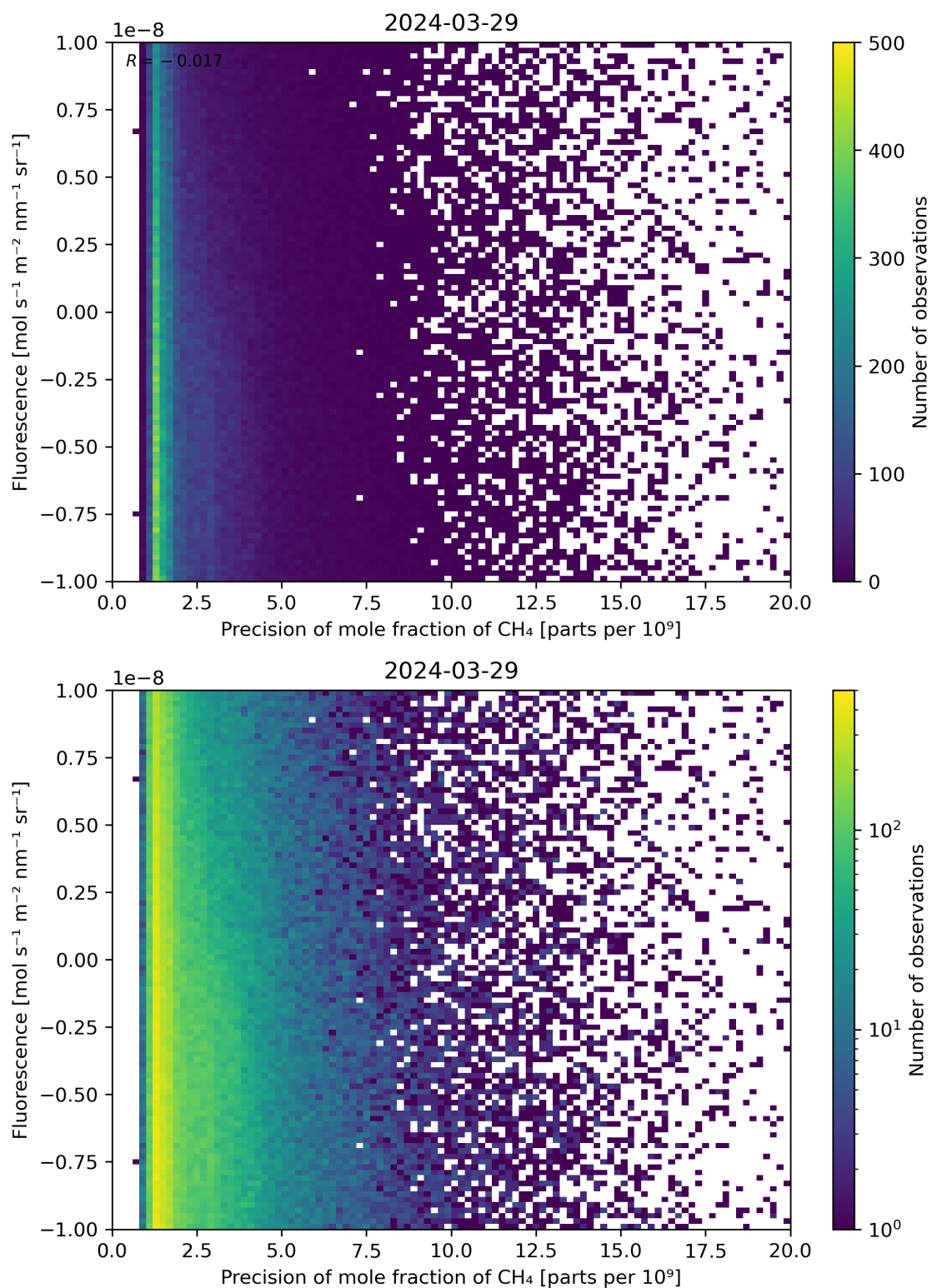
Figure 81: Scatter density plot of “Precision of mole fraction of \text{CH}_4 ” against “Fluorescence” for 2024-03-28 to 2024-03-30.
