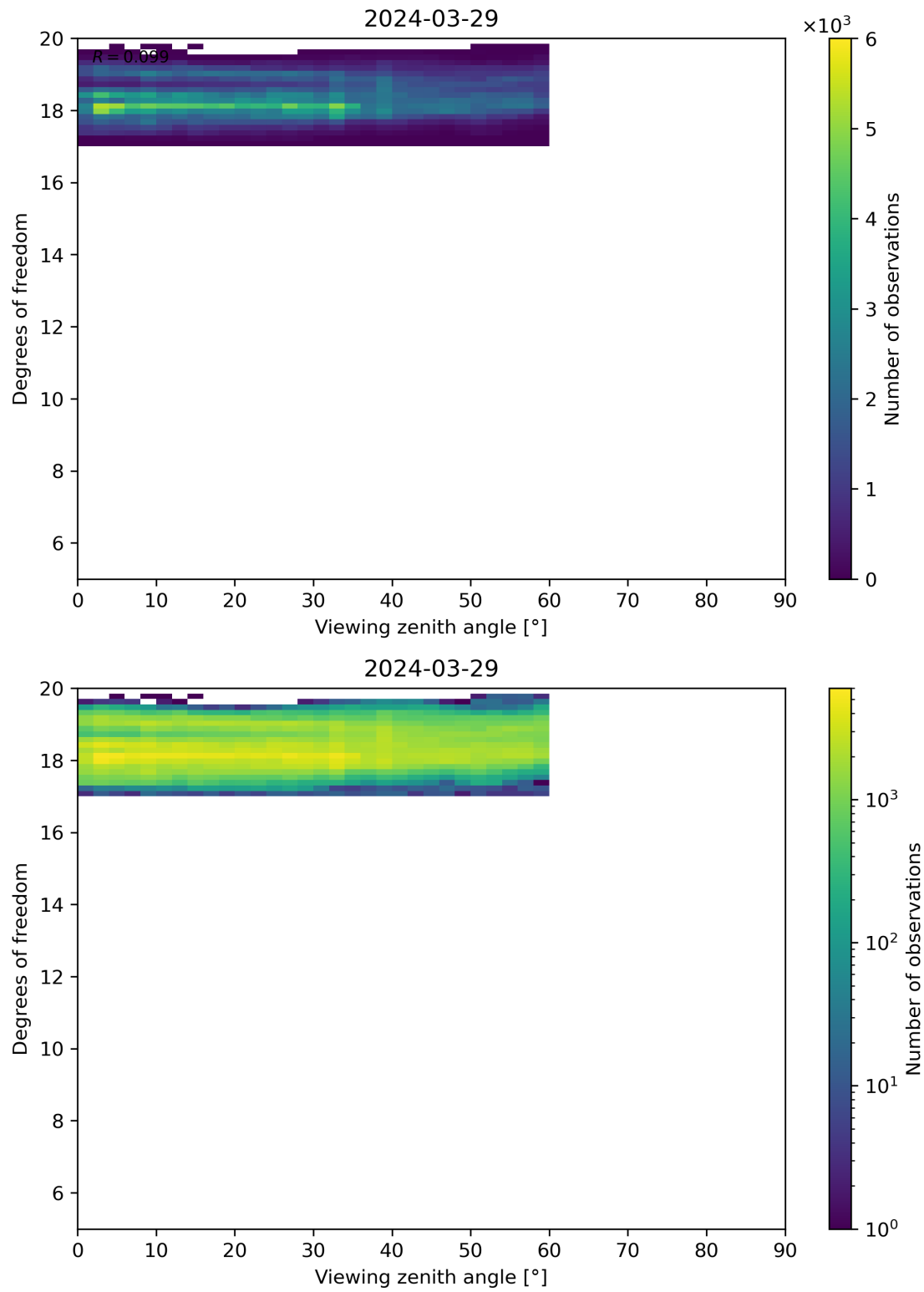
Figure 107: Scatter density plot of “Viewing zenith angle” against “Degrees of freedom” for 2024-03-28 to 2024-03-30.
