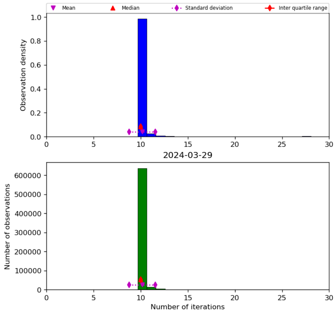
Figure 31: Histogram of “Number of iterations” for 2024-03-28 to 2024-03-30
