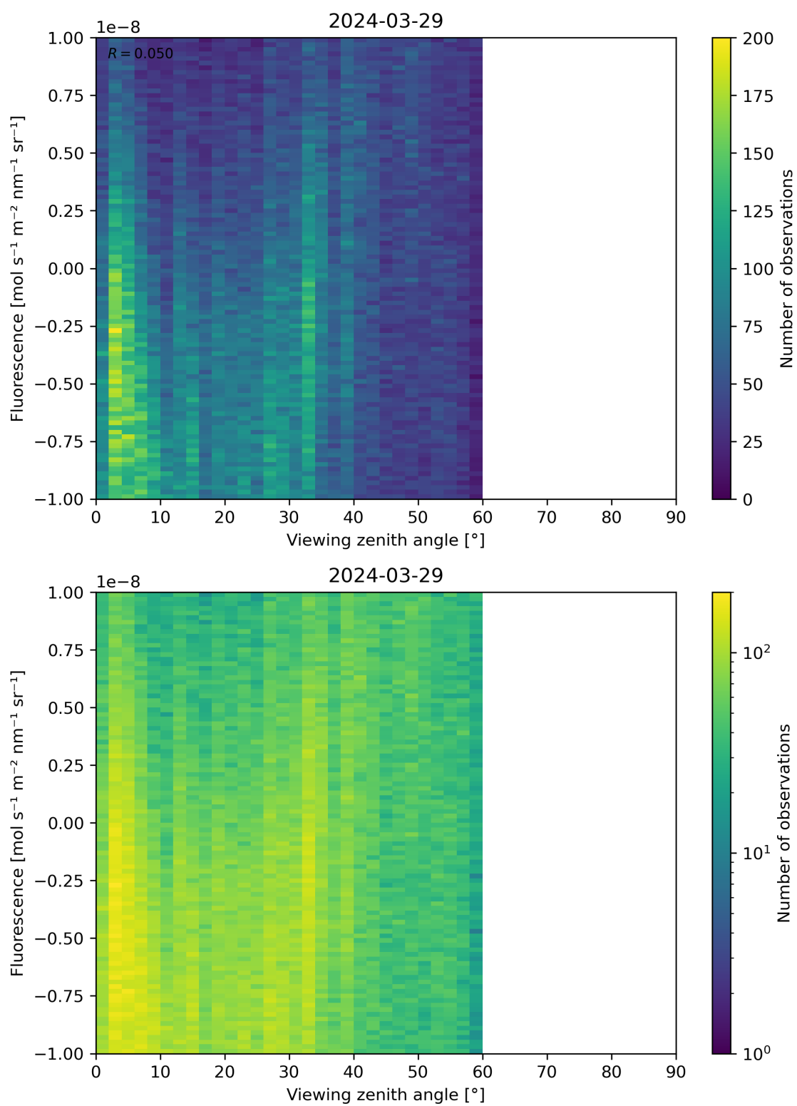
Figure 108: Scatter density plot of “Viewing zenith angle” against “Fluorescence” for 2024-03-28 to 2024-03-30.
