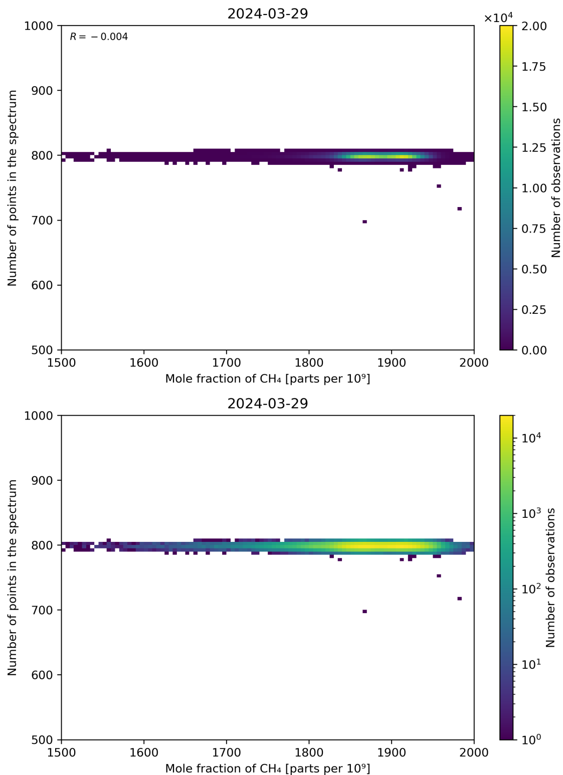
Figure 77: Scatter density plot of “Mole fraction of CH 4 ” against “Number of points in the spectrum” for 2024-03-28 to 2024-03-30.
