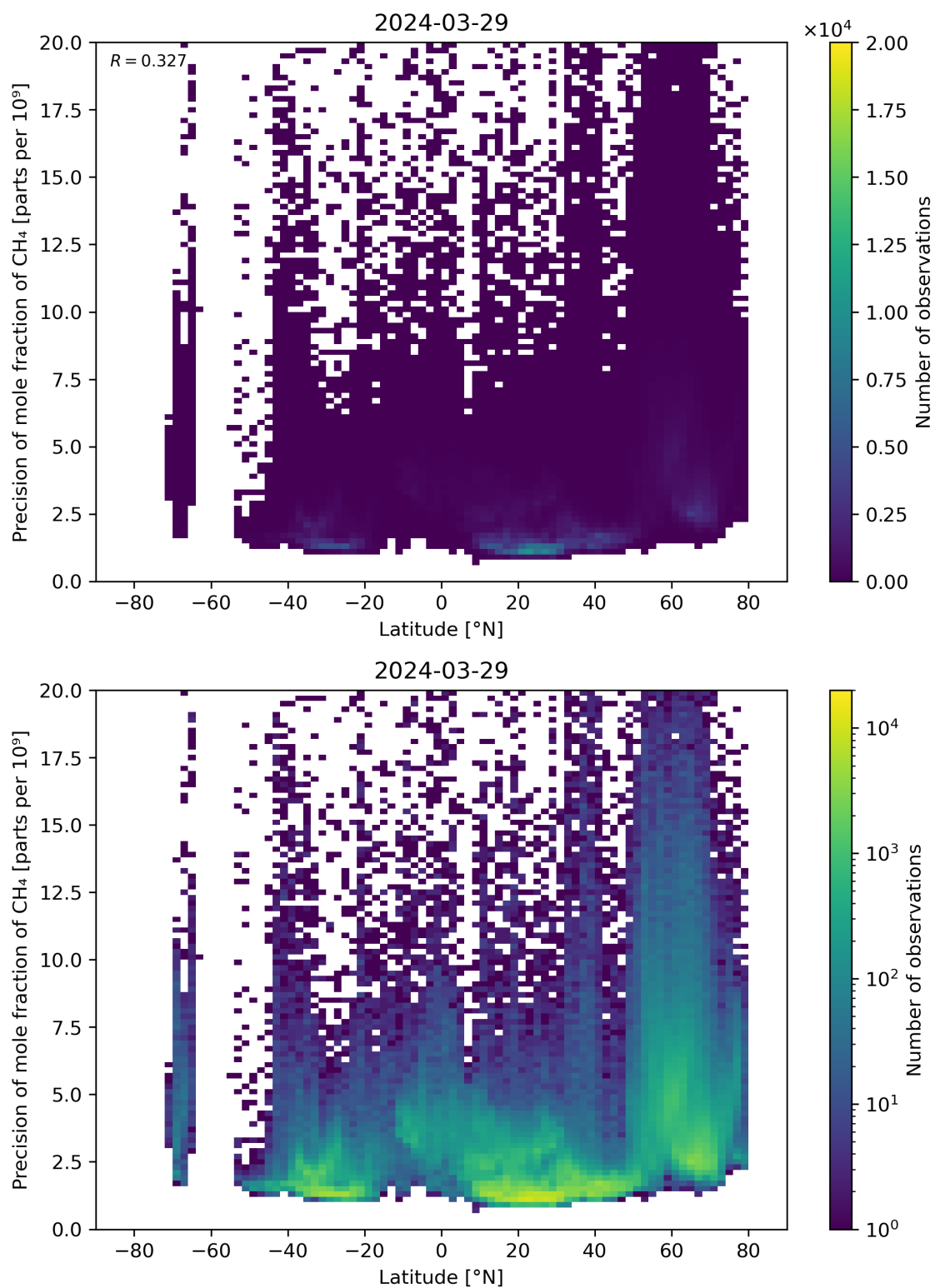
Figure 59: Scatter density plot of “Latitude” against “Precision of mole fraction of \text{CH}_4 ” for 2024-03-28 to 2024-03-30.
