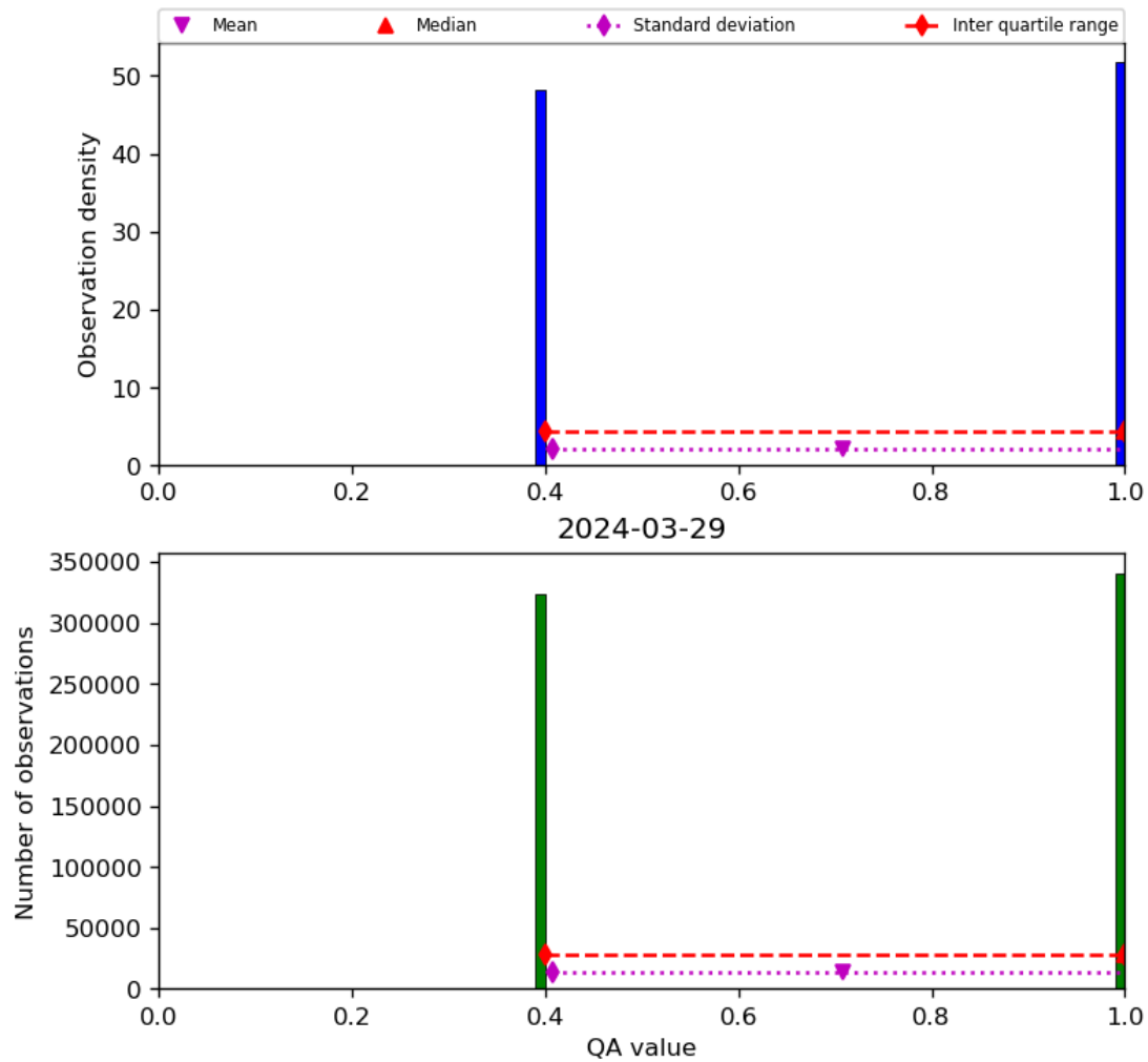
Figure 22: Histogram of “QA value” for 2024-03-28 to 2024-03-30
