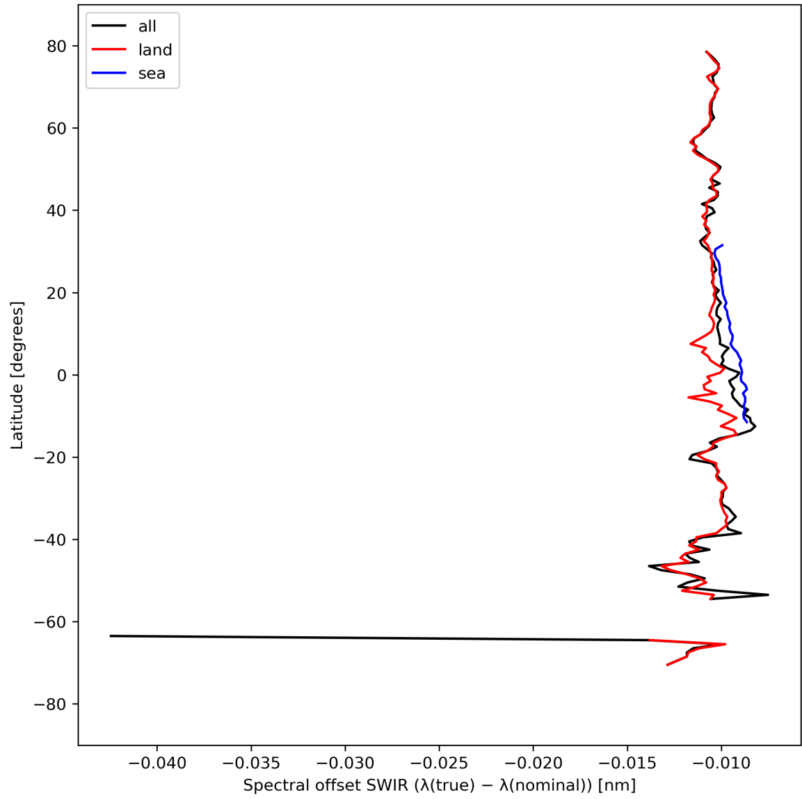
Figure 16: Zonal average of “Spectral offset SWIR ( \lambda(\text{true}) - \lambda(\text{nominal}) )” for 2024-03-28 to 2024-03-30.
