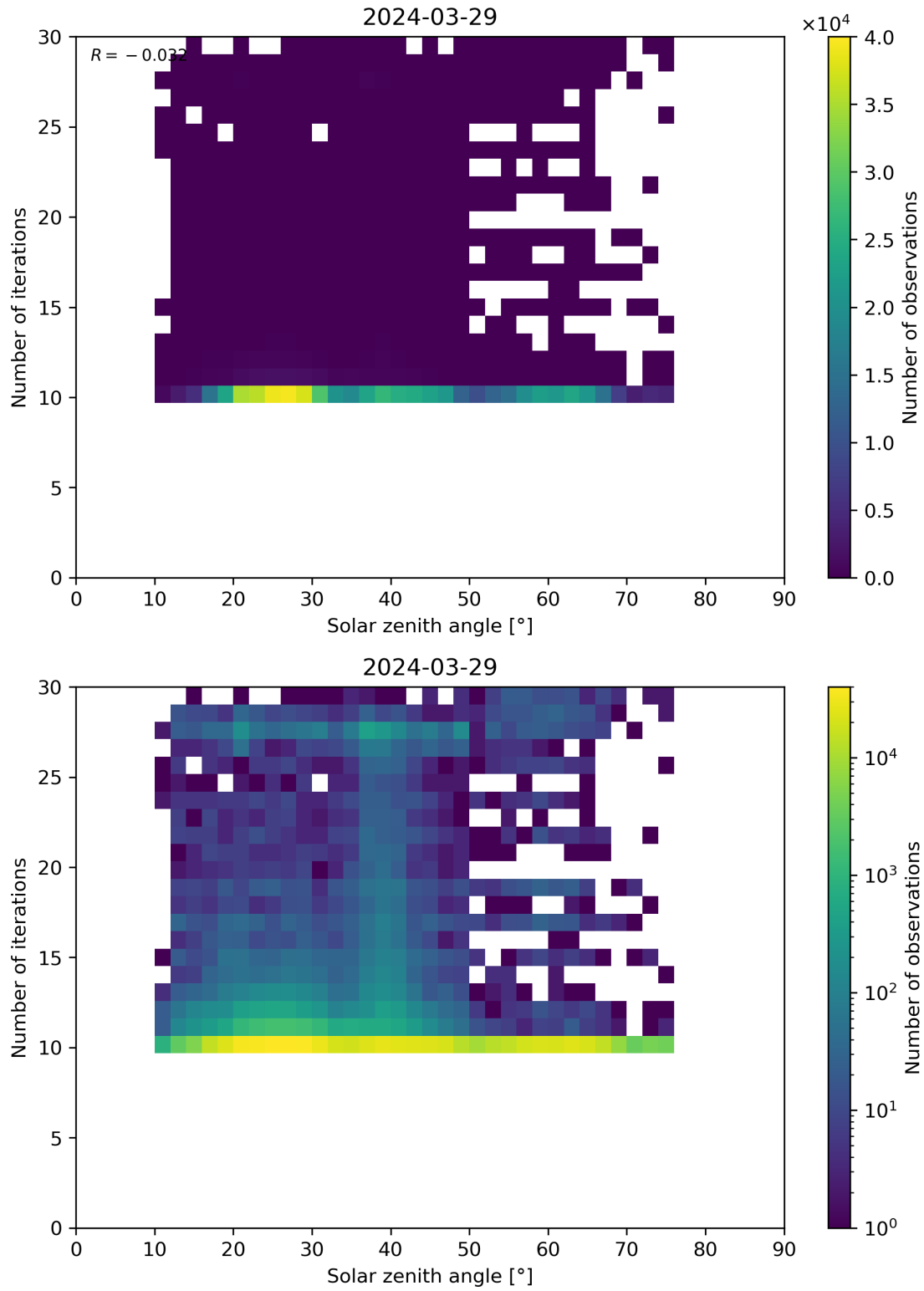
Figure 102: Scatter density plot of “Solar zenith angle” against “Number of iterations” for 2024-03-28 to 2024-03-30.
