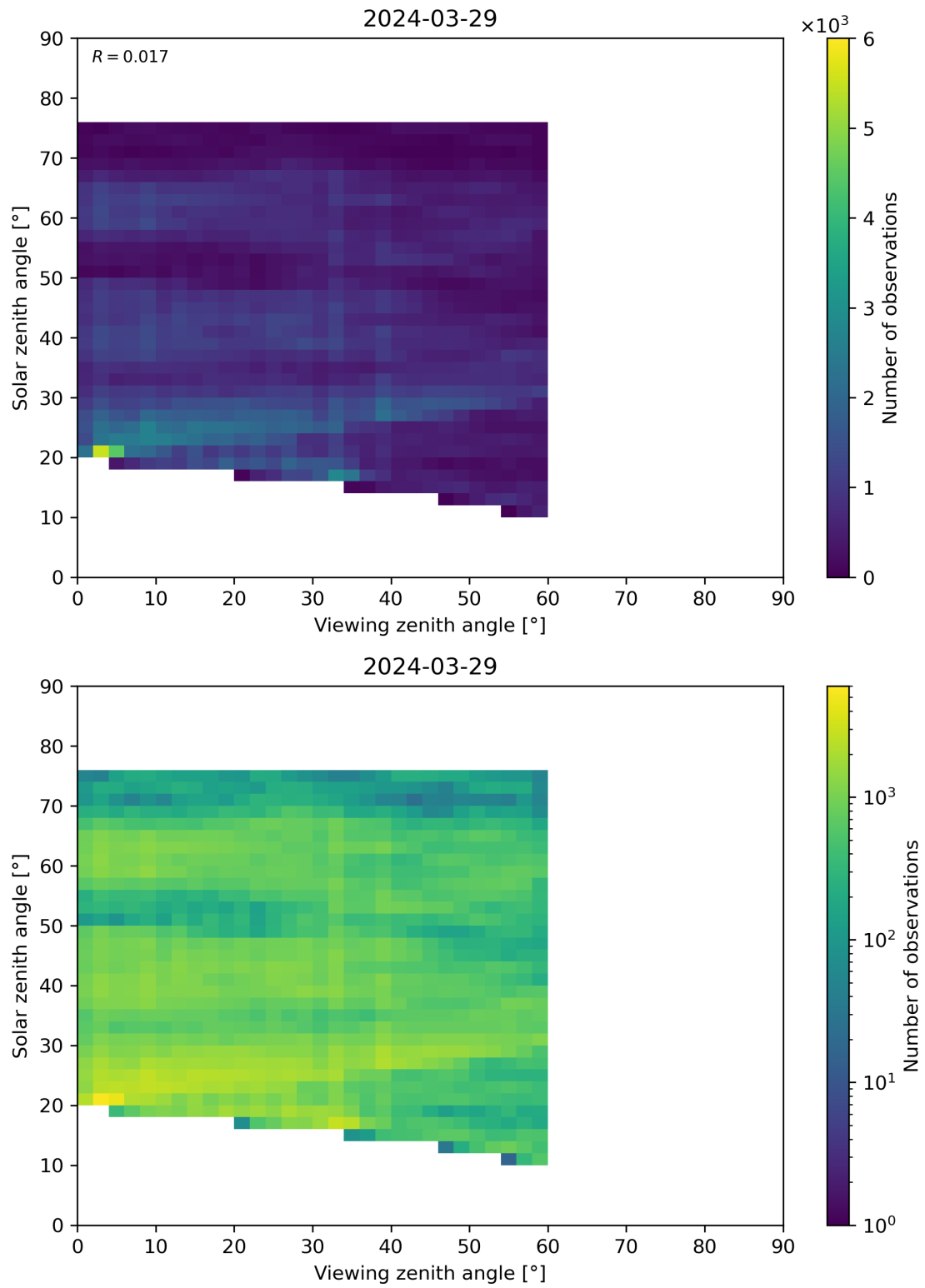
Figure 115: Scatter density plot of “Viewing zenith angle” against “Solar zenith angle” for 2024-03-28 to 2024-03-30.
