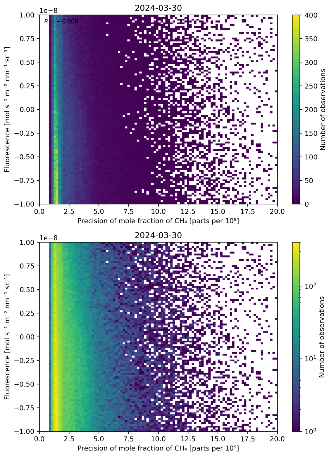
Figure 81: Scatter density plot of “Precision of mole fraction of \text{CH}_4 ” against “Fluorescence” for 2024-03-30 to 2024-03-31.
