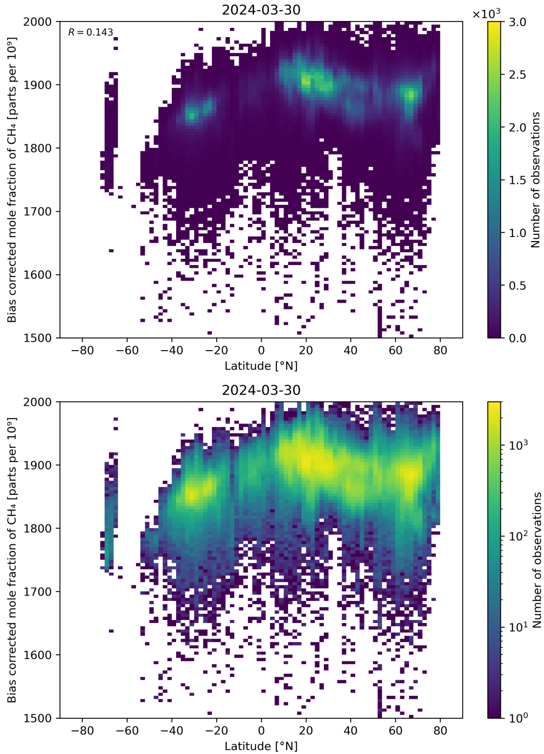
Figure 58: Scatter density plot of “Latitude” against “Bias corrected mole fraction of CH 4 ” for 2024-03-30 to 2024-03-31.
