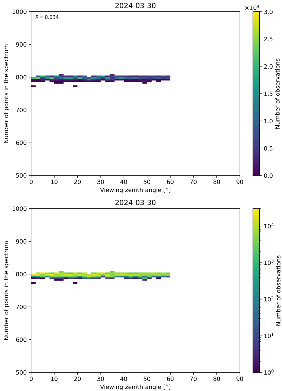
Figure 114: Scatter density plot of “Viewing zenith angle” against “Number of points in the spectrum” for 2024-03-30 to 2024-03-31.
