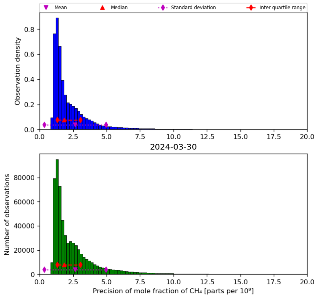
Figure 24: Histogram of “Precision of mole fraction of CH 4 ” for 2024-03-30 to 2024-03-31
