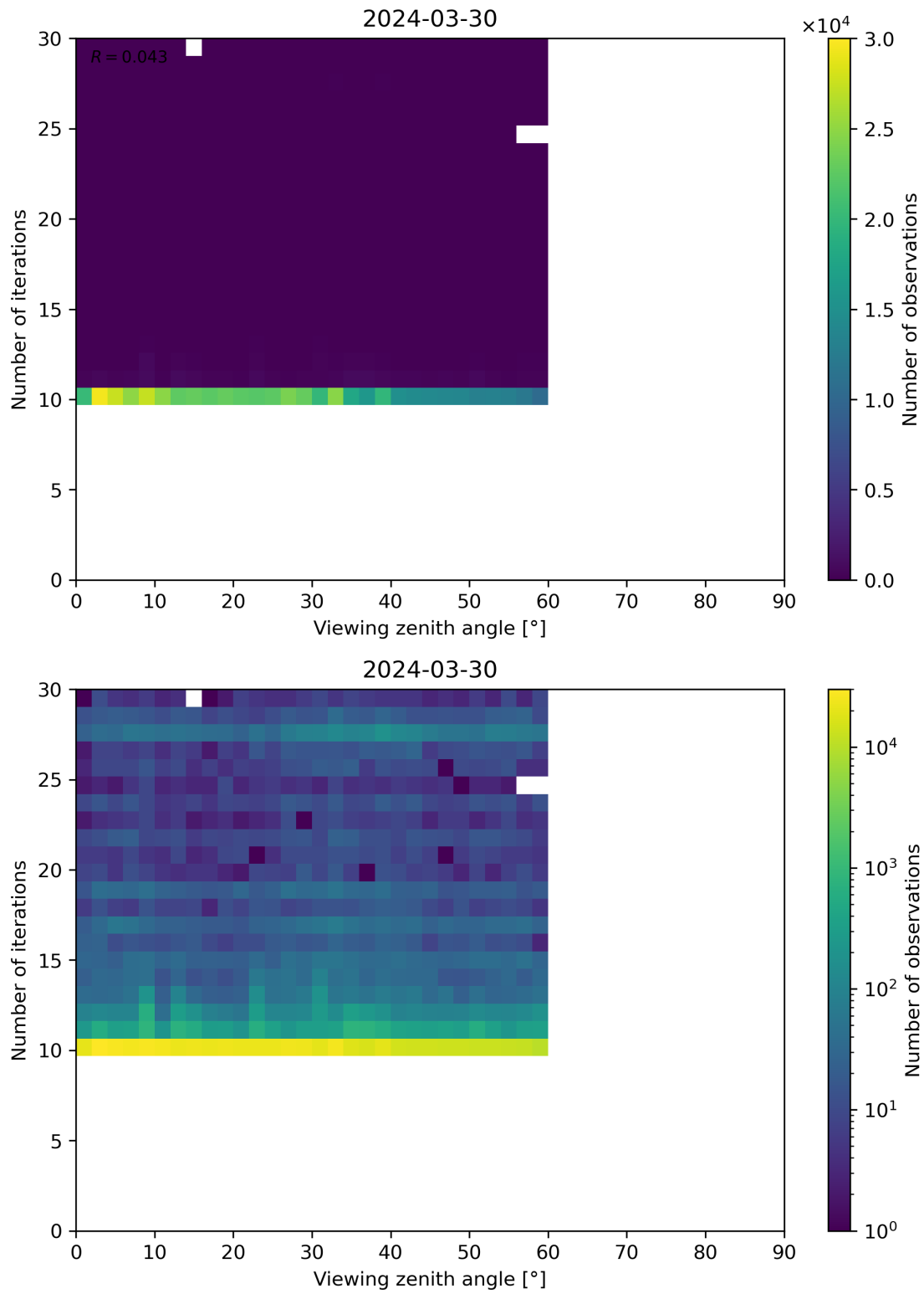
Figure 113: Scatter density plot of “Viewing zenith angle” against “Number of iterations” for 2024-03-30 to 2024-03-31.
