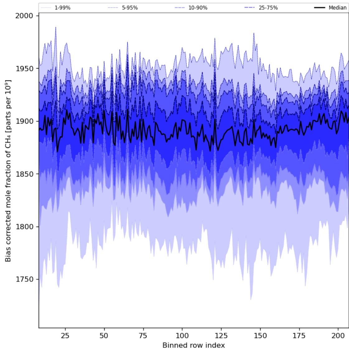
Figure 36: Along track statistics of “Bias corrected mole fraction of CH 4 ” for 2024-03-30 to 2024-03-31
