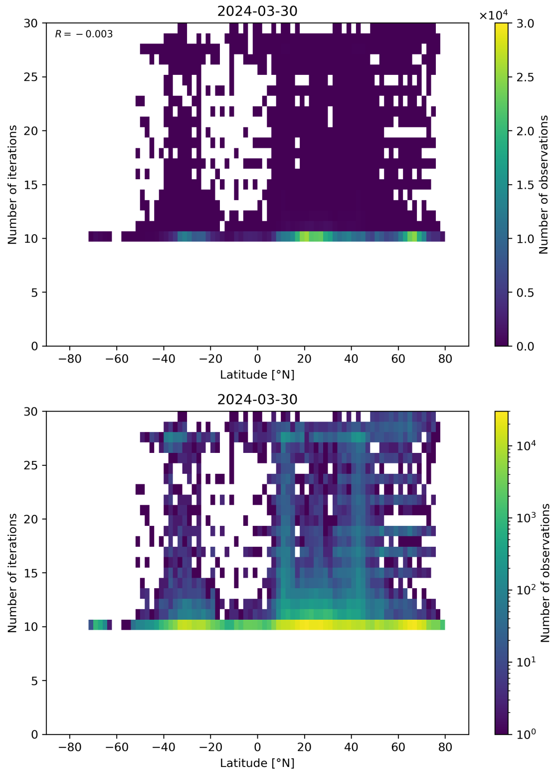
Figure 60: Scatter density plot of “Latitude” against “Number of iterations” for 2024-03-30 to 2024-03-31.
