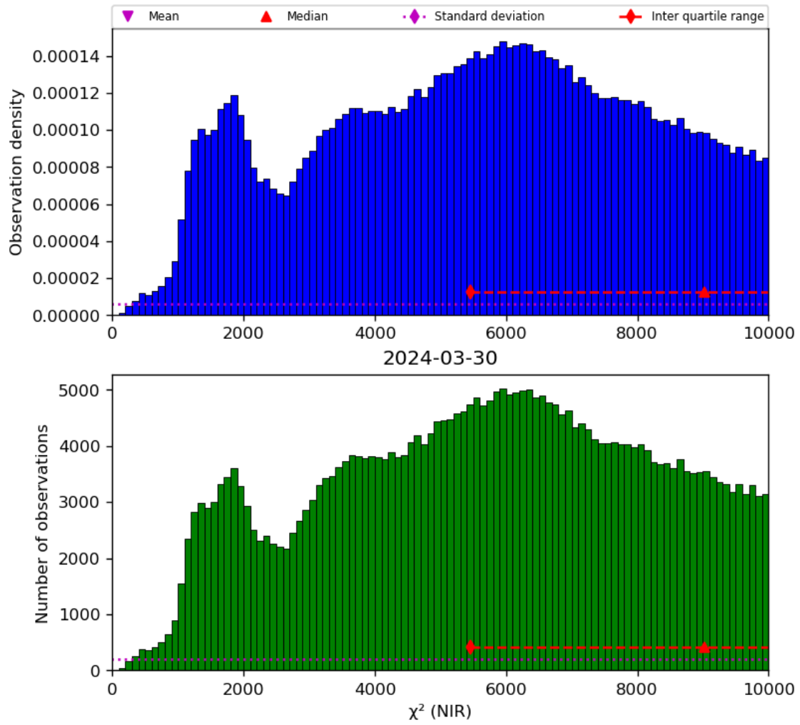
Figure 29: Histogram of " \chi^2 (NIR)" for 2024-03-30 to 2024-03-31
