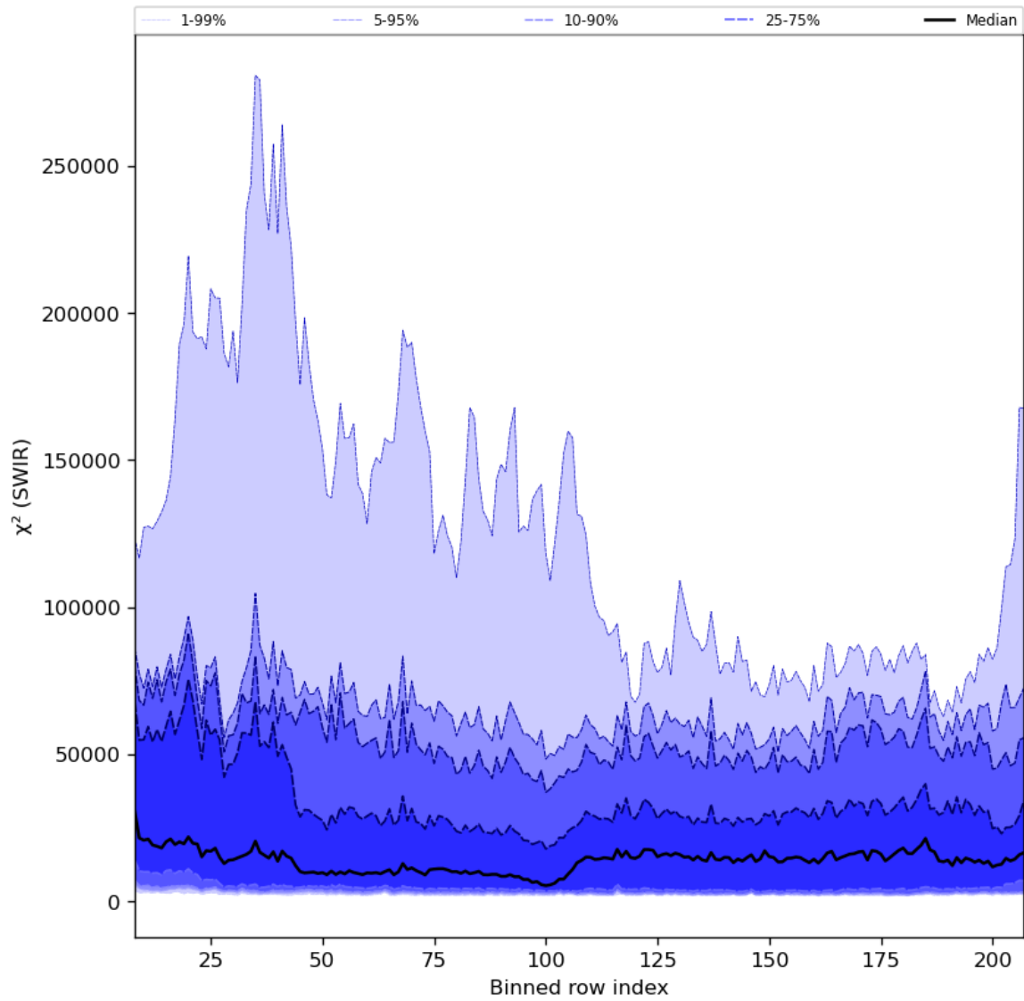
Figure 39: Along track statistics of “ \chi^2 (SWIR)” for 2024-03-30 to 2024-03-31
