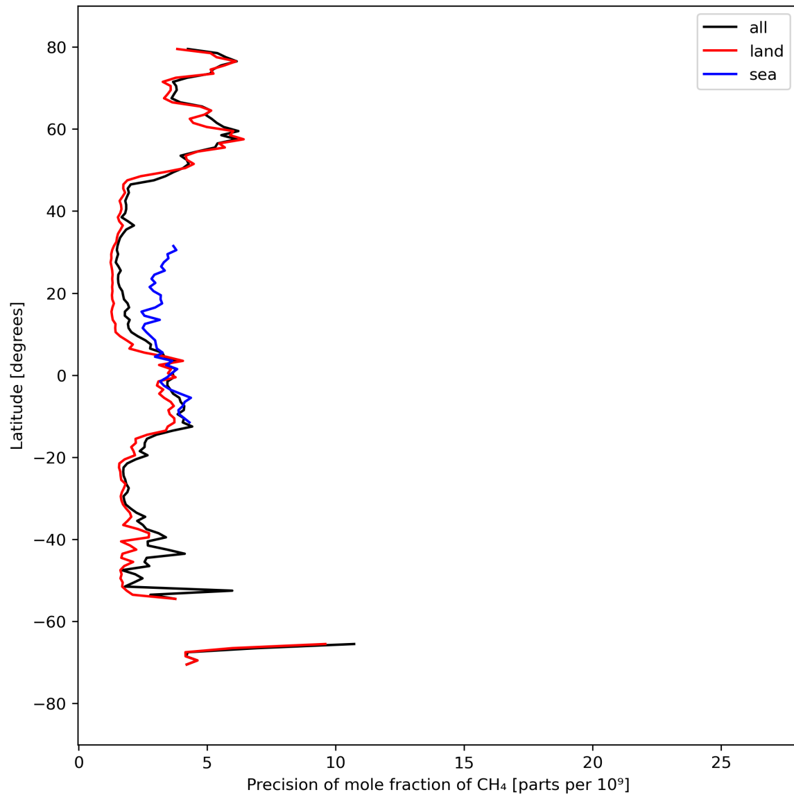
Figure 13: Zonal average of “Precision of mole fraction of CH 4 ” for 2024-03-30 to 2024-03-31.
