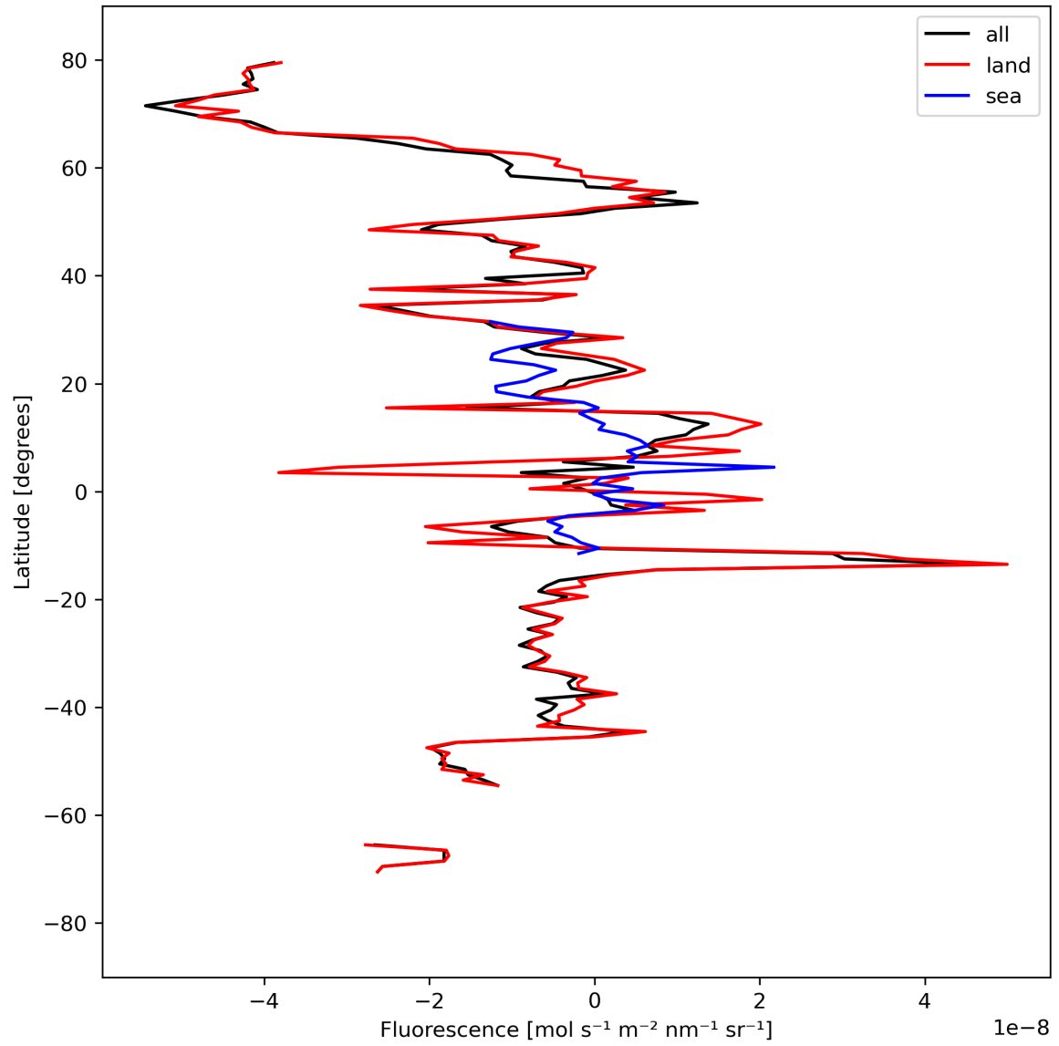
Figure 21: Zonal average of “Fluorescence” for 2024-03-30 to 2024-03-31.
