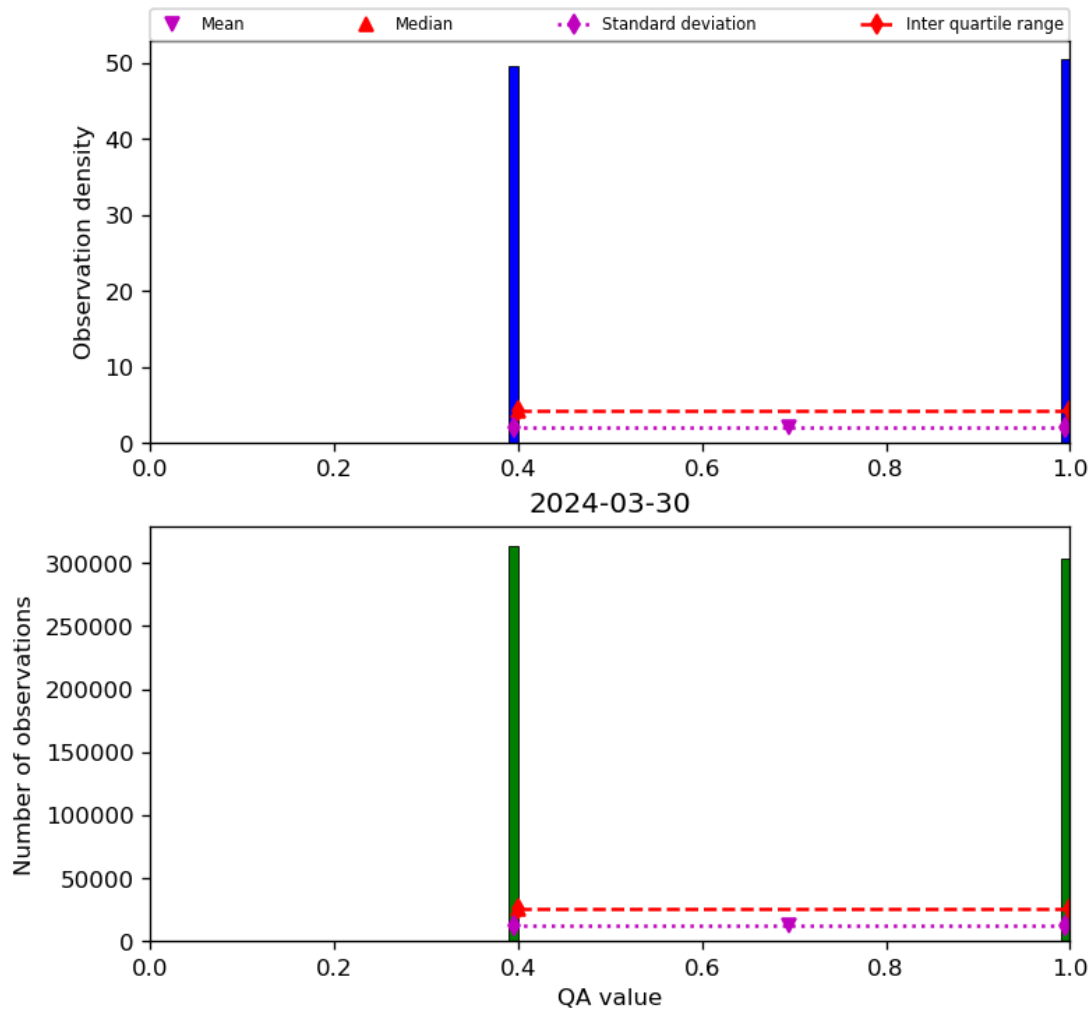
Figure 22: Histogram of “QA value” for 2024-03-30 to 2024-03-31
