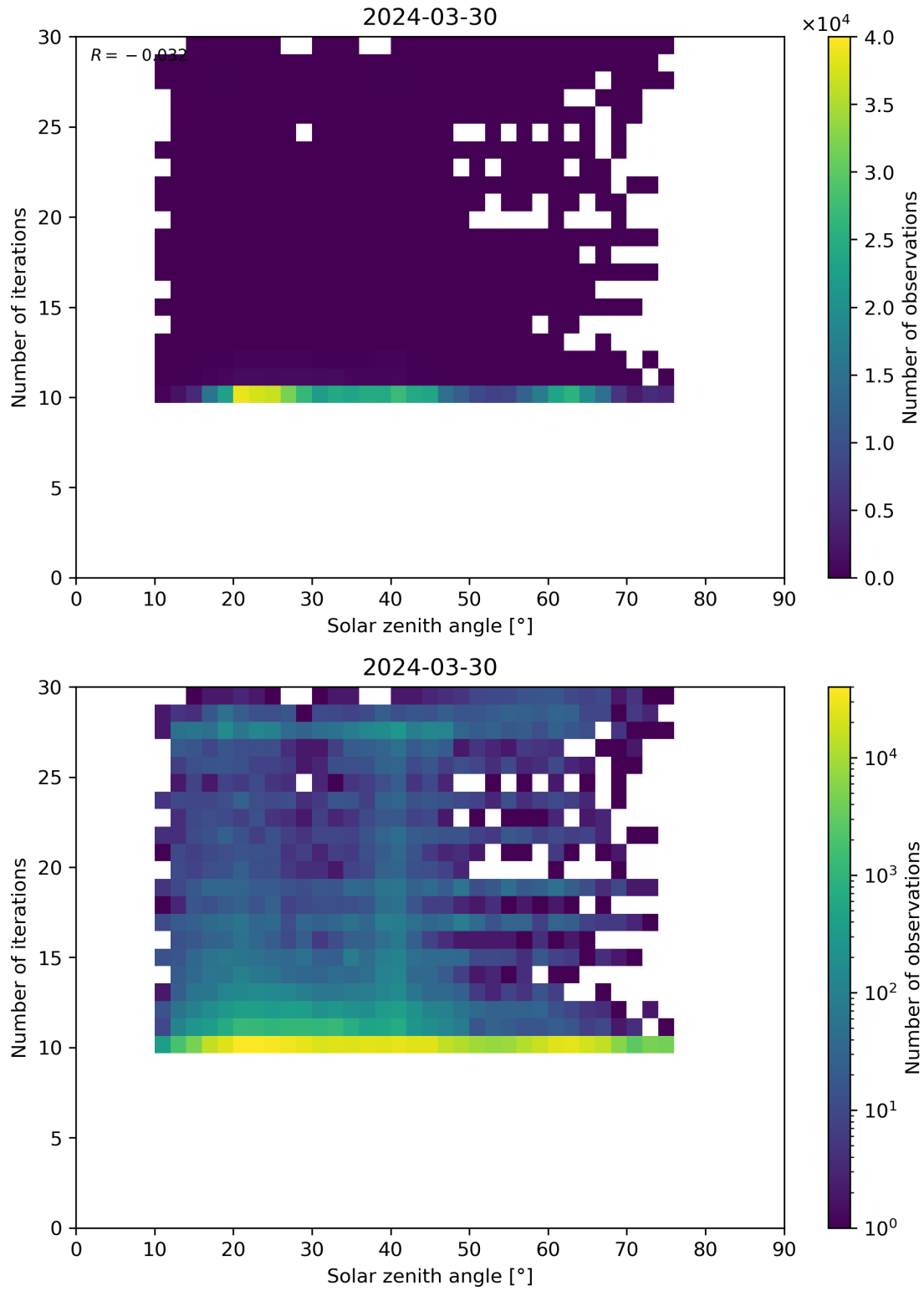
Figure 102: Scatter density plot of “Solar zenith angle” against “Number of iterations” for 2024-03-30 to 2024-03-31.
