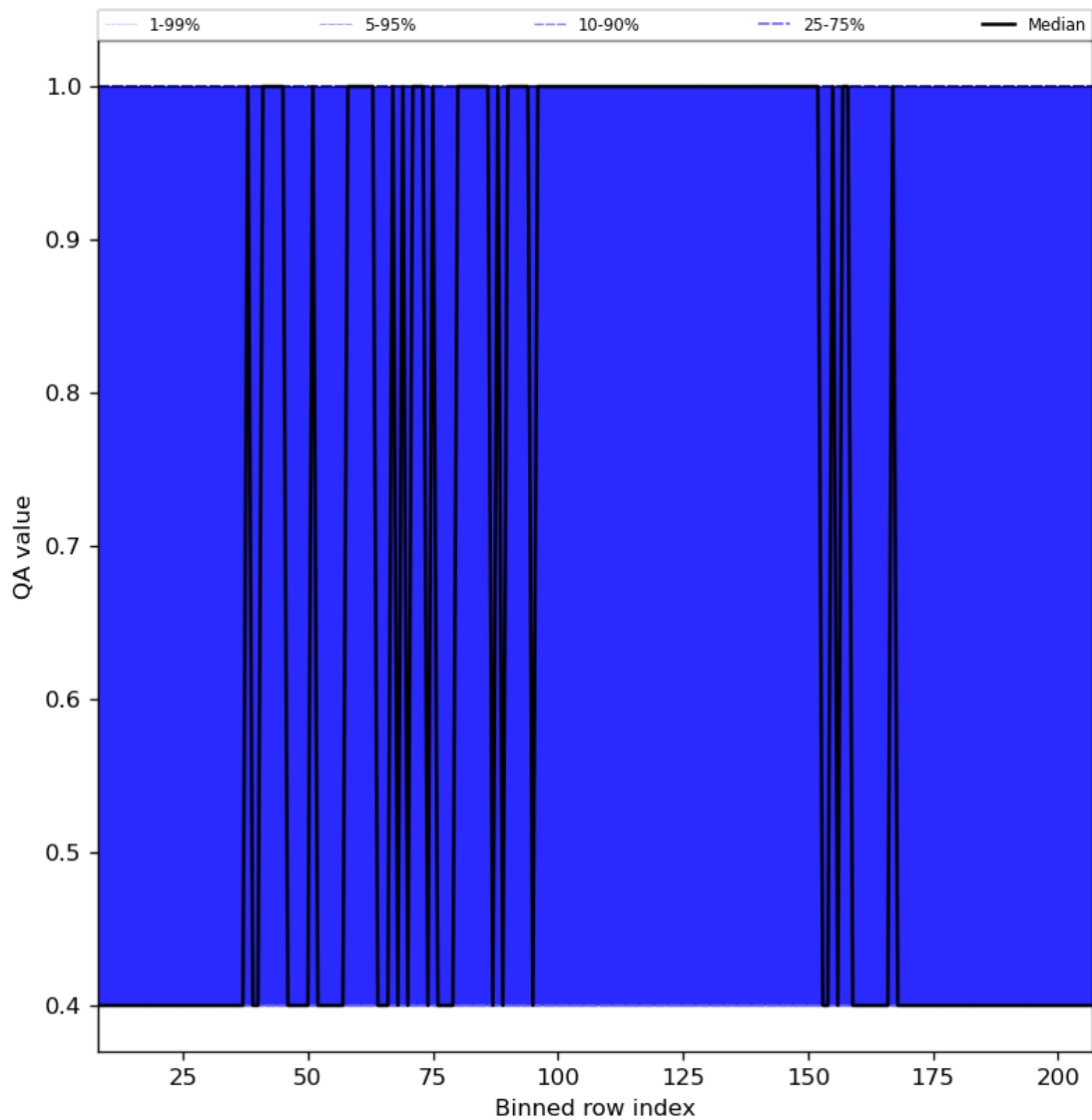
Figure 33: Along track statistics of “QA value” for 2024-03-30 to 2024-03-31
