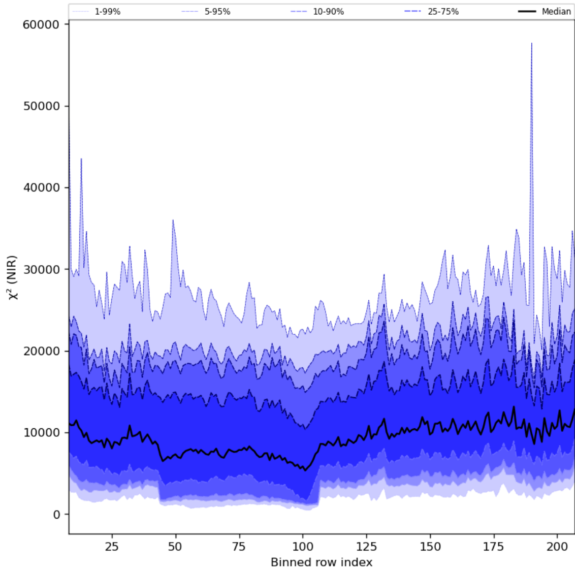
Figure 40: Along track statistics of “ \chi^2 (NIR)” for 2024-03-30 to 2024-03-31
