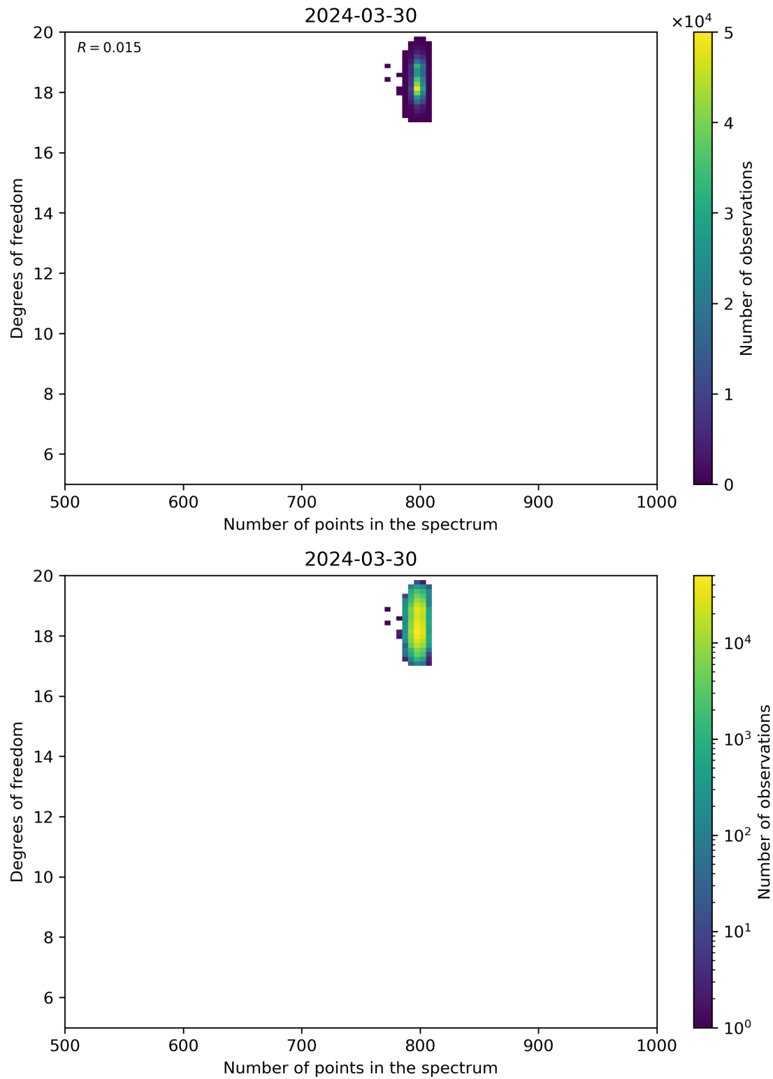
Figure 90: Scatter density plot of “Number of points in the spectrum” against “Degrees of freedom” for 2024-03-30 to 2024-03-31.
