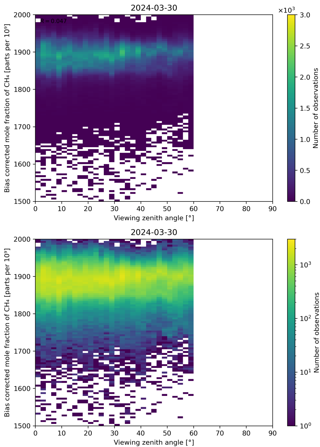
Figure 111: Scatter density plot of “Viewing zenith angle” against “Bias corrected mole fraction of \text{CH}_4 ” for 2024-03-30 to 2024-03-31.
