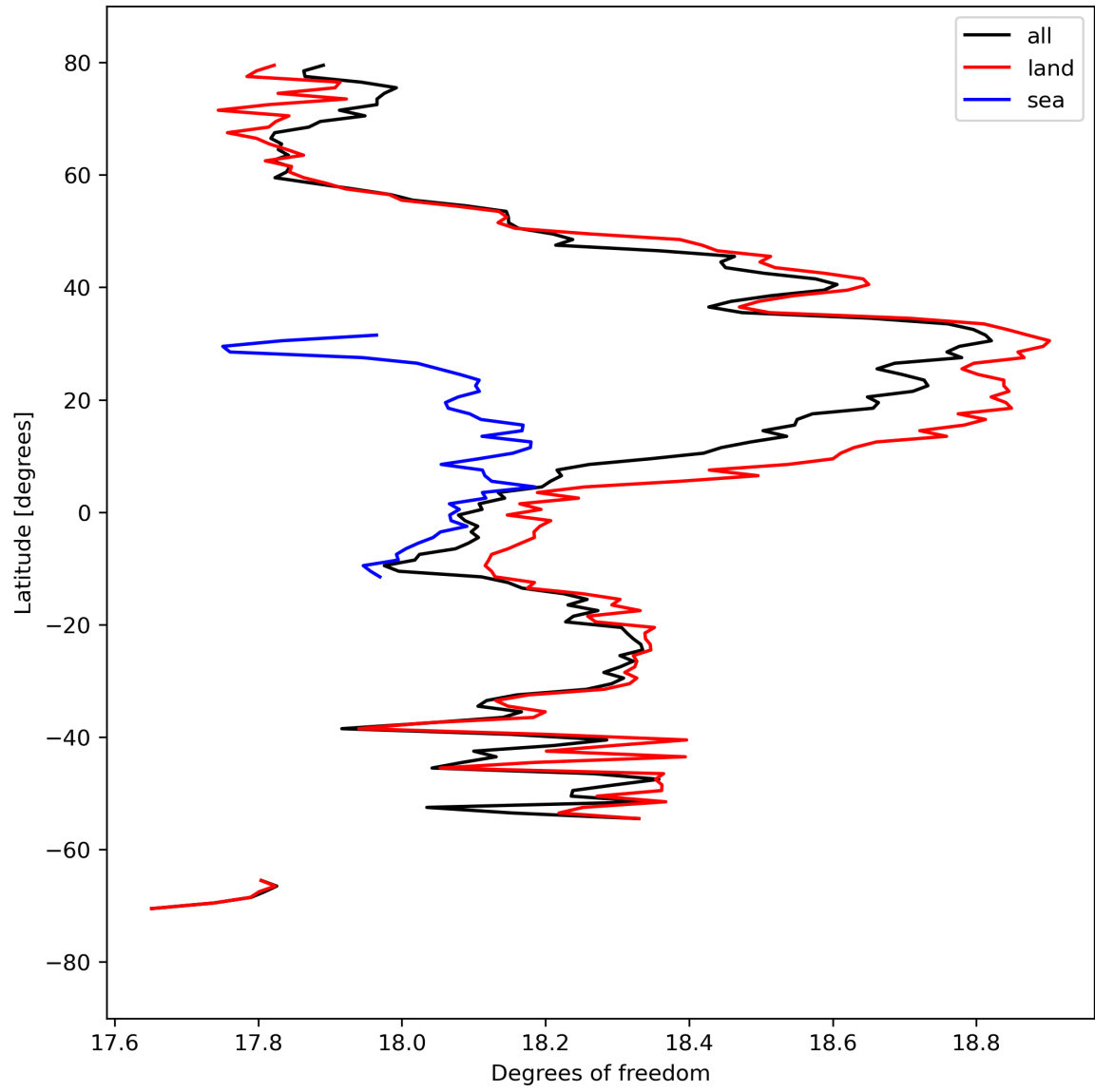
Figure 19: Zonal average of “Degrees of freedom” for 2024-03-30 to 2024-03-31.
