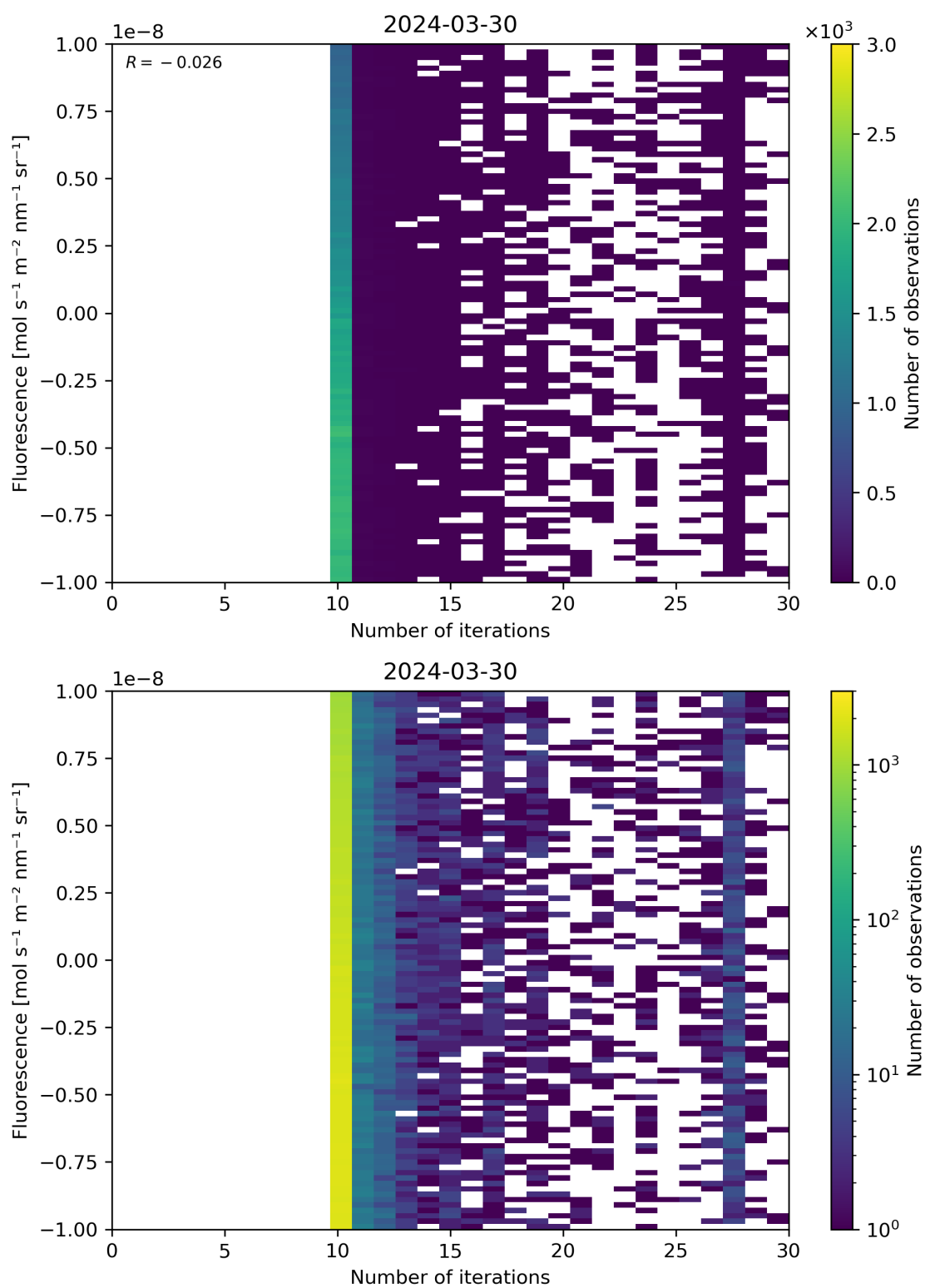
Figure 87: Scatter density plot of “Number of iterations” against “Fluorescence” for 2024-03-30 to 2024-03-31.
