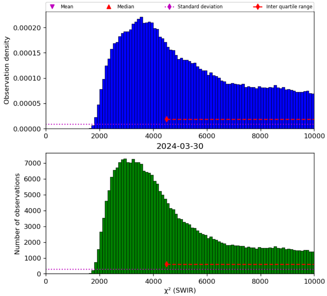
Figure 28: Histogram of “ \chi^2 (SWIR)” for 2024-03-30 to 2024-03-31
