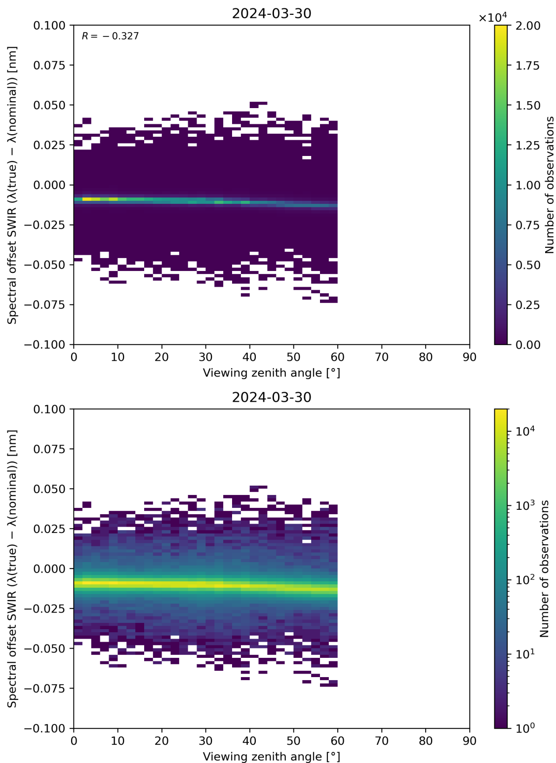
Figure 116: Scatter density plot of “Viewing zenith angle” against “Spectral offset SWIR ( \lambda(\text{true}) - \lambda(\text{nominal}) )” for 2024-03-30 to 2024-03-31.
