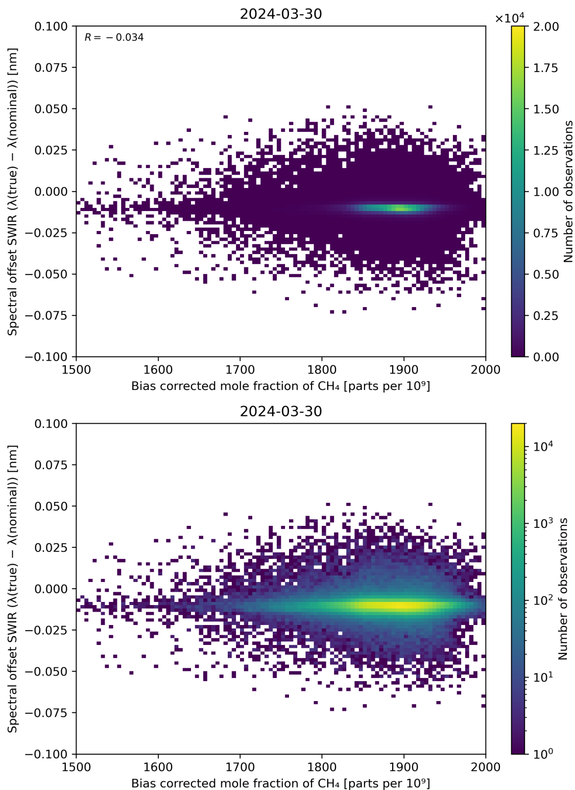
Figure 69: Scatter density plot of “Bias corrected mole fraction of \text{CH}_4 ” against “Spectral offset SWIR ( \lambda(\text{true}) - \lambda(\text{nominal}) )” for 2024-03-30 to 2024-03-31.
