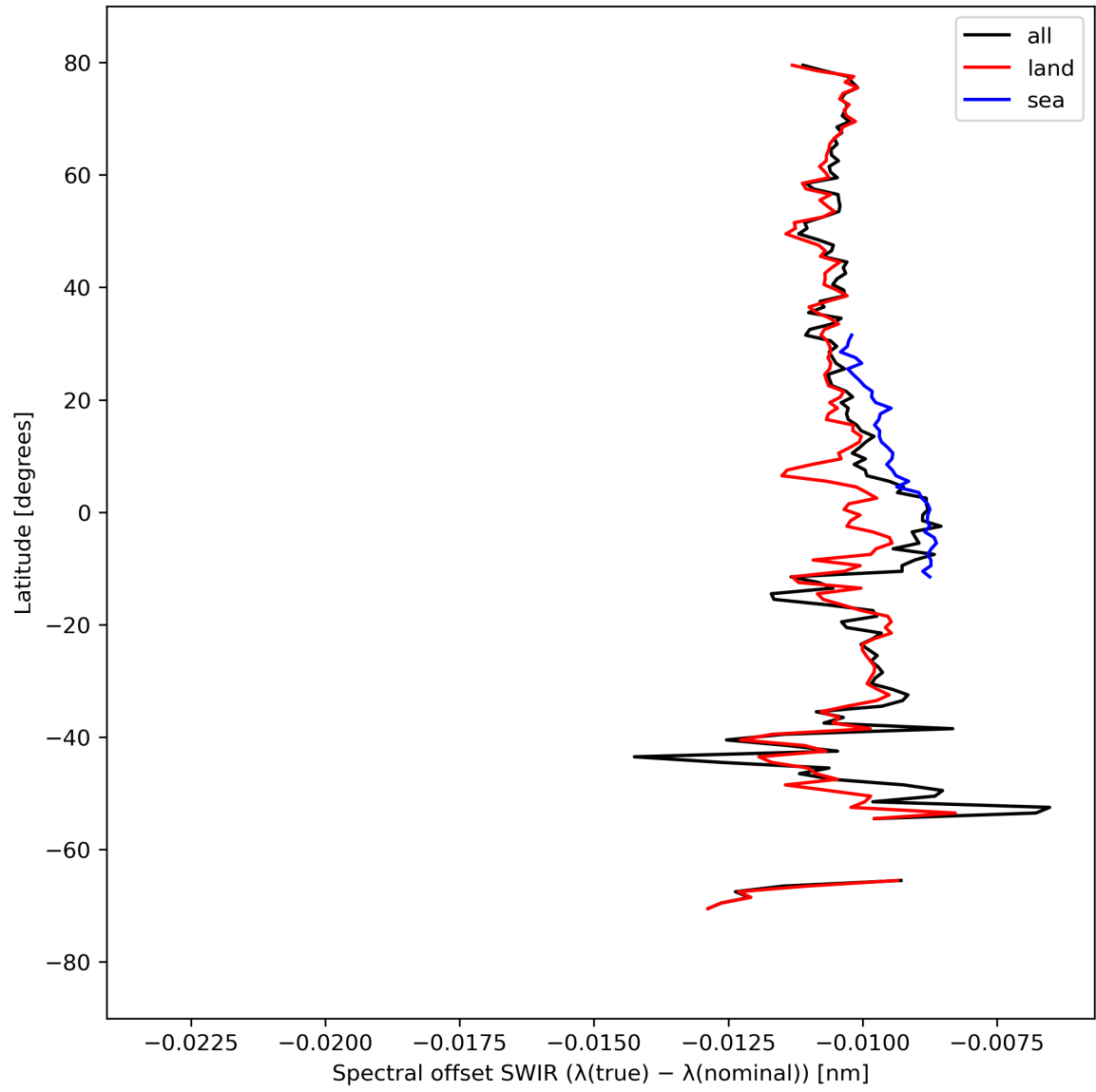
Figure 16: Zonal average of “Spectral offset SWIR ( \lambda(\text{true}) - \lambda(\text{nominal}) )” for 2024-03-30 to 2024-03-31.
