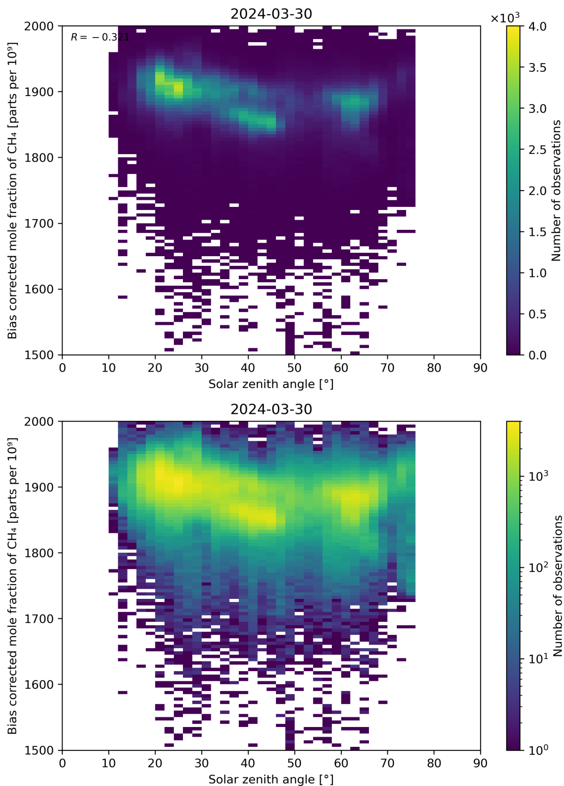
Figure 100: Scatter density plot of “Solar zenith angle” against “Bias corrected mole fraction of CH 4 ” for 2024-03-30 to 2024-03-31.
