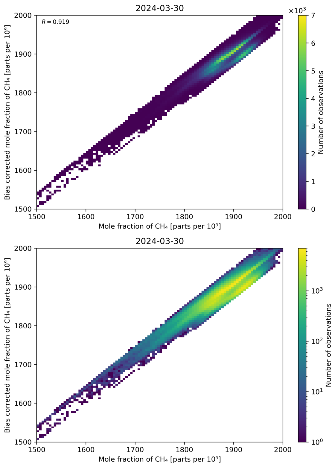
Figure 74: Scatter density plot of “Mole fraction of CH 4 ” against “Bias corrected mole fraction of CH 4 ” for 2024-03-30 to 2024-03-31.
