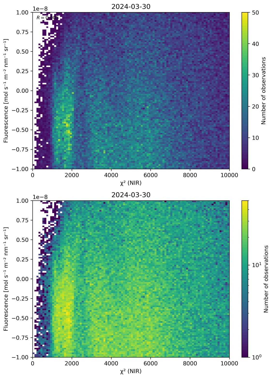
Figure 45: Scatter density plot of “ \chi^2 (NIR)” against “Fluorescence” for 2024-03-30 to 2024-03-31.
