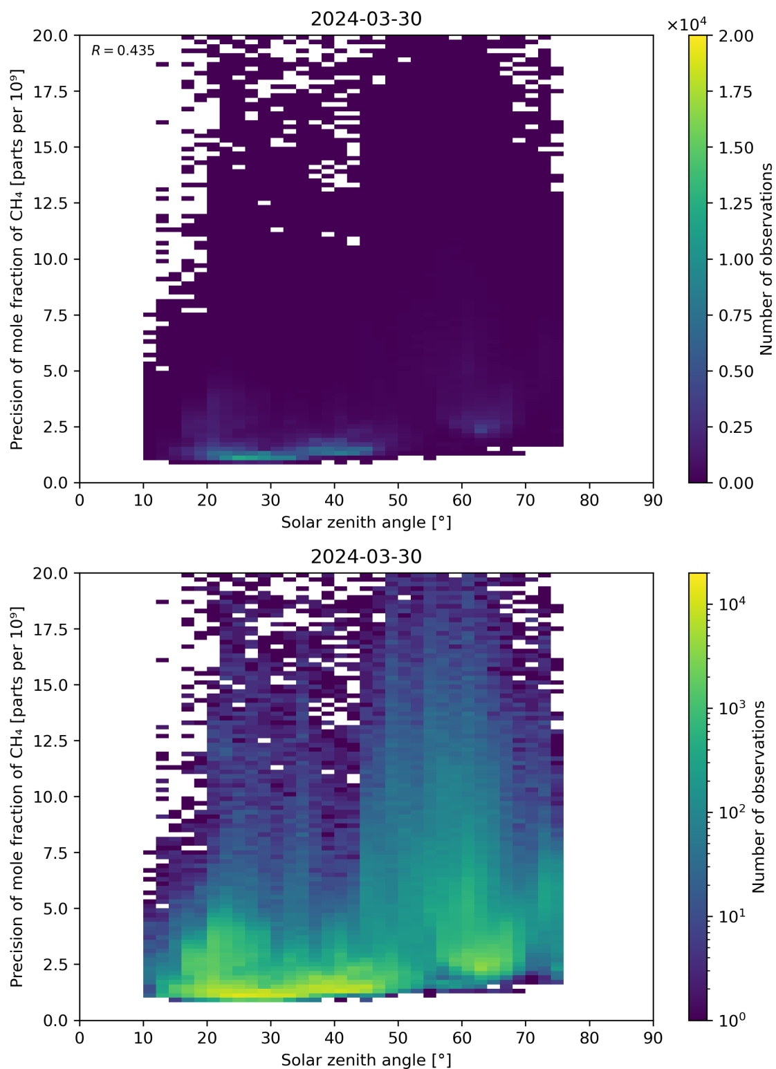
Figure 101: Scatter density plot of “Solar zenith angle” against “Precision of mole fraction of CH 4 ” for 2024-03-30 to 2024-03-31.
