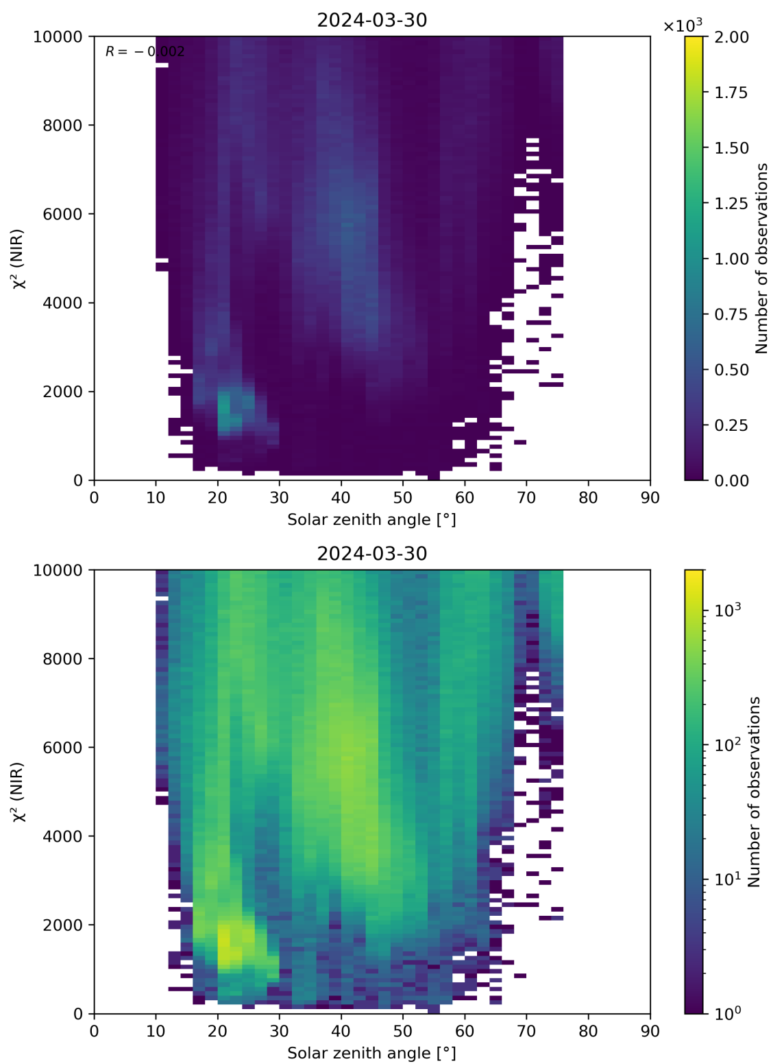
Figure 94: Scatter density plot of “Solar zenith angle” against “ \chi^2 (NIR)” for 2024-03-30 to 2024-03-31.
