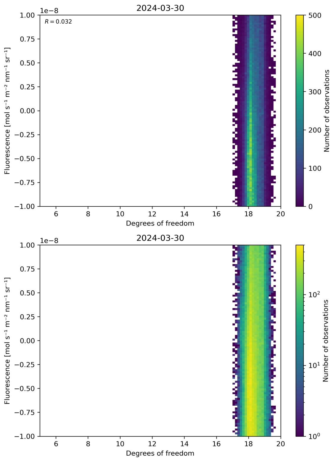
Figure 51: Scatter density plot of “Degrees of freedom” against “Fluorescence” for 2024-03-30 to 2024-03-31.
