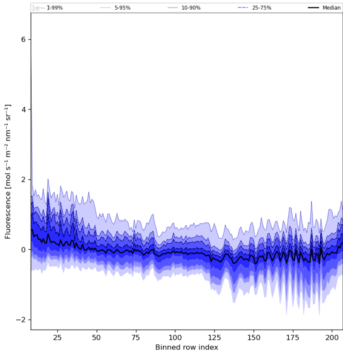
Figure 43: Along track statistics of “Fluorescence” for 2024-03-30 to 2024-03-31
