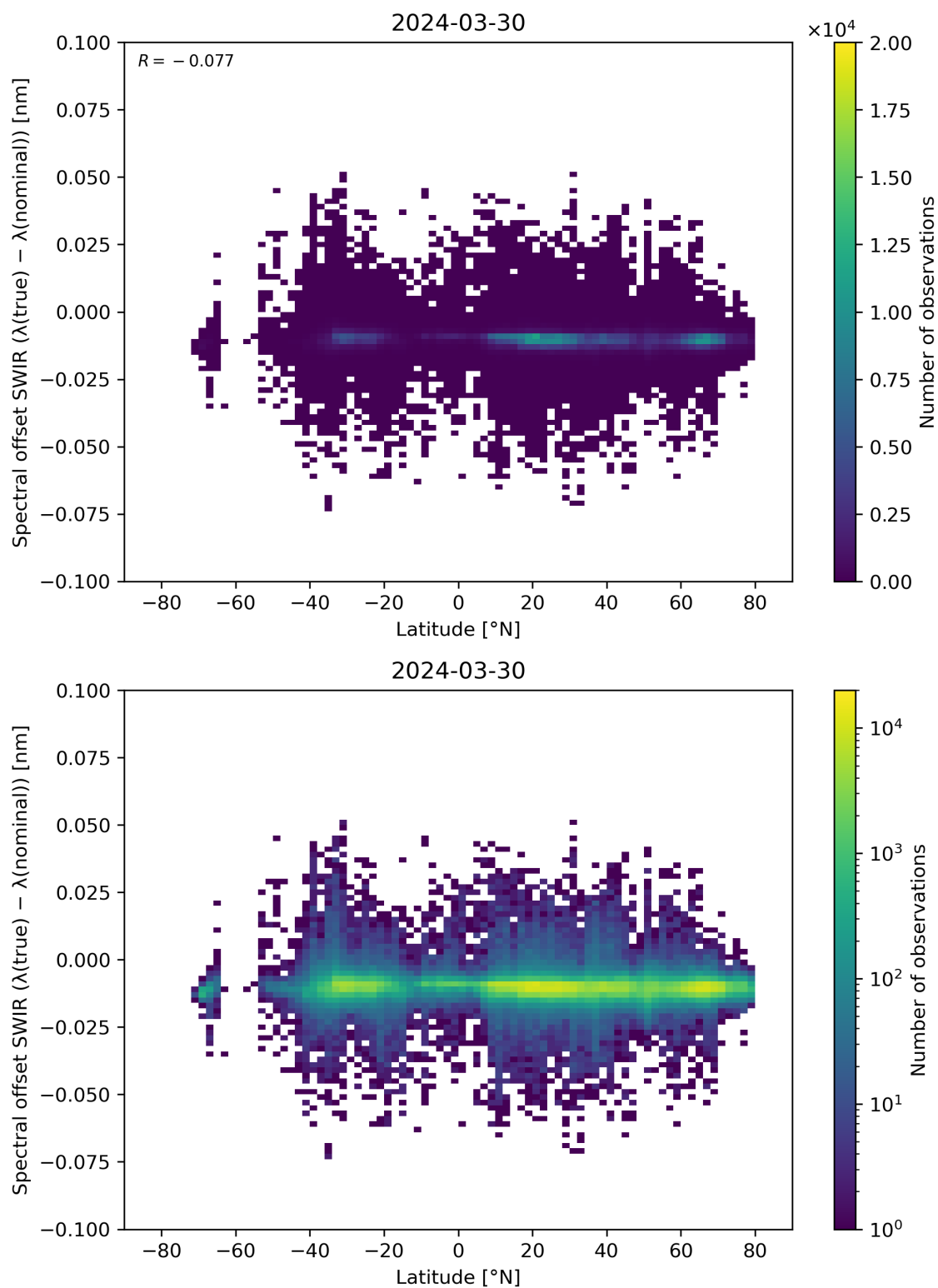
Figure 62: Scatter density plot of “Latitude” against “Spectral offset SWIR ( \lambda(\text{true}) - \lambda(\text{nominal}) )” for 2024-03-30 to 2024-03-31.
