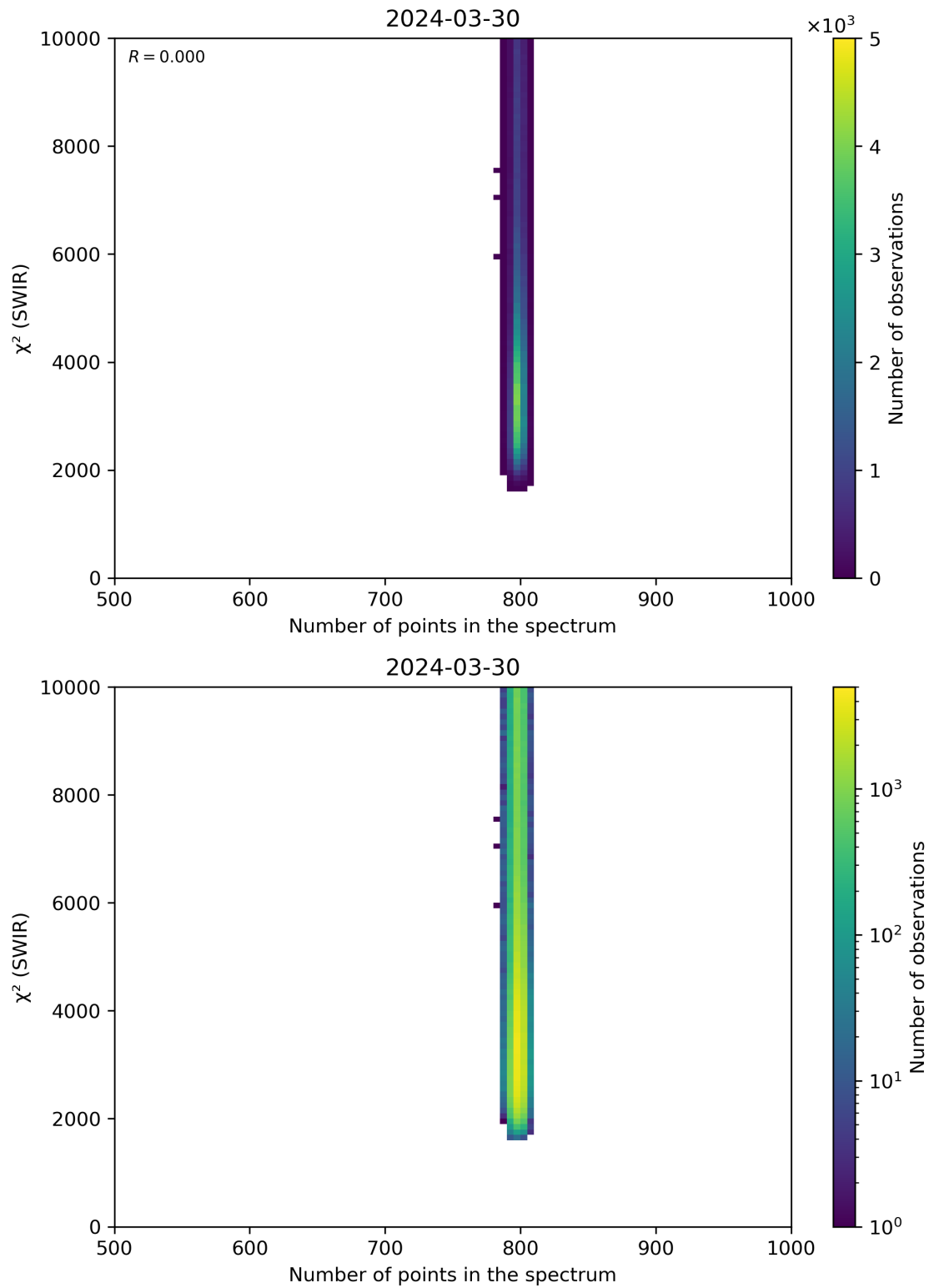
Figure 89: Scatter density plot of “Number of points in the spectrum” against “ \chi^2 (SWIR)” for 2024-03-30 to 2024-03-31.
