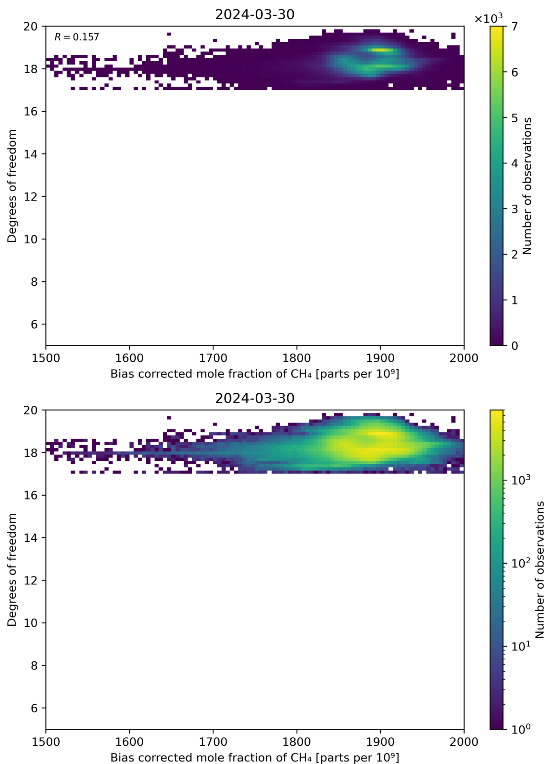
Figure 65: Scatter density plot of “Bias corrected mole fraction of CH 4 ” against “Degrees of freedom” for 2024-03-30 to 2024-03-31.
