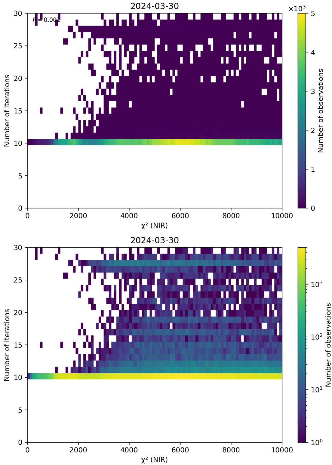
Figure 46: Scatter density plot of “ \chi^2 (NIR)” against “Number of iterations” for 2024-03-30 to 2024-03-31.
