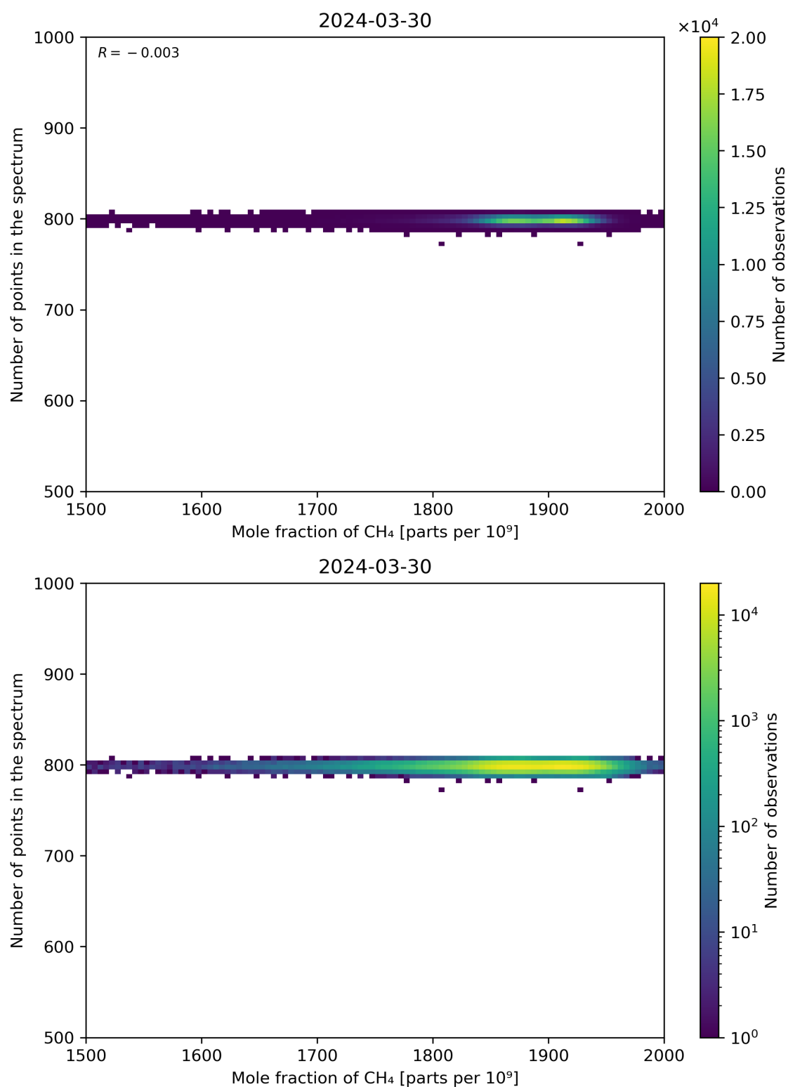
Figure 77: Scatter density plot of “Mole fraction of CH 4 ” against “Number of points in the spectrum” for 2024-03-30 to 2024-03-31.
