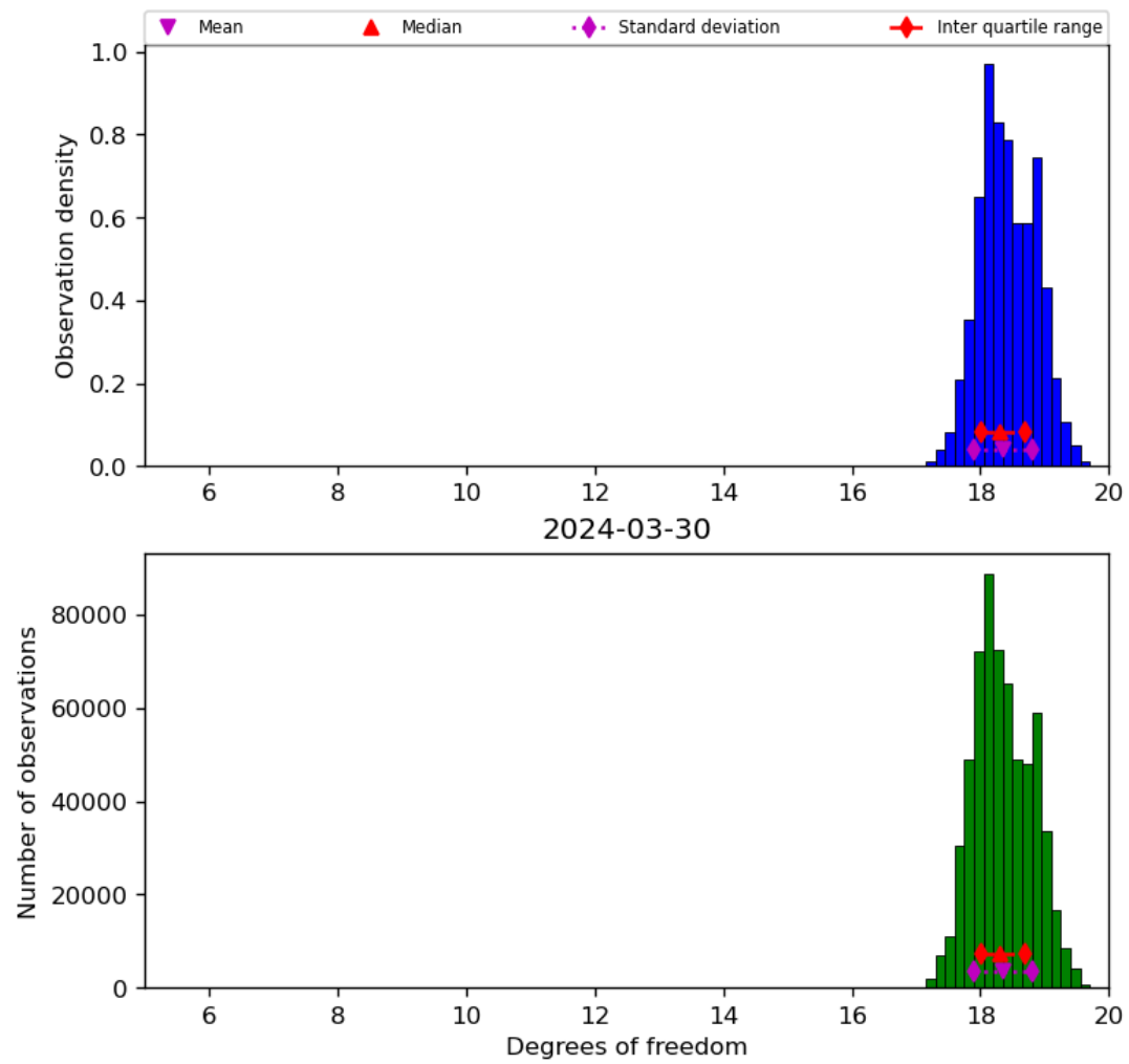
Figure 30: Histogram of “Degrees of freedom” for 2024-03-30 to 2024-03-31
