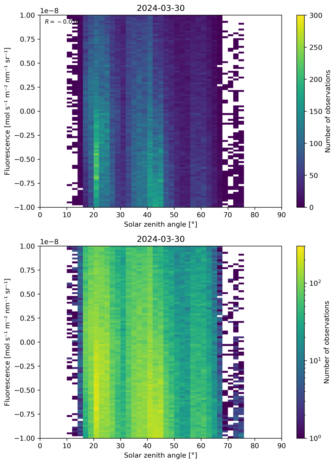
Figure 97: Scatter density plot of “Solar zenith angle” against “Fluorescence” for 2024-03-30 to 2024-03-31.
