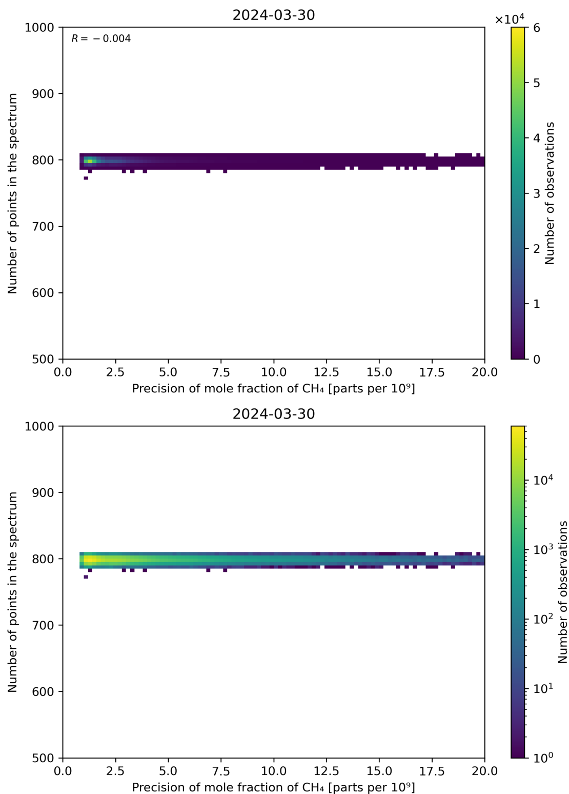
Figure 84: Scatter density plot of “Precision of mole fraction of CH 4 ” against “Number of points in the spectrum” for 2024-03-30 to 2024-03-31.
