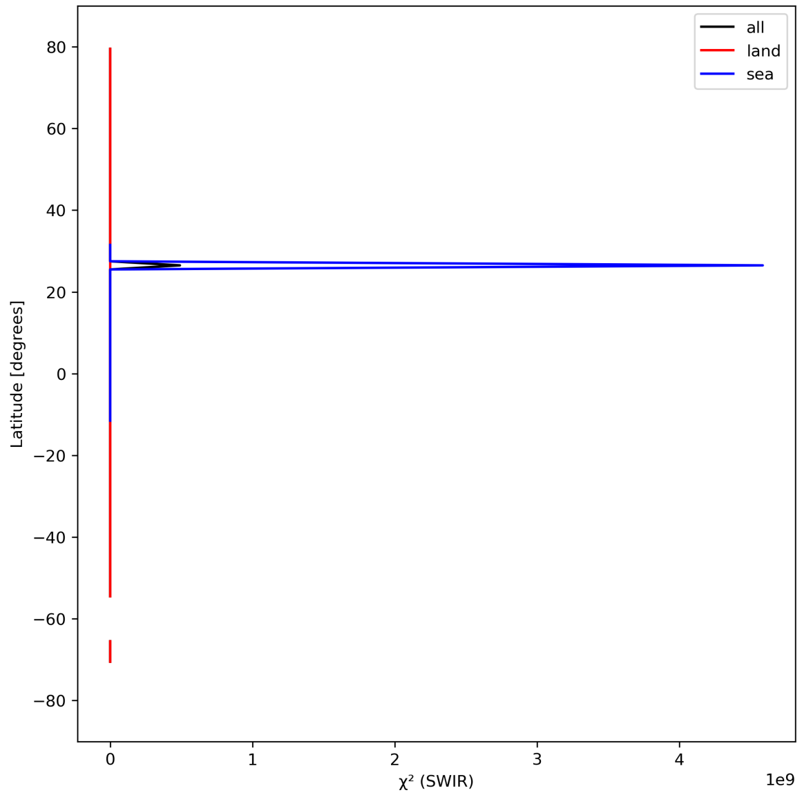
Figure 17: Zonal average of “ \chi^2 (SWIR)” for 2024-03-30 to 2024-03-31.
