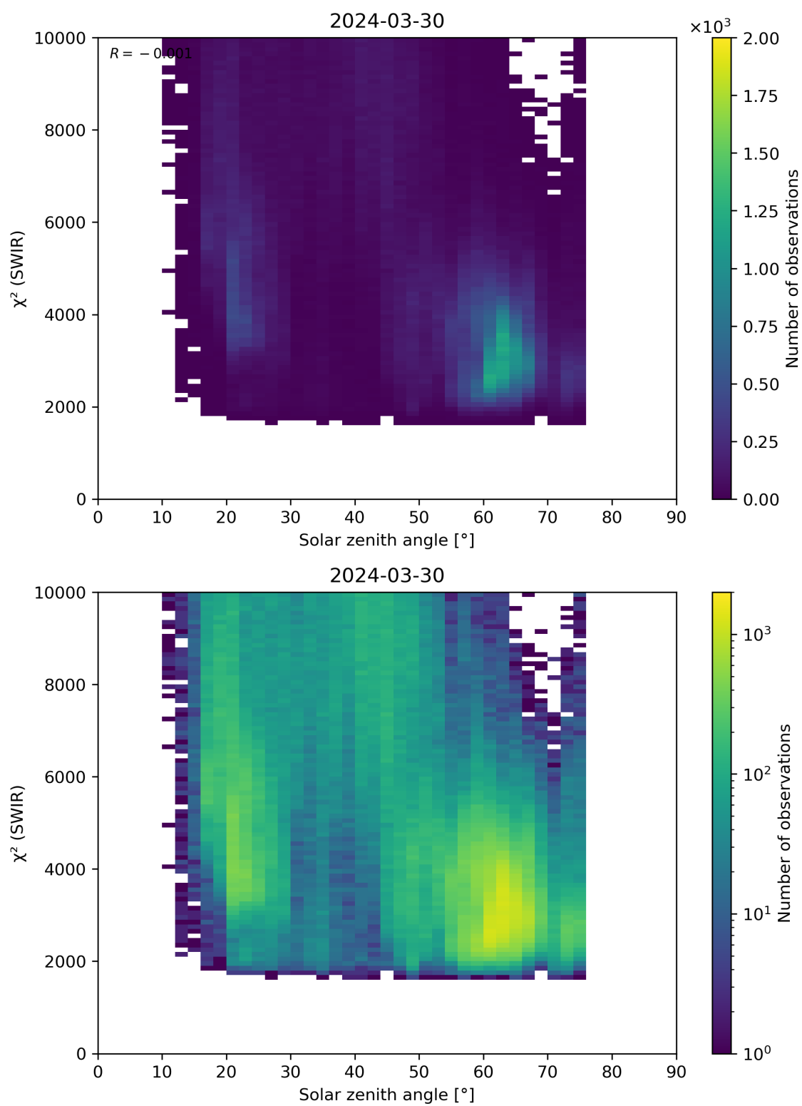
Figure 95: Scatter density plot of “Solar zenith angle” against “ \chi^2 (SWIR)” for 2024-03-30 to 2024-03-31.
