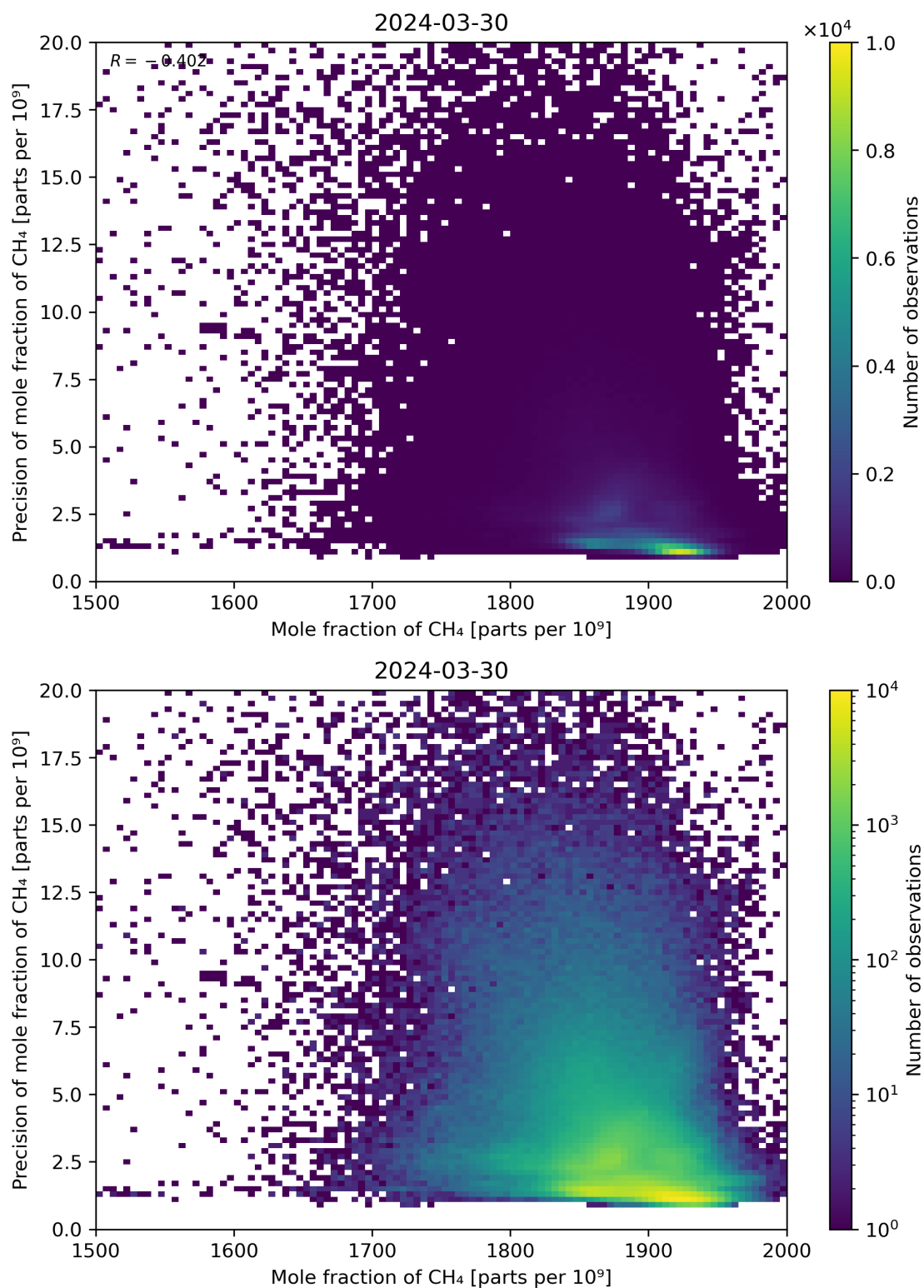
Figure 75: Scatter density plot of “Mole fraction of CH 4 ” against “Precision of mole fraction of CH 4 ” for 2024-03-30 to 2024-03-31.
