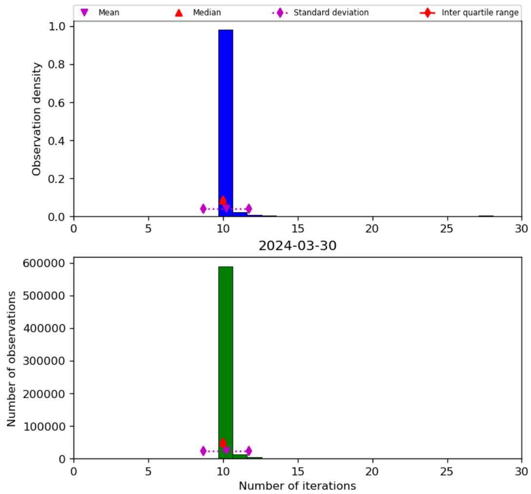
Figure 31: Histogram of “Number of iterations” for 2024-03-30 to 2024-03-31
