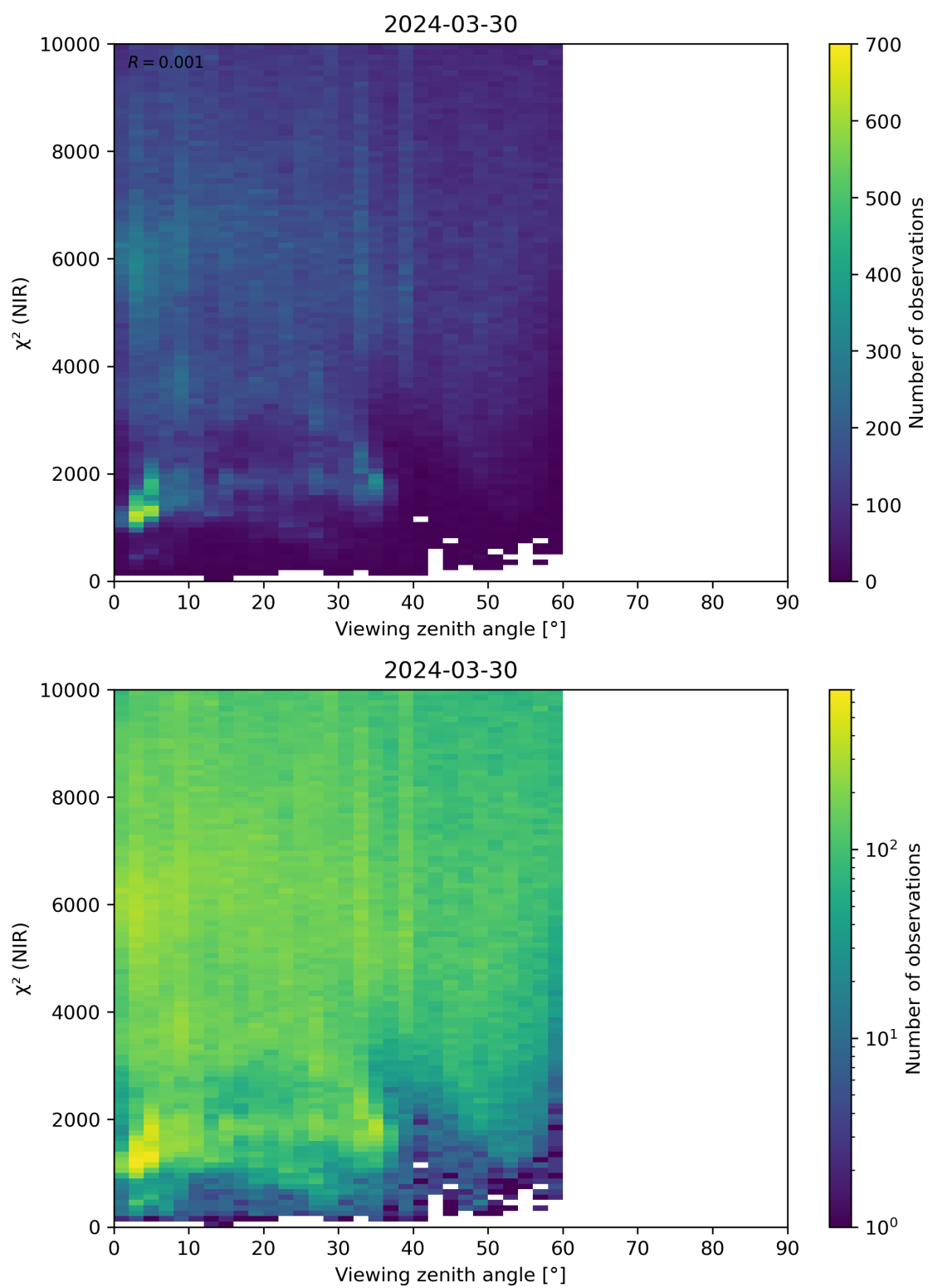
Figure 105: Scatter density plot of “Viewing zenith angle” against “ \chi^2 (NIR)” for 2024-03-30 to 2024-03-31.
