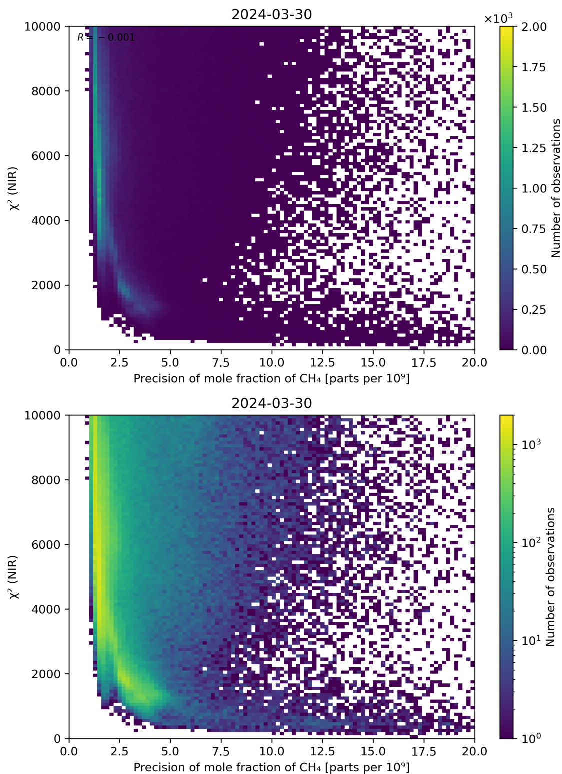
Figure 78: Scatter density plot of “Precision of mole fraction of CH 4 ” against “ \chi^2 (NIR)” for 2024-03-30 to 2024-03-31.
