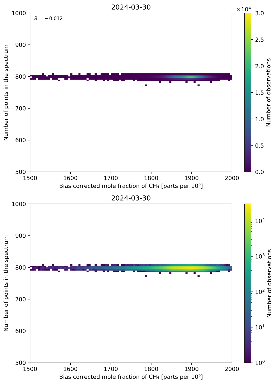
Figure 68: Scatter density plot of “Bias corrected mole fraction of CH 4 ” against “Number of points in the spectrum” for 2024-03-30 to 2024-03-31.
