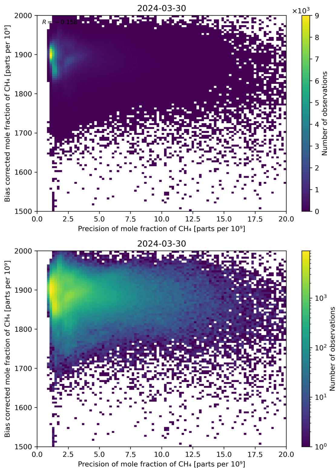
Figure 82: Scatter density plot of “Precision of mole fraction of CH 4 ” against “Bias corrected mole fraction of CH 4 ” for 2024-03-30 to 2024-03-31.
