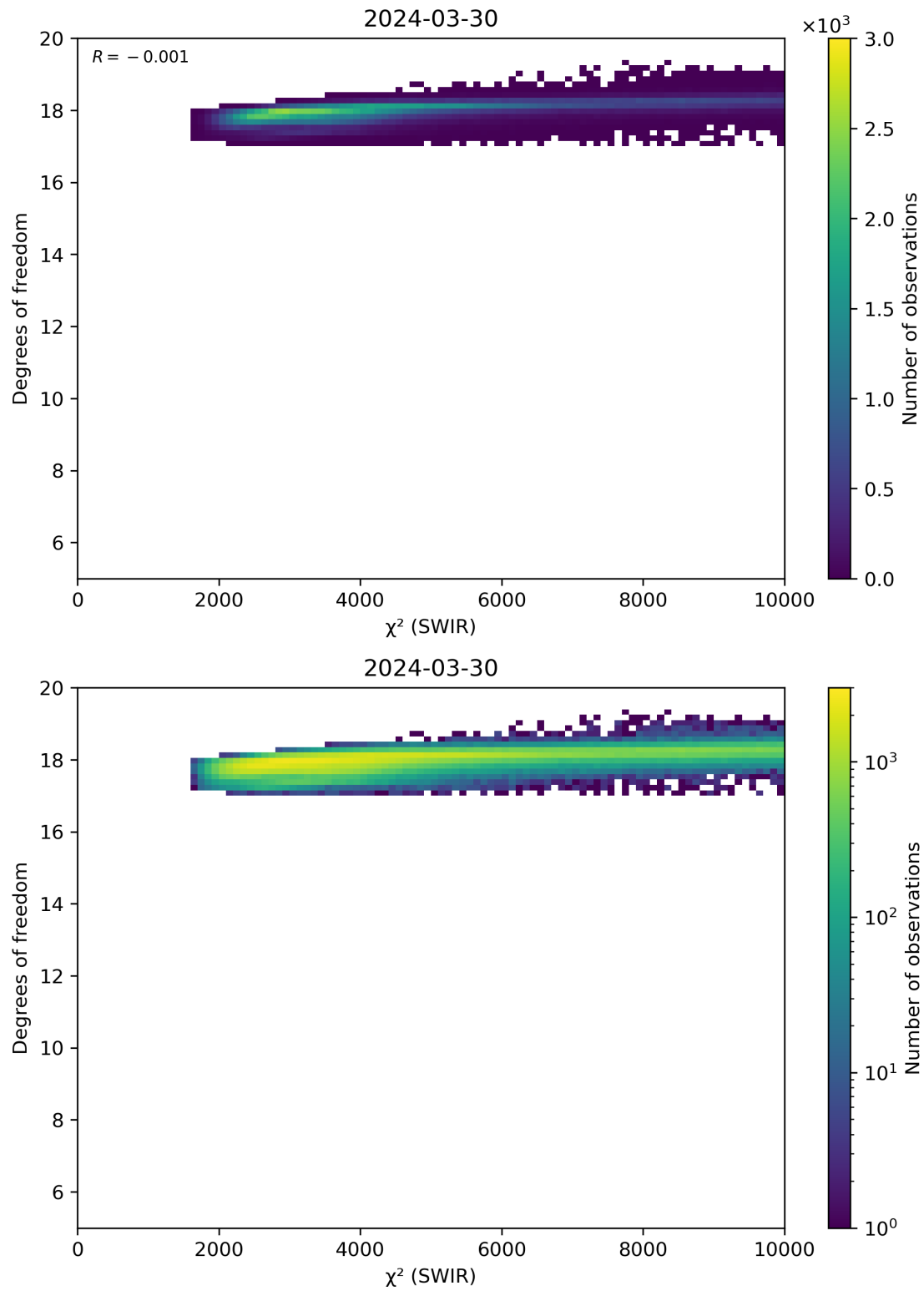
Figure 48: Scatter density plot of “ \chi^2 (SWIR)” against “Degrees of freedom” for 2024-03-30 to 2024-03-31.
