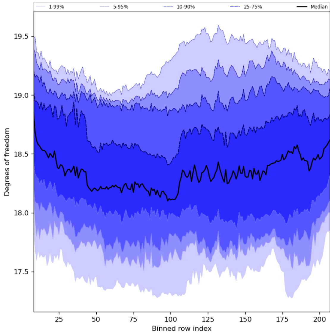
Figure 41: Along track statistics of “Degrees of freedom” for 2024-03-30 to 2024-03-31
