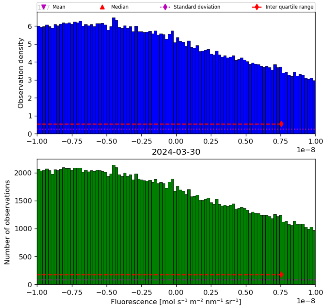
Figure 32: Histogram of “Fluorescence” for 2024-03-30 to 2024-03-31
