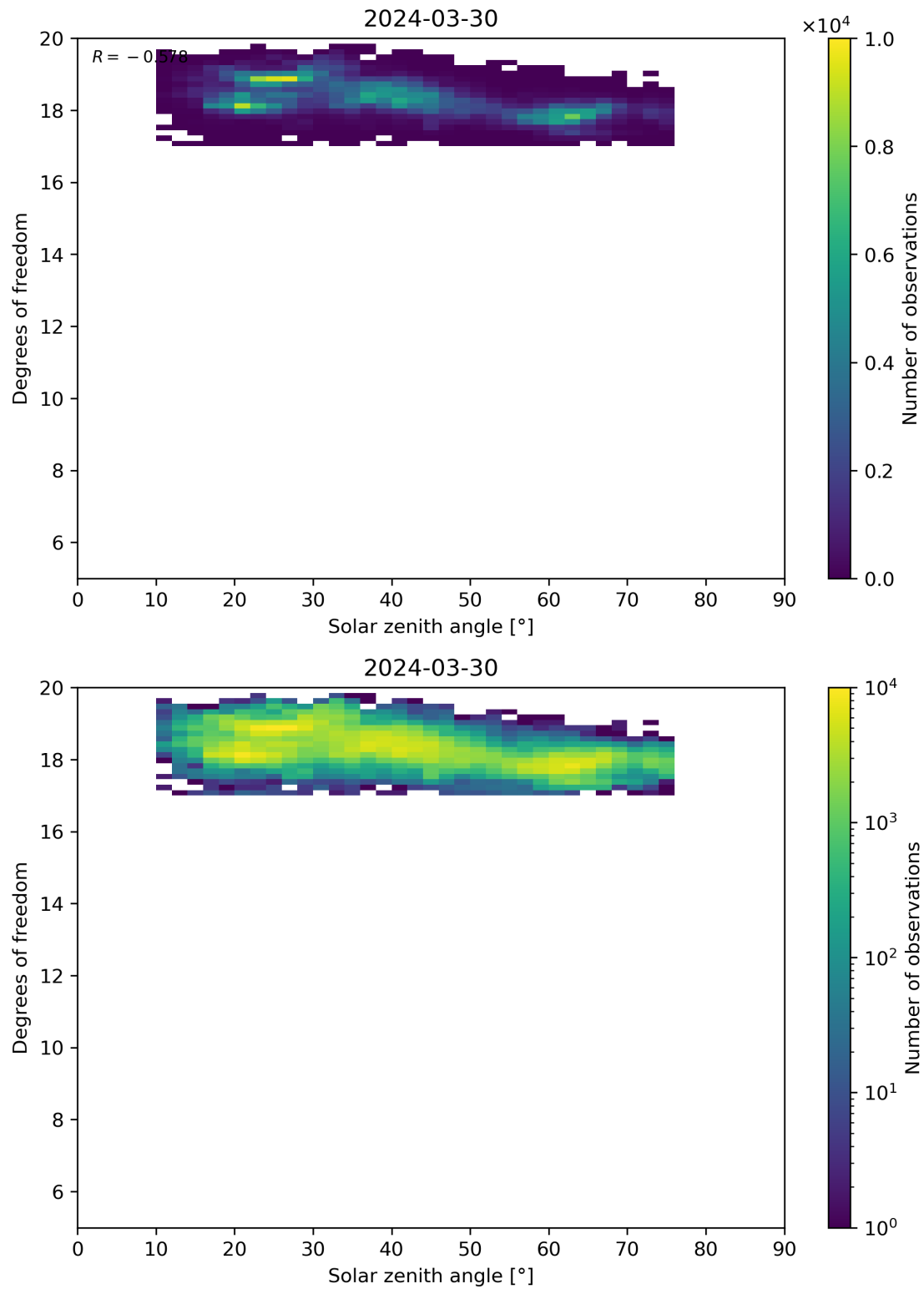
Figure 96: Scatter density plot of “Solar zenith angle” against “Degrees of freedom” for 2024-03-30 to 2024-03-31.
