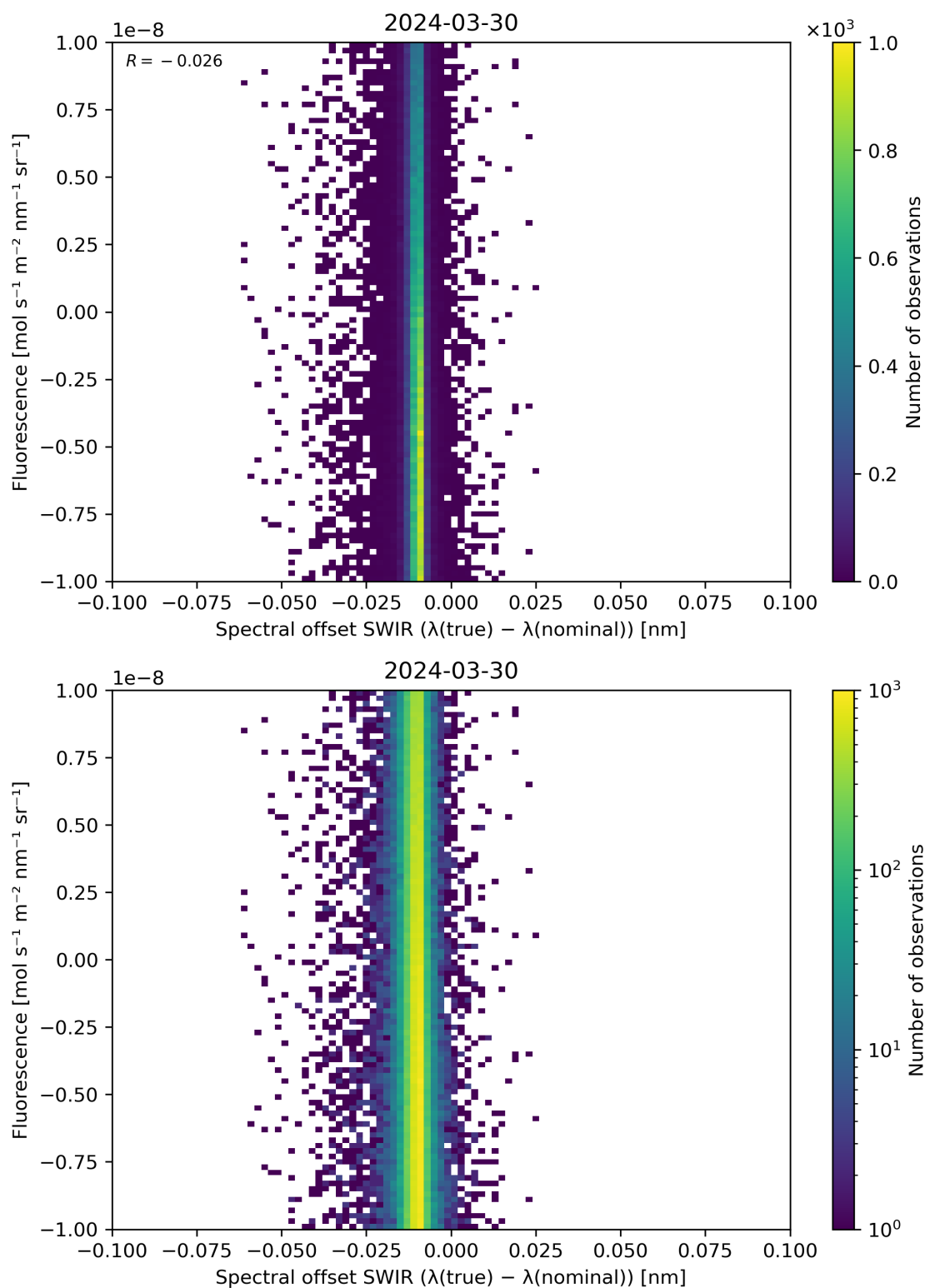
Figure 120: Scatter density plot of “Spectral offset SWIR ( \lambda(\text{true}) - \lambda(\text{nominal}) )” against “Fluorescence” for 2024-03-30 to 2024-03-31.
