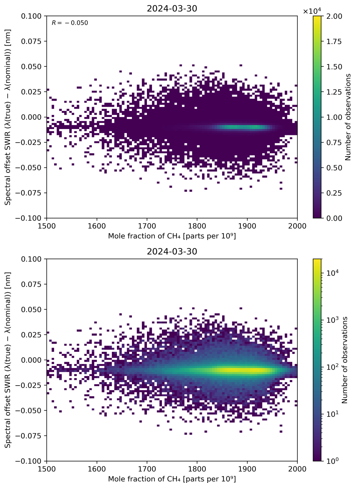
Figure 86: Scatter density plot of “Mole fraction of CH 4 ” against “Spectral offset SWIR ( \lambda(\text{true}) - \lambda(\text{nominal}) )” for 2024-03-30 to 2024-03-31.
