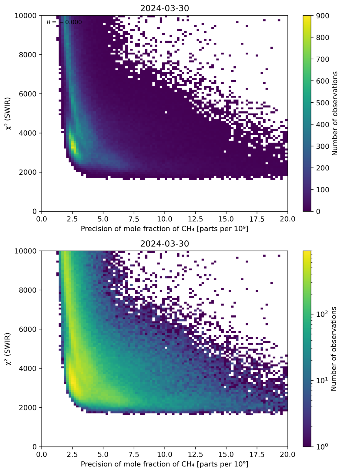
Figure 79: Scatter density plot of “Precision of mole fraction of \text{CH}_4 ” against “ \chi^2 (SWIR)” for 2024-03-30 to 2024-03-31.
