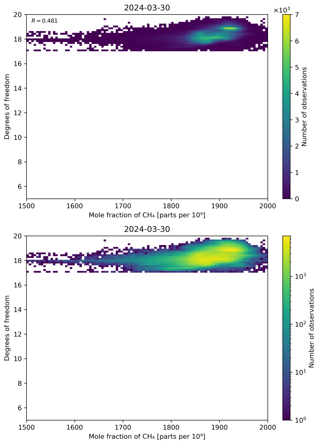
Figure 72: Scatter density plot of “Mole fraction of CH 4 ” against “Degrees of freedom” for 2024-03-30 to 2024-03-31.
