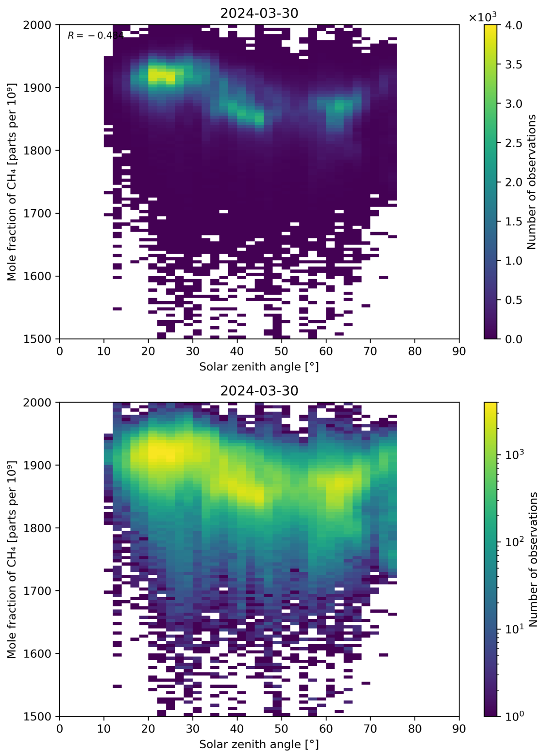
Figure 99: Scatter density plot of “Solar zenith angle” against “Mole fraction of CH 4 ” for 2024-03-30 to 2024-03-31.
