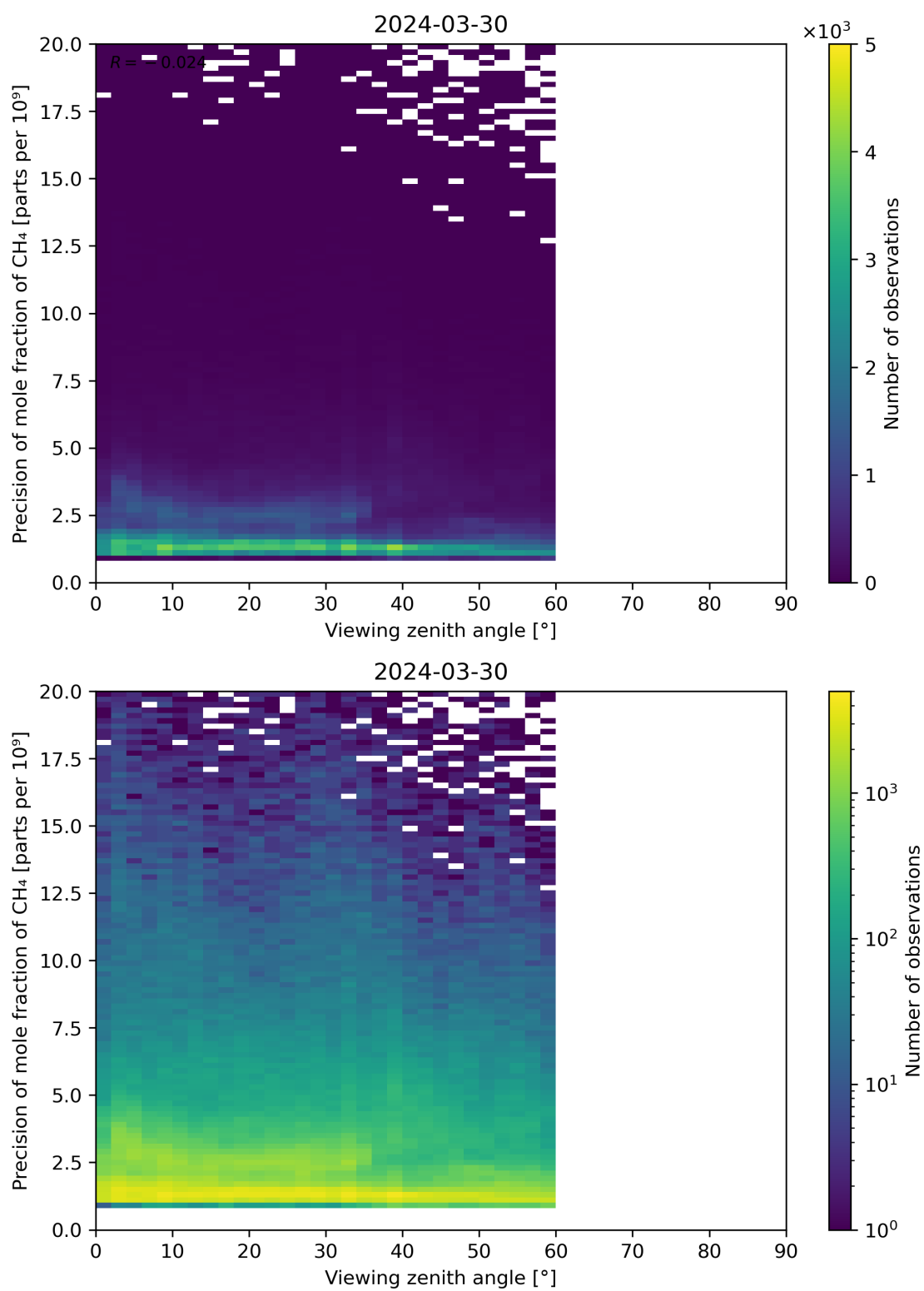
Figure 112: Scatter density plot of “Viewing zenith angle” against “Precision of mole fraction of CH 4 ” for 2024-03-30 to 2024-03-31.
