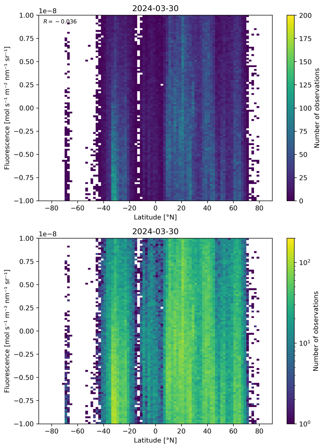
Figure 56: Scatter density plot of “Latitude” against “Fluorescence” for 2024-03-30 to 2024-03-31.
