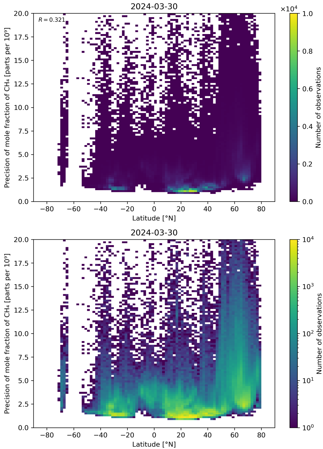
Figure 59: Scatter density plot of “Latitude” against “Precision of mole fraction of \text{CH}_4 ” for 2024-03-30 to 2024-03-31.
