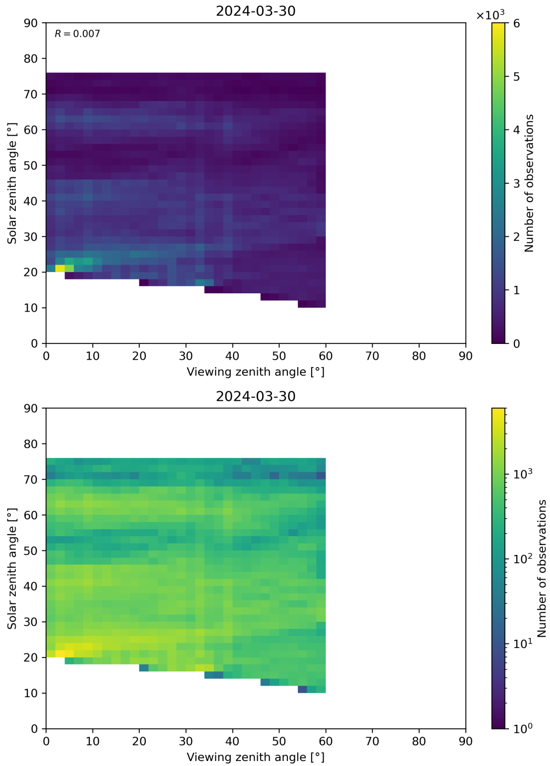
Figure 115: Scatter density plot of “Viewing zenith angle” against “Solar zenith angle” for 2024-03-30 to 2024-03-31.
