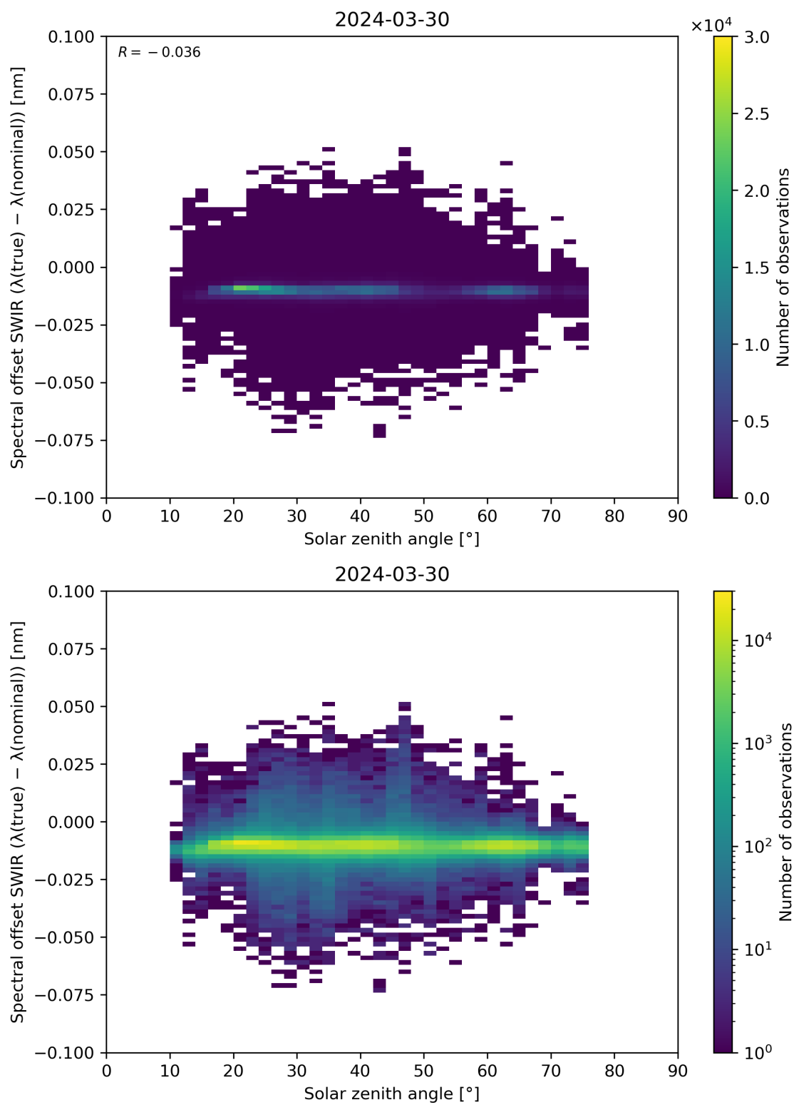
Figure 104: Scatter density plot of “Solar zenith angle” against “Spectral offset SWIR ( \lambda(\text{true}) - \lambda(\text{nominal}) )” for 2024-03-30 to 2024-03-31.
