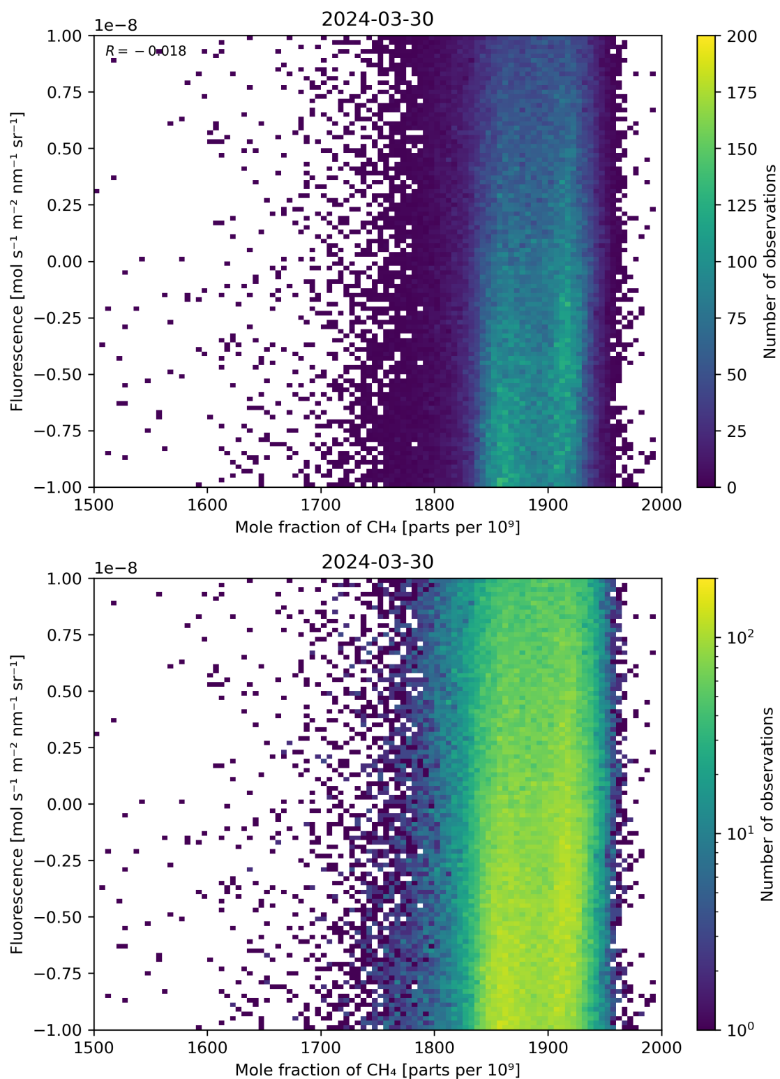
Figure 73: Scatter density plot of “Mole fraction of \text{CH}_4 ” against “Fluorescence” for 2024-03-30 to 2024-03-31.
