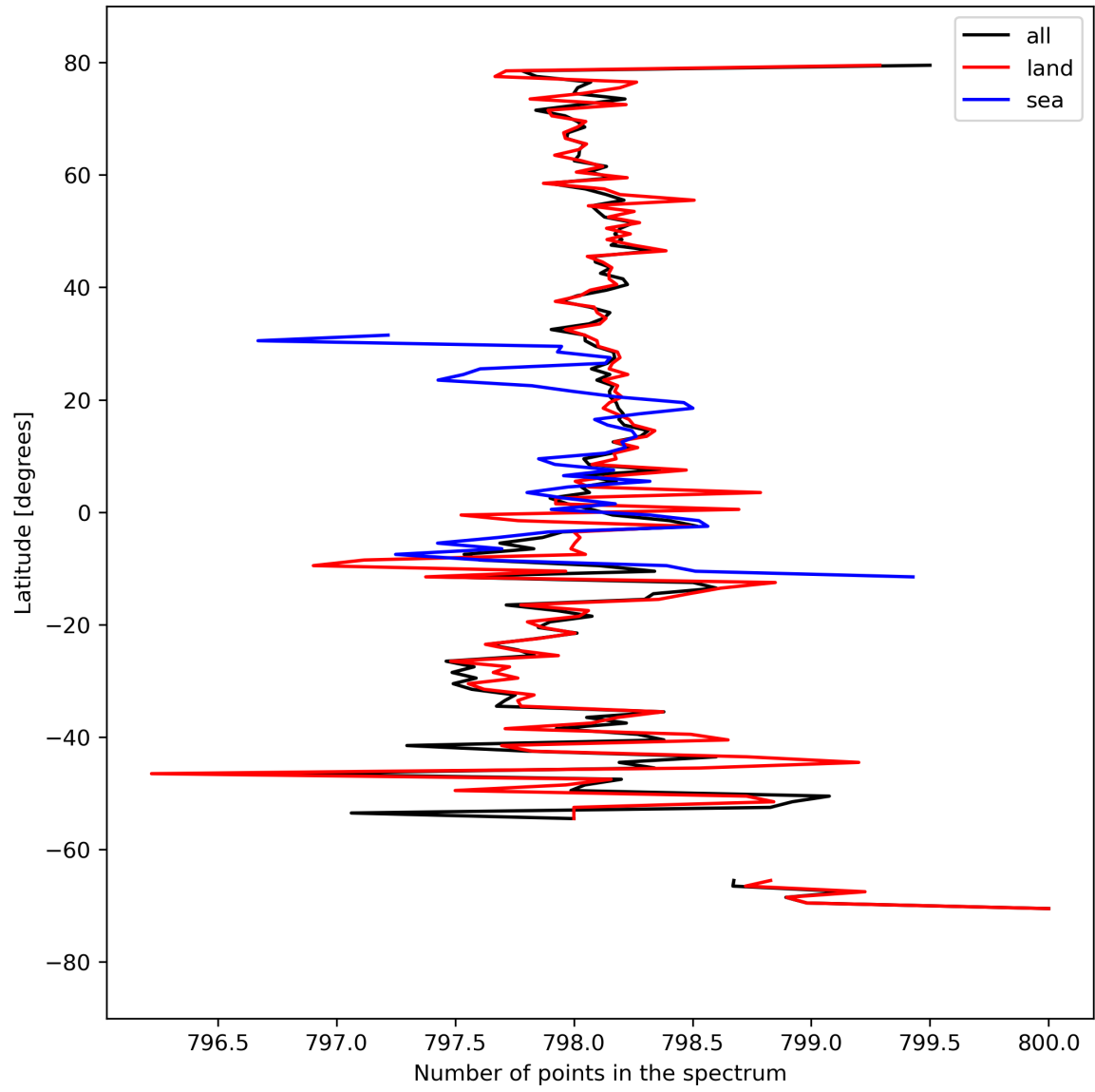
Figure 15: Zonal average of “Number of points in the spectrum” for 2024-03-30 to 2024-03-31.
