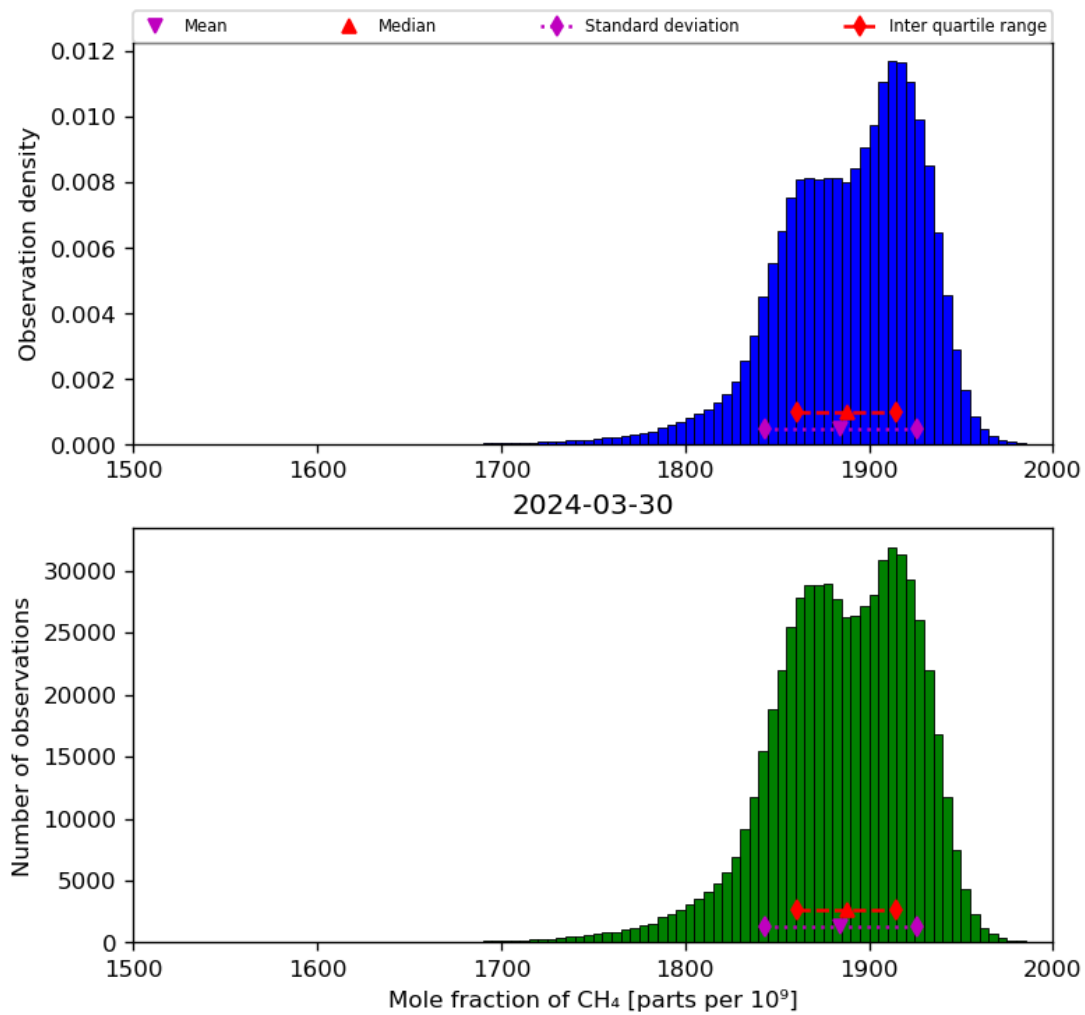
Figure 23: Histogram of “Mole fraction of CH 4 ” for 2024-03-30 to 2024-03-31
