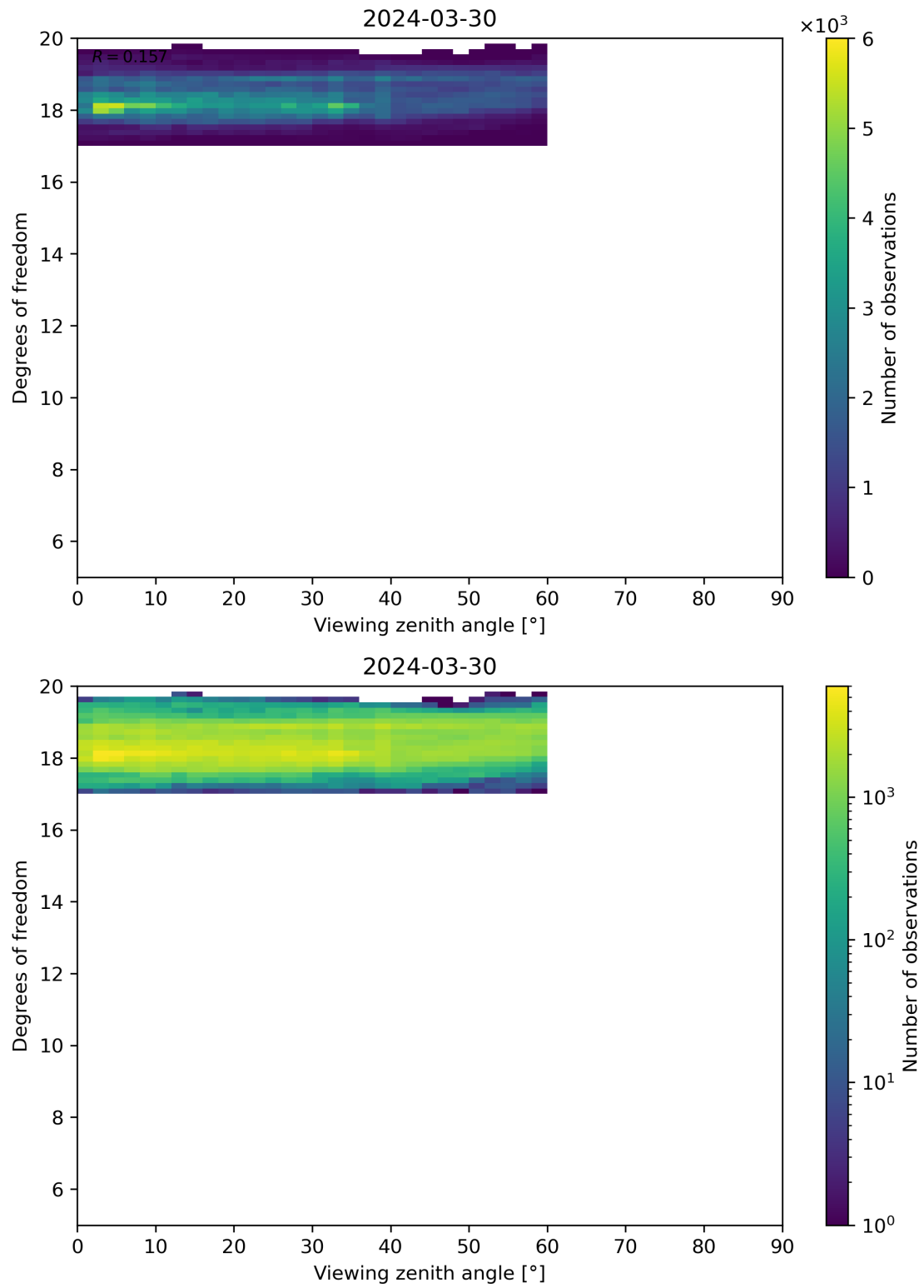
Figure 107: Scatter density plot of “Viewing zenith angle” against “Degrees of freedom” for 2024-03-30 to 2024-03-31.
