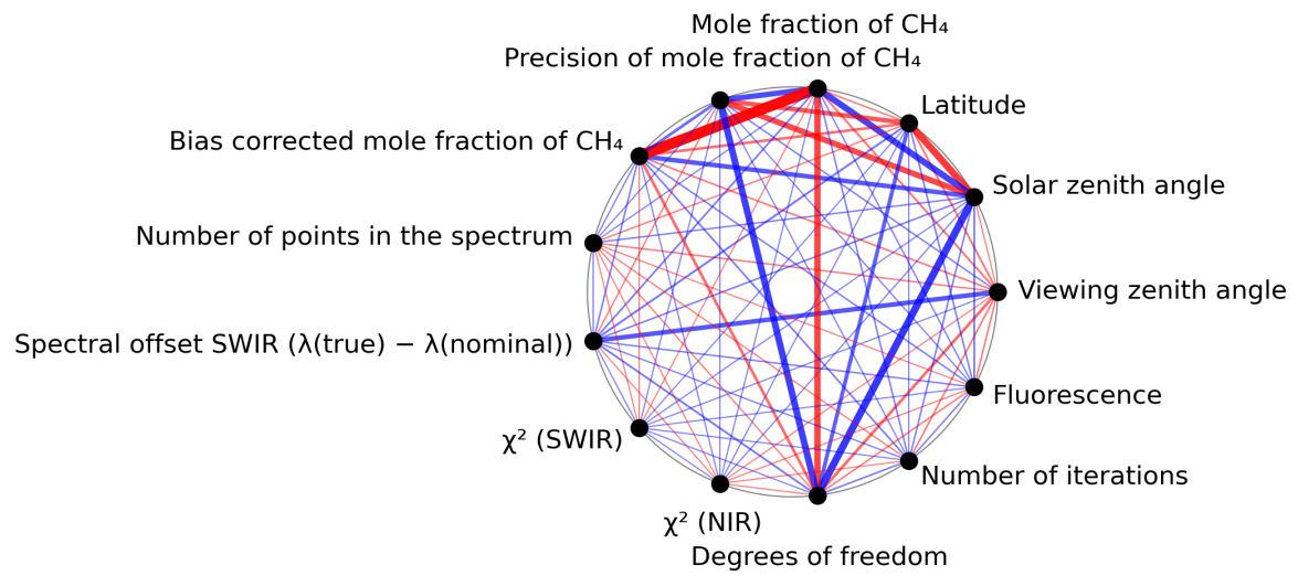
Figure 1: Map of correlation graph for 2024-03-30 to 2024-03-31.
