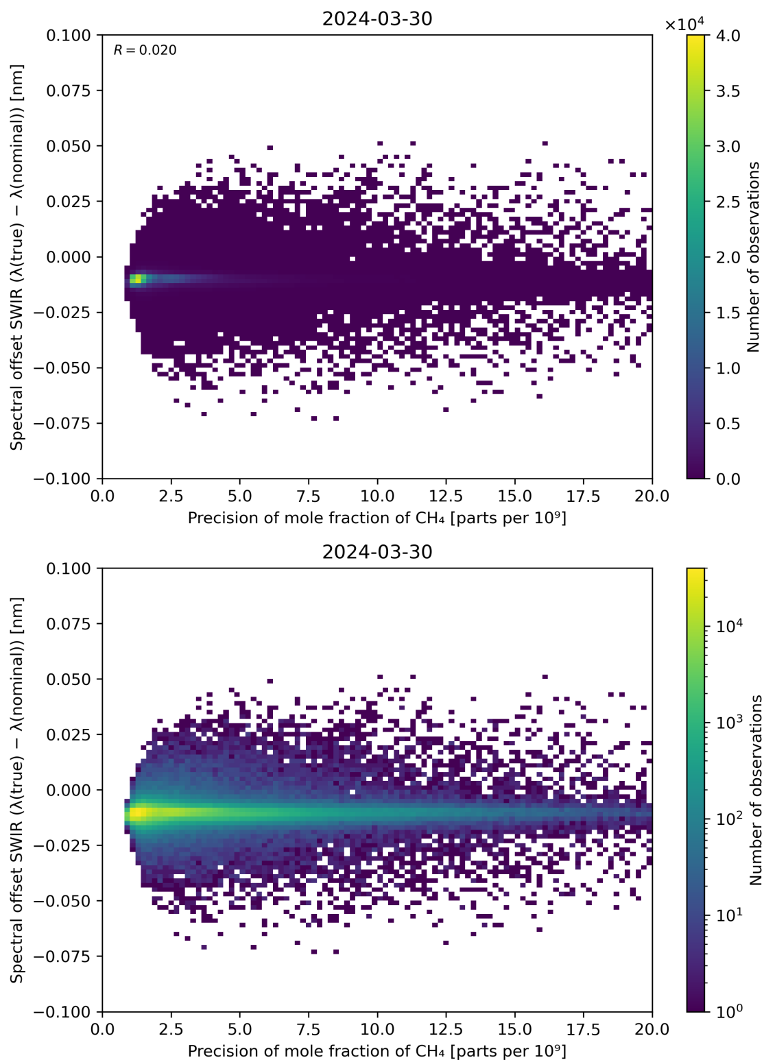
Figure 85: Scatter density plot of “Precision of mole fraction of \text{CH}_4 ” against “Spectral offset SWIR ( \lambda(\text{true}) - \lambda(\text{nominal}) )” for 2024-03-30 to 2024-03-31.
