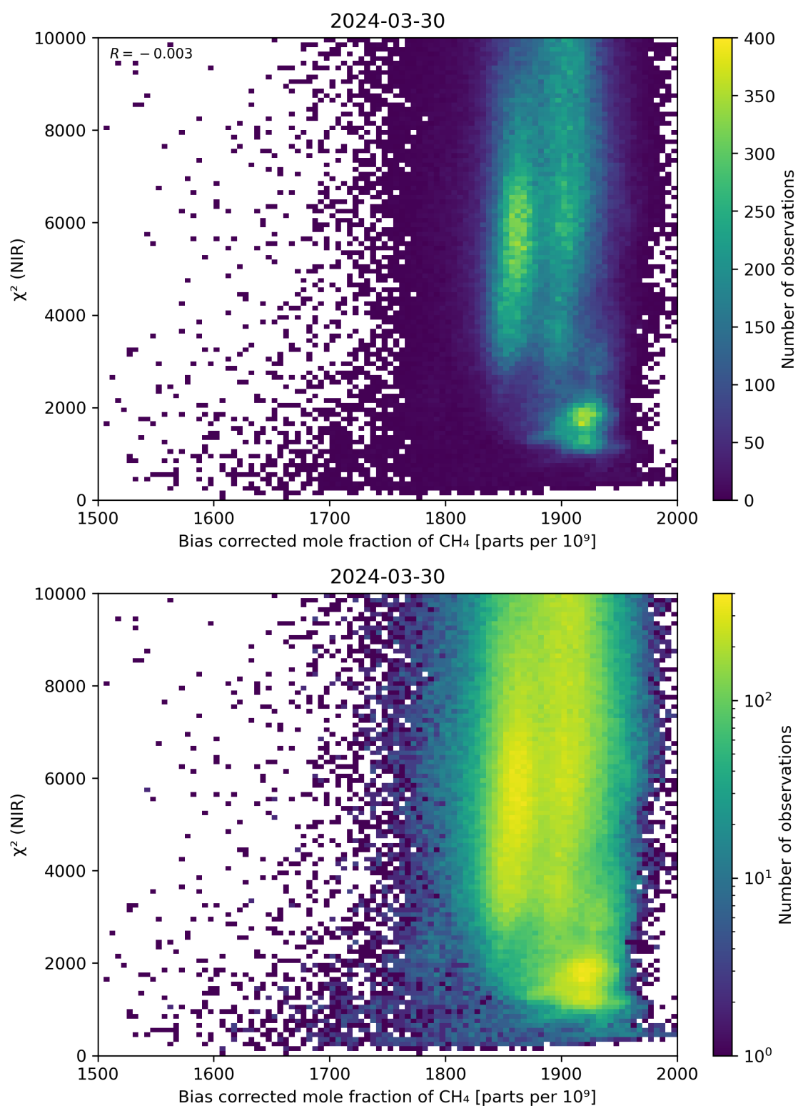
Figure 63: Scatter density plot of “Bias corrected mole fraction of CH 4 ” against “ \chi^2 (NIR)” for 2024-03-30 to 2024-03-31.
