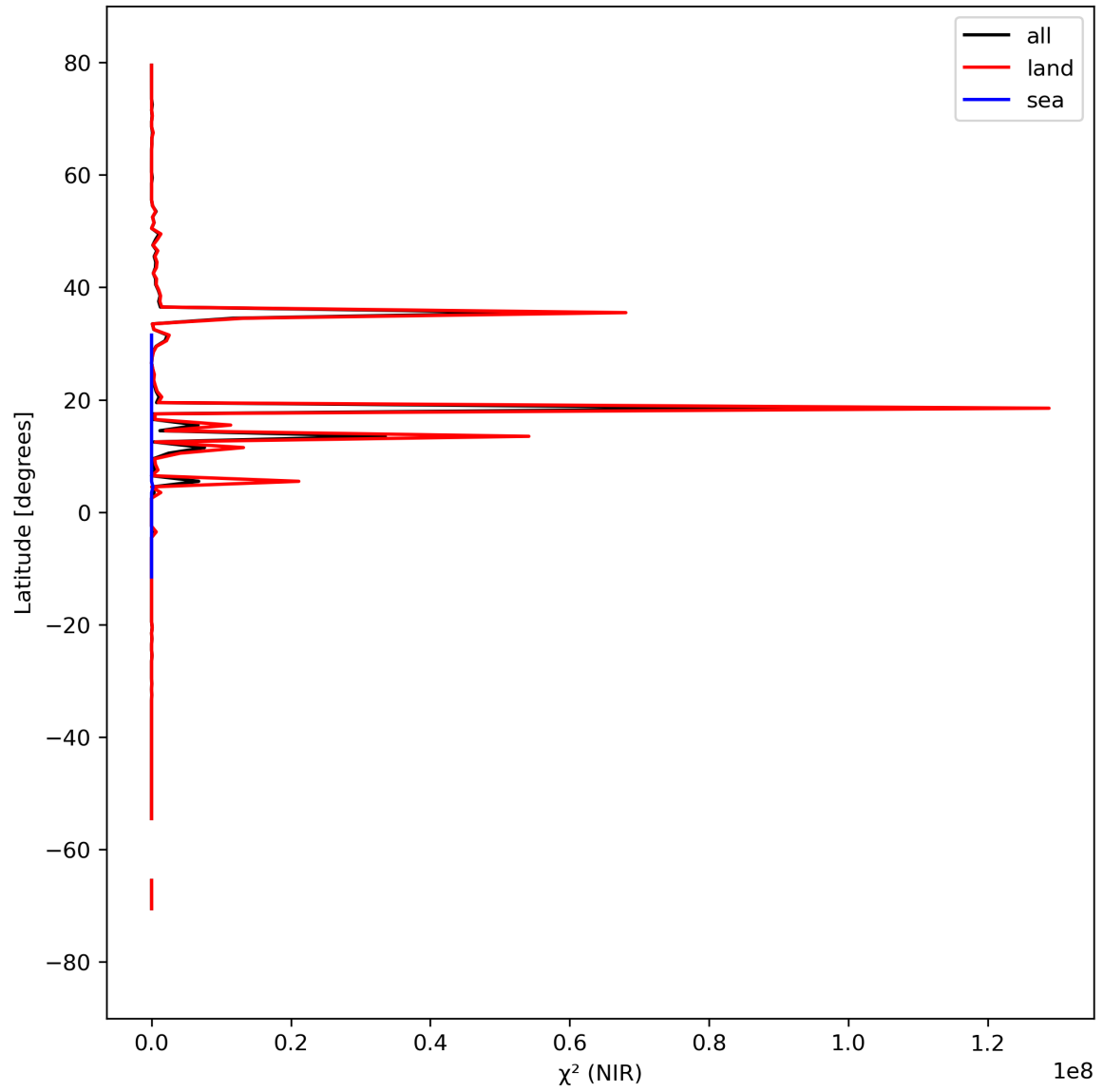
Figure 18: Zonal average of “ \chi^2 (NIR)” for 2024-03-30 to 2024-03-31.
