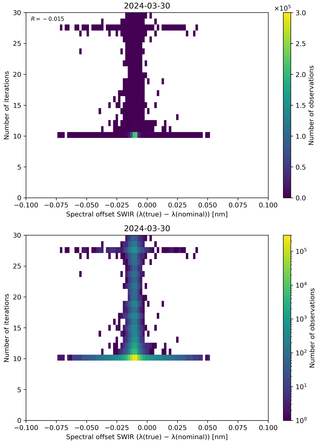
Figure 121: Scatter density plot of “Spectral offset SWIR ( \lambda(\text{true}) - \lambda(\text{nominal}) )” against “Number of iterations” for 2024-03-30 to 2024-03-31.
