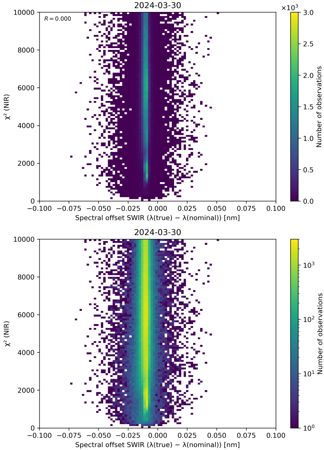
Figure 117: Scatter density plot of “Spectral offset SWIR ( \lambda(\text{true}) - \lambda(\text{nominal}) )” against “ \chi^2 (NIR)” for 2024-03-30 to 2024-03-31.
