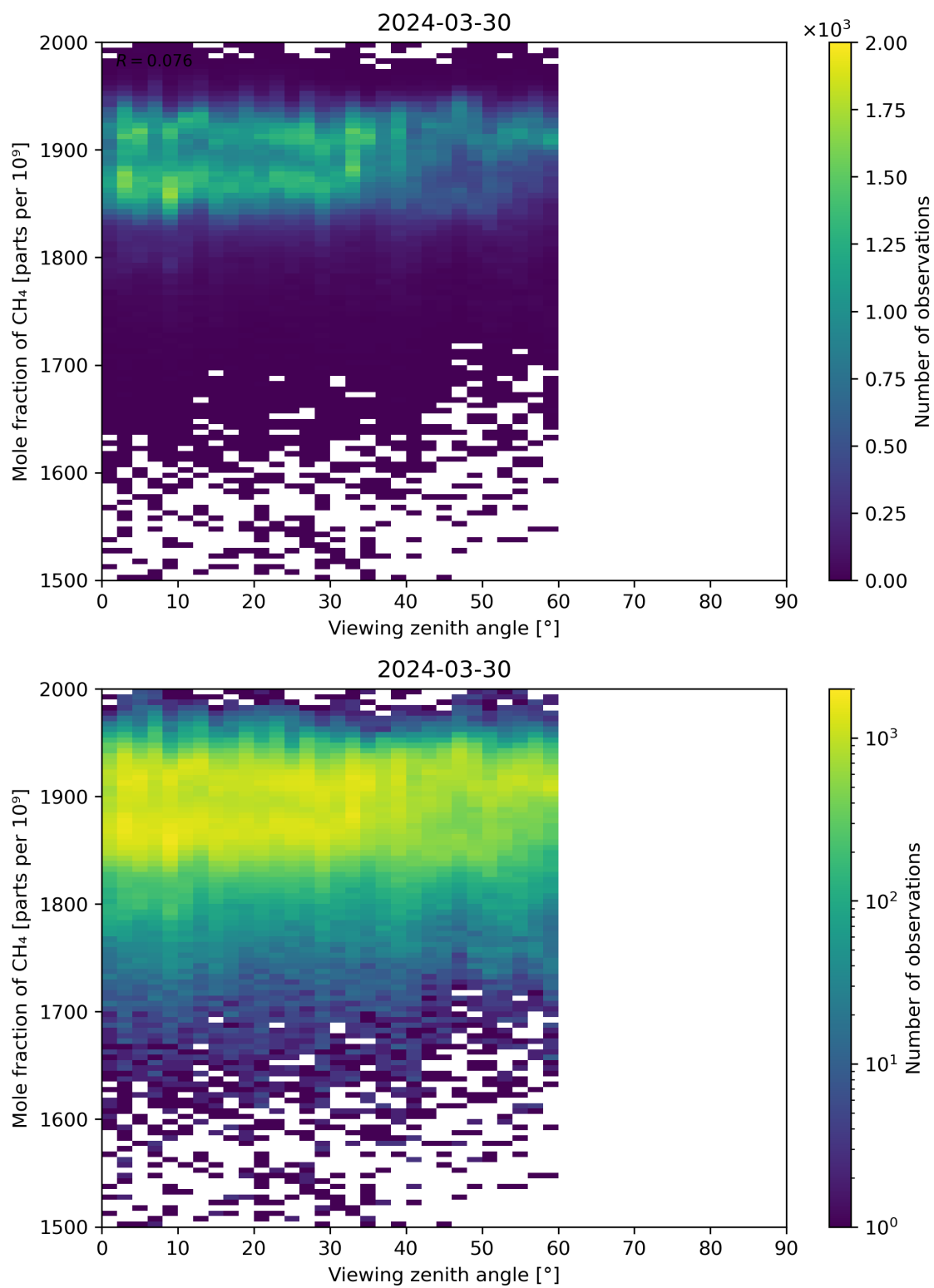
Figure 110: Scatter density plot of “Viewing zenith angle” against “Mole fraction of CH 4 ” for 2024-03-30 to 2024-03-31.
