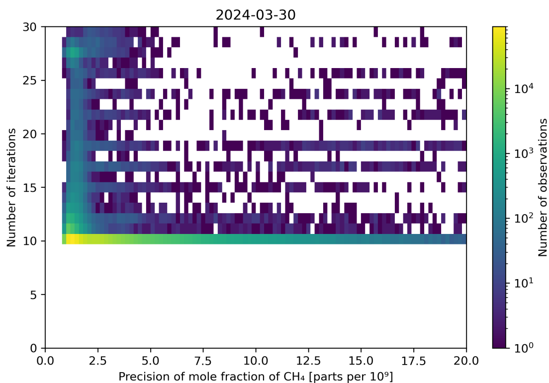
Figure 83: Scatter density plot of “Precision of mole fraction of CH 4 ” against “Number of iterations” for 2024-03-30 to 2024-03-31.
