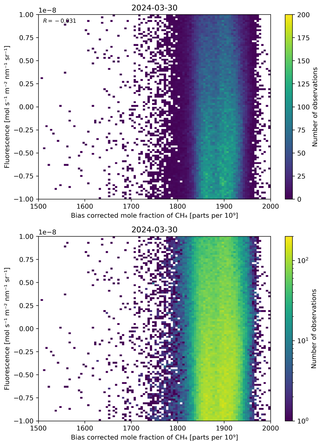
Figure 66: Scatter density plot of “Bias corrected mole fraction of \text{CH}_4 ” against “Fluorescence” for 2024-03-30 to 2024-03-31.
