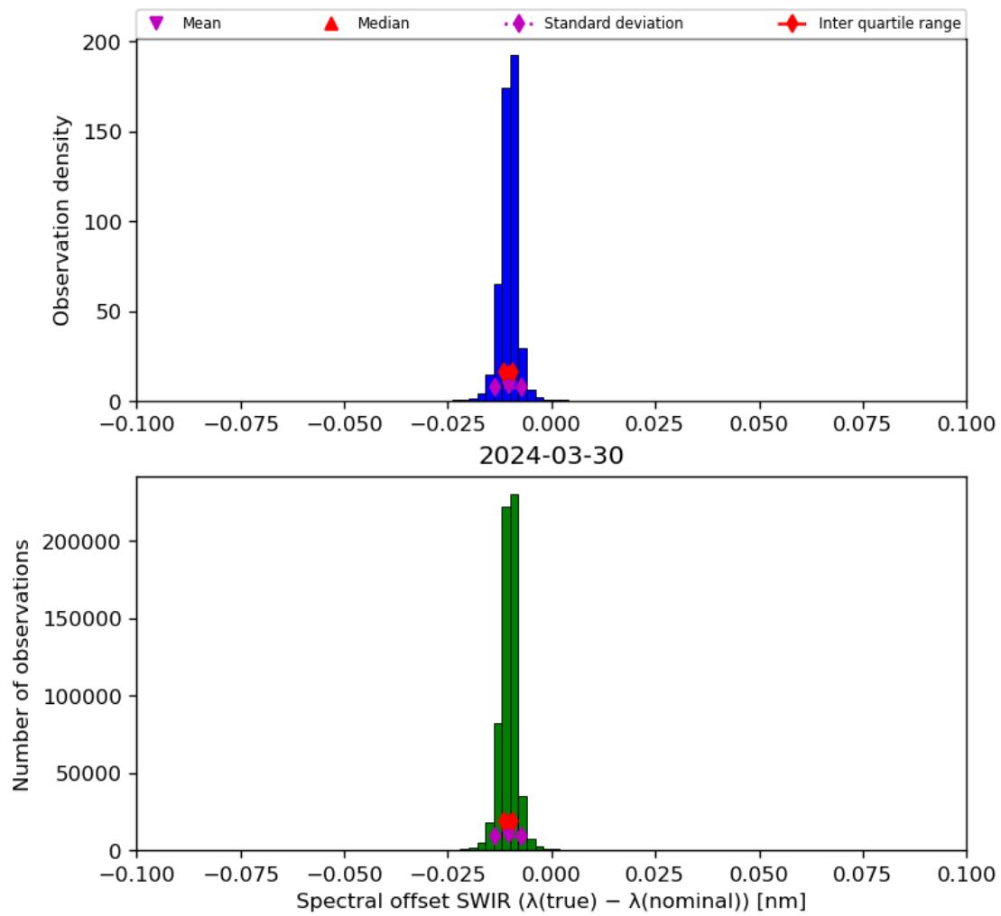
Figure 27: Histogram of “Spectral offset SWIR ( \lambda(\text{true}) - \lambda(\text{nominal}) )” for 2024-03-30 to 2024-03-31
