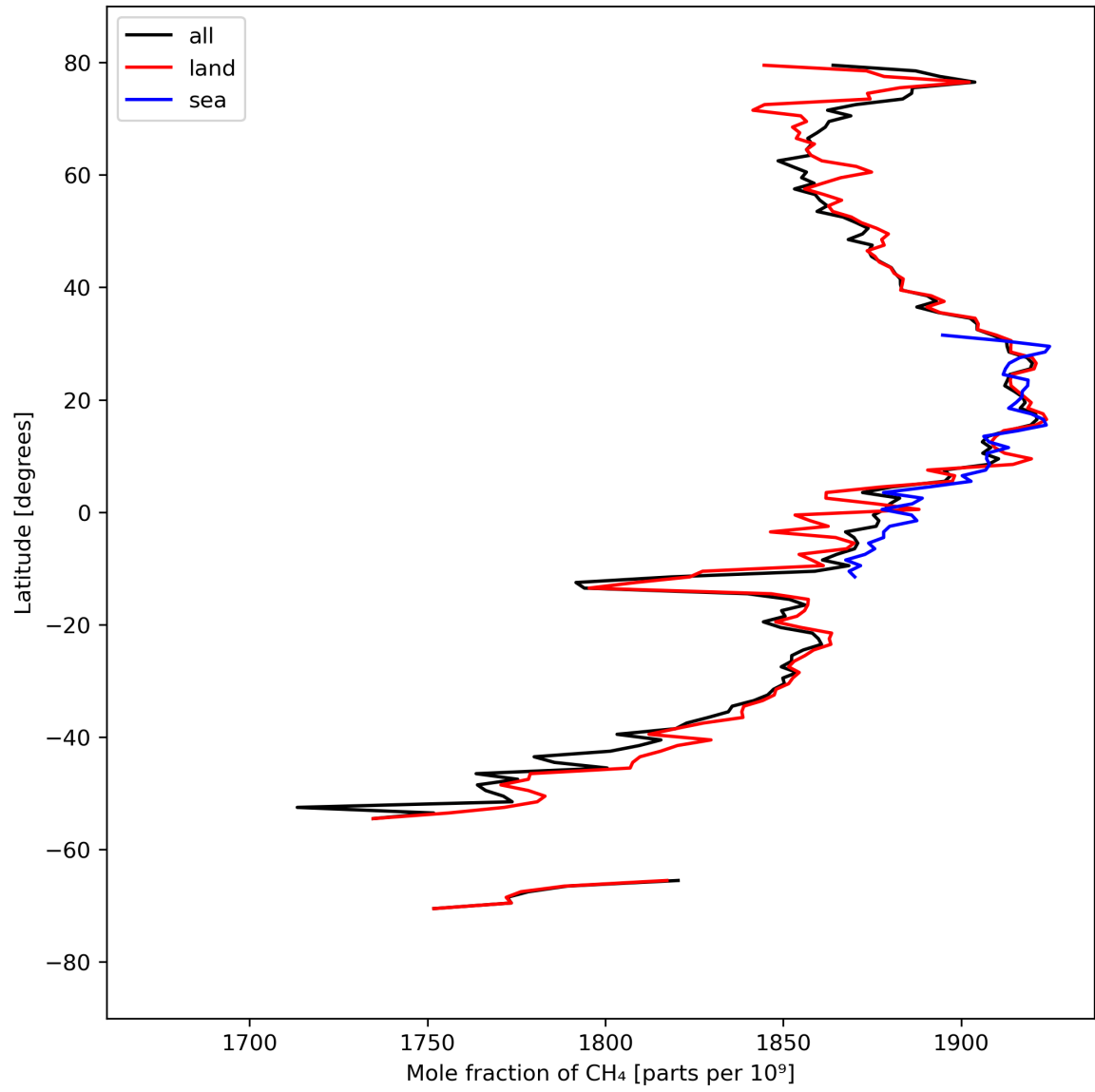
Figure 12: Zonal average of “Mole fraction of \text{CH}_4 ” for 2024-03-30 to 2024-03-31.
