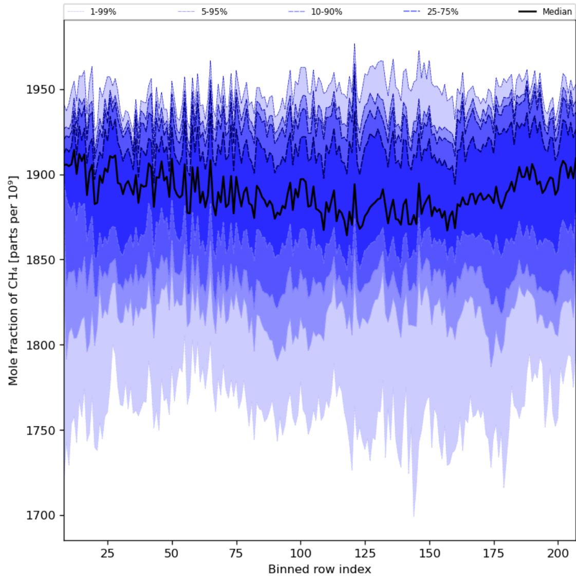
Figure 34: Along track statistics of “Mole fraction of CH 4 ” for 2024-03-30 to 2024-03-31
