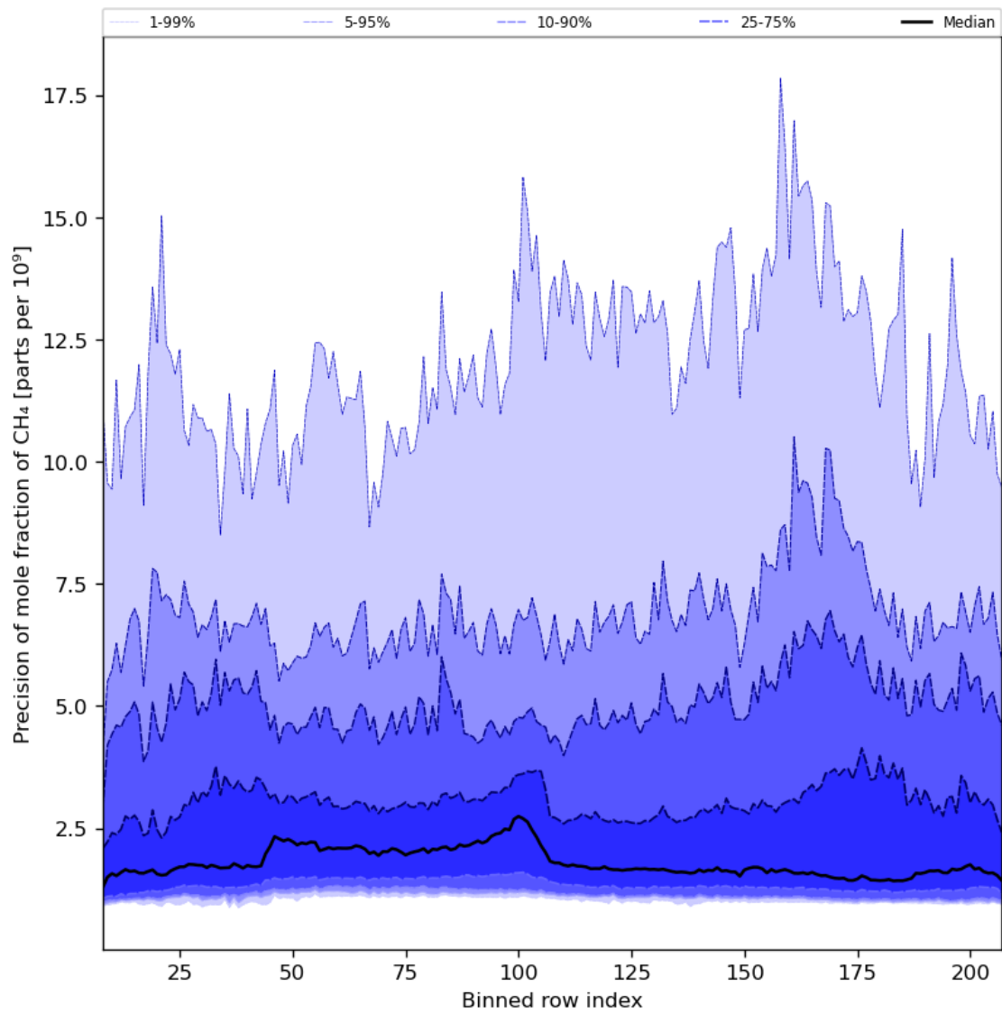
Figure 35: Along track statistics of “Precision of mole fraction of CH 4 ” for 2024-03-30 to 2024-03-31
