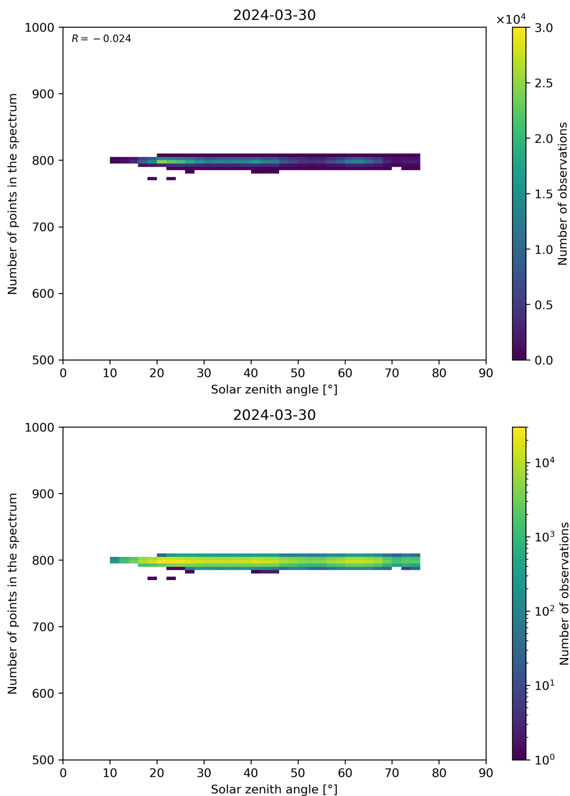
Figure 103: Scatter density plot of “Solar zenith angle” against “Number of points in the spectrum” for 2024-03-30 to 2024-03-31.
