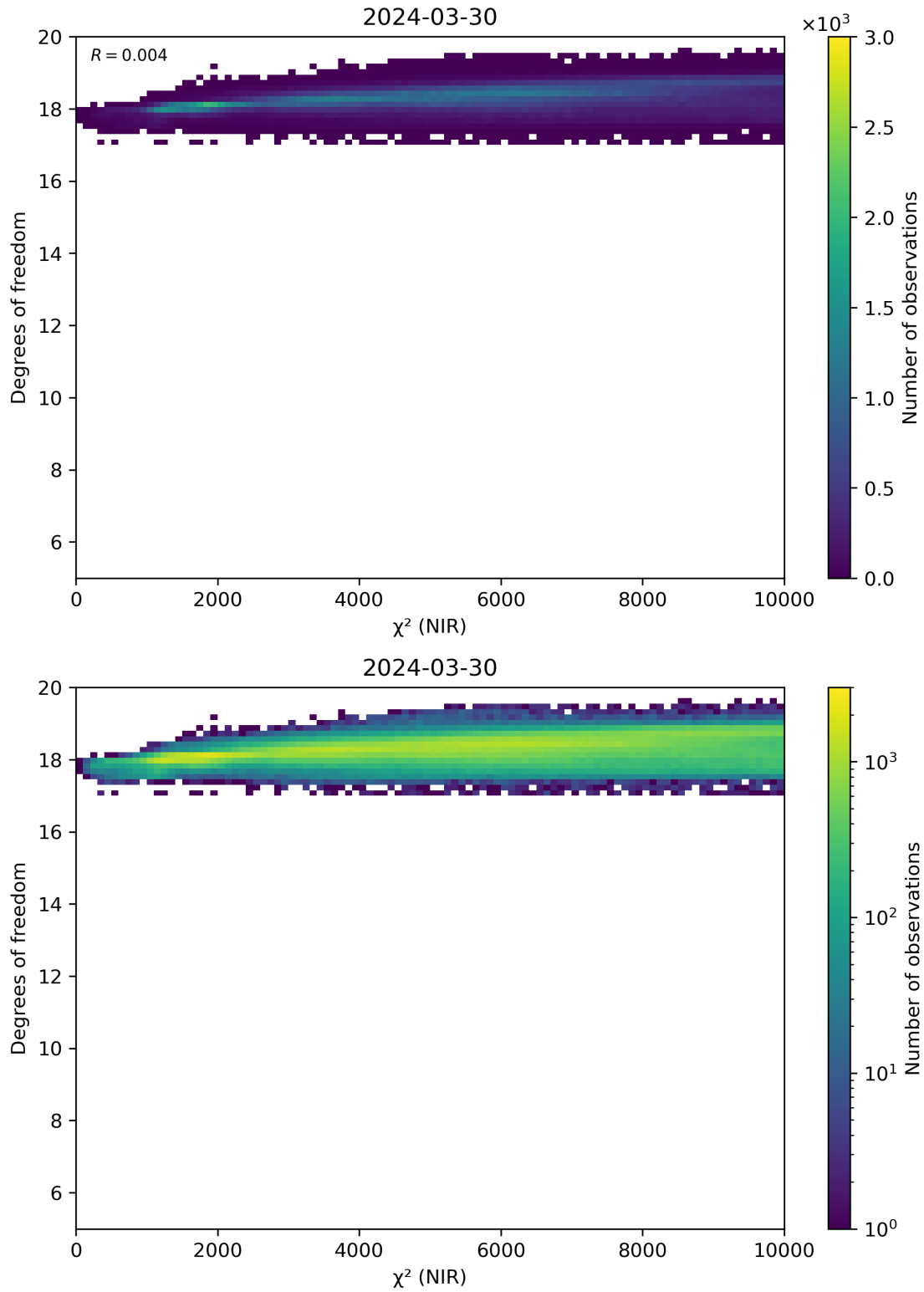
Figure 44: Scatter density plot of “ \chi^2 (NIR)” against “Degrees of freedom” for 2024-03-30 to 2024-03-31.
