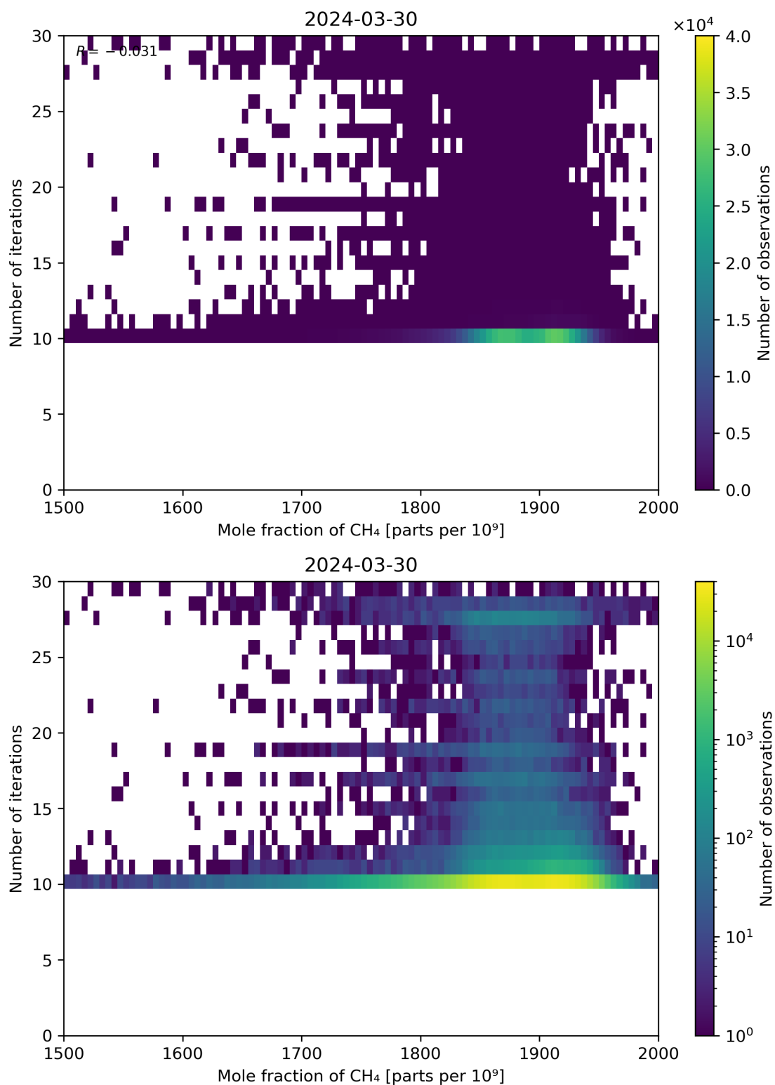
Figure 76: Scatter density plot of “Mole fraction of CH 4 ” against “Number of iterations” for 2024-03-30 to 2024-03-31.
