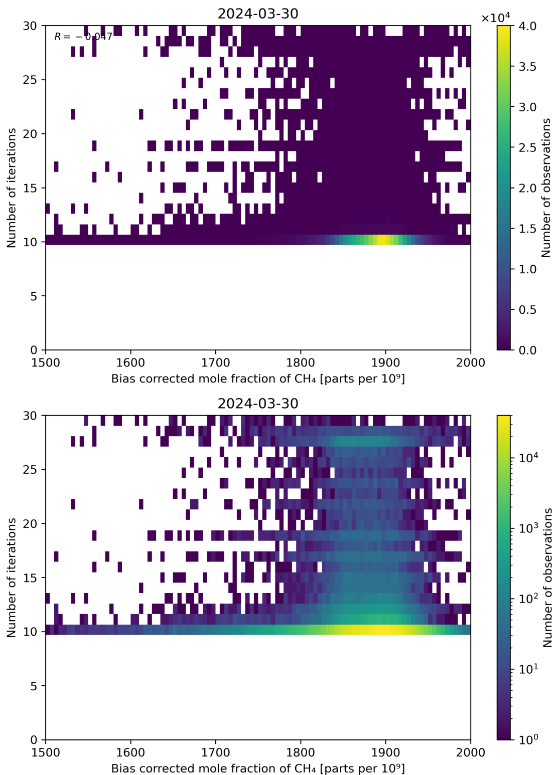
Figure 67: Scatter density plot of “Bias corrected mole fraction of CH 4 ” against “Number of iterations” for 2024-03-30 to 2024-03-31.
