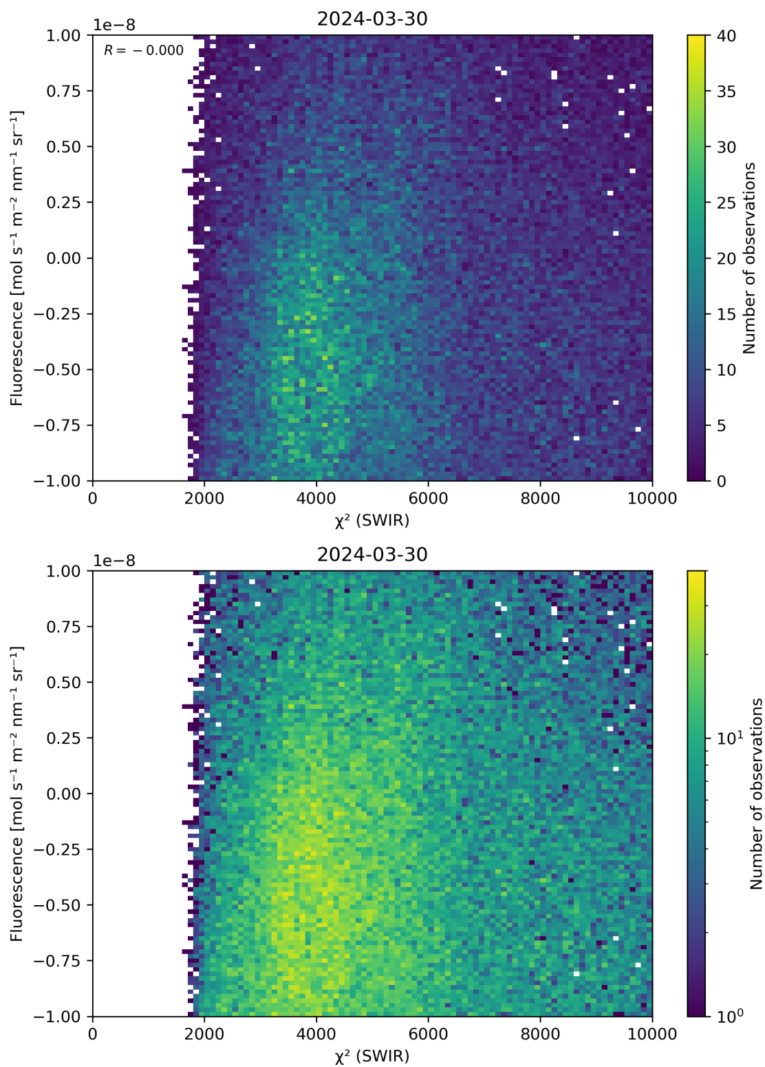
Figure 49: Scatter density plot of “ \chi^2 (SWIR)” against “Fluorescence” for 2024-03-30 to 2024-03-31.
