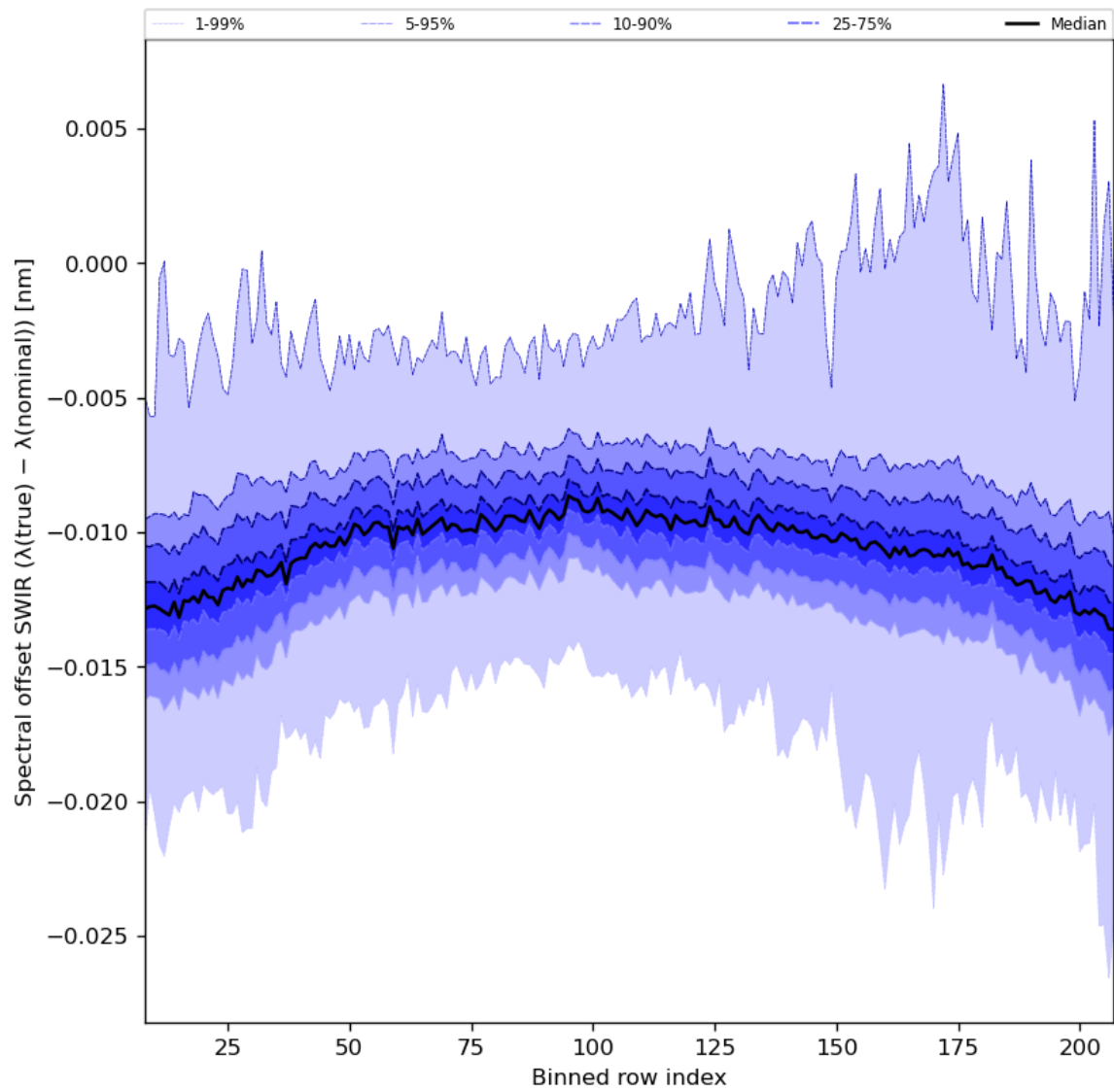
Figure 38: Along track statistics of “Spectral offset SWIR ( \lambda(\text{true}) - \lambda(\text{nominal}) )” for 2024-03-30 to 2024-03-31
