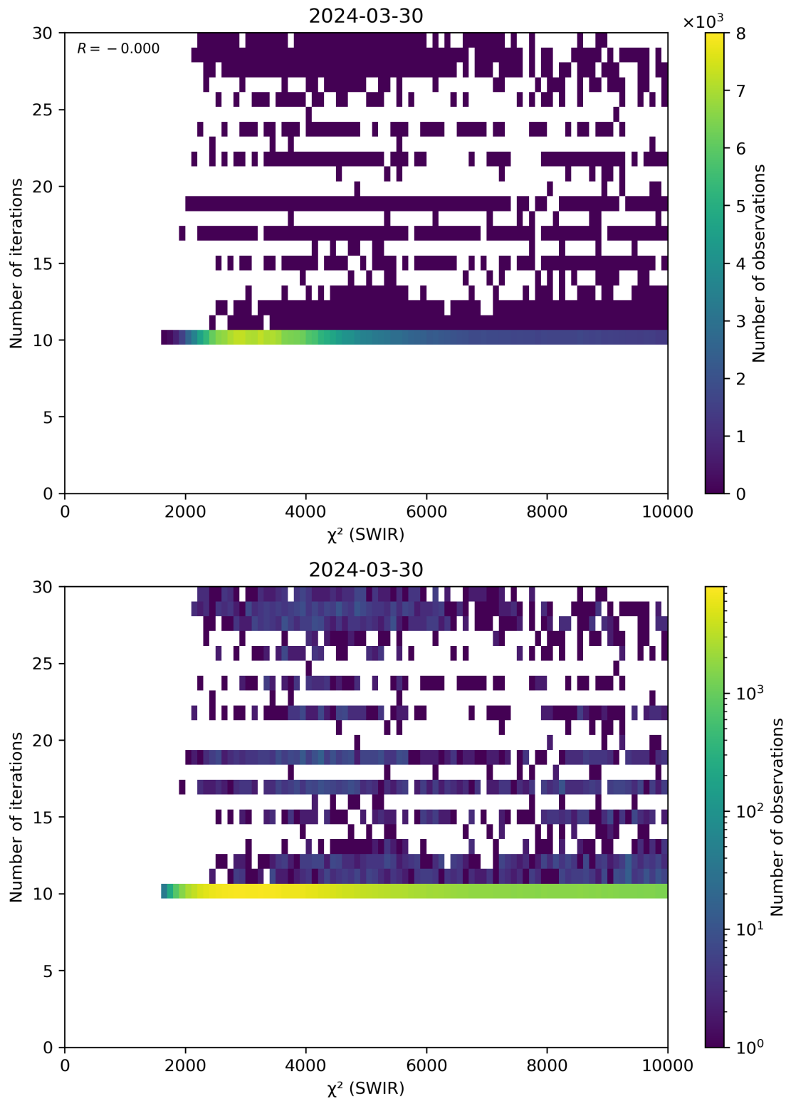
Figure 50: Scatter density plot of “ \chi^2 (SWIR)” against “Number of iterations” for 2024-03-30 to 2024-03-31.
