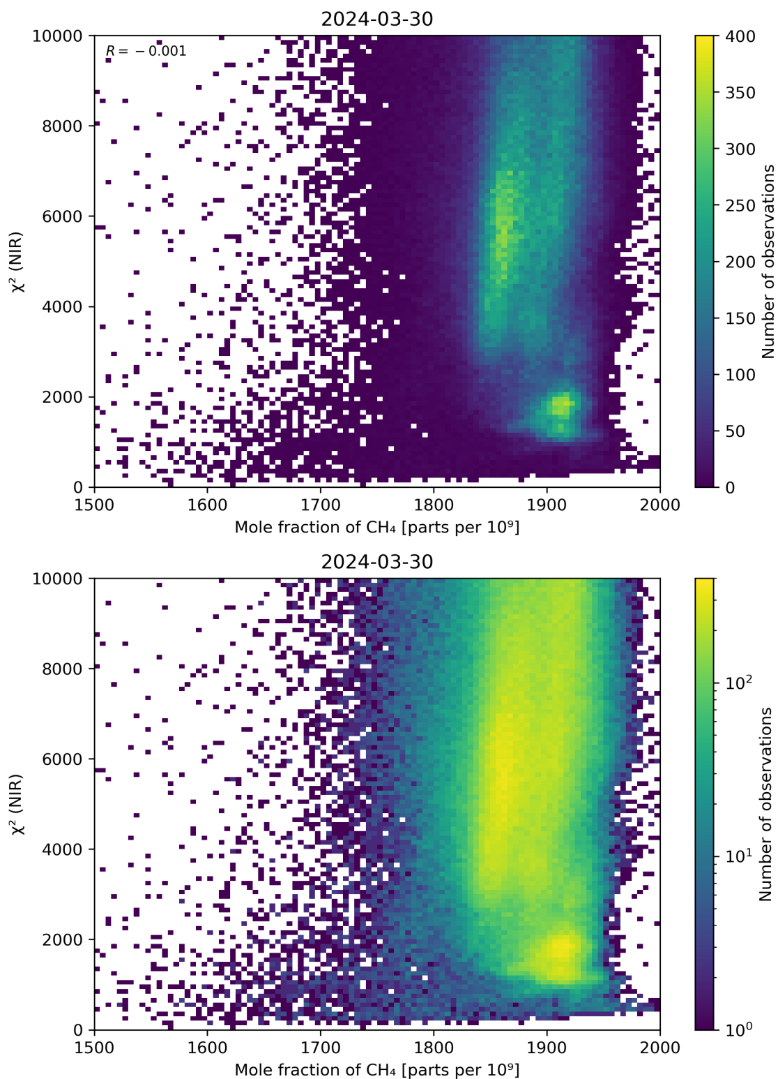
Figure 70: Scatter density plot of “Mole fraction of \text{CH}_4 ” against “ \chi^2 (NIR)” for 2024-03-30 to 2024-03-31.
