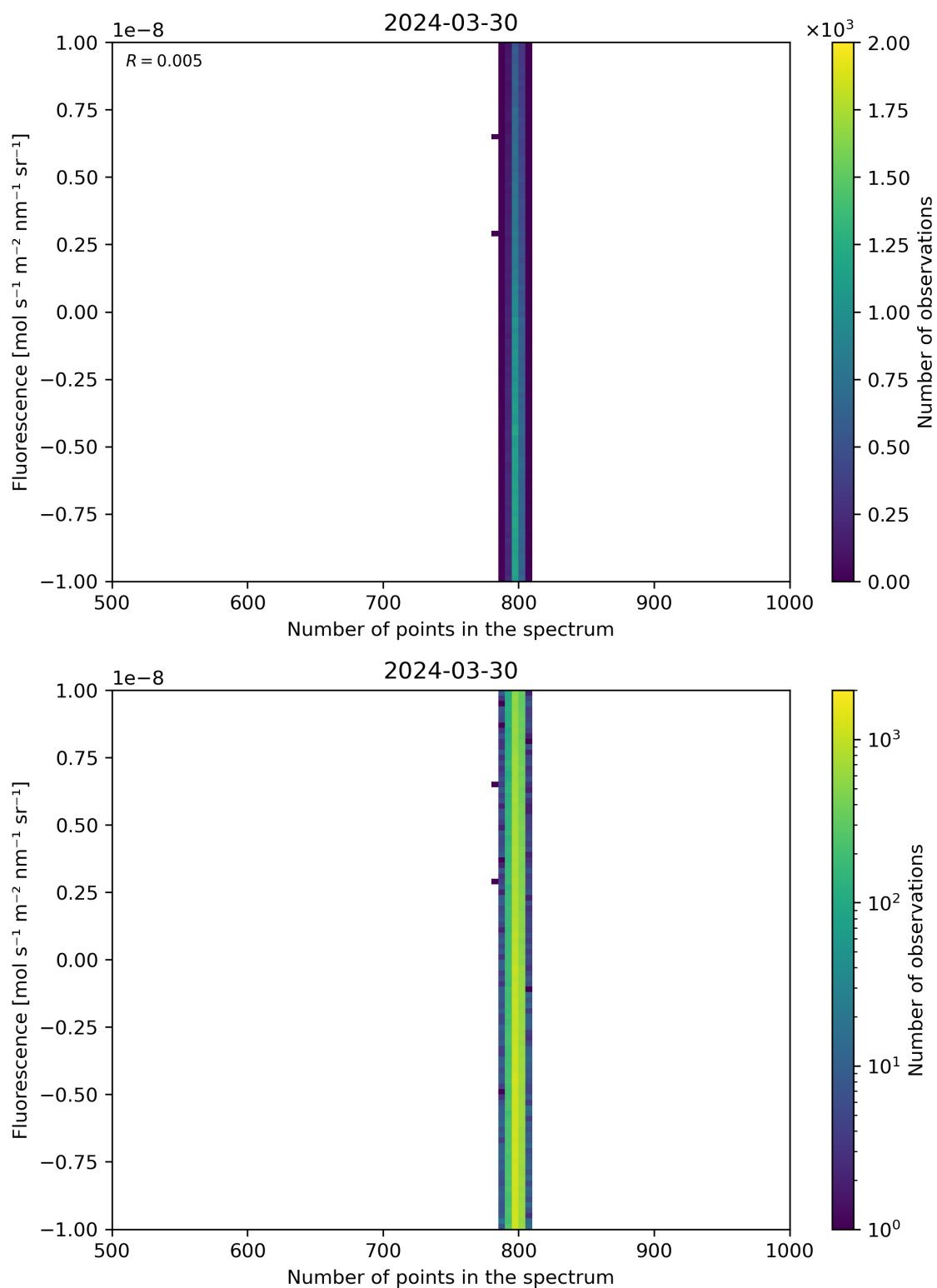
Figure 91: Scatter density plot of “Number of points in the spectrum” against “Fluorescence” for 2024-03-30 to 2024-03-31.
