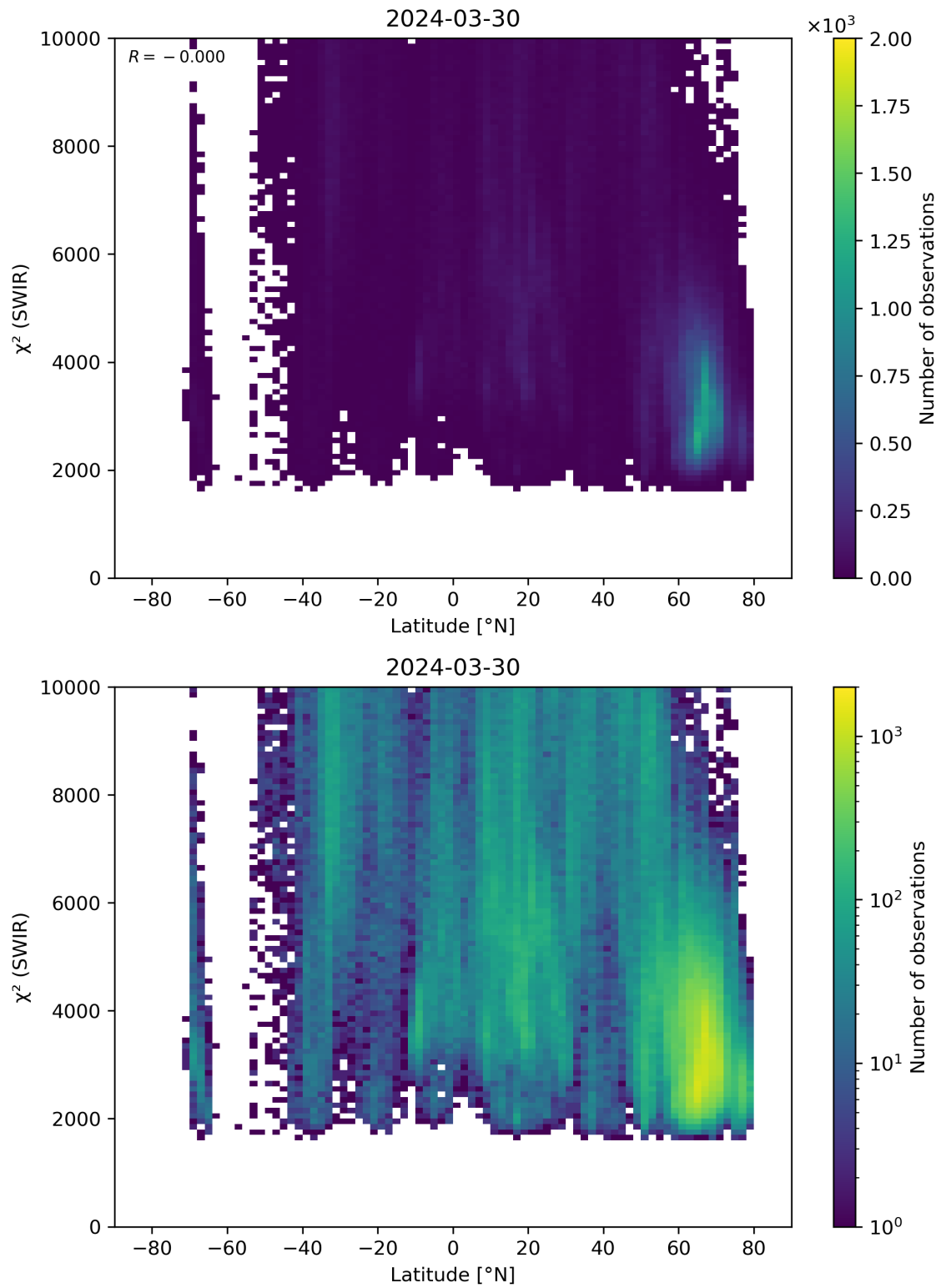
Figure 54: Scatter density plot of “Latitude” against “ \chi^2 (SWIR)” for 2024-03-30 to 2024-03-31.
