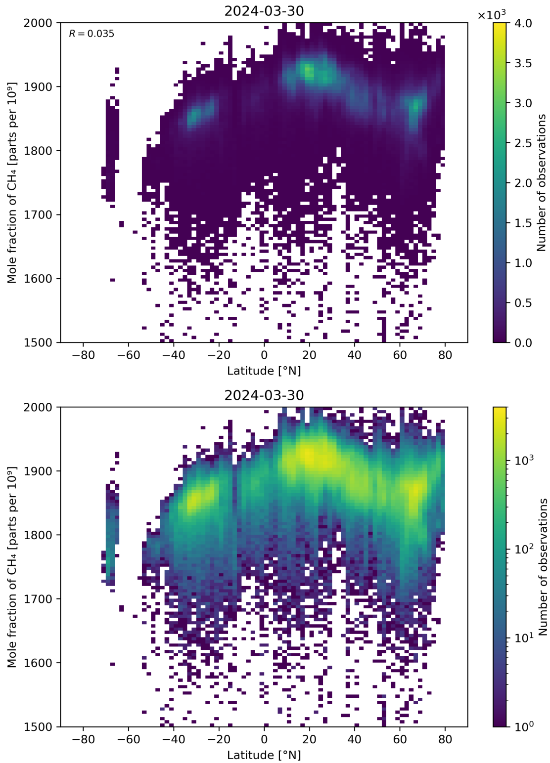
Figure 57: Scatter density plot of “Latitude” against “Mole fraction of CH 4 ” for 2024-03-30 to 2024-03-31.
