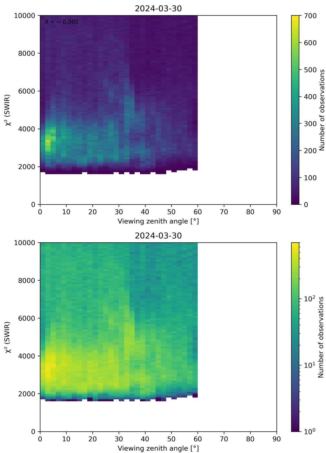
Figure 106: Scatter density plot of “Viewing zenith angle” against “ \chi^2 (SWIR)” for 2024-03-30 to 2024-03-31.
