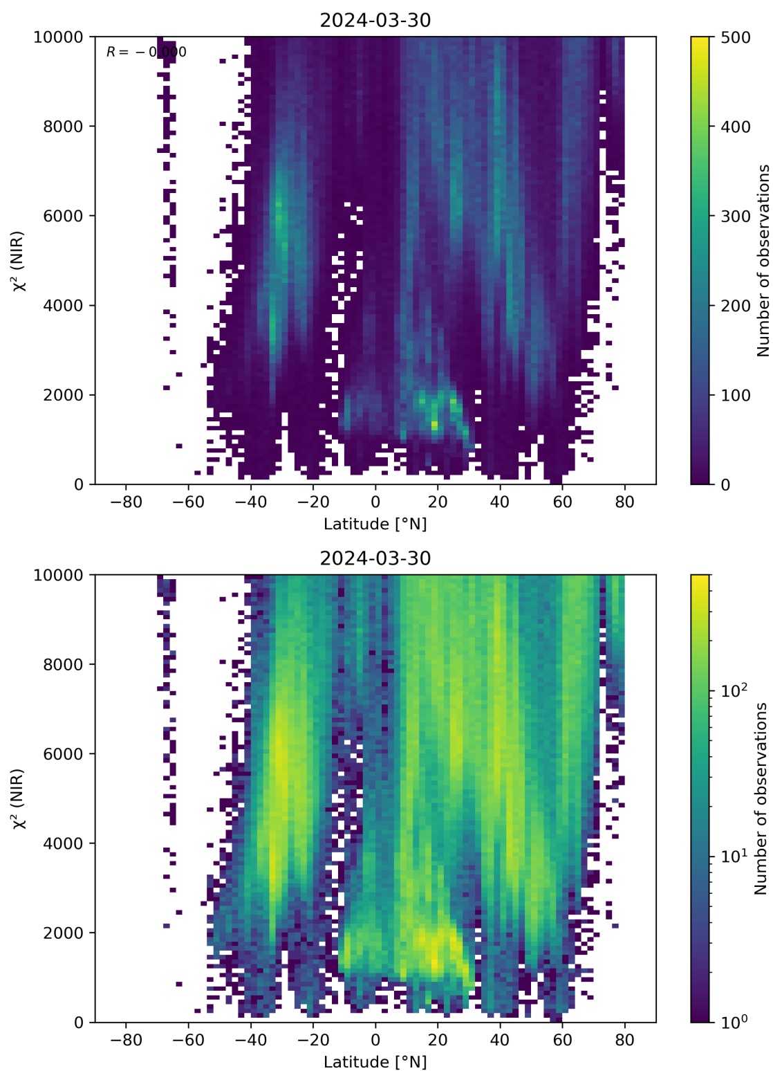
Figure 53: Scatter density plot of “Latitude” against “ \chi^2 (NIR)” for 2024-03-30 to 2024-03-31.
