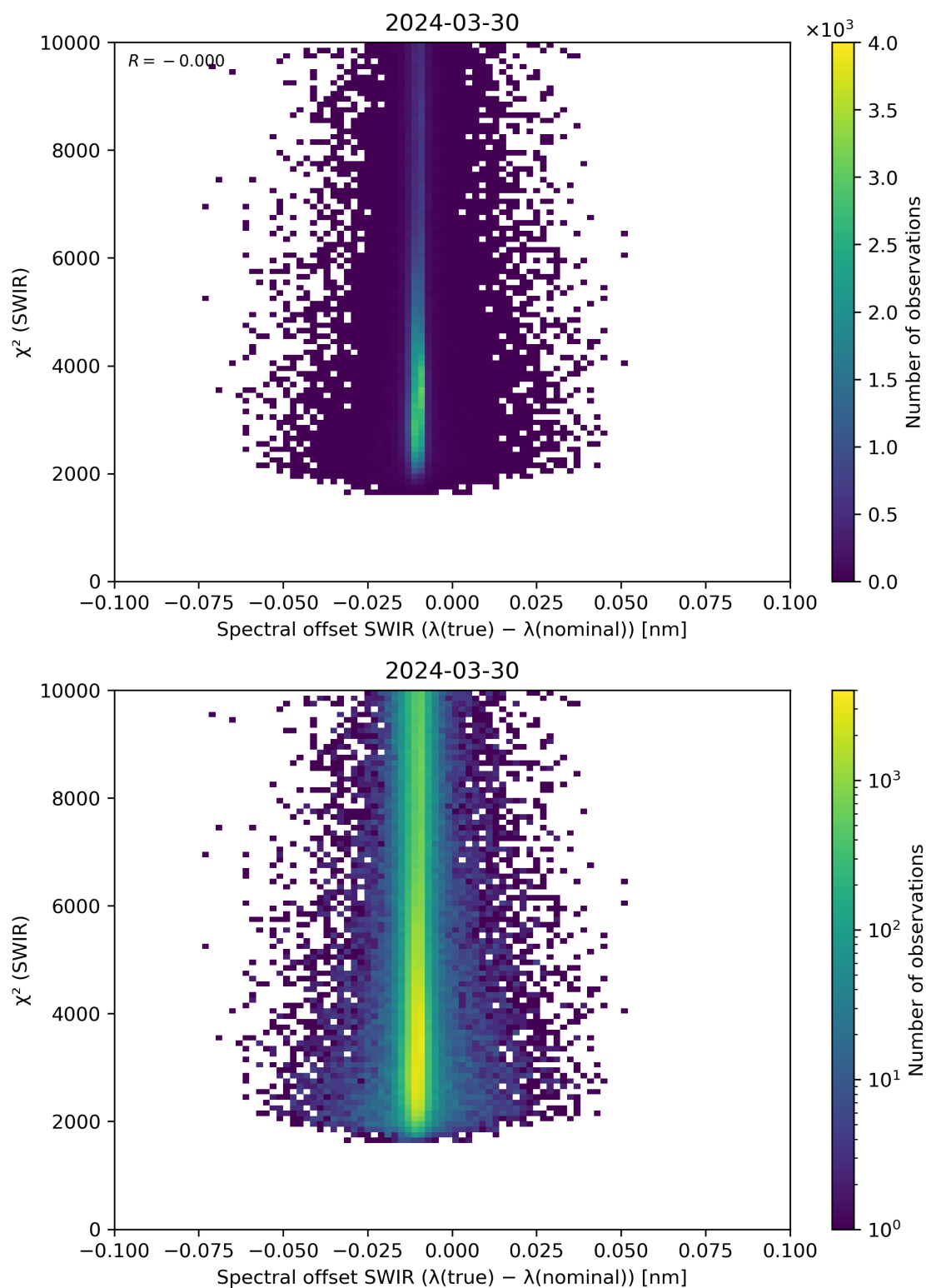
Figure 118: Scatter density plot of “Spectral offset SWIR ( \lambda(\text{true}) - \lambda(\text{nominal}) )” against “ \chi^2 (SWIR)” for 2024-03-30 to 2024-03-31.
