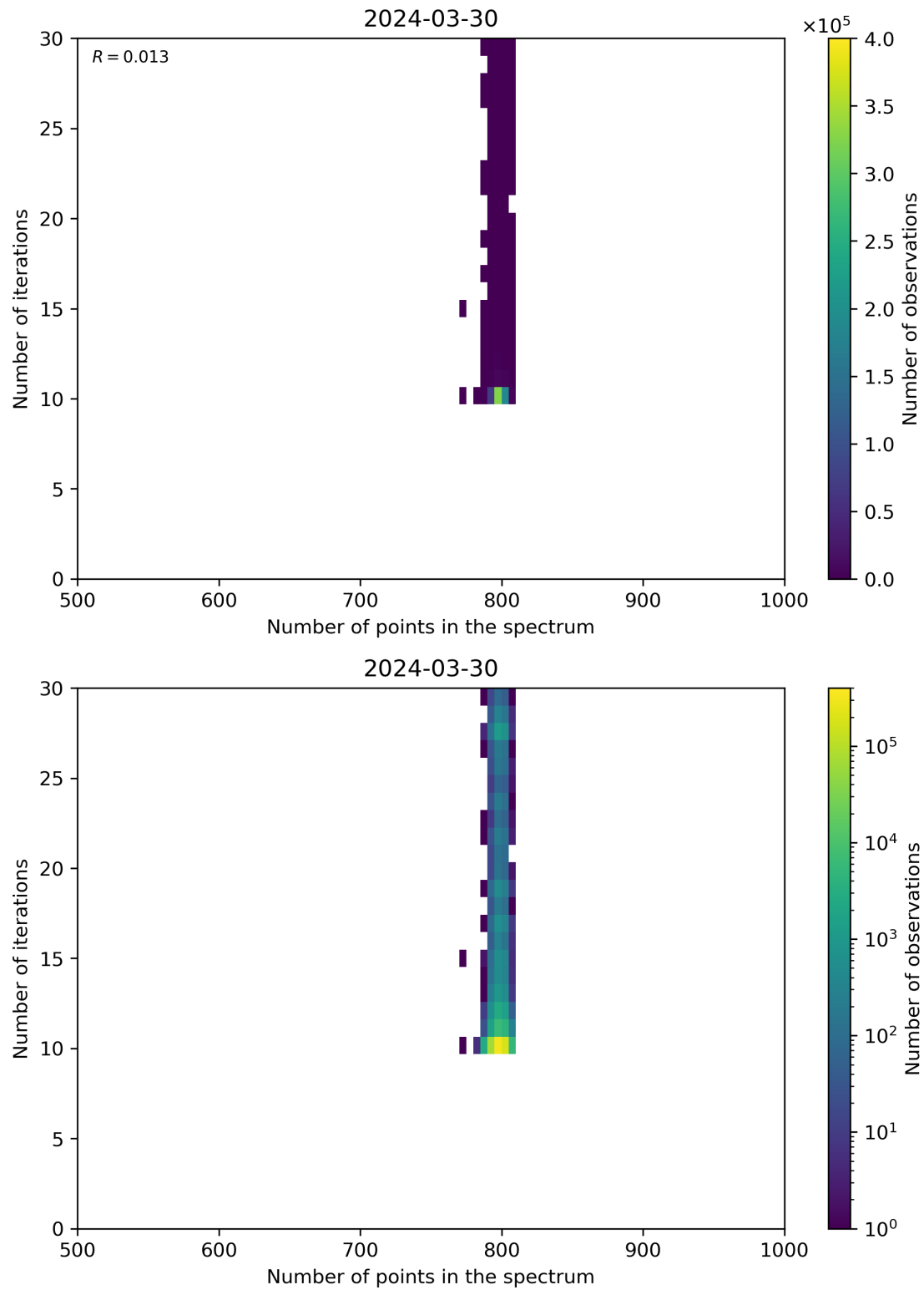
Figure 92: Scatter density plot of “Number of points in the spectrum” against “Number of iterations” for 2024-03-30 to 2024-03-31.
