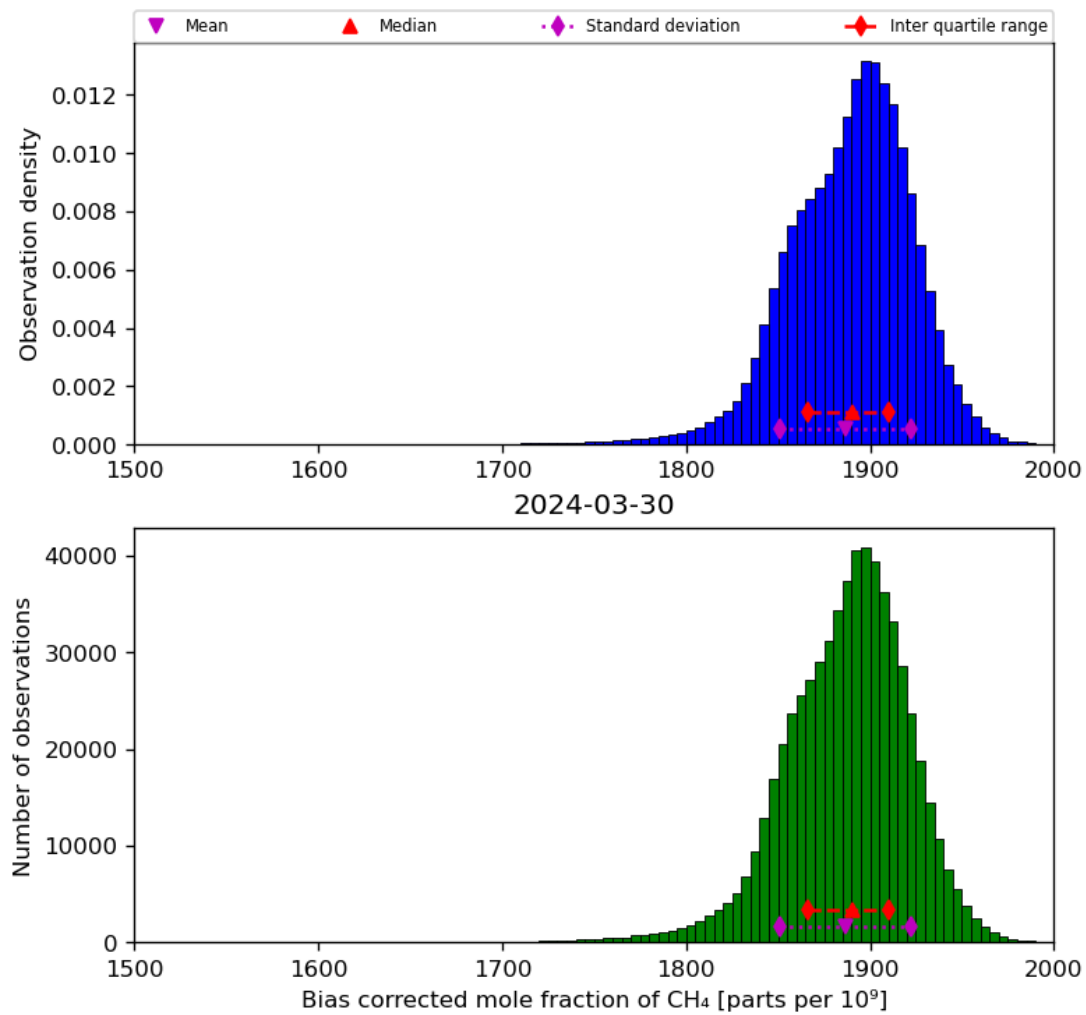
Figure 25: Histogram of “Bias corrected mole fraction of CH 4 ” for 2024-03-30 to 2024-03-31
