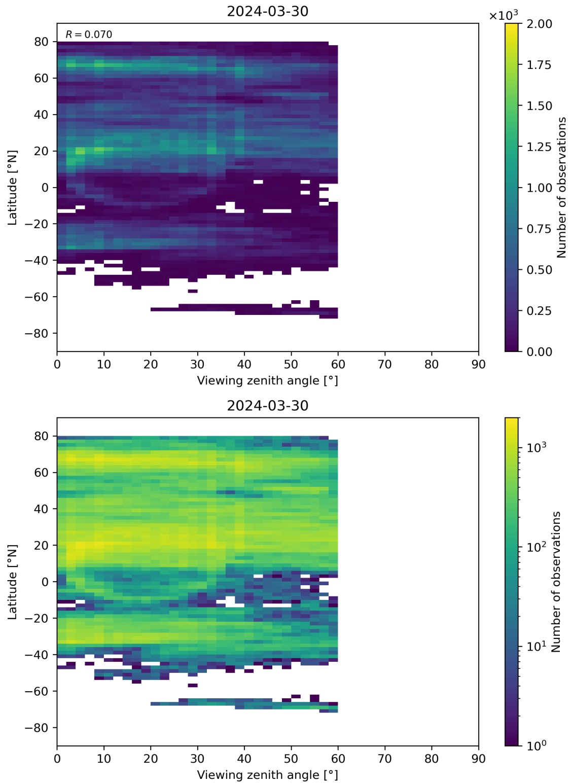
Figure 109: Scatter density plot of “Viewing zenith angle” against “Latitude” for 2024-03-30 to 2024-03-31.
