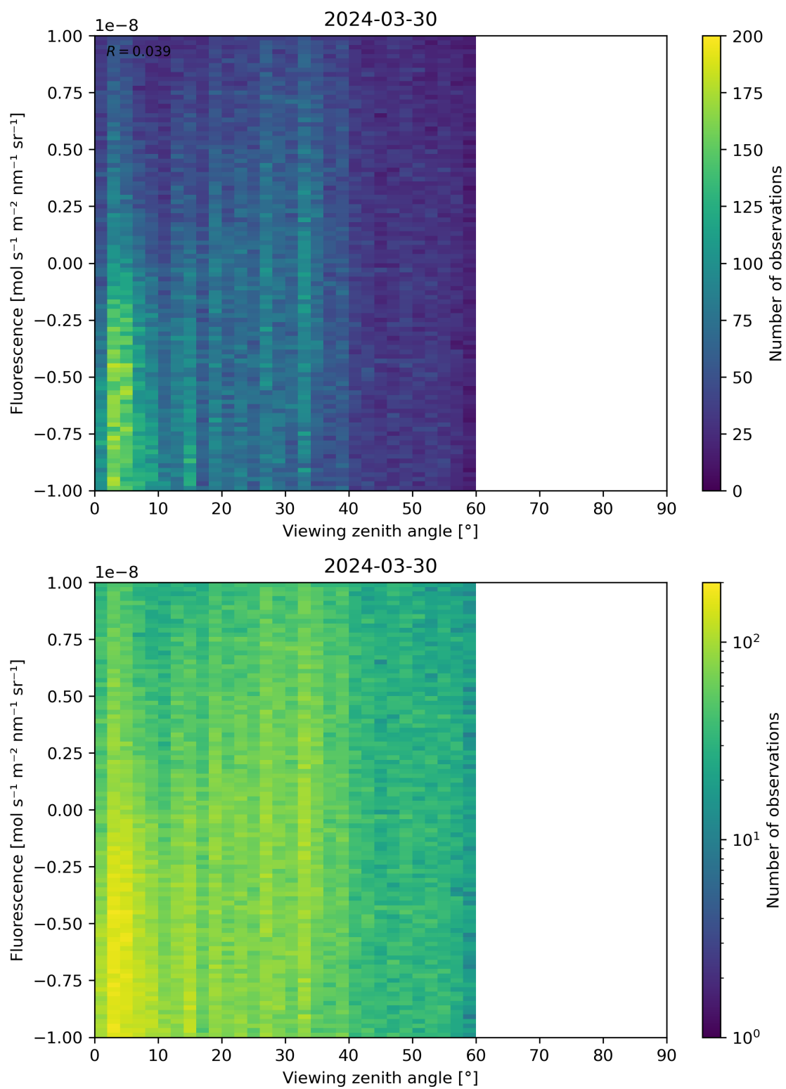
Figure 108: Scatter density plot of “Viewing zenith angle” against “Fluorescence” for 2024-03-30 to 2024-03-31.
