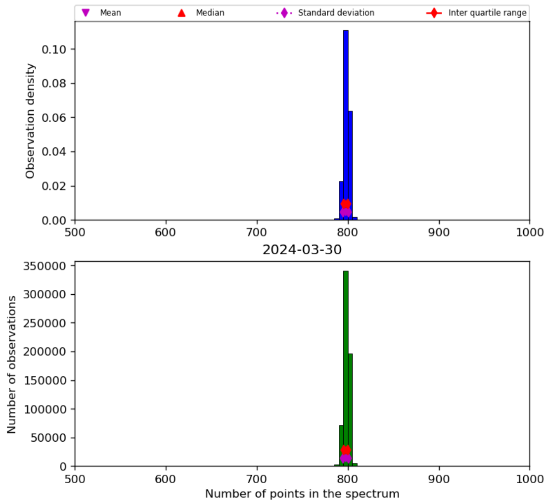
Figure 26: Histogram of “Number of points in the spectrum” for 2024-03-30 to 2024-03-31
