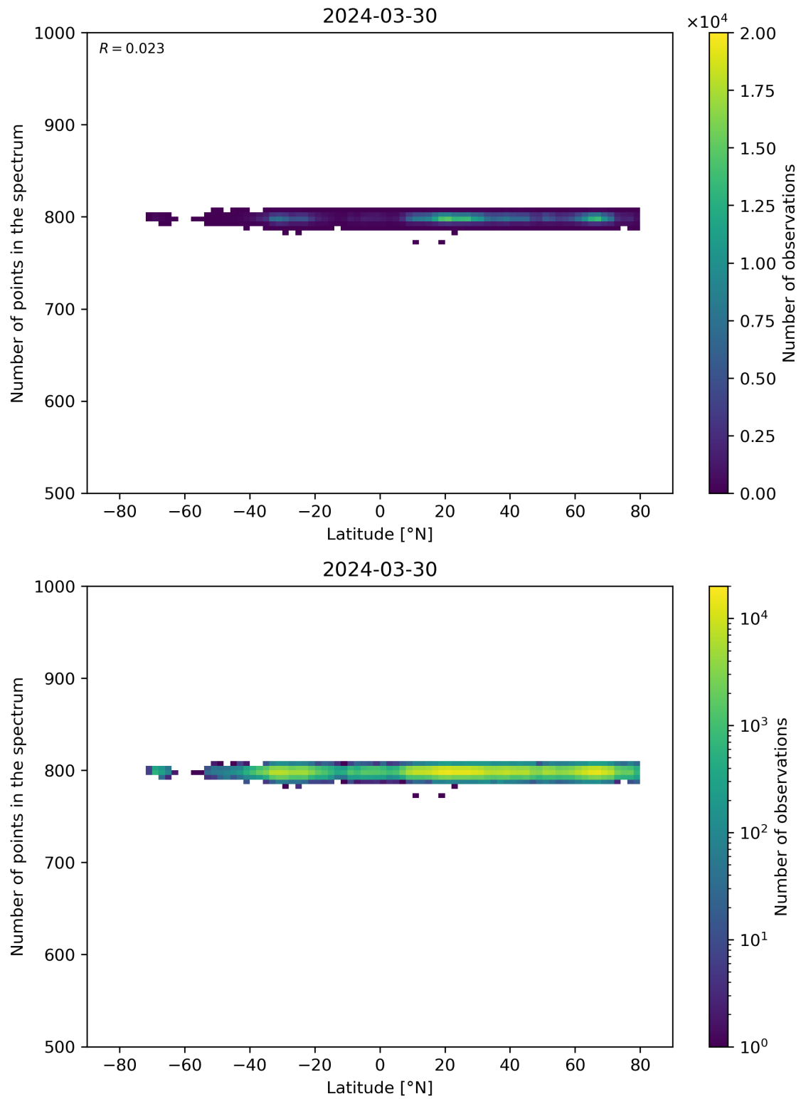
Figure 61: Scatter density plot of “Latitude” against “Number of points in the spectrum” for 2024-03-30 to 2024-03-31.
