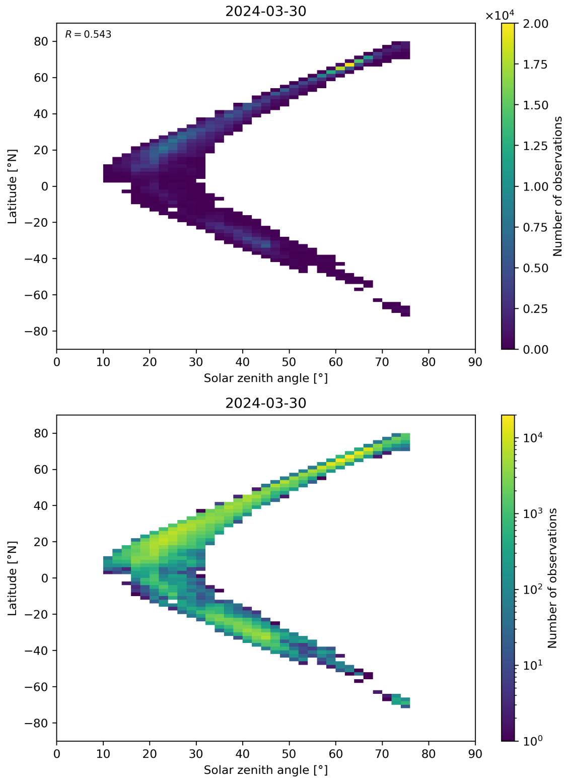
Figure 98: Scatter density plot of “Solar zenith angle” against “Latitude” for 2024-03-30 to 2024-03-31.
