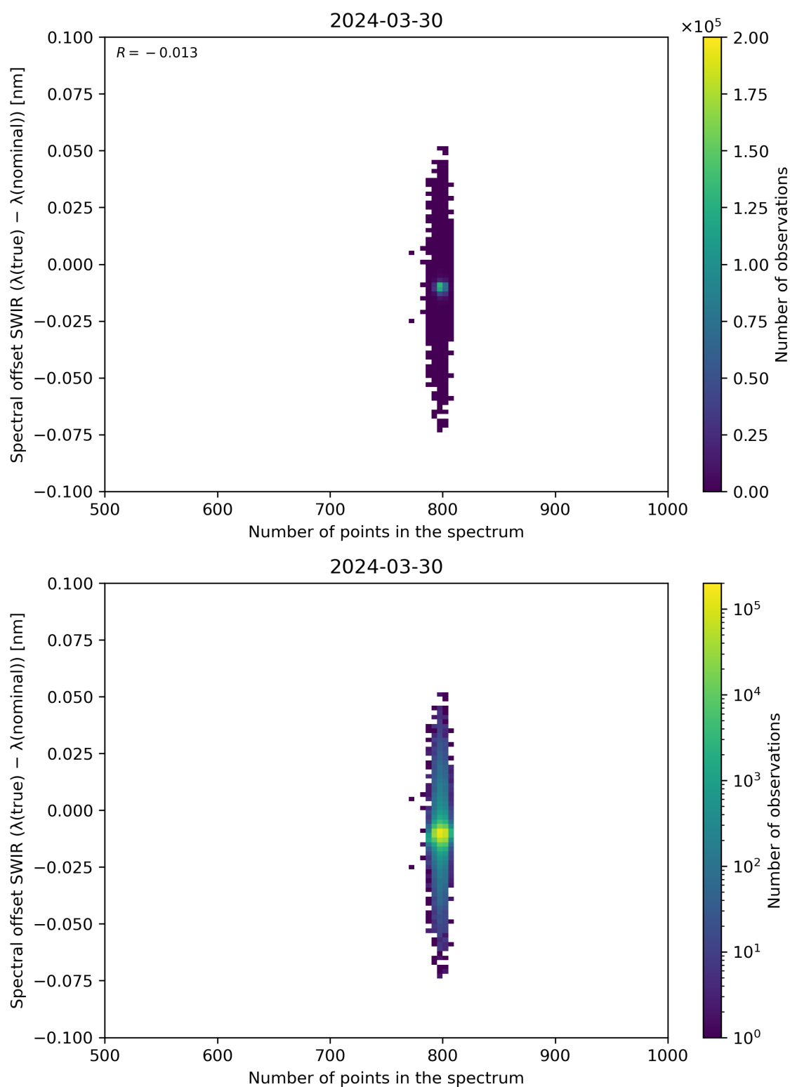
Figure 93: Scatter density plot of “Number of points in the spectrum” against “Spectral offset SWIR ( \lambda(\text{true}) - \lambda(\text{nominal}) )” for 2024-03-30 to 2024-03-31.
