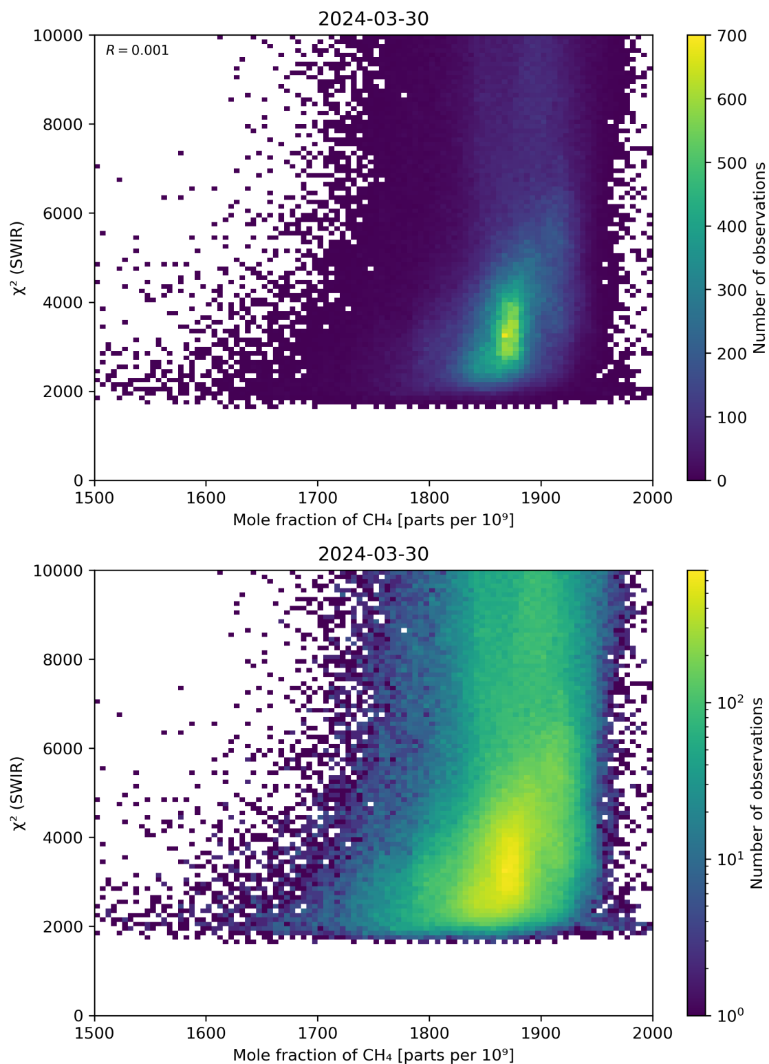
Figure 71: Scatter density plot of “Mole fraction of \text{CH}_4 ” against “ \chi^2 (SWIR)” for 2024-03-30 to 2024-03-31.
