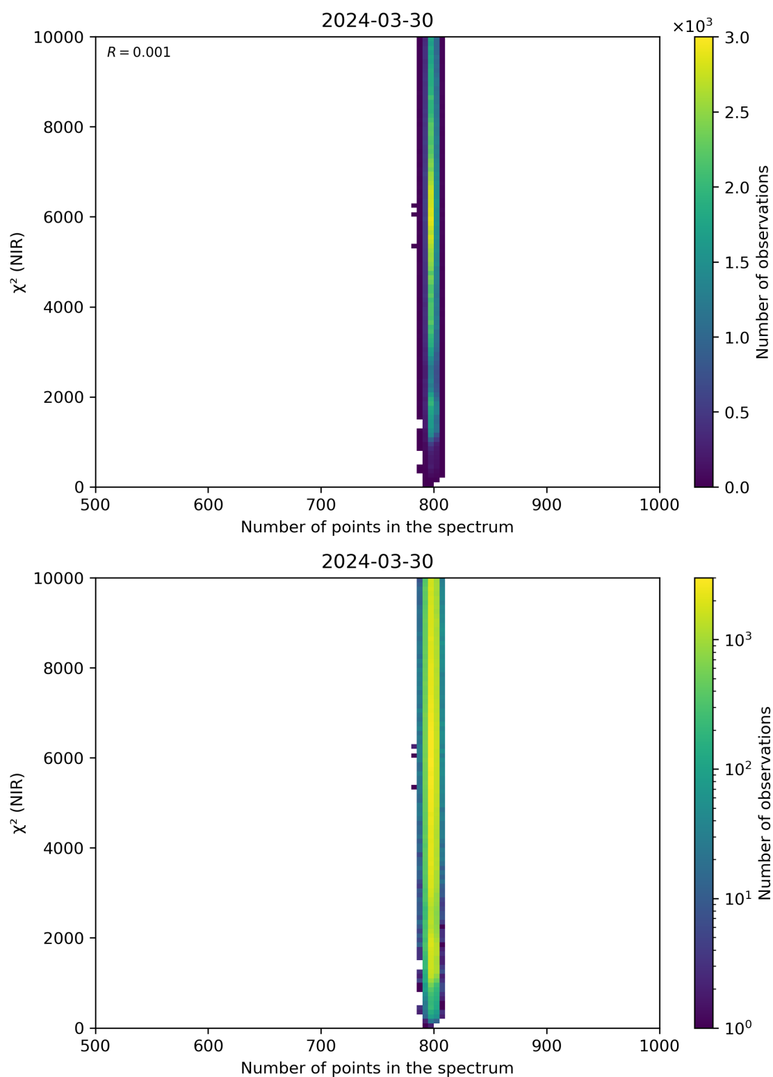
Figure 88: Scatter density plot of “Number of points in the spectrum” against “ \chi^2 (NIR)” for 2024-03-30 to 2024-03-31.
