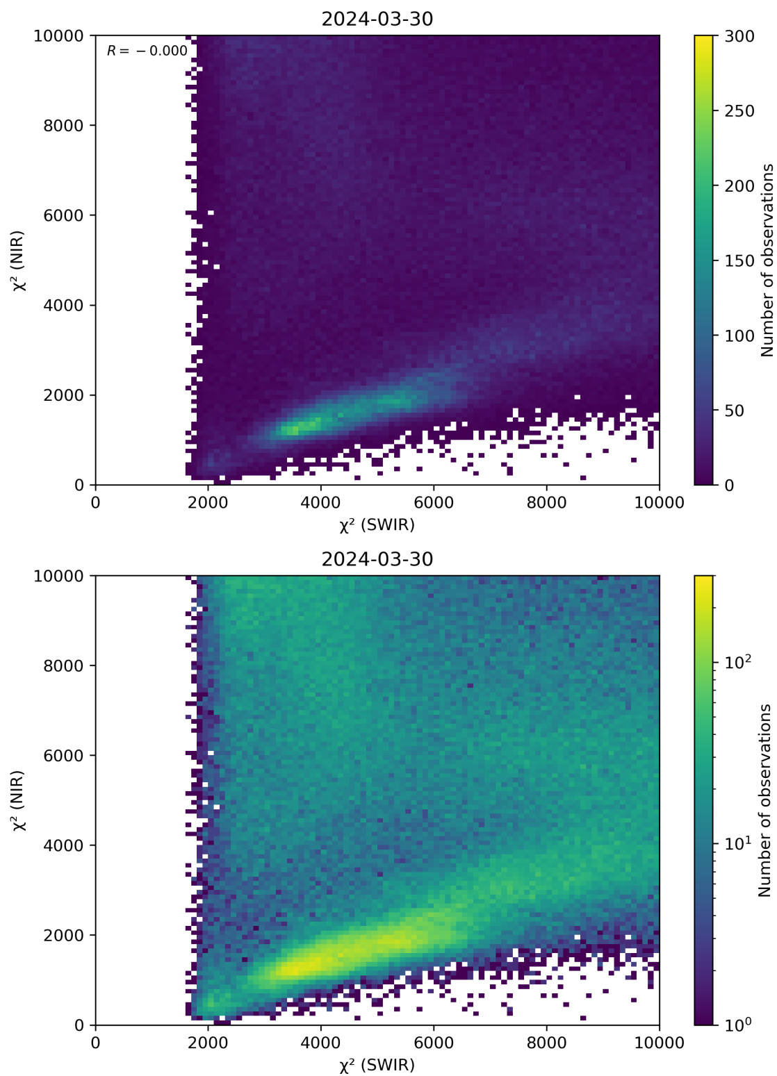
Figure 47: Scatter density plot of “ \chi^2 (SWIR)” against “ \chi^2 (NIR)” for 2024-03-30 to 2024-03-31.
