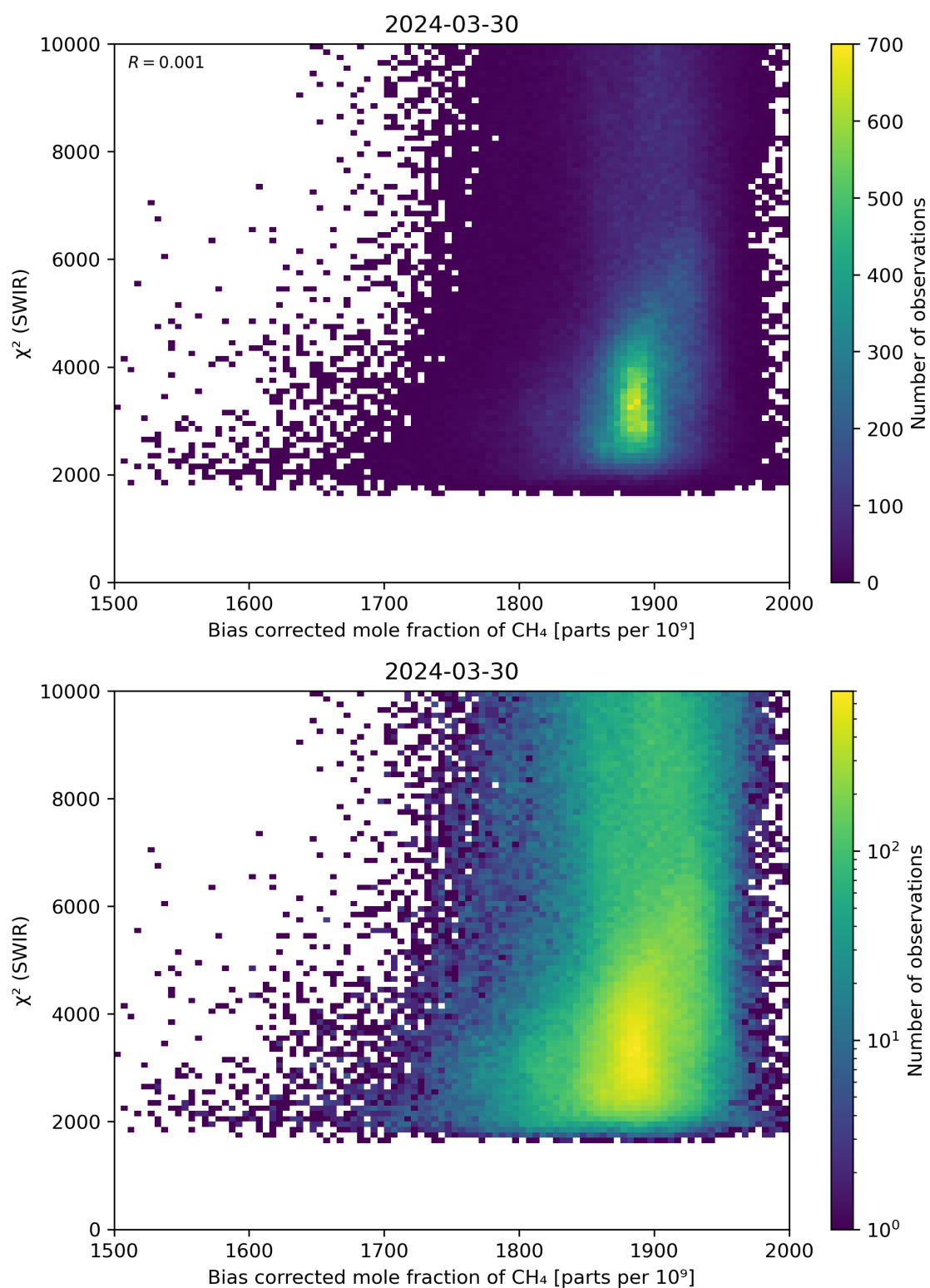
Figure 64: Scatter density plot of “Bias corrected mole fraction of CH 4 ” against “ \chi^2 (SWIR)” for 2024-03-30 to 2024-03-31.
