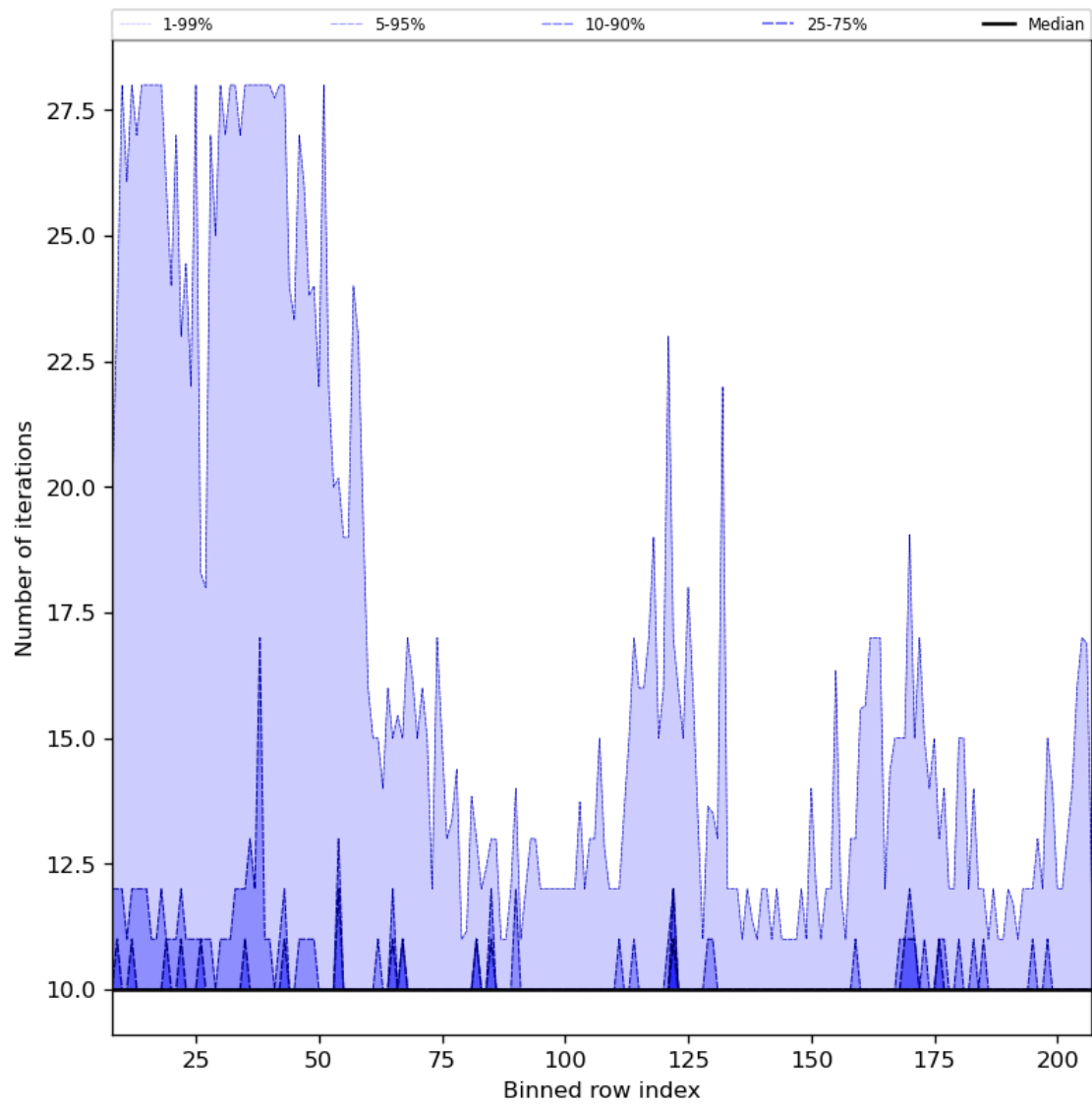
Figure 42: Along track statistics of “Number of iterations” for 2024-03-30 to 2024-03-31
