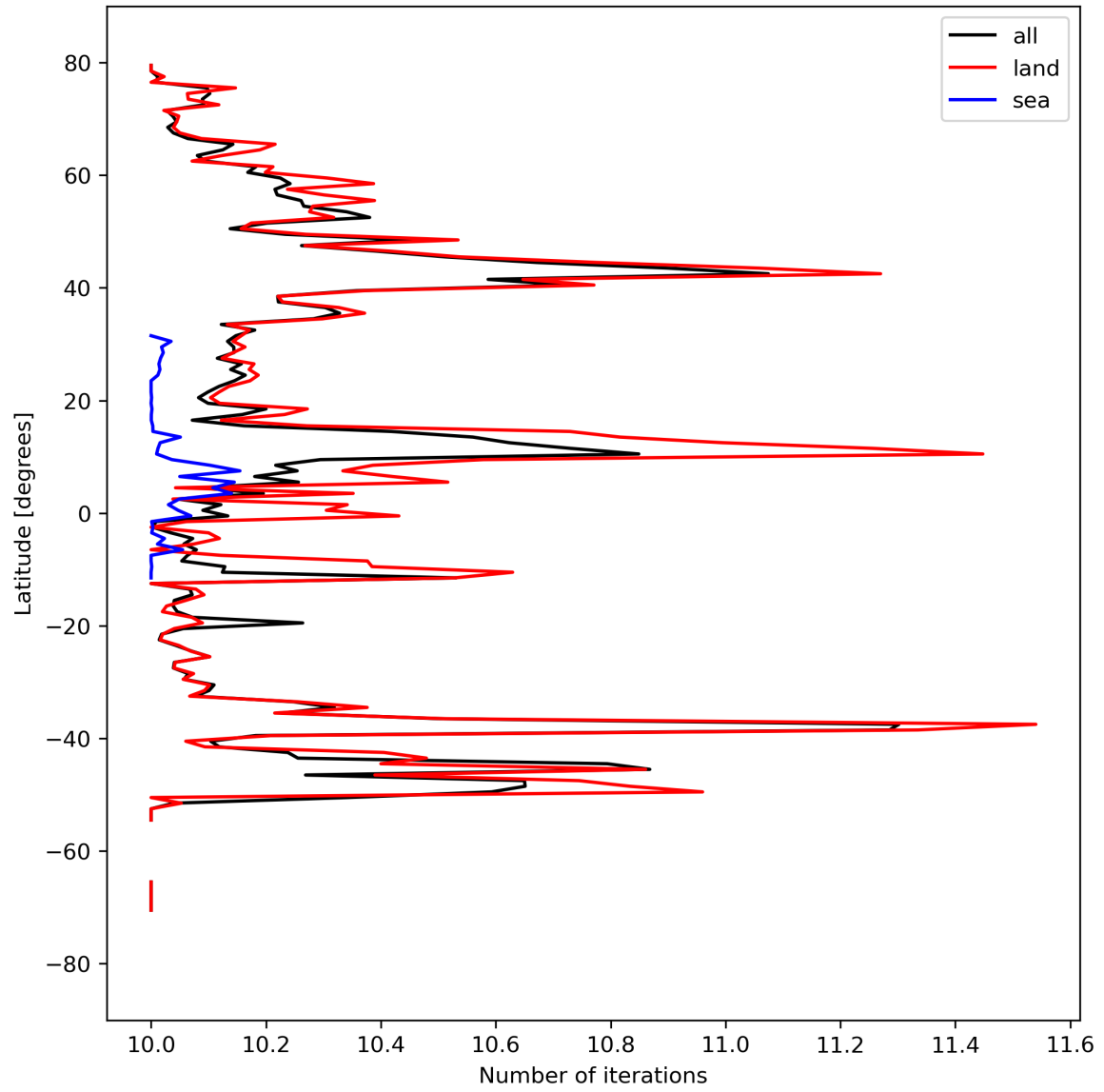
Figure 20: Zonal average of “Number of iterations” for 2024-03-30 to 2024-03-31.
