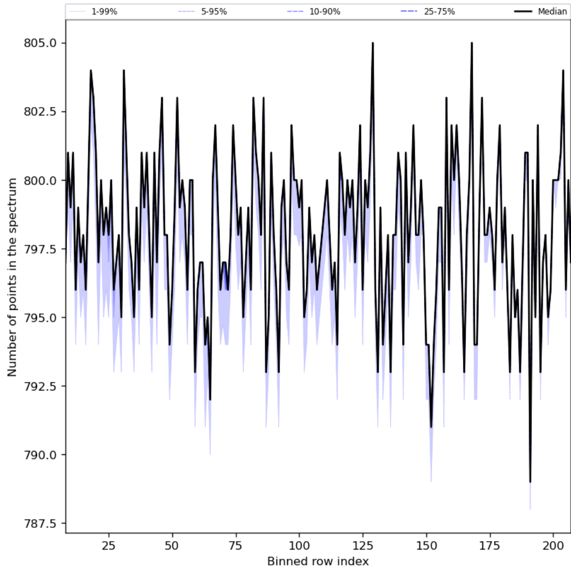
Figure 37: Along track statistics of “Number of points in the spectrum” for 2024-03-30 to 2024-03-31
