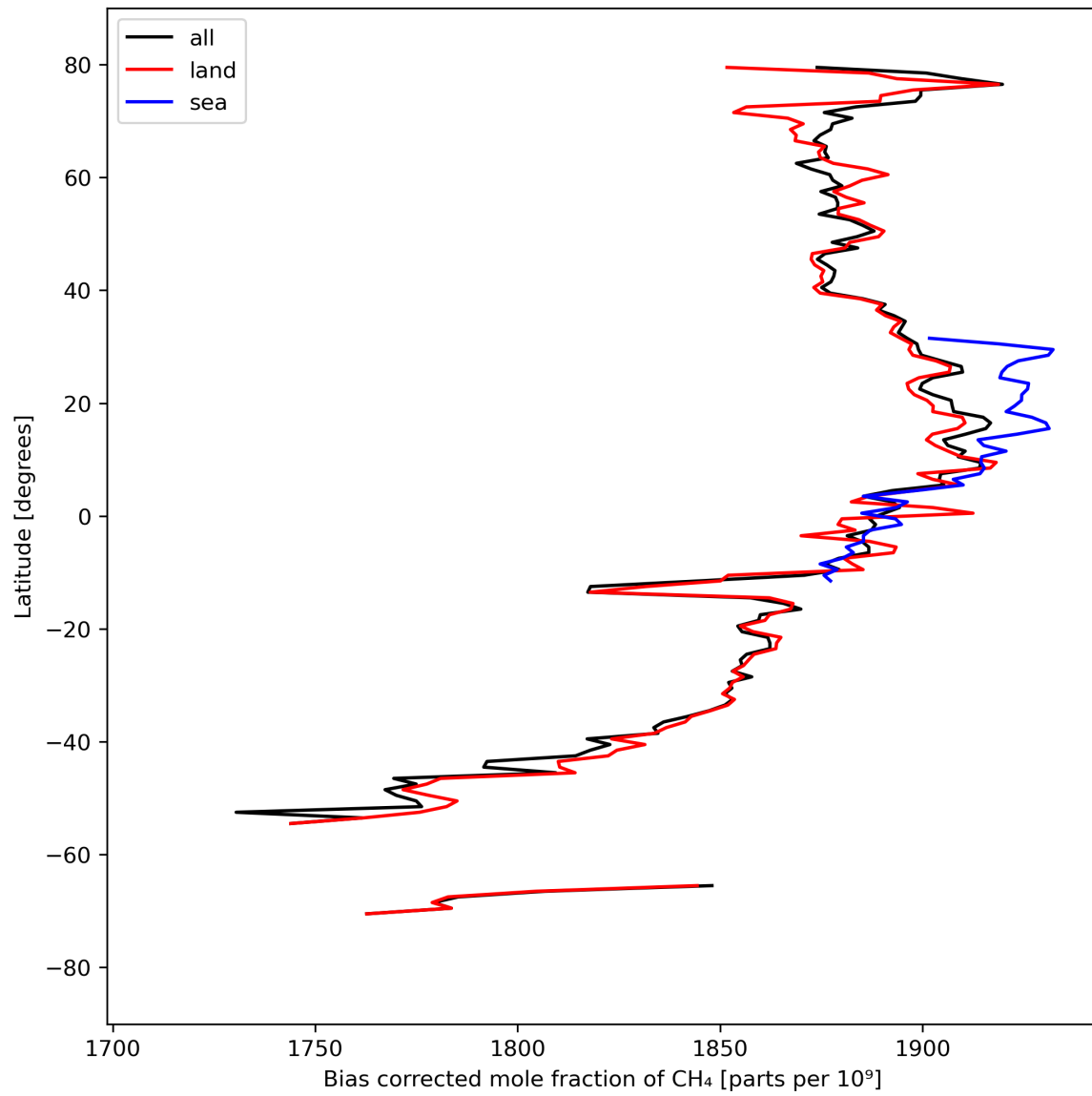
Figure 14: Zonal average of “Bias corrected mole fraction of CH 4 ” for 2024-03-30 to 2024-03-31.
