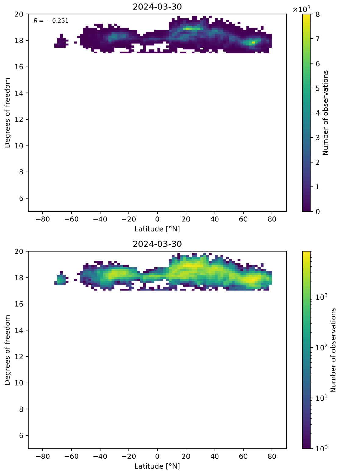
Figure 55: Scatter density plot of “Latitude” against “Degrees of freedom” for 2024-03-30 to 2024-03-31.
