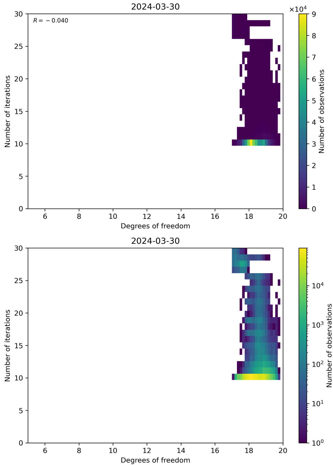
Figure 52: Scatter density plot of “Degrees of freedom” against “Number of iterations” for 2024-03-30 to 2024-03-31.
