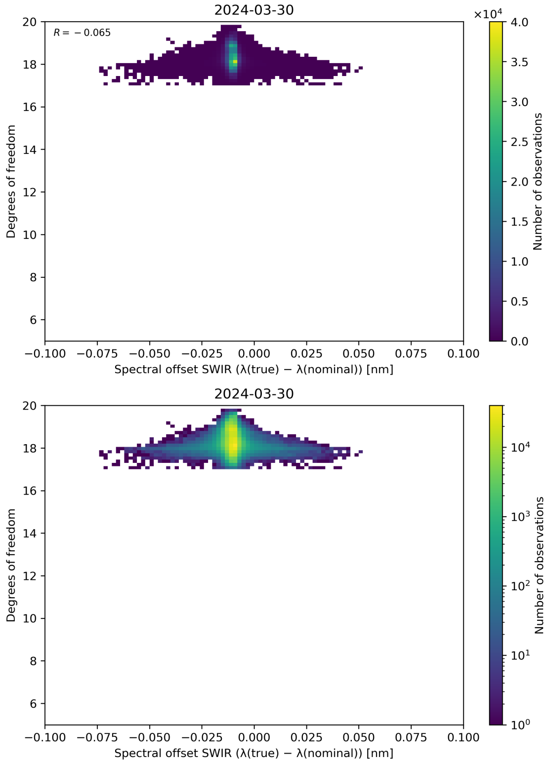
Figure 119: Scatter density plot of “Spectral offset SWIR ( \lambda(\text{true}) - \lambda(\text{nominal}) )” against “Degrees of freedom” for 2024-03-30 to 2024-03-31.
