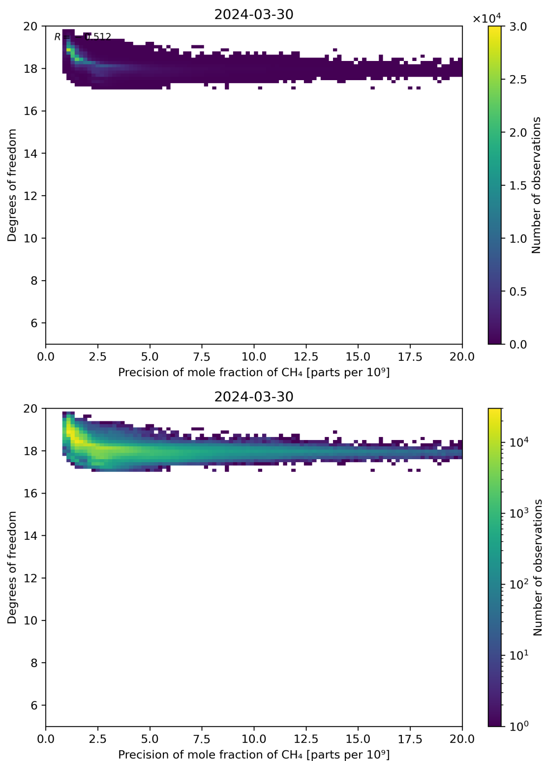
Figure 80: Scatter density plot of “Precision of mole fraction of CH 4 ” against “Degrees of freedom” for 2024-03-30 to 2024-03-31.
