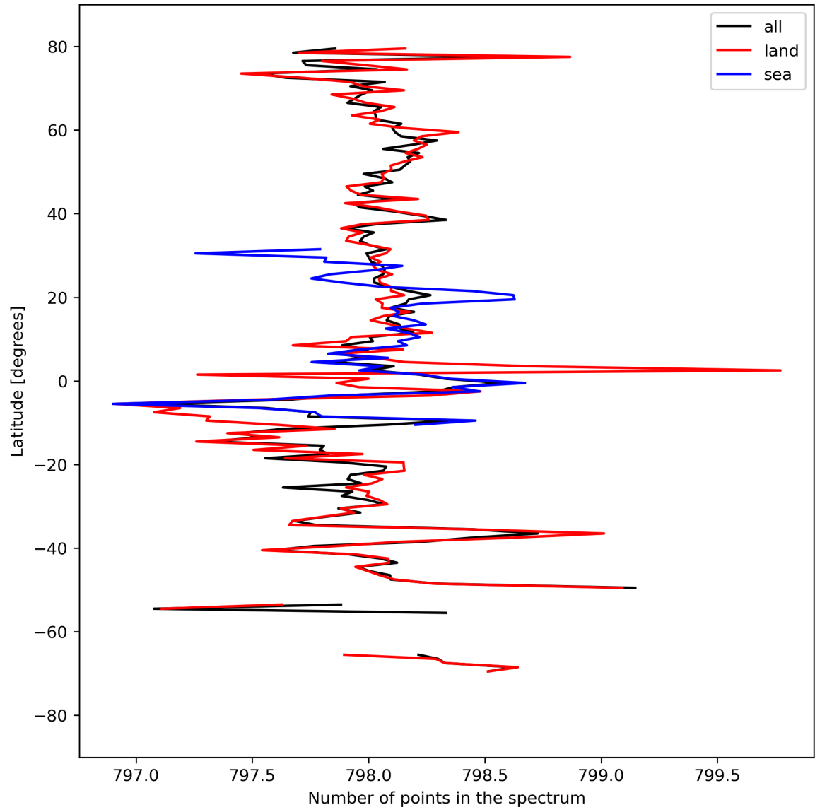
Figure 15: Zonal average of “Number of points in the spectrum” for 2024-03-31 to 2024-04-01.
