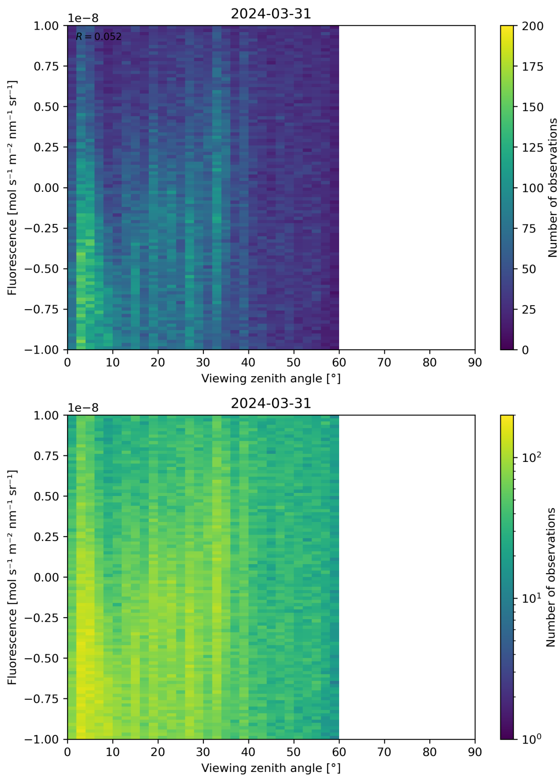
Figure 108: Scatter density plot of “Viewing zenith angle” against “Fluorescence” for 2024-03-31 to 2024-04-01.
