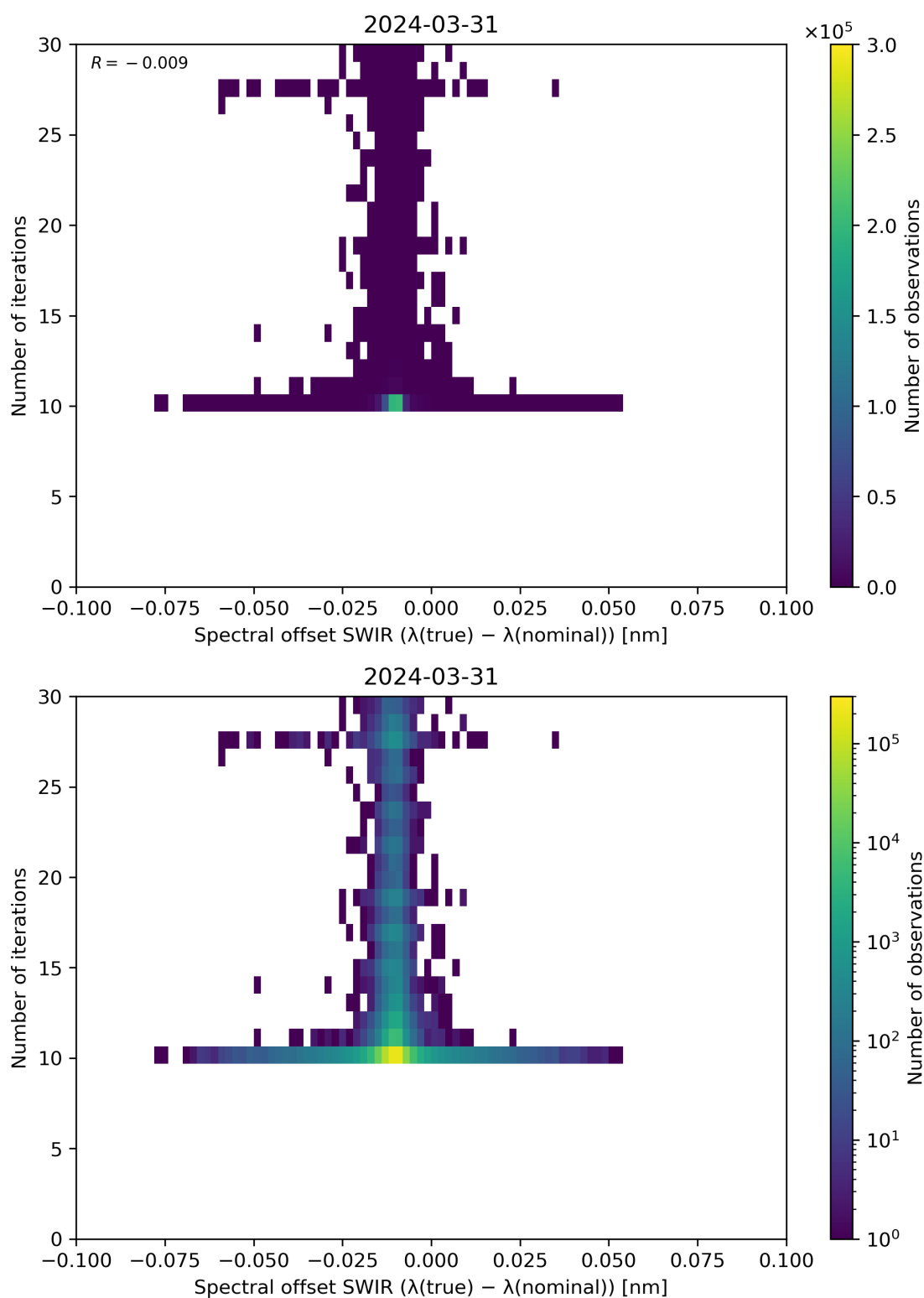
Figure 121: Scatter density plot of “Spectral offset SWIR ( \lambda(\text{true}) - \lambda(\text{nominal}) )” against “Number of iterations” for 2024-03-31 to 2024-04-01.
