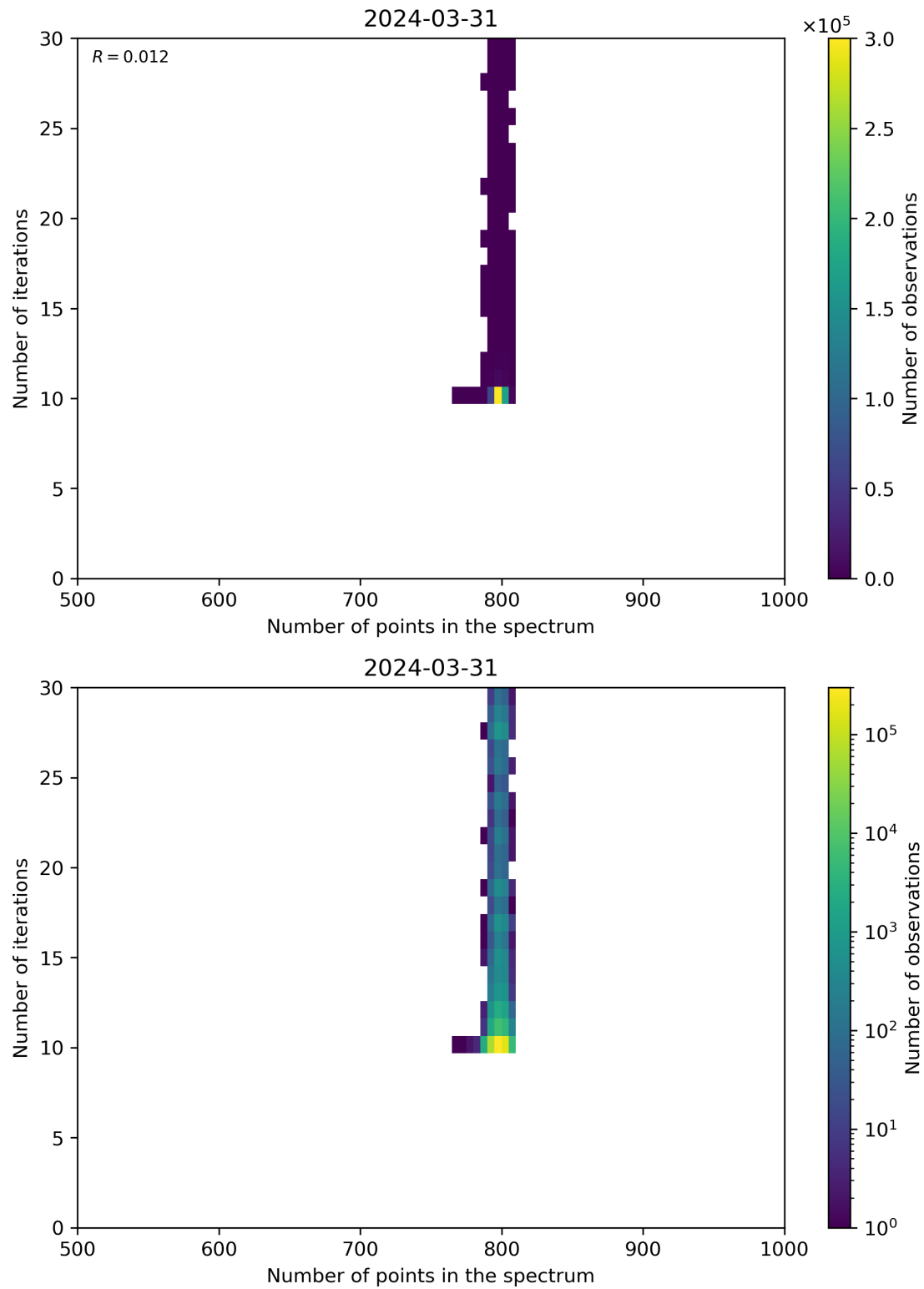
Figure 92: Scatter density plot of “Number of points in the spectrum” against “Number of iterations” for 2024-03-31 to 2024-04-01.
