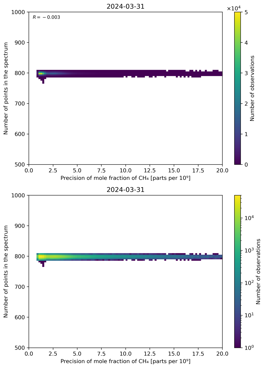
Figure 84: Scatter density plot of “Precision of mole fraction of CH 4 ” against “Number of points in the spectrum” for 2024-03-31 to 2024-04-01.
