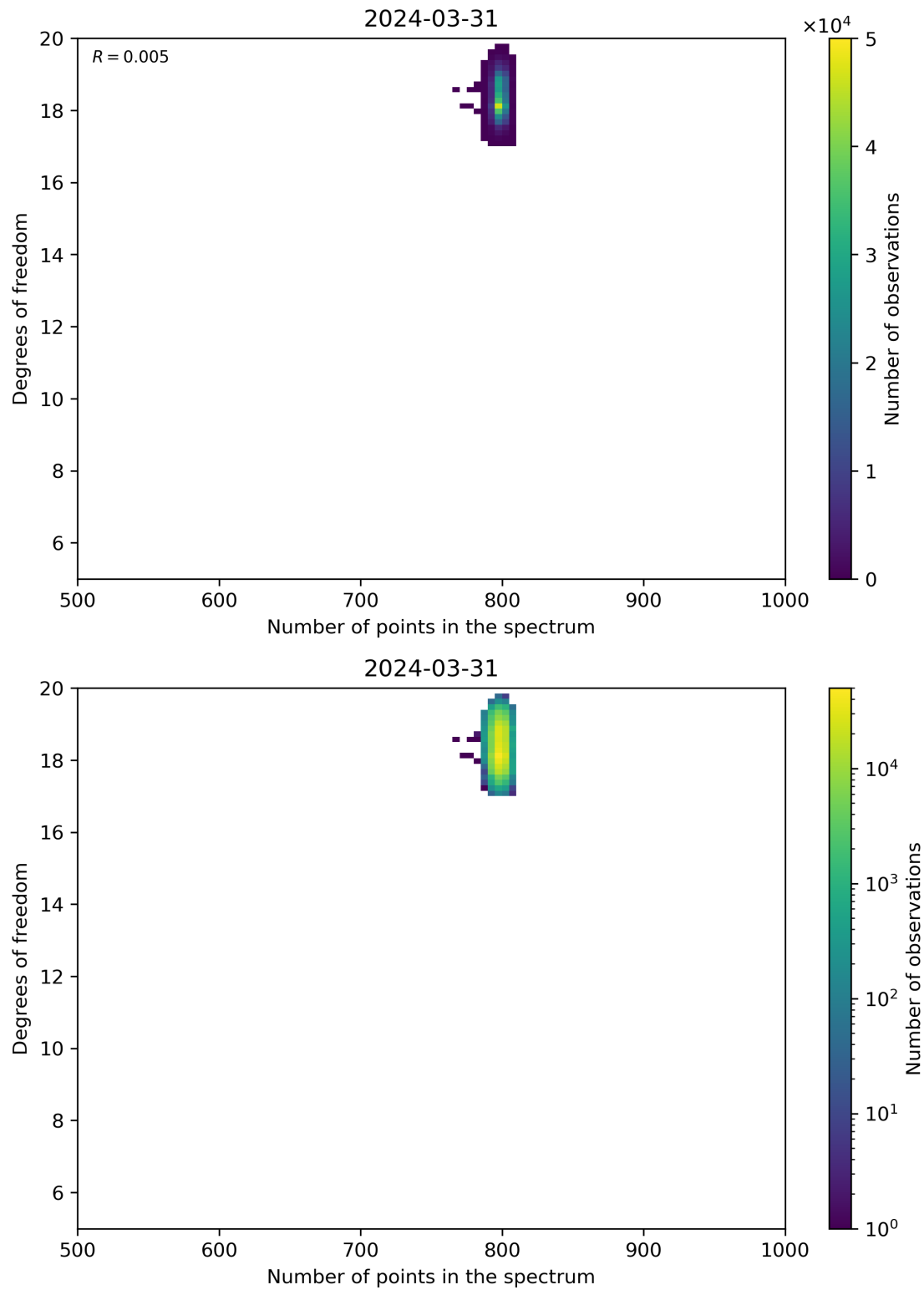
Figure 90: Scatter density plot of “Number of points in the spectrum” against “Degrees of freedom” for 2024-03-31 to 2024-04-01.
