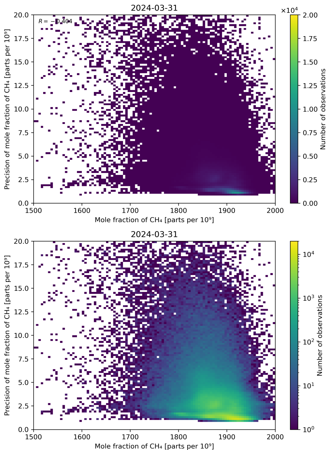
Figure 75: Scatter density plot of “Mole fraction of CH 4 ” against “Precision of mole fraction of CH 4 ” for 2024-03-31 to 2024-04-01.
