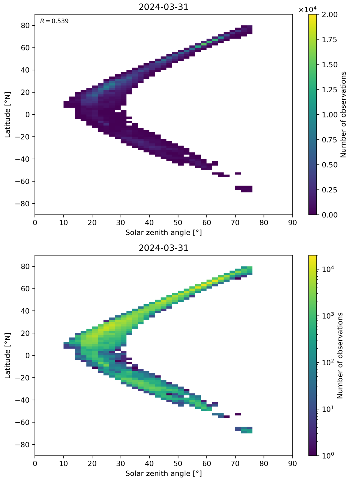
Figure 98: Scatter density plot of “Solar zenith angle” against “Latitude” for 2024-03-31 to 2024-04-01.
