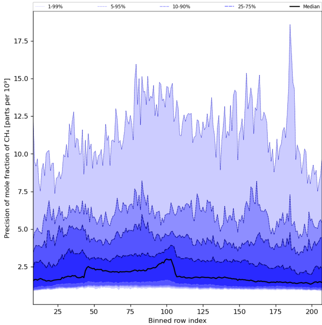
Figure 35: Along track statistics of “Precision of mole fraction of CH 4 ” for 2024-03-31 to 2024-04-01
