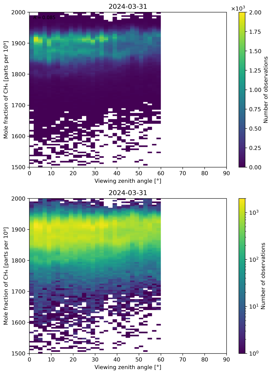
Figure 110: Scatter density plot of “Viewing zenith angle” against “Mole fraction of CH 4 ” for 2024-03-31 to 2024-04-01.
