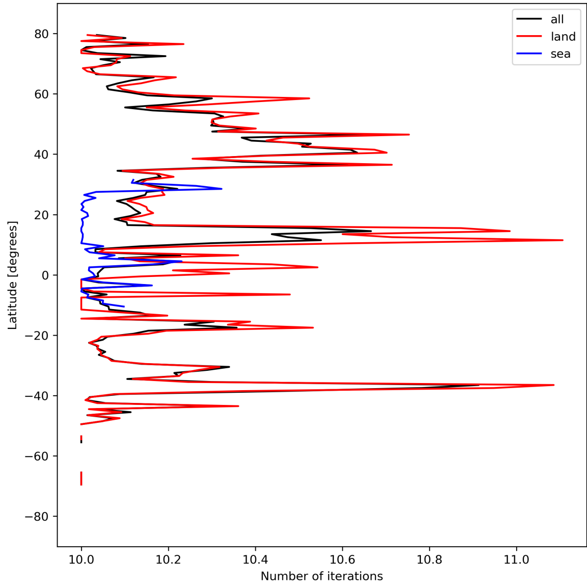
Figure 20: Zonal average of “Number of iterations” for 2024-03-31 to 2024-04-01.
