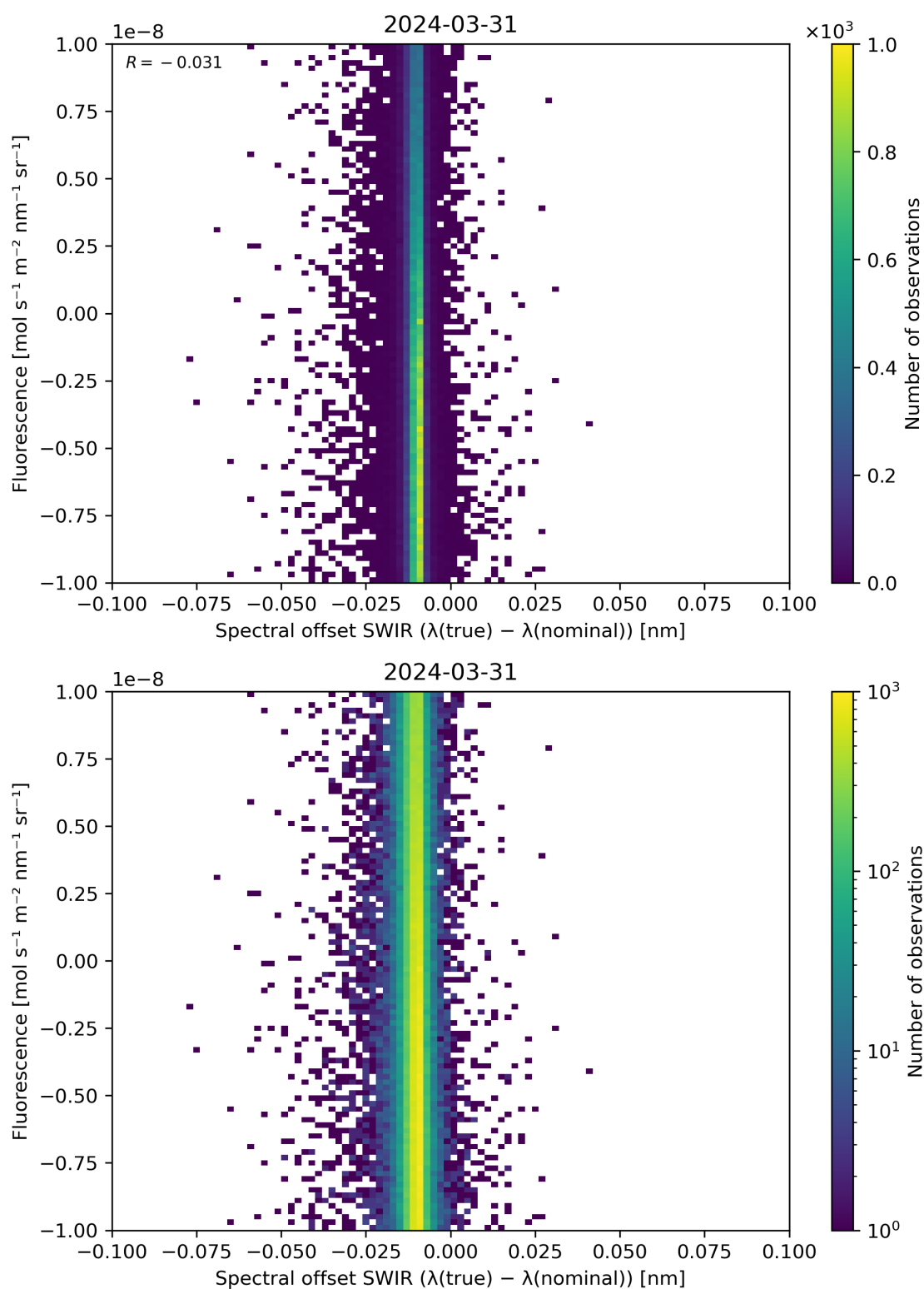
Figure 120: Scatter density plot of “Spectral offset SWIR ( \lambda(\text{true}) - \lambda(\text{nominal}) )” against “Fluorescence” for 2024-03-31 to 2024-04-01.
