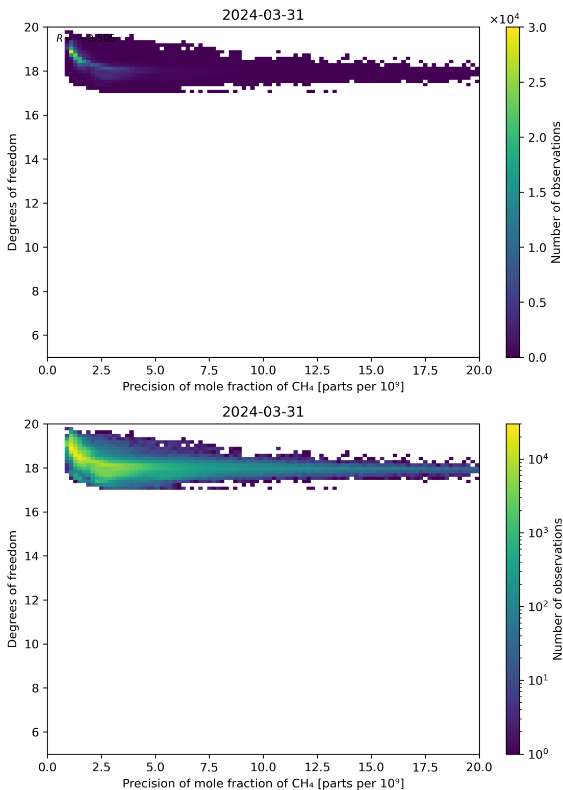
Figure 80: Scatter density plot of “Precision of mole fraction of CH 4 ” against “Degrees of freedom” for 2024-03-31 to 2024-04-01.
