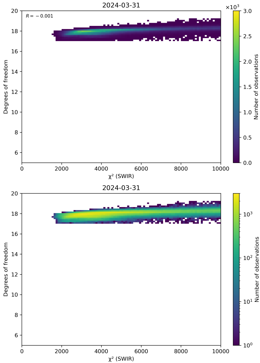
Figure 48: Scatter density plot of “ \chi^2 (SWIR)” against “Degrees of freedom” for 2024-03-31 to 2024-04-01.
