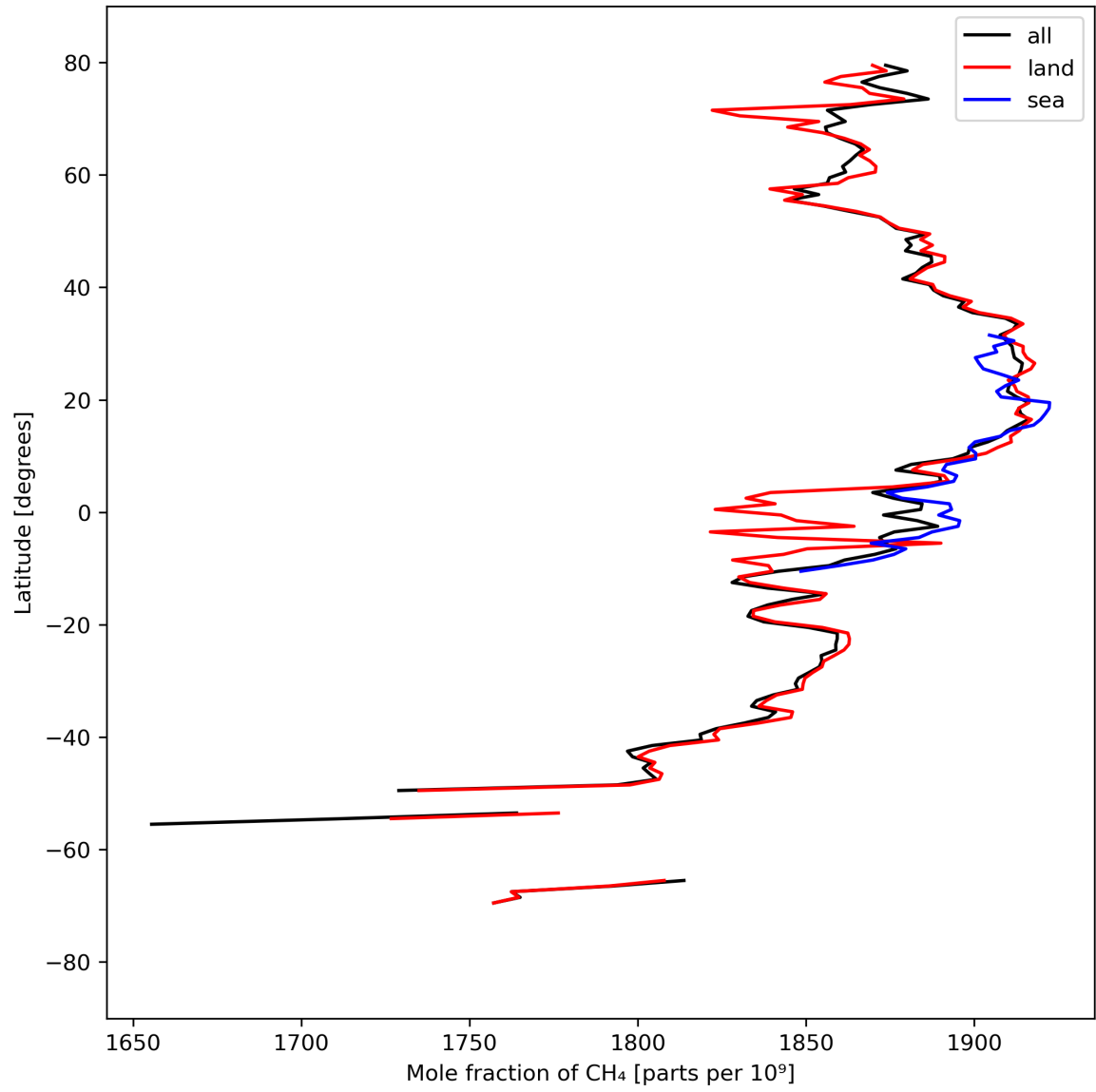
Figure 12: Zonal average of “Mole fraction of \text{CH}_4 ” for 2024-03-31 to 2024-04-01.
