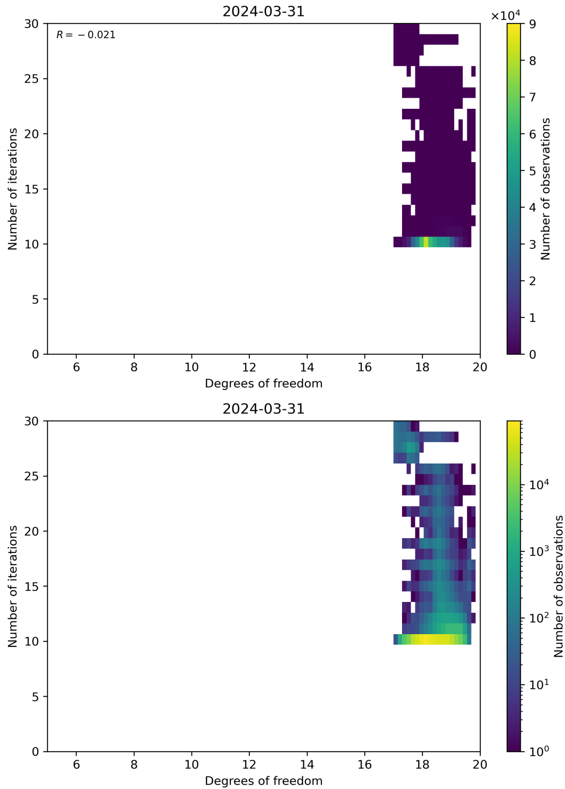
Figure 52: Scatter density plot of “Degrees of freedom” against “Number of iterations” for 2024-03-31 to 2024-04-01.
