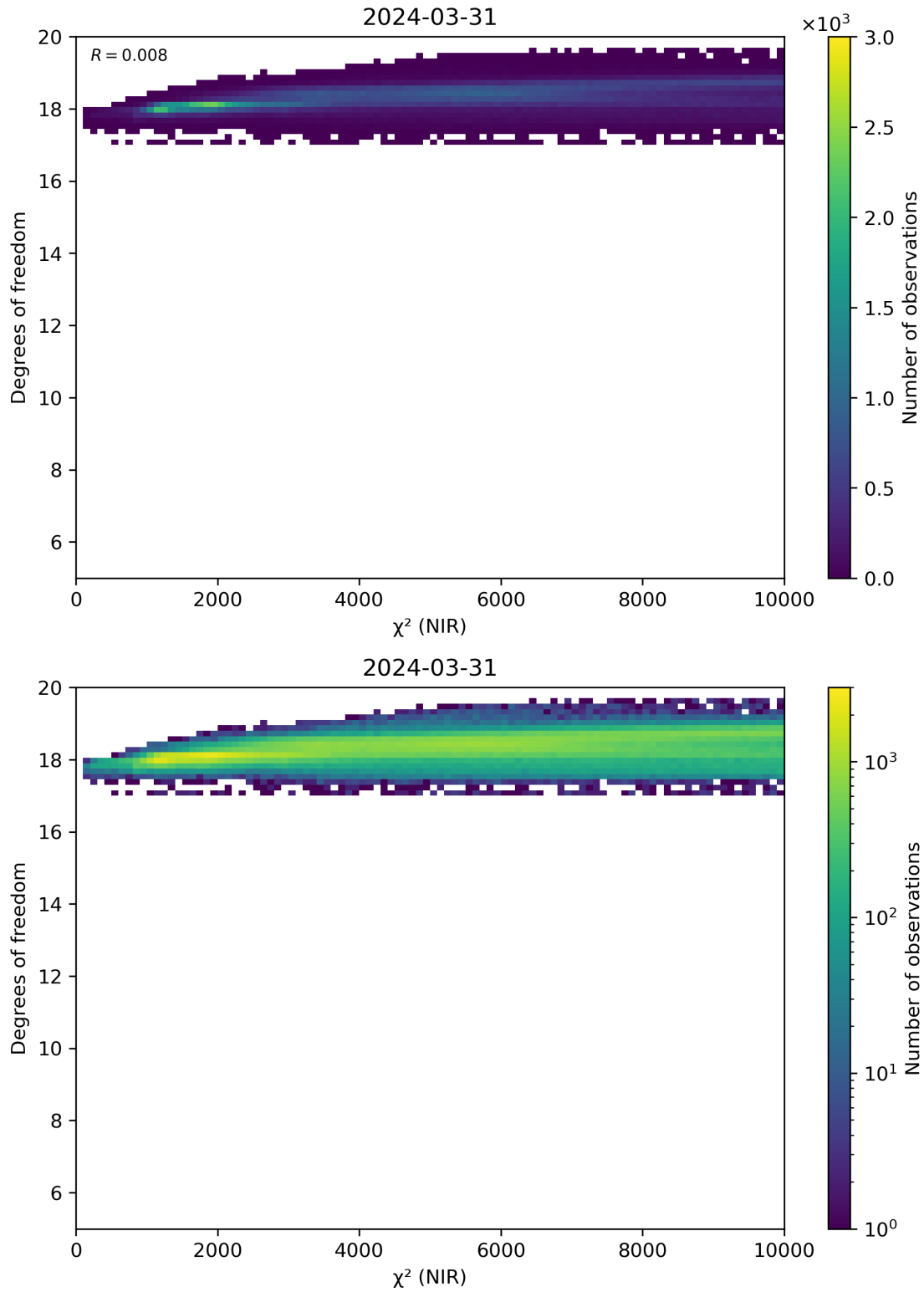
Figure 44: Scatter density plot of “ \chi^2 (NIR)” against “Degrees of freedom” for 2024-03-31 to 2024-04-01.
