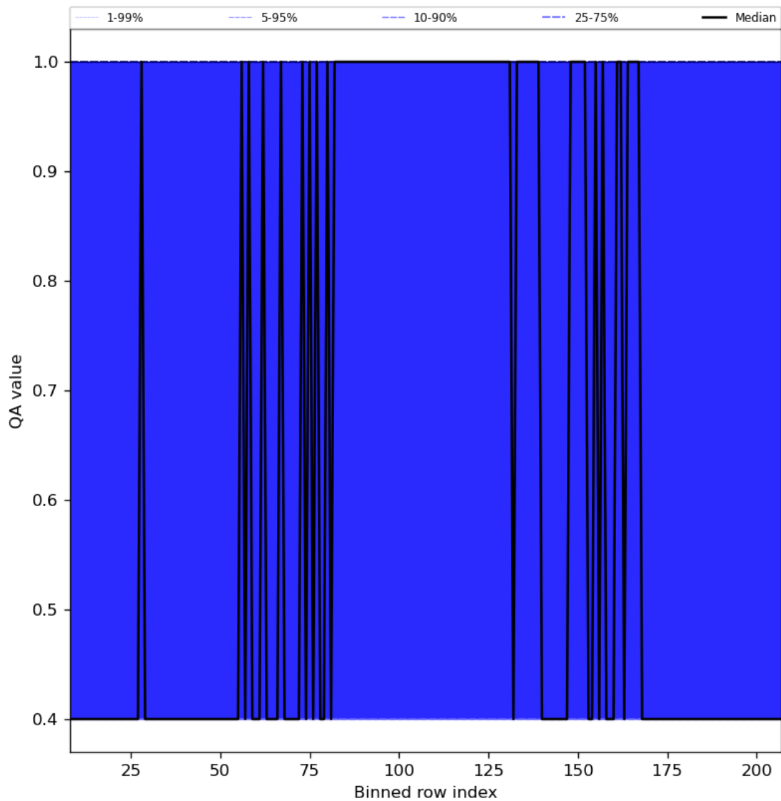
Figure 33: Along track statistics of “QA value” for 2024-03-31 to 2024-04-01
