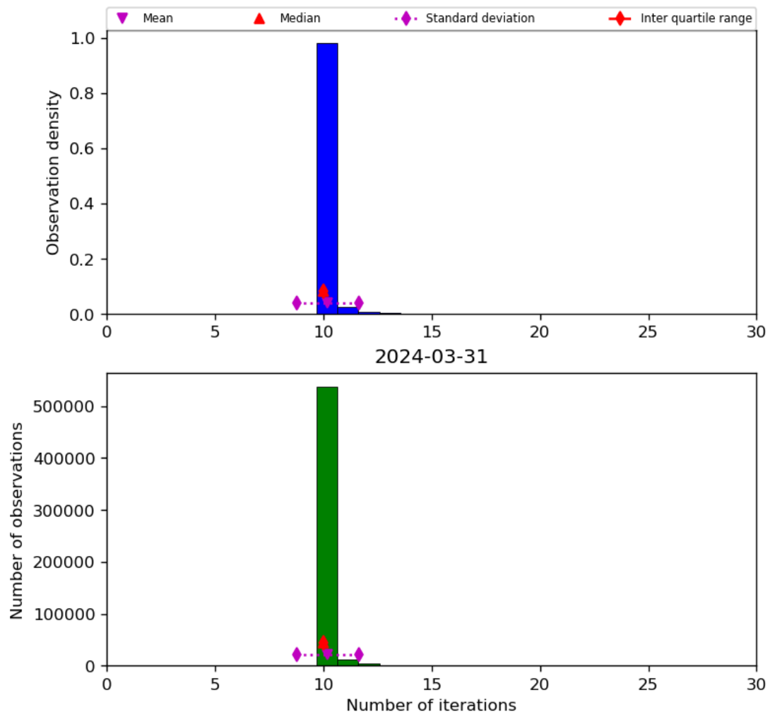
Figure 31: Histogram of “Number of iterations” for 2024-03-31 to 2024-04-01
