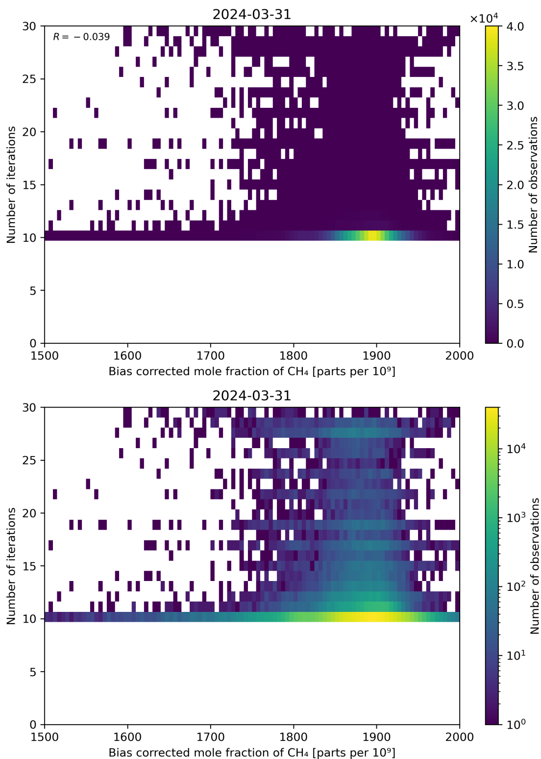
Figure 67: Scatter density plot of “Bias corrected mole fraction of \text{CH}_4 ” against “Number of iterations” for 2024-03-31 to 2024-04-01.
