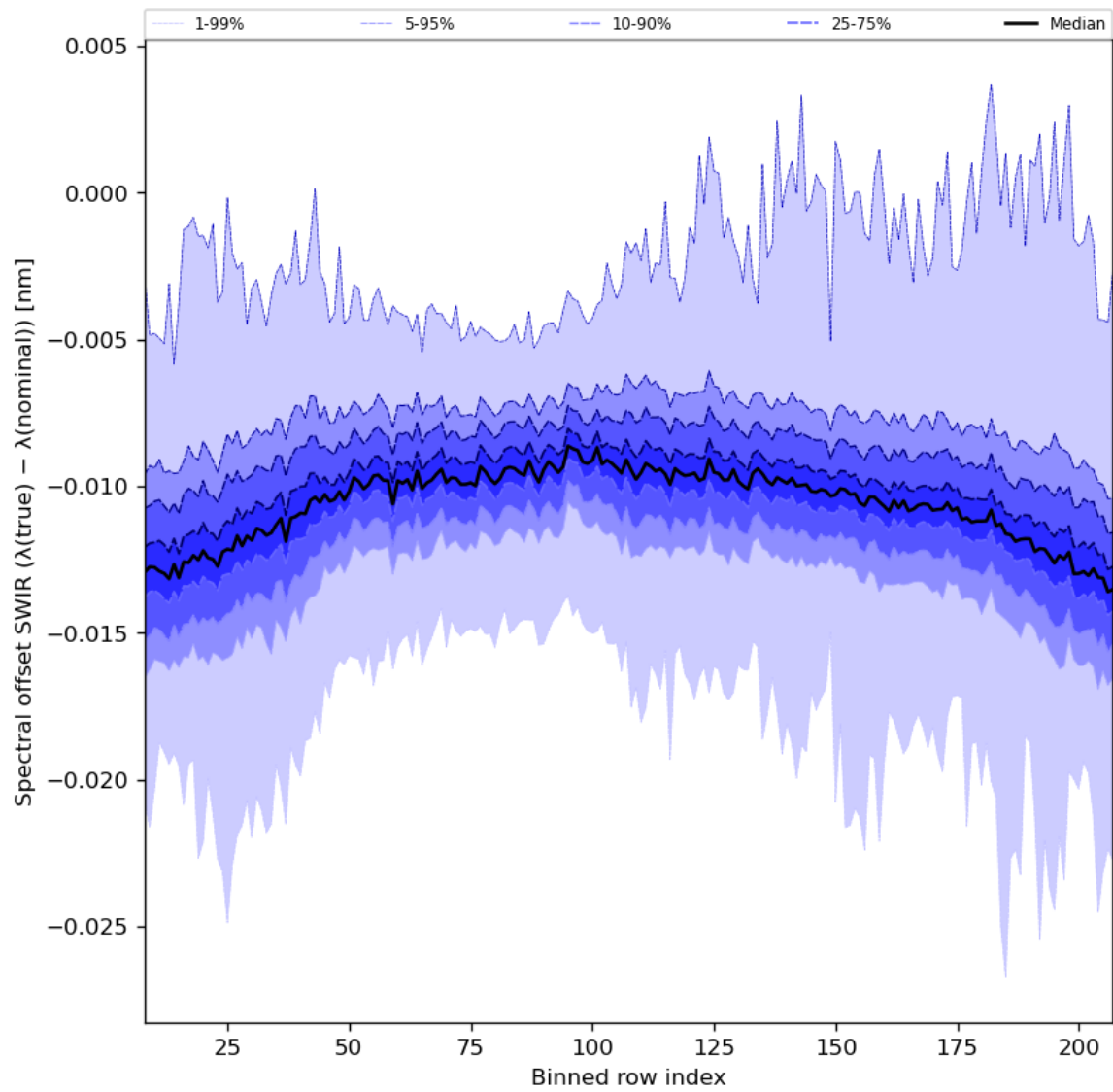
Figure 38: Along track statistics of “Spectral offset SWIR ( \lambda(\text{true}) - \lambda(\text{nominal}) )” for 2024-03-31 to 2024-04-01
