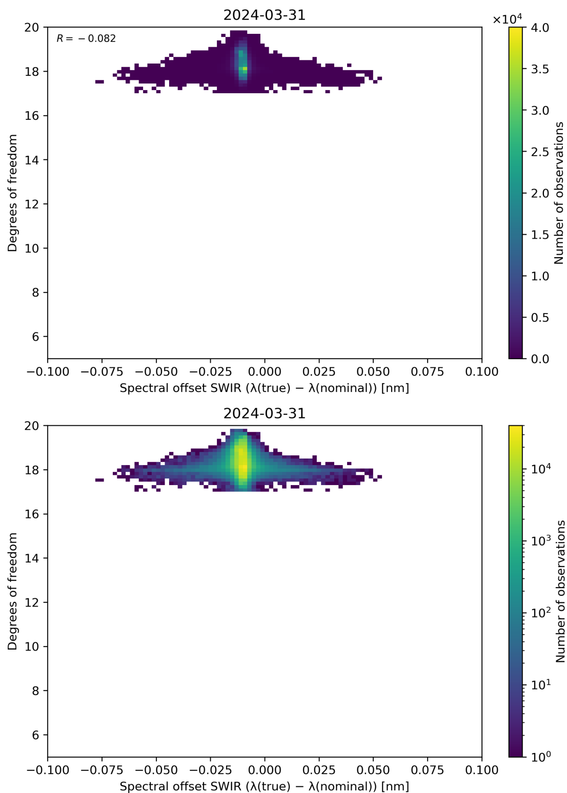
Figure 119: Scatter density plot of “Spectral offset SWIR ( \lambda(\text{true}) - \lambda(\text{nominal}) )” against “Degrees of freedom” for 2024-03-31 to 2024-04-01.
