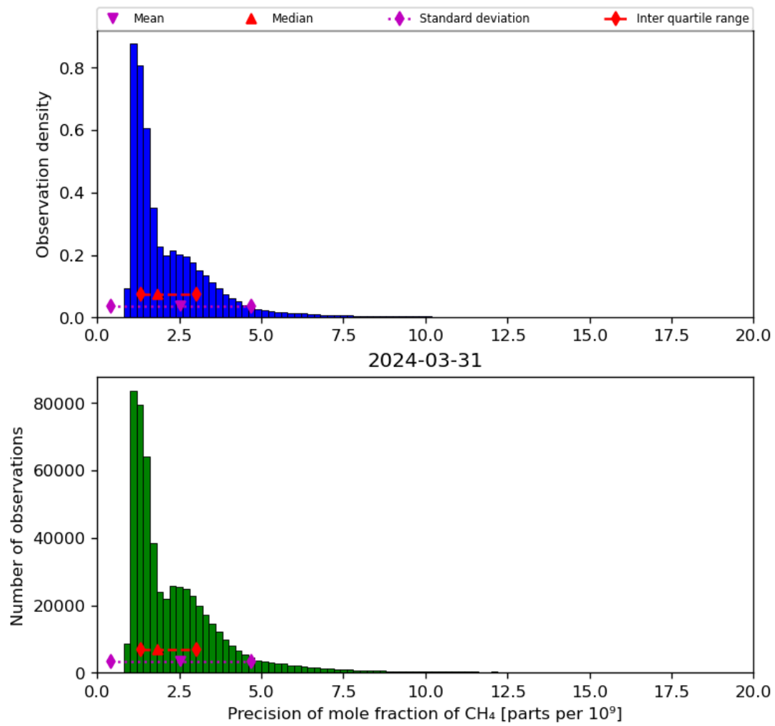
Figure 24: Histogram of “Precision of mole fraction of CH 4 ” for 2024-03-31 to 2024-04-01
