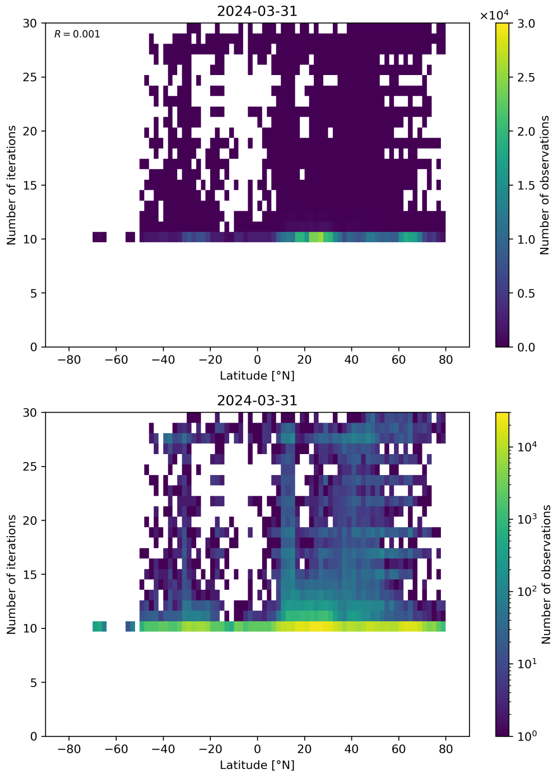
Figure 60: Scatter density plot of “Latitude” against “Number of iterations” for 2024-03-31 to 2024-04-01.
