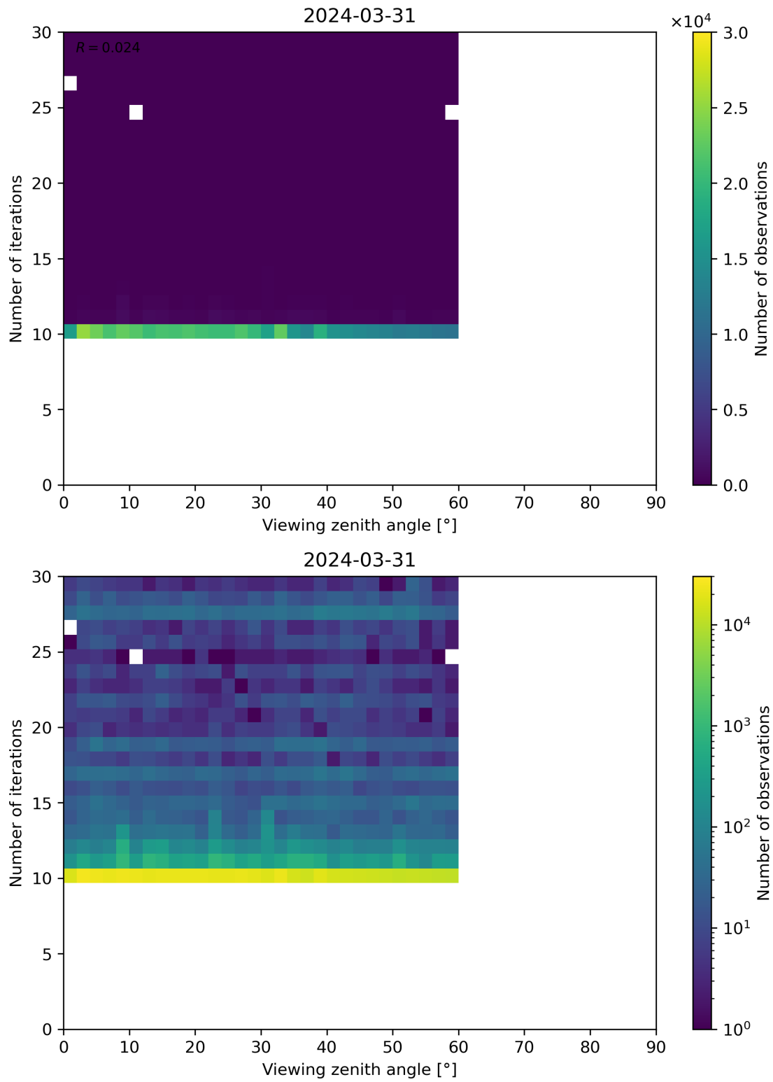
Figure 113: Scatter density plot of “Viewing zenith angle” against “Number of iterations” for 2024-03-31 to 2024-04-01.
