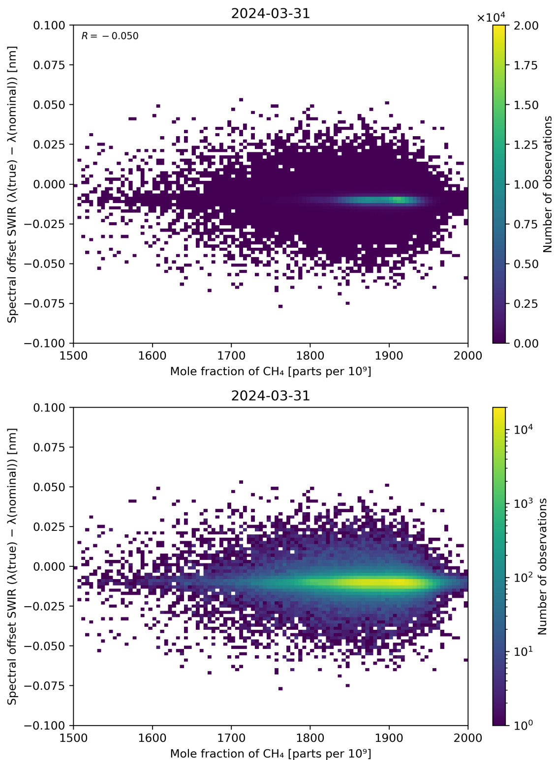
Figure 86: Scatter density plot of “Mole fraction of CH 4 ” against “Spectral offset SWIR ( \lambda(\text{true}) - \lambda(\text{nominal}) )” for 2024-03-31 to 2024-04-01.
