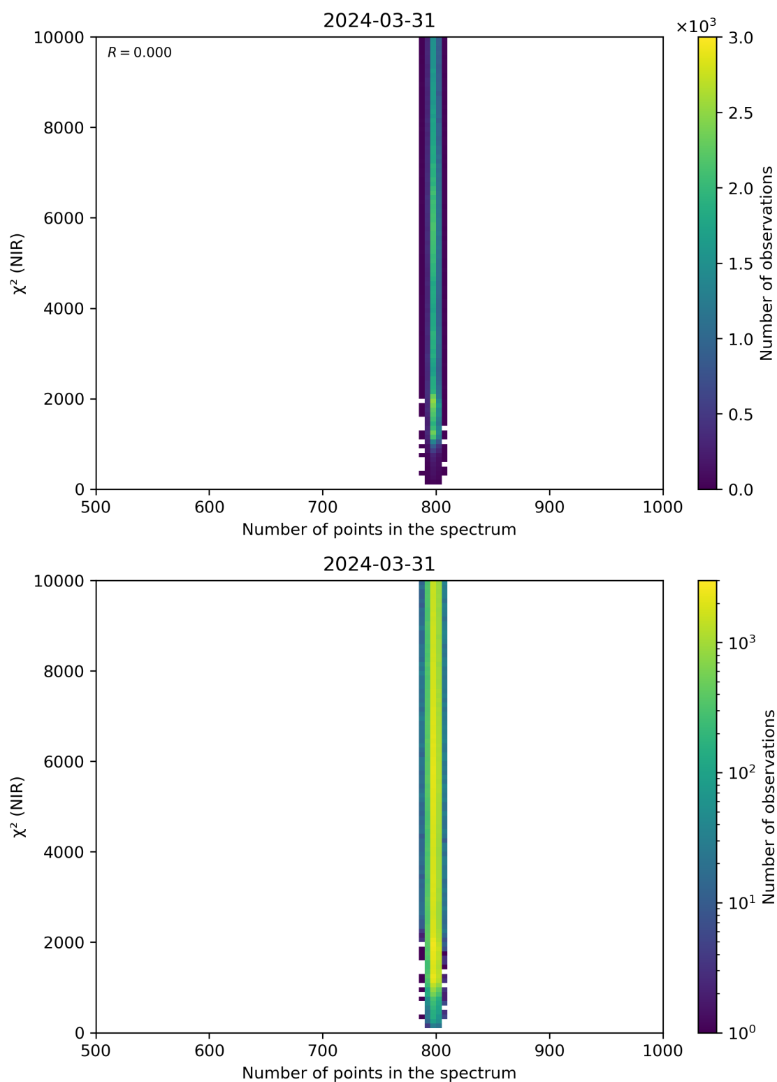
Figure 88: Scatter density plot of “Number of points in the spectrum” against “ \chi^2 (NIR)” for 2024-03-31 to 2024-04-01.
