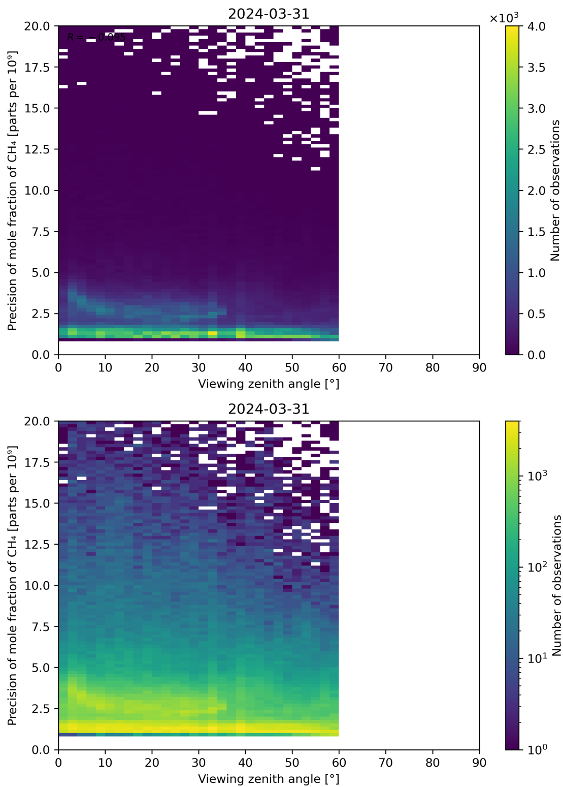
Figure 112: Scatter density plot of “Viewing zenith angle” against “Precision of mole fraction of CH 4 ” for 2024-03-31 to 2024-04-01.
