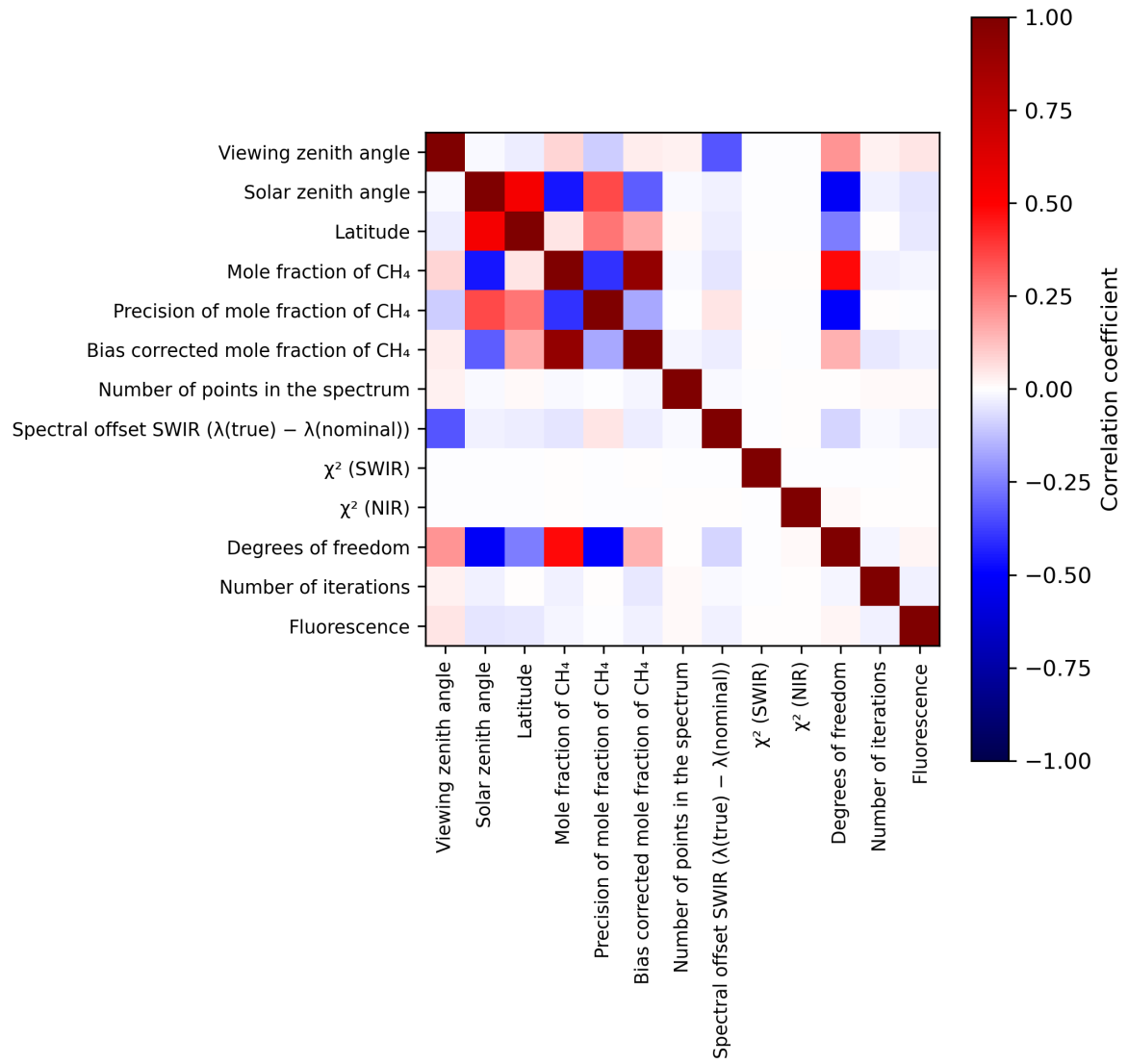
Figure 2: Map of correlation matrix for 2024-03-31 to 2024-04-01.
