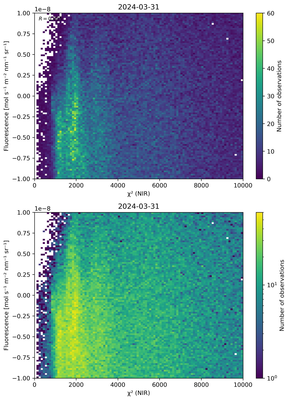
Figure 45: Scatter density plot of “ \chi^2 (NIR)” against “Fluorescence” for 2024-03-31 to 2024-04-01.
