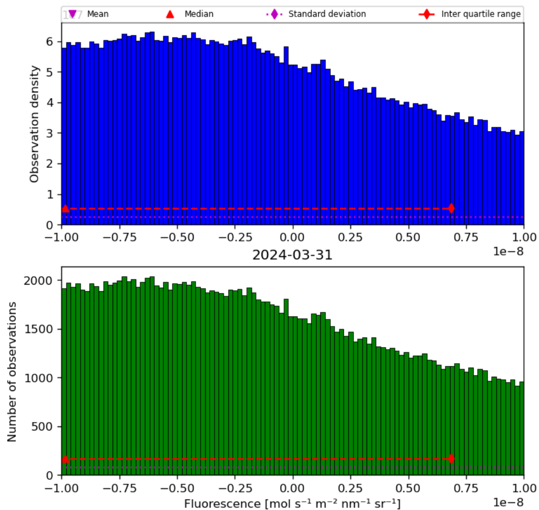
Figure 32: Histogram of “Fluorescence” for 2024-03-31 to 2024-04-01
