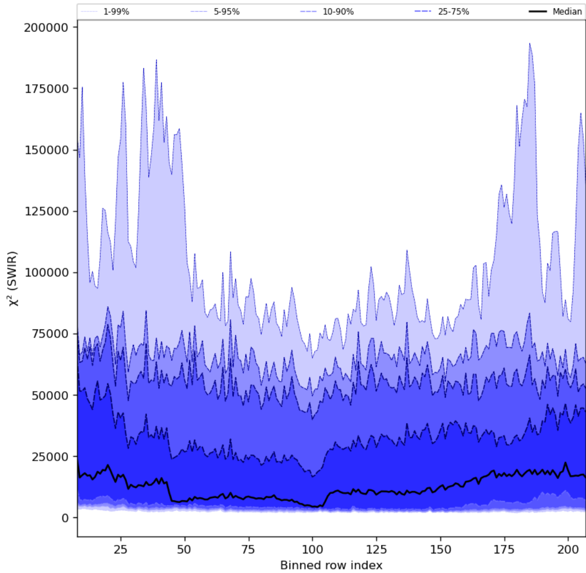
Figure 39: Along track statistics of " \chi^2 (SWIR)" for 2024-03-31 to 2024-04-01
