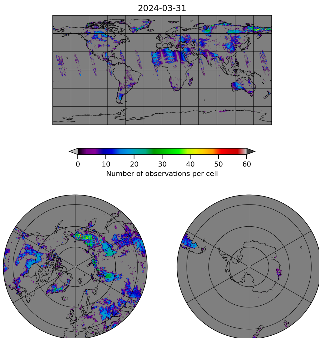
Figure 10: Map of the number of observations for 2024-03-31 to 2024-04-01
