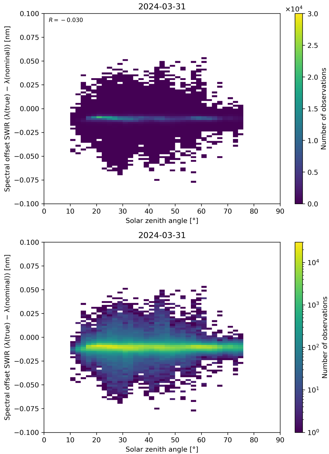
Figure 104: Scatter density plot of “Solar zenith angle” against “Spectral offset SWIR ( \lambda(\text{true}) - \lambda(\text{nominal}) )” for 2024-03-31 to 2024-04-01.
