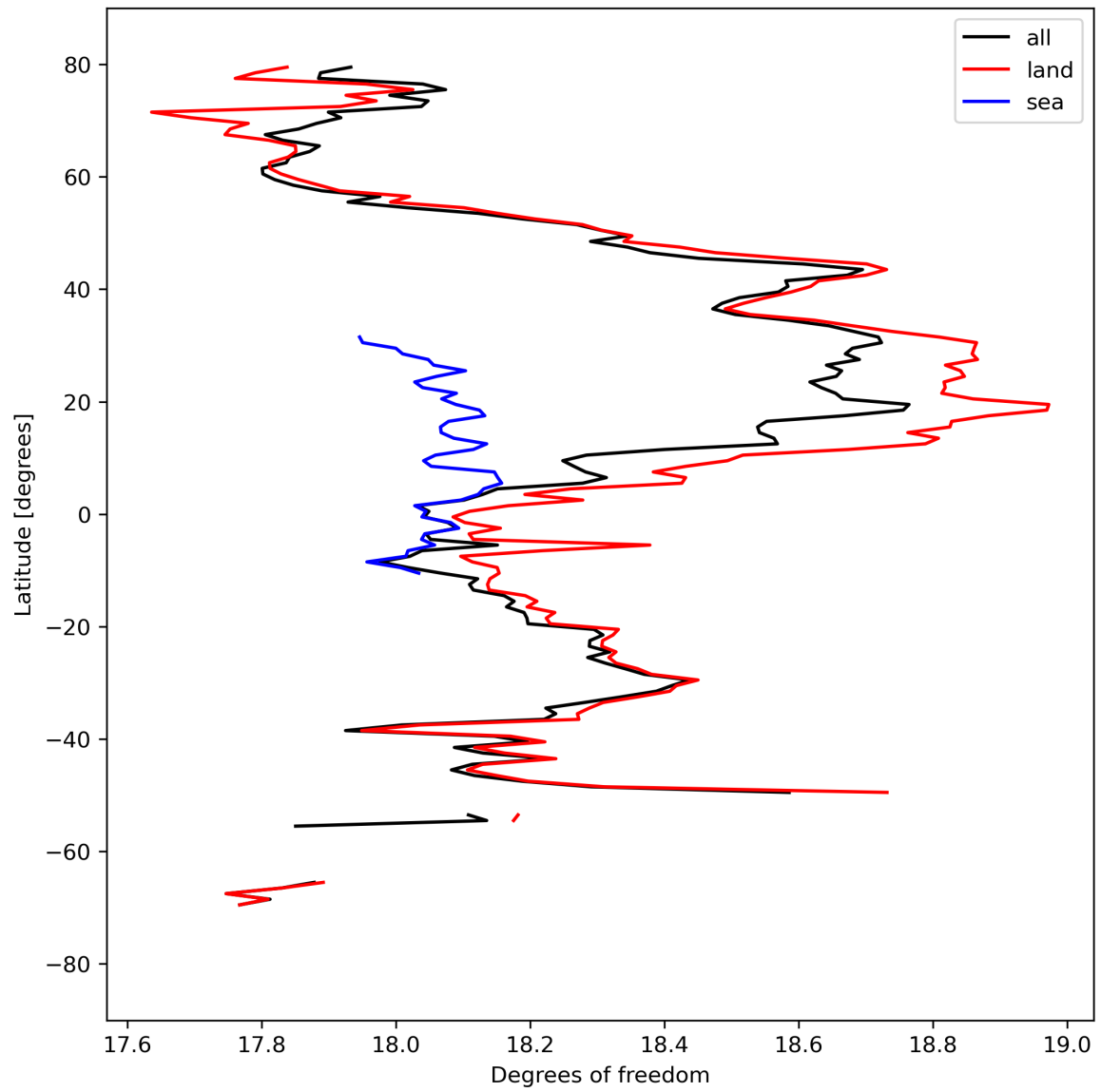
Figure 19: Zonal average of “Degrees of freedom” for 2024-03-31 to 2024-04-01.
