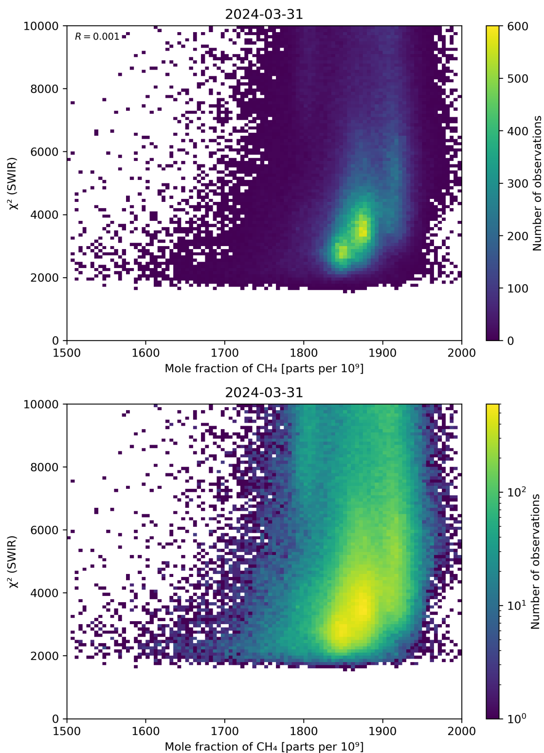
Figure 71: Scatter density plot of “Mole fraction of \text{CH}_4 ” against “ \chi^2 (SWIR)” for 2024-03-31 to 2024-04-01.
