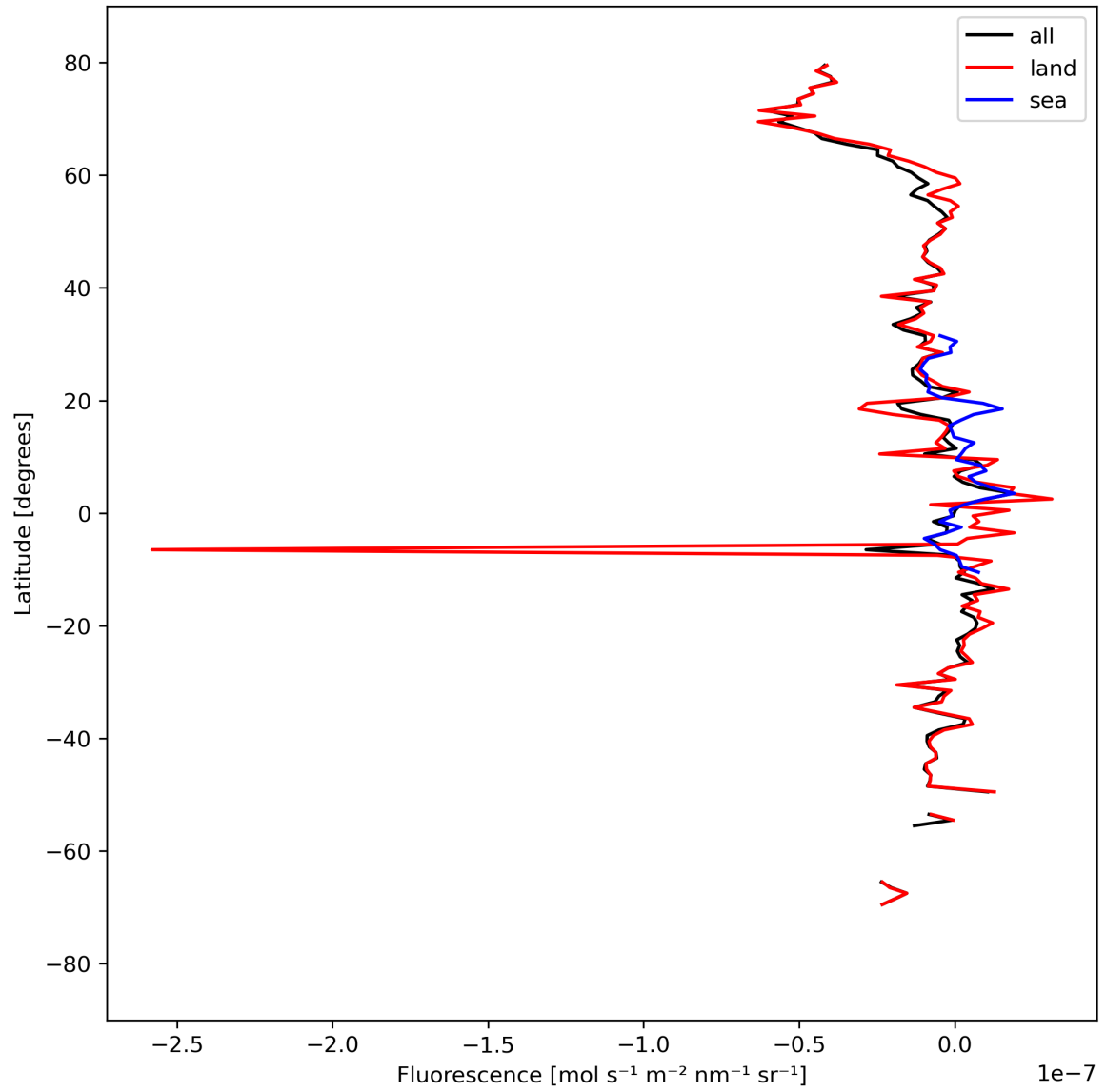
Figure 21: Zonal average of “Fluorescence” for 2024-03-31 to 2024-04-01.
