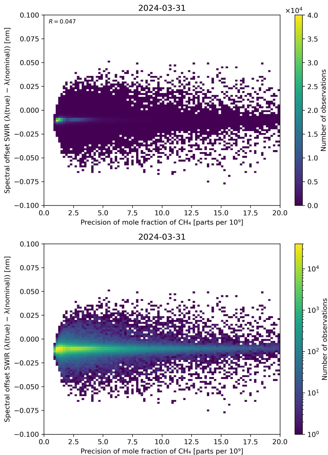
Figure 85: Scatter density plot of “Precision of mole fraction of \text{CH}_4 ” against “Spectral offset SWIR ( \lambda(\text{true}) - \lambda(\text{nominal}) )” for 2024-03-31 to 2024-04-01.
