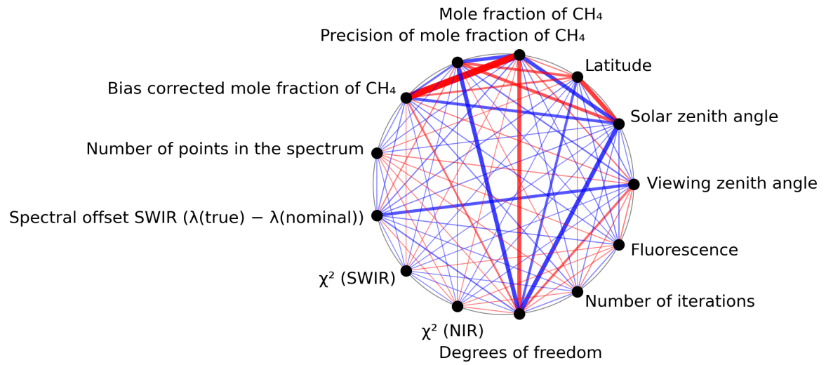
Figure 1: Map of correlation graph for 2024-03-31 to 2024-04-01.
