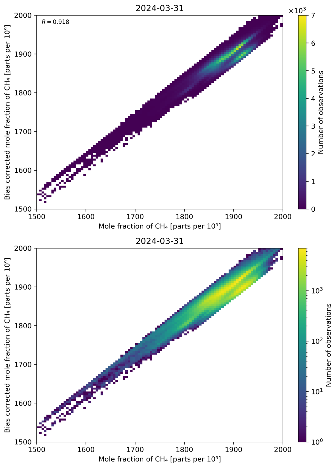
Figure 74: Scatter density plot of “Mole fraction of CH 4 ” against “Bias corrected mole fraction of CH 4 ” for 2024-03-31 to 2024-04-01.
