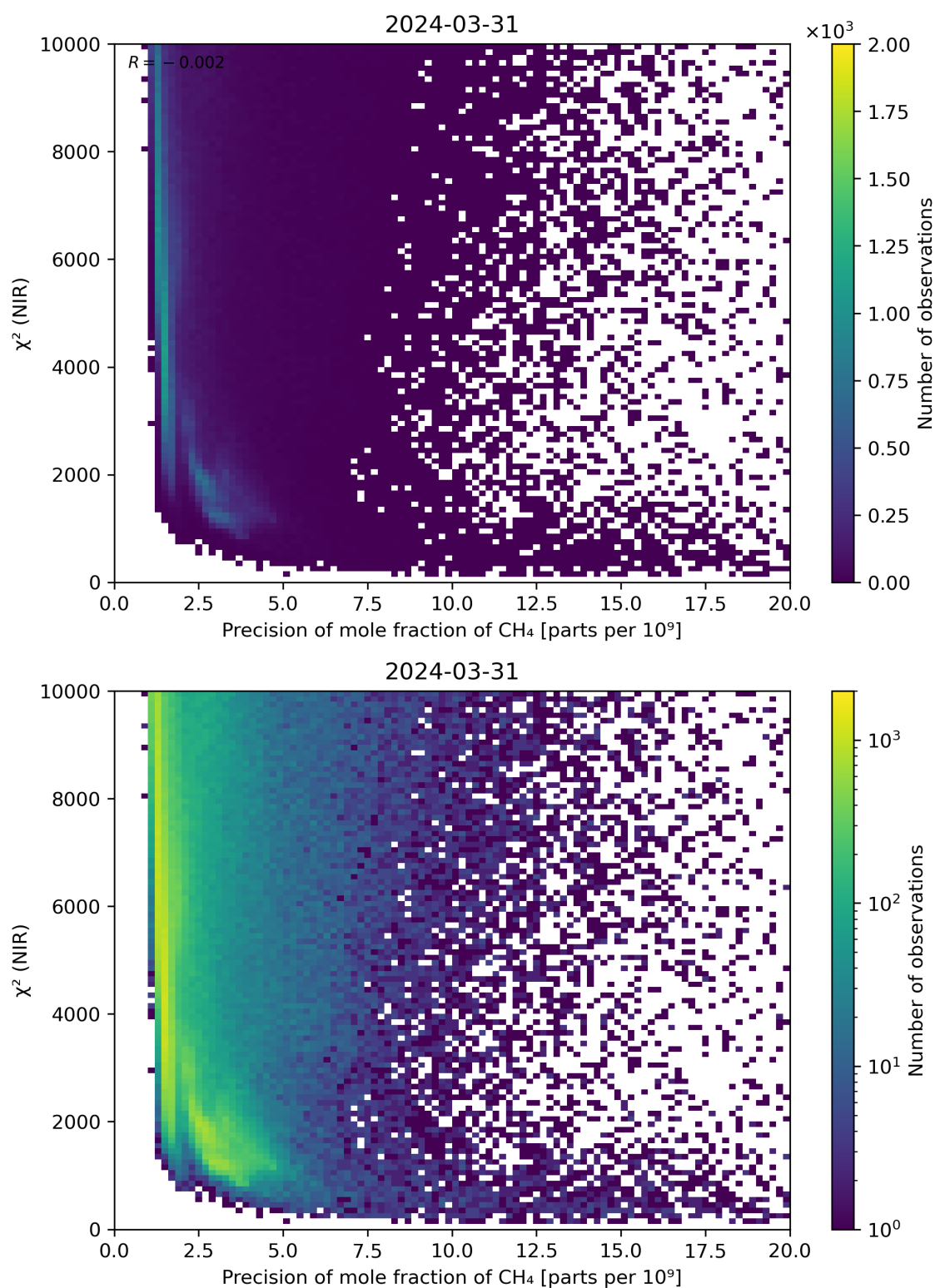
Figure 78: Scatter density plot of “Precision of mole fraction of CH 4 ” against “ \chi^2 (NIR)” for 2024-03-31 to 2024-04-01.
