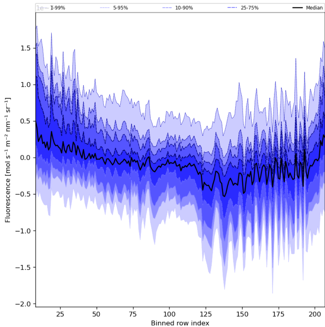
Figure 43: Along track statistics of “Fluorescence” for 2024-03-31 to 2024-04-01
