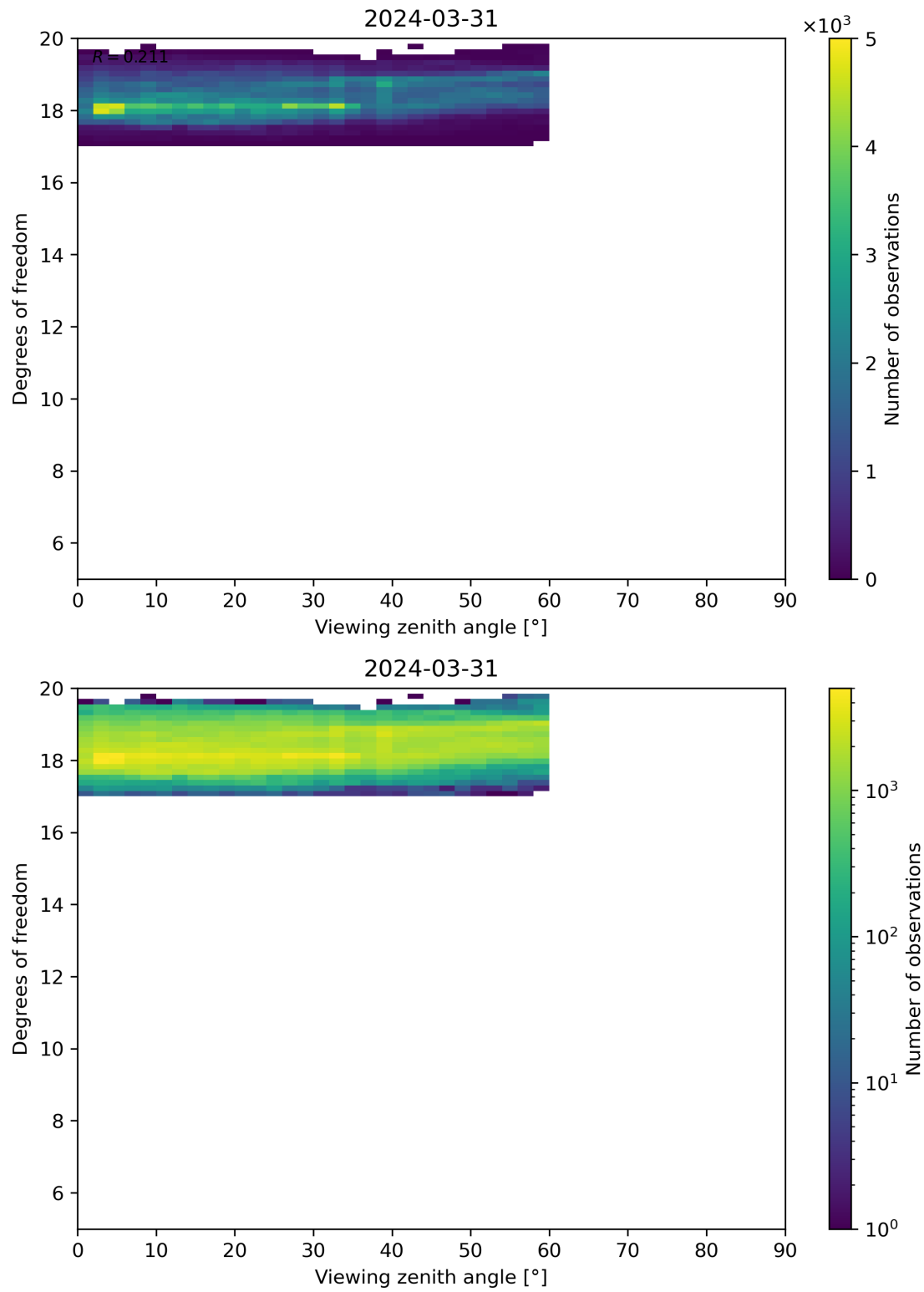
Figure 107: Scatter density plot of “Viewing zenith angle” against “Degrees of freedom” for 2024-03-31 to 2024-04-01.
