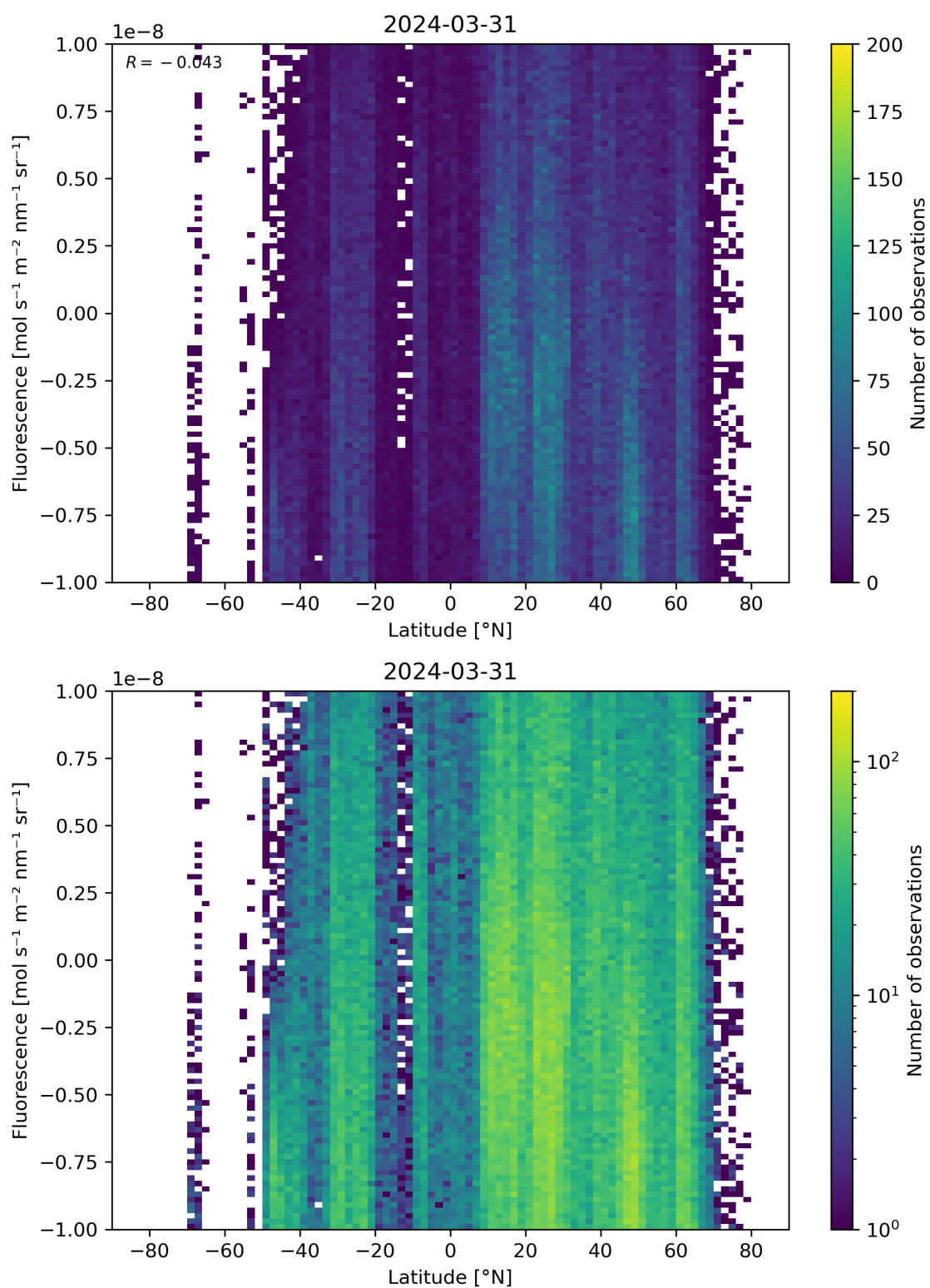
Figure 56: Scatter density plot of “Latitude” against “Fluorescence” for 2024-03-31 to 2024-04-01.
