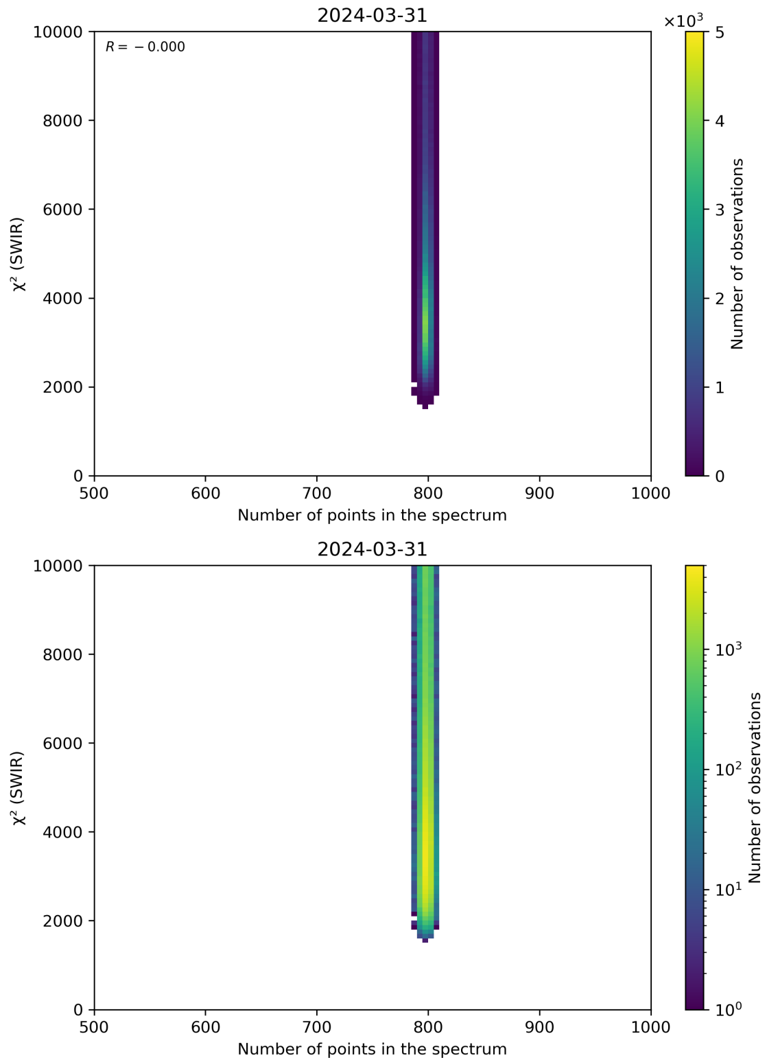
Figure 89: Scatter density plot of “Number of points in the spectrum” against “ \chi^2 (SWIR)” for 2024-03-31 to 2024-04-01.
