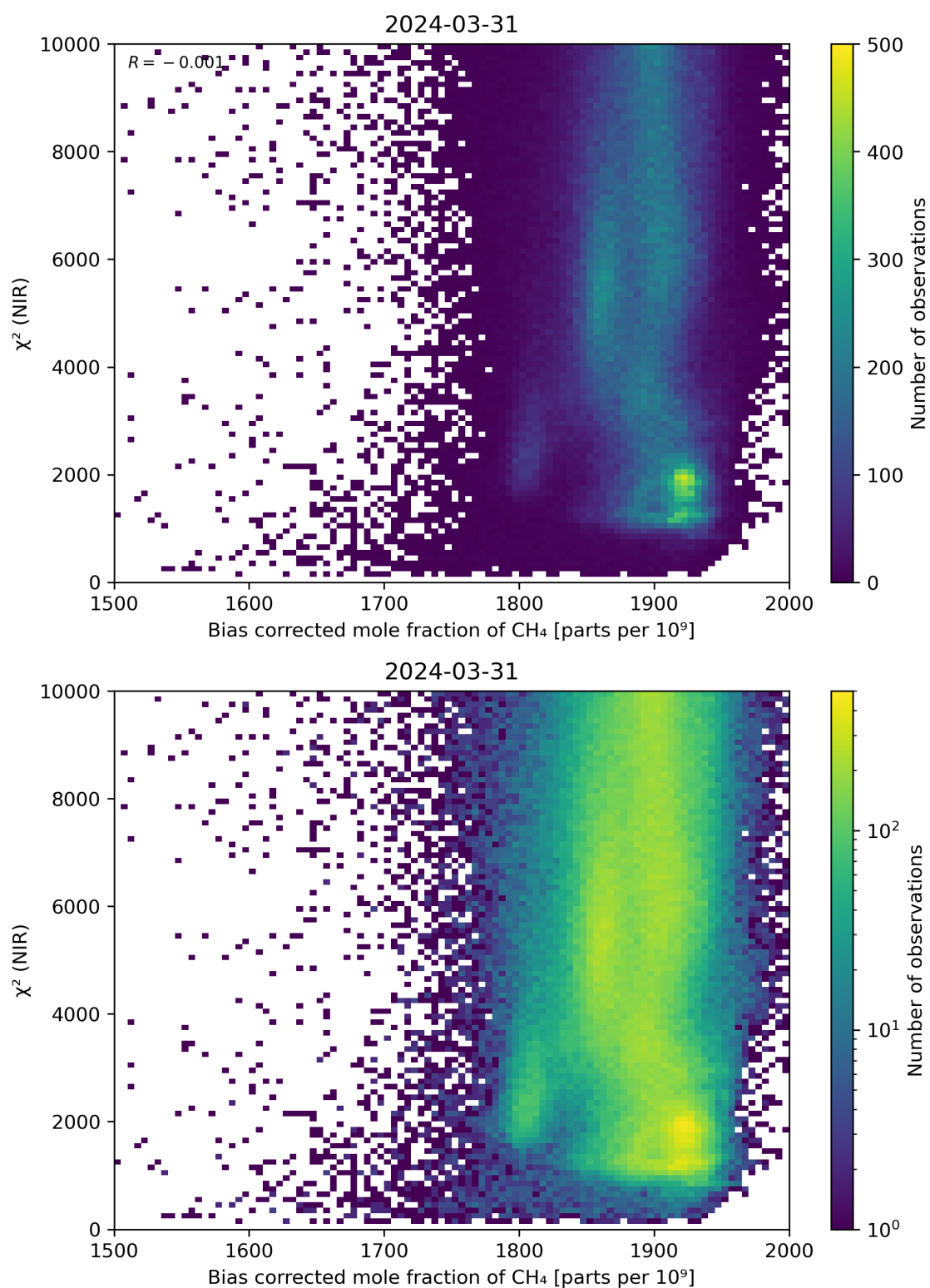
Figure 63: Scatter density plot of “Bias corrected mole fraction of CH 4 ” against “ \chi^2 (NIR)” for 2024-03-31 to 2024-04-01.
