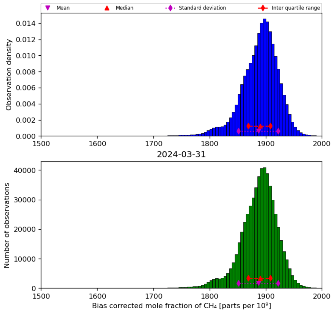
Figure 25: Histogram of “Bias corrected mole fraction of CH 4 ” for 2024-03-31 to 2024-04-01
