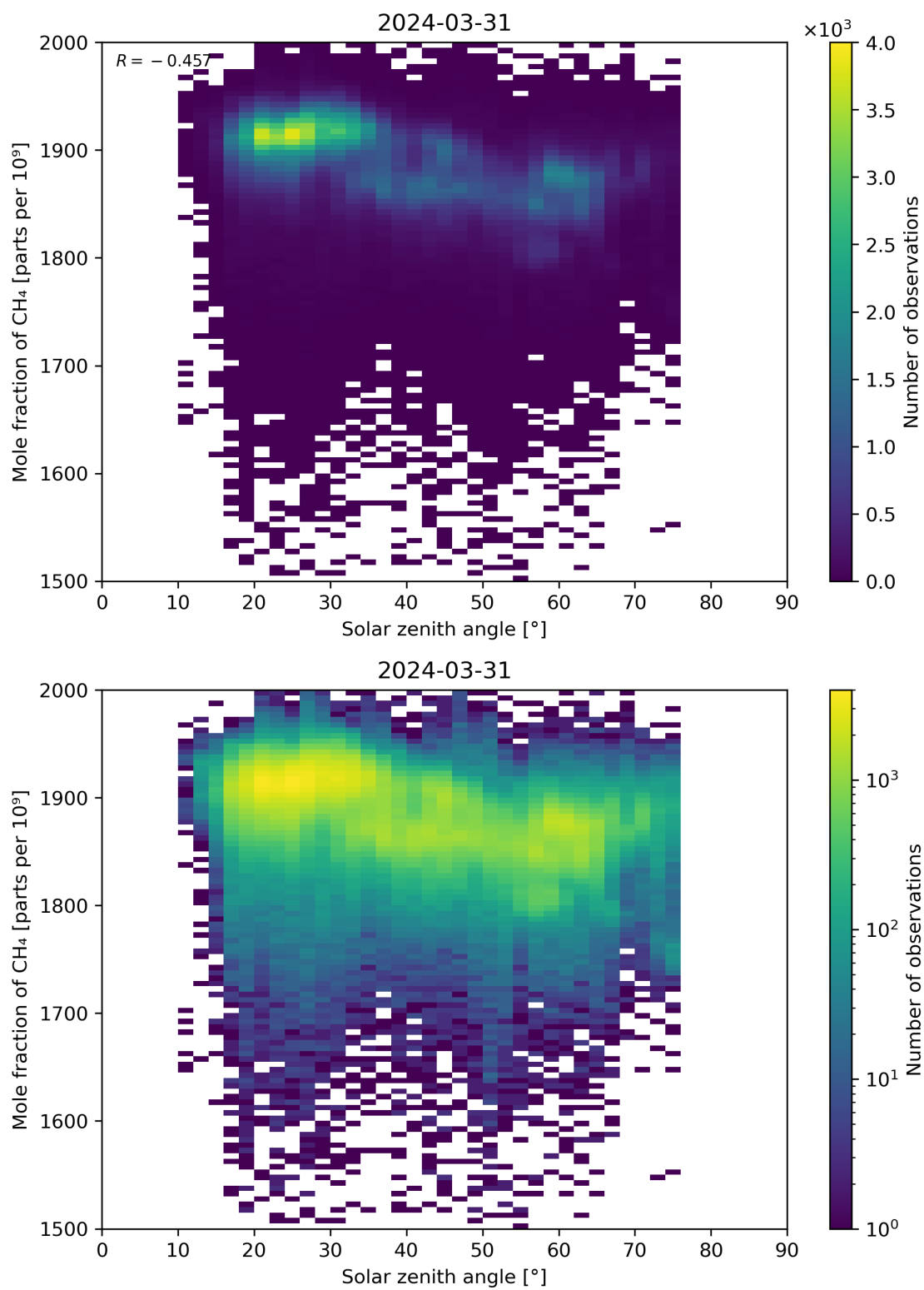
Figure 99: Scatter density plot of “Solar zenith angle” against “Mole fraction of CH 4 ” for 2024-03-31 to 2024-04-01.
