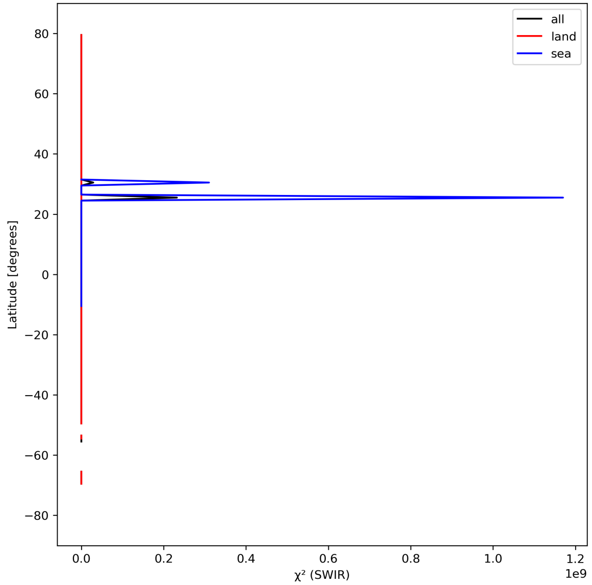
Figure 17: Zonal average of “ \chi^2 (SWIR)” for 2024-03-31 to 2024-04-01.
