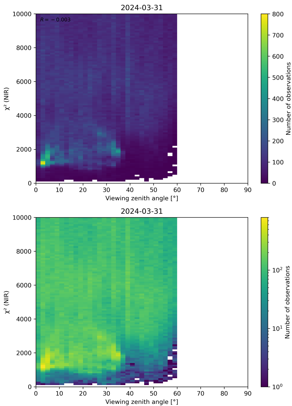
Figure 105: Scatter density plot of “Viewing zenith angle” against “ \chi^2 (NIR)” for 2024-03-31 to 2024-04-01.
