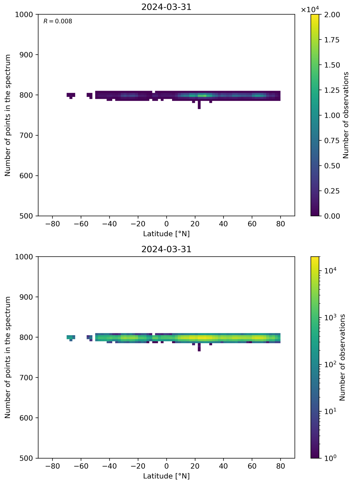
Figure 61: Scatter density plot of “Latitude” against “Number of points in the spectrum” for 2024-03-31 to 2024-04-01.
