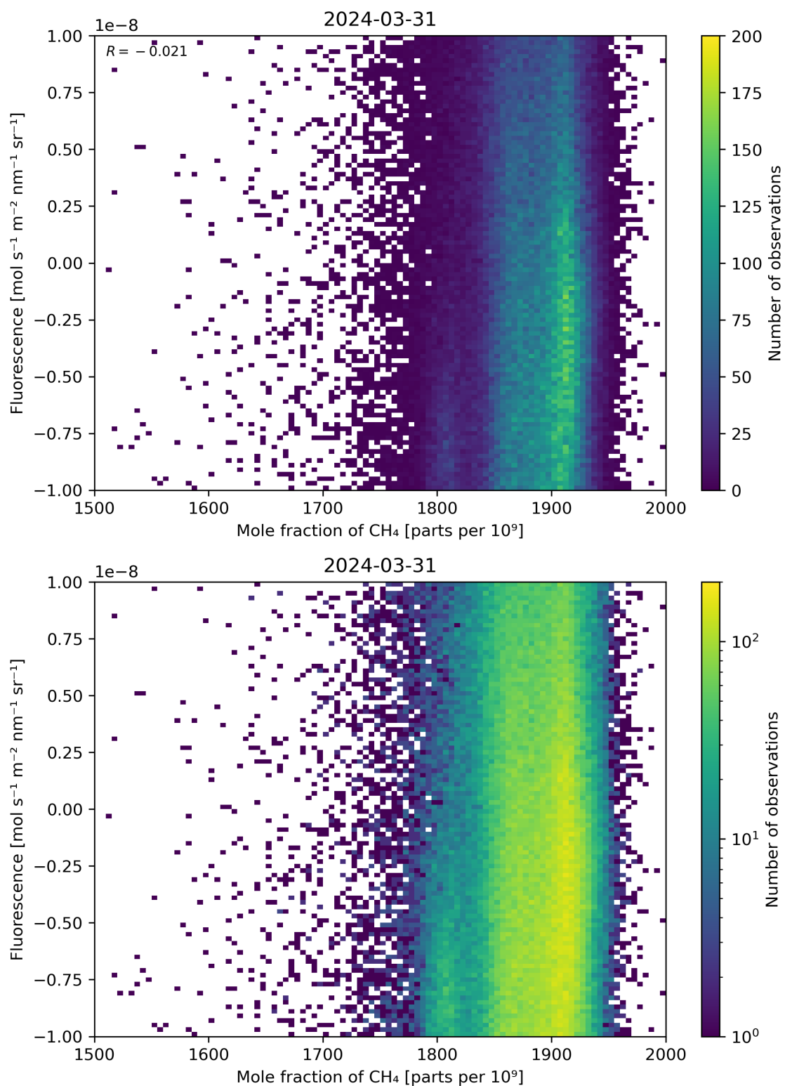
Figure 73: Scatter density plot of “Mole fraction of \text{CH}_4 ” against “Fluorescence” for 2024-03-31 to 2024-04-01.
