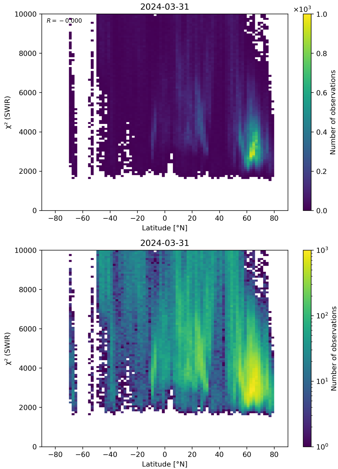
Figure 54: Scatter density plot of “Latitude” against “ \chi^2 (SWIR)” for 2024-03-31 to 2024-04-01.
