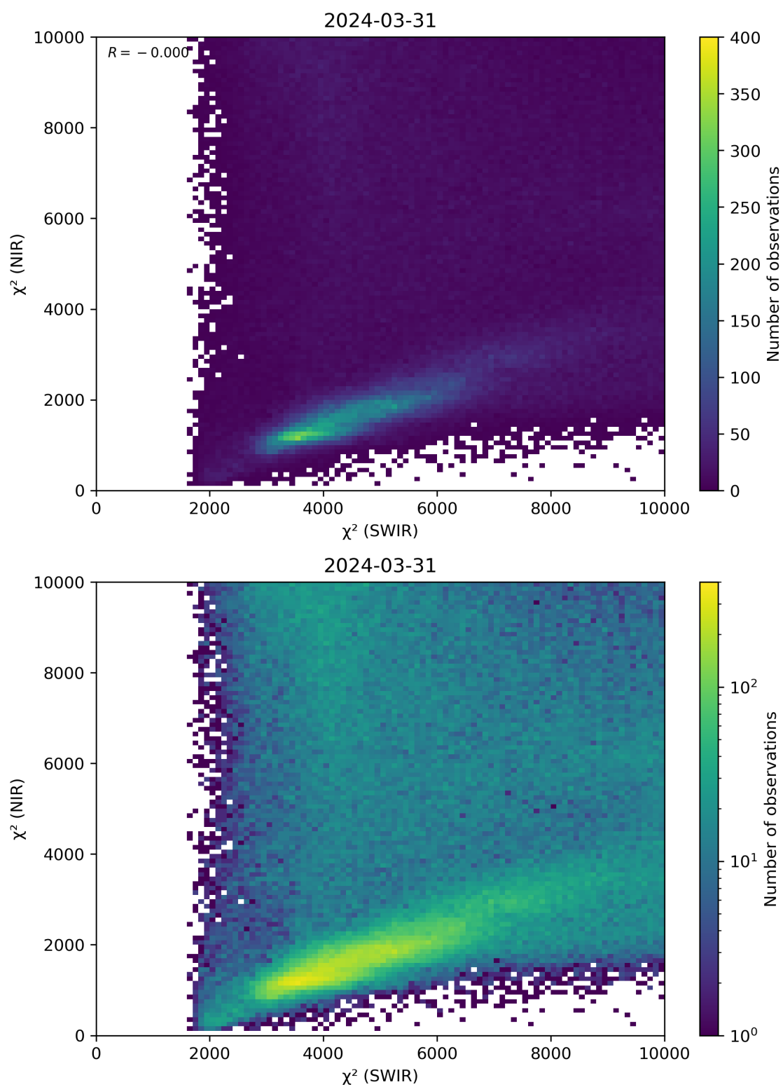
Figure 47: Scatter density plot of “ \chi^2 (SWIR)” against “ \chi^2 (NIR)” for 2024-03-31 to 2024-04-01.
