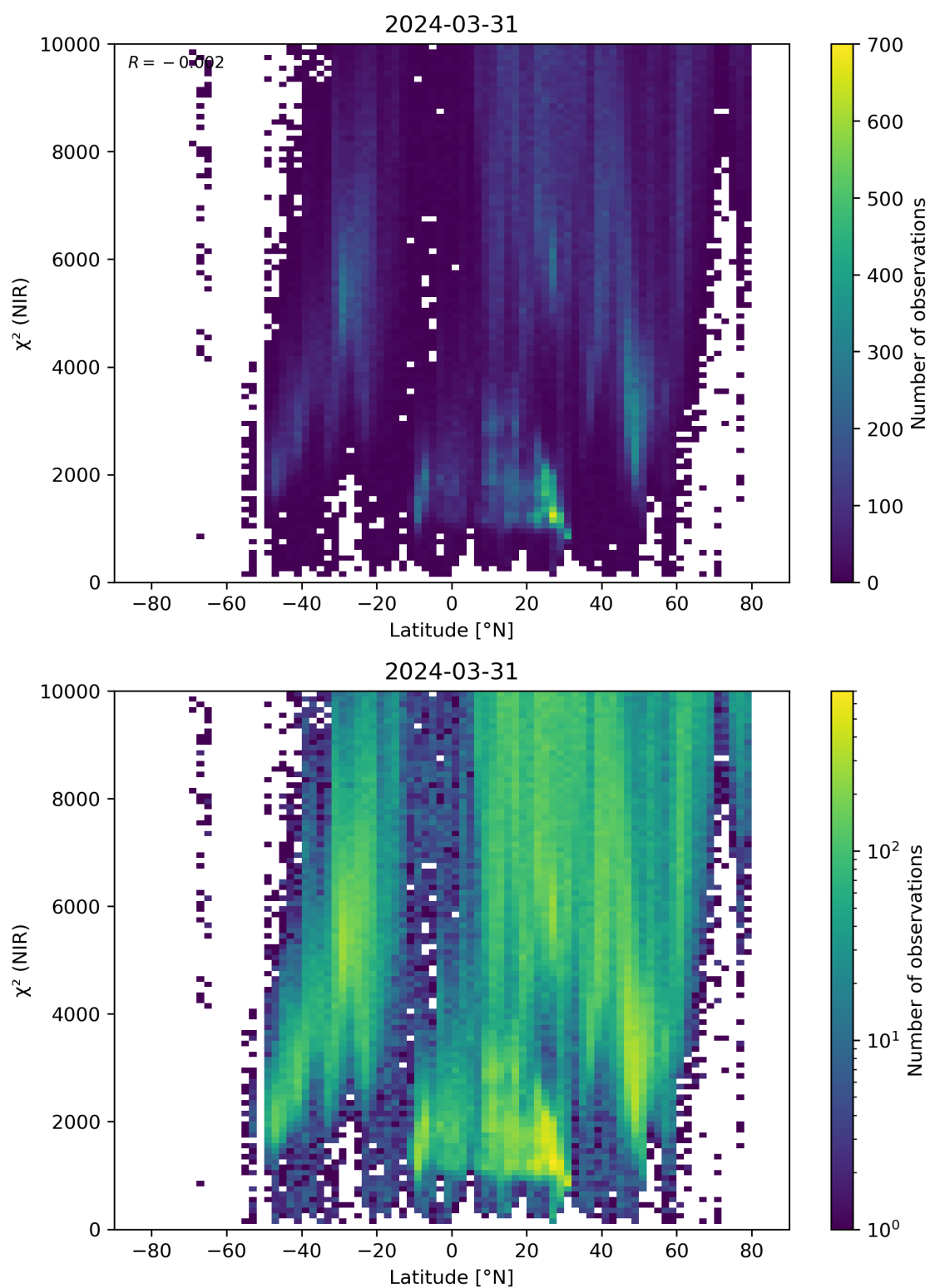
Figure 53: Scatter density plot of “Latitude” against “ \chi^2 (NIR)” for 2024-03-31 to 2024-04-01.
