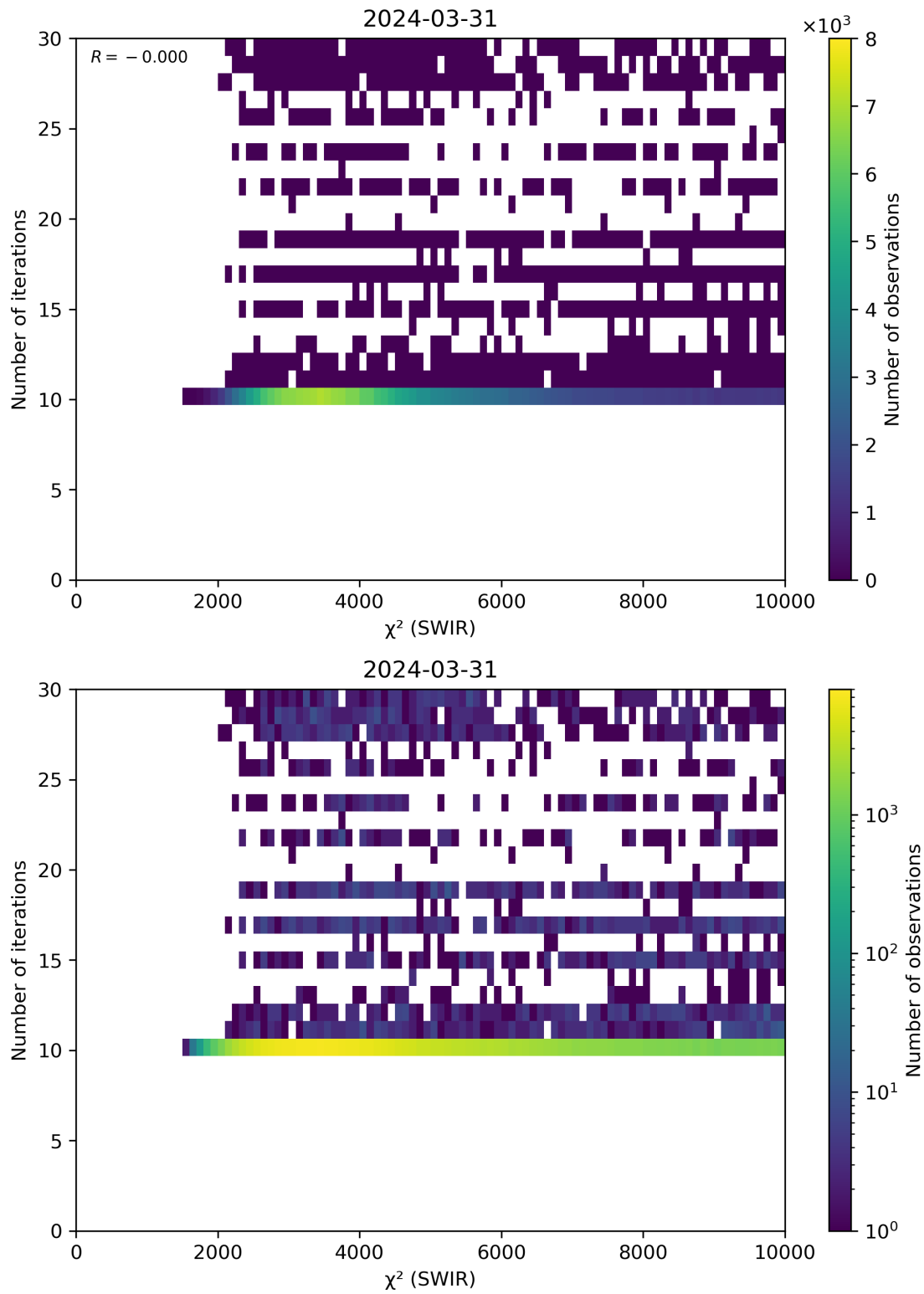
Figure 50: Scatter density plot of “ \chi^2 (SWIR)” against “Number of iterations” for 2024-03-31 to 2024-04-01.
