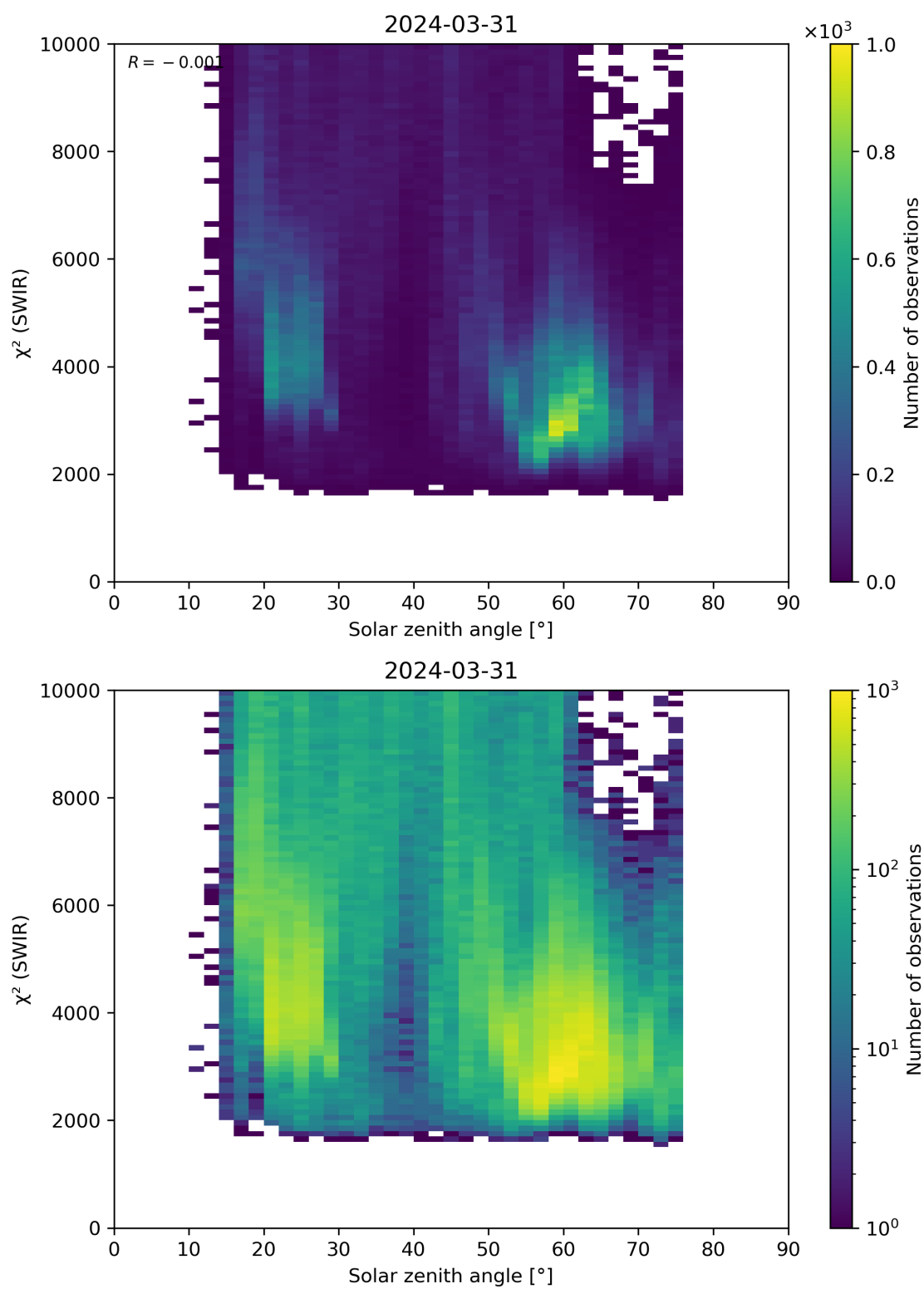
Figure 95: Scatter density plot of “Solar zenith angle” against “ \chi^2 (SWIR)” for 2024-03-31 to 2024-04-01.
