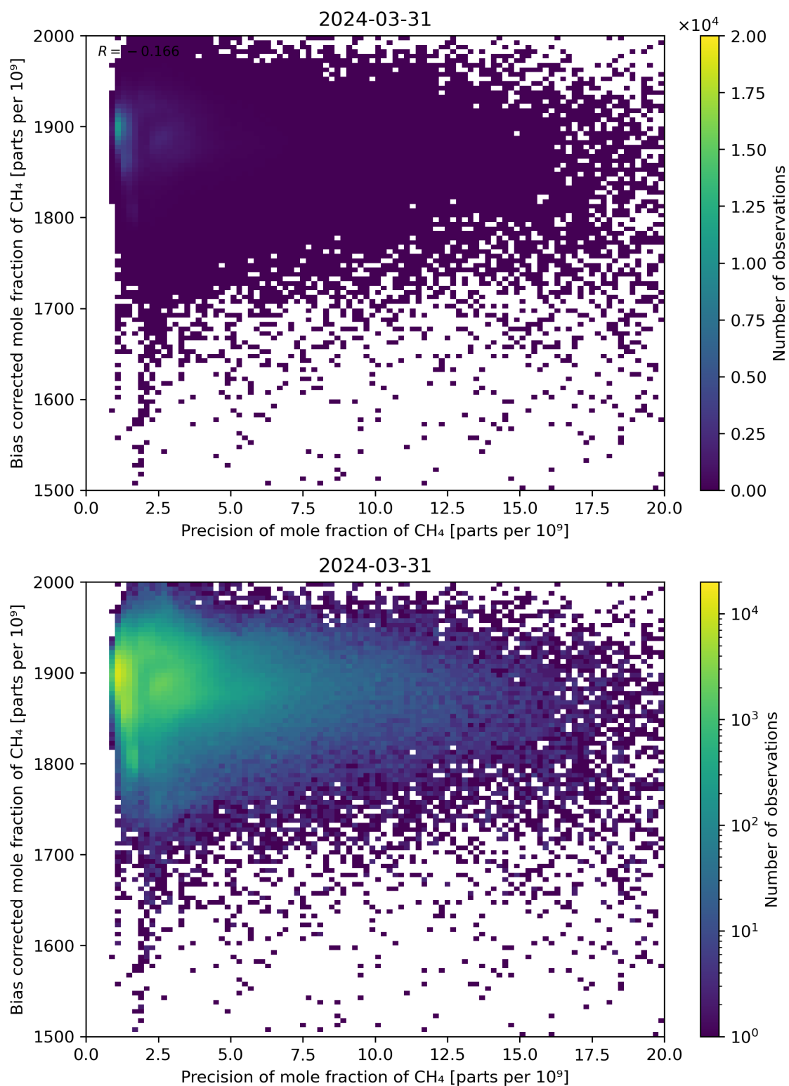
Figure 82: Scatter density plot of “Precision of mole fraction of CH 4 ” against “Bias corrected mole fraction of CH 4 ” for 2024-03-31 to 2024-04-01.
