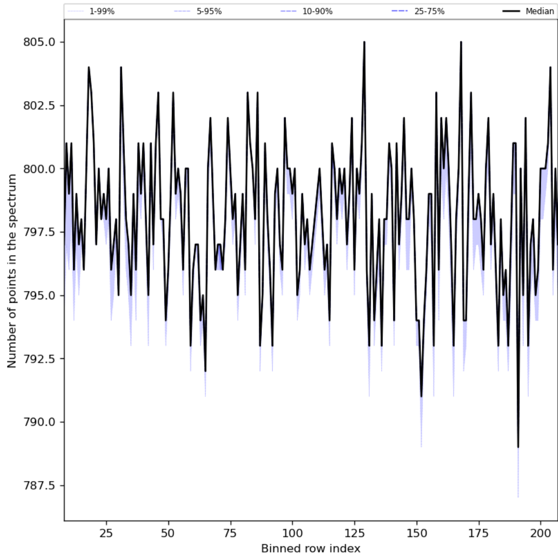
Figure 37: Along track statistics of “Number of points in the spectrum” for 2024-03-31 to 2024-04-01
