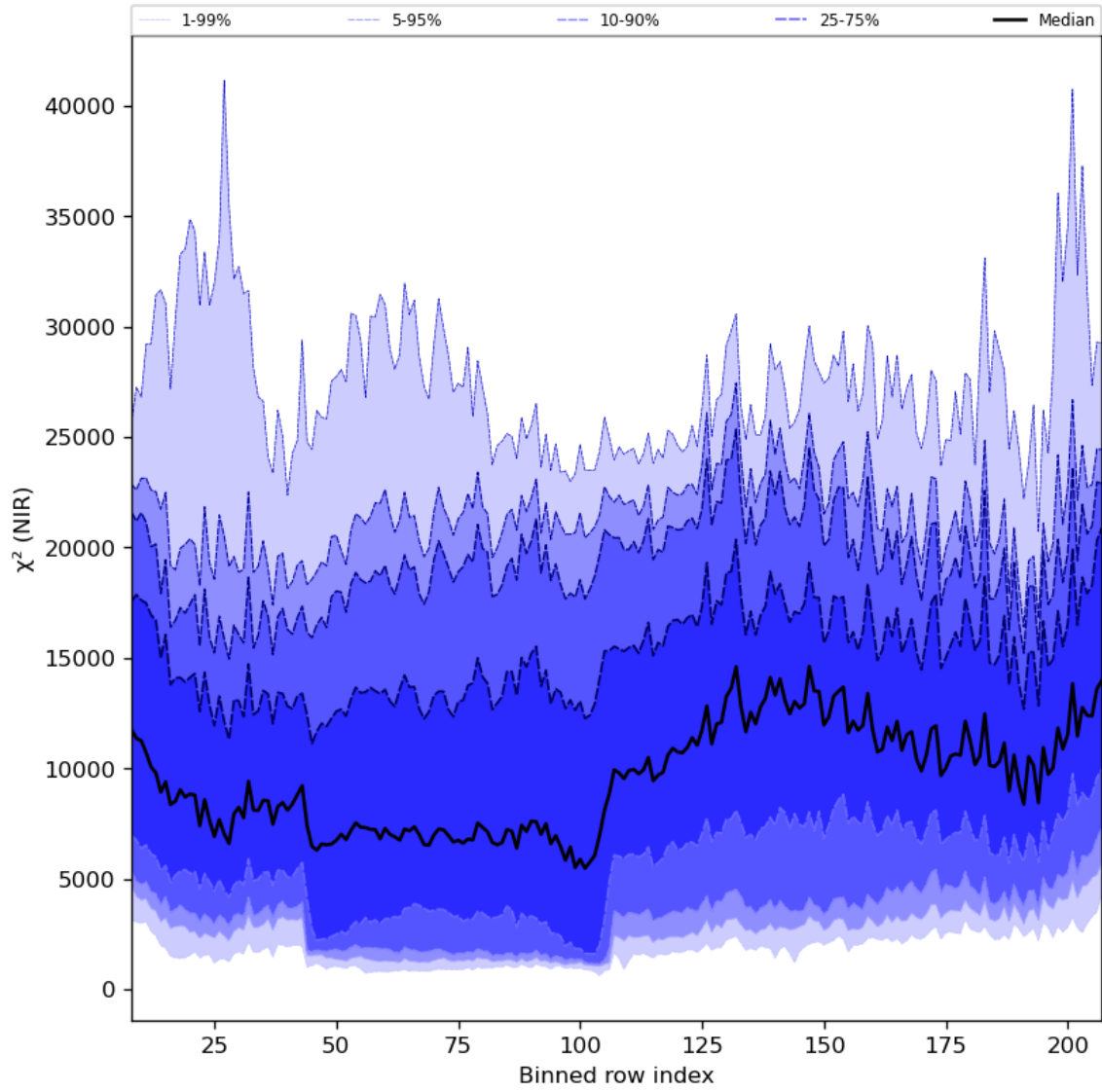
Figure 40: Along track statistics of “ \chi^2 (NIR)” for 2024-03-31 to 2024-04-01
