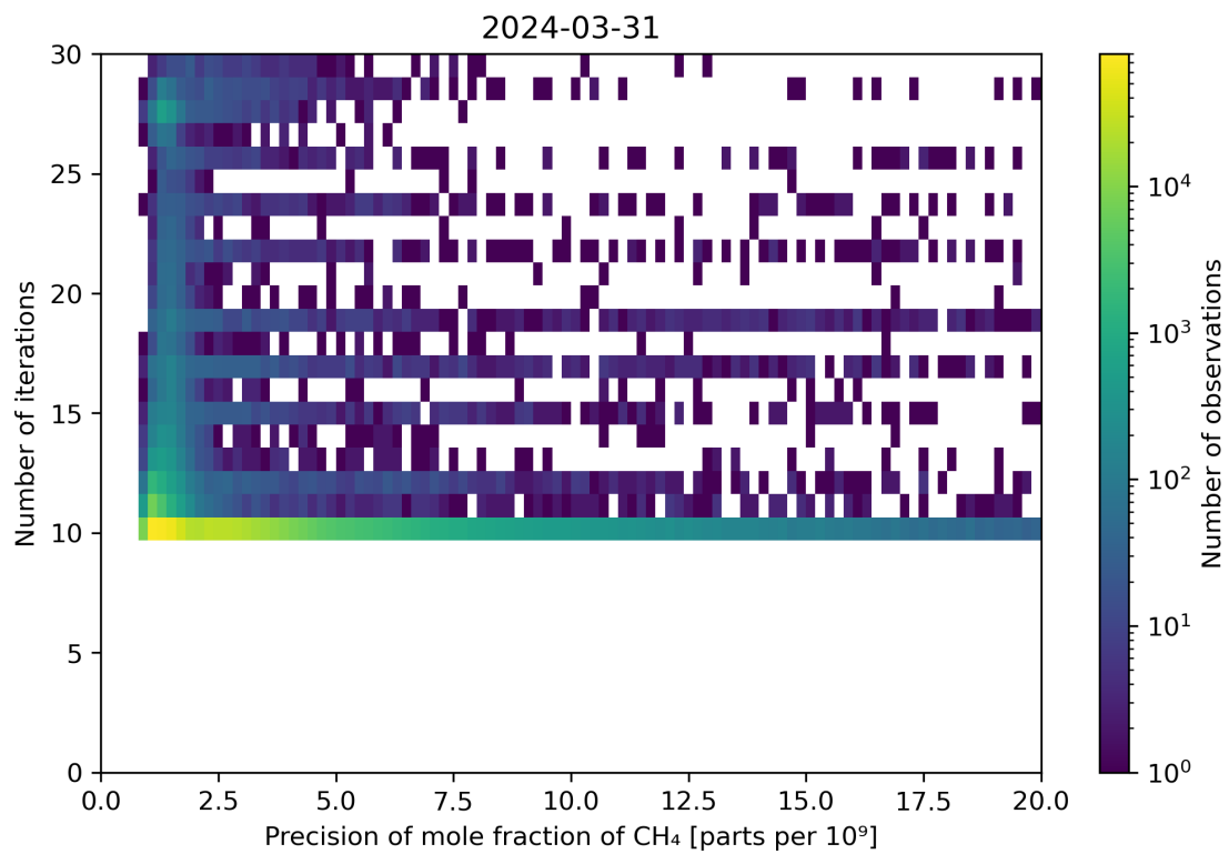
Figure 83: Scatter density plot of “Precision of mole fraction of CH 4 ” against “Number of iterations” for 2024-03-31 to 2024-04-01.
