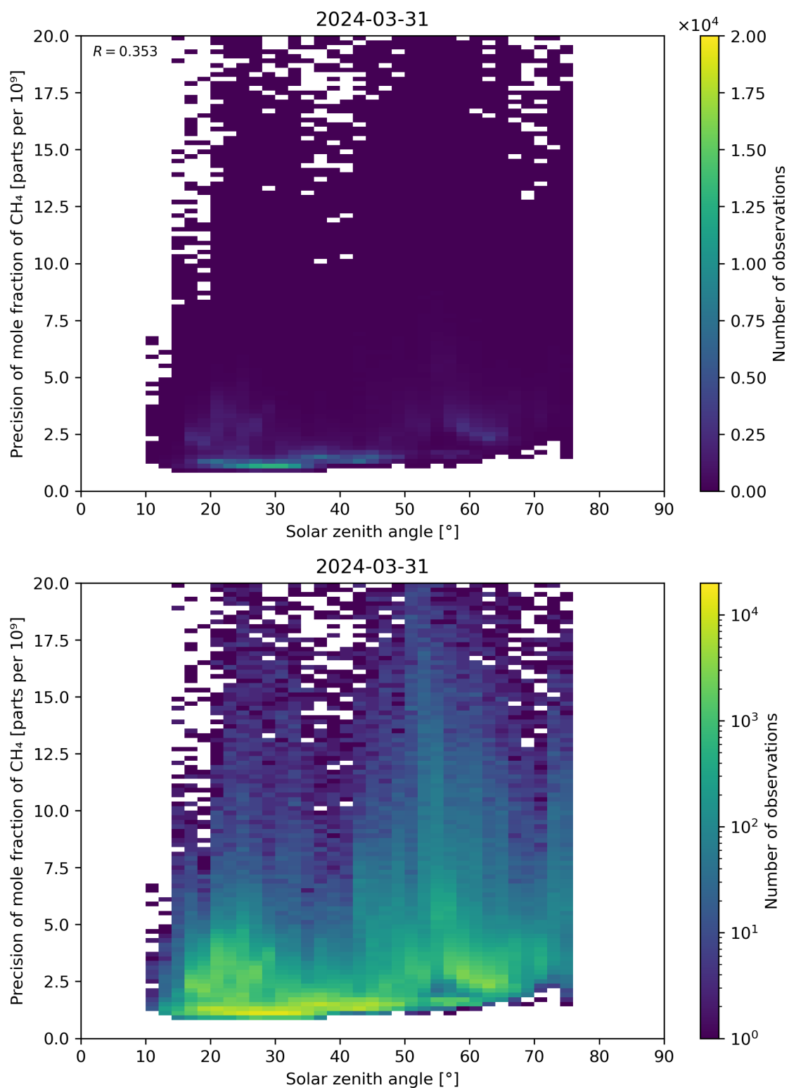
Figure 101: Scatter density plot of “Solar zenith angle” against “Precision of mole fraction of CH 4 ” for 2024-03-31 to 2024-04-01.
