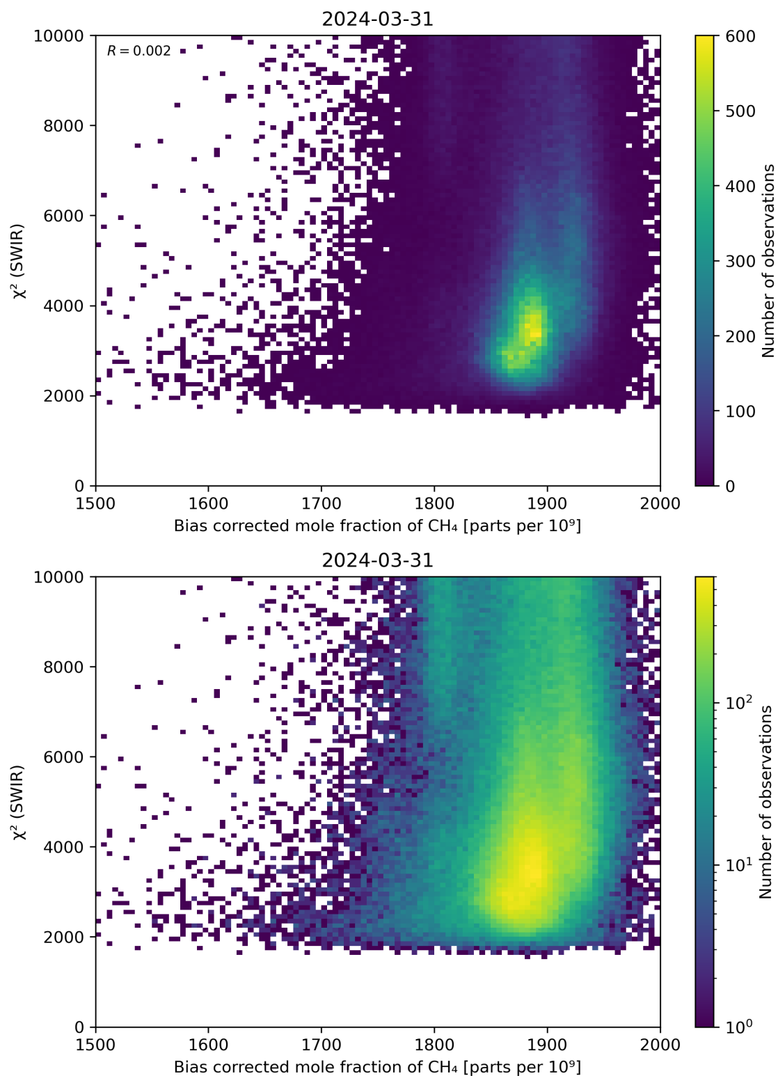
Figure 64: Scatter density plot of “Bias corrected mole fraction of CH 4 ” against “ \chi^2 (SWIR)” for 2024-03-31 to 2024-04-01.
