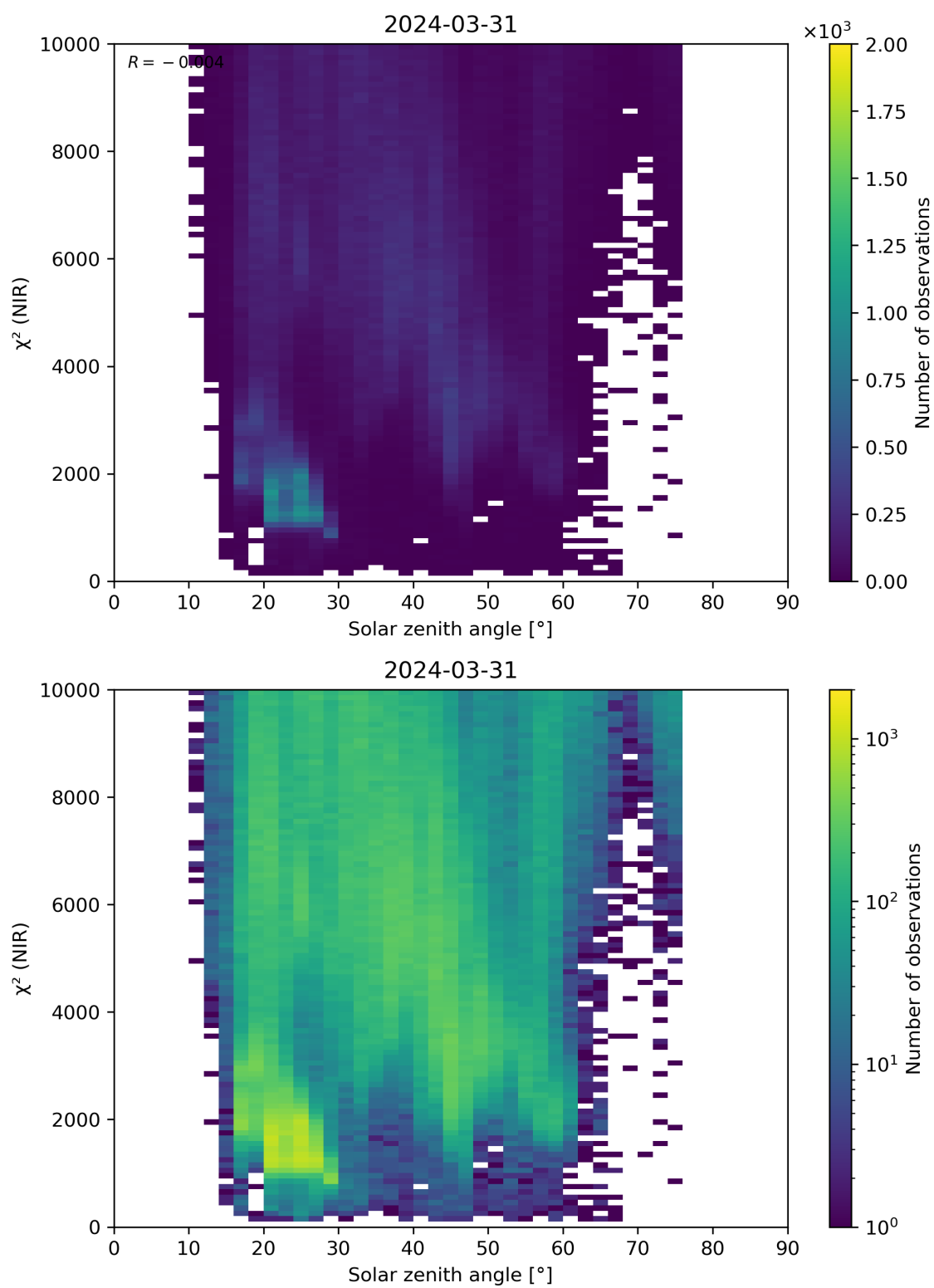
Figure 94: Scatter density plot of “Solar zenith angle” against “ \chi^2 (NIR)” for 2024-03-31 to 2024-04-01.
