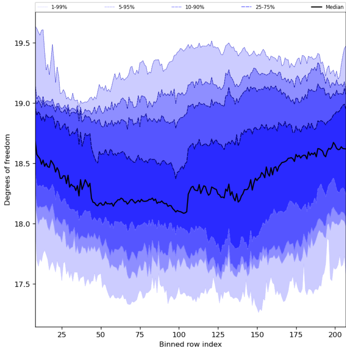
Figure 41: Along track statistics of “Degrees of freedom” for 2024-03-31 to 2024-04-01
