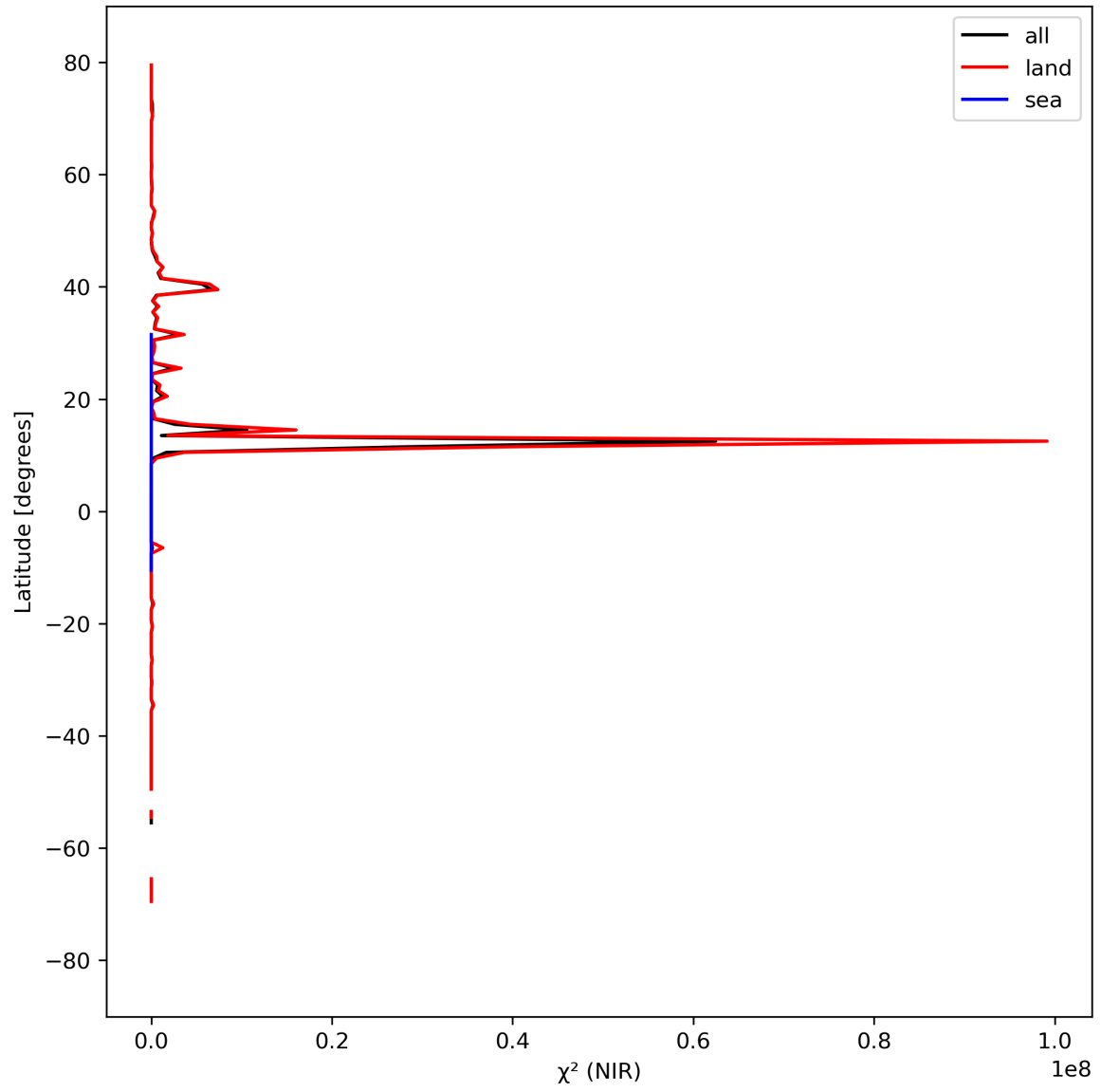
Figure 18: Zonal average of “ \chi^2 (NIR)” for 2024-03-31 to 2024-04-01.
