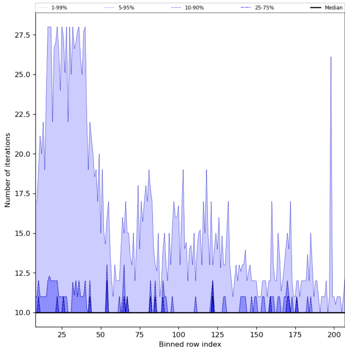
Figure 42: Along track statistics of “Number of iterations” for 2024-03-31 to 2024-04-01
