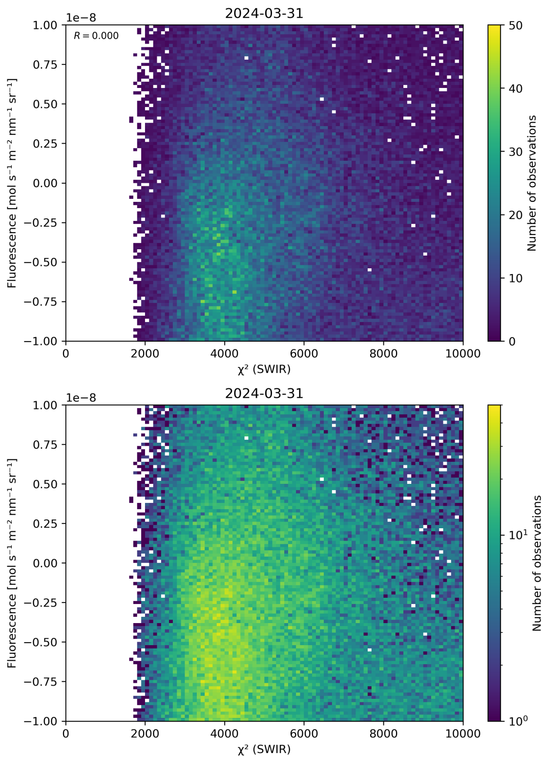
Figure 49: Scatter density plot of “ \chi^2 (SWIR)” against “Fluorescence” for 2024-03-31 to 2024-04-01.
