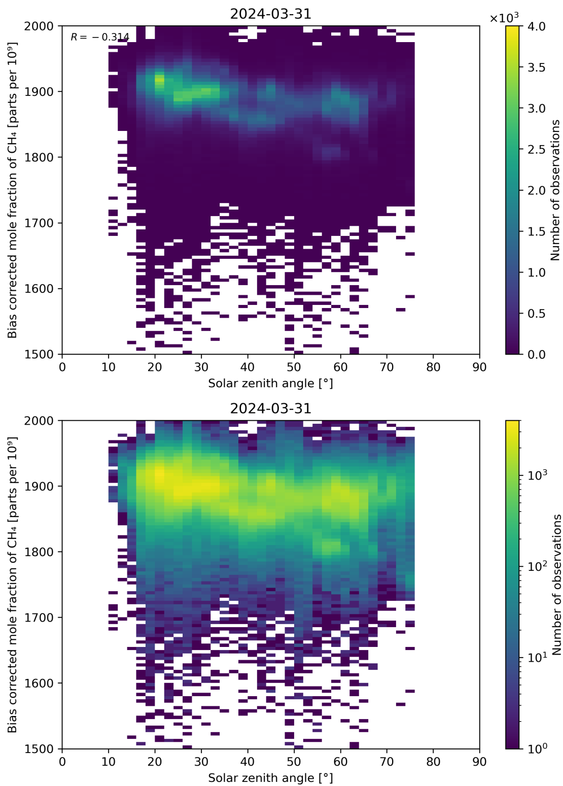
Figure 100: Scatter density plot of “Solar zenith angle” against “Bias corrected mole fraction of CH 4 ” for 2024-03-31 to 2024-04-01.
