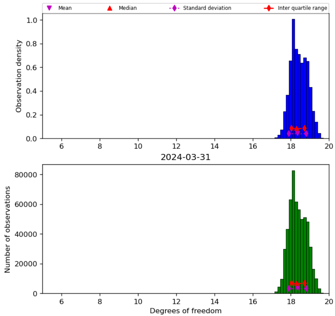
Figure 30: Histogram of “Degrees of freedom” for 2024-03-31 to 2024-04-01
