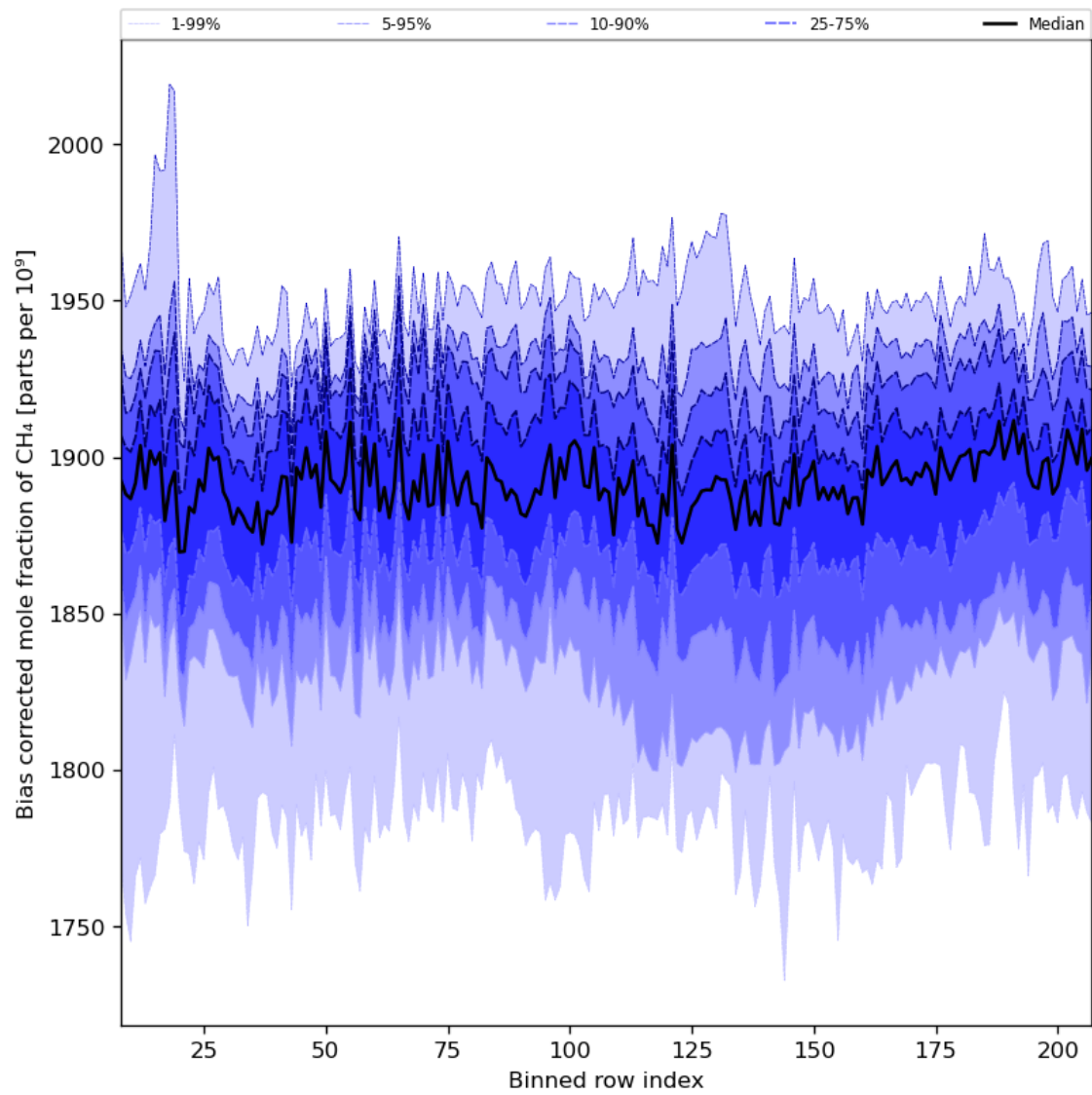
Figure 36: Along track statistics of “Bias corrected mole fraction of CH 4 ” for 2024-03-31 to 2024-04-01
