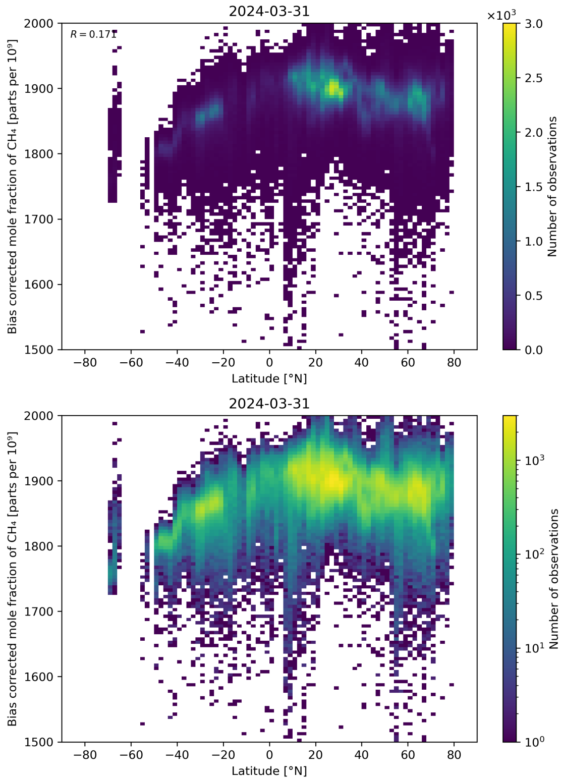
Figure 58: Scatter density plot of “Latitude” against “Bias corrected mole fraction of CH 4 ” for 2024-03-31 to 2024-04-01.
