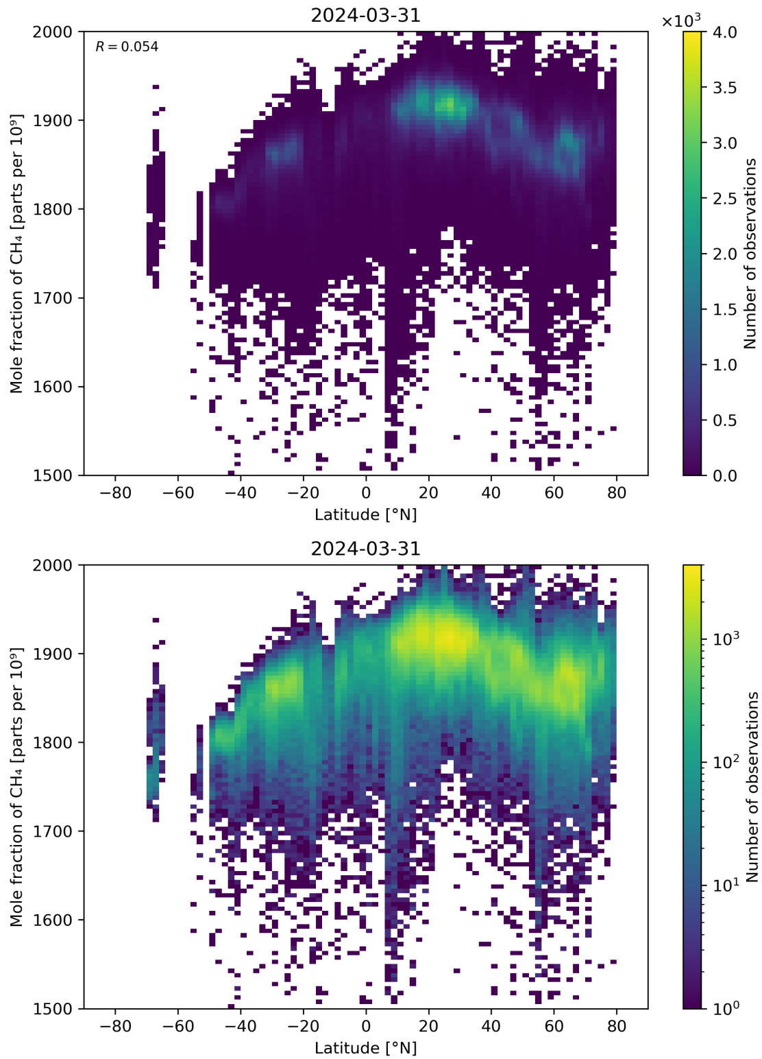
Figure 57: Scatter density plot of “Latitude” against “Mole fraction of \text{CH}_4 ” for 2024-03-31 to 2024-04-01.
