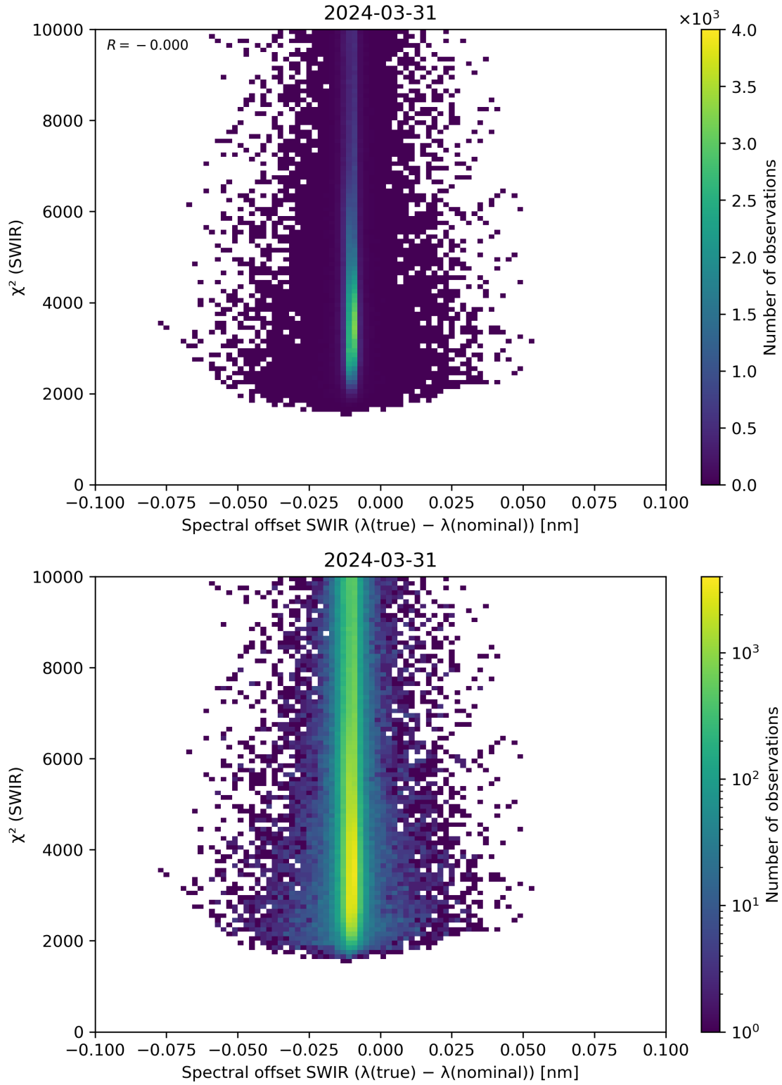
Figure 118: Scatter density plot of “Spectral offset SWIR ( \lambda(\text{true}) - \lambda(\text{nominal}) )” against “ \chi^2 (SWIR)” for 2024-03-31 to 2024-04-01.
