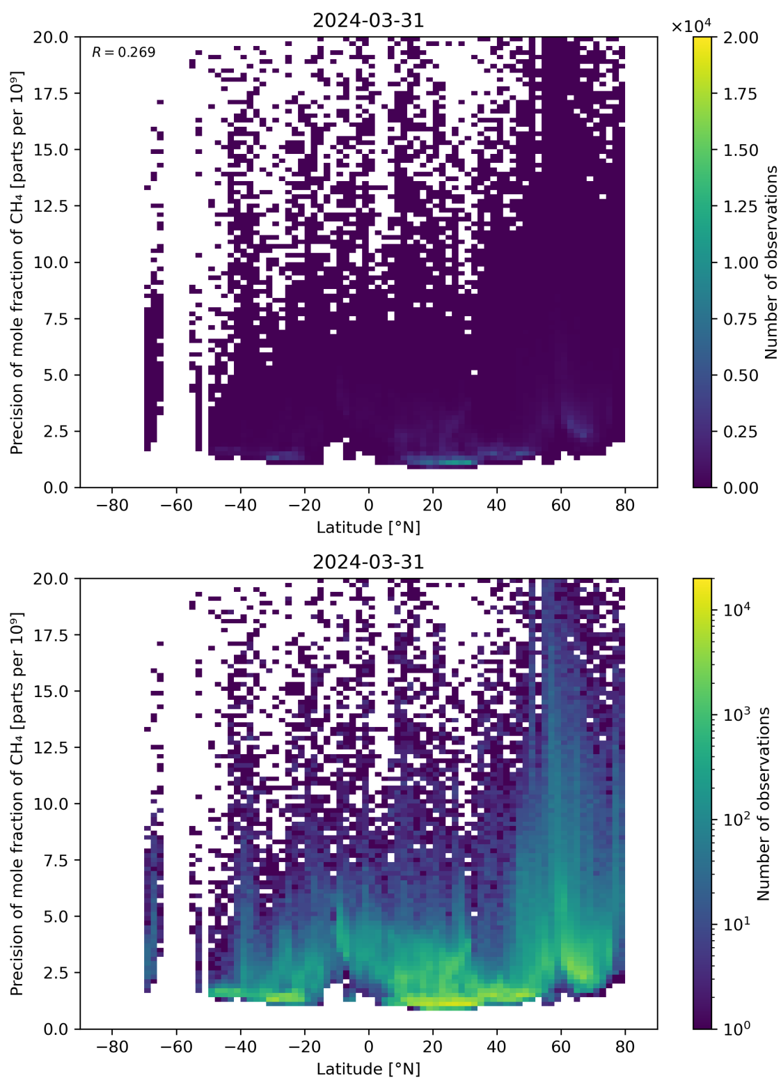
Figure 59: Scatter density plot of “Latitude” against “Precision of mole fraction of \text{CH}_4 ” for 2024-03-31 to 2024-04-01.
