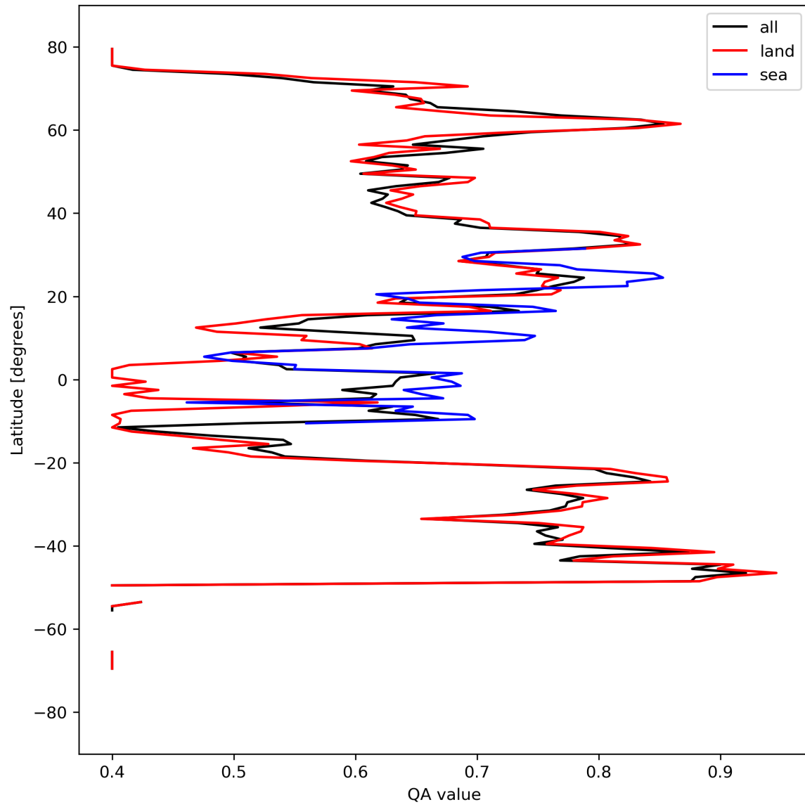
Figure 11: Zonal average of “QA value” for 2024-03-31 to 2024-04-01.
