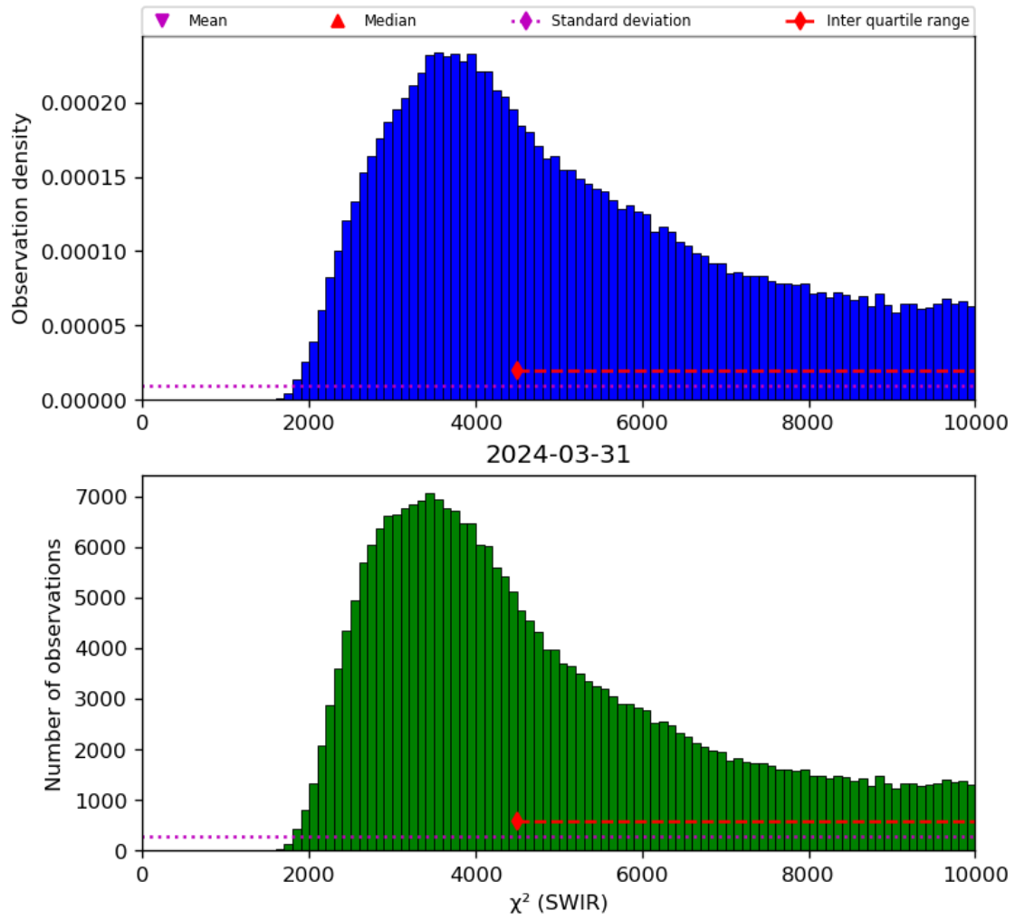
Figure 28: Histogram of “ \chi^2 (SWIR)” for 2024-03-31 to 2024-04-01
