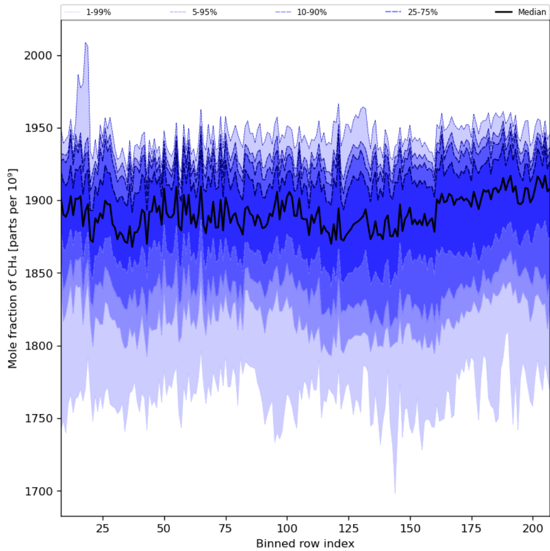
Figure 34: Along track statistics of “Mole fraction of CH 4 ” for 2024-03-31 to 2024-04-01
