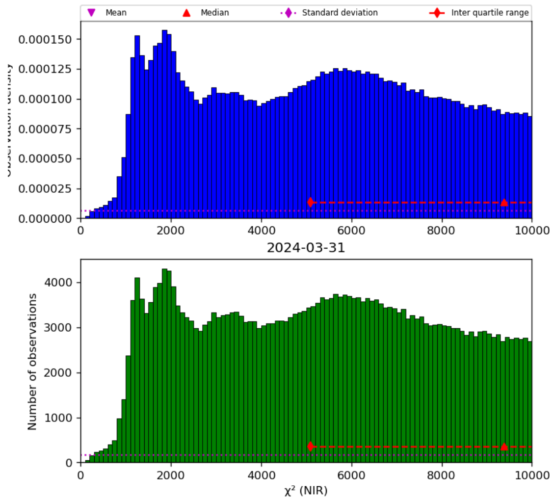
Figure 29: Histogram of “ \chi^2 (NIR)” for 2024-03-31 to 2024-04-01
