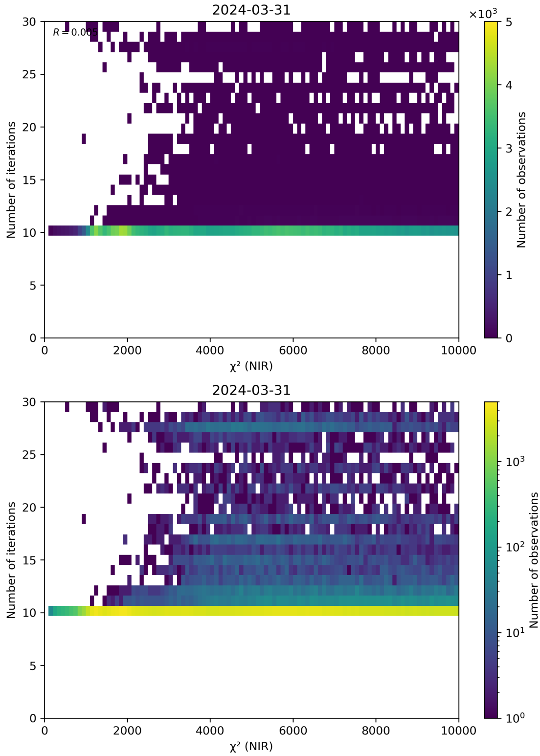
Figure 46: Scatter density plot of “ \chi^2 (NIR)” against “Number of iterations” for 2024-03-31 to 2024-04-01.
