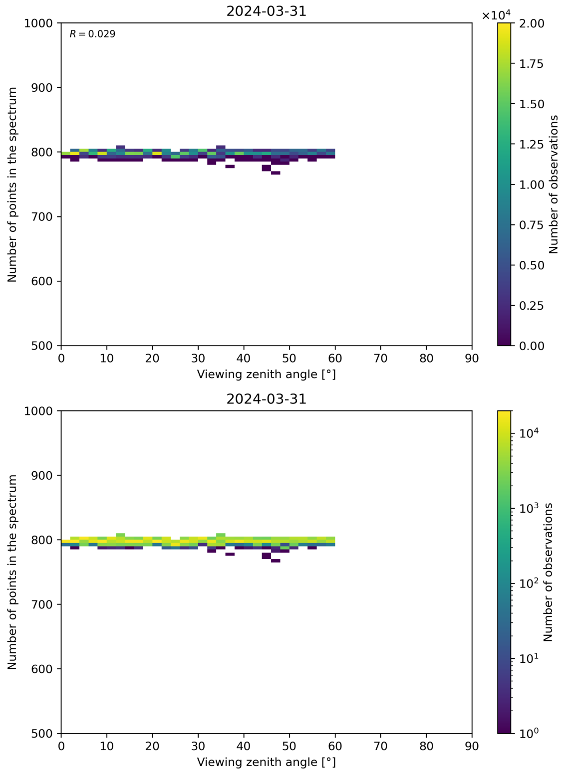
Figure 114: Scatter density plot of “Viewing zenith angle” against “Number of points in the spectrum” for 2024-03-31 to 2024-04-01.
