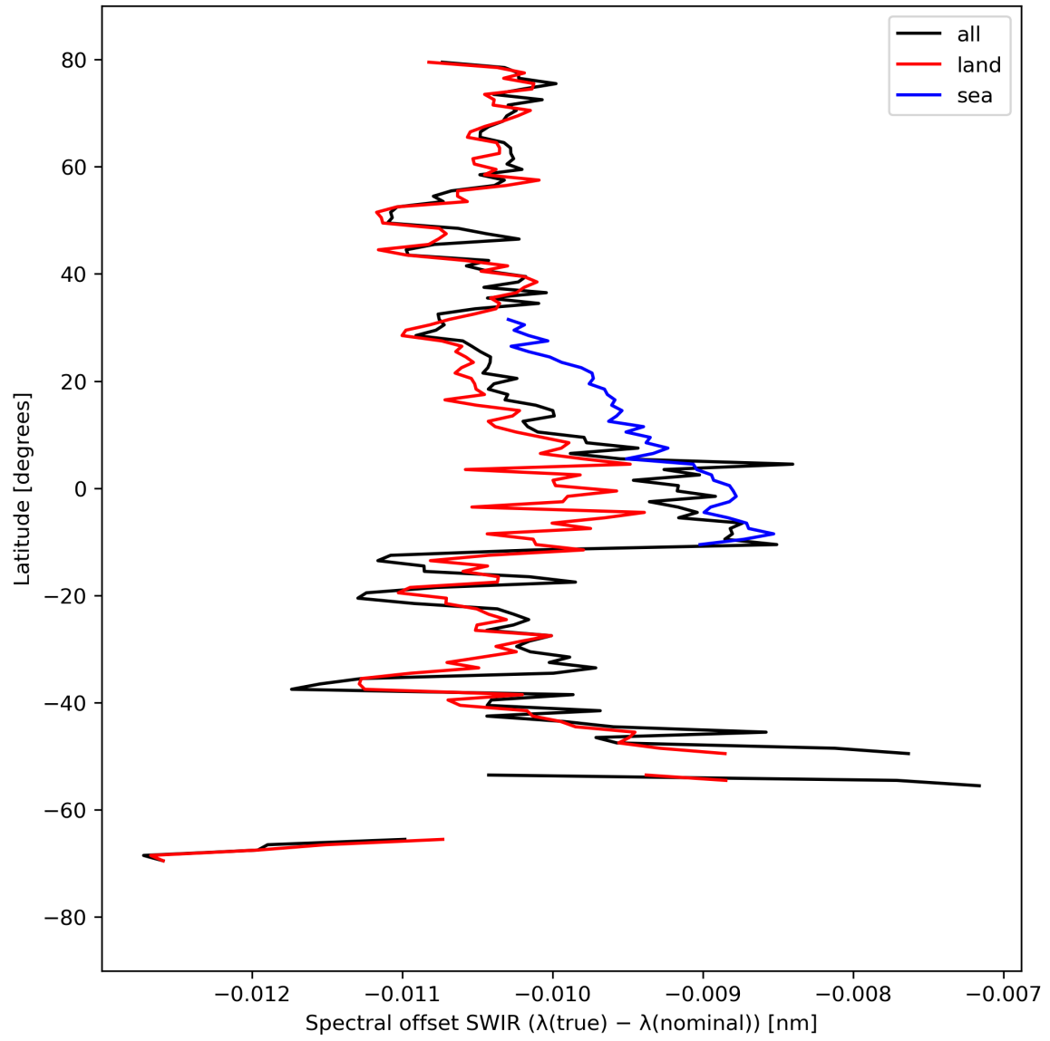
Figure 16: Zonal average of “Spectral offset SWIR ( \lambda(\text{true}) - \lambda(\text{nominal}) )” for 2024-03-31 to 2024-04-01.
