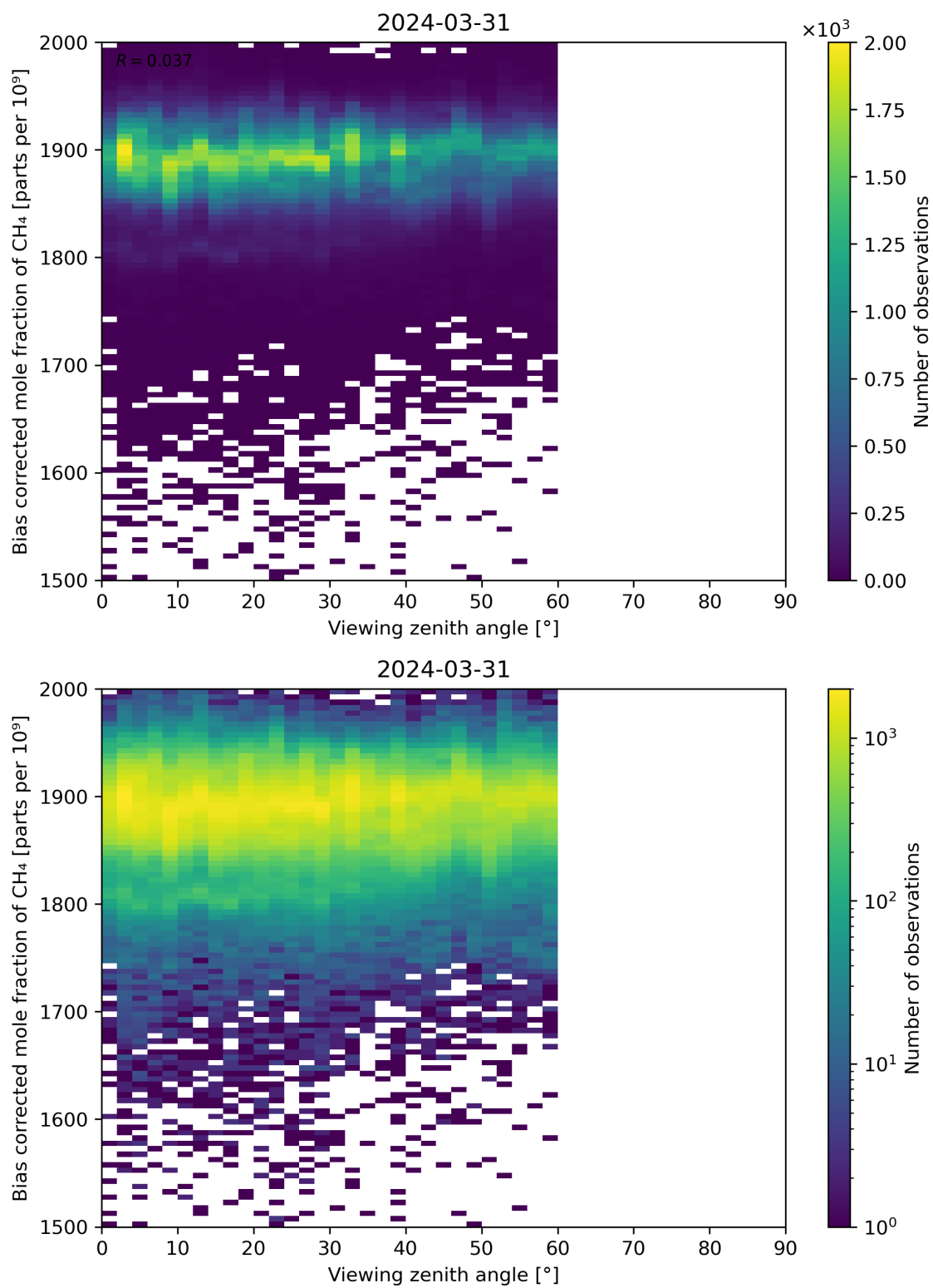
Figure 111: Scatter density plot of “Viewing zenith angle” against “Bias corrected mole fraction of CH 4 ” for 2024-03-31 to 2024-04-01.
