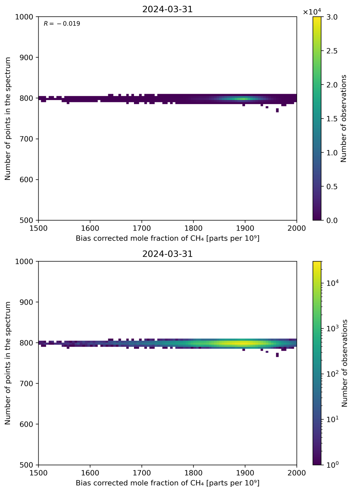
Figure 68: Scatter density plot of “Bias corrected mole fraction of CH 4 ” against “Number of points in the spectrum” for 2024-03-31 to 2024-04-01.
