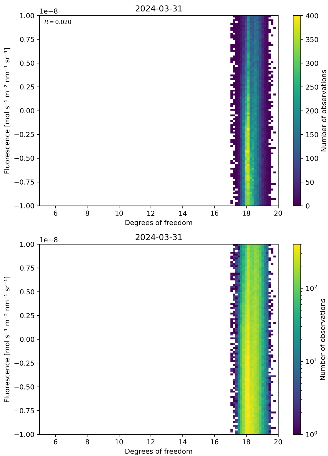
Figure 51: Scatter density plot of “Degrees of freedom” against “Fluorescence” for 2024-03-31 to 2024-04-01.
