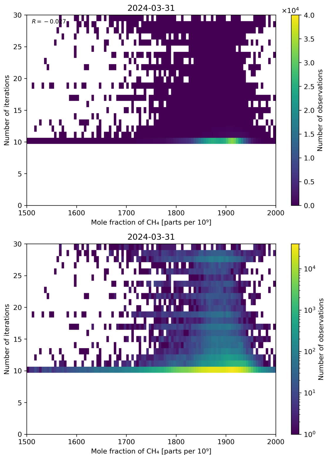
Figure 76: Scatter density plot of “Mole fraction of CH 4 ” against “Number of iterations” for 2024-03-31 to 2024-04-01.
