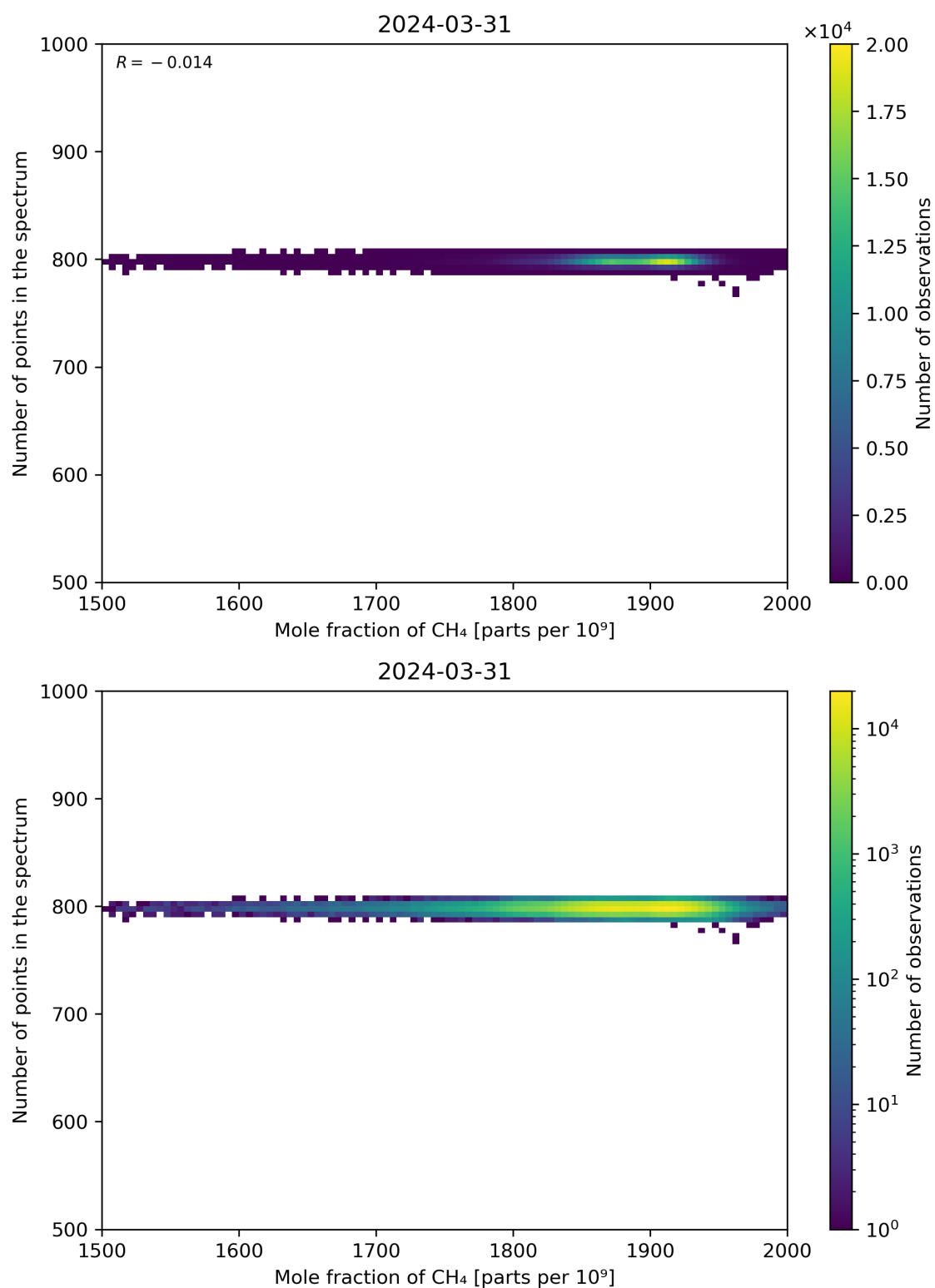
Figure 77: Scatter density plot of “Mole fraction of CH 4 ” against “Number of points in the spectrum” for 2024-03-31 to 2024-04-01.
