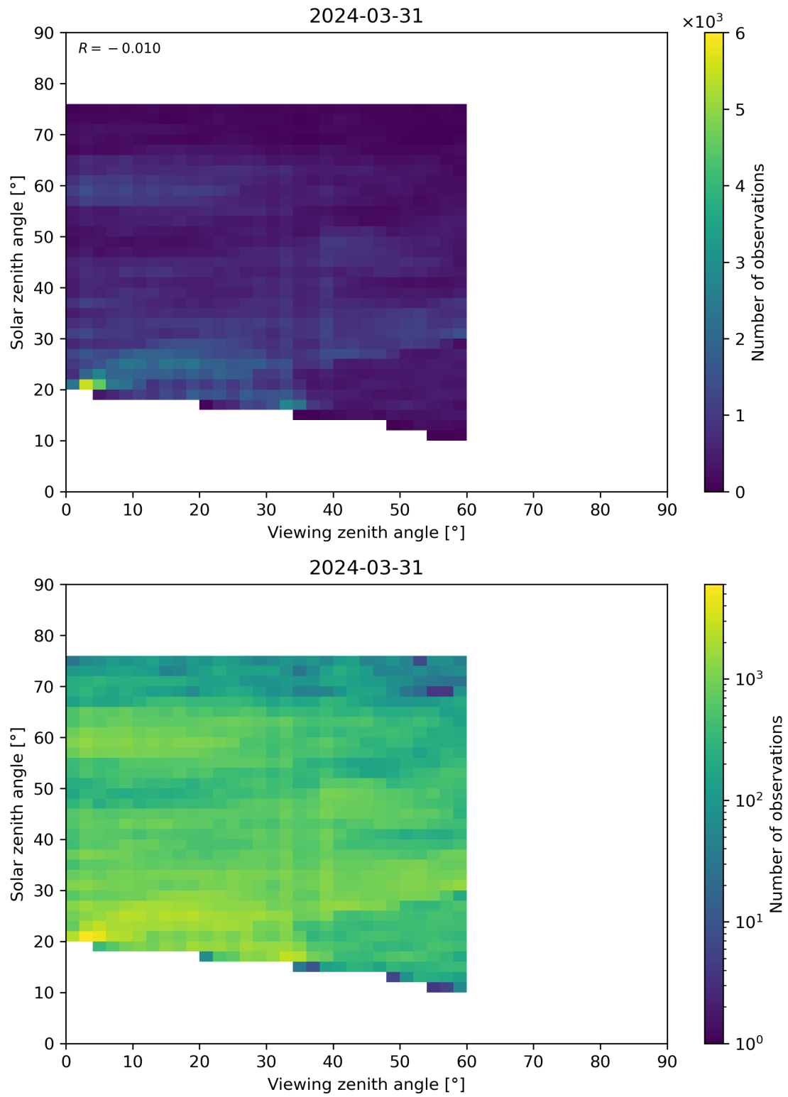
Figure 115: Scatter density plot of “Viewing zenith angle” against “Solar zenith angle” for 2024-03-31 to 2024-04-01.
