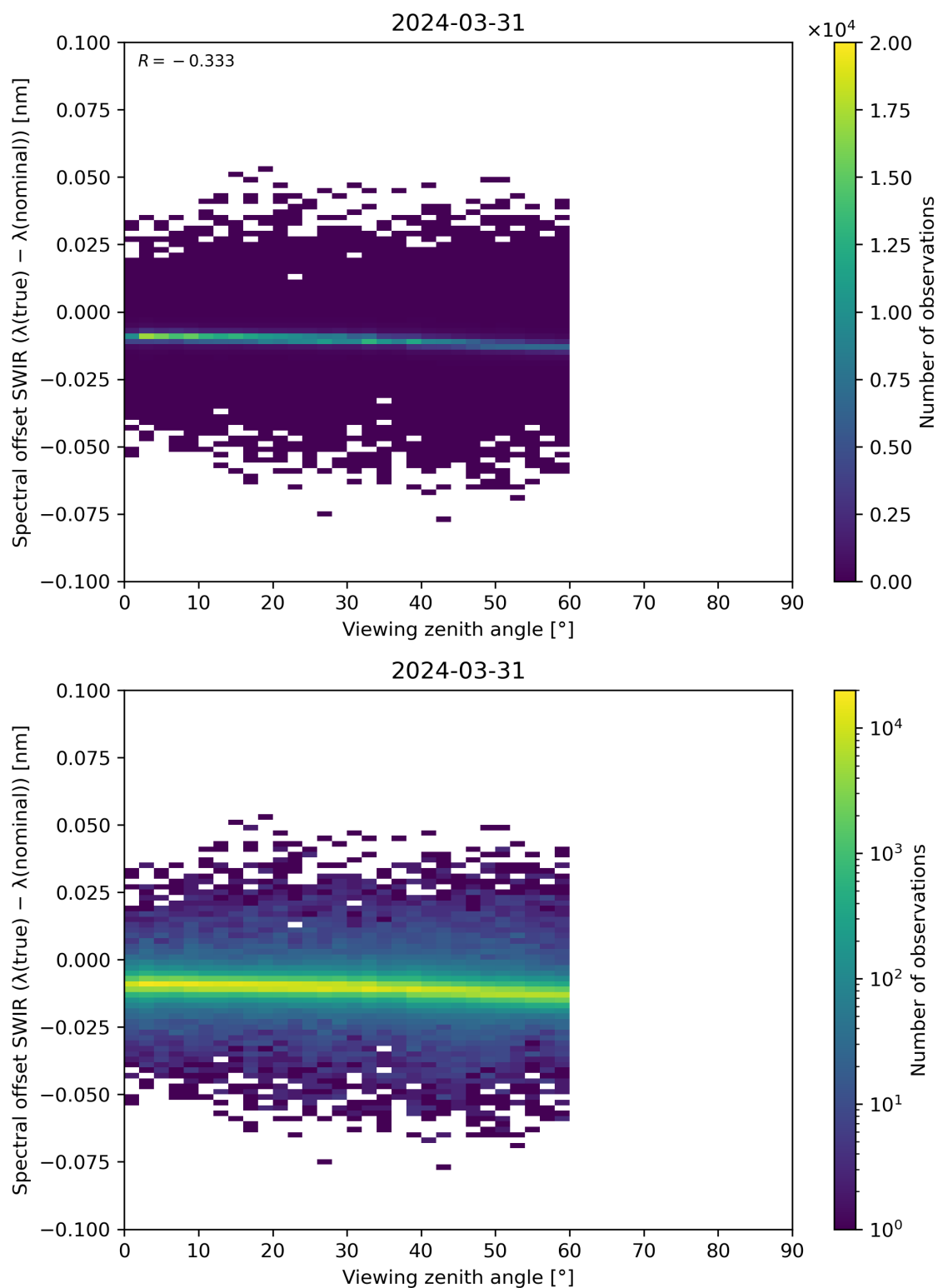
Figure 116: Scatter density plot of “Viewing zenith angle” against “Spectral offset SWIR ( \lambda(\text{true}) - \lambda(\text{nominal}) )” for 2024-03-31 to 2024-04-01.
