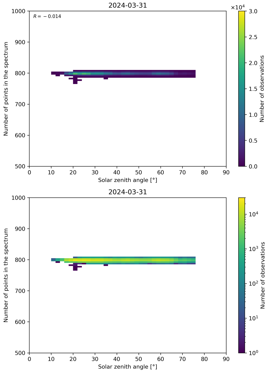
Figure 103: Scatter density plot of “Solar zenith angle” against “Number of points in the spectrum” for 2024-03-31 to 2024-04-01.
