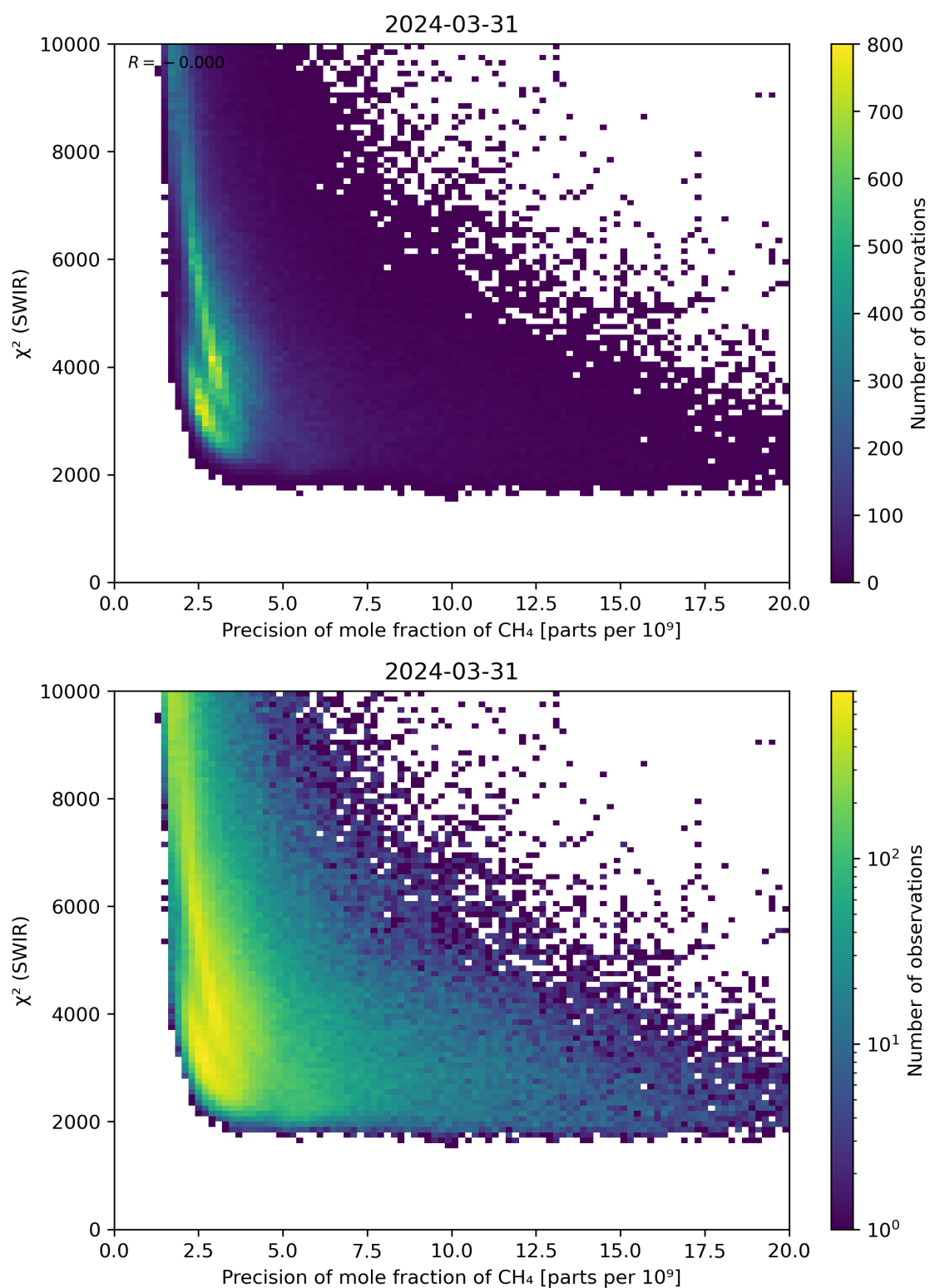
Figure 79: Scatter density plot of “Precision of mole fraction of \text{CH}_4 ” against “ \chi^2 (SWIR)” for 2024-03-31 to 2024-04-01.
