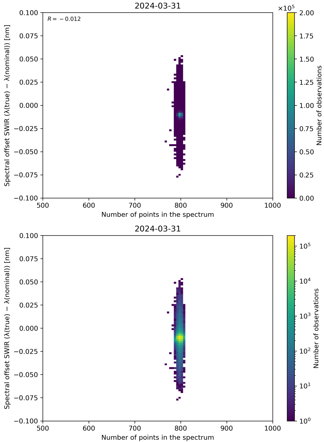
Figure 93: Scatter density plot of “Number of points in the spectrum” against “Spectral offset SWIR ( \lambda(\text{true}) - \lambda(\text{nominal}) )” for 2024-03-31 to 2024-04-01.
