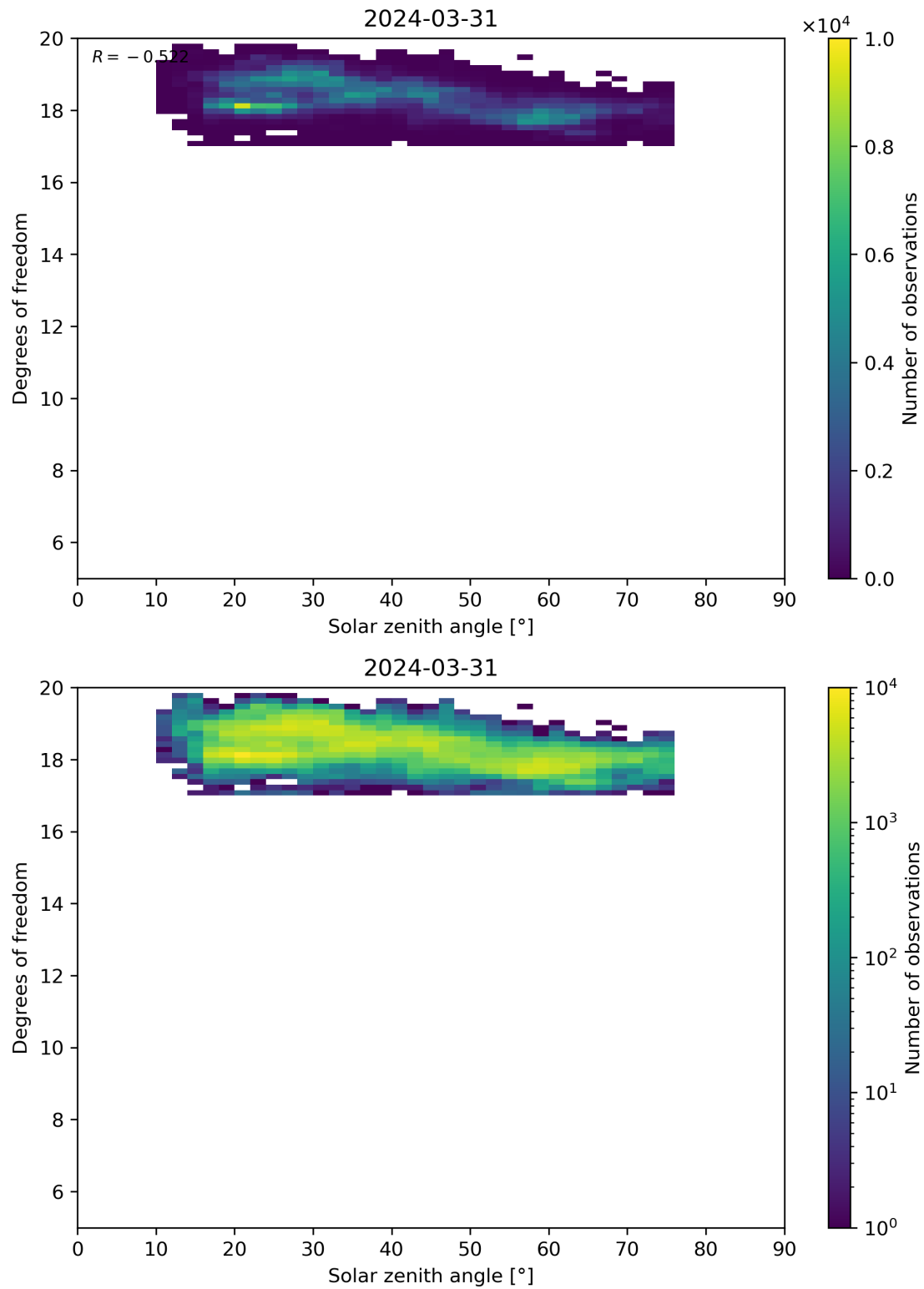
Figure 96: Scatter density plot of “Solar zenith angle” against “Degrees of freedom” for 2024-03-31 to 2024-04-01.
