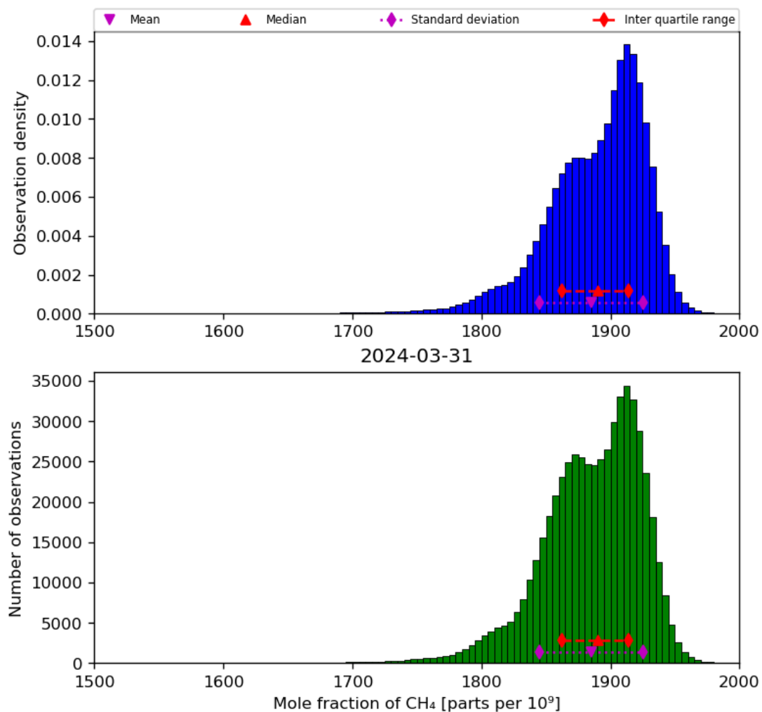
Figure 23: Histogram of “Mole fraction of CH 4 ” for 2024-03-31 to 2024-04-01
