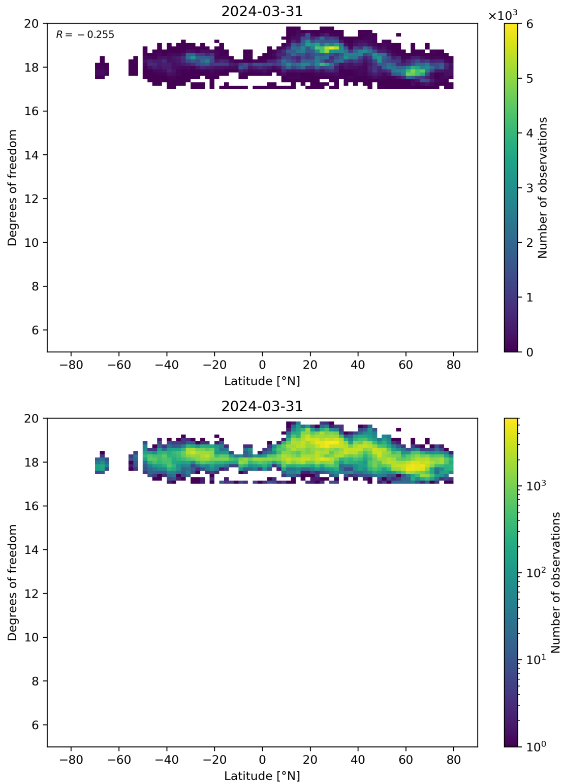
Figure 55: Scatter density plot of “Latitude” against “Degrees of freedom” for 2024-03-31 to 2024-04-01.
