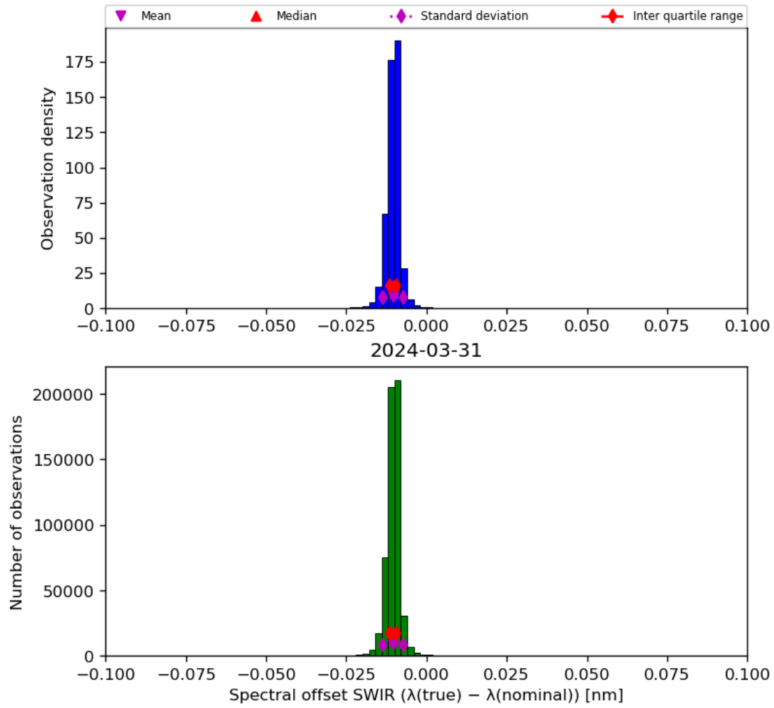
Figure 27: Histogram of “Spectral offset SWIR ( \lambda(\text{true}) - \lambda(\text{nominal}) )” for 2024-03-31 to 2024-04-01
