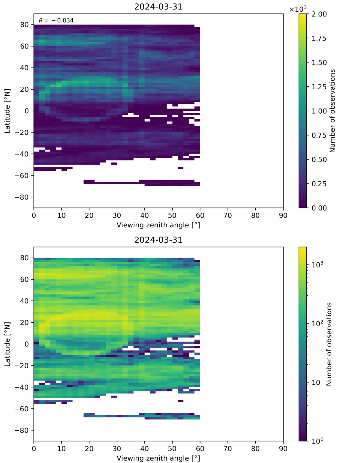
Figure 109: Scatter density plot of “Viewing zenith angle” against “Latitude” for 2024-03-31 to 2024-04-01.
