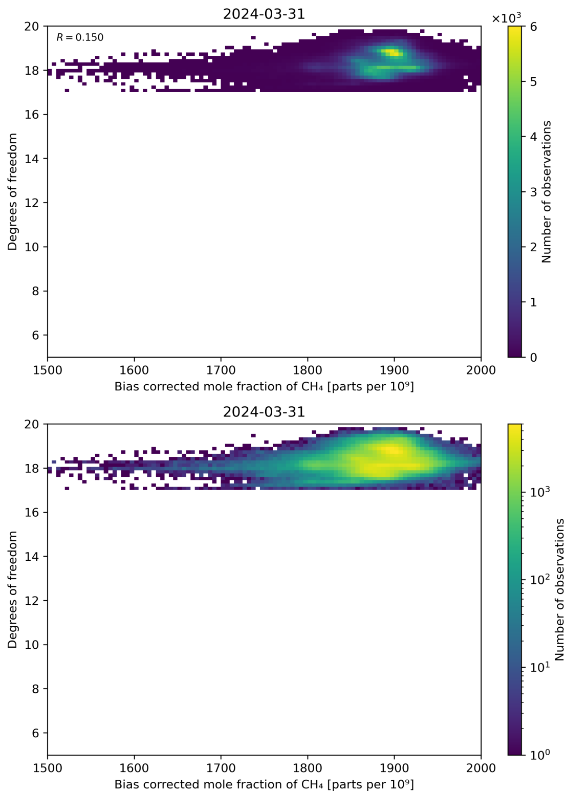
Figure 65: Scatter density plot of “Bias corrected mole fraction of CH 4 ” against “Degrees of freedom” for 2024-03-31 to 2024-04-01.
