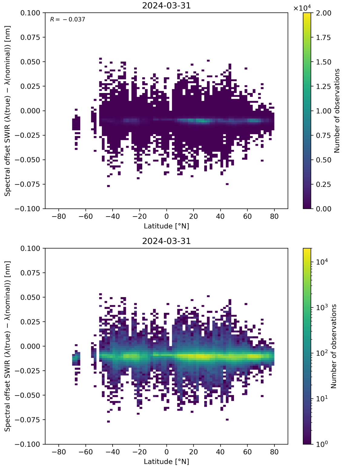
Figure 62: Scatter density plot of “Latitude” against “Spectral offset SWIR ( \lambda(\text{true}) - \lambda(\text{nominal}) )” for 2024-03-31 to 2024-04-01.
