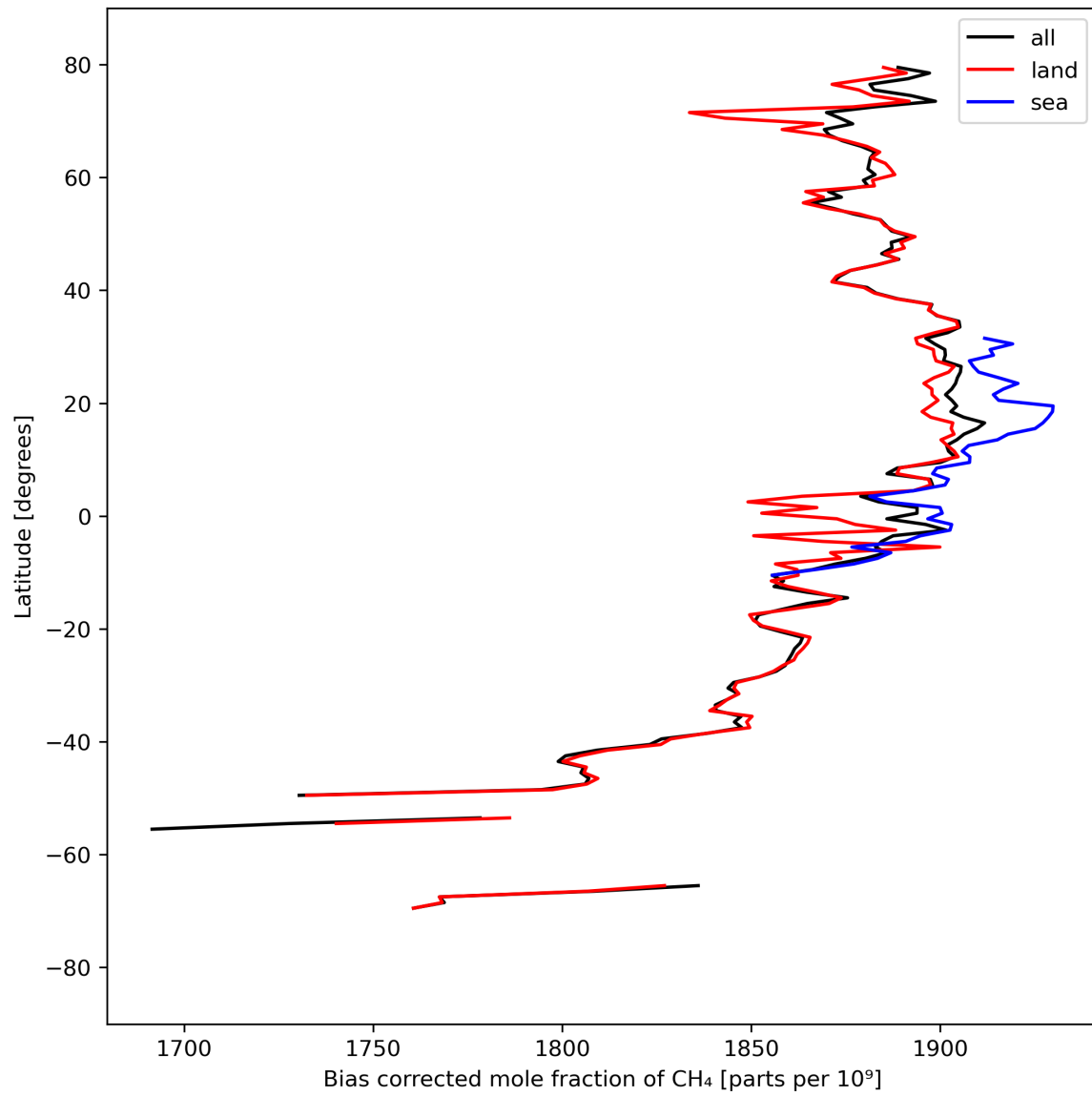
Figure 14: Zonal average of “Bias corrected mole fraction of CH 4 ” for 2024-03-31 to 2024-04-01.
