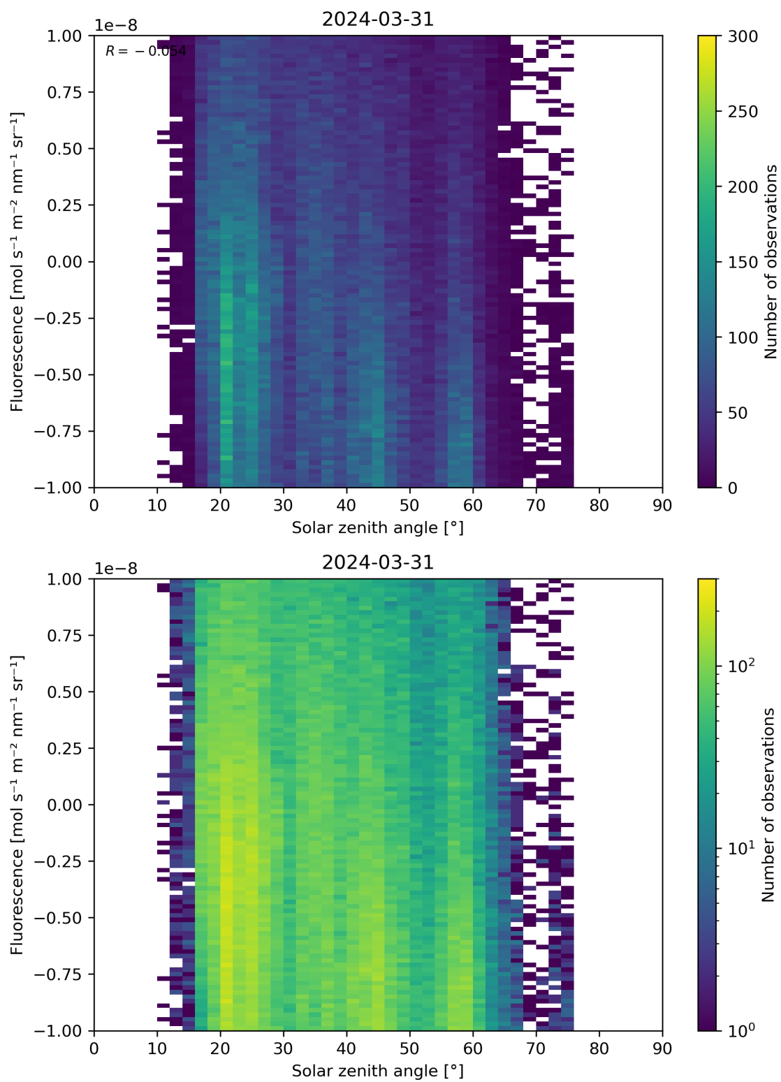
Figure 97: Scatter density plot of “Solar zenith angle” against “Fluorescence” for 2024-03-31 to 2024-04-01.
