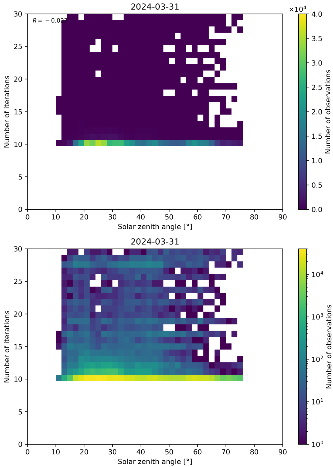
Figure 102: Scatter density plot of “Solar zenith angle” against “Number of iterations” for 2024-03-31 to 2024-04-01.
