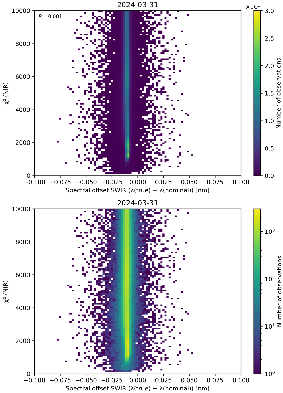
Figure 117: Scatter density plot of “Spectral offset SWIR ( \lambda(\text{true}) - \lambda(\text{nominal}) )” against “ \chi^2 (NIR)” for 2024-03-31 to 2024-04-01.
