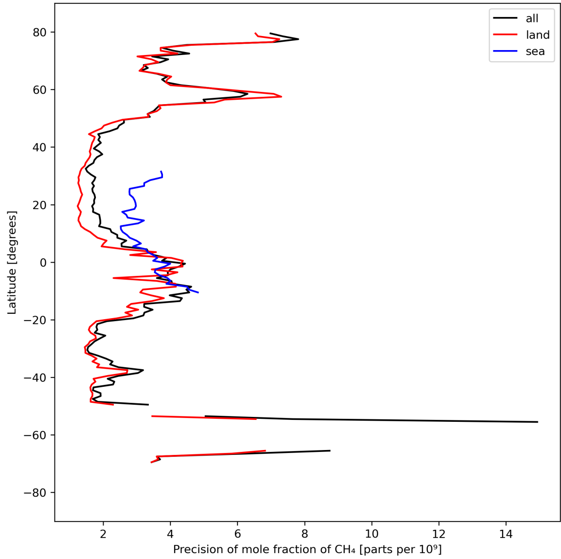
Figure 13: Zonal average of “Precision of mole fraction of CH 4 ” for 2024-03-31 to 2024-04-01.
