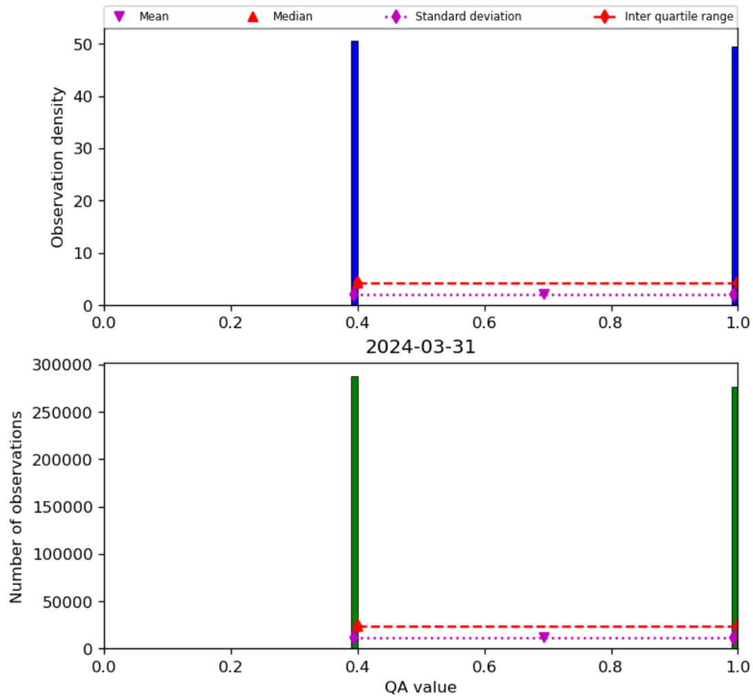
Figure 22: Histogram of “QA value” for 2024-03-31 to 2024-04-01
