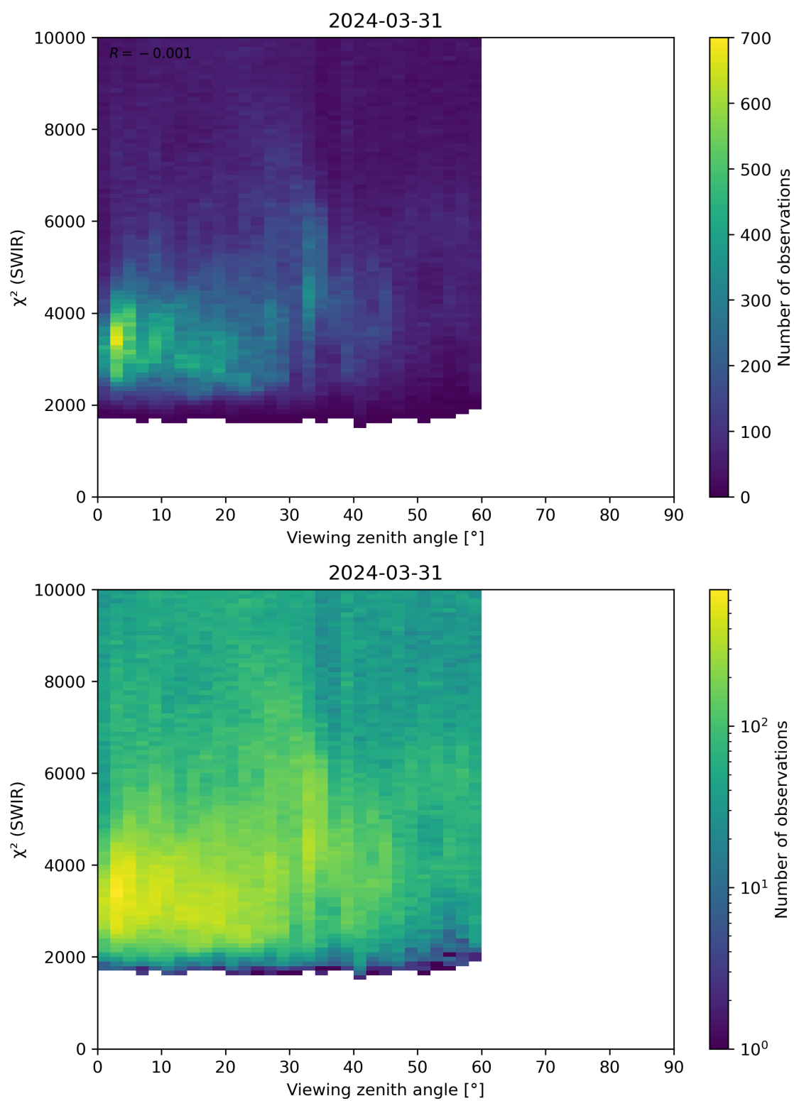
Figure 106: Scatter density plot of “Viewing zenith angle” against “ \chi^2 (SWIR)” for 2024-03-31 to 2024-04-01.
