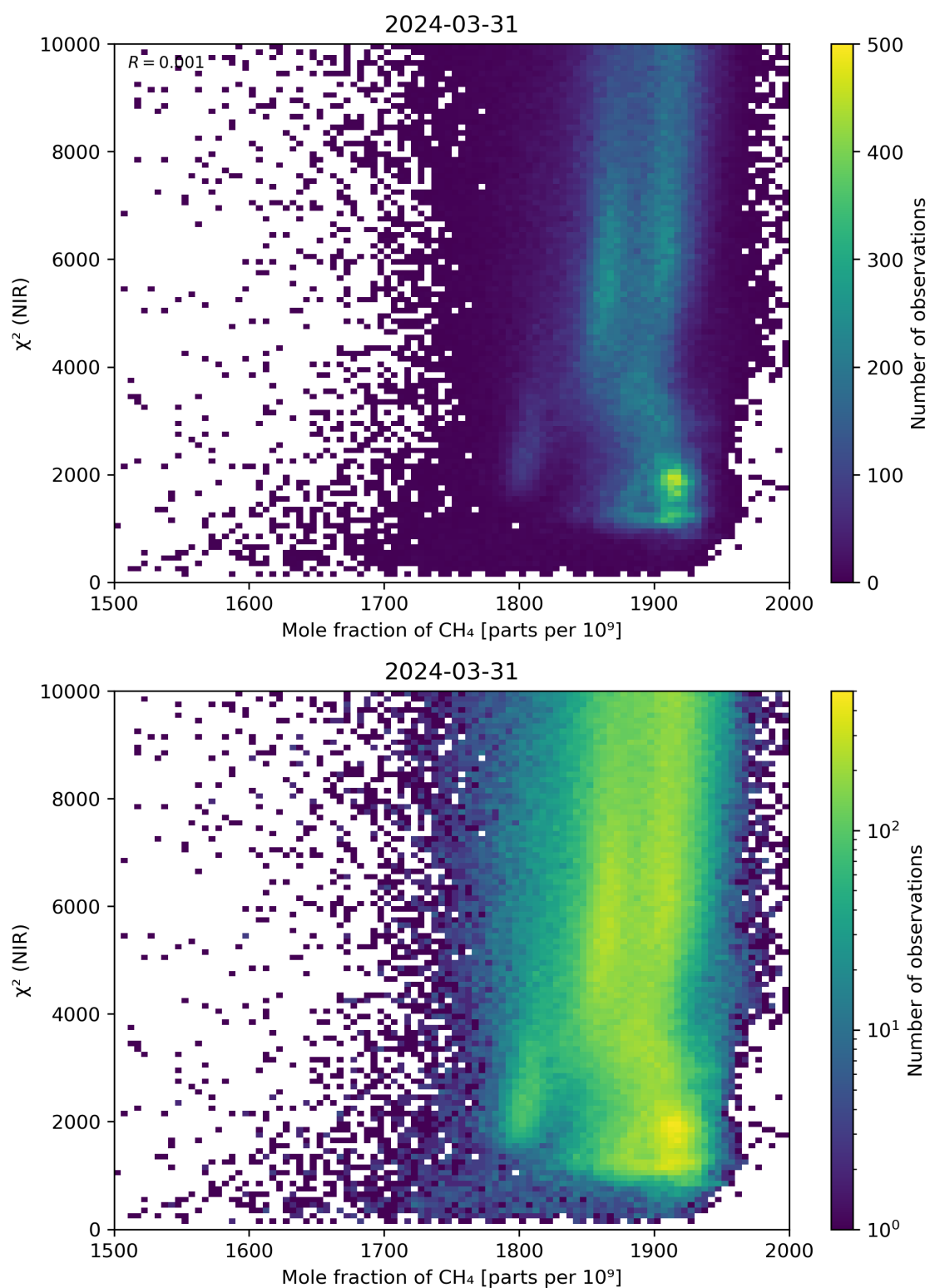
Figure 70: Scatter density plot of “Mole fraction of CH 4 ” against “ \chi^2 (NIR)” for 2024-03-31 to 2024-04-01.
