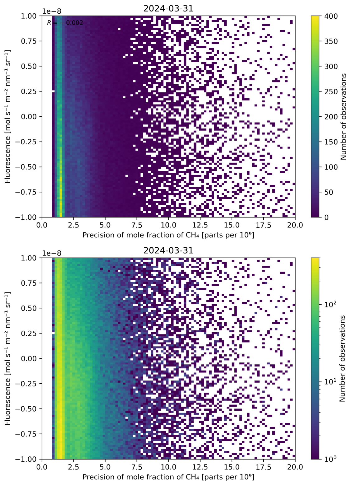
Figure 81: Scatter density plot of “Precision of mole fraction of \text{CH}_4 ” against “Fluorescence” for 2024-03-31 to 2024-04-01.
