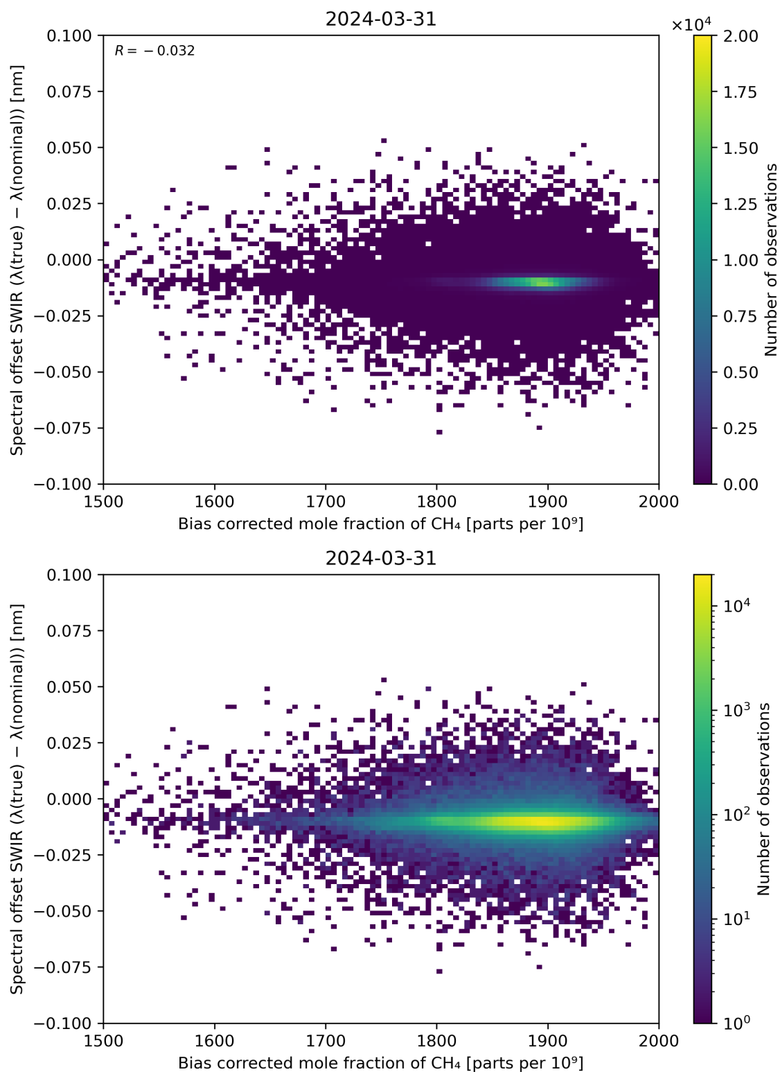
Figure 69: Scatter density plot of “Bias corrected mole fraction of \text{CH}_4 ” against “Spectral offset SWIR ( \lambda(\text{true}) - \lambda(\text{nominal}) )” for 2024-03-31 to 2024-04-01.
