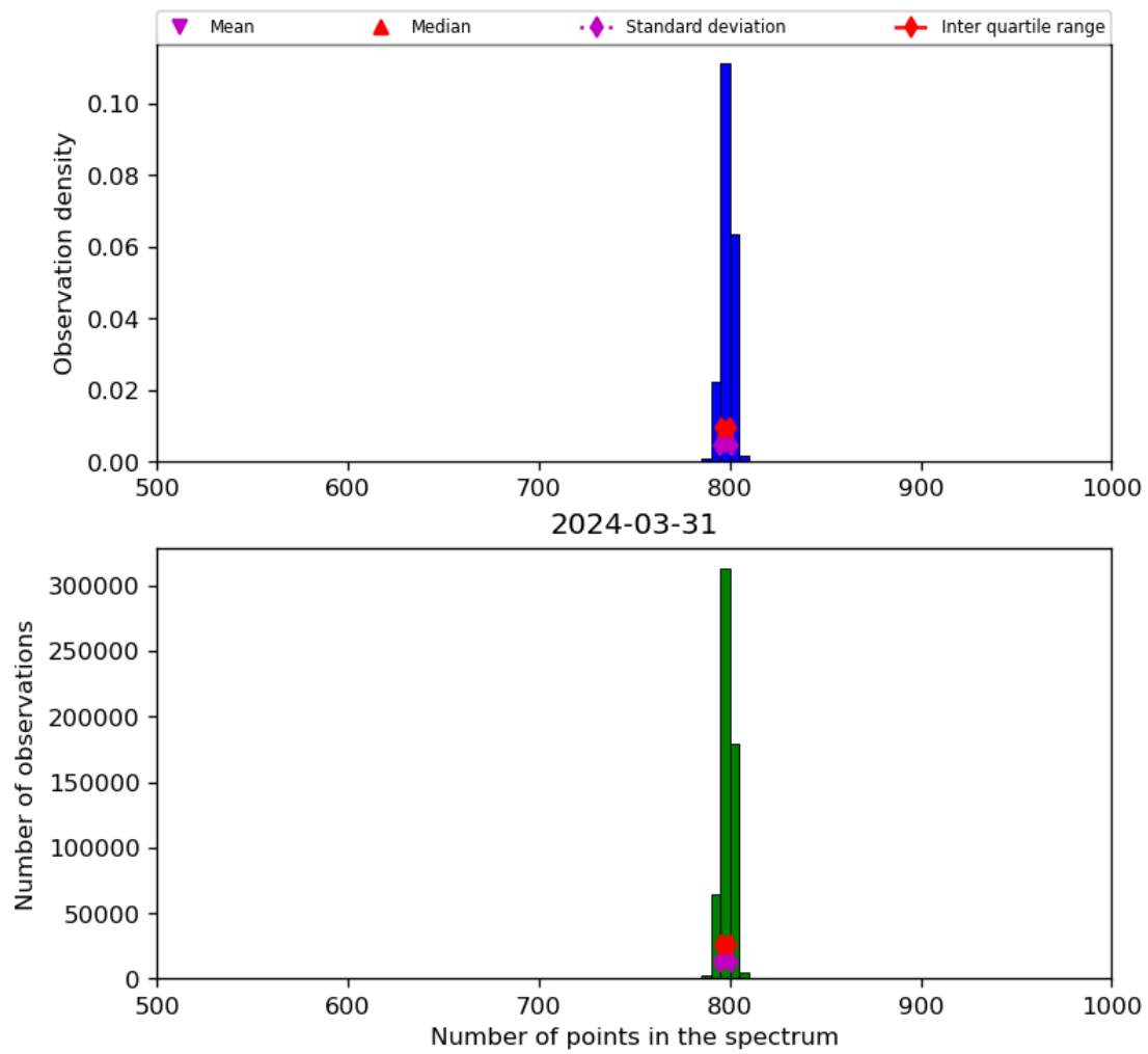
Figure 26: Histogram of “Number of points in the spectrum” for 2024-03-31 to 2024-04-01
