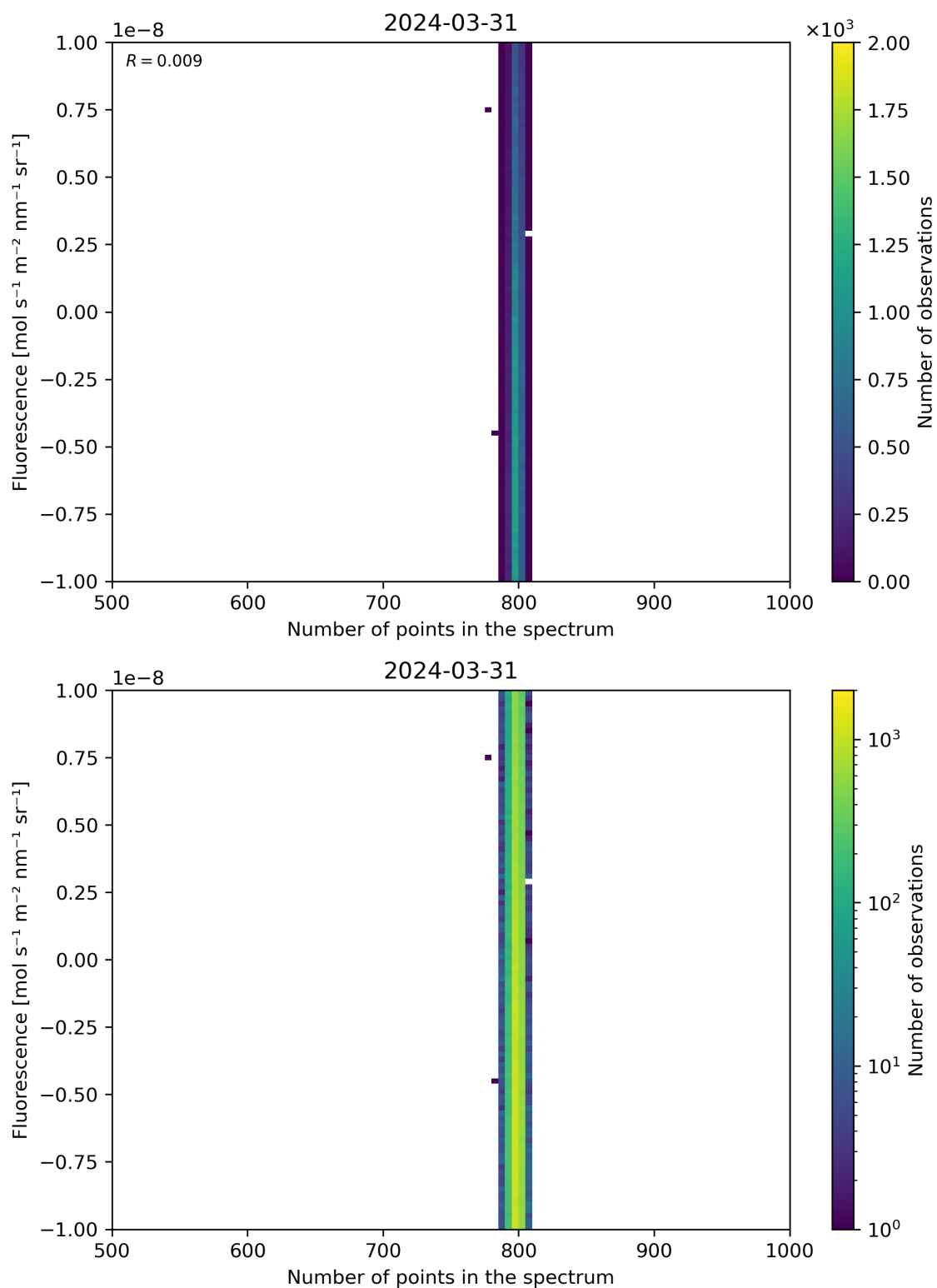
Figure 91: Scatter density plot of “Number of points in the spectrum” against “Fluorescence” for 2024-03-31 to 2024-04-01.
