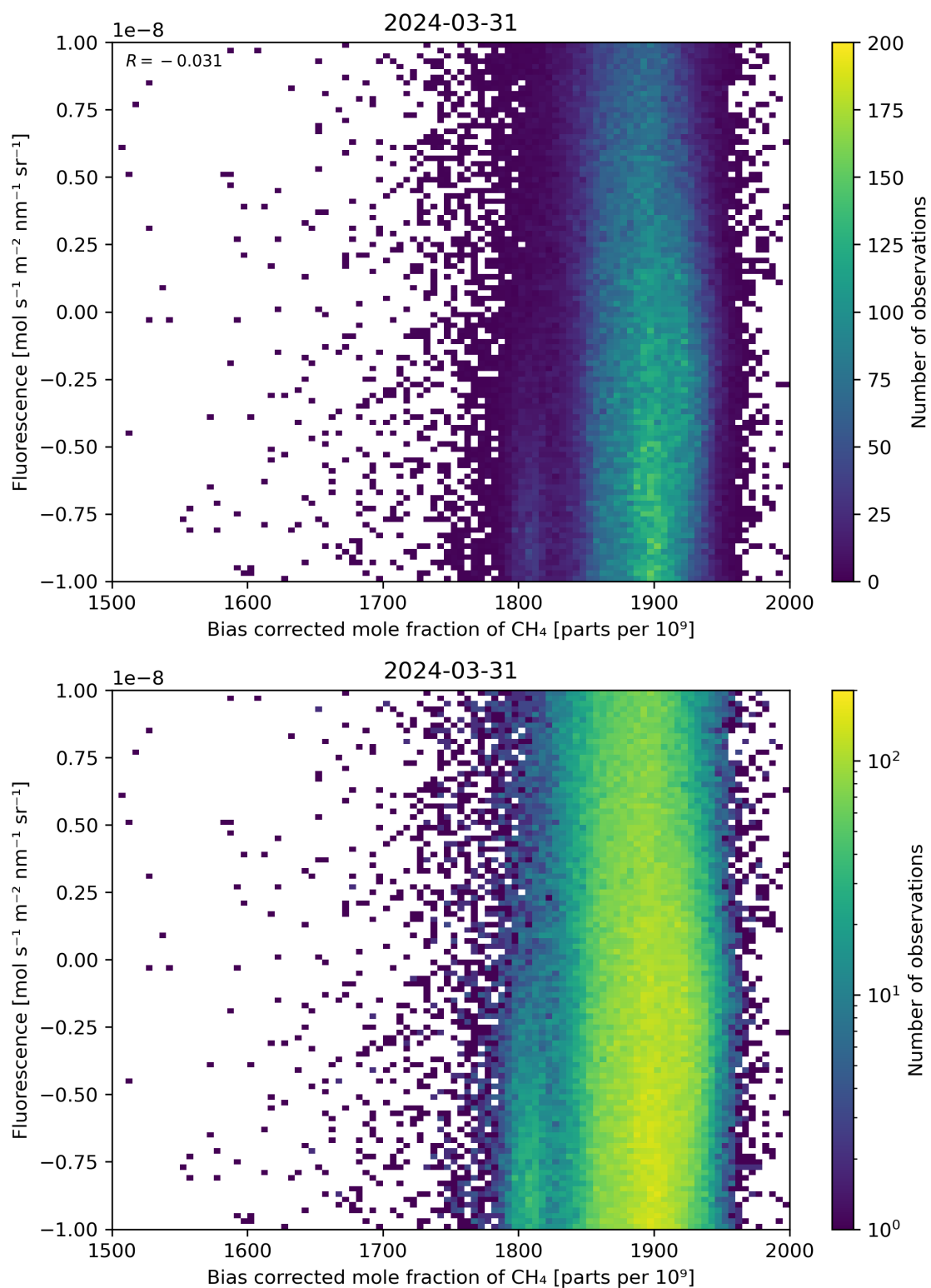
Figure 66: Scatter density plot of “Bias corrected mole fraction of CH 4 ” against “Fluorescence” for 2024-03-31 to 2024-04-01.
