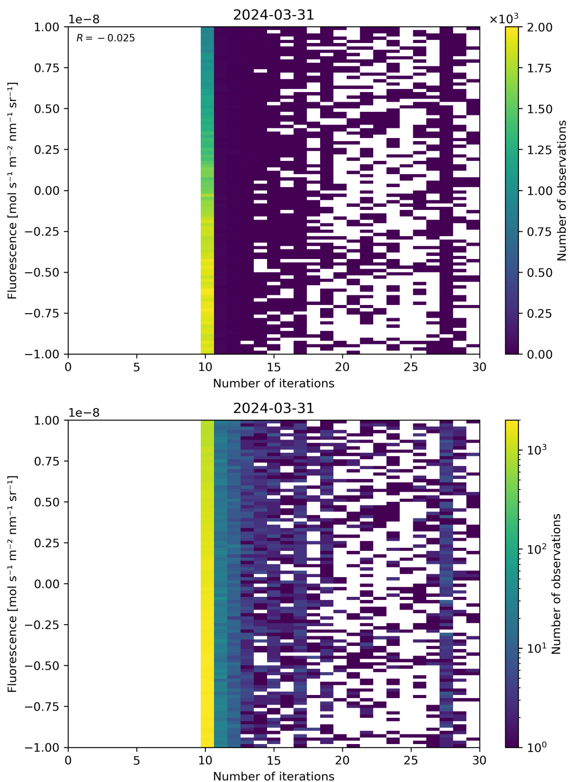
Figure 87: Scatter density plot of “Number of iterations” against “Fluorescence” for 2024-03-31 to 2024-04-01.
