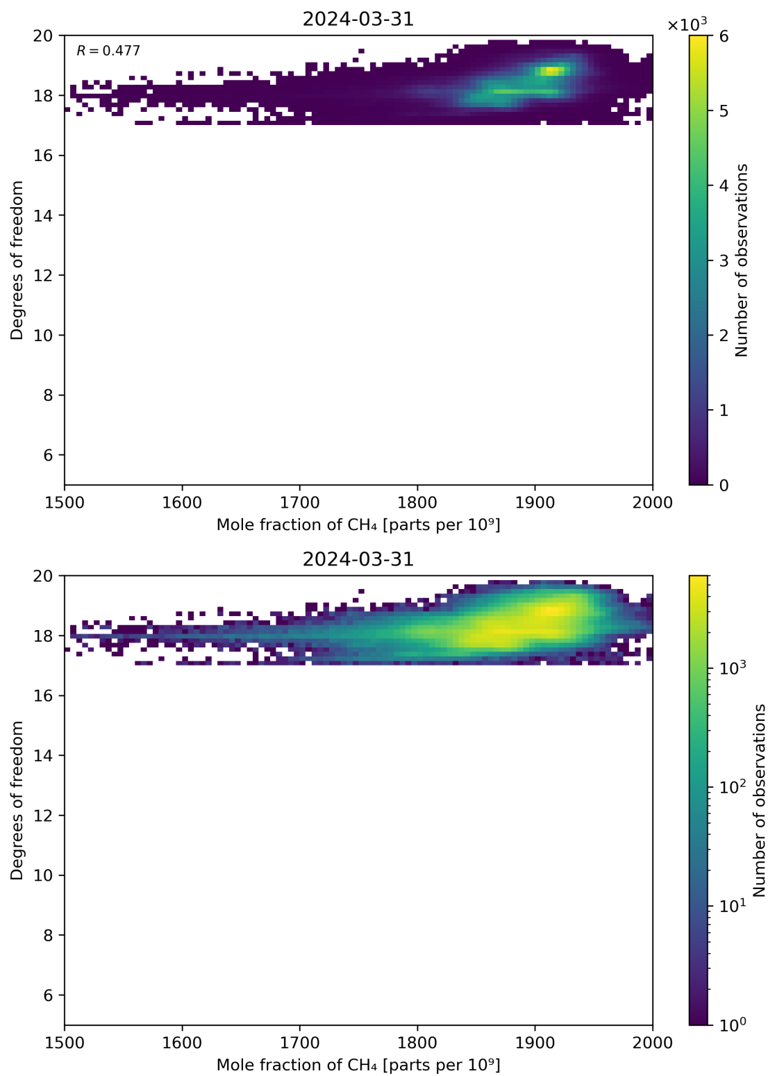
Figure 72: Scatter density plot of “Mole fraction of CH 4 ” against “Degrees of freedom” for 2024-03-31 to 2024-04-01.
