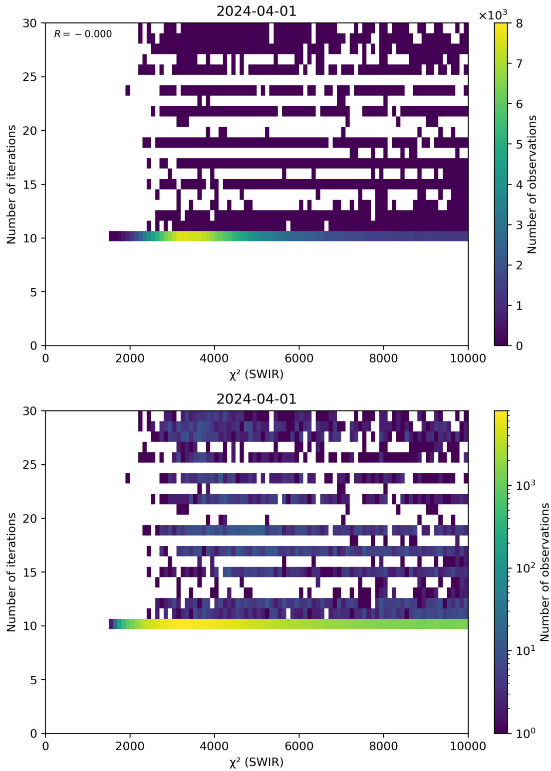
Figure 50: Scatter density plot of “ \chi^2 (SWIR)” against “Number of iterations” for 2024-03-31 to 2024-04-02.
