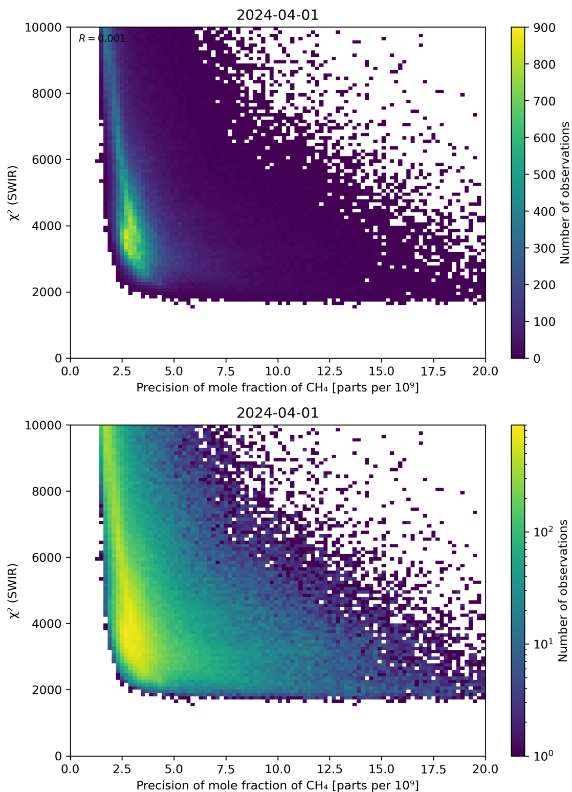
Figure 79: Scatter density plot of “Precision of mole fraction of \text{CH}_4 ” against “ \chi^2 (SWIR)” for 2024-03-31 to 2024-04-02.
