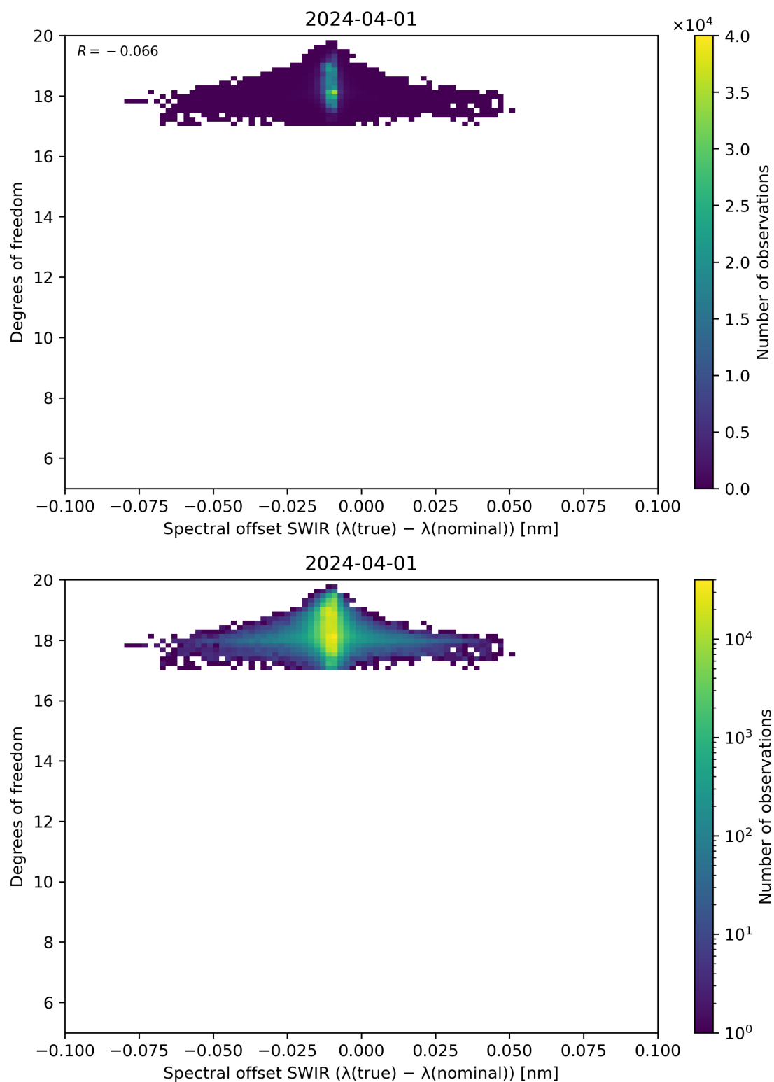
Figure 119: Scatter density plot of “Spectral offset SWIR ( \lambda(\text{true}) - \lambda(\text{nominal}) )” against “Degrees of freedom” for 2024-03-31 to 2024-04-02.
