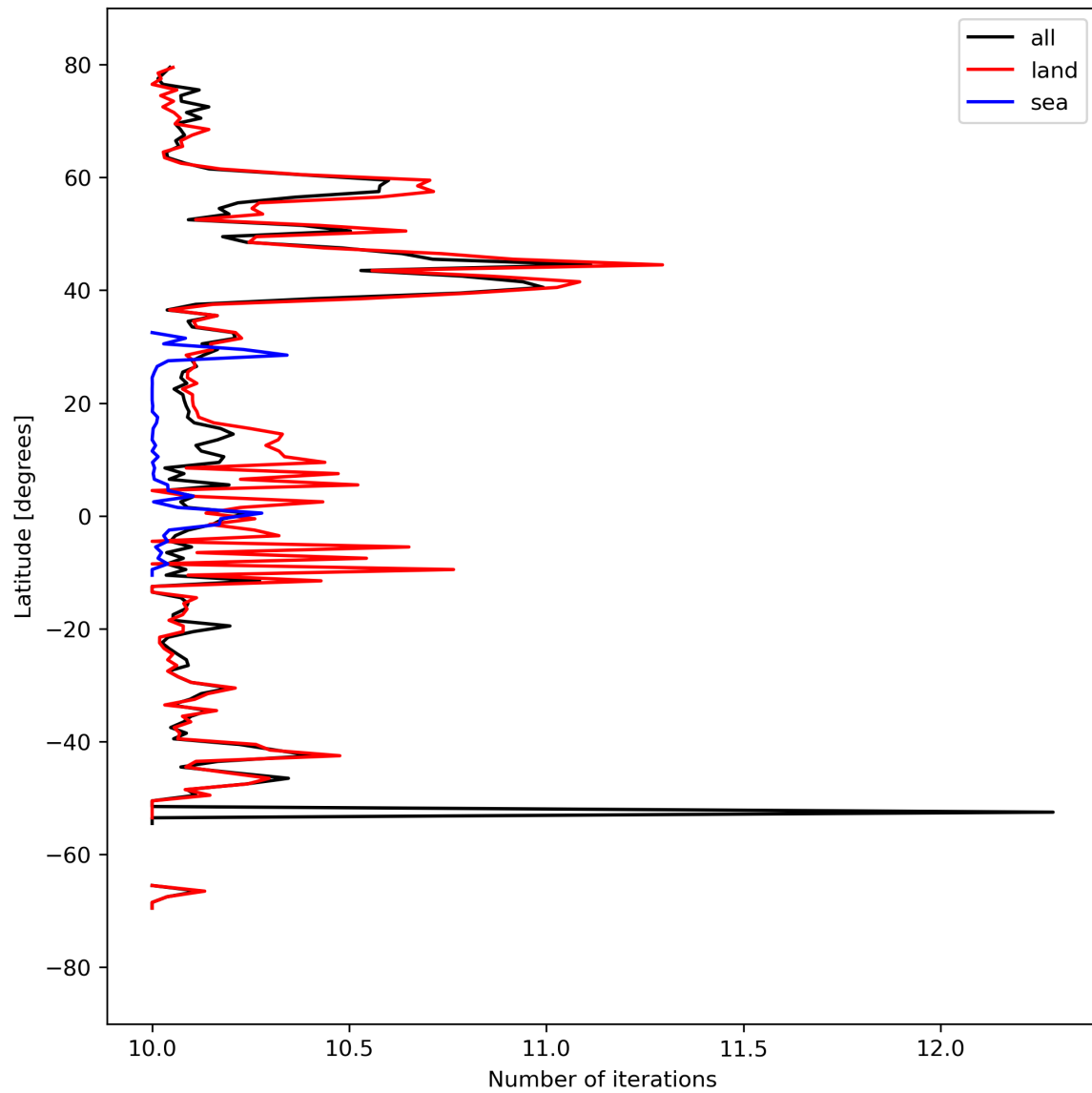
Figure 20: Zonal average of “Number of iterations” for 2024-03-31 to 2024-04-02.
