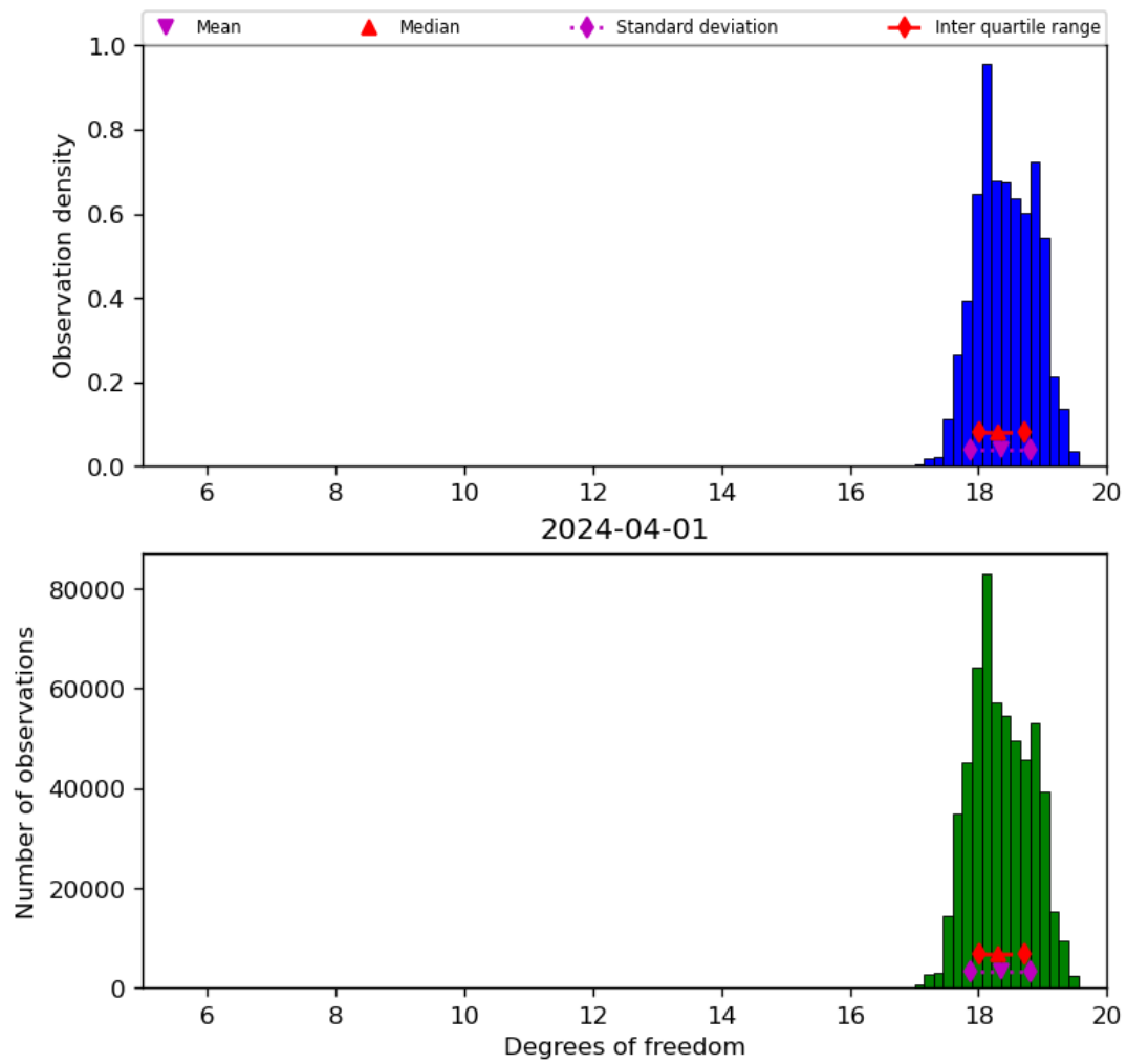
Figure 30: Histogram of “Degrees of freedom” for 2024-03-31 to 2024-04-02
