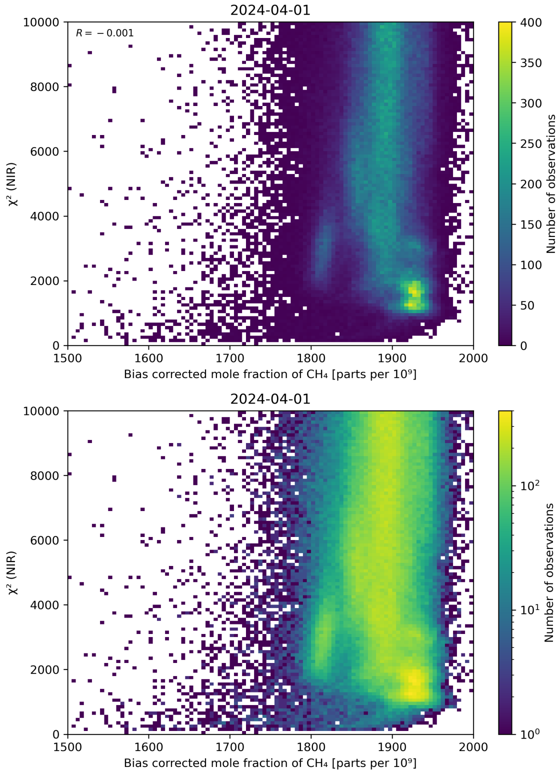
Figure 63: Scatter density plot of “Bias corrected mole fraction of CH 4 ” against “ \chi^2 (NIR)” for 2024-03-31 to 2024-04-02.
