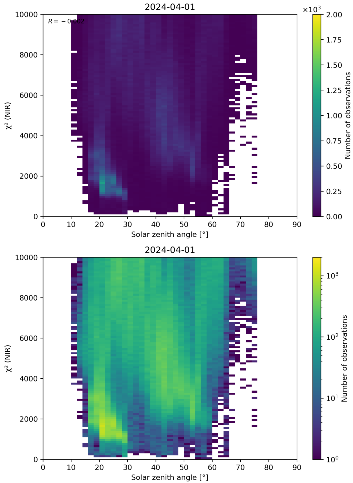
Figure 94: Scatter density plot of “Solar zenith angle” against “ \chi^2 (NIR)” for 2024-03-31 to 2024-04-02.
