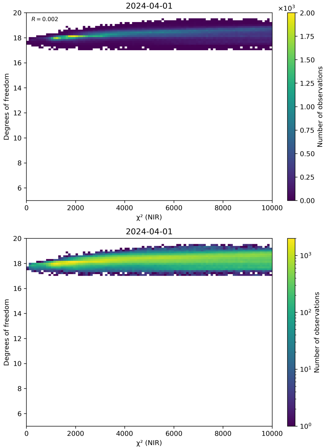
Figure 44: Scatter density plot of “ \chi^2 (NIR)” against “Degrees of freedom” for 2024-03-31 to 2024-04-02.
