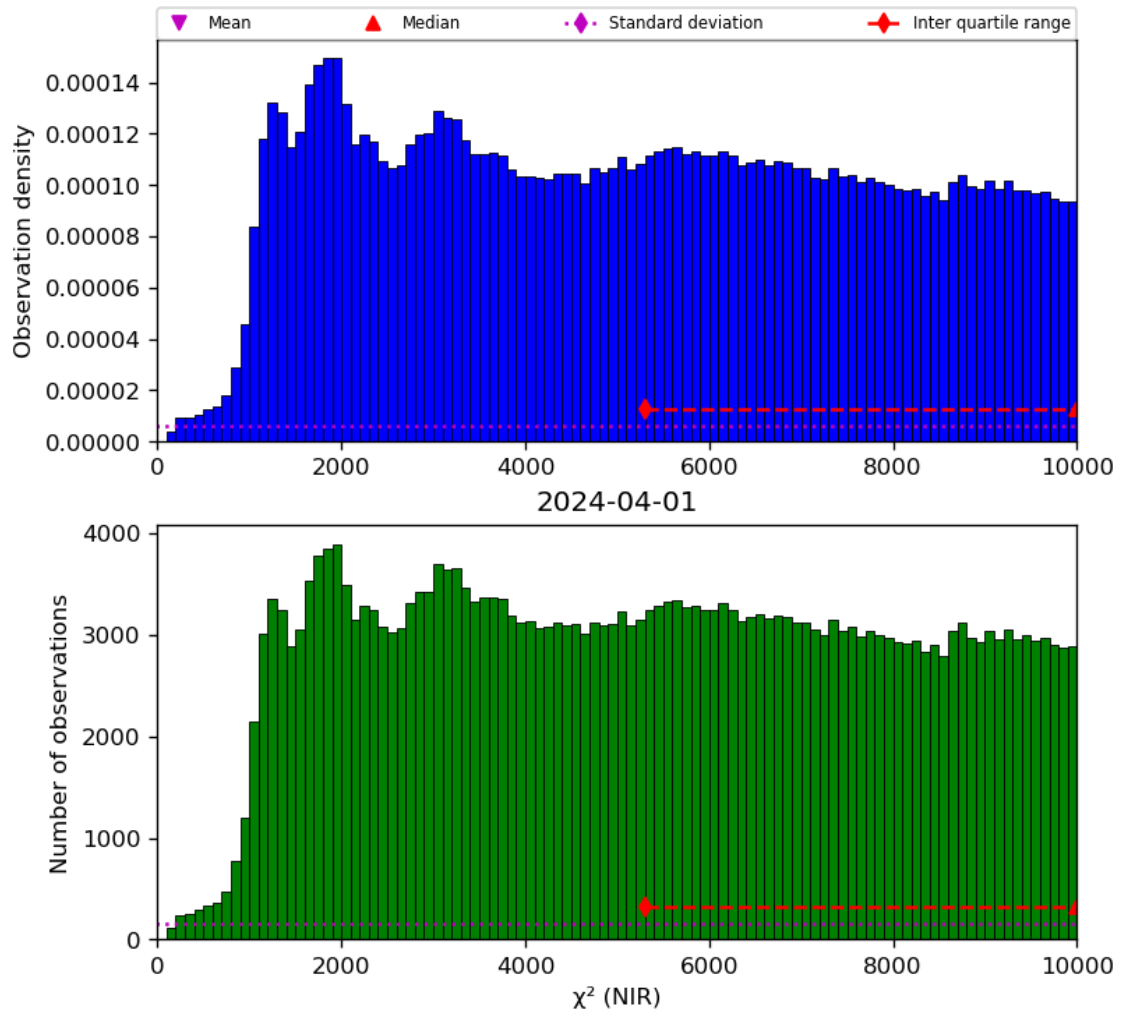
Figure 29: Histogram of “ \chi^2 (NIR)” for 2024-03-31 to 2024-04-02
