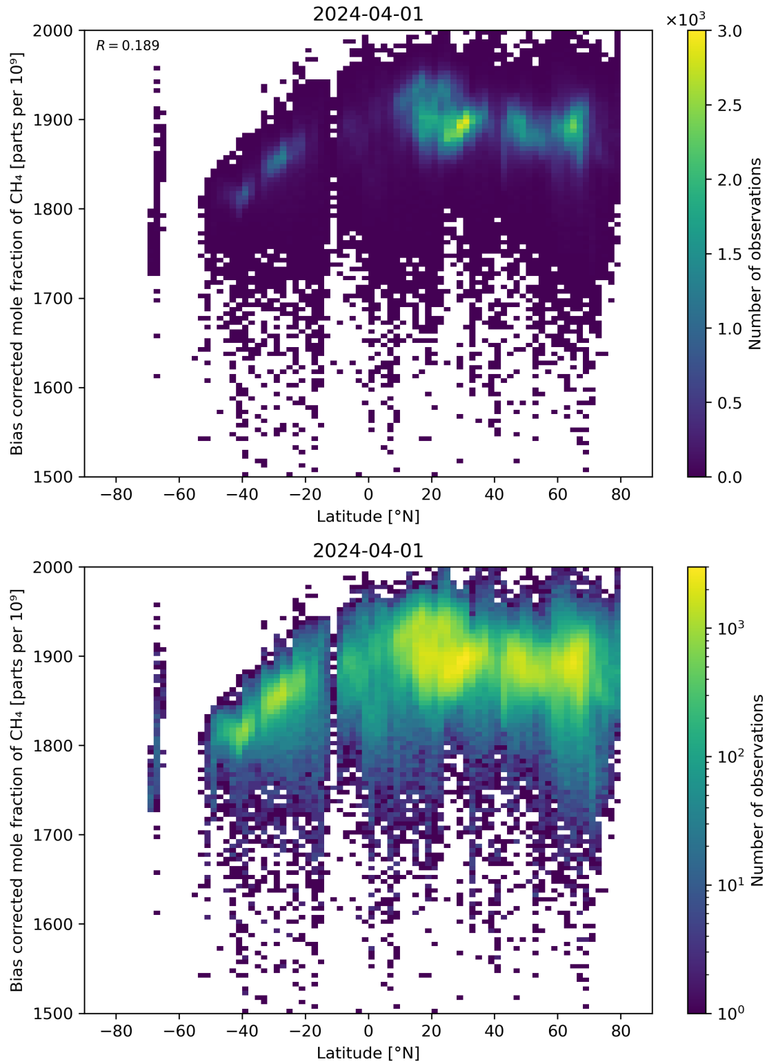
Figure 58: Scatter density plot of “Latitude” against “Bias corrected mole fraction of CH 4 ” for 2024-03-31 to 2024-04-02.
