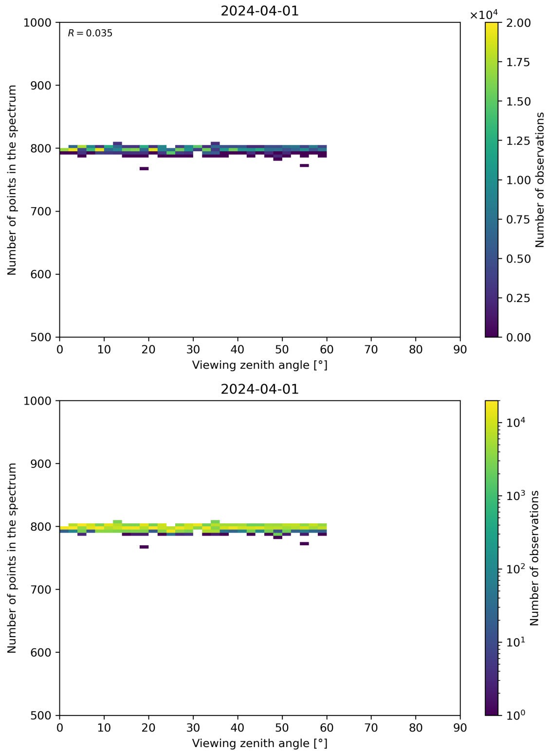
Figure 114: Scatter density plot of “Viewing zenith angle” against “Number of points in the spectrum” for 2024-03-31 to 2024-04-02.
