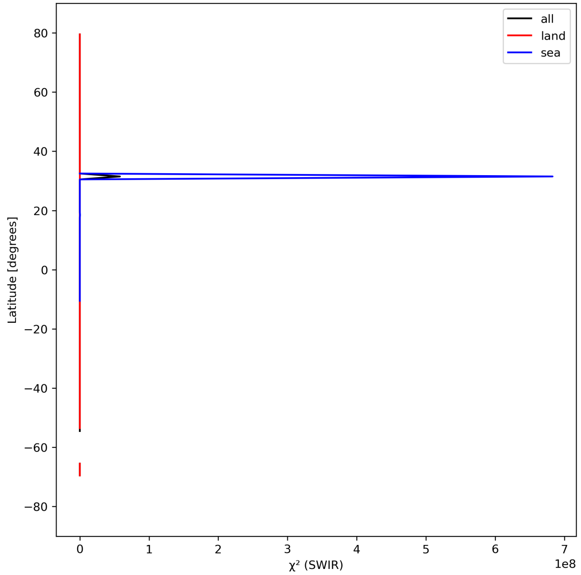
Figure 17: Zonal average of “ \chi^2 (SWIR)” for 2024-03-31 to 2024-04-02.
