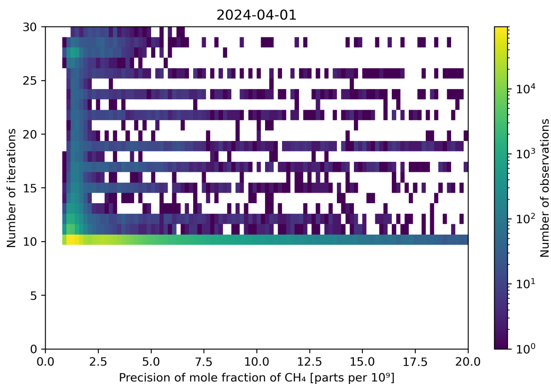
Figure 83: Scatter density plot of “Precision of mole fraction of CH 4 ” against “Number of iterations” for 2024-03-31 to 2024-04-02.
