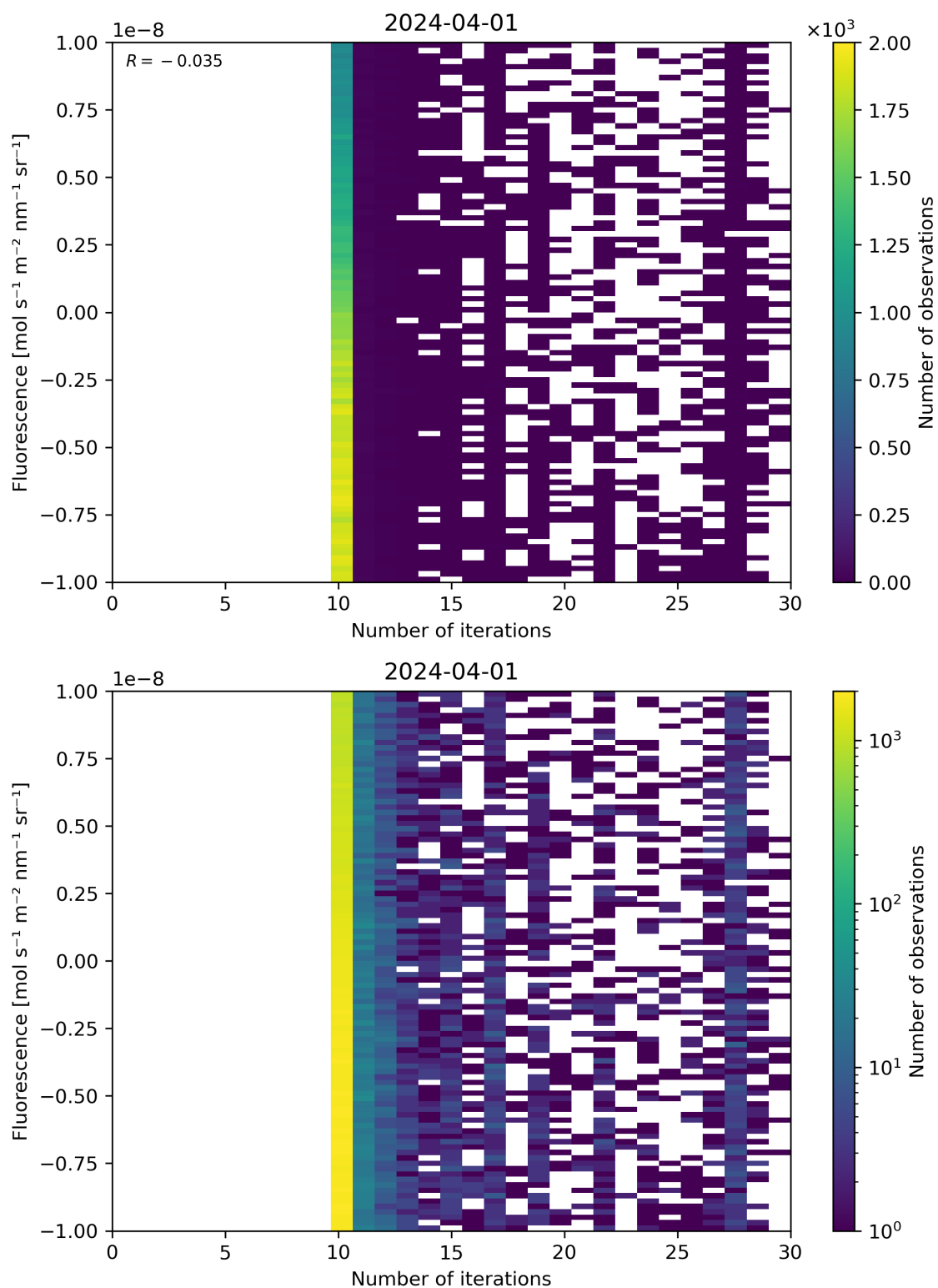
Figure 87: Scatter density plot of “Number of iterations” against “Fluorescence” for 2024-03-31 to 2024-04-02.
