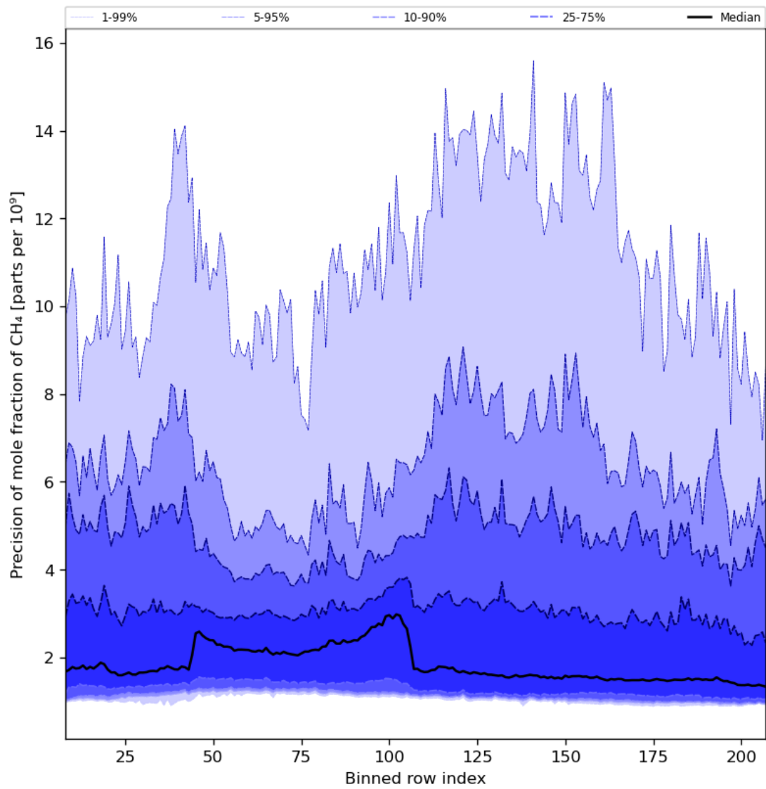
Figure 35: Along track statistics of “Precision of mole fraction of CH 4 ” for 2024-03-31 to 2024-04-02
