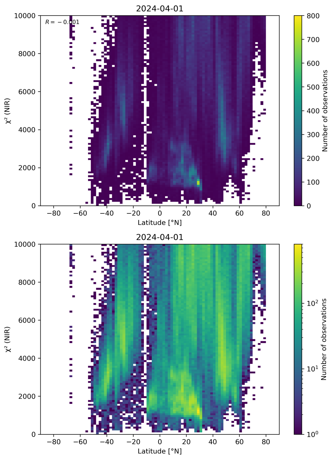
Figure 53: Scatter density plot of “Latitude” against “ \chi^2 (NIR)” for 2024-03-31 to 2024-04-02.
