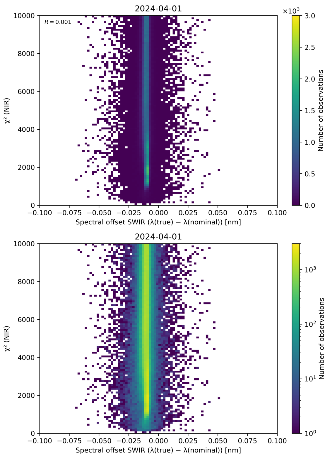
Figure 117: Scatter density plot of “Spectral offset SWIR ( \lambda(\text{true}) - \lambda(\text{nominal}) )” against “ \chi^2 (NIR)” for 2024-03-31 to 2024-04-02.
