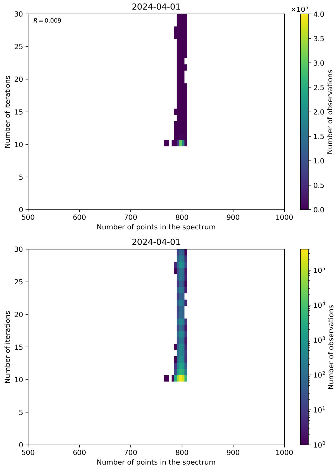
Figure 92: Scatter density plot of “Number of points in the spectrum” against “Number of iterations” for 2024-03-31 to 2024-04-02.
