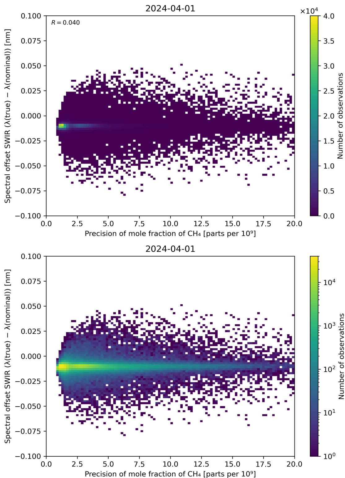
Figure 85: Scatter density plot of “Precision of mole fraction of \text{CH}_4 ” against “Spectral offset SWIR ( \lambda(\text{true}) - \lambda(\text{nominal}) )” for 2024-03-31 to 2024-04-02.
