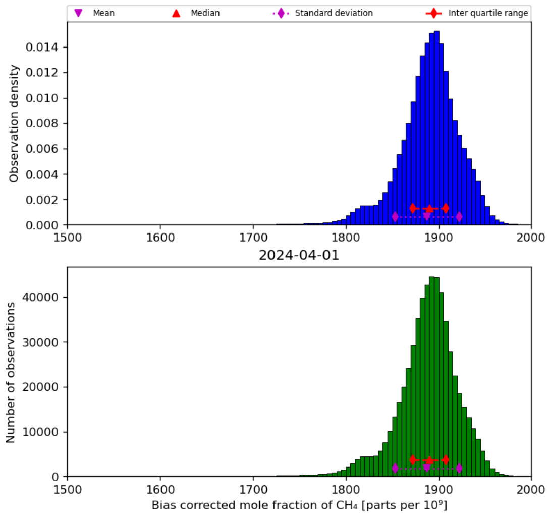
Figure 25: Histogram of “Bias corrected mole fraction of CH 4 ” for 2024-03-31 to 2024-04-02
