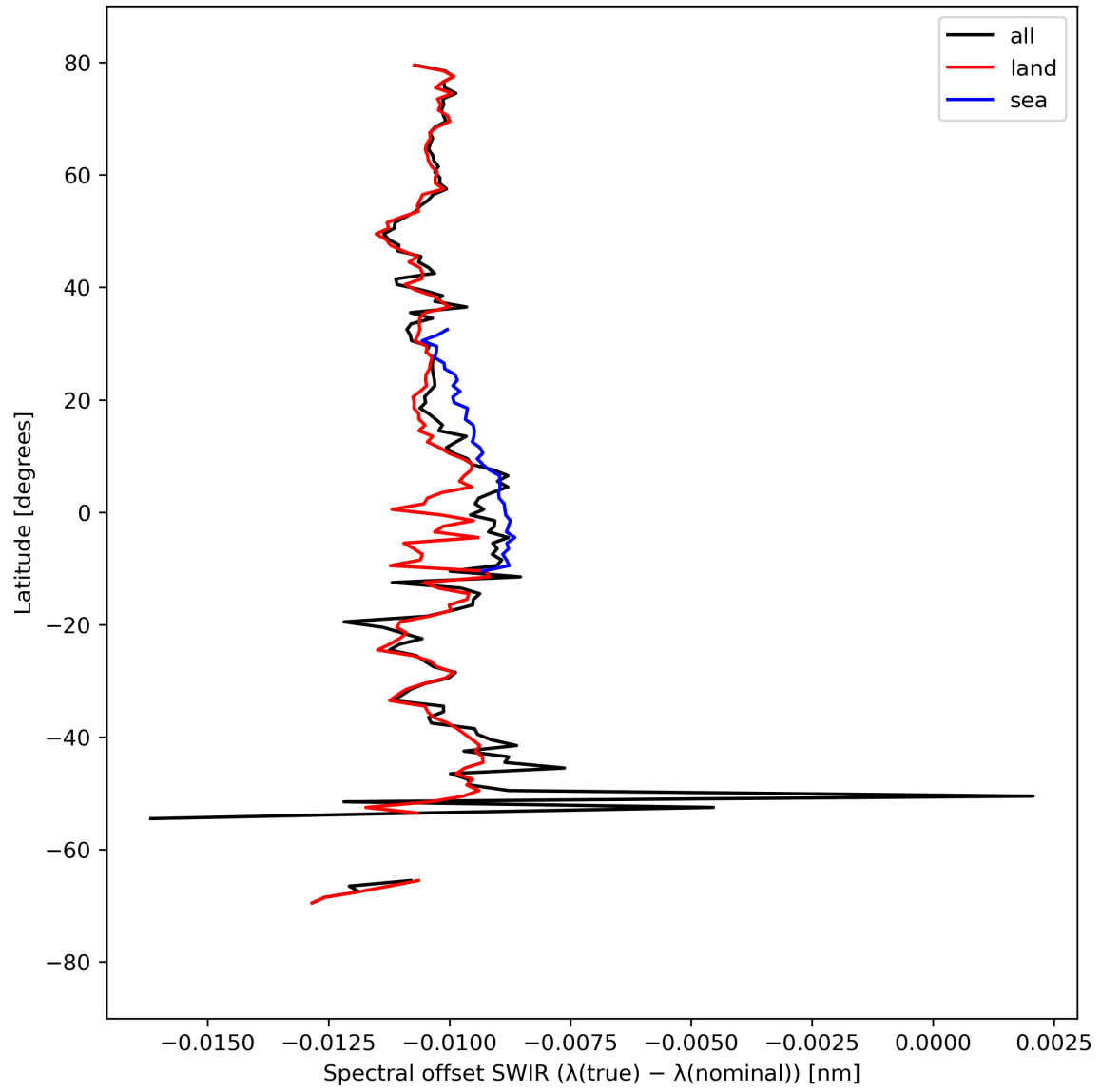
Figure 16: Zonal average of “Spectral offset SWIR ( \lambda(\text{true}) - \lambda(\text{nominal}) )” for 2024-03-31 to 2024-04-02.
