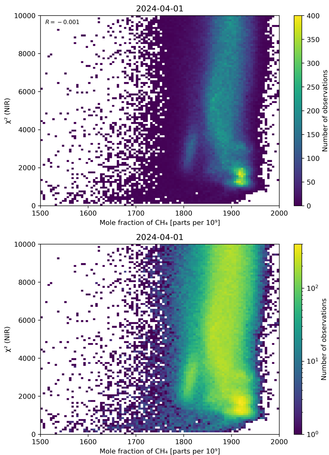
Figure 70: Scatter density plot of “Mole fraction of CH 4 ” against “ \chi^2 (NIR)” for 2024-03-31 to 2024-04-02.
