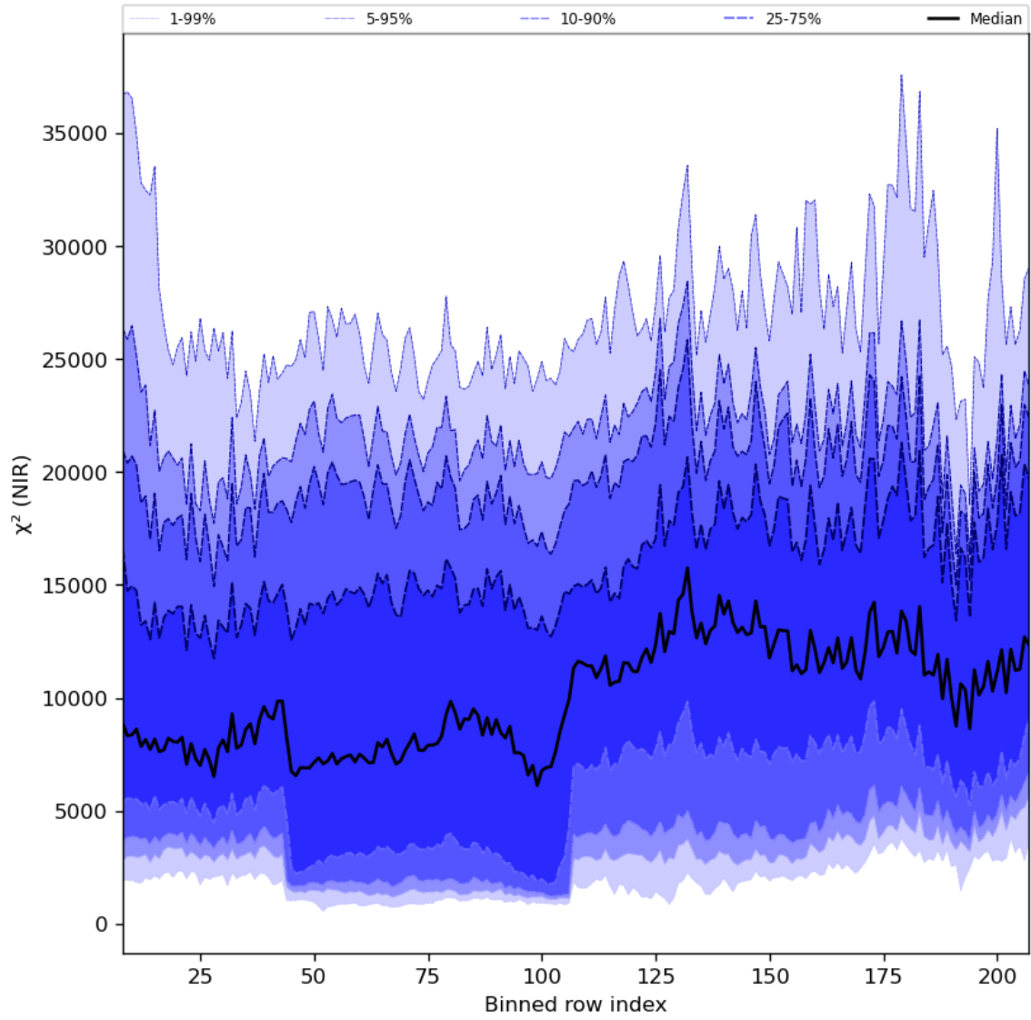
Figure 40: Along track statistics of “ \chi^2 (NIR)” for 2024-03-31 to 2024-04-02
