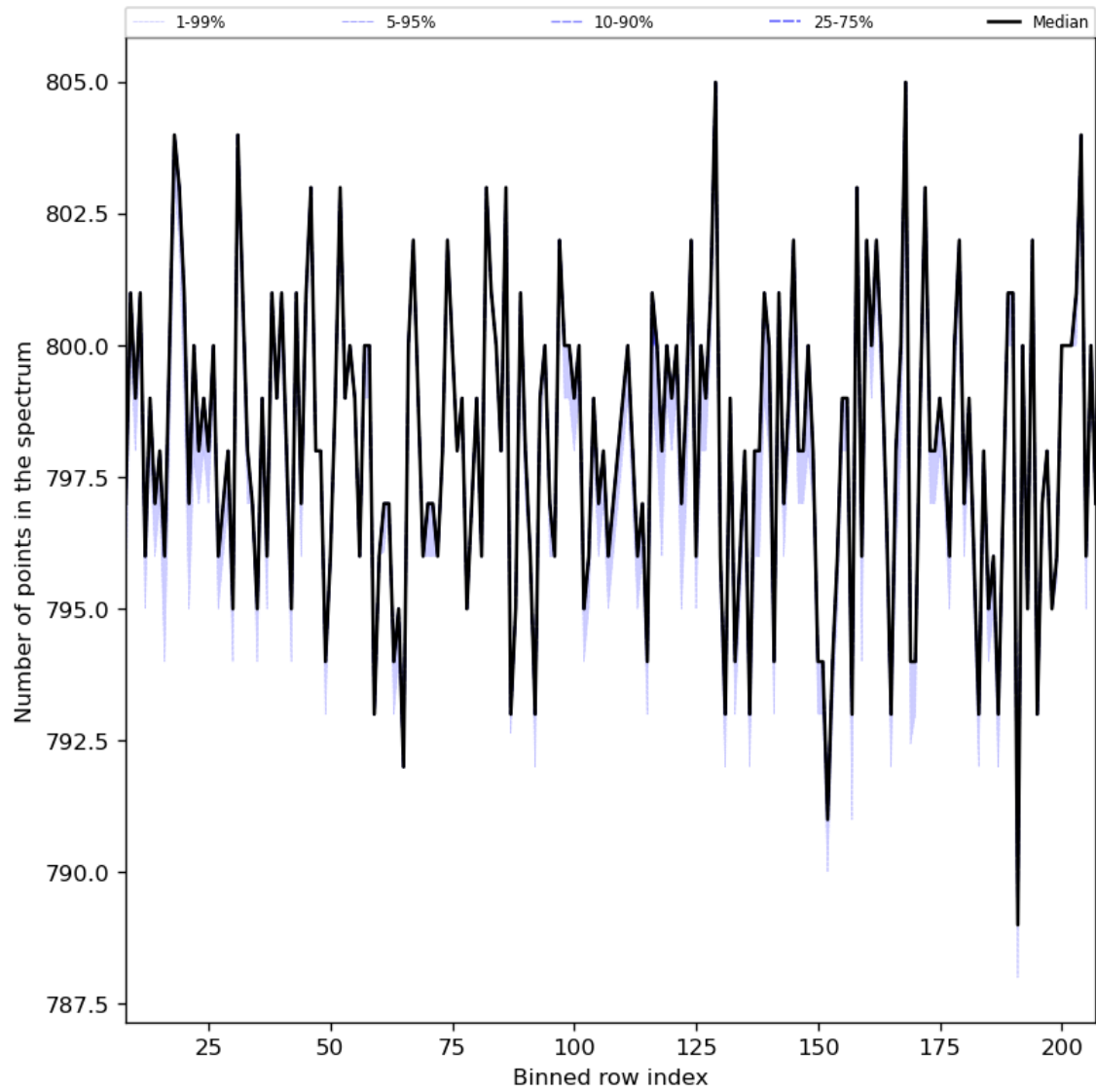
Figure 37: Along track statistics of “Number of points in the spectrum” for 2024-03-31 to 2024-04-02
