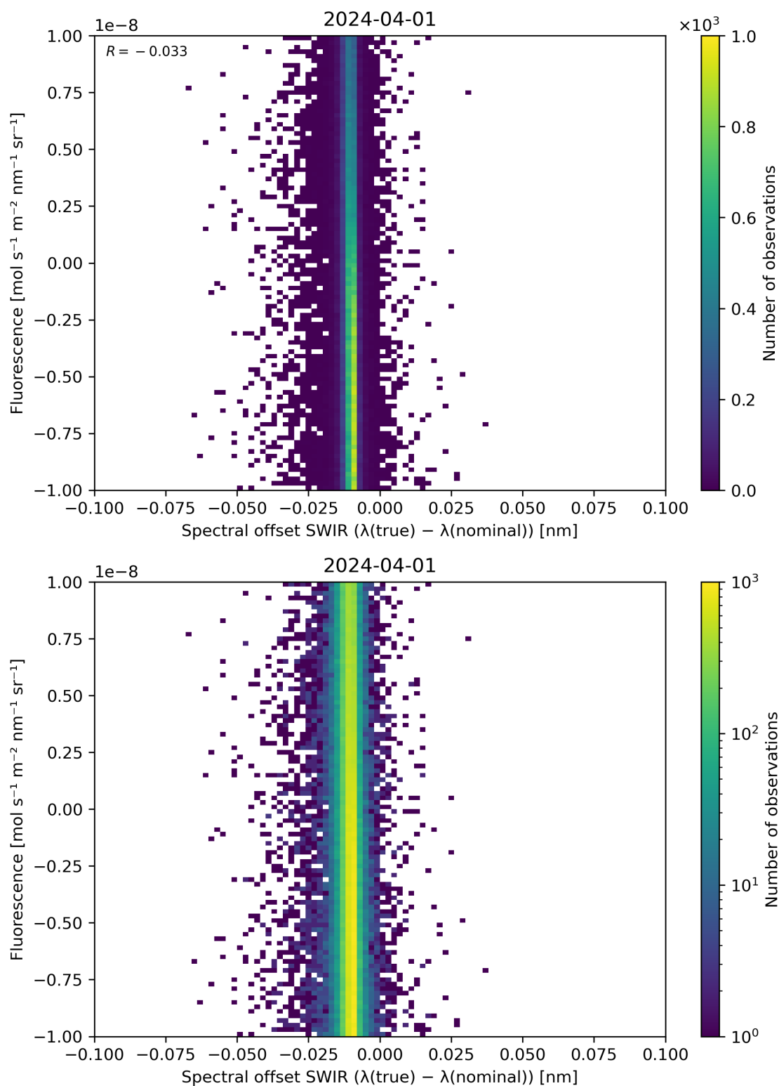
Figure 120: Scatter density plot of “Spectral offset SWIR ( \lambda(\text{true}) - \lambda(\text{nominal}) )” against “Fluorescence” for 2024-03-31 to 2024-04-02.
