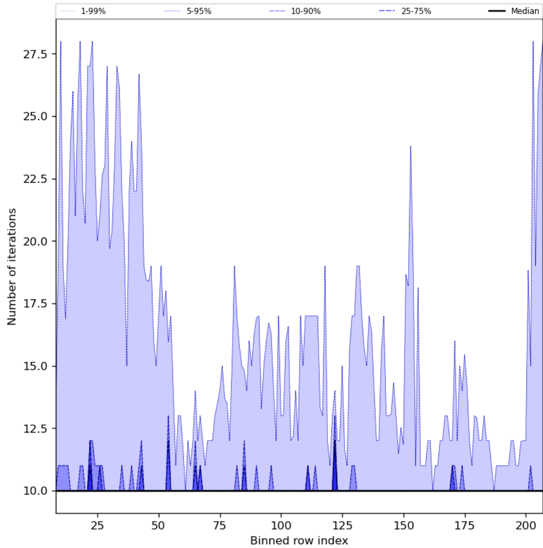
Figure 42: Along track statistics of “Number of iterations” for 2024-03-31 to 2024-04-02
