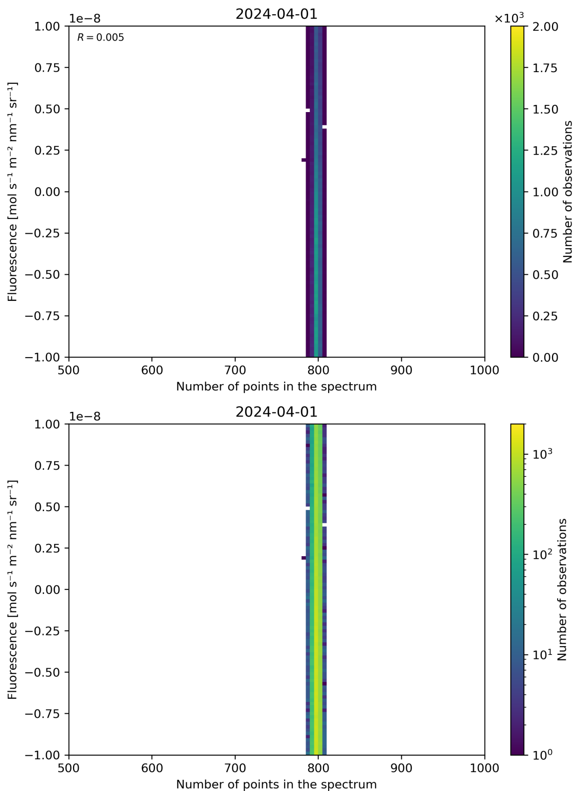
Figure 91: Scatter density plot of “Number of points in the spectrum” against “Fluorescence” for 2024-03-31 to 2024-04-02.
