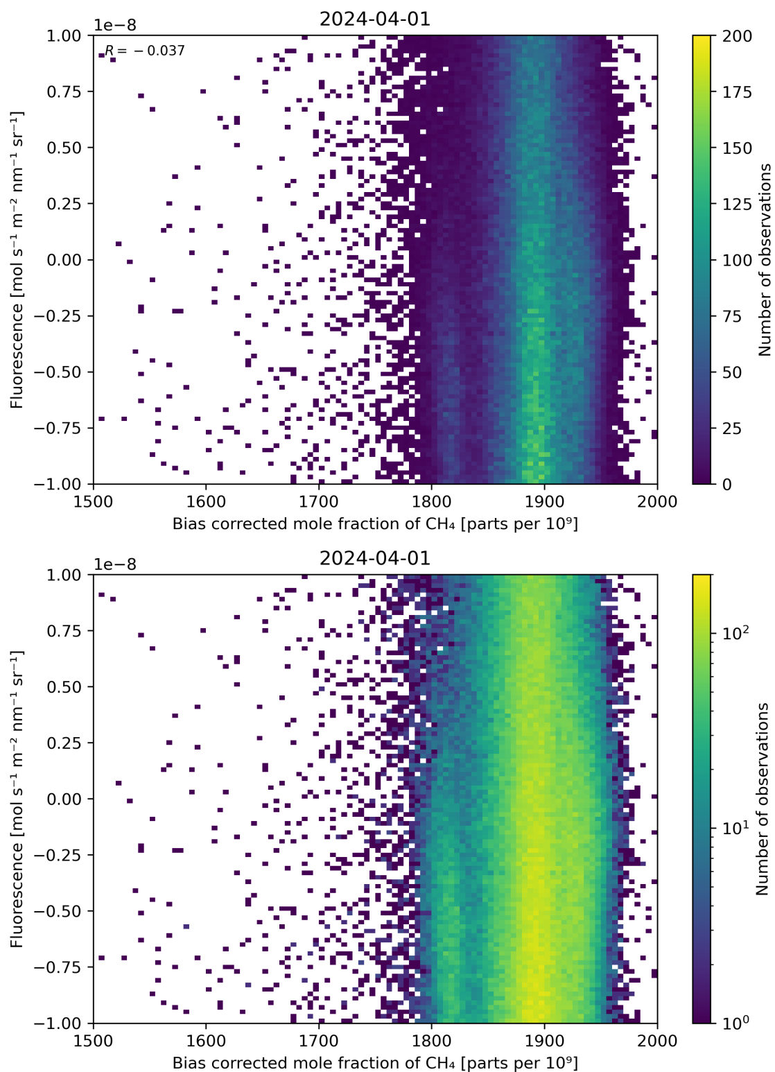
Figure 66: Scatter density plot of “Bias corrected mole fraction of \text{CH}_4 ” against “Fluorescence” for 2024-03-31 to 2024-04-02.
