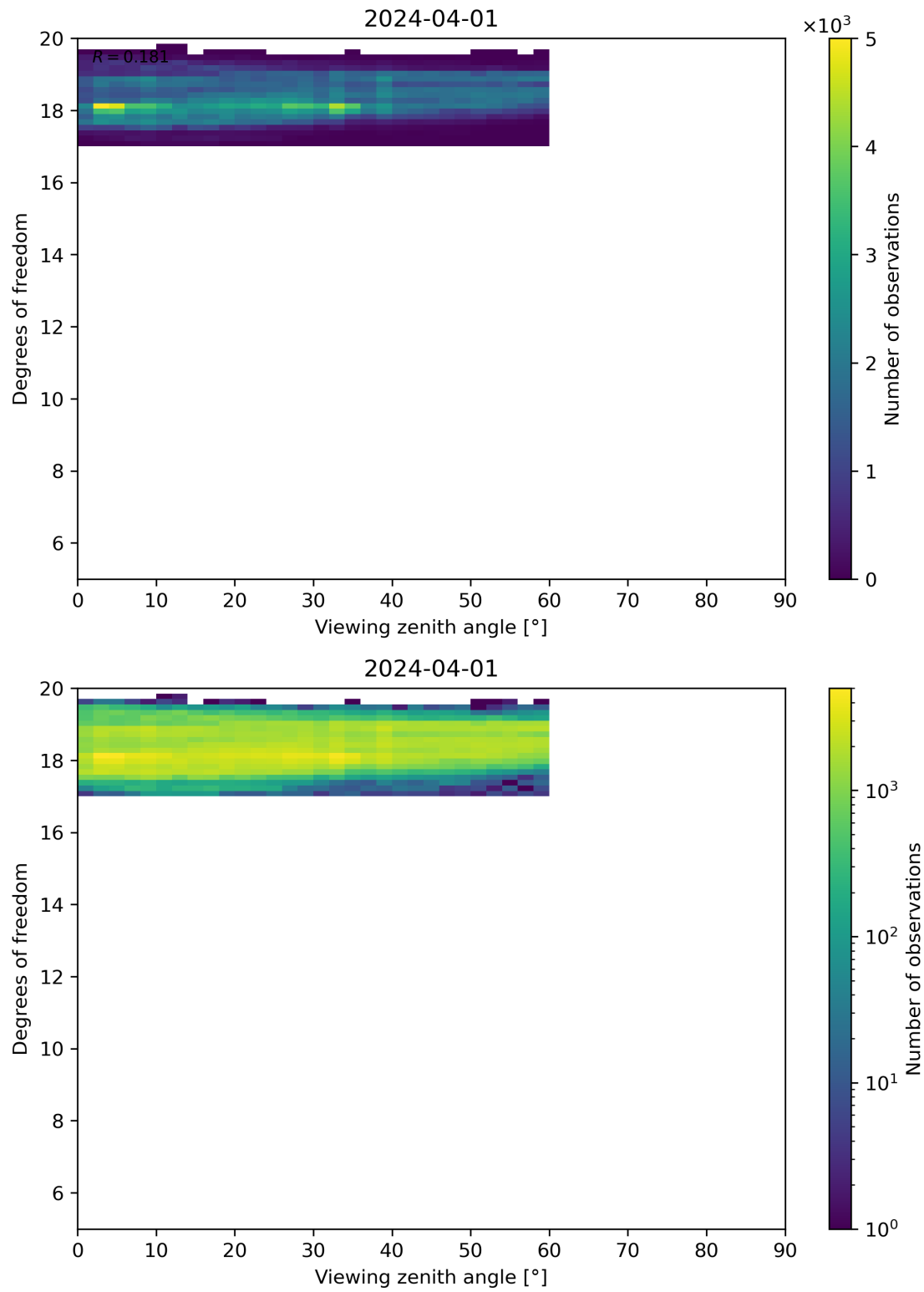
Figure 107: Scatter density plot of “Viewing zenith angle” against “Degrees of freedom” for 2024-03-31 to 2024-04-02.
