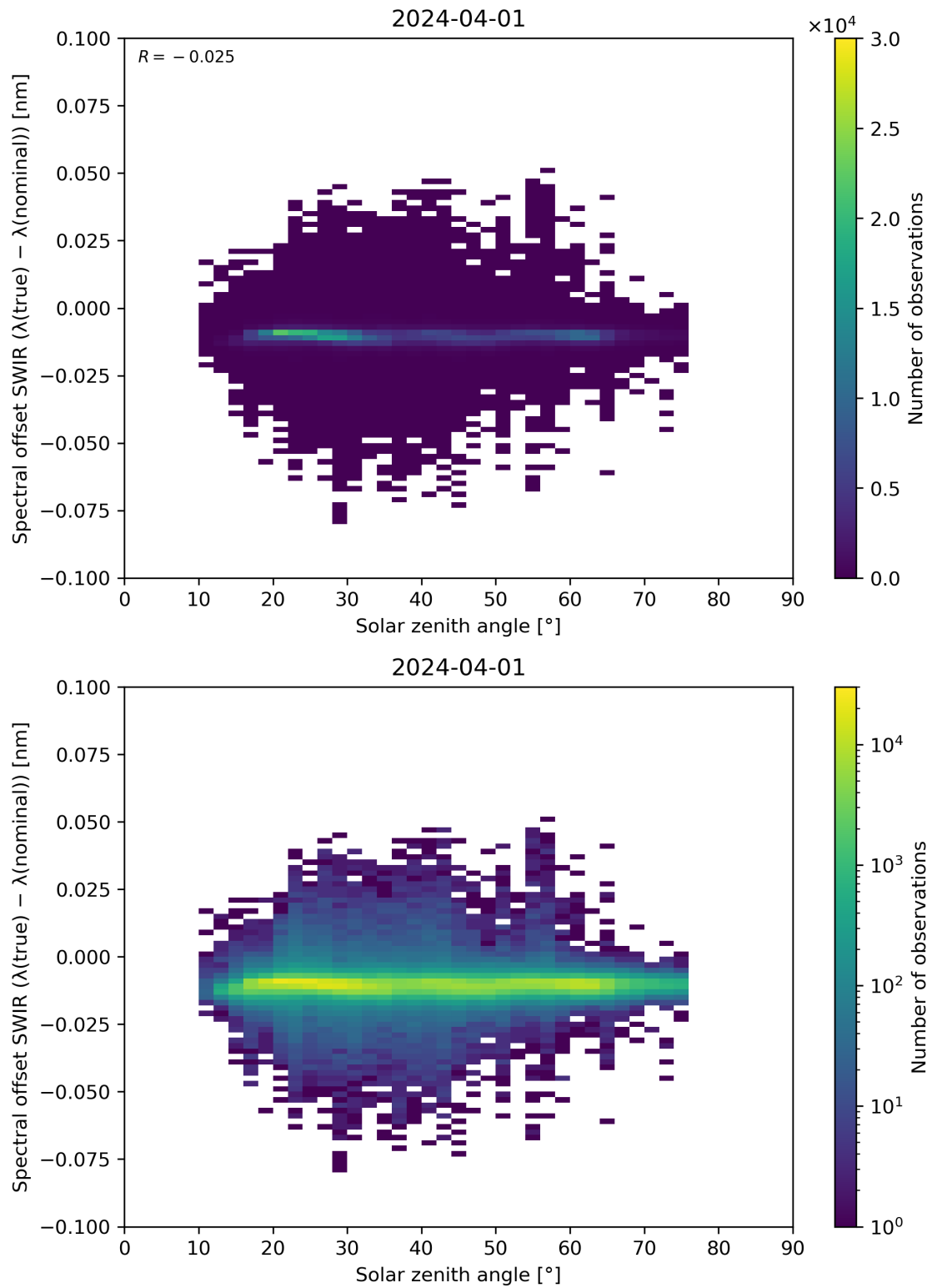
Figure 104: Scatter density plot of “Solar zenith angle” against “Spectral offset SWIR ( \lambda(\text{true}) - \lambda(\text{nominal}) )” for 2024-03-31 to 2024-04-02.
