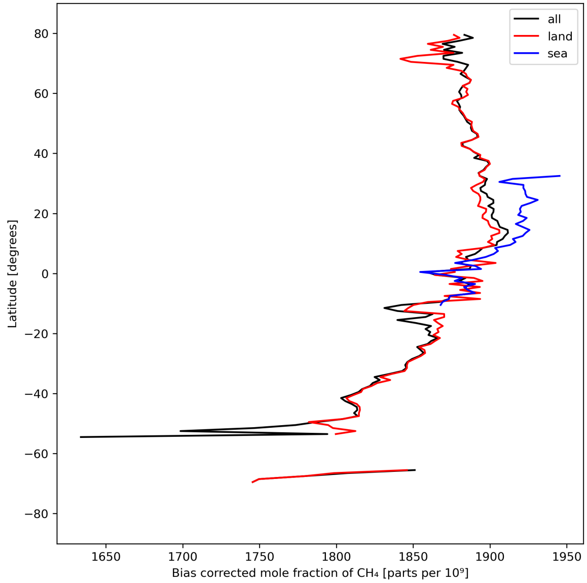
Figure 14: Zonal average of “Bias corrected mole fraction of CH 4 ” for 2024-03-31 to 2024-04-02.
