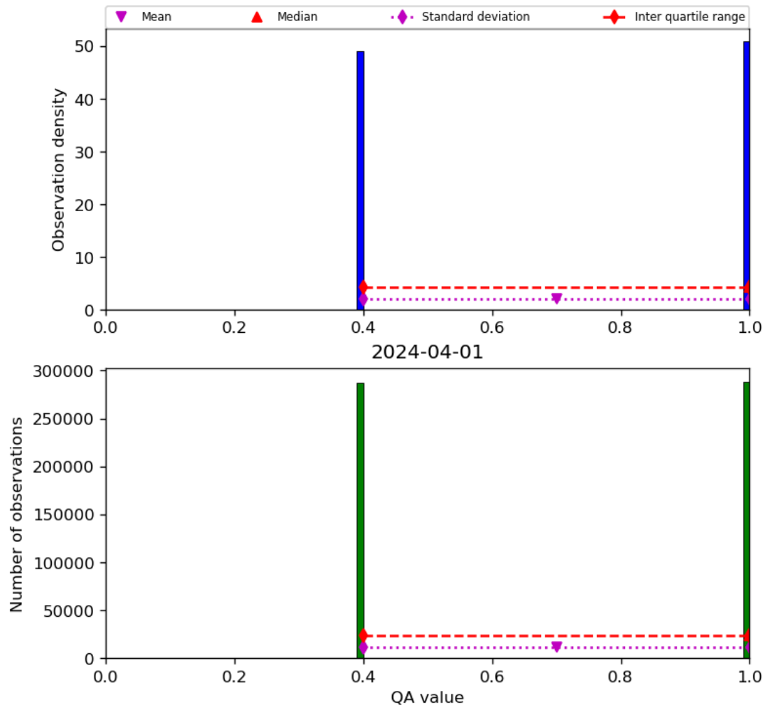
Figure 22: Histogram of “QA value” for 2024-03-31 to 2024-04-02
