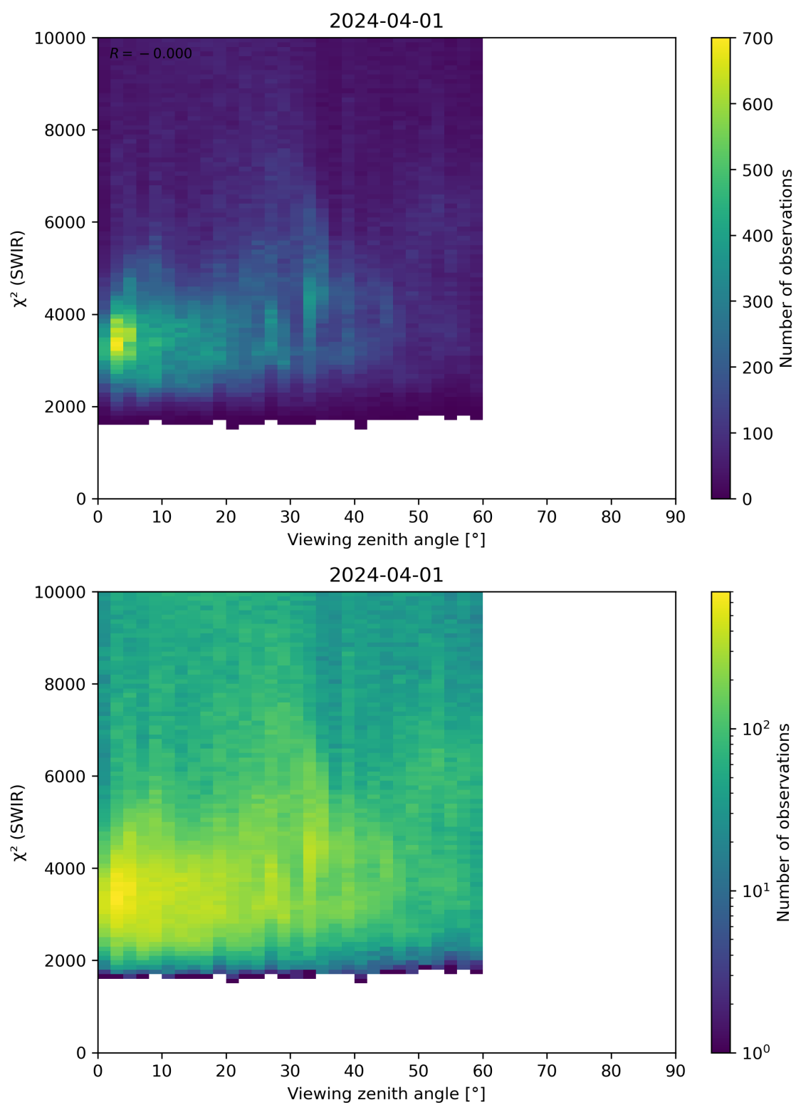
Figure 106: Scatter density plot of “Viewing zenith angle” against “ \chi^2 (SWIR)” for 2024-03-31 to 2024-04-02.
