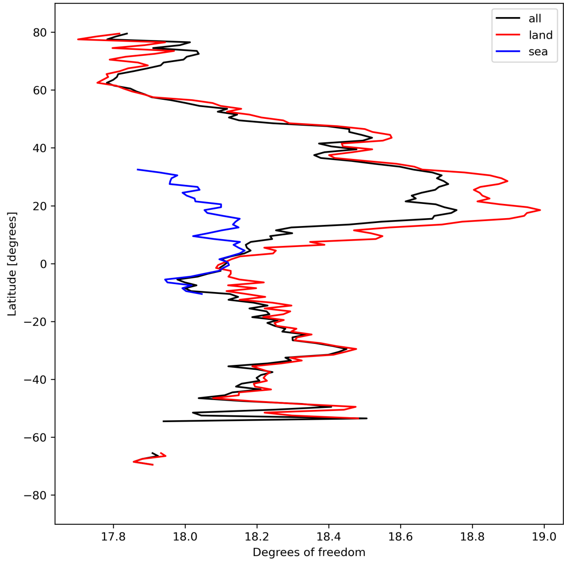
Figure 19: Zonal average of “Degrees of freedom” for 2024-03-31 to 2024-04-02.
