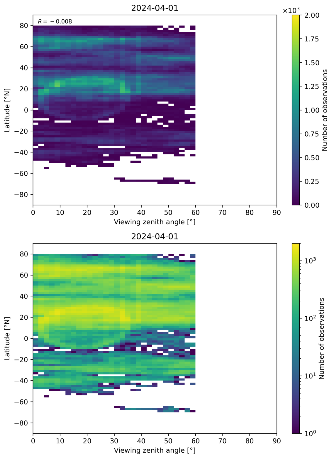
Figure 109: Scatter density plot of “Viewing zenith angle” against “Latitude” for 2024-03-31 to 2024-04-02.
