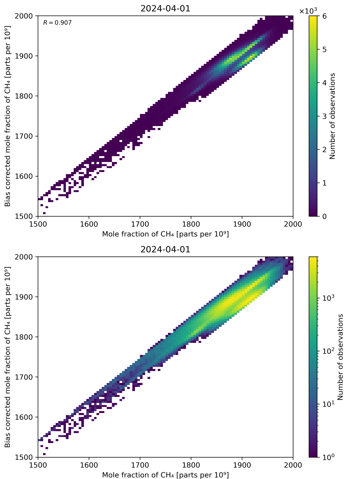
Figure 74: Scatter density plot of “Mole fraction of CH 4 ” against “Bias corrected mole fraction of CH 4 ” for 2024-03-31 to 2024-04-02.
