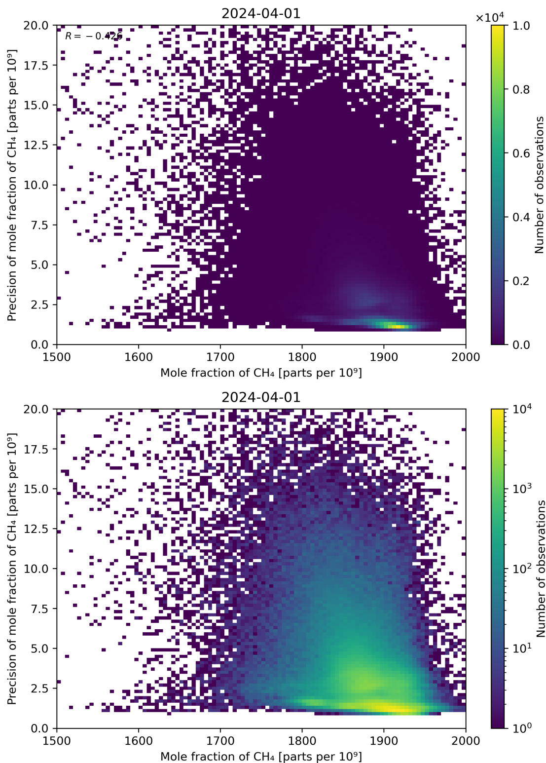
Figure 75: Scatter density plot of “Mole fraction of CH 4 ” against “Precision of mole fraction of CH 4 ” for 2024-03-31 to 2024-04-02.
