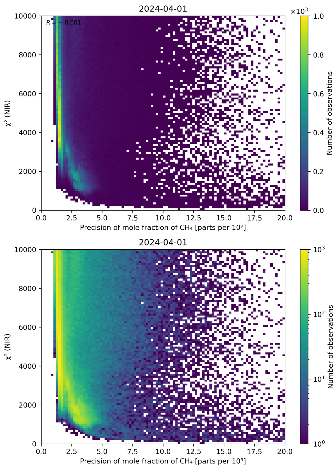
Figure 78: Scatter density plot of “Precision of mole fraction of CH 4 ” against “ \chi^2 (NIR)” for 2024-03-31 to 2024-04-02.
