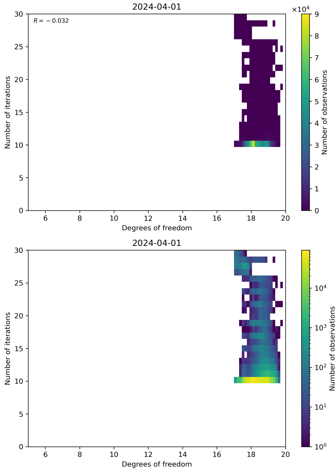
Figure 52: Scatter density plot of “Degrees of freedom” against “Number of iterations” for 2024-03-31 to 2024-04-02.
