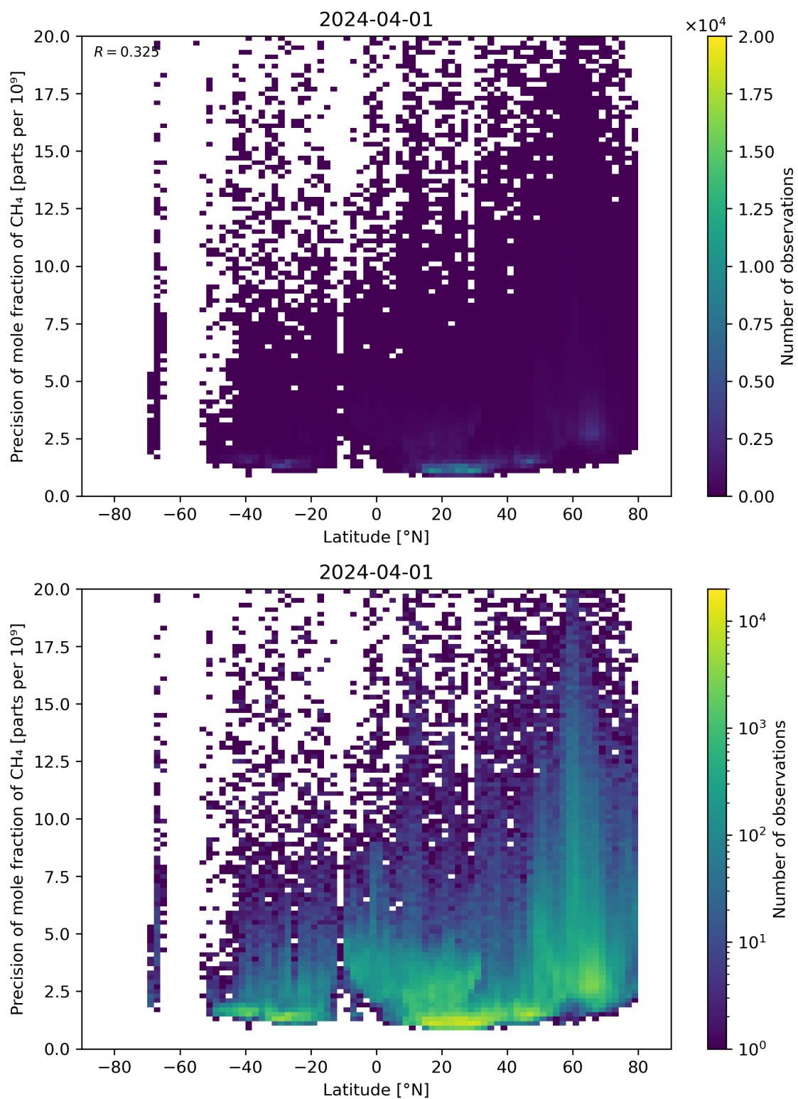
Figure 59: Scatter density plot of “Latitude” against “Precision of mole fraction of CH 4 ” for 2024-03-31 to 2024-04-02.
