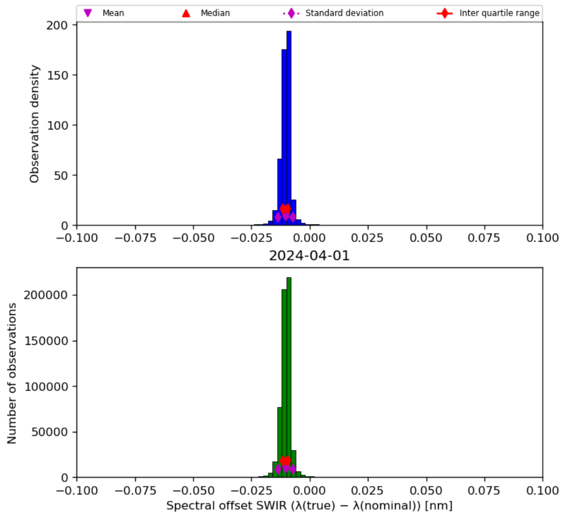
Figure 27: Histogram of “Spectral offset SWIR ( \lambda(\text{true}) - \lambda(\text{nominal}) )” for 2024-03-31 to 2024-04-02
