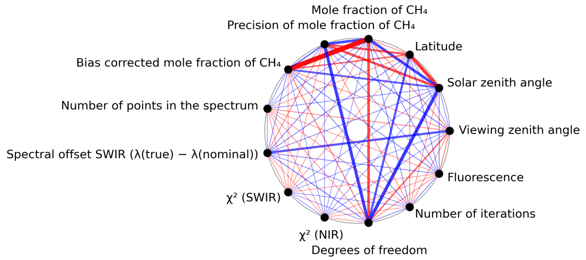
Figure 1: Map of correlation graph for 2024-03-31 to 2024-04-02.
