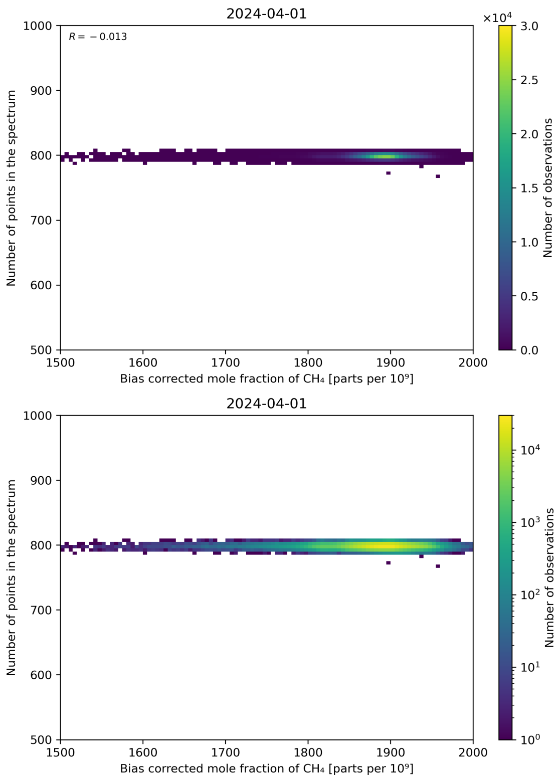
Figure 68: Scatter density plot of “Bias corrected mole fraction of CH 4 ” against “Number of points in the spectrum” for 2024-03-31 to 2024-04-02.
