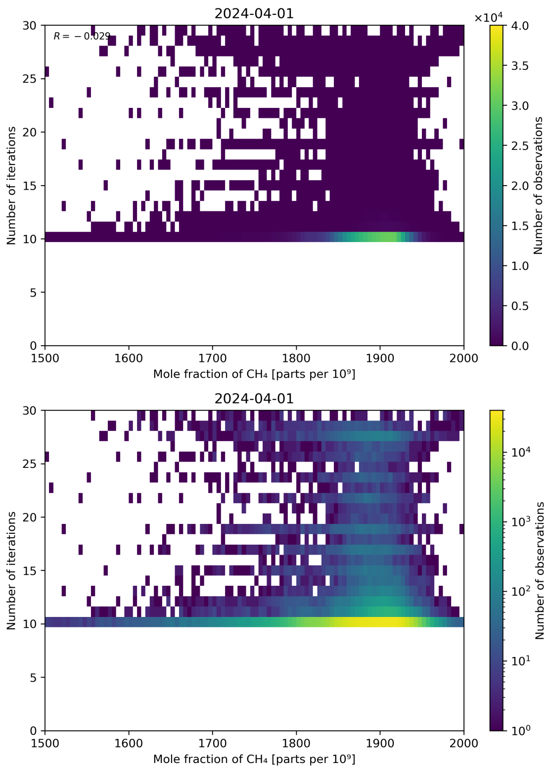
Figure 76: Scatter density plot of “Mole fraction of CH 4 ” against “Number of iterations” for 2024-03-31 to 2024-04-02.
