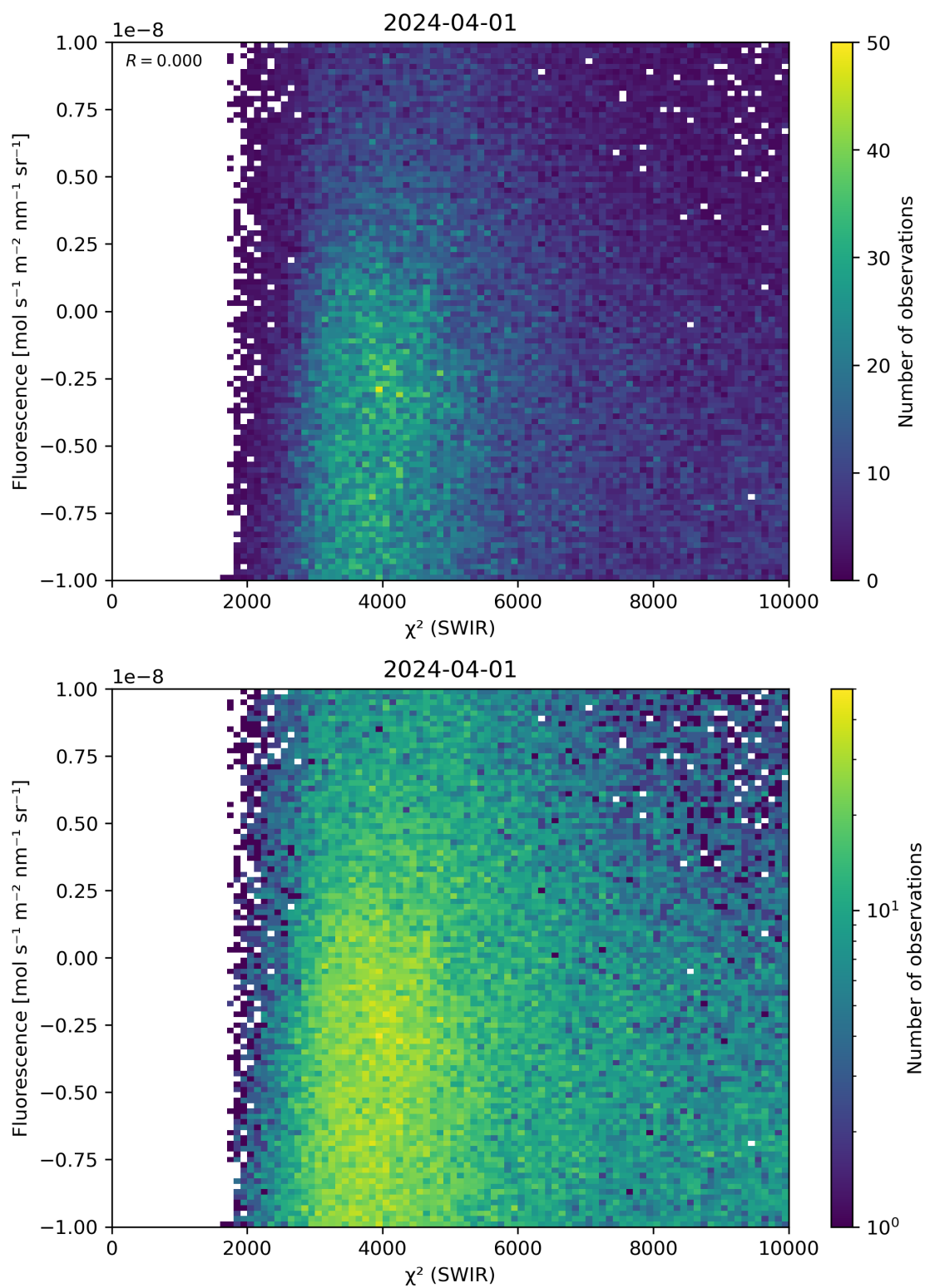
Figure 49: Scatter density plot of “ \chi^2 (SWIR)” against “Fluorescence” for 2024-03-31 to 2024-04-02.
