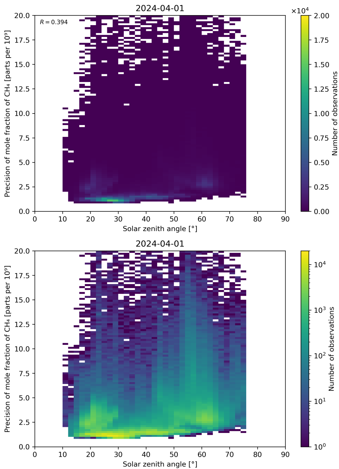
Figure 101: Scatter density plot of “Solar zenith angle” against “Precision of mole fraction of CH 4 ” for 2024-03-31 to 2024-04-02.
