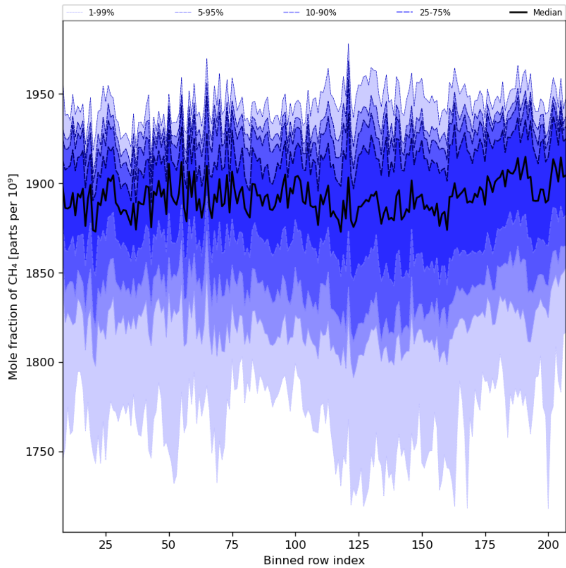
Figure 34: Along track statistics of “Mole fraction of CH 4 ” for 2024-03-31 to 2024-04-02
