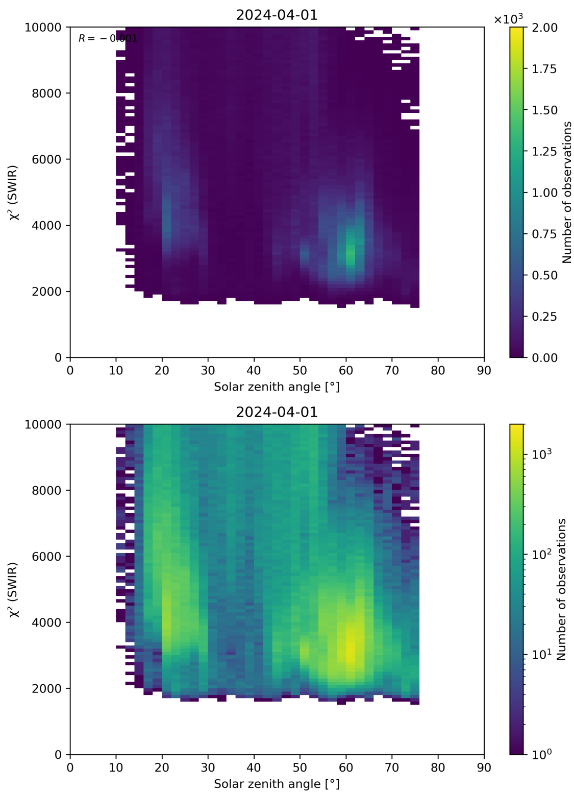
Figure 95: Scatter density plot of “Solar zenith angle” against “ \chi^2 (SWIR)” for 2024-03-31 to 2024-04-02.
