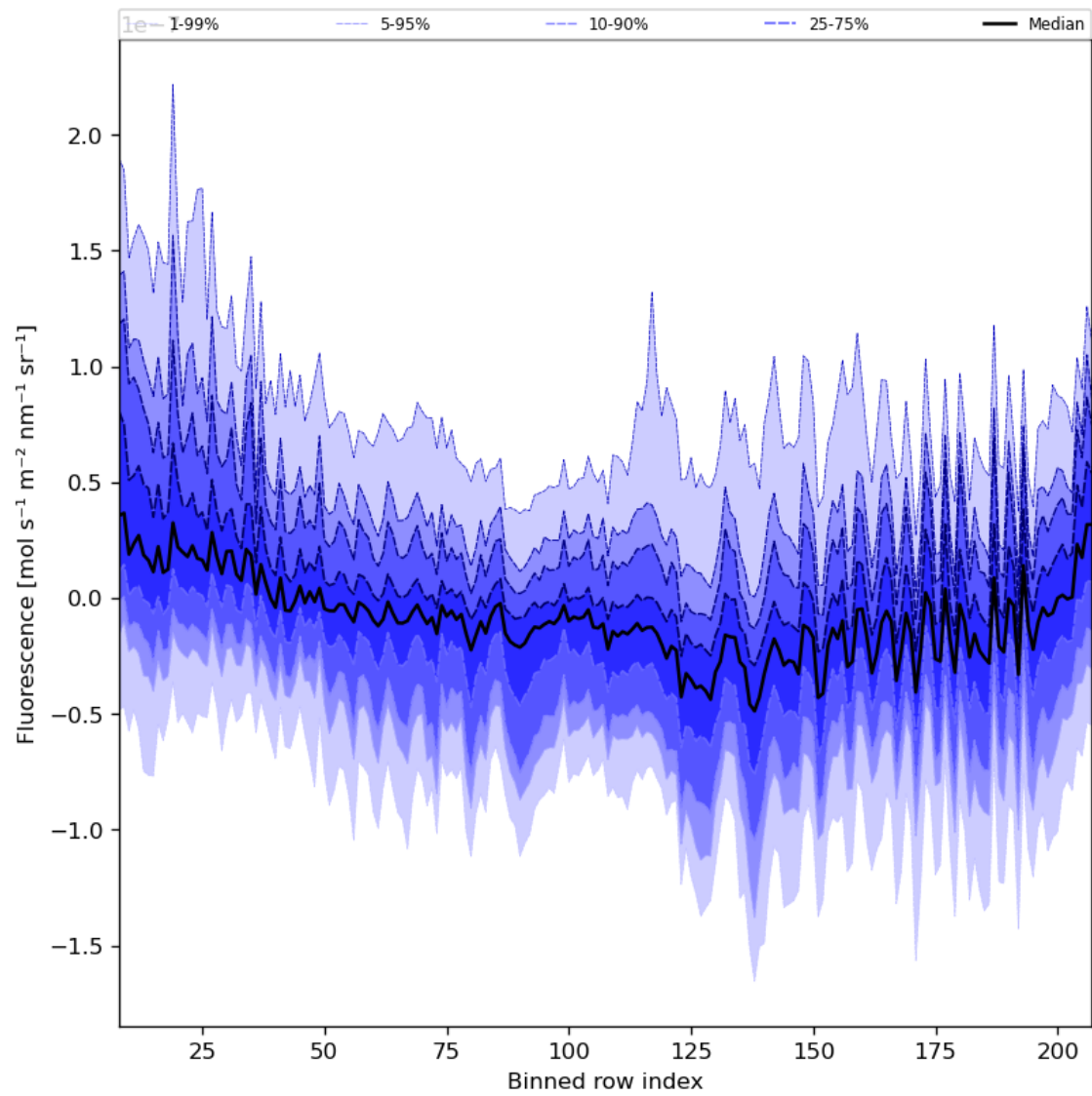
Figure 43: Along track statistics of “Fluorescence” for 2024-03-31 to 2024-04-02
