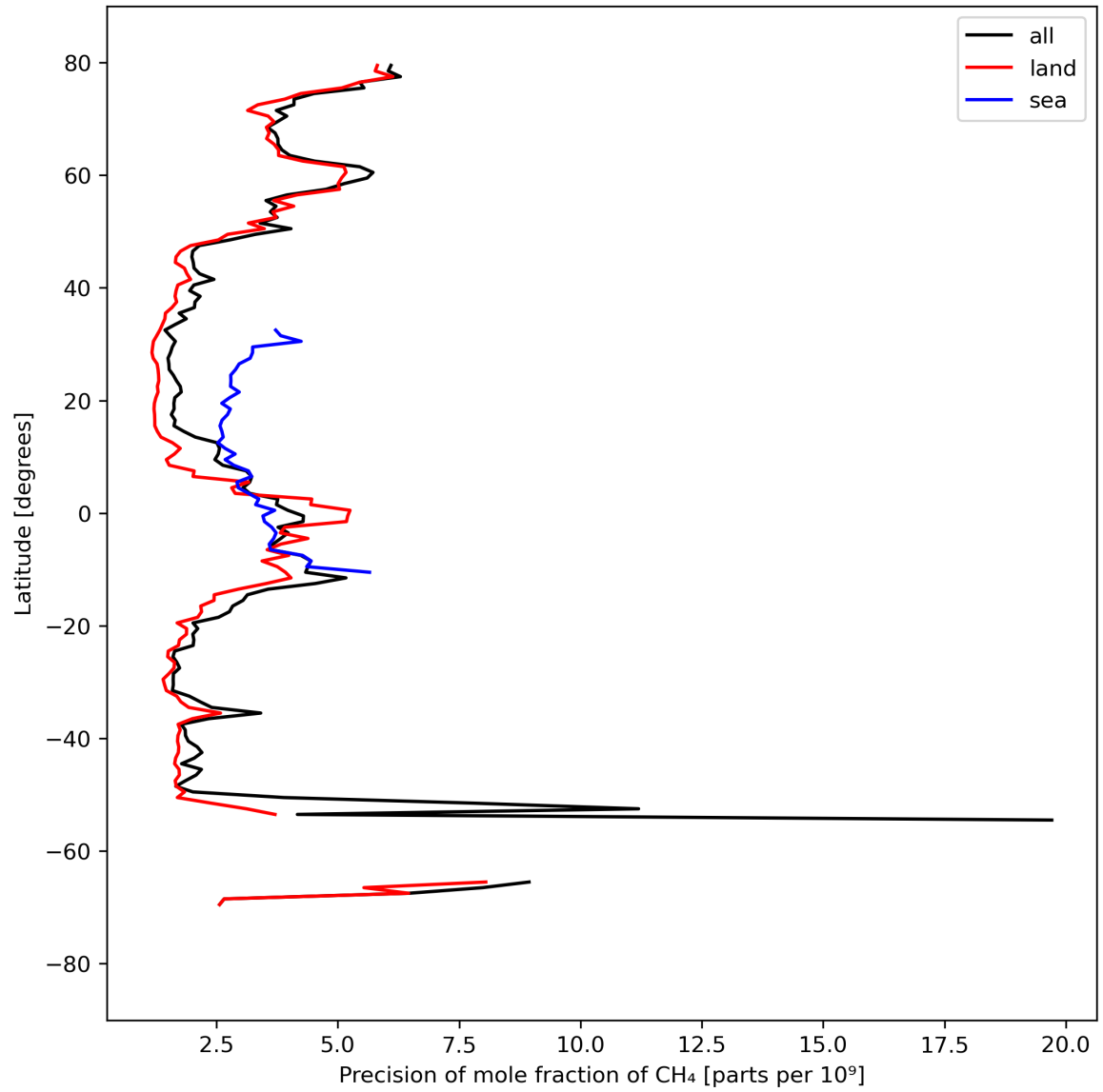
Figure 13: Zonal average of “Precision of mole fraction of CH 4 ” for 2024-03-31 to 2024-04-02.
