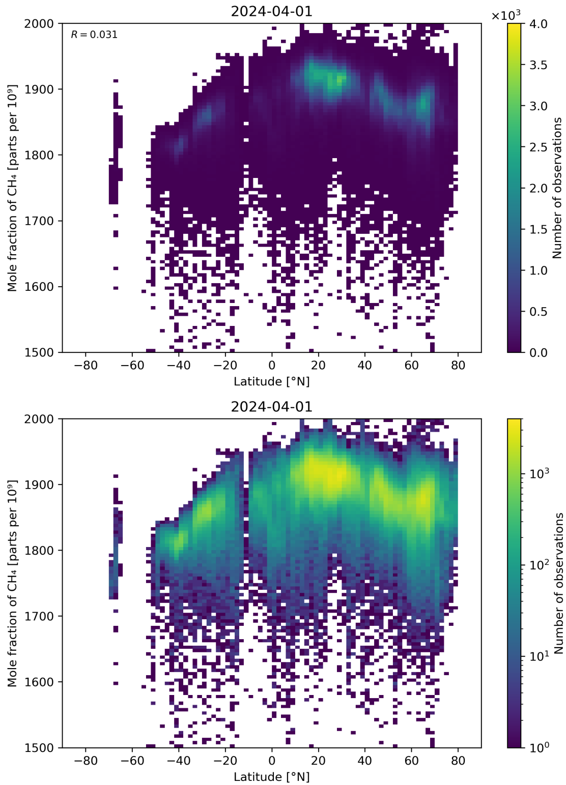
Figure 57: Scatter density plot of “Latitude” against “Mole fraction of CH 4 ” for 2024-03-31 to 2024-04-02.
