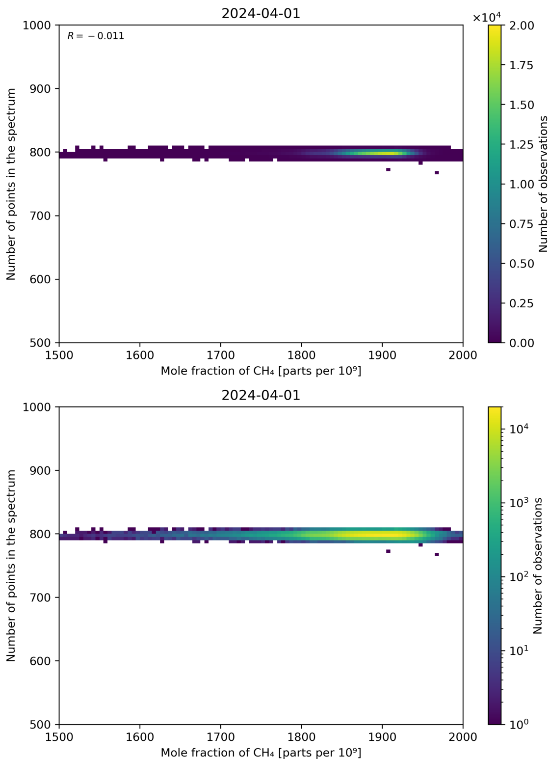
Figure 77: Scatter density plot of “Mole fraction of CH 4 ” against “Number of points in the spectrum” for 2024-03-31 to 2024-04-02.
