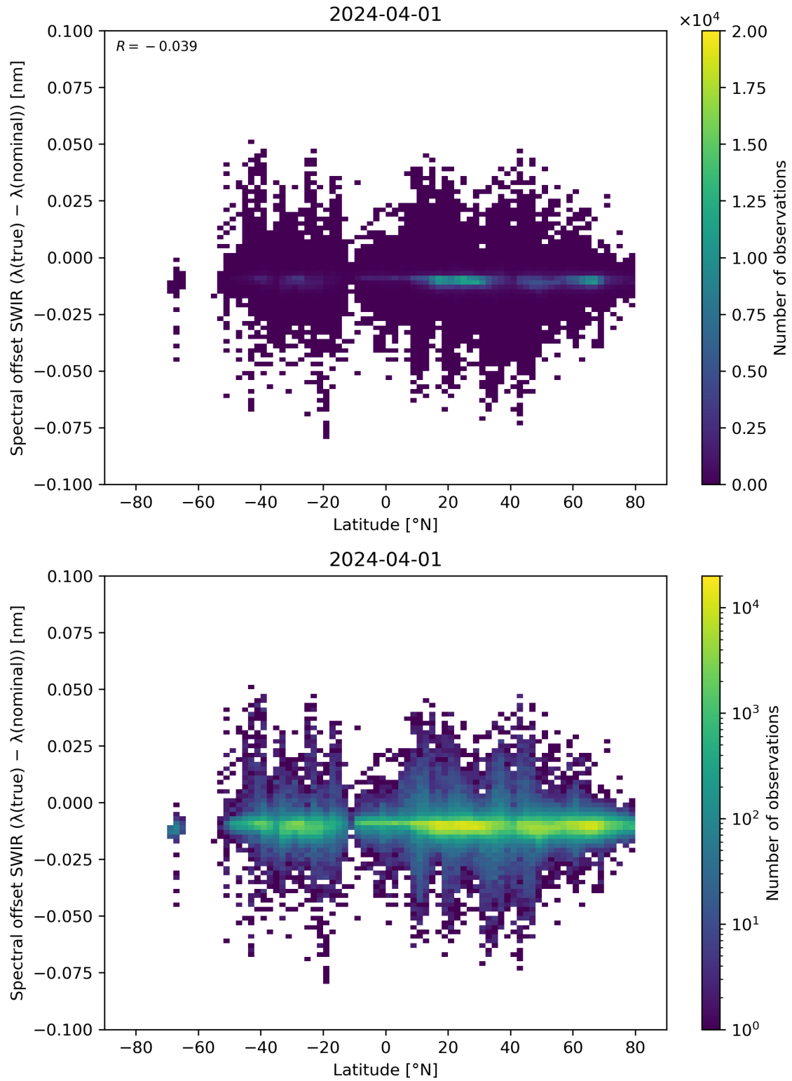
Figure 62: Scatter density plot of “Latitude” against “Spectral offset SWIR ( \lambda(\text{true}) - \lambda(\text{nominal}) )” for 2024-03-31 to 2024-04-02.
