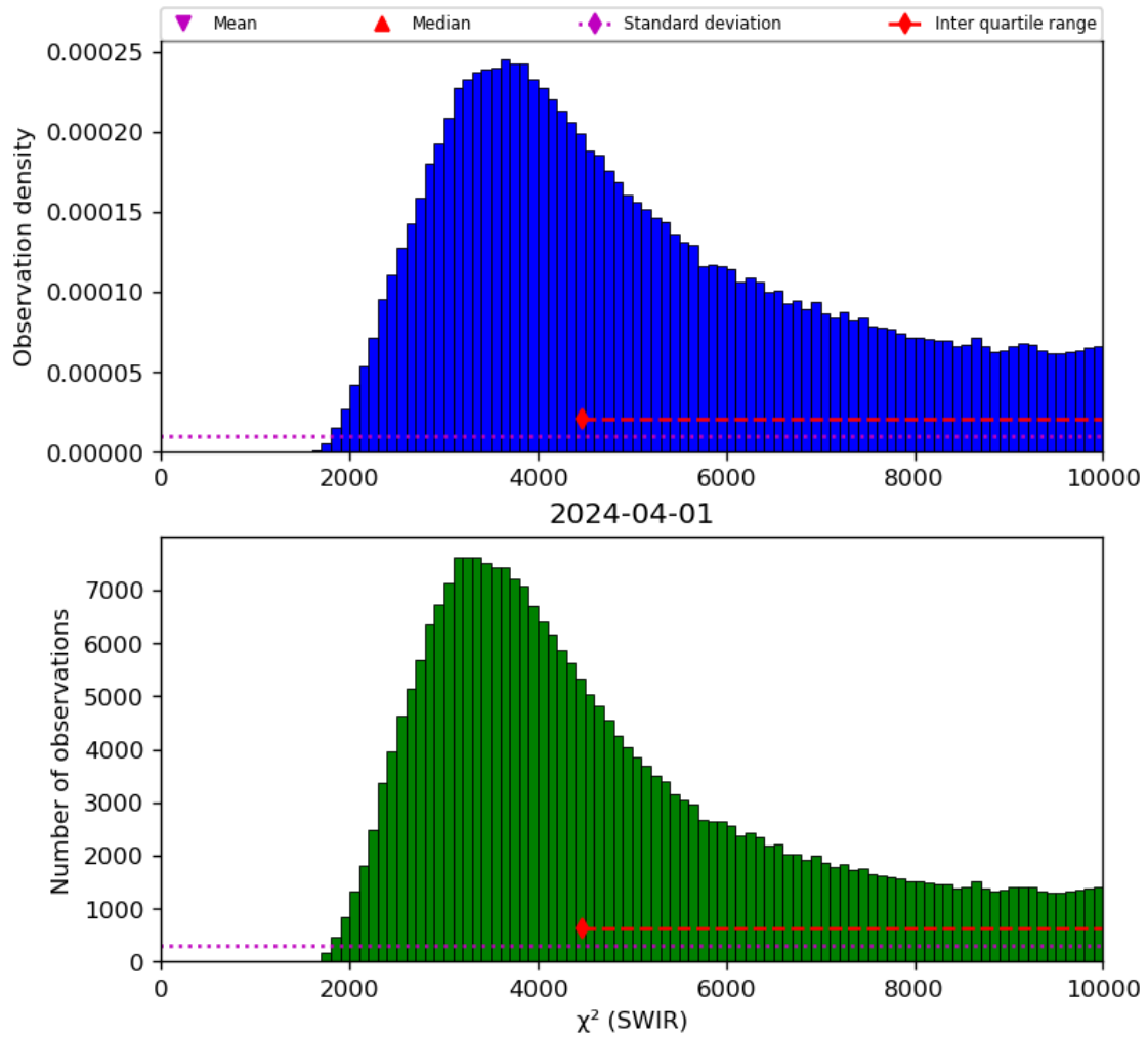
Figure 28: Histogram of “ \chi^2 (SWIR)” for 2024-03-31 to 2024-04-02
