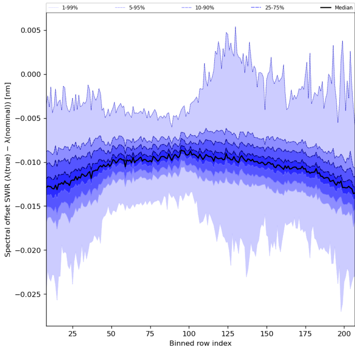
Figure 38: Along track statistics of “Spectral offset SWIR ( \lambda(\text{true}) - \lambda(\text{nominal}) )” for 2024-03-31 to 2024-04-02
