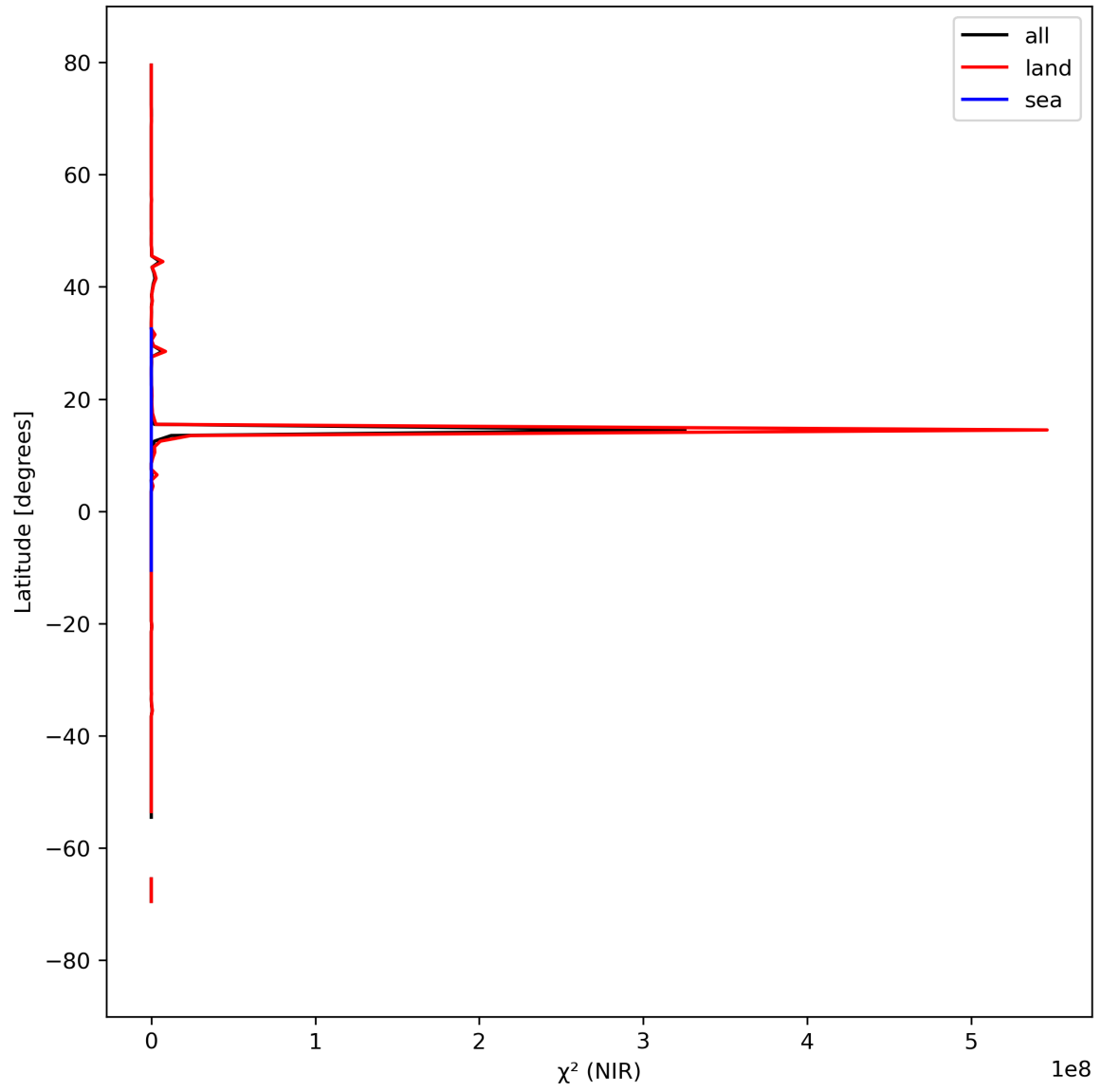
Figure 18: Zonal average of “ \chi^2 (NIR)” for 2024-03-31 to 2024-04-02.
