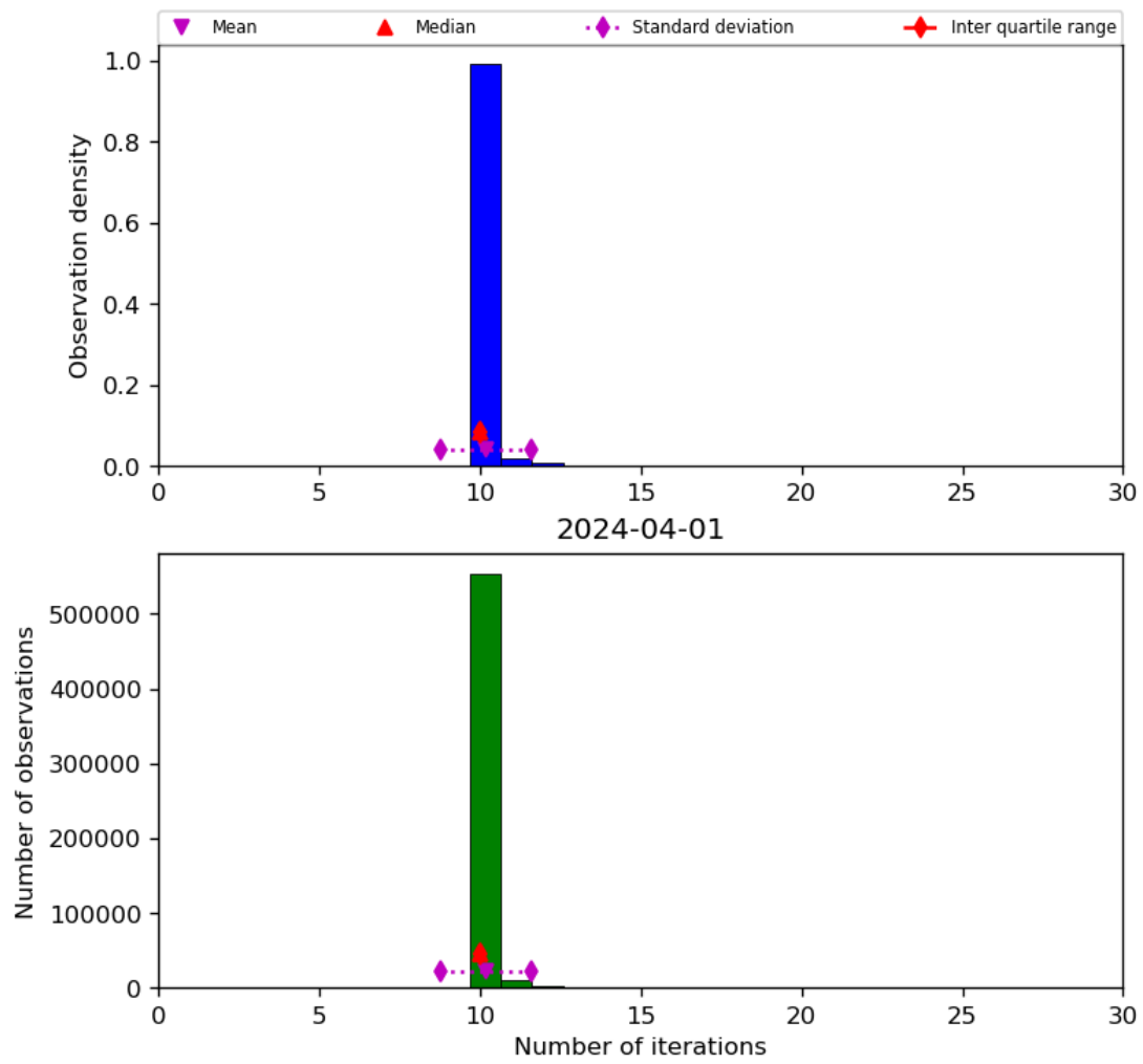
Figure 31: Histogram of "Number of iterations" for 2024-03-31 to 2024-04-02
