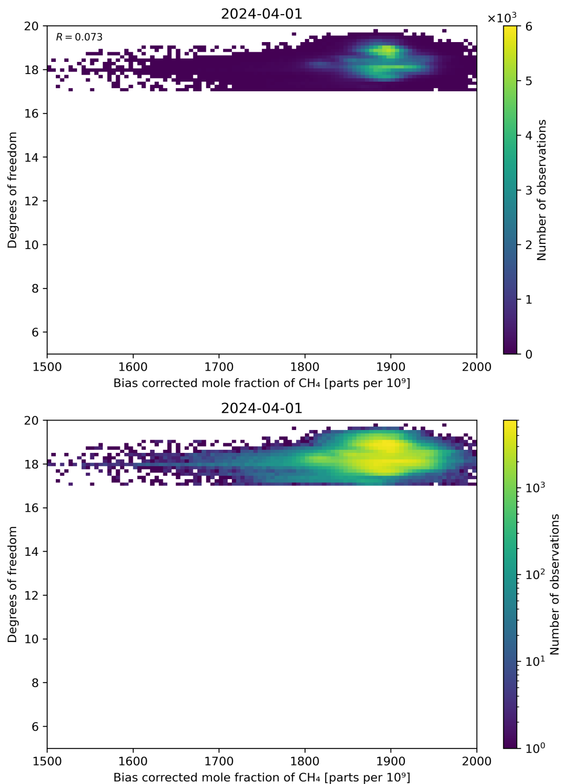
Figure 65: Scatter density plot of “Bias corrected mole fraction of CH 4 ” against “Degrees of freedom” for 2024-03-31 to 2024-04-02.
