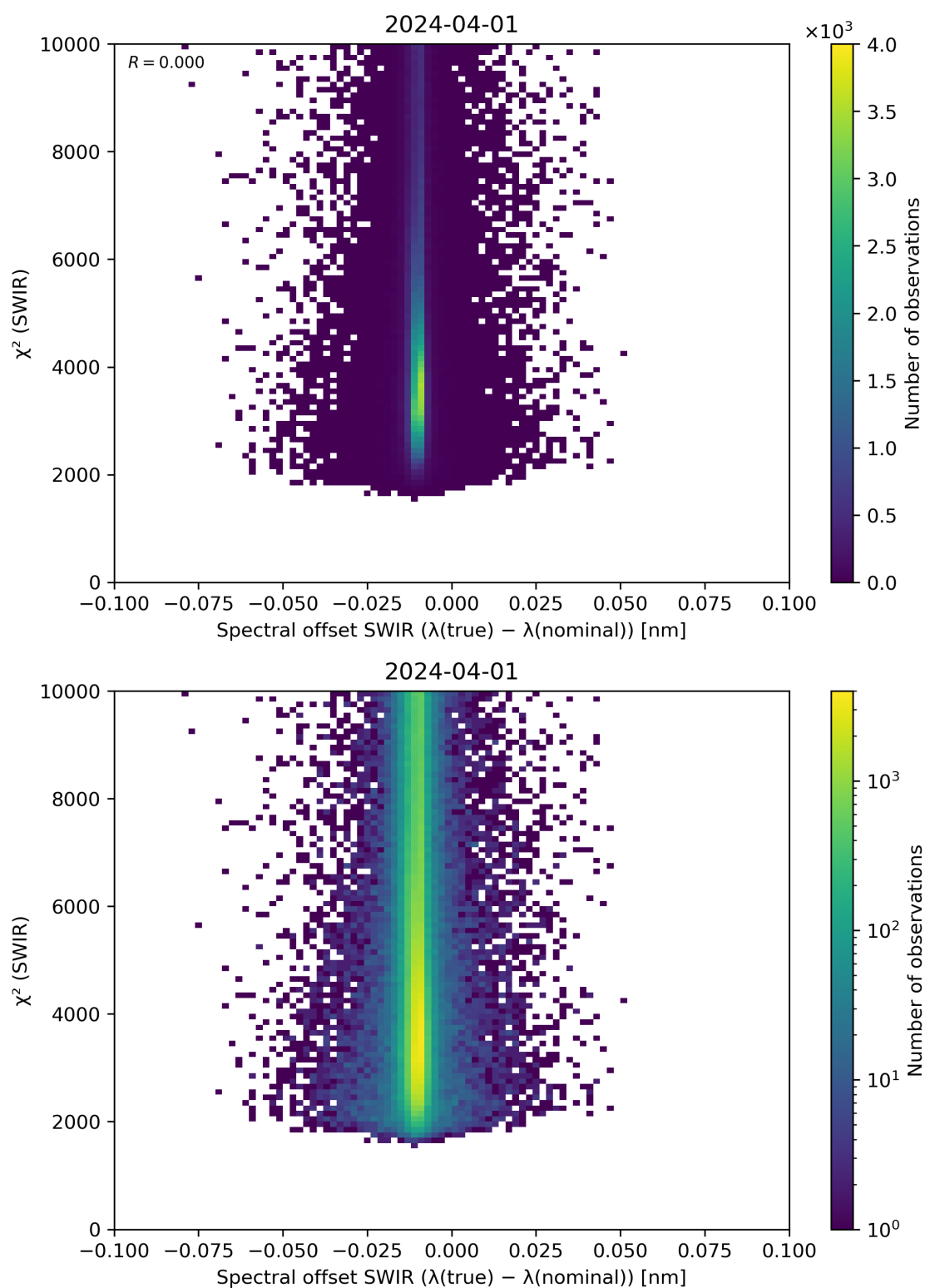
Figure 118: Scatter density plot of “Spectral offset SWIR ( \lambda(\text{true}) - \lambda(\text{nominal}) )” against “ \chi^2 (SWIR)” for 2024-03-31 to 2024-04-02.
