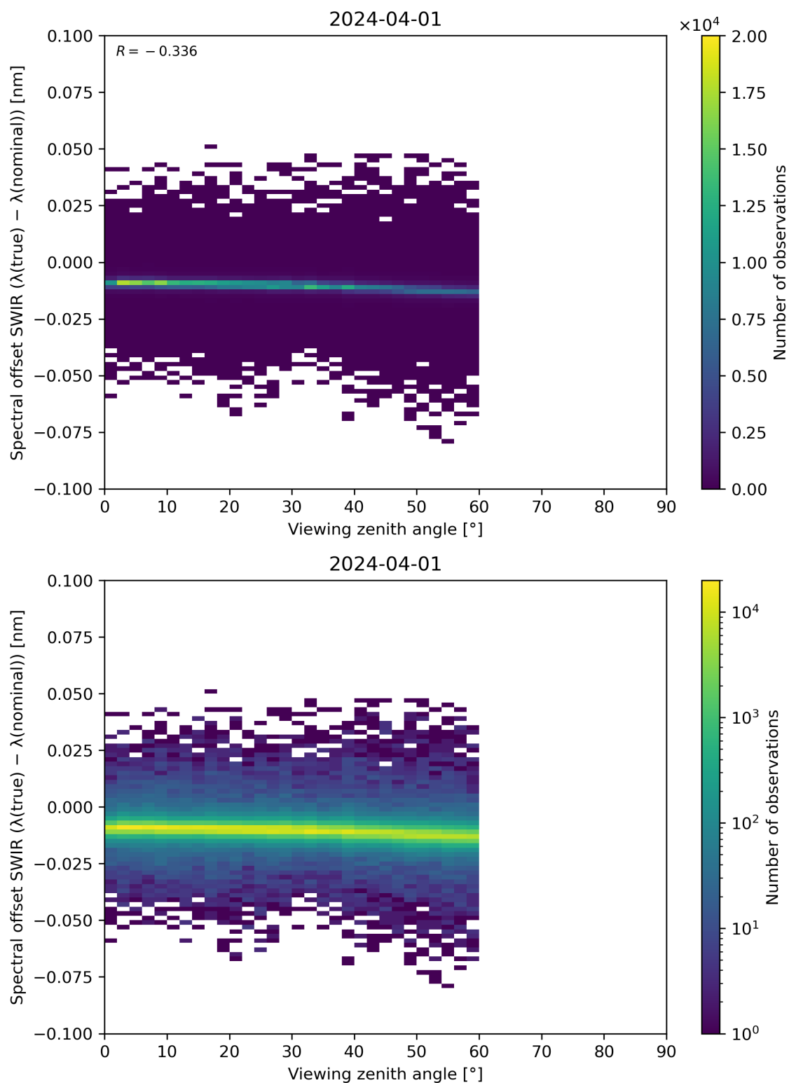
Figure 116: Scatter density plot of “Viewing zenith angle” against “Spectral offset SWIR ( \lambda(\text{true}) - \lambda(\text{nominal}) )” for 2024-03-31 to 2024-04-02.
