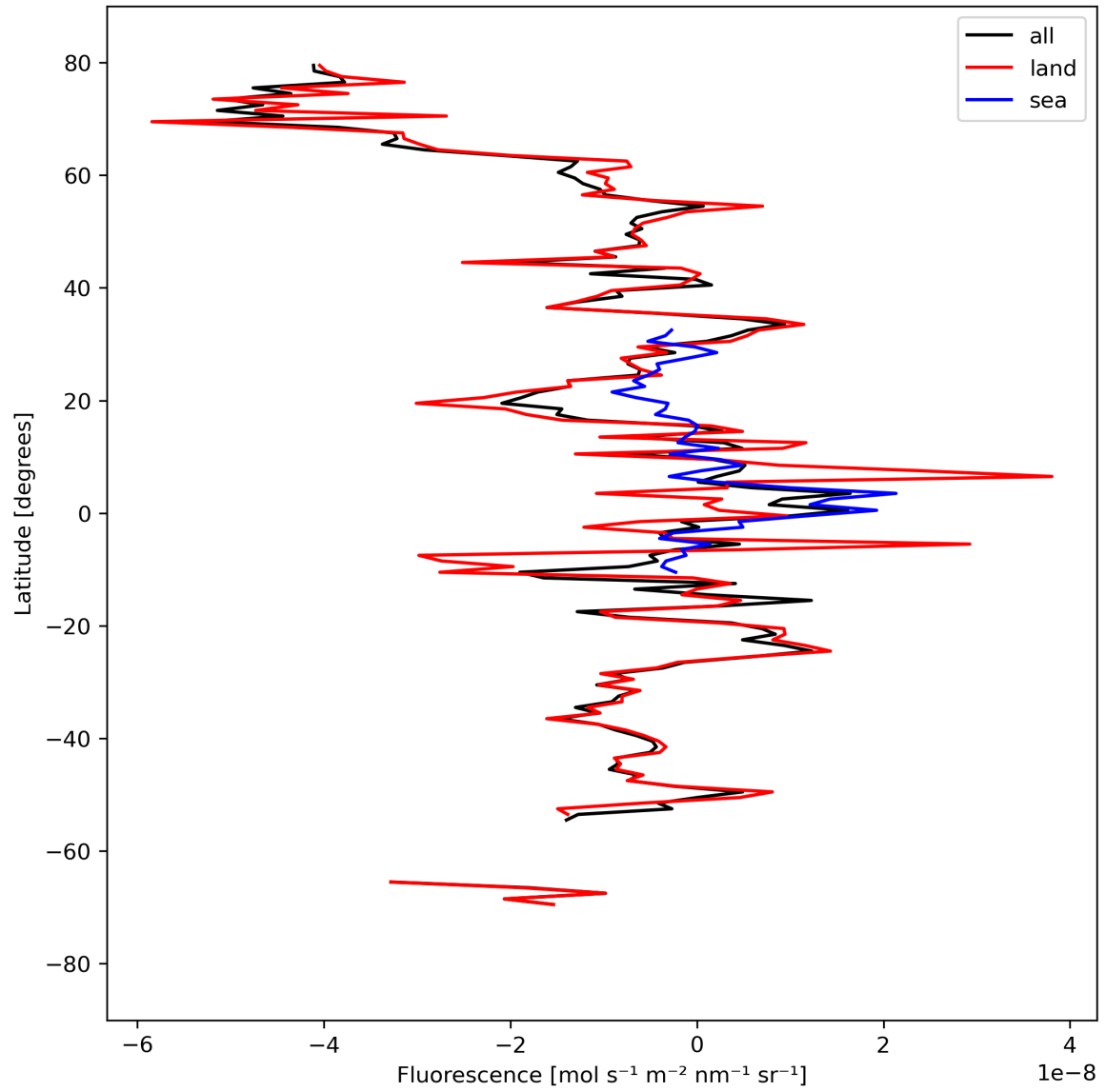
Figure 21: Zonal average of “Fluorescence” for 2024-03-31 to 2024-04-02.
