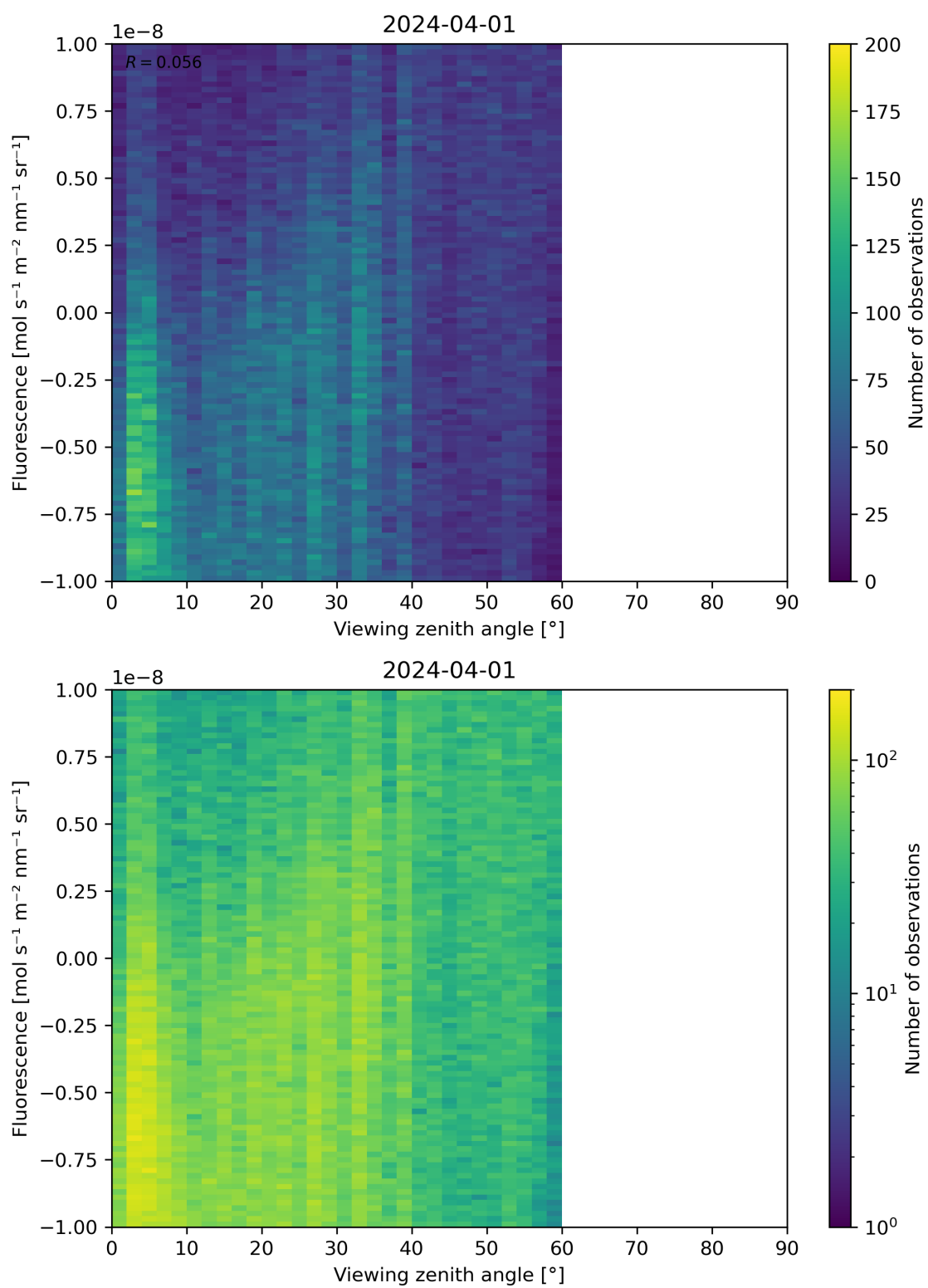
Figure 108: Scatter density plot of “Viewing zenith angle” against “Fluorescence” for 2024-03-31 to 2024-04-02.
