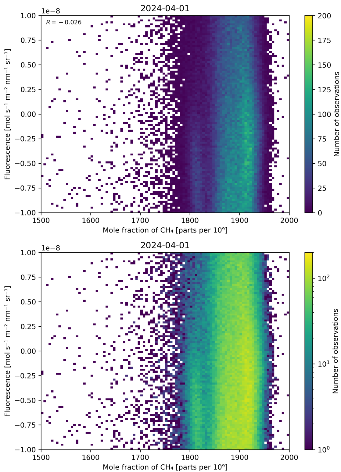
Figure 73: Scatter density plot of “Mole fraction of \text{CH}_4 ” against “Fluorescence” for 2024-03-31 to 2024-04-02.
