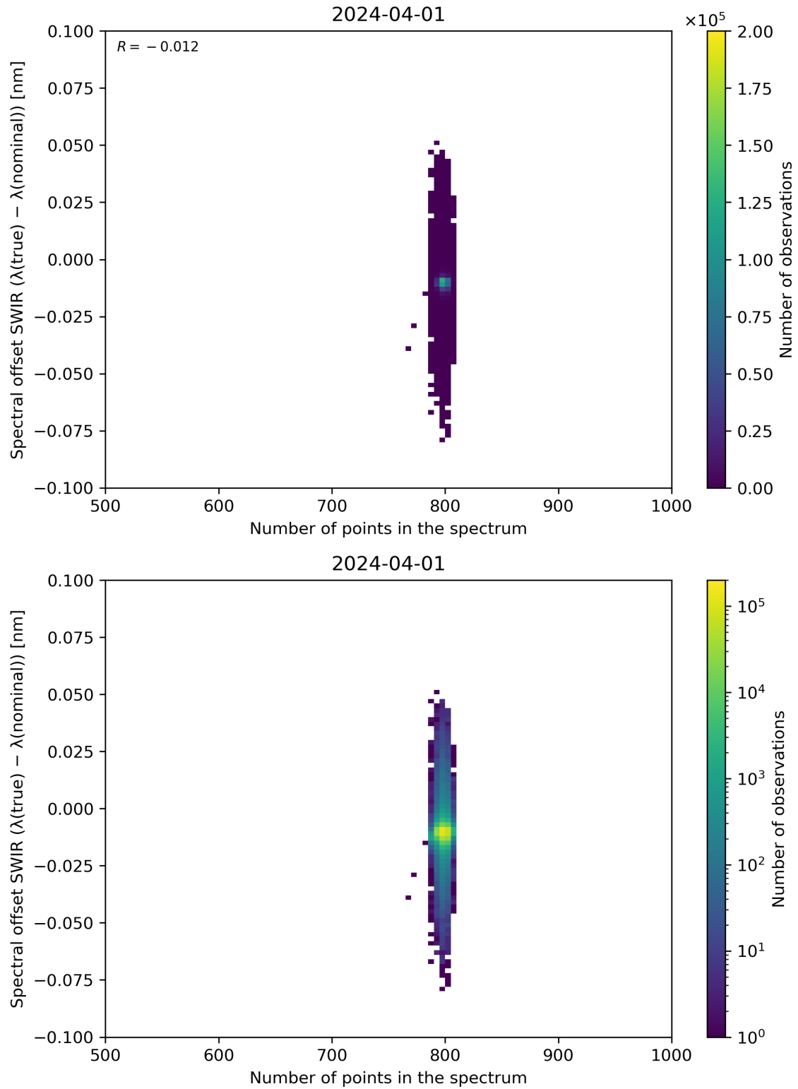
Figure 93: Scatter density plot of “Number of points in the spectrum” against “Spectral offset SWIR ( \lambda(\text{true}) - \lambda(\text{nominal}) )” for 2024-03-31 to 2024-04-02.
