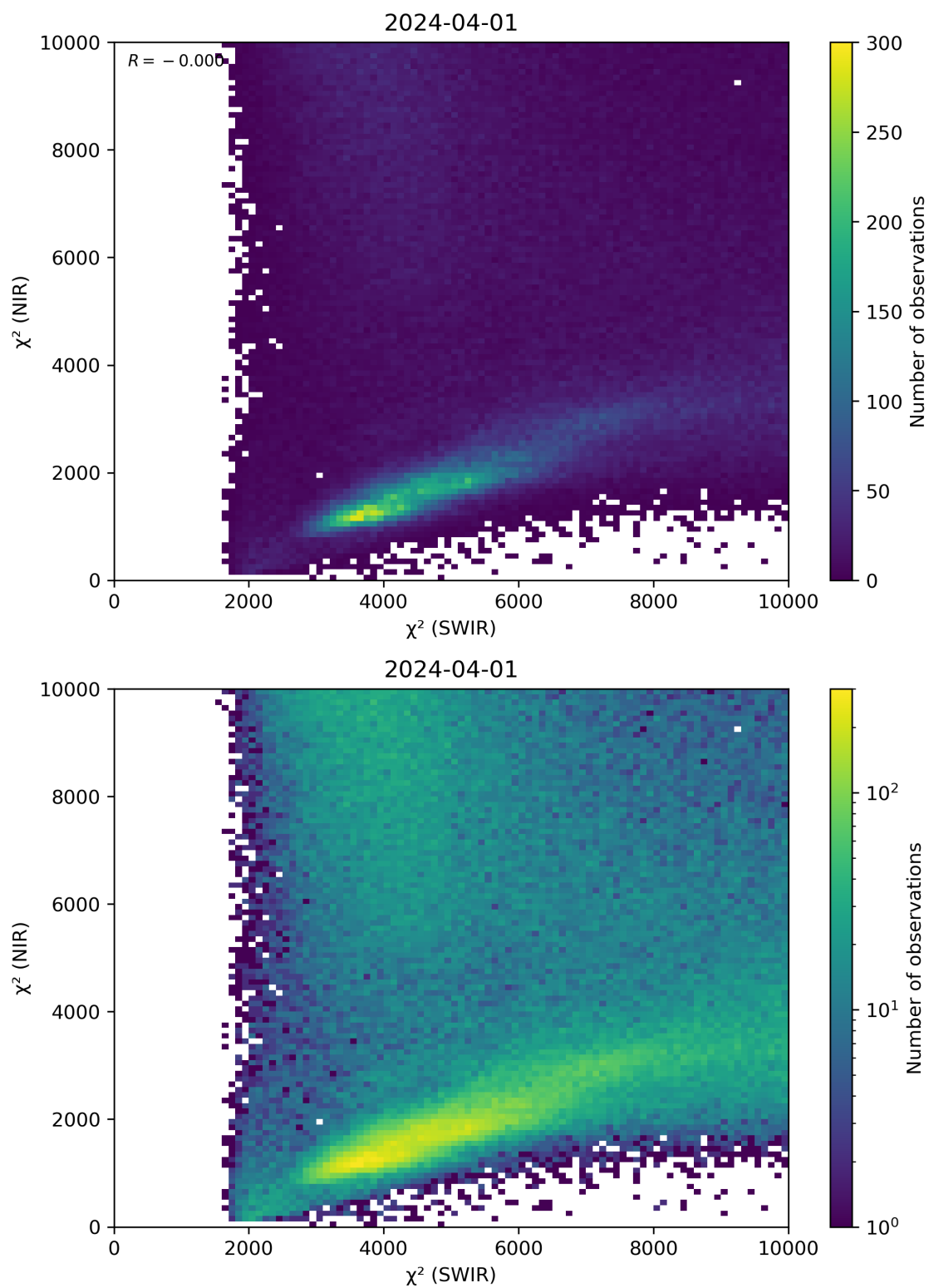
Figure 47: Scatter density plot of “ \chi^2 (SWIR)” against “ \chi^2 (NIR)” for 2024-03-31 to 2024-04-02.
