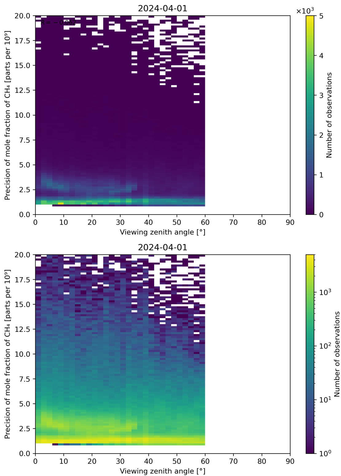
Figure 112: Scatter density plot of “Viewing zenith angle” against “Precision of mole fraction of CH 4 ” for 2024-03-31 to 2024-04-02.
