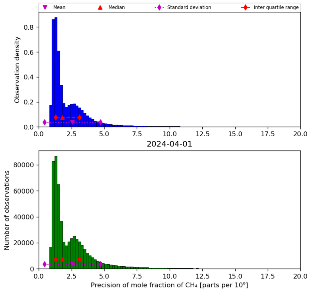
Figure 24: Histogram of “Precision of mole fraction of CH 4 ” for 2024-03-31 to 2024-04-02
