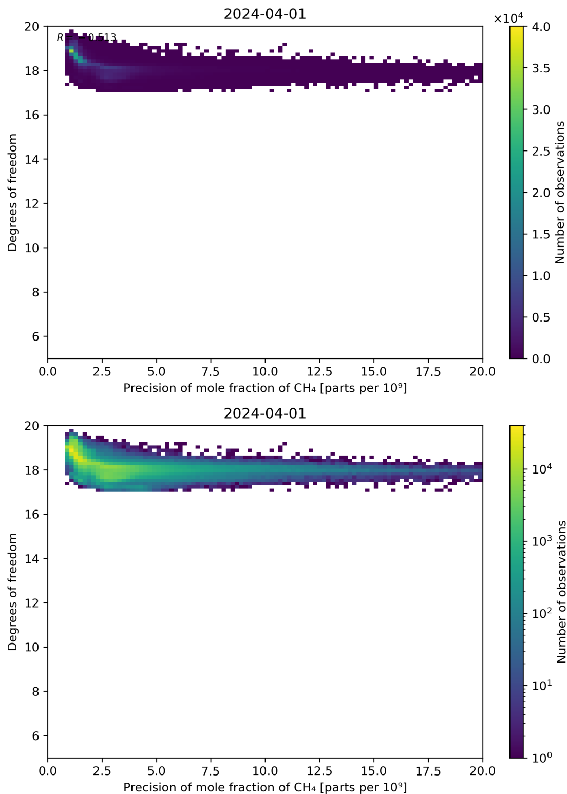
Figure 80: Scatter density plot of “Precision of mole fraction of CH 4 ” against “Degrees of freedom” for 2024-03-31 to 2024-04-02.
