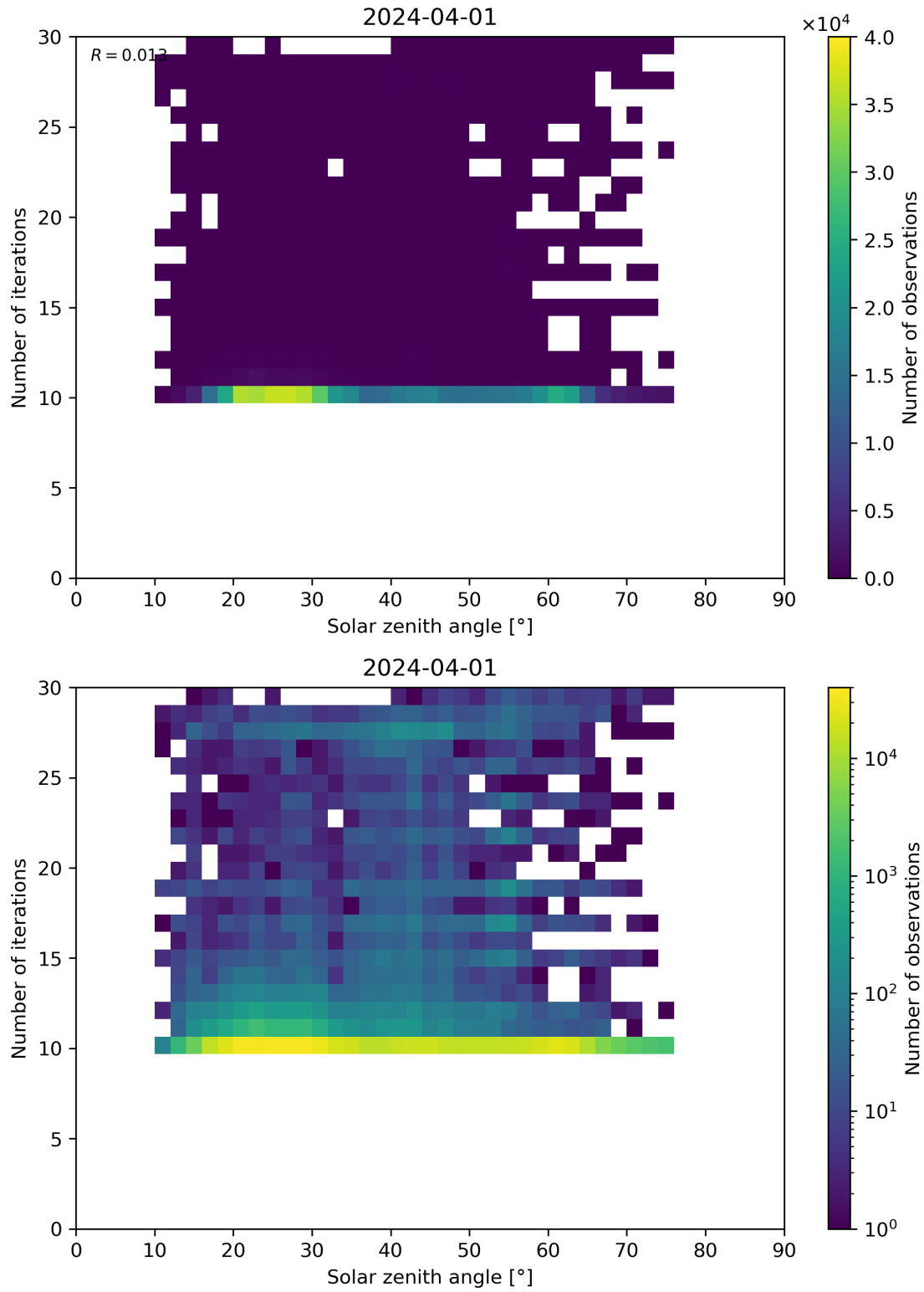
Figure 102: Scatter density plot of “Solar zenith angle” against “Number of iterations” for 2024-03-31 to 2024-04-02.
