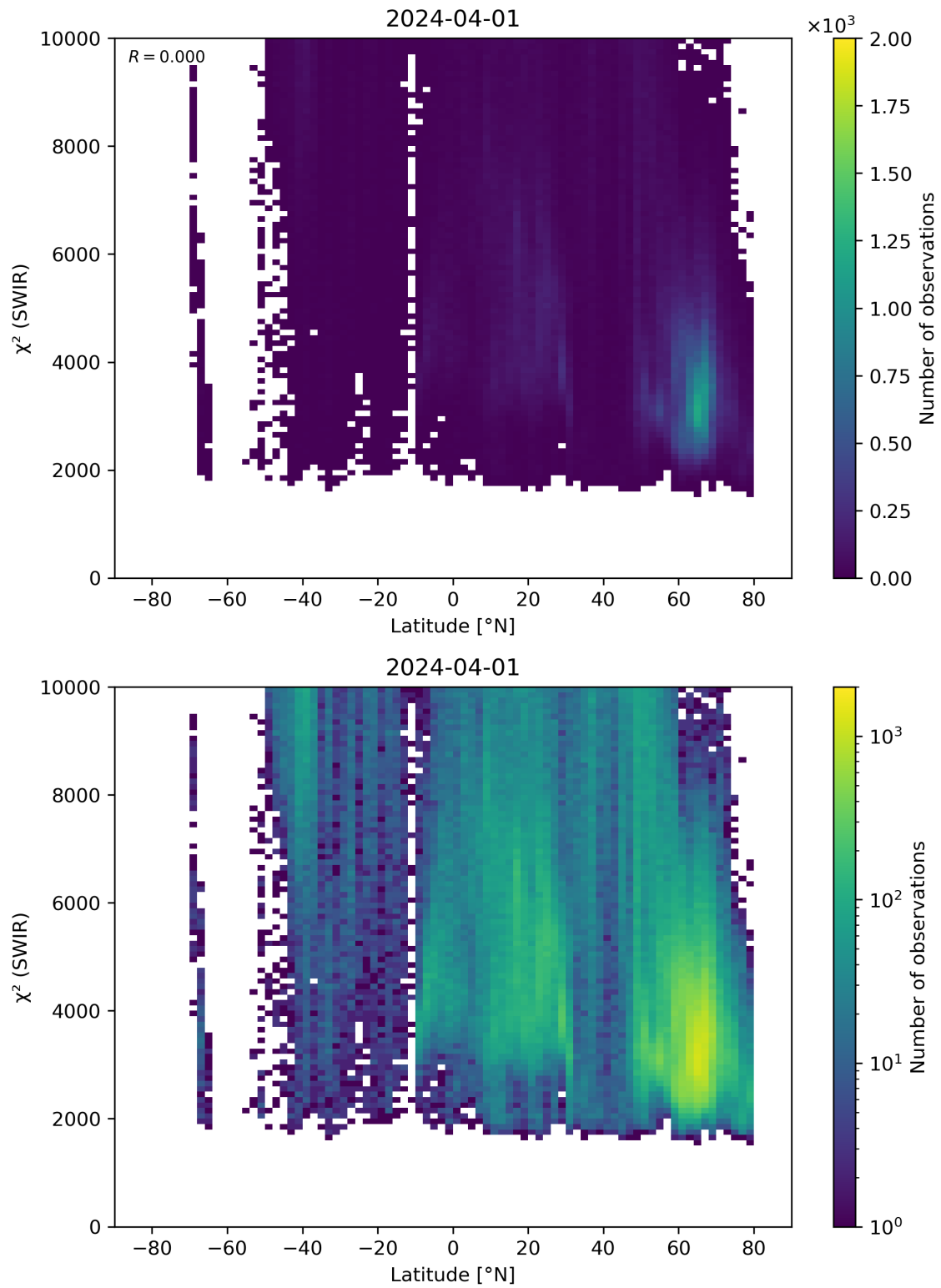
Figure 54: Scatter density plot of “Latitude” against “ \chi^2 (SWIR)” for 2024-03-31 to 2024-04-02.
