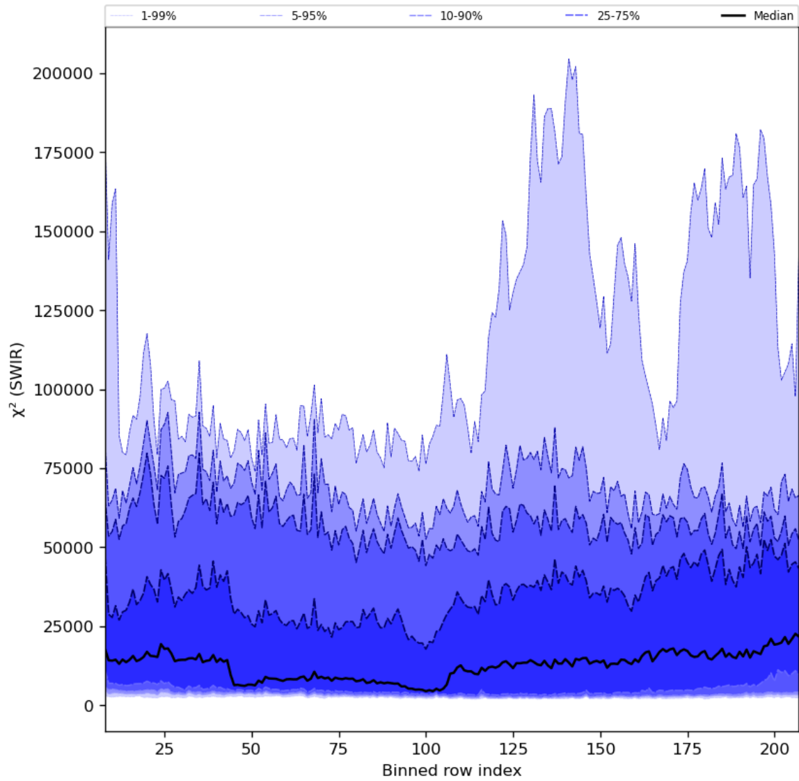
Figure 39: Along track statistics of “ \chi^2 (SWIR)” for 2024-03-31 to 2024-04-02
