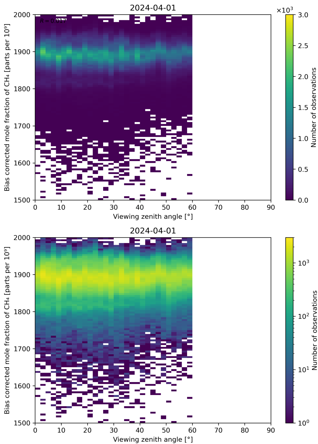
Figure 111: Scatter density plot of “Viewing zenith angle” against “Bias corrected mole fraction of CH 4 ” for 2024-03-31 to 2024-04-02.
