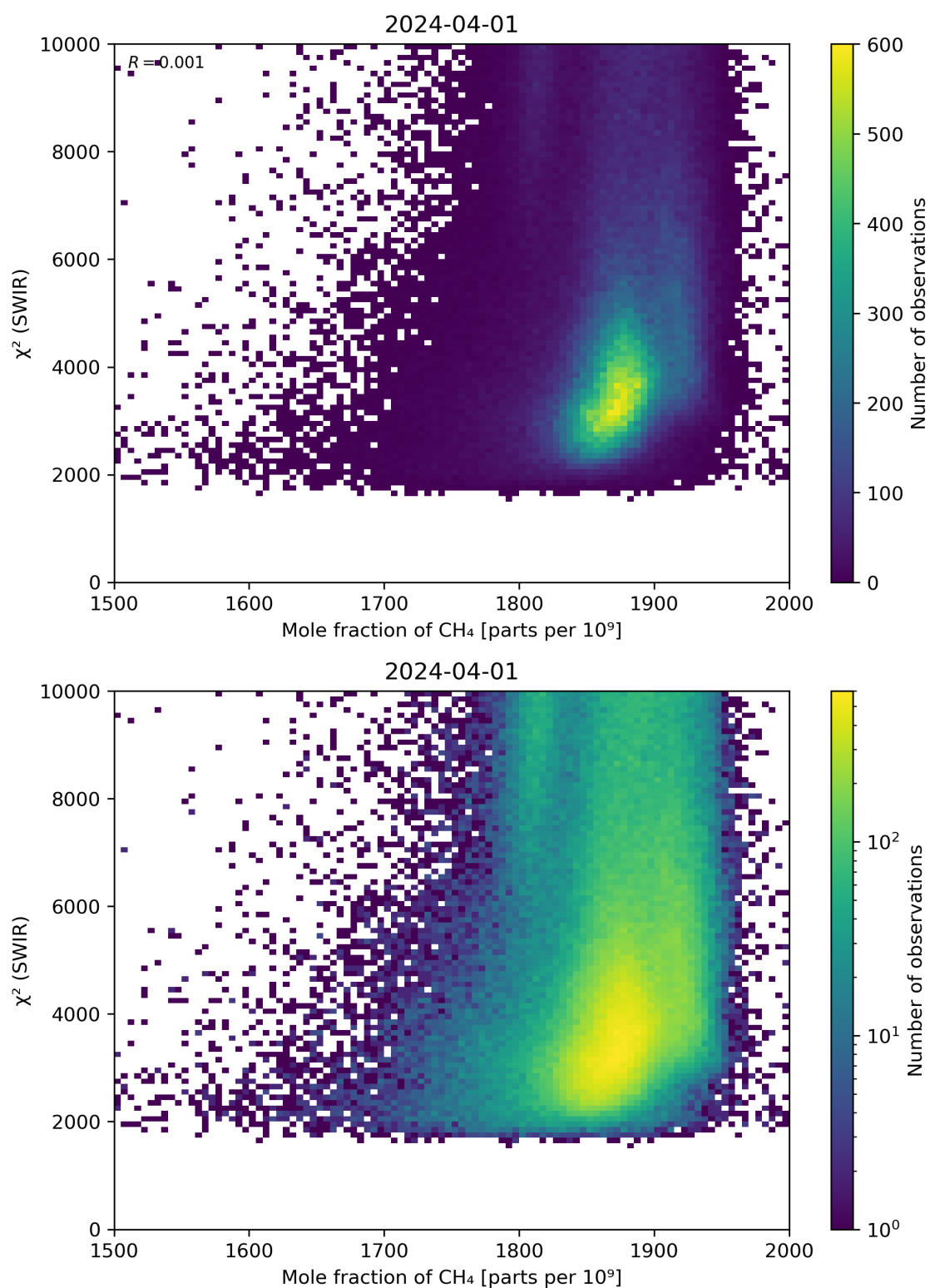
Figure 71: Scatter density plot of “Mole fraction of \text{CH}_4 ” against “ \chi^2 (SWIR)” for 2024-03-31 to 2024-04-02.
