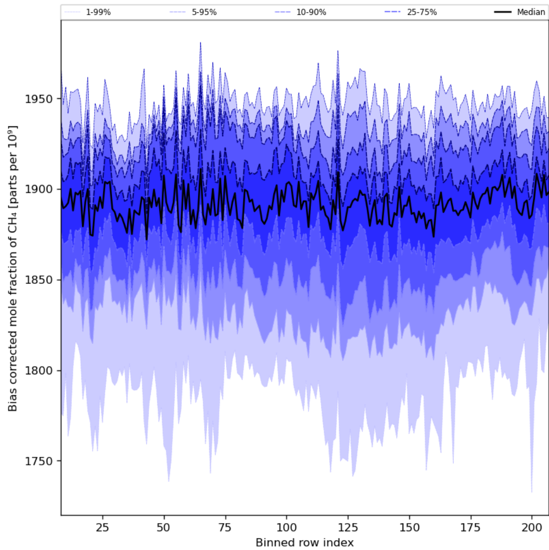
Figure 36: Along track statistics of “Bias corrected mole fraction of CH 4 ” for 2024-03-31 to 2024-04-02
