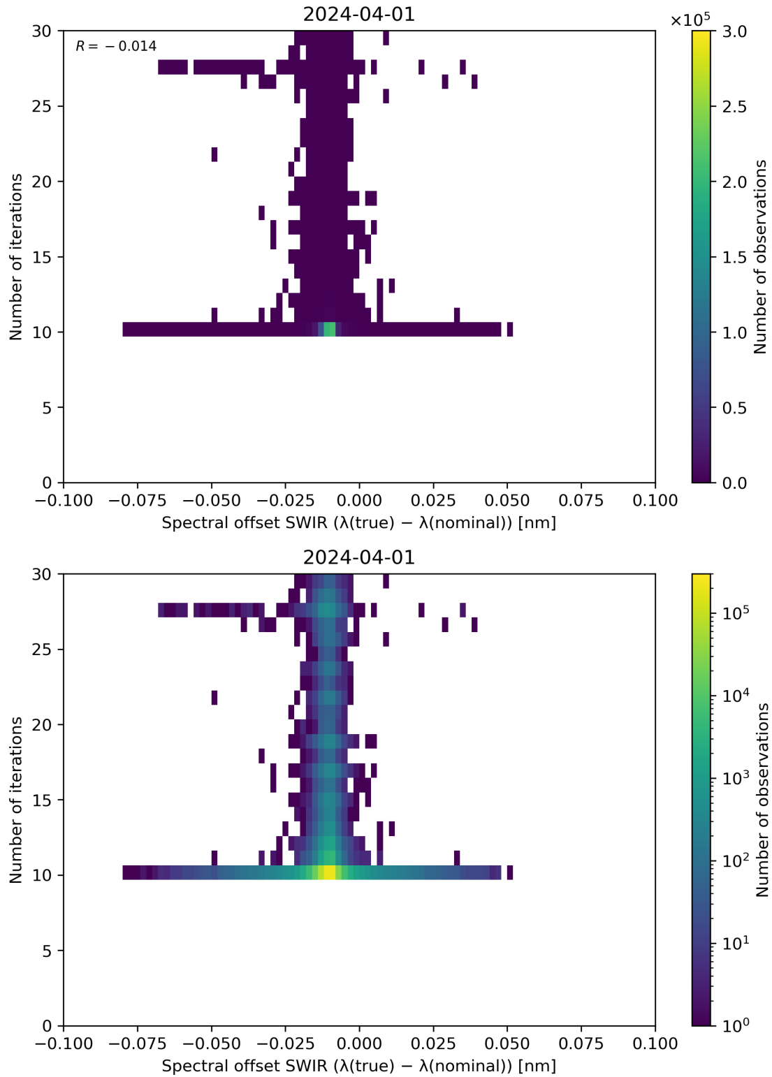
Figure 121: Scatter density plot of “Spectral offset SWIR ( \lambda(\text{true}) - \lambda(\text{nominal}) )” against “Number of iterations” for 2024-03-31 to 2024-04-02.
