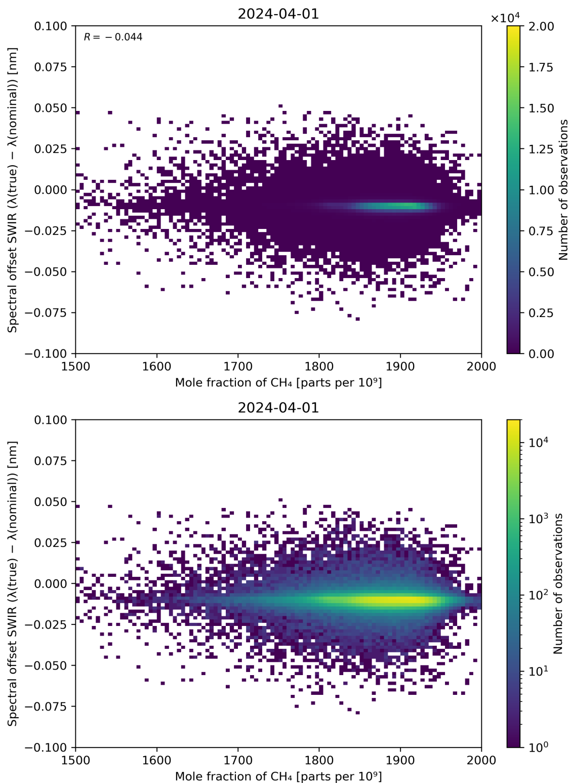
Figure 86: Scatter density plot of “Mole fraction of CH 4 ” against “Spectral offset SWIR ( \lambda(\text{true}) - \lambda(\text{nominal}) )” for 2024-03-31 to 2024-04-02.
