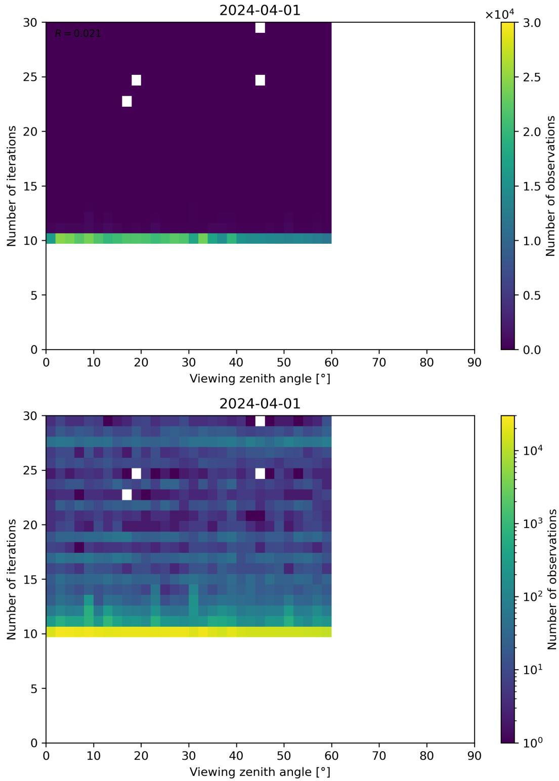
Figure 113: Scatter density plot of “Viewing zenith angle” against “Number of iterations” for 2024-03-31 to 2024-04-02.
