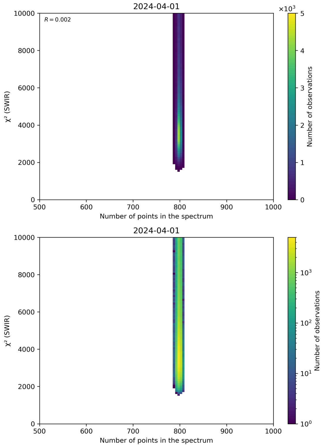
Figure 89: Scatter density plot of “Number of points in the spectrum” against “ \chi^2 (SWIR)” for 2024-03-31 to 2024-04-02.
