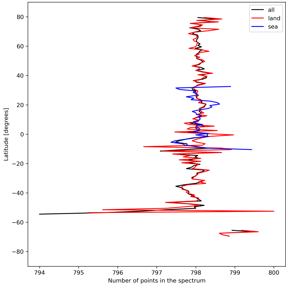
Figure 15: Zonal average of “Number of points in the spectrum” for 2024-03-31 to 2024-04-02.
