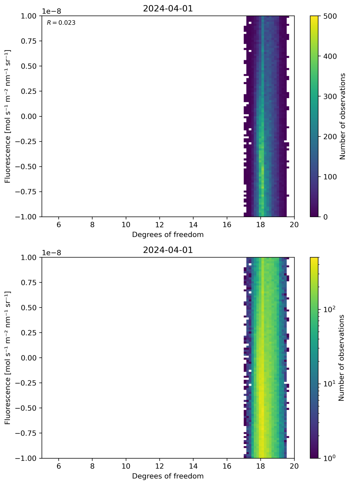
Figure 51: Scatter density plot of “Degrees of freedom” against “Fluorescence” for 2024-03-31 to 2024-04-02.
