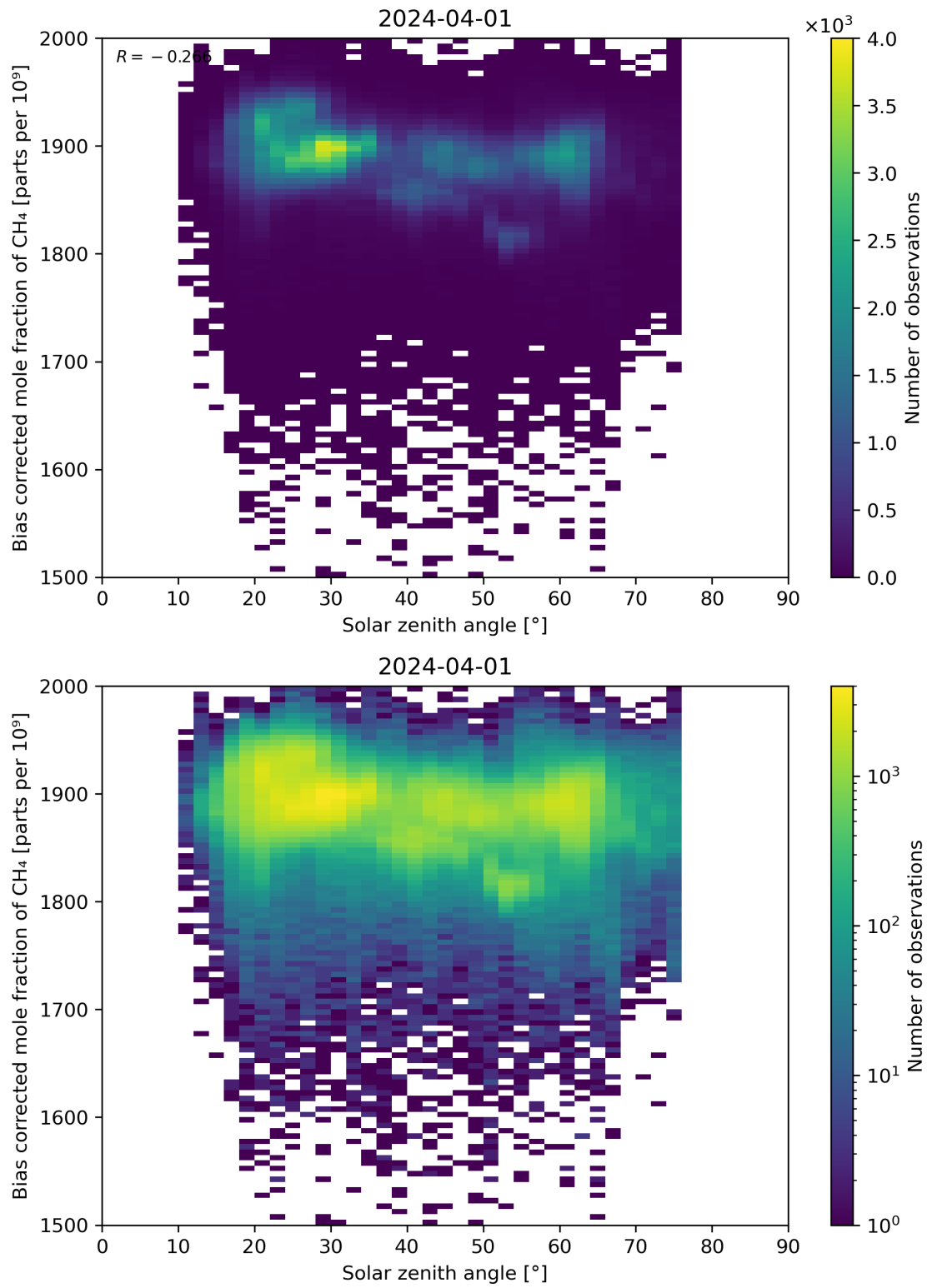
Figure 100: Scatter density plot of “Solar zenith angle” against “Bias corrected mole fraction of \text{CH}_4 ” for 2024-03-31 to 2024-04-02.
