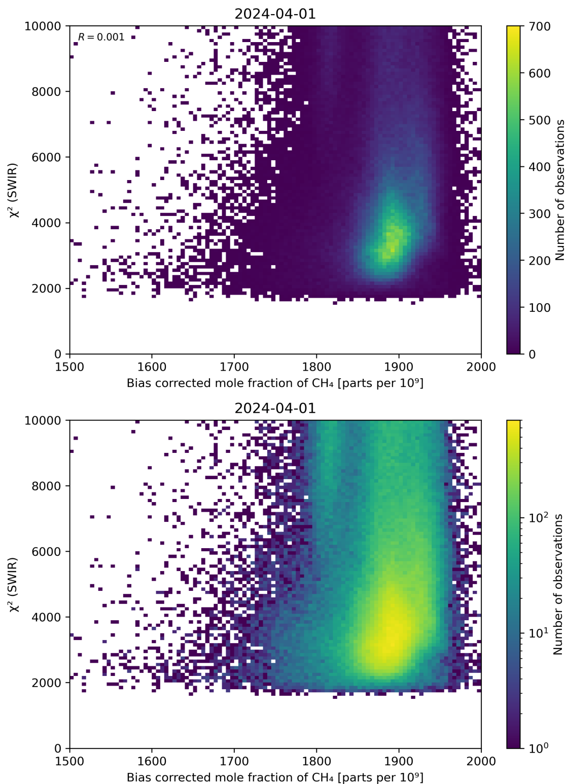
Figure 64: Scatter density plot of “Bias corrected mole fraction of CH 4 ” against “ \chi^2 (SWIR)” for 2024-03-31 to 2024-04-02.
