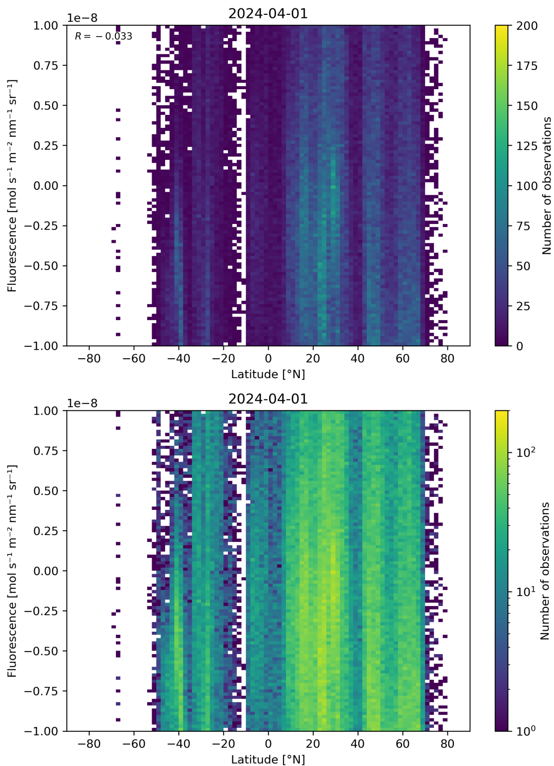
Figure 56: Scatter density plot of “Latitude” against “Fluorescence” for 2024-03-31 to 2024-04-02.
