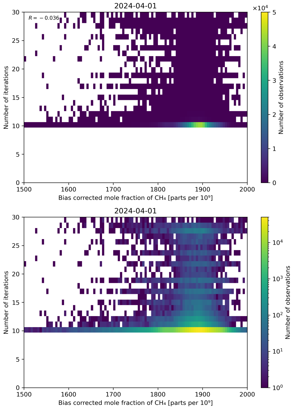
Figure 67: Scatter density plot of “Bias corrected mole fraction of CH 4 ” against “Number of iterations” for 2024-03-31 to 2024-04-02.
