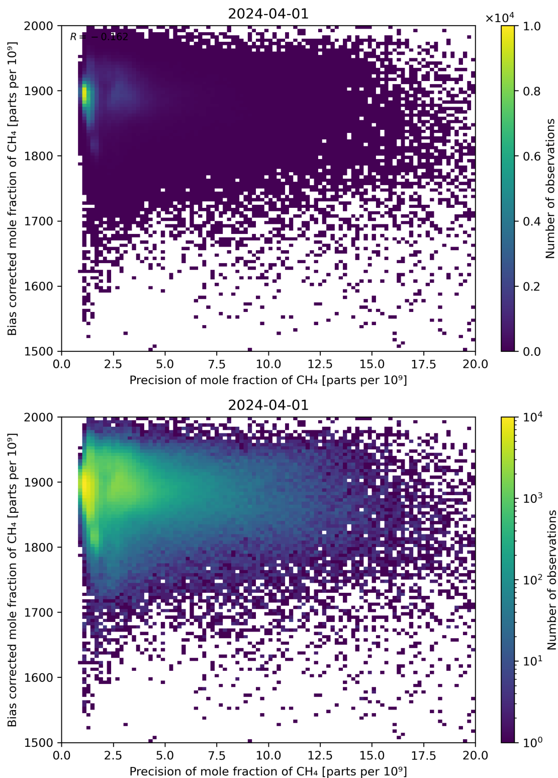
Figure 82: Scatter density plot of “Precision of mole fraction of CH 4 ” against “Bias corrected mole fraction of CH 4 ” for 2024-03-31 to 2024-04-02.
