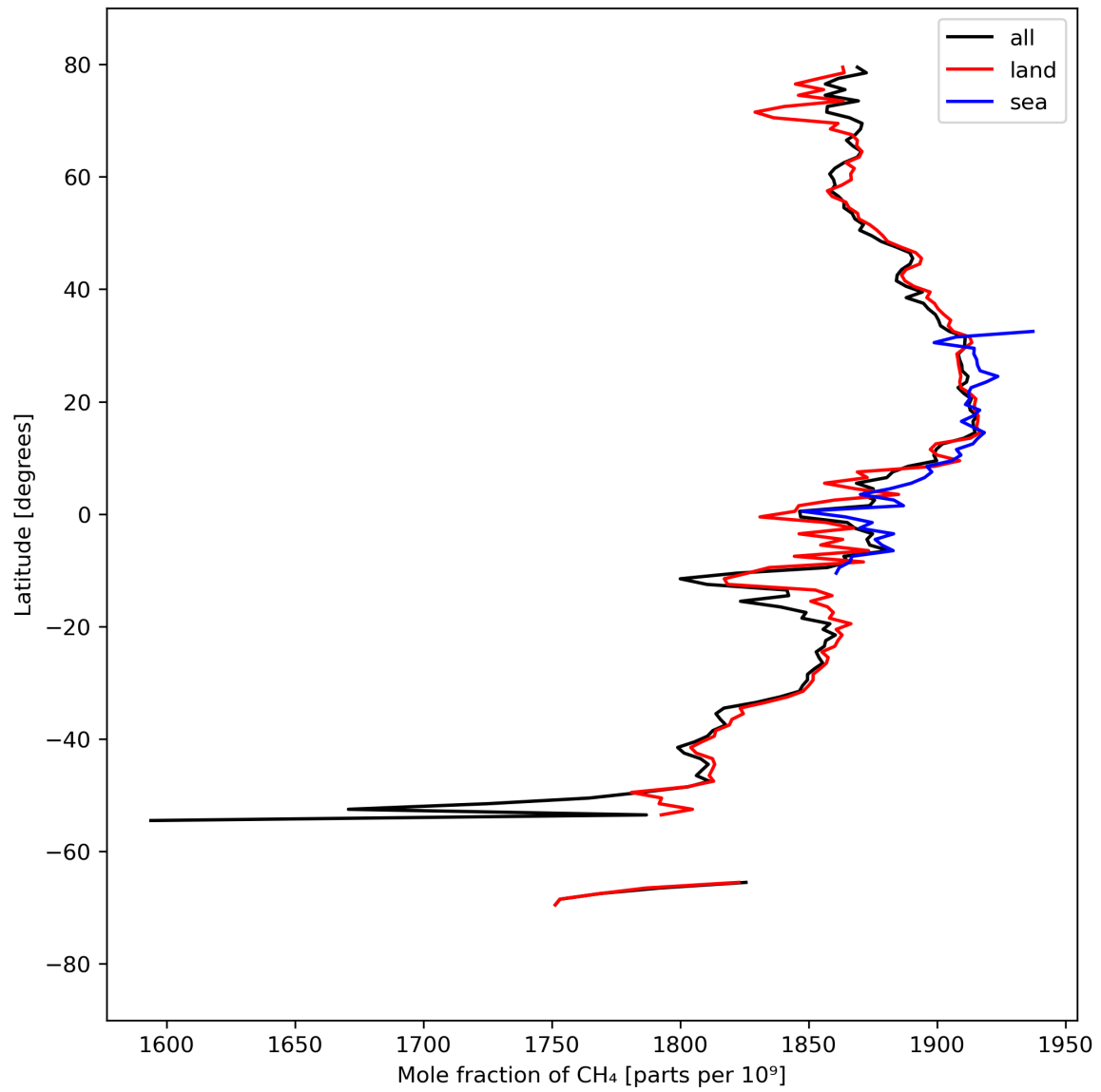
Figure 12: Zonal average of “Mole fraction of CH 4 ” for 2024-03-31 to 2024-04-02.
