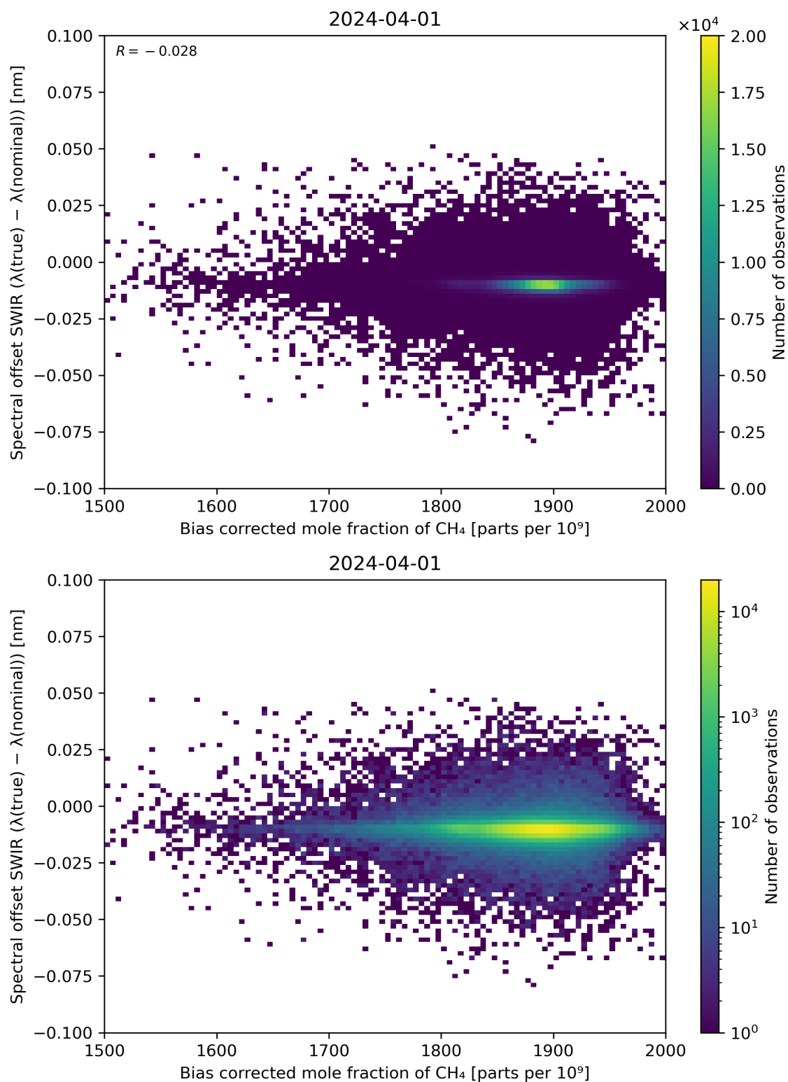
Figure 69: Scatter density plot of “Bias corrected mole fraction of \text{CH}_4 ” against “Spectral offset SWIR ( \lambda(\text{true}) - \lambda(\text{nominal}) )” for 2024-03-31 to 2024-04-02.
