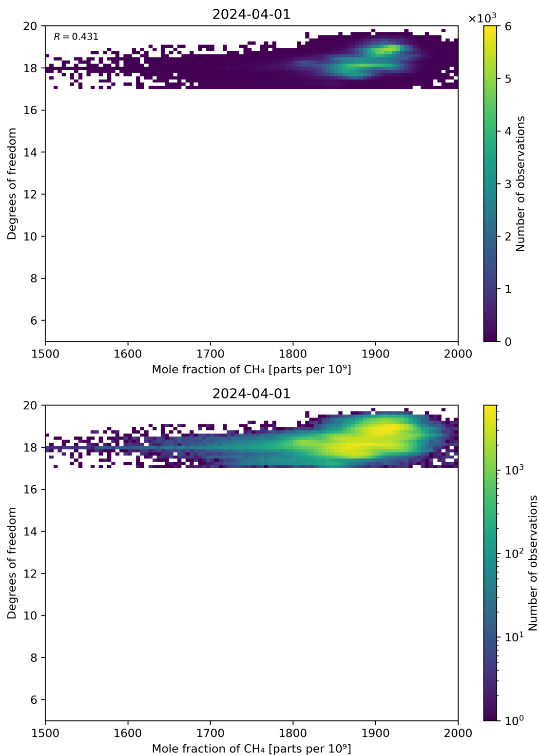
Figure 72: Scatter density plot of “Mole fraction of CH 4 ” against “Degrees of freedom” for 2024-03-31 to 2024-04-02.
