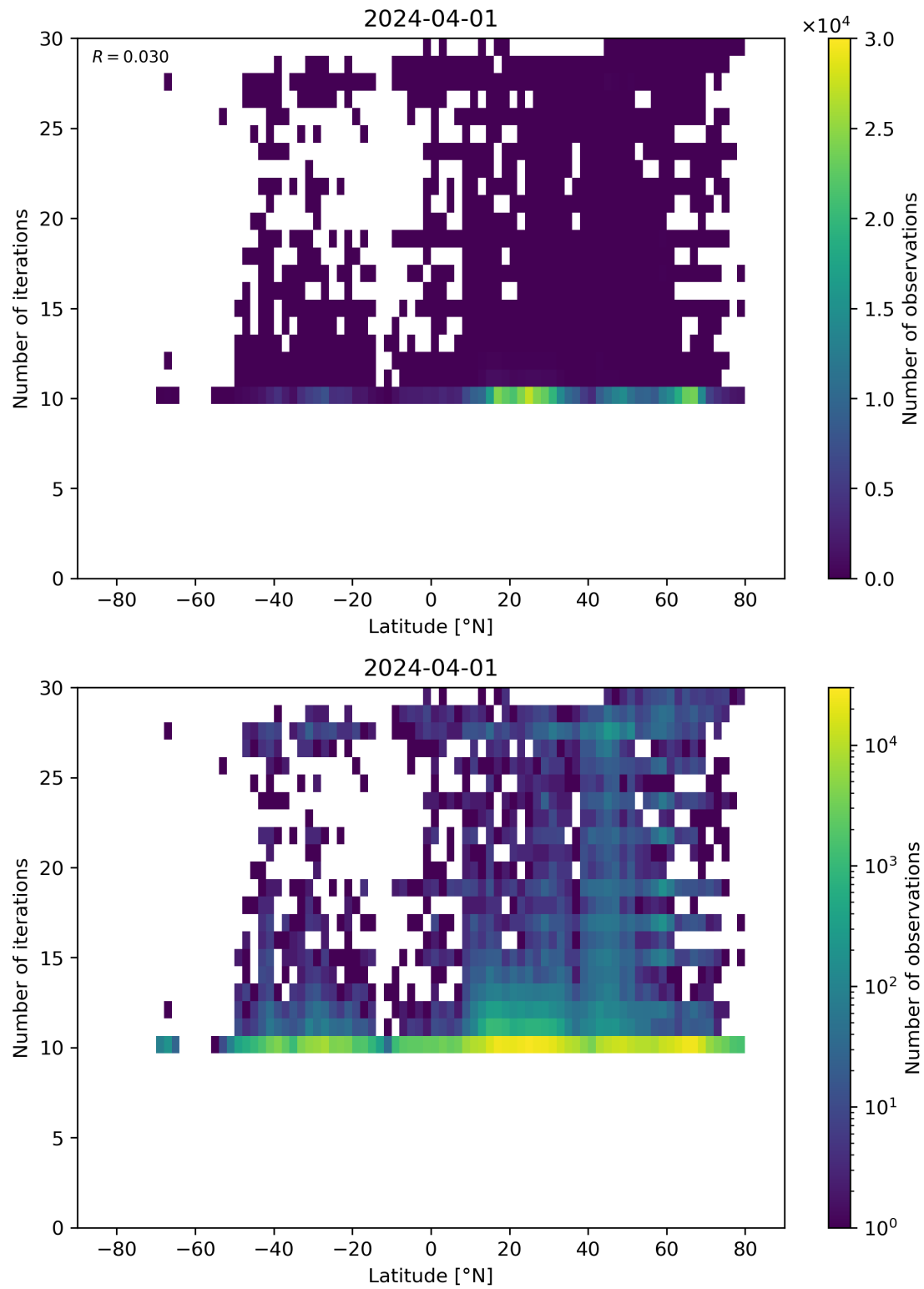
Figure 60: Scatter density plot of “Latitude” against “Number of iterations” for 2024-03-31 to 2024-04-02.
