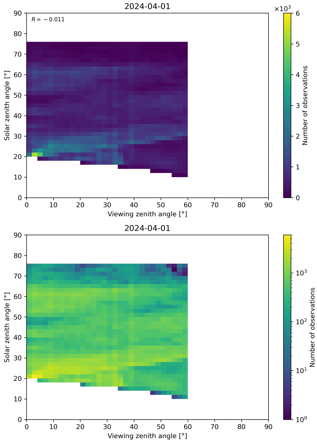
Figure 115: Scatter density plot of “Viewing zenith angle” against “Solar zenith angle” for 2024-03-31 to 2024-04-02.
