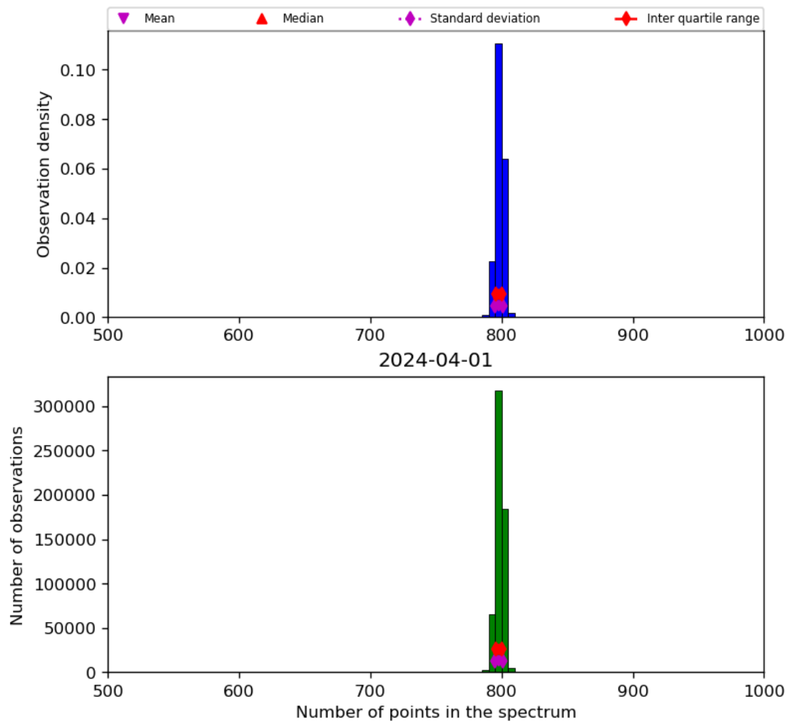
Figure 26: Histogram of “Number of points in the spectrum” for 2024-03-31 to 2024-04-02
