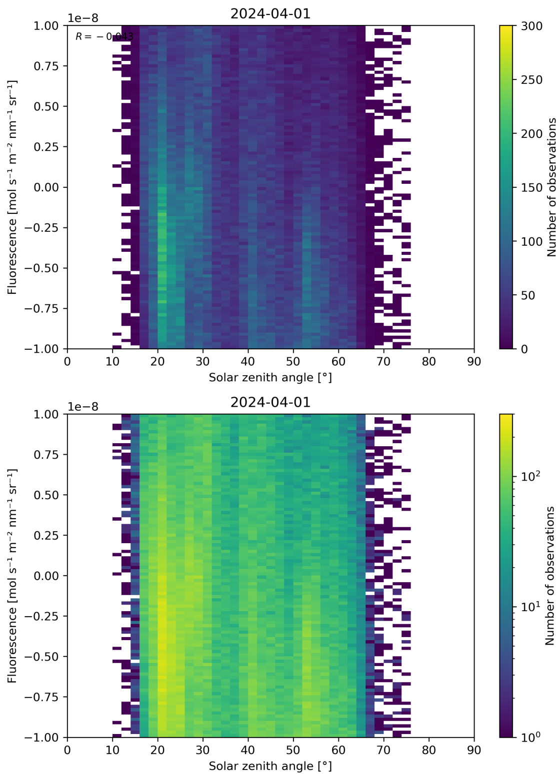
Figure 97: Scatter density plot of “Solar zenith angle” against “Fluorescence” for 2024-03-31 to 2024-04-02.
