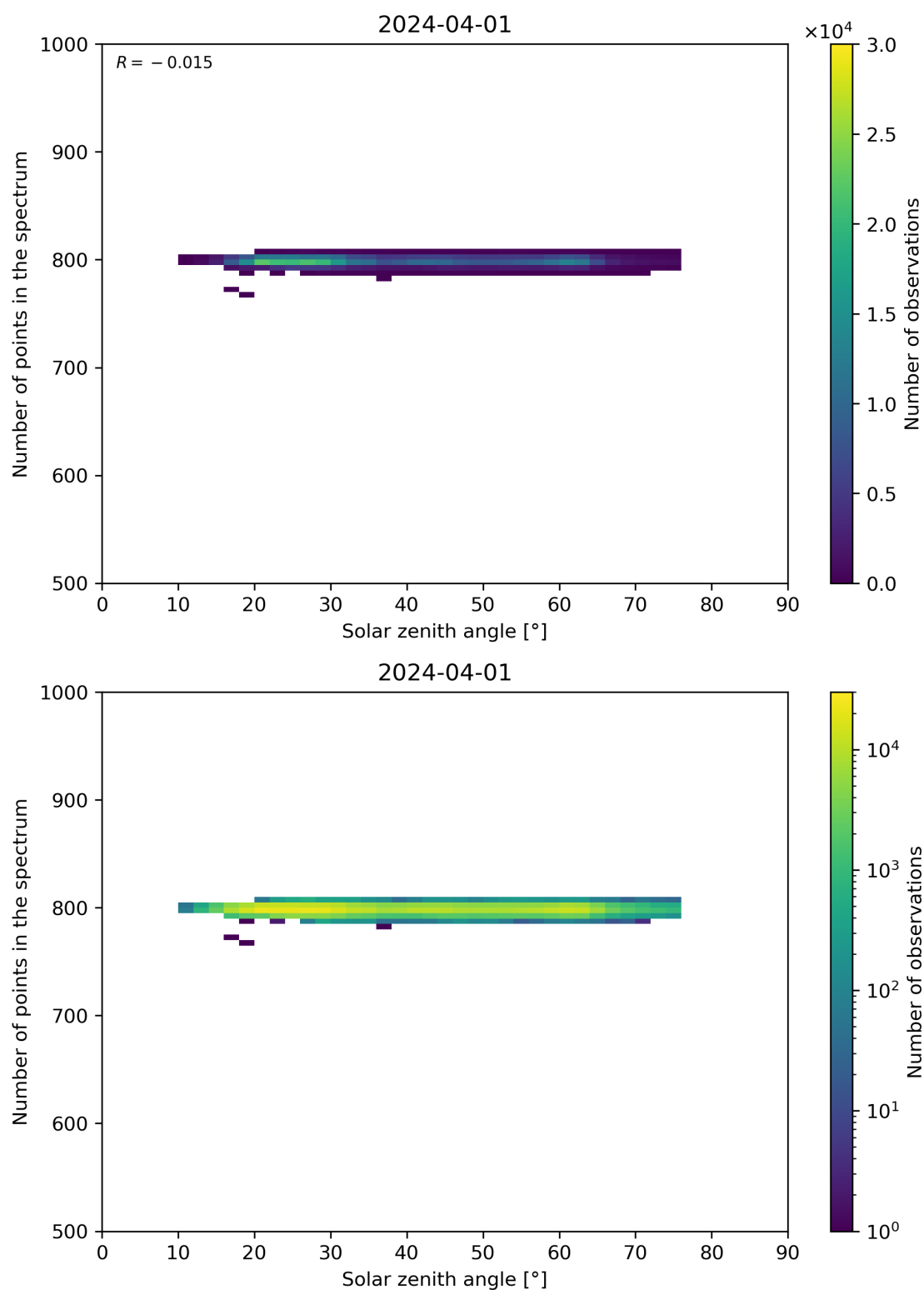
Figure 103: Scatter density plot of “Solar zenith angle” against “Number of points in the spectrum” for 2024-03-31 to 2024-04-02.
