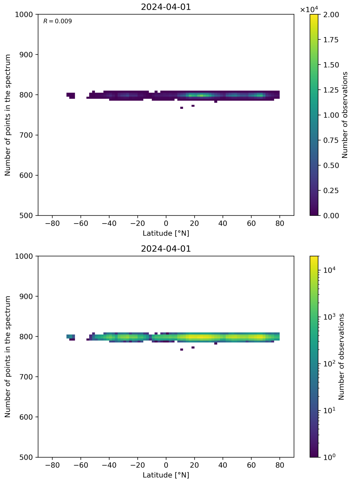
Figure 61: Scatter density plot of “Latitude” against “Number of points in the spectrum” for 2024-03-31 to 2024-04-02.
