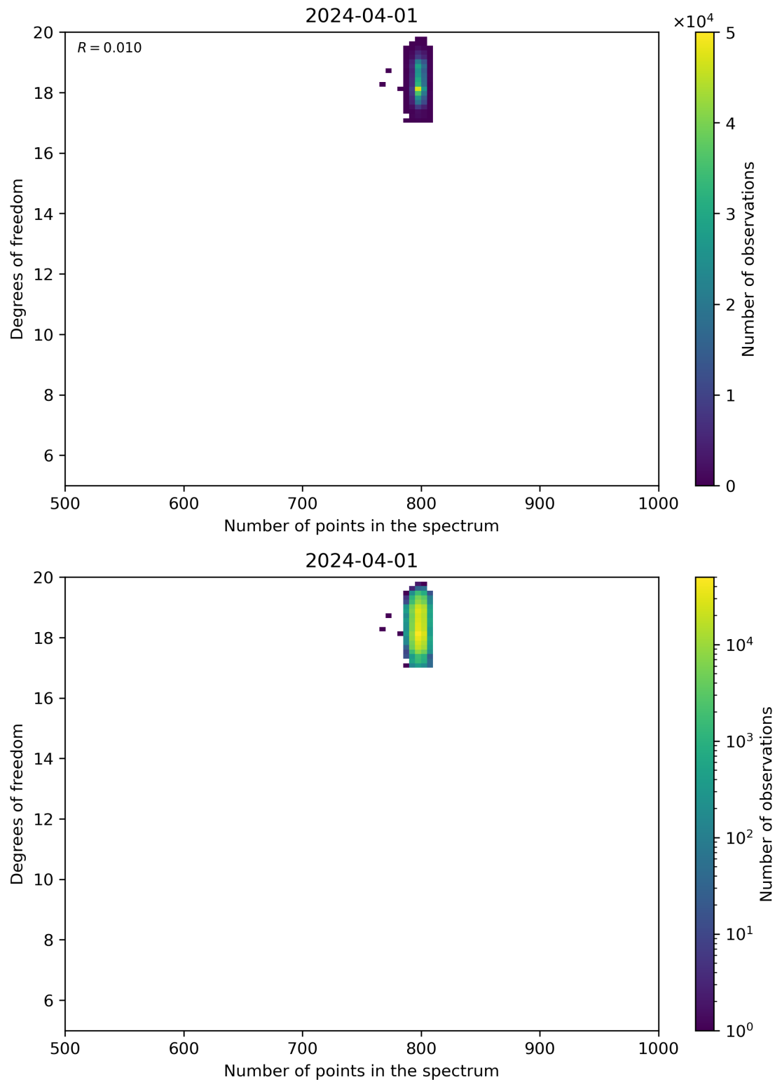
Figure 90: Scatter density plot of “Number of points in the spectrum” against “Degrees of freedom” for 2024-03-31 to 2024-04-02.
