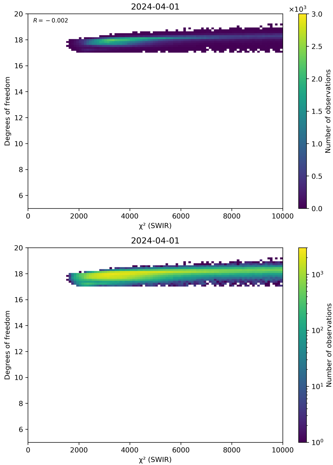
Figure 48: Scatter density plot of " \chi^2 (SWIR)" against "Degrees of freedom" for 2024-03-31 to 2024-04-02.
