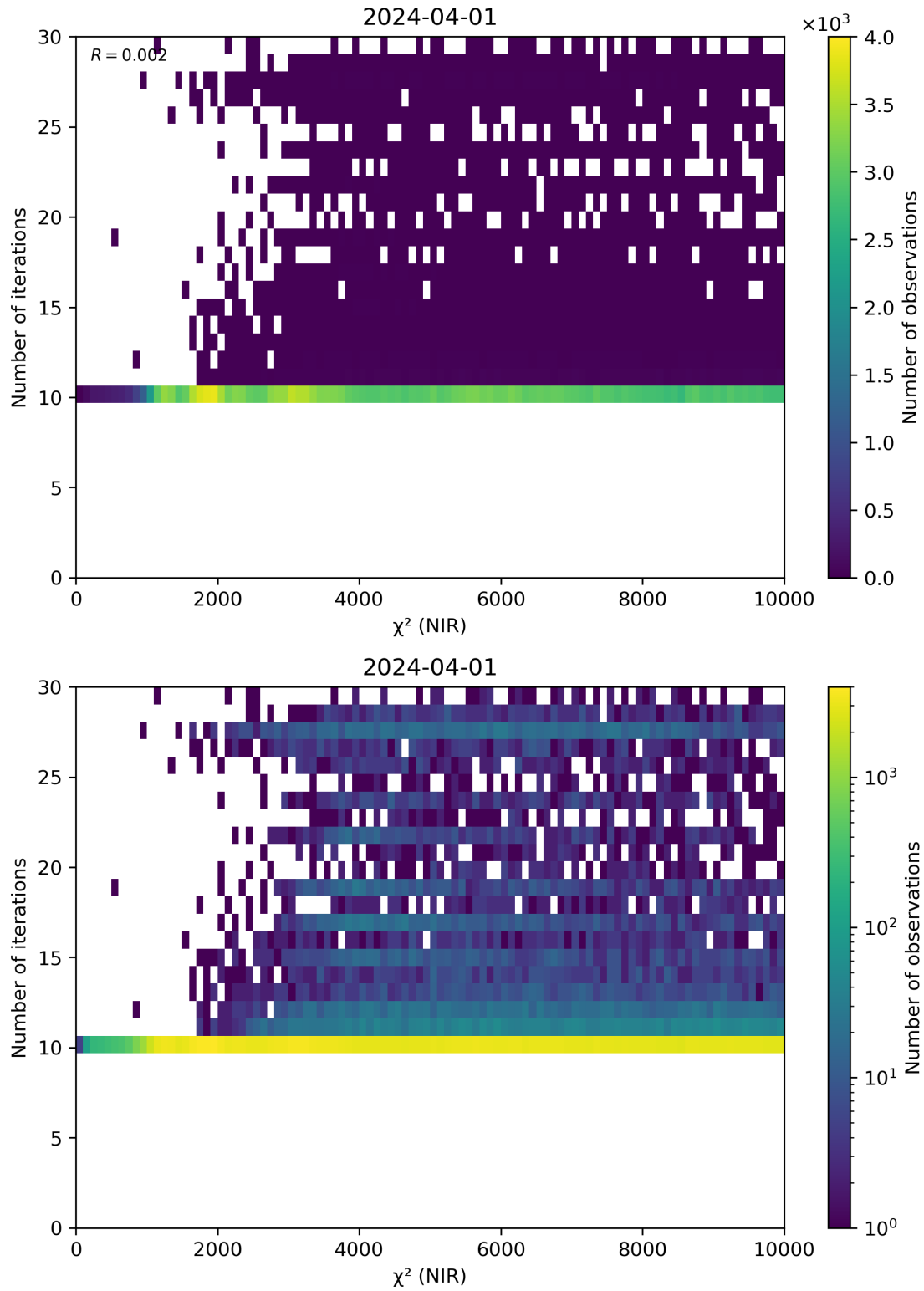
Figure 46: Scatter density plot of “ \chi^2 (NIR)” against “Number of iterations” for 2024-03-31 to 2024-04-02.
