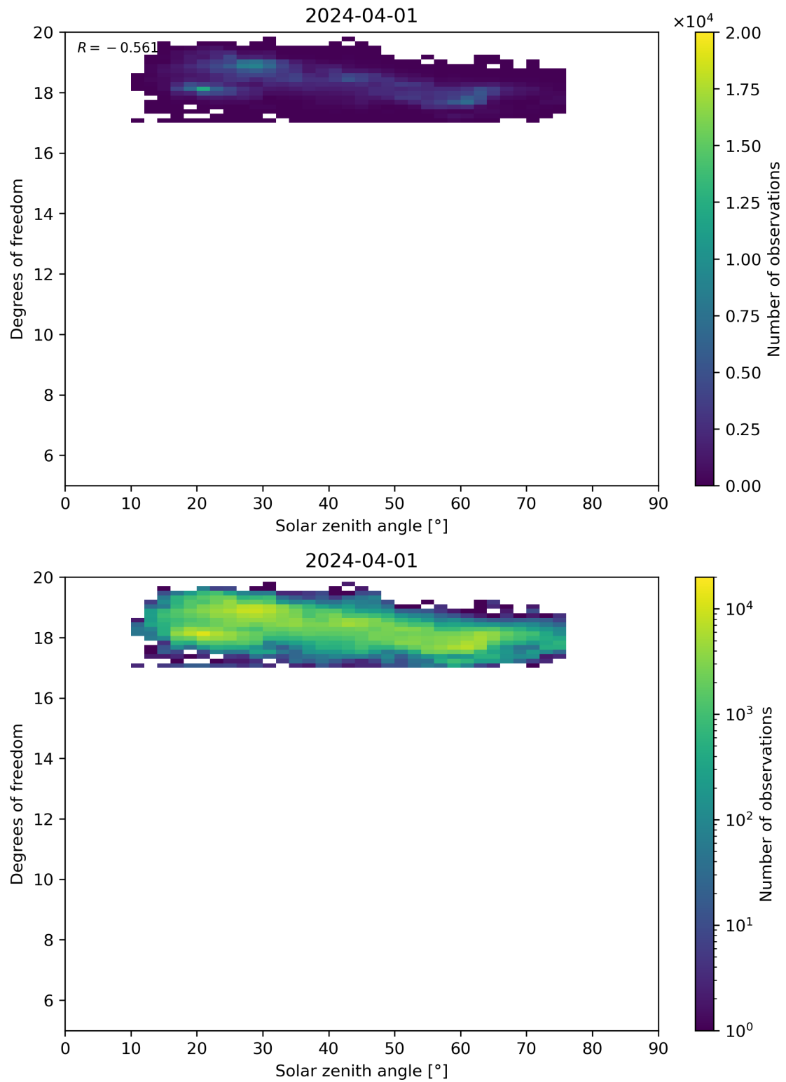
Figure 96: Scatter density plot of “Solar zenith angle” against “Degrees of freedom” for 2024-03-31 to 2024-04-02.
