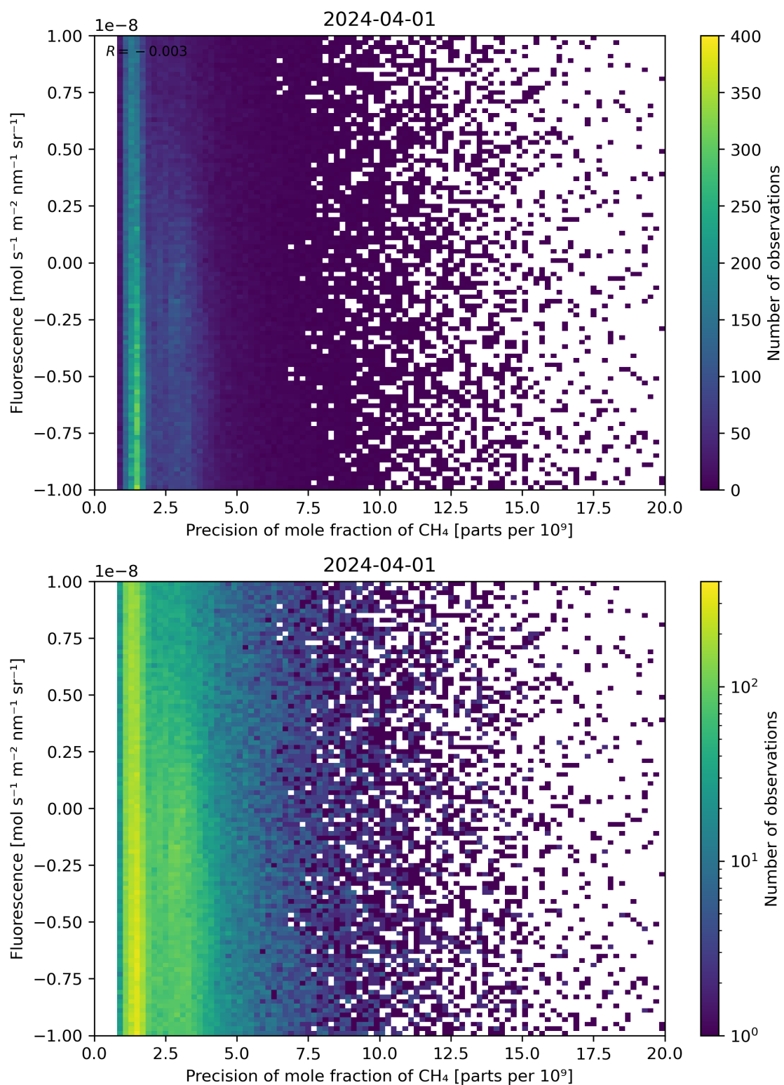
Figure 81: Scatter density plot of “Precision of mole fraction of \text{CH}_4 ” against “Fluorescence” for 2024-03-31 to 2024-04-02.
