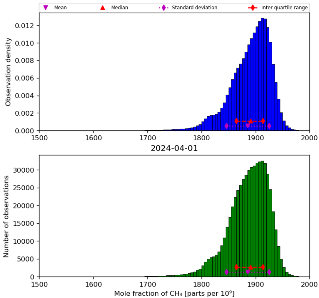
Figure 23: Histogram of “Mole fraction of CH 4 ” for 2024-03-31 to 2024-04-02
