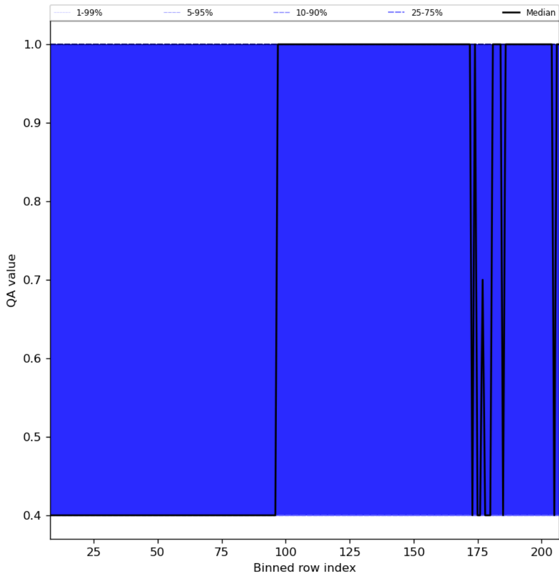
Figure 33: Along track statistics of “QA value” for 2024-03-31 to 2024-04-02
