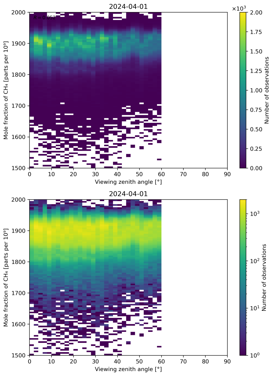
Figure 110: Scatter density plot of “Viewing zenith angle” against “Mole fraction of CH 4 ” for 2024-03-31 to 2024-04-02.
