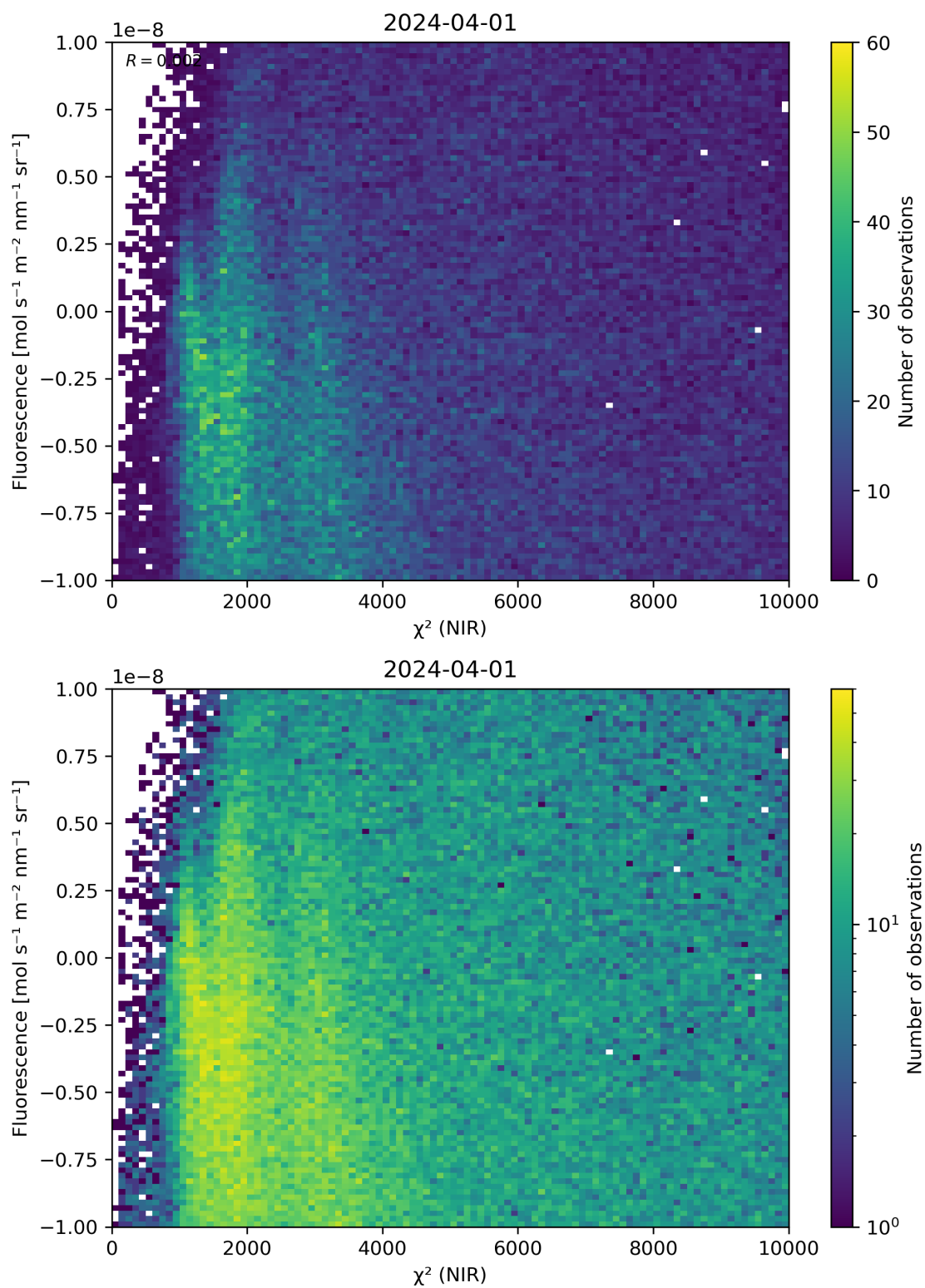
Figure 45: Scatter density plot of “ \chi^2 (NIR)” against “Fluorescence” for 2024-03-31 to 2024-04-02.
