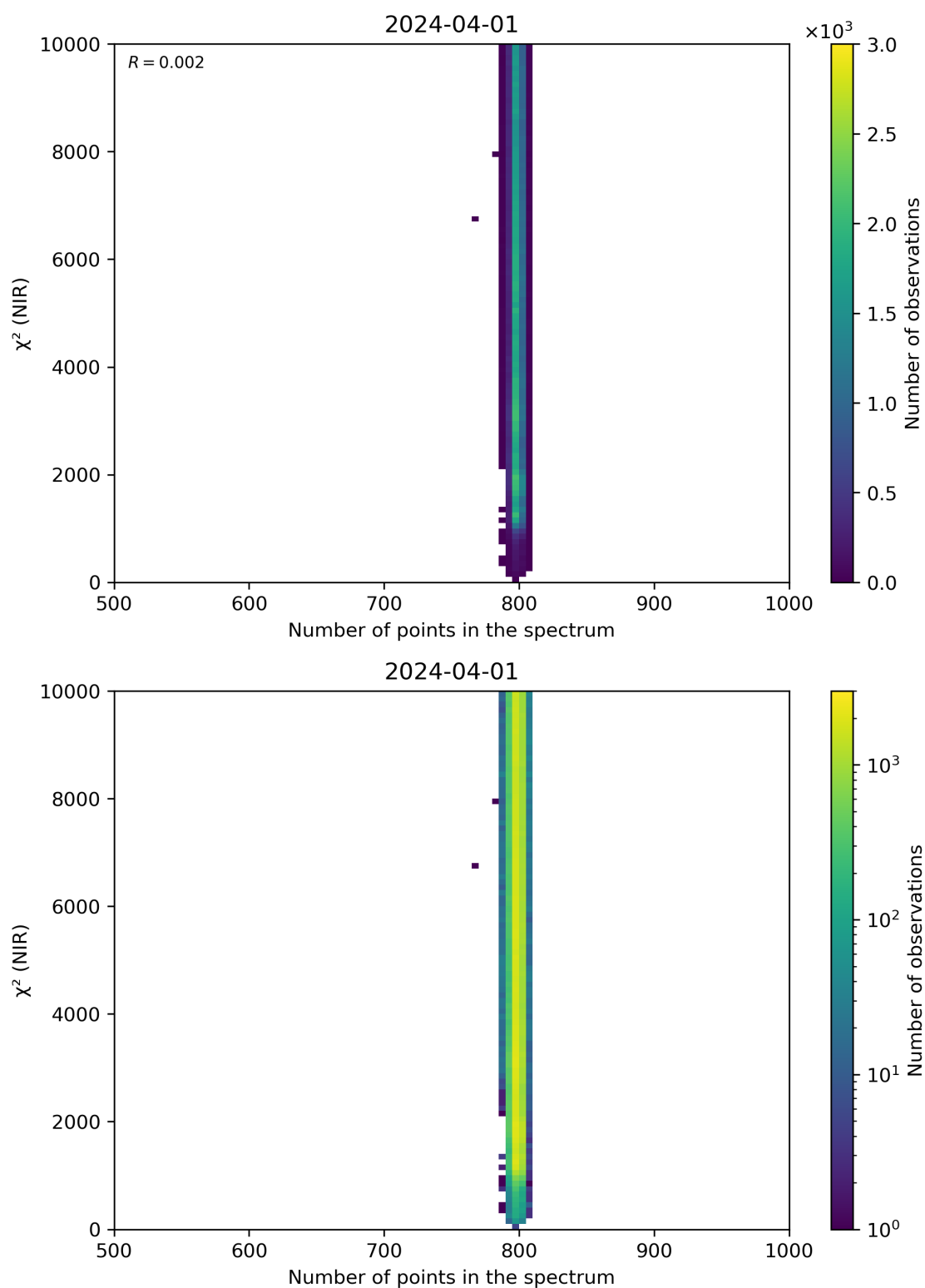
Figure 88: Scatter density plot of “Number of points in the spectrum” against “ \chi^2 (NIR)” for 2024-03-31 to 2024-04-02.
