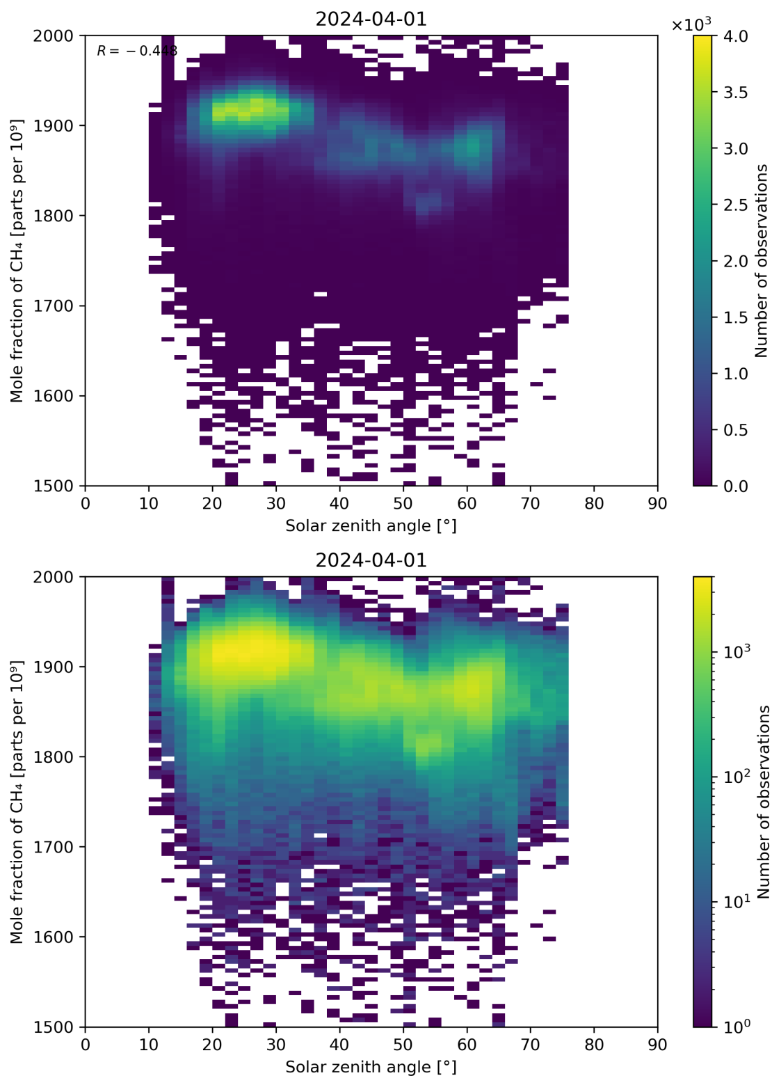
Figure 99: Scatter density plot of “Solar zenith angle” against “Mole fraction of CH 4 ” for 2024-03-31 to 2024-04-02.
