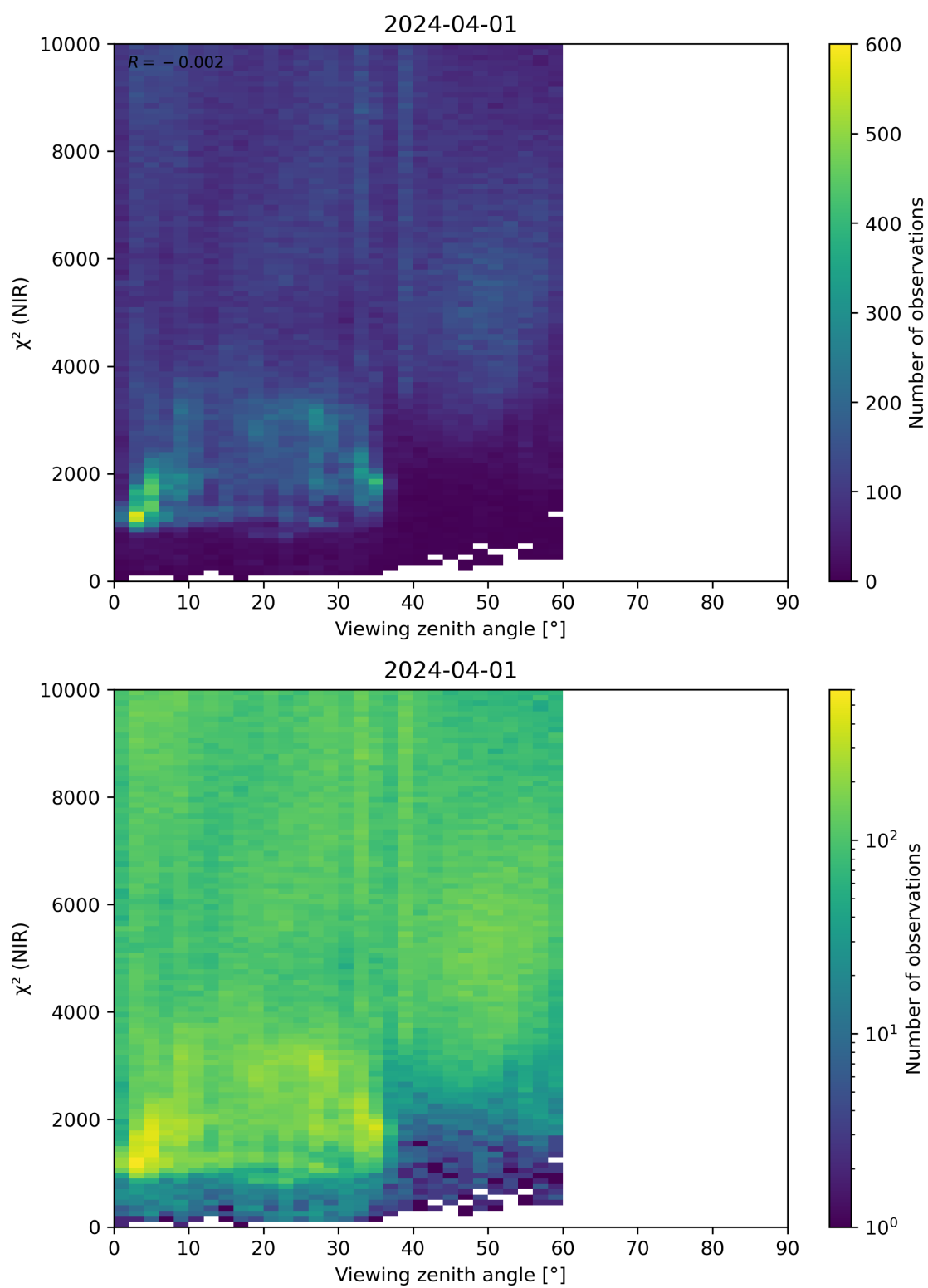
Figure 105: Scatter density plot of “Viewing zenith angle” against “ \chi^2 (NIR)” for 2024-03-31 to 2024-04-02.
