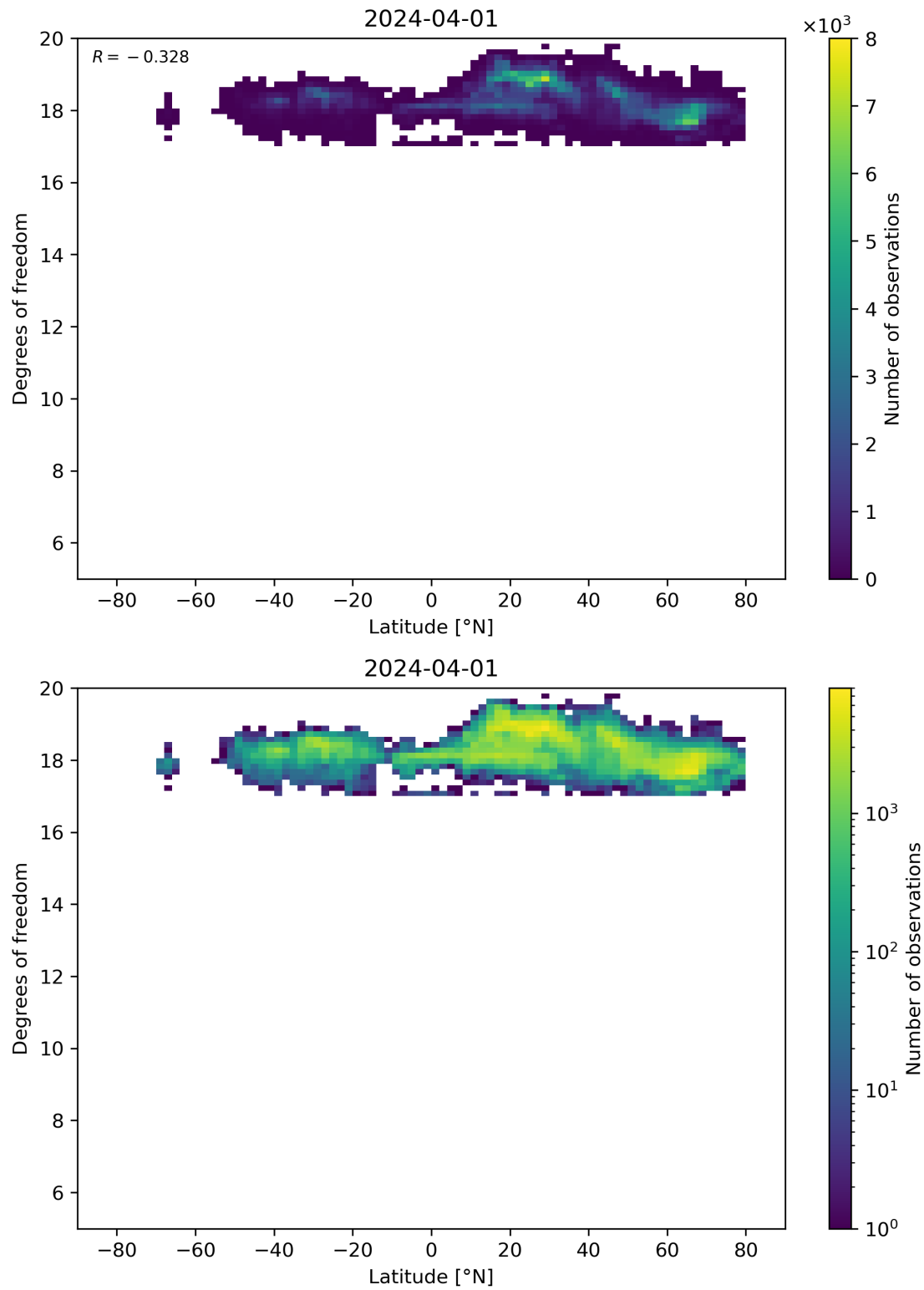
Figure 55: Scatter density plot of “Latitude” against “Degrees of freedom” for 2024-03-31 to 2024-04-02.
