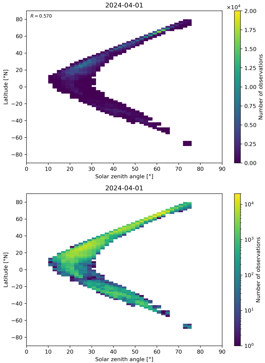
Figure 98: Scatter density plot of “Solar zenith angle” against “Latitude” for 2024-03-31 to 2024-04-02.
