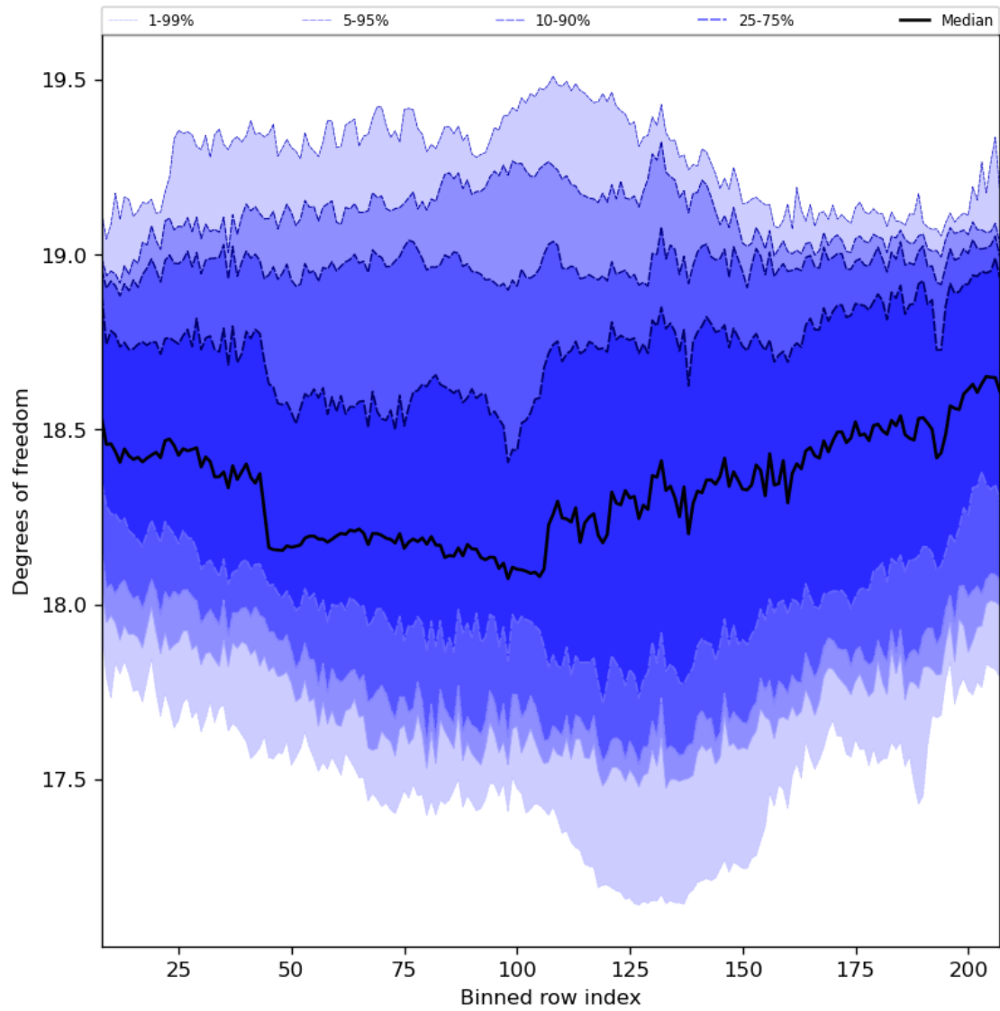
Figure 41: Along track statistics of “Degrees of freedom” for 2024-03-31 to 2024-04-02
