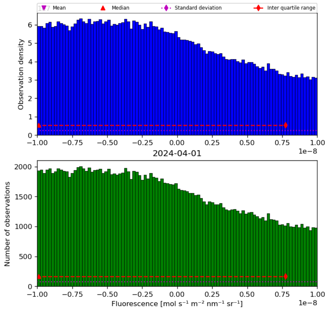
Figure 32: Histogram of “Fluorescence” for 2024-03-31 to 2024-04-02
