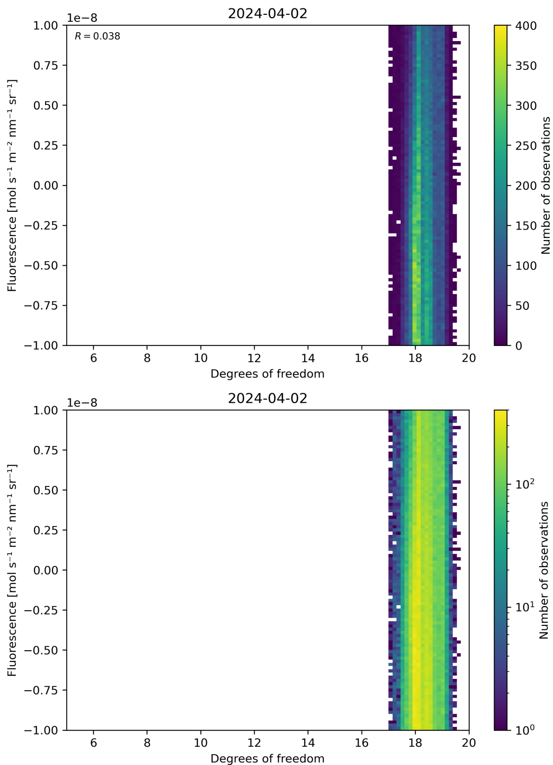
Figure 51: Scatter density plot of “Degrees of freedom” against “Fluorescence” for 2024-04-01 to 2024-04-03.
