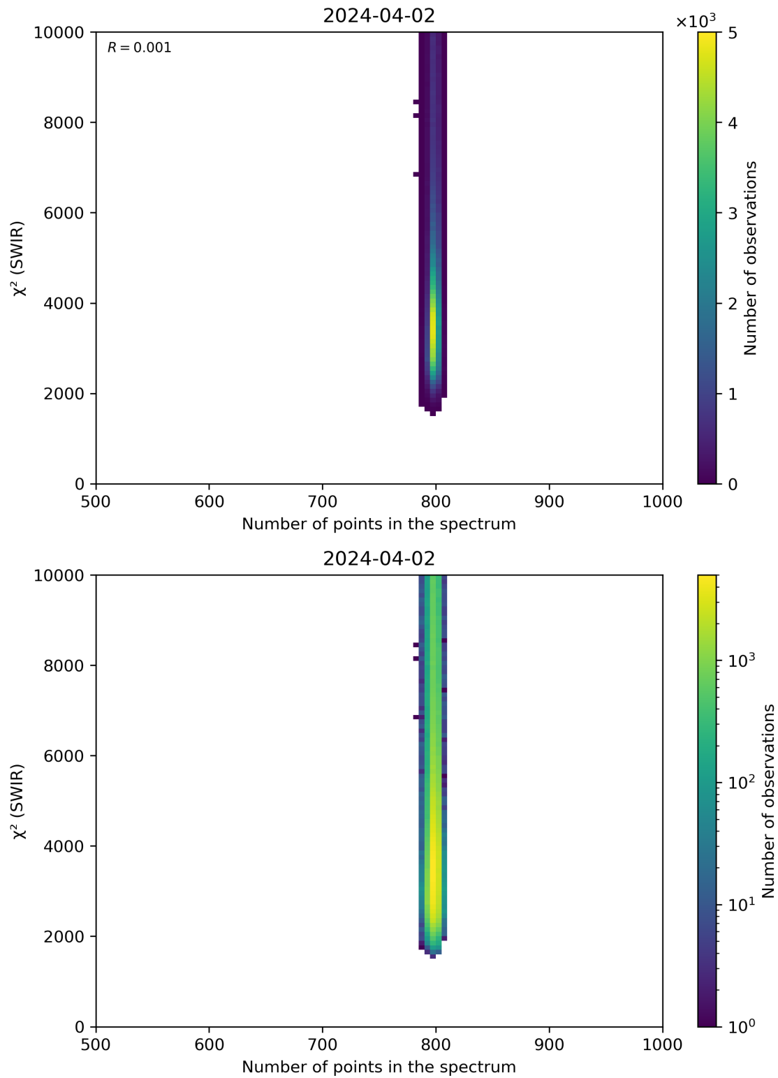
Figure 89: Scatter density plot of “Number of points in the spectrum” against “ \chi^2 (SWIR)” for 2024-04-01 to 2024-04-03.
