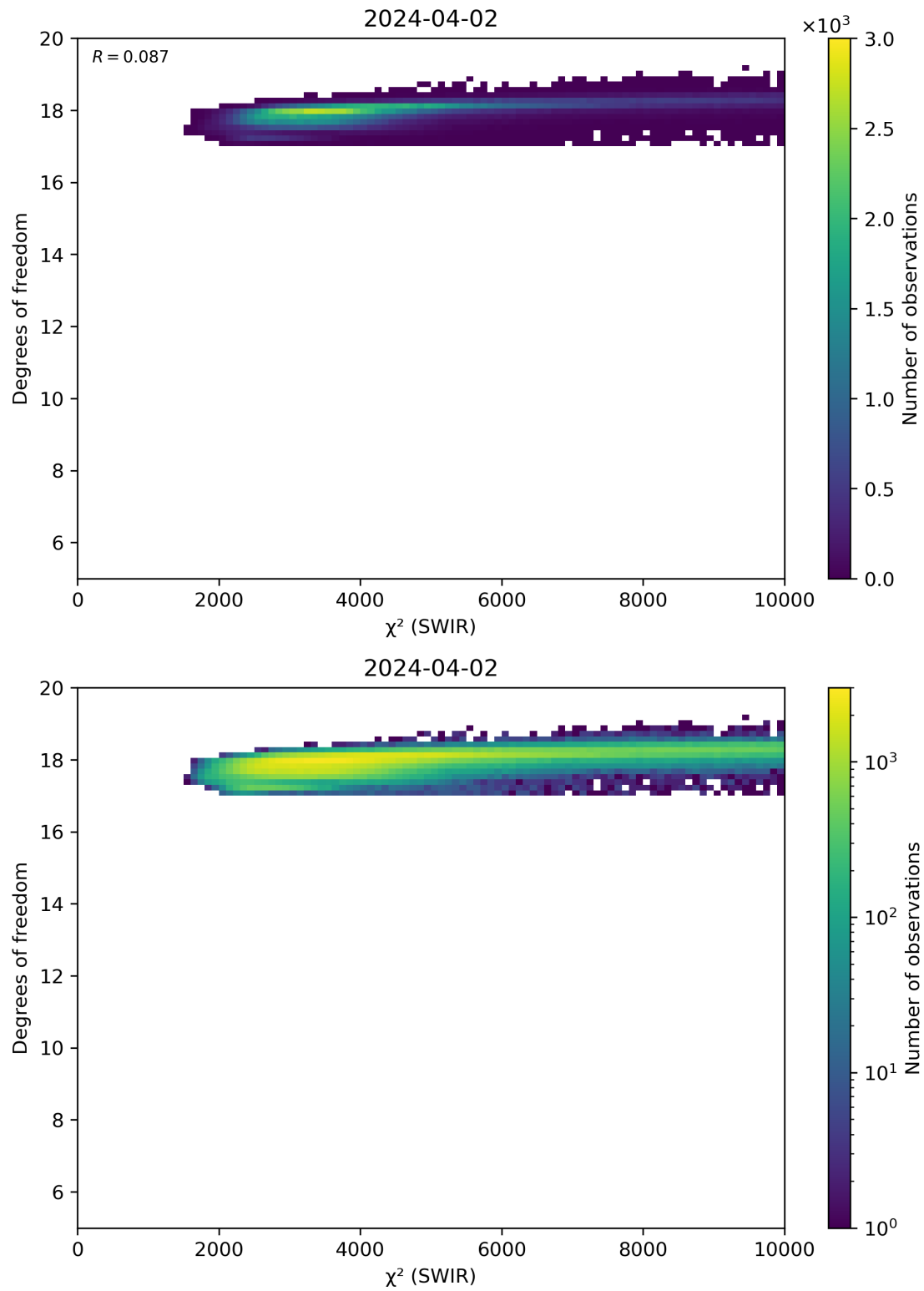
Figure 48: Scatter density plot of " \chi^2 (SWIR)" against "Degrees of freedom" for 2024-04-01 to 2024-04-03.
