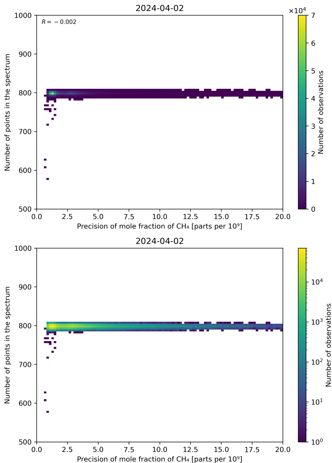
Figure 84: Scatter density plot of “Precision of mole fraction of CH 4 ” against “Number of points in the spectrum” for 2024-04-01 to 2024-04-03.
