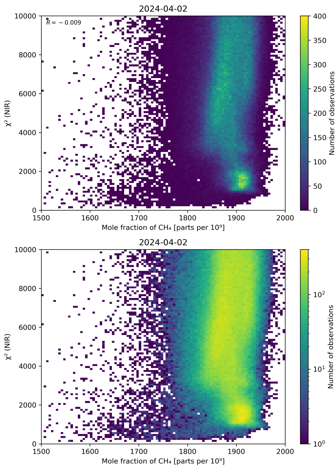
Figure 70: Scatter density plot of “Mole fraction of \text{CH}_4 ” against “ \chi^2 (NIR)” for 2024-04-01 to 2024-04-03.
