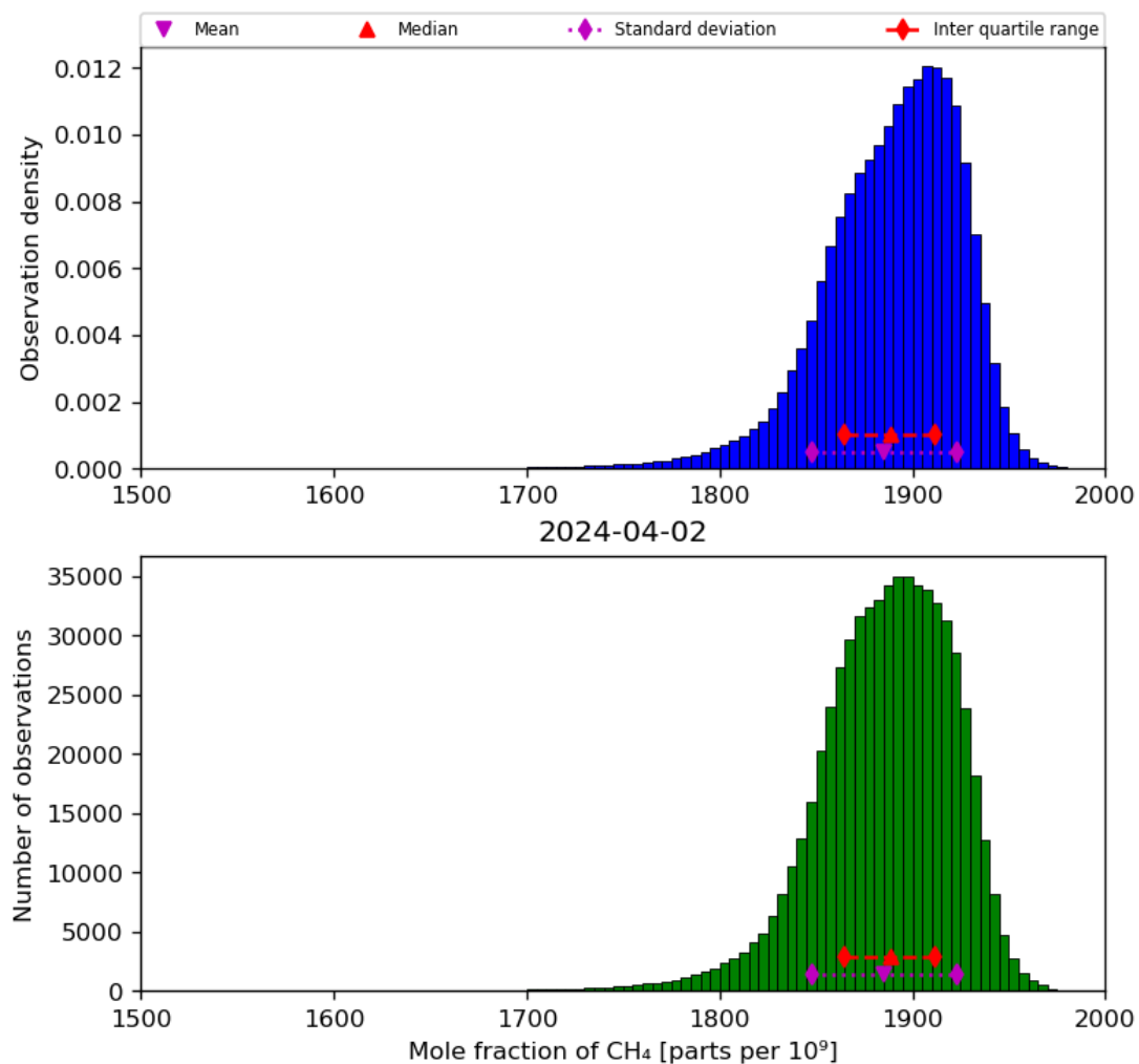
Figure 23: Histogram of “Mole fraction of CH 4 ” for 2024-04-01 to 2024-04-03
