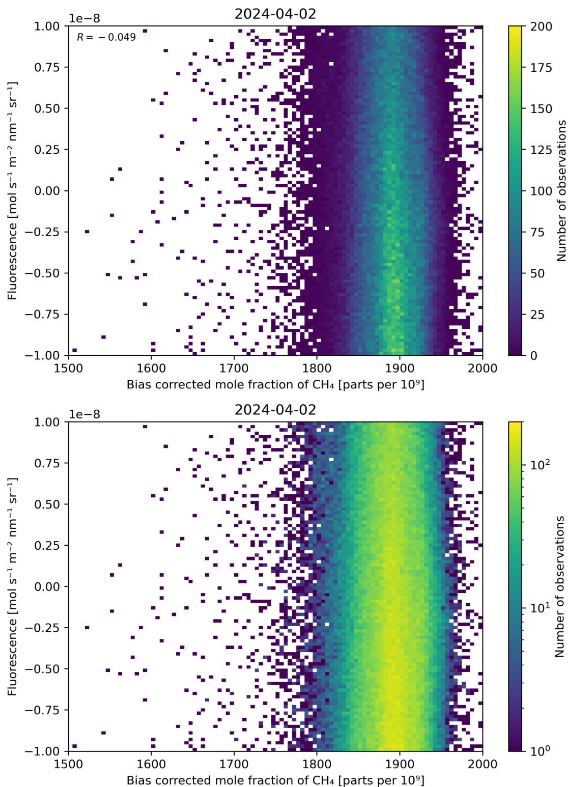
Figure 66: Scatter density plot of “Bias corrected mole fraction of \text{CH}_4 ” against “Fluorescence” for 2024-04-01 to 2024-04-03.
