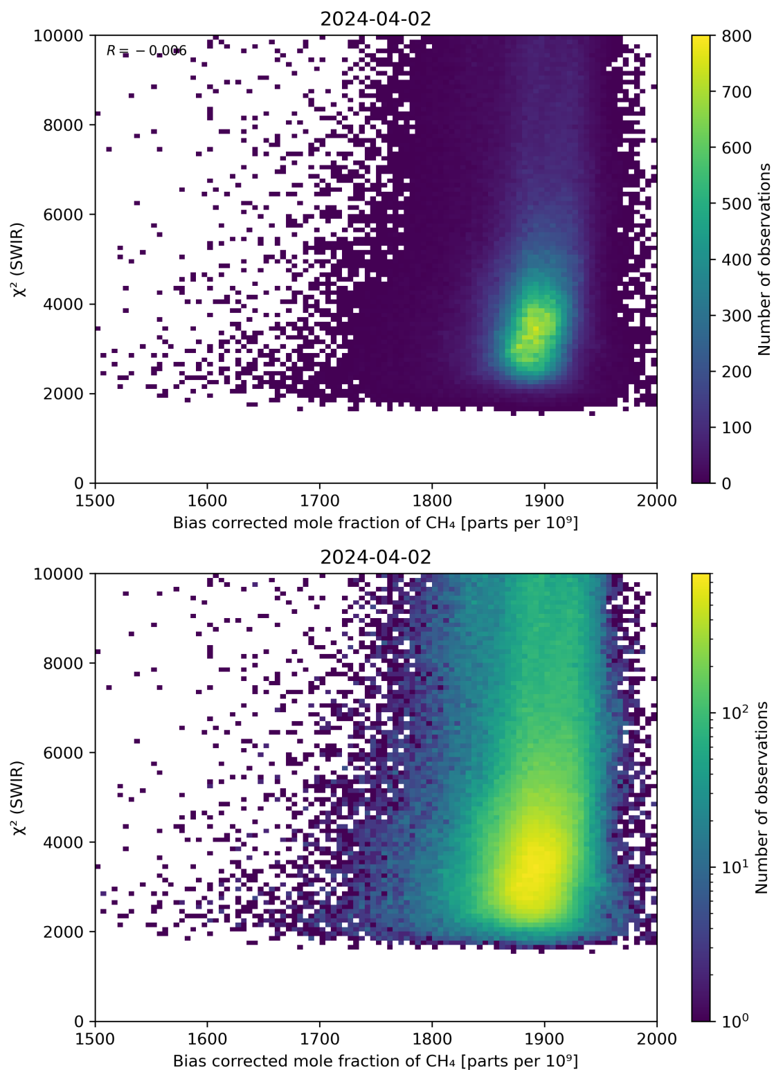
Figure 64: Scatter density plot of “Bias corrected mole fraction of CH 4 ” against “ \chi^2 (SWIR)” for 2024-04-01 to 2024-04-03.
