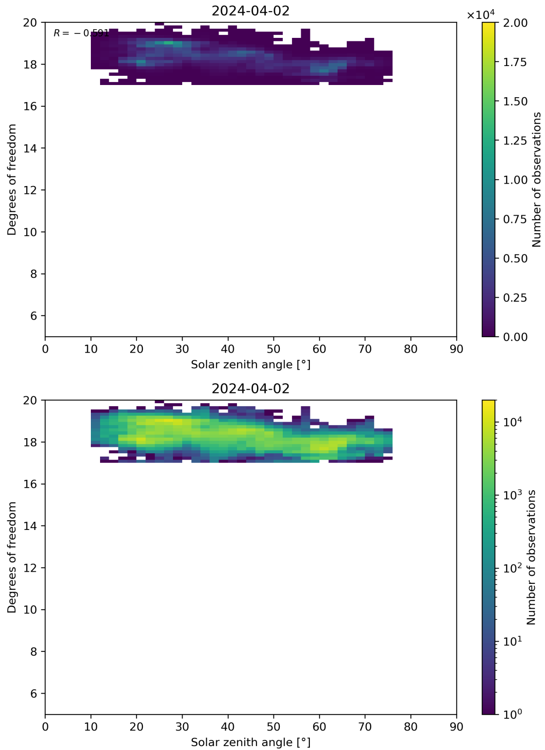
Figure 96: Scatter density plot of “Solar zenith angle” against “Degrees of freedom” for 2024-04-01 to 2024-04-03.
