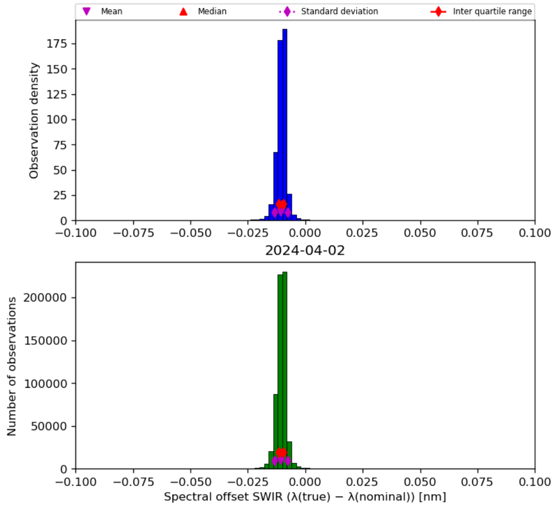
Figure 27: Histogram of “Spectral offset SWIR ( \lambda(\text{true}) - \lambda(\text{nominal}) )” for 2024-04-01 to 2024-04-03
