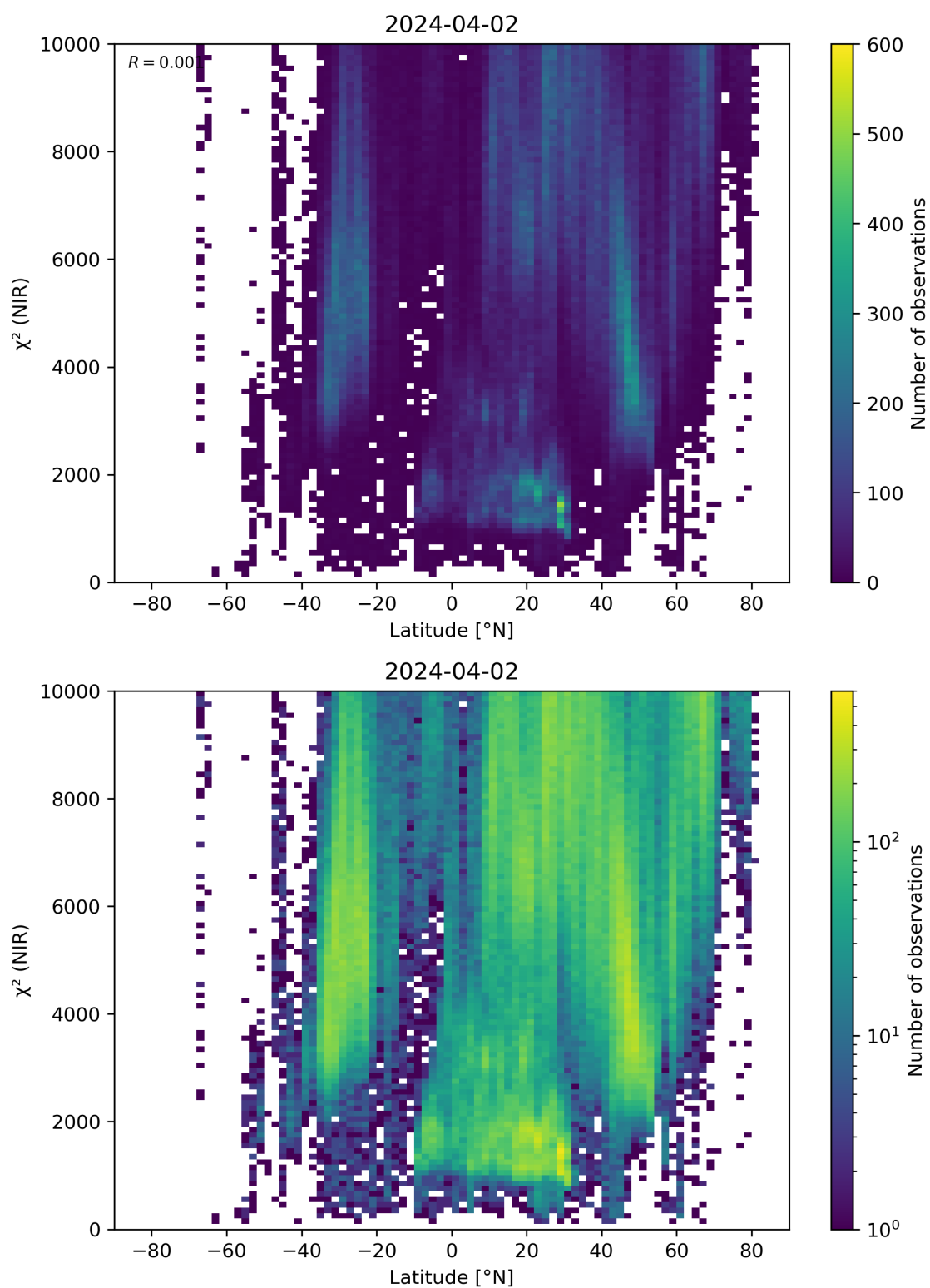
Figure 53: Scatter density plot of “Latitude” against “ \chi^2 (NIR)” for 2024-04-01 to 2024-04-03.
