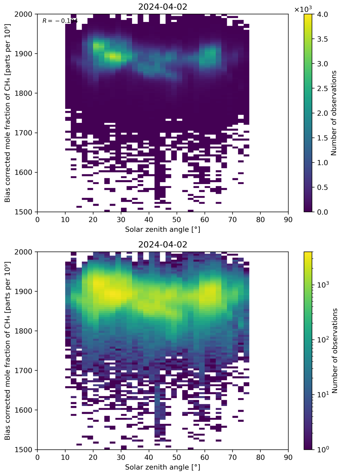
Figure 100: Scatter density plot of “Solar zenith angle” against “Bias corrected mole fraction of \text{CH}_4 ” for 2024-04-01 to 2024-04-03.
