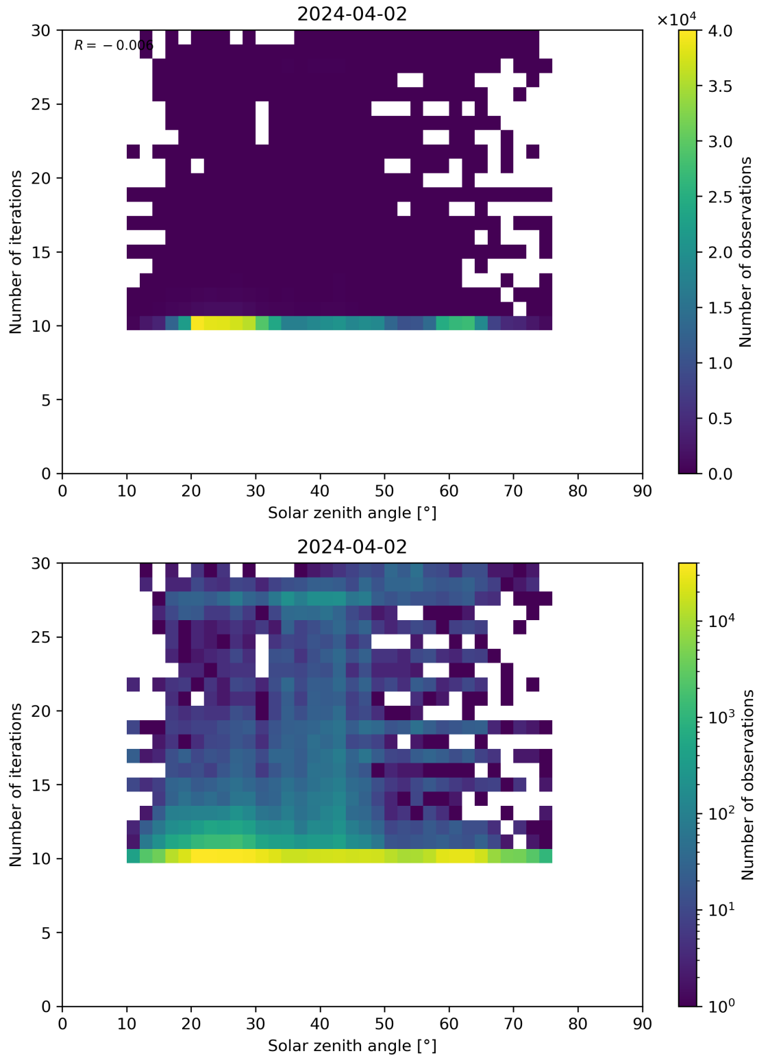
Figure 102: Scatter density plot of “Solar zenith angle” against “Number of iterations” for 2024-04-01 to 2024-04-03.
