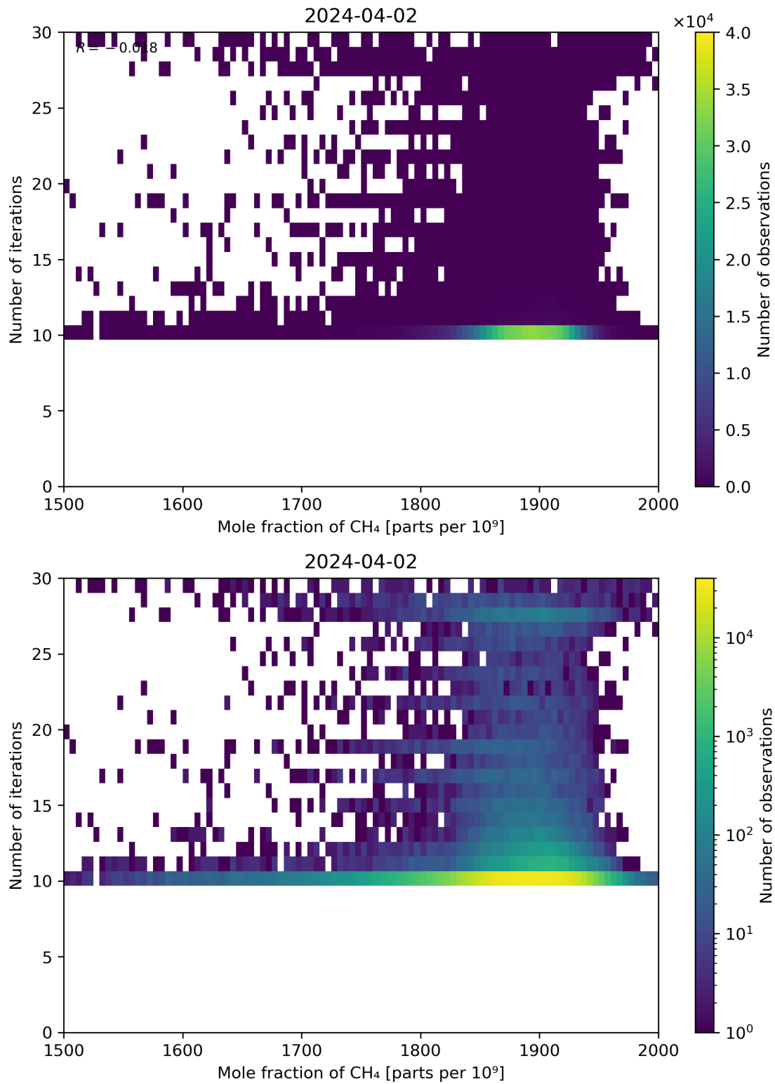
Figure 76: Scatter density plot of “Mole fraction of CH 4 ” against “Number of iterations” for 2024-04-01 to 2024-04-03.
