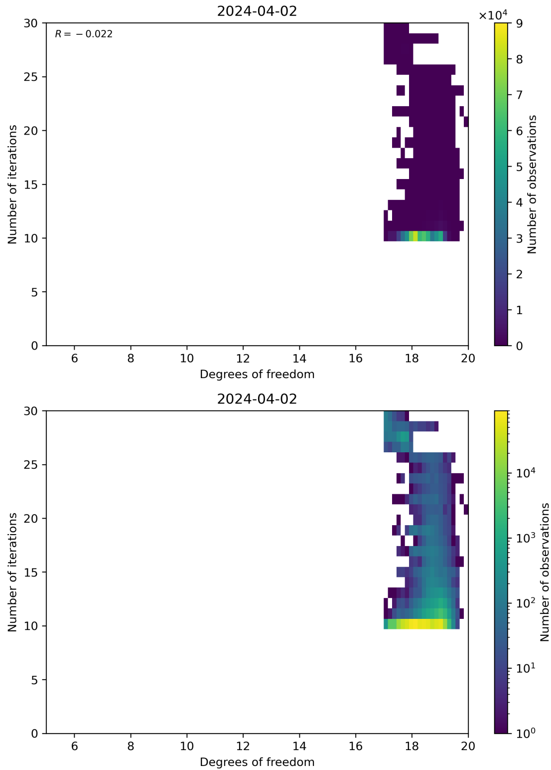
Figure 52: Scatter density plot of “Degrees of freedom” against “Number of iterations” for 2024-04-01 to 2024-04-03.
