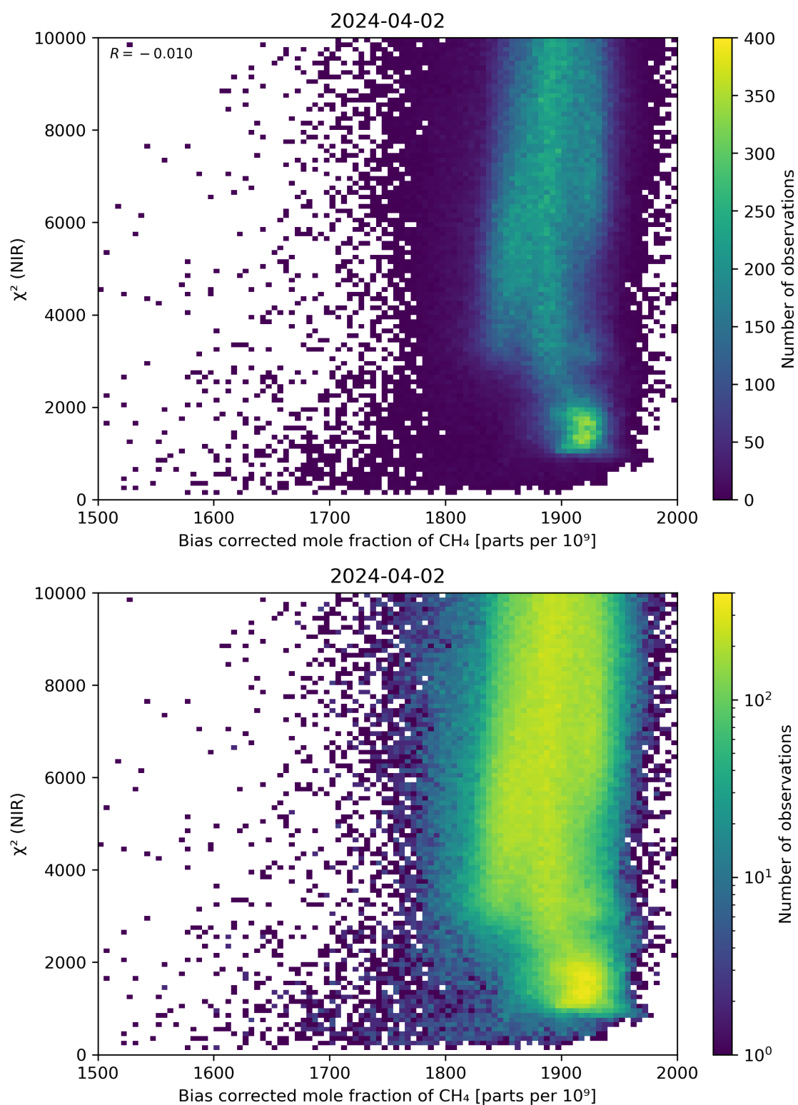
Figure 63: Scatter density plot of “Bias corrected mole fraction of CH 4 ” against “ \chi^2 (NIR)” for 2024-04-01 to 2024-04-03.
