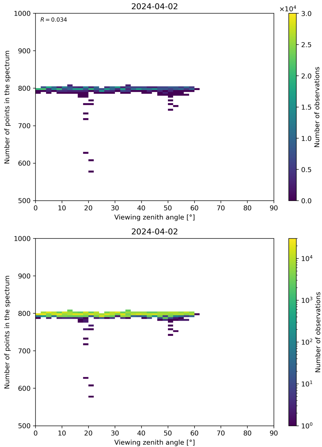
Figure 114: Scatter density plot of “Viewing zenith angle” against “Number of points in the spectrum” for 2024-04-01 to 2024-04-03.
