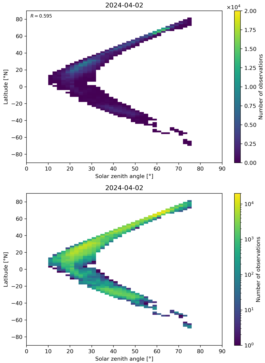
Figure 98: Scatter density plot of “Solar zenith angle” against “Latitude” for 2024-04-01 to 2024-04-03.
