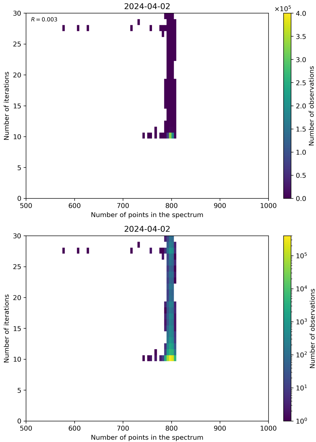
Figure 92: Scatter density plot of “Number of points in the spectrum” against “Number of iterations” for 2024-04-01 to 2024-04-03.
