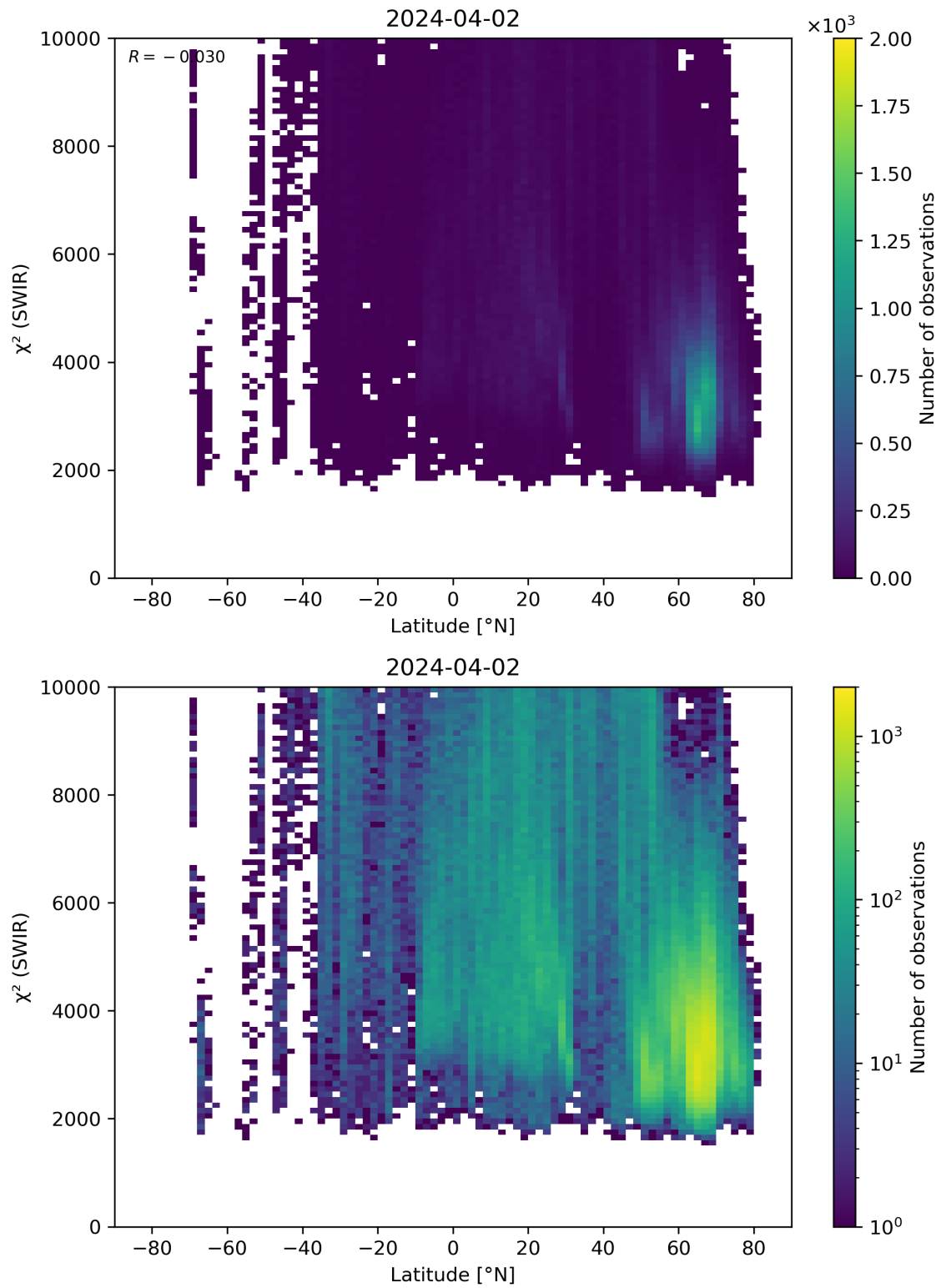
Figure 54: Scatter density plot of “Latitude” against “ \chi^2 (SWIR)” for 2024-04-01 to 2024-04-03.
