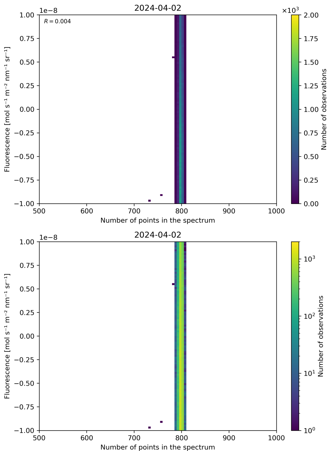
Figure 91: Scatter density plot of “Number of points in the spectrum” against “Fluorescence” for 2024-04-01 to 2024-04-03.
