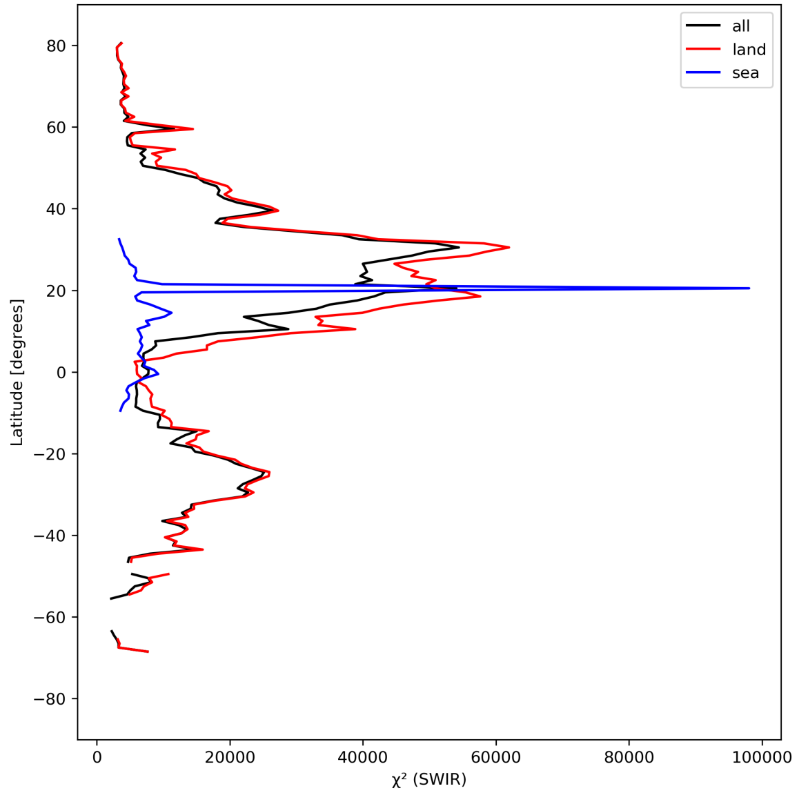
Figure 17: Zonal average of “ \chi^2 (SWIR)” for 2024-04-01 to 2024-04-03.
