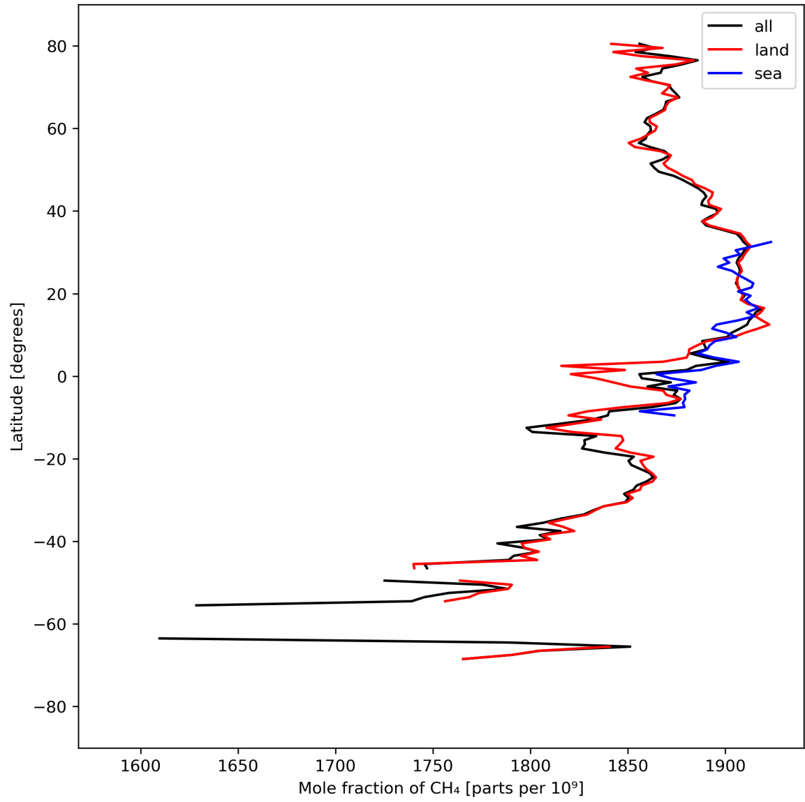
Figure 12: Zonal average of “Mole fraction of CH 4 ” for 2024-04-01 to 2024-04-03.
