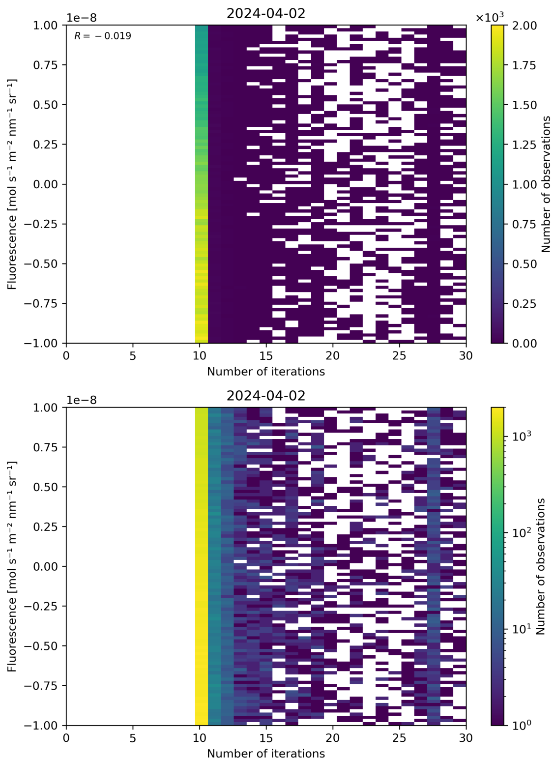
Figure 87: Scatter density plot of “Number of iterations” against “Fluorescence” for 2024-04-01 to 2024-04-03.
