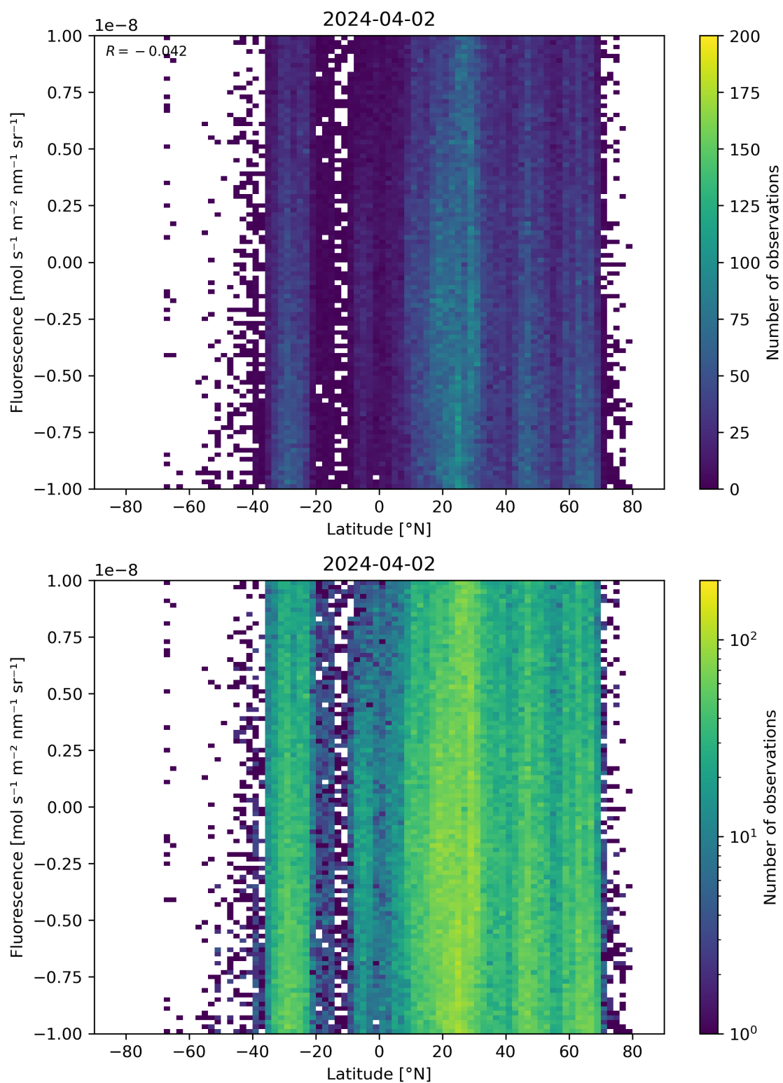
Figure 56: Scatter density plot of “Latitude” against “Fluorescence” for 2024-04-01 to 2024-04-03.
