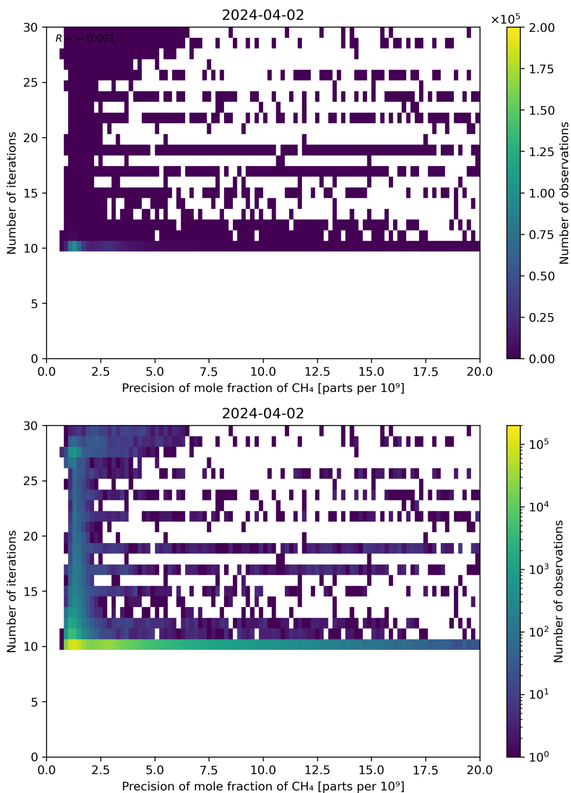
Figure 83: Scatter density plot of “Precision of mole fraction of CH 4 ” against “Number of iterations” for 2024-04-01 to 2024-04-03.
