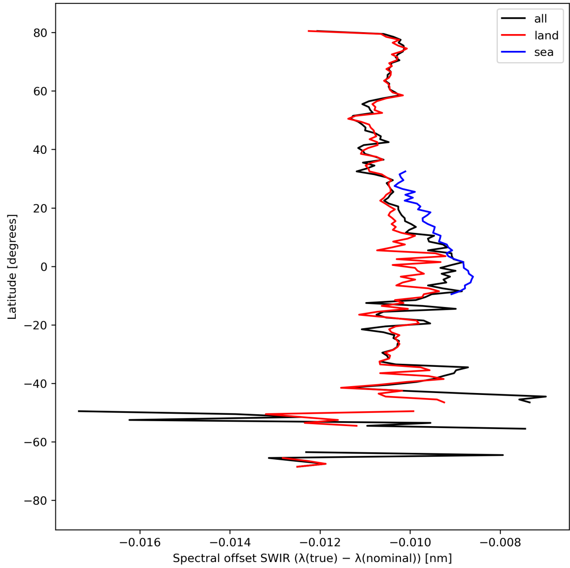
Figure 16: Zonal average of “Spectral offset SWIR ( \lambda(\text{true}) - \lambda(\text{nominal}) )” for 2024-04-01 to 2024-04-03.
