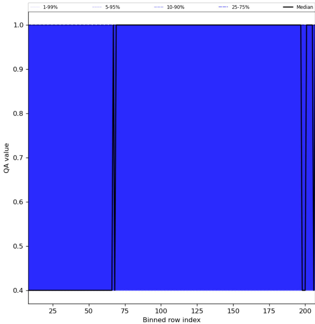
Figure 33: Along track statistics of “QA value” for 2024-04-01 to 2024-04-03
