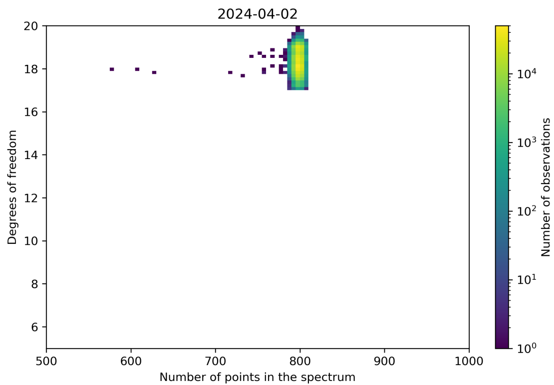
Figure 90: Scatter density plot of “Number of points in the spectrum” against “Degrees of freedom” for 2024-04-01 to 2024-04-03.
