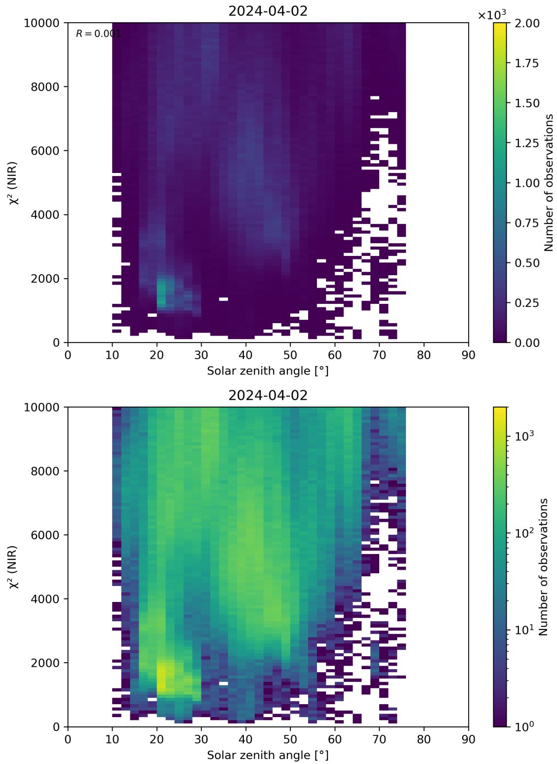
Figure 94: Scatter density plot of “Solar zenith angle” against “ \chi^2 (NIR)” for 2024-04-01 to 2024-04-03.
