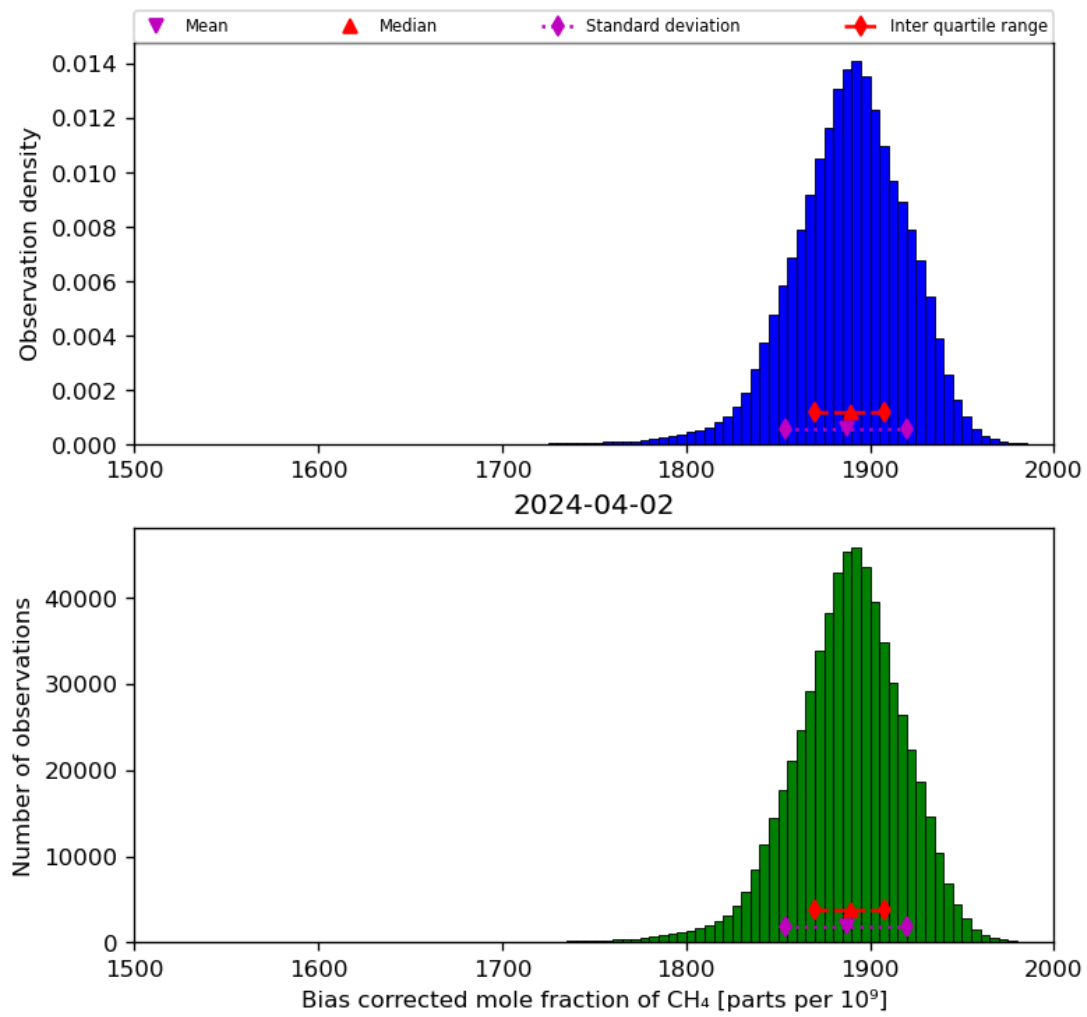
Figure 25: Histogram of “Bias corrected mole fraction of CH 4 ” for 2024-04-01 to 2024-04-03
