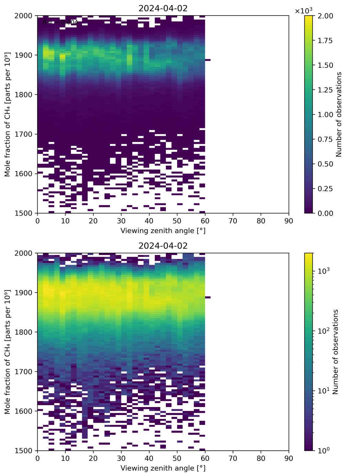
Figure 110: Scatter density plot of “Viewing zenith angle” against “Mole fraction of CH 4 ” for 2024-04-01 to 2024-04-03.
