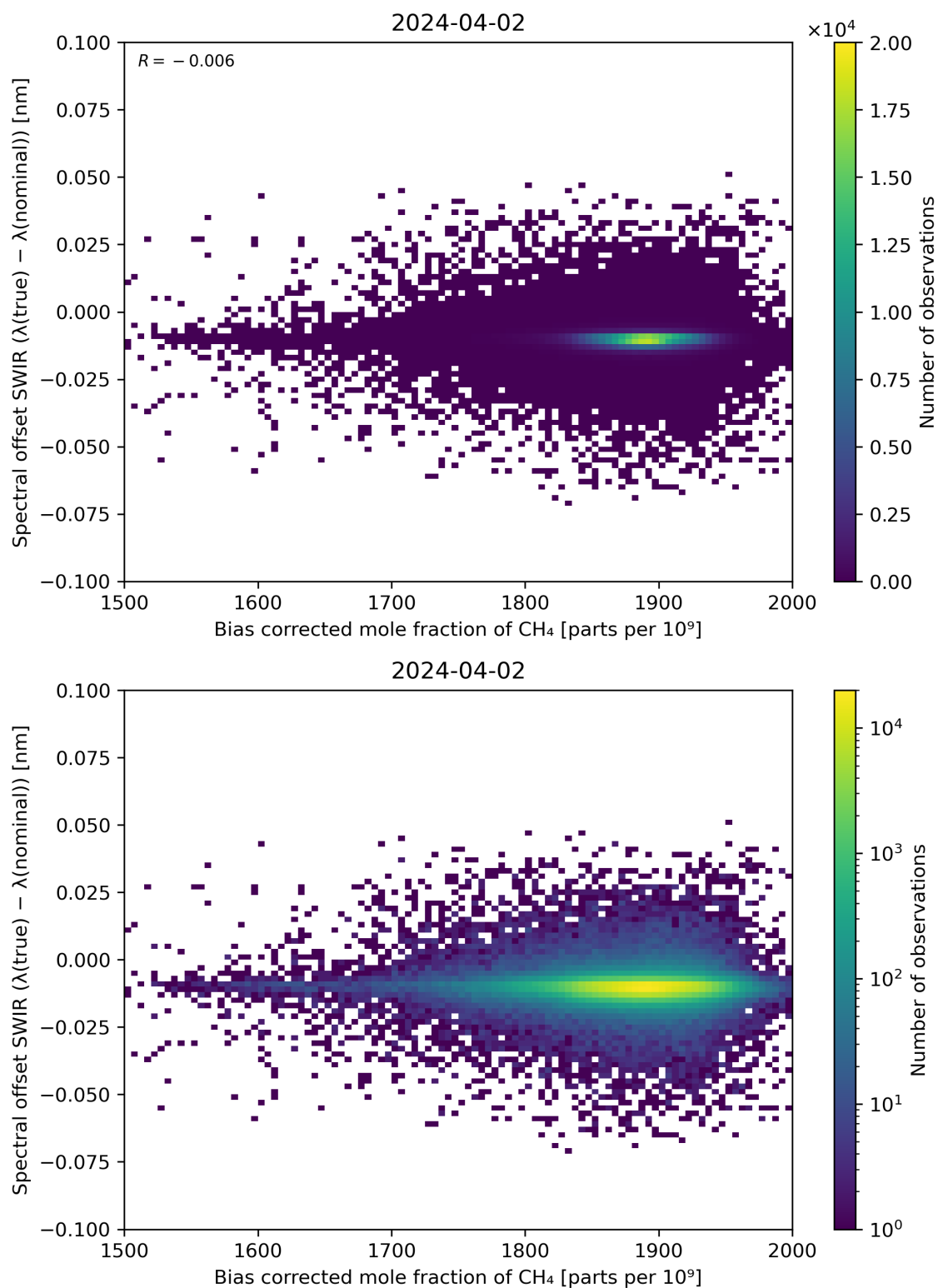
Figure 69: Scatter density plot of “Bias corrected mole fraction of \text{CH}_4 ” against “Spectral offset SWIR ( \lambda(\text{true}) - \lambda(\text{nominal}) )” for 2024-04-01 to 2024-04-03.
