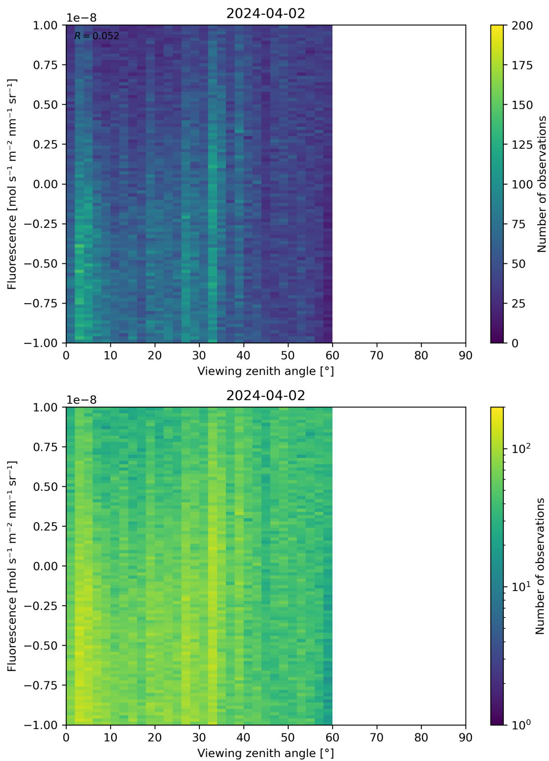
Figure 108: Scatter density plot of “Viewing zenith angle” against “Fluorescence” for 2024-04-01 to 2024-04-03.
