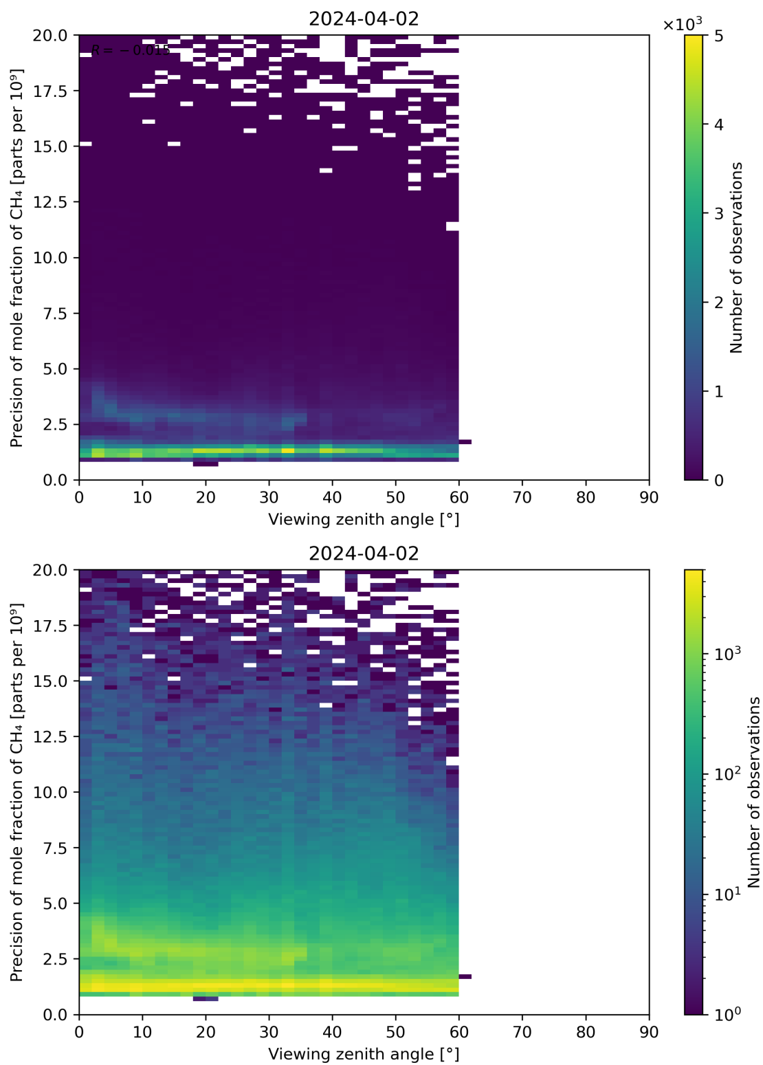
Figure 112: Scatter density plot of “Viewing zenith angle” against “Precision of mole fraction of \text{CH}_4 ” for 2024-04-01 to 2024-04-03.
