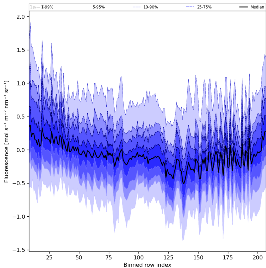
Figure 43: Along track statistics of “Fluorescence” for 2024-04-01 to 2024-04-03
