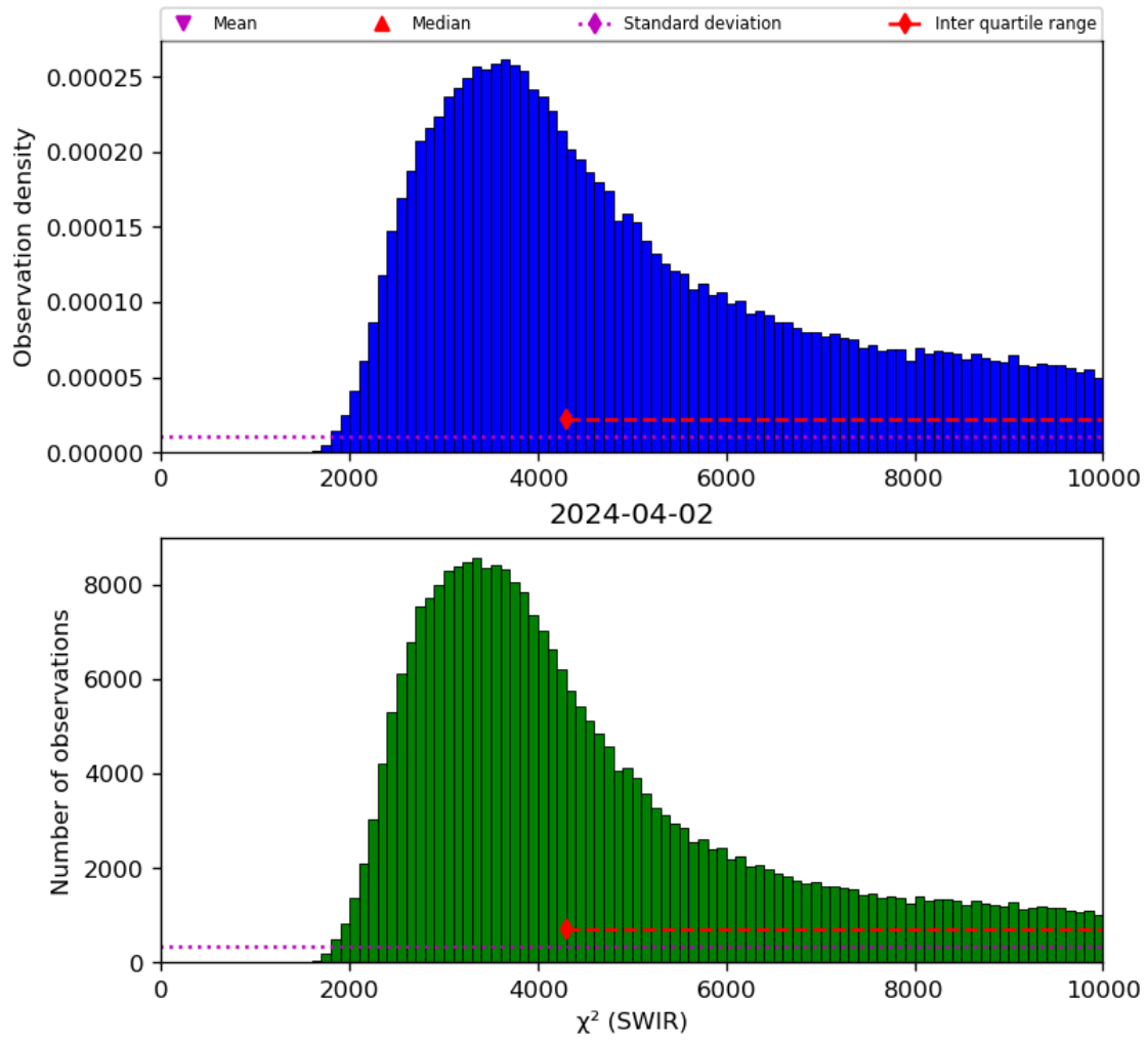
Figure 28: Histogram of “ \chi^2 (SWIR)” for 2024-04-01 to 2024-04-03
