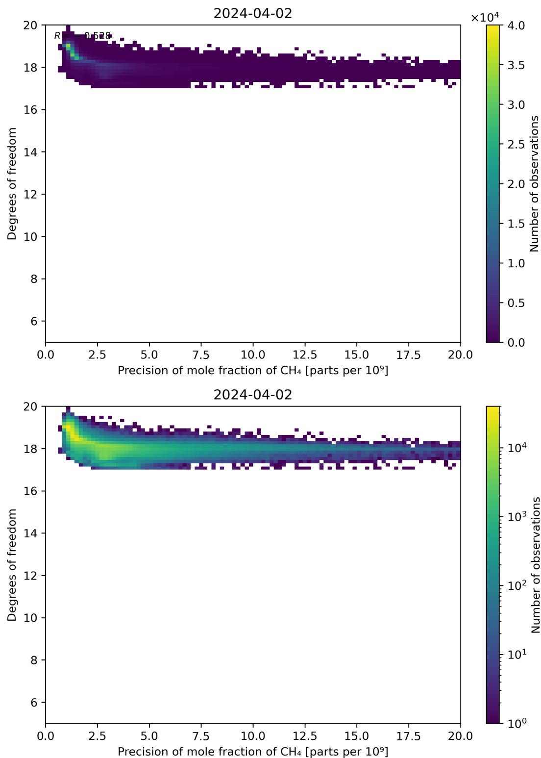
Figure 80: Scatter density plot of “Precision of mole fraction of CH 4 ” against “Degrees of freedom” for 2024-04-01 to 2024-04-03.
