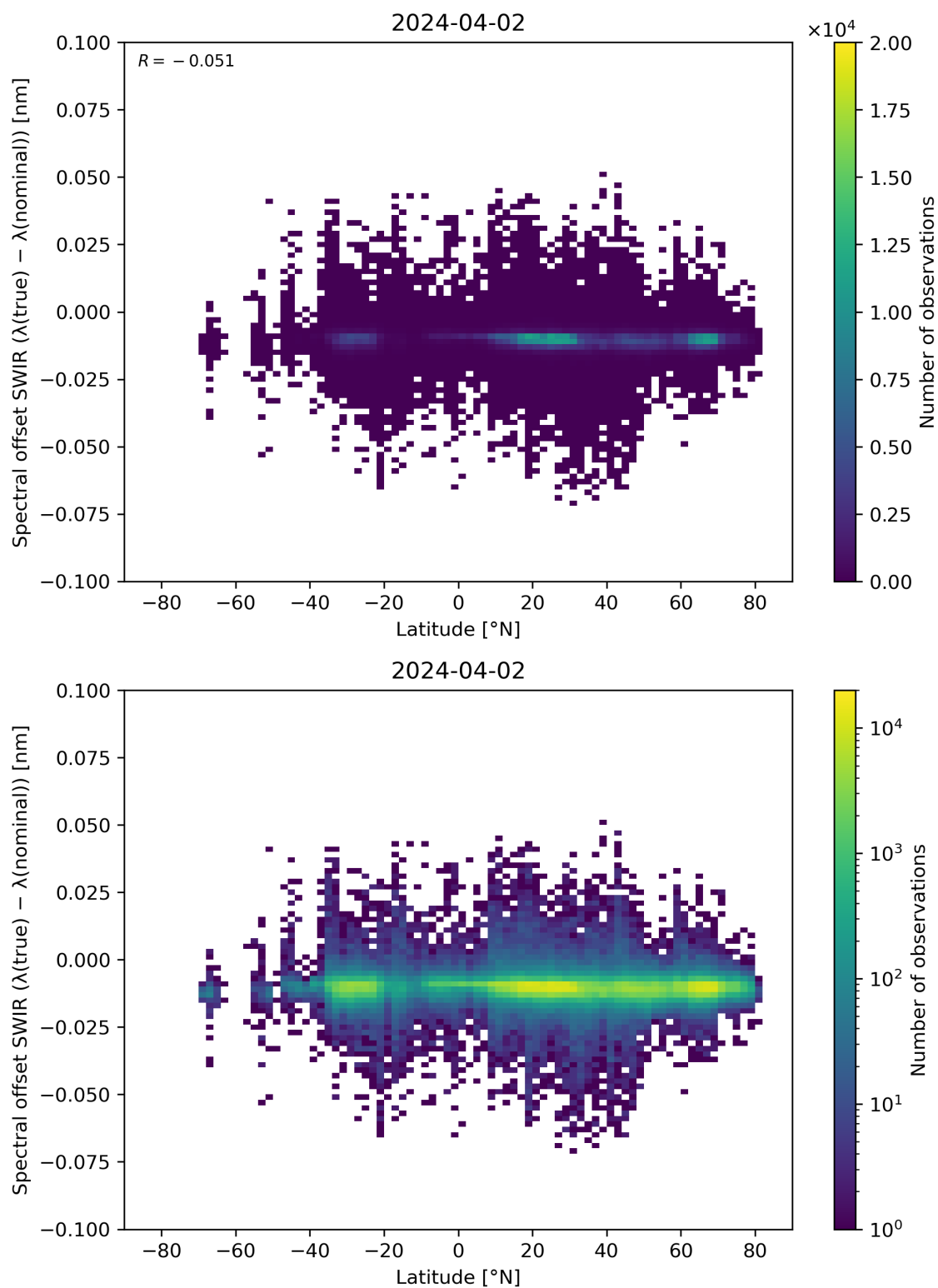
Figure 62: Scatter density plot of “Latitude” against “Spectral offset SWIR ( \lambda(\text{true}) - \lambda(\text{nominal}) )” for 2024-04-01 to 2024-04-03.
