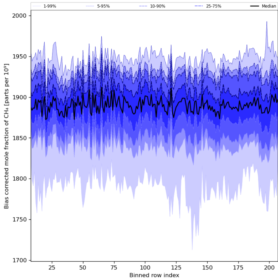
Figure 36: Along track statistics of “Bias corrected mole fraction of CH 4 ” for 2024-04-01 to 2024-04-03
