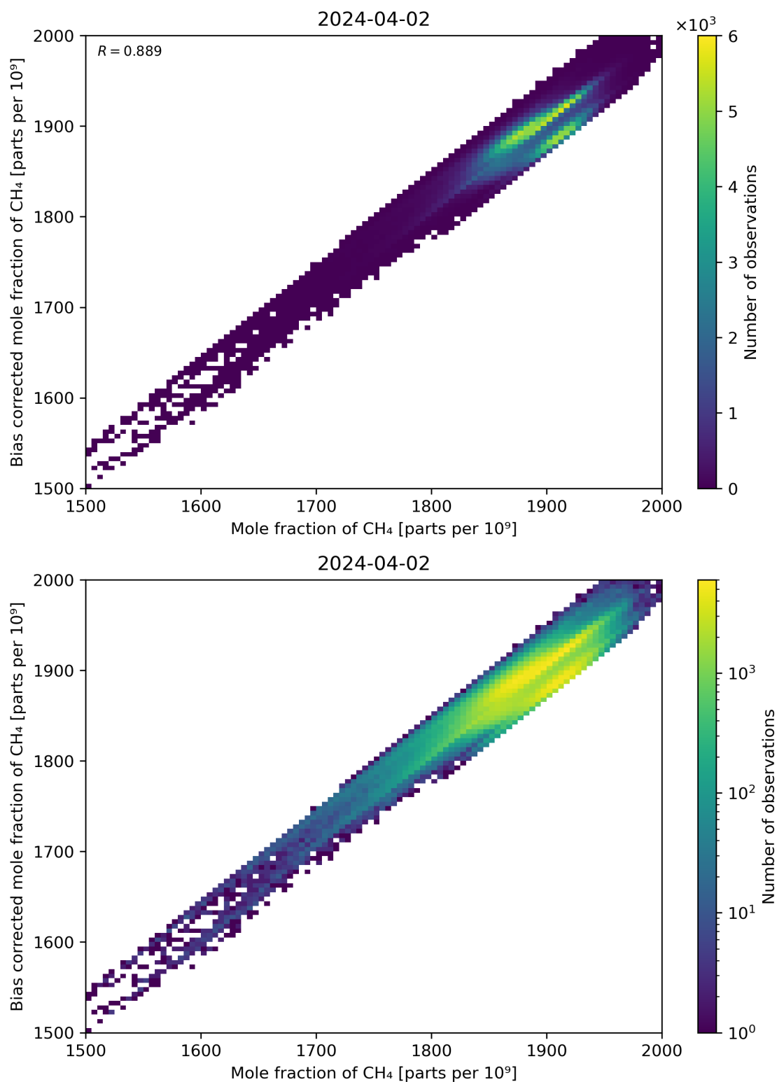
Figure 74: Scatter density plot of “Mole fraction of CH 4 ” against “Bias corrected mole fraction of CH 4 ” for 2024-04-01 to 2024-04-03.
