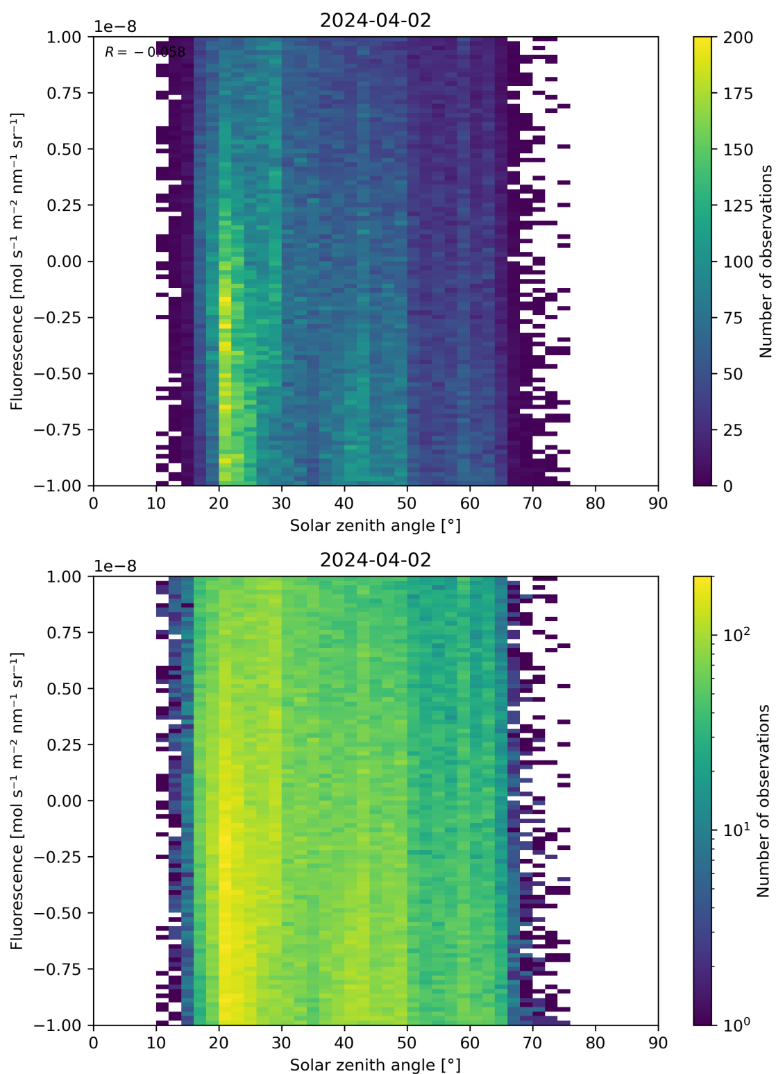
Figure 97: Scatter density plot of “Solar zenith angle” against “Fluorescence” for 2024-04-01 to 2024-04-03.
