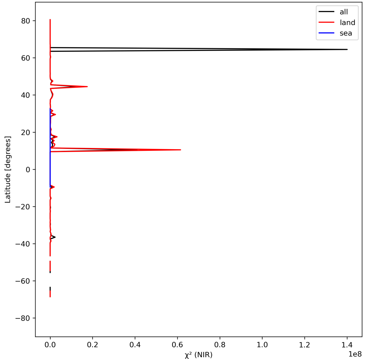
Figure 18: Zonal average of “ \chi^2 (NIR)” for 2024-04-01 to 2024-04-03.
