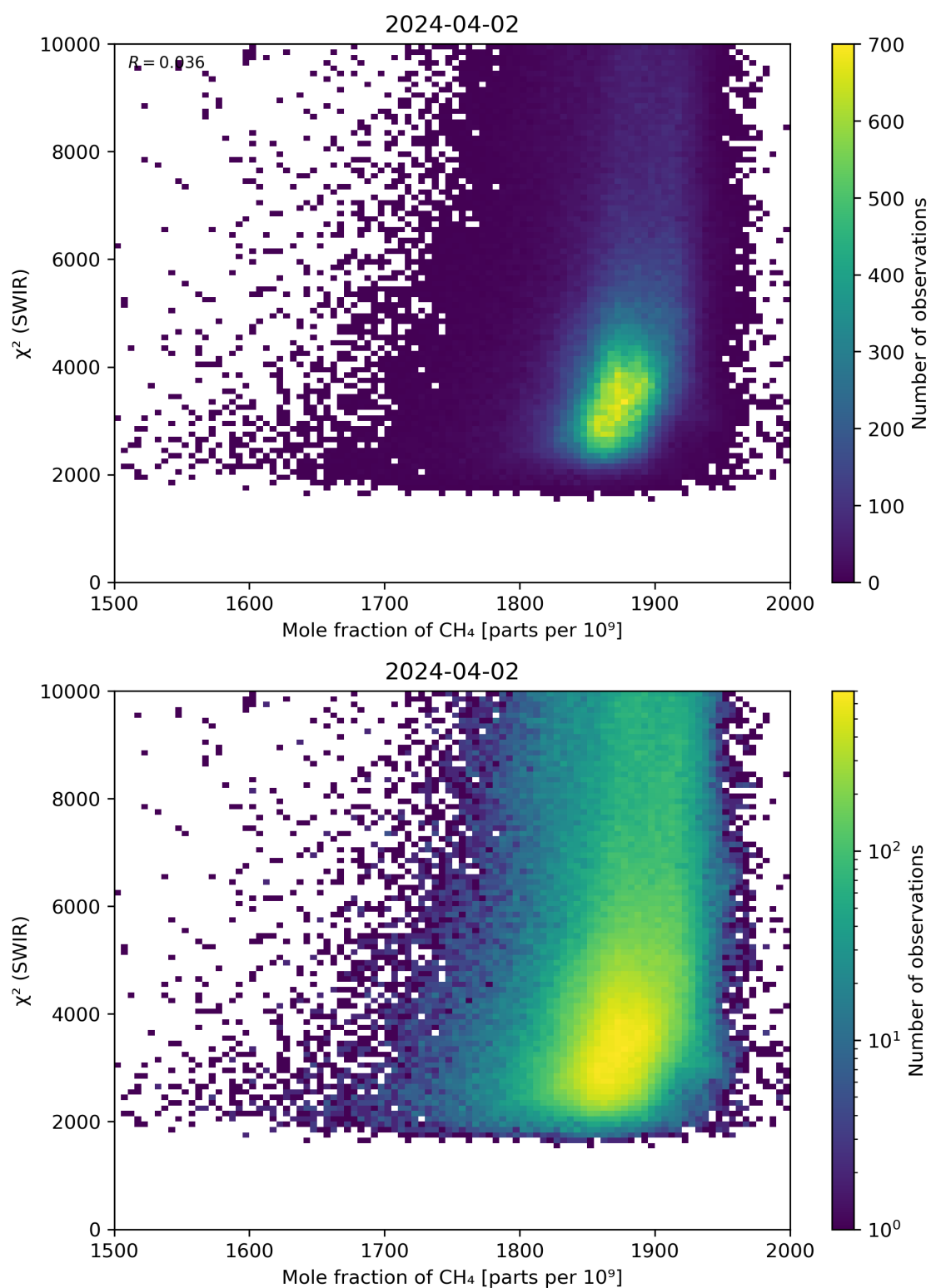
Figure 71: Scatter density plot of “Mole fraction of \text{CH}_4 ” against “ \chi^2 (SWIR)” for 2024-04-01 to 2024-04-03.
