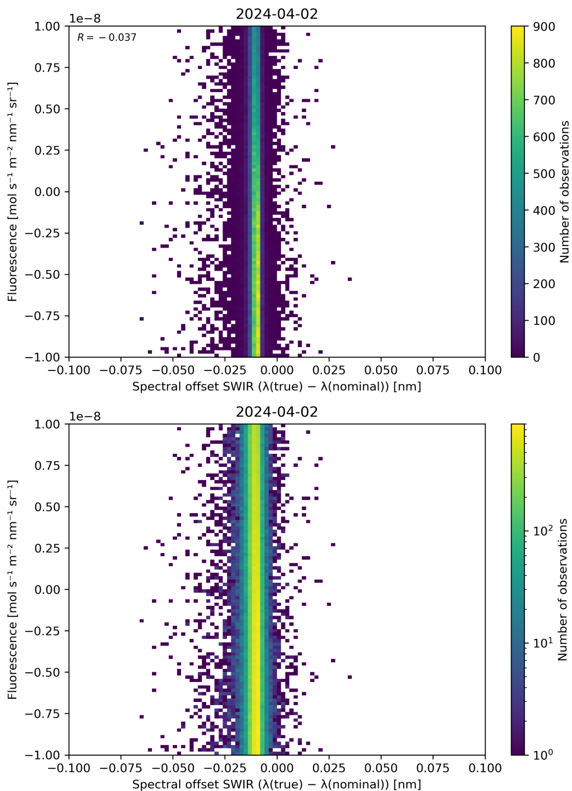
Figure 120: Scatter density plot of “Spectral offset SWIR ( \lambda(\text{true}) - \lambda(\text{nominal}) )” against “Fluorescence” for 2024-04-01 to 2024-04-03.
