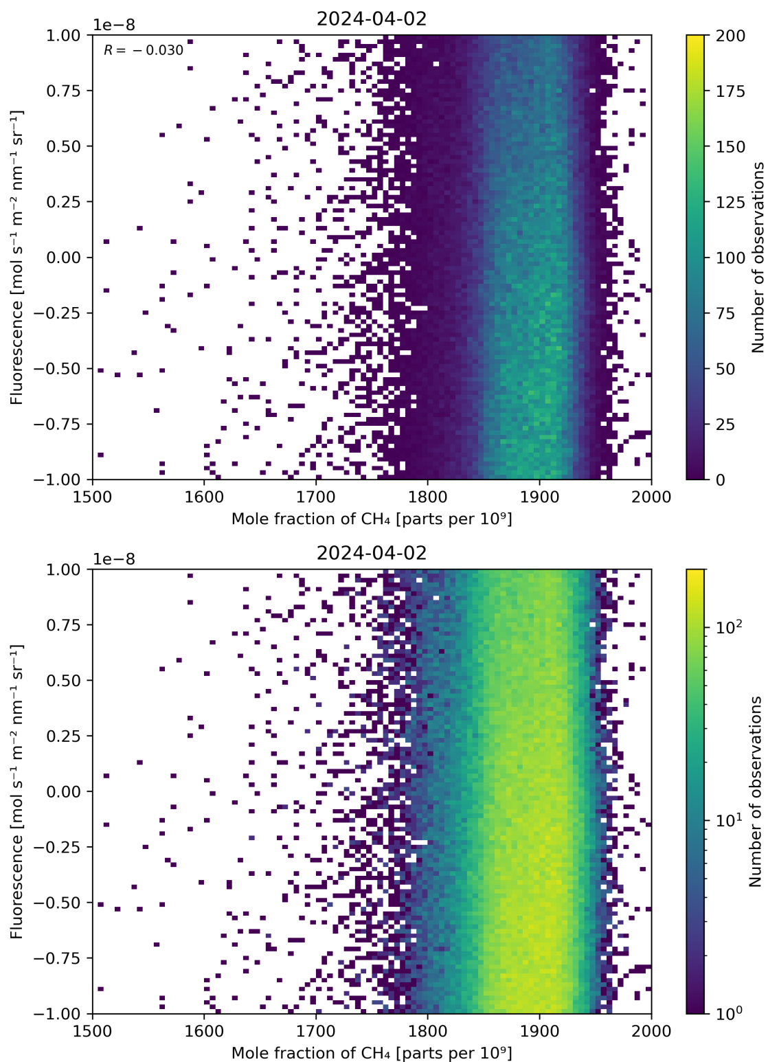
Figure 73: Scatter density plot of “Mole fraction of \text{CH}_4 ” against “Fluorescence” for 2024-04-01 to 2024-04-03.
