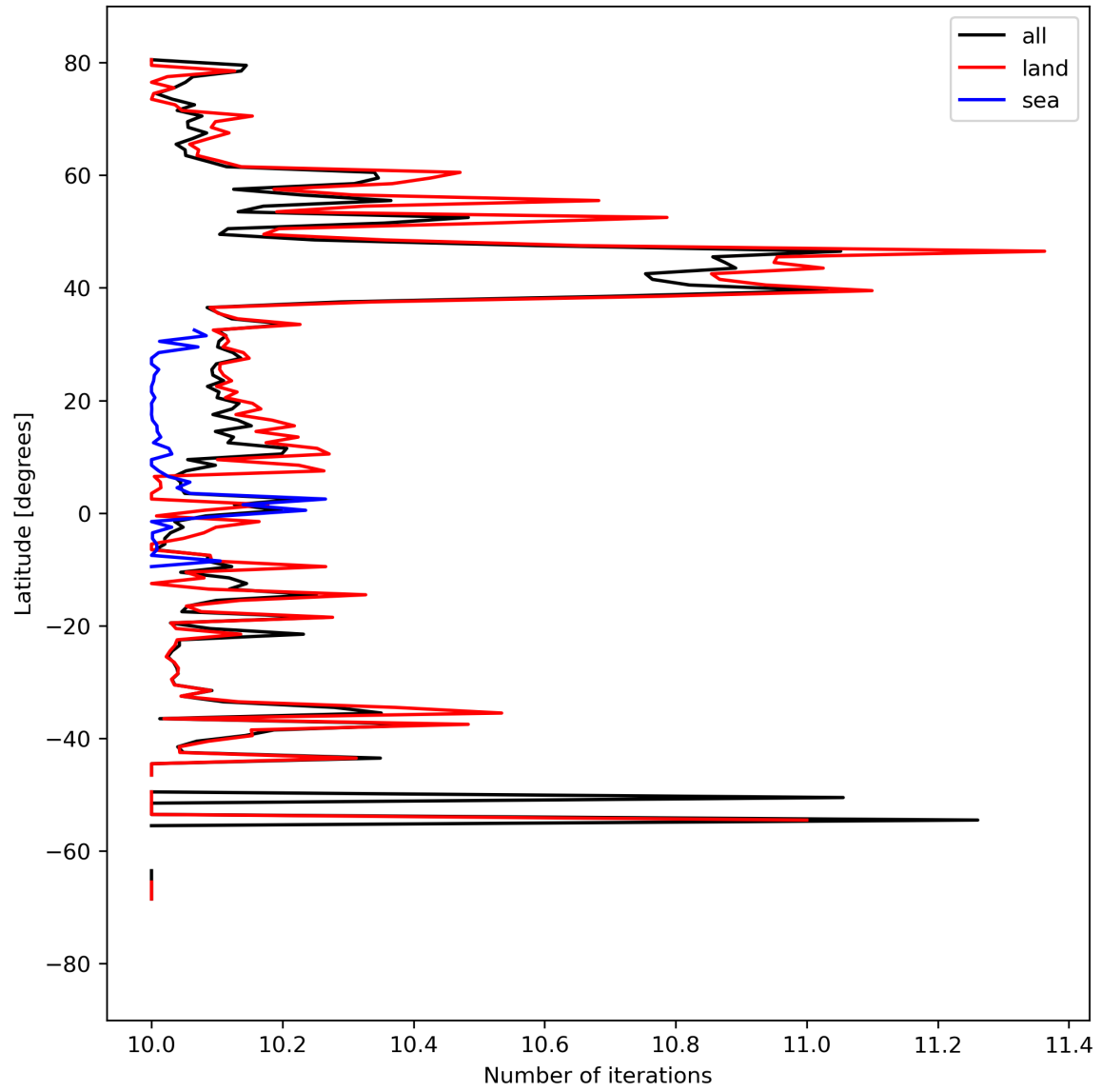
Figure 20: Zonal average of “Number of iterations” for 2024-04-01 to 2024-04-03.
