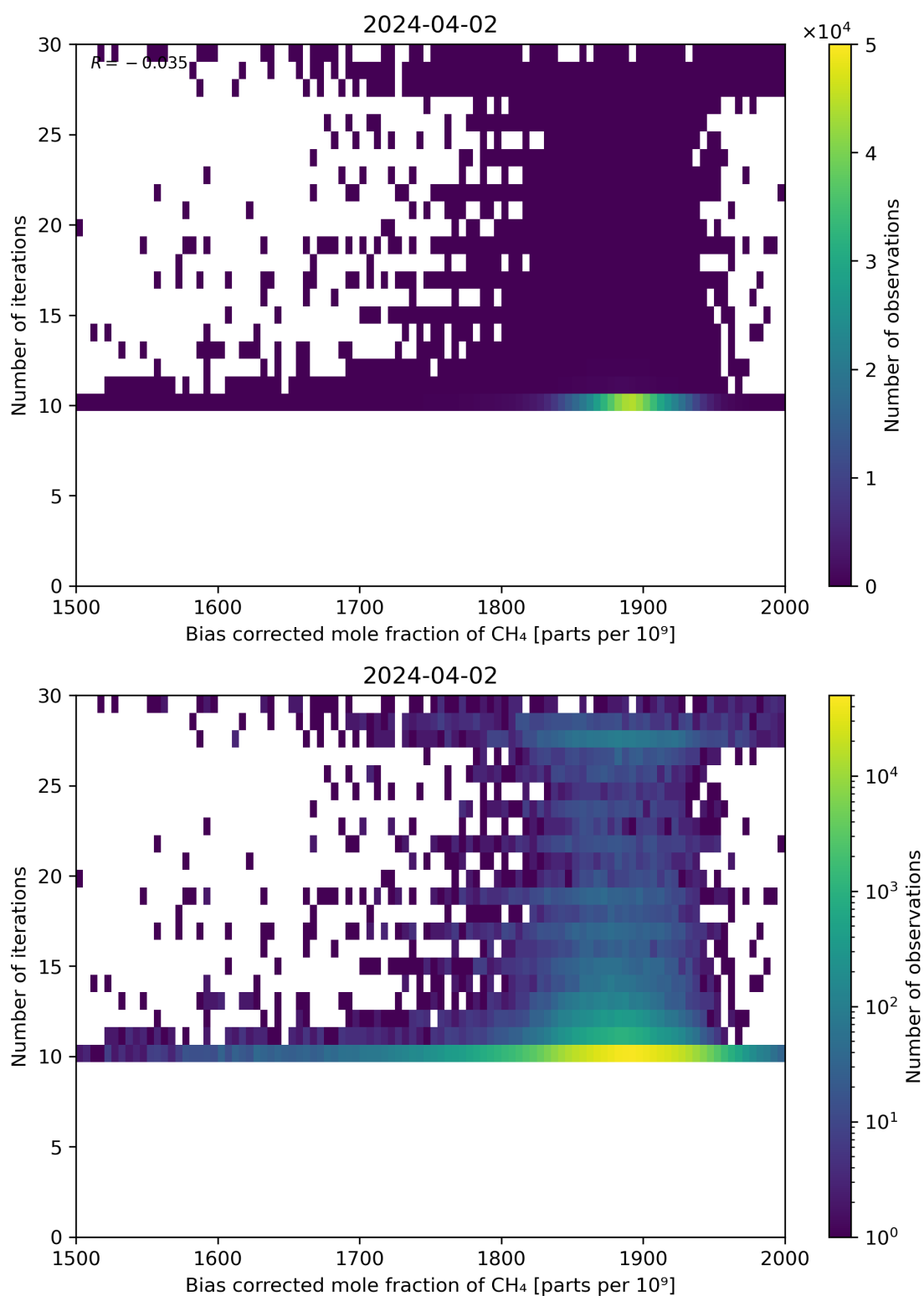
Figure 67: Scatter density plot of “Bias corrected mole fraction of CH 4 ” against “Number of iterations” for 2024-04-01 to 2024-04-03.
