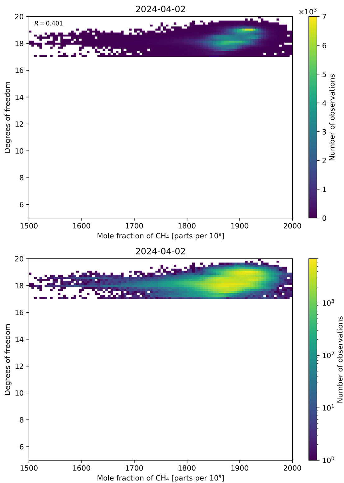
Figure 72: Scatter density plot of “Mole fraction of CH 4 ” against “Degrees of freedom” for 2024-04-01 to 2024-04-03.
