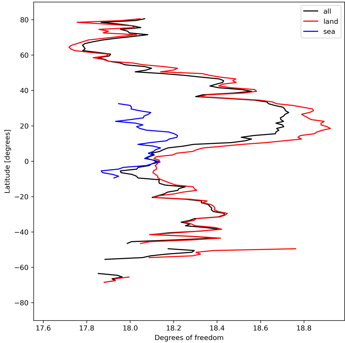
Figure 19: Zonal average of “Degrees of freedom” for 2024-04-01 to 2024-04-03.
