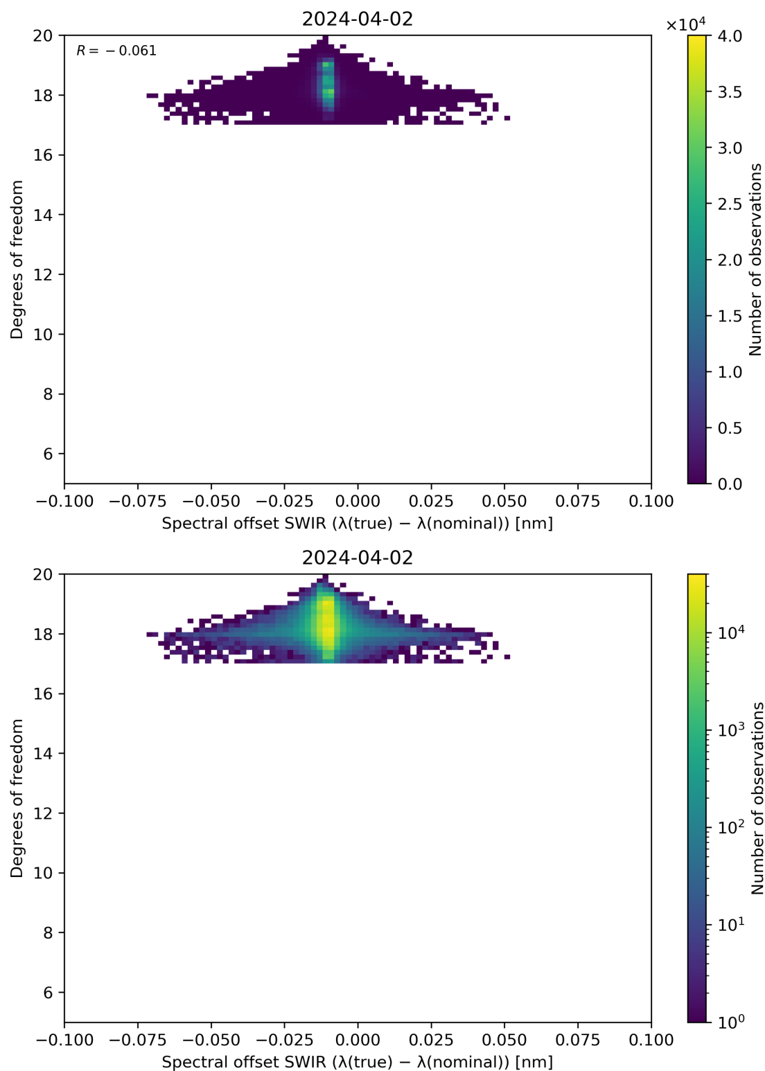
Figure 119: Scatter density plot of “Spectral offset SWIR ( \lambda(\text{true}) - \lambda(\text{nominal}) )” against “Degrees of freedom” for 2024-04-01 to 2024-04-03.
