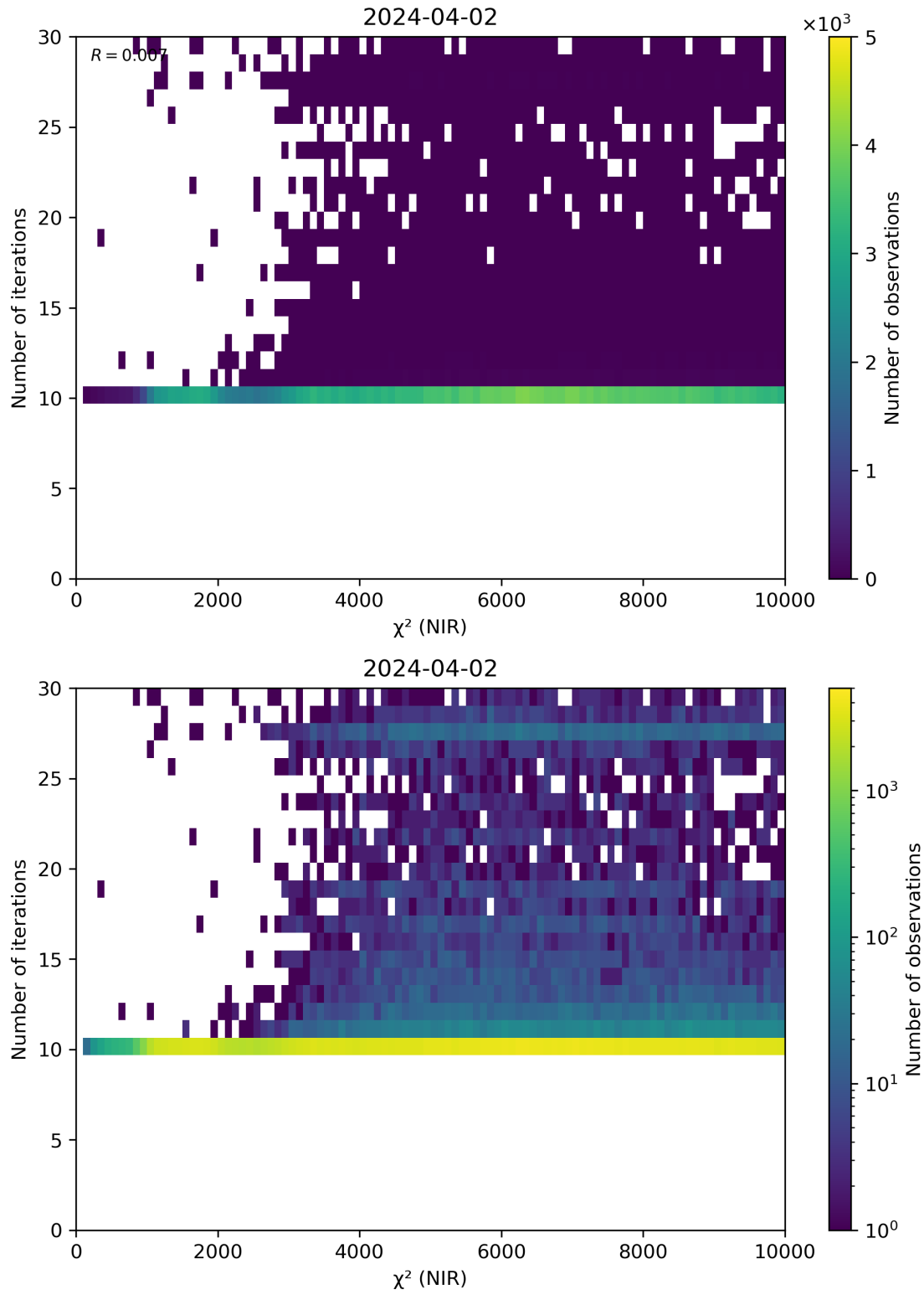
Figure 46: Scatter density plot of “ \chi^2 (NIR)” against “Number of iterations” for 2024-04-01 to 2024-04-03.
