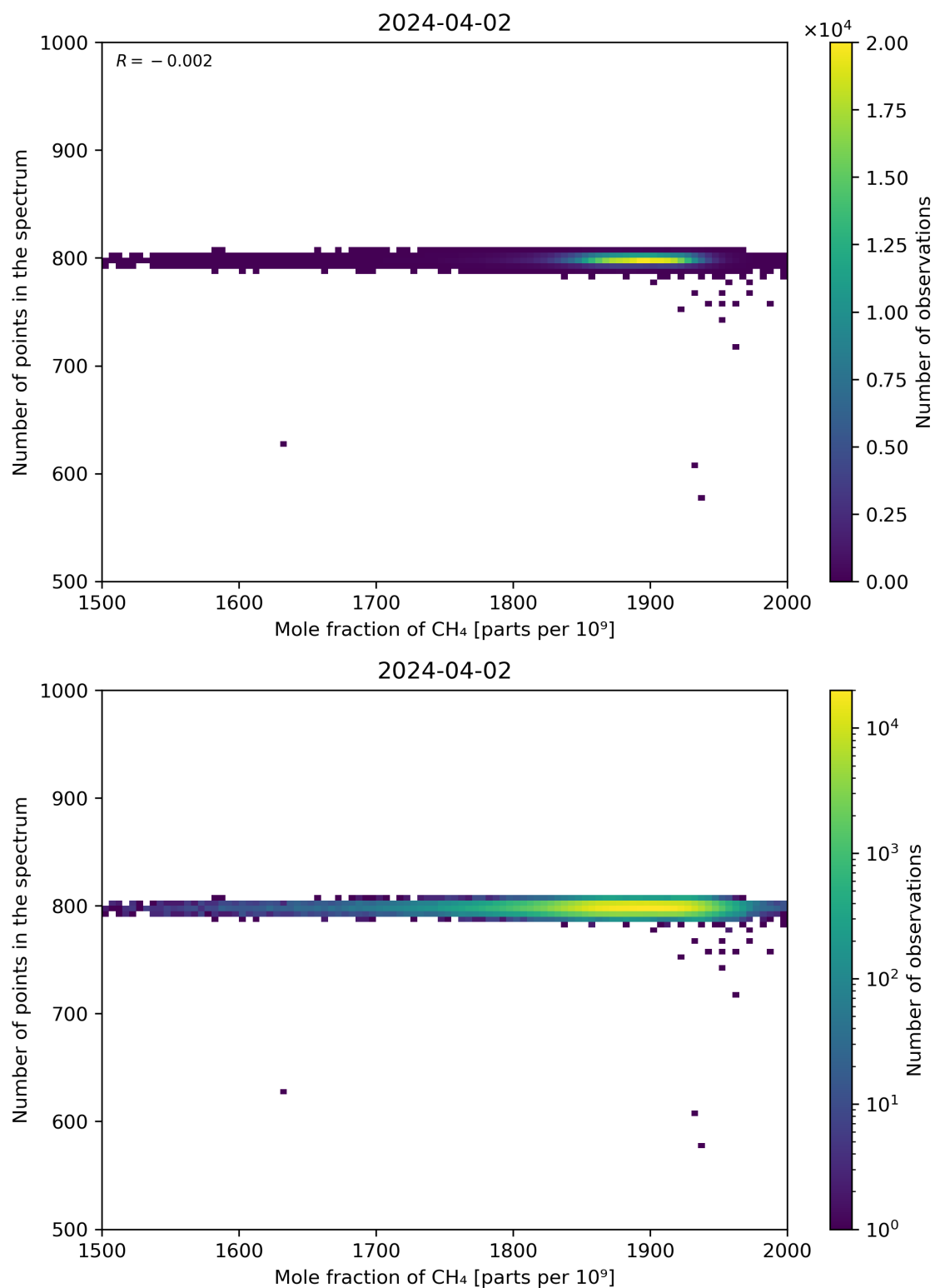
Figure 77: Scatter density plot of “Mole fraction of CH 4 ” against “Number of points in the spectrum” for 2024-04-01 to 2024-04-03.
