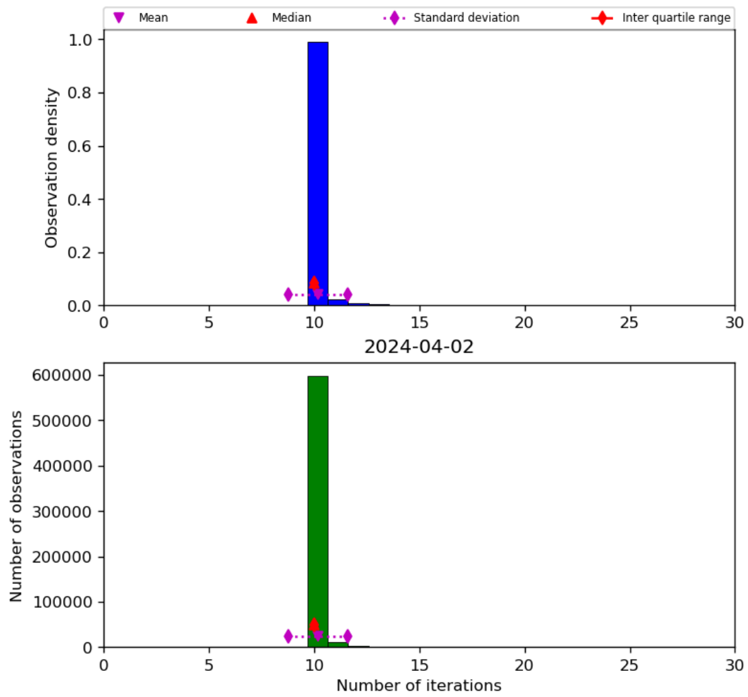
Figure 31: Histogram of “Number of iterations” for 2024-04-01 to 2024-04-03
