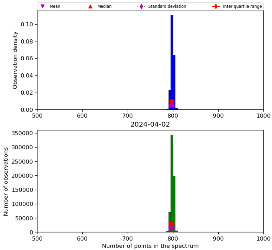
Figure 26: Histogram of “Number of points in the spectrum” for 2024-04-01 to 2024-04-03
