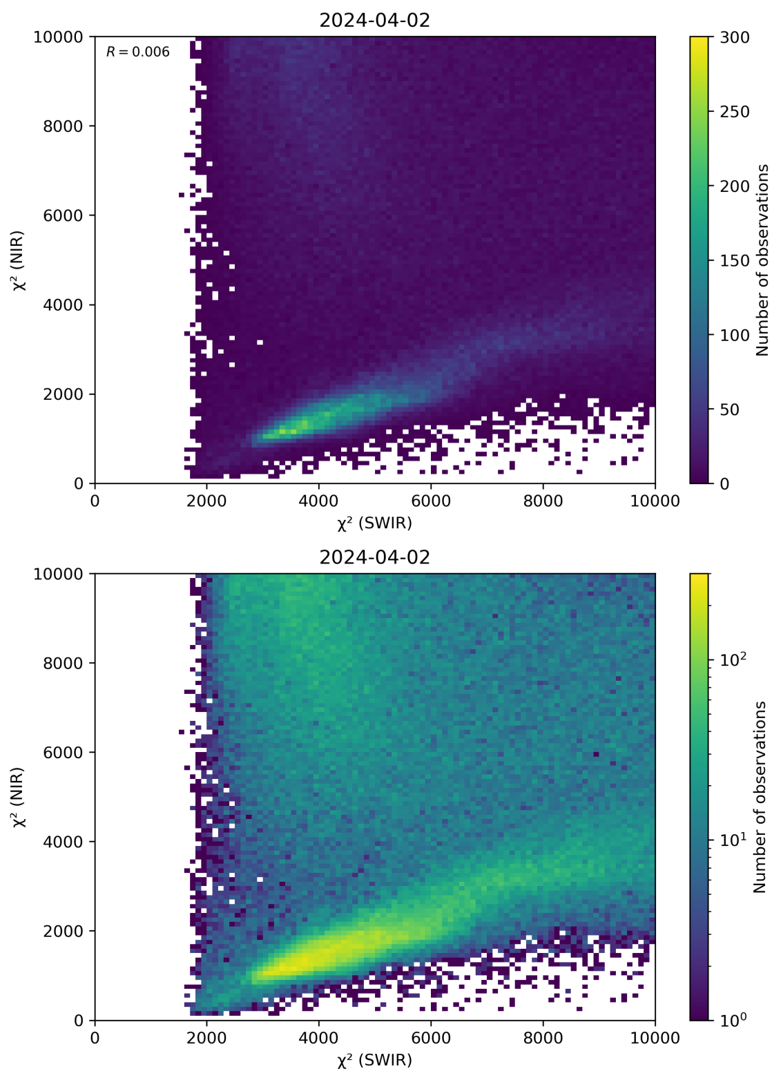
Figure 47: Scatter density plot of “ \chi^2 (SWIR)” against “ \chi^2 (NIR)” for 2024-04-01 to 2024-04-03.
