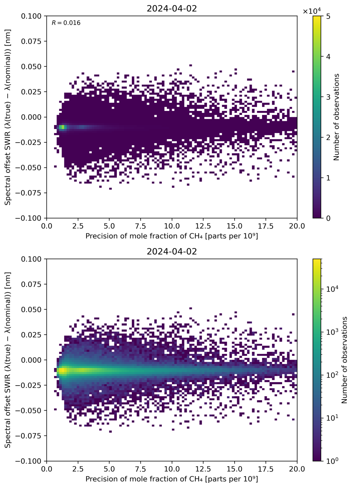
Figure 85: Scatter density plot of “Precision of mole fraction of \text{CH}_4 ” against “Spectral offset SWIR ( \lambda(\text{true}) - \lambda(\text{nominal}) )” for 2024-04-01 to 2024-04-03.
