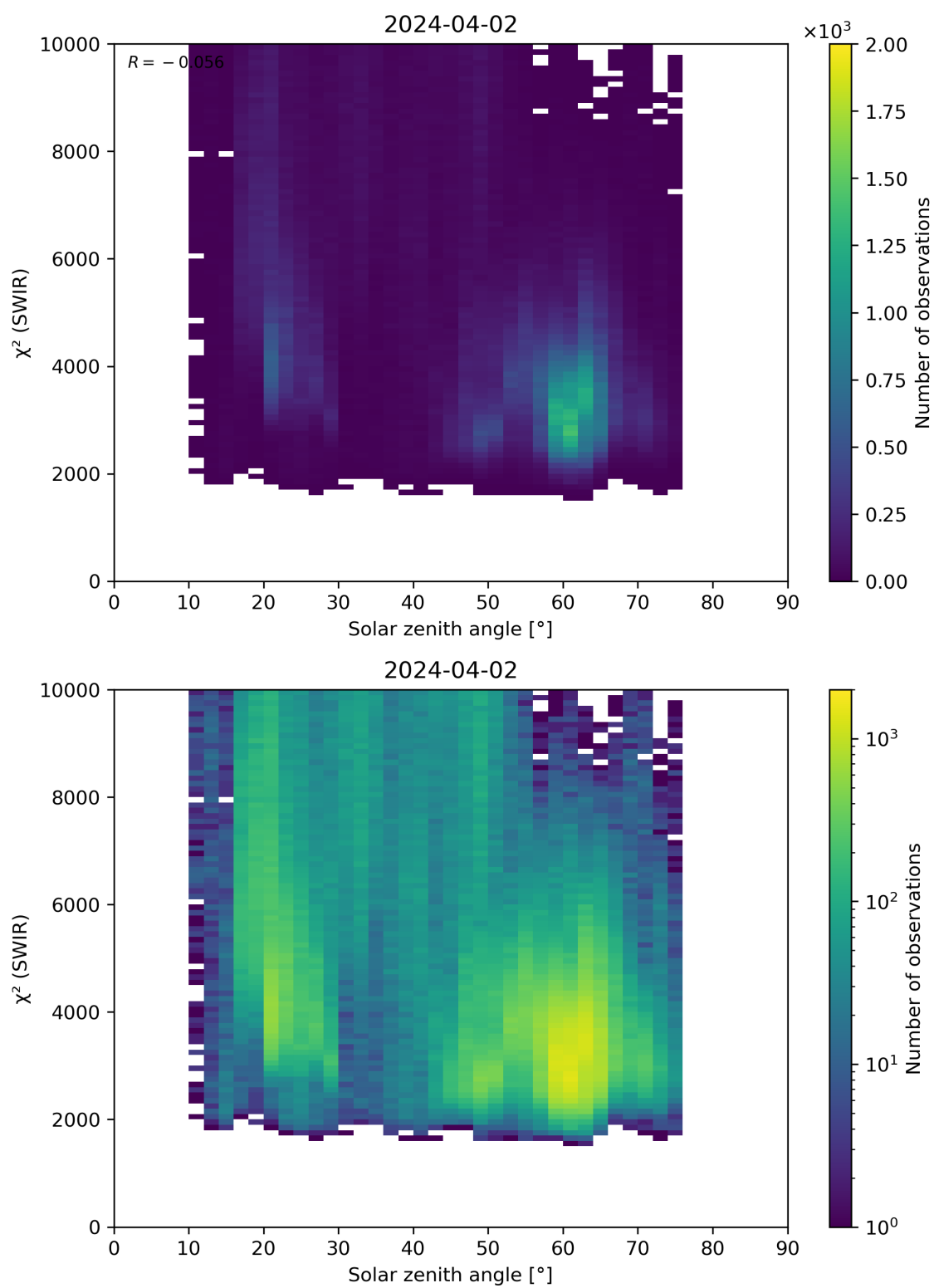
Figure 95: Scatter density plot of “Solar zenith angle” against “ \chi^2 (SWIR)” for 2024-04-01 to 2024-04-03.
