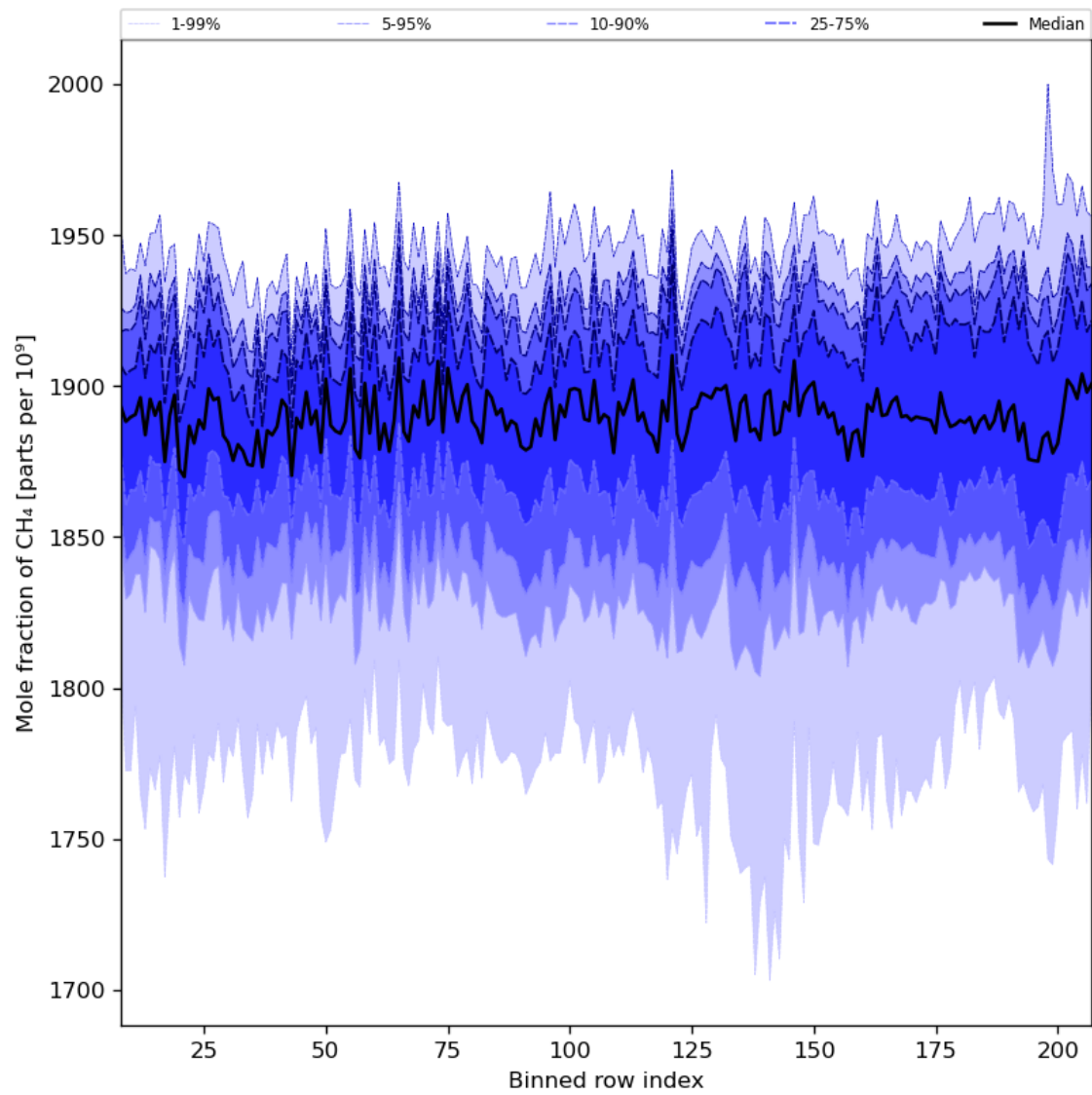
Figure 34: Along track statistics of “Mole fraction of CH 4 ” for 2024-04-01 to 2024-04-03
