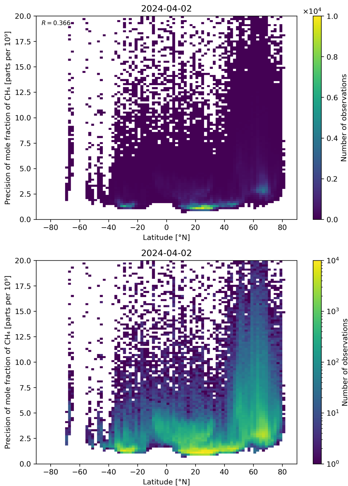
Figure 59: Scatter density plot of “Latitude” against “Precision of mole fraction of \text{CH}_4 ” for 2024-04-01 to 2024-04-03.
