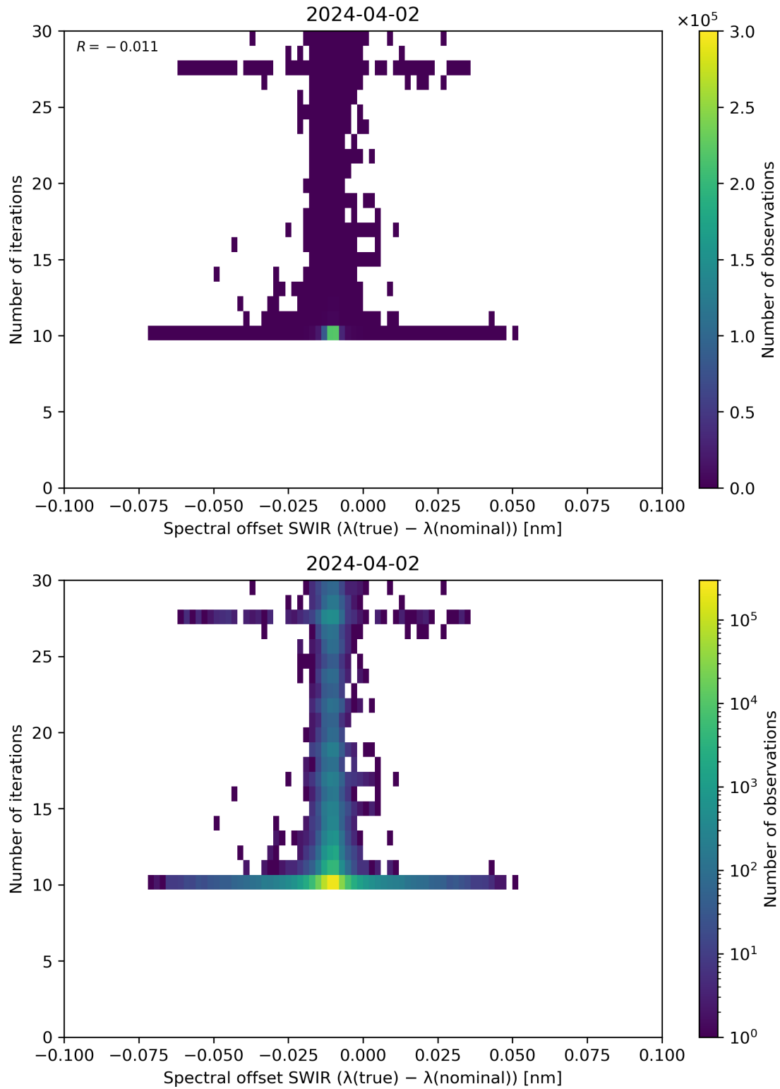
Figure 121: Scatter density plot of “Spectral offset SWIR ( \lambda(\text{true}) - \lambda(\text{nominal}) )” against “Number of iterations” for 2024-04-01 to 2024-04-03.
