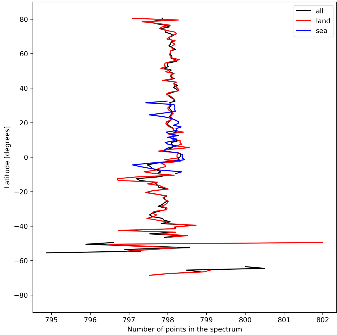
Figure 15: Zonal average of “Number of points in the spectrum” for 2024-04-01 to 2024-04-03.
