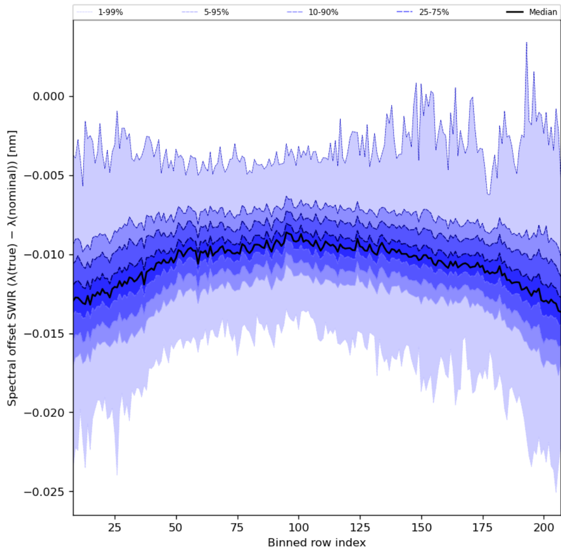
Figure 38: Along track statistics of “Spectral offset SWIR ( \lambda(\text{true}) - \lambda(\text{nominal}) )” for 2024-04-01 to 2024-04-03
