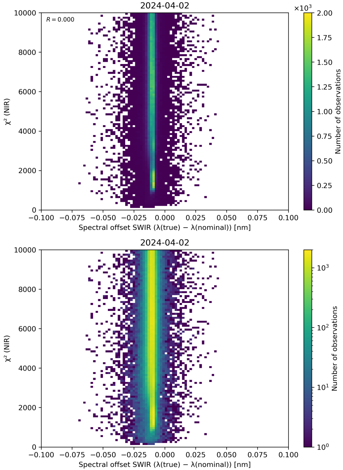
Figure 117: Scatter density plot of “Spectral offset SWIR ( \lambda(\text{true}) - \lambda(\text{nominal}) )” against “ \chi^2 (NIR)” for 2024-04-01 to 2024-04-03.
