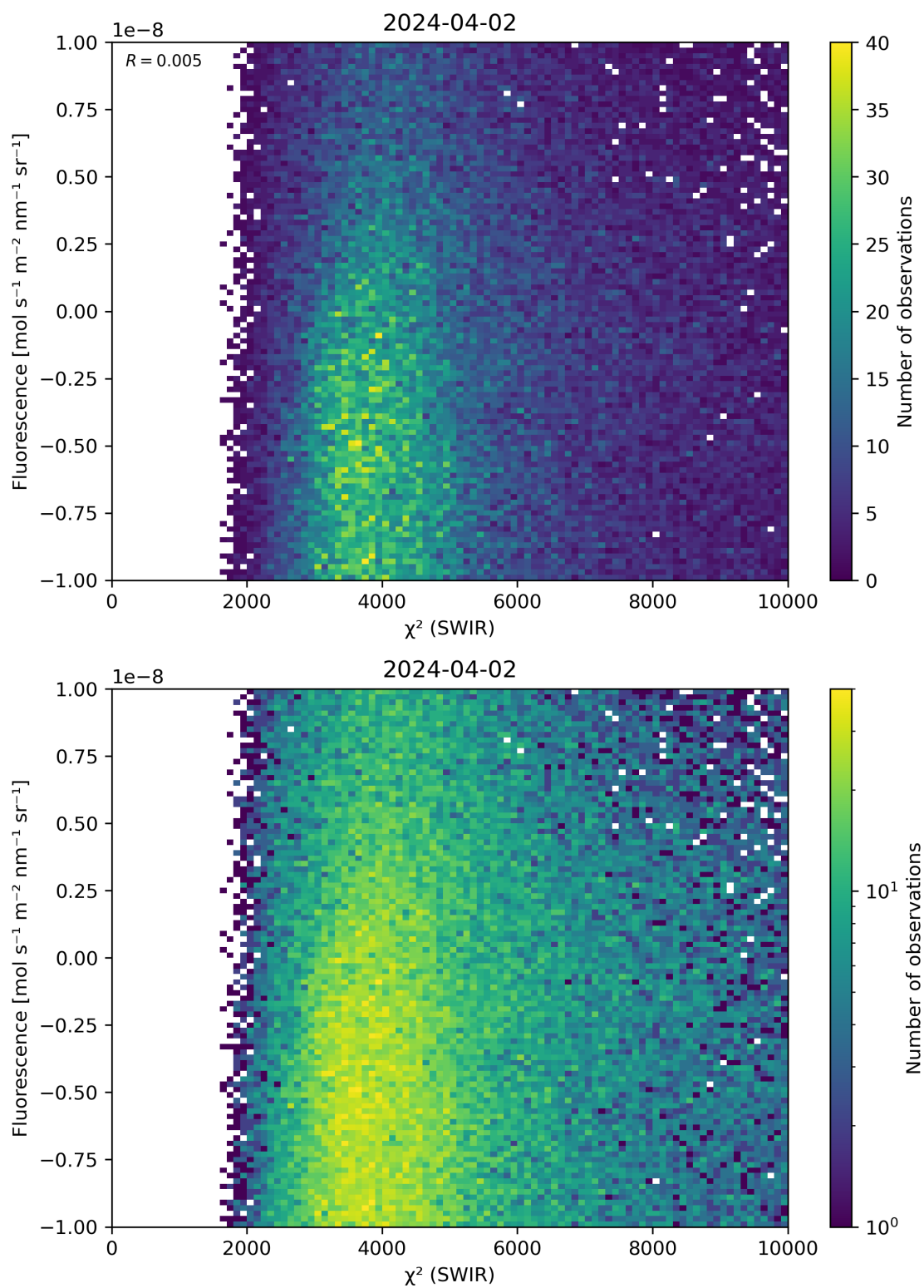
Figure 49: Scatter density plot of “ \chi^2 (SWIR)” against “Fluorescence” for 2024-04-01 to 2024-04-03.
