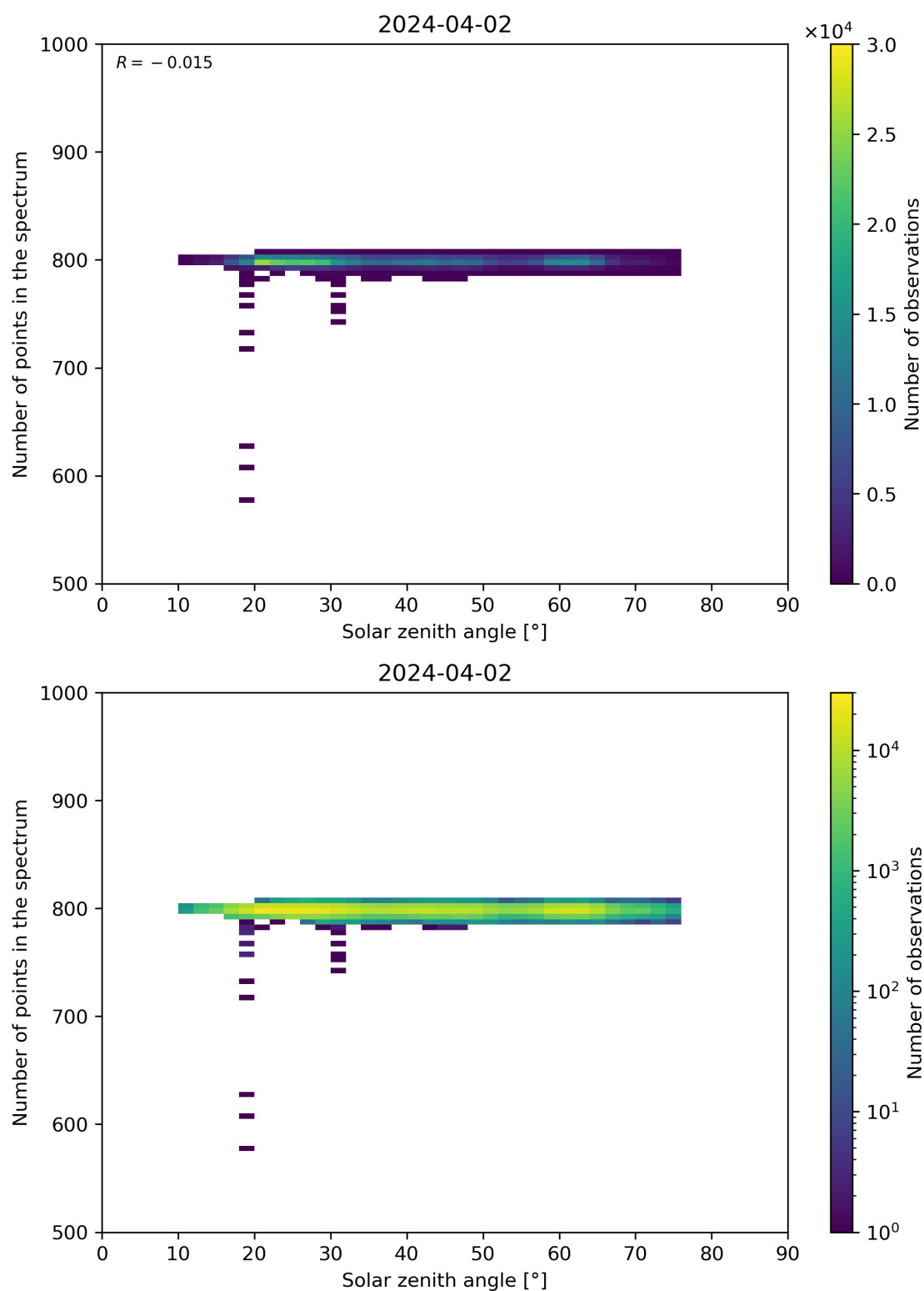
Figure 103: Scatter density plot of “Solar zenith angle” against “Number of points in the spectrum” for 2024-04-01 to 2024-04-03.
