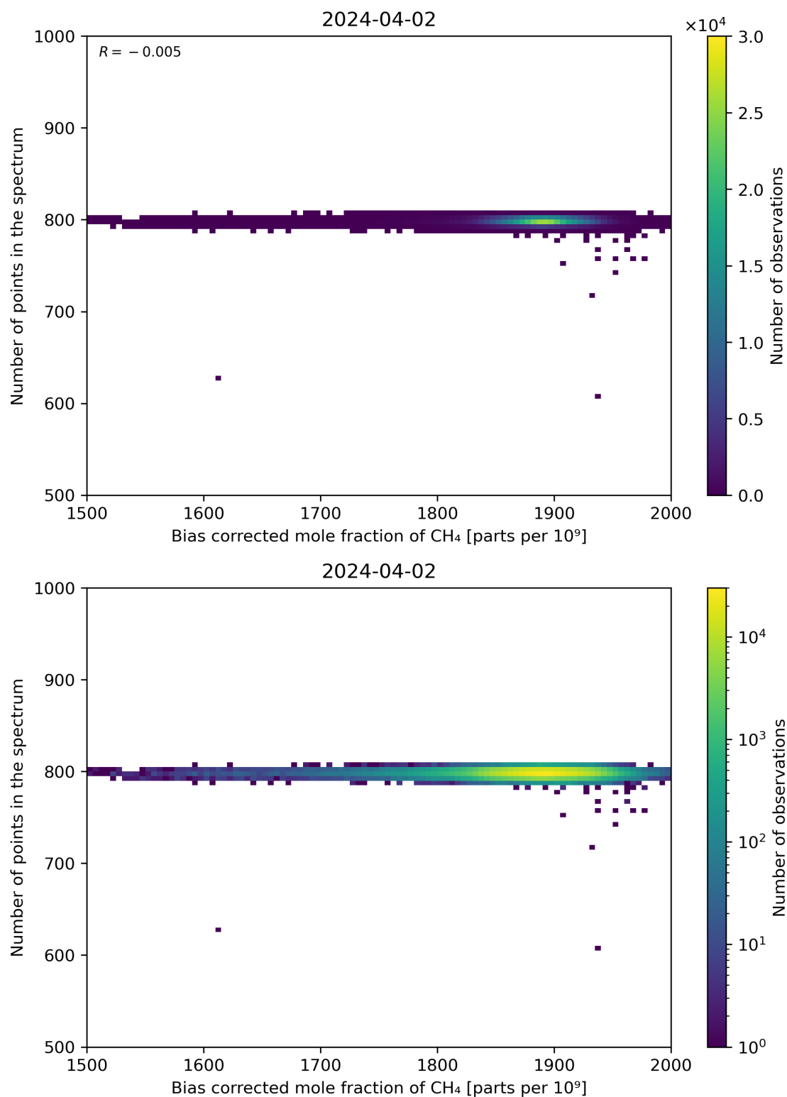
Figure 68: Scatter density plot of “Bias corrected mole fraction of CH 4 ” against “Number of points in the spectrum” for 2024-04-01 to 2024-04-03.
