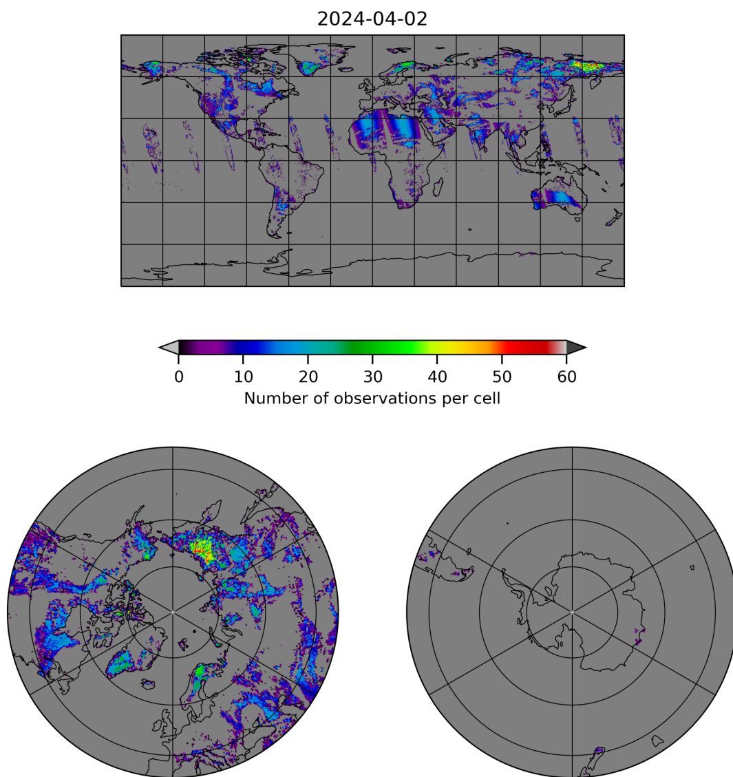
Figure 10: Map of the number of observations for 2024-04-01 to 2024-04-03
