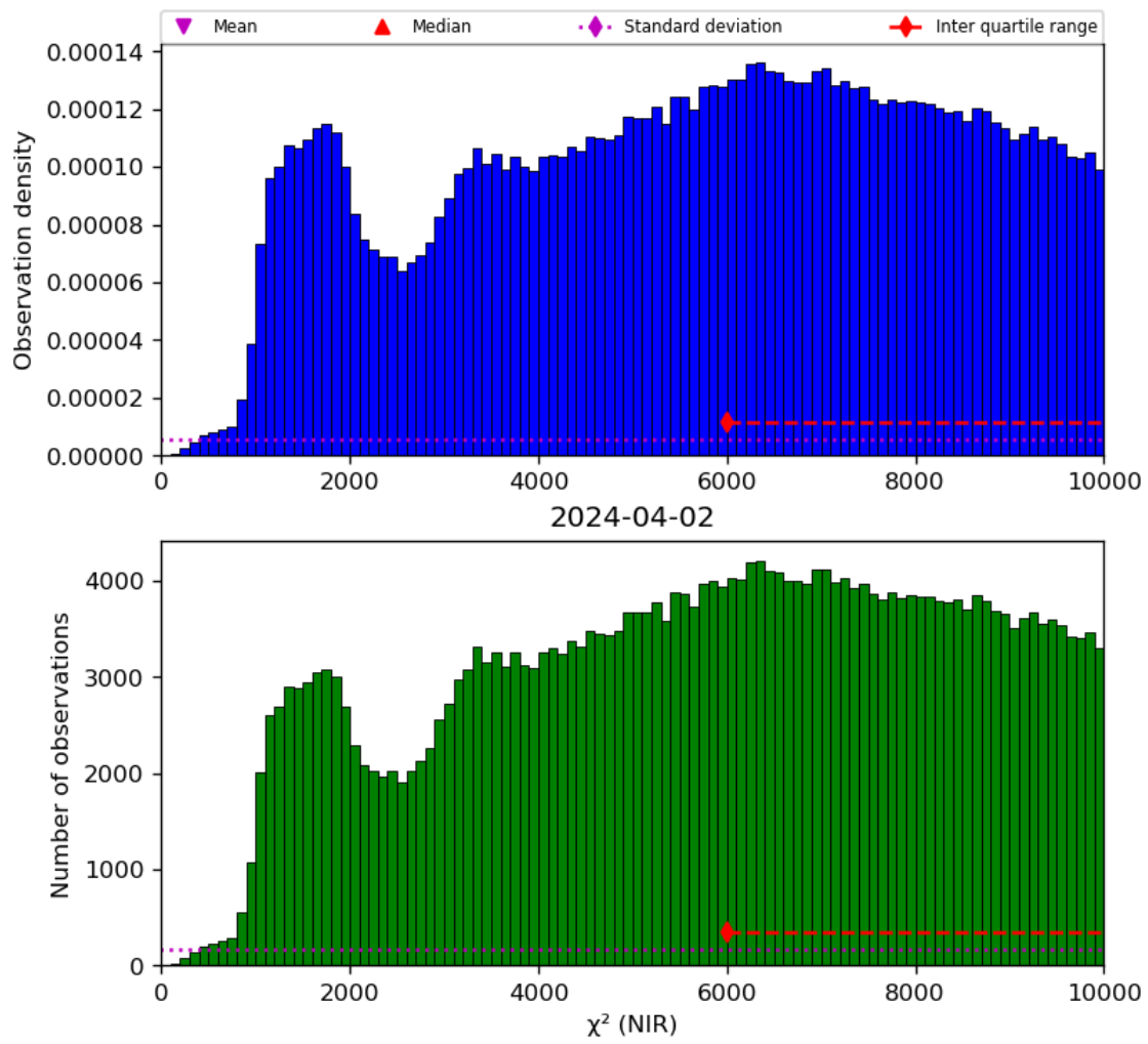
Figure 29: Histogram of “ \chi^2 (NIR)” for 2024-04-01 to 2024-04-03
