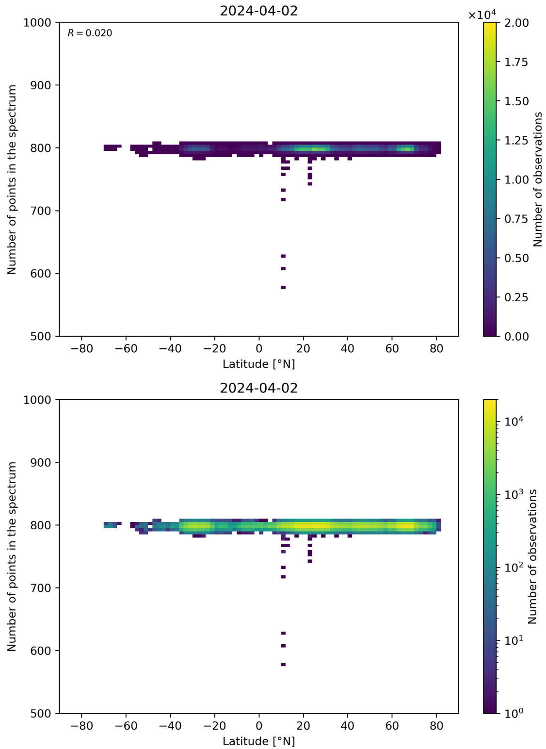
Figure 61: Scatter density plot of “Latitude” against “Number of points in the spectrum” for 2024-04-01 to 2024-04-03.
