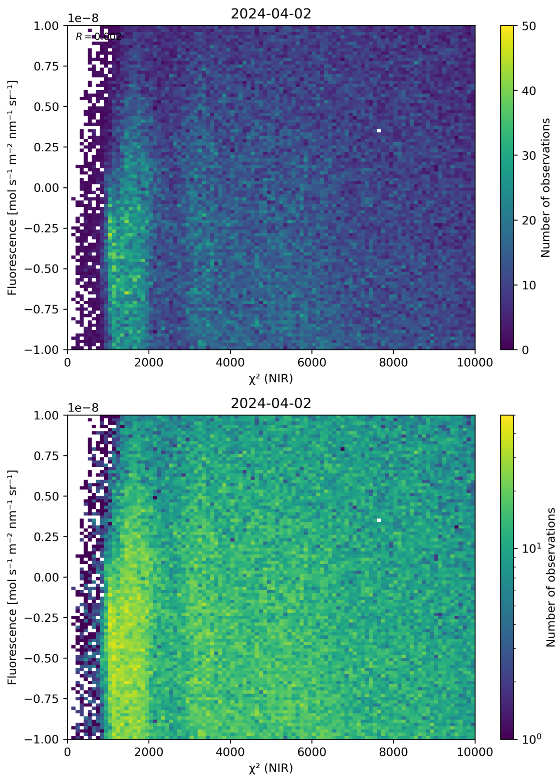
Figure 45: Scatter density plot of “ \chi^2 (NIR)” against “Fluorescence” for 2024-04-01 to 2024-04-03.
