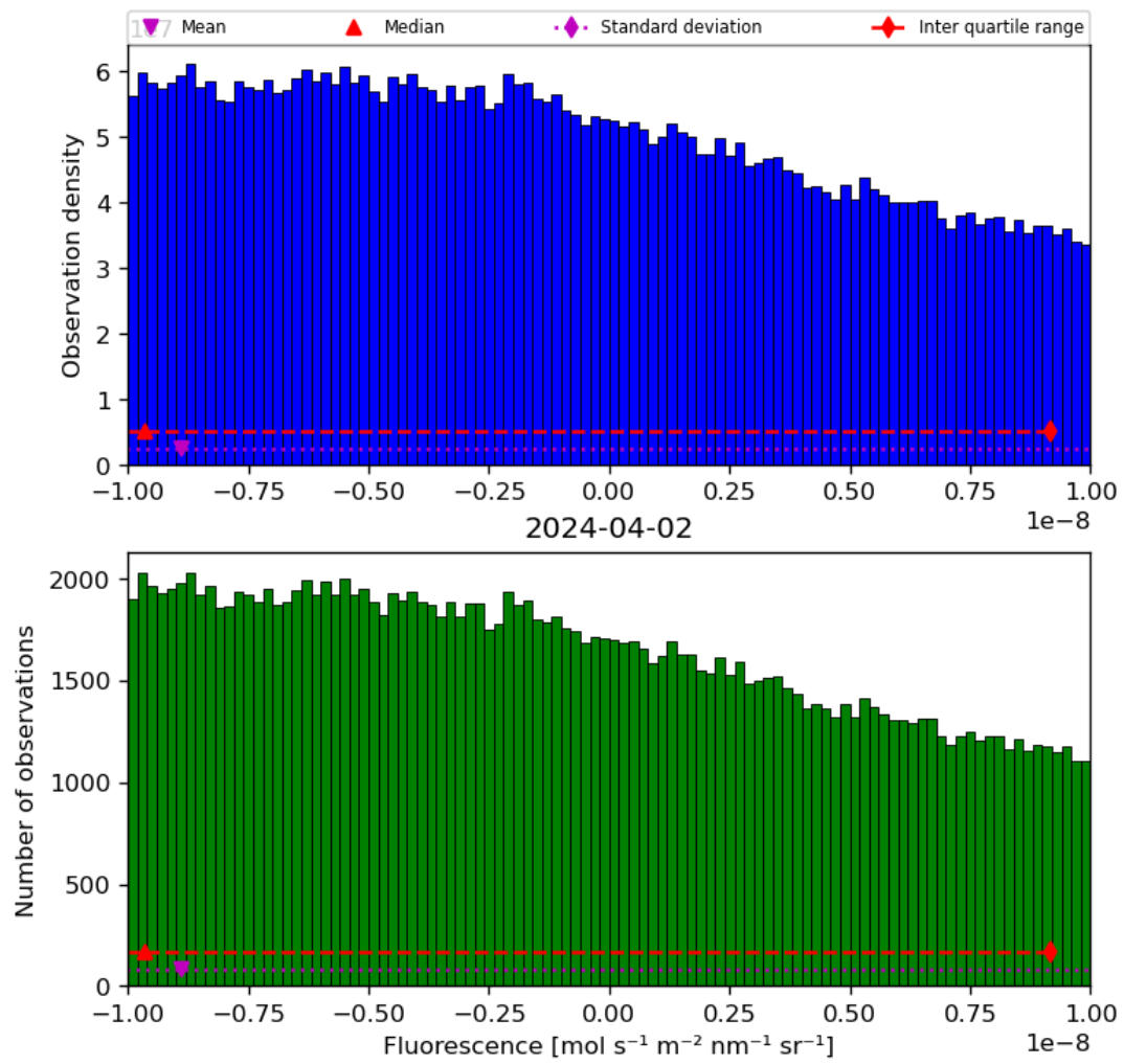
Figure 32: Histogram of “Fluorescence” for 2024-04-01 to 2024-04-03
