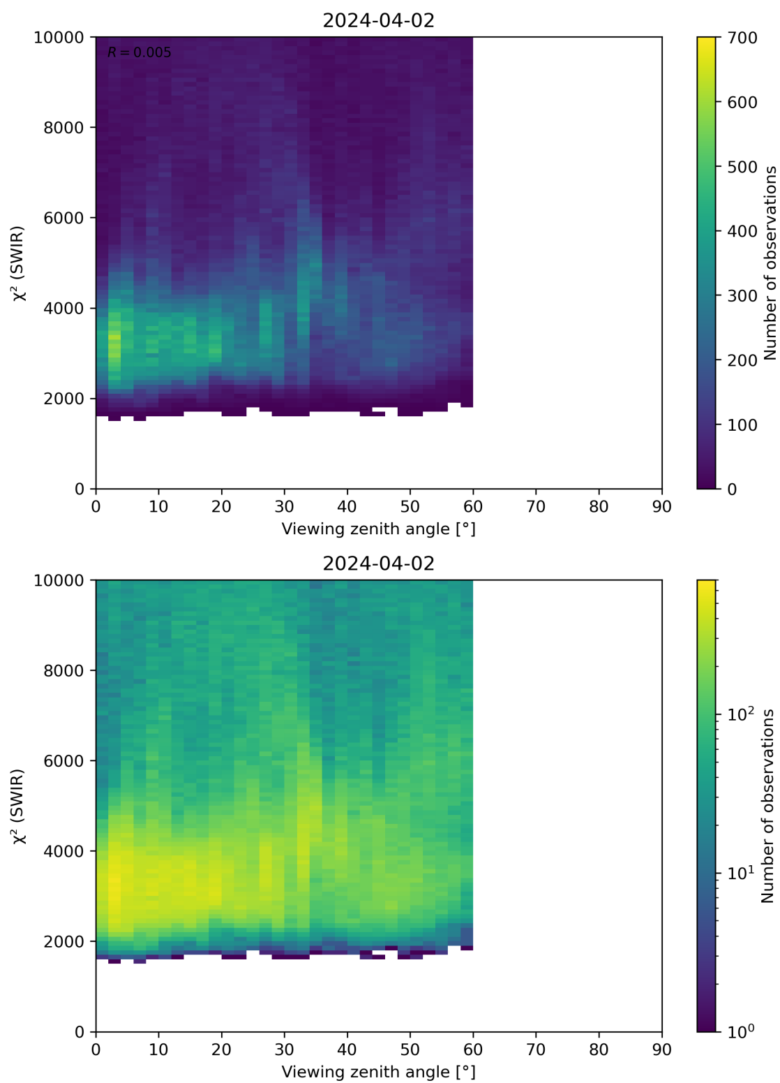
Figure 106: Scatter density plot of “Viewing zenith angle” against “ \chi^2 (SWIR)” for 2024-04-01 to 2024-04-03.
