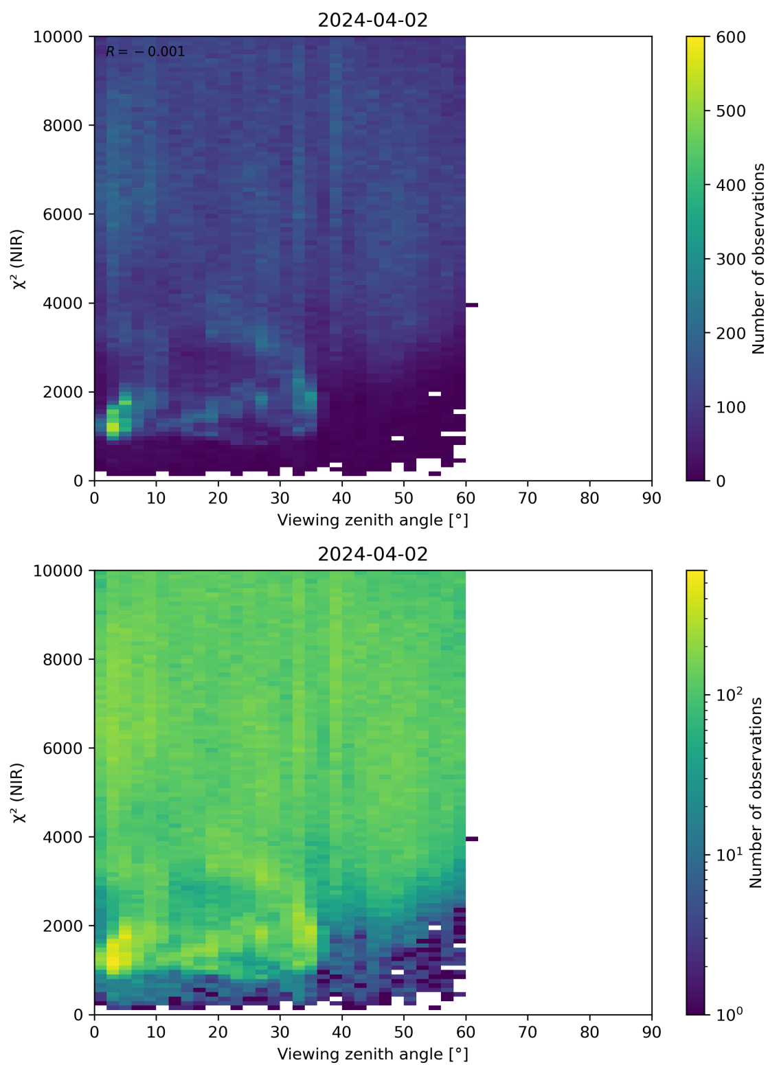
Figure 105: Scatter density plot of “Viewing zenith angle” against “ \chi^2 (NIR)” for 2024-04-01 to 2024-04-03.
