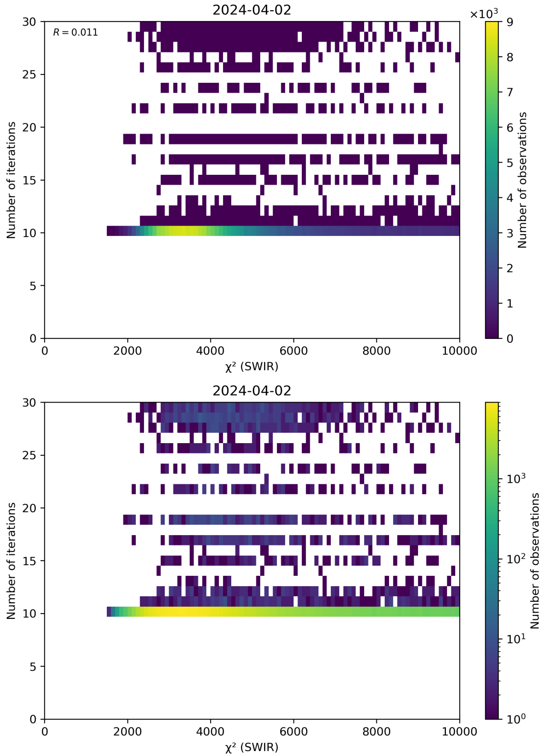
Figure 50: Scatter density plot of “ \chi^2 (SWIR)” against “Number of iterations” for 2024-04-01 to 2024-04-03.
