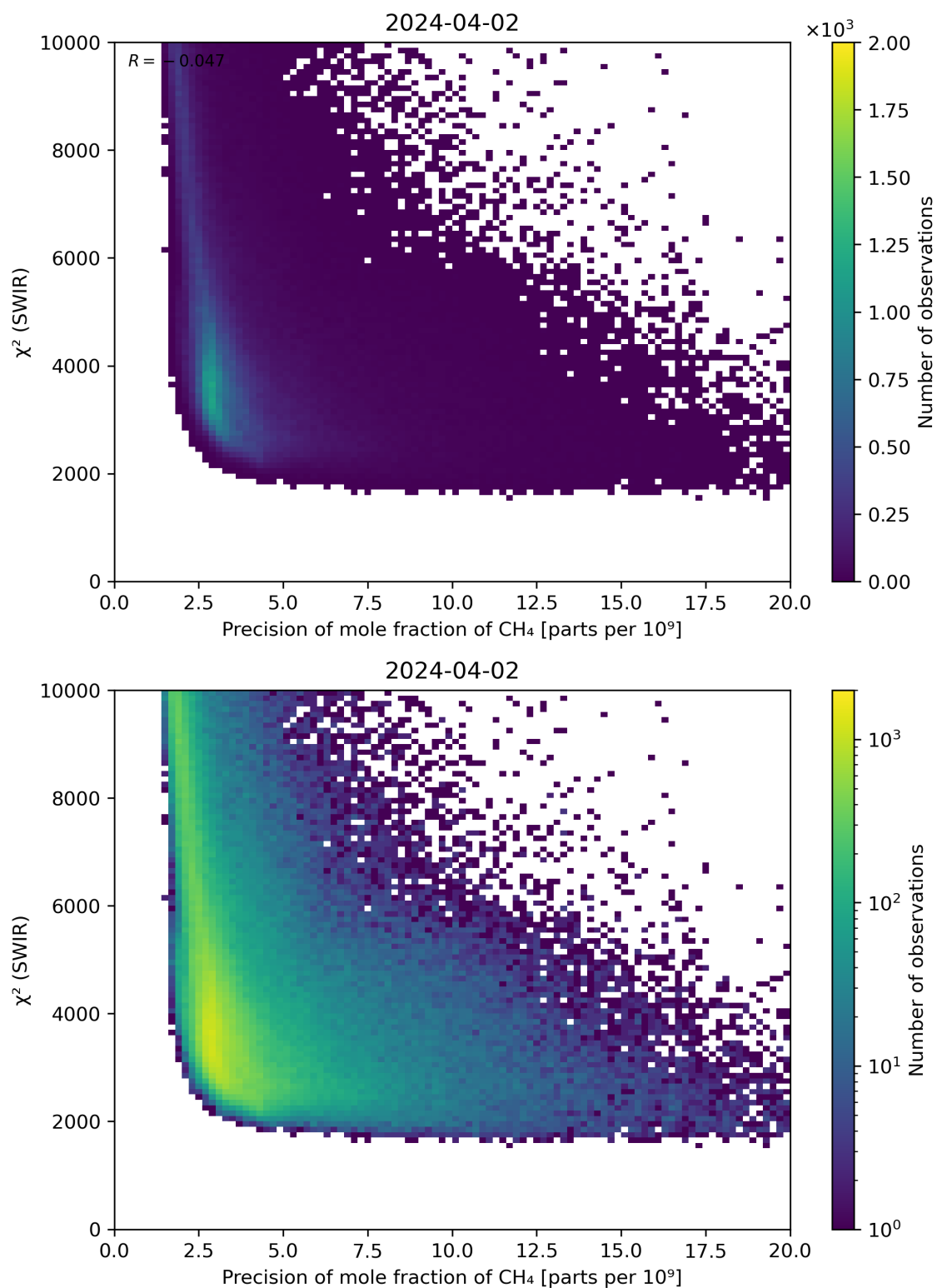
Figure 79: Scatter density plot of “Precision of mole fraction of CH 4 ” against “ \chi^2 (SWIR)” for 2024-04-01 to 2024-04-03.
