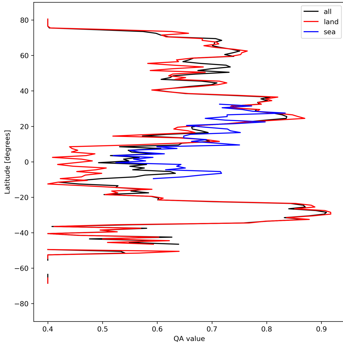
Figure 11: Zonal average of “QA value” for 2024-04-01 to 2024-04-03.
