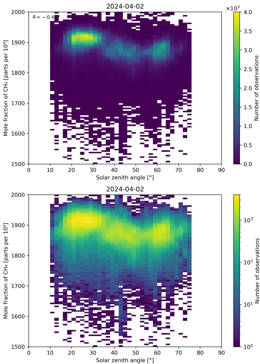
Figure 99: Scatter density plot of “Solar zenith angle” against “Mole fraction of CH 4 ” for 2024-04-01 to 2024-04-03.
