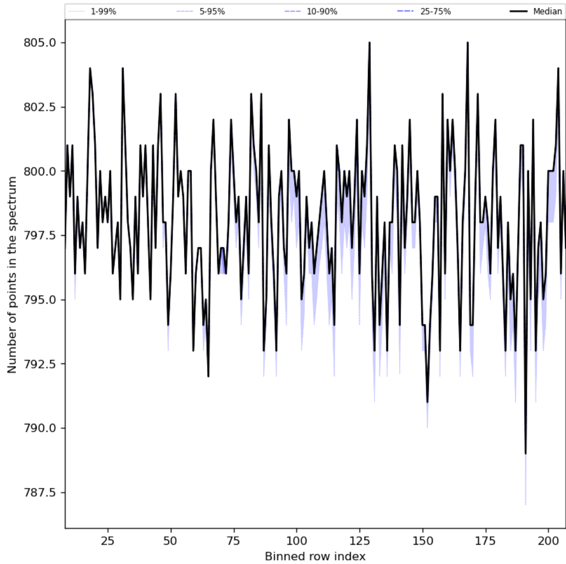
Figure 37: Along track statistics of “Number of points in the spectrum” for 2024-04-01 to 2024-04-03
