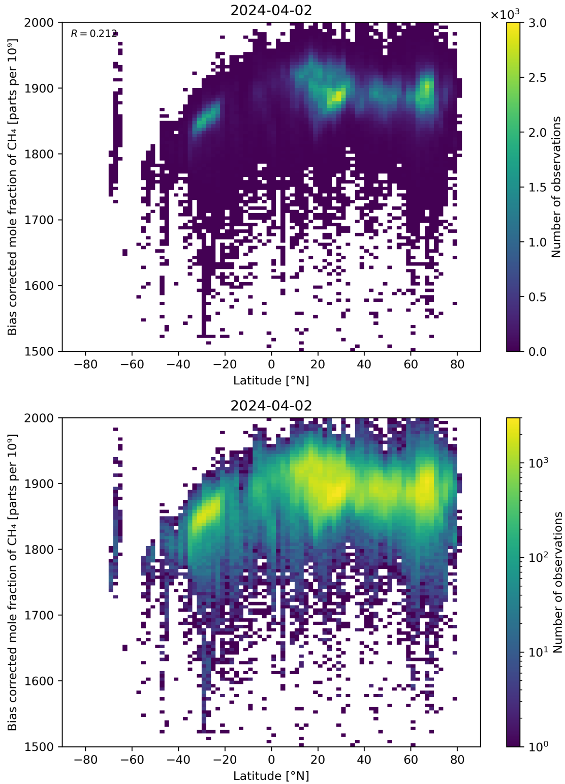
Figure 58: Scatter density plot of “Latitude” against “Bias corrected mole fraction of CH 4 ” for 2024-04-01 to 2024-04-03.
