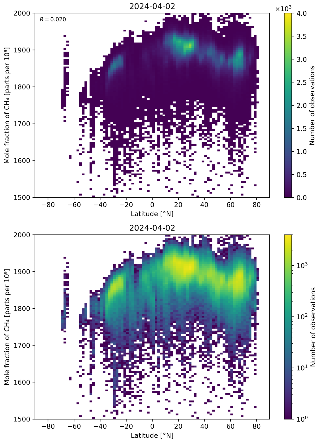
Figure 57: Scatter density plot of “Latitude” against “Mole fraction of \text{CH}_4 ” for 2024-04-01 to 2024-04-03.
