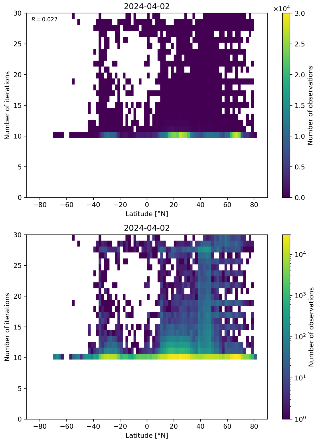
Figure 60: Scatter density plot of “Latitude” against “Number of iterations” for 2024-04-01 to 2024-04-03.
