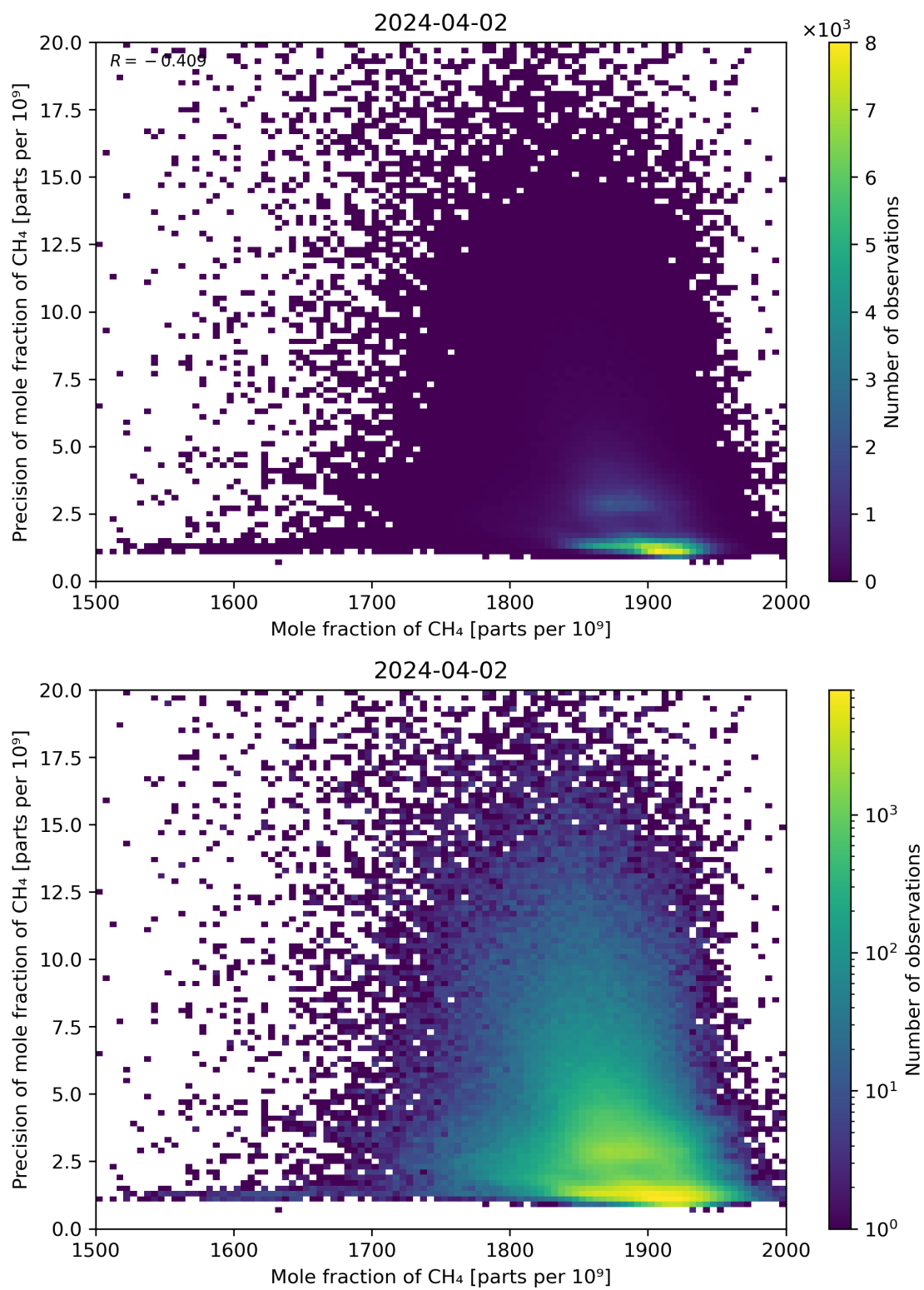
Figure 75: Scatter density plot of “Mole fraction of CH 4 ” against “Precision of mole fraction of CH 4 ” for 2024-04-01 to 2024-04-03.
