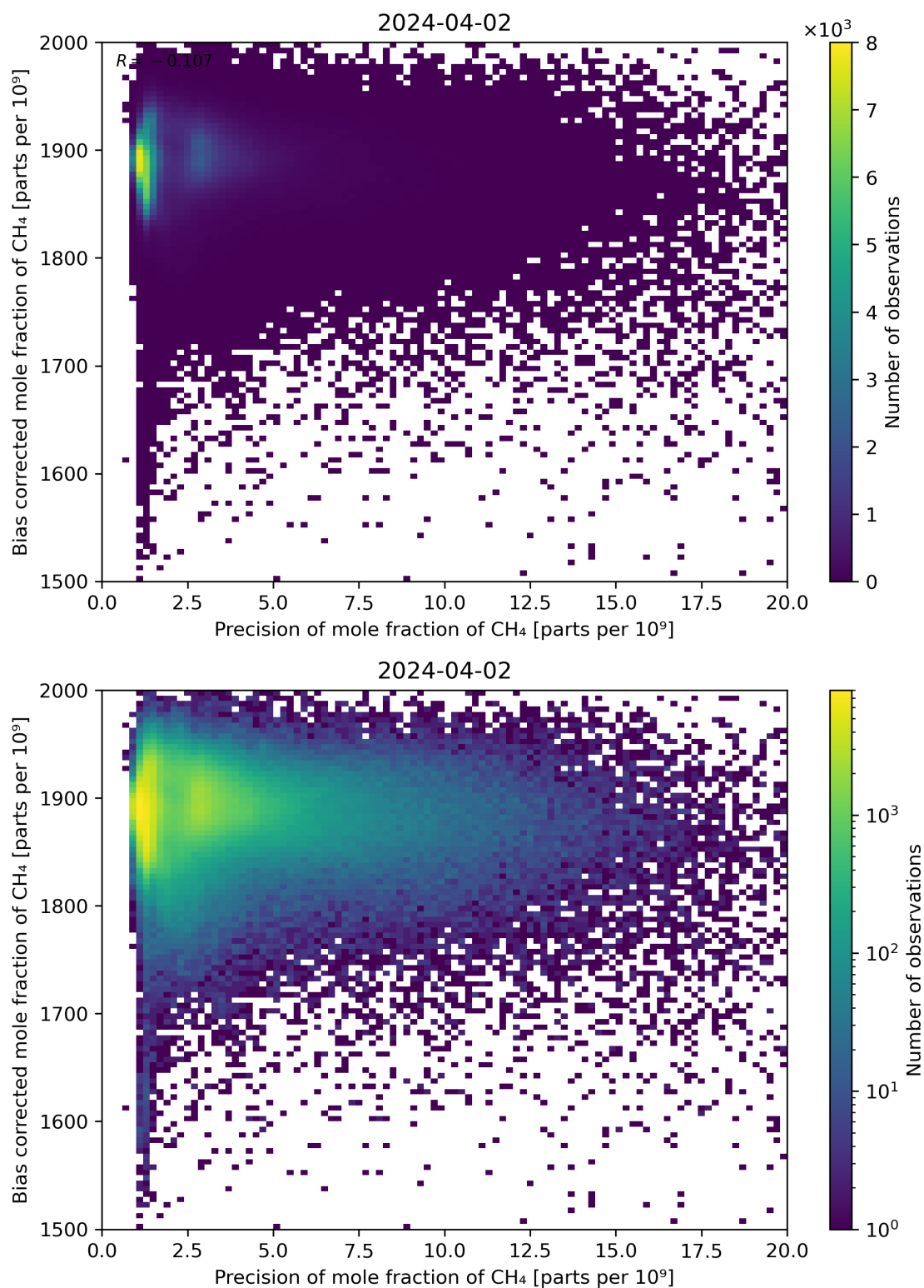
Figure 82: Scatter density plot of “Precision of mole fraction of CH 4 ” against “Bias corrected mole fraction of CH 4 ” for 2024-04-01 to 2024-04-03.
