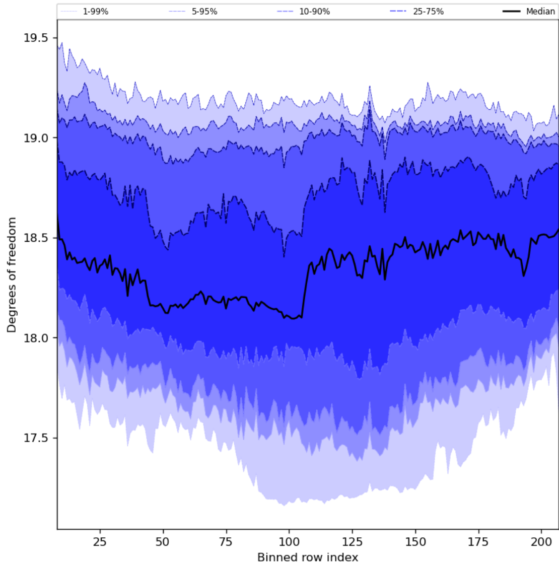
Figure 41: Along track statistics of “Degrees of freedom” for 2024-04-01 to 2024-04-03
