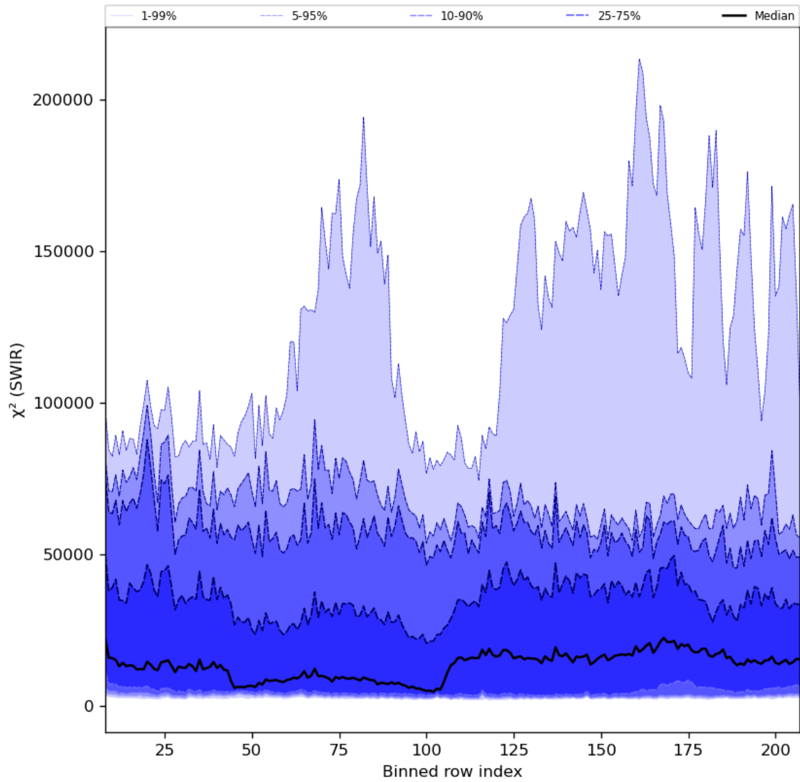
Figure 39: Along track statistics of “ \chi^2 (SWIR)” for 2024-04-01 to 2024-04-03
