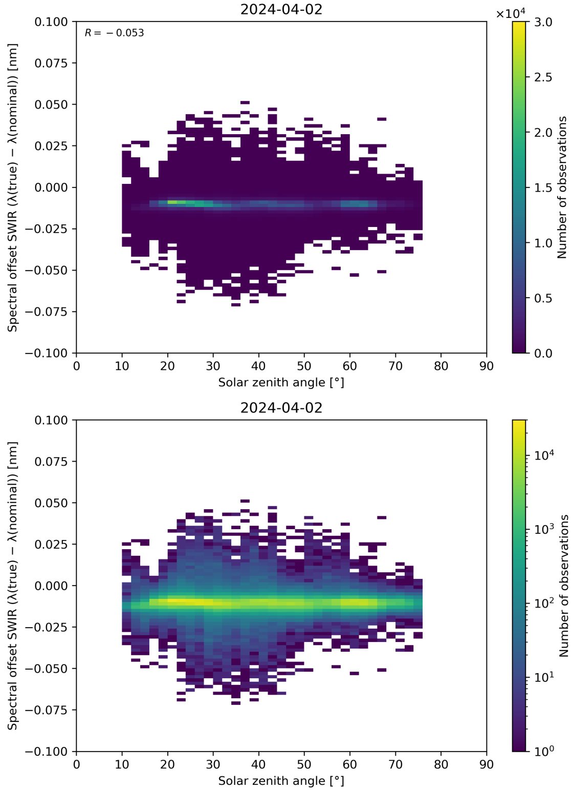
Figure 104: Scatter density plot of “Solar zenith angle” against “Spectral offset SWIR ( \lambda(\text{true}) - \lambda(\text{nominal}) )” for 2024-04-01 to 2024-04-03.
