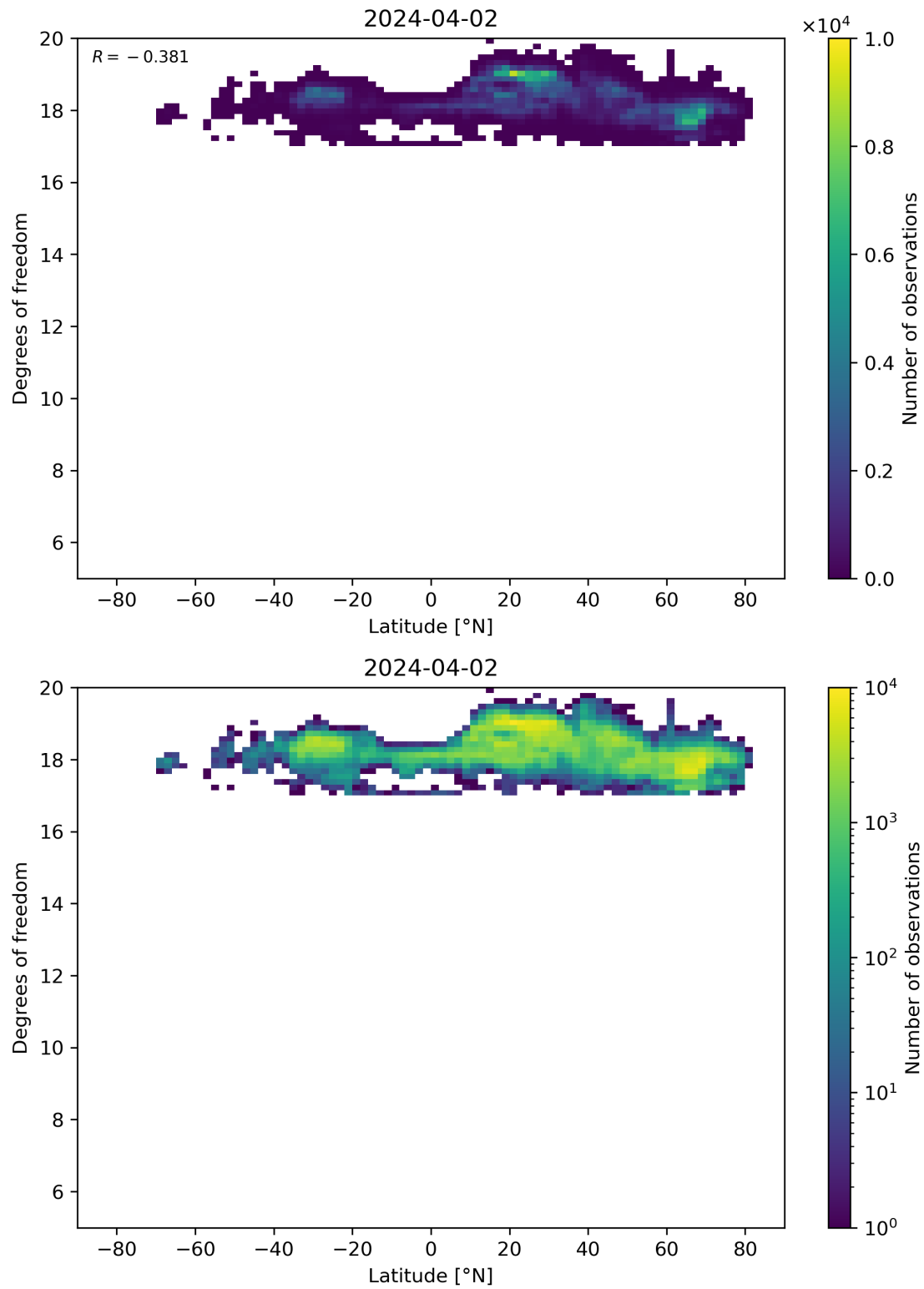
Figure 55: Scatter density plot of “Latitude” against “Degrees of freedom” for 2024-04-01 to 2024-04-03.
