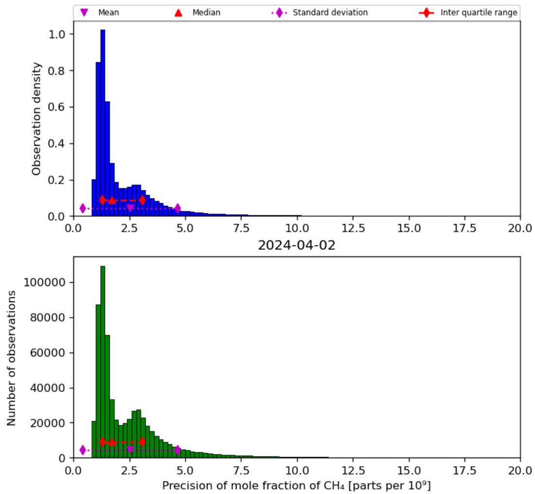
Figure 24: Histogram of “Precision of mole fraction of CH 4 ” for 2024-04-01 to 2024-04-03
