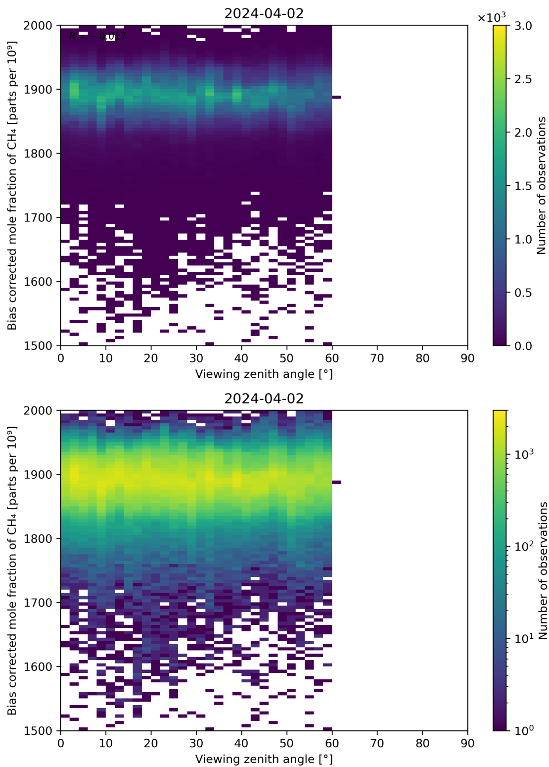
Figure 111: Scatter density plot of “Viewing zenith angle” against “Bias corrected mole fraction of CH 4 ” for 2024-04-01 to 2024-04-03.
