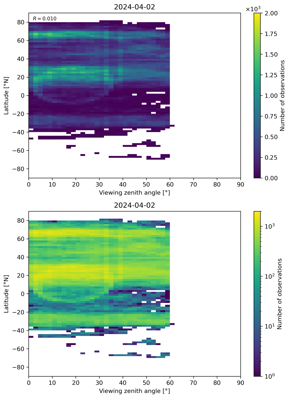
Figure 109: Scatter density plot of “Viewing zenith angle” against “Latitude” for 2024-04-01 to 2024-04-03.
