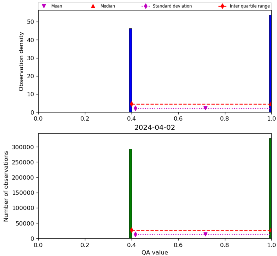
Figure 22: Histogram of “QA value” for 2024-04-01 to 2024-04-03
