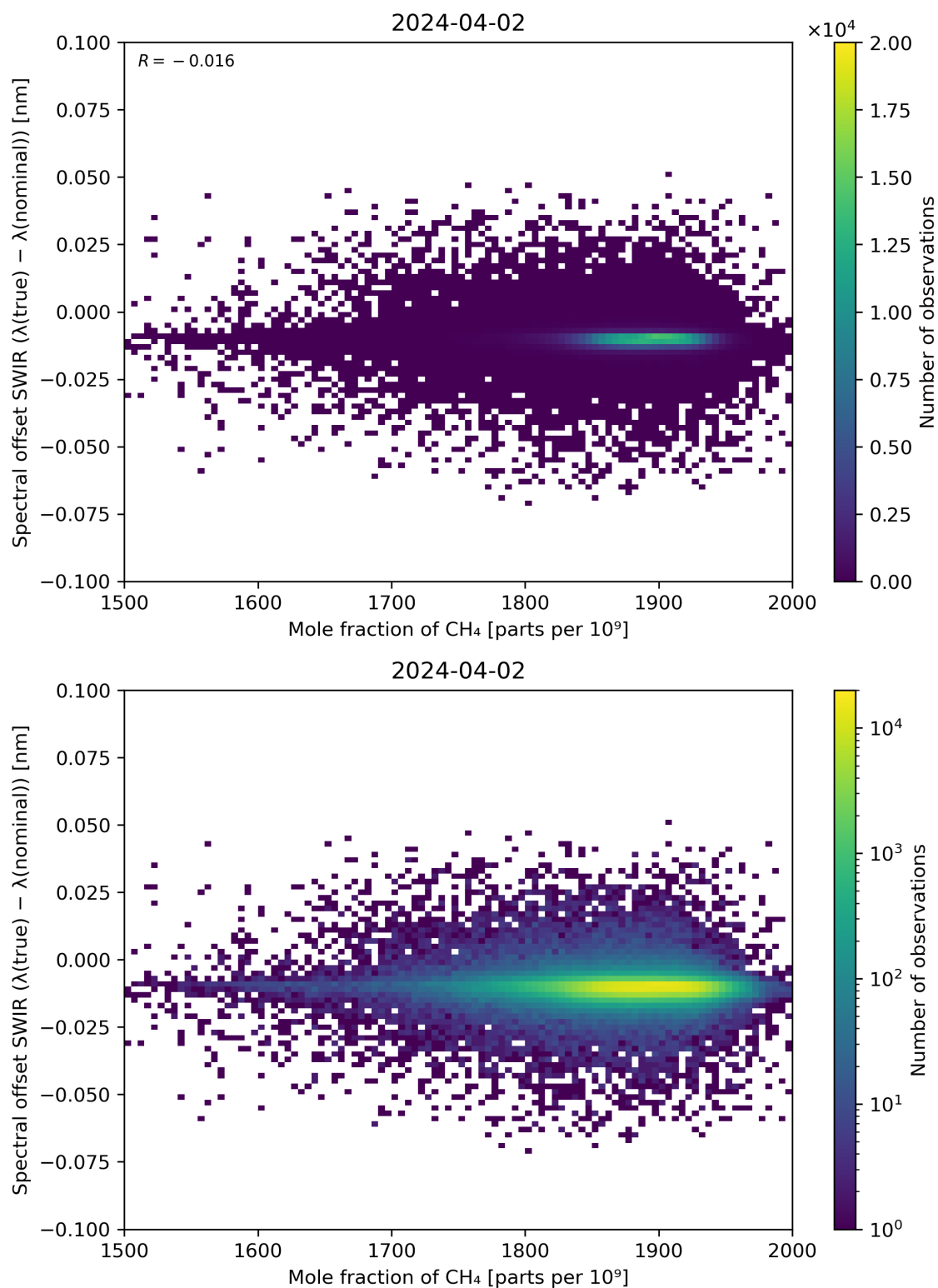
Figure 86: Scatter density plot of “Mole fraction of CH 4 ” against “Spectral offset SWIR ( \lambda(\text{true}) - \lambda(\text{nominal}) )” for 2024-04-01 to 2024-04-03.
