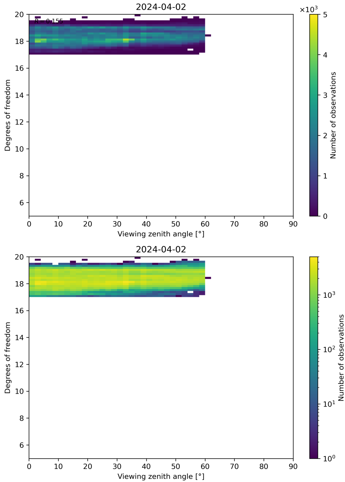
Figure 107: Scatter density plot of “Viewing zenith angle” against “Degrees of freedom” for 2024-04-01 to 2024-04-03.
