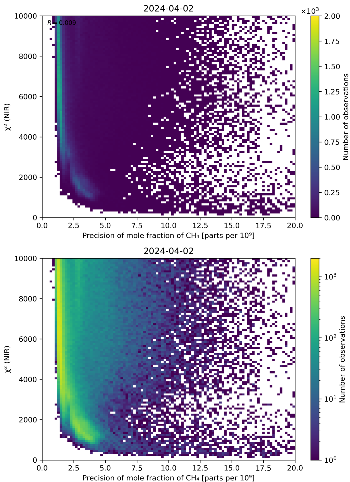
Figure 78: Scatter density plot of “Precision of mole fraction of CH 4 ” against “ \chi^2 (NIR)” for 2024-04-01 to 2024-04-03.
