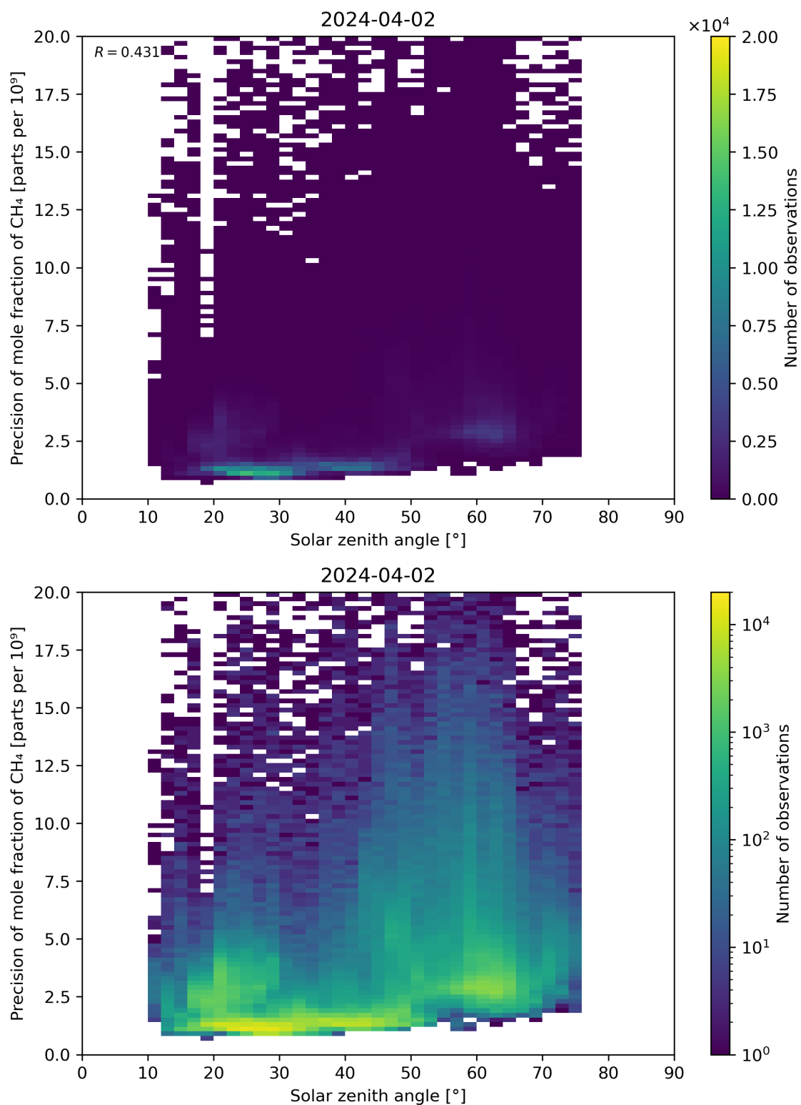
Figure 101: Scatter density plot of “Solar zenith angle” against “Precision of mole fraction of CH 4 ” for 2024-04-01 to 2024-04-03.
