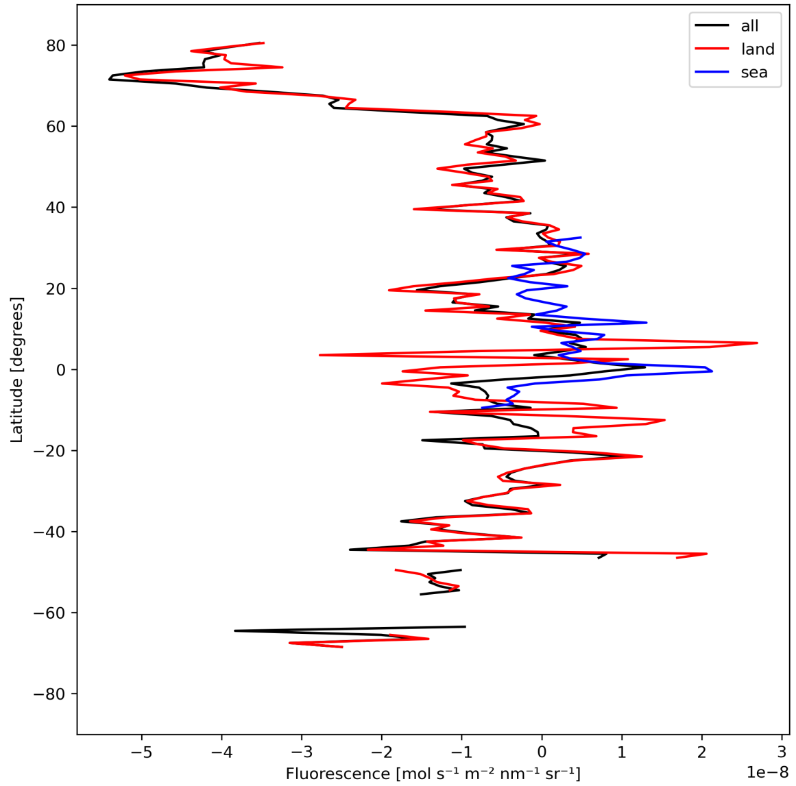
Figure 21: Zonal average of “Fluorescence” for 2024-04-01 to 2024-04-03.
