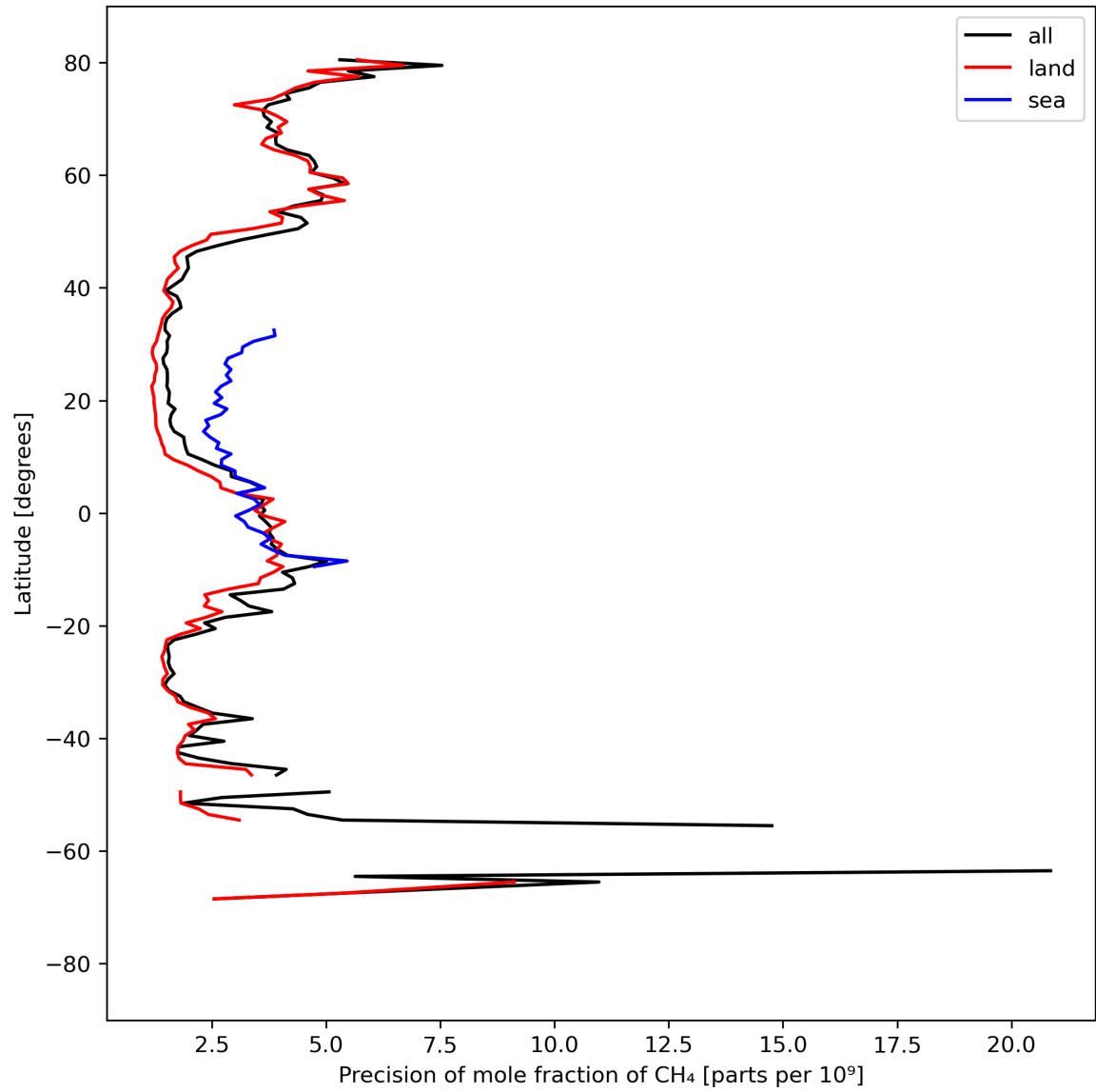
Figure 13: Zonal average of “Precision of mole fraction of CH 4 ” for 2024-04-01 to 2024-04-03.
