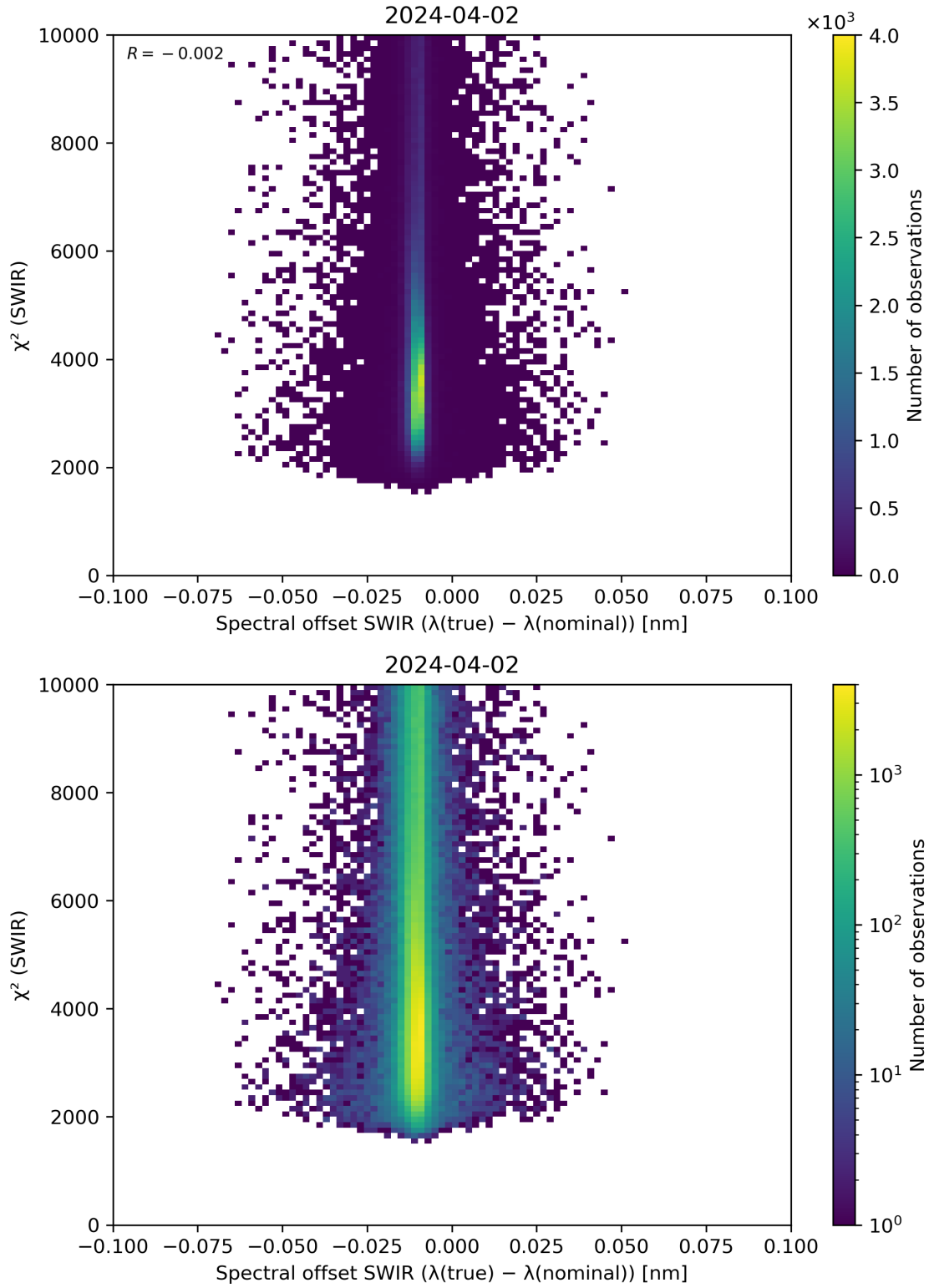
Figure 118: Scatter density plot of “Spectral offset SWIR ( \lambda(\text{true}) - \lambda(\text{nominal}) )” against “ \chi^2 (SWIR)” for 2024-04-01 to 2024-04-03.
