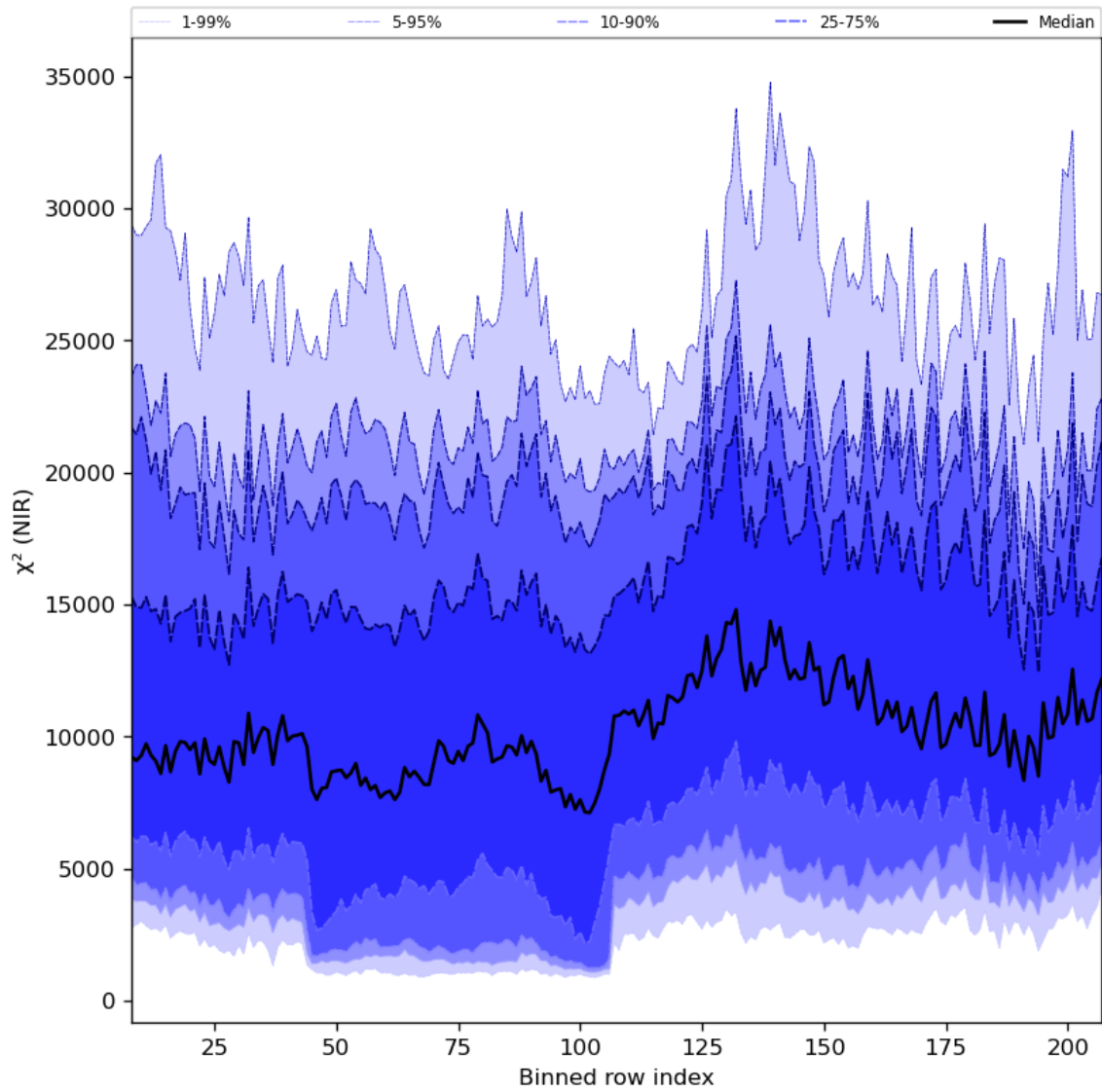
Figure 40: Along track statistics of “ \chi^2 (NIR)” for 2024-04-01 to 2024-04-03
