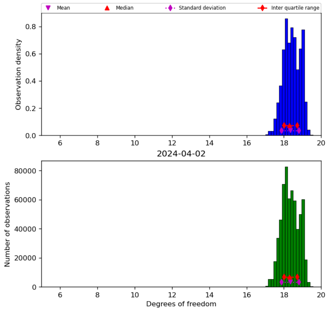
Figure 30: Histogram of “Degrees of freedom” for 2024-04-01 to 2024-04-03
