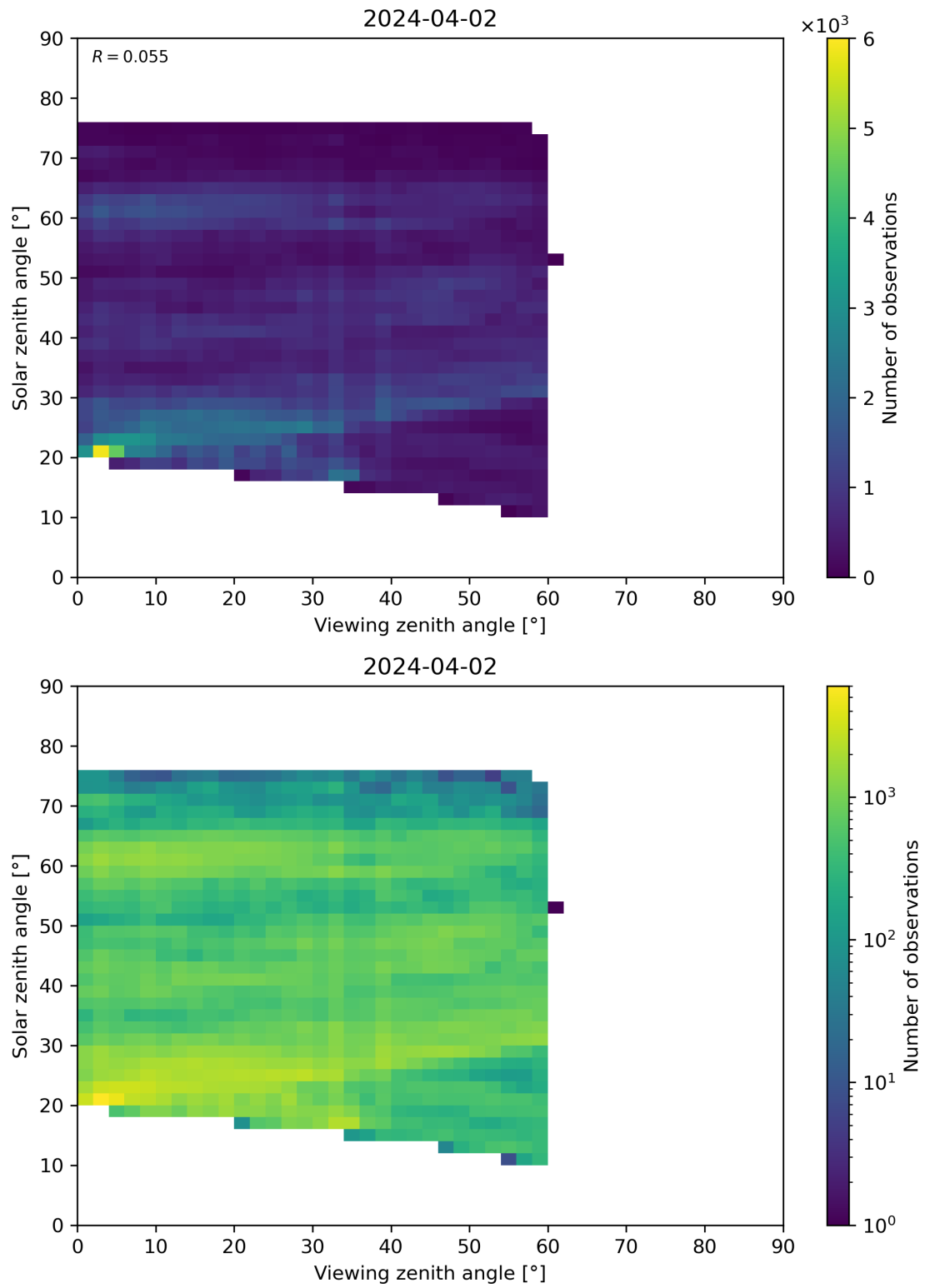
Figure 115: Scatter density plot of “Viewing zenith angle” against “Solar zenith angle” for 2024-04-01 to 2024-04-03.
