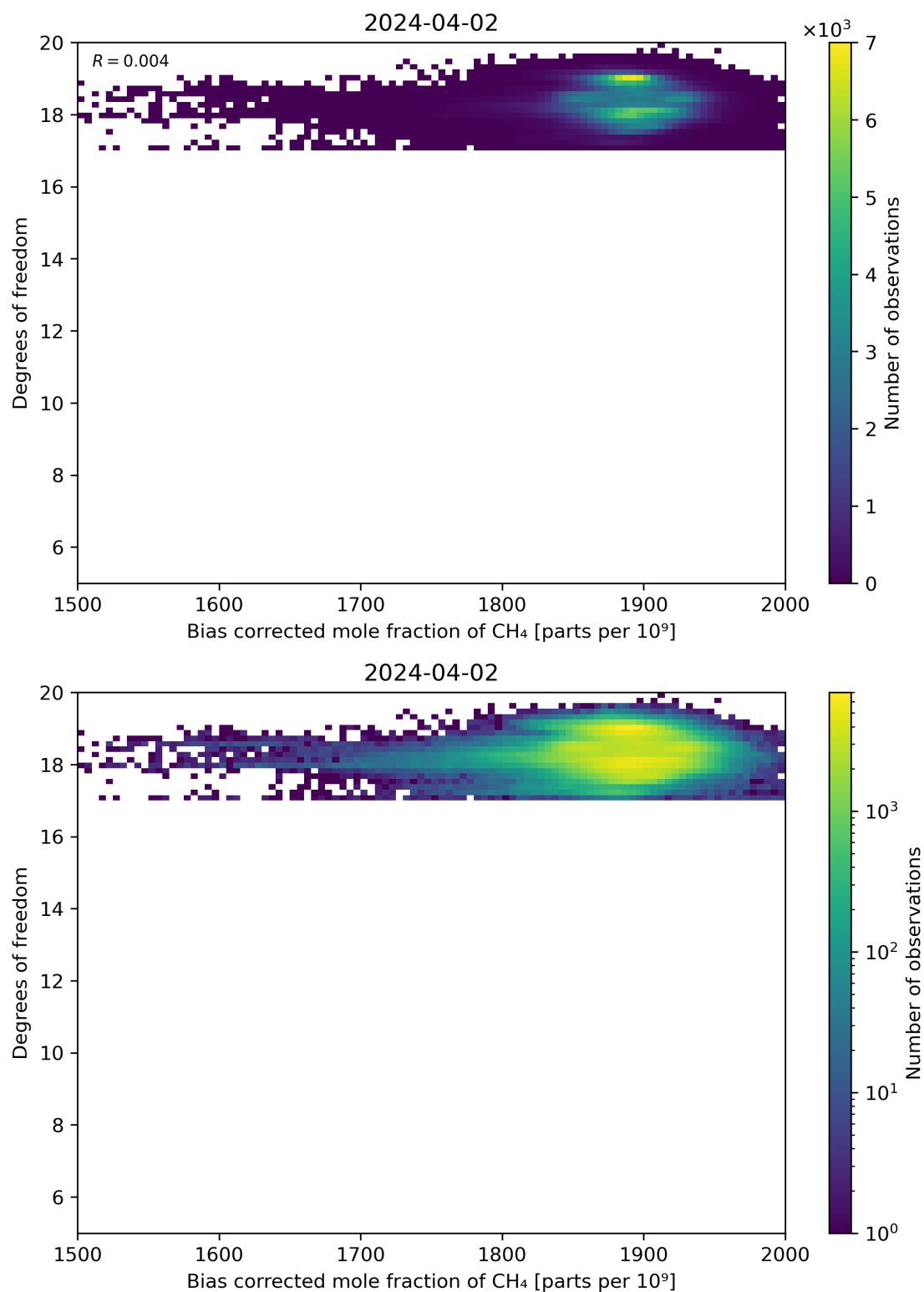
Figure 65: Scatter density plot of “Bias corrected mole fraction of CH 4 ” against “Degrees of freedom” for 2024-04-01 to 2024-04-03.
