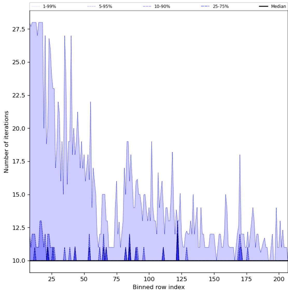
Figure 42: Along track statistics of “Number of iterations” for 2024-04-01 to 2024-04-03
