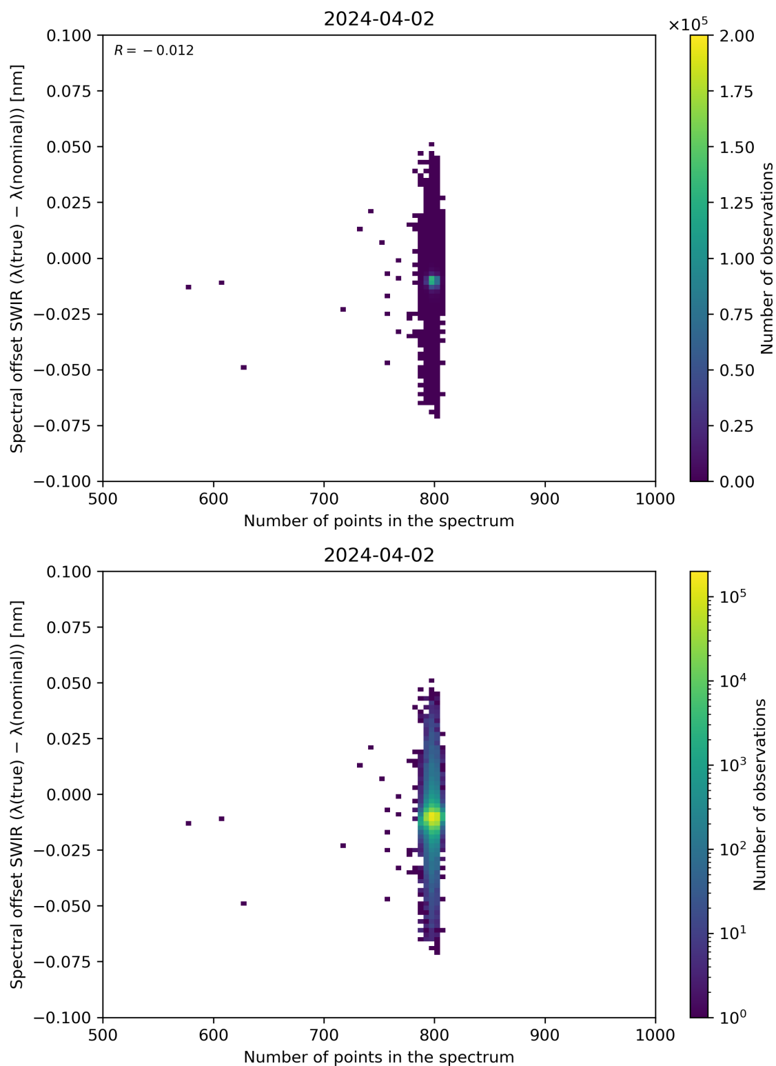
Figure 93: Scatter density plot of “Number of points in the spectrum” against “Spectral offset SWIR ( \lambda(\text{true}) - \lambda(\text{nominal}) )” for 2024-04-01 to 2024-04-03.
