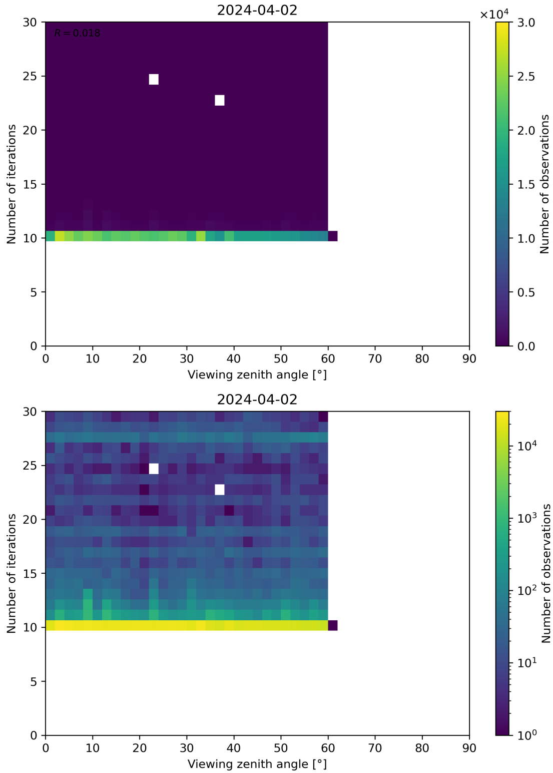
Figure 113: Scatter density plot of “Viewing zenith angle” against “Number of iterations” for 2024-04-01 to 2024-04-03.
