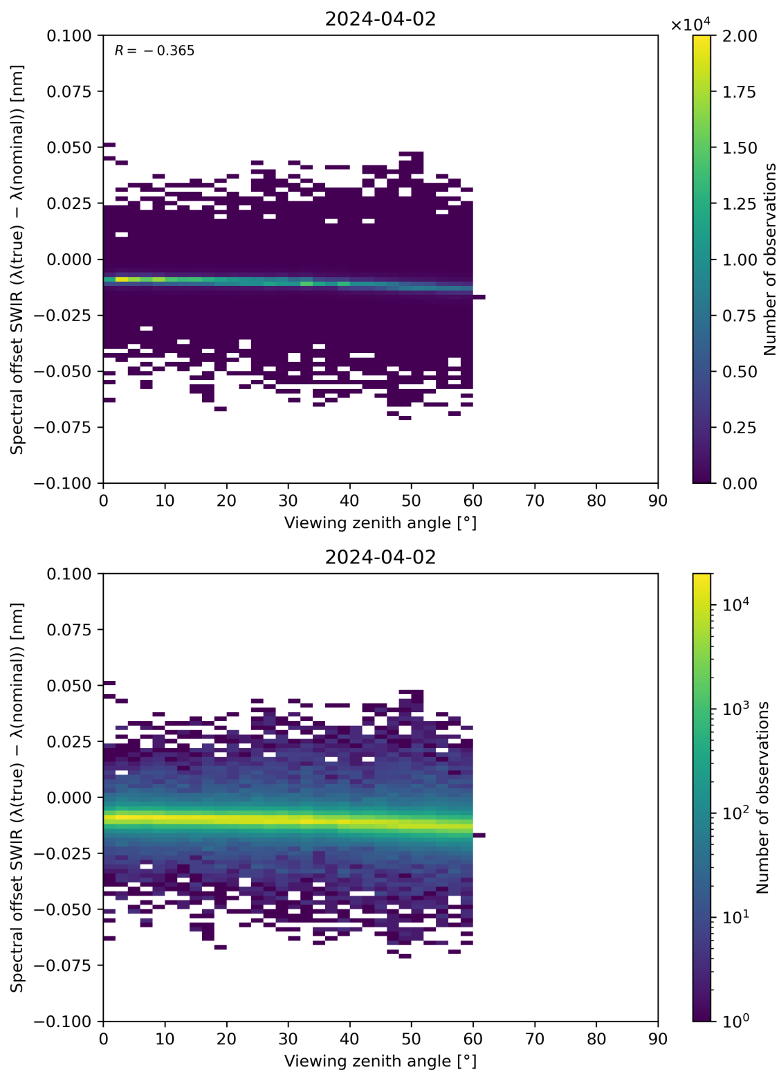
Figure 116: Scatter density plot of “Viewing zenith angle” against “Spectral offset SWIR ( \lambda(\text{true}) - \lambda(\text{nominal}) )” for 2024-04-01 to 2024-04-03.
