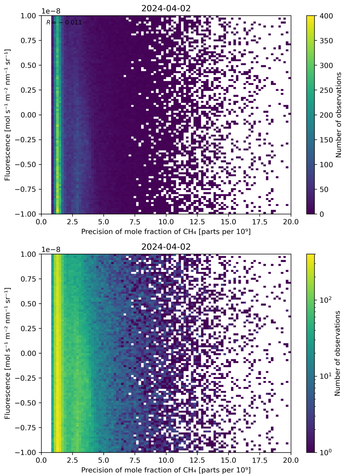
Figure 81: Scatter density plot of “Precision of mole fraction of \text{CH}_4 ” against “Fluorescence” for 2024-04-01 to 2024-04-03.
