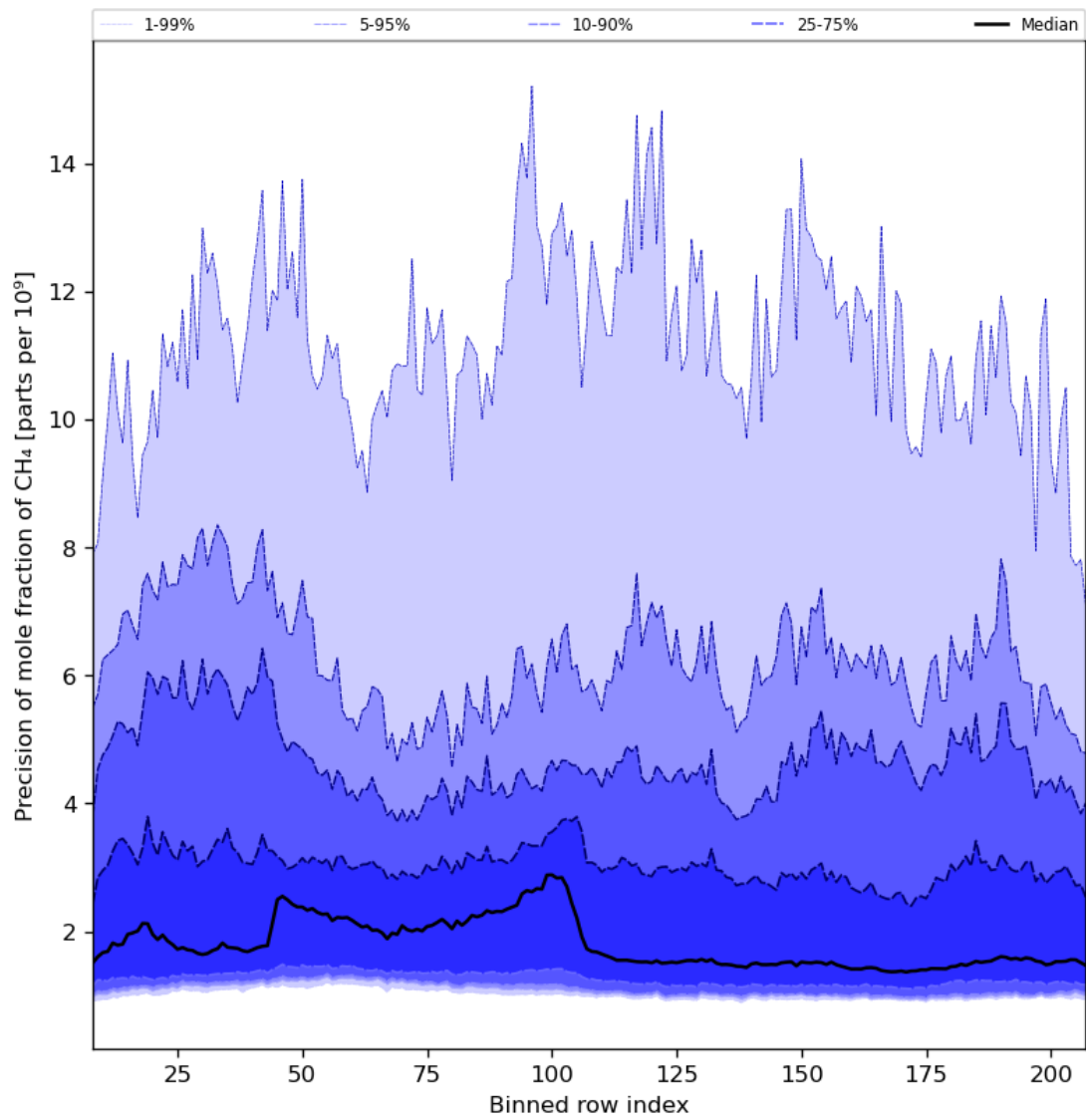
Figure 35: Along track statistics of “Precision of mole fraction of CH 4 ” for 2024-04-01 to 2024-04-03
