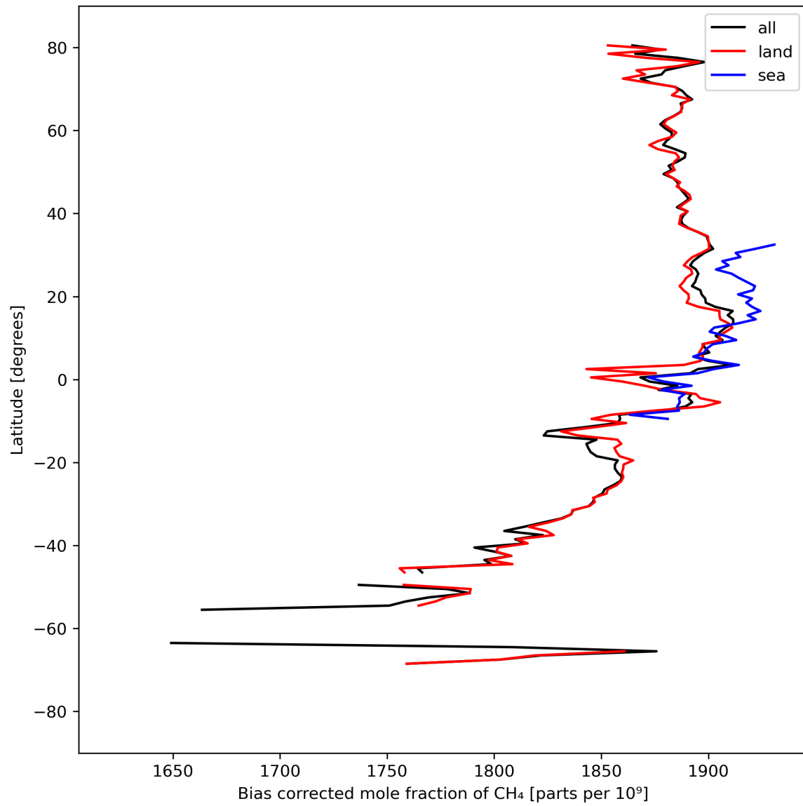
Figure 14: Zonal average of “Bias corrected mole fraction of CH 4 ” for 2024-04-01 to 2024-04-03.
