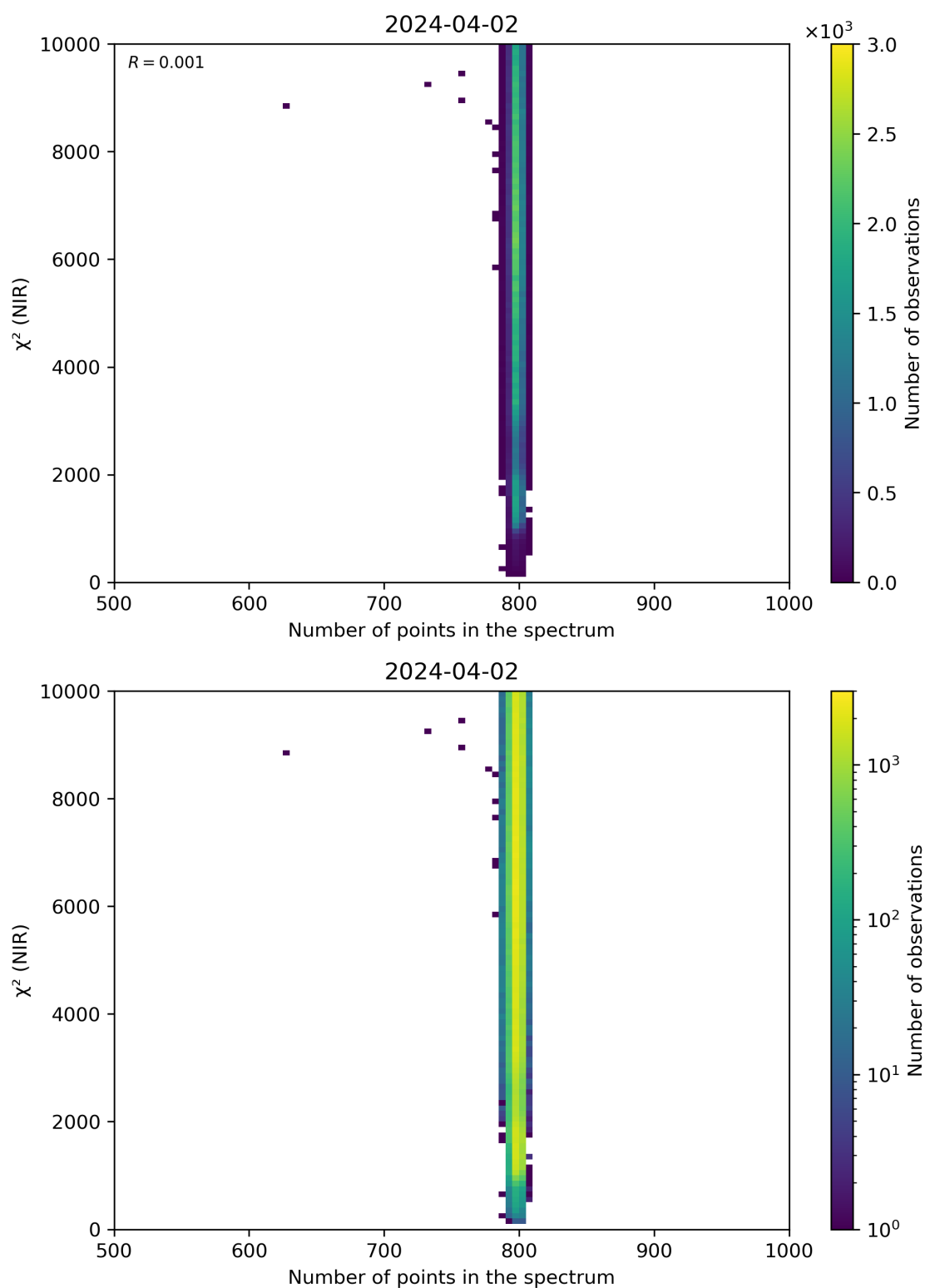
Figure 88: Scatter density plot of “Number of points in the spectrum” against “ \chi^2 (NIR)” for 2024-04-01 to 2024-04-03.
