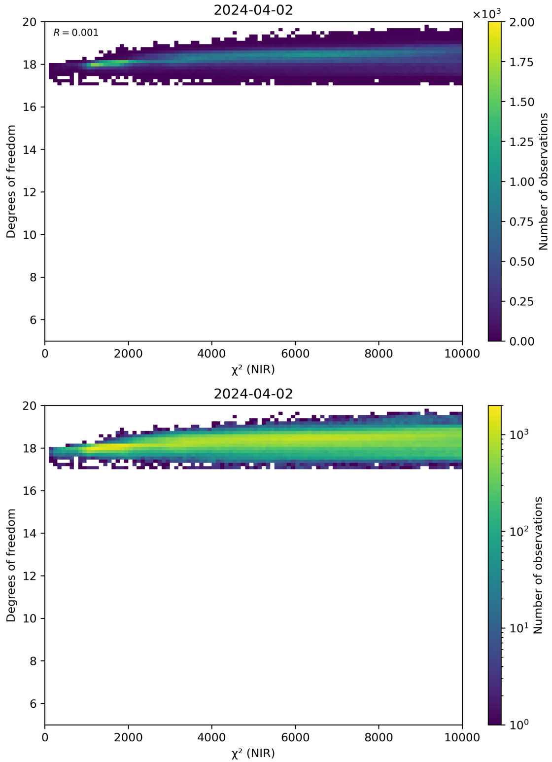
Figure 44: Scatter density plot of “ \chi^2 (NIR)” against “Degrees of freedom” for 2024-04-01 to 2024-04-03.
