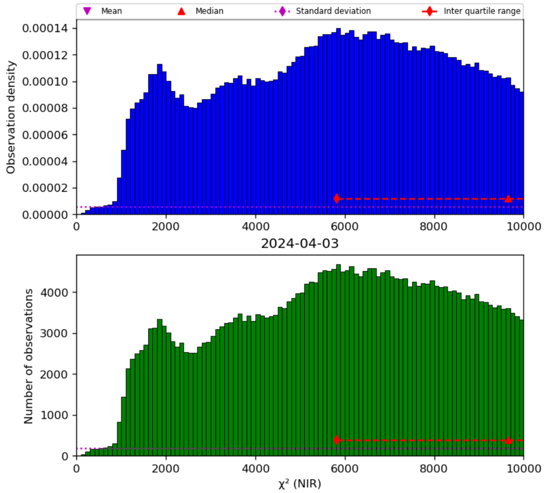
Figure 29: Histogram of “ \chi^2 (NIR)” for 2024-04-02 to 2024-04-04
