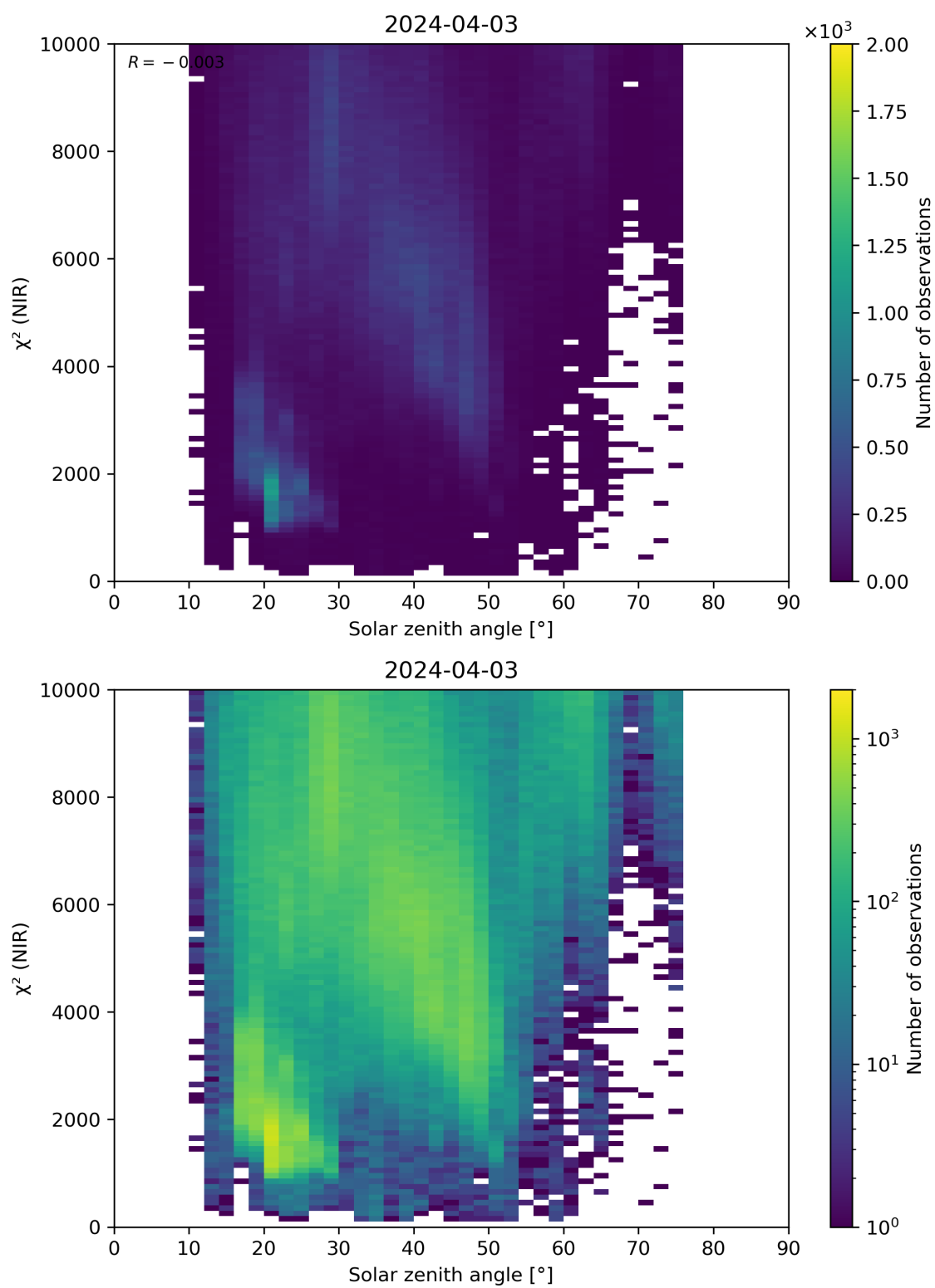
Figure 94: Scatter density plot of “Solar zenith angle” against “ \chi^2 (NIR)” for 2024-04-02 to 2024-04-04.
