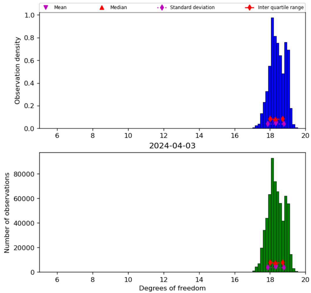
Figure 30: Histogram of “Degrees of freedom” for 2024-04-02 to 2024-04-04
