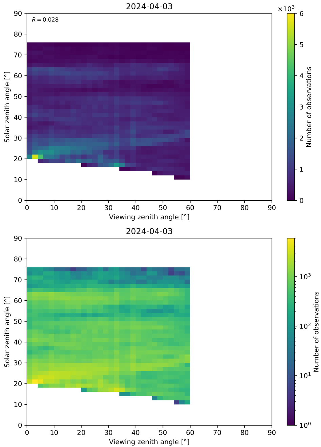
Figure 115: Scatter density plot of “Viewing zenith angle” against “Solar zenith angle” for 2024-04-02 to 2024-04-04.
