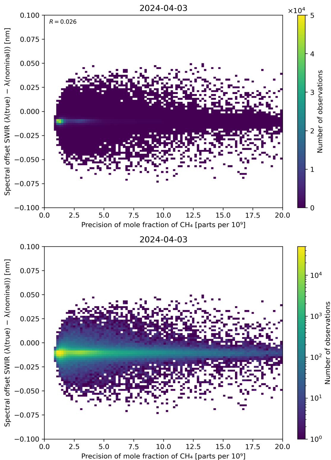
Figure 85: Scatter density plot of “Precision of mole fraction of CH 4 ” against “Spectral offset SWIR ( \lambda(\text{true}) - \lambda(\text{nominal}) )” for 2024-04-02 to 2024-04-04.
