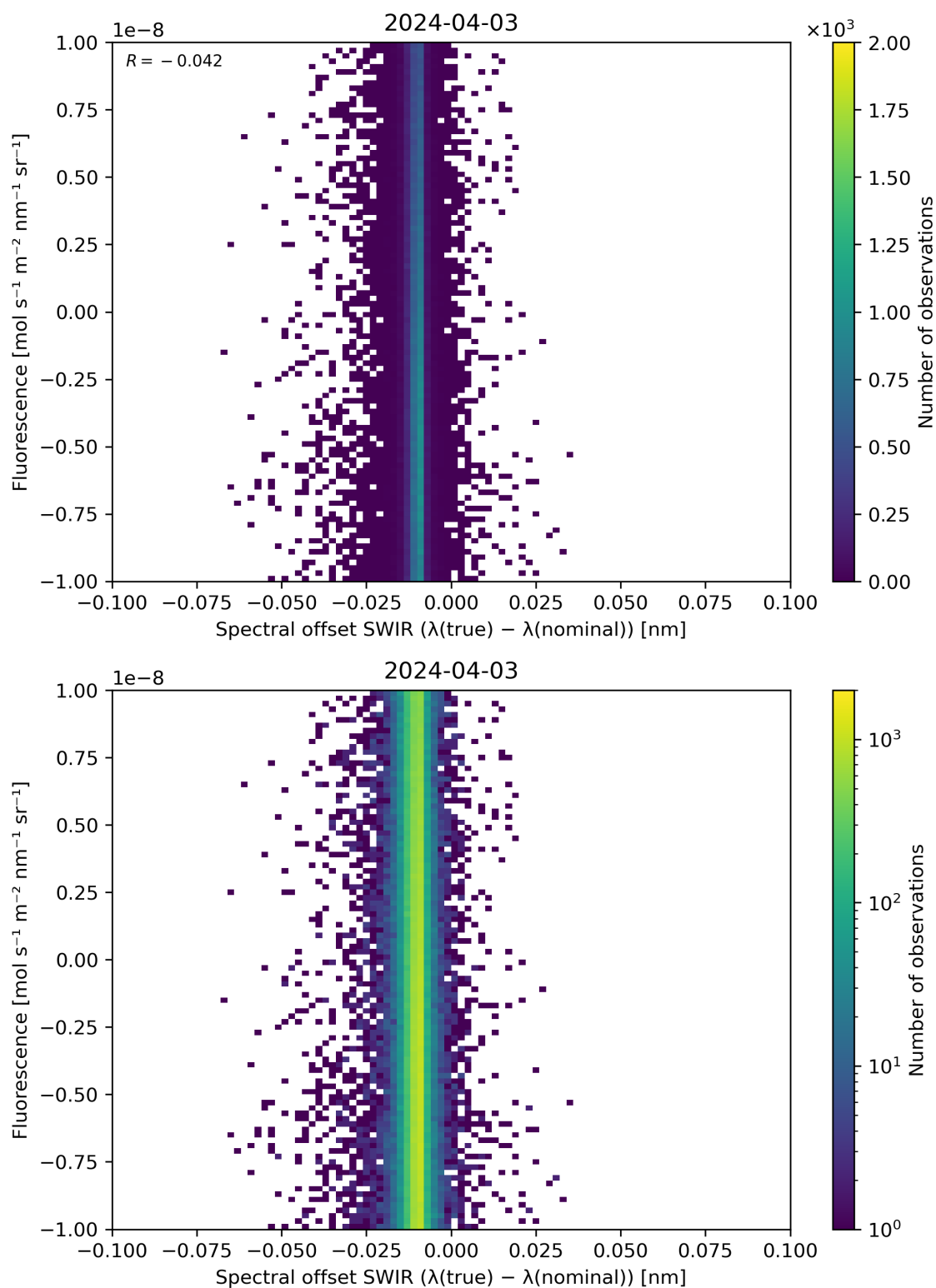
Figure 120: Scatter density plot of “Spectral offset SWIR ( \lambda(\text{true}) - \lambda(\text{nominal}) )” against “Fluorescence” for 2024-04-02 to 2024-04-04.
