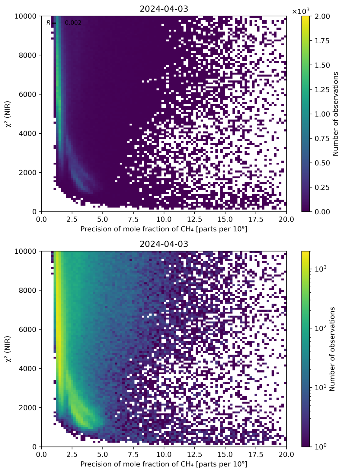
Figure 78: Scatter density plot of “Precision of mole fraction of CH 4 ” against “ \chi^2 (NIR)” for 2024-04-02 to 2024-04-04.
