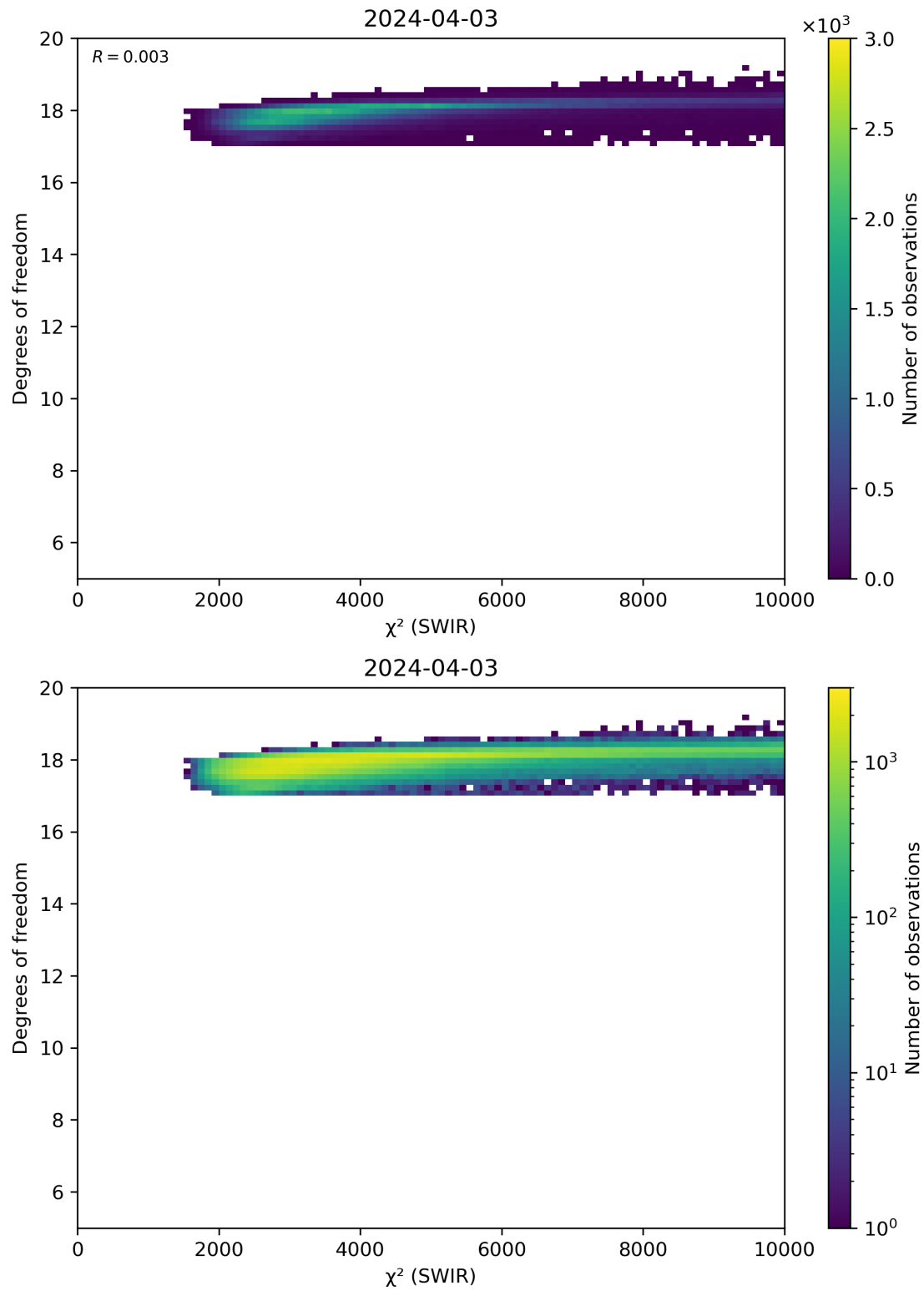
Figure 48: Scatter density plot of “ \chi^2 (SWIR)” against “Degrees of freedom” for 2024-04-02 to 2024-04-04.
