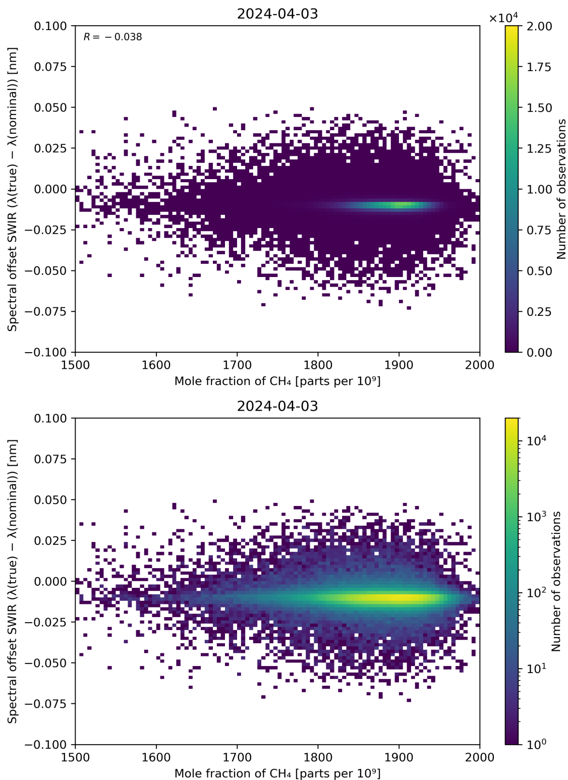
Figure 86: Scatter density plot of “Mole fraction of CH 4 ” against “Spectral offset SWIR ( \lambda(\text{true}) - \lambda(\text{nominal}) )” for 2024-04-02 to 2024-04-04.
