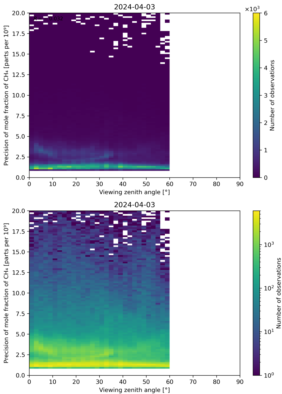
Figure 112: Scatter density plot of “Viewing zenith angle” against “Precision of mole fraction of CH 4 ” for 2024-04-02 to 2024-04-04.
