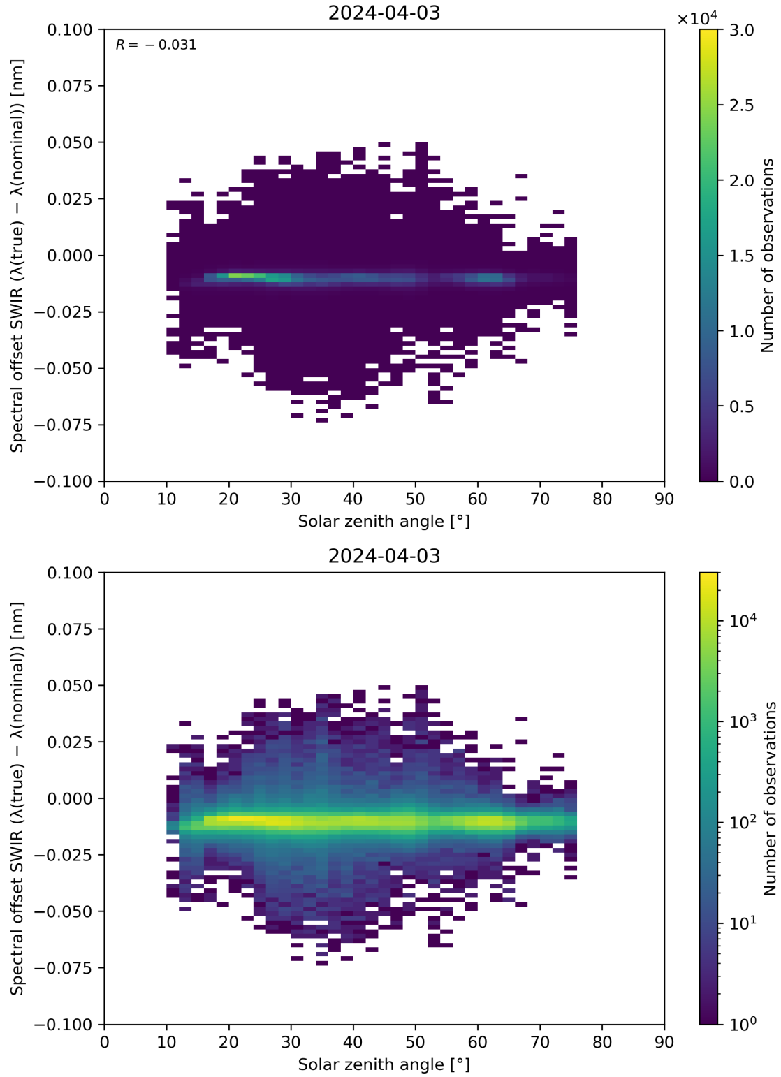
Figure 104: Scatter density plot of “Solar zenith angle” against “Spectral offset SWIR ( \lambda(\text{true}) - \lambda(\text{nominal}) )” for 2024-04-02 to 2024-04-04.
