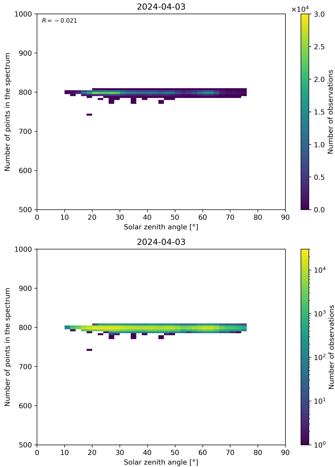
Figure 103: Scatter density plot of “Solar zenith angle” against “Number of points in the spectrum” for 2024-04-02 to 2024-04-04.
