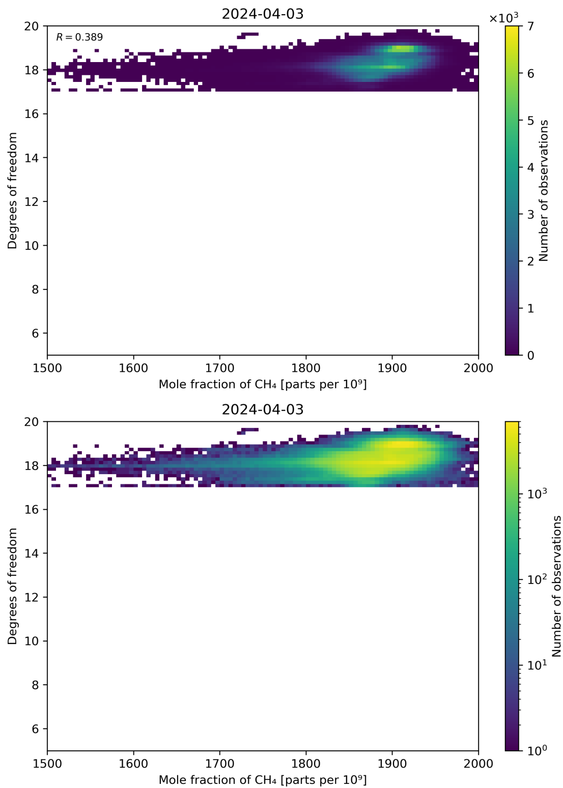
Figure 72: Scatter density plot of “Mole fraction of CH 4 ” against “Degrees of freedom” for 2024-04-02 to 2024-04-04.
