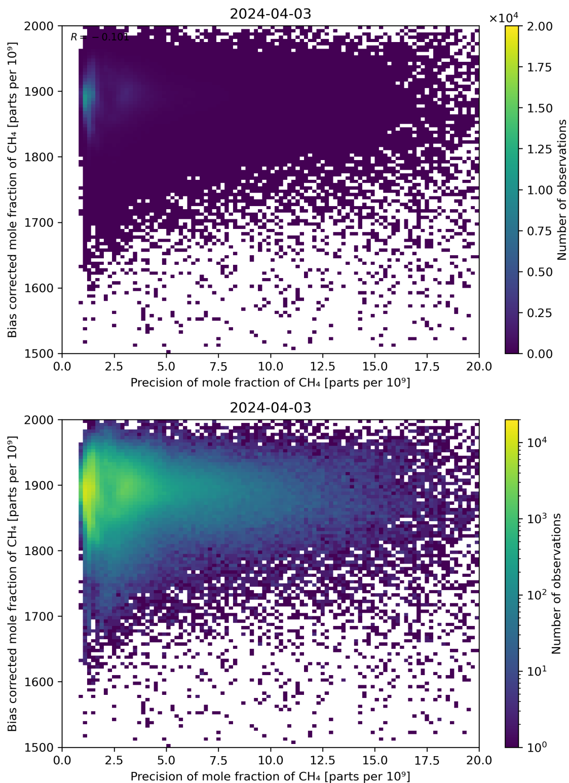
Figure 82: Scatter density plot of “Precision of mole fraction of CH 4 ” against “Bias corrected mole fraction of CH 4 ” for 2024-04-02 to 2024-04-04.
