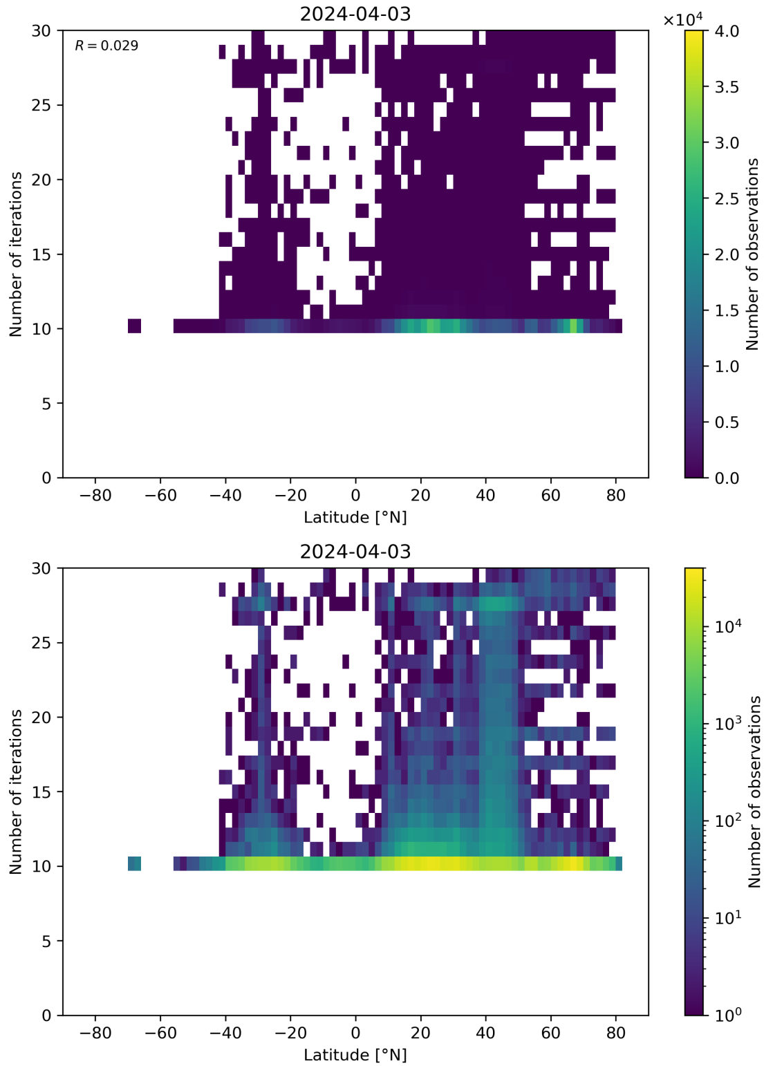
Figure 60: Scatter density plot of “Latitude” against “Number of iterations” for 2024-04-02 to 2024-04-04.
