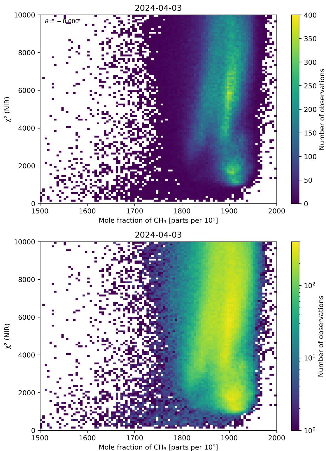
Figure 70: Scatter density plot of “Mole fraction of CH 4 ” against “ \chi^2 (NIR)” for 2024-04-02 to 2024-04-04.
