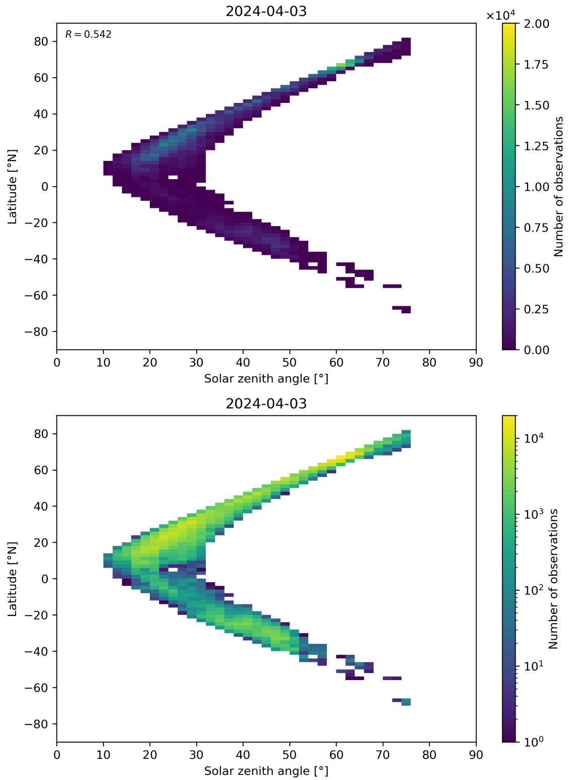
Figure 98: Scatter density plot of “Solar zenith angle” against “Latitude” for 2024-04-02 to 2024-04-04.
