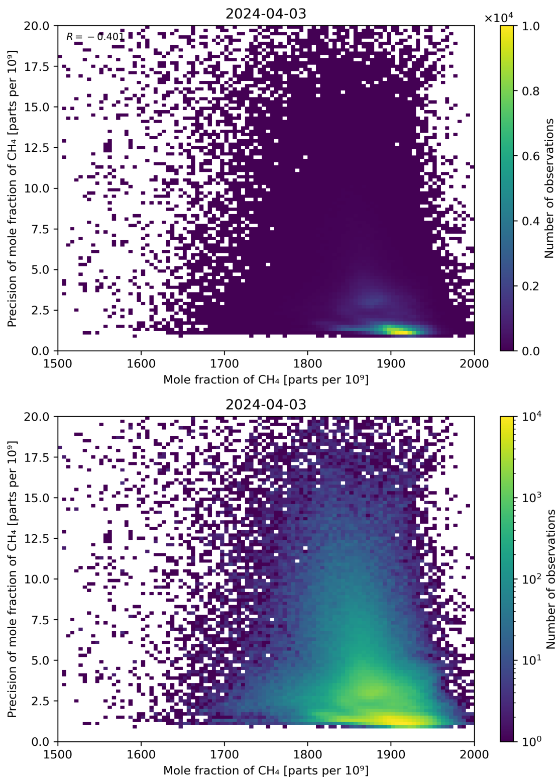
Figure 75: Scatter density plot of “Mole fraction of CH 4 ” against “Precision of mole fraction of CH 4 ” for 2024-04-02 to 2024-04-04.
