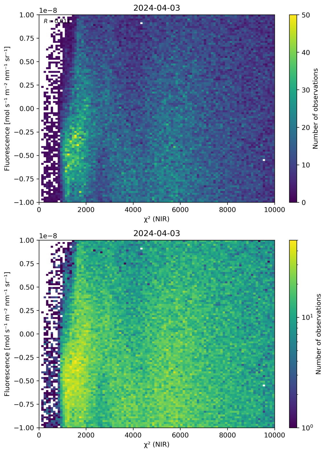
Figure 45: Scatter density plot of “ \chi^2 (NIR)” against “Fluorescence” for 2024-04-02 to 2024-04-04.
