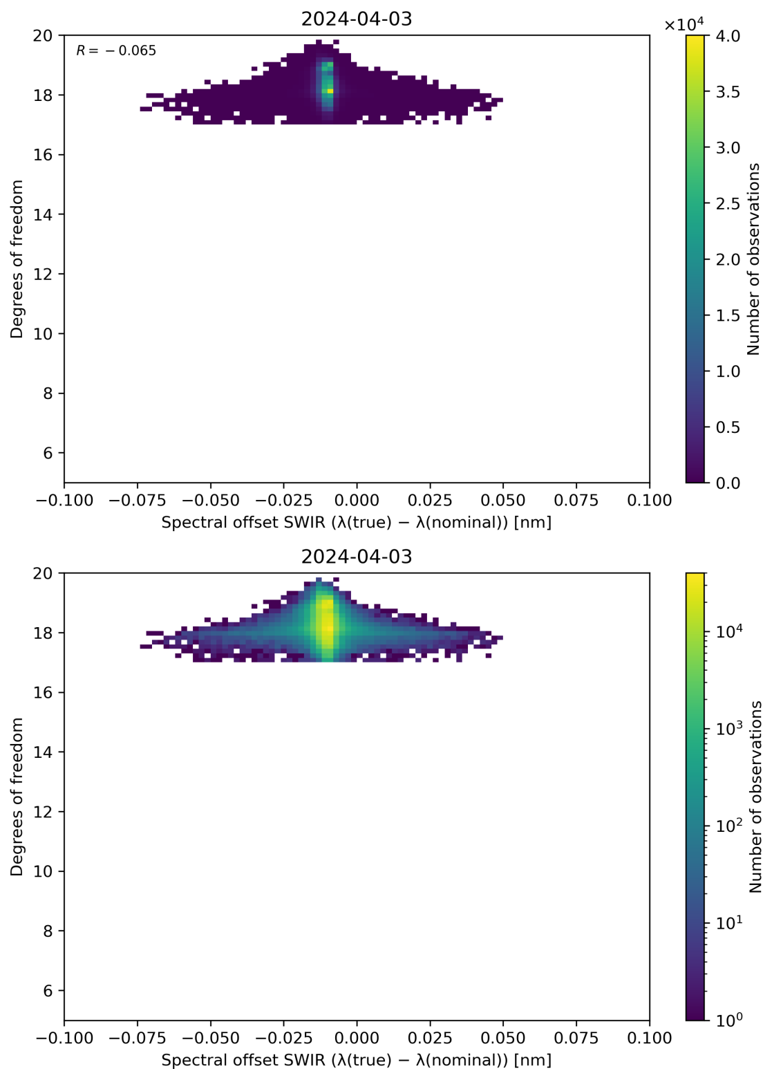
Figure 119: Scatter density plot of “Spectral offset SWIR ( \lambda(\text{true}) - \lambda(\text{nominal}) )” against “Degrees of freedom” for 2024-04-02 to 2024-04-04.
