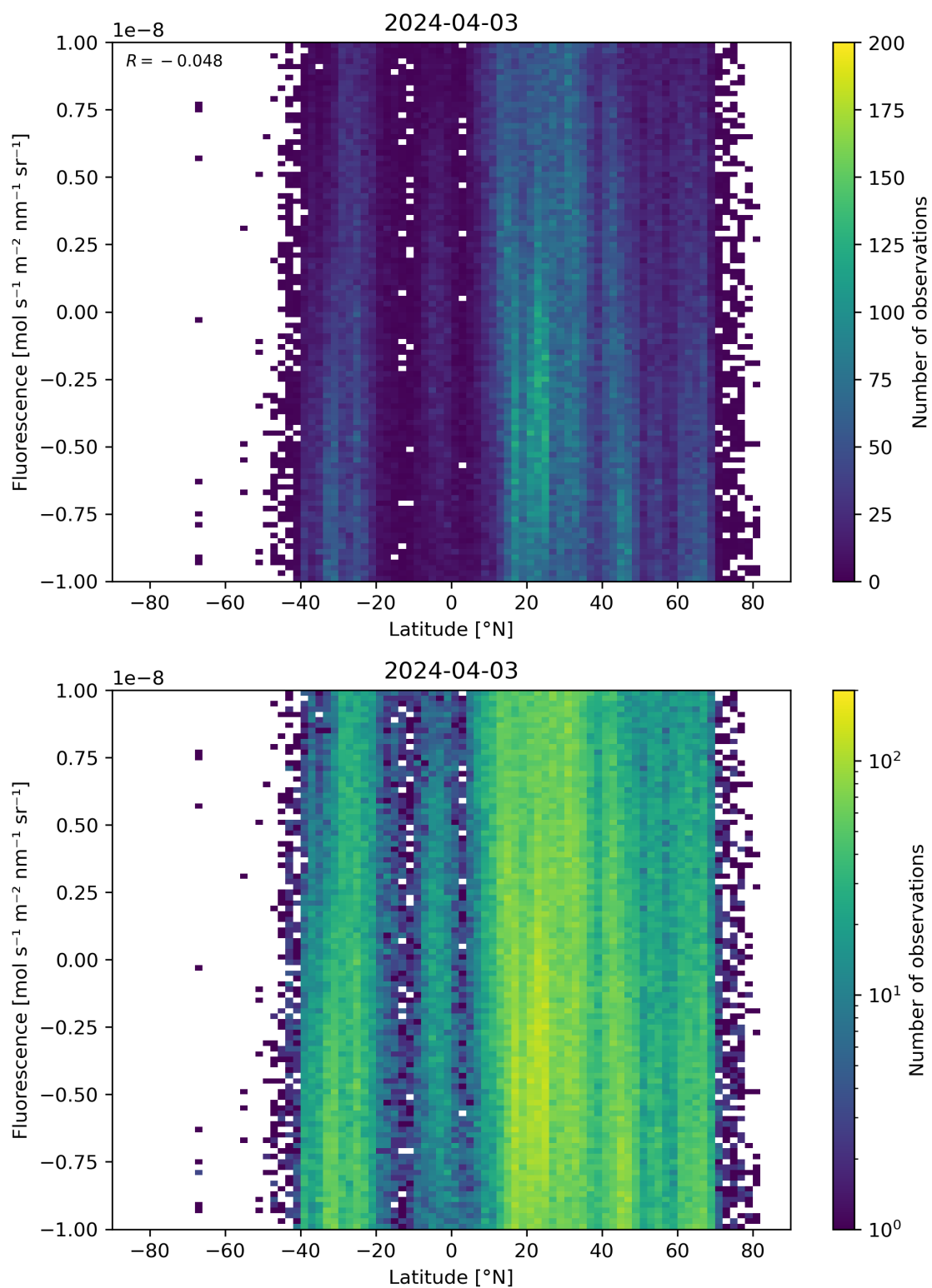
Figure 56: Scatter density plot of “Latitude” against “Fluorescence” for 2024-04-02 to 2024-04-04.
