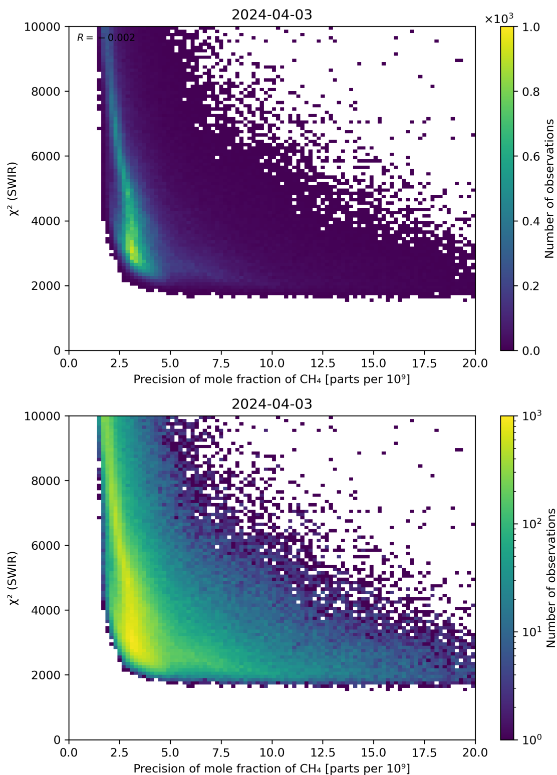
Figure 79: Scatter density plot of “Precision of mole fraction of \text{CH}_4 ” against “ \chi^2 (SWIR)” for 2024-04-02 to 2024-04-04.
