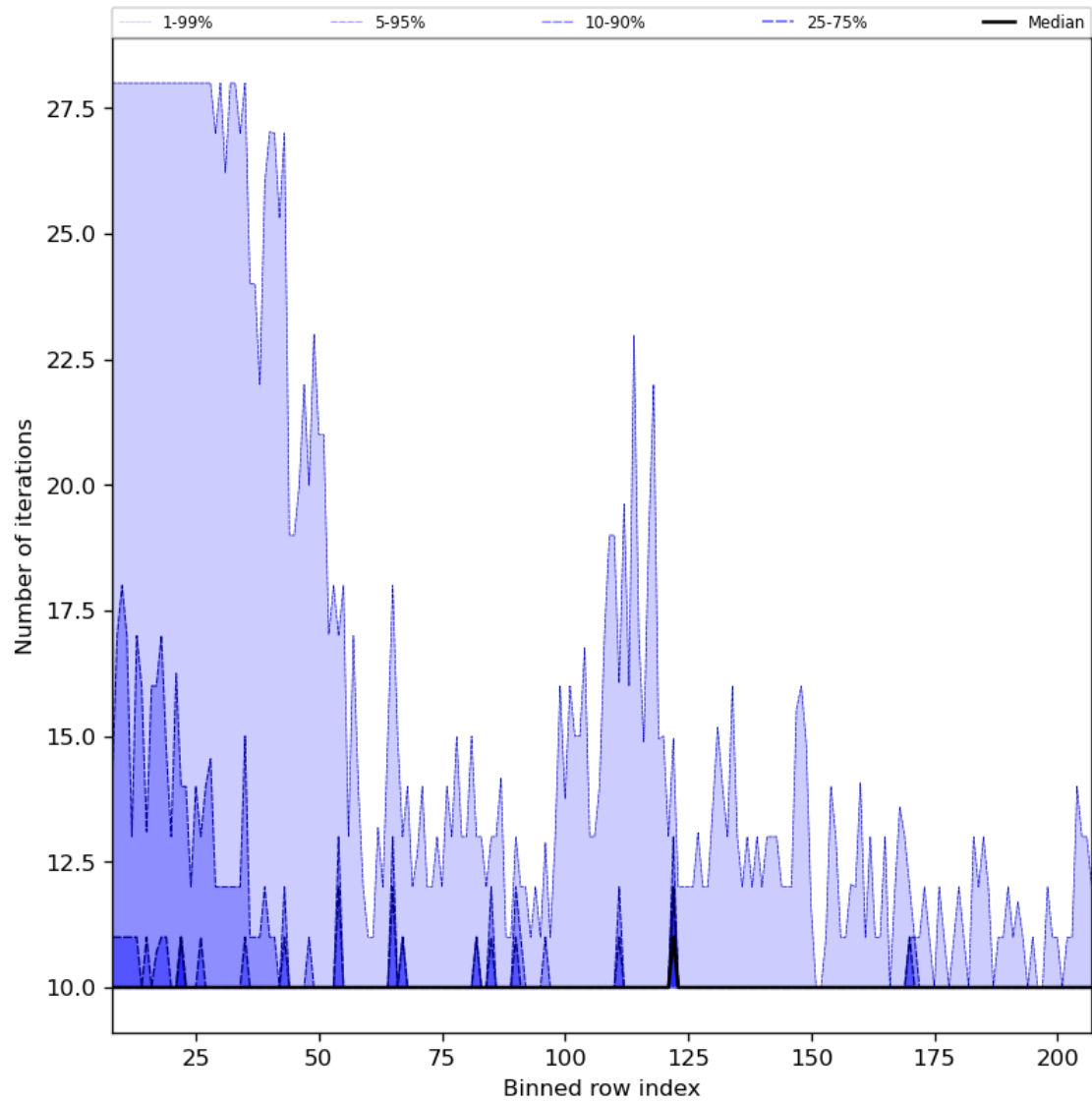
Figure 42: Along track statistics of “Number of iterations” for 2024-04-02 to 2024-04-04
