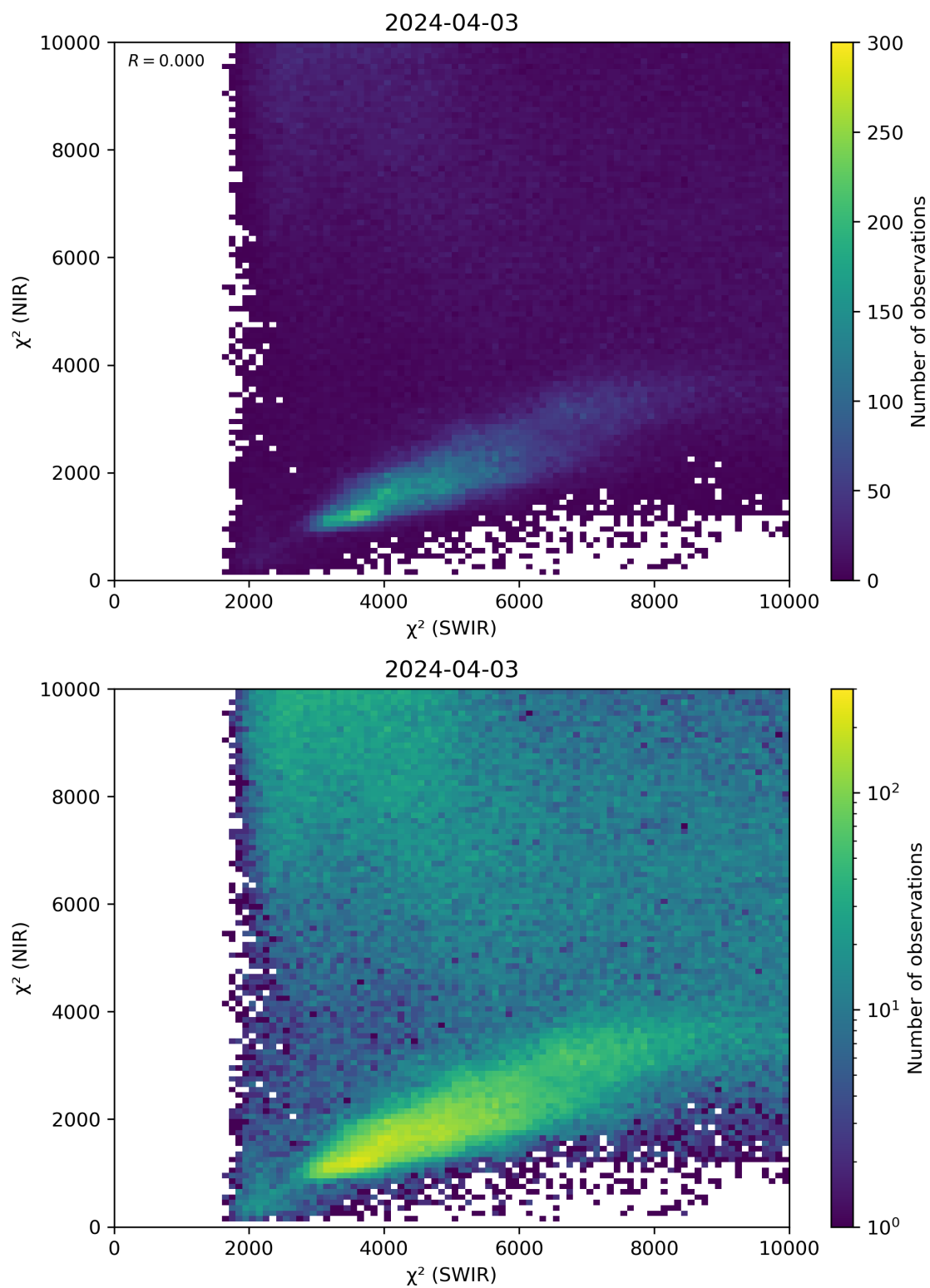
Figure 47: Scatter density plot of “ \chi^2 (SWIR)” against “ \chi^2 (NIR)” for 2024-04-02 to 2024-04-04.
