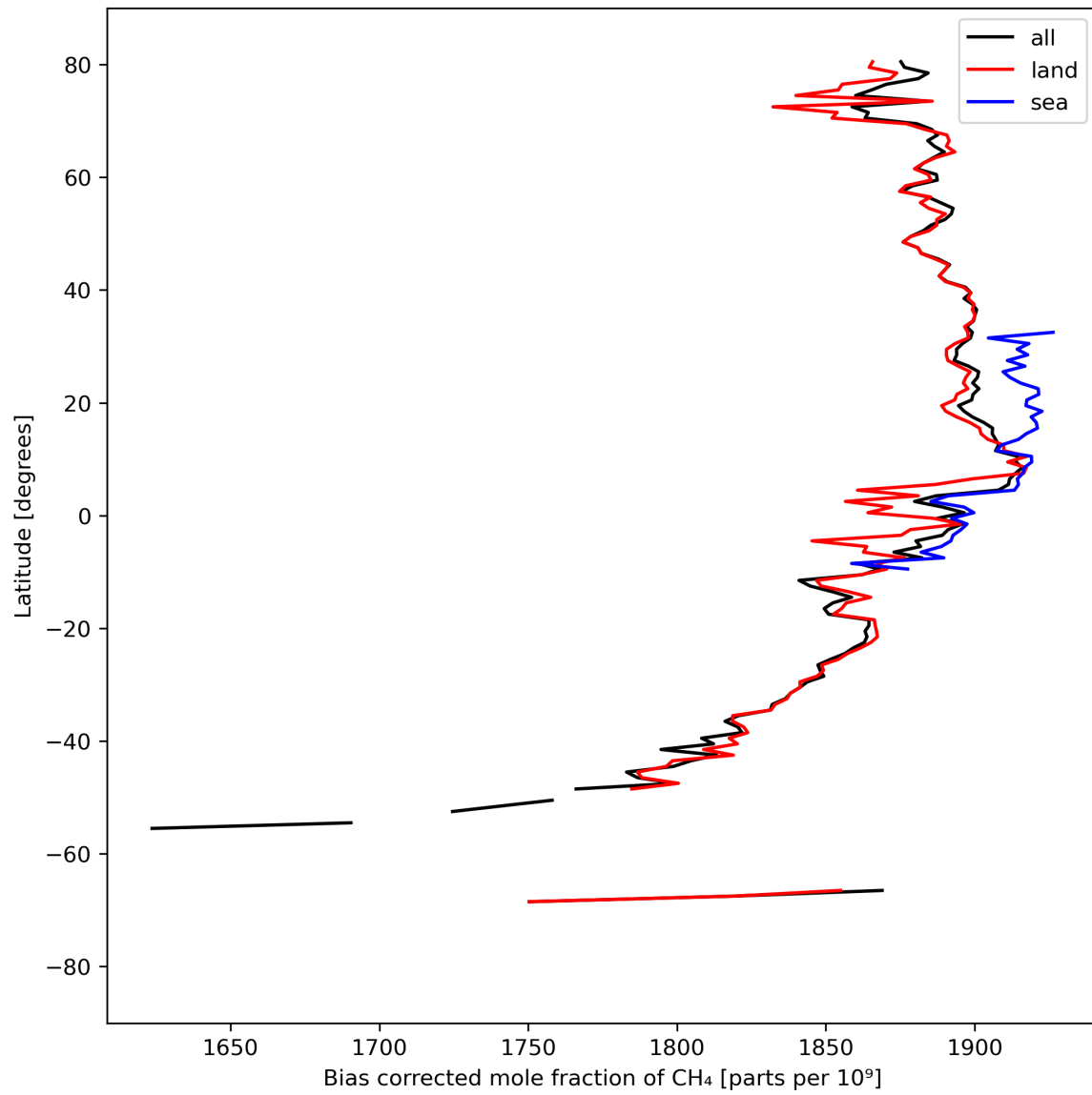
Figure 14: Zonal average of “Bias corrected mole fraction of CH 4 ” for 2024-04-02 to 2024-04-04.
