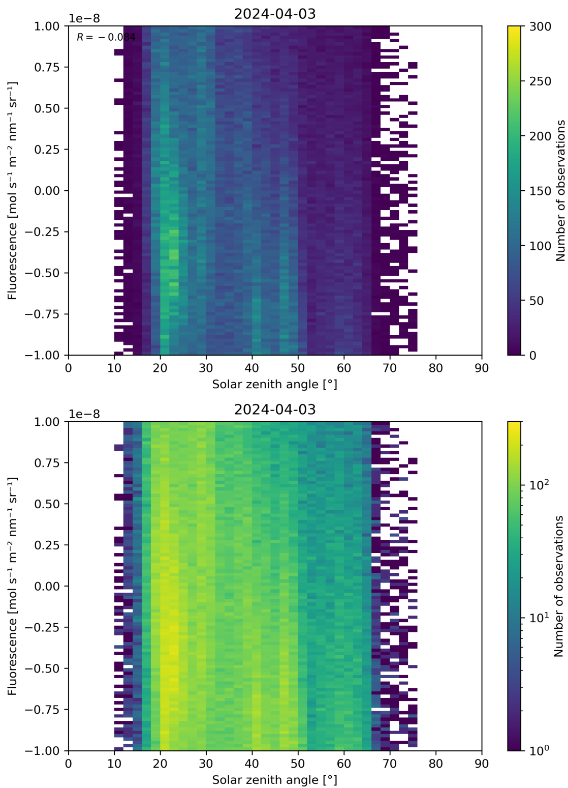
Figure 97: Scatter density plot of “Solar zenith angle” against “Fluorescence” for 2024-04-02 to 2024-04-04.
