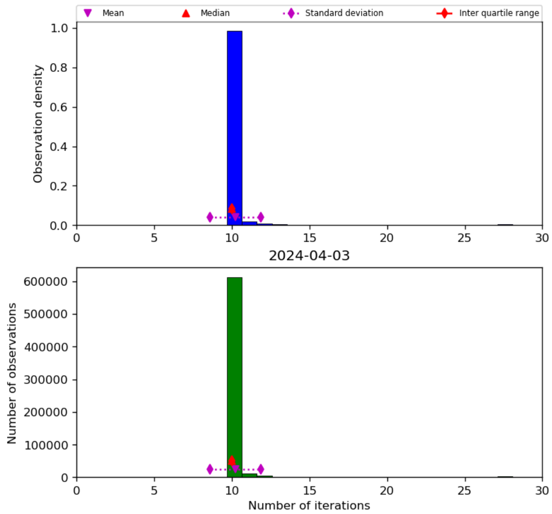
Figure 31: Histogram of “Number of iterations” for 2024-04-02 to 2024-04-04
