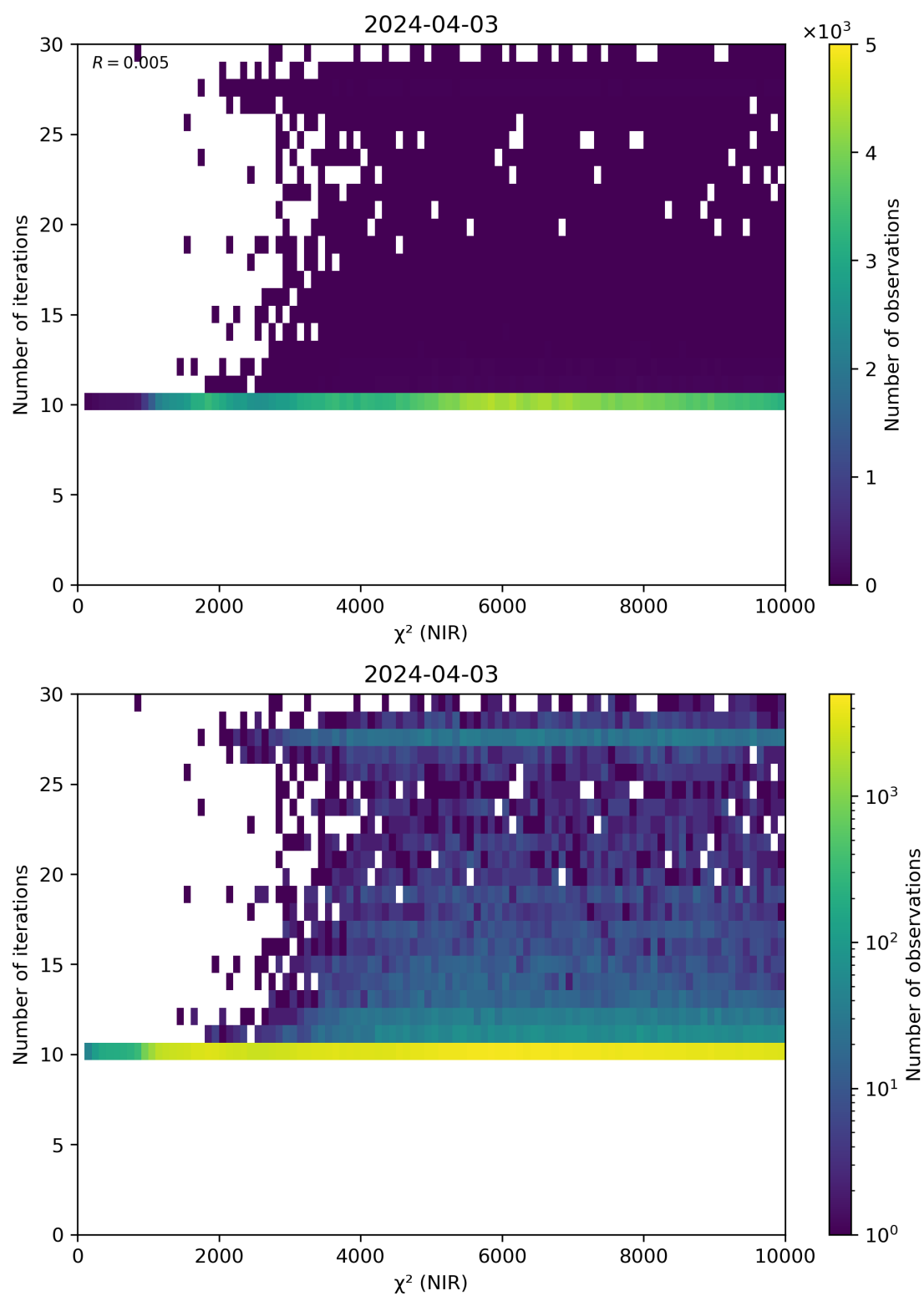
Figure 46: Scatter density plot of “ \chi^2 (NIR)” against “Number of iterations” for 2024-04-02 to 2024-04-04.
