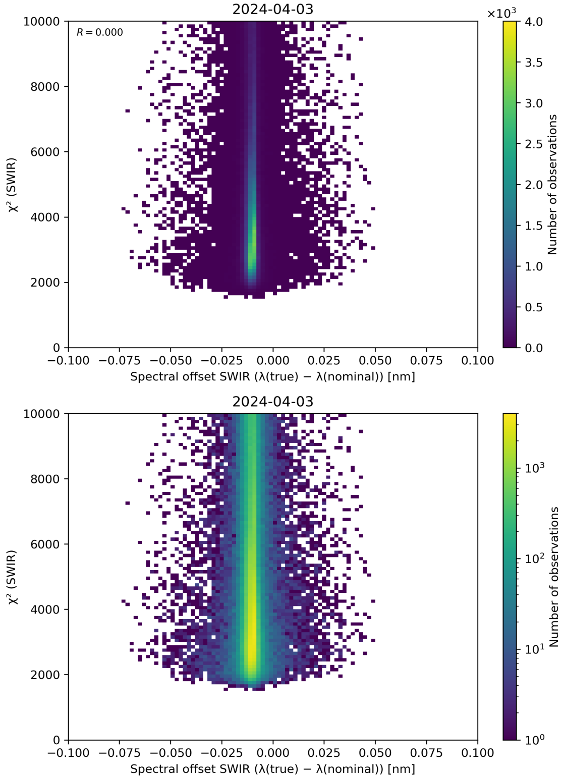
Figure 118: Scatter density plot of “Spectral offset SWIR ( \lambda(\text{true}) - \lambda(\text{nominal}) )” against “ \chi^2 (SWIR)” for 2024-04-02 to 2024-04-04.
