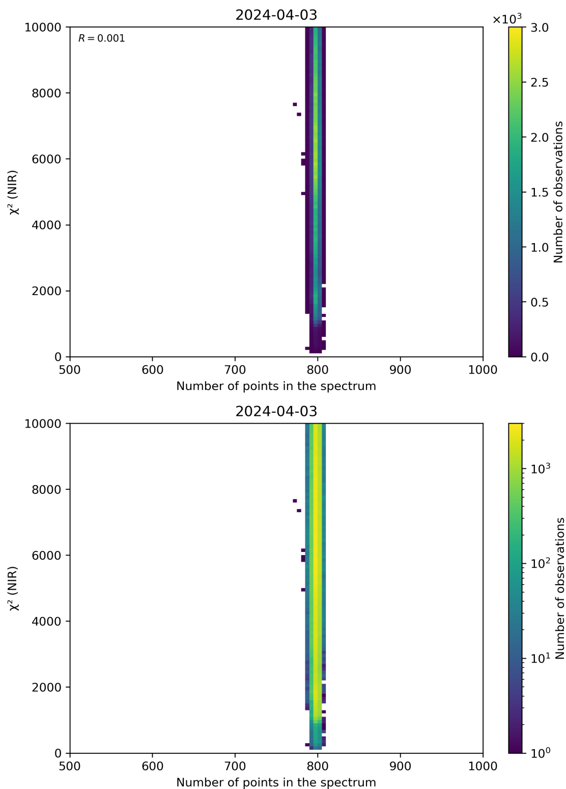
Figure 88: Scatter density plot of “Number of points in the spectrum” against “ \chi^2 (NIR)” for 2024-04-02 to 2024-04-04.
