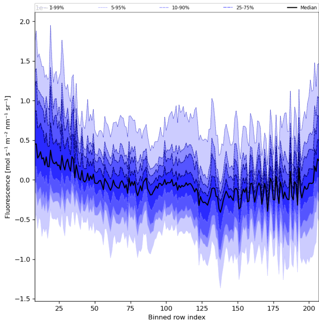
Figure 43: Along track statistics of “Fluorescence” for 2024-04-02 to 2024-04-04
