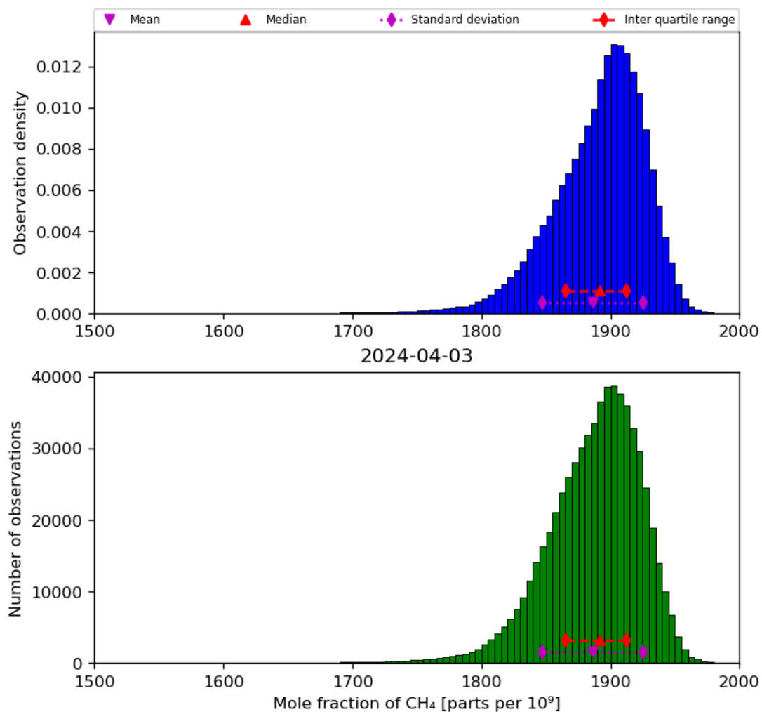
Figure 23: Histogram of “Mole fraction of CH 4 ” for 2024-04-02 to 2024-04-04
