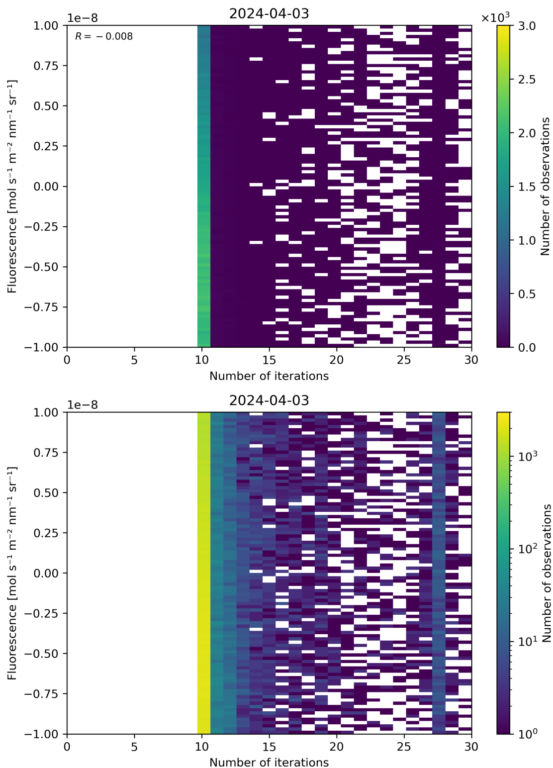
Figure 87: Scatter density plot of “Number of iterations” against “Fluorescence” for 2024-04-02 to 2024-04-04.
