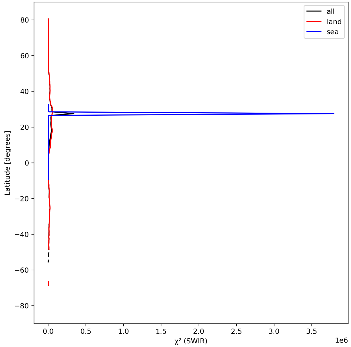
Figure 17: Zonal average of “ \chi^2 (SWIR)” for 2024-04-02 to 2024-04-04.
