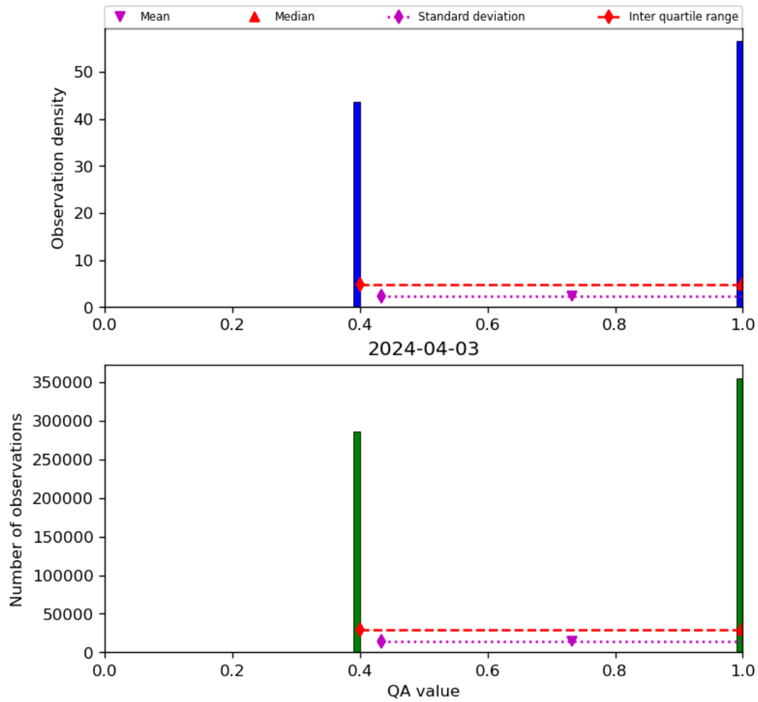
Figure 22: Histogram of “QA value” for 2024-04-02 to 2024-04-04
