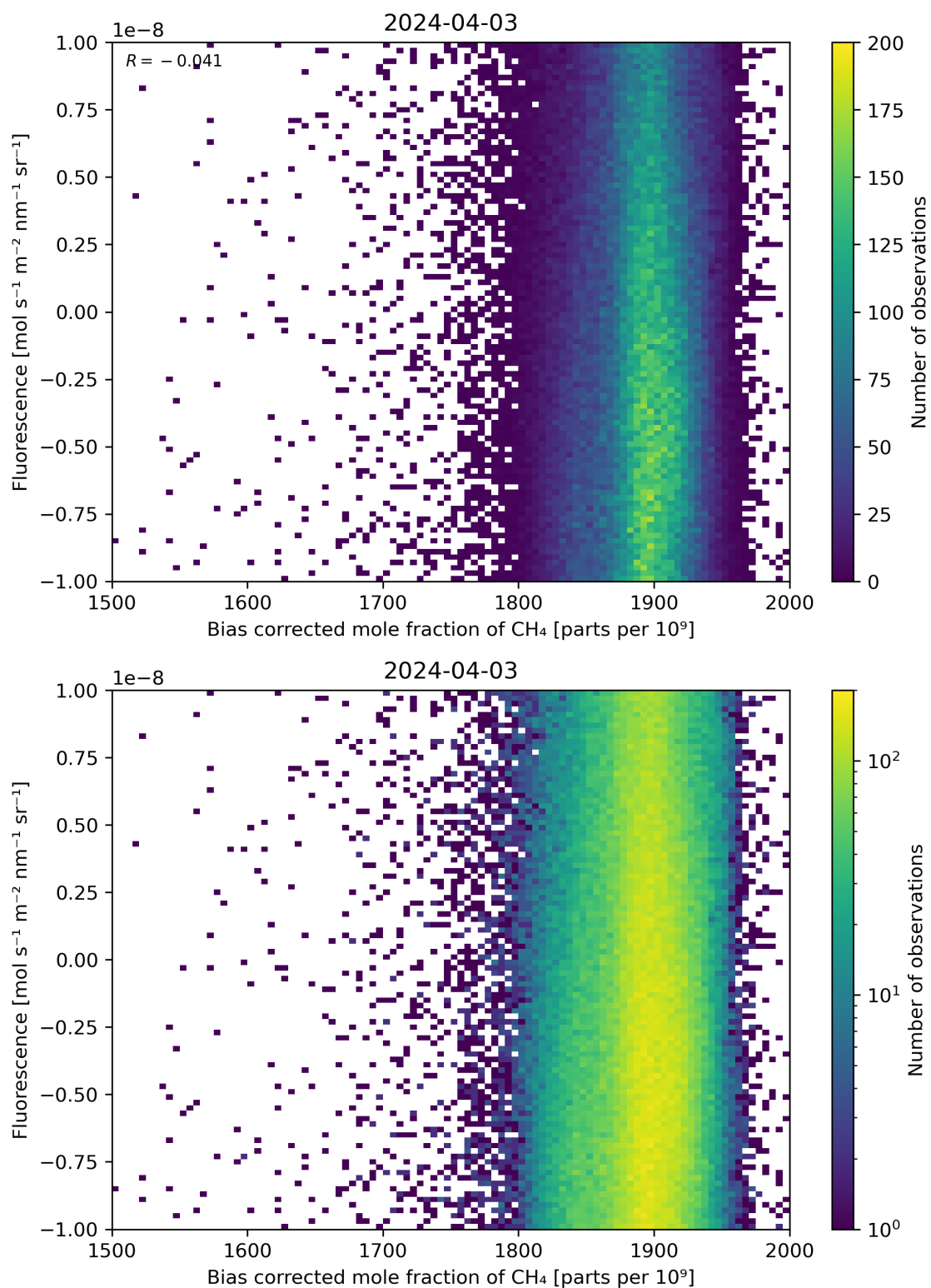
Figure 66: Scatter density plot of “Bias corrected mole fraction of \text{CH}_4 ” against “Fluorescence” for 2024-04-02 to 2024-04-04.
