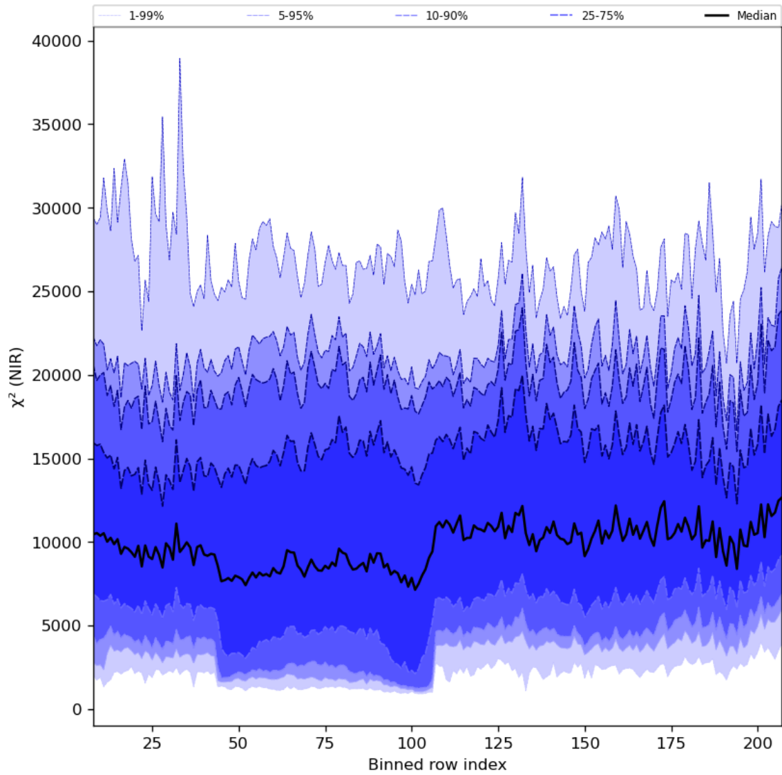
Figure 40: Along track statistics of “ \chi^2 (NIR)” for 2024-04-02 to 2024-04-04
