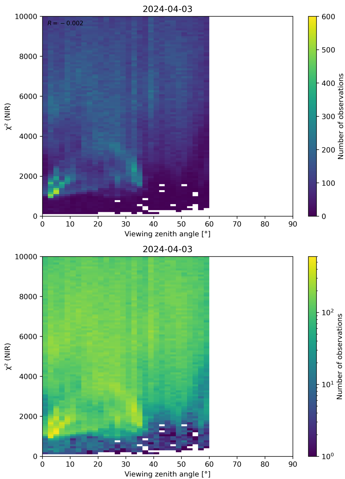
Figure 105: Scatter density plot of “Viewing zenith angle” against “ \chi^2 (NIR)” for 2024-04-02 to 2024-04-04.
