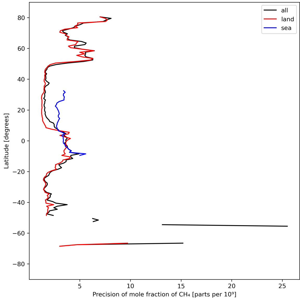
Figure 13: Zonal average of “Precision of mole fraction of CH 4 ” for 2024-04-02 to 2024-04-04.
