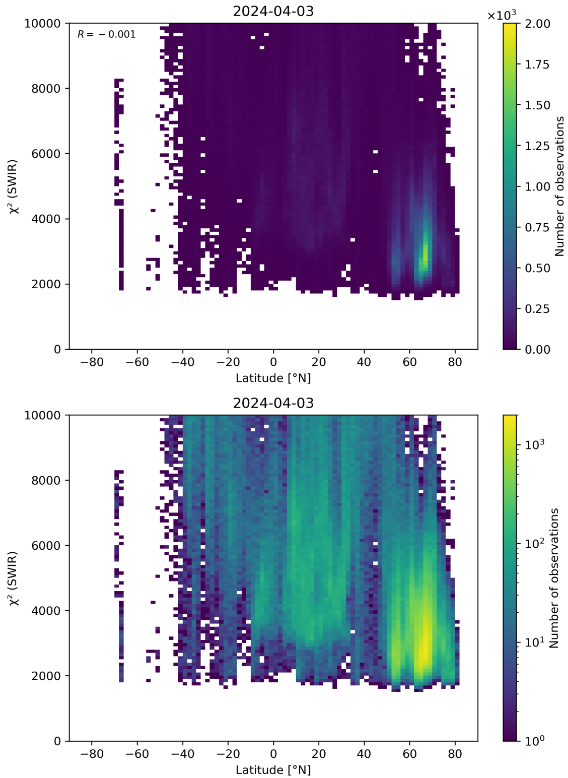
Figure 54: Scatter density plot of “Latitude” against “ \chi^2 (SWIR)” for 2024-04-02 to 2024-04-04.
