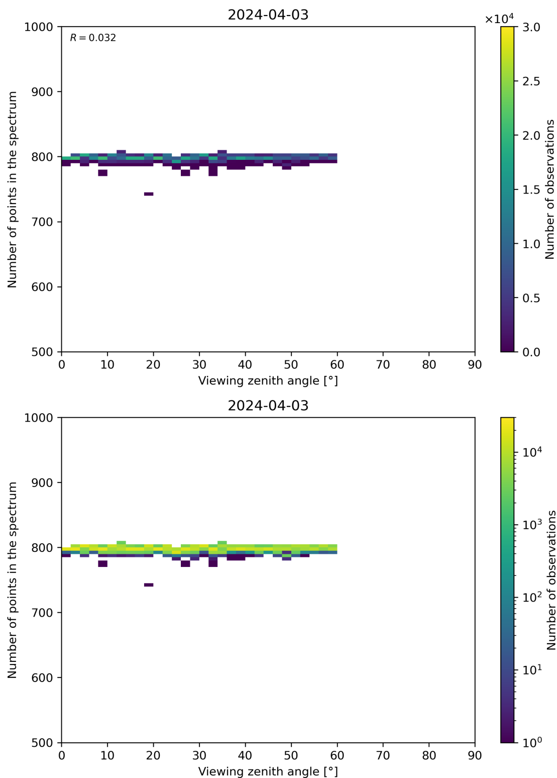
Figure 114: Scatter density plot of “Viewing zenith angle” against “Number of points in the spectrum” for 2024-04-02 to 2024-04-04.
