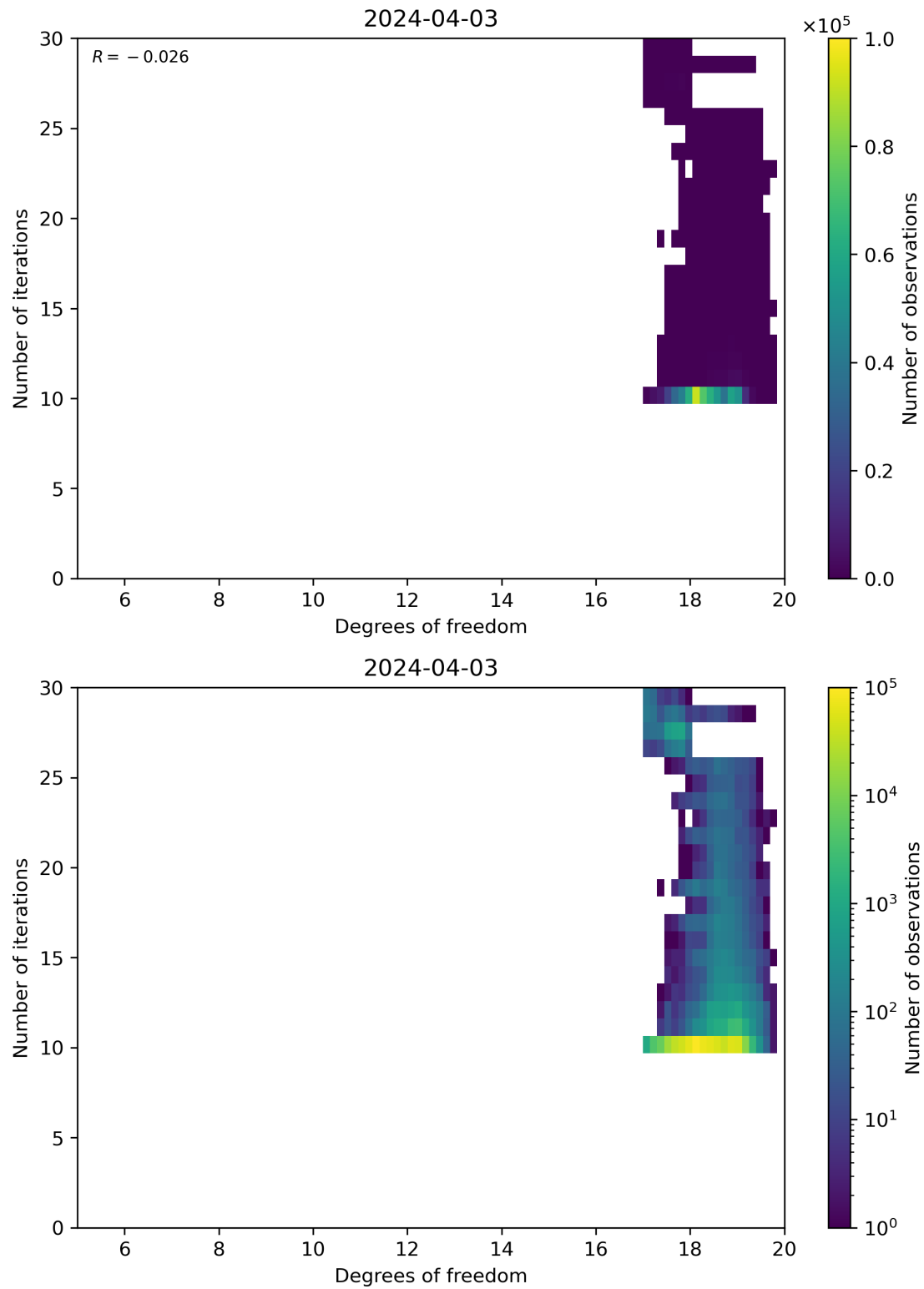
Figure 52: Scatter density plot of “Degrees of freedom” against “Number of iterations” for 2024-04-02 to 2024-04-04.
