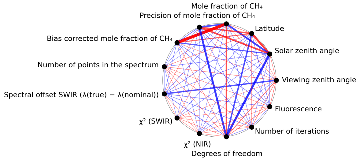
Figure 1: Map of correlation graph for 2024-04-02 to 2024-04-04.
