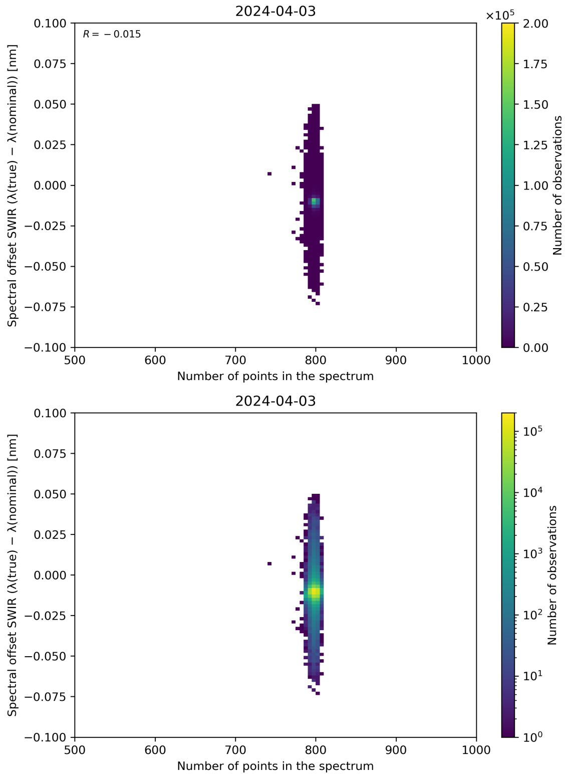
Figure 93: Scatter density plot of “Number of points in the spectrum” against “Spectral offset SWIR ( \lambda(\text{true}) - \lambda(\text{nominal}) )” for 2024-04-02 to 2024-04-04.
