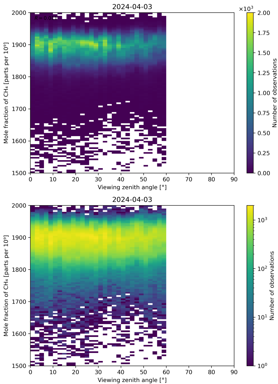
Figure 110: Scatter density plot of “Viewing zenith angle” against “Mole fraction of CH 4 ” for 2024-04-02 to 2024-04-04.
