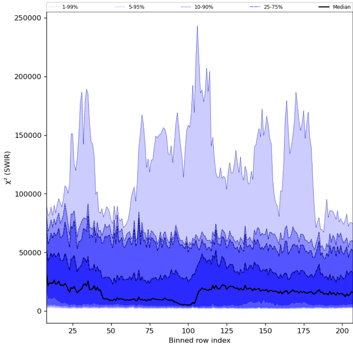
Figure 39: Along track statistics of “ \chi^2 (SWIR)” for 2024-04-02 to 2024-04-04
