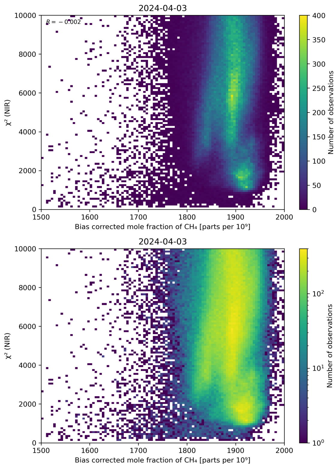
Figure 63: Scatter density plot of “Bias corrected mole fraction of CH 4 ” against “ \chi^2 (NIR)” for 2024-04-02 to 2024-04-04.
