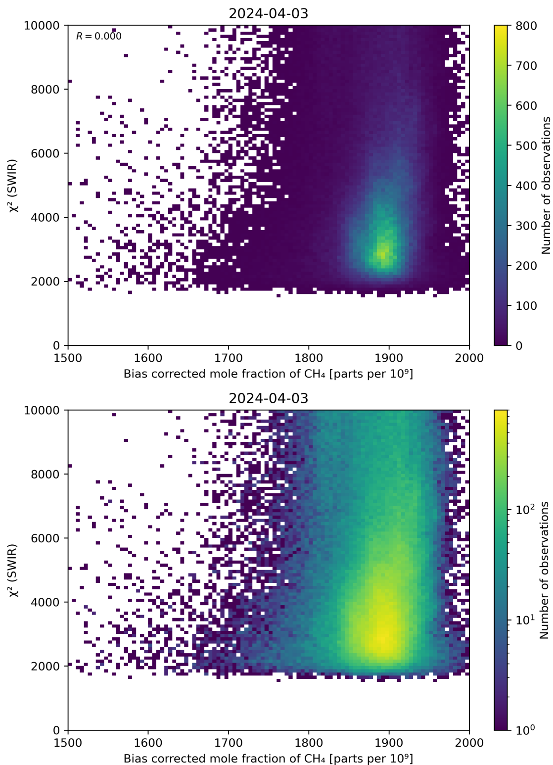
Figure 64: Scatter density plot of “Bias corrected mole fraction of \text{CH}_4 ” against “ \chi^2 (SWIR)” for 2024-04-02 to 2024-04-04.
