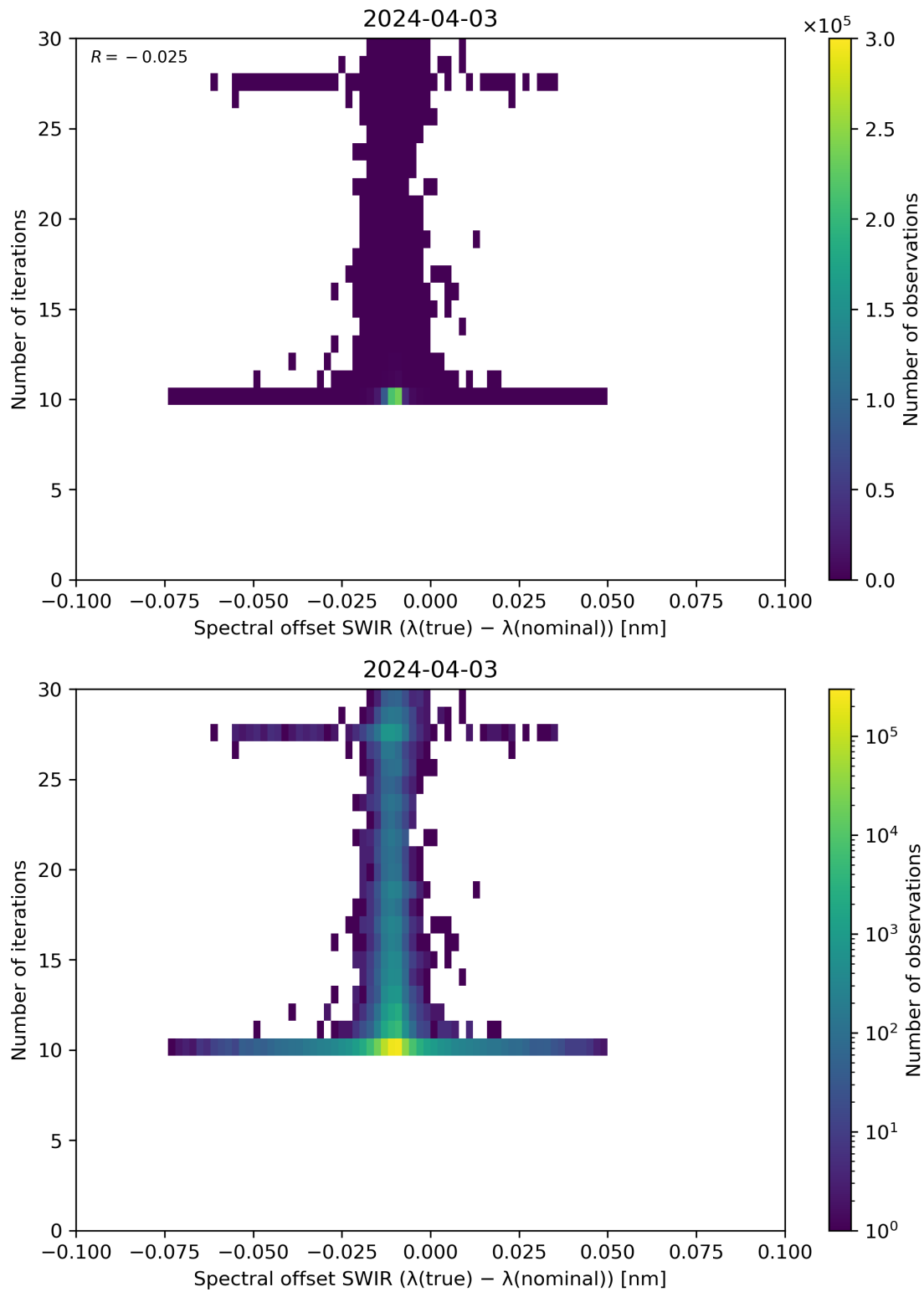
Figure 121: Scatter density plot of “Spectral offset SWIR ( \lambda(\text{true}) - \lambda(\text{nominal}) )” against “Number of iterations” for 2024-04-02 to 2024-04-04.
