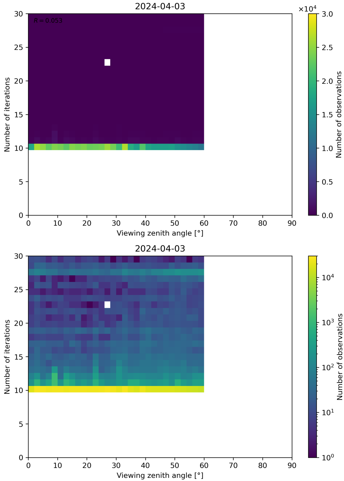
Figure 113: Scatter density plot of “Viewing zenith angle” against “Number of iterations” for 2024-04-02 to 2024-04-04.
