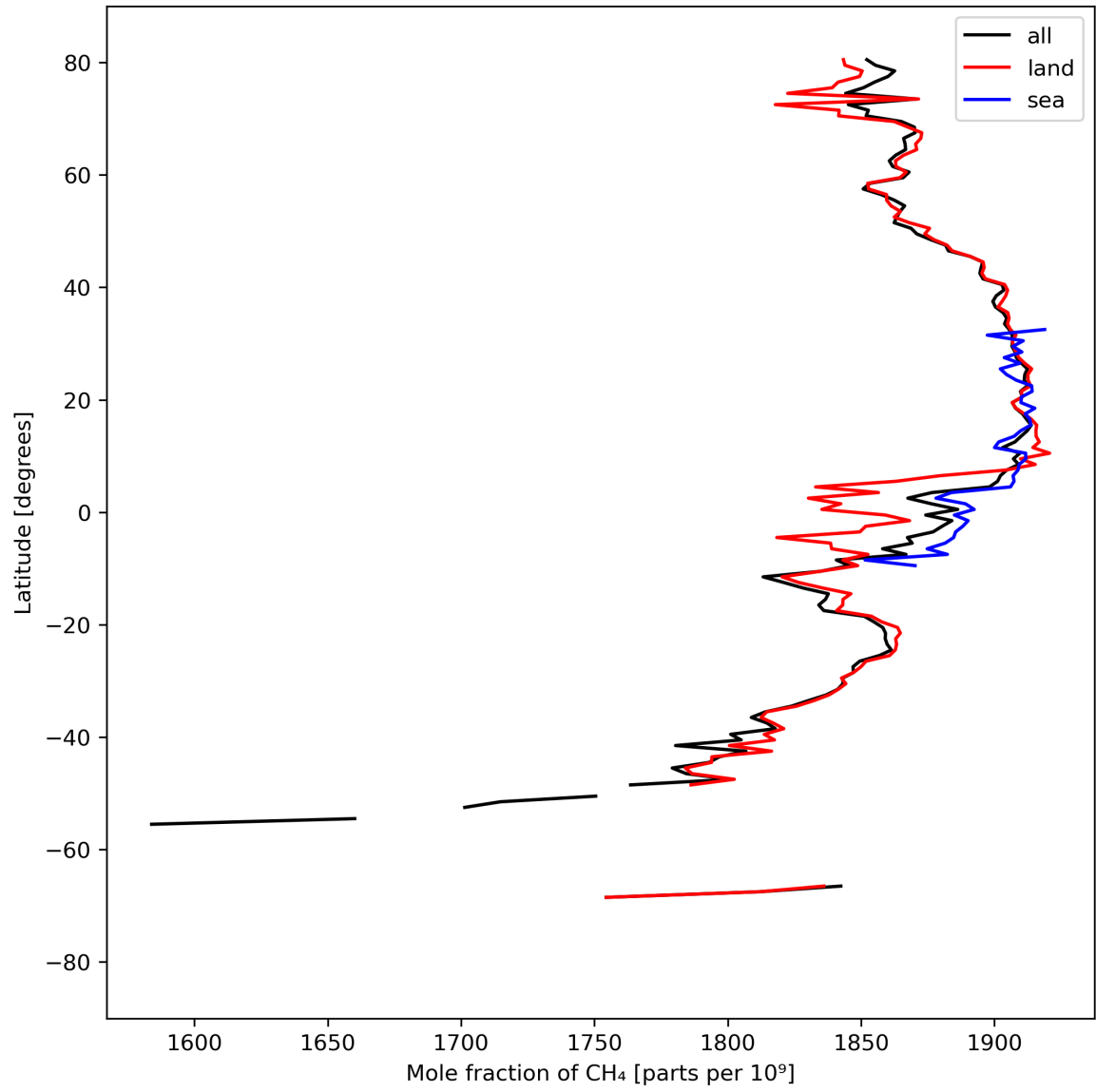
Figure 12: Zonal average of “Mole fraction of \text{CH}_4 ” for 2024-04-02 to 2024-04-04.
