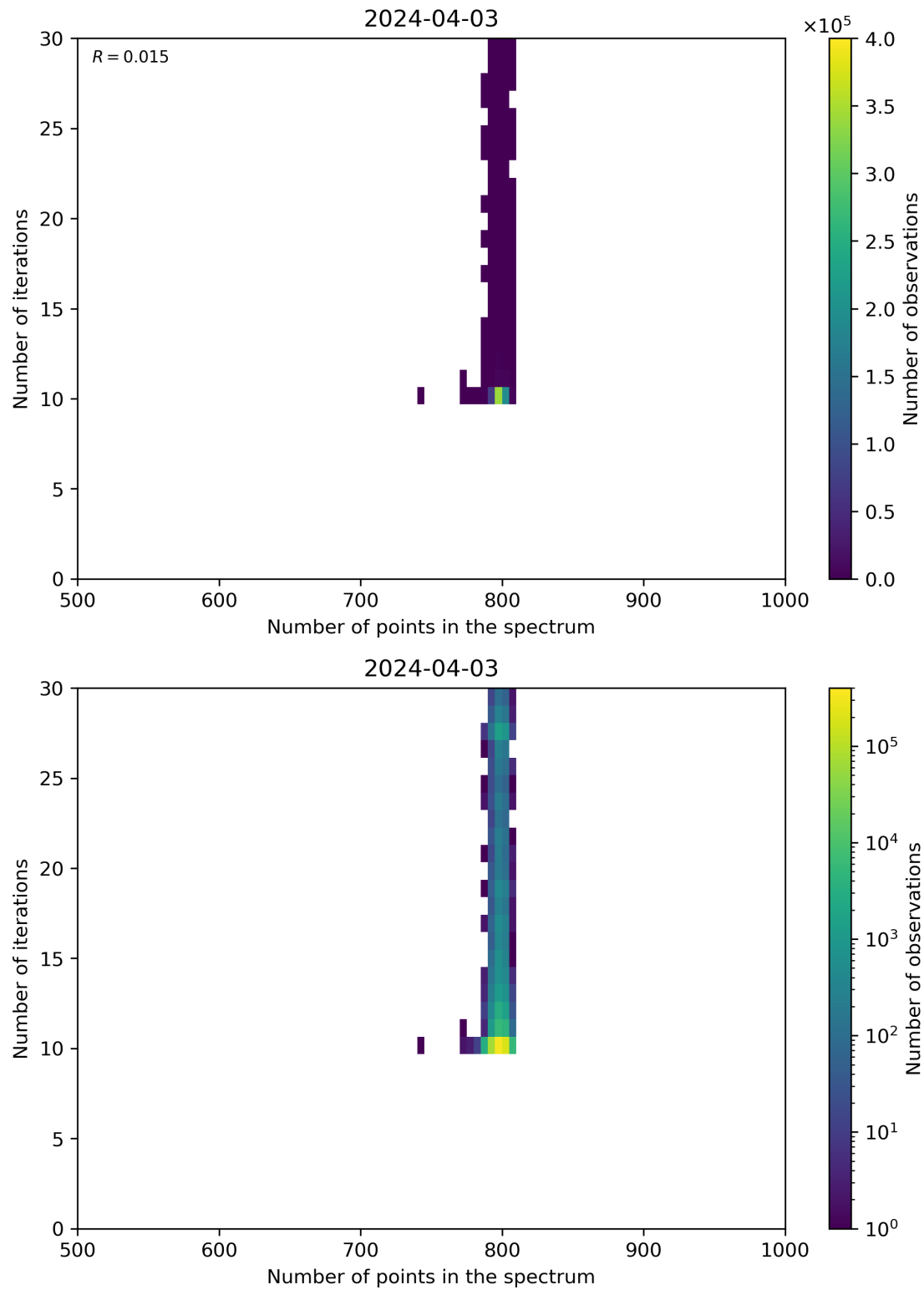
Figure 92: Scatter density plot of “Number of points in the spectrum” against “Number of iterations” for 2024-04-02 to 2024-04-04.
