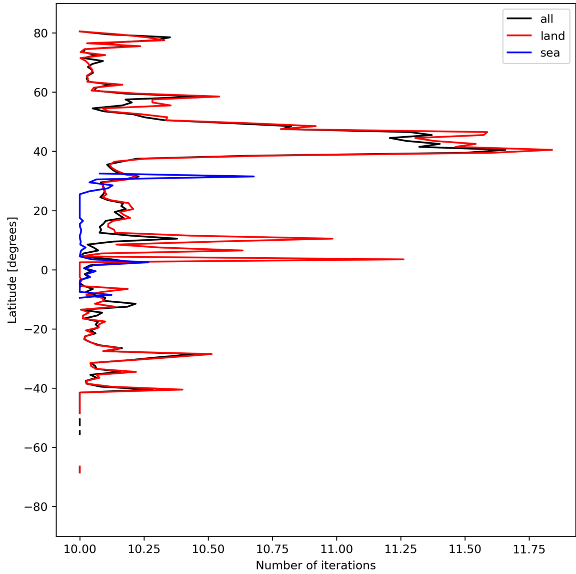
Figure 20: Zonal average of “Number of iterations” for 2024-04-02 to 2024-04-04.
