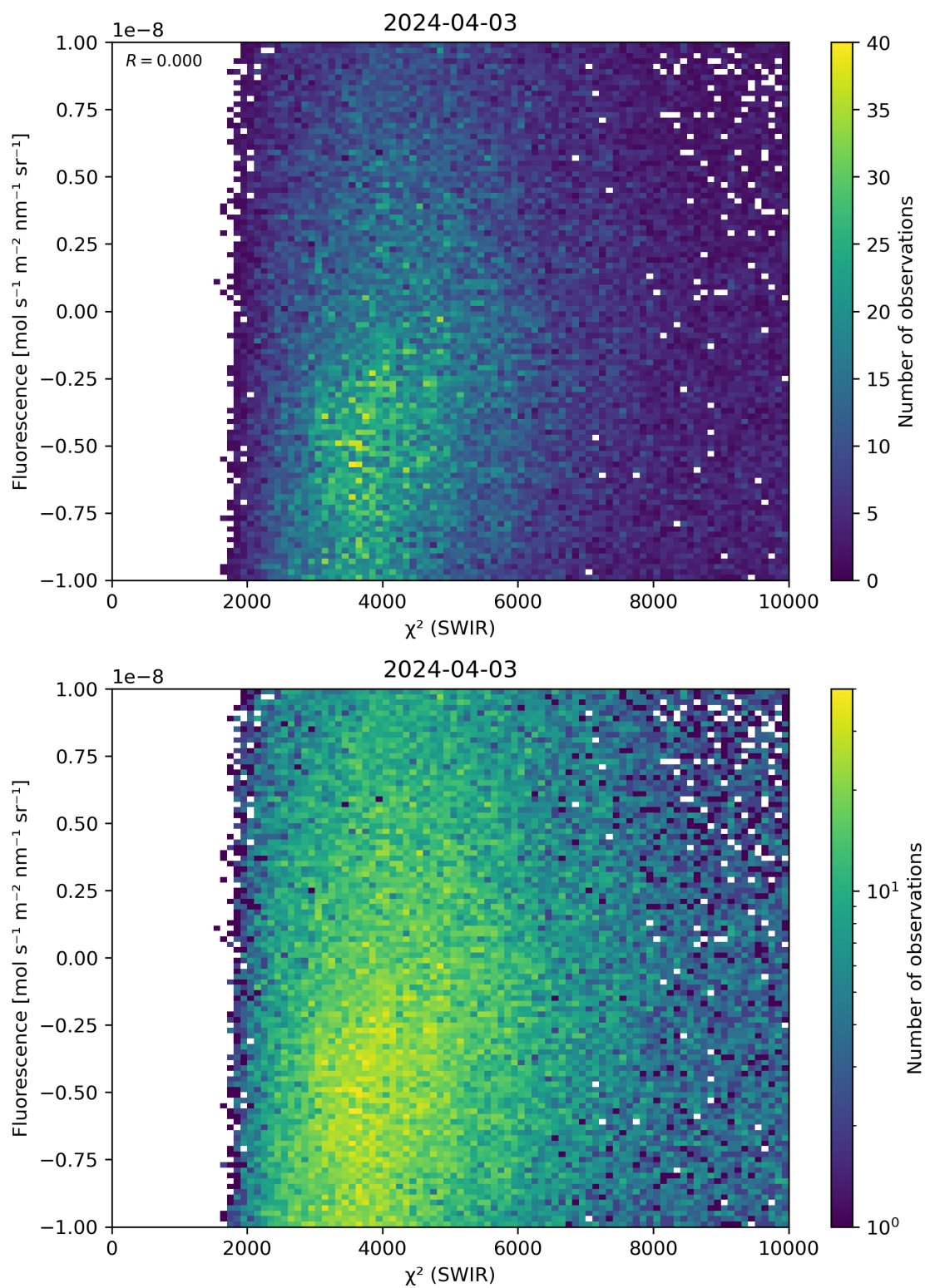
Figure 49: Scatter density plot of “ \chi^2 (SWIR)” against “Fluorescence” for 2024-04-02 to 2024-04-04.
