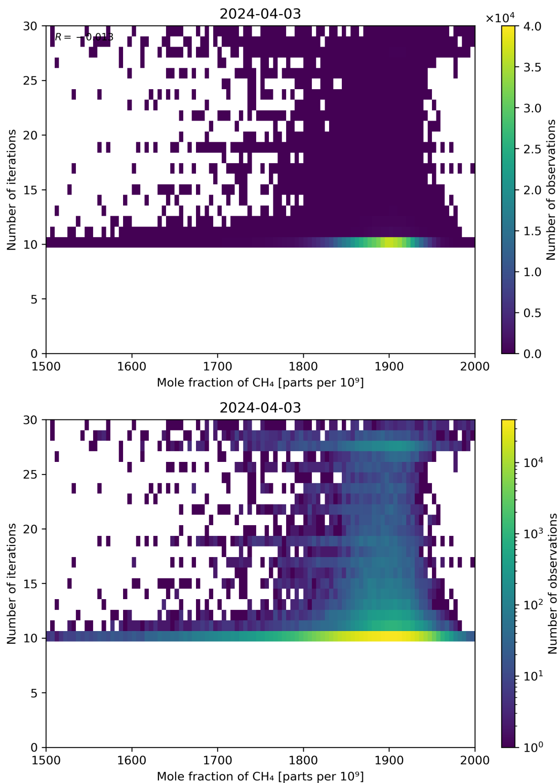
Figure 76: Scatter density plot of “Mole fraction of CH 4 ” against “Number of iterations” for 2024-04-02 to 2024-04-04.
