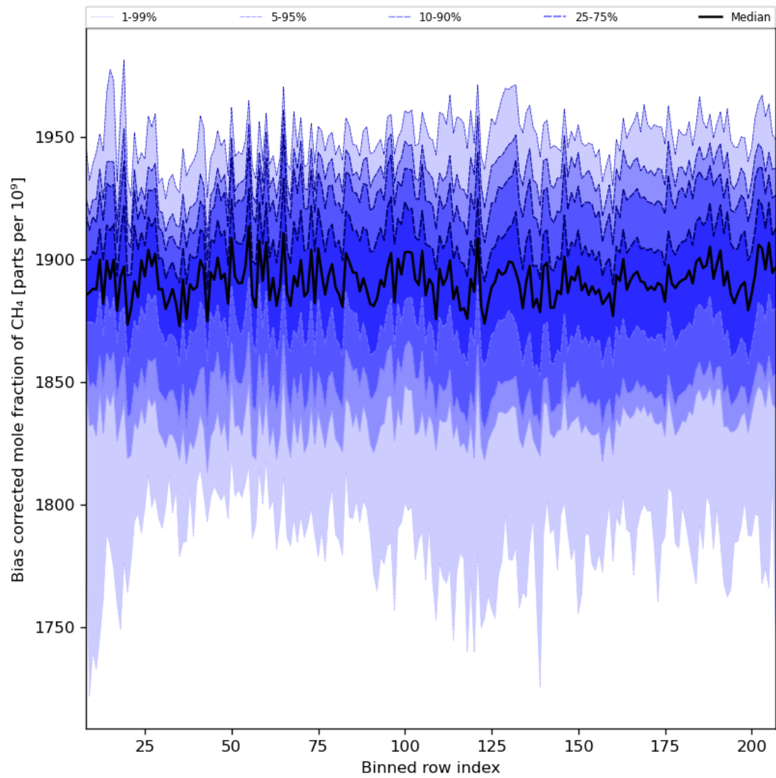
Figure 36: Along track statistics of “Bias corrected mole fraction of CH 4 ” for 2024-04-02 to 2024-04-04
