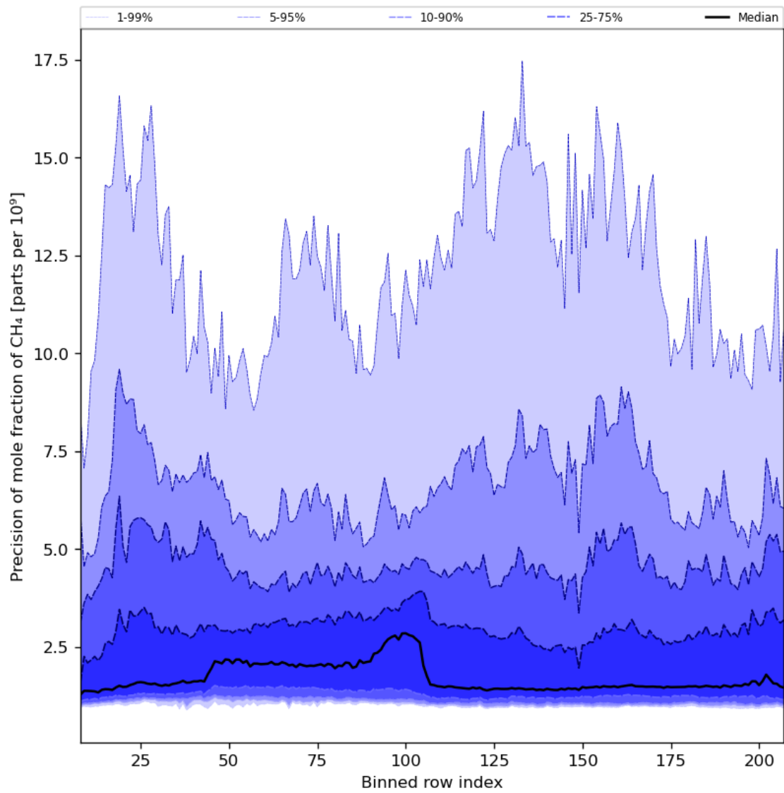
Figure 35: Along track statistics of “Precision of mole fraction of CH 4 ” for 2024-04-02 to 2024-04-04
