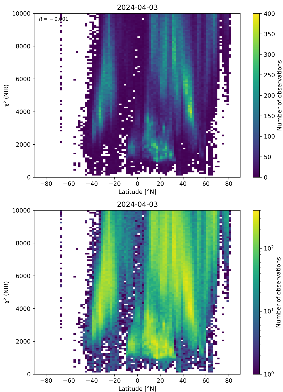
Figure 53: Scatter density plot of “Latitude” against “ \chi^2 (NIR)” for 2024-04-02 to 2024-04-04.
