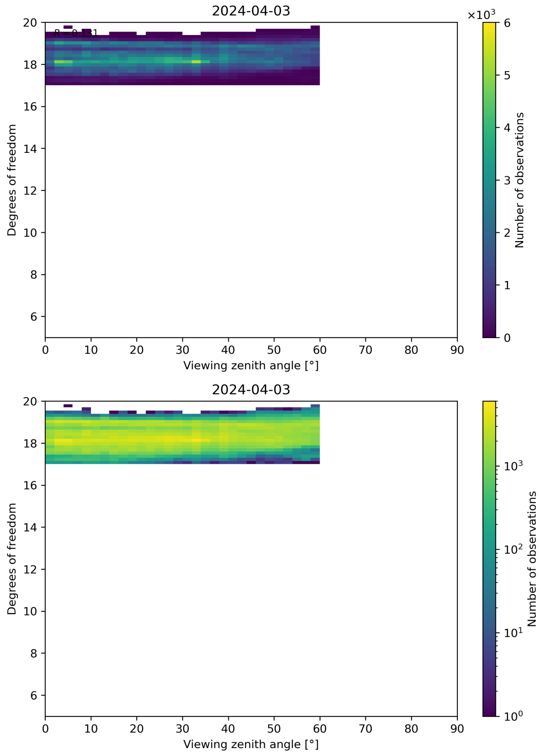
Figure 107: Scatter density plot of “Viewing zenith angle” against “Degrees of freedom” for 2024-04-02 to 2024-04-04.
