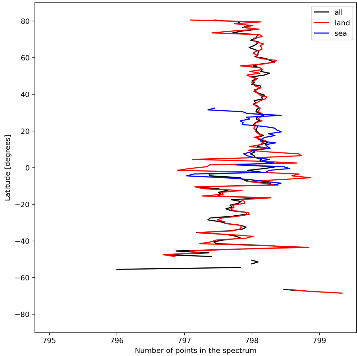
Figure 15: Zonal average of “Number of points in the spectrum” for 2024-04-02 to 2024-04-04.
