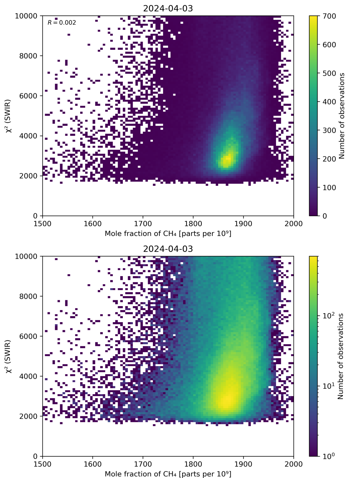
Figure 71: Scatter density plot of “Mole fraction of CH 4 ” against “ \chi^2 (SWIR)” for 2024-04-02 to 2024-04-04.
