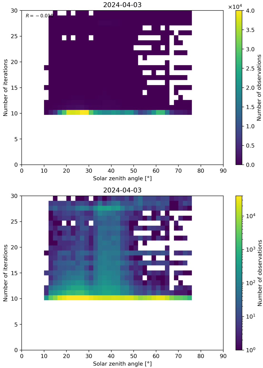
Figure 102: Scatter density plot of “Solar zenith angle” against “Number of iterations” for 2024-04-02 to 2024-04-04.
