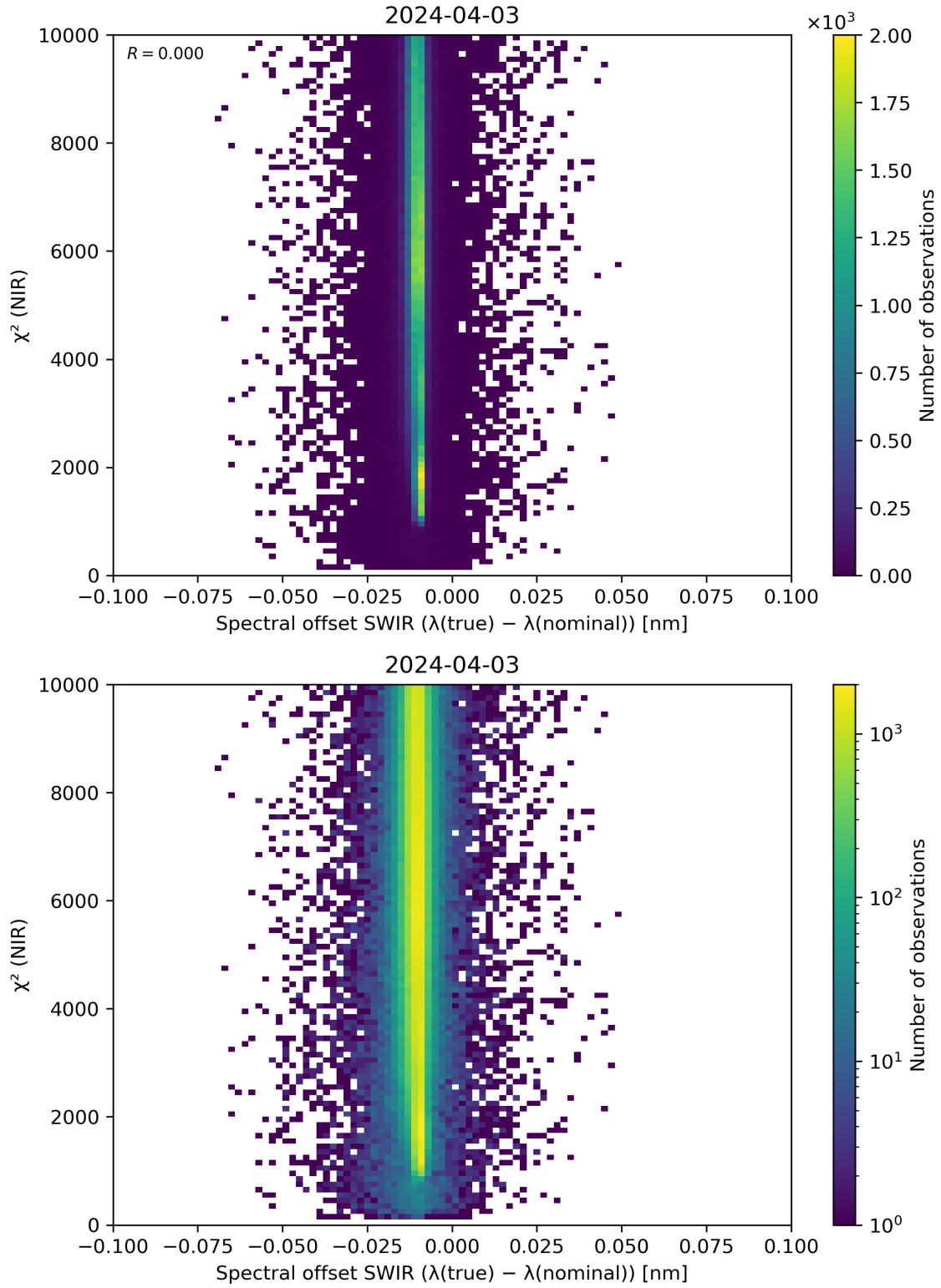
Figure 117: Scatter density plot of “Spectral offset SWIR ( \lambda(\text{true}) - \lambda(\text{nominal}) )” against “ \chi^2 (NIR)” for 2024-04-02 to 2024-04-04.
