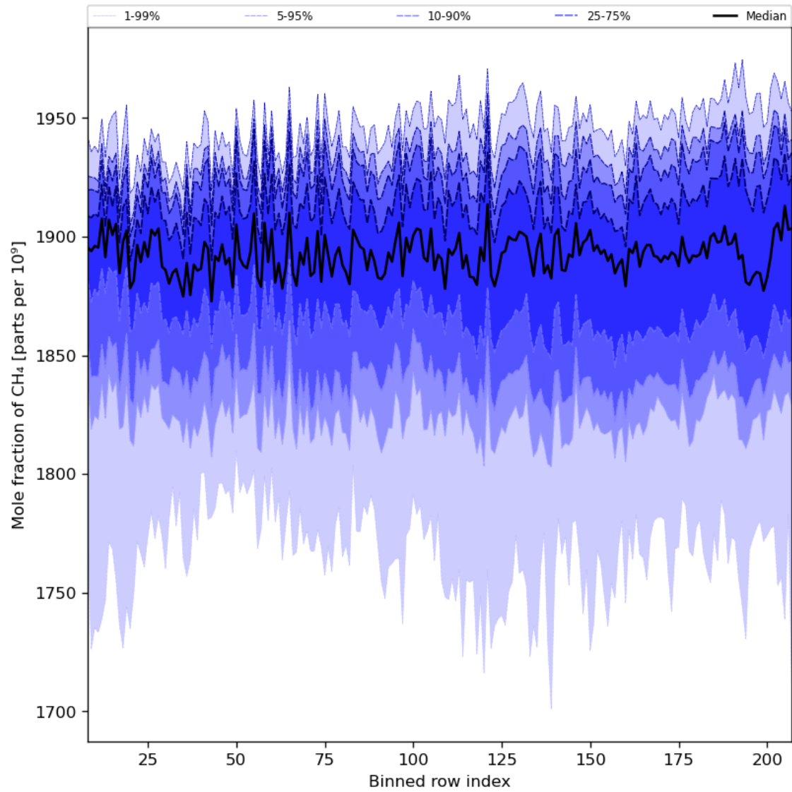
Figure 34: Along track statistics of “Mole fraction of CH 4 ” for 2024-04-02 to 2024-04-04
