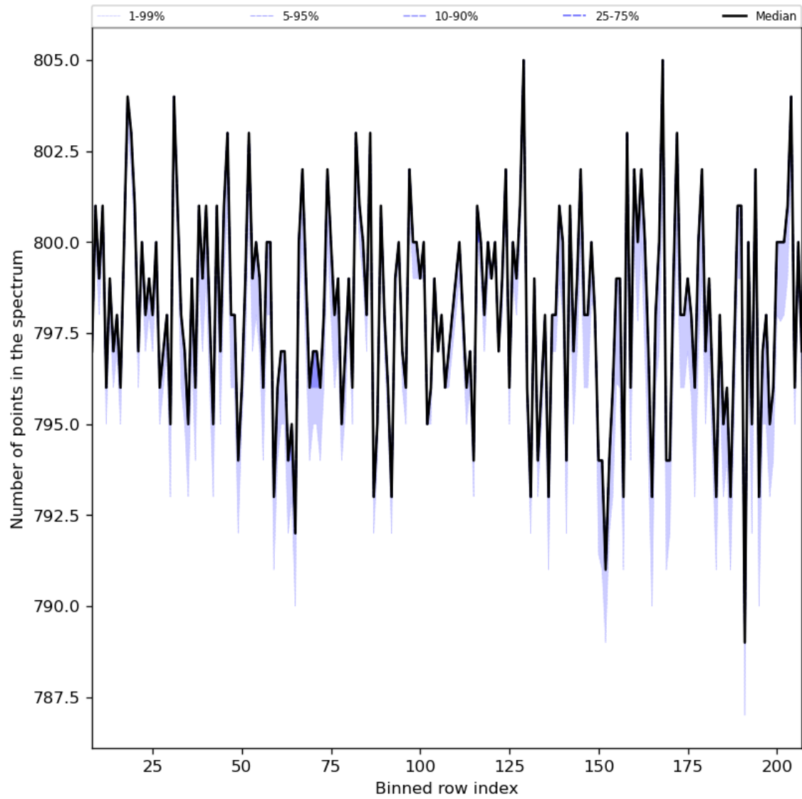
Figure 37: Along track statistics of “Number of points in the spectrum” for 2024-04-02 to 2024-04-04
