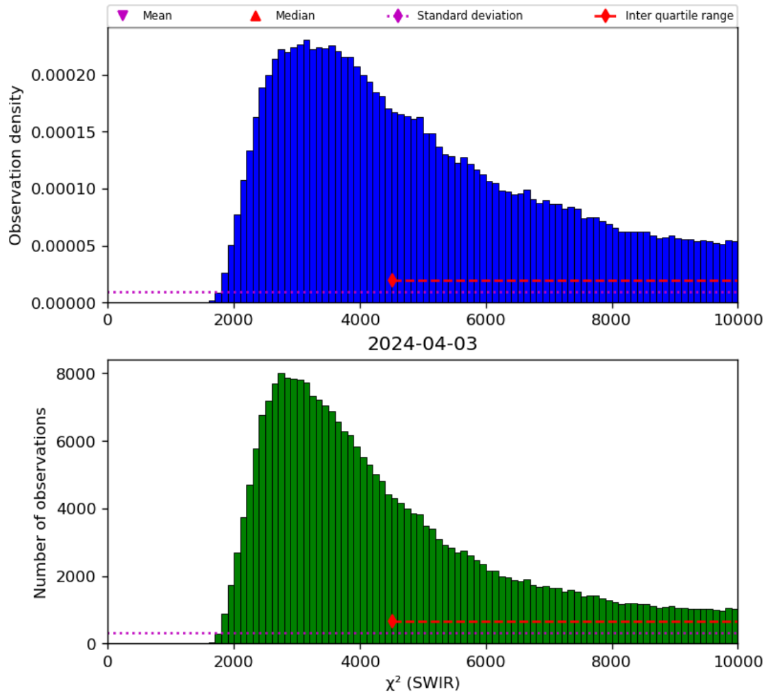
Figure 28: Histogram of “ \chi^2 (SWIR)” for 2024-04-02 to 2024-04-04
