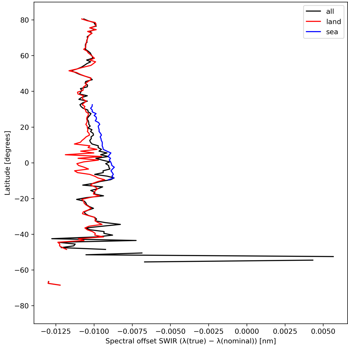
Figure 16: Zonal average of “Spectral offset SWIR ( \lambda(\text{true}) - \lambda(\text{nominal}) )” for 2024-04-02 to 2024-04-04.
