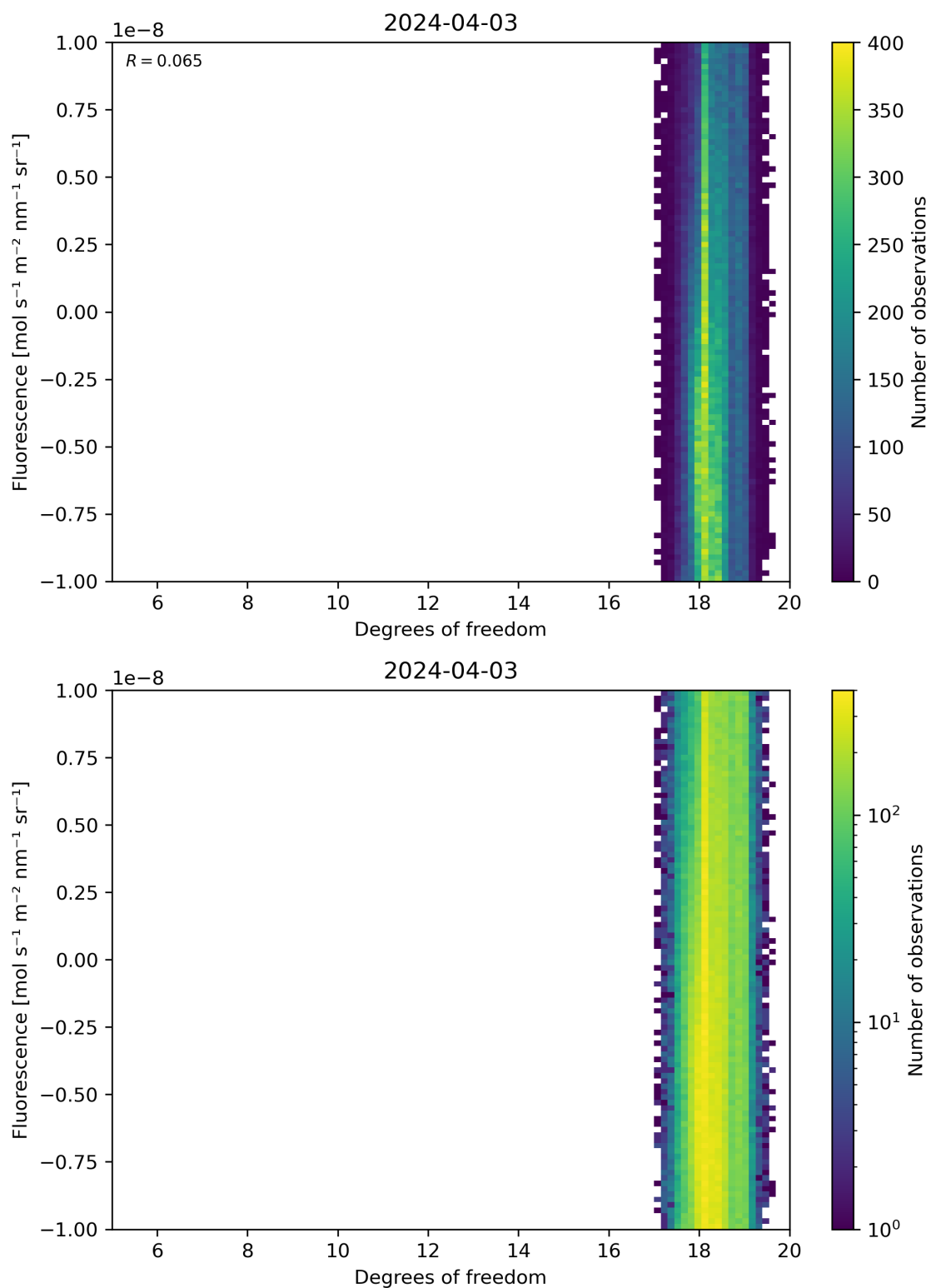
Figure 51: Scatter density plot of “Degrees of freedom” against “Fluorescence” for 2024-04-02 to 2024-04-04.
