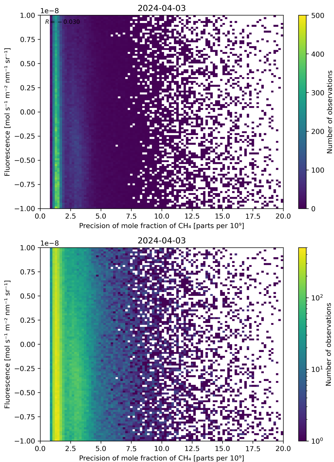
Figure 81: Scatter density plot of “Precision of mole fraction of \text{CH}_4 ” against “Fluorescence” for 2024-04-02 to 2024-04-04.
