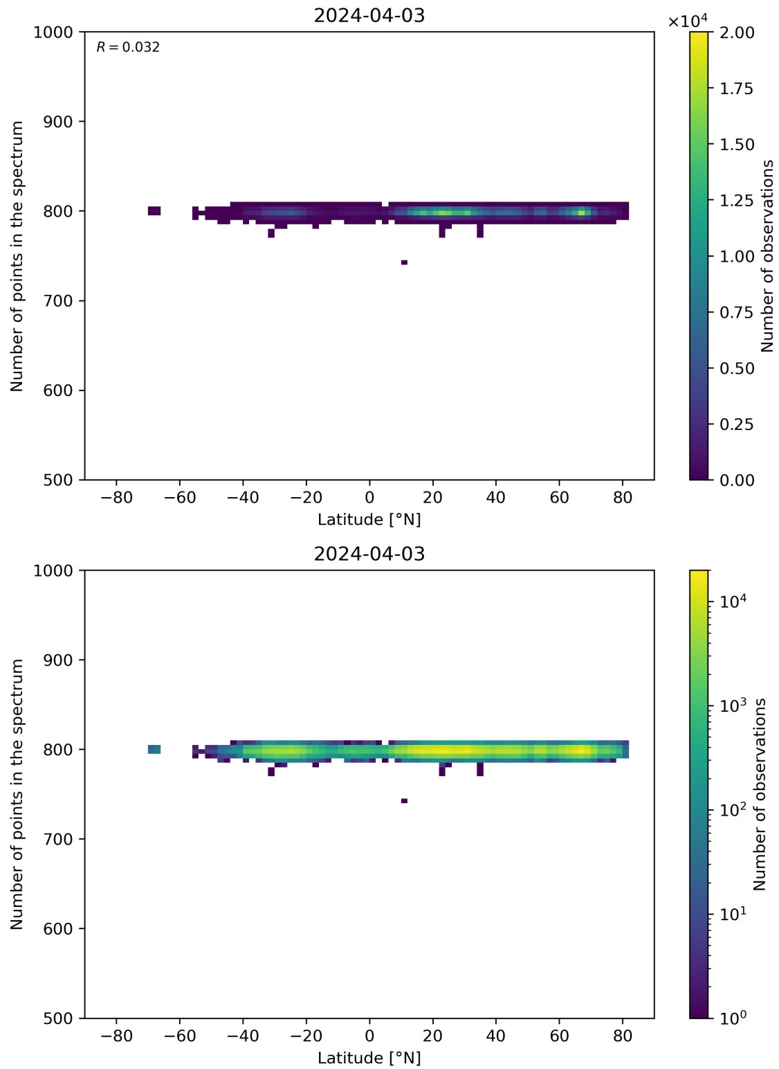
Figure 61: Scatter density plot of “Latitude” against “Number of points in the spectrum” for 2024-04-02 to 2024-04-04.
