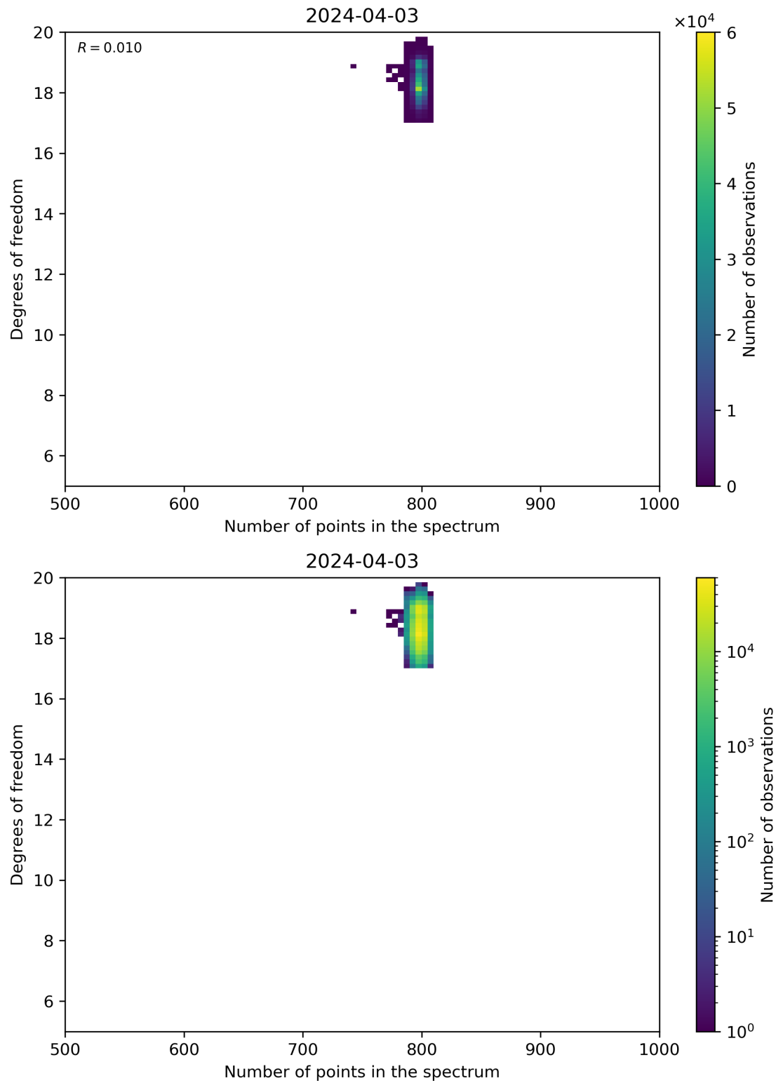
Figure 90: Scatter density plot of “Number of points in the spectrum” against “Degrees of freedom” for 2024-04-02 to 2024-04-04.
