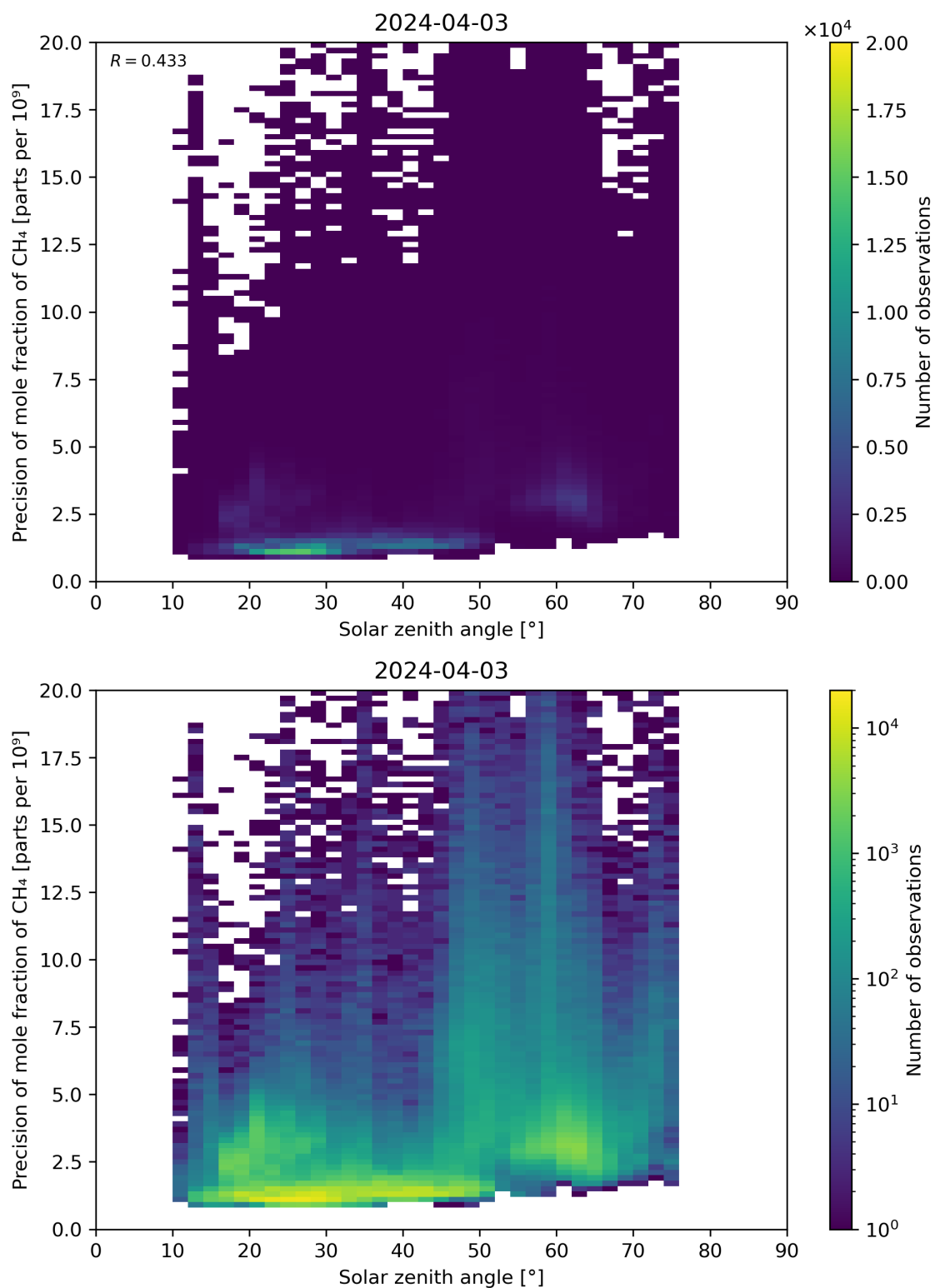
Figure 101: Scatter density plot of “Solar zenith angle” against “Precision of mole fraction of CH 4 ” for 2024-04-02 to 2024-04-04.
