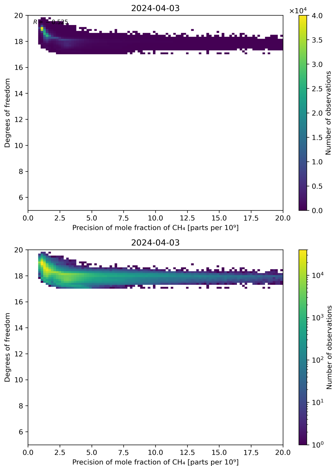
Figure 80: Scatter density plot of “Precision of mole fraction of CH 4 ” against “Degrees of freedom” for 2024-04-02 to 2024-04-04.
