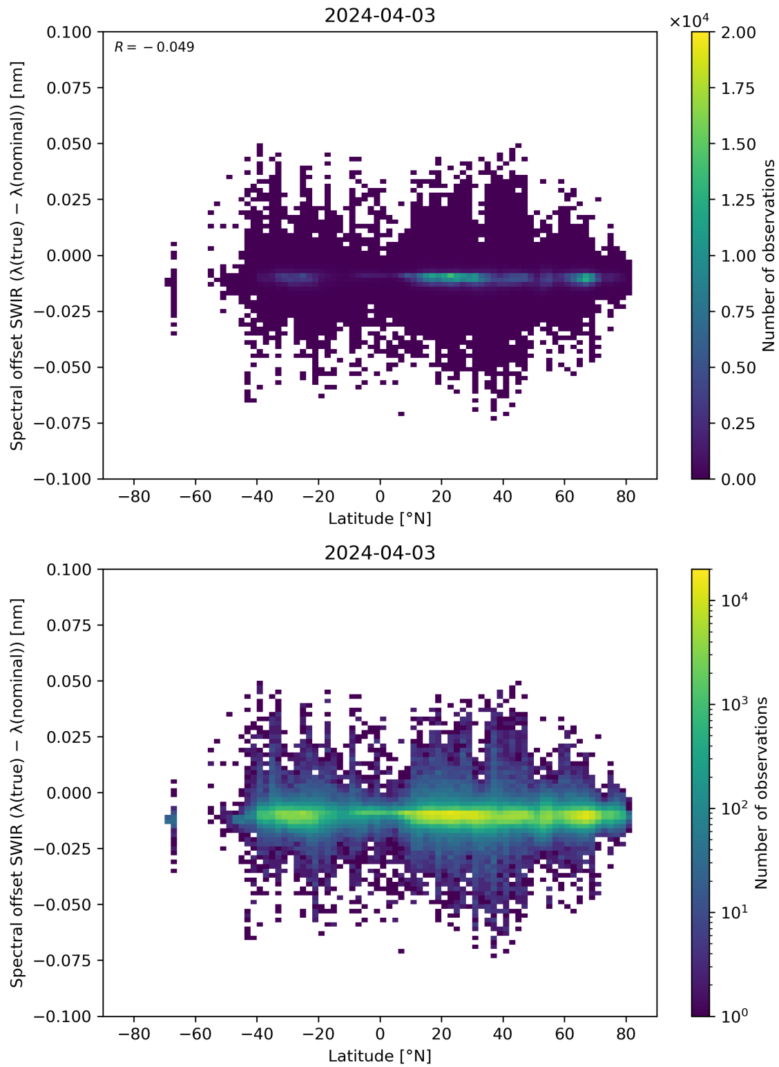
Figure 62: Scatter density plot of “Latitude” against “Spectral offset SWIR ( \lambda(\text{true}) - \lambda(\text{nominal}) )” for 2024-04-02 to 2024-04-04.
