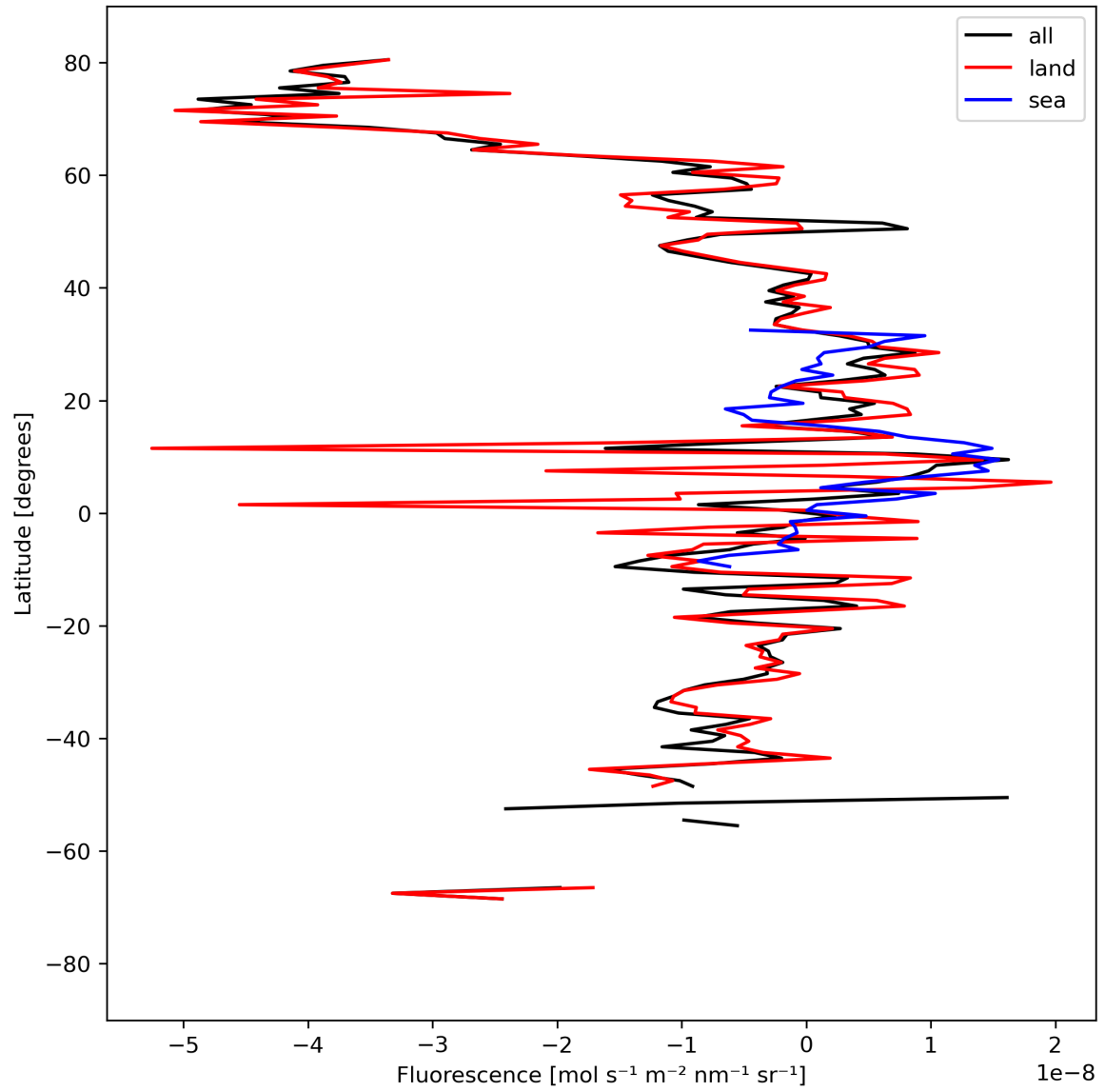
Figure 21: Zonal average of “Fluorescence” for 2024-04-02 to 2024-04-04.
