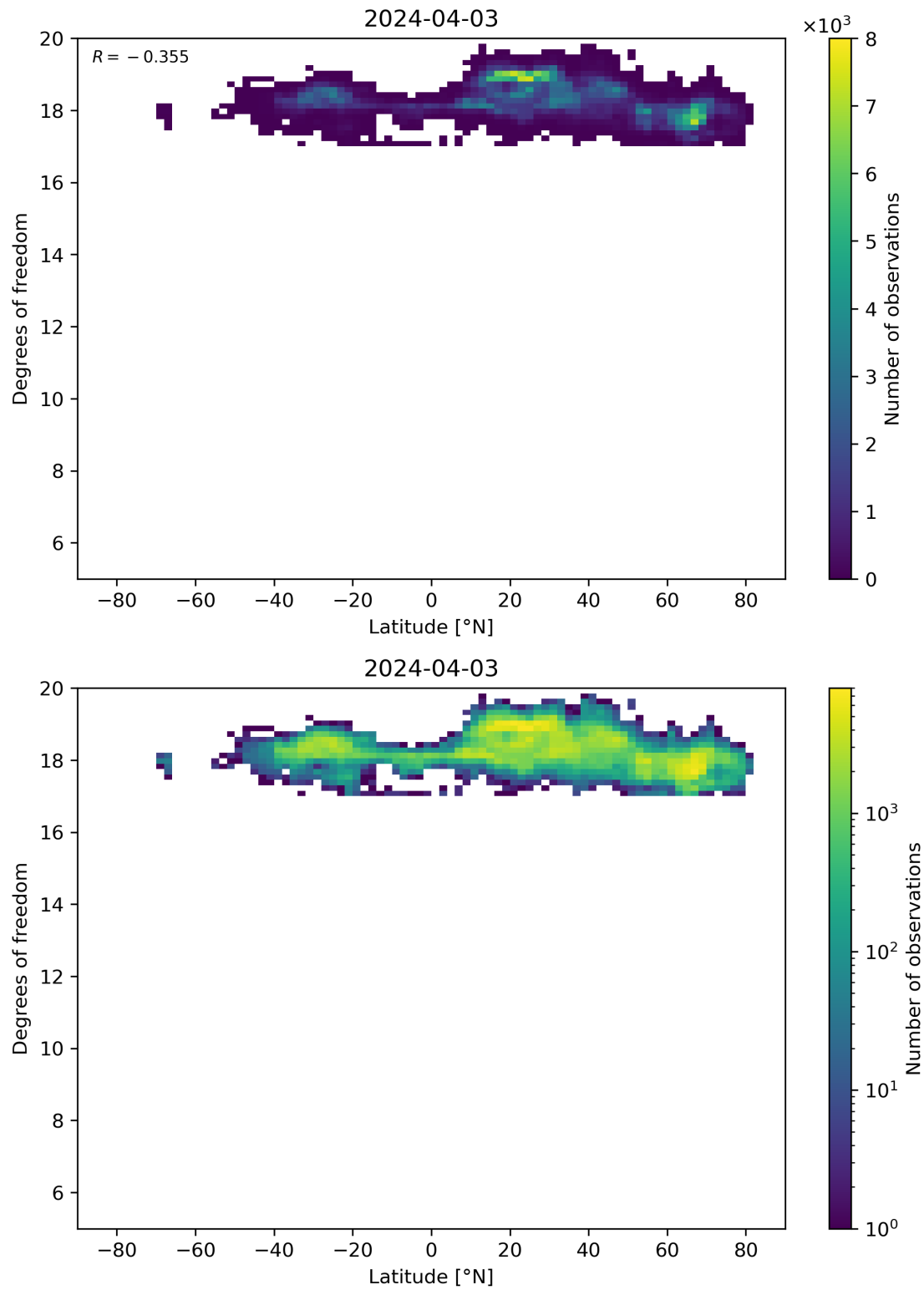
Figure 55: Scatter density plot of “Latitude” against “Degrees of freedom” for 2024-04-02 to 2024-04-04.
