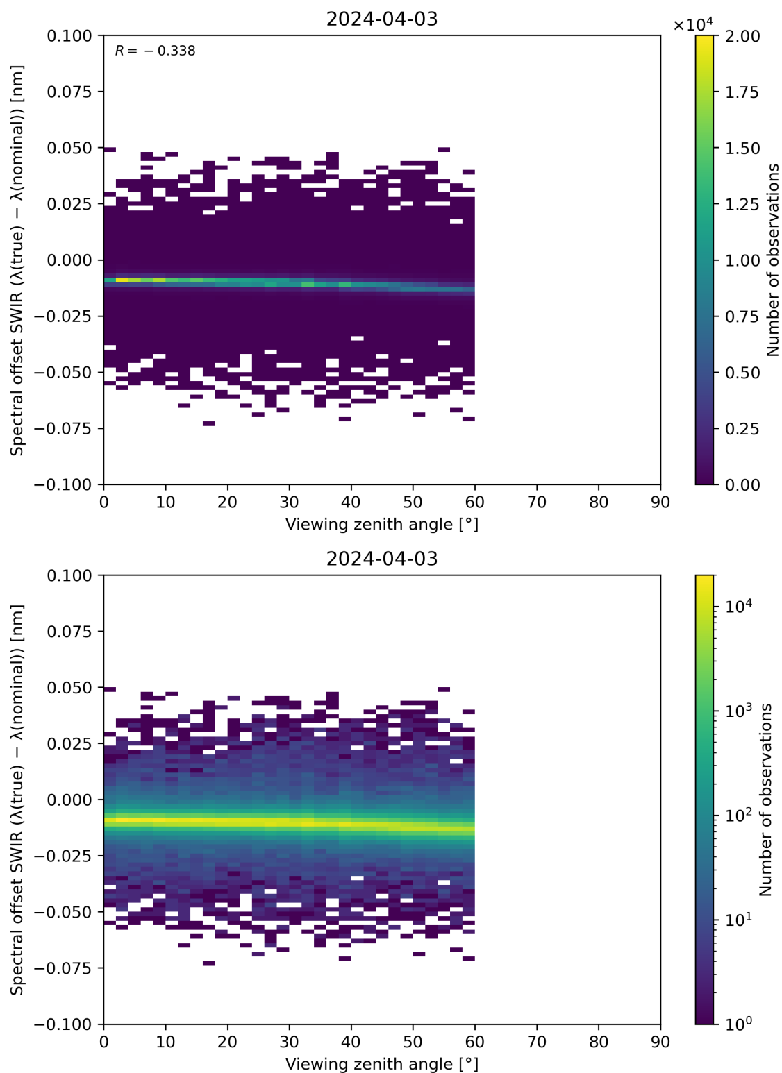
Figure 116: Scatter density plot of “Viewing zenith angle” against “Spectral offset SWIR ( \lambda(\text{true}) - \lambda(\text{nominal}) )” for 2024-04-02 to 2024-04-04.
