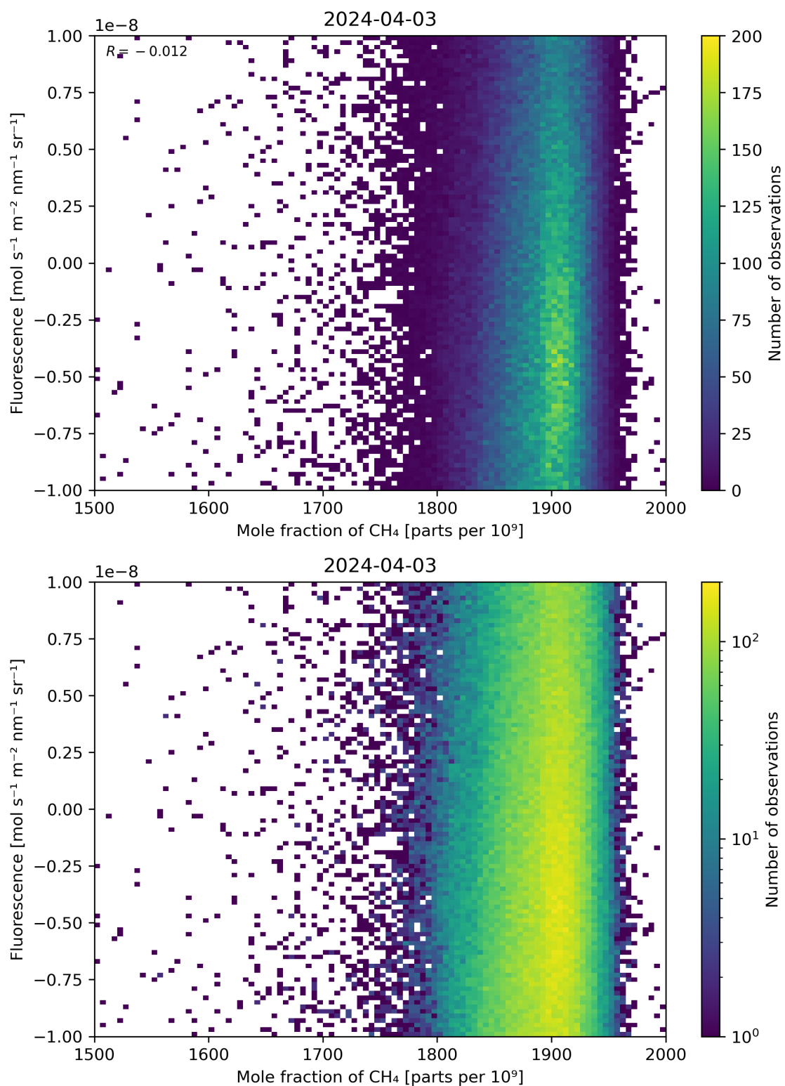
Figure 73: Scatter density plot of “Mole fraction of \text{CH}_4 ” against “Fluorescence” for 2024-04-02 to 2024-04-04.
