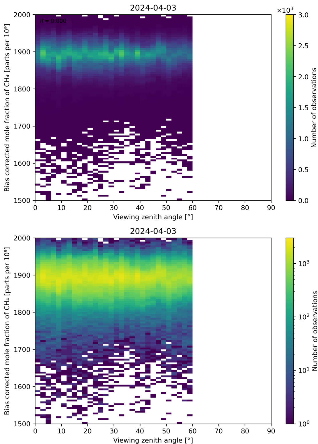
Figure 111: Scatter density plot of “Viewing zenith angle” against “Bias corrected mole fraction of CH 4 ” for 2024-04-02 to 2024-04-04.
