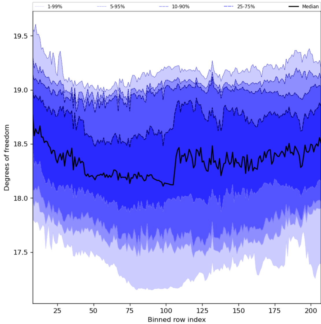
Figure 41: Along track statistics of “Degrees of freedom” for 2024-04-02 to 2024-04-04
