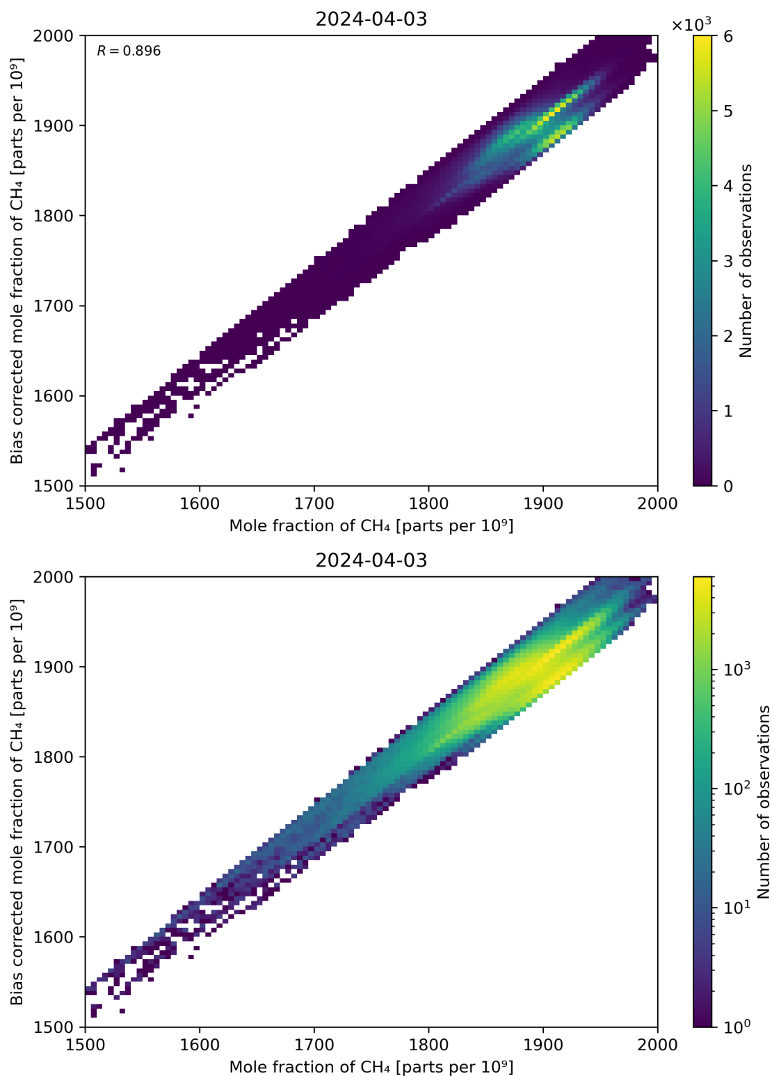
Figure 74: Scatter density plot of “Mole fraction of CH 4 ” against “Bias corrected mole fraction of CH 4 ” for 2024-04-02 to 2024-04-04.
