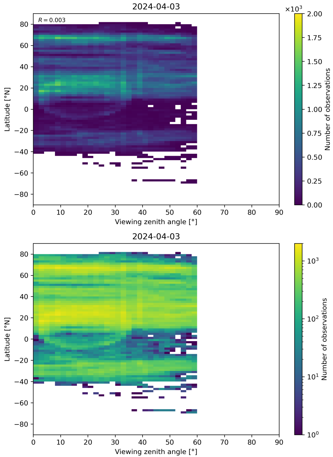
Figure 109: Scatter density plot of “Viewing zenith angle” against “Latitude” for 2024-04-02 to 2024-04-04.
