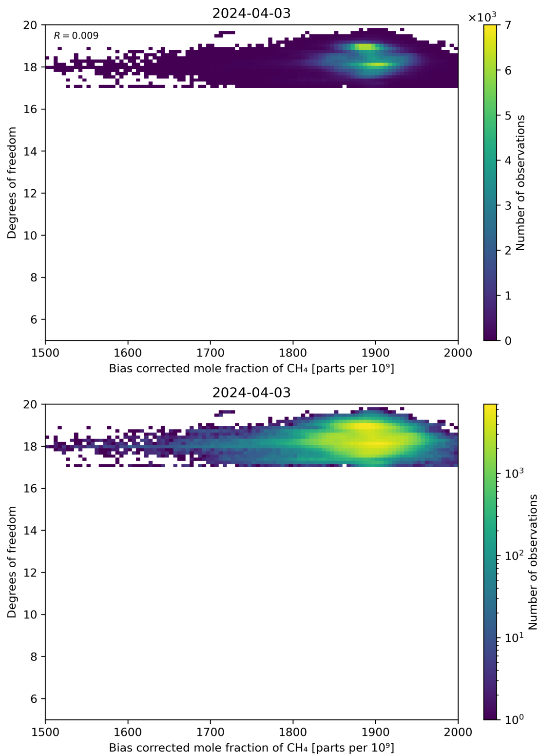
Figure 65: Scatter density plot of “Bias corrected mole fraction of CH 4 ” against “Degrees of freedom” for 2024-04-02 to 2024-04-04.
