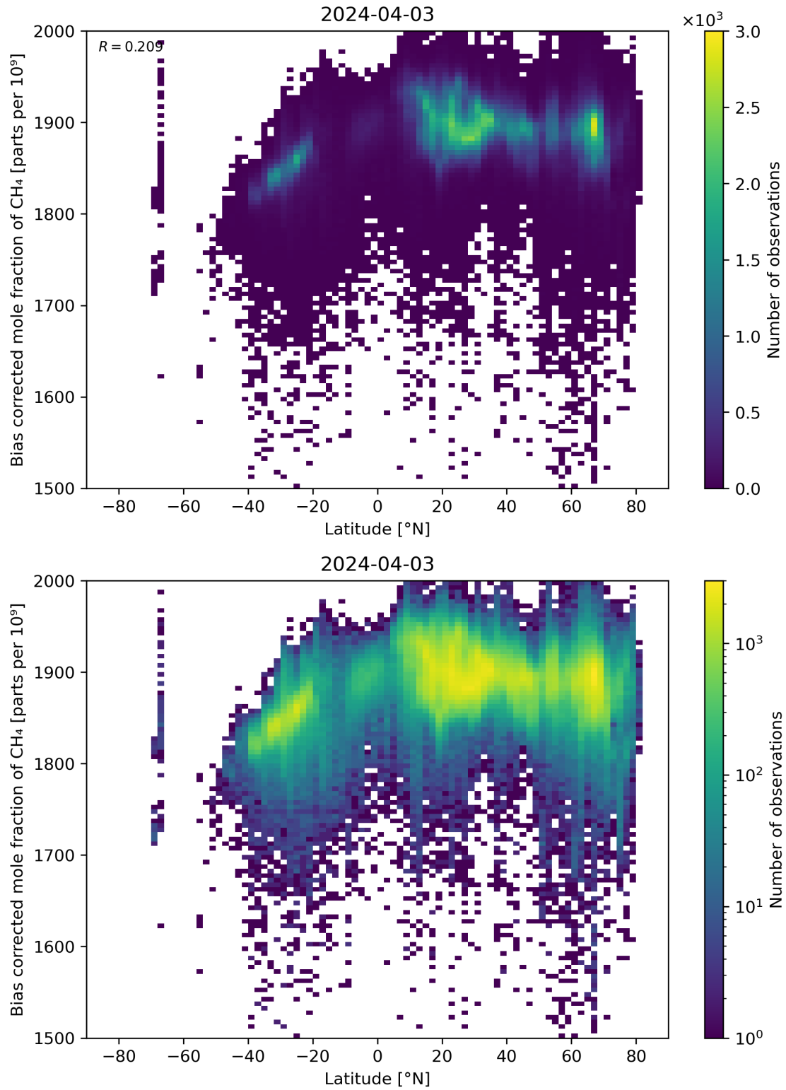
Figure 58: Scatter density plot of “Latitude” against “Bias corrected mole fraction of \text{CH}_4 ” for 2024-04-02 to 2024-04-04.
