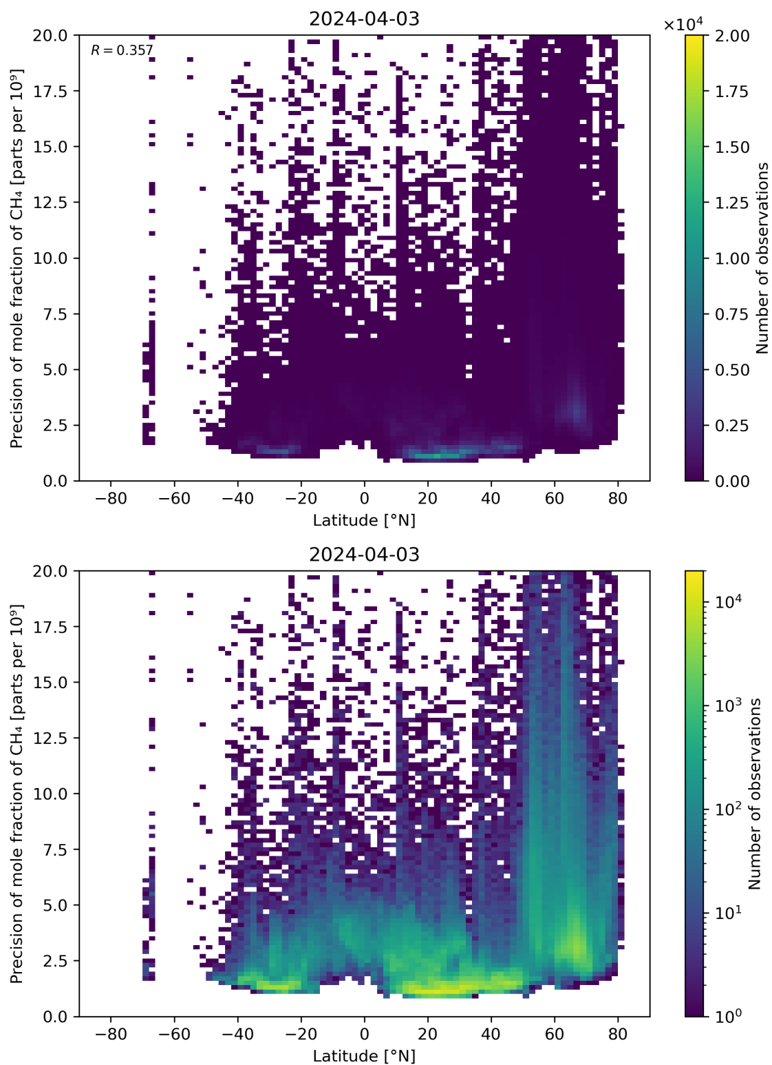
Figure 59: Scatter density plot of “Latitude” against “Precision of mole fraction of CH 4 ” for 2024-04-02 to 2024-04-04.
