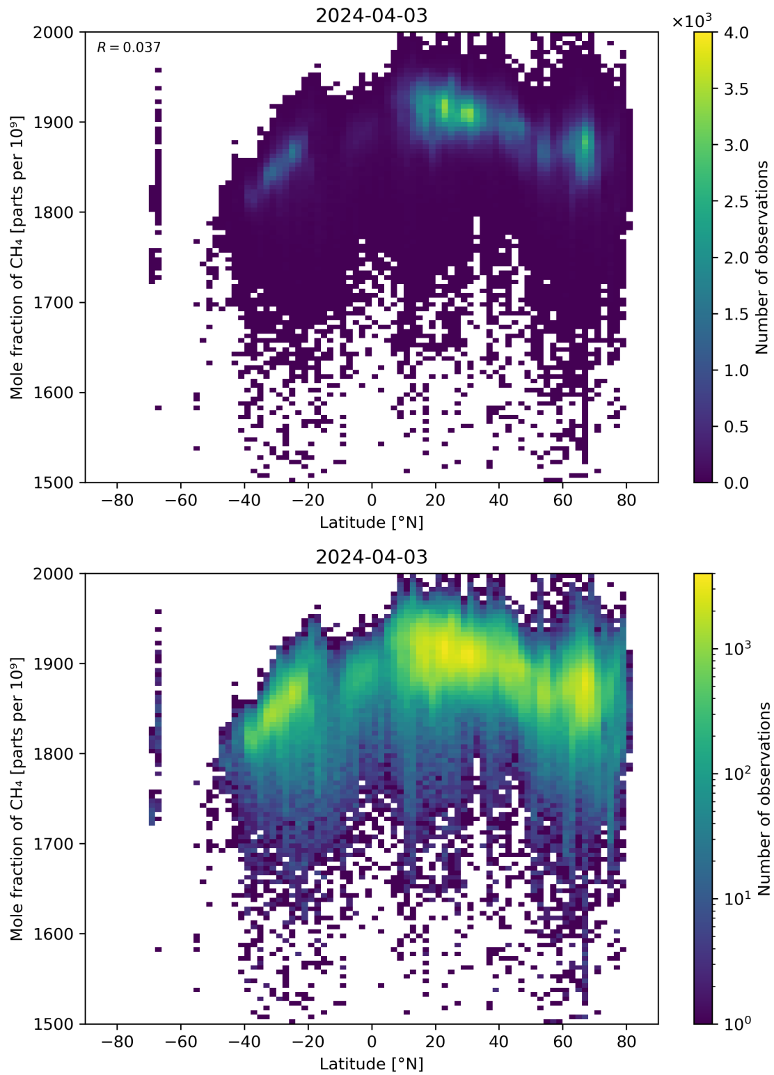
Figure 57: Scatter density plot of “Latitude” against “Mole fraction of CH 4 ” for 2024-04-02 to 2024-04-04.
