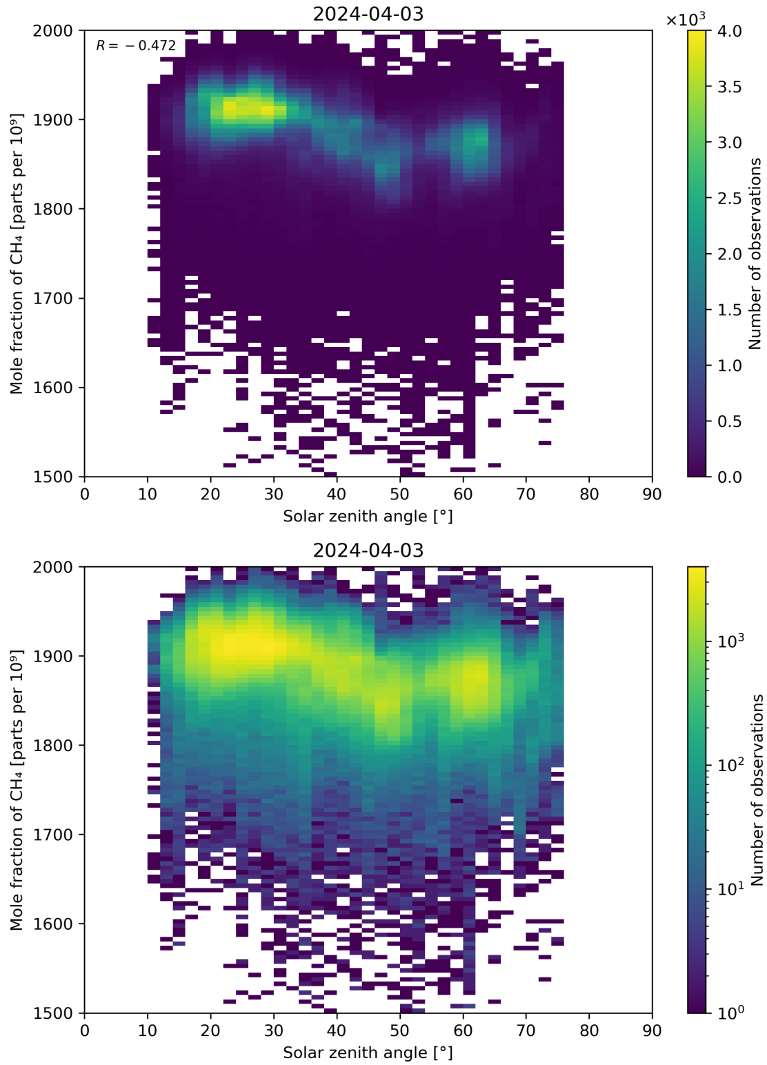
Figure 99: Scatter density plot of “Solar zenith angle” against “Mole fraction of \text{CH}_4 ” for 2024-04-02 to 2024-04-04.
