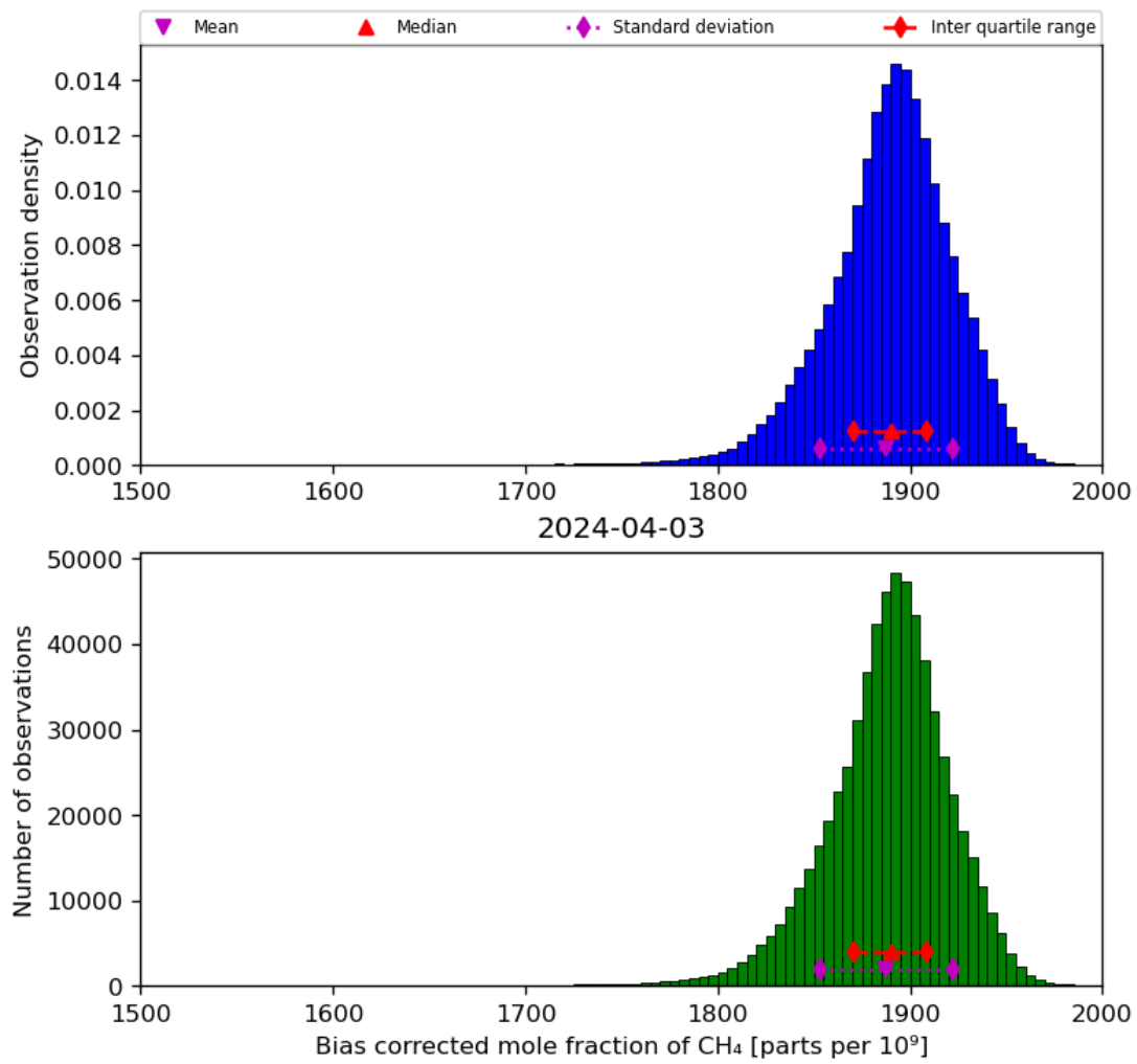
Figure 25: Histogram of “Bias corrected mole fraction of CH 4 ” for 2024-04-02 to 2024-04-04
