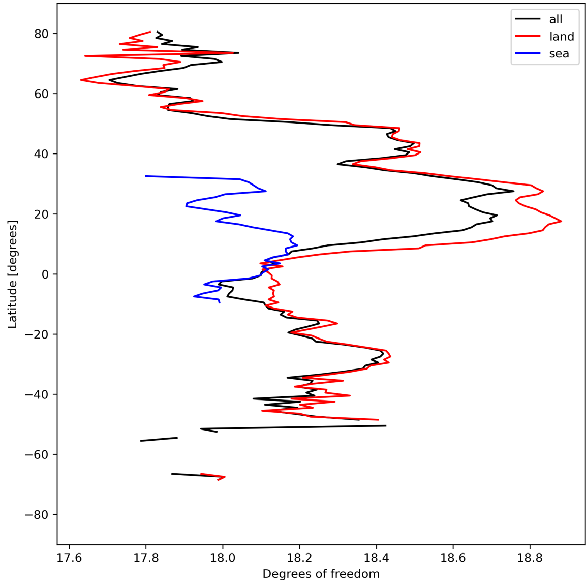
Figure 19: Zonal average of “Degrees of freedom” for 2024-04-02 to 2024-04-04.
