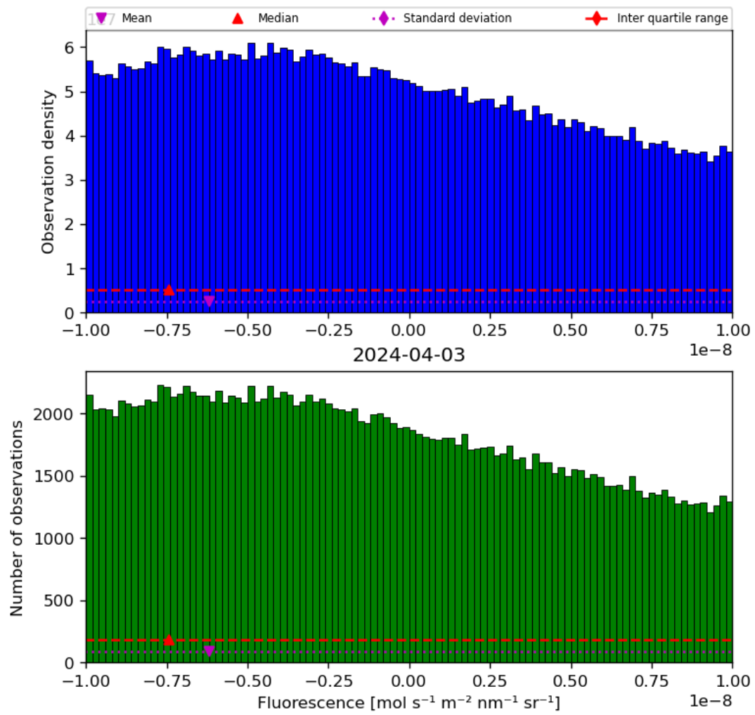
Figure 32: Histogram of “Fluorescence” for 2024-04-02 to 2024-04-04
