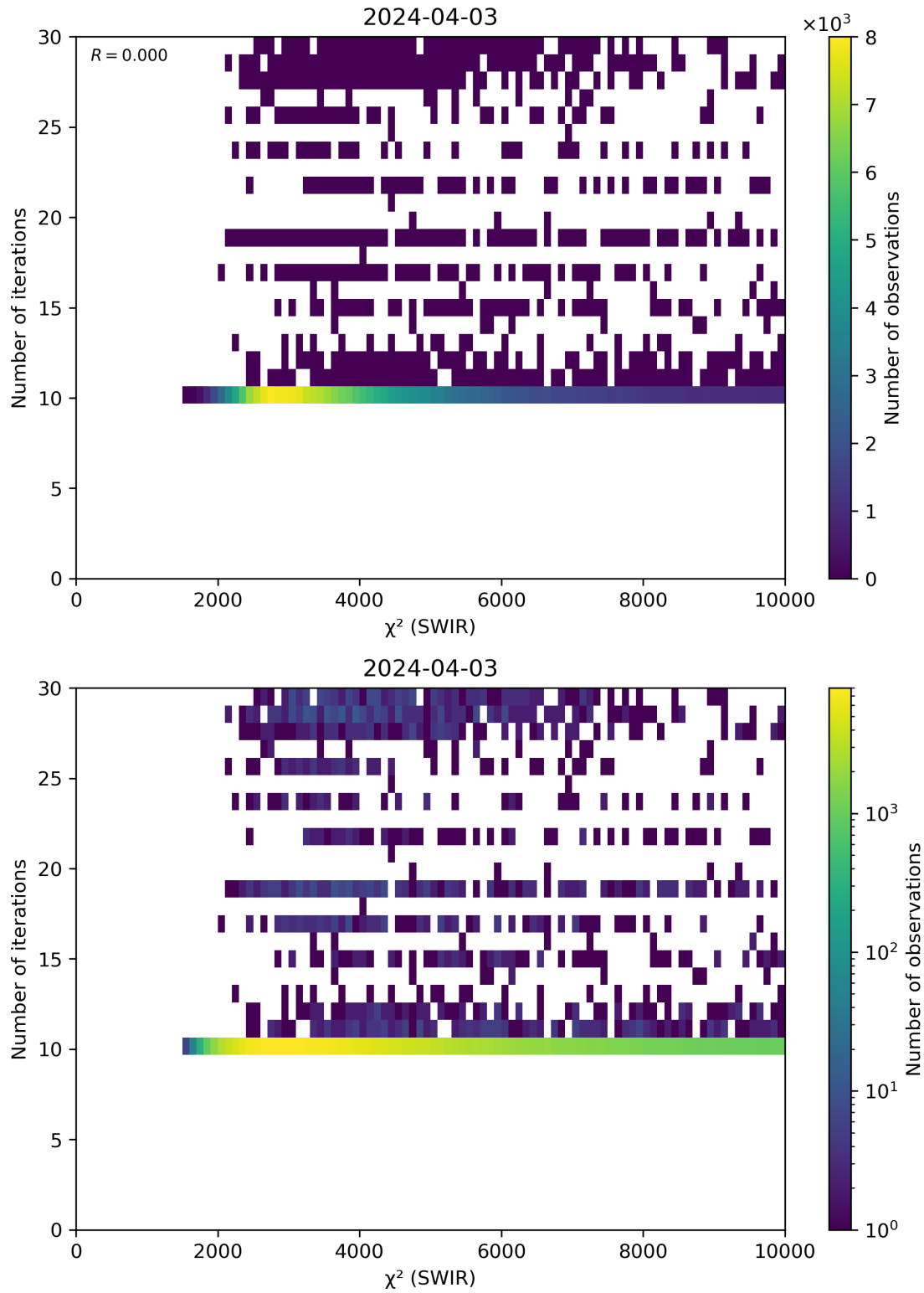
Figure 50: Scatter density plot of “ \chi^2 (SWIR)” against “Number of iterations” for 2024-04-02 to 2024-04-04.
