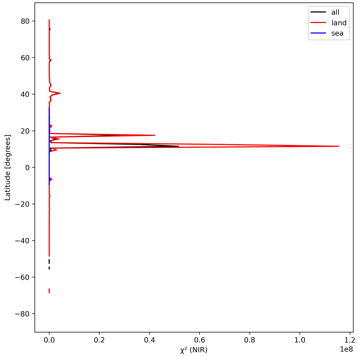
Figure 18: Zonal average of “ \chi^2 (NIR)” for 2024-04-02 to 2024-04-04.
