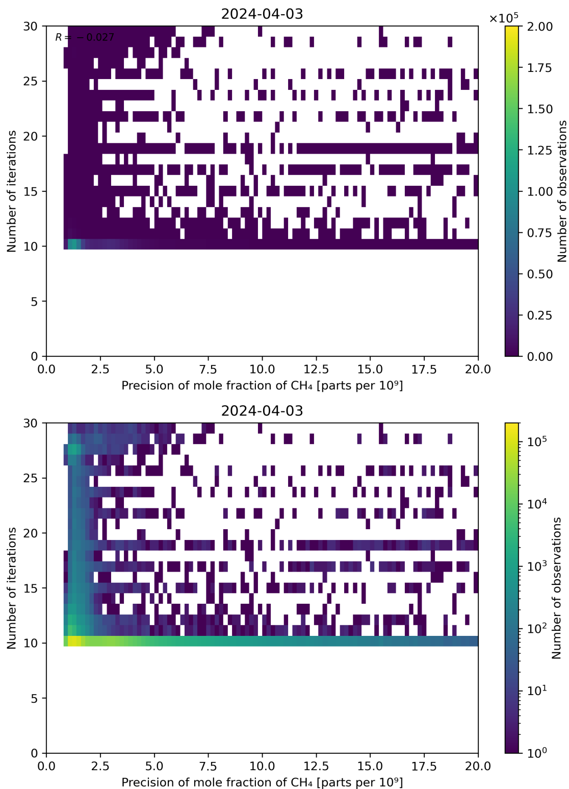
Figure 83: Scatter density plot of “Precision of mole fraction of CH 4 ” against “Number of iterations” for 2024-04-02 to 2024-04-04.
