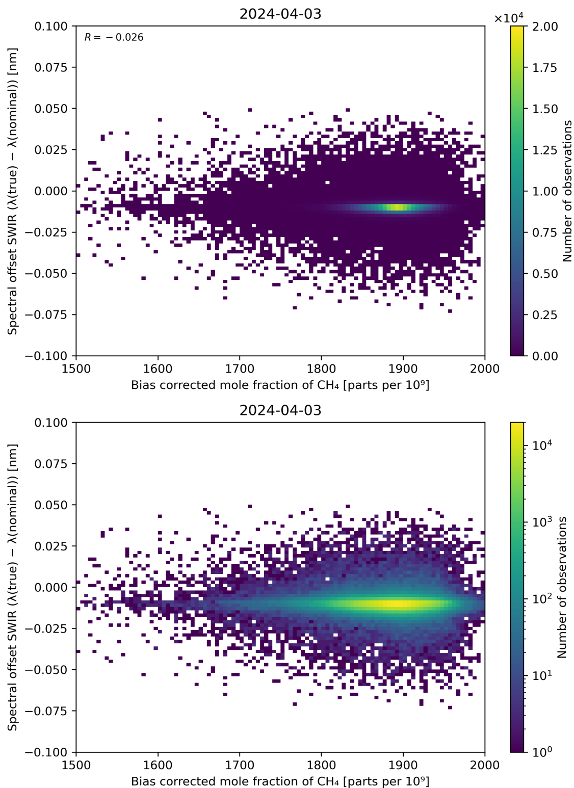
Figure 69: Scatter density plot of “Bias corrected mole fraction of \text{CH}_4 ” against “Spectral offset SWIR ( \lambda(\text{true}) - \lambda(\text{nominal}) )” for 2024-04-02 to 2024-04-04.
