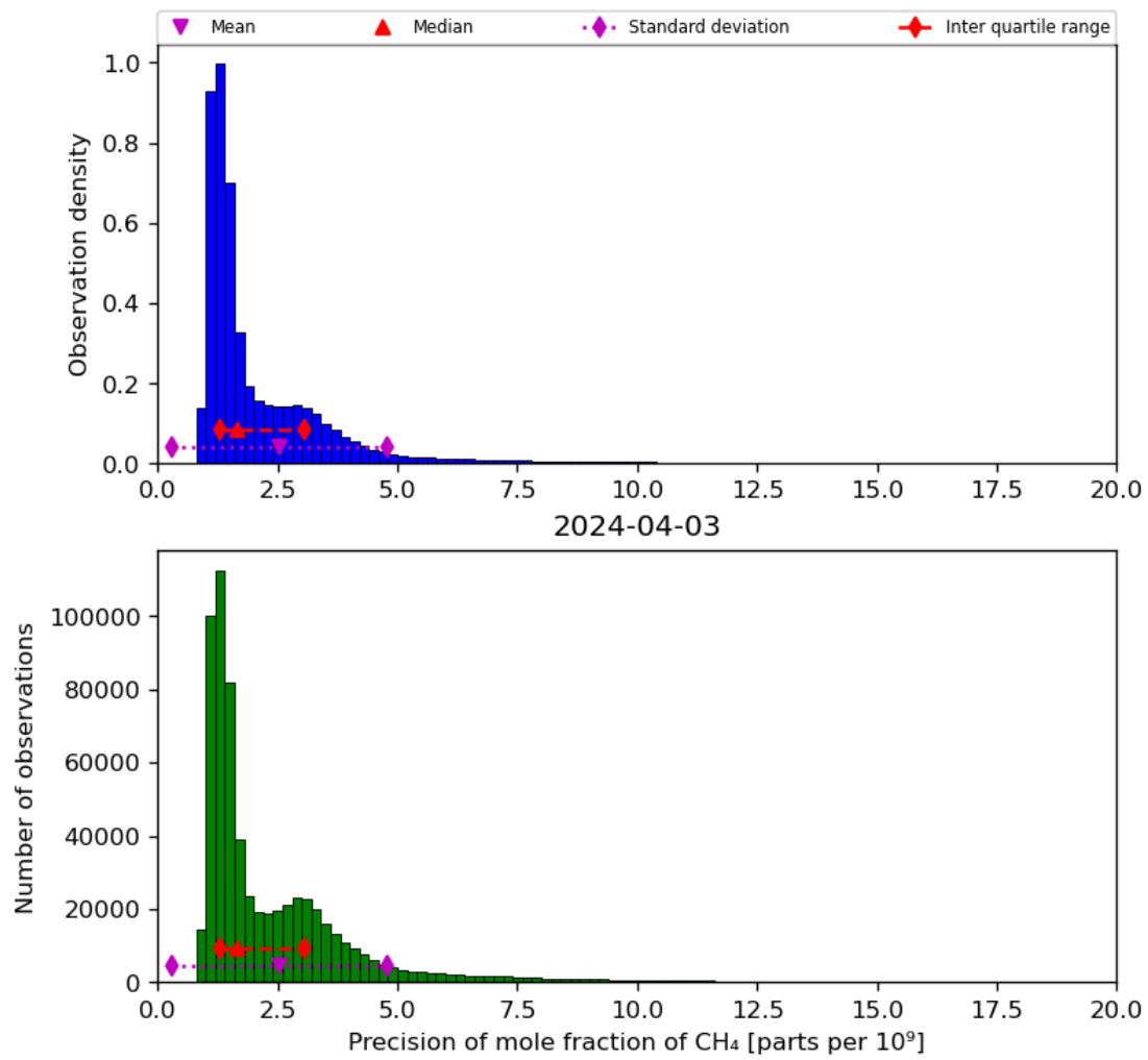
Figure 24: Histogram of “Precision of mole fraction of CH 4 ” for 2024-04-02 to 2024-04-04
