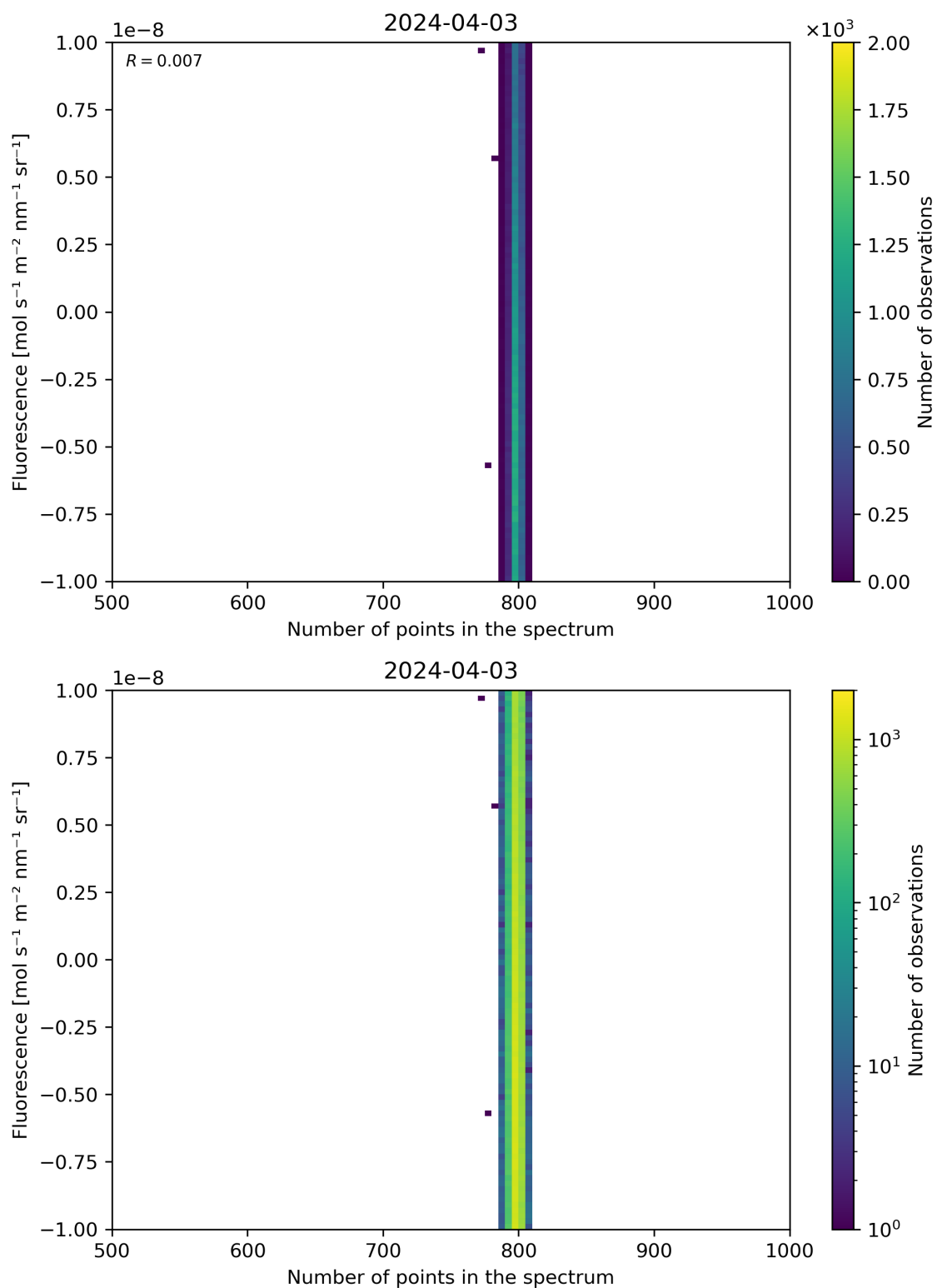
Figure 91: Scatter density plot of “Number of points in the spectrum” against “Fluorescence” for 2024-04-02 to 2024-04-04.
