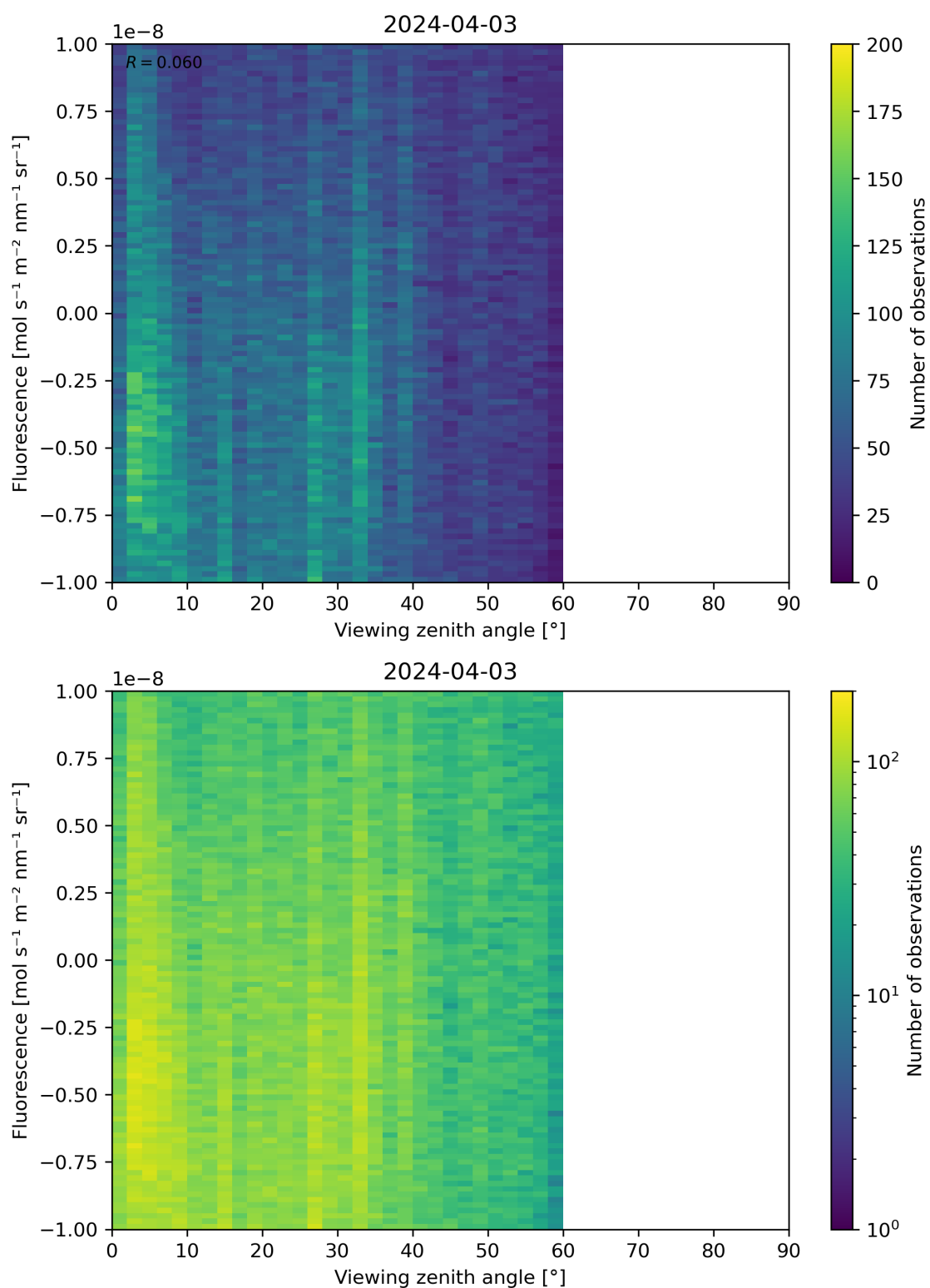
Figure 108: Scatter density plot of “Viewing zenith angle” against “Fluorescence” for 2024-04-02 to 2024-04-04.
