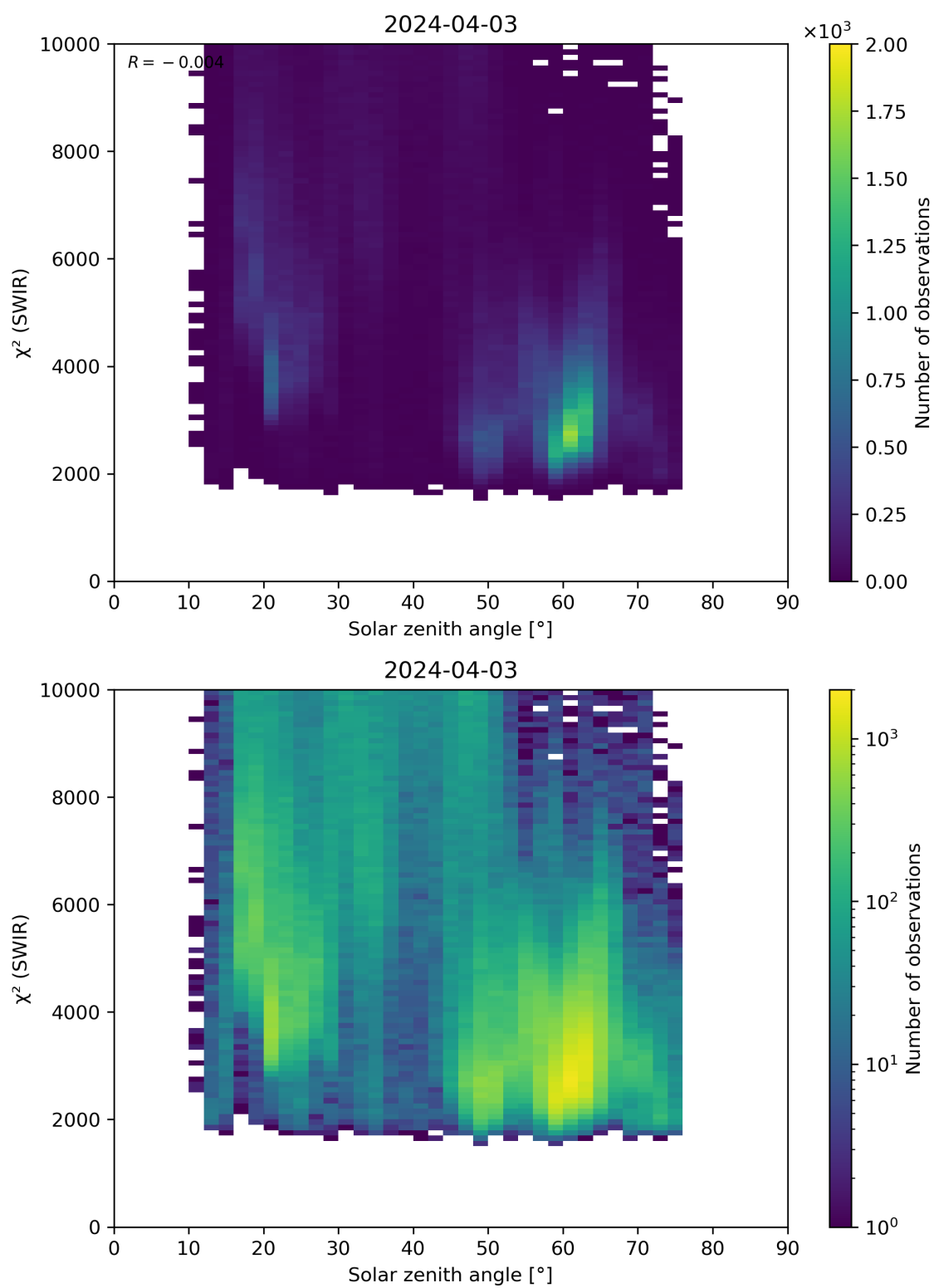
Figure 95: Scatter density plot of “Solar zenith angle” against “ \chi^2 (SWIR)” for 2024-04-02 to 2024-04-04.
