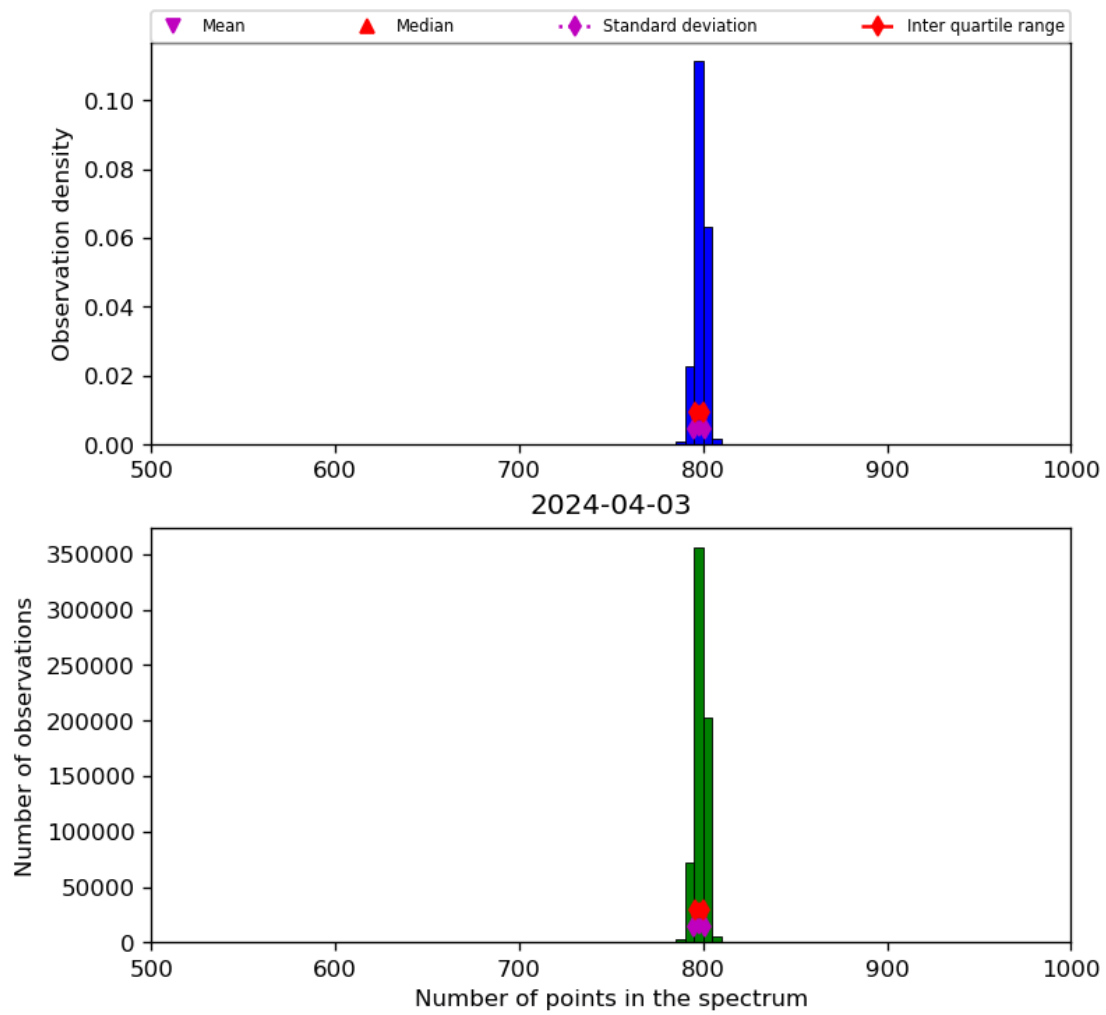
Figure 26: Histogram of “Number of points in the spectrum” for 2024-04-02 to 2024-04-04
