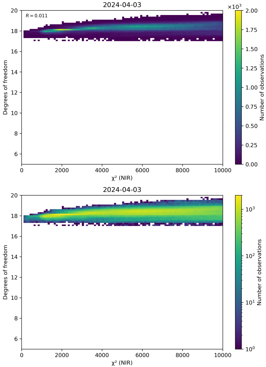
Figure 44: Scatter density plot of “ \chi^2 (NIR)” against “Degrees of freedom” for 2024-04-02 to 2024-04-04.
