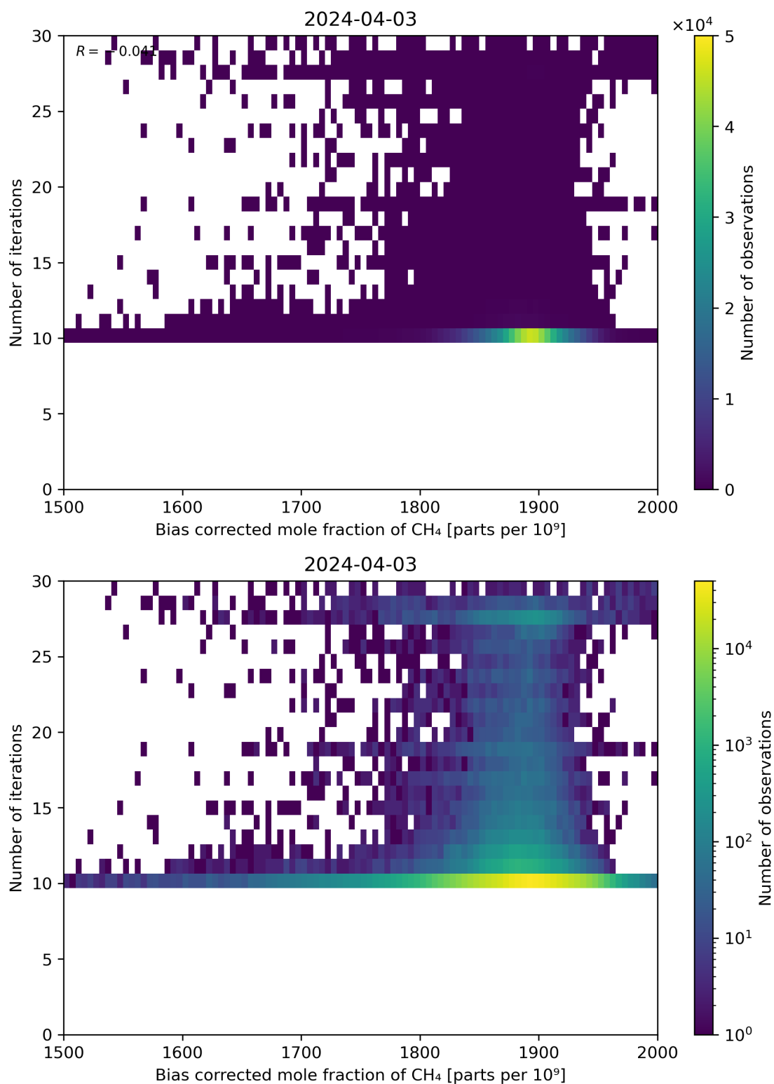
Figure 67: Scatter density plot of “Bias corrected mole fraction of CH 4 ” against “Number of iterations” for 2024-04-02 to 2024-04-04.
