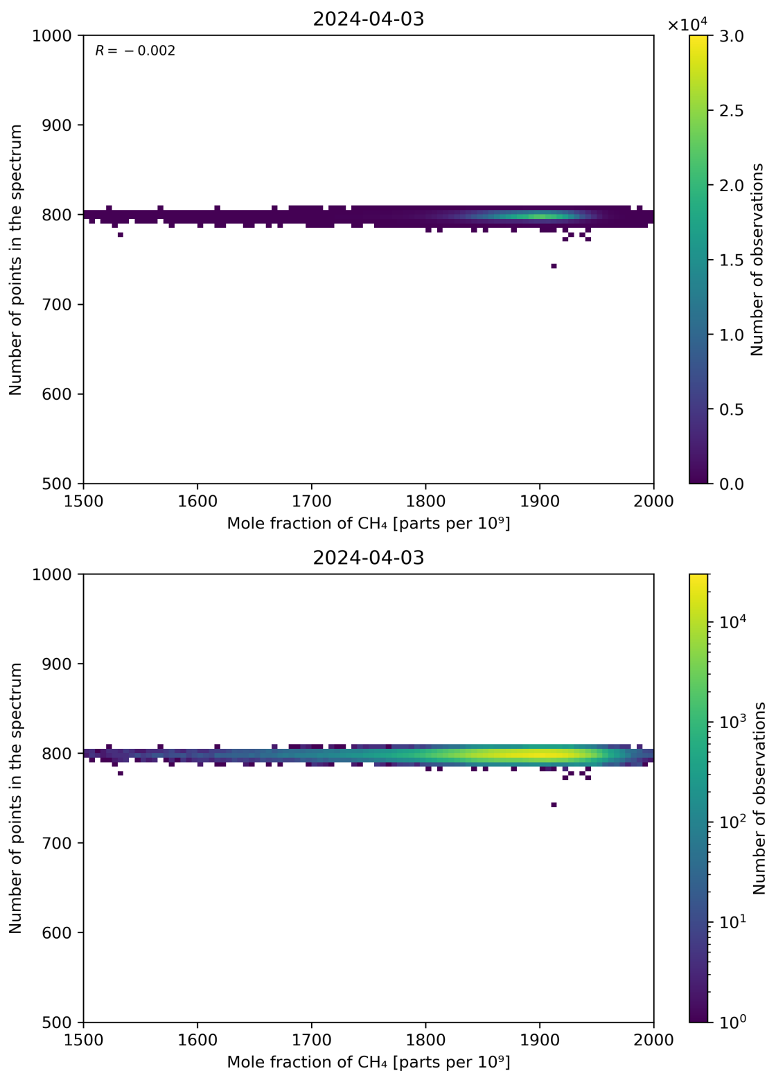
Figure 77: Scatter density plot of “Mole fraction of CH 4 ” against “Number of points in the spectrum” for 2024-04-02 to 2024-04-04.
