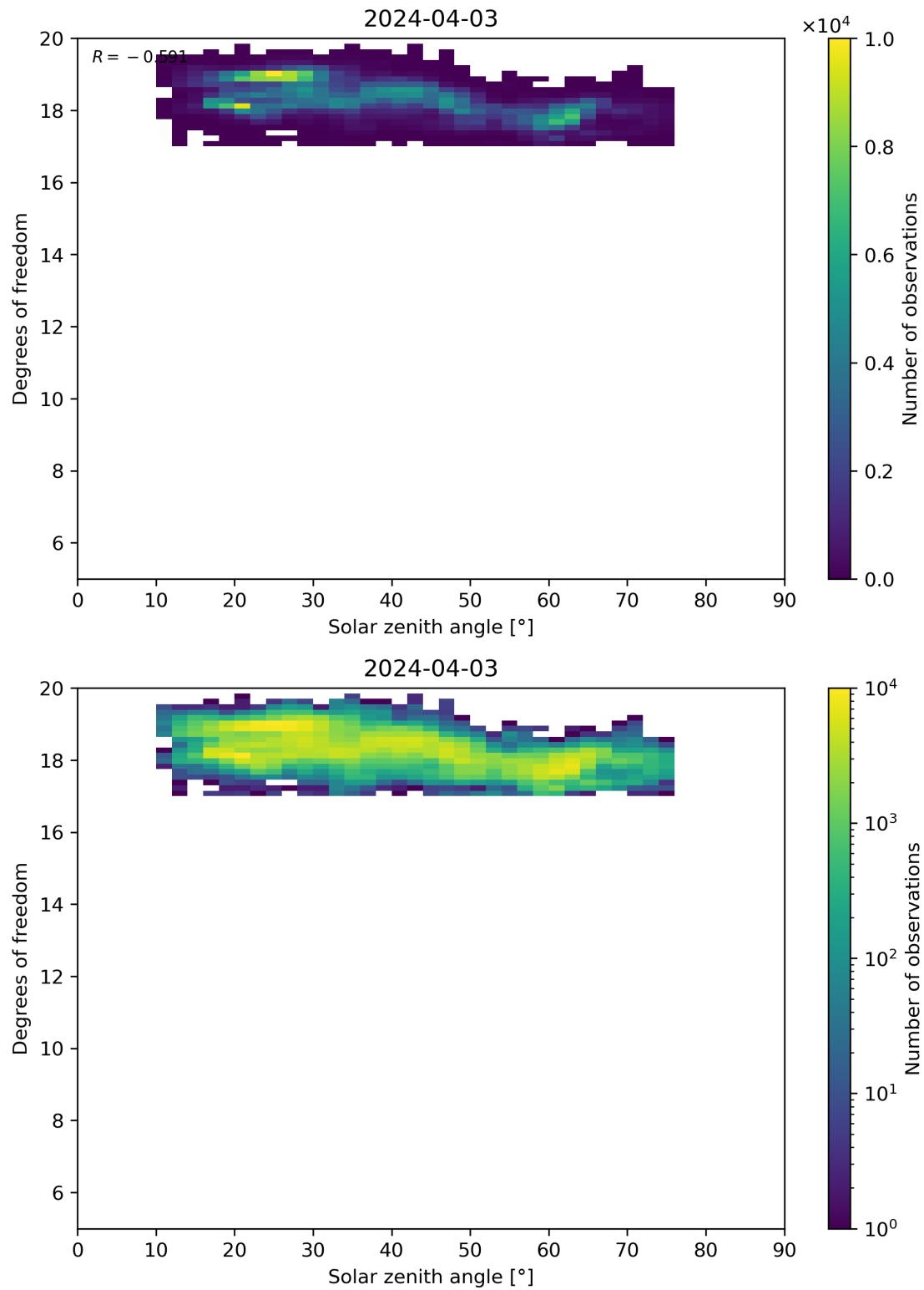
Figure 96: Scatter density plot of “Solar zenith angle” against “Degrees of freedom” for 2024-04-02 to 2024-04-04.
