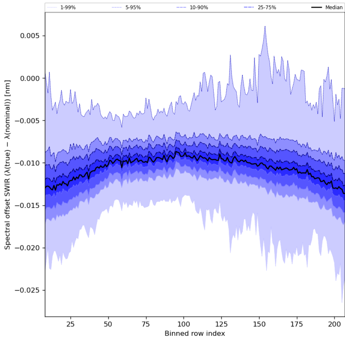
Figure 38: Along track statistics of “Spectral offset SWIR ( \lambda(\text{true}) - \lambda(\text{nominal}) )” for 2024-04-02 to 2024-04-04
