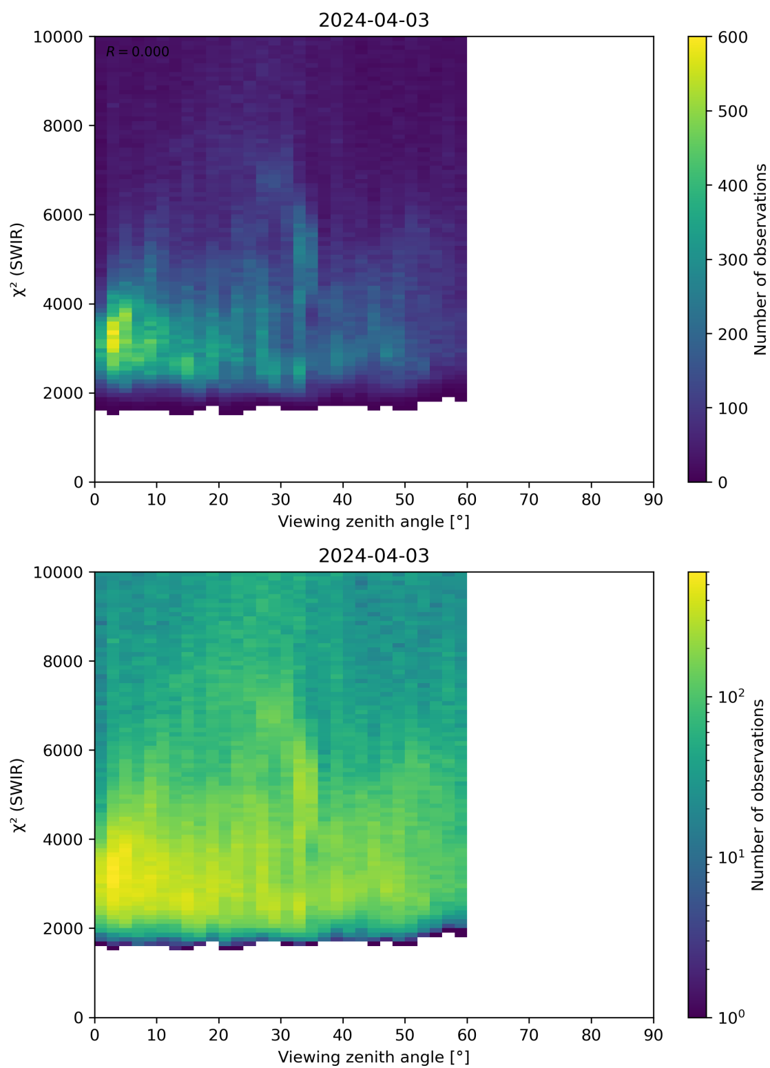
Figure 106: Scatter density plot of “Viewing zenith angle” against “ \chi^2 (SWIR)” for 2024-04-02 to 2024-04-04.
