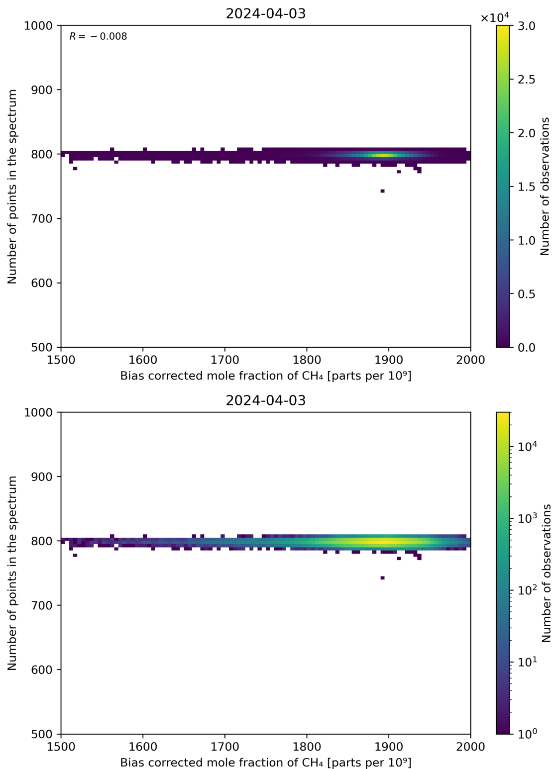
Figure 68: Scatter density plot of “Bias corrected mole fraction of CH 4 ” against “Number of points in the spectrum” for 2024-04-02 to 2024-04-04.
