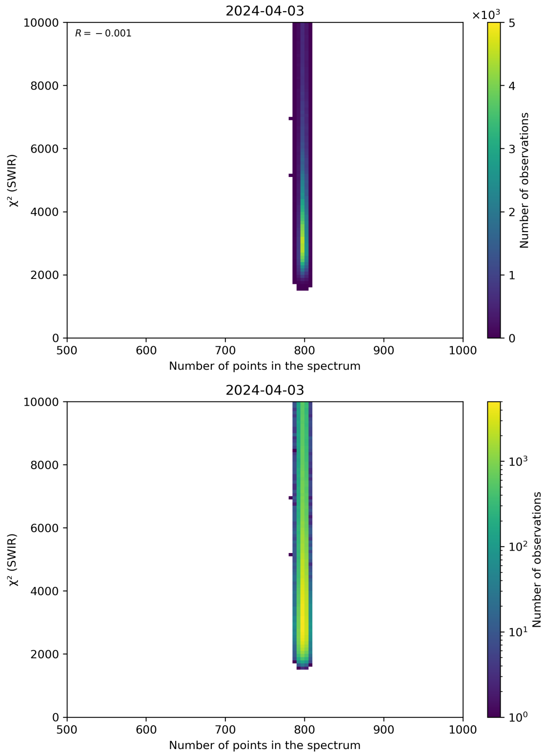
Figure 89: Scatter density plot of “Number of points in the spectrum” against “ \chi^2 (SWIR)” for 2024-04-02 to 2024-04-04.
