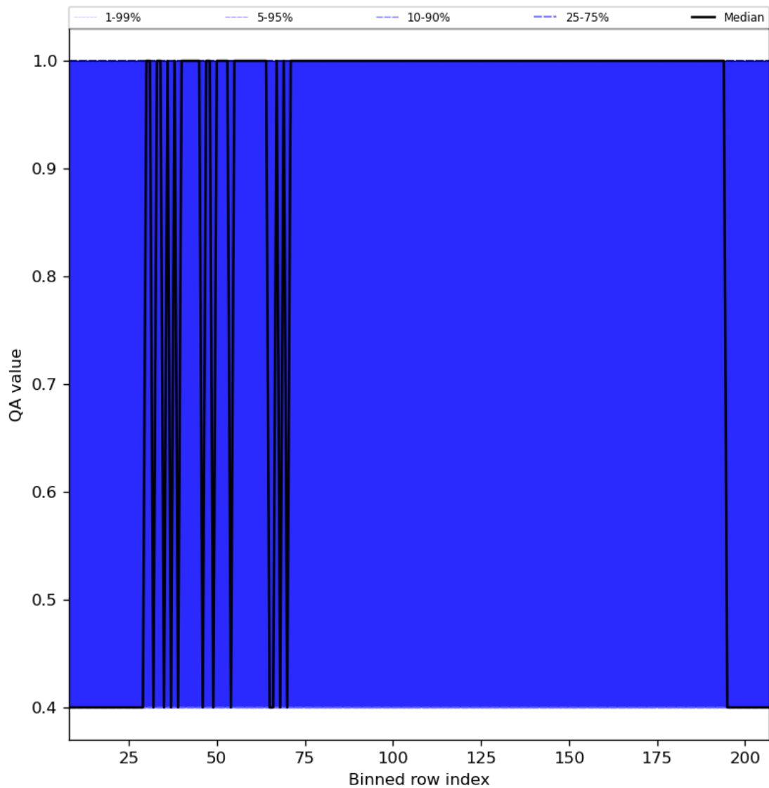
Figure 33: Along track statistics of “QA value” for 2024-04-02 to 2024-04-04
