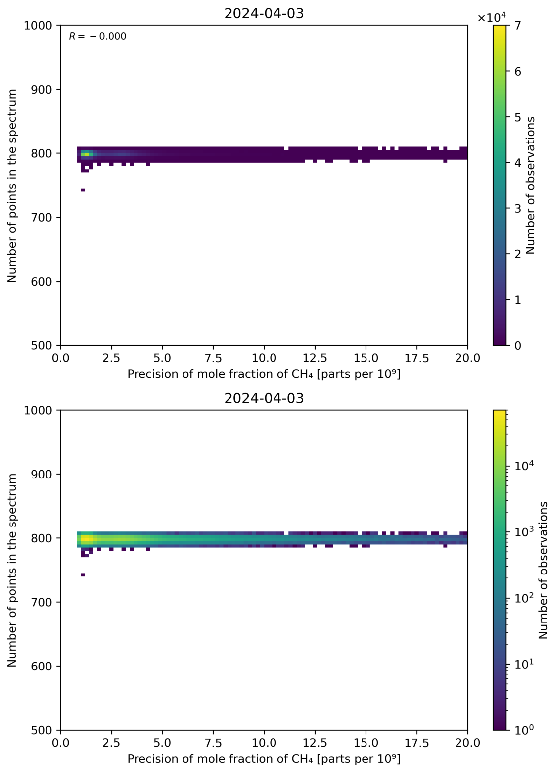
Figure 84: Scatter density plot of “Precision of mole fraction of CH 4 ” against “Number of points in the spectrum” for 2024-04-02 to 2024-04-04.
