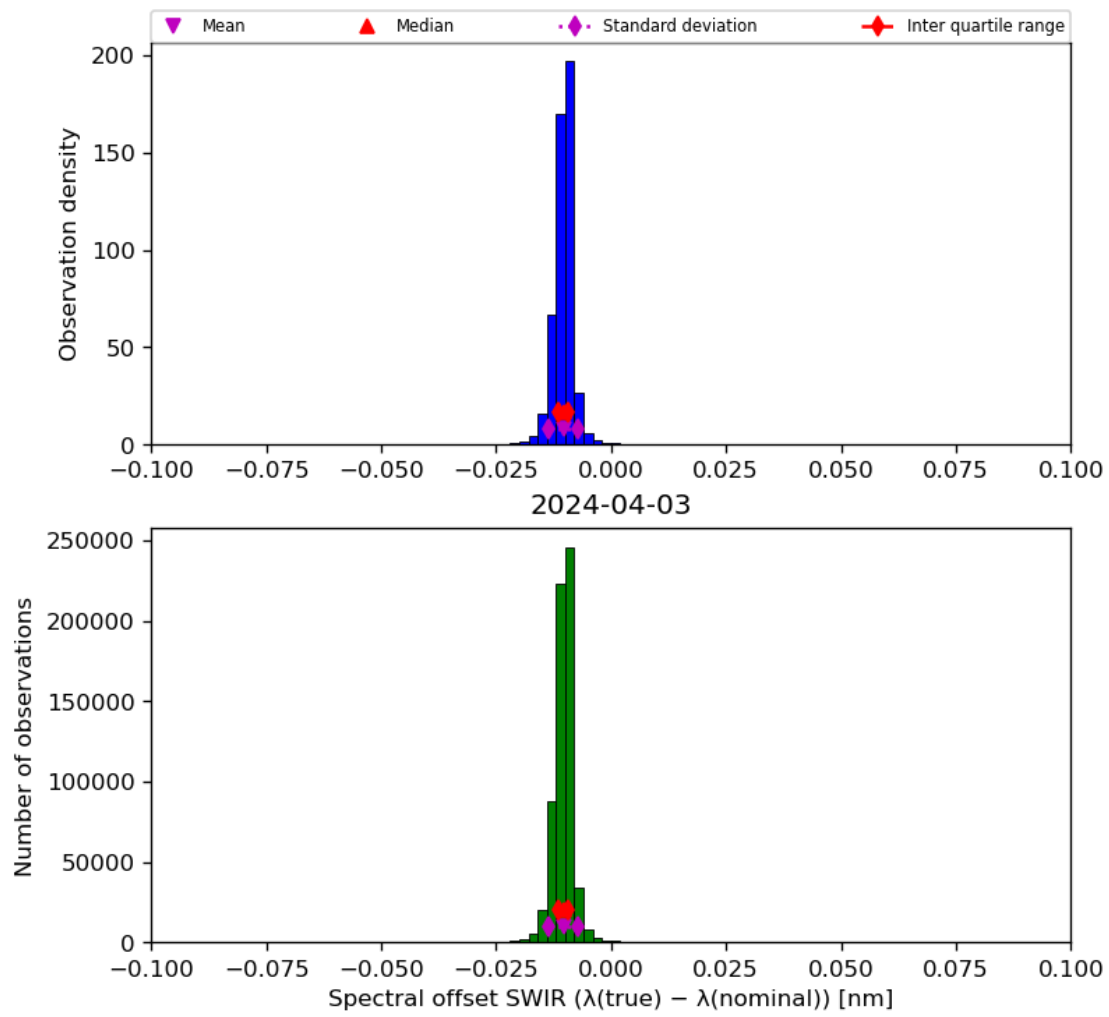
Figure 27: Histogram of “Spectral offset SWIR ( \lambda(\text{true}) - \lambda(\text{nominal}) )” for 2024-04-02 to 2024-04-04
