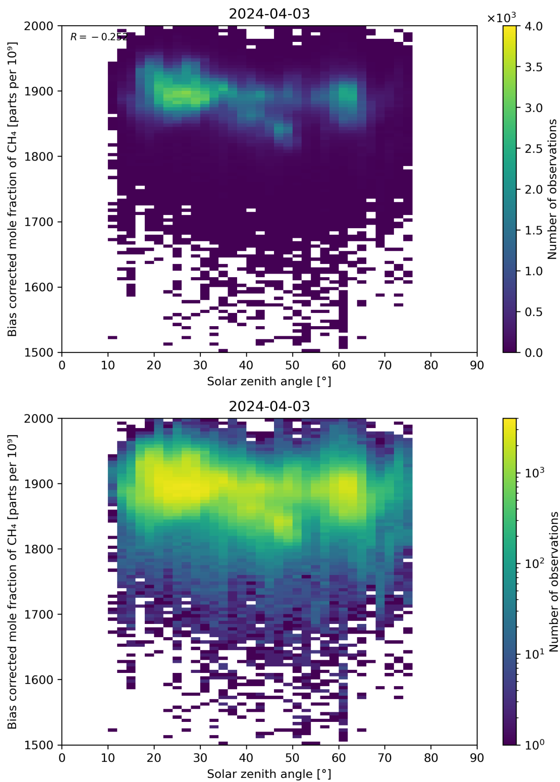
Figure 100: Scatter density plot of “Solar zenith angle” against “Bias corrected mole fraction of CH 4 ” for 2024-04-02 to 2024-04-04.
