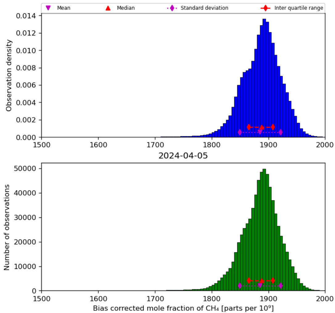
Figure 25: Histogram of “Bias corrected mole fraction of CH 4 ” for 2024-04-05 to 2024-04-06
