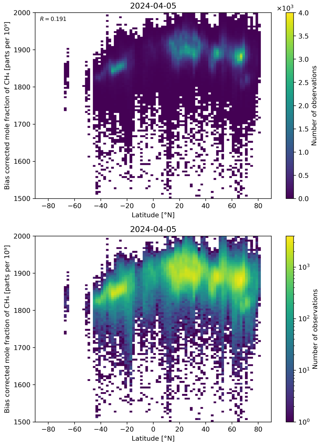
Figure 58: Scatter density plot of “Latitude” against “Bias corrected mole fraction of \text{CH}_4 ” for 2024-04-05 to 2024-04-06.
