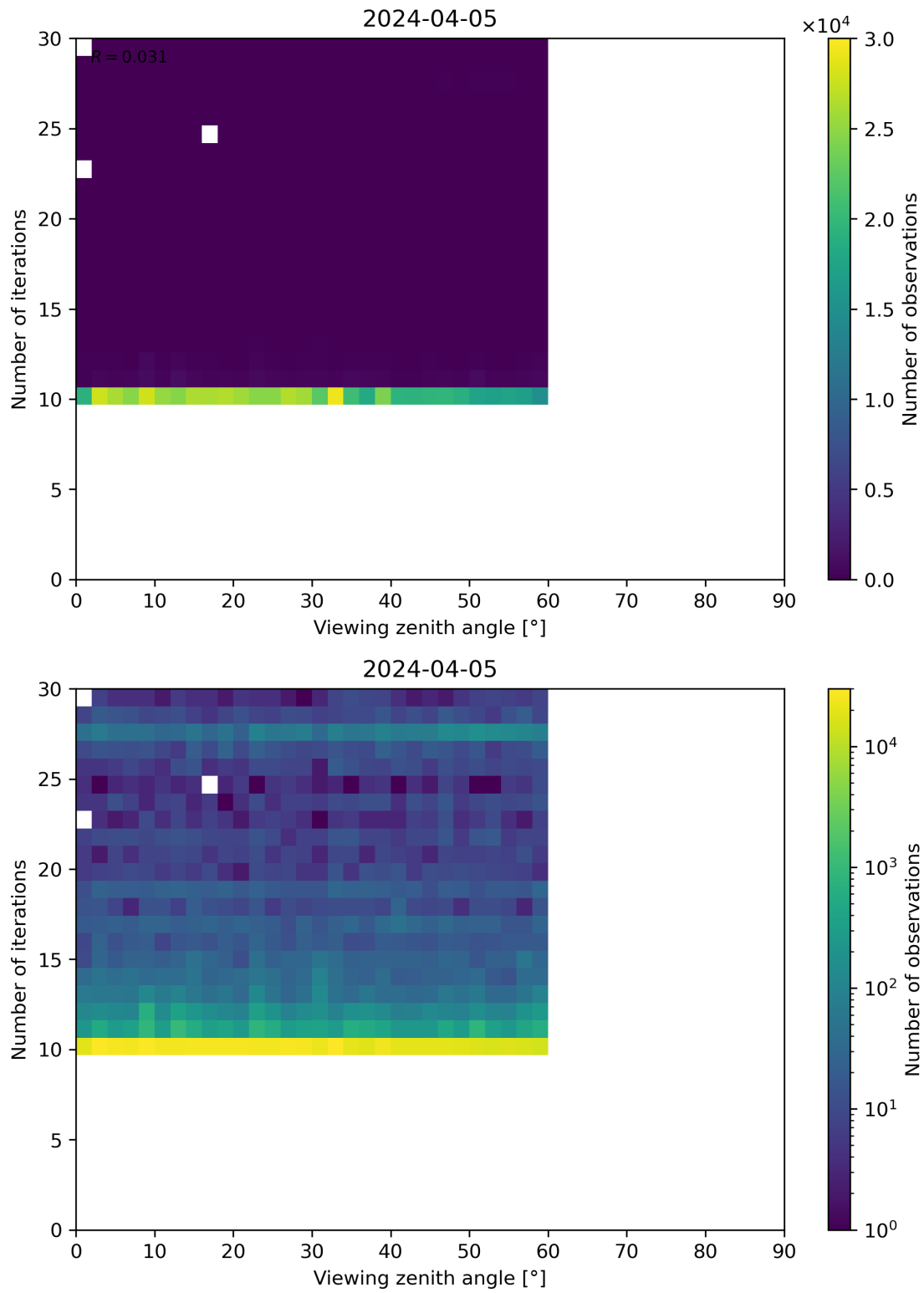
Figure 113: Scatter density plot of “Viewing zenith angle” against “Number of iterations” for 2024-04-05 to 2024-04-06.
