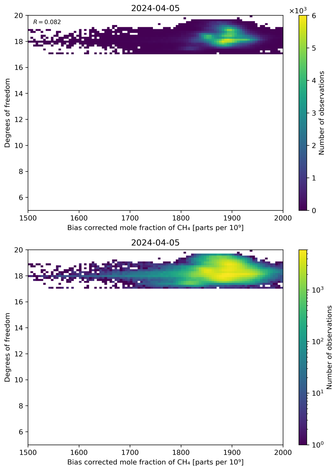
Figure 65: Scatter density plot of “Bias corrected mole fraction of CH 4 ” against “Degrees of freedom” for 2024-04-05 to 2024-04-06.
