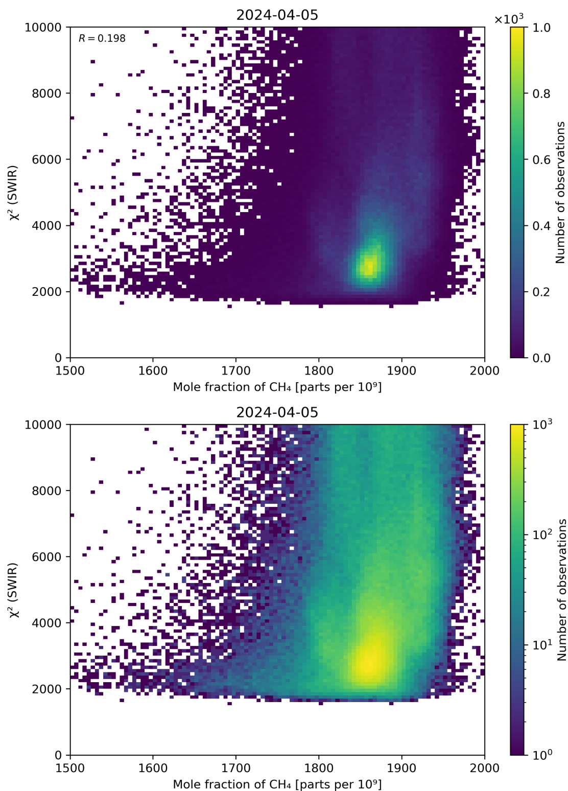
Figure 71: Scatter density plot of “Mole fraction of \text{CH}_4 ” against “ \chi^2 (SWIR)” for 2024-04-05 to 2024-04-06.
