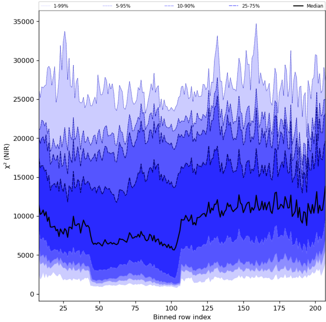
Figure 40: Along track statistics of “ \chi^2 (NIR)” for 2024-04-05 to 2024-04-06
