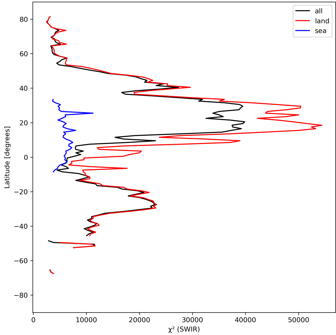
Figure 17: Zonal average of “ \chi^2 (SWIR)” for 2024-04-05 to 2024-04-06.
