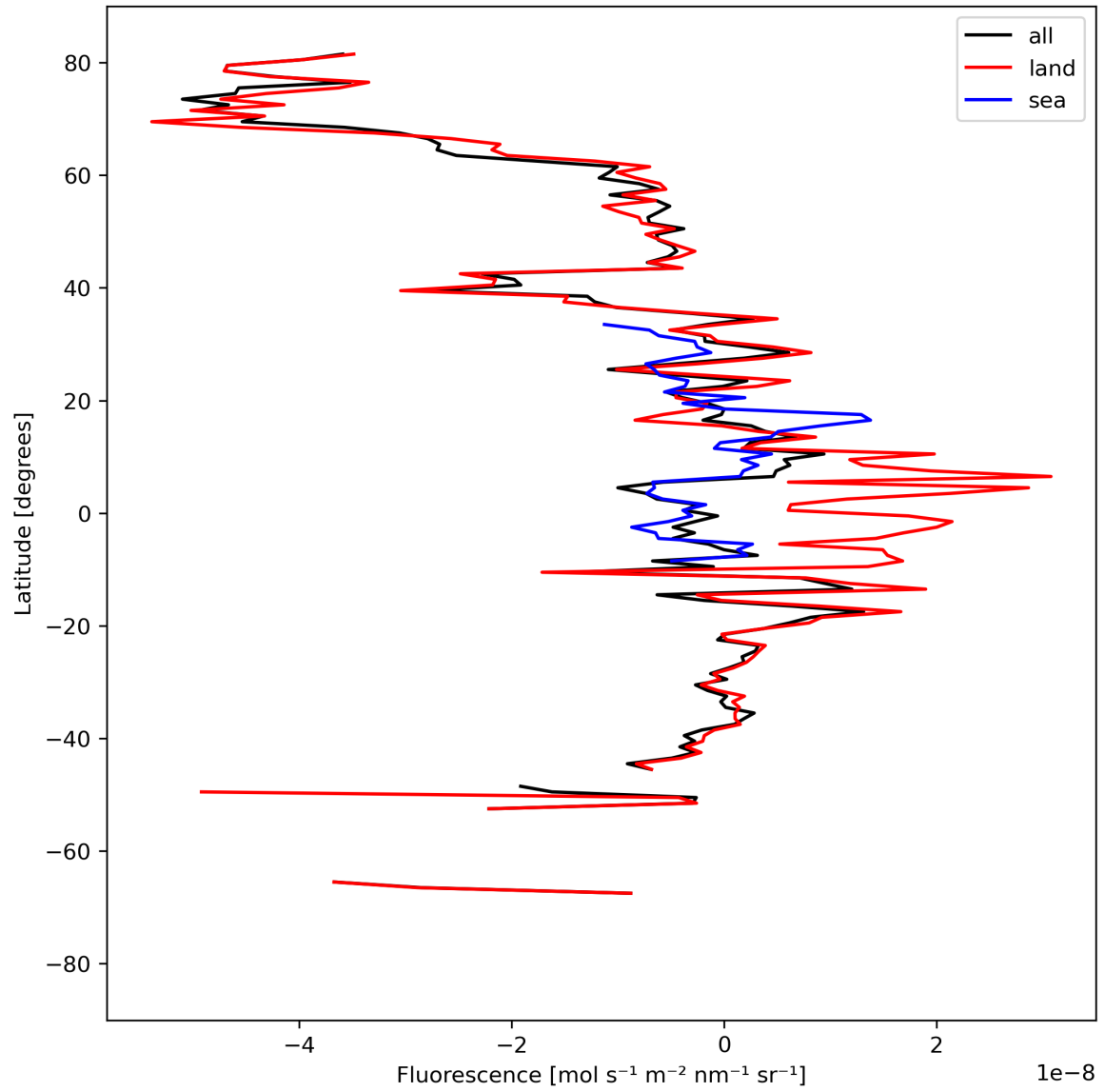
Figure 21: Zonal average of “Fluorescence” for 2024-04-05 to 2024-04-06.
