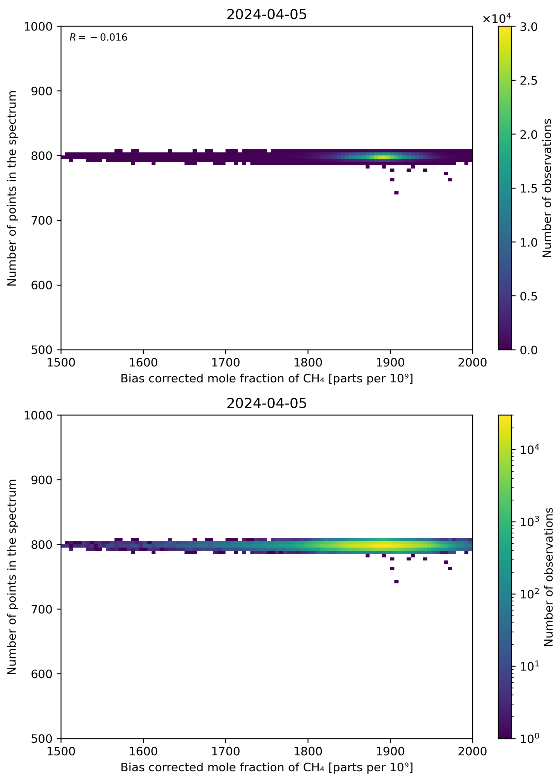
Figure 68: Scatter density plot of “Bias corrected mole fraction of CH 4 ” against “Number of points in the spectrum” for 2024-04-05 to 2024-04-06.
