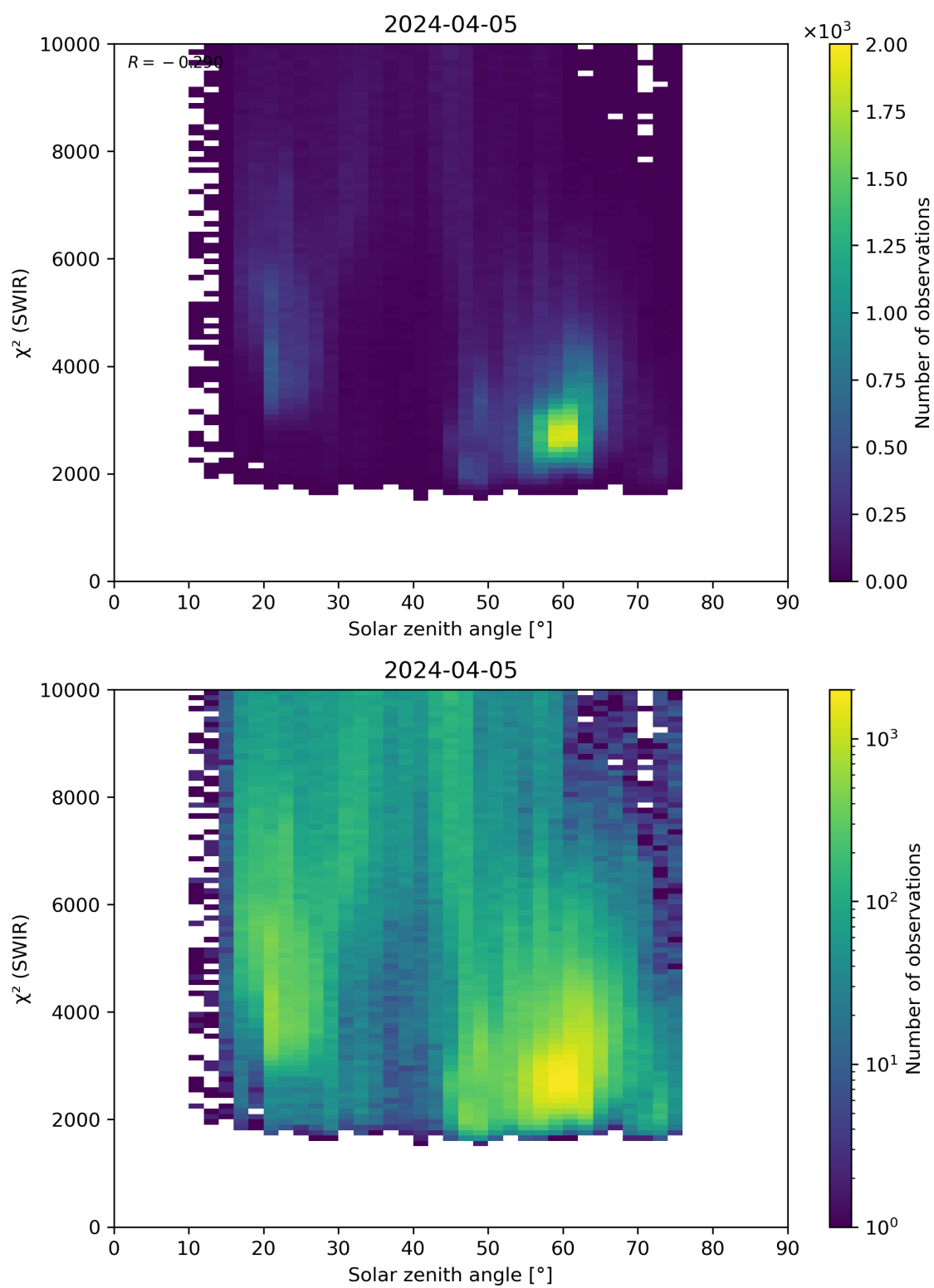
Figure 95: Scatter density plot of “Solar zenith angle” against “ \chi^2 (SWIR)” for 2024-04-05 to 2024-04-06.
