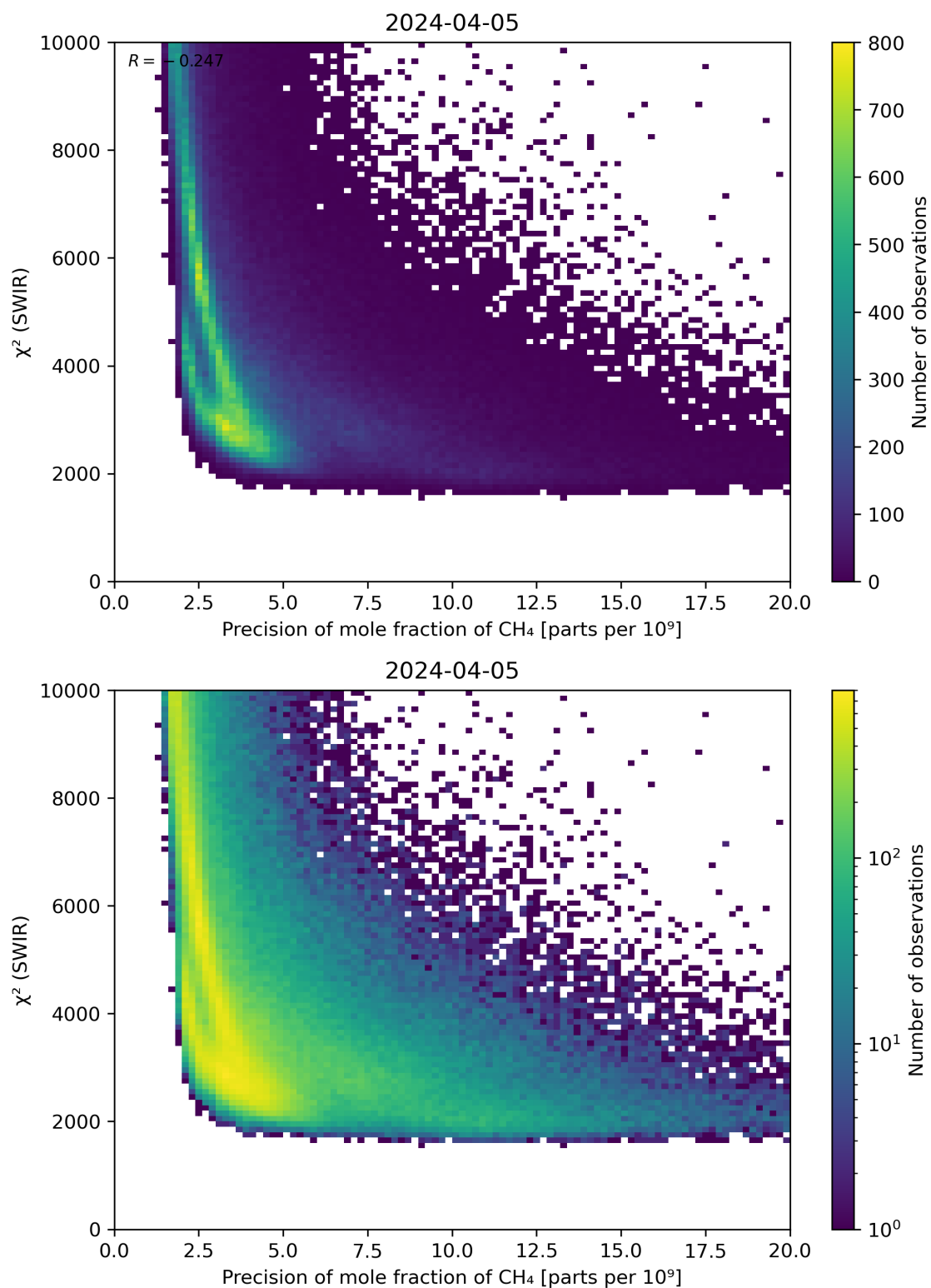
Figure 79: Scatter density plot of “Precision of mole fraction of CH 4 ” against “ \chi^2 (SWIR)” for 2024-04-05 to 2024-04-06.
