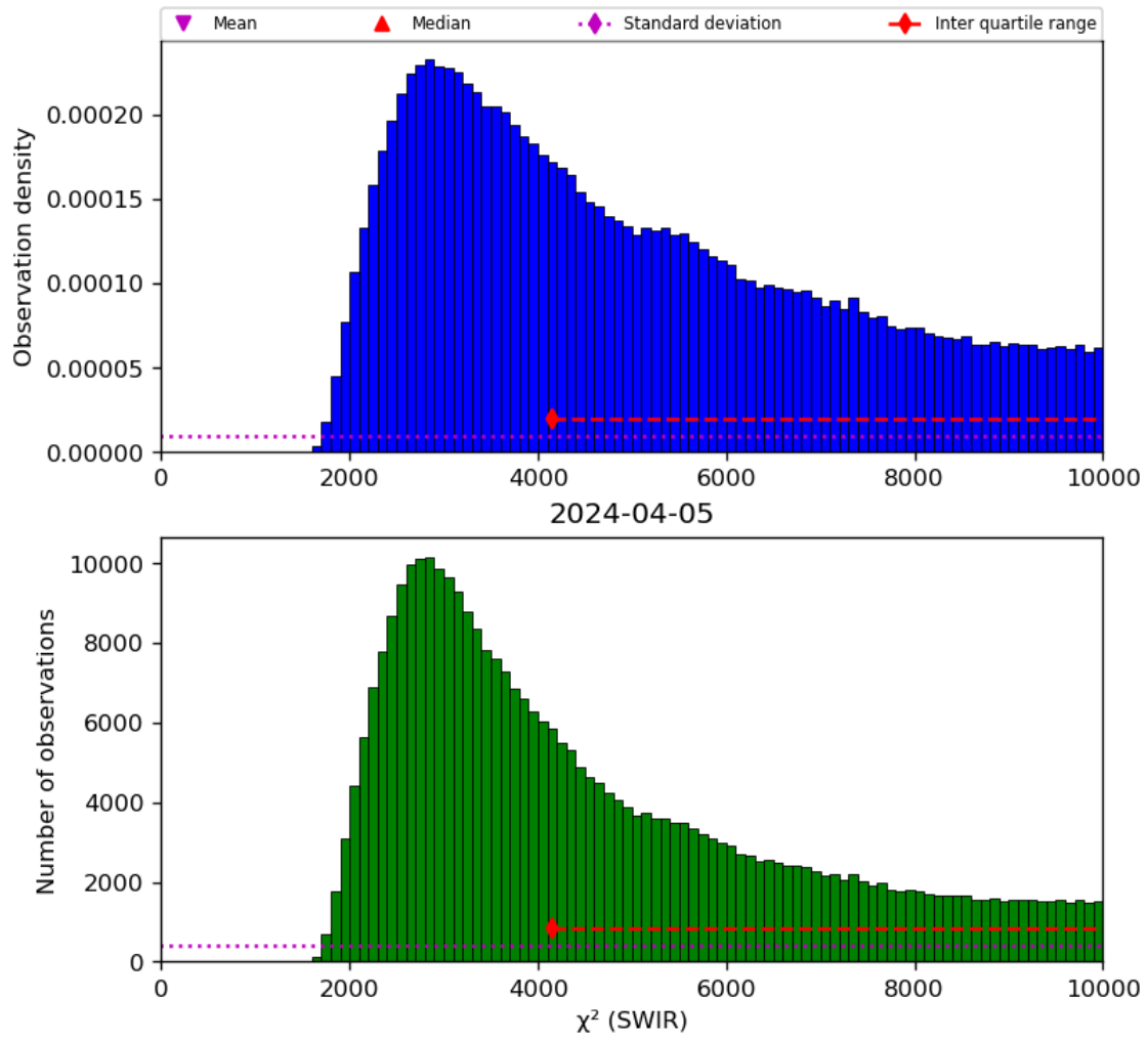
Figure 28: Histogram of “ \chi^2 (SWIR)” for 2024-04-05 to 2024-04-06
