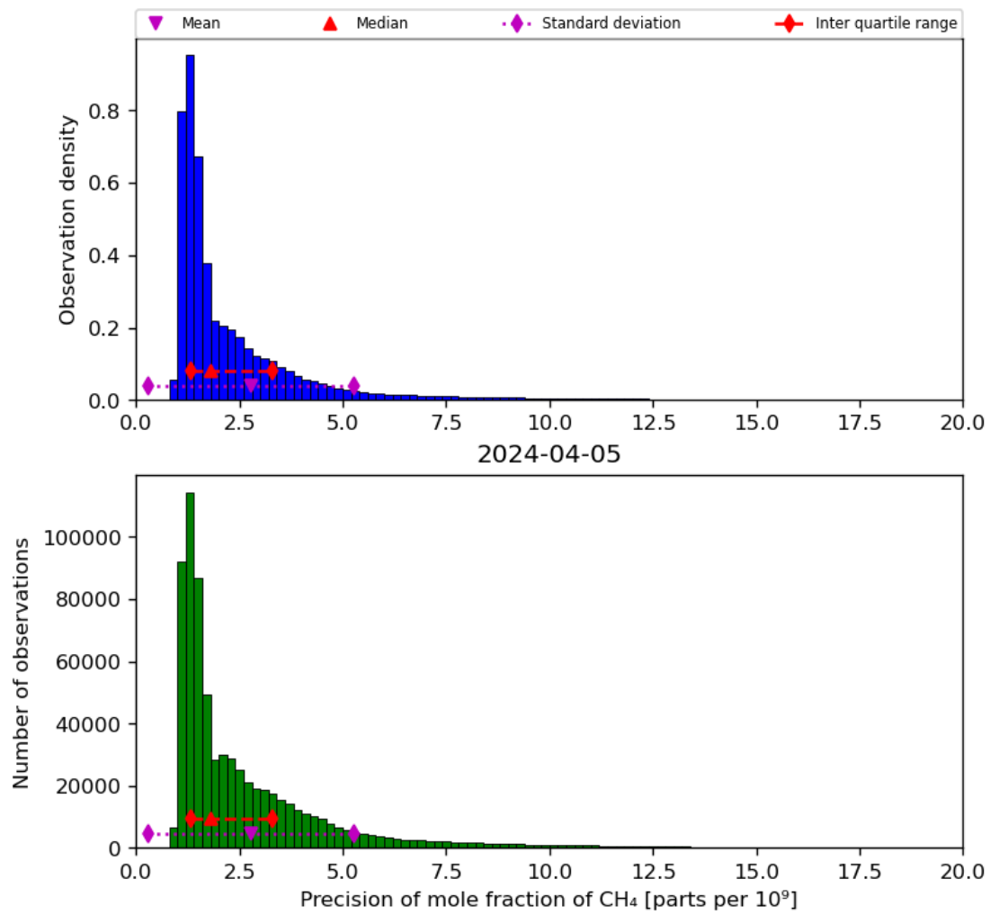
Figure 24: Histogram of “Precision of mole fraction of CH 4 ” for 2024-04-05 to 2024-04-06
