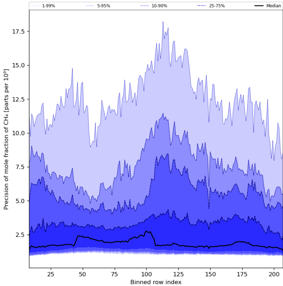
Figure 35: Along track statistics of “Precision of mole fraction of CH 4 ” for 2024-04-05 to 2024-04-06
