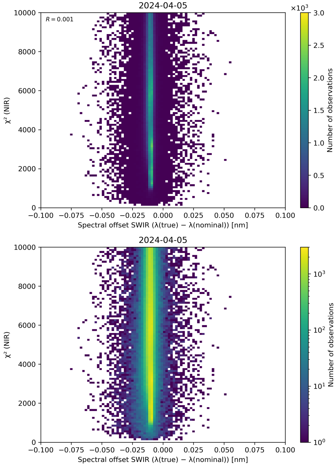
Figure 117: Scatter density plot of “Spectral offset SWIR ( \lambda(\text{true}) - \lambda(\text{nominal}) )” against “ \chi^2 (NIR)” for 2024-04-05 to 2024-04-06.
