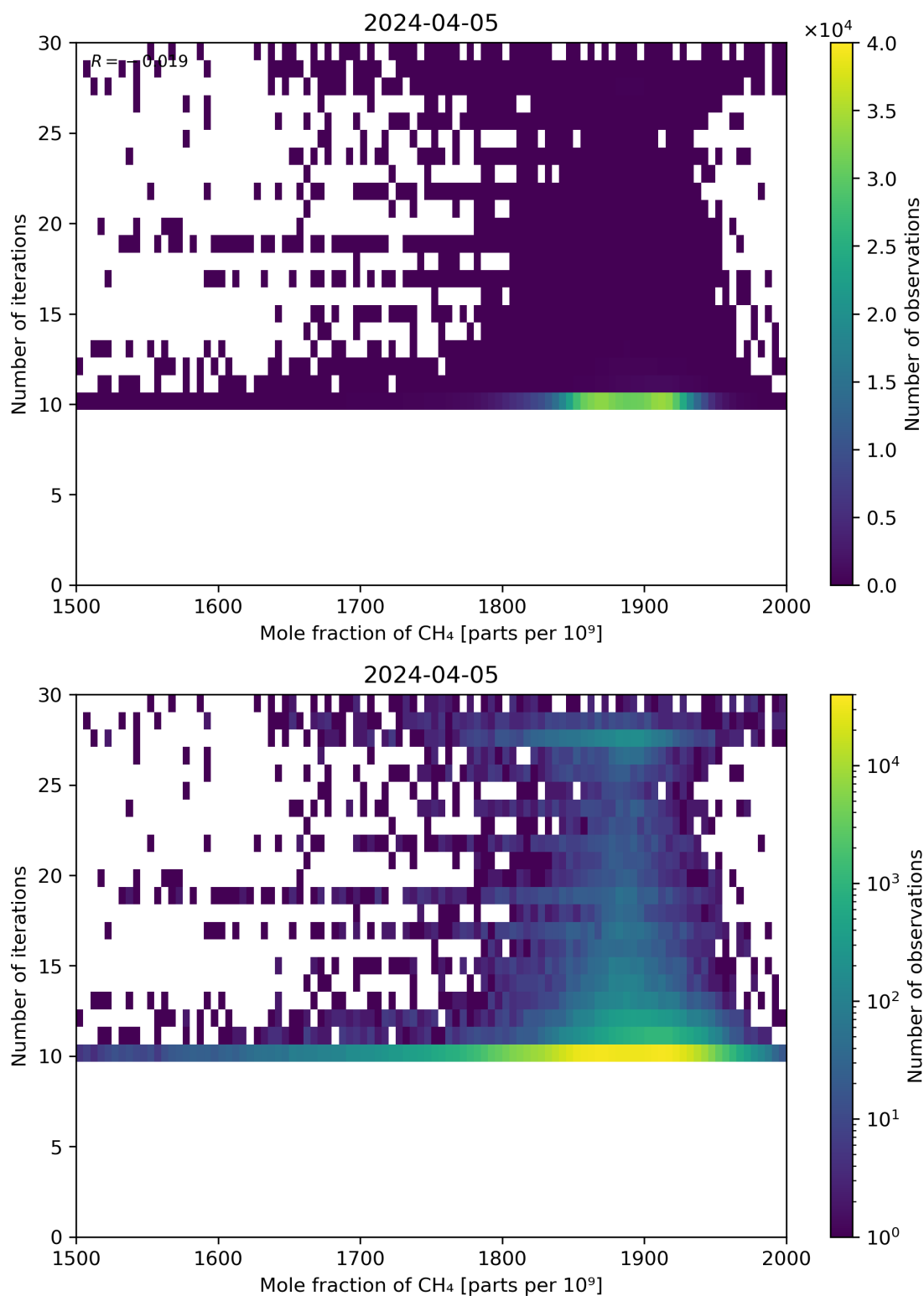
Figure 76: Scatter density plot of “Mole fraction of CH 4 ” against “Number of iterations” for 2024-04-05 to 2024-04-06.
