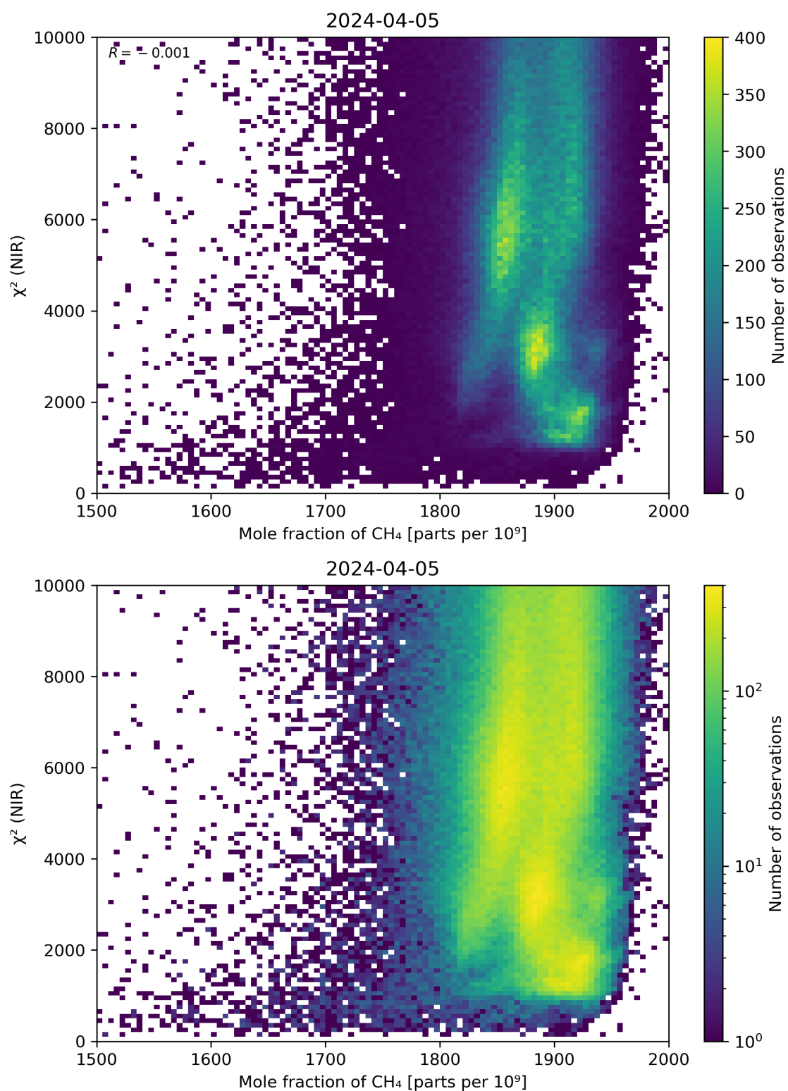
Figure 70: Scatter density plot of “Mole fraction of CH 4 ” against “ \chi^2 (NIR)” for 2024-04-05 to 2024-04-06.
