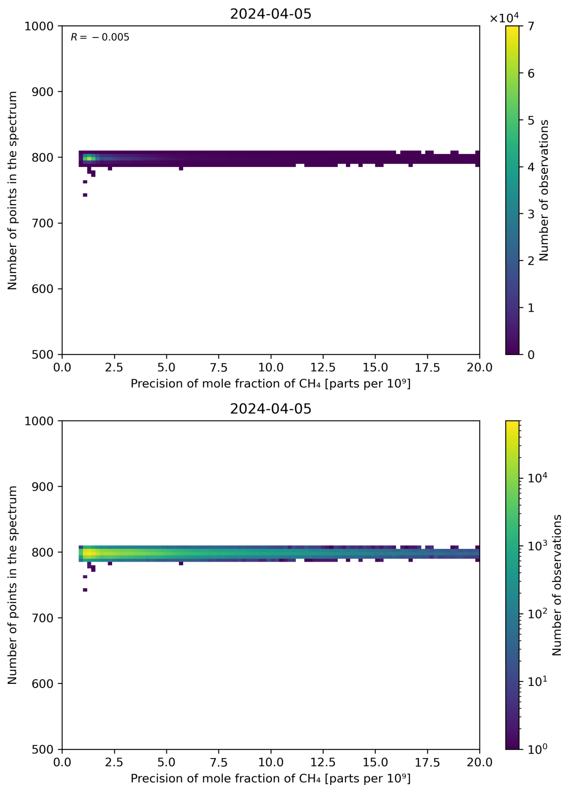
Figure 84: Scatter density plot of “Precision of mole fraction of CH 4 ” against “Number of points in the spectrum” for 2024-04-05 to 2024-04-06.
