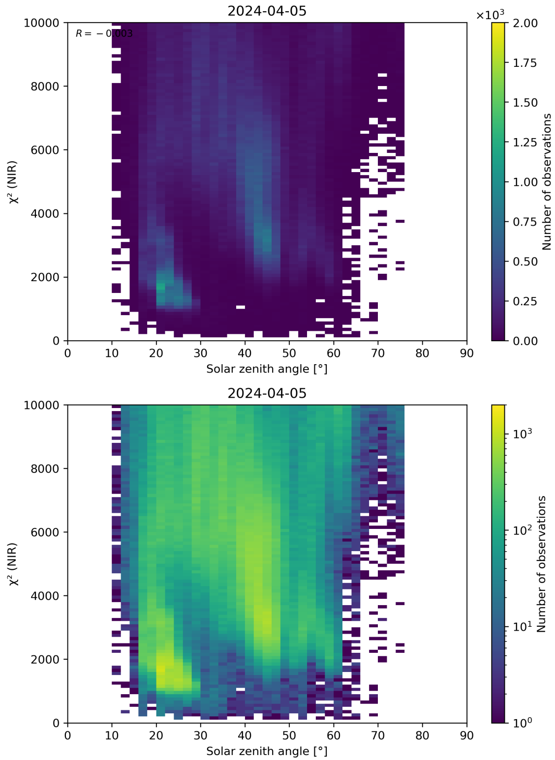
Figure 94: Scatter density plot of “Solar zenith angle” against “ \chi^2 (NIR)” for 2024-04-05 to 2024-04-06.
