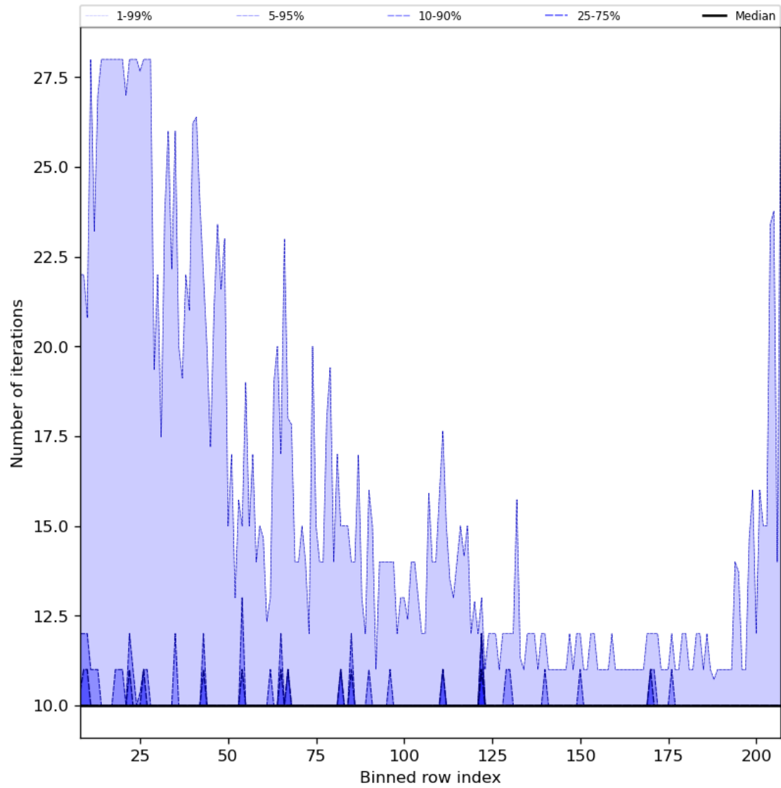
Figure 42: Along track statistics of “Number of iterations” for 2024-04-05 to 2024-04-06
