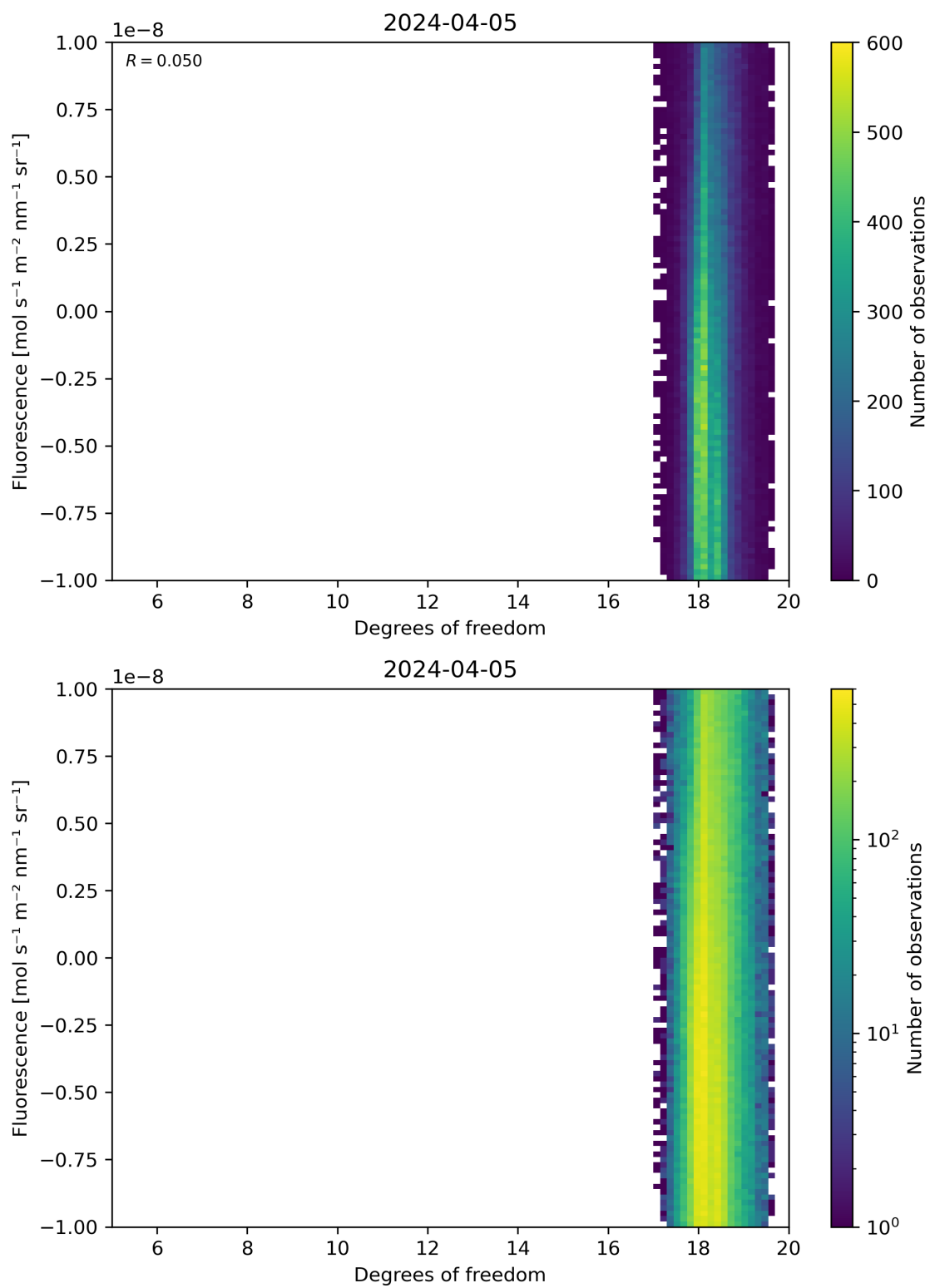
Figure 51: Scatter density plot of “Degrees of freedom” against “Fluorescence” for 2024-04-05 to 2024-04-06.
