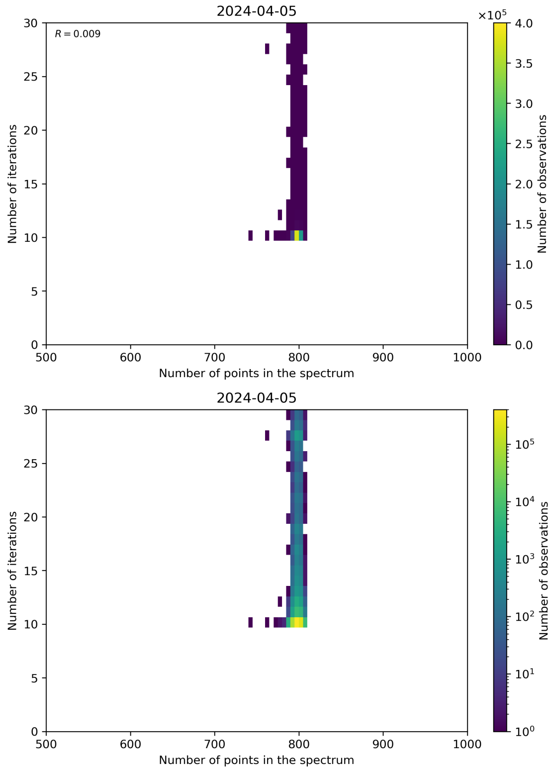
Figure 92: Scatter density plot of “Number of points in the spectrum” against “Number of iterations” for 2024-04-05 to 2024-04-06.
