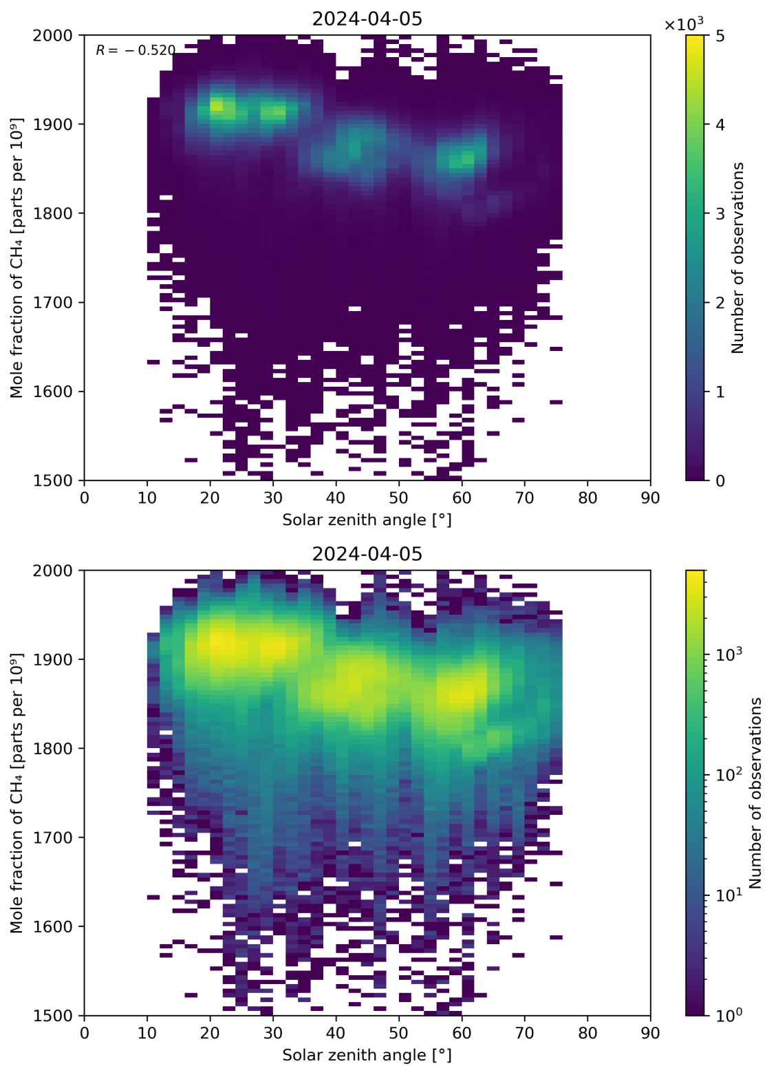
Figure 99: Scatter density plot of “Solar zenith angle” against “Mole fraction of CH 4 ” for 2024-04-05 to 2024-04-06.
