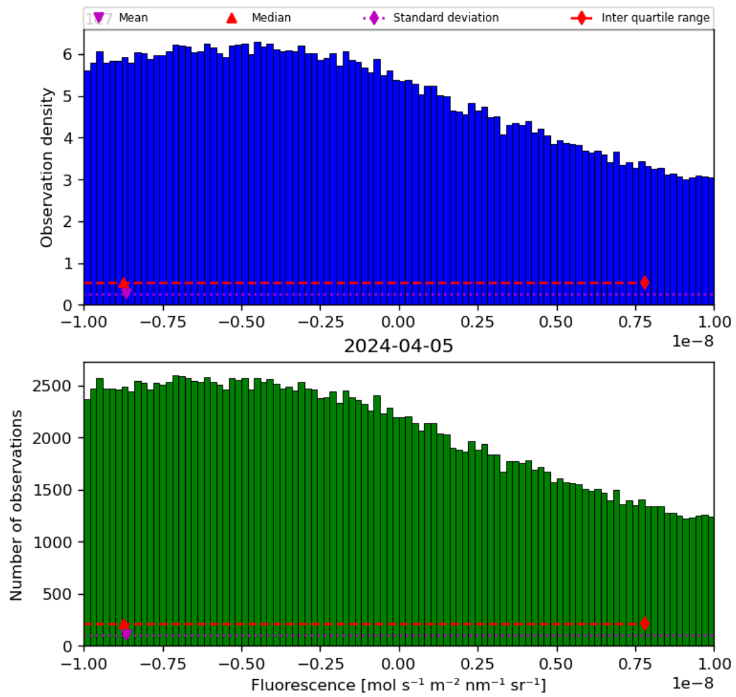
Figure 32: Histogram of “Fluorescence” for 2024-04-05 to 2024-04-06
