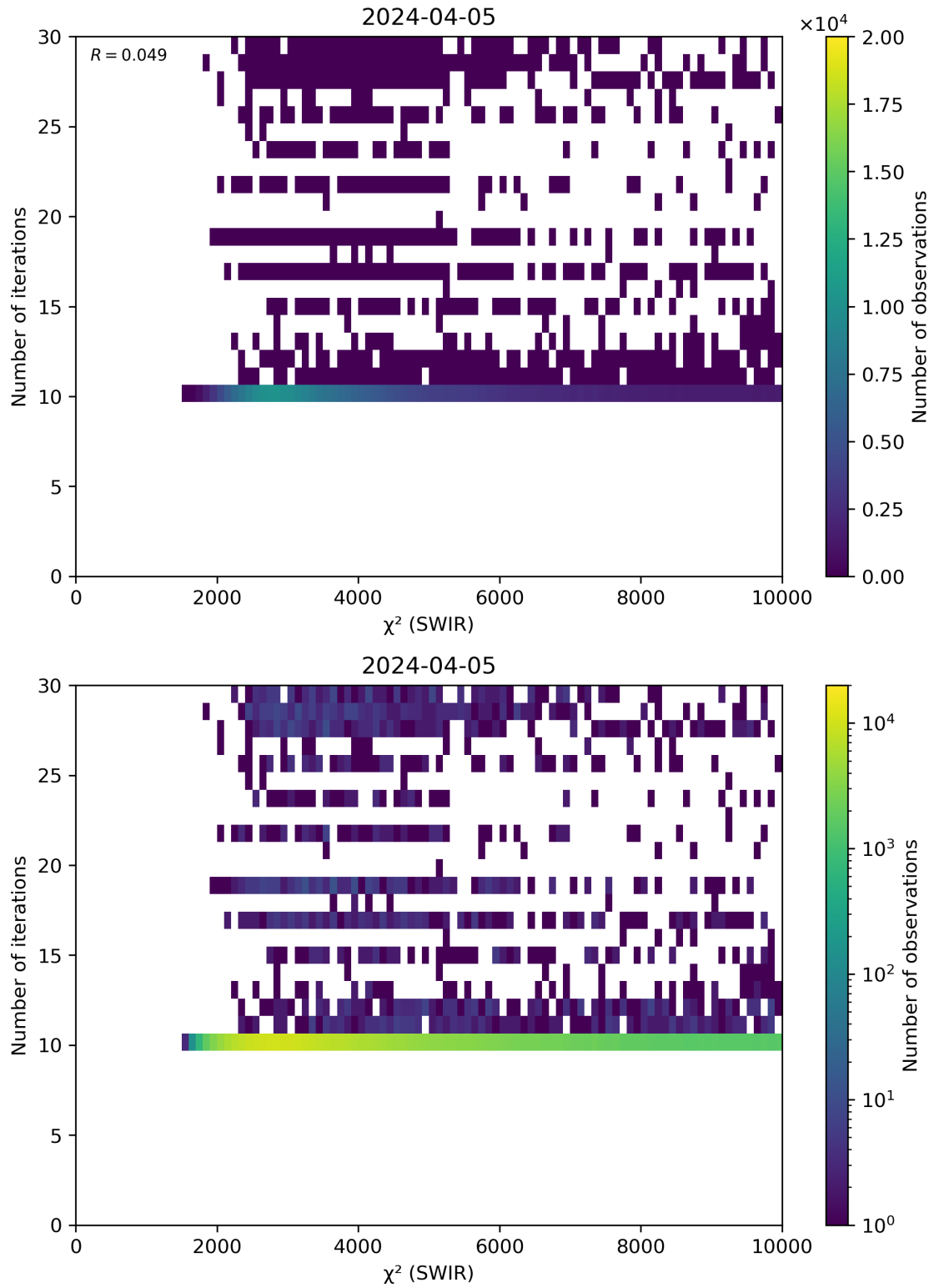
Figure 50: Scatter density plot of “ \chi^2 (SWIR)” against “Number of iterations” for 2024-04-05 to 2024-04-06.
