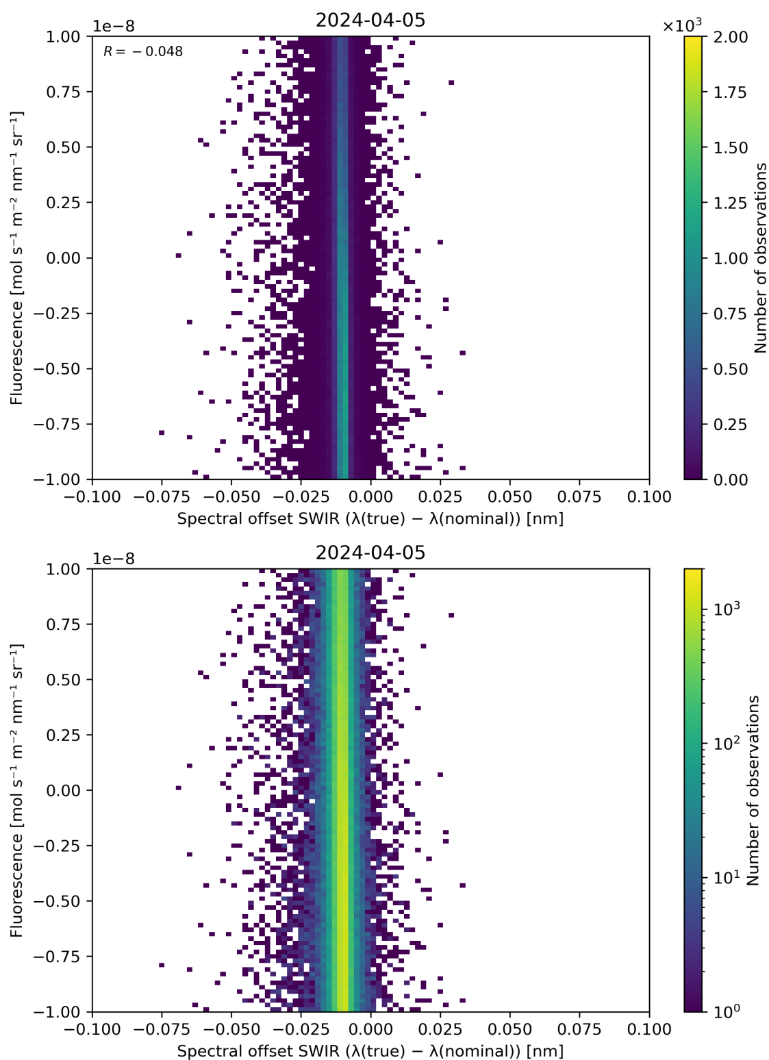
Figure 120: Scatter density plot of “Spectral offset SWIR ( \lambda(\text{true}) - \lambda(\text{nominal}) )” against “Fluorescence” for 2024-04-05 to 2024-04-06.
