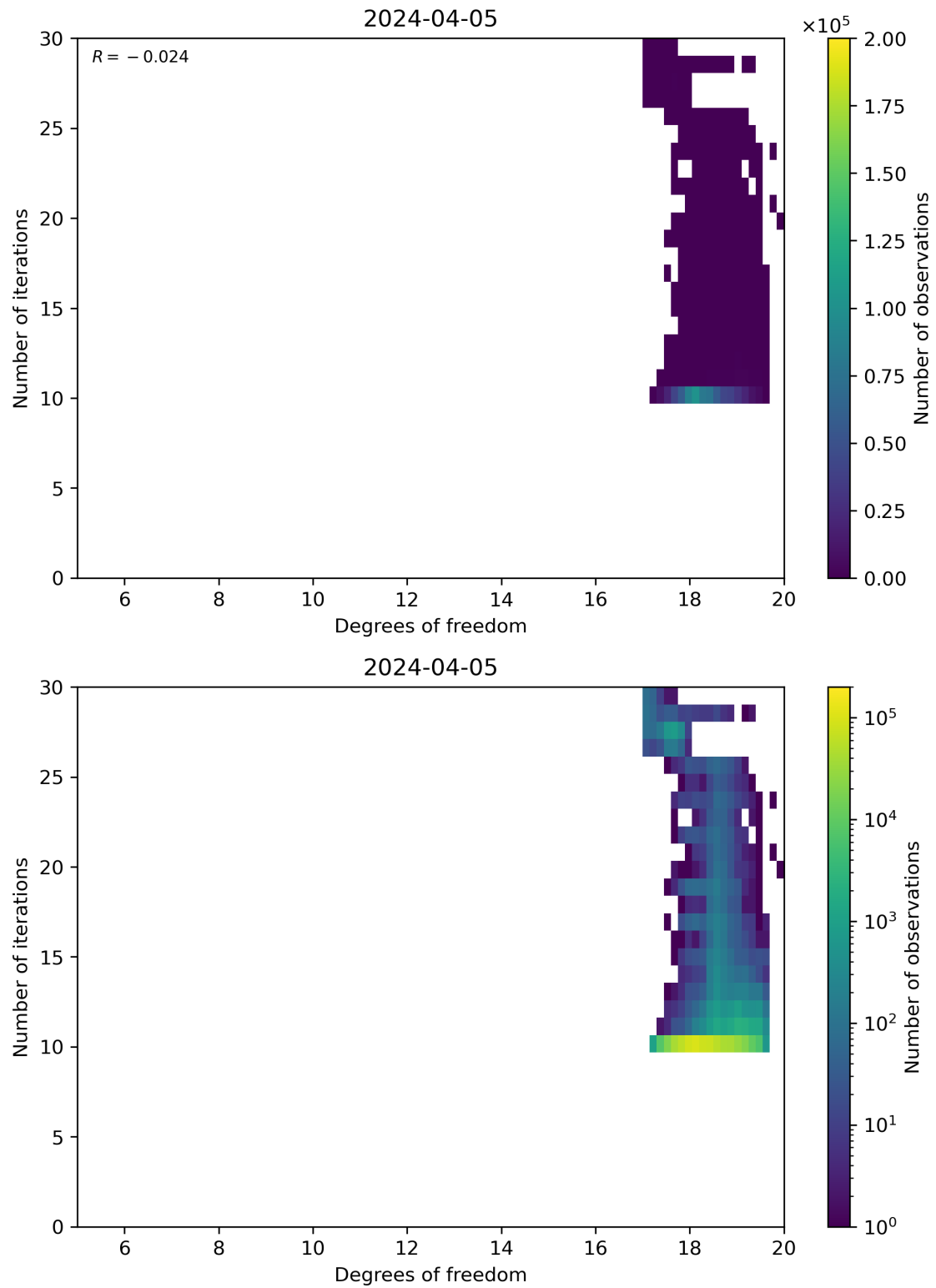
Figure 52: Scatter density plot of “Degrees of freedom” against “Number of iterations” for 2024-04-05 to 2024-04-06.
