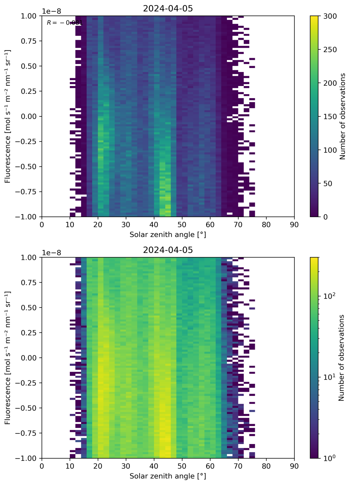
Figure 97: Scatter density plot of “Solar zenith angle” against “Fluorescence” for 2024-04-05 to 2024-04-06.
