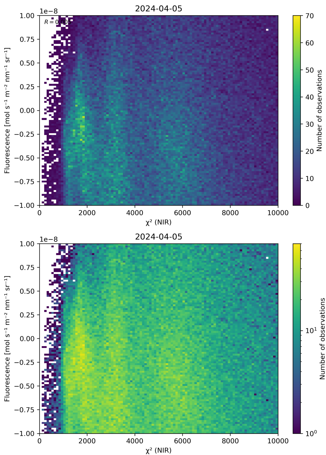
Figure 45: Scatter density plot of “ \chi^2 (NIR)” against “Fluorescence” for 2024-04-05 to 2024-04-06.
