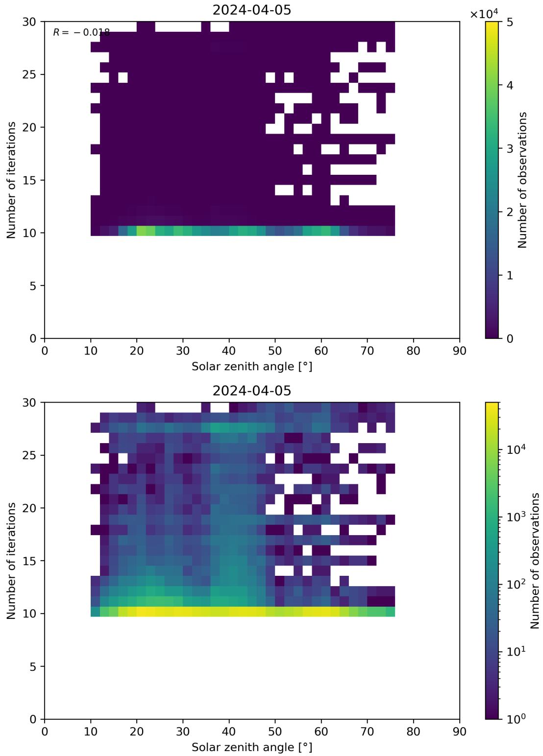
Figure 102: Scatter density plot of “Solar zenith angle” against “Number of iterations” for 2024-04-05 to 2024-04-06.
