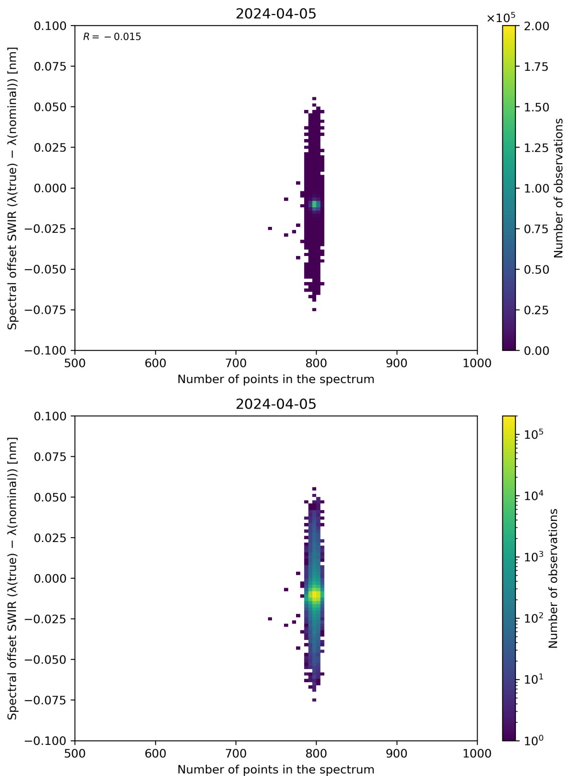
Figure 93: Scatter density plot of “Number of points in the spectrum” against “Spectral offset SWIR ( \lambda(\text{true}) - \lambda(\text{nominal}) )” for 2024-04-05 to 2024-04-06.
