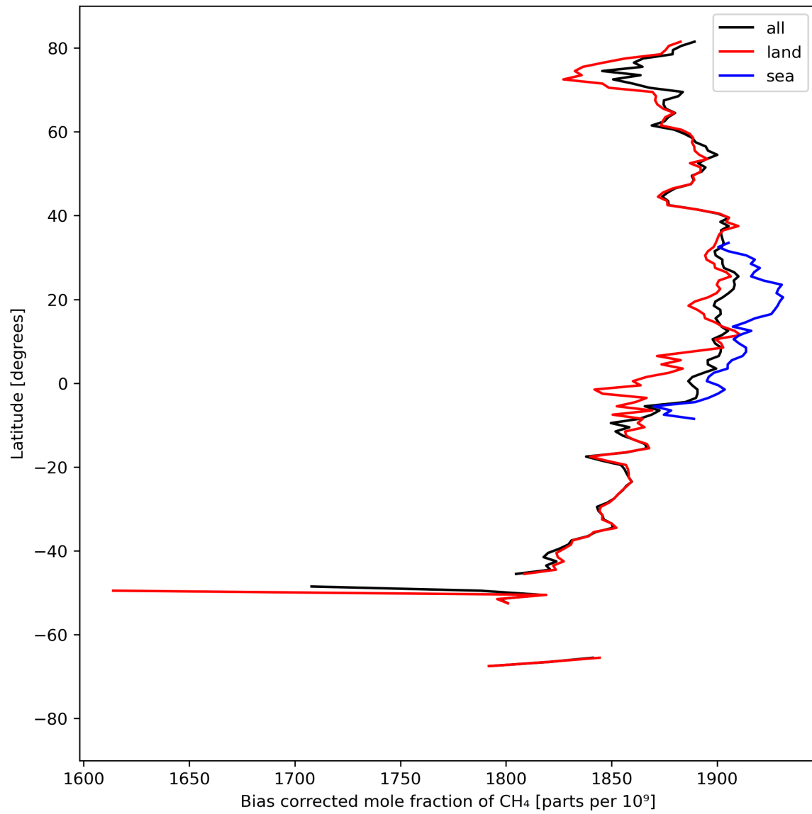
Figure 14: Zonal average of “Bias corrected mole fraction of CH 4 ” for 2024-04-05 to 2024-04-06.
