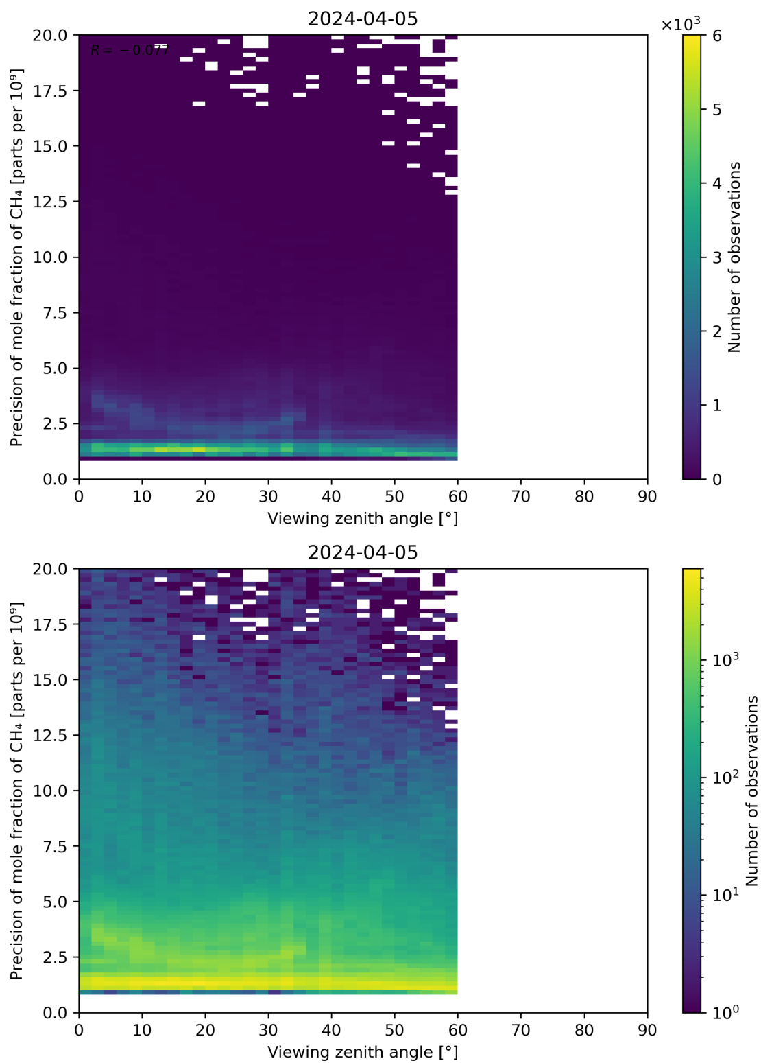
Figure 112: Scatter density plot of “Viewing zenith angle” against “Precision of mole fraction of CH 4 ” for 2024-04-05 to 2024-04-06.
