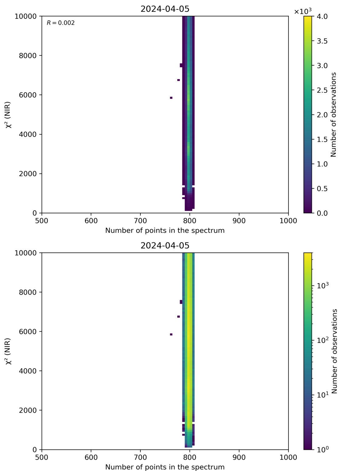
Figure 88: Scatter density plot of “Number of points in the spectrum” against “ \chi^2 (NIR)” for 2024-04-05 to 2024-04-06.
