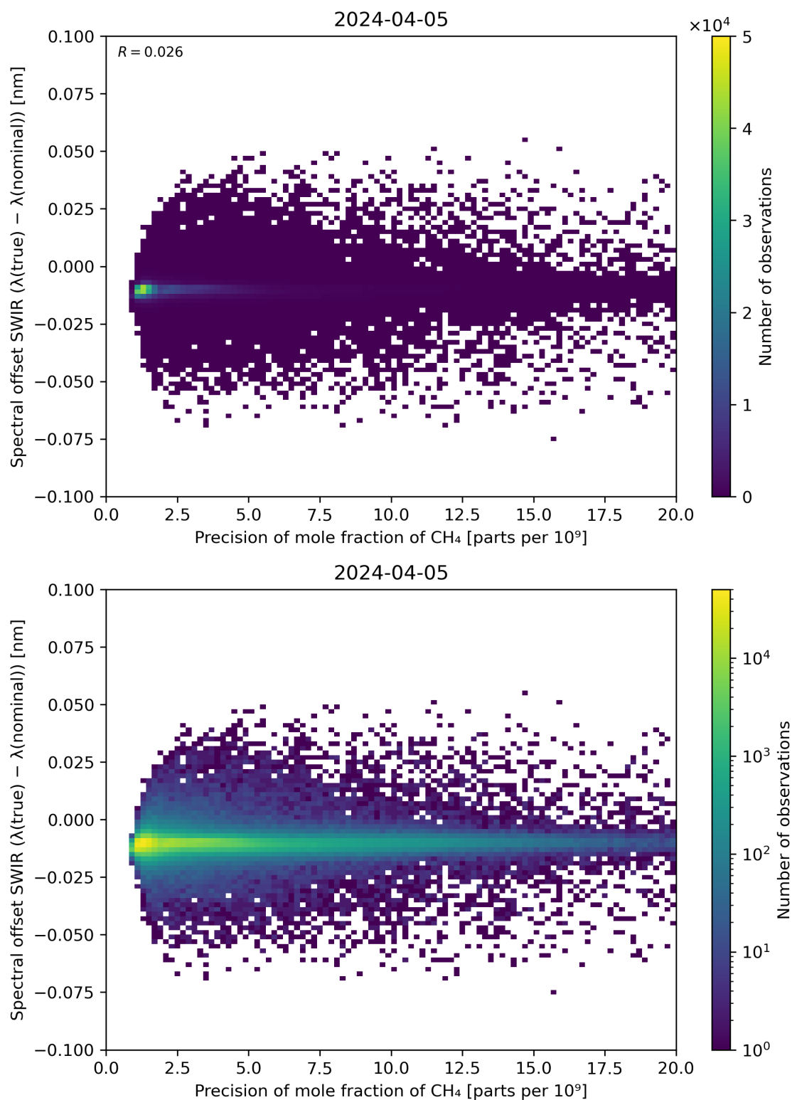
Figure 85: Scatter density plot of “Precision of mole fraction of CH 4 ” against “Spectral offset SWIR ( \lambda(\text{true}) - \lambda(\text{nominal}) )” for 2024-04-05 to 2024-04-06.
