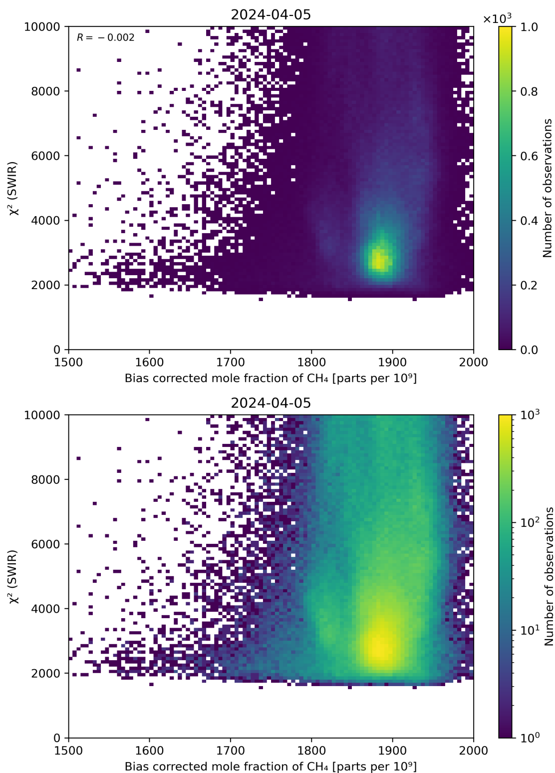
Figure 64: Scatter density plot of “Bias corrected mole fraction of CH 4 ” against “ \chi^2 (SWIR)” for 2024-04-05 to 2024-04-06.
