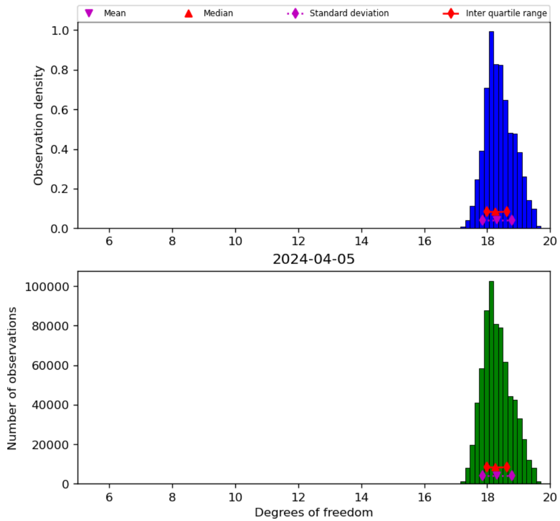
Figure 30: Histogram of “Degrees of freedom” for 2024-04-05 to 2024-04-06
