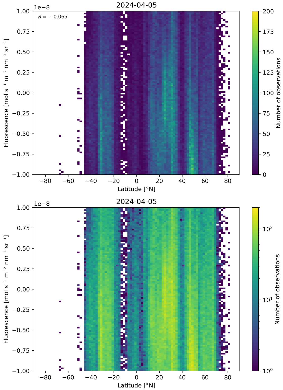
Figure 56: Scatter density plot of “Latitude” against “Fluorescence” for 2024-04-05 to 2024-04-06.
