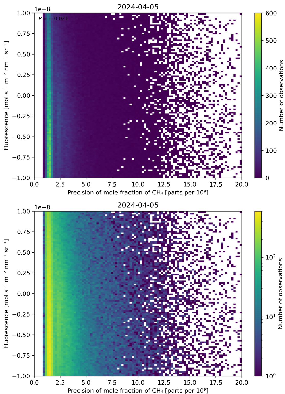
Figure 81: Scatter density plot of “Precision of mole fraction of CH 4 ” against “Fluorescence” for 2024-04-05 to 2024-04-06.
