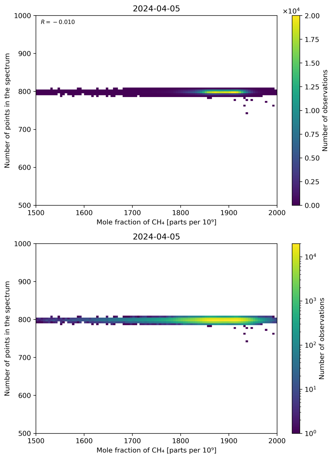
Figure 77: Scatter density plot of “Mole fraction of CH 4 ” against “Number of points in the spectrum” for 2024-04-05 to 2024-04-06.
