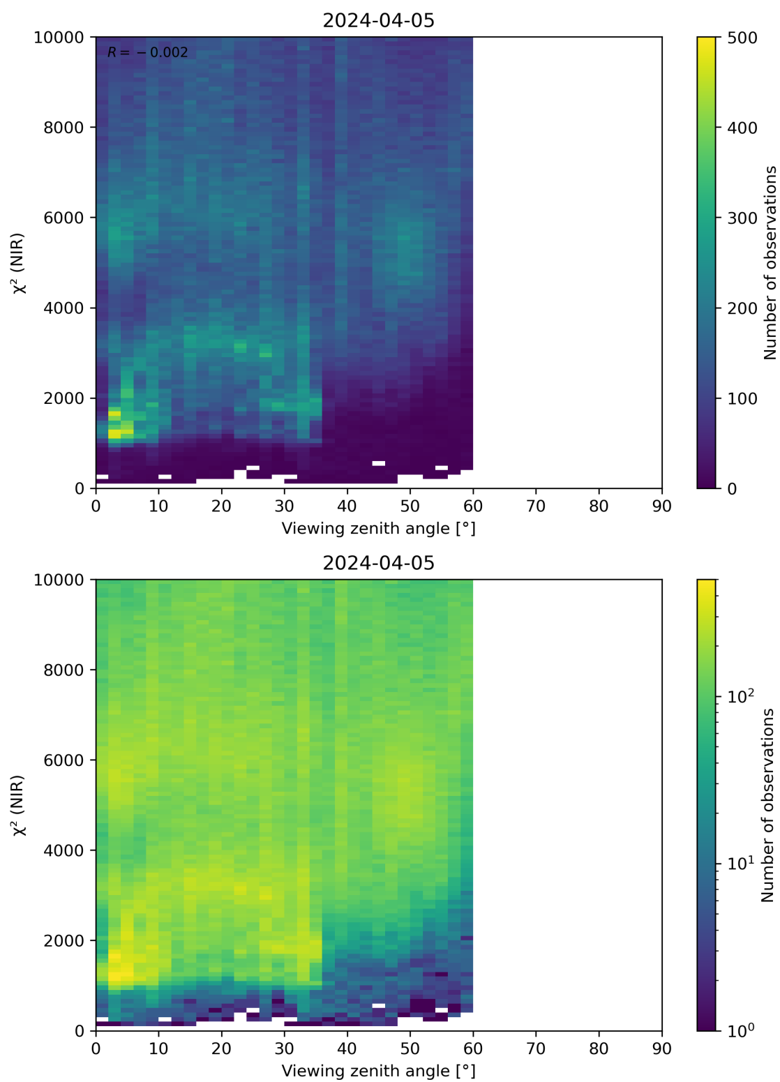
Figure 105: Scatter density plot of “Viewing zenith angle” against “ \chi^2 (NIR)” for 2024-04-05 to 2024-04-06.
