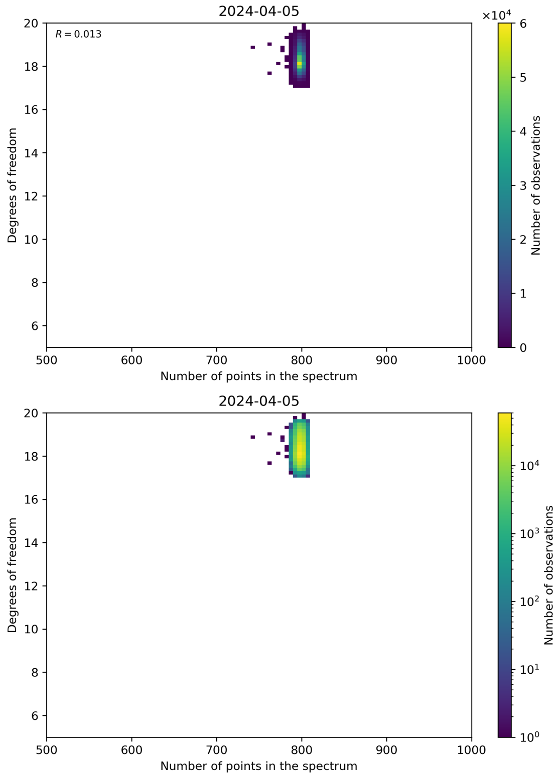
Figure 90: Scatter density plot of “Number of points in the spectrum” against “Degrees of freedom” for 2024-04-05 to 2024-04-06.
