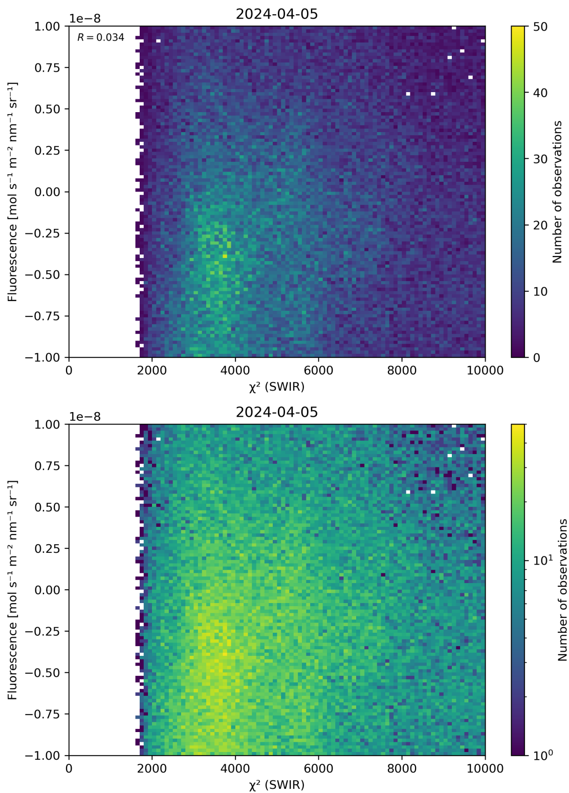
Figure 49: Scatter density plot of “ \chi^2 (SWIR)” against “Fluorescence” for 2024-04-05 to 2024-04-06.
