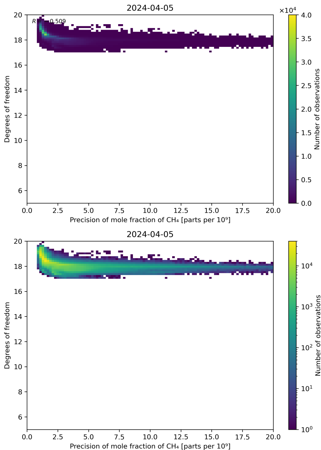
Figure 80: Scatter density plot of “Precision of mole fraction of CH 4 ” against “Degrees of freedom” for 2024-04-05 to 2024-04-06.
