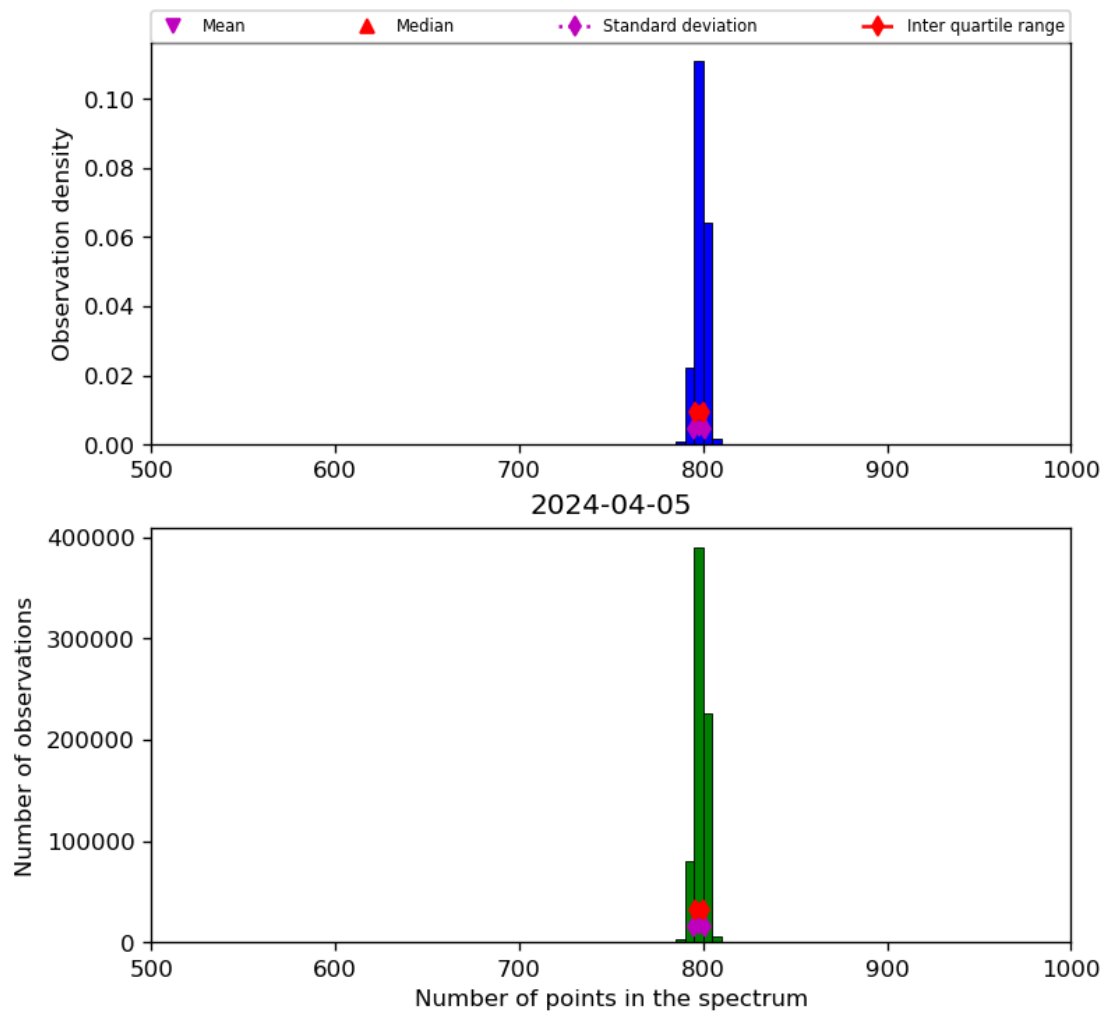
Figure 26: Histogram of “Number of points in the spectrum” for 2024-04-05 to 2024-04-06
