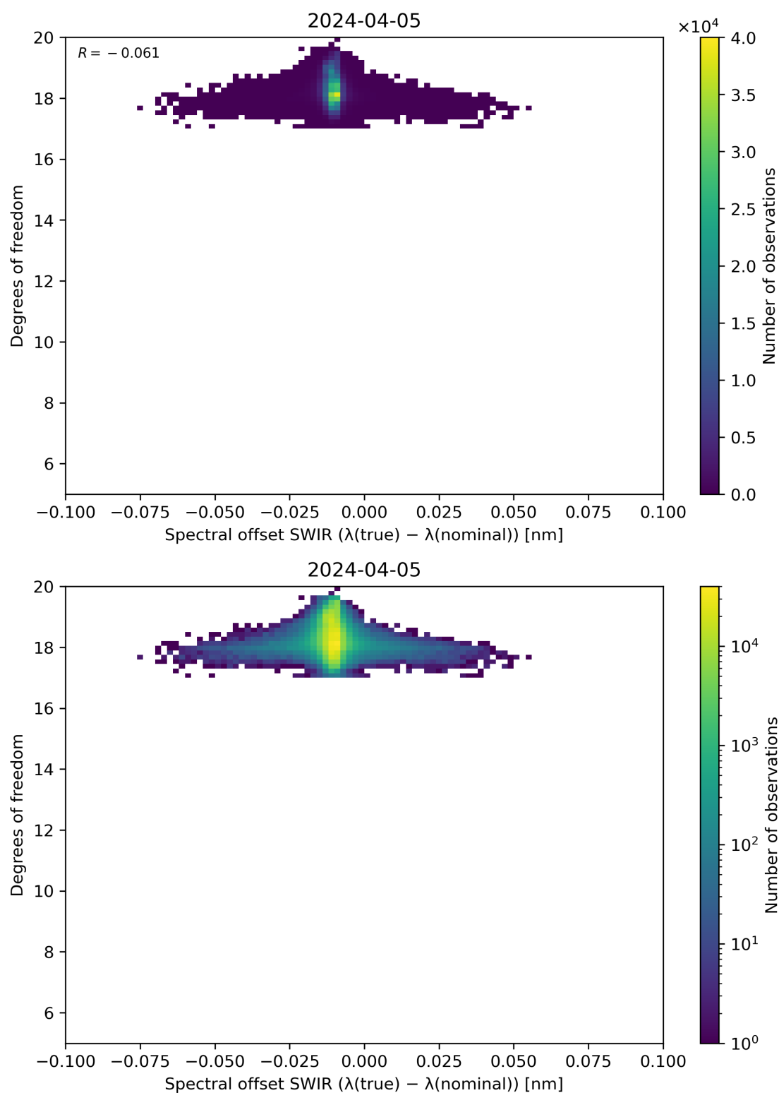
Figure 119: Scatter density plot of “Spectral offset SWIR ( \lambda(\text{true}) - \lambda(\text{nominal}) )” against “Degrees of freedom” for 2024-04-05 to 2024-04-06.
