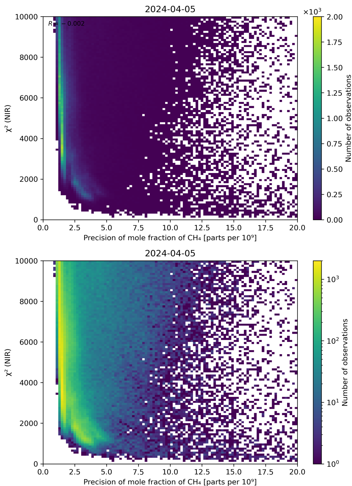
Figure 78: Scatter density plot of “Precision of mole fraction of \text{CH}_4 ” against “ \chi^2 (NIR)” for 2024-04-05 to 2024-04-06.
