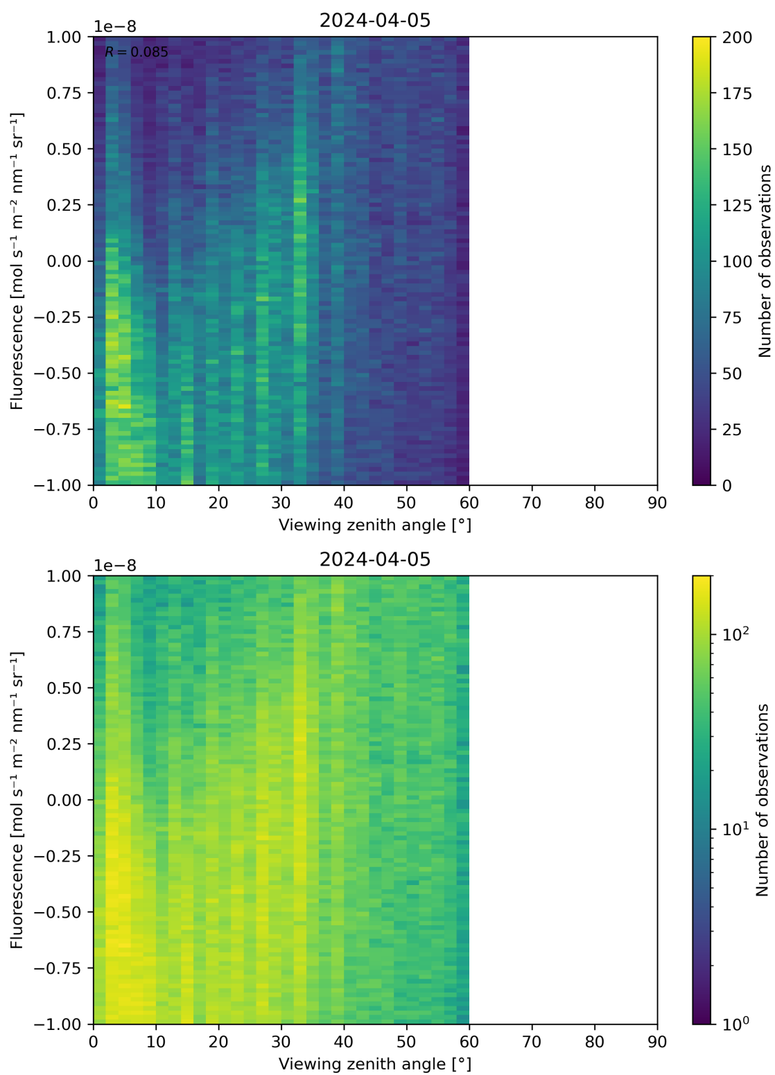
Figure 108: Scatter density plot of “Viewing zenith angle” against “Fluorescence” for 2024-04-05 to 2024-04-06.
