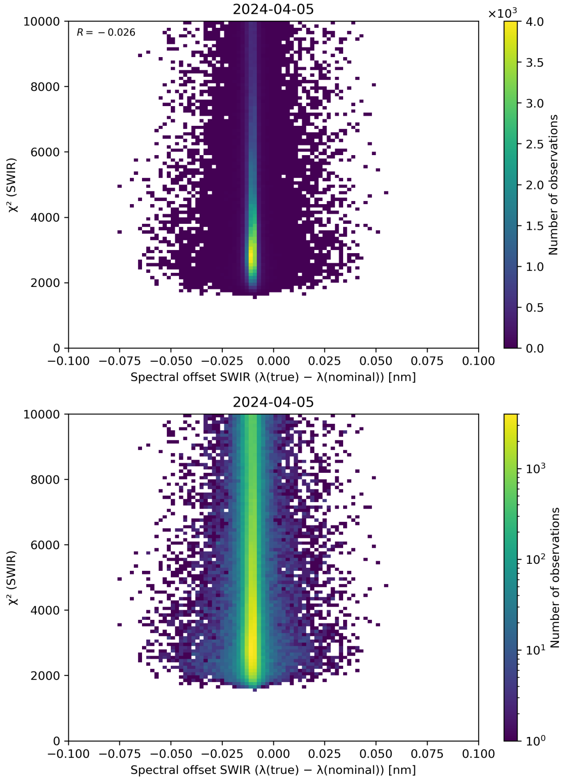
Figure 118: Scatter density plot of “Spectral offset SWIR ( \lambda(\text{true}) - \lambda(\text{nominal}) )” against “ \chi^2 (SWIR)” for 2024-04-05 to 2024-04-06.
