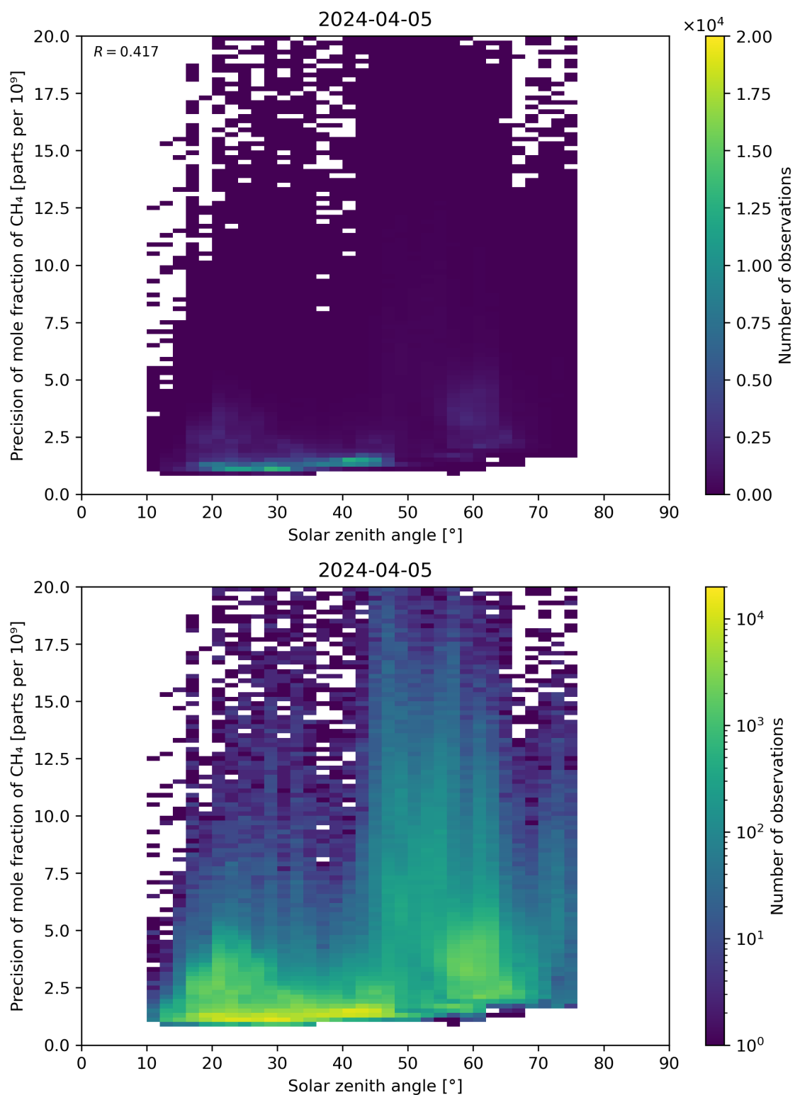
Figure 101: Scatter density plot of “Solar zenith angle” against “Precision of mole fraction of CH 4 ” for 2024-04-05 to 2024-04-06.
