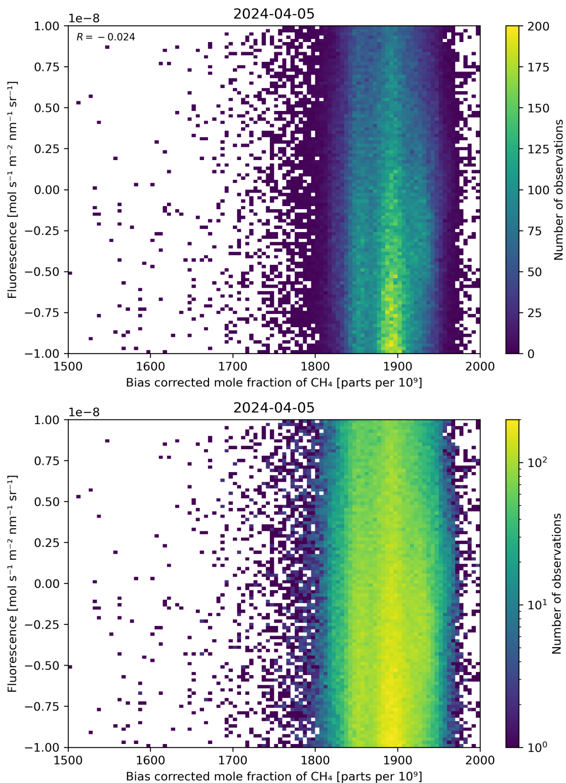
Figure 66: Scatter density plot of “Bias corrected mole fraction of \text{CH}_4 ” against “Fluorescence” for 2024-04-05 to 2024-04-06.
