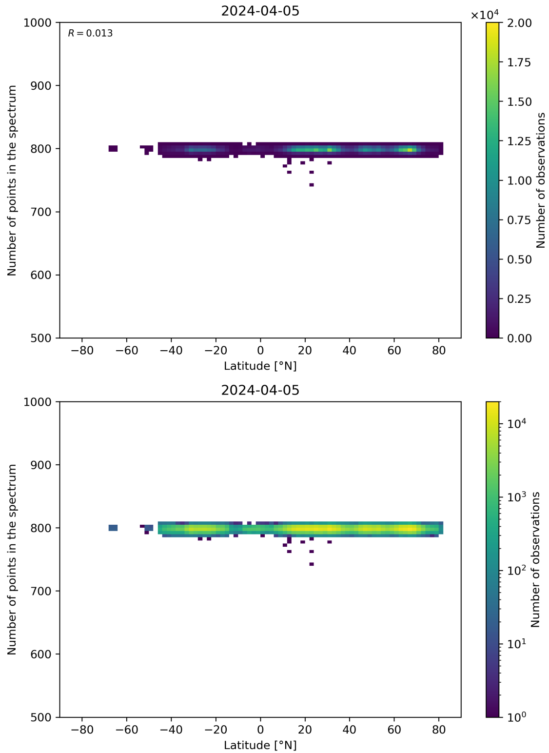
Figure 61: Scatter density plot of “Latitude” against “Number of points in the spectrum” for 2024-04-05 to 2024-04-06.
