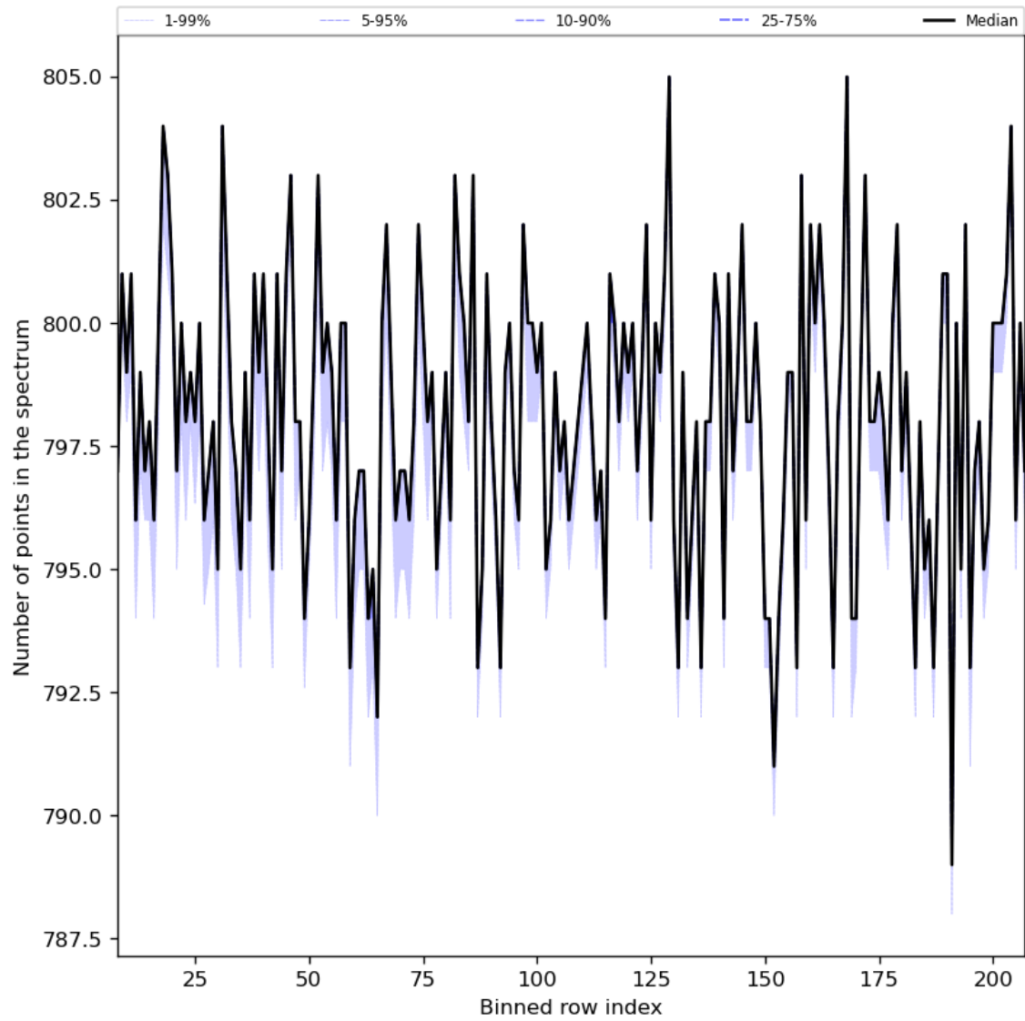
Figure 37: Along track statistics of “Number of points in the spectrum” for 2024-04-05 to 2024-04-06
