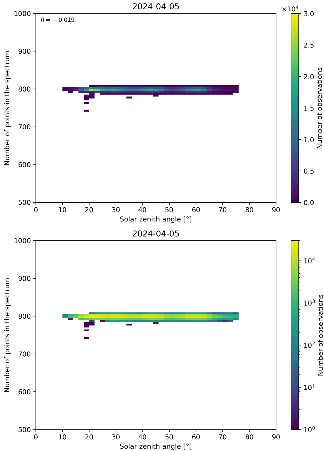
Figure 103: Scatter density plot of “Solar zenith angle” against “Number of points in the spectrum” for 2024-04-05 to 2024-04-06.
