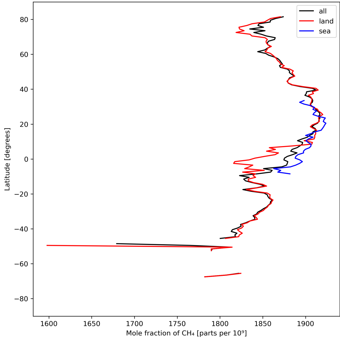
Figure 12: Zonal average of “Mole fraction of \text{CH}_4 ” for 2024-04-05 to 2024-04-06.
