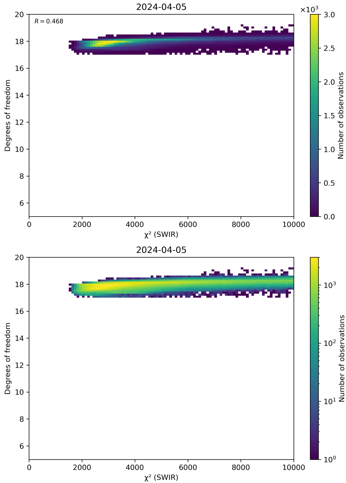
Figure 48: Scatter density plot of " \chi^2 (SWIR)" against "Degrees of freedom" for 2024-04-05 to 2024-04-06.
