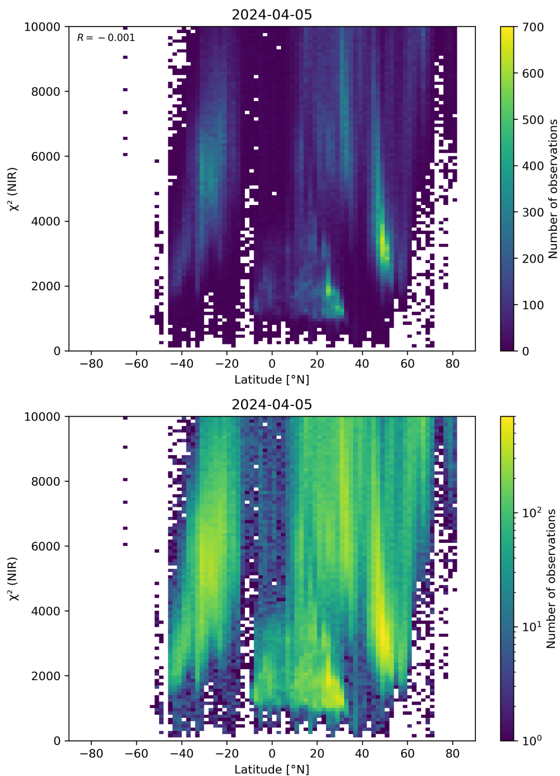
Figure 53: Scatter density plot of “Latitude” against “ \chi^2 (NIR)” for 2024-04-05 to 2024-04-06.
