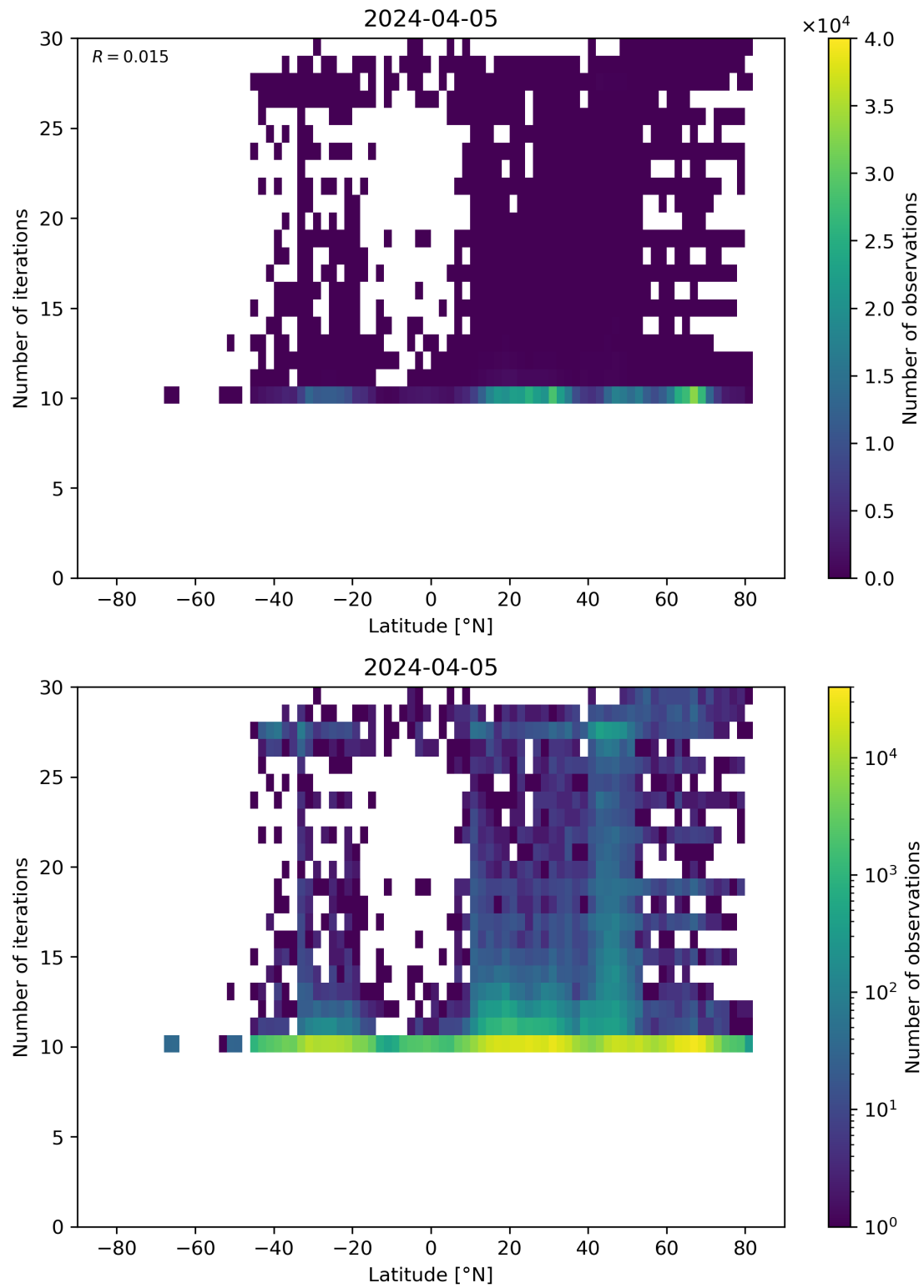
Figure 60: Scatter density plot of “Latitude” against “Number of iterations” for 2024-04-05 to 2024-04-06.
