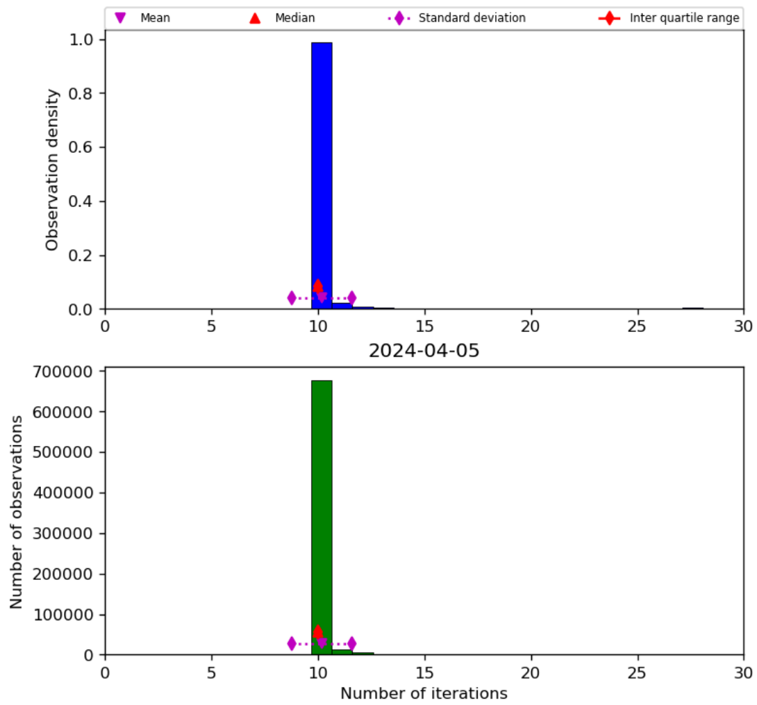
Figure 31: Histogram of “Number of iterations” for 2024-04-05 to 2024-04-06
