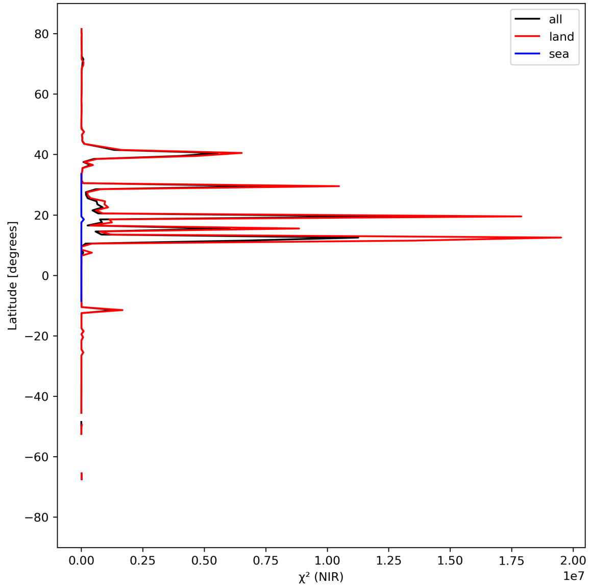
Figure 18: Zonal average of “ \chi^2 (NIR)” for 2024-04-05 to 2024-04-06.
