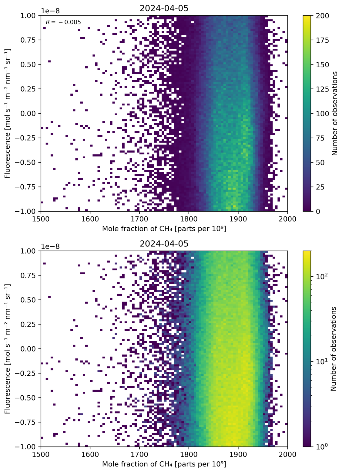
Figure 73: Scatter density plot of “Mole fraction of \text{CH}_4 ” against “Fluorescence” for 2024-04-05 to 2024-04-06.
