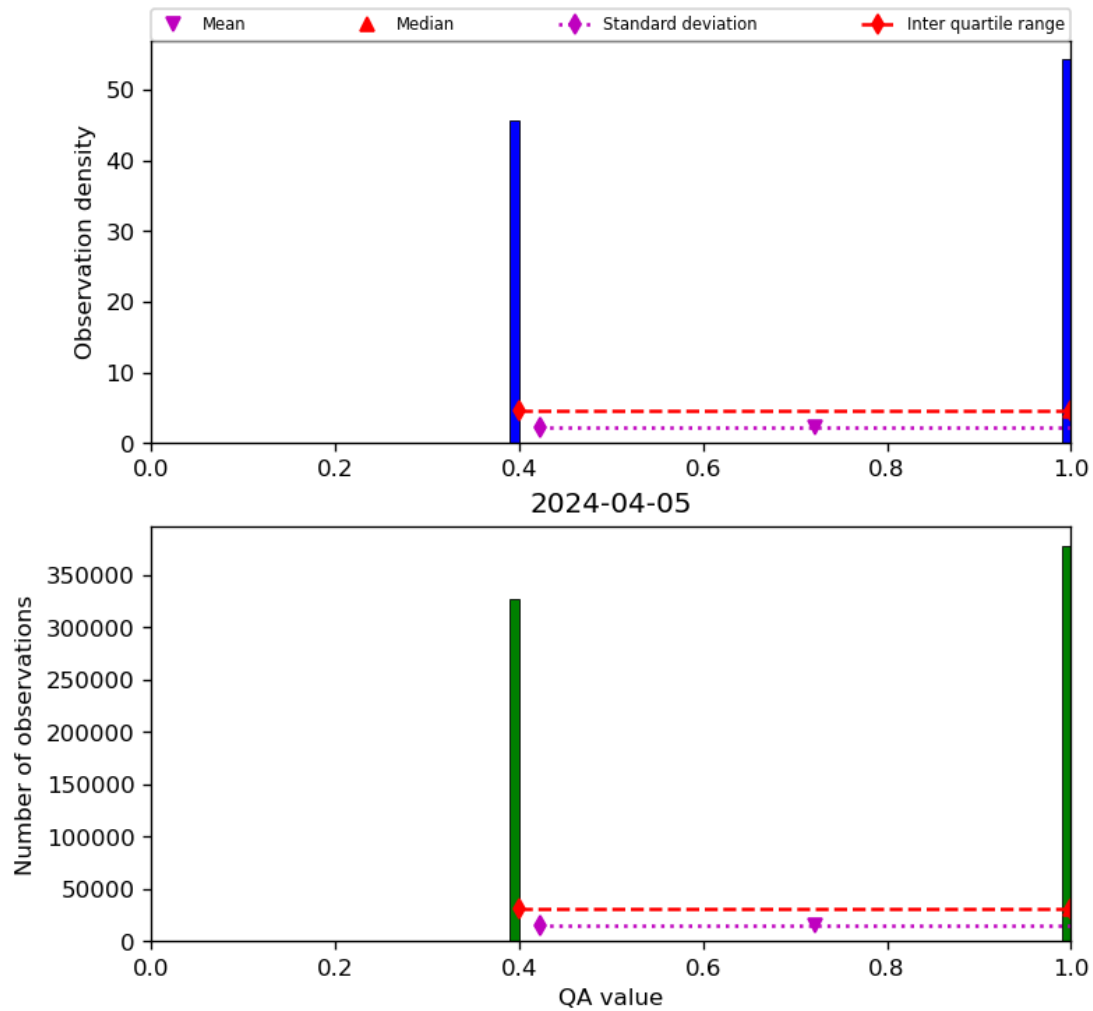
Figure 22: Histogram of “QA value” for 2024-04-05 to 2024-04-06
