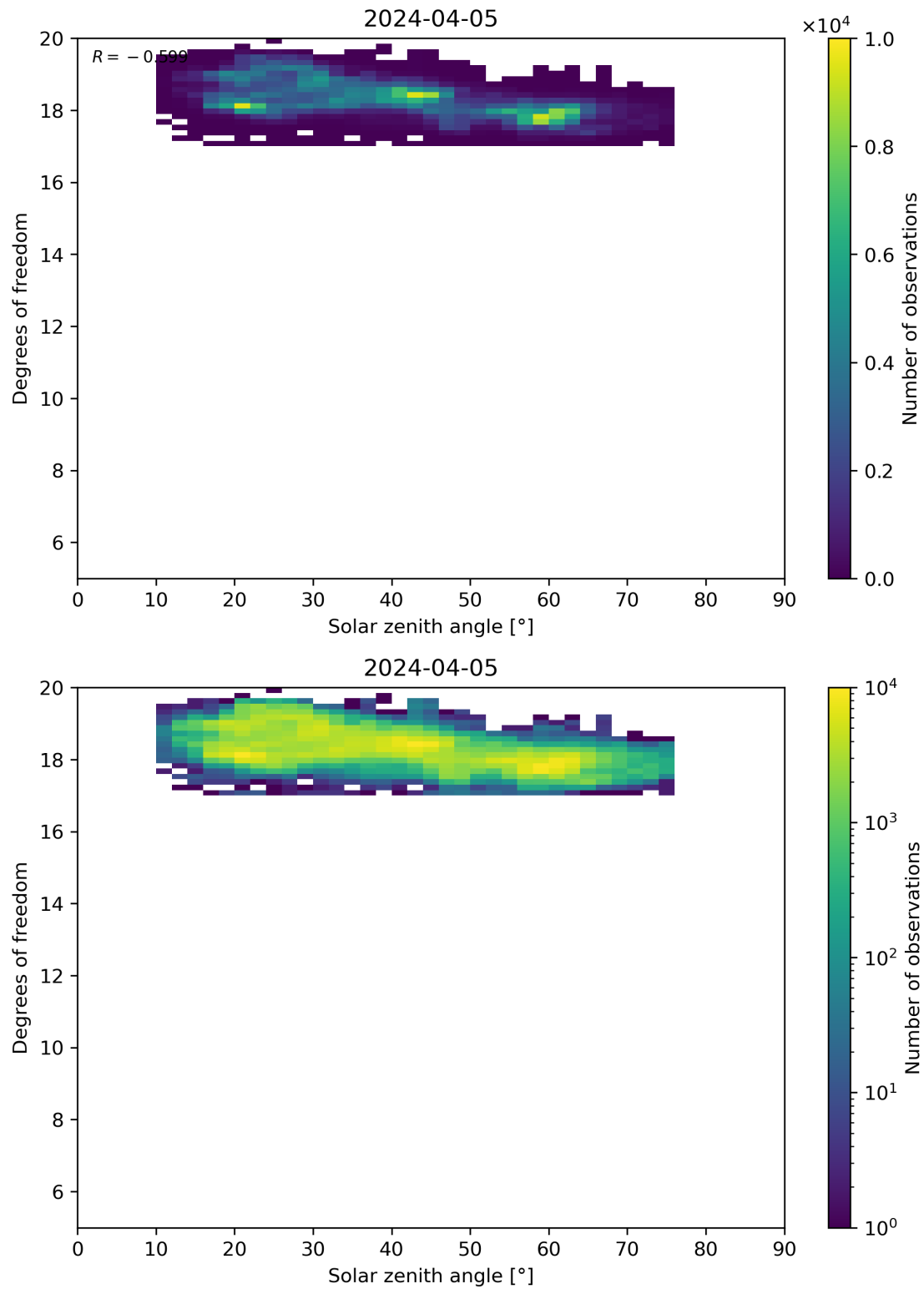
Figure 96: Scatter density plot of “Solar zenith angle” against “Degrees of freedom” for 2024-04-05 to 2024-04-06.
