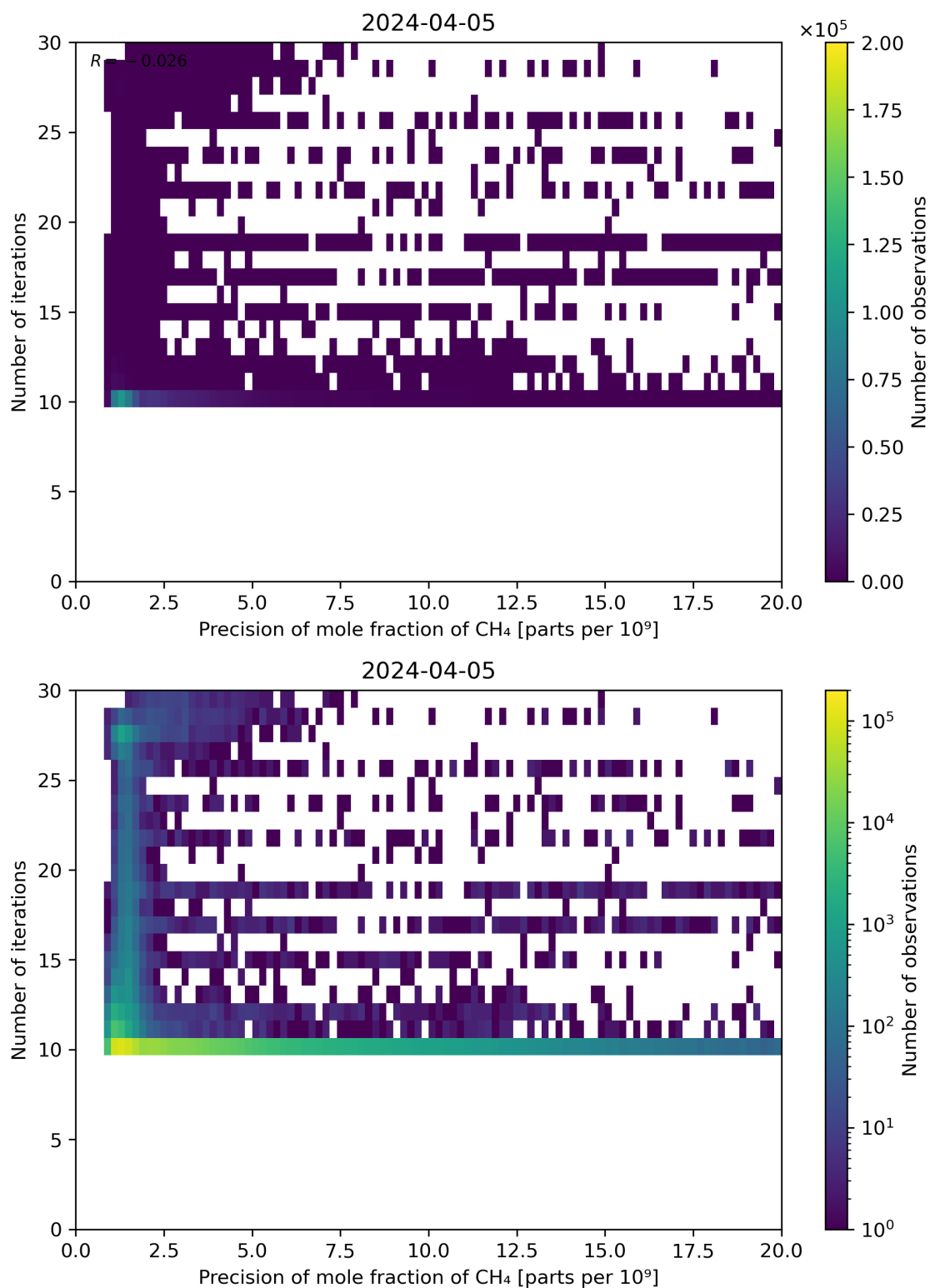
Figure 83: Scatter density plot of “Precision of mole fraction of CH 4 ” against “Number of iterations” for 2024-04-05 to 2024-04-06.
