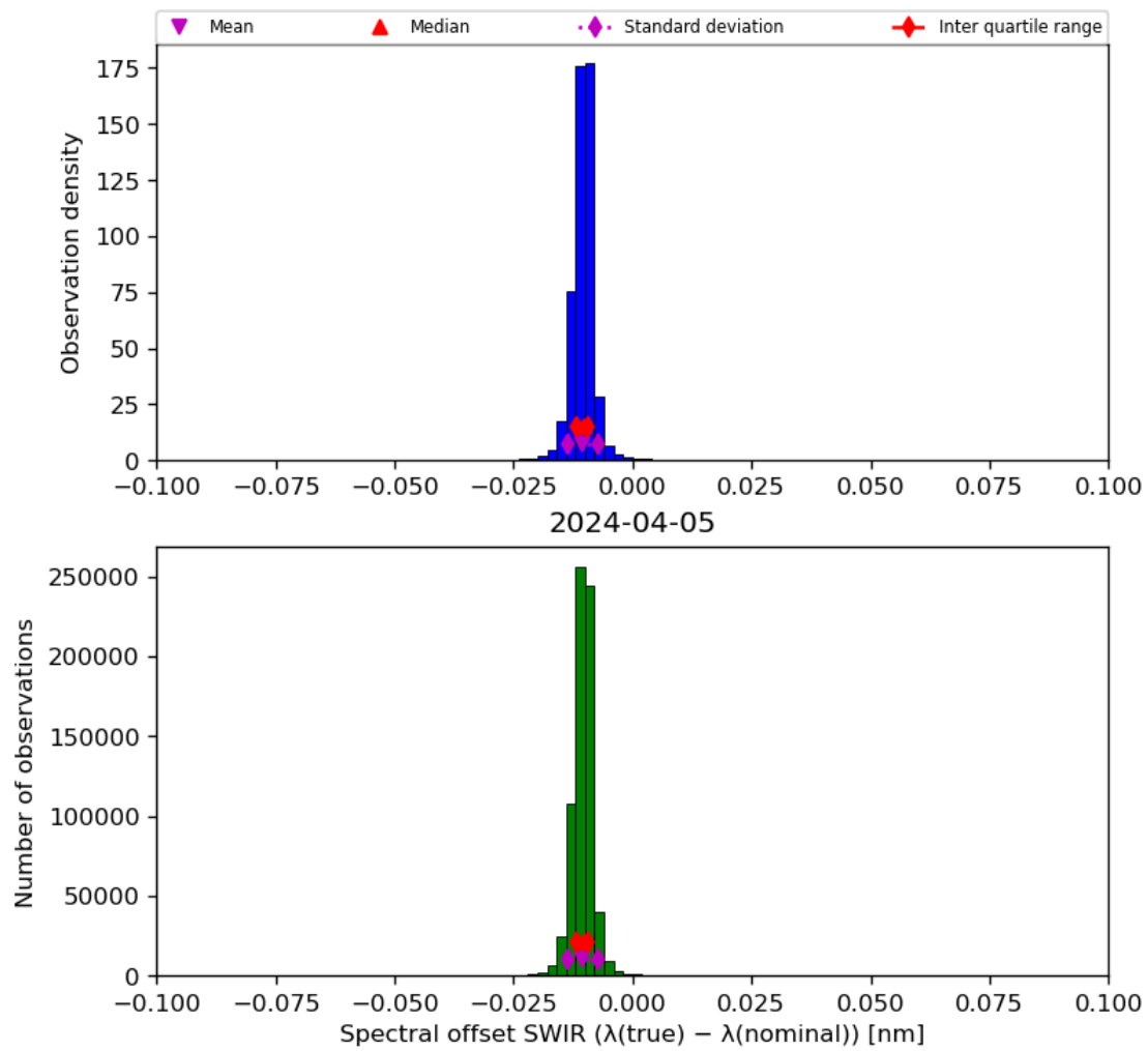
Figure 27: Histogram of “Spectral offset SWIR ( \lambda(\text{true}) - \lambda(\text{nominal}) )” for 2024-04-05 to 2024-04-06
