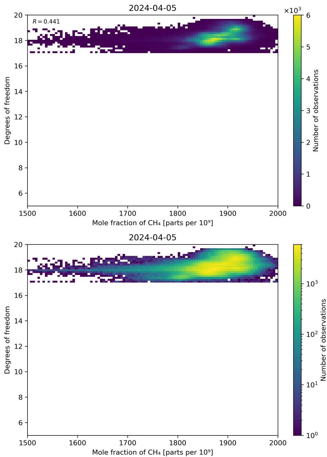
Figure 72: Scatter density plot of “Mole fraction of CH 4 ” against “Degrees of freedom” for 2024-04-05 to 2024-04-06.
