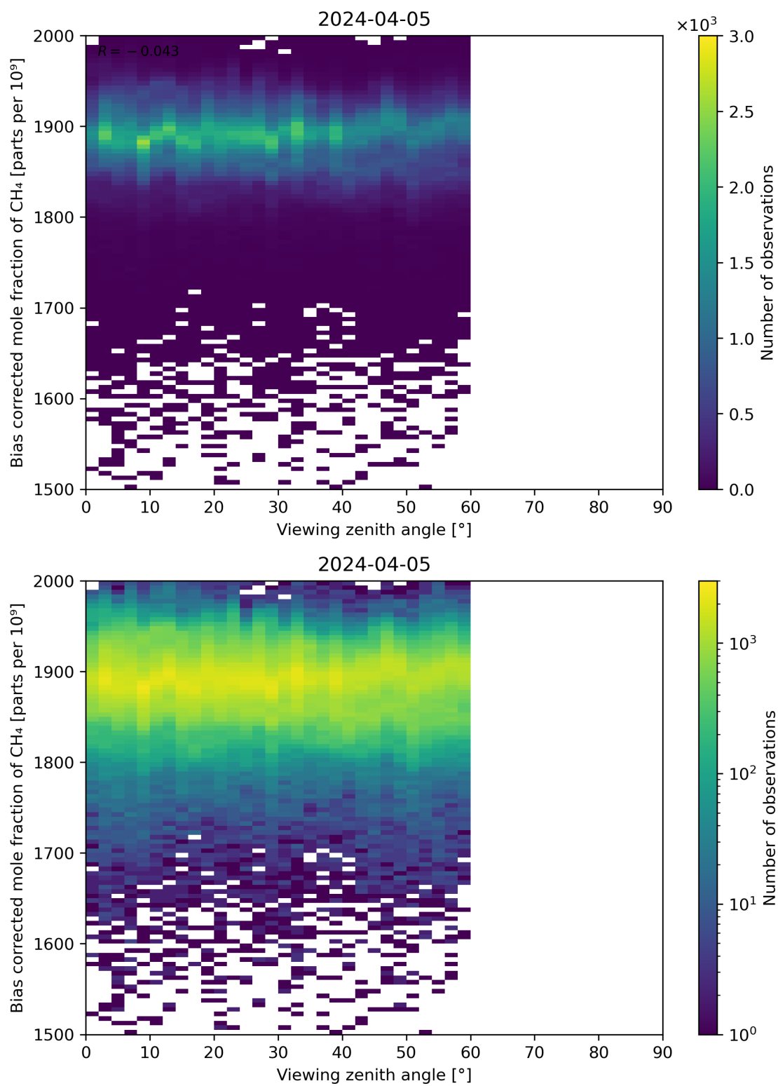
Figure 111: Scatter density plot of “Viewing zenith angle” against “Bias corrected mole fraction of CH 4 ” for 2024-04-05 to 2024-04-06.
