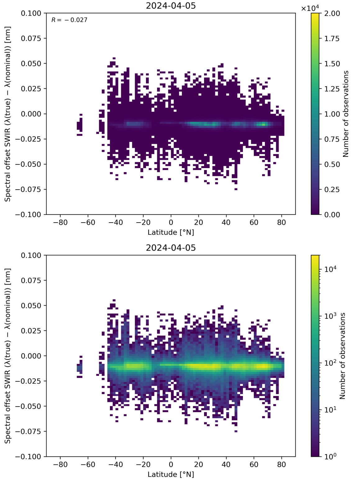
Figure 62: Scatter density plot of “Latitude” against “Spectral offset SWIR ( \lambda(\text{true}) - \lambda(\text{nominal}) )” for 2024-04-05 to 2024-04-06.
