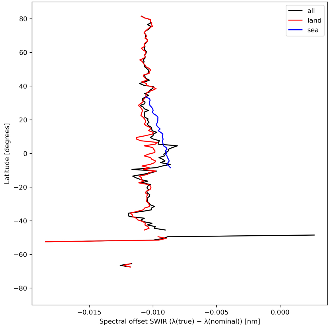
Figure 16: Zonal average of “Spectral offset SWIR ( \lambda(\text{true}) - \lambda(\text{nominal}) )” for 2024-04-05 to 2024-04-06.
