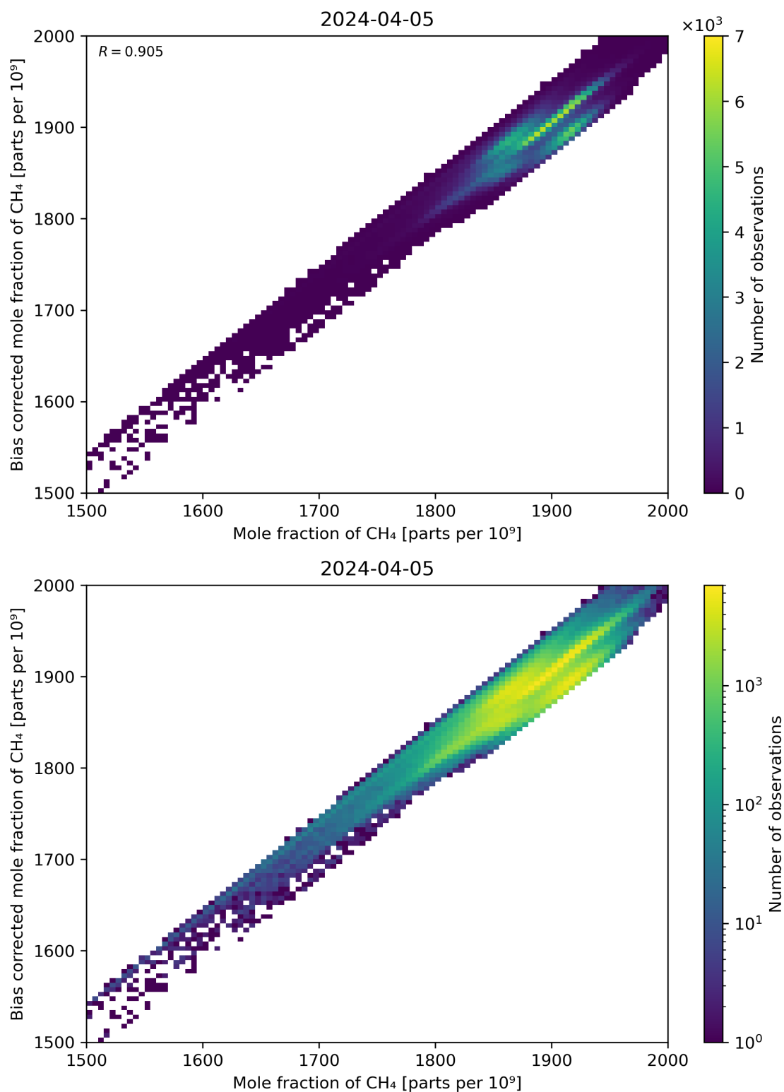
Figure 74: Scatter density plot of “Mole fraction of CH 4 ” against “Bias corrected mole fraction of CH 4 ” for 2024-04-05 to 2024-04-06.
