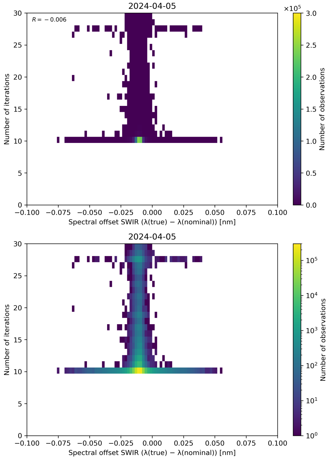
Figure 121: Scatter density plot of “Spectral offset SWIR ( \lambda(\text{true}) - \lambda(\text{nominal}) )” against “Number of iterations” for 2024-04-05 to 2024-04-06.
