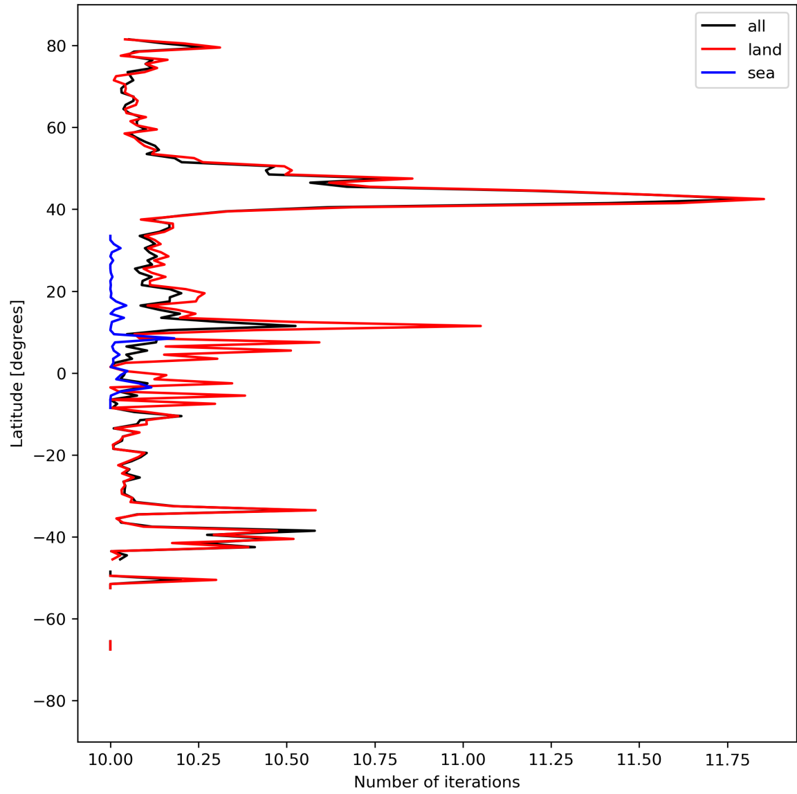
Figure 20: Zonal average of “Number of iterations” for 2024-04-05 to 2024-04-06.
