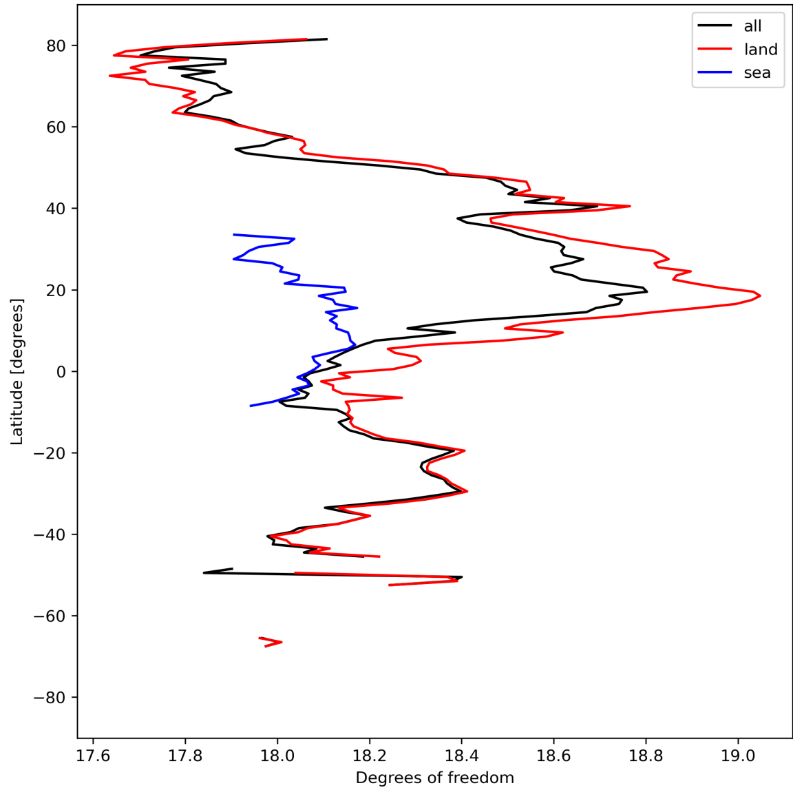
Figure 19: Zonal average of “Degrees of freedom” for 2024-04-05 to 2024-04-06.
