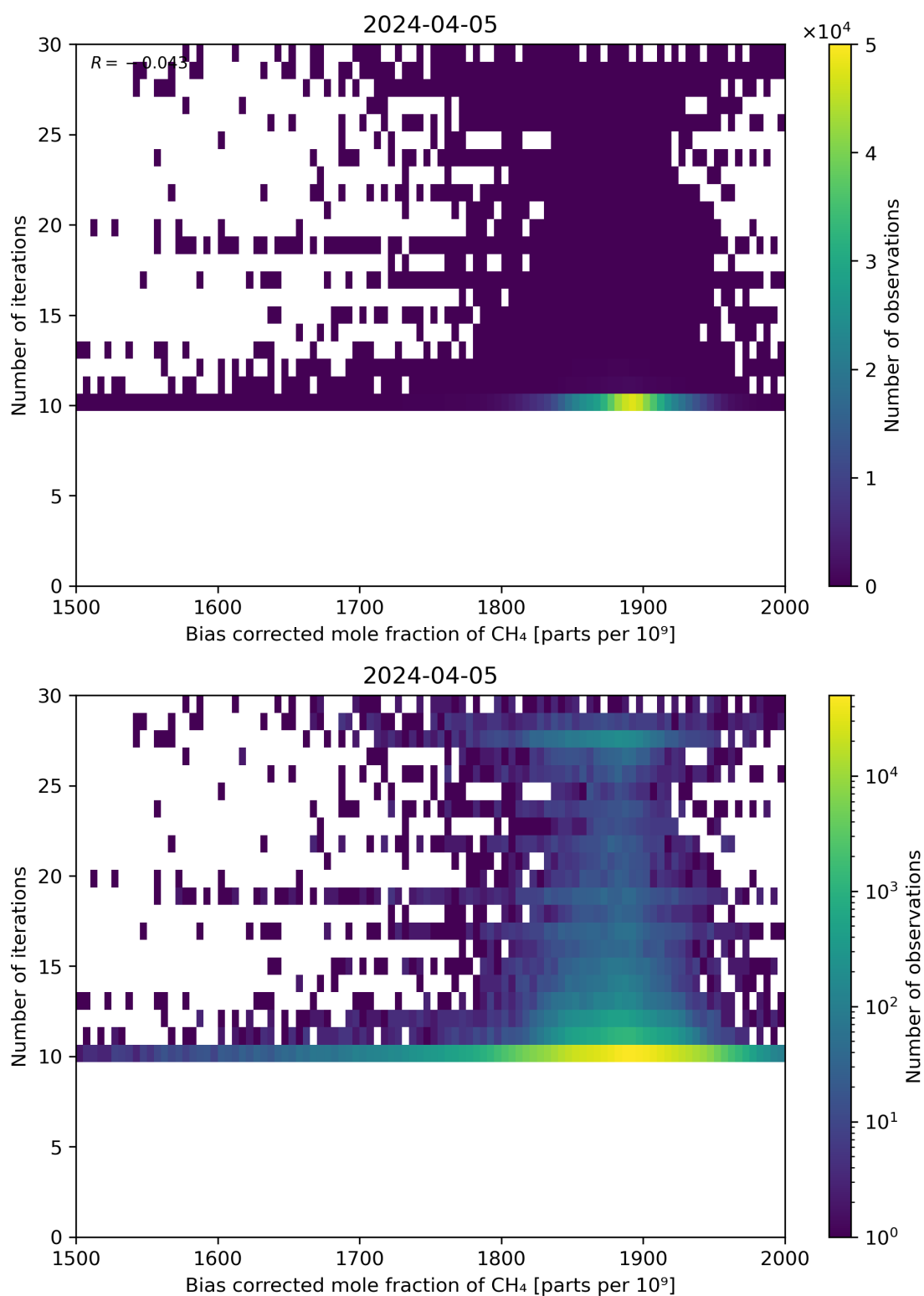
Figure 67: Scatter density plot of “Bias corrected mole fraction of CH 4 ” against “Number of iterations” for 2024-04-05 to 2024-04-06.
