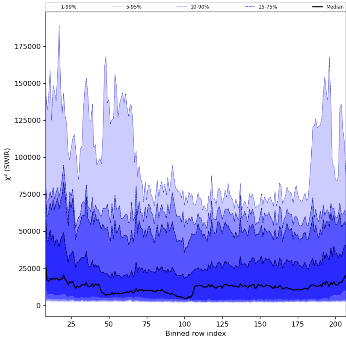
Figure 39: Along track statistics of " \chi^2 (SWIR)" for 2024-04-05 to 2024-04-06
