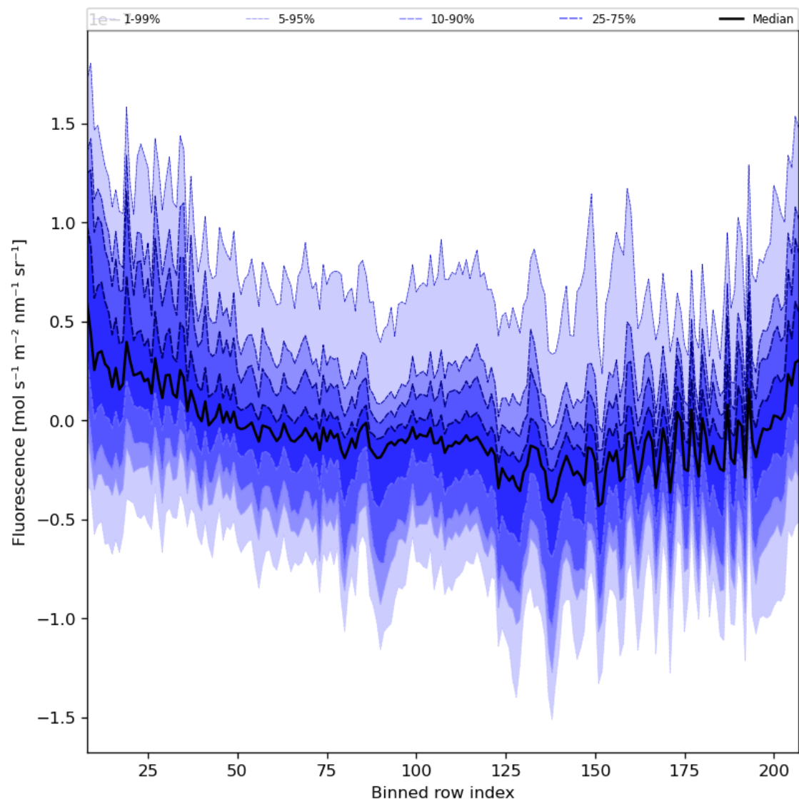
Figure 43: Along track statistics of “Fluorescence” for 2024-04-05 to 2024-04-06
