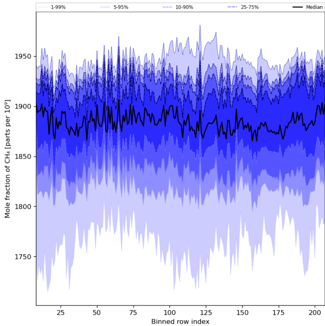
Figure 34: Along track statistics of “Mole fraction of CH 4 ” for 2024-04-05 to 2024-04-06
