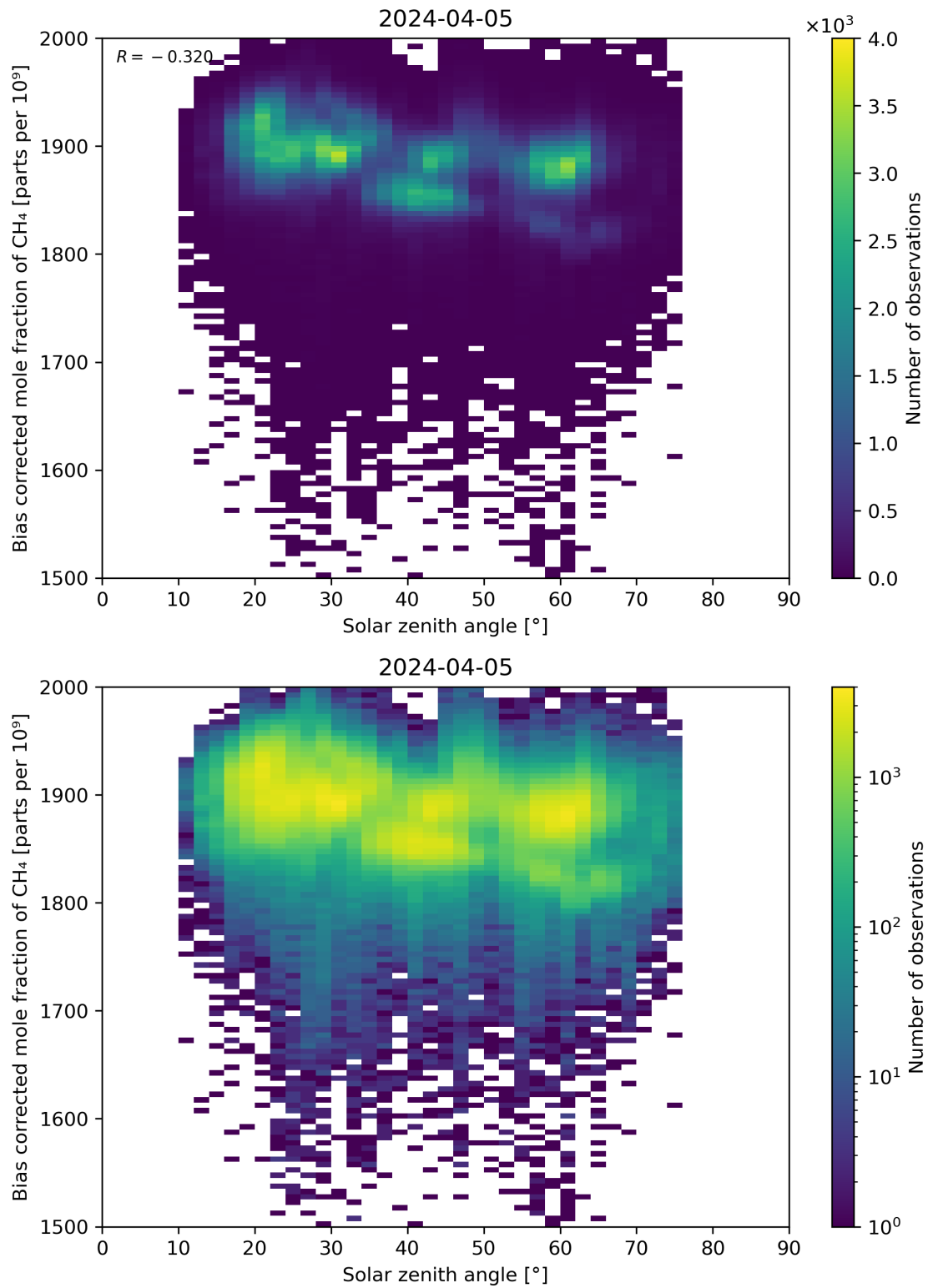
Figure 100: Scatter density plot of “Solar zenith angle” against “Bias corrected mole fraction of CH 4 ” for 2024-04-05 to 2024-04-06.
