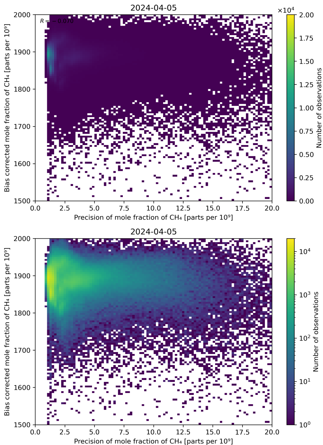
Figure 82: Scatter density plot of “Precision of mole fraction of CH 4 ” against “Bias corrected mole fraction of CH 4 ” for 2024-04-05 to 2024-04-06.
