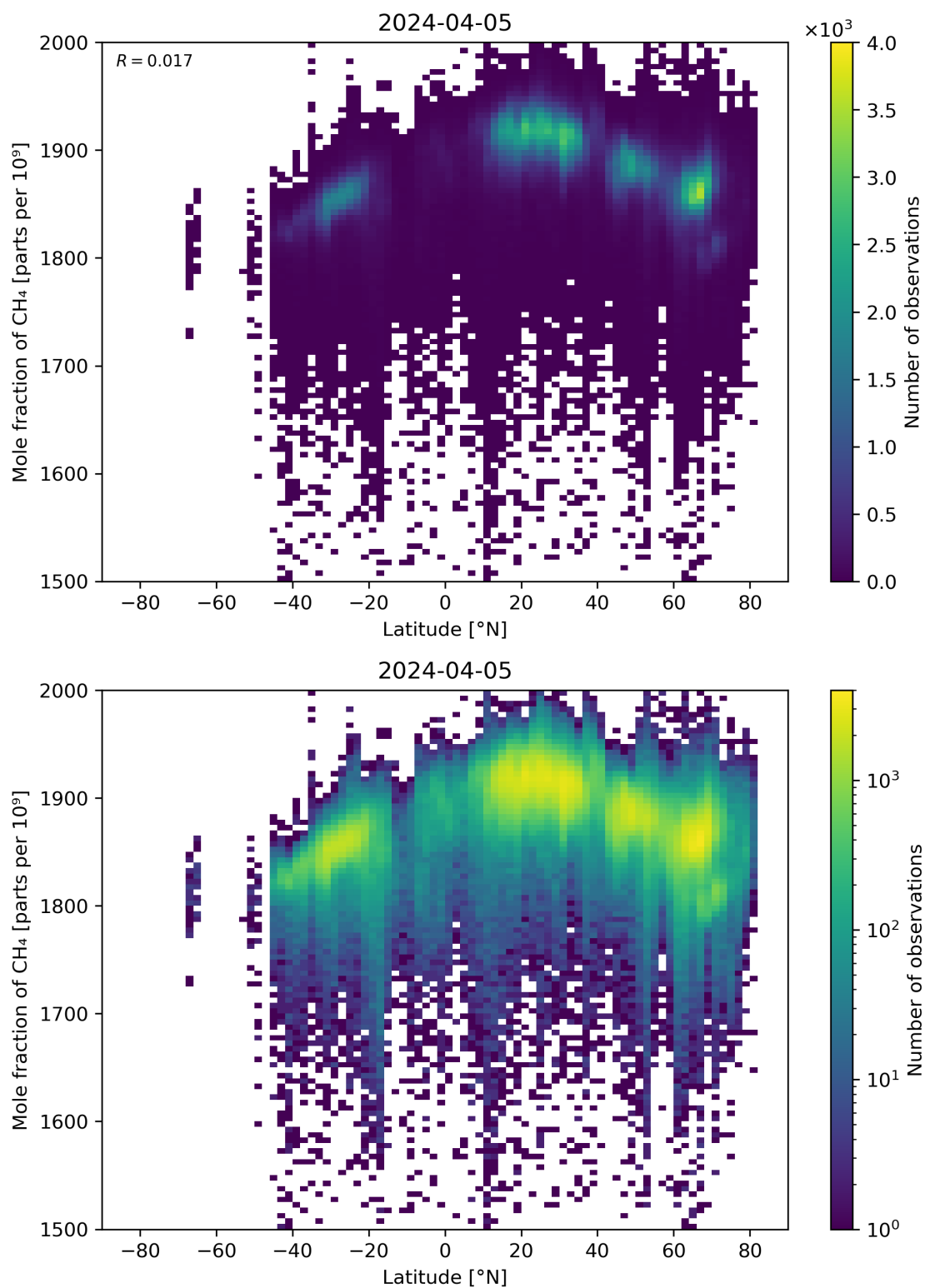
Figure 57: Scatter density plot of “Latitude” against “Mole fraction of \text{CH}_4 ” for 2024-04-05 to 2024-04-06.
