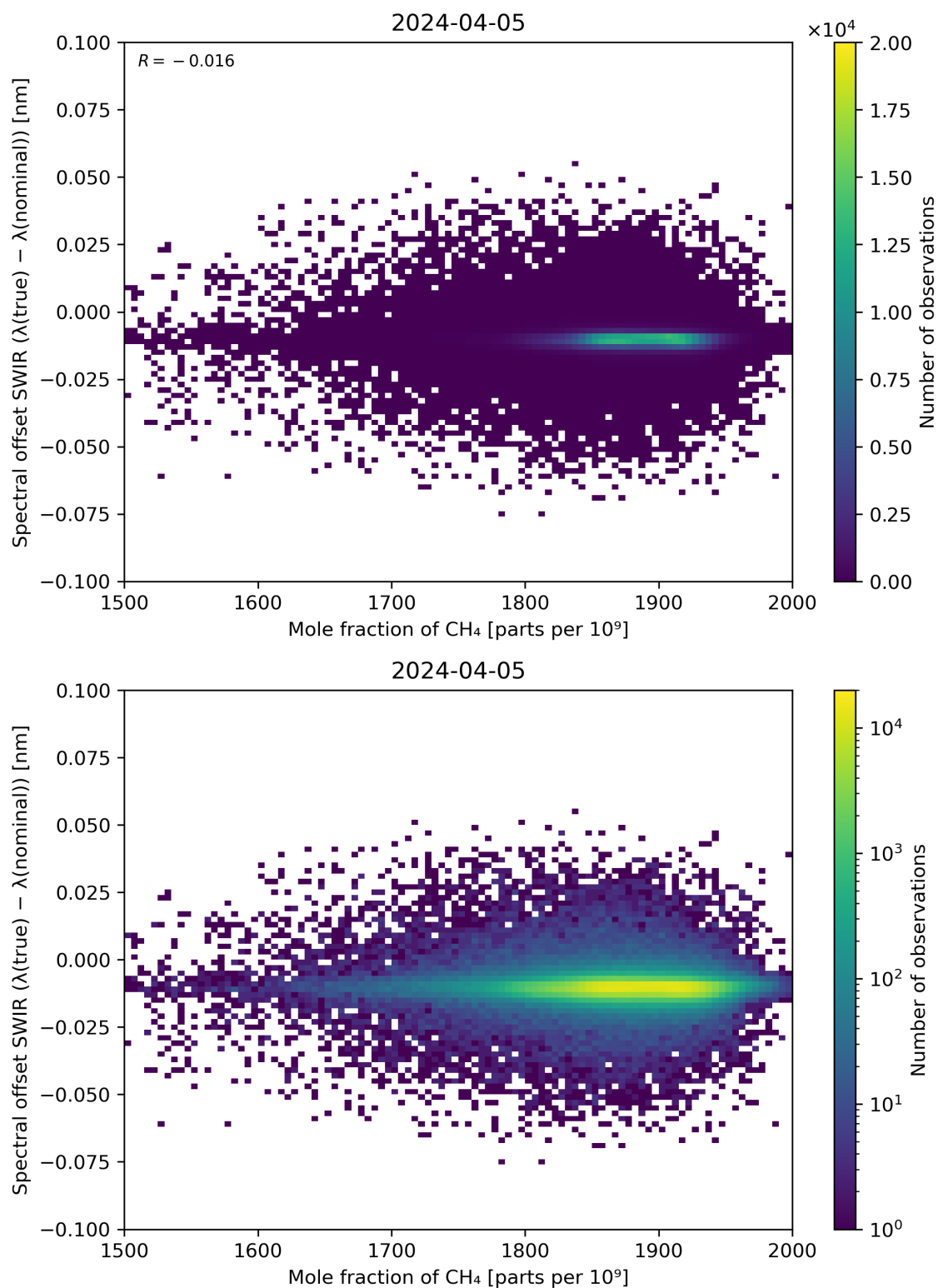
Figure 86: Scatter density plot of “Mole fraction of CH 4 ” against “Spectral offset SWIR ( \lambda(\text{true}) - \lambda(\text{nominal}) )” for 2024-04-05 to 2024-04-06.
