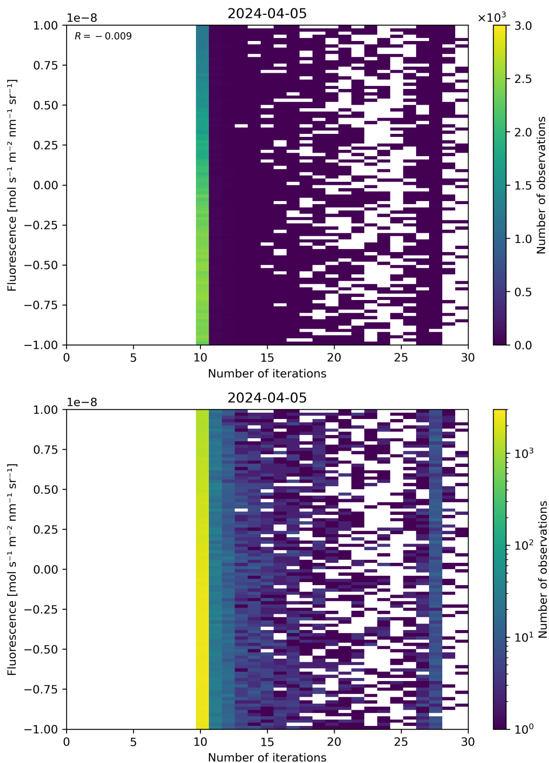
Figure 87: Scatter density plot of “Number of iterations” against “Fluorescence” for 2024-04-05 to 2024-04-06.
