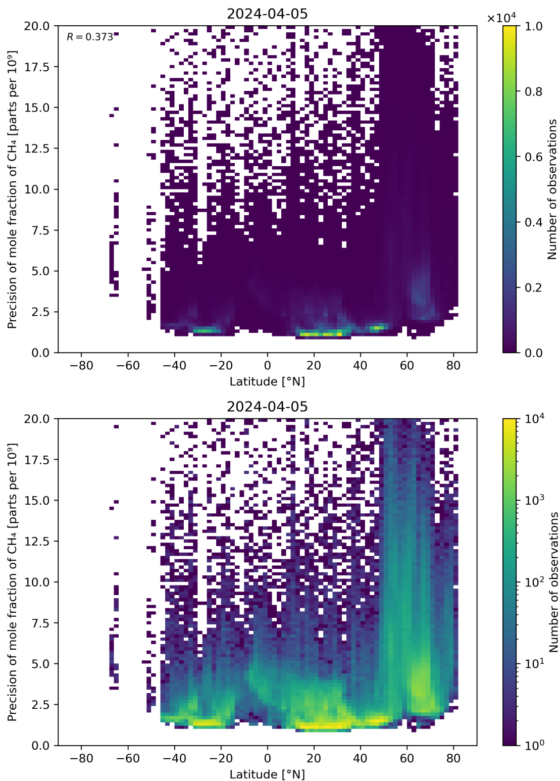
Figure 59: Scatter density plot of “Latitude” against “Precision of mole fraction of \text{CH}_4 ” for 2024-04-05 to 2024-04-06.
