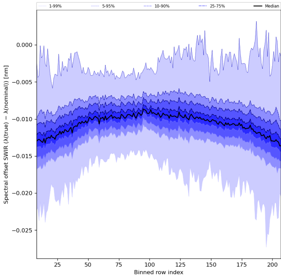
Figure 38: Along track statistics of “Spectral offset SWIR ( \lambda(\text{true}) - \lambda(\text{nominal}) )” for 2024-04-05 to 2024-04-06
