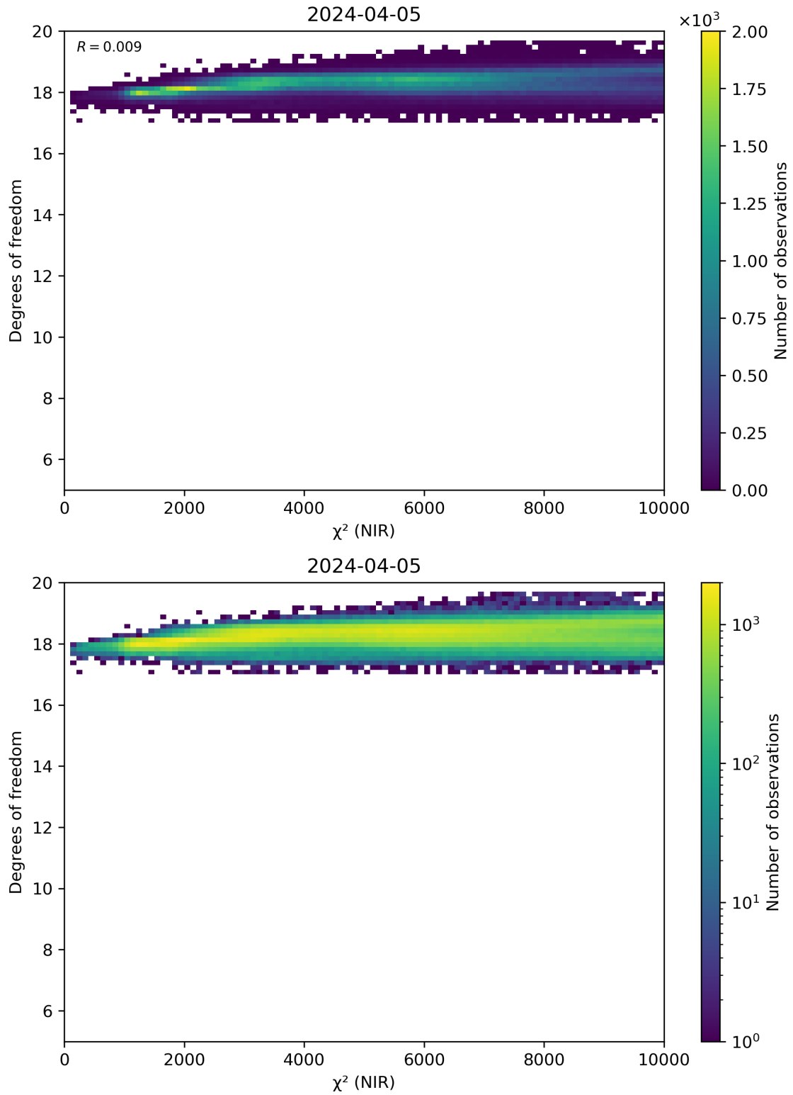
Figure 44: Scatter density plot of “ \chi^2 (NIR)” against “Degrees of freedom” for 2024-04-05 to 2024-04-06.
