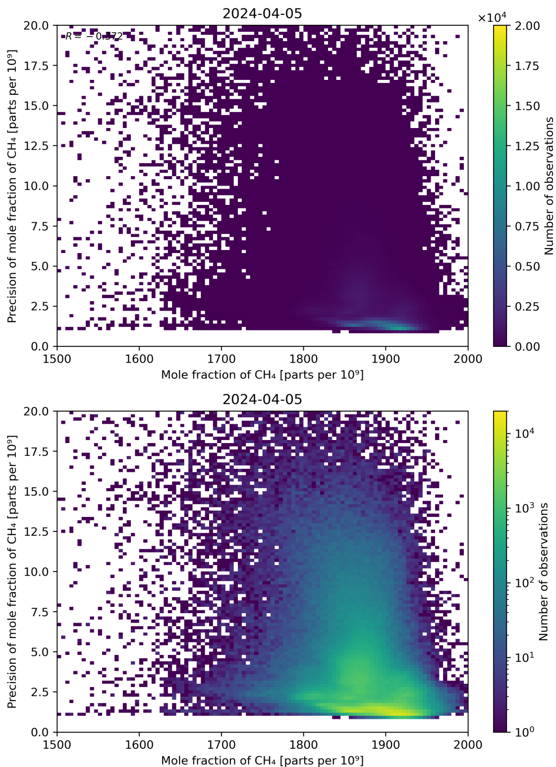
Figure 75: Scatter density plot of “Mole fraction of CH 4 ” against “Precision of mole fraction of CH 4 ” for 2024-04-05 to 2024-04-06.
