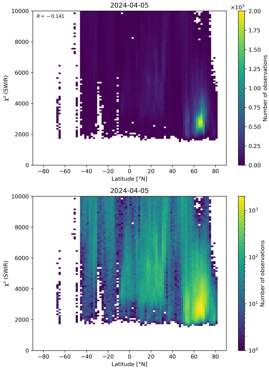
Figure 54: Scatter density plot of “Latitude” against “ \chi^2 (SWIR)” for 2024-04-05 to 2024-04-06.
