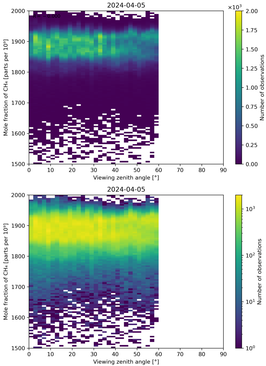
Figure 110: Scatter density plot of “Viewing zenith angle” against “Mole fraction of CH 4 ” for 2024-04-05 to 2024-04-06.
