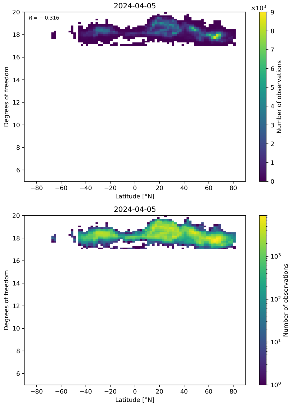
Figure 55: Scatter density plot of “Latitude” against “Degrees of freedom” for 2024-04-05 to 2024-04-06.
