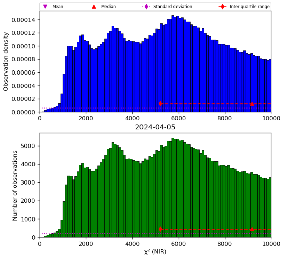
Figure 29: Histogram of " \chi^2 (NIR)" for 2024-04-05 to 2024-04-06
