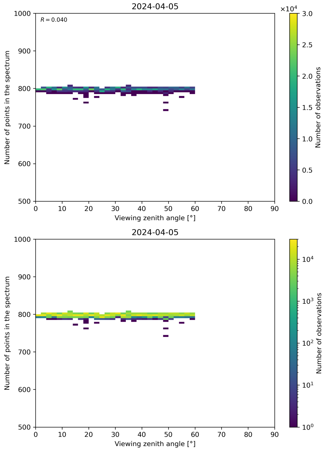
Figure 114: Scatter density plot of “Viewing zenith angle” against “Number of points in the spectrum” for 2024-04-05 to 2024-04-06.
