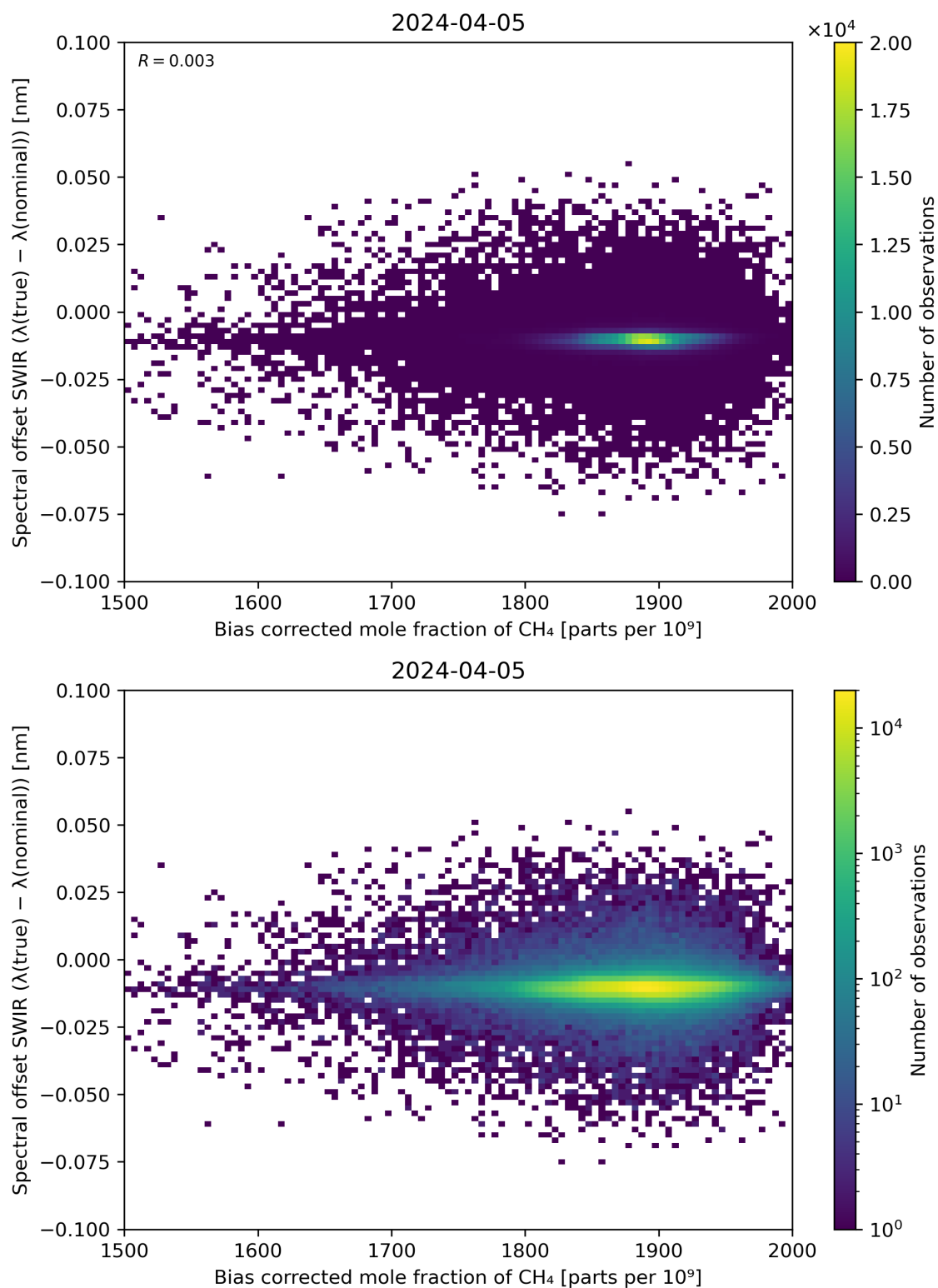
Figure 69: Scatter density plot of “Bias corrected mole fraction of \text{CH}_4 ” against “Spectral offset SWIR ( \lambda(\text{true}) - \lambda(\text{nominal}) )” for 2024-04-05 to 2024-04-06.
