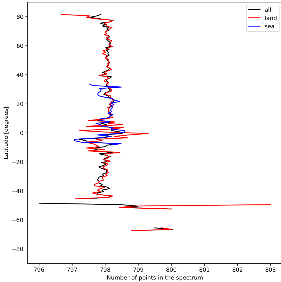
Figure 15: Zonal average of “Number of points in the spectrum” for 2024-04-05 to 2024-04-06.
