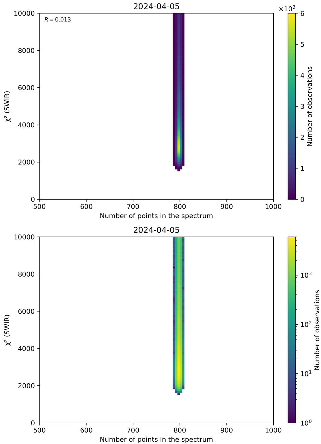
Figure 89: Scatter density plot of “Number of points in the spectrum” against “ \chi^2 (SWIR)” for 2024-04-05 to 2024-04-06.
