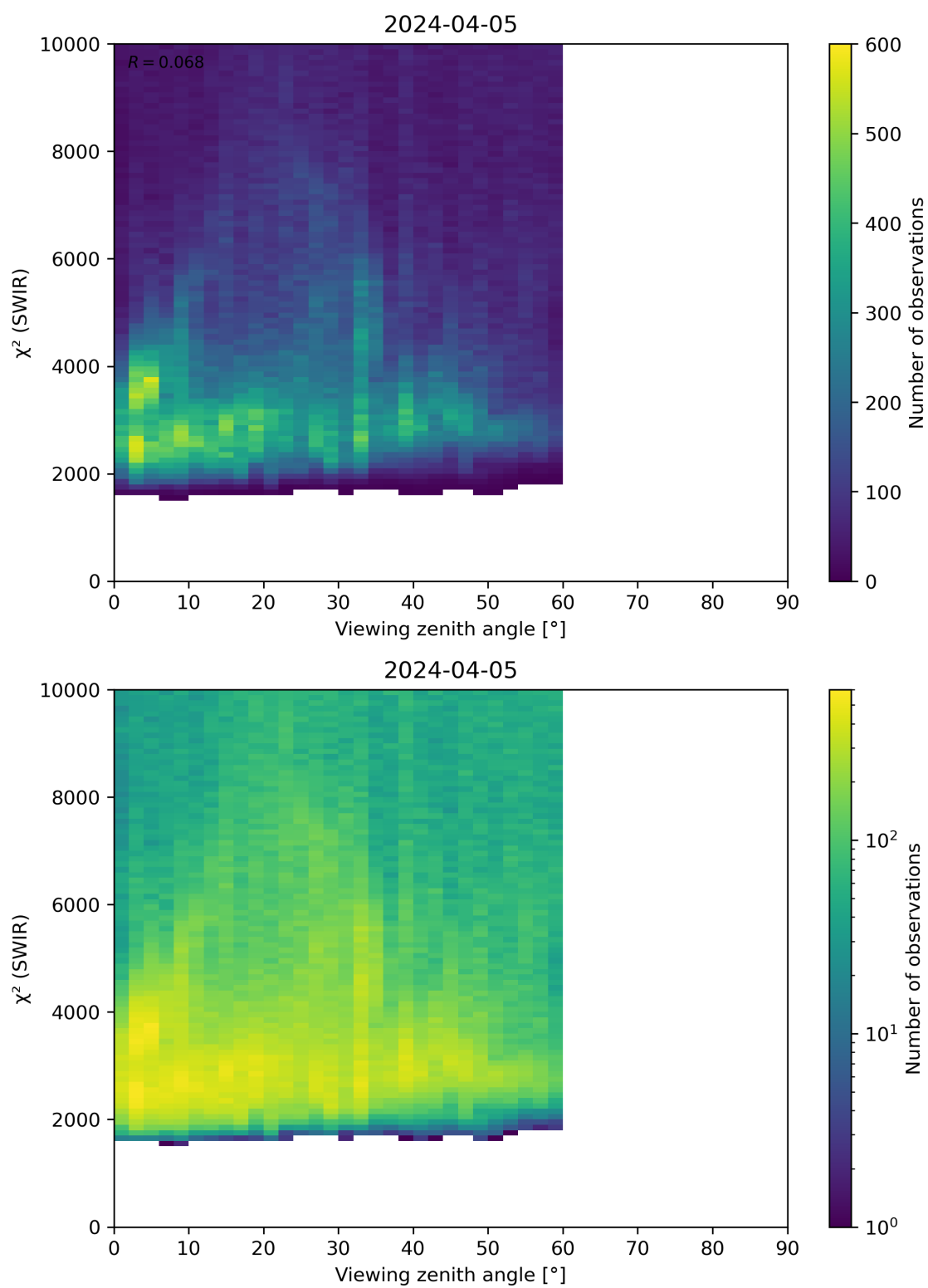
Figure 106: Scatter density plot of “Viewing zenith angle” against “ \chi^2 (SWIR)” for 2024-04-05 to 2024-04-06.
