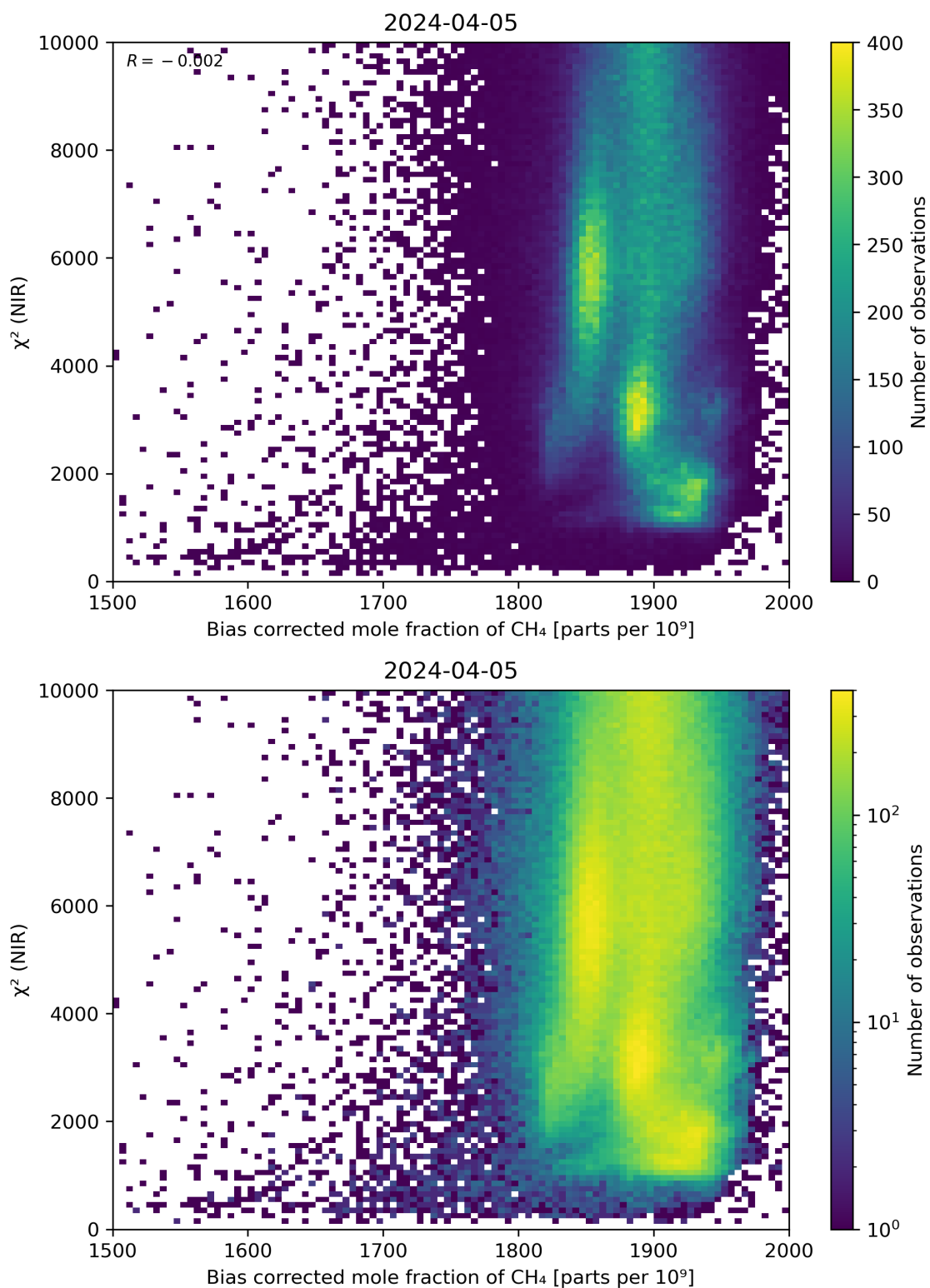
Figure 63: Scatter density plot of “Bias corrected mole fraction of \text{CH}_4 ” against “ \chi^2 (NIR)” for 2024-04-05 to 2024-04-06.
