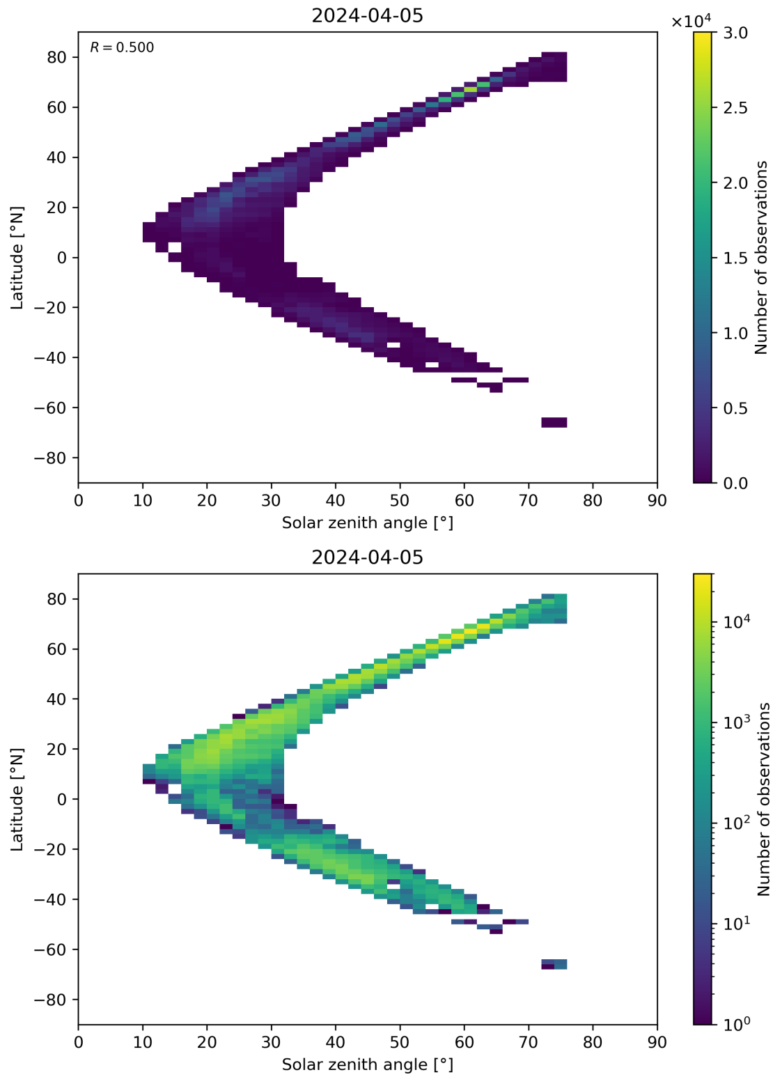
Figure 98: Scatter density plot of “Solar zenith angle” against “Latitude” for 2024-04-05 to 2024-04-06.
