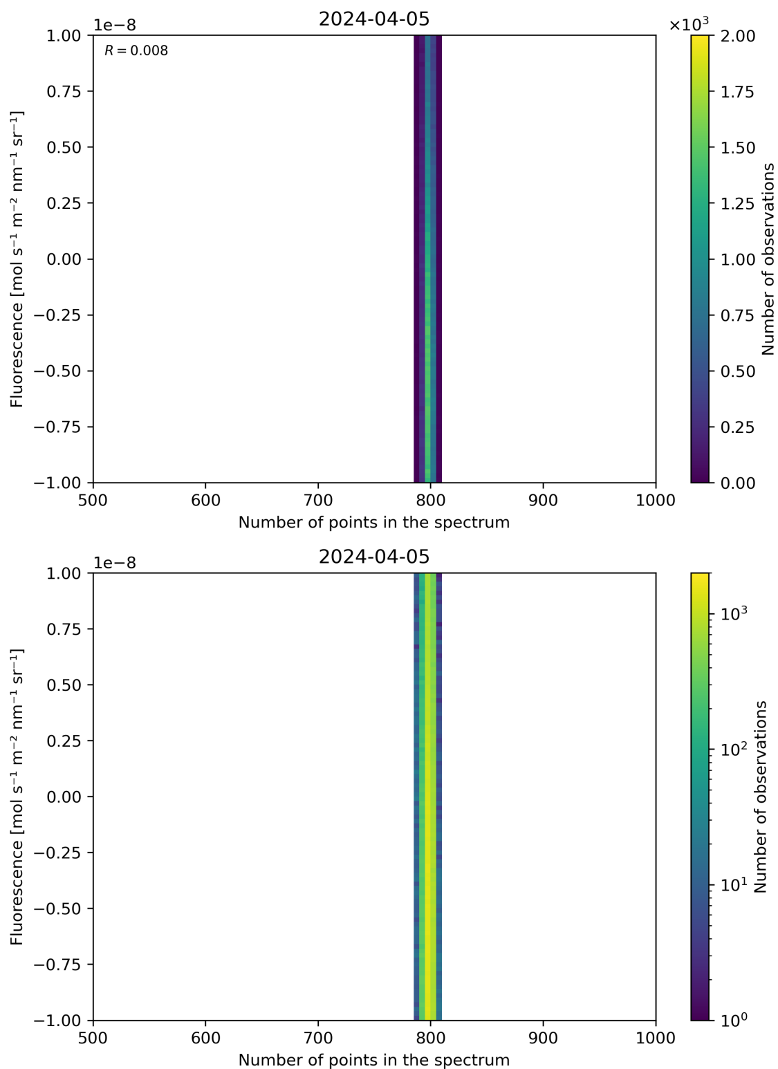
Figure 91: Scatter density plot of “Number of points in the spectrum” against “Fluorescence” for 2024-04-05 to 2024-04-06.
