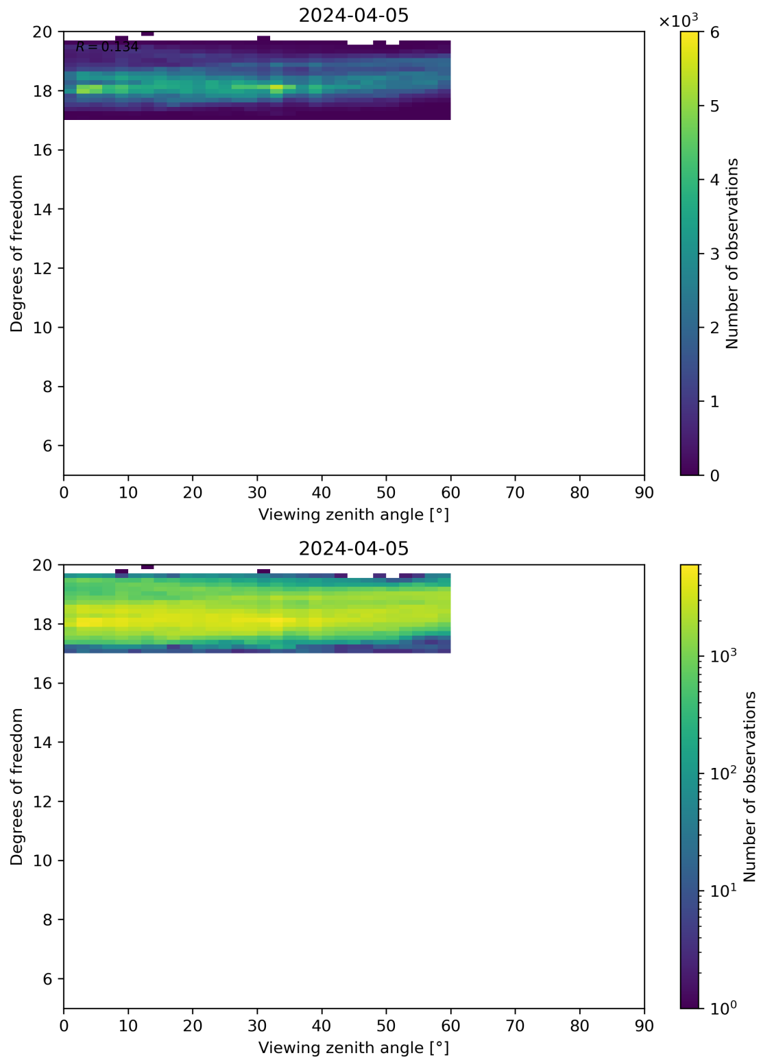
Figure 107: Scatter density plot of “Viewing zenith angle” against “Degrees of freedom” for 2024-04-05 to 2024-04-06.
