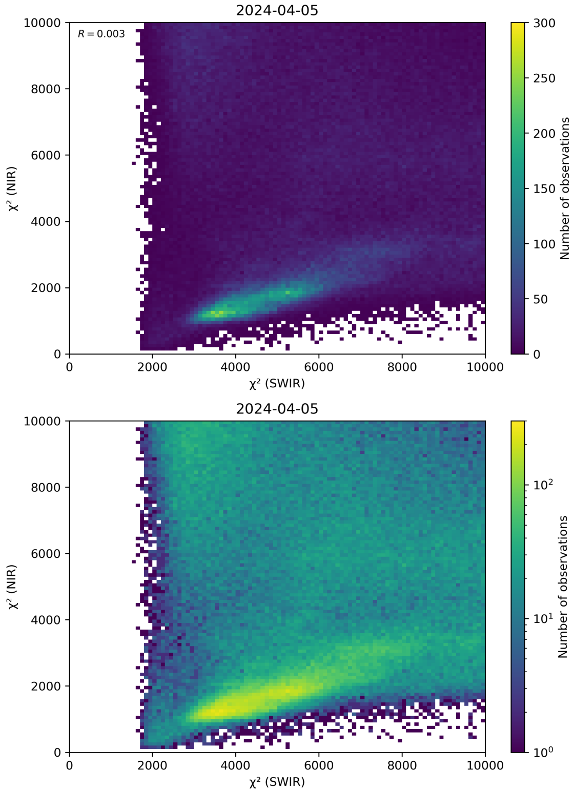
Figure 47: Scatter density plot of “ \chi^2 (SWIR)” against “ \chi^2 (NIR)” for 2024-04-05 to 2024-04-06.
