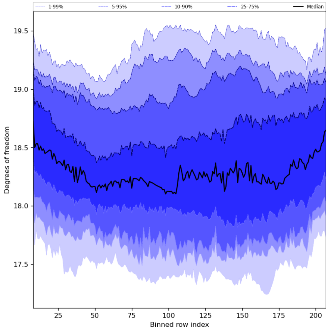
Figure 41: Along track statistics of “Degrees of freedom” for 2024-04-05 to 2024-04-06
