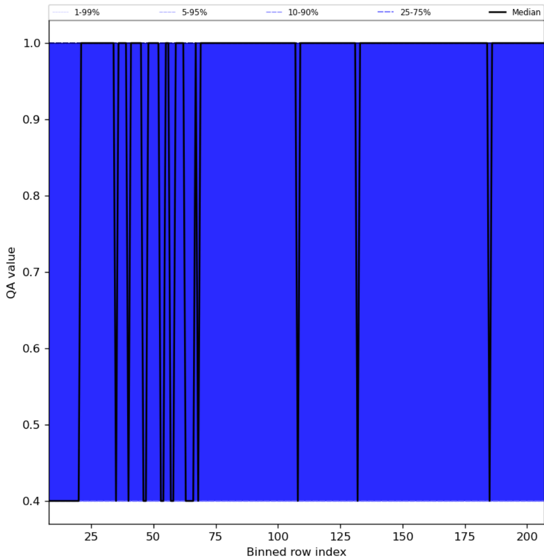
Figure 33: Along track statistics of “QA value” for 2024-04-05 to 2024-04-06
