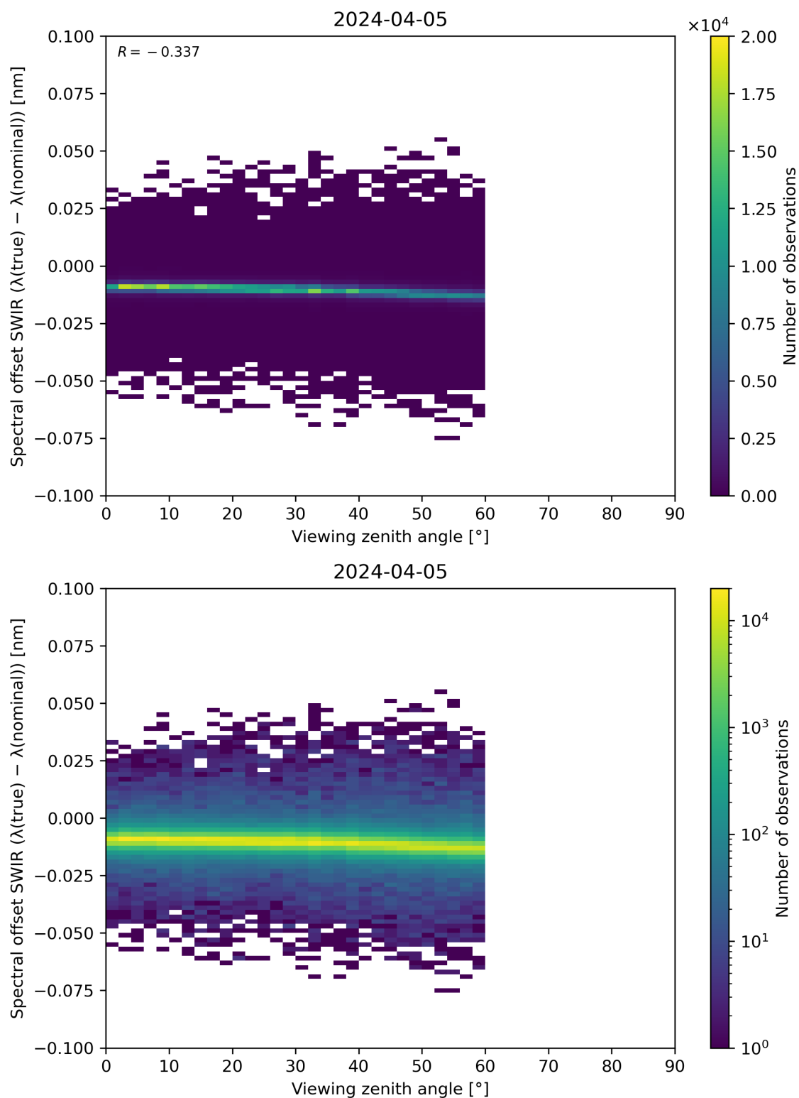
Figure 116: Scatter density plot of “Viewing zenith angle” against “Spectral offset SWIR ( \lambda(\text{true}) - \lambda(\text{nominal}) )” for 2024-04-05 to 2024-04-06.
