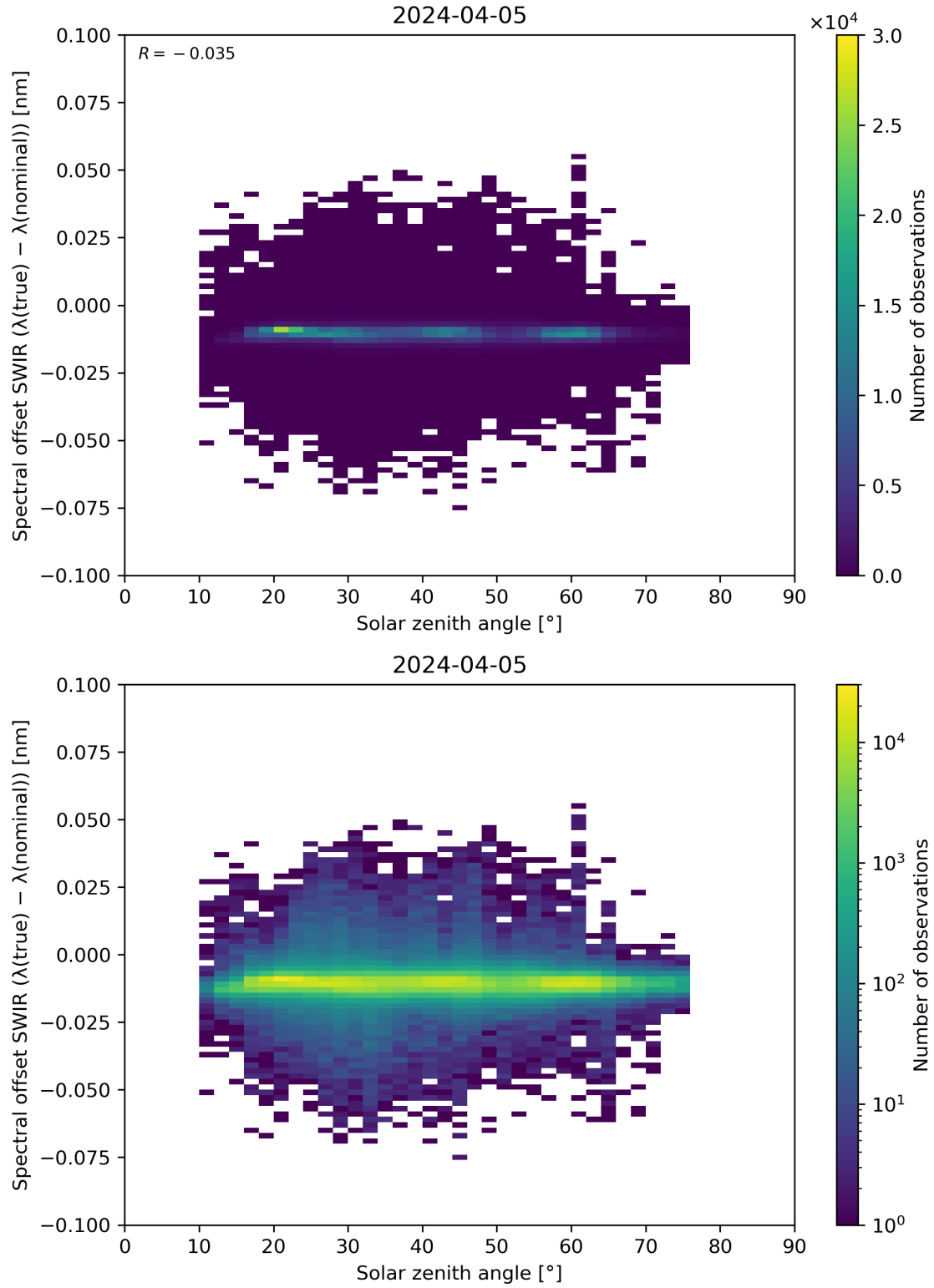
Figure 104: Scatter density plot of “Solar zenith angle” against “Spectral offset SWIR ( \lambda(\text{true}) - \lambda(\text{nominal}) )” for 2024-04-05 to 2024-04-06.
