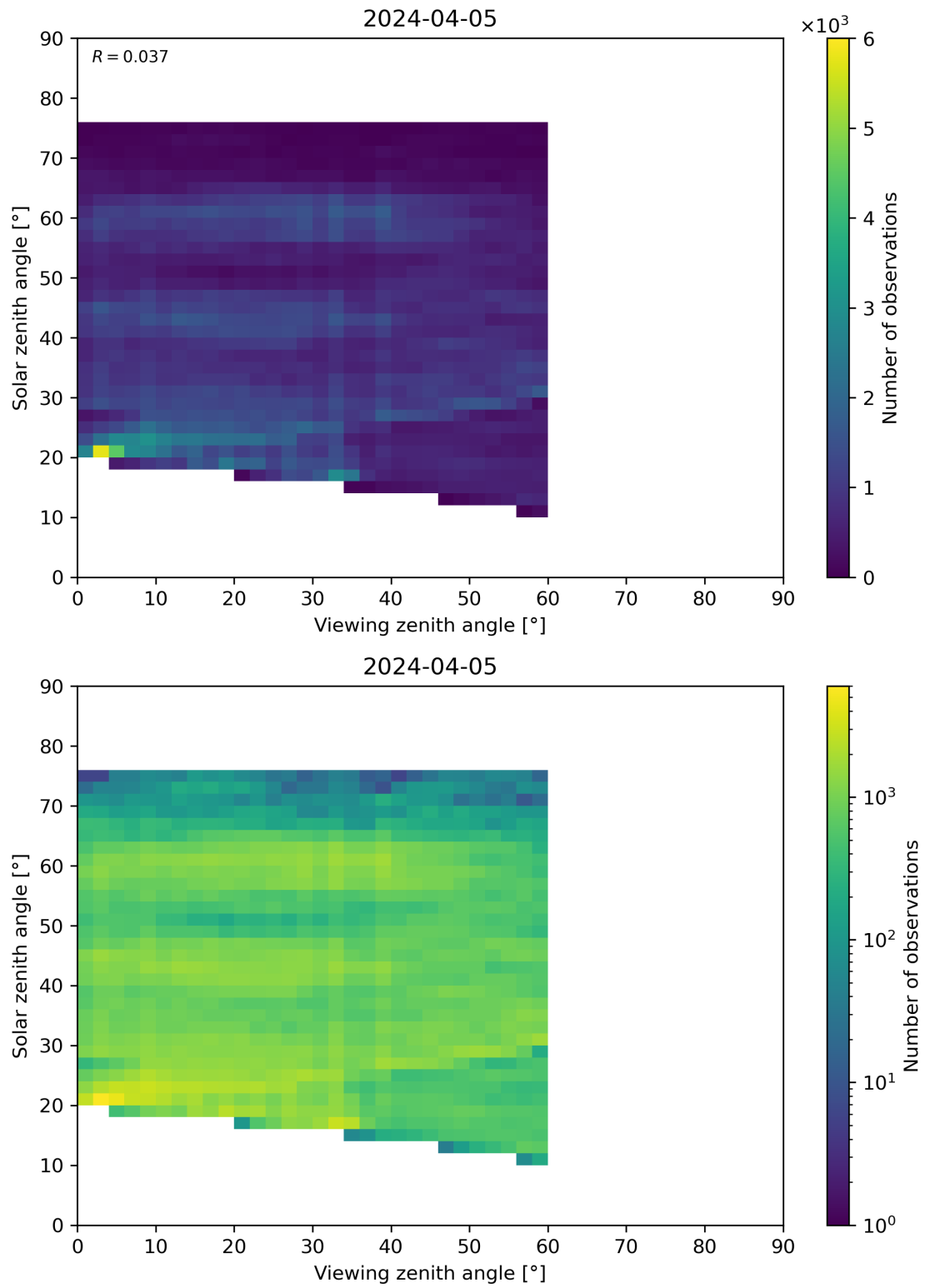
Figure 115: Scatter density plot of “Viewing zenith angle” against “Solar zenith angle” for 2024-04-05 to 2024-04-06.
