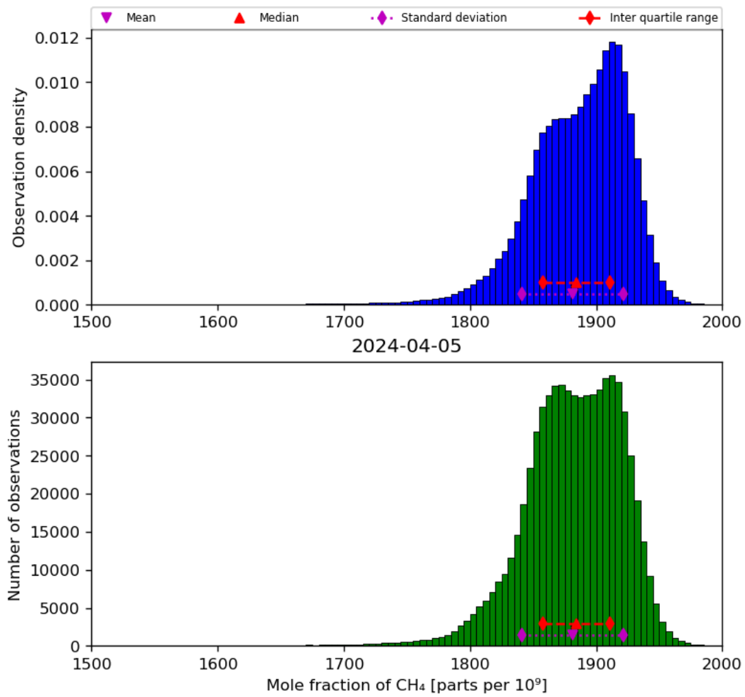
Figure 23: Histogram of “Mole fraction of CH 4 ” for 2024-04-05 to 2024-04-06
