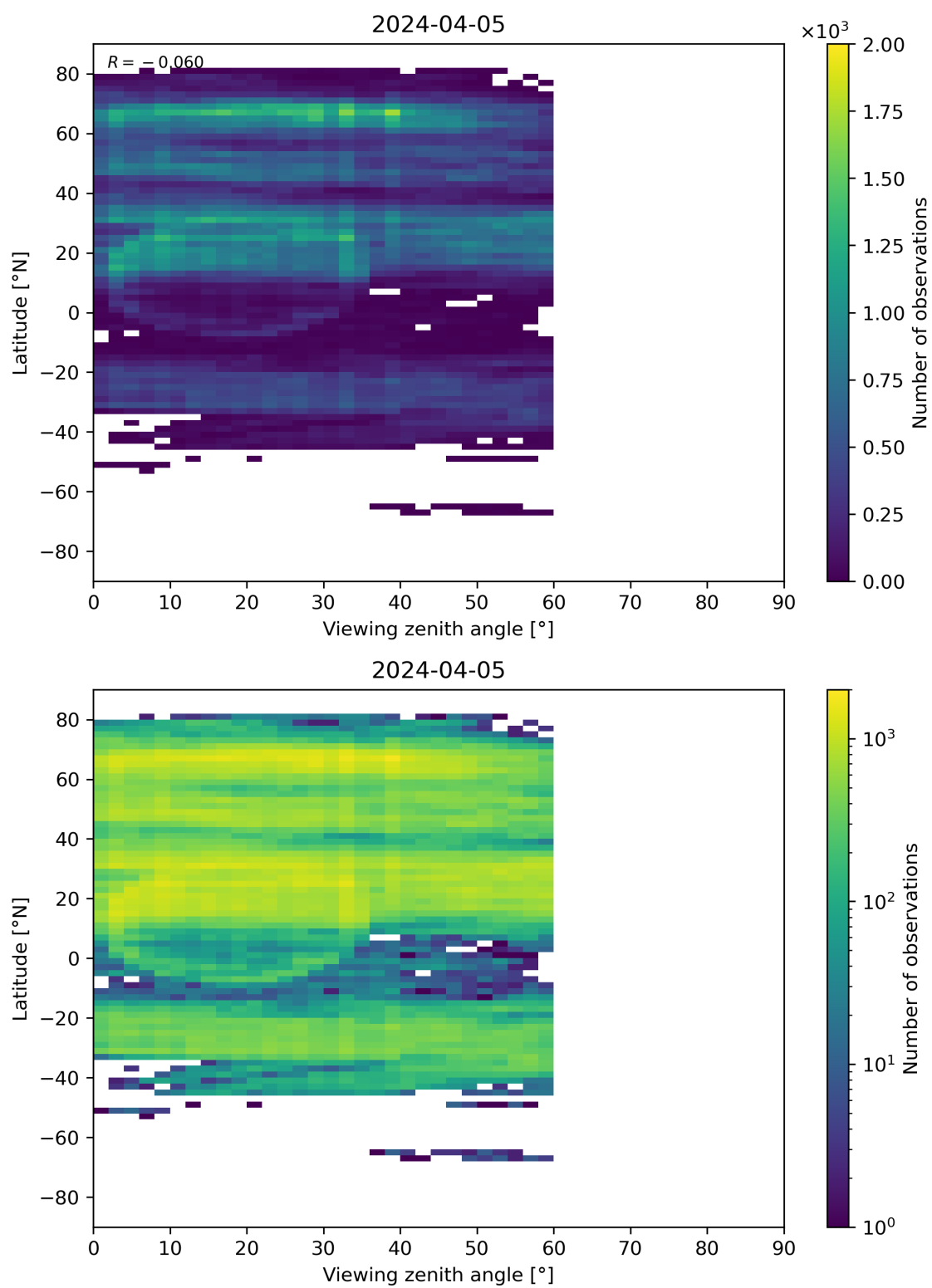
Figure 109: Scatter density plot of “Viewing zenith angle” against “Latitude” for 2024-04-05 to 2024-04-06.
