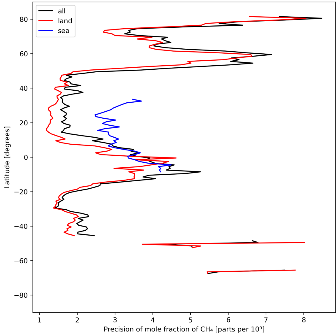
Figure 13: Zonal average of “Precision of mole fraction of CH 4 ” for 2024-04-05 to 2024-04-06.
