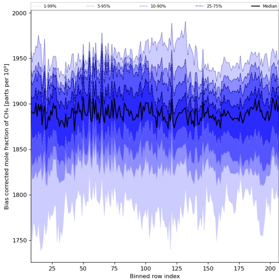
Figure 36: Along track statistics of “Bias corrected mole fraction of CH 4 ” for 2024-04-05 to 2024-04-06
