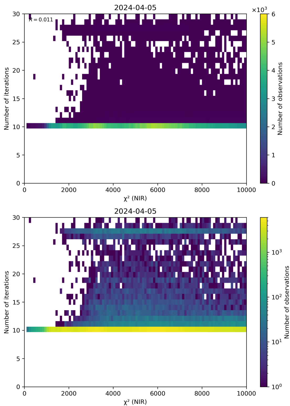
Figure 46: Scatter density plot of “ \chi^2 (NIR)” against “Number of iterations” for 2024-04-05 to 2024-04-06.
