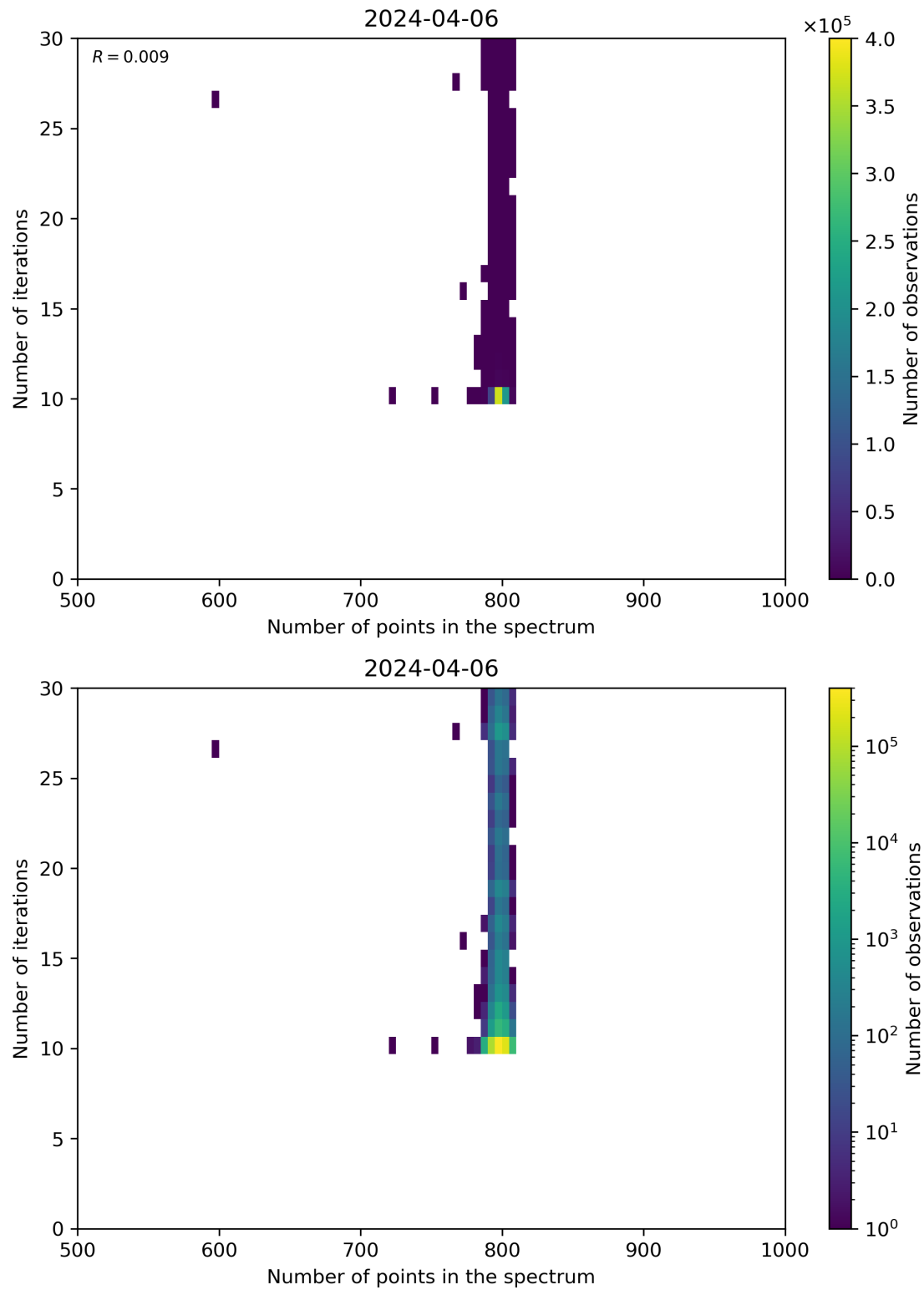
Figure 92: Scatter density plot of “Number of points in the spectrum” against “Number of iterations” for 2024-04-05 to 2024-04-07.
