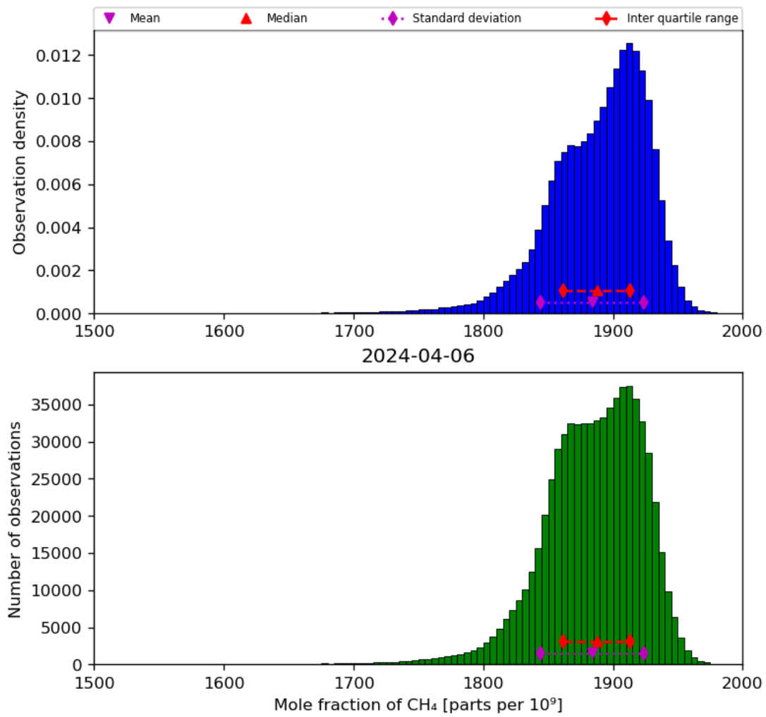
Figure 23: Histogram of “Mole fraction of CH 4 ” for 2024-04-05 to 2024-04-07
