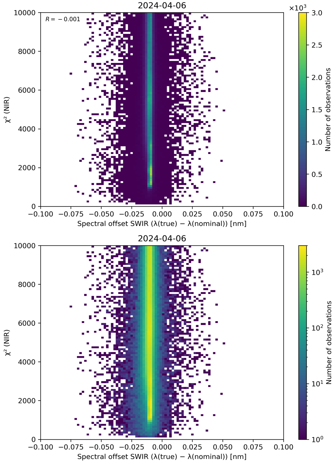
Figure 117: Scatter density plot of “Spectral offset SWIR ( \lambda(\text{true}) - \lambda(\text{nominal}) )” against “ \chi^2 (NIR)” for 2024-04-05 to 2024-04-07.
