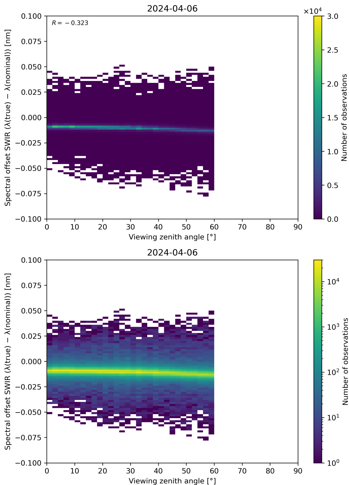
Figure 116: Scatter density plot of “Viewing zenith angle” against “Spectral offset SWIR ( \lambda(\text{true}) - \lambda(\text{nominal}) )” for 2024-04-05 to 2024-04-07.
