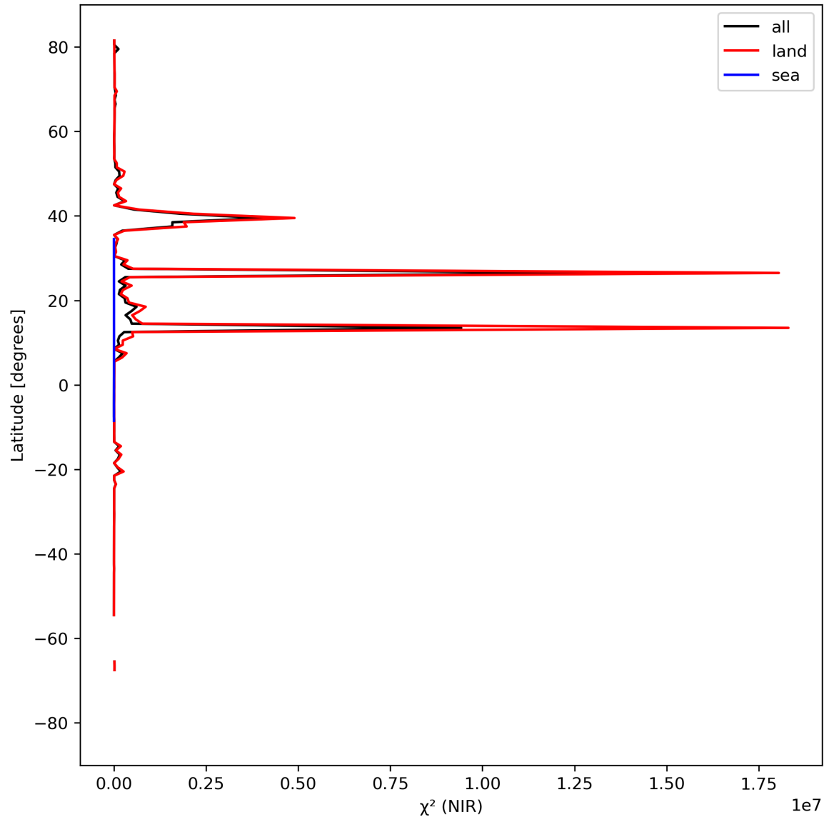
Figure 18: Zonal average of “ \chi^2 (NIR)” for 2024-04-05 to 2024-04-07.
