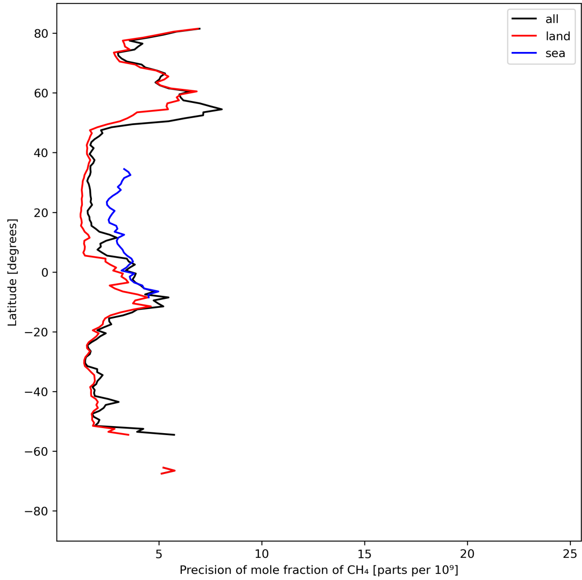
Figure 13: Zonal average of “Precision of mole fraction of CH 4 ” for 2024-04-05 to 2024-04-07.
