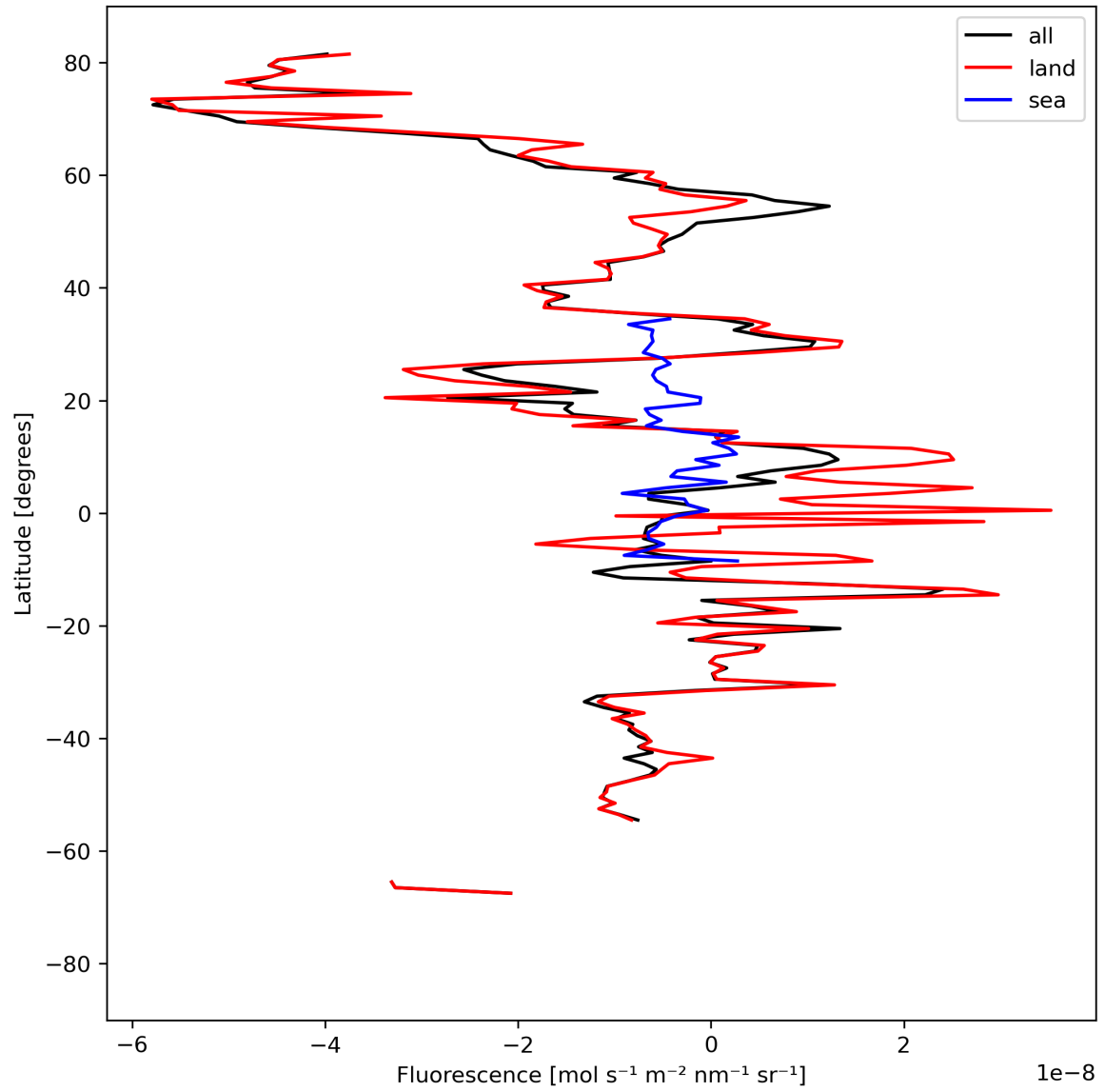
Figure 21: Zonal average of “Fluorescence” for 2024-04-05 to 2024-04-07.
