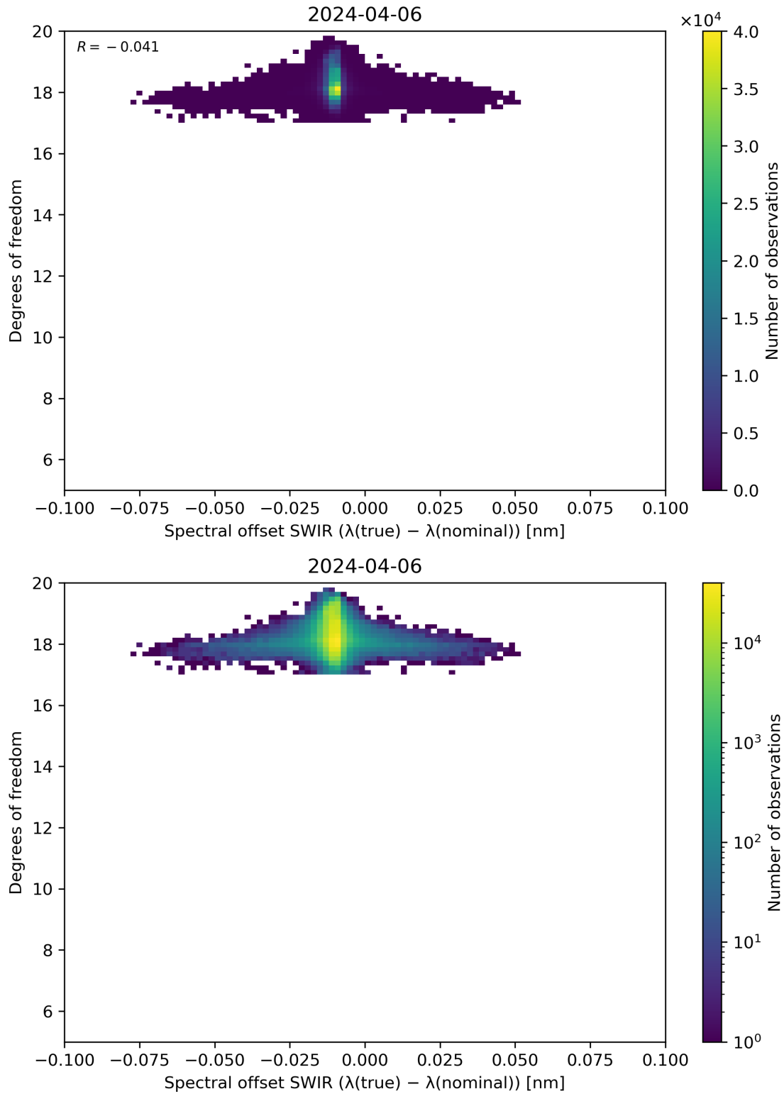
Figure 119: Scatter density plot of “Spectral offset SWIR ( \lambda(\text{true}) - \lambda(\text{nominal}) )” against “Degrees of freedom” for 2024-04-05 to 2024-04-07.
