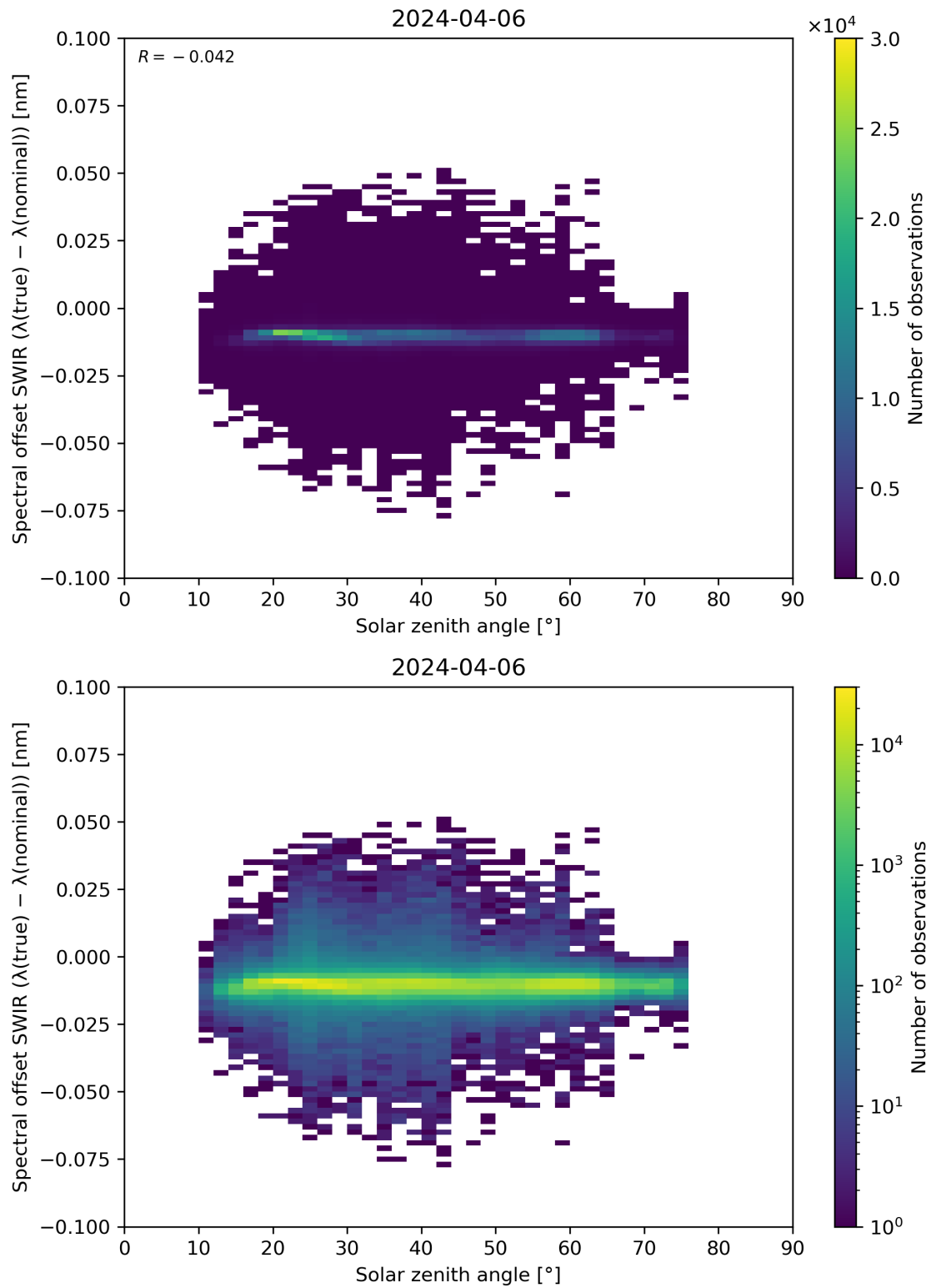
Figure 104: Scatter density plot of “Solar zenith angle” against “Spectral offset SWIR ( \lambda(\text{true}) - \lambda(\text{nominal}) )” for 2024-04-05 to 2024-04-07.
