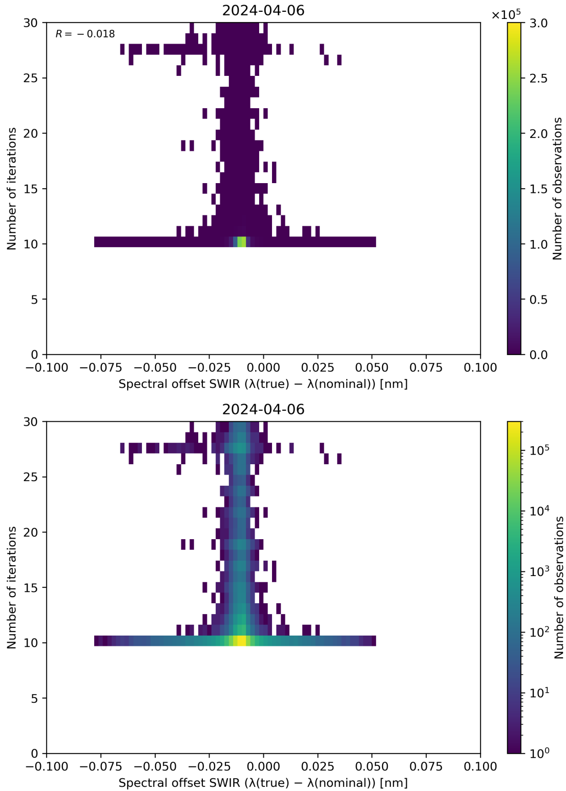
Figure 121: Scatter density plot of “Spectral offset SWIR ( \lambda(\text{true}) - \lambda(\text{nominal}) )” against “Number of iterations” for 2024-04-05 to 2024-04-07.
