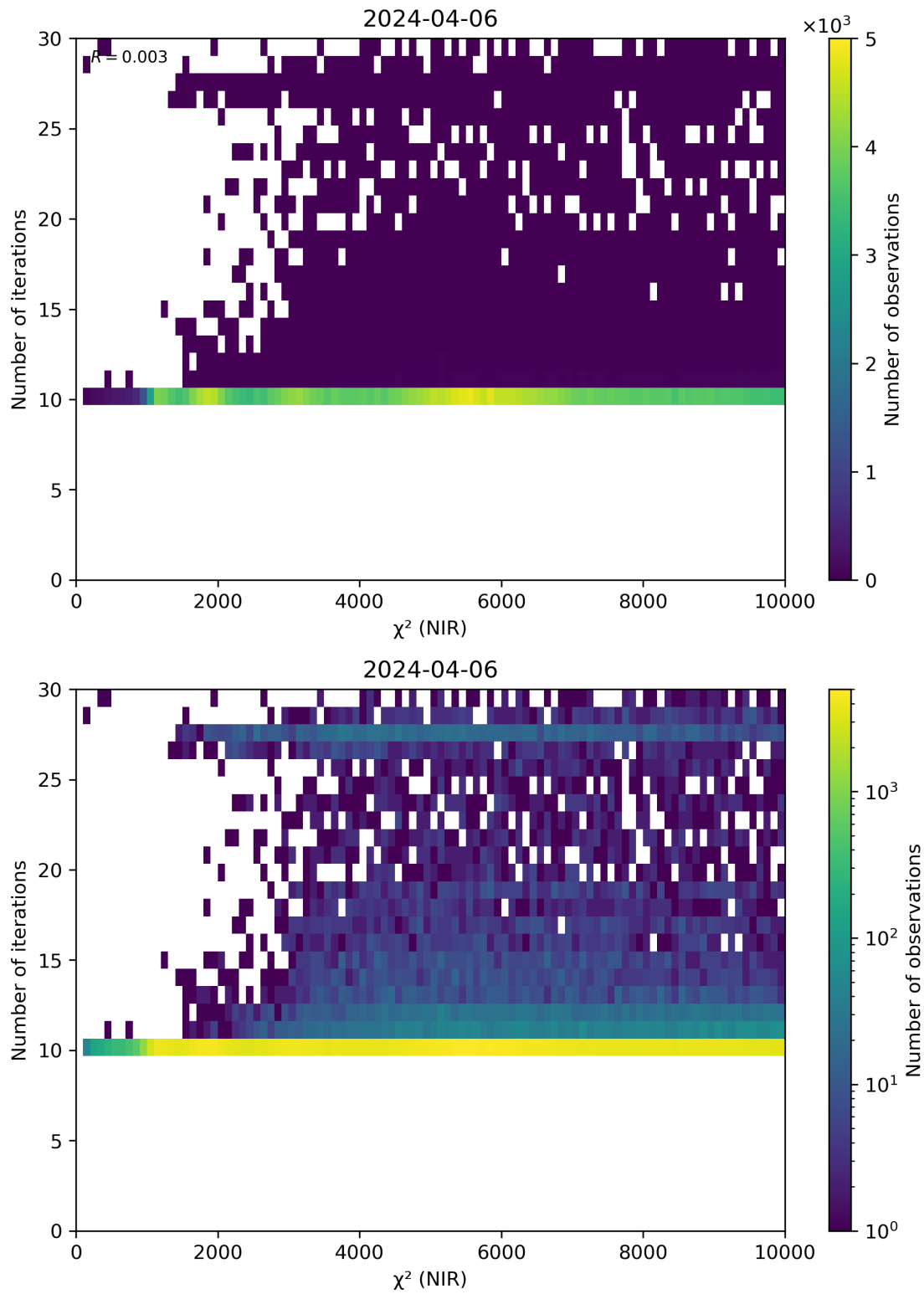
Figure 46: Scatter density plot of “ \chi^2 (NIR)” against “Number of iterations” for 2024-04-05 to 2024-04-07.
