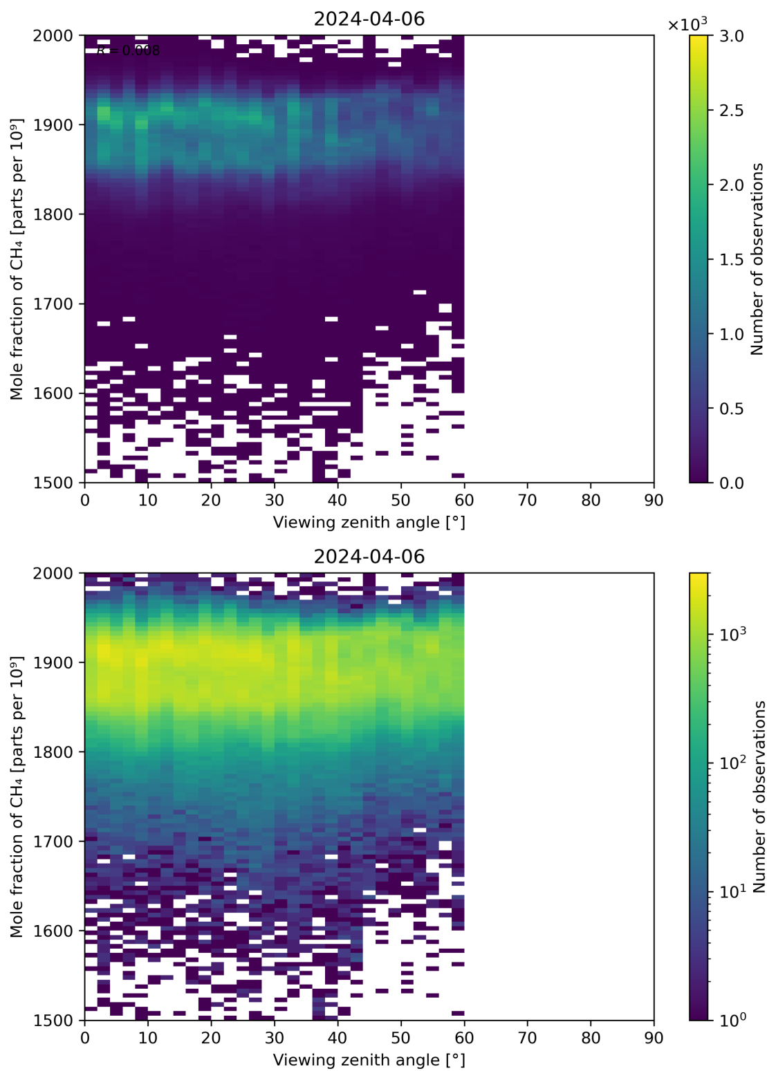
Figure 110: Scatter density plot of “Viewing zenith angle” against “Mole fraction of CH 4 ” for 2024-04-05 to 2024-04-07.
