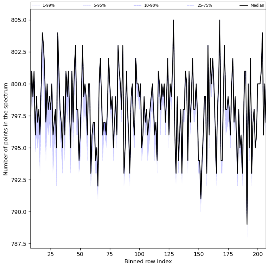
Figure 37: Along track statistics of “Number of points in the spectrum” for 2024-04-05 to 2024-04-07
