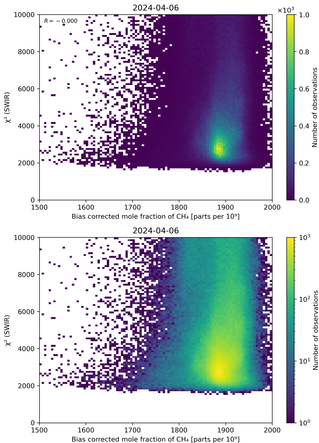
Figure 64: Scatter density plot of “Bias corrected mole fraction of CH 4 ” against “ \chi^2 (SWIR)” for 2024-04-05 to 2024-04-07.
