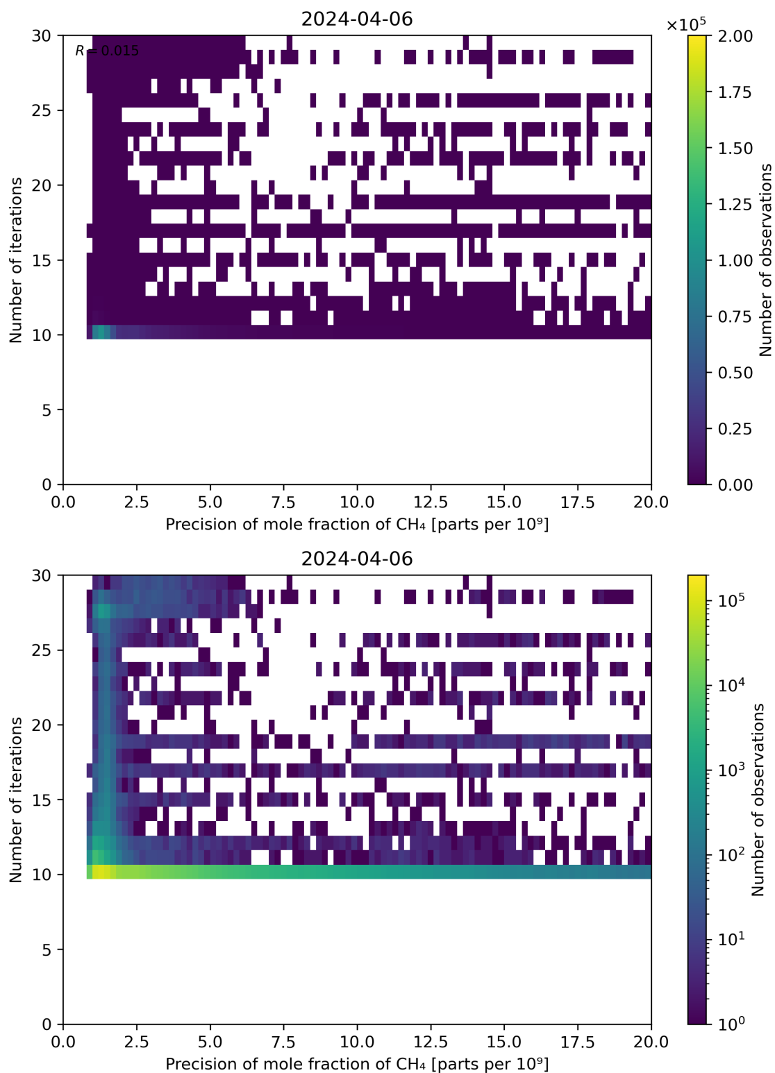
Figure 83: Scatter density plot of “Precision of mole fraction of CH 4 ” against “Number of iterations” for 2024-04-05 to 2024-04-07.
