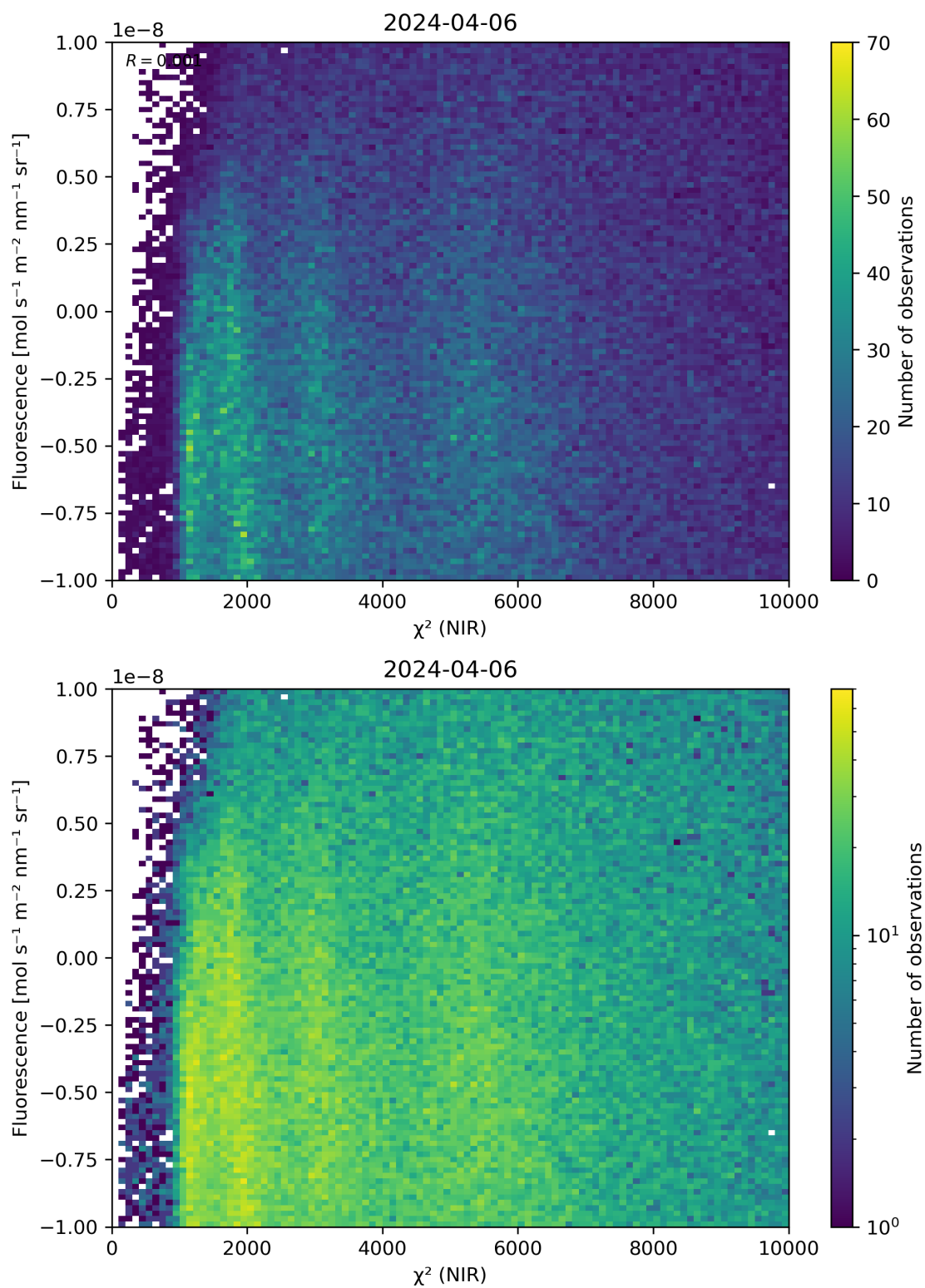
Figure 45: Scatter density plot of “ \chi^2 (NIR)” against “Fluorescence” for 2024-04-05 to 2024-04-07.
