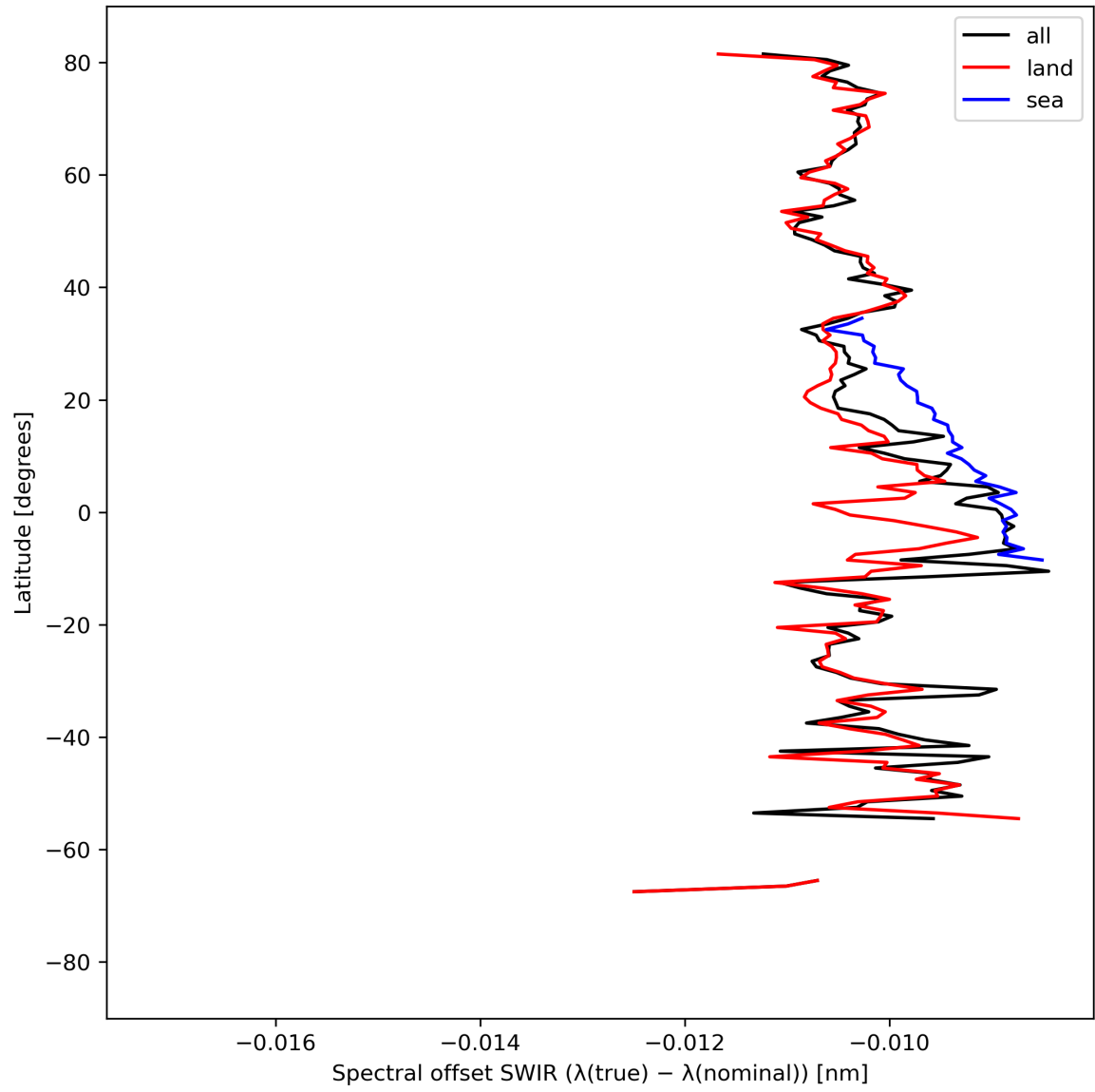
Figure 16: Zonal average of “Spectral offset SWIR ( \lambda(\text{true}) - \lambda(\text{nominal}) )” for 2024-04-05 to 2024-04-07.
