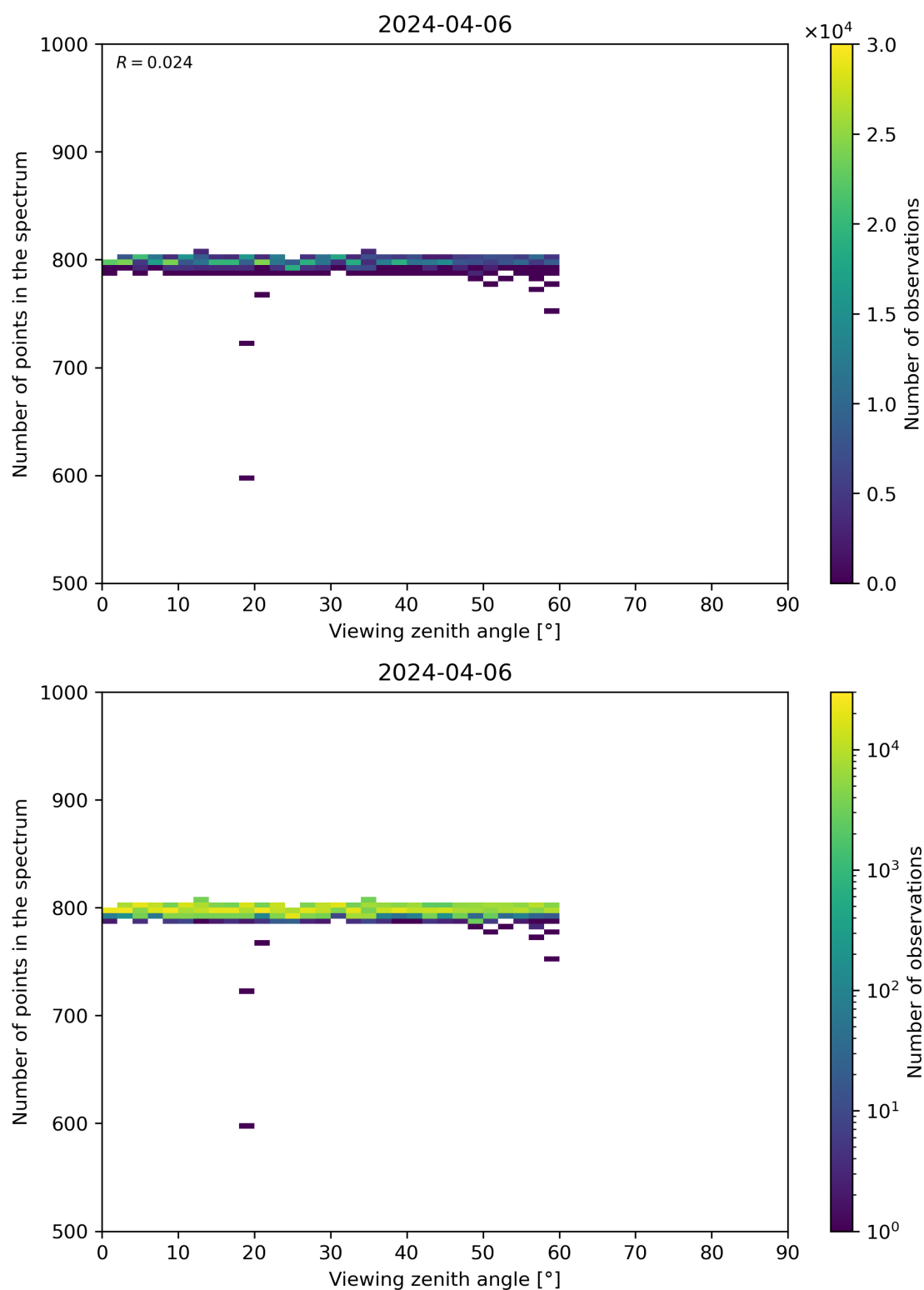
Figure 114: Scatter density plot of “Viewing zenith angle” against “Number of points in the spectrum” for 2024-04-05 to 2024-04-07.
