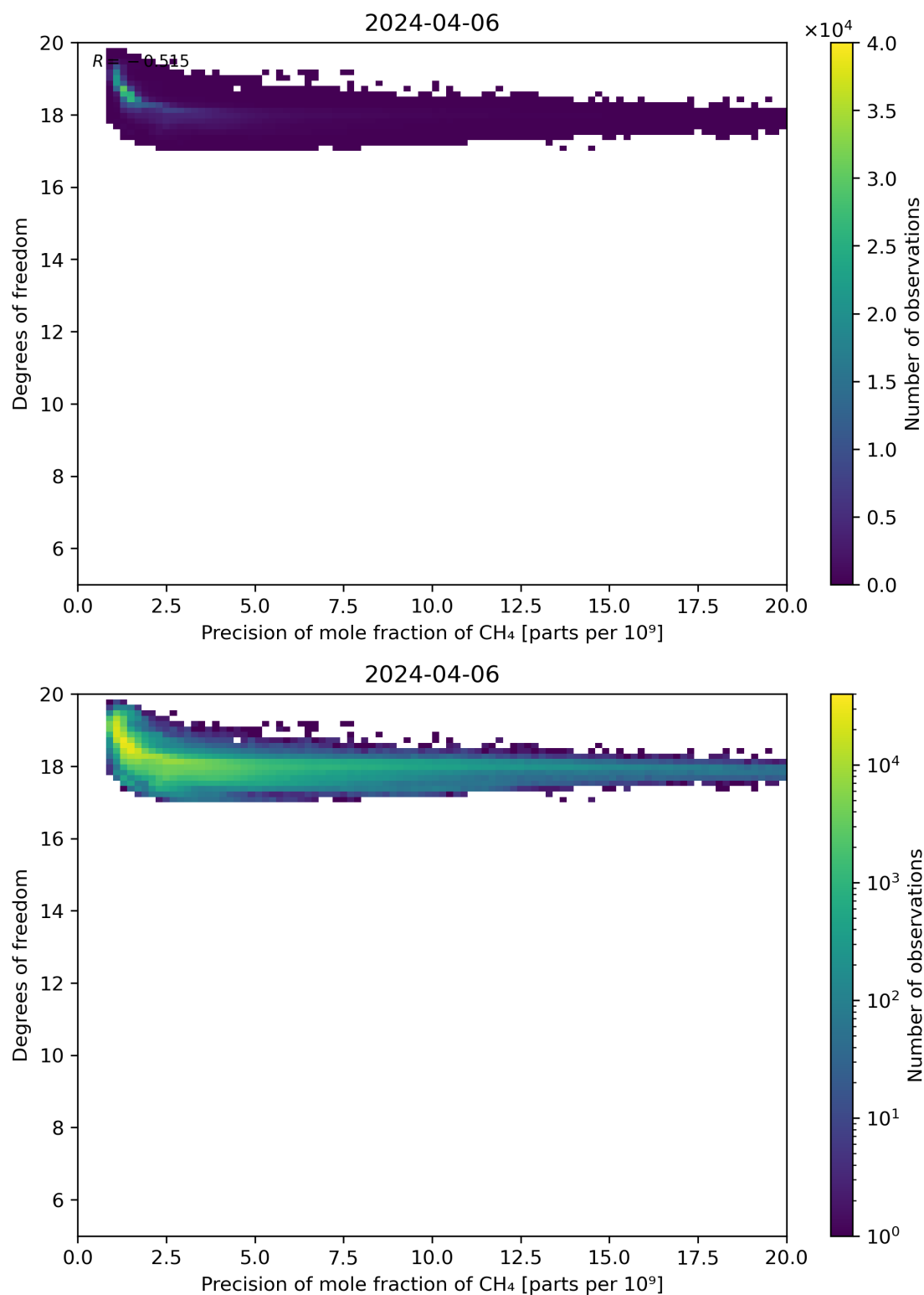
Figure 80: Scatter density plot of “Precision of mole fraction of \text{CH}_4 ” against “Degrees of freedom” for 2024-04-05 to 2024-04-07.
