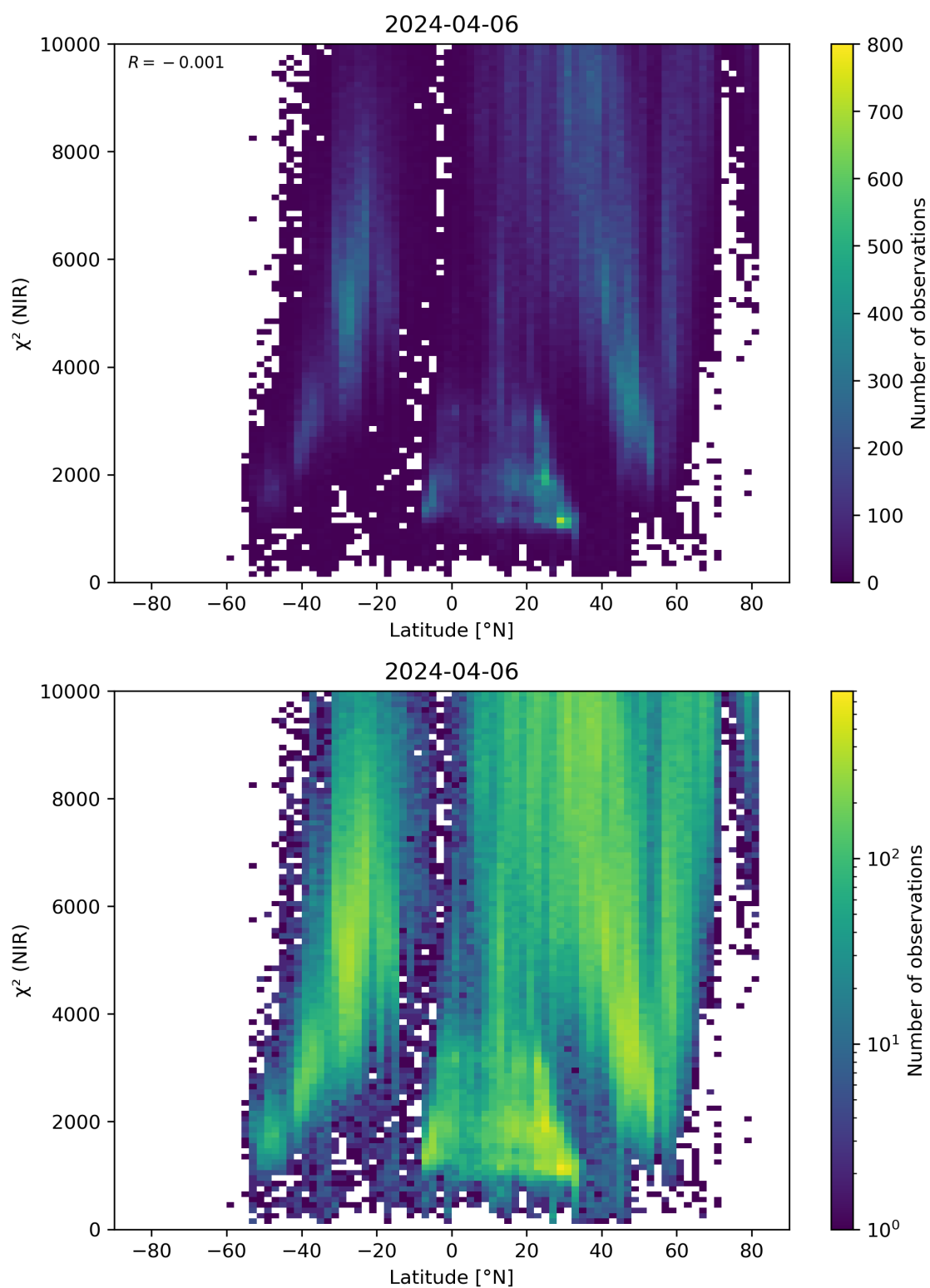
Figure 53: Scatter density plot of “Latitude” against “ \chi^2 (NIR)” for 2024-04-05 to 2024-04-07.
