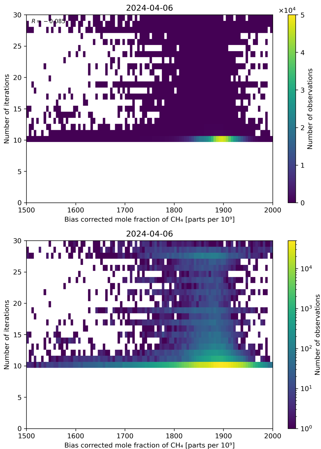
Figure 67: Scatter density plot of “Bias corrected mole fraction of \text{CH}_4 ” against “Number of iterations” for 2024-04-05 to 2024-04-07.
