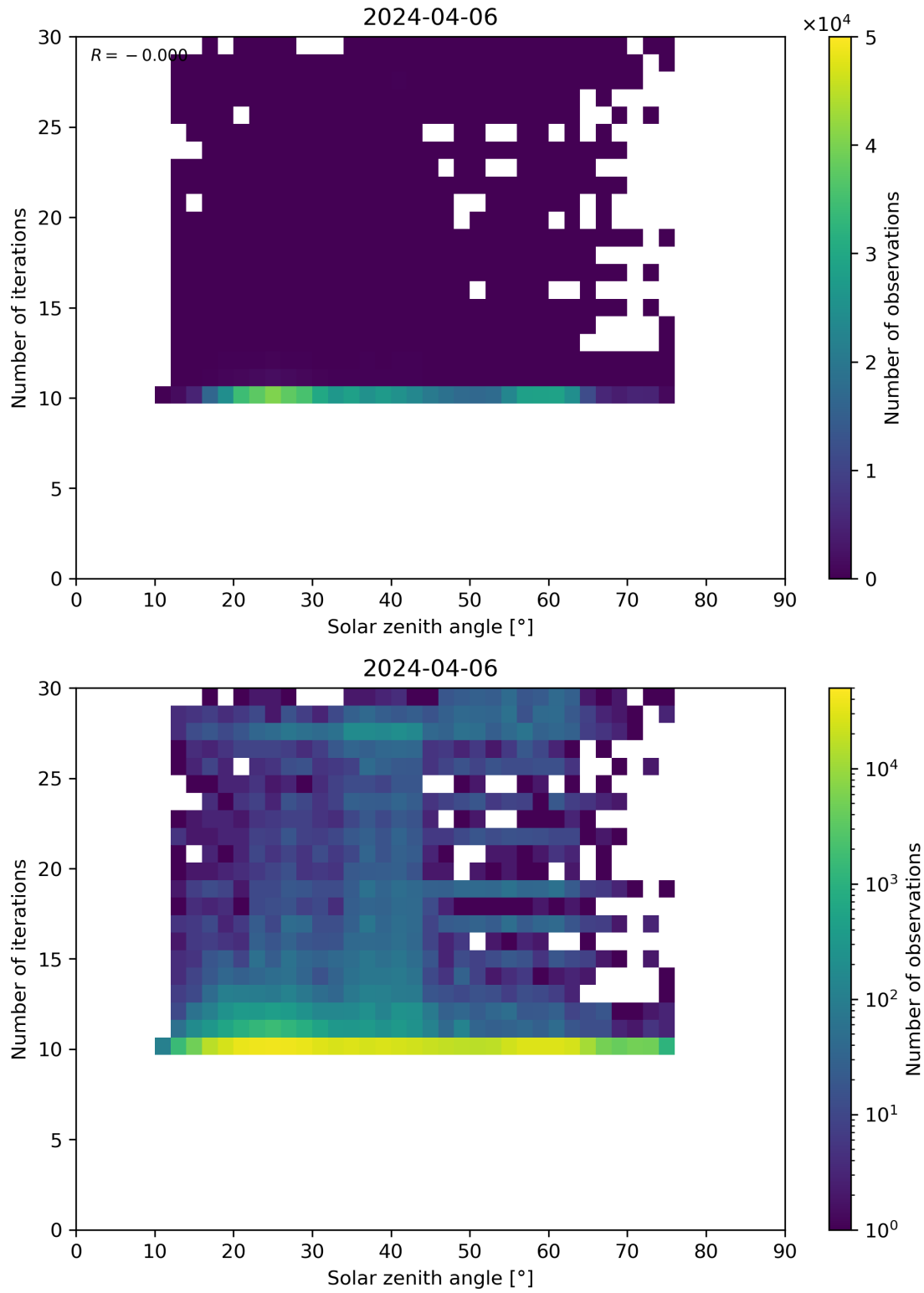
Figure 102: Scatter density plot of “Solar zenith angle” against “Number of iterations” for 2024-04-05 to 2024-04-07.
