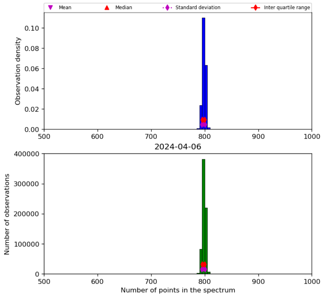
Figure 26: Histogram of “Number of points in the spectrum” for 2024-04-05 to 2024-04-07
