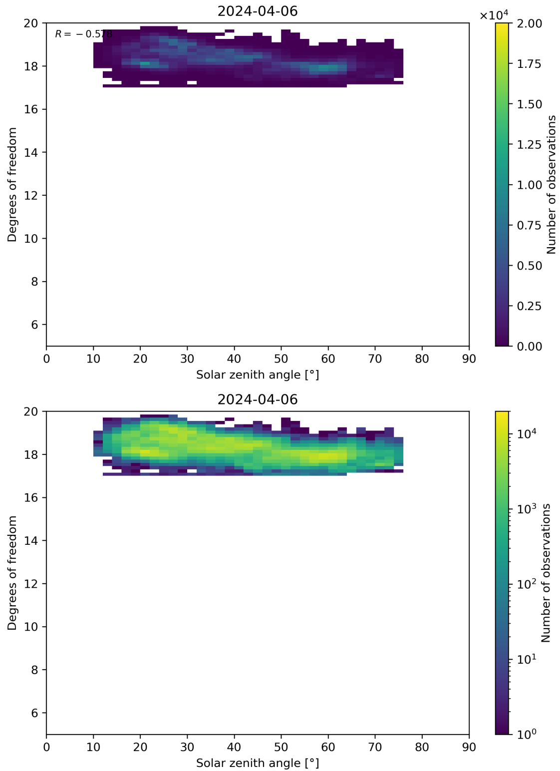
Figure 96: Scatter density plot of “Solar zenith angle” against “Degrees of freedom” for 2024-04-05 to 2024-04-07.
