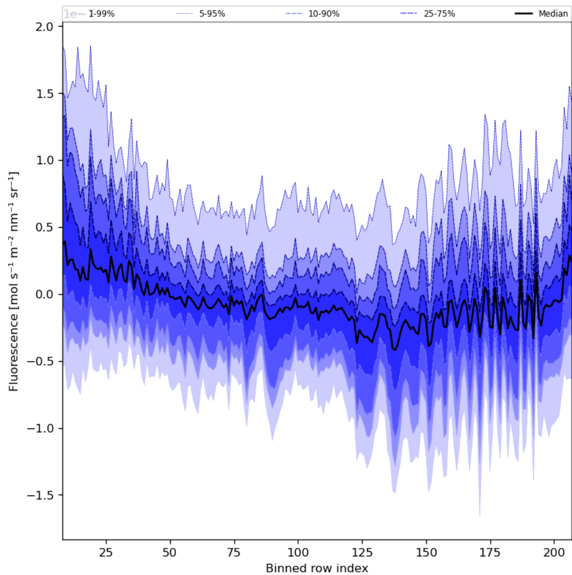
Figure 43: Along track statistics of “Fluorescence” for 2024-04-05 to 2024-04-07
