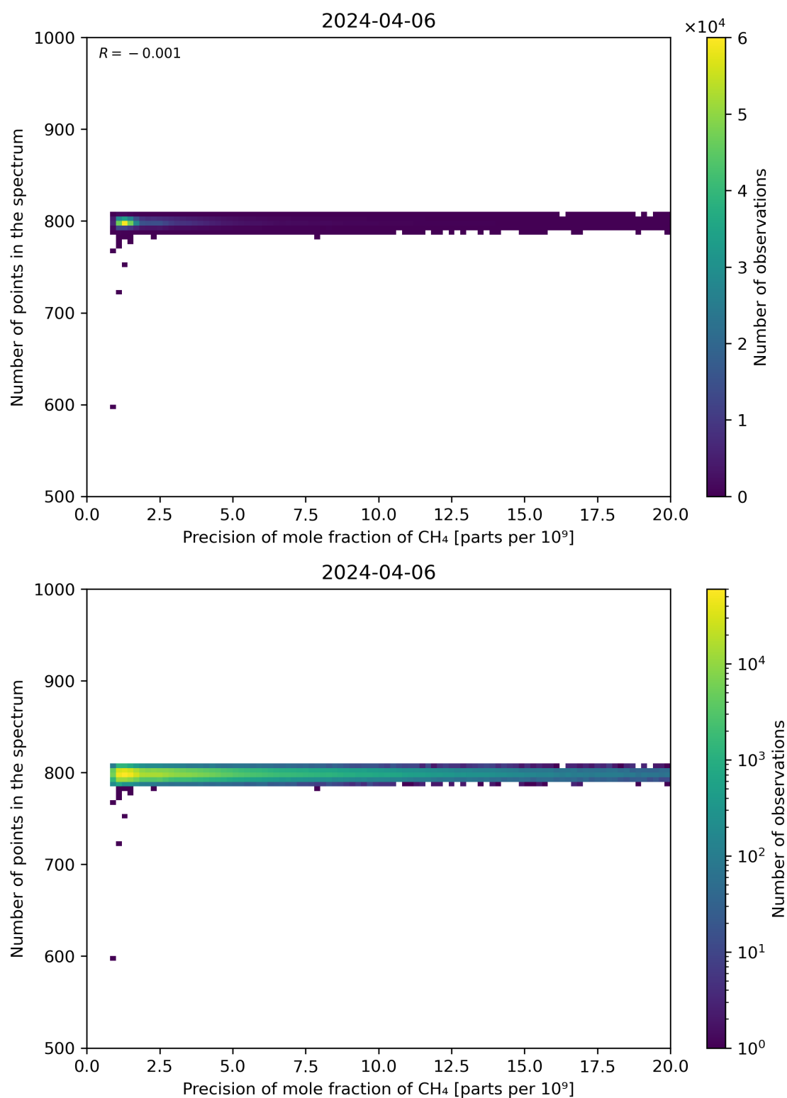
Figure 84: Scatter density plot of “Precision of mole fraction of CH 4 ” against “Number of points in the spectrum” for 2024-04-05 to 2024-04-07.
