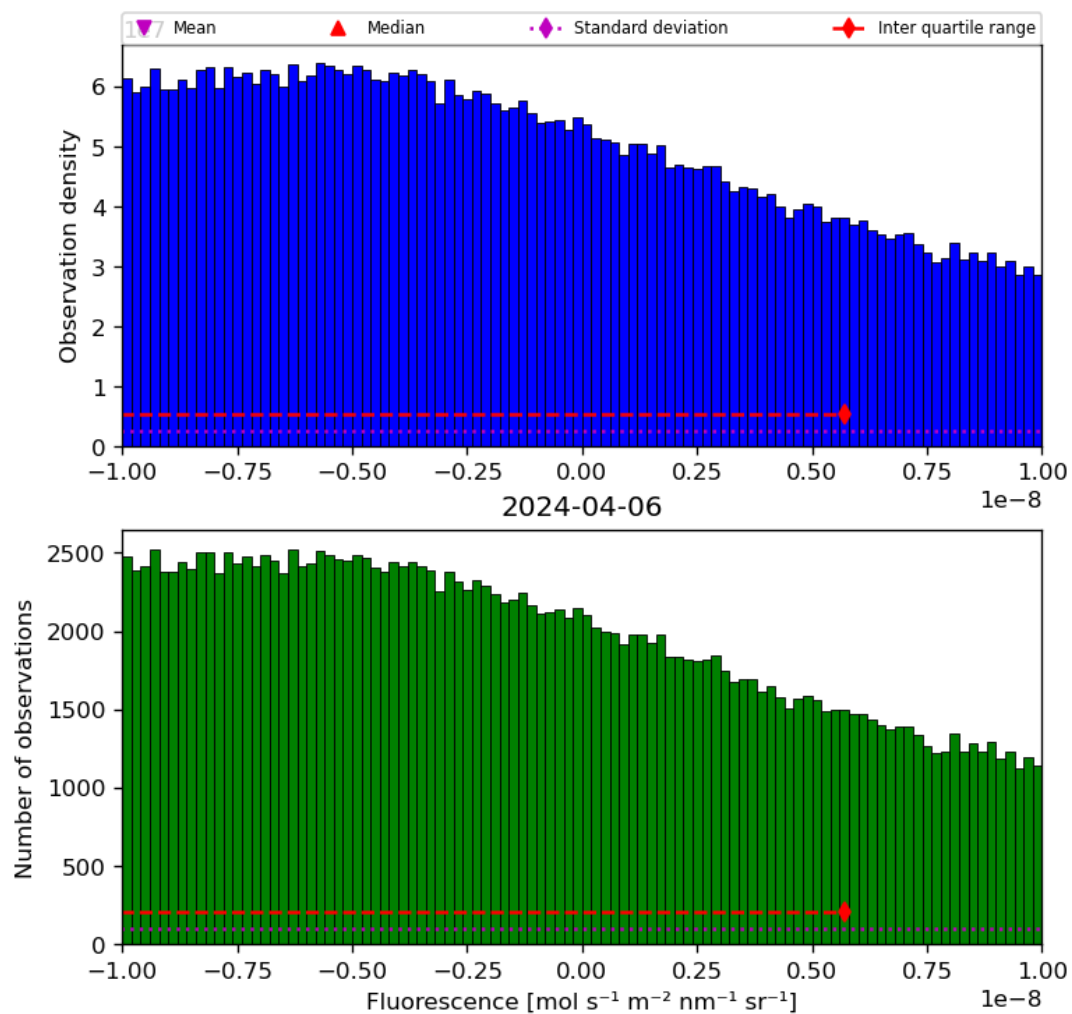
Figure 32: Histogram of “Fluorescence” for 2024-04-05 to 2024-04-07
