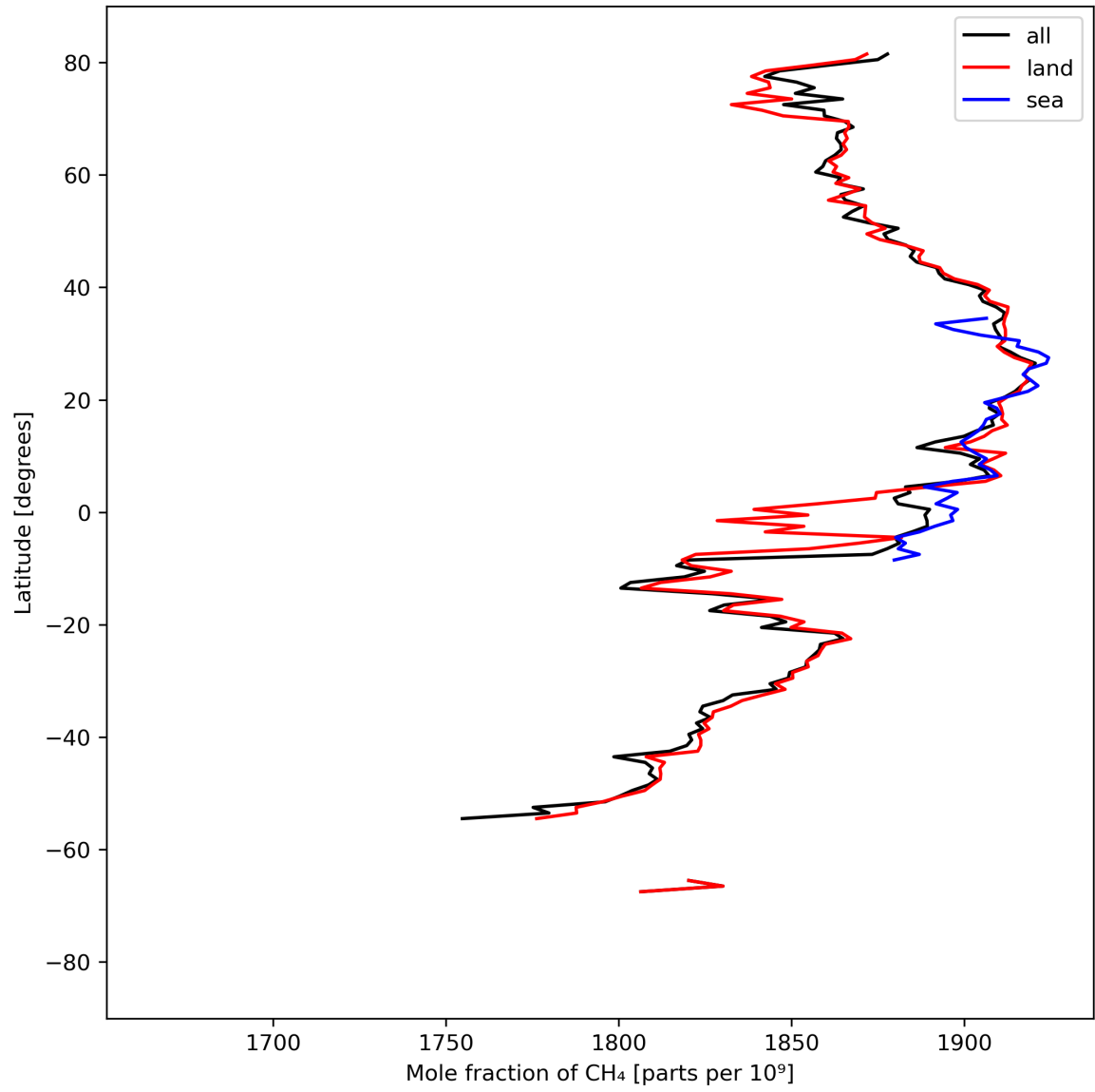
Figure 12: Zonal average of “Mole fraction of \text{CH}_4 ” for 2024-04-05 to 2024-04-07.
