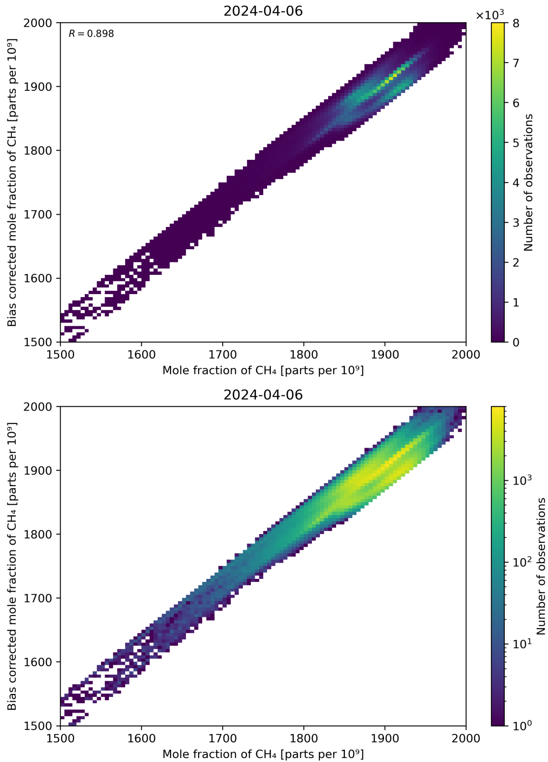
Figure 74: Scatter density plot of “Mole fraction of CH 4 ” against “Bias corrected mole fraction of CH 4 ” for 2024-04-05 to 2024-04-07.
