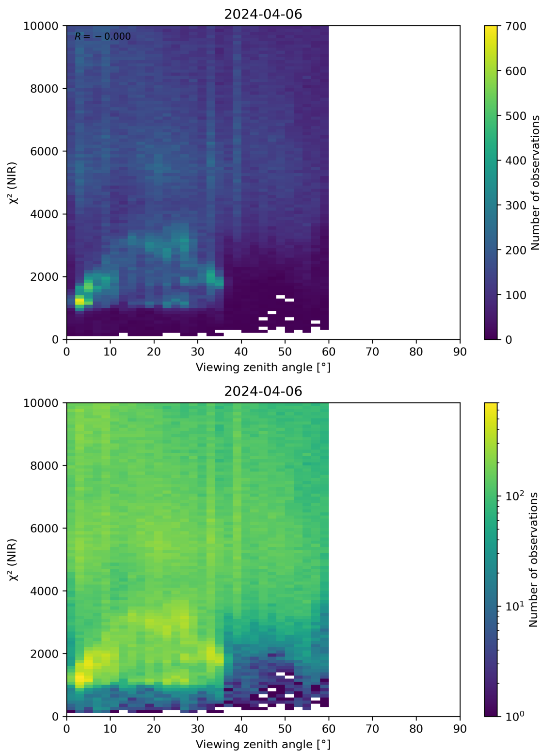
Figure 105: Scatter density plot of “Viewing zenith angle” against “ \chi^2 (NIR)” for 2024-04-05 to 2024-04-07.
