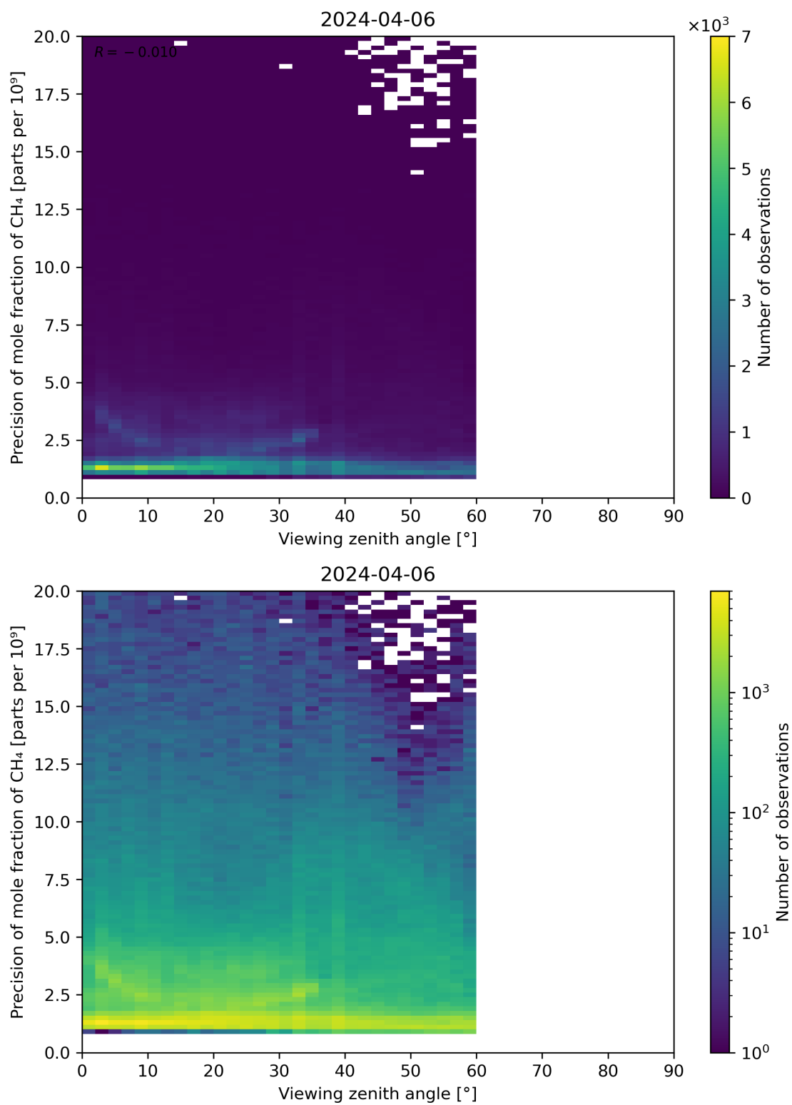
Figure 112: Scatter density plot of “Viewing zenith angle” against “Precision of mole fraction of CH 4 ” for 2024-04-05 to 2024-04-07.
