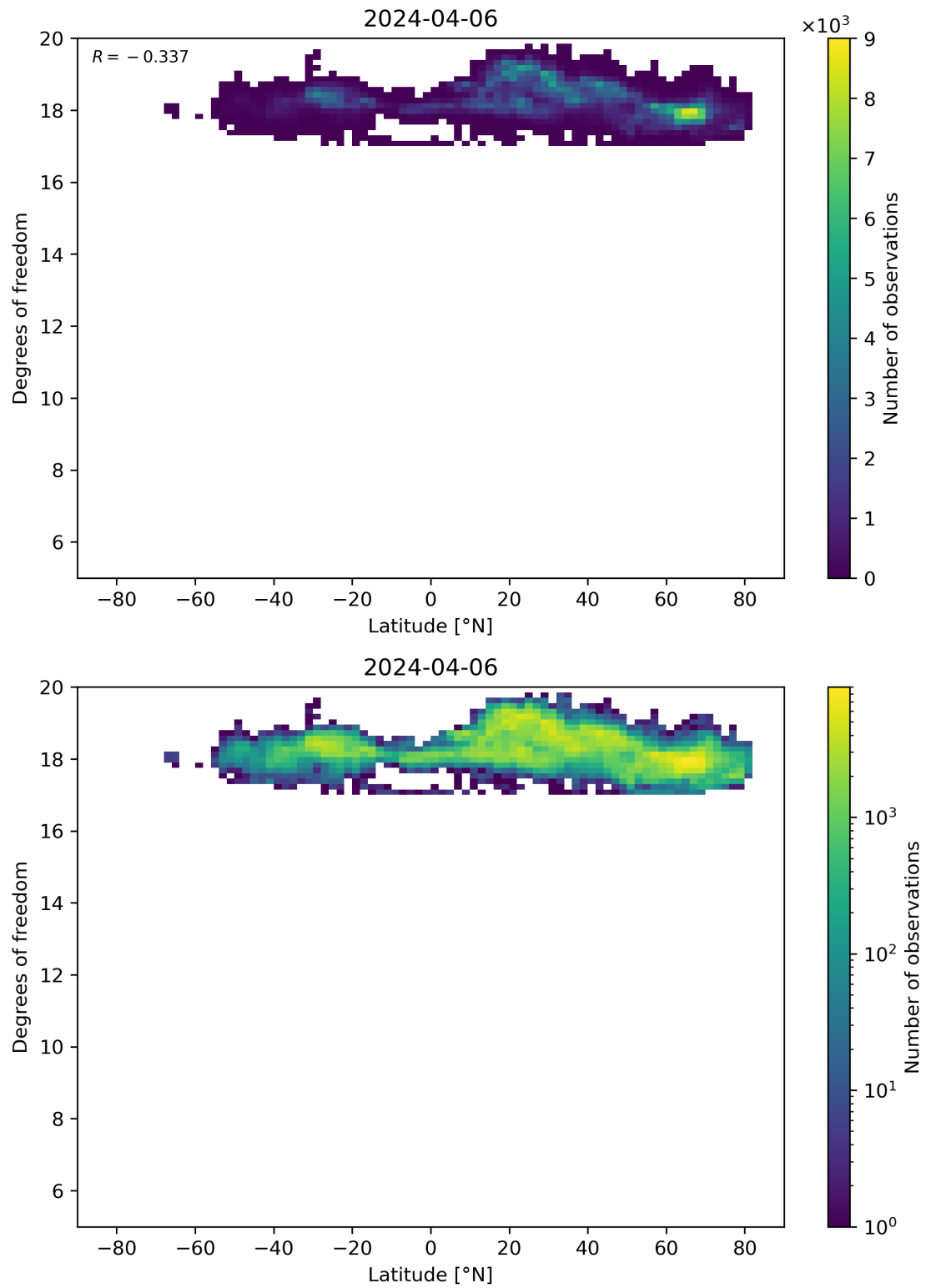
Figure 55: Scatter density plot of “Latitude” against “Degrees of freedom” for 2024-04-05 to 2024-04-07.
