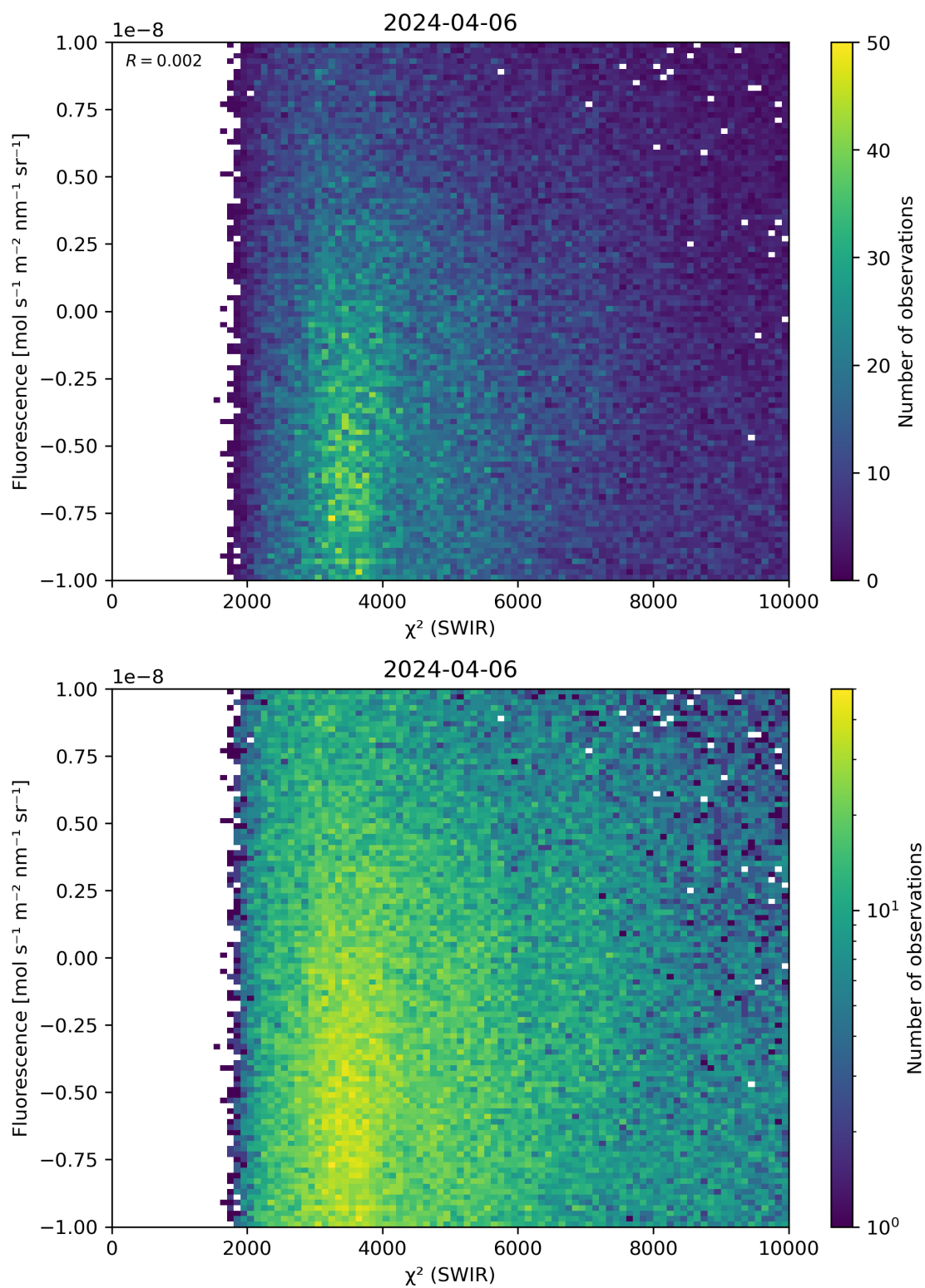
Figure 49: Scatter density plot of “ \chi^2 (SWIR)” against “Fluorescence” for 2024-04-05 to 2024-04-07.
