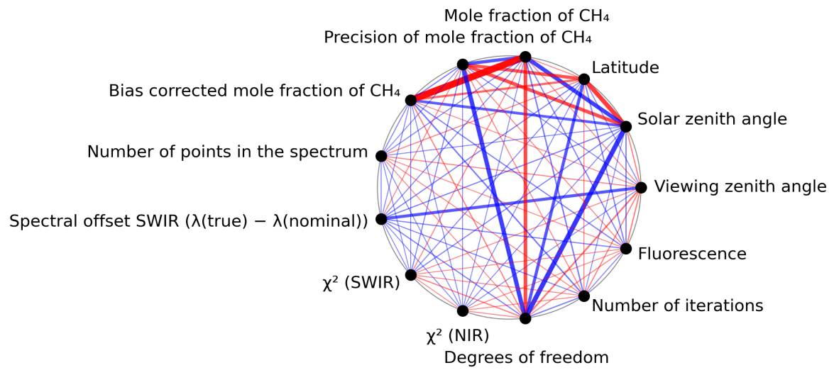
Figure 1: Map of correlation graph for 2024-04-05 to 2024-04-07.
