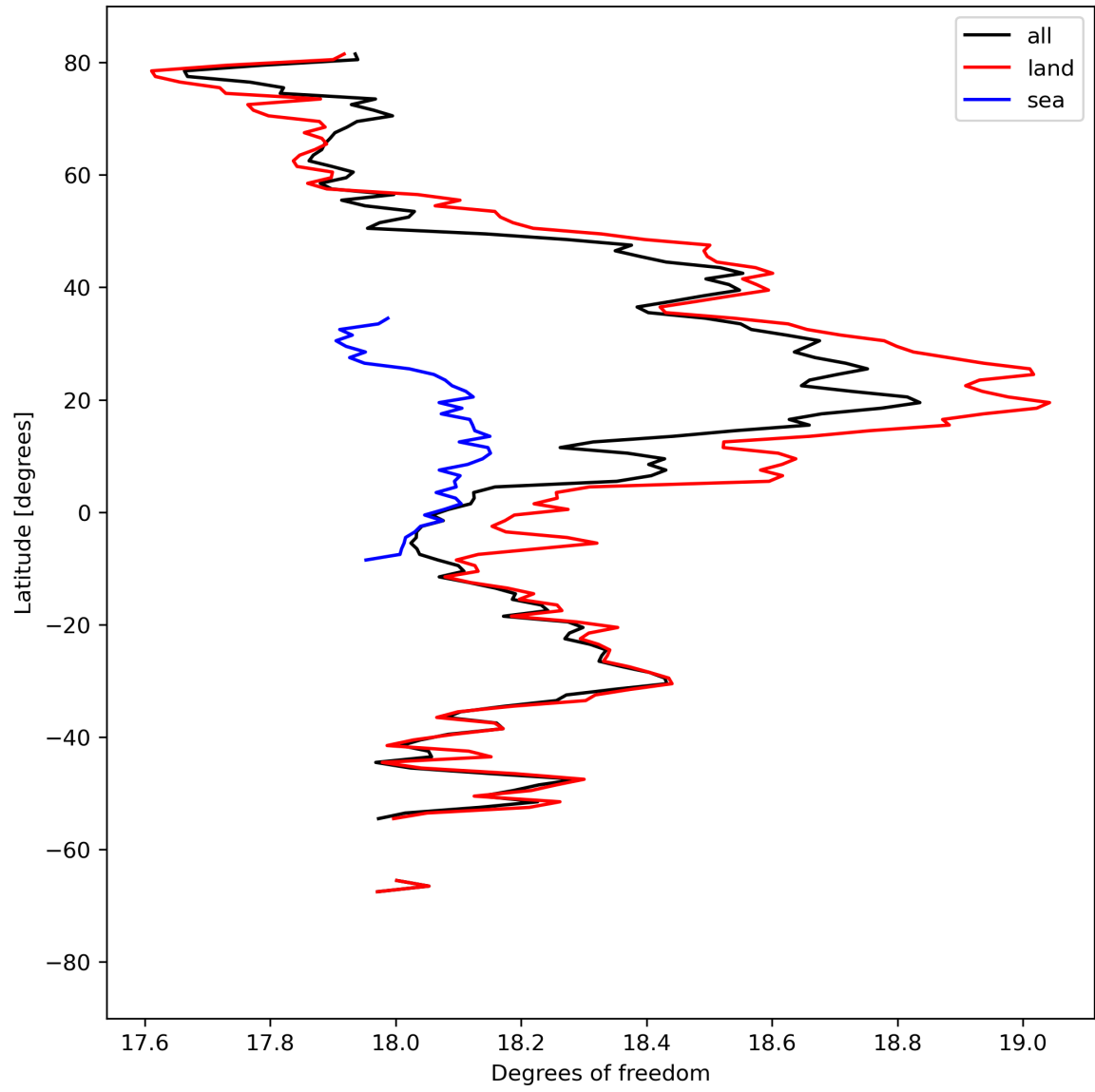
Figure 19: Zonal average of “Degrees of freedom” for 2024-04-05 to 2024-04-07.
