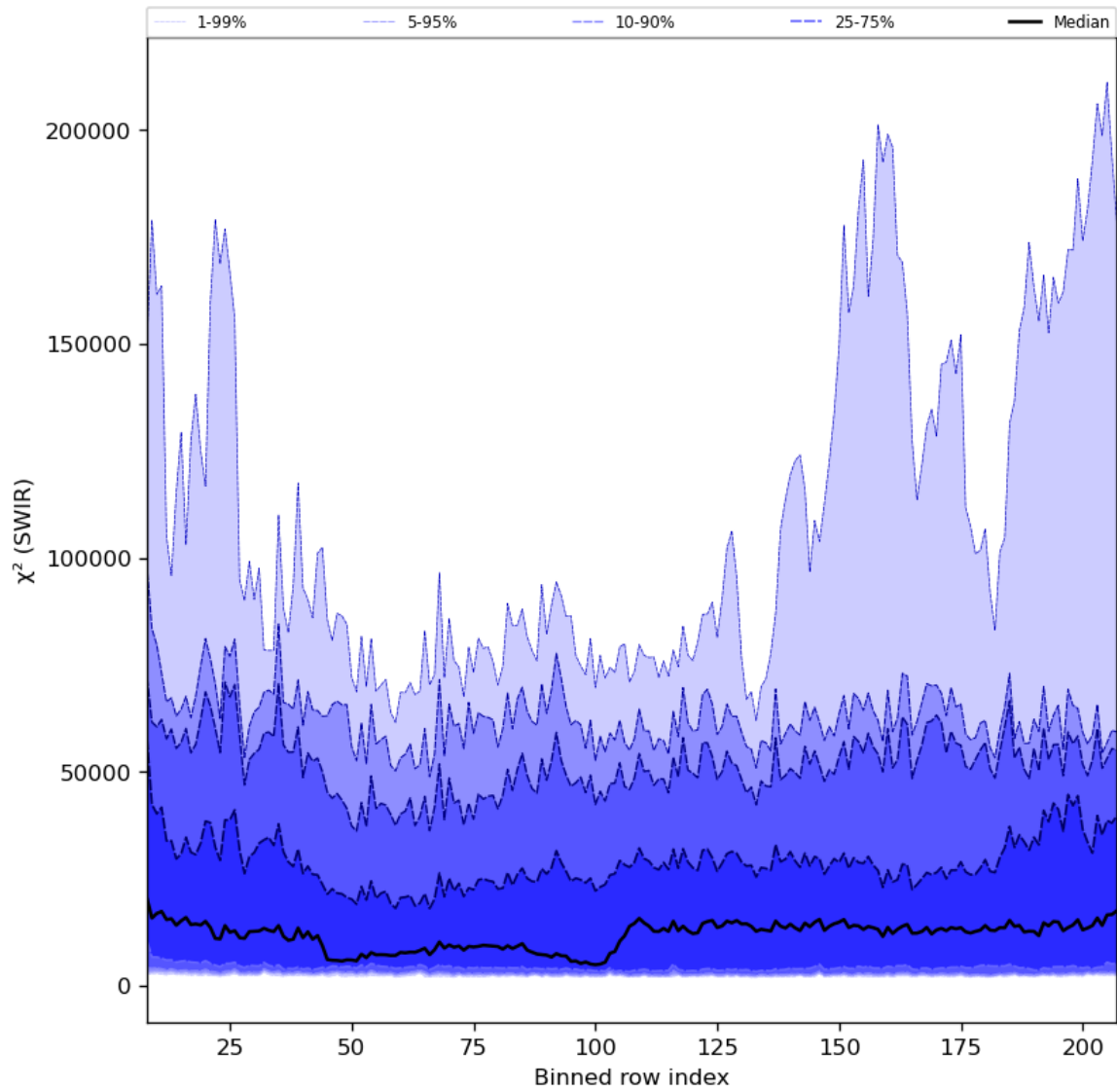
Figure 39: Along track statistics of “ \chi^2 (SWIR)” for 2024-04-05 to 2024-04-07
