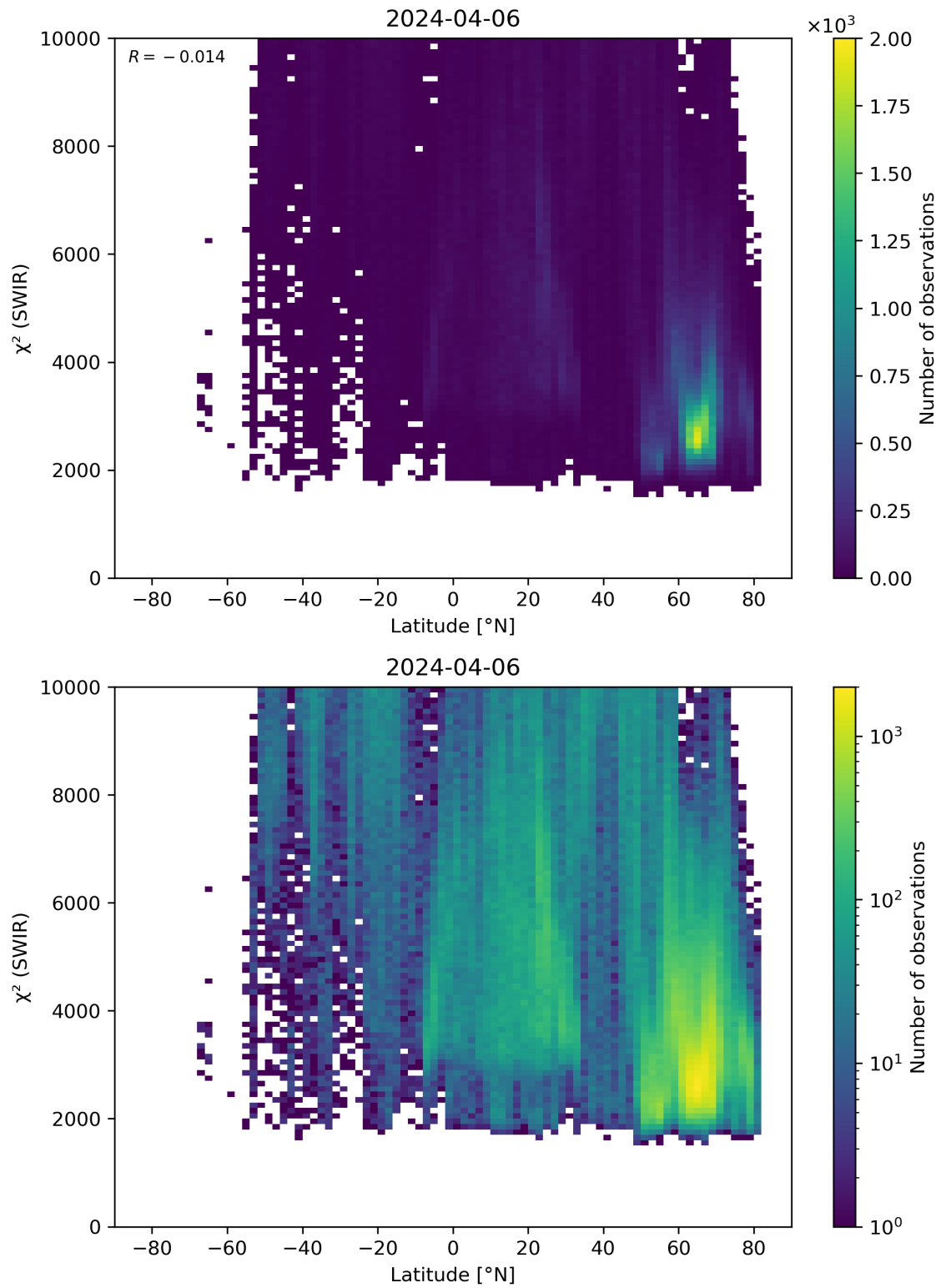
Figure 54: Scatter density plot of “Latitude” against “ \chi^2 (SWIR)” for 2024-04-05 to 2024-04-07.
