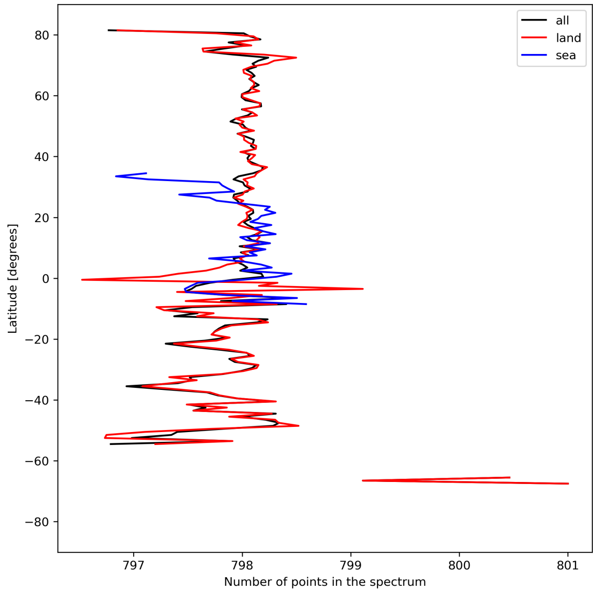
Figure 15: Zonal average of “Number of points in the spectrum” for 2024-04-05 to 2024-04-07.
