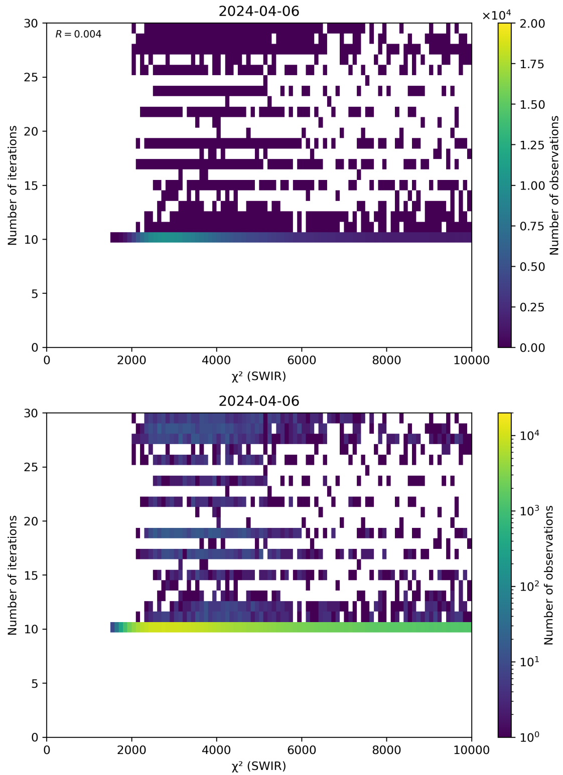
Figure 50: Scatter density plot of “ \chi^2 (SWIR)” against “Number of iterations” for 2024-04-05 to 2024-04-07.
