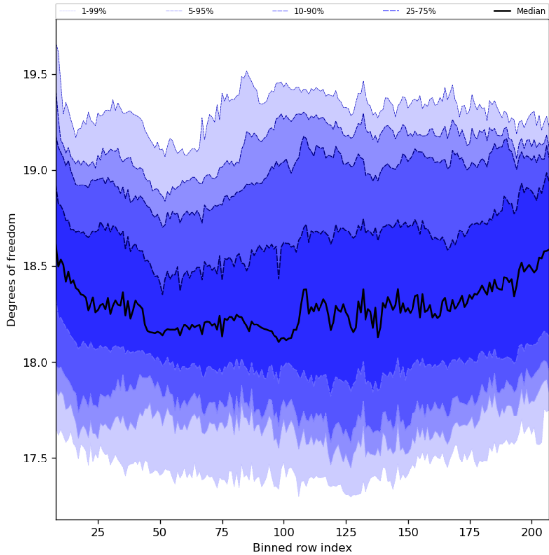
Figure 41: Along track statistics of “Degrees of freedom” for 2024-04-05 to 2024-04-07
