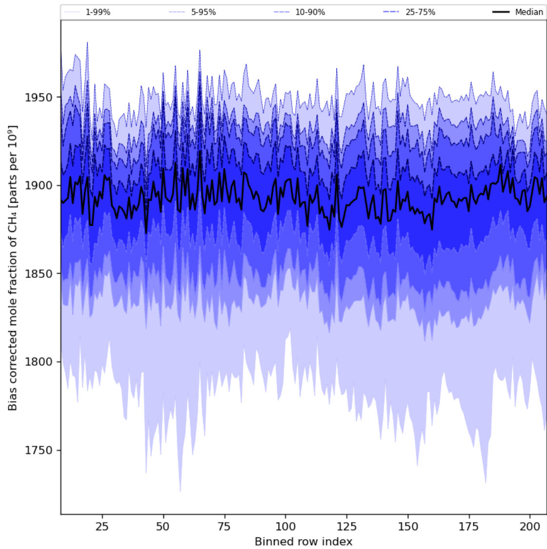
Figure 36: Along track statistics of “Bias corrected mole fraction of CH 4 ” for 2024-04-05 to 2024-04-07
