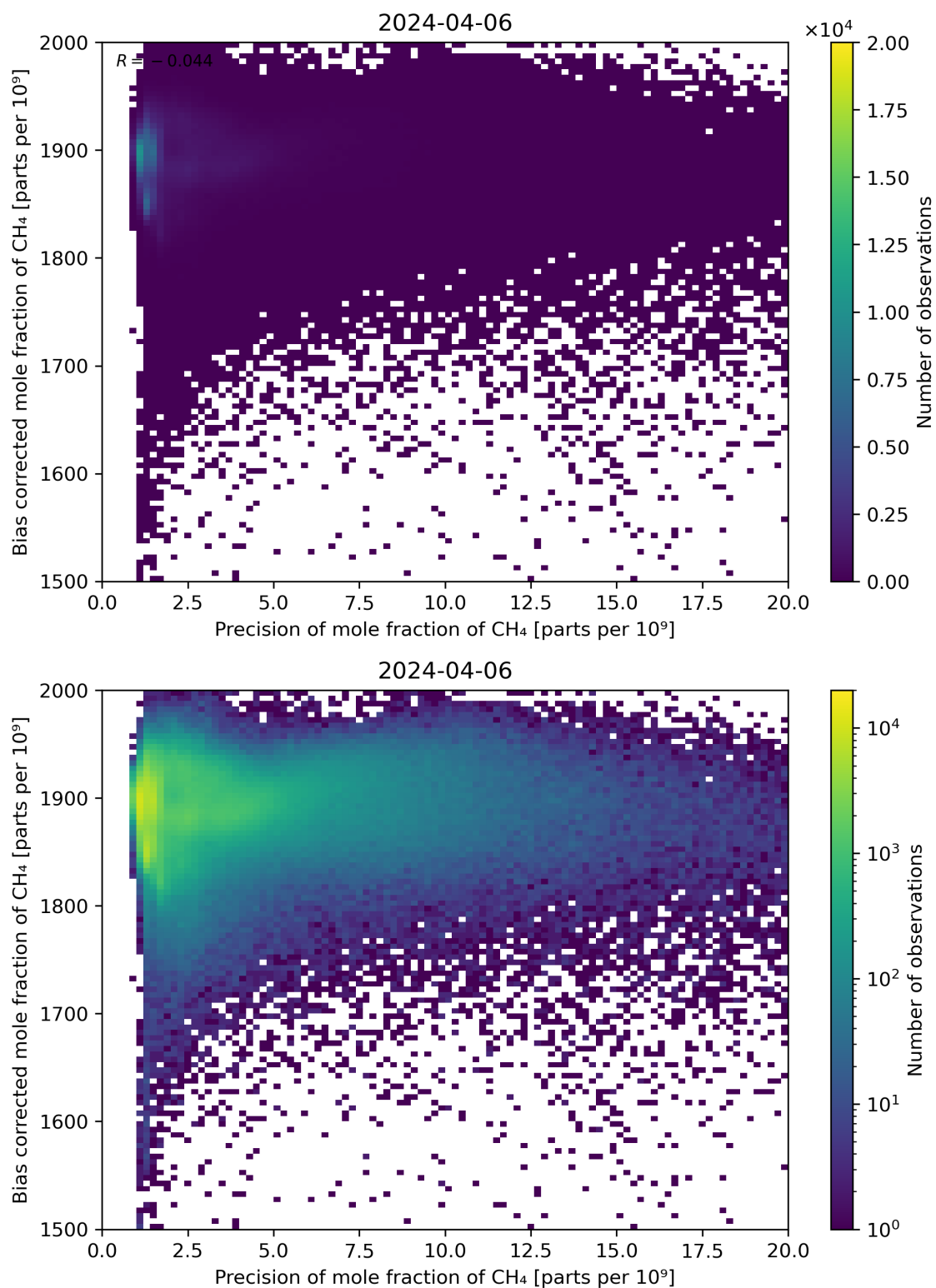
Figure 82: Scatter density plot of “Precision of mole fraction of CH 4 ” against “Bias corrected mole fraction of CH 4 ” for 2024-04-05 to 2024-04-07.
