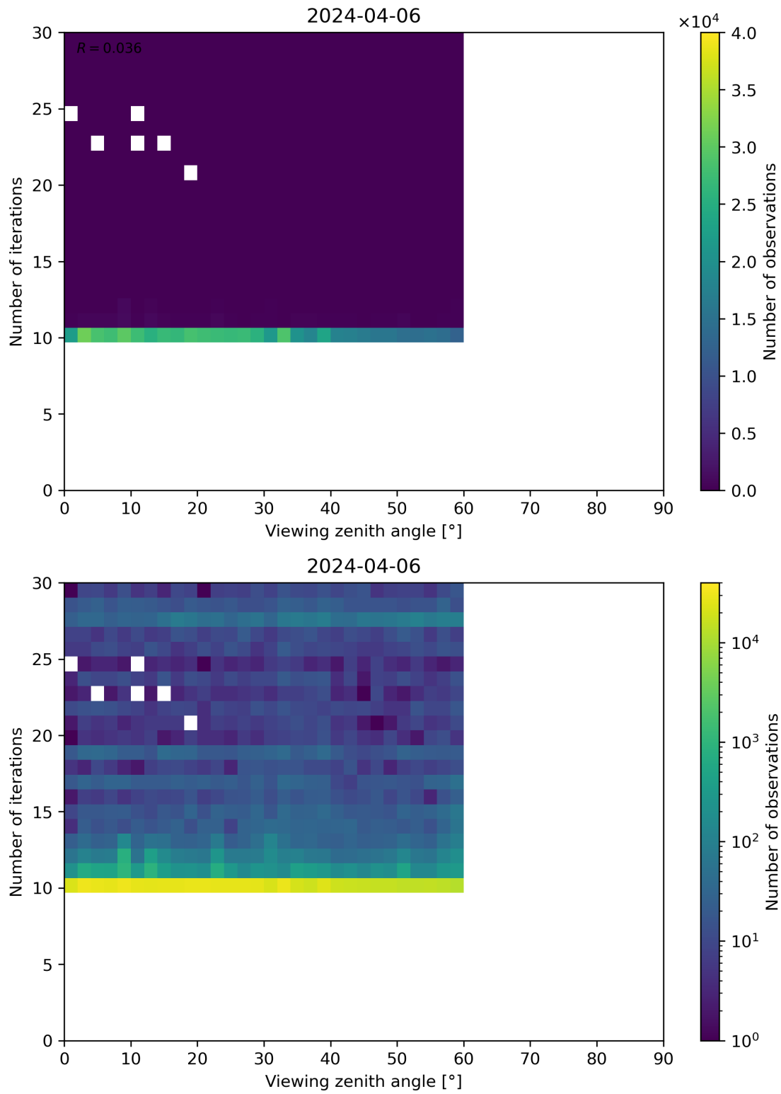
Figure 113: Scatter density plot of “Viewing zenith angle” against “Number of iterations” for 2024-04-05 to 2024-04-07.
