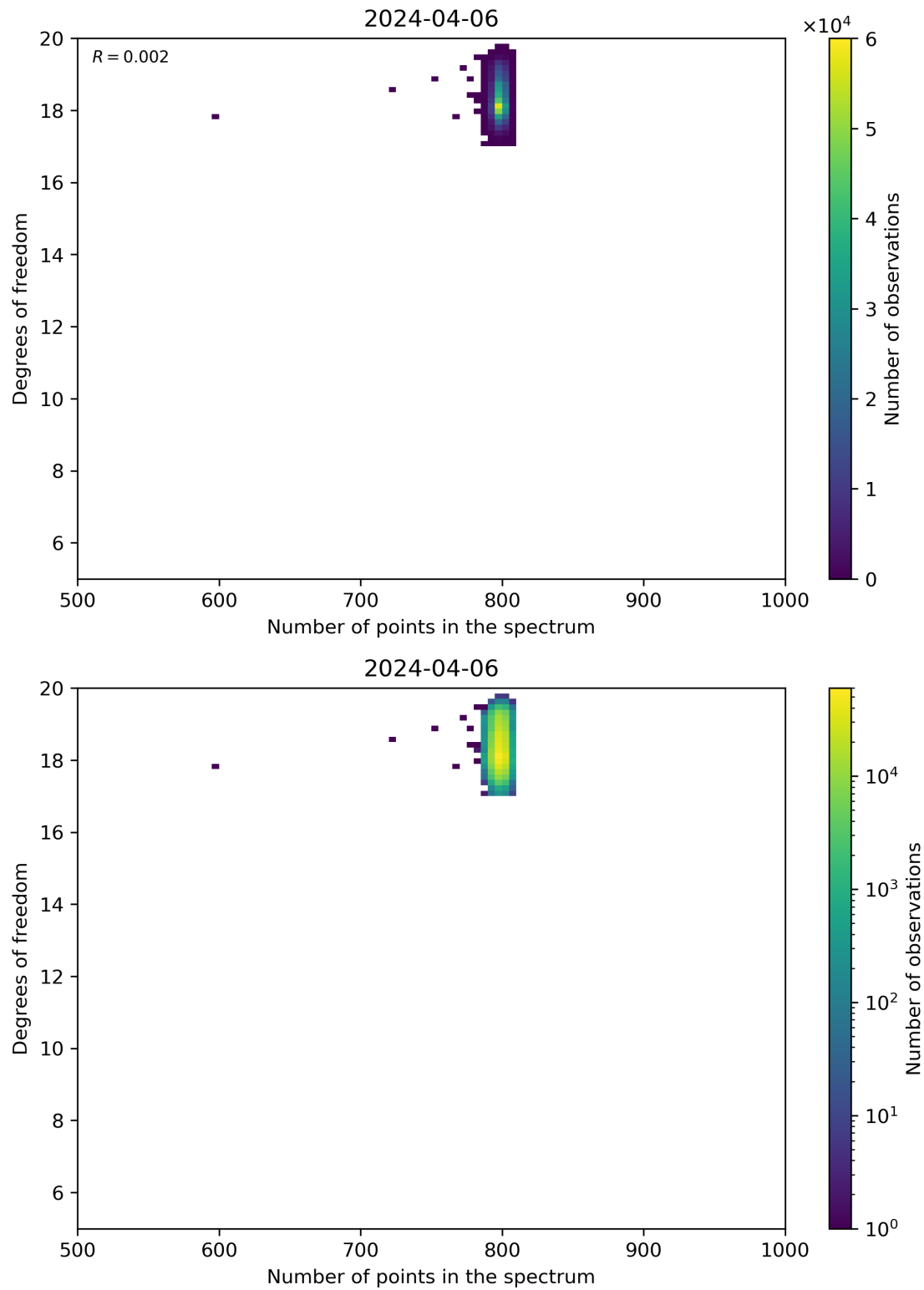
Figure 90: Scatter density plot of “Number of points in the spectrum” against “Degrees of freedom” for 2024-04-05 to 2024-04-07.
