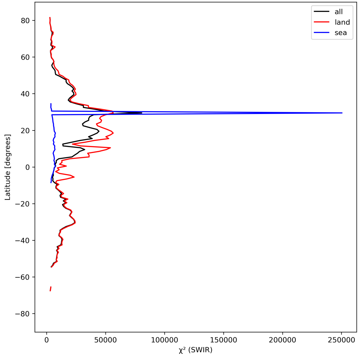
Figure 17: Zonal average of “ \chi^2 (SWIR)” for 2024-04-05 to 2024-04-07.
