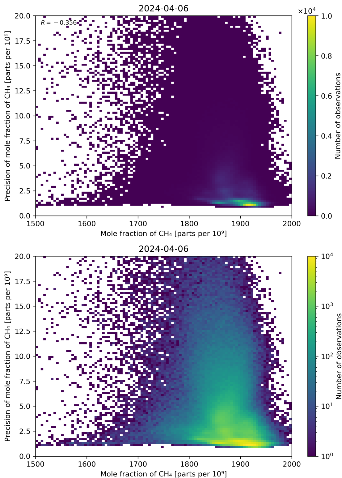
Figure 75: Scatter density plot of “Mole fraction of CH 4 ” against “Precision of mole fraction of CH 4 ” for 2024-04-05 to 2024-04-07.
