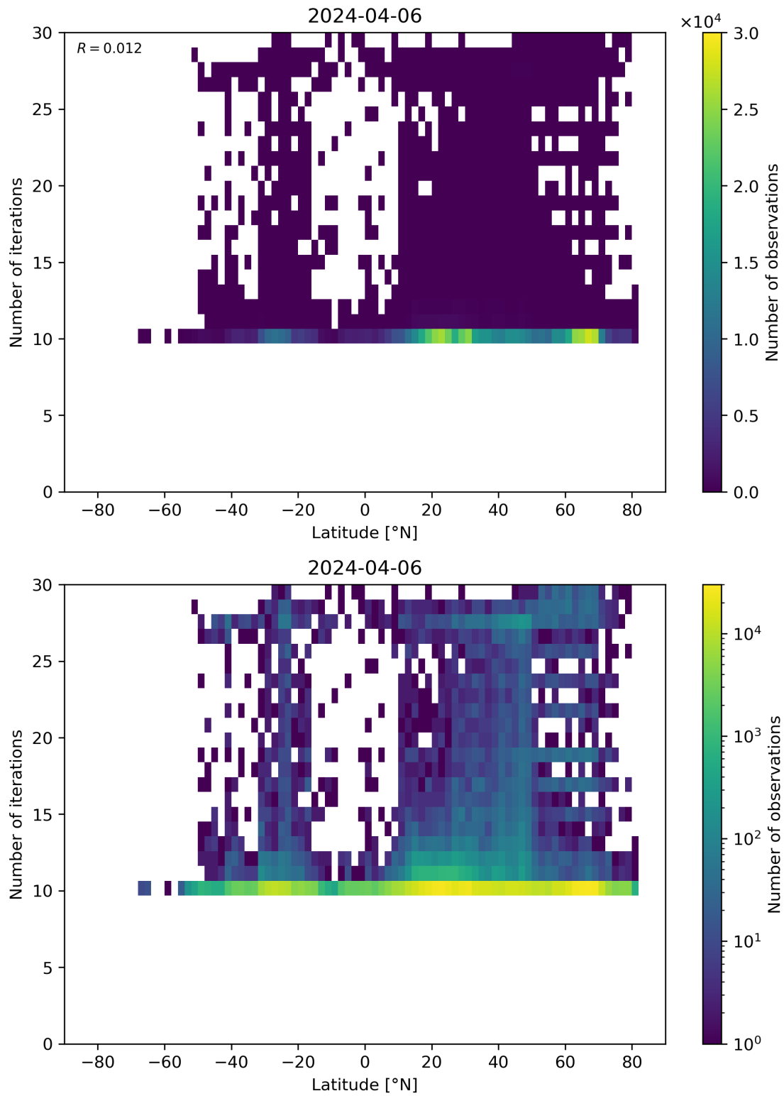
Figure 60: Scatter density plot of “Latitude” against “Number of iterations” for 2024-04-05 to 2024-04-07.
