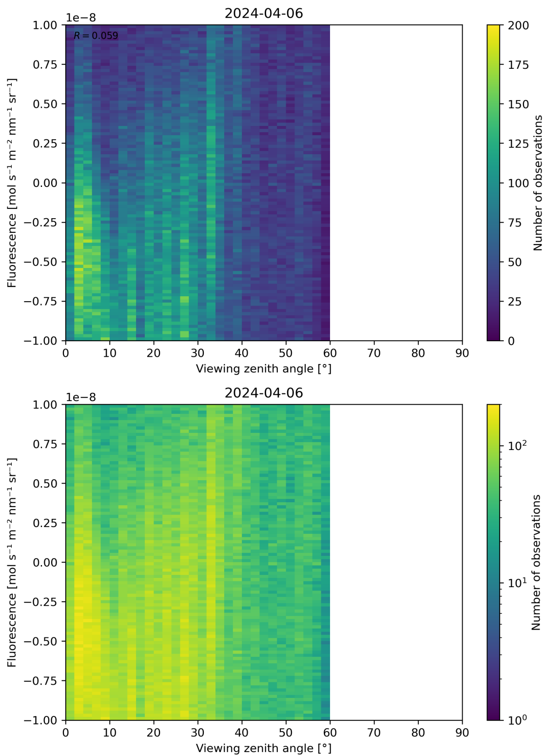
Figure 108: Scatter density plot of “Viewing zenith angle” against “Fluorescence” for 2024-04-05 to 2024-04-07.
