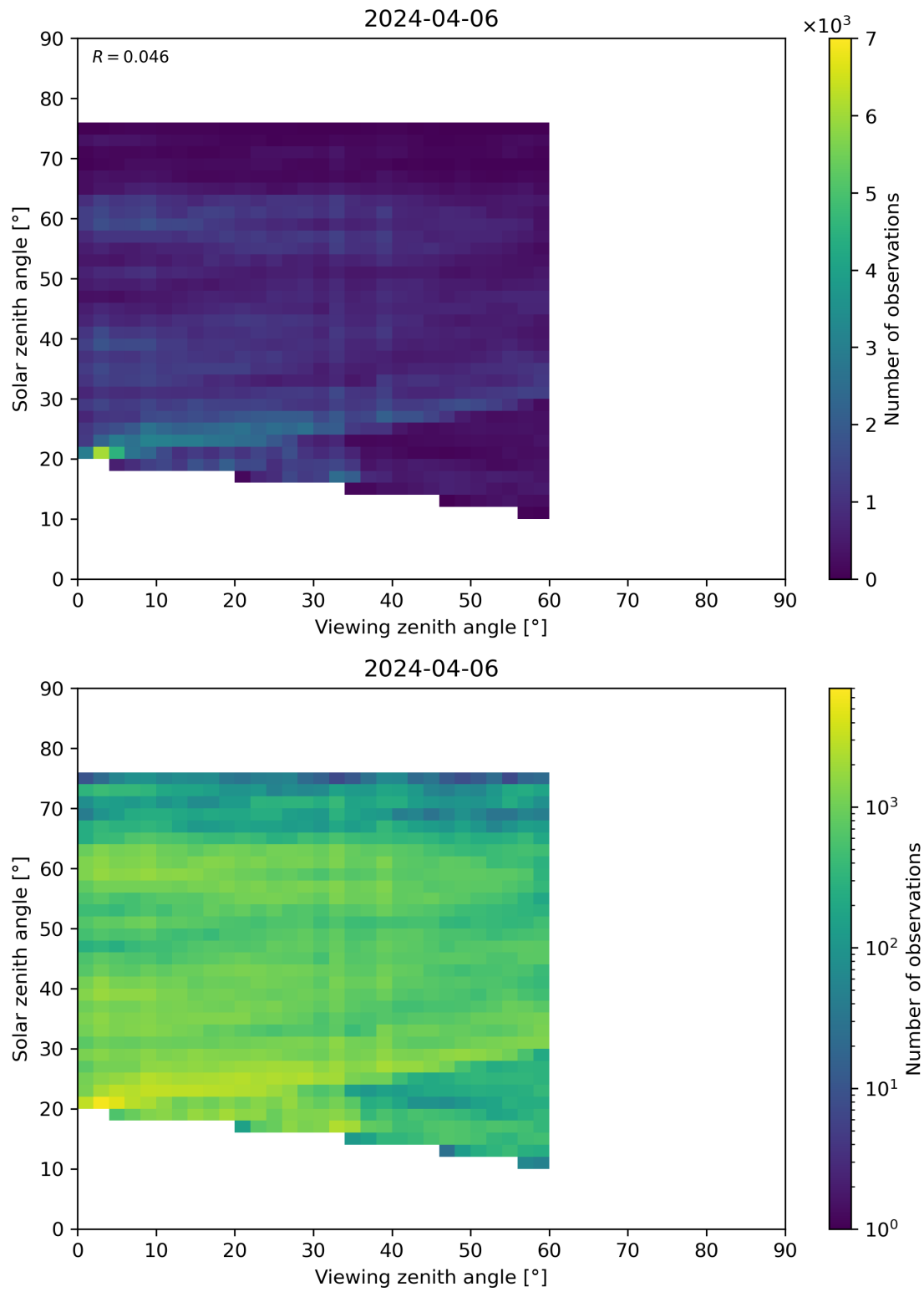
Figure 115: Scatter density plot of “Viewing zenith angle” against “Solar zenith angle” for 2024-04-05 to 2024-04-07.
