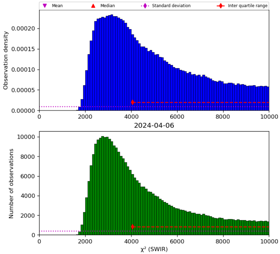
Figure 28: Histogram of “ \chi^2 (SWIR)” for 2024-04-05 to 2024-04-07
