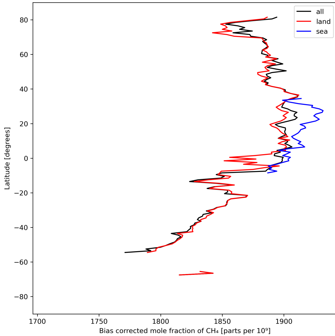
Figure 14: Zonal average of “Bias corrected mole fraction of CH 4 ” for 2024-04-05 to 2024-04-07.
