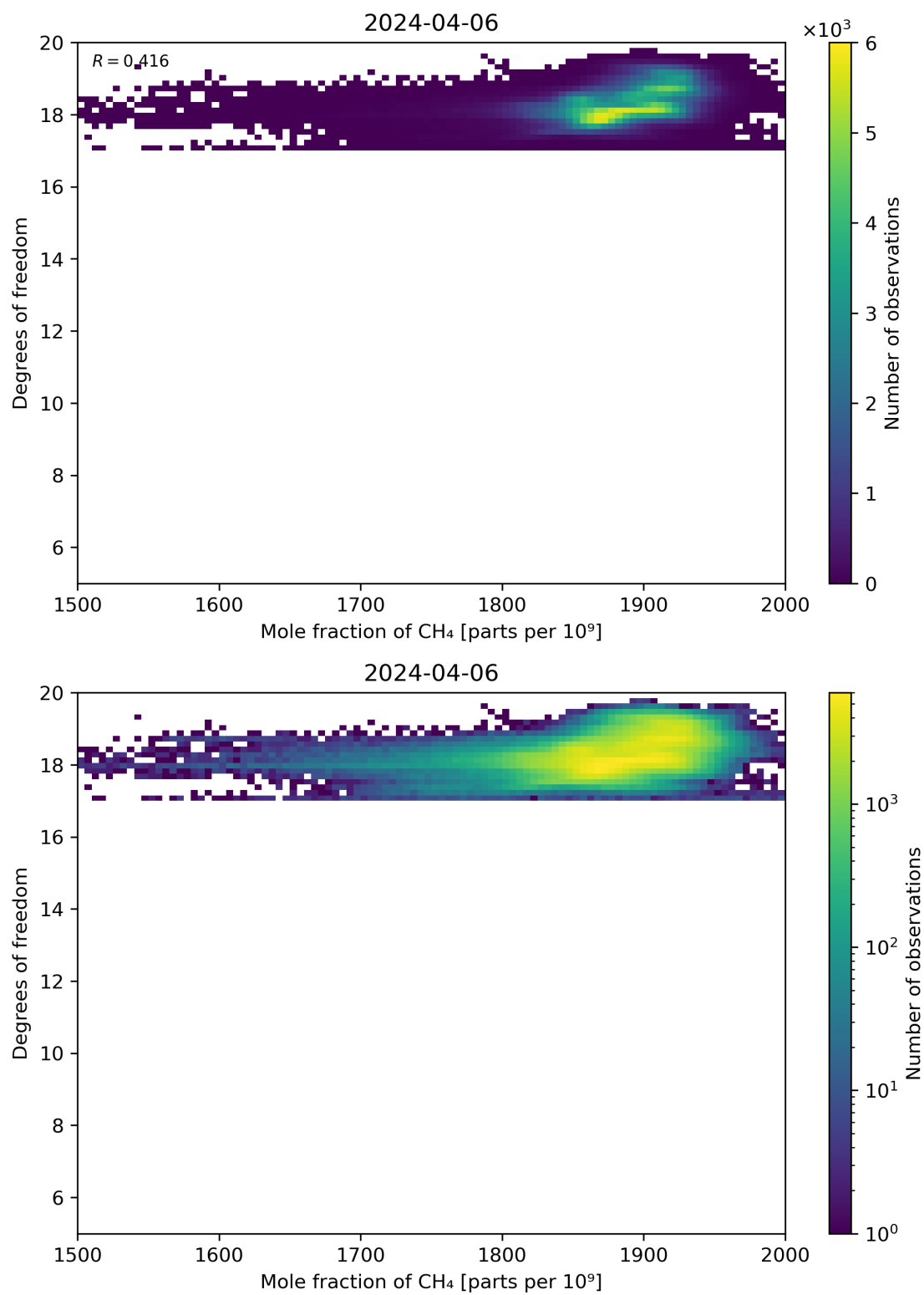
Figure 72: Scatter density plot of “Mole fraction of CH 4 ” against “Degrees of freedom” for 2024-04-05 to 2024-04-07.
