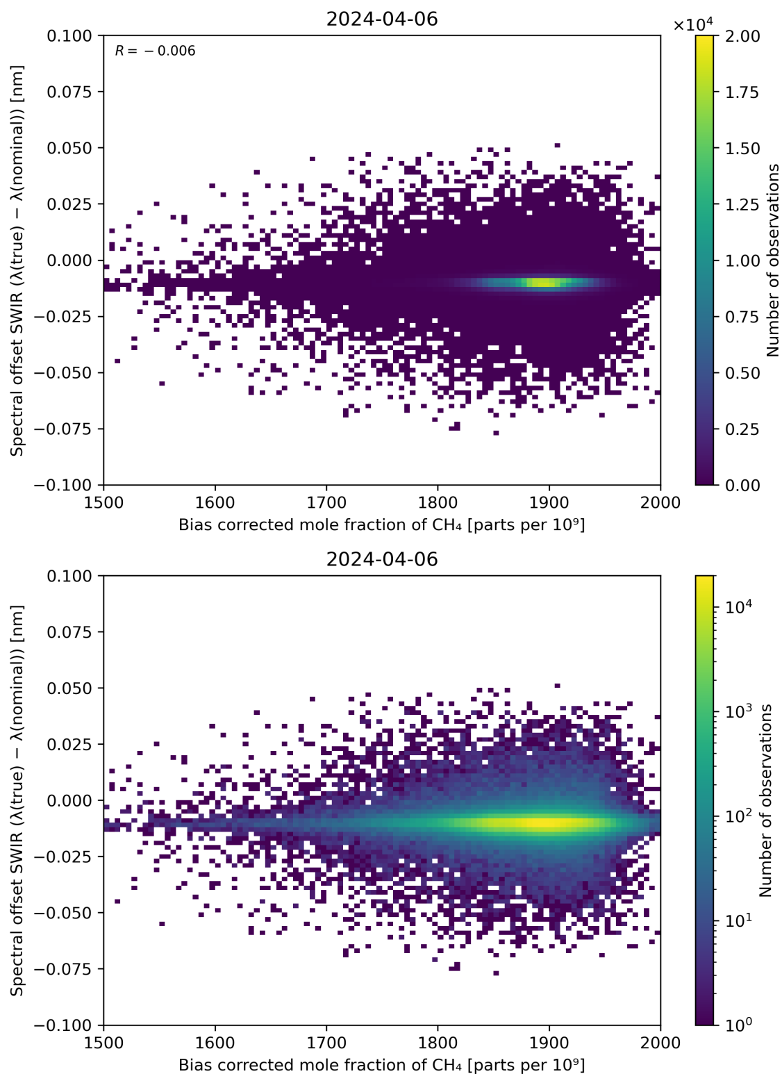
Figure 69: Scatter density plot of “Bias corrected mole fraction of \text{CH}_4 ” against “Spectral offset SWIR ( \lambda(\text{true}) - \lambda(\text{nominal}) )” for 2024-04-05 to 2024-04-07.
