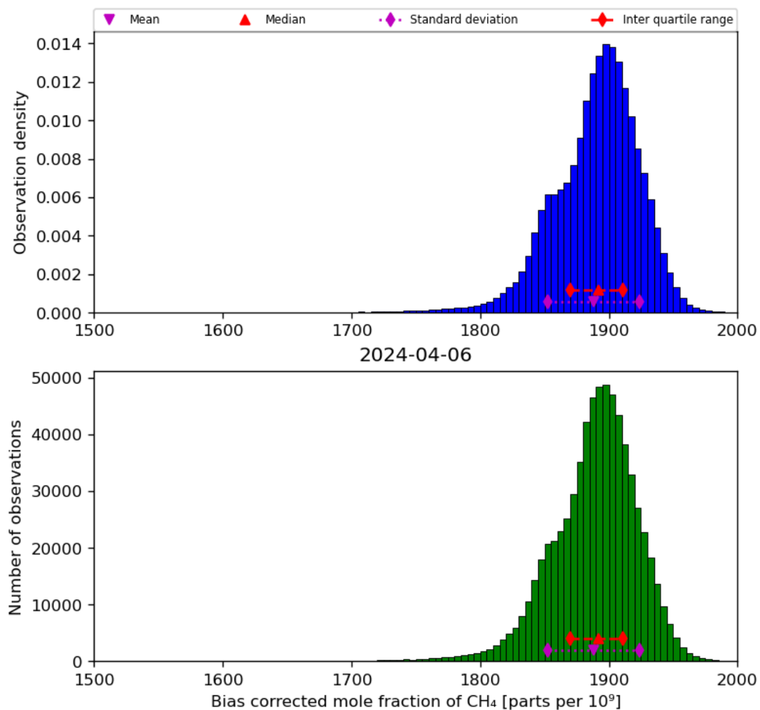
Figure 25: Histogram of “Bias corrected mole fraction of CH 4 ” for 2024-04-05 to 2024-04-07
