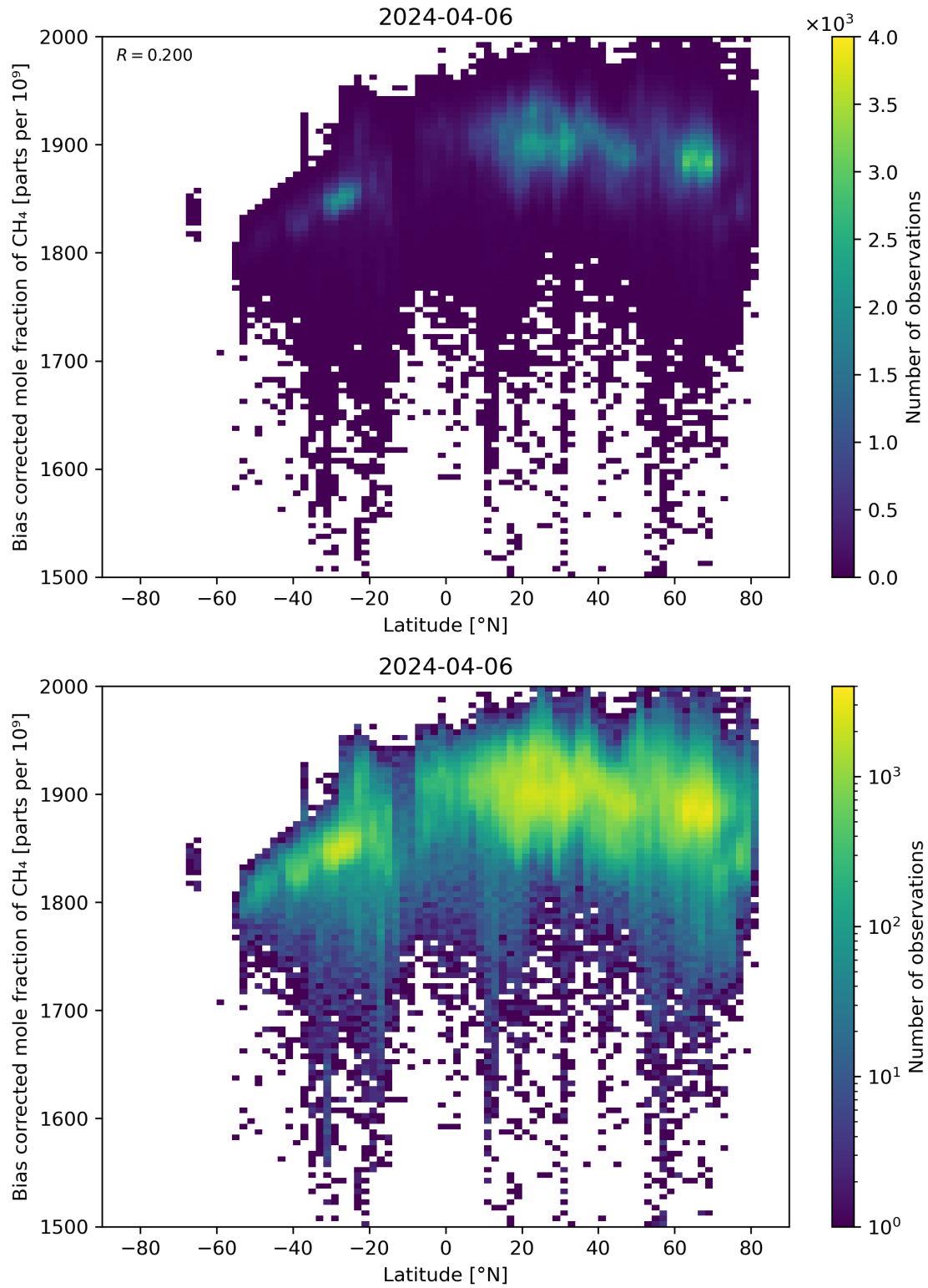
Figure 58: Scatter density plot of “Latitude” against “Bias corrected mole fraction of CH 4 ” for 2024-04-05 to 2024-04-07.
