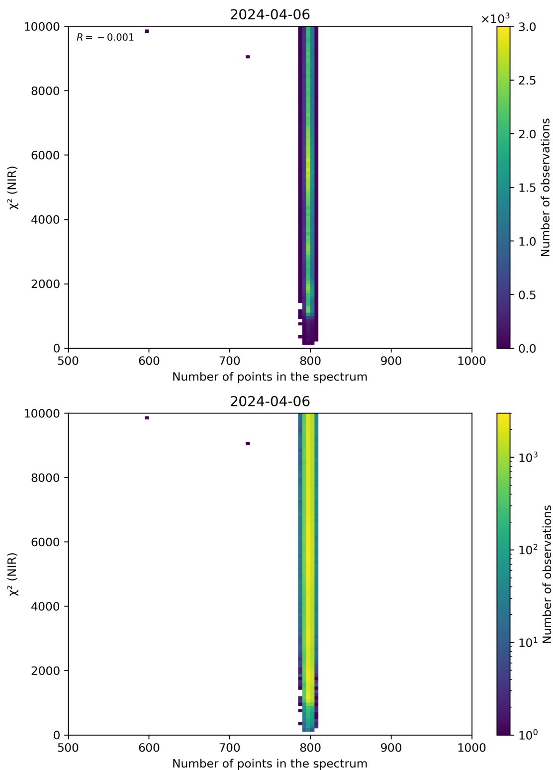
Figure 88: Scatter density plot of “Number of points in the spectrum” against “ \chi^2 (NIR)” for 2024-04-05 to 2024-04-07.
