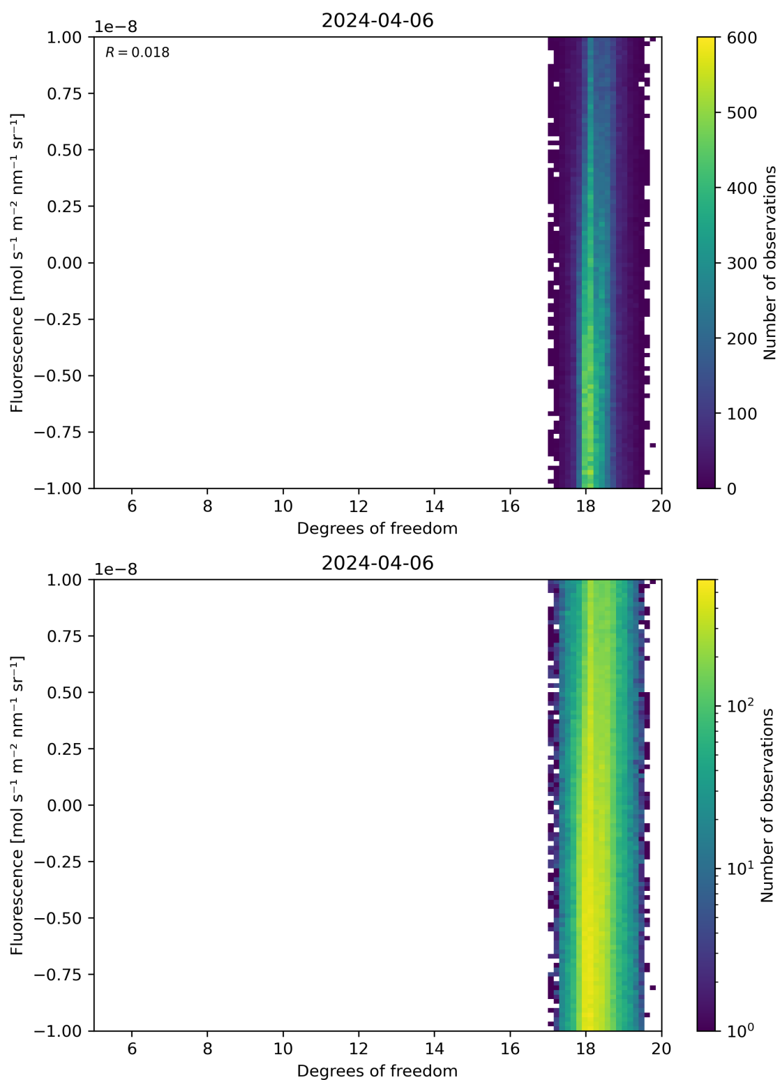
Figure 51: Scatter density plot of “Degrees of freedom” against “Fluorescence” for 2024-04-05 to 2024-04-07.
