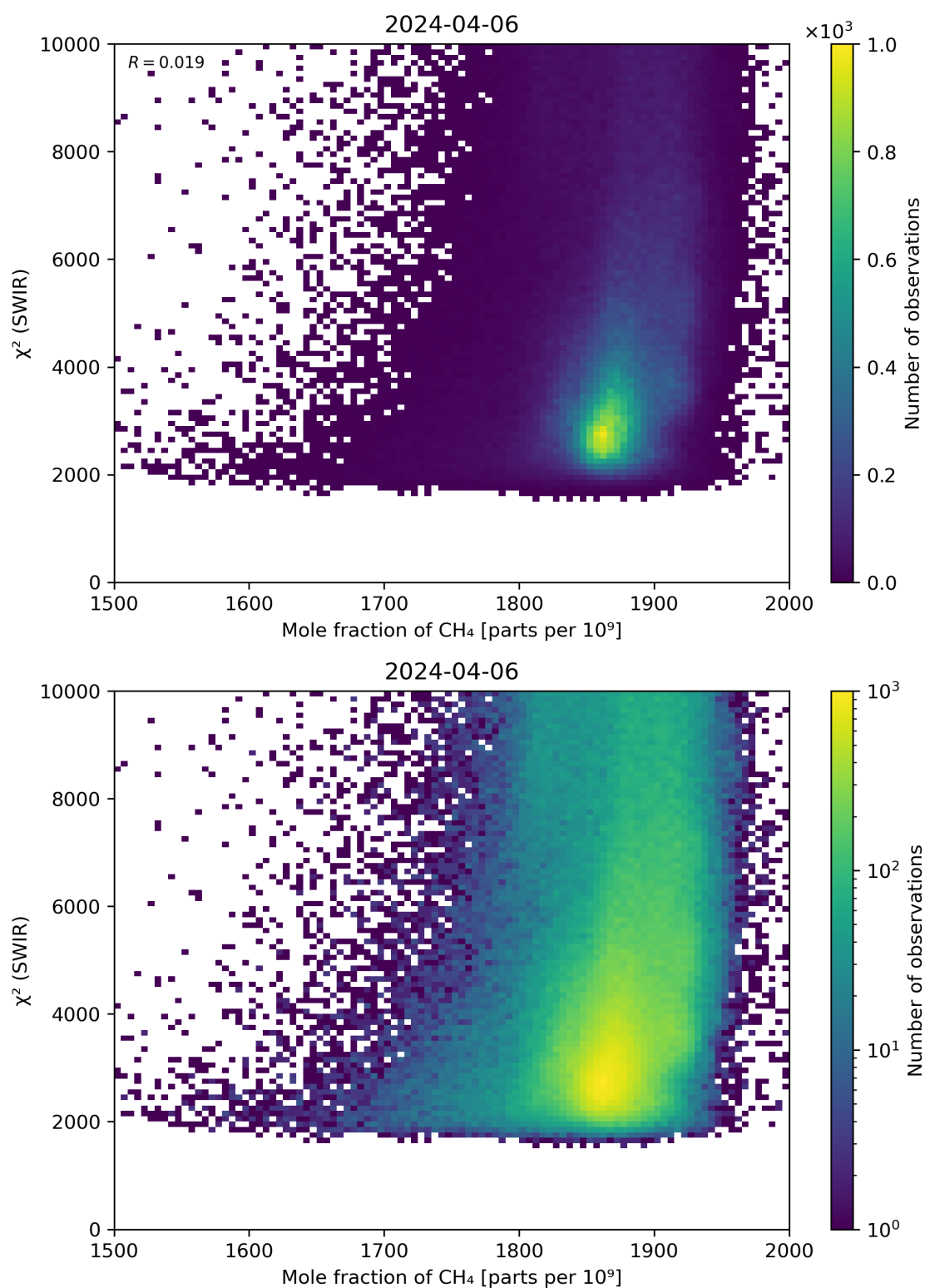
Figure 71: Scatter density plot of “Mole fraction of \text{CH}_4 ” against “ \chi^2 (SWIR)” for 2024-04-05 to 2024-04-07.
