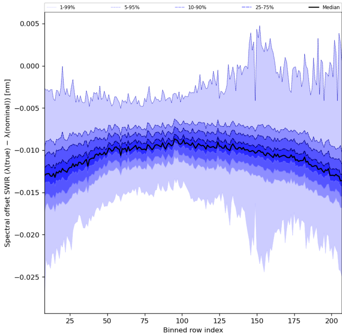
Figure 38: Along track statistics of “Spectral offset SWIR ( \lambda(\text{true}) - \lambda(\text{nominal}) )” for 2024-04-05 to 2024-04-07
