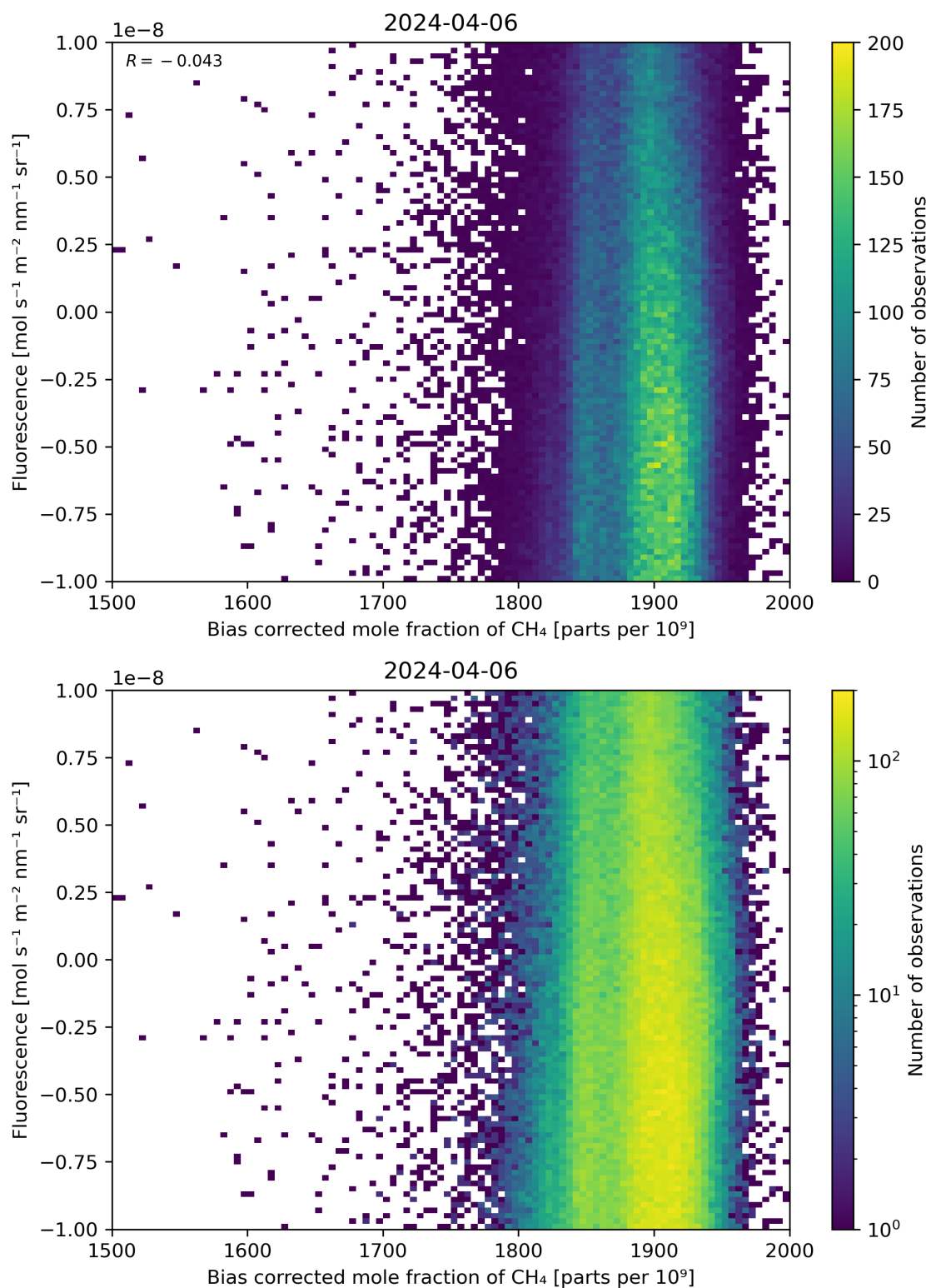
Figure 66: Scatter density plot of “Bias corrected mole fraction of \text{CH}_4 ” against “Fluorescence” for 2024-04-05 to 2024-04-07.
