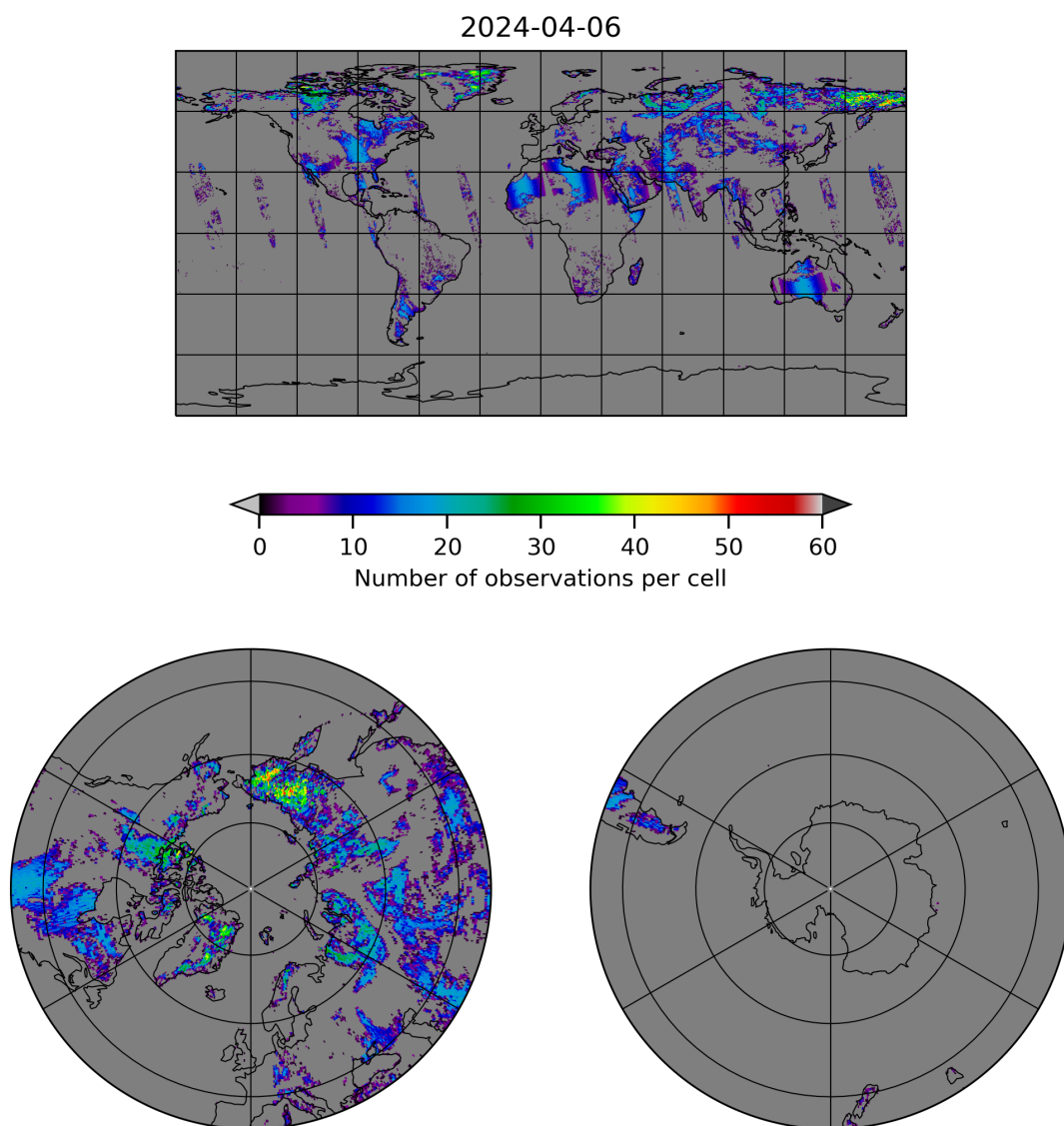
Figure 10: Map of the number of observations for 2024-04-05 to 2024-04-07
