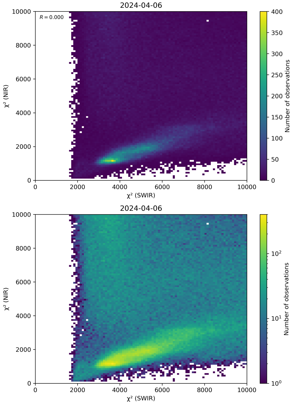
Figure 47: Scatter density plot of “ \chi^2 (SWIR)” against “ \chi^2 (NIR)” for 2024-04-05 to 2024-04-07.
