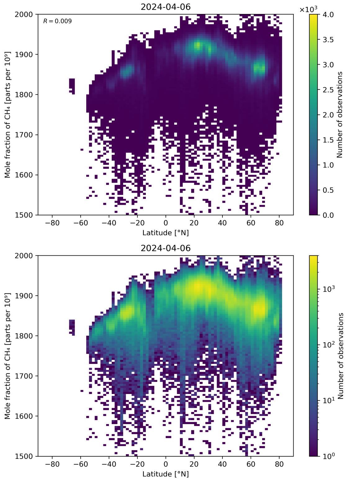
Figure 57: Scatter density plot of “Latitude” against “Mole fraction of CH 4 ” for 2024-04-05 to 2024-04-07.
