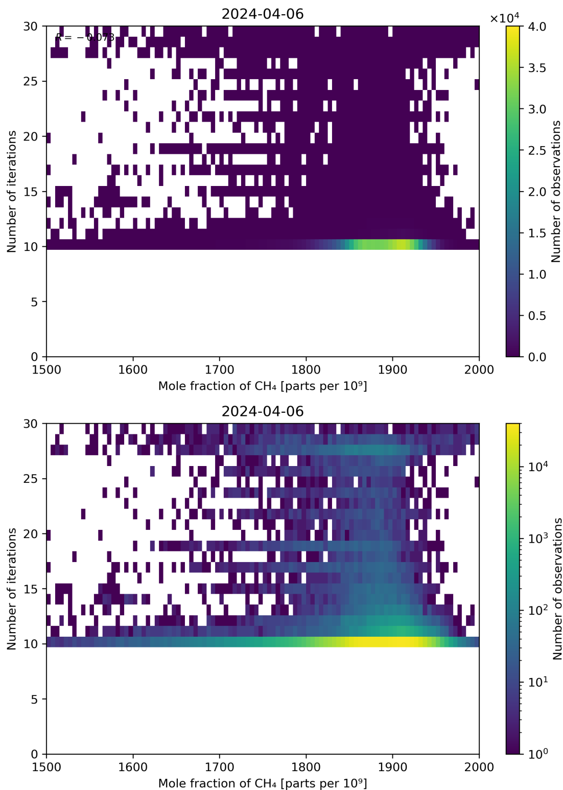
Figure 76: Scatter density plot of “Mole fraction of CH 4 ” against “Number of iterations” for 2024-04-05 to 2024-04-07.
