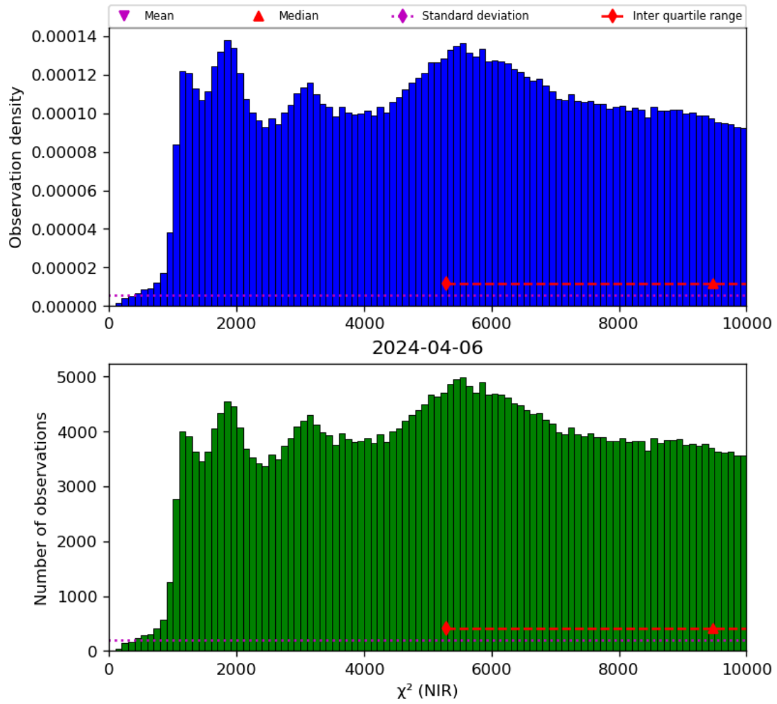
Figure 29: Histogram of " \chi^2 (NIR)" for 2024-04-05 to 2024-04-07
