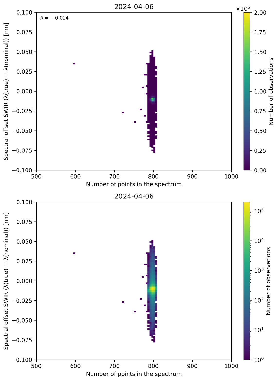
Figure 93: Scatter density plot of “Number of points in the spectrum” against “Spectral offset SWIR ( \lambda(\text{true}) - \lambda(\text{nominal}) )” for 2024-04-05 to 2024-04-07.
