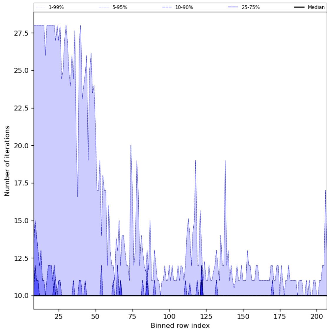
Figure 42: Along track statistics of “Number of iterations” for 2024-04-05 to 2024-04-07
