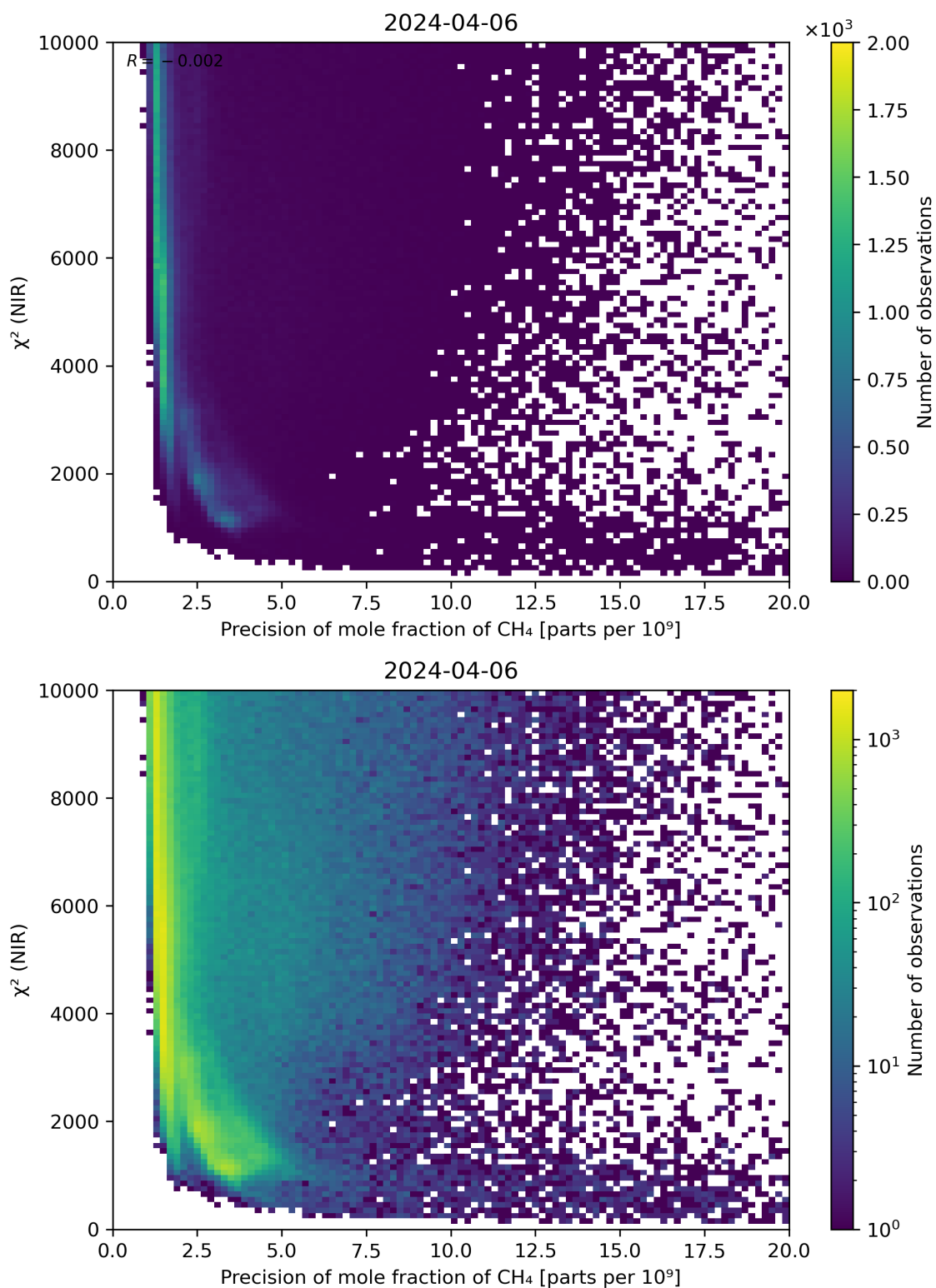
Figure 78: Scatter density plot of “Precision of mole fraction of CH 4 ” against “ \chi^2 (NIR)” for 2024-04-05 to 2024-04-07.
