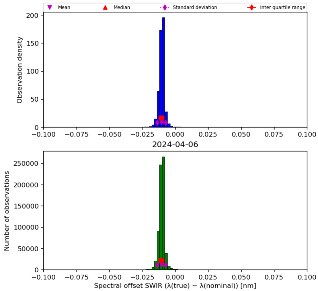
Figure 27: Histogram of “Spectral offset SWIR ( \lambda(\text{true}) - \lambda(\text{nominal}) )” for 2024-04-05 to 2024-04-07
