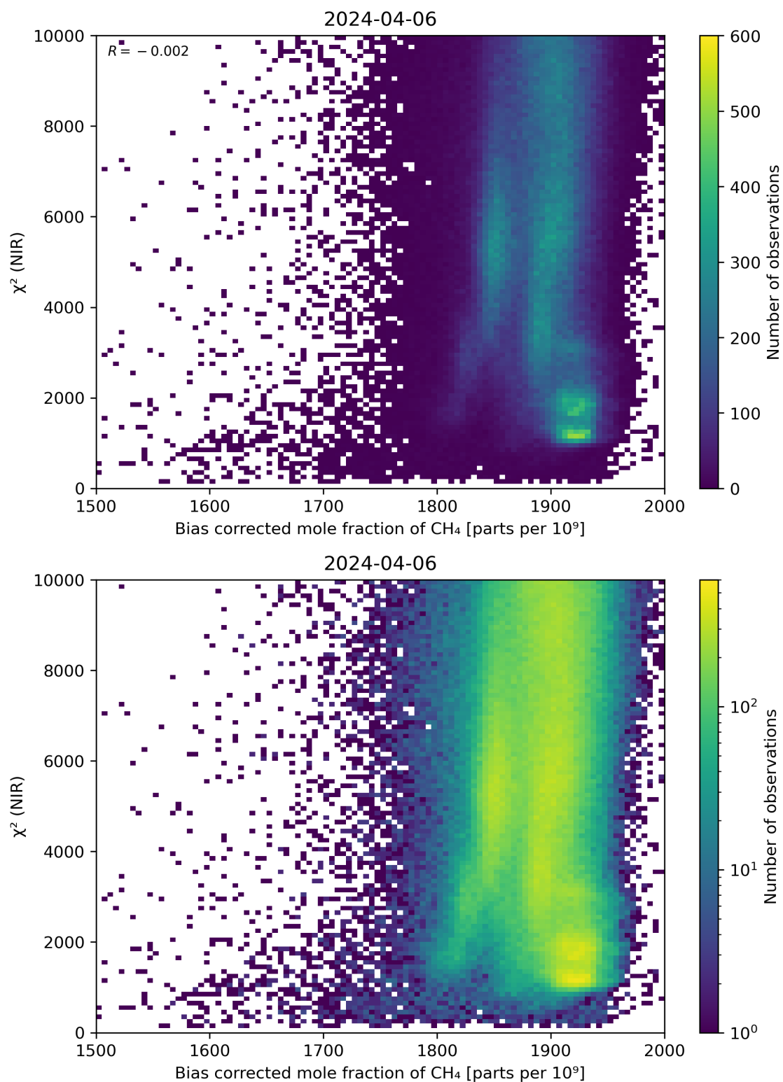
Figure 63: Scatter density plot of “Bias corrected mole fraction of CH 4 ” against “ \chi^2 (NIR)” for 2024-04-05 to 2024-04-07.
