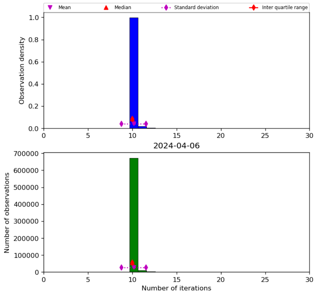
Figure 31: Histogram of “Number of iterations” for 2024-04-05 to 2024-04-07
