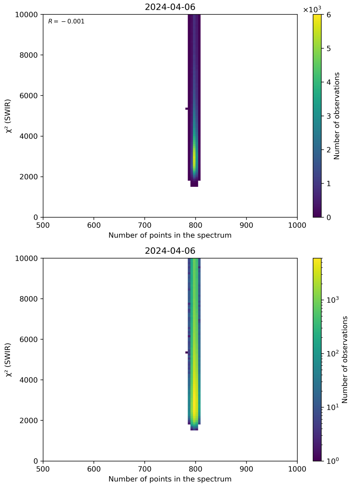
Figure 89: Scatter density plot of “Number of points in the spectrum” against “ \chi^2 (SWIR)” for 2024-04-05 to 2024-04-07.
