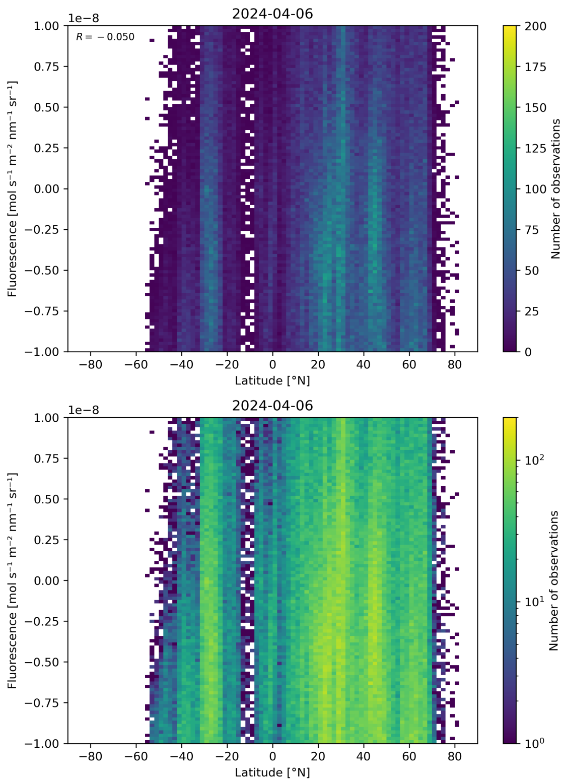
Figure 56: Scatter density plot of “Latitude” against “Fluorescence” for 2024-04-05 to 2024-04-07.
