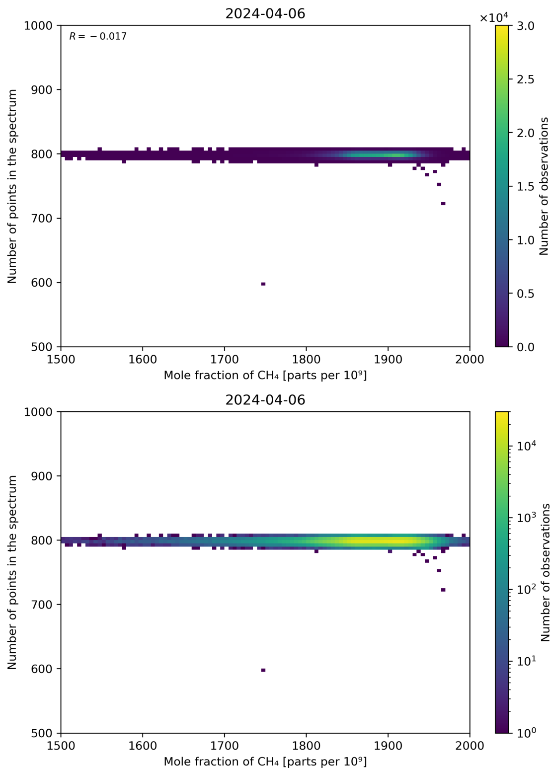
Figure 77: Scatter density plot of “Mole fraction of CH 4 ” against “Number of points in the spectrum” for 2024-04-05 to 2024-04-07.
