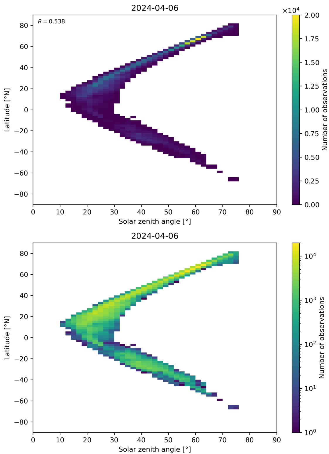
Figure 98: Scatter density plot of “Solar zenith angle” against “Latitude” for 2024-04-05 to 2024-04-07.
