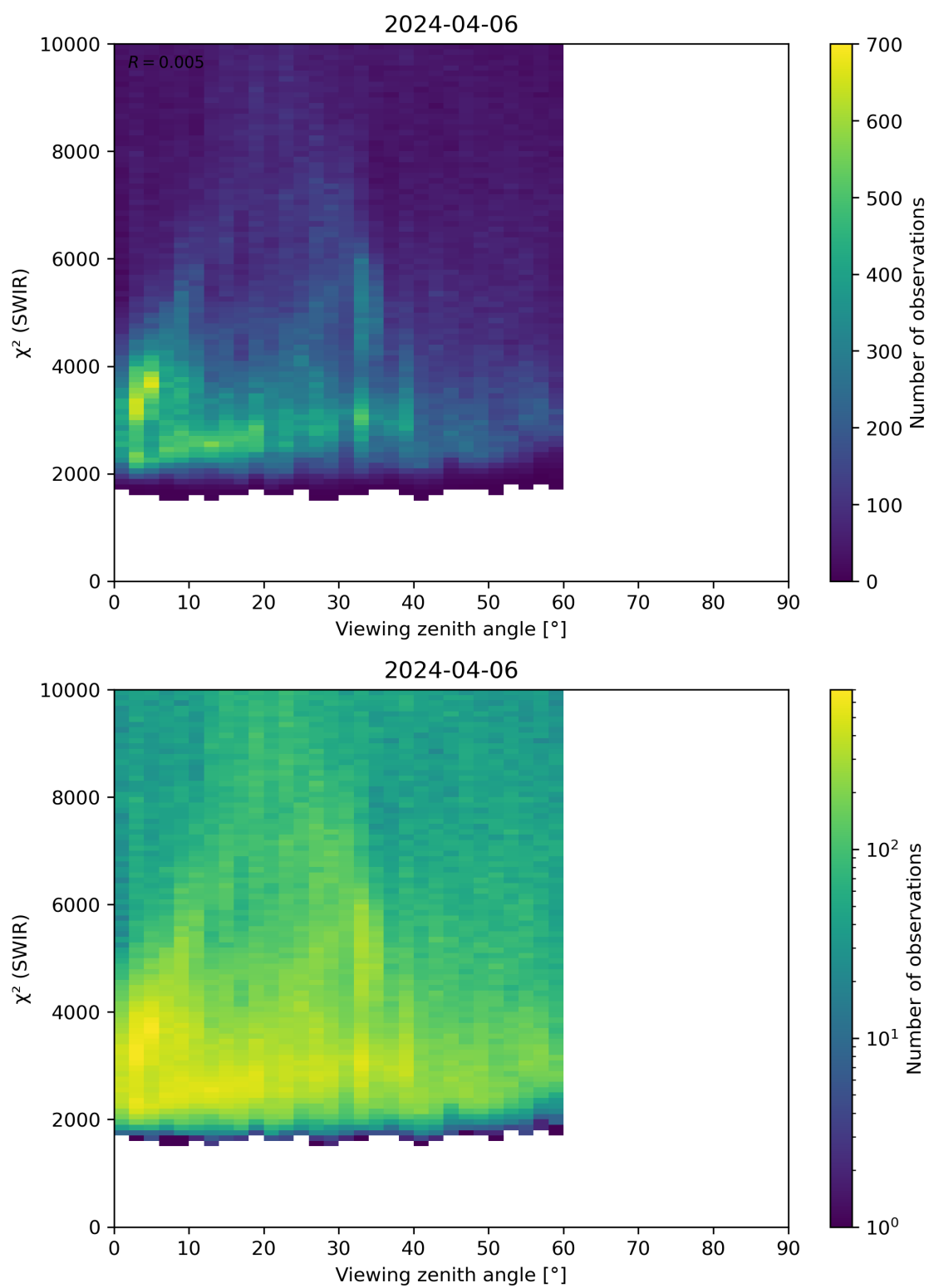
Figure 106: Scatter density plot of “Viewing zenith angle” against “ \chi^2 (SWIR)” for 2024-04-05 to 2024-04-07.
