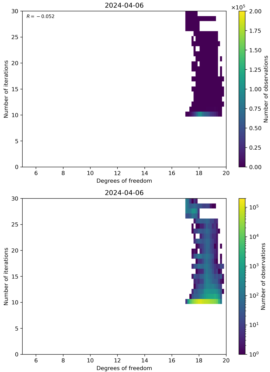
Figure 52: Scatter density plot of “Degrees of freedom” against “Number of iterations” for 2024-04-05 to 2024-04-07.
