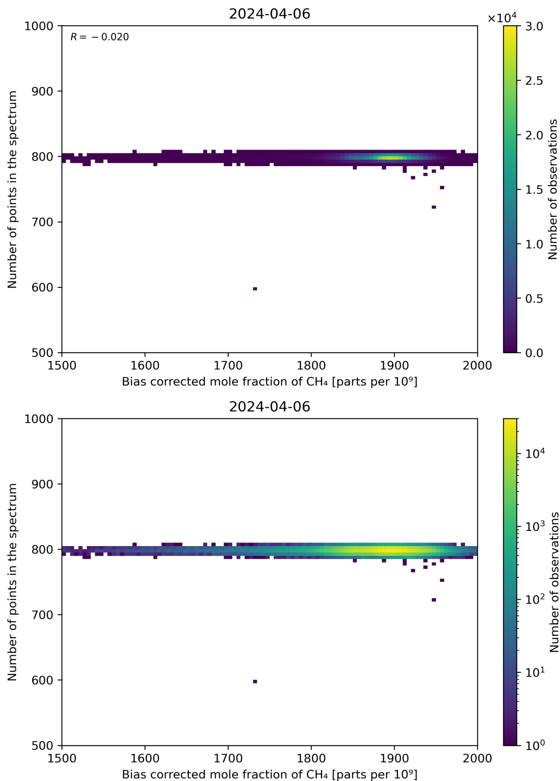
Figure 68: Scatter density plot of “Bias corrected mole fraction of CH 4 ” against “Number of points in the spectrum” for 2024-04-05 to 2024-04-07.
