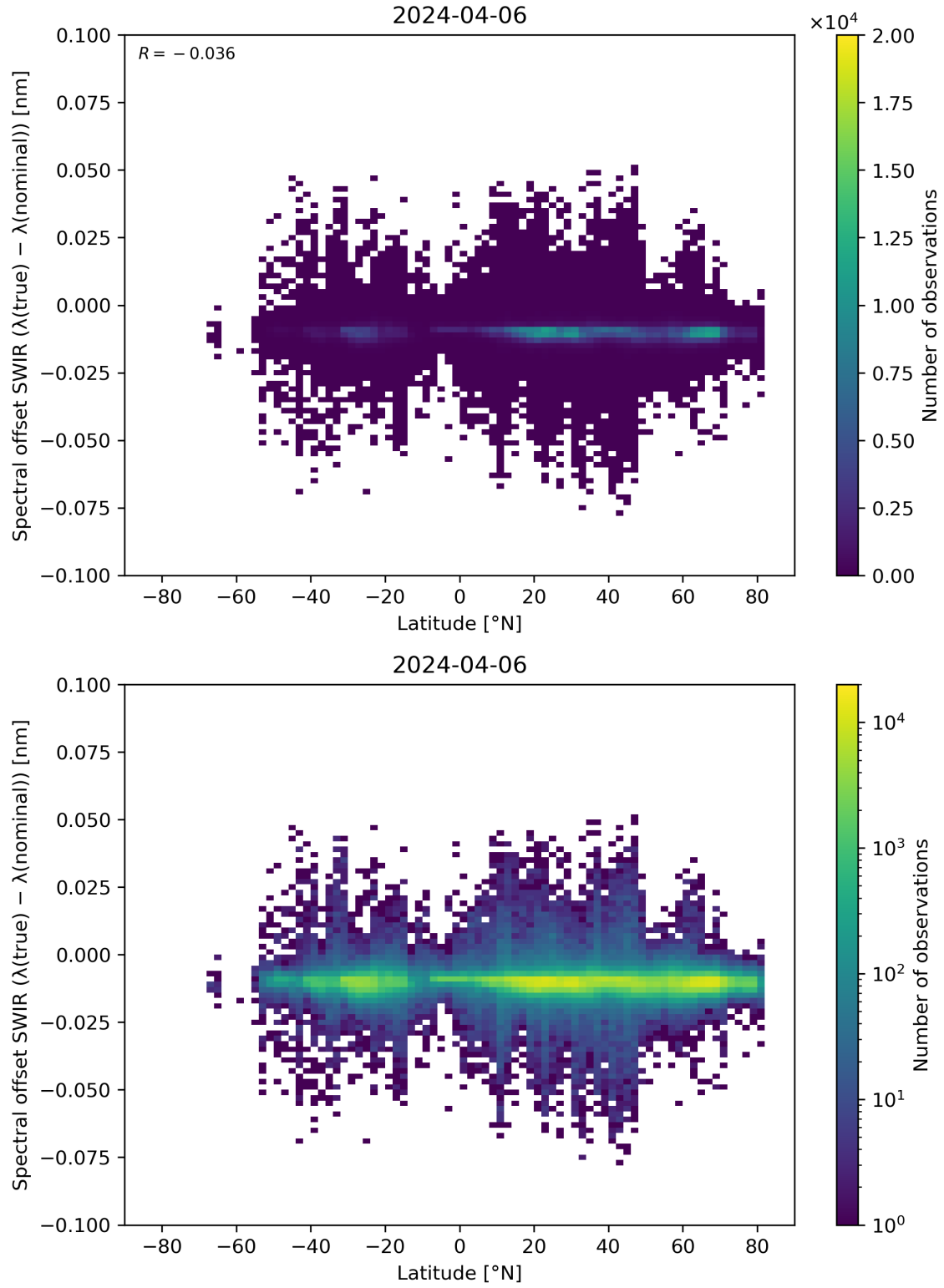
Figure 62: Scatter density plot of “Latitude” against “Spectral offset SWIR ( \lambda(\text{true}) - \lambda(\text{nominal}) )” for 2024-04-05 to 2024-04-07.
