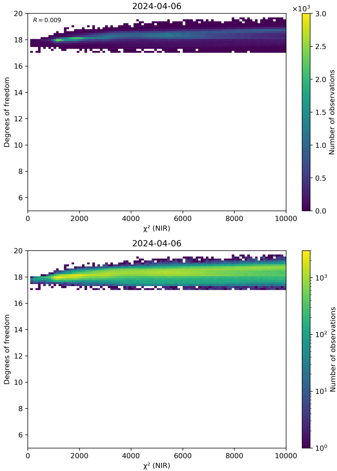
Figure 44: Scatter density plot of “ \chi^2 (NIR)” against “Degrees of freedom” for 2024-04-05 to 2024-04-07.
