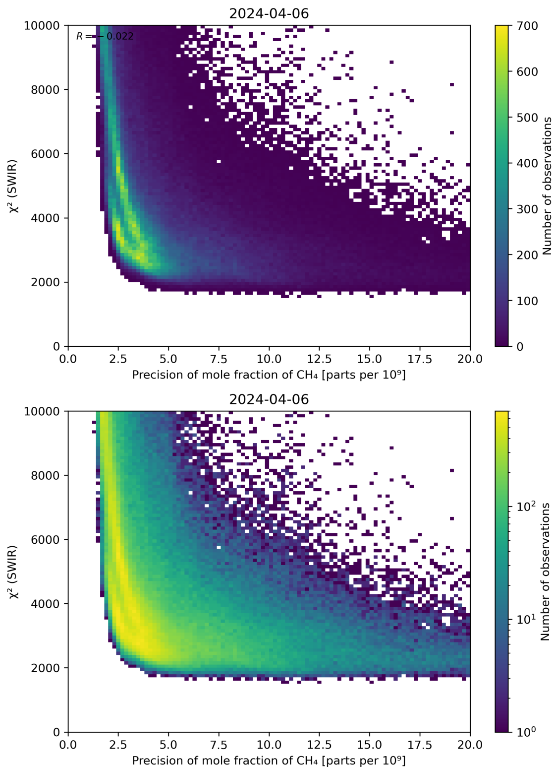
Figure 79: Scatter density plot of “Precision of mole fraction of \text{CH}_4 ” against “ \chi^2 (SWIR)” for 2024-04-05 to 2024-04-07.
