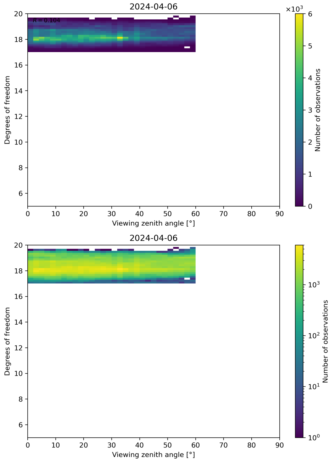
Figure 107: Scatter density plot of “Viewing zenith angle” against “Degrees of freedom” for 2024-04-05 to 2024-04-07.
