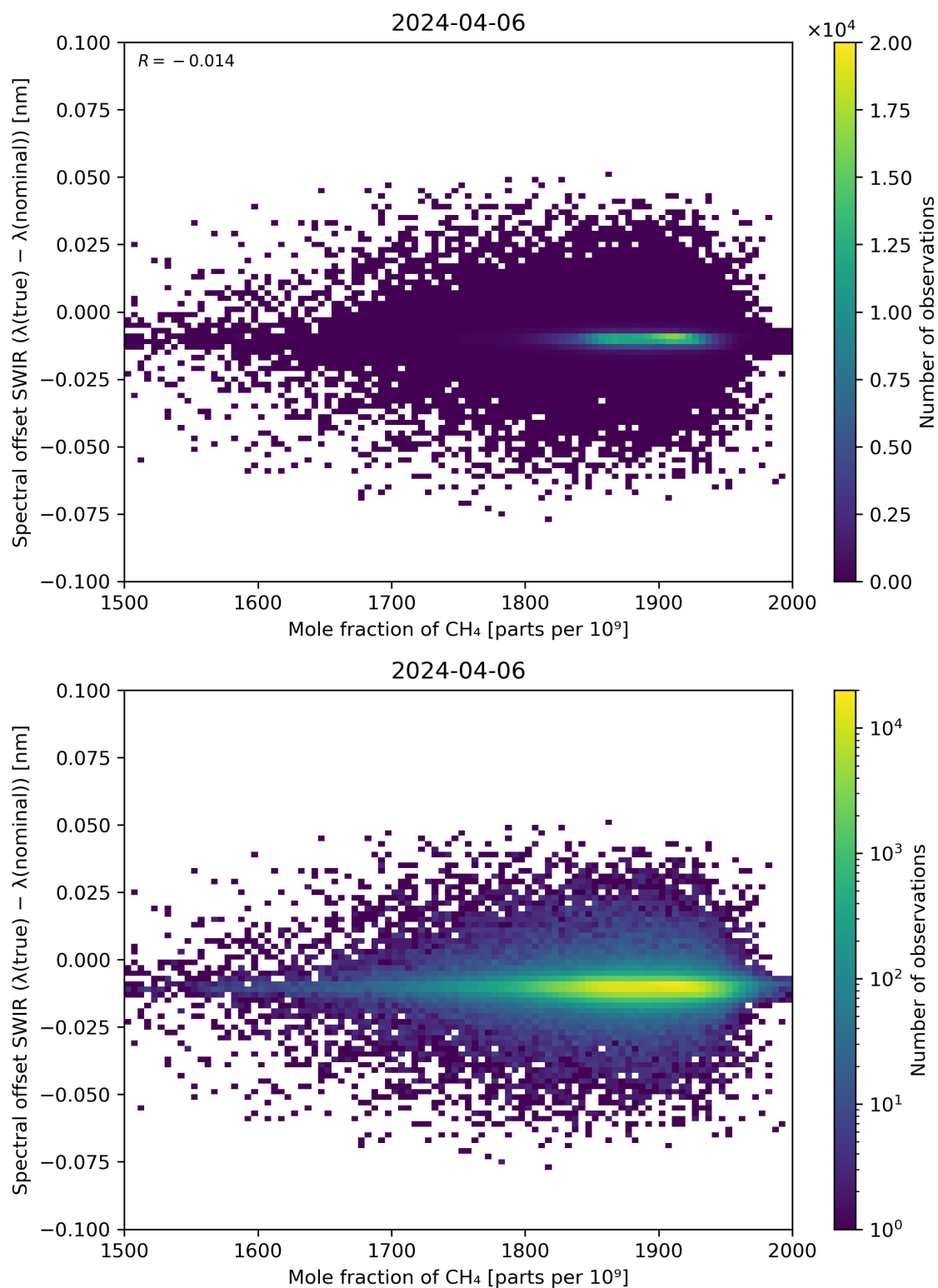
Figure 86: Scatter density plot of “Mole fraction of CH 4 ” against “Spectral offset SWIR ( \lambda(\text{true}) - \lambda(\text{nominal}) )” for 2024-04-05 to 2024-04-07.
