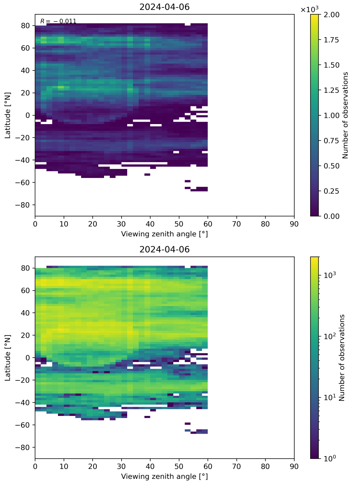
Figure 109: Scatter density plot of “Viewing zenith angle” against “Latitude” for 2024-04-05 to 2024-04-07.
