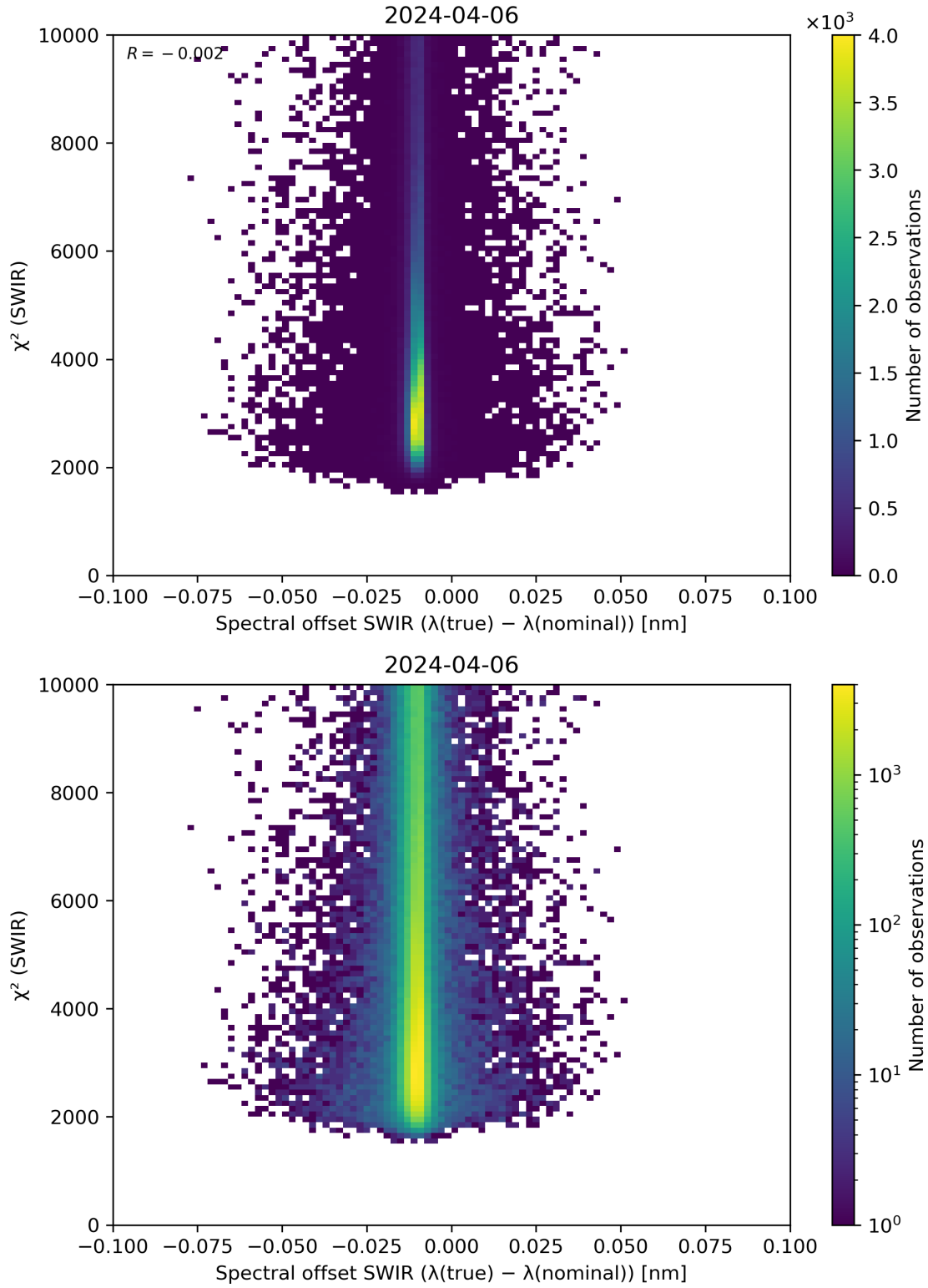
Figure 118: Scatter density plot of “Spectral offset SWIR ( \lambda(\text{true}) - \lambda(\text{nominal}) )” against “ \chi^2 (SWIR)” for 2024-04-05 to 2024-04-07.
