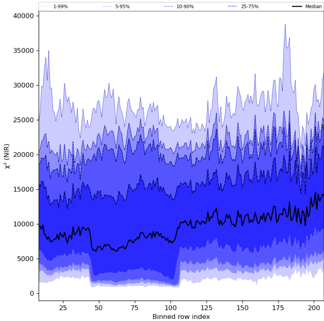
Figure 40: Along track statistics of “ \chi^2 (NIR)” for 2024-04-05 to 2024-04-07
