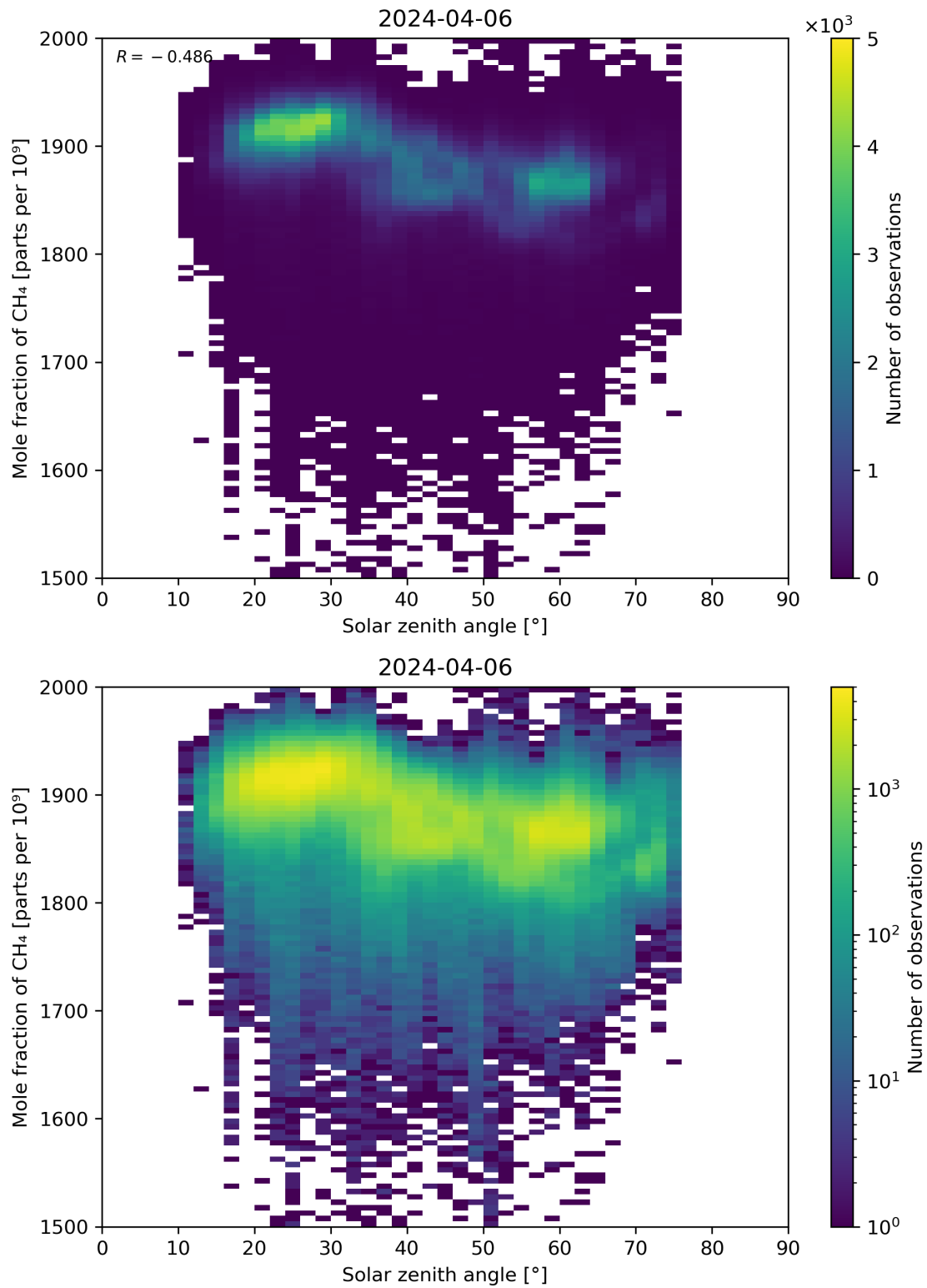
Figure 99: Scatter density plot of “Solar zenith angle” against “Mole fraction of \text{CH}_4 ” for 2024-04-05 to 2024-04-07.
