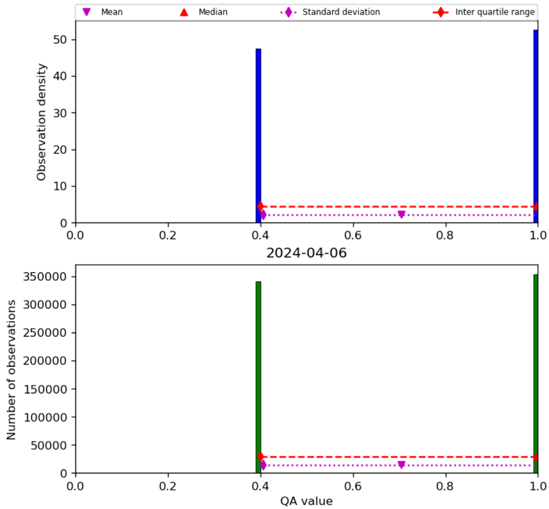
Figure 22: Histogram of “QA value” for 2024-04-05 to 2024-04-07
