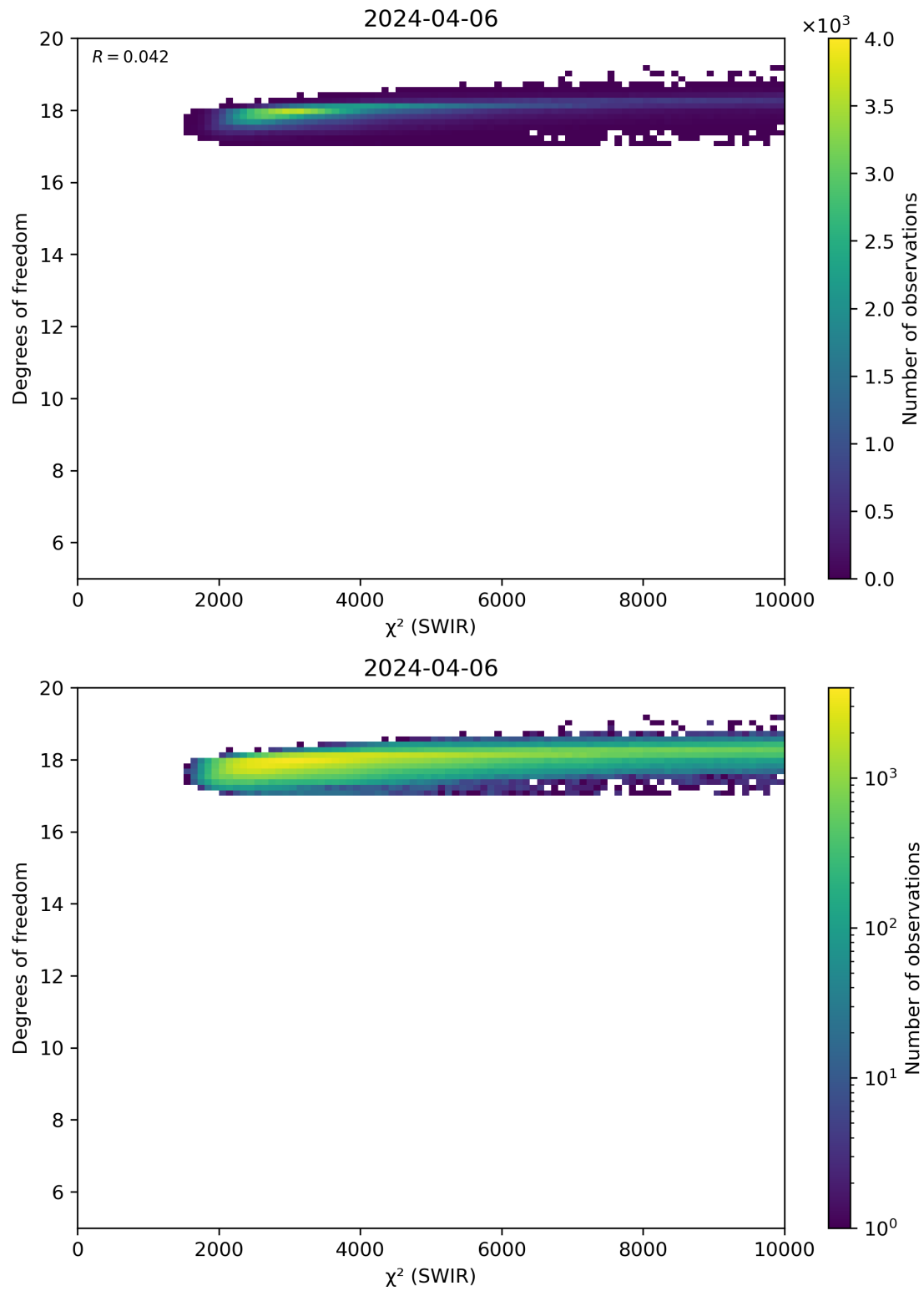
Figure 48: Scatter density plot of “ \chi^2 (SWIR)” against “Degrees of freedom” for 2024-04-05 to 2024-04-07.
