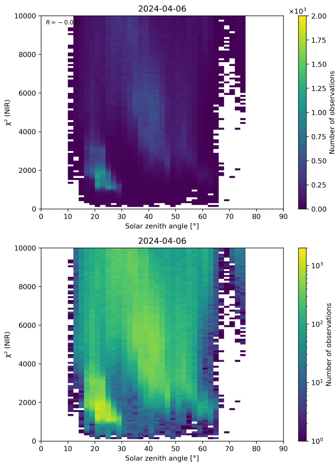
Figure 94: Scatter density plot of “Solar zenith angle” against “ \chi^2 (NIR)” for 2024-04-05 to 2024-04-07.
