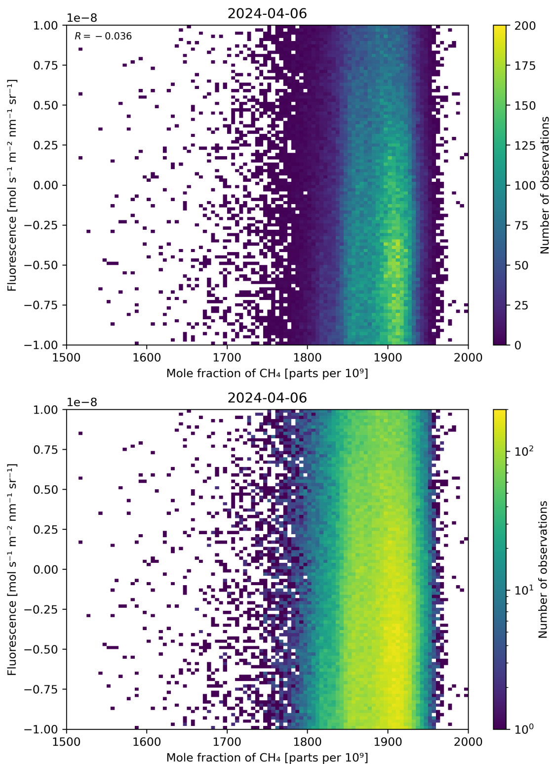
Figure 73: Scatter density plot of “Mole fraction of \text{CH}_4 ” against “Fluorescence” for 2024-04-05 to 2024-04-07.
