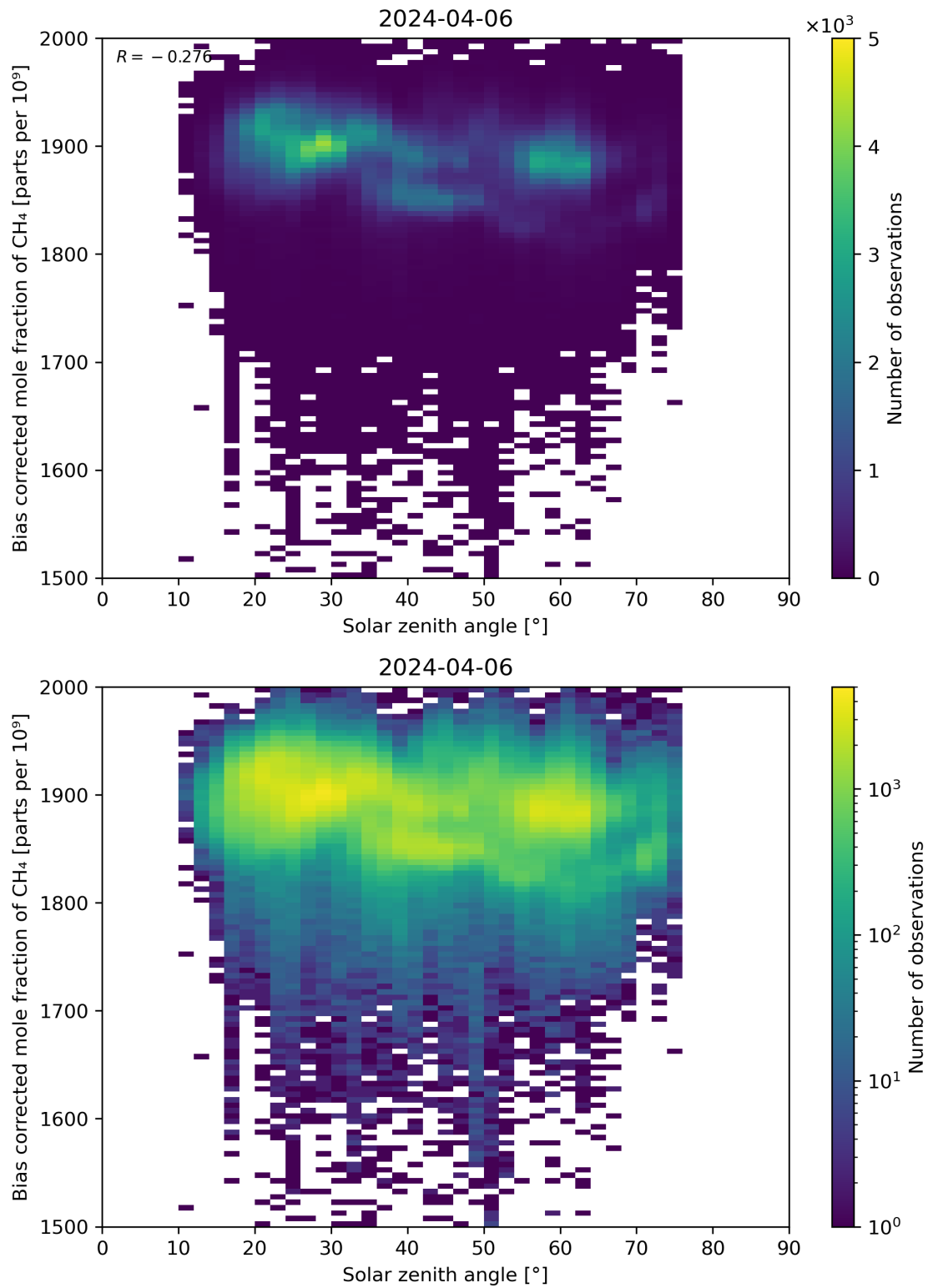
Figure 100: Scatter density plot of “Solar zenith angle” against “Bias corrected mole fraction of CH 4 ” for 2024-04-05 to 2024-04-07.
