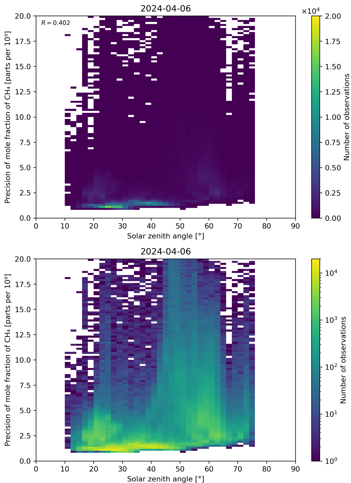
Figure 101: Scatter density plot of “Solar zenith angle” against “Precision of mole fraction of CH 4 ” for 2024-04-05 to 2024-04-07.
