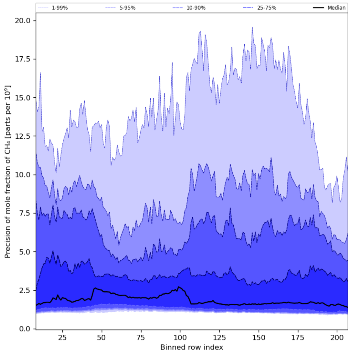
Figure 35: Along track statistics of “Precision of mole fraction of CH 4 ” for 2024-04-05 to 2024-04-07
