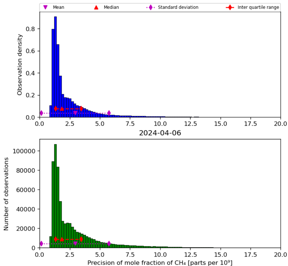
Figure 24: Histogram of “Precision of mole fraction of CH 4 ” for 2024-04-05 to 2024-04-07
