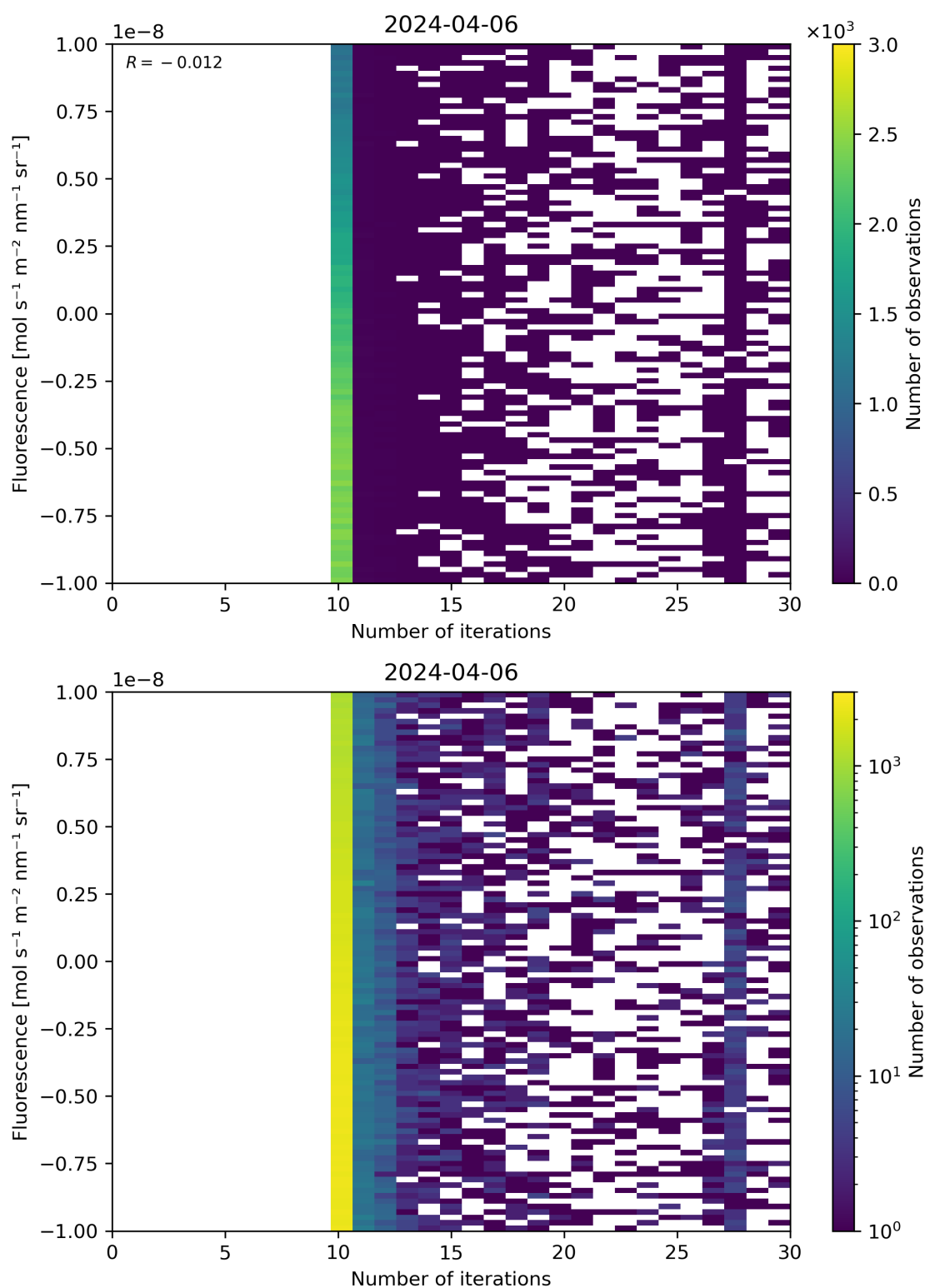
Figure 87: Scatter density plot of “Number of iterations” against “Fluorescence” for 2024-04-05 to 2024-04-07.
