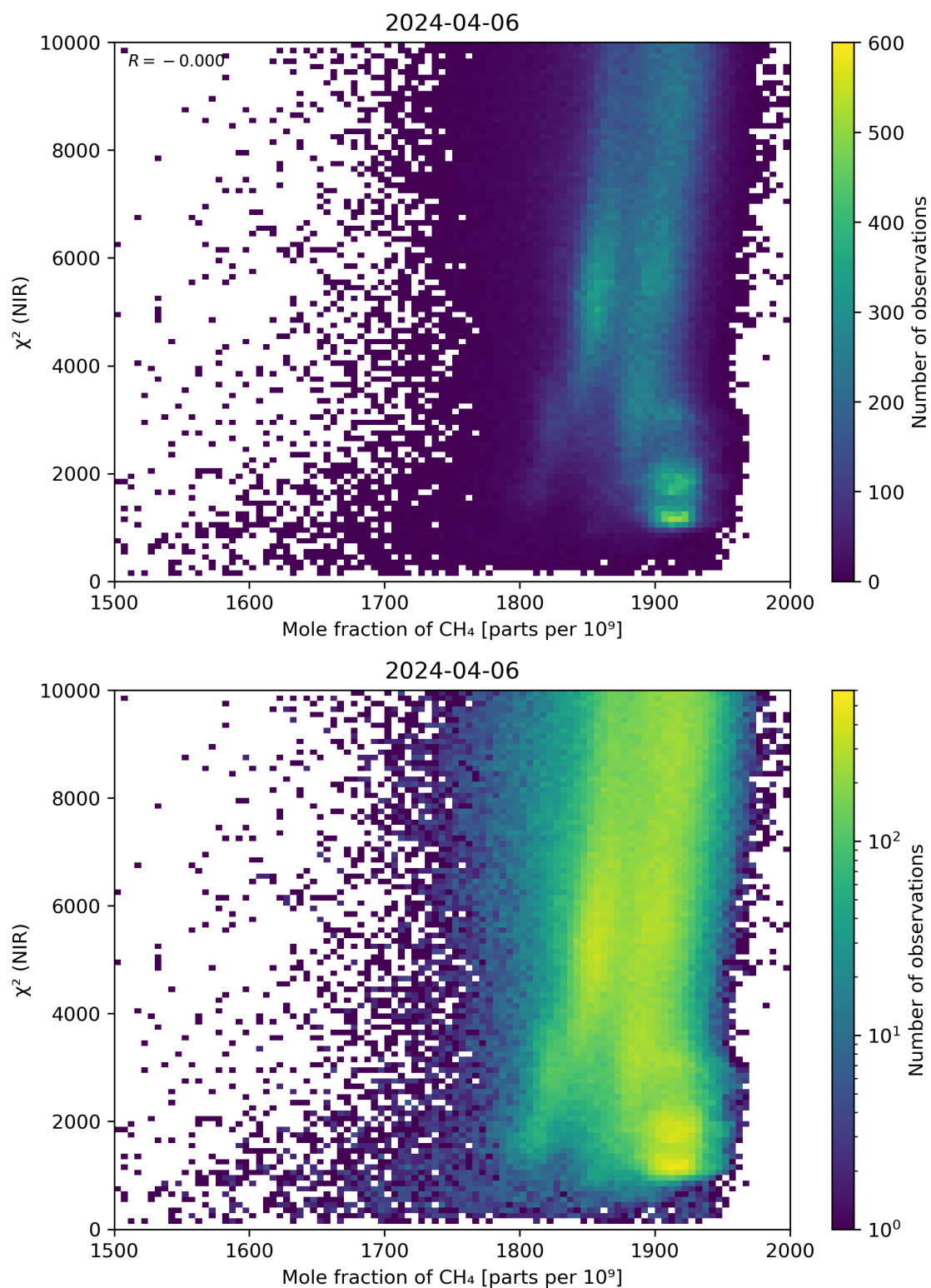
Figure 70: Scatter density plot of “Mole fraction of CH 4 ” against “ \chi^2 (NIR)” for 2024-04-05 to 2024-04-07.
