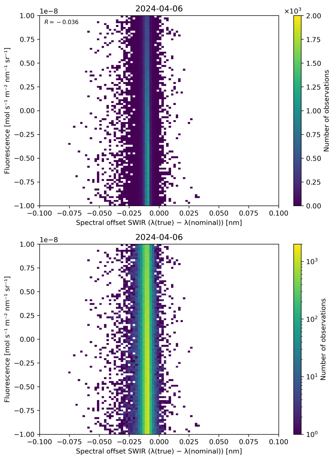
Figure 120: Scatter density plot of “Spectral offset SWIR ( \lambda(\text{true}) - \lambda(\text{nominal}) )” against “Fluorescence” for 2024-04-05 to 2024-04-07.
