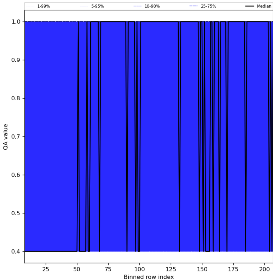
Figure 33: Along track statistics of “QA value” for 2024-04-05 to 2024-04-07
