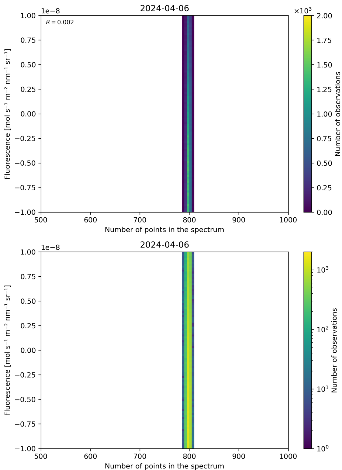
Figure 91: Scatter density plot of “Number of points in the spectrum” against “Fluorescence” for 2024-04-05 to 2024-04-07.
