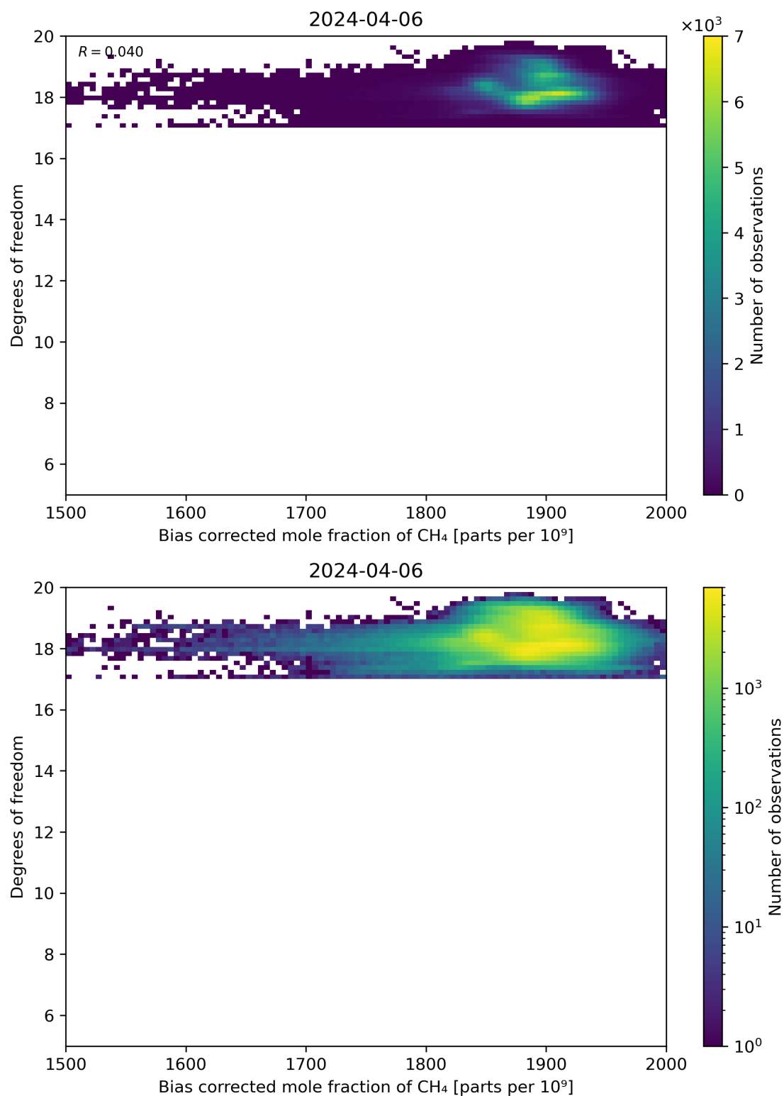
Figure 65: Scatter density plot of “Bias corrected mole fraction of CH 4 ” against “Degrees of freedom” for 2024-04-05 to 2024-04-07.
