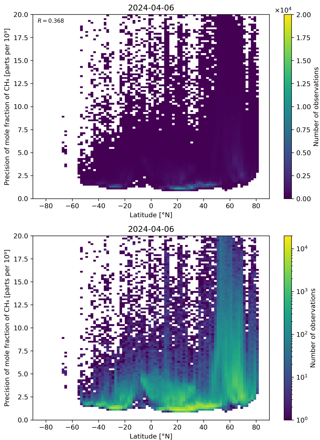
Figure 59: Scatter density plot of “Latitude” against “Precision of mole fraction of \text{CH}_4 ” for 2024-04-05 to 2024-04-07.
