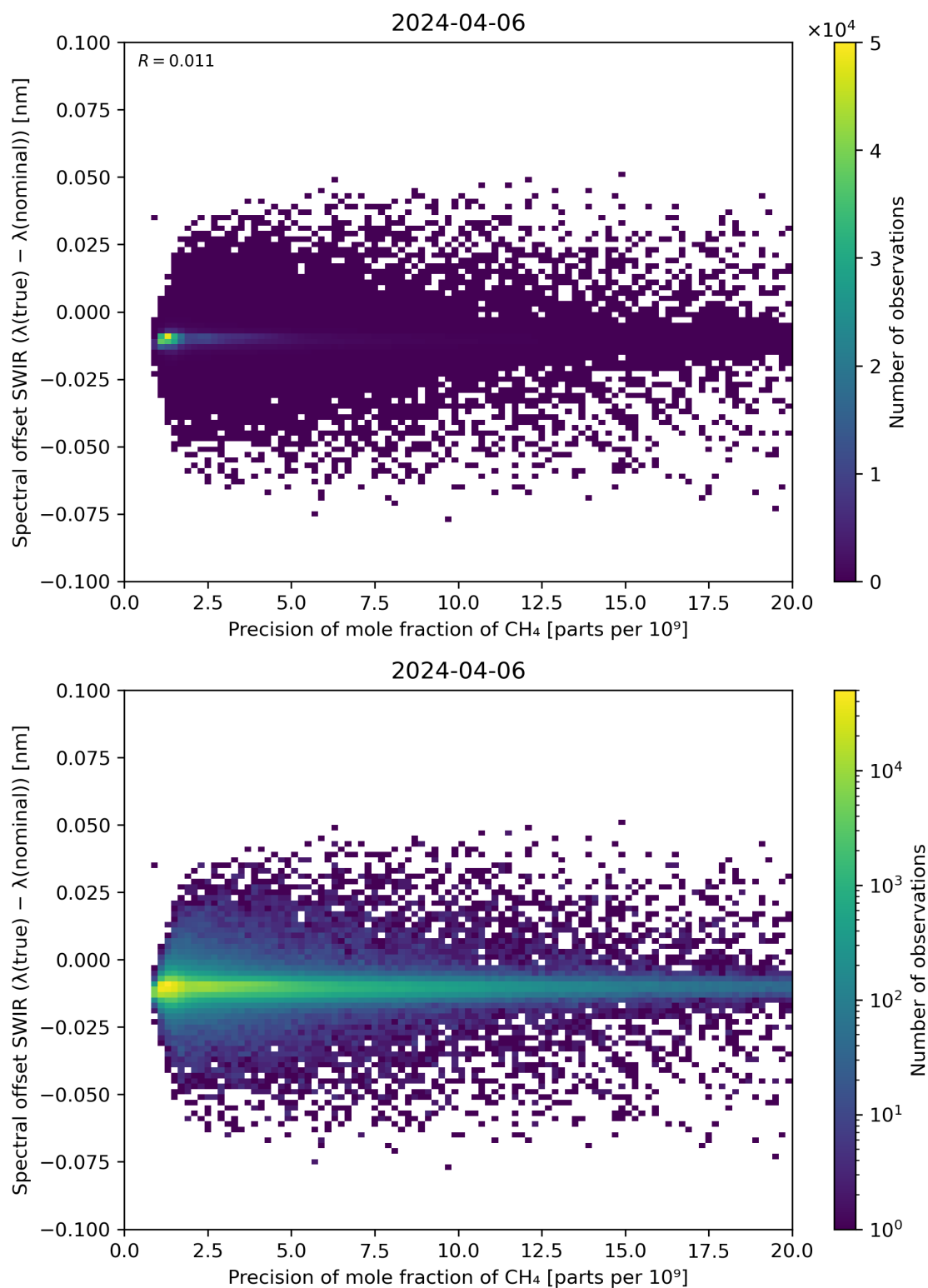
Figure 85: Scatter density plot of “Precision of mole fraction of CH 4 ” against “Spectral offset SWIR ( \lambda(\text{true}) - \lambda(\text{nominal}) )” for 2024-04-05 to 2024-04-07.
