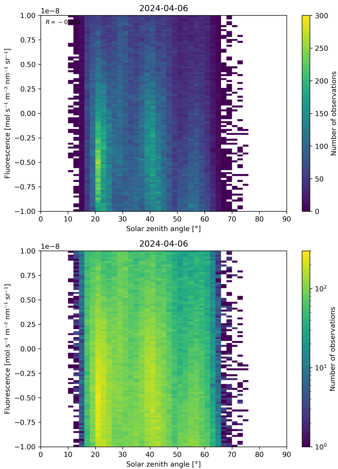
Figure 97: Scatter density plot of “Solar zenith angle” against “Fluorescence” for 2024-04-05 to 2024-04-07.
