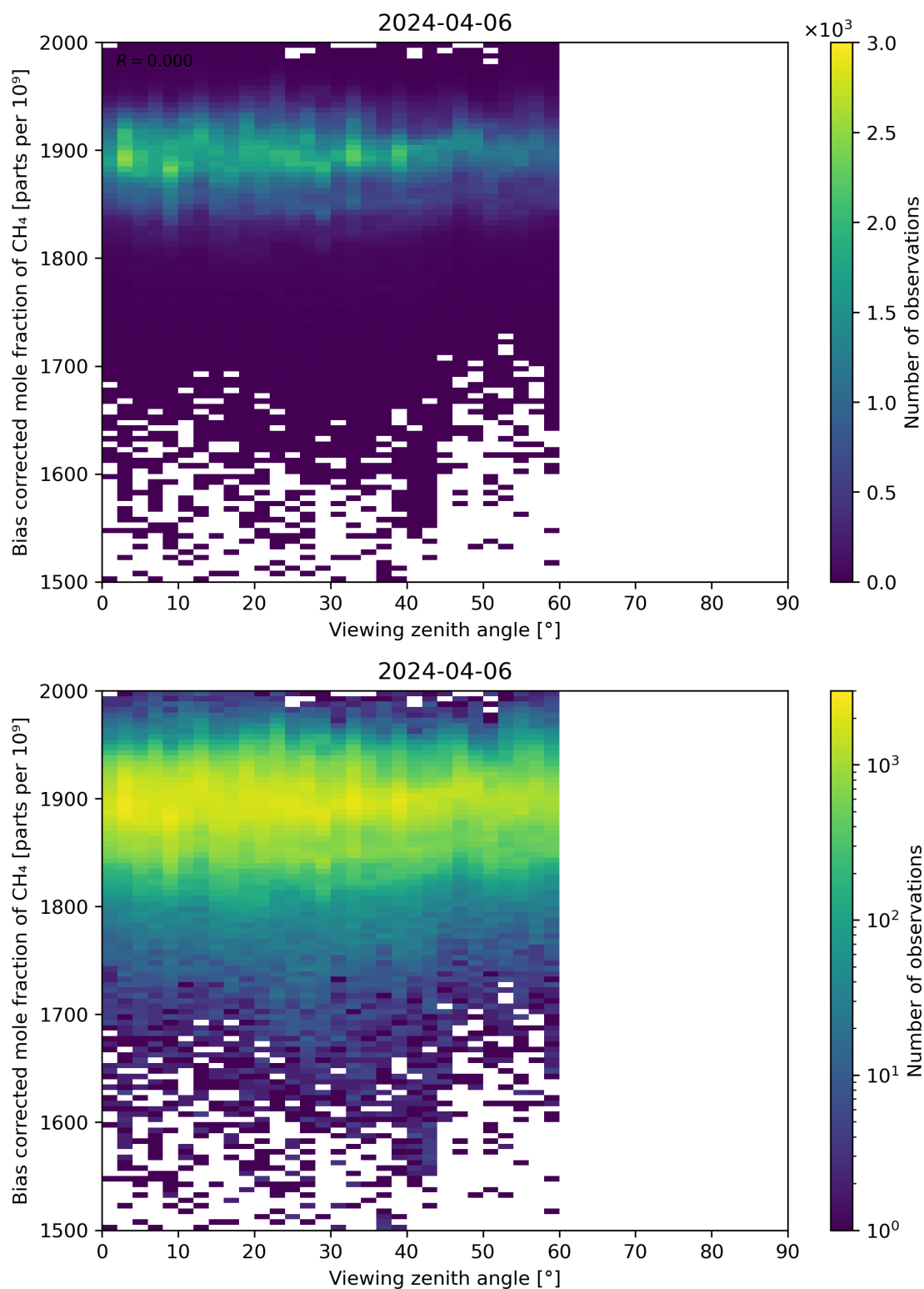
Figure 111: Scatter density plot of “Viewing zenith angle” against “Bias corrected mole fraction of CH 4 ” for 2024-04-05 to 2024-04-07.
