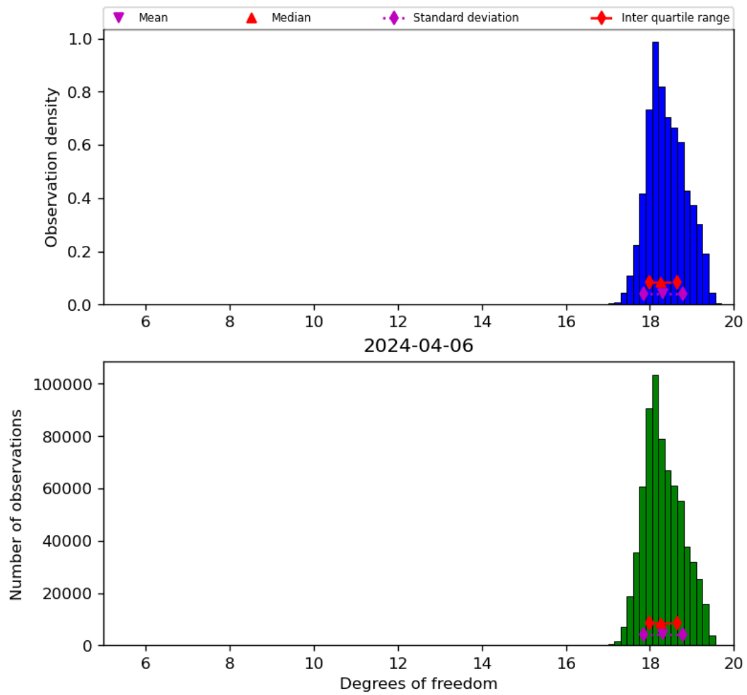
Figure 30: Histogram of “Degrees of freedom” for 2024-04-05 to 2024-04-07
