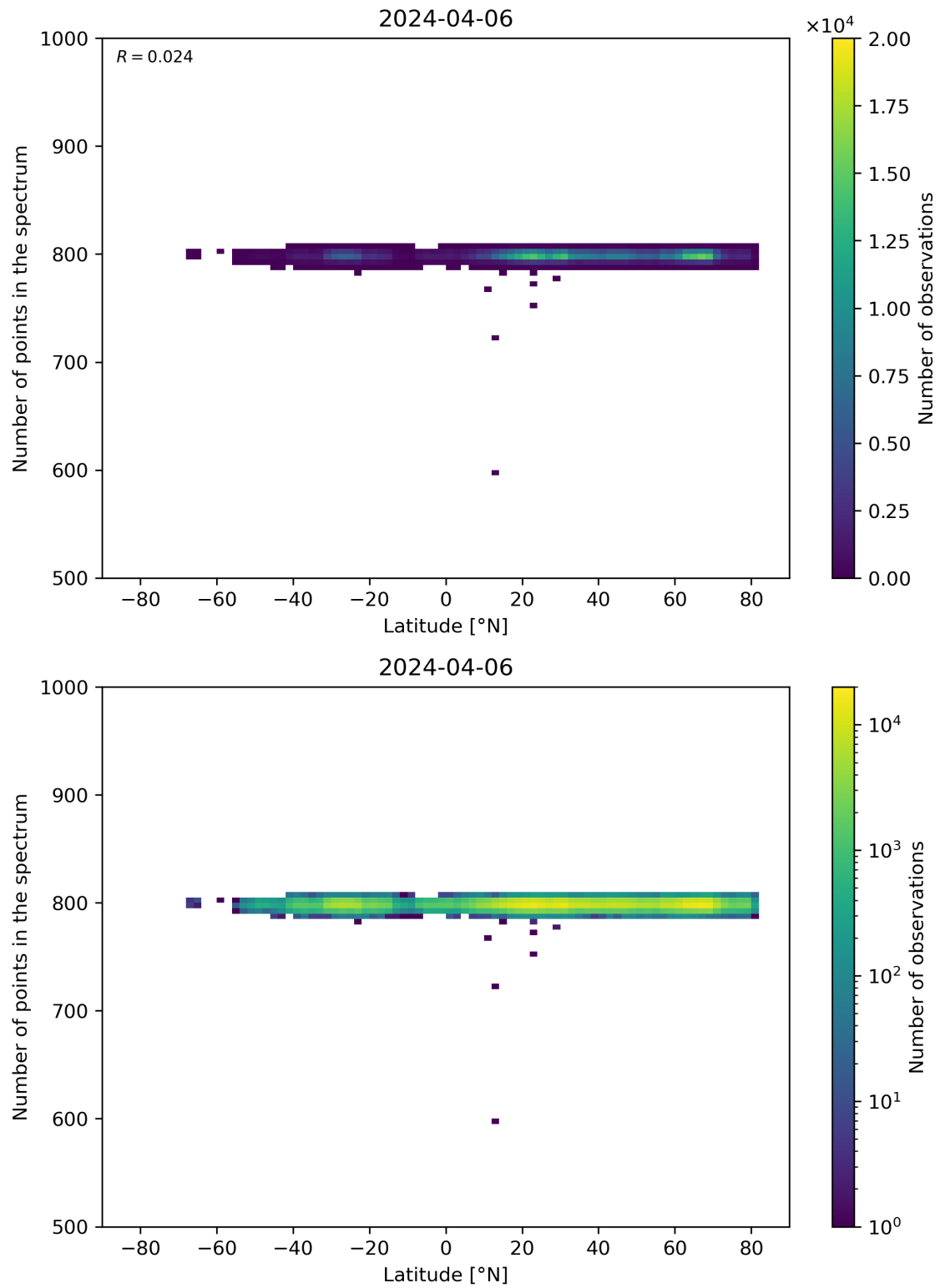
Figure 61: Scatter density plot of “Latitude” against “Number of points in the spectrum” for 2024-04-05 to 2024-04-07.
