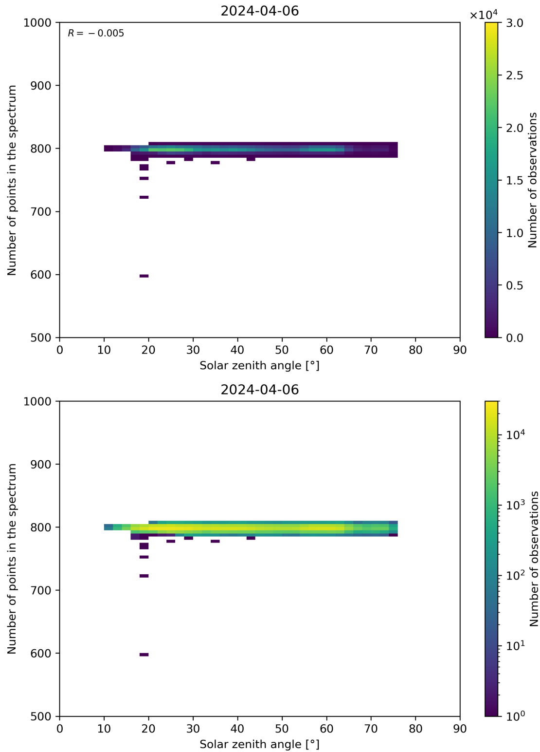
Figure 103: Scatter density plot of “Solar zenith angle” against “Number of points in the spectrum” for 2024-04-05 to 2024-04-07.
