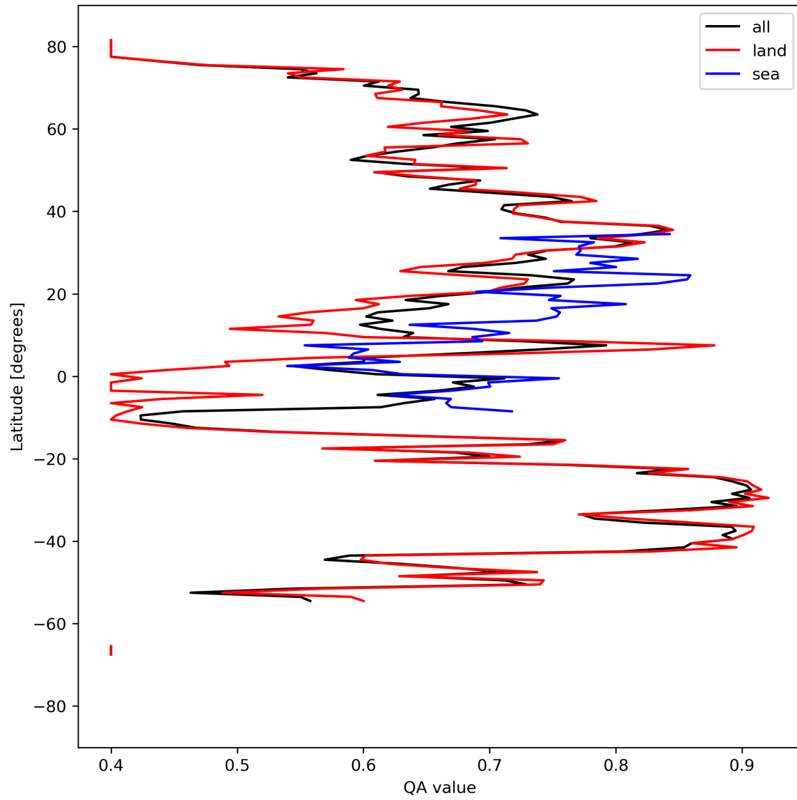
Figure 11: Zonal average of “QA value” for 2024-04-05 to 2024-04-07.
