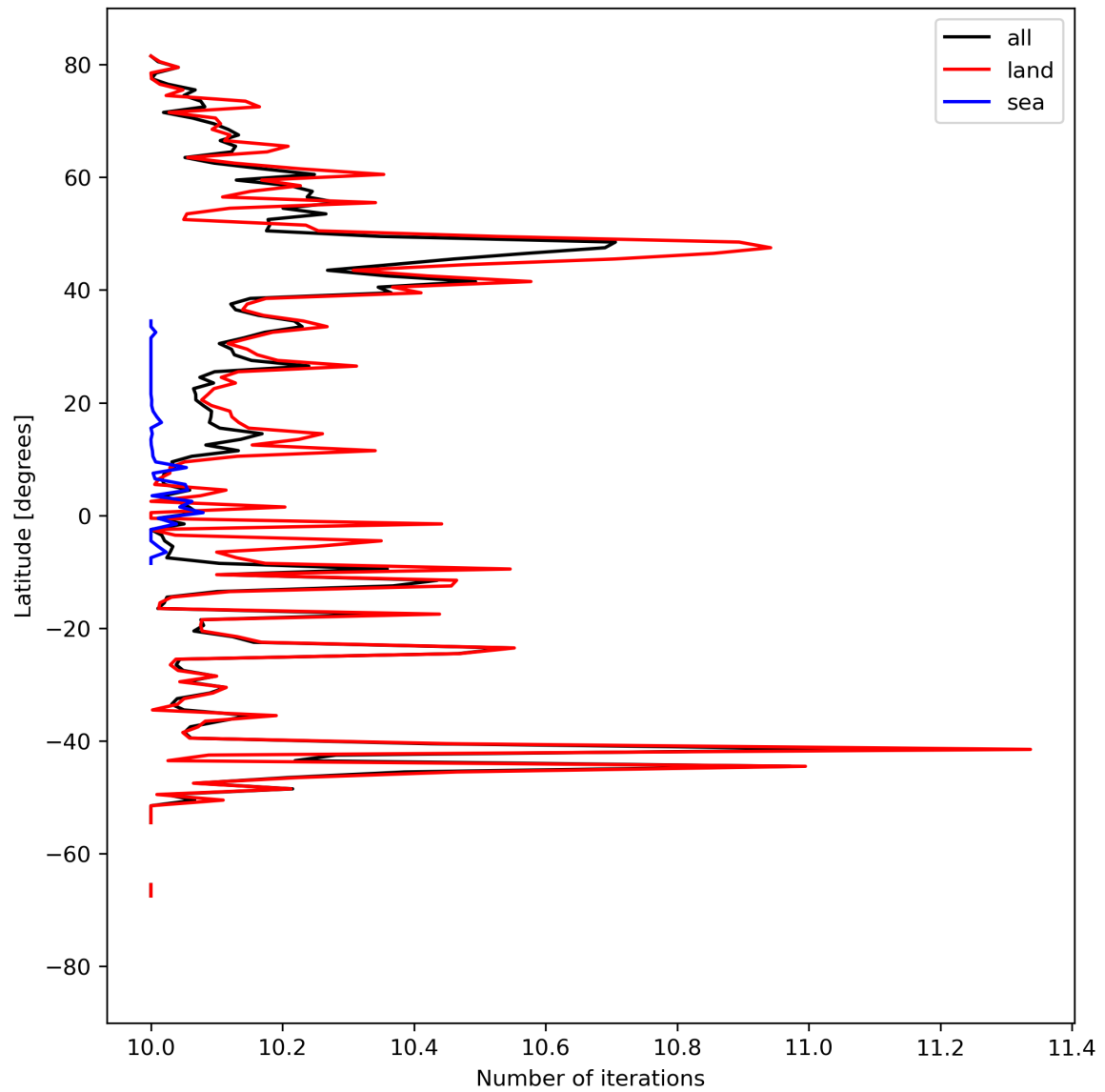
Figure 20: Zonal average of “Number of iterations” for 2024-04-05 to 2024-04-07.
