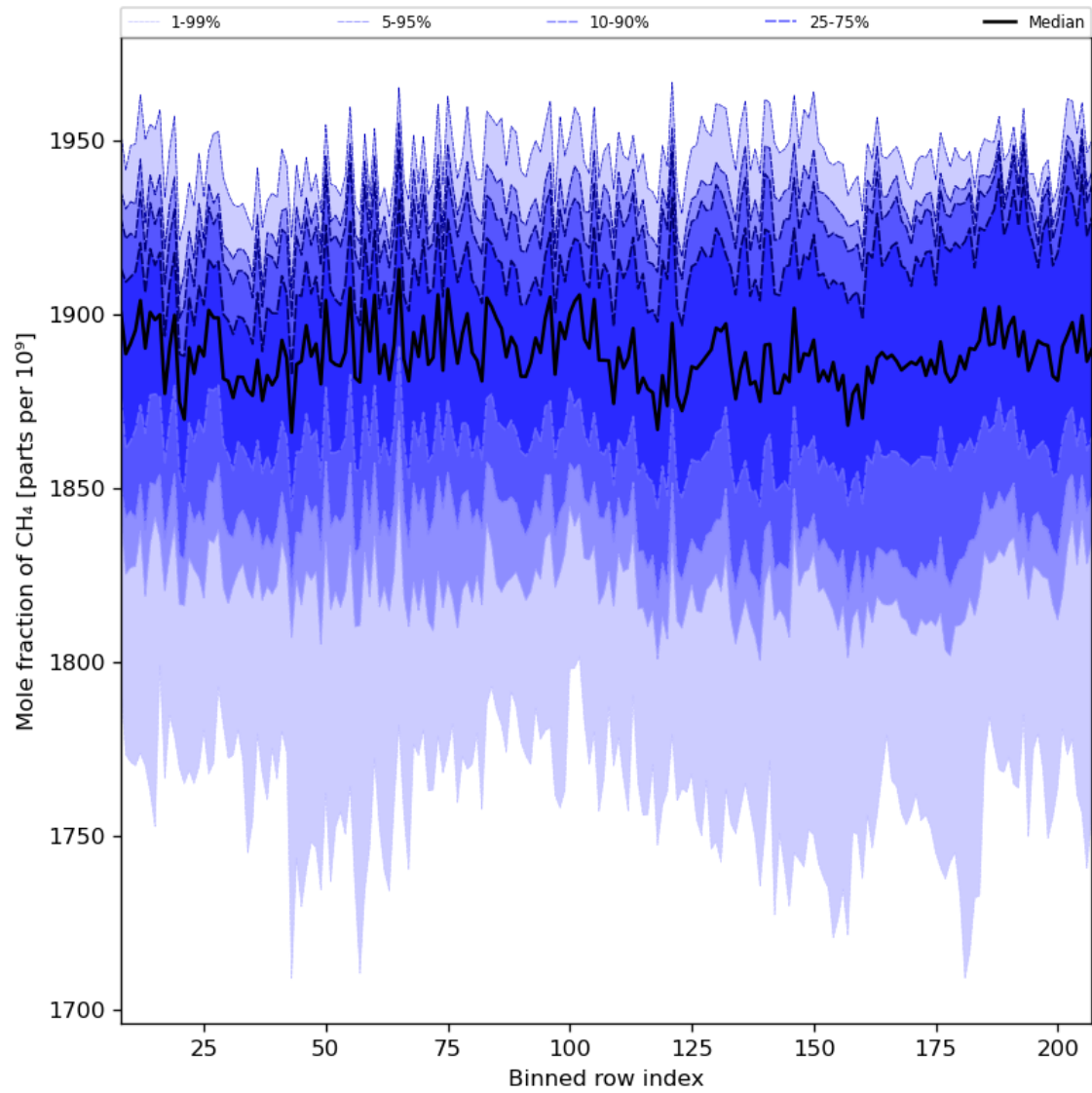
Figure 34: Along track statistics of “Mole fraction of CH 4 ” for 2024-04-05 to 2024-04-07
