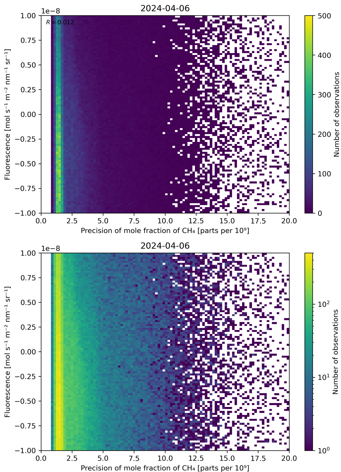
Figure 81: Scatter density plot of “Precision of mole fraction of \text{CH}_4 ” against “Fluorescence” for 2024-04-05 to 2024-04-07.
