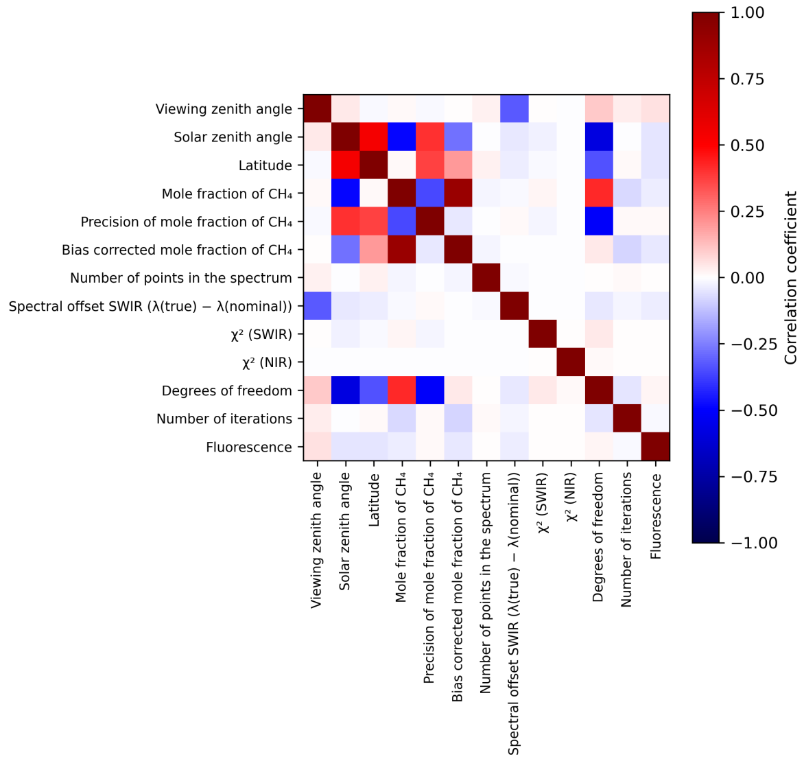
Figure 2: Map of correlation matrix for 2024-04-05 to 2024-04-07.
