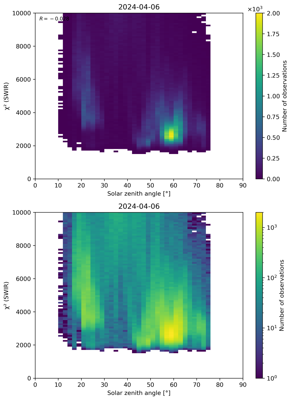
Figure 95: Scatter density plot of “Solar zenith angle” against “ \chi^2 (SWIR)” for 2024-04-05 to 2024-04-07.
