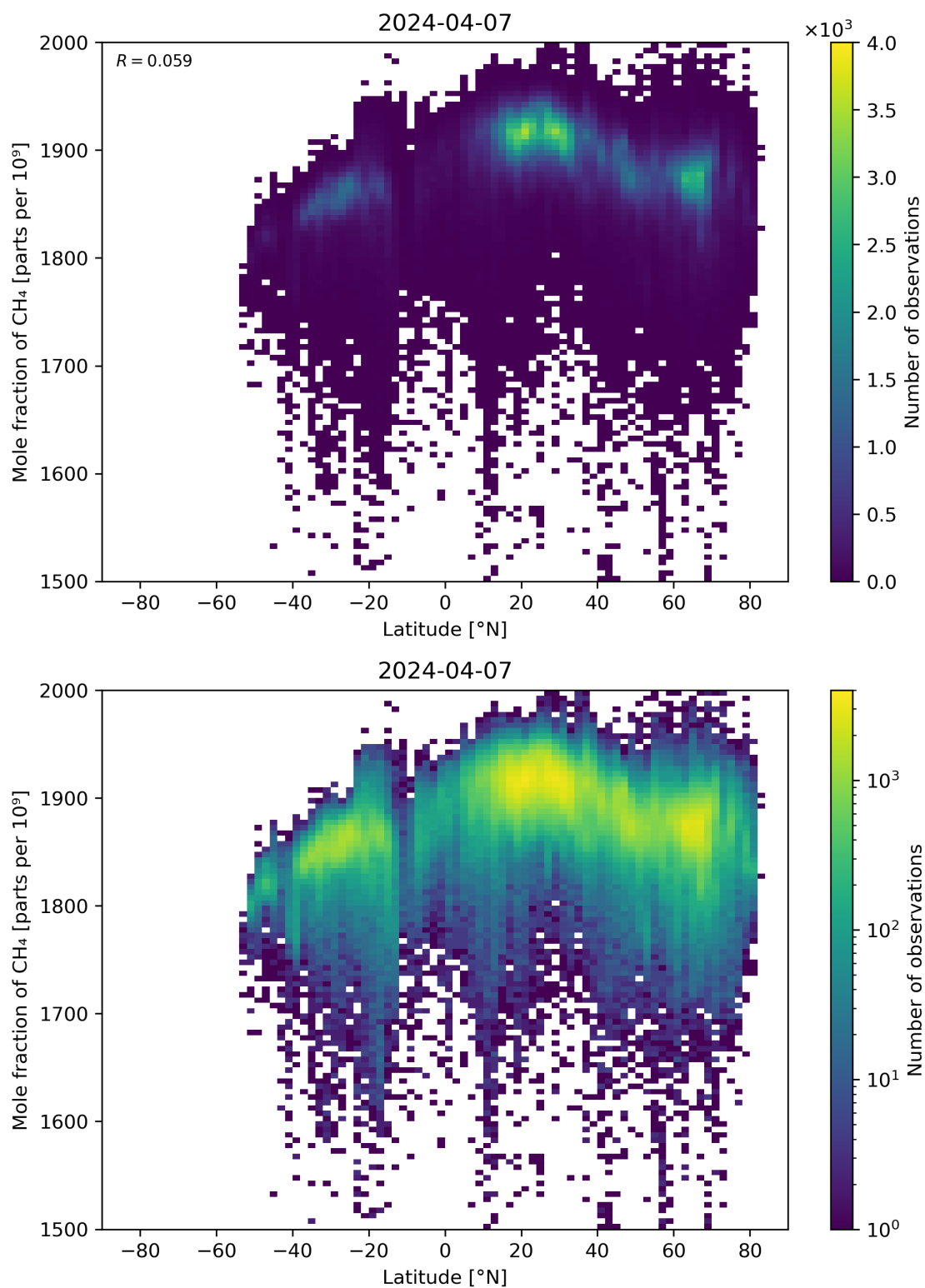
Figure 57: Scatter density plot of “Latitude” against “Mole fraction of \text{CH}_4 ” for 2024-04-06 to 2024-04-08.
