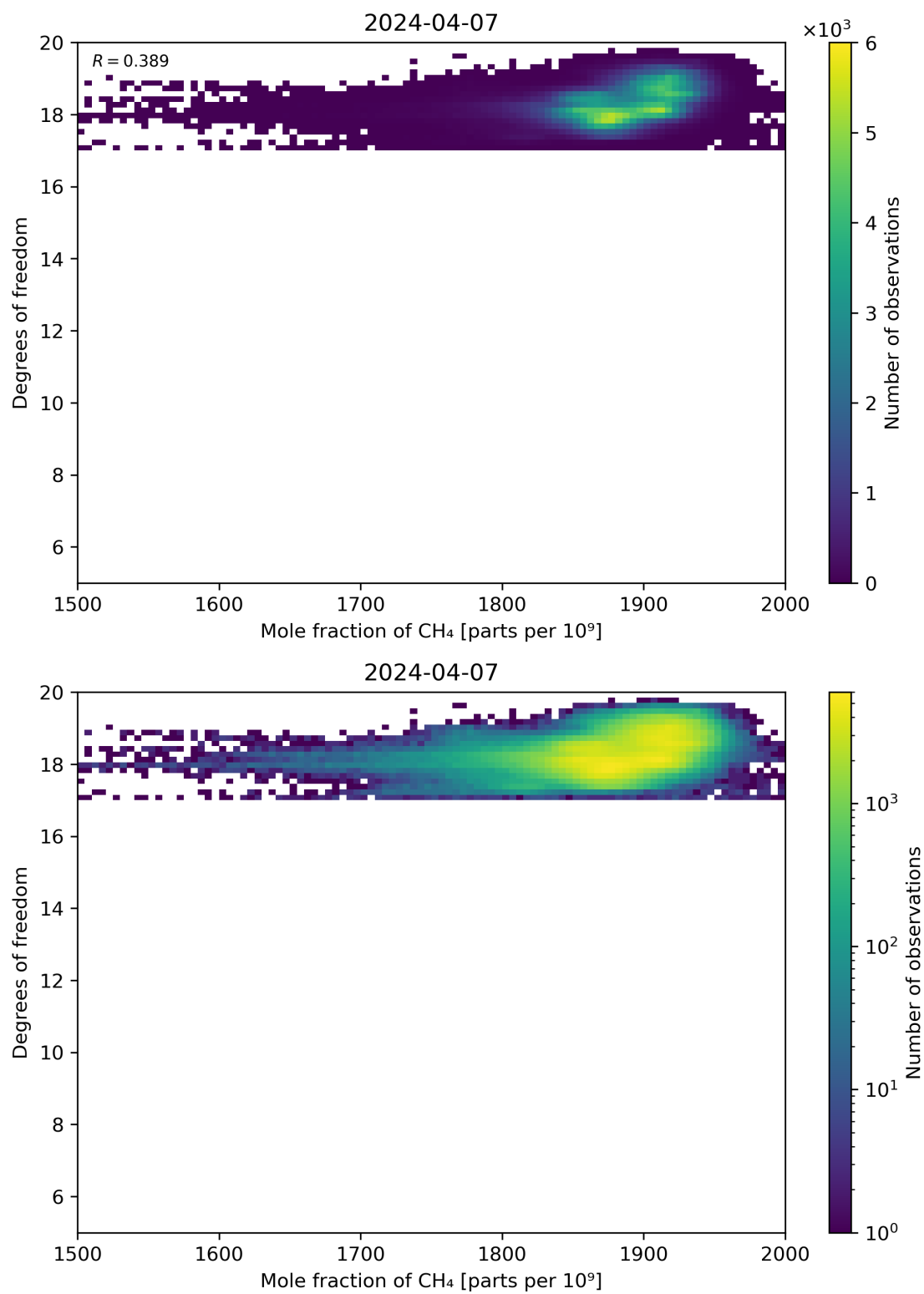
Figure 72: Scatter density plot of “Mole fraction of CH 4 ” against “Degrees of freedom” for 2024-04-06 to 2024-04-08.
