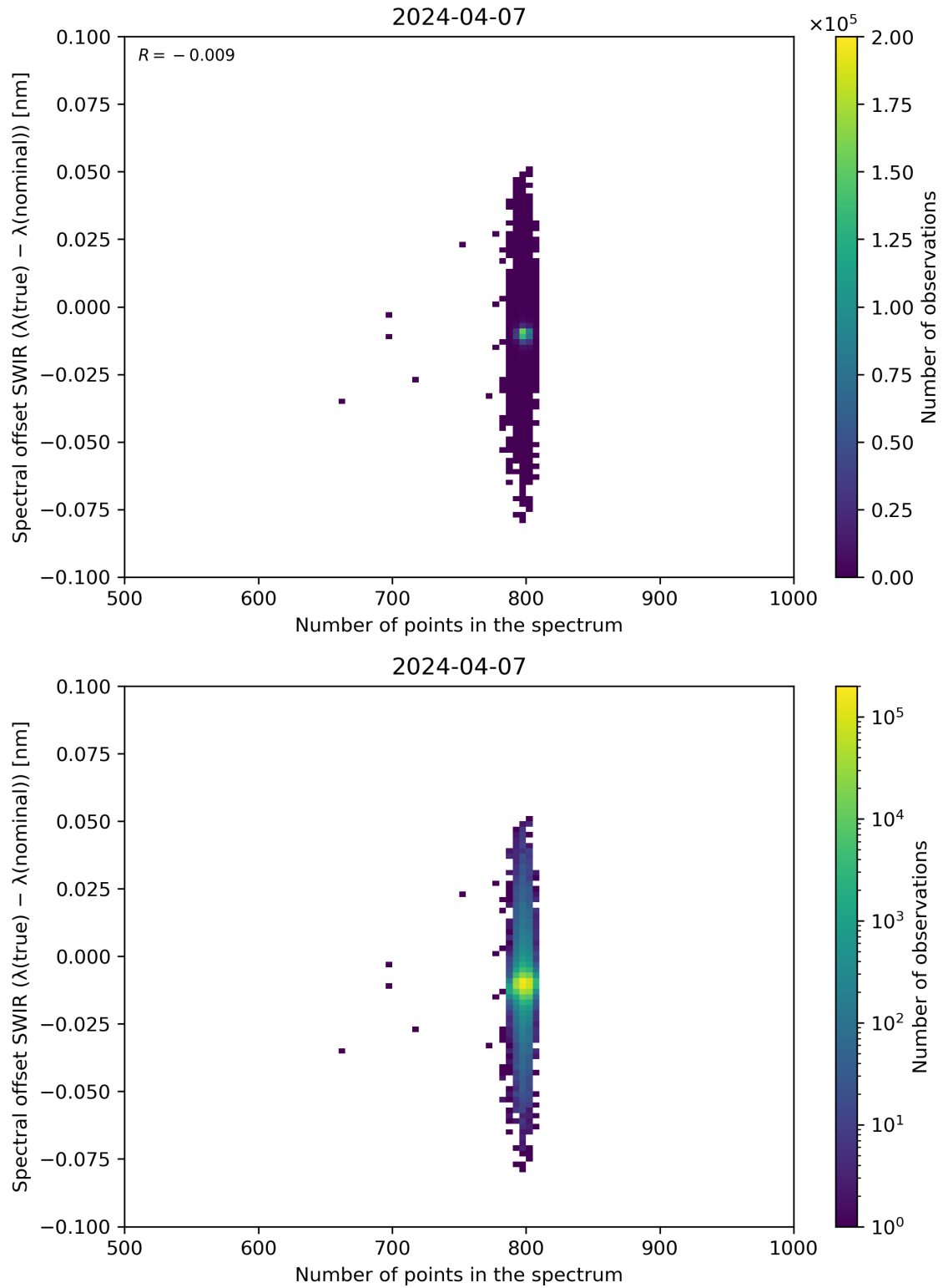
Figure 93: Scatter density plot of “Number of points in the spectrum” against “Spectral offset SWIR ( \lambda(\text{true}) - \lambda(\text{nominal}) )” for 2024-04-06 to 2024-04-08.
