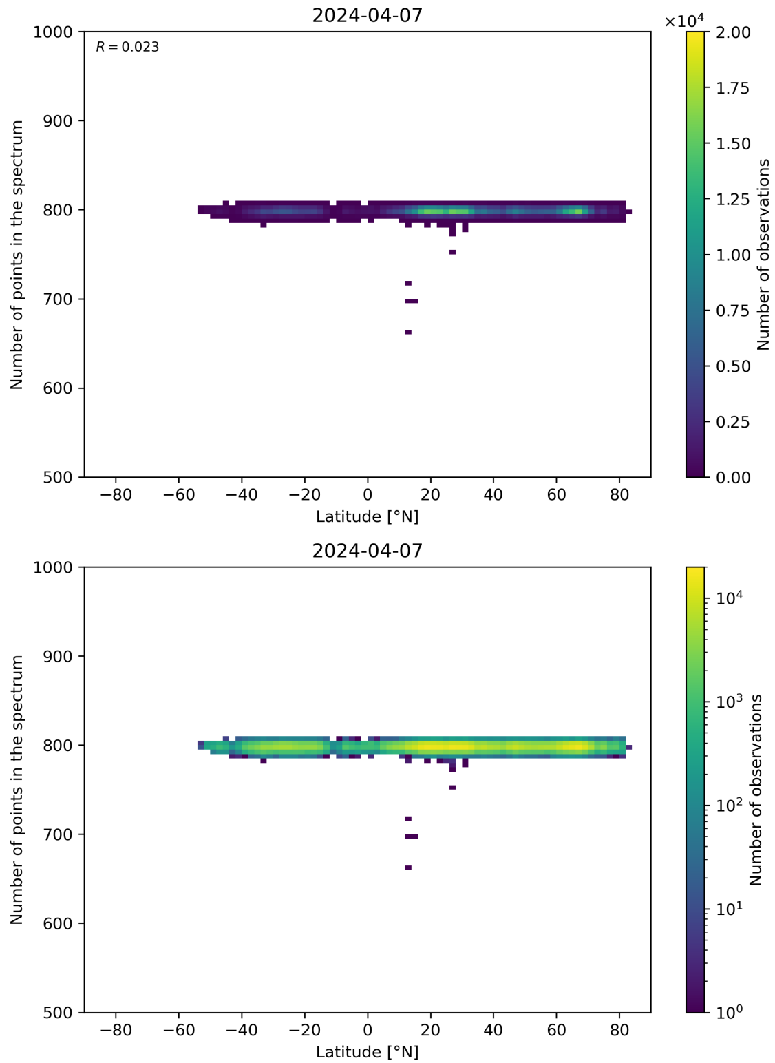
Figure 61: Scatter density plot of “Latitude” against “Number of points in the spectrum” for 2024-04-06 to 2024-04-08.
