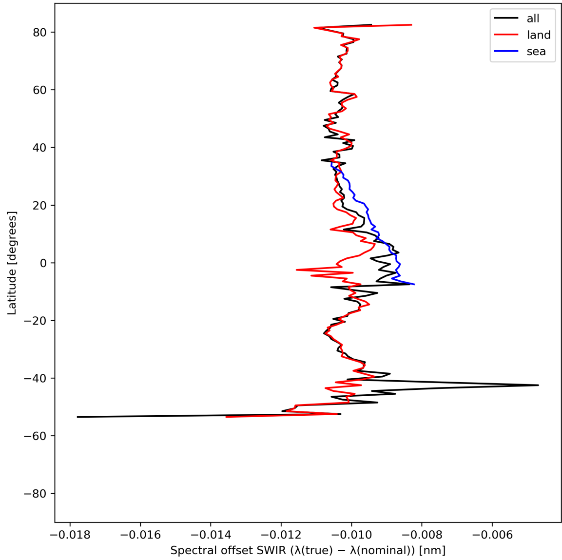
Figure 16: Zonal average of “Spectral offset SWIR ( \lambda(\text{true}) - \lambda(\text{nominal}) )” for 2024-04-06 to 2024-04-08.
