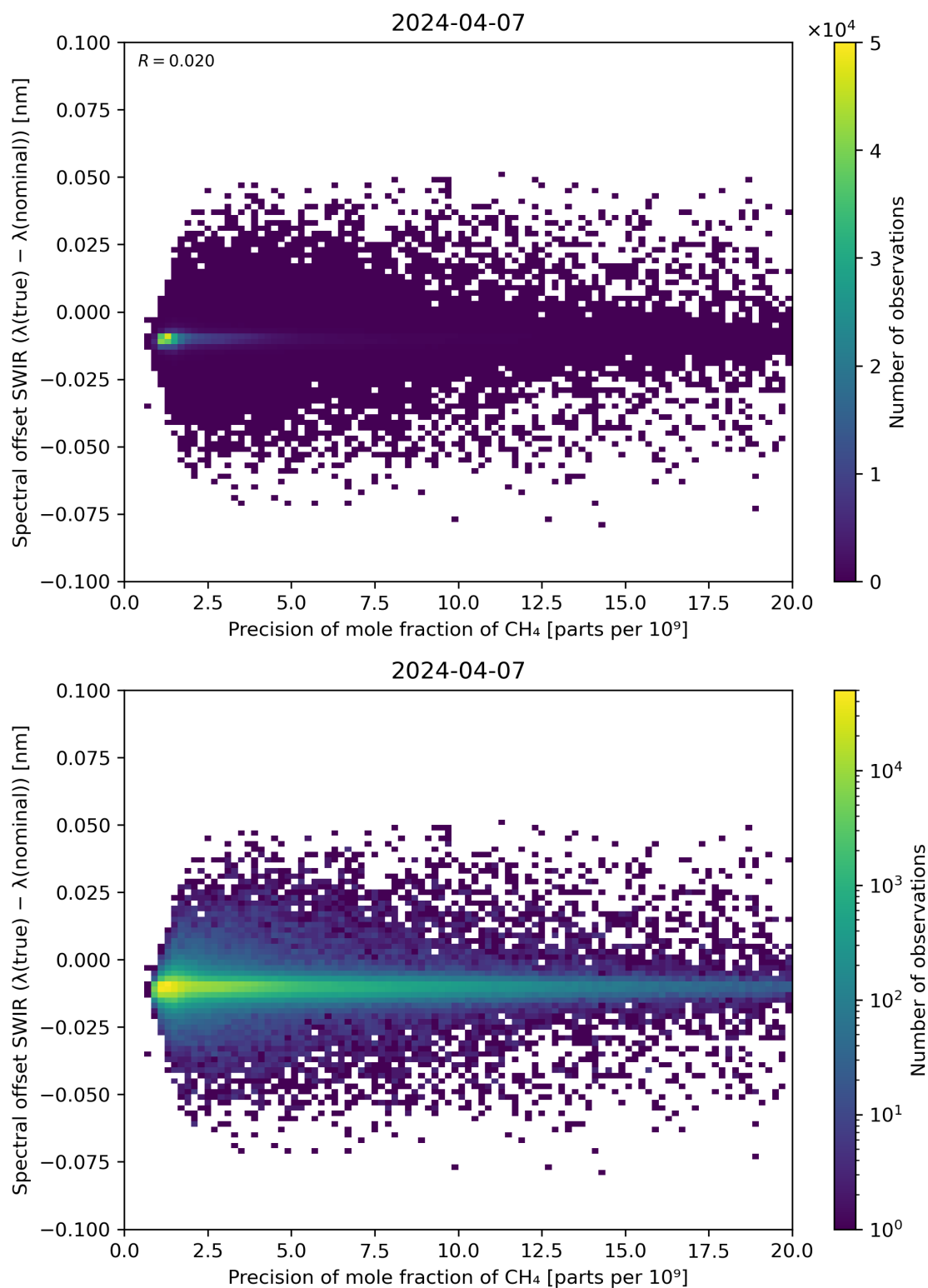
Figure 85: Scatter density plot of “Precision of mole fraction of CH 4 ” against “Spectral offset SWIR ( \lambda(\text{true}) - \lambda(\text{nominal}) )” for 2024-04-06 to 2024-04-08.
