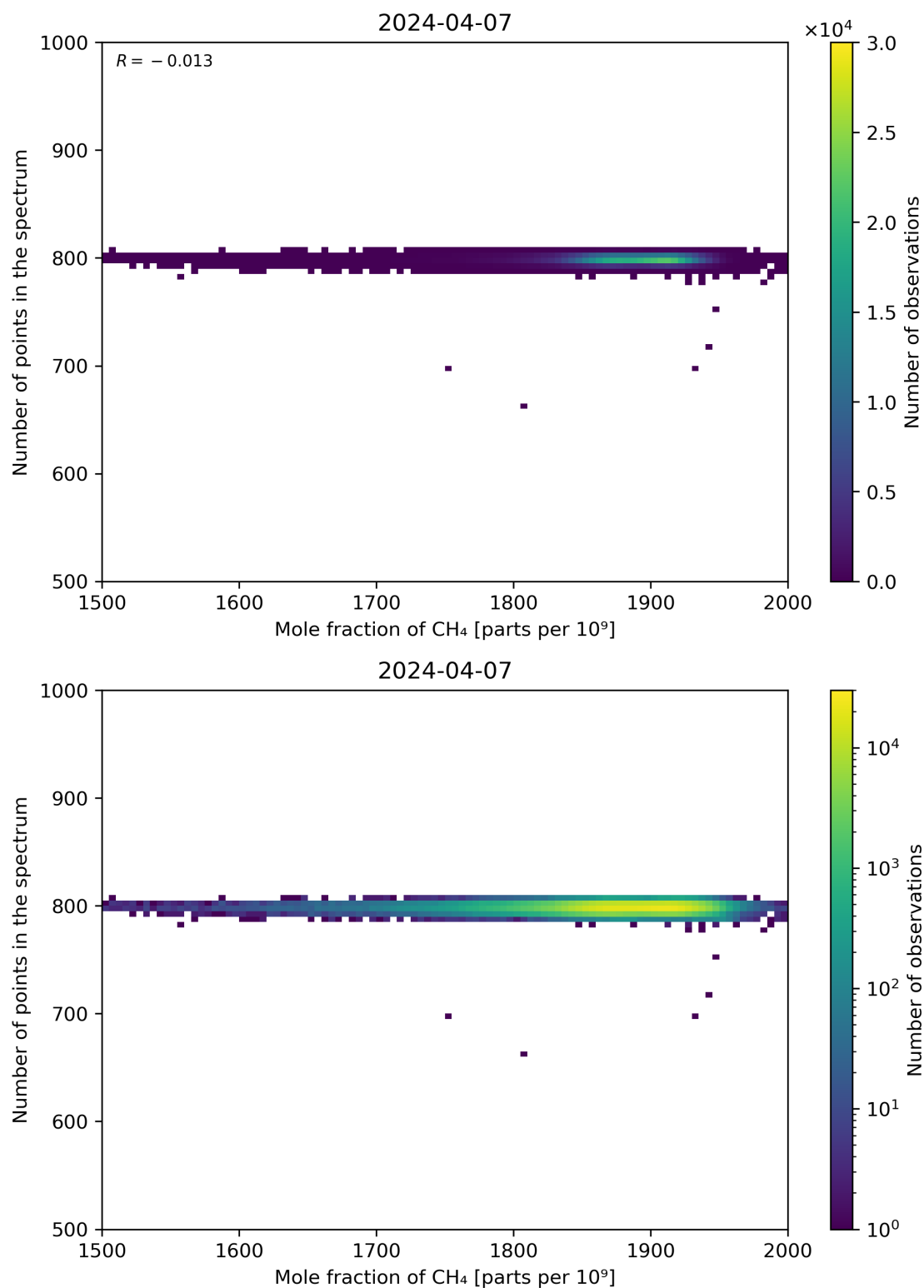
Figure 77: Scatter density plot of “Mole fraction of CH 4 ” against “Number of points in the spectrum” for 2024-04-06 to 2024-04-08.
