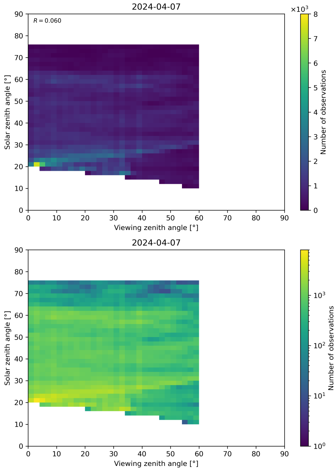
Figure 115: Scatter density plot of “Viewing zenith angle” against “Solar zenith angle” for 2024-04-06 to 2024-04-08.
