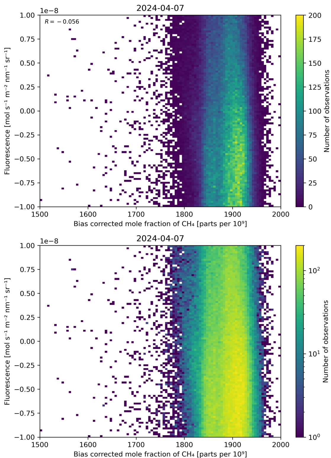
Figure 66: Scatter density plot of “Bias corrected mole fraction of \text{CH}_4 ” against “Fluorescence” for 2024-04-06 to 2024-04-08.
