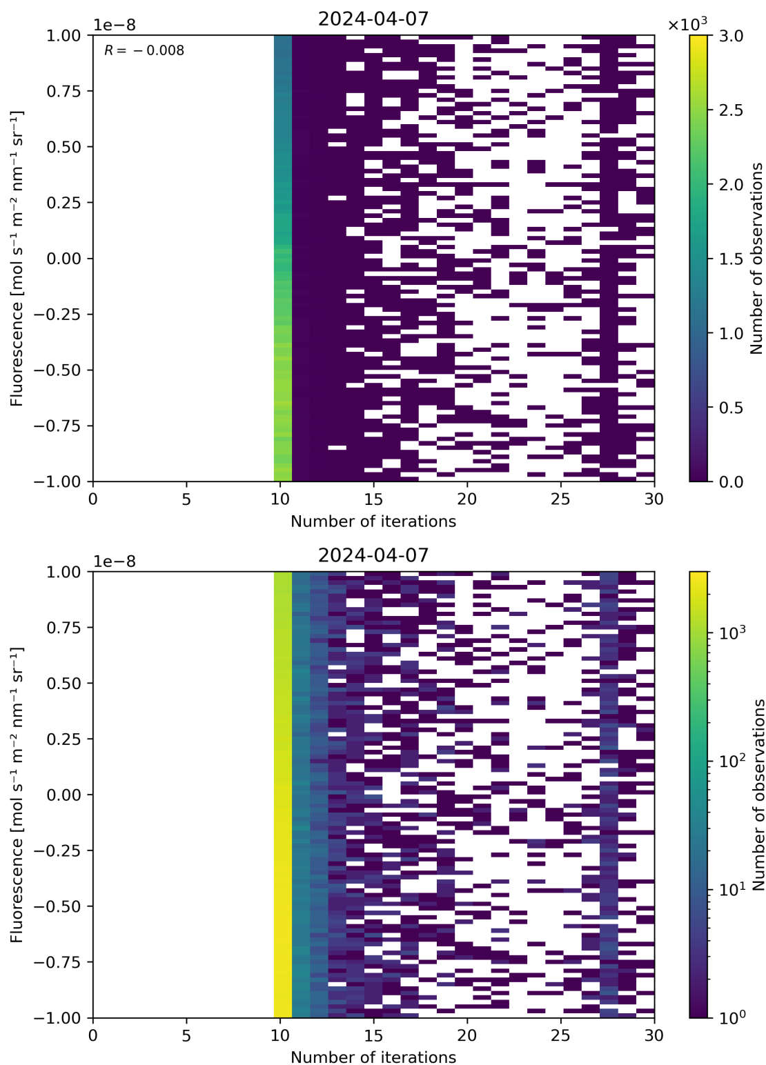
Figure 87: Scatter density plot of “Number of iterations” against “Fluorescence” for 2024-04-06 to 2024-04-08.
