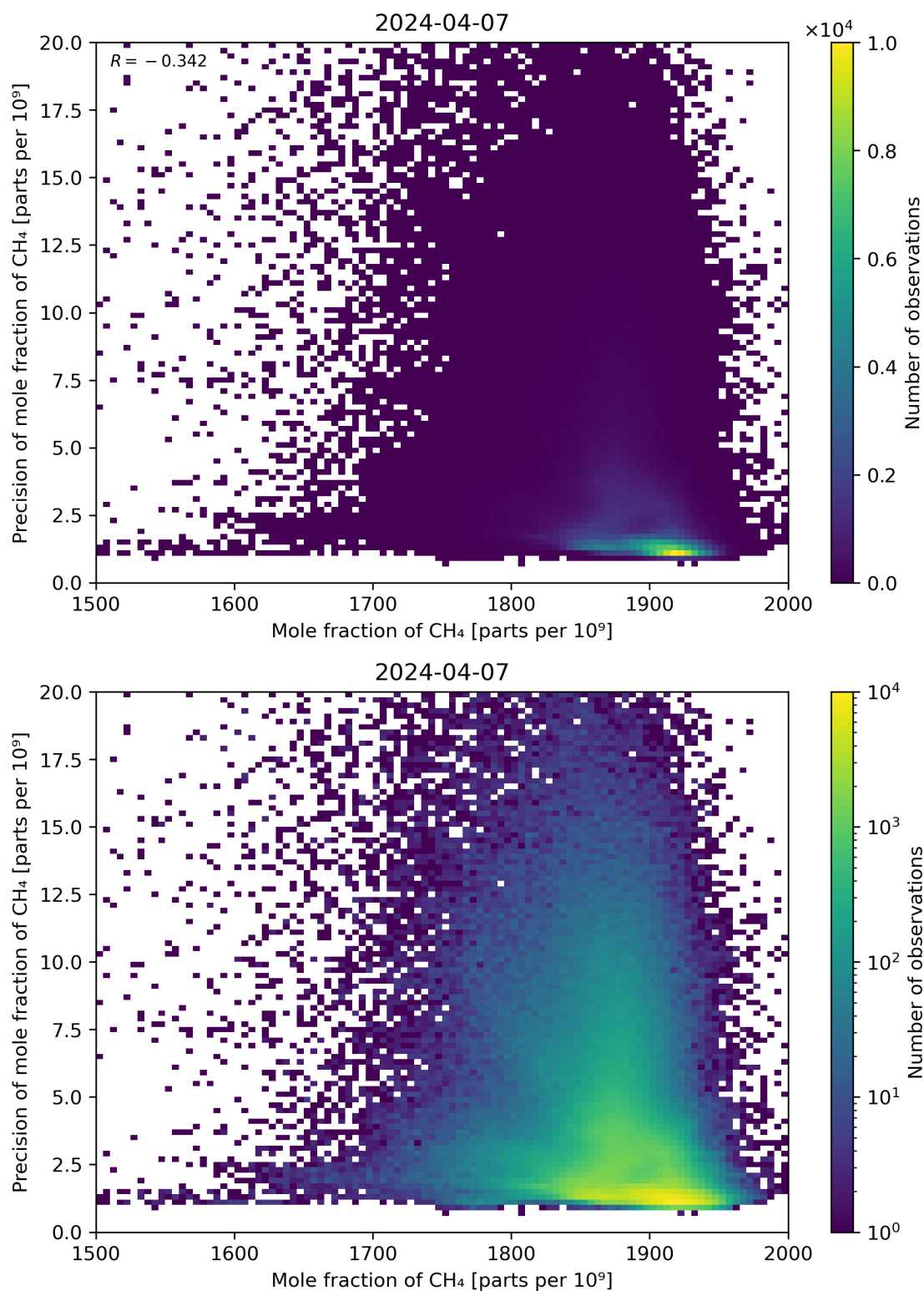
Figure 75: Scatter density plot of “Mole fraction of CH 4 ” against “Precision of mole fraction of CH 4 ” for 2024-04-06 to 2024-04-08.
