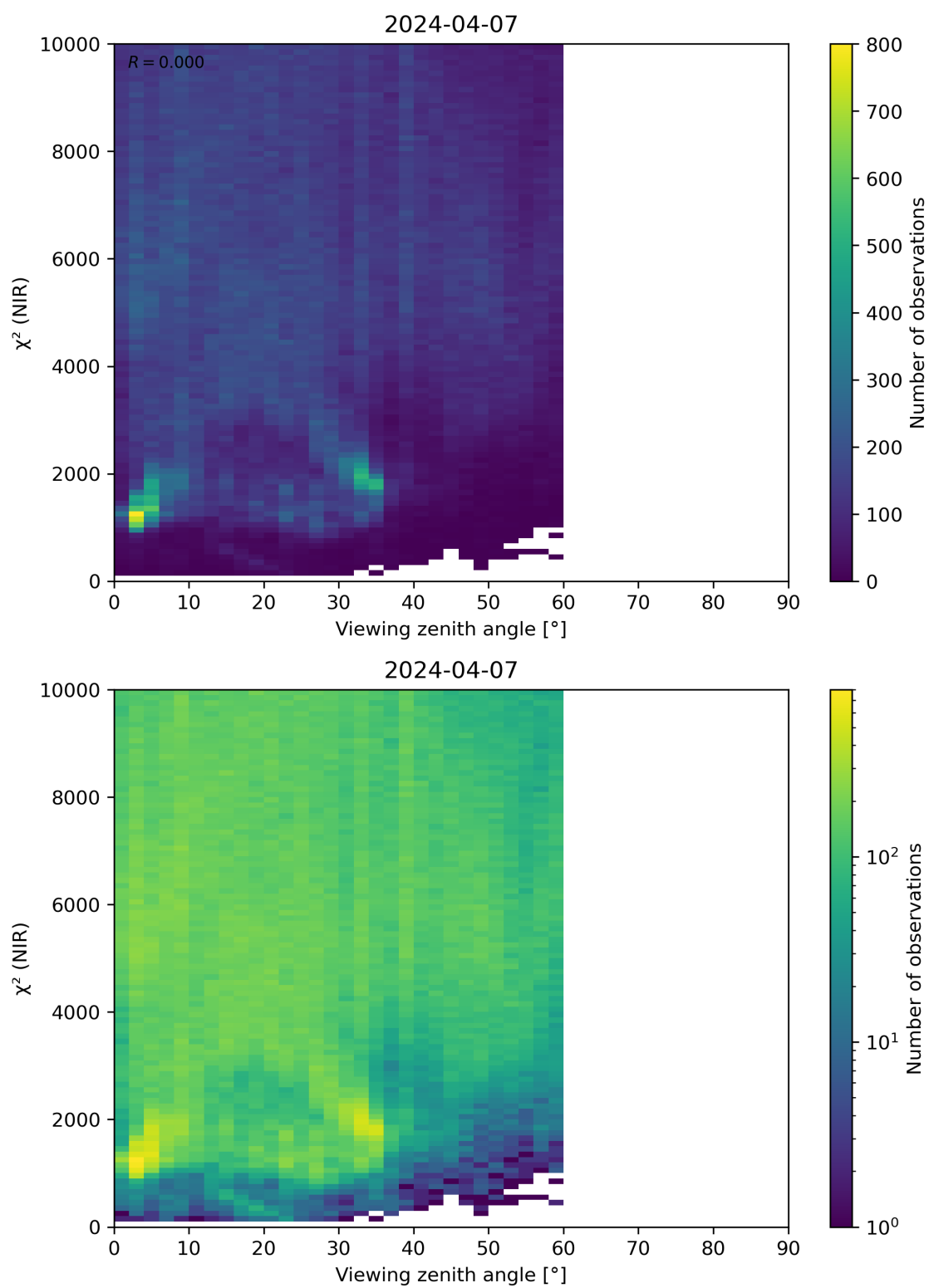
Figure 105: Scatter density plot of “Viewing zenith angle” against “ \chi^2 (NIR)” for 2024-04-06 to 2024-04-08.
