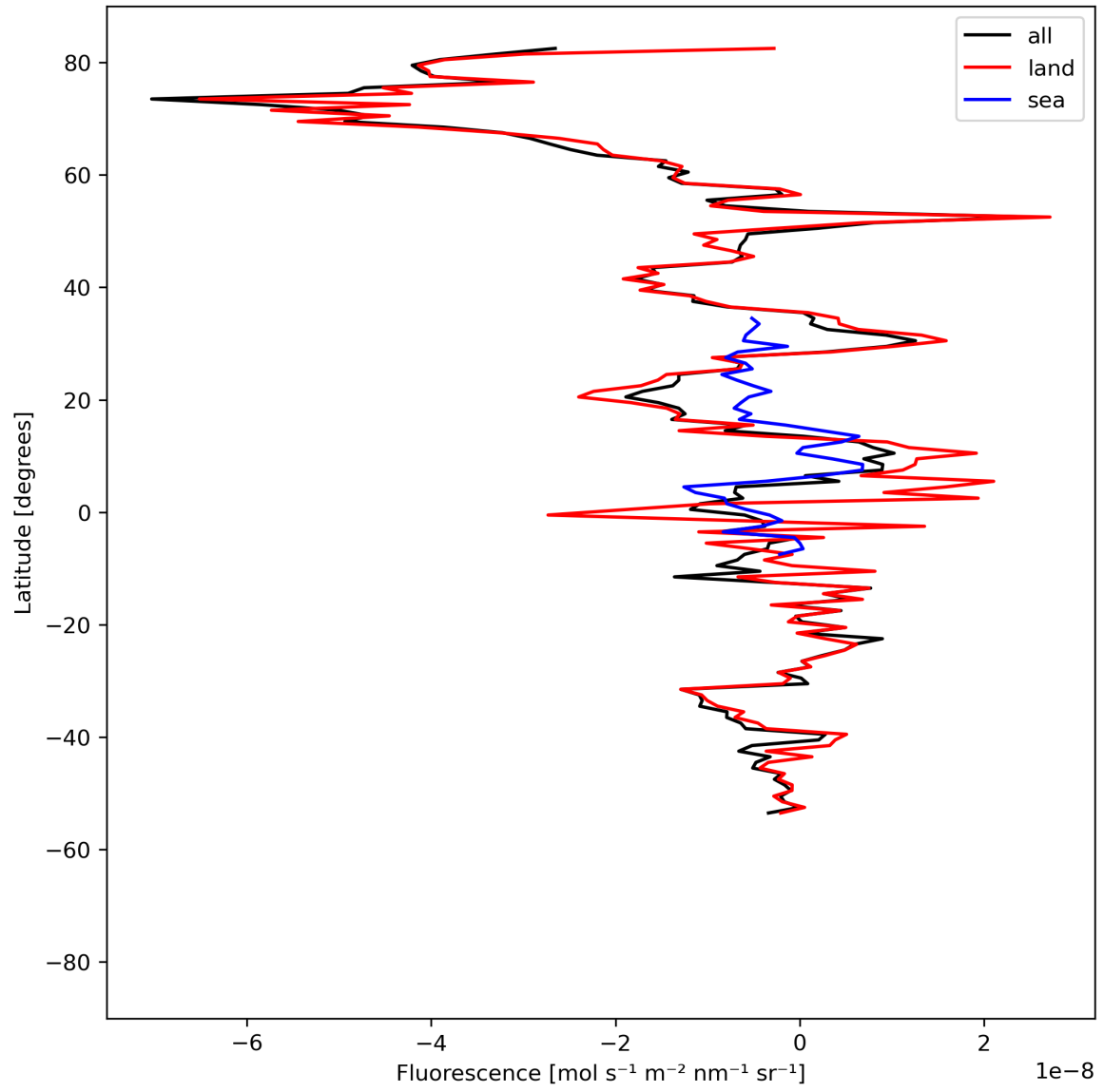
Figure 21: Zonal average of “Fluorescence” for 2024-04-06 to 2024-04-08.
