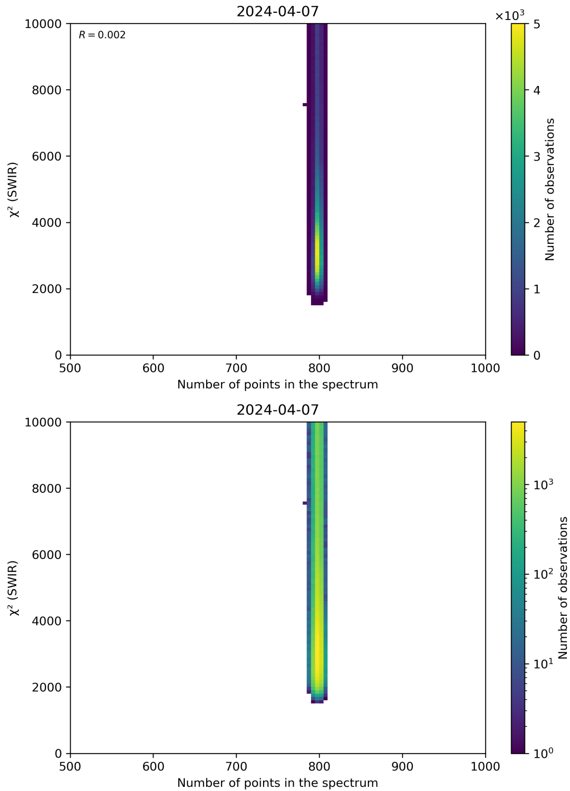
Figure 89: Scatter density plot of “Number of points in the spectrum” against “ \chi^2 (SWIR)” for 2024-04-06 to 2024-04-08.
