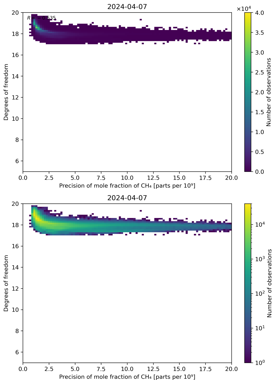
Figure 80: Scatter density plot of “Precision of mole fraction of CH 4 ” against “Degrees of freedom” for 2024-04-06 to 2024-04-08.
