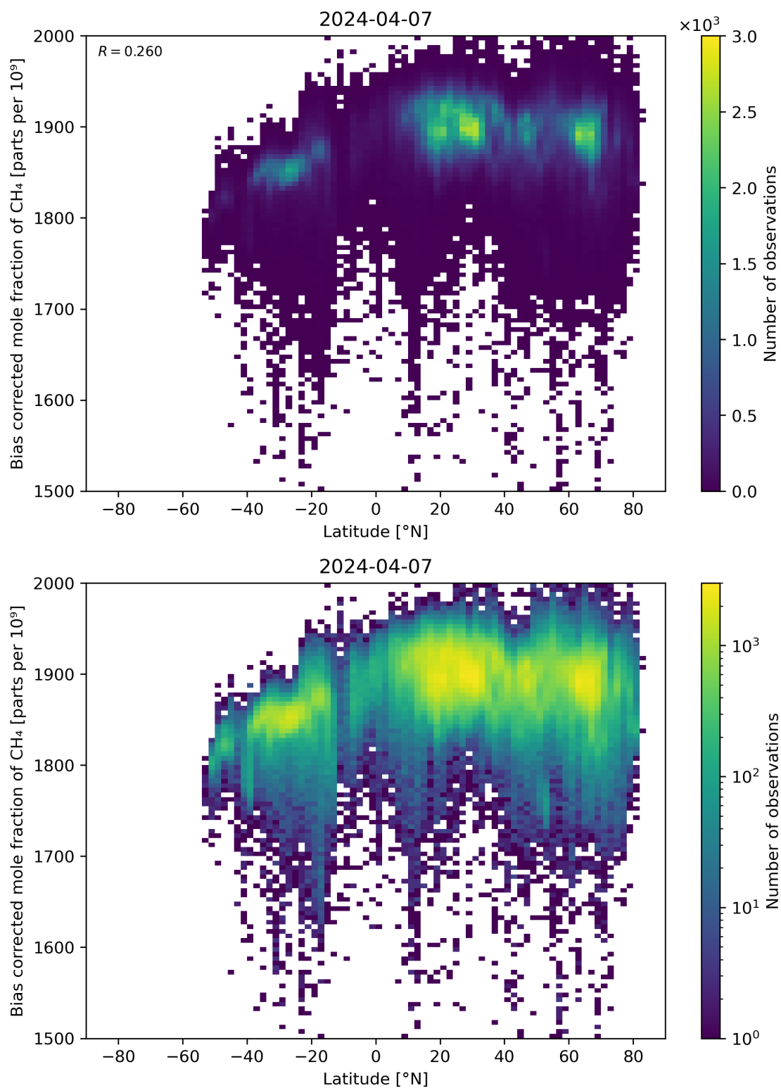
Figure 58: Scatter density plot of “Latitude” against “Bias corrected mole fraction of \text{CH}_4 ” for 2024-04-06 to 2024-04-08.
