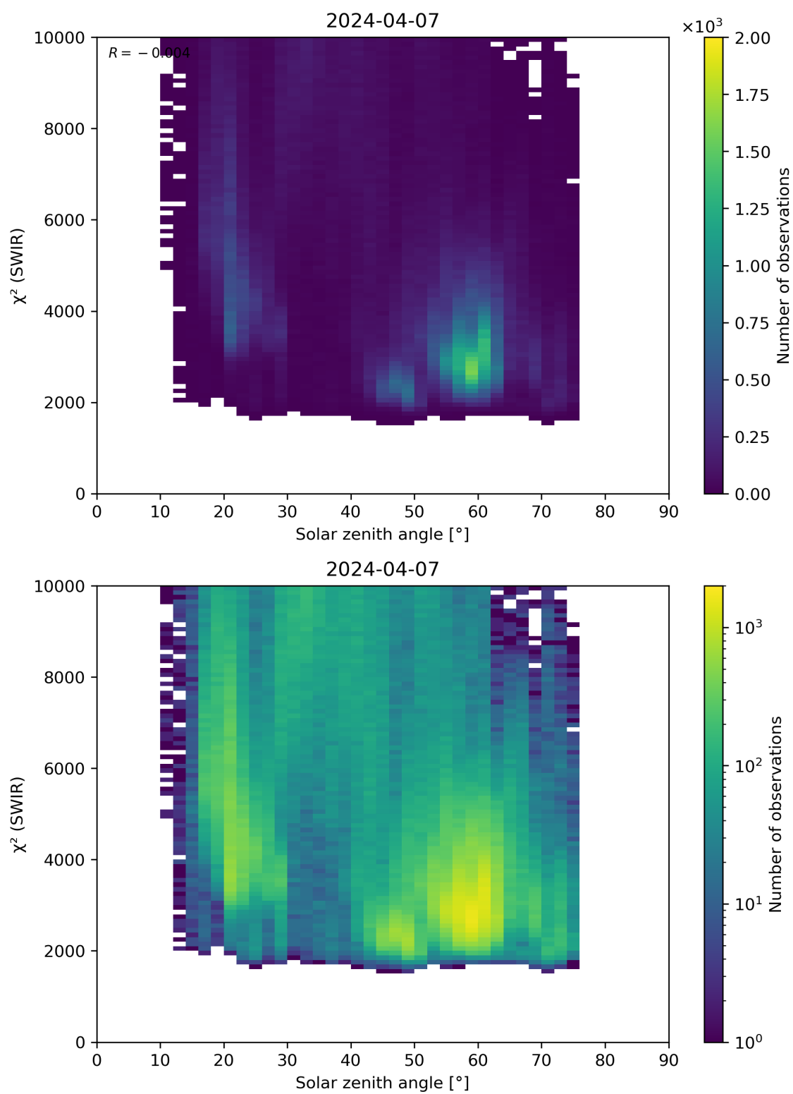
Figure 95: Scatter density plot of “Solar zenith angle” against “ \chi^2 (SWIR)” for 2024-04-06 to 2024-04-08.
