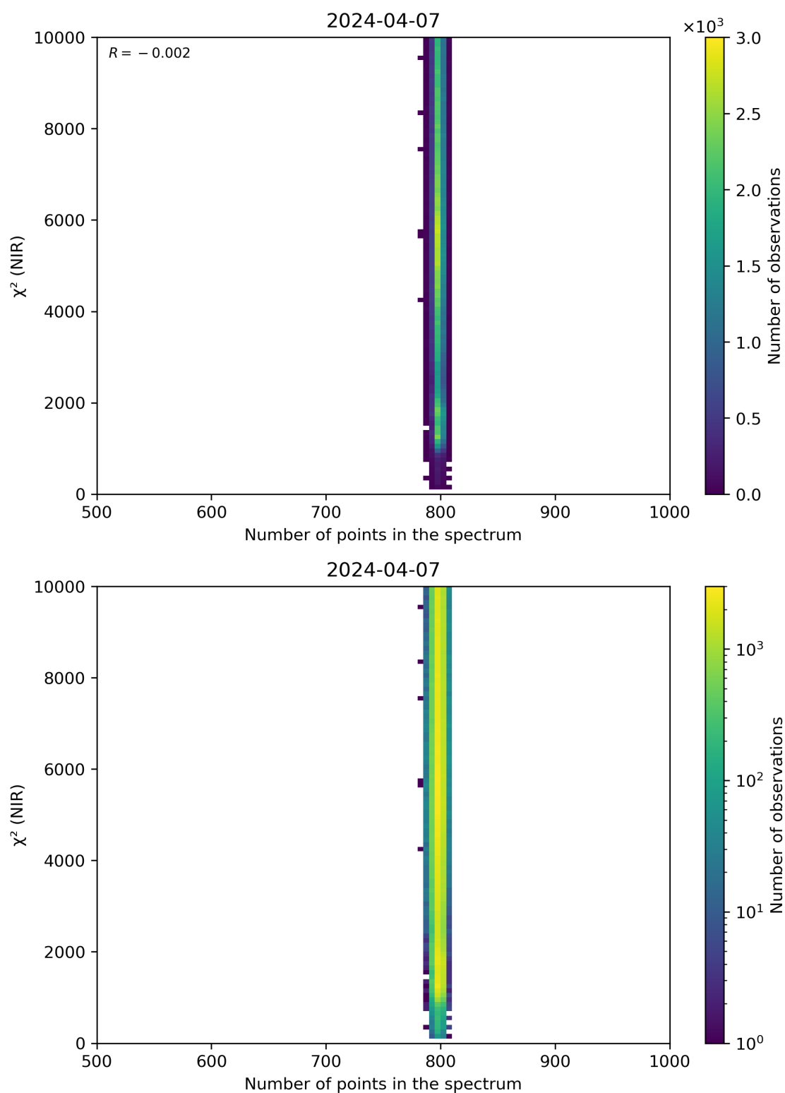
Figure 88: Scatter density plot of “Number of points in the spectrum” against “ \chi^2 (NIR)” for 2024-04-06 to 2024-04-08.
