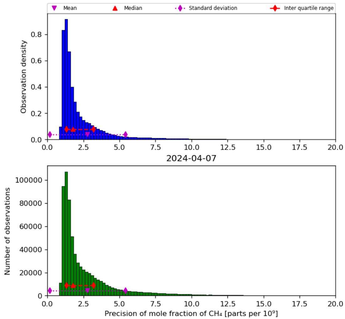
Figure 24: Histogram of “Precision of mole fraction of CH 4 ” for 2024-04-06 to 2024-04-08
