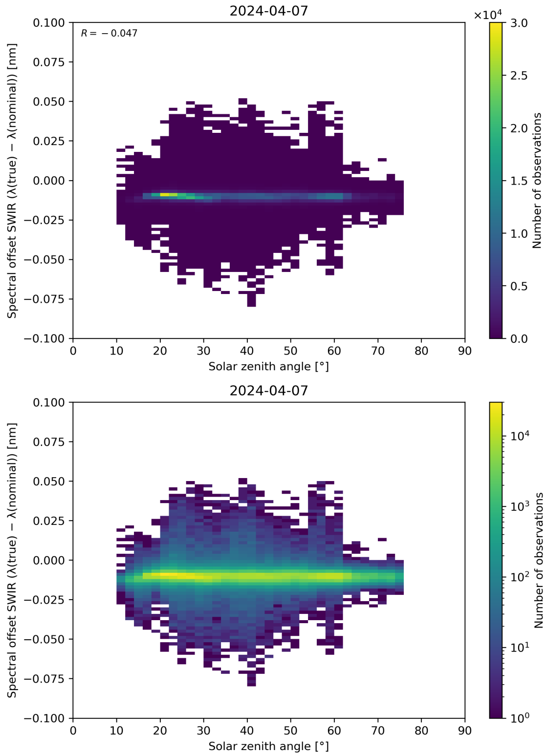
Figure 104: Scatter density plot of “Solar zenith angle” against “Spectral offset SWIR ( \lambda(\text{true}) - \lambda(\text{nominal}) )” for 2024-04-06 to 2024-04-08.
