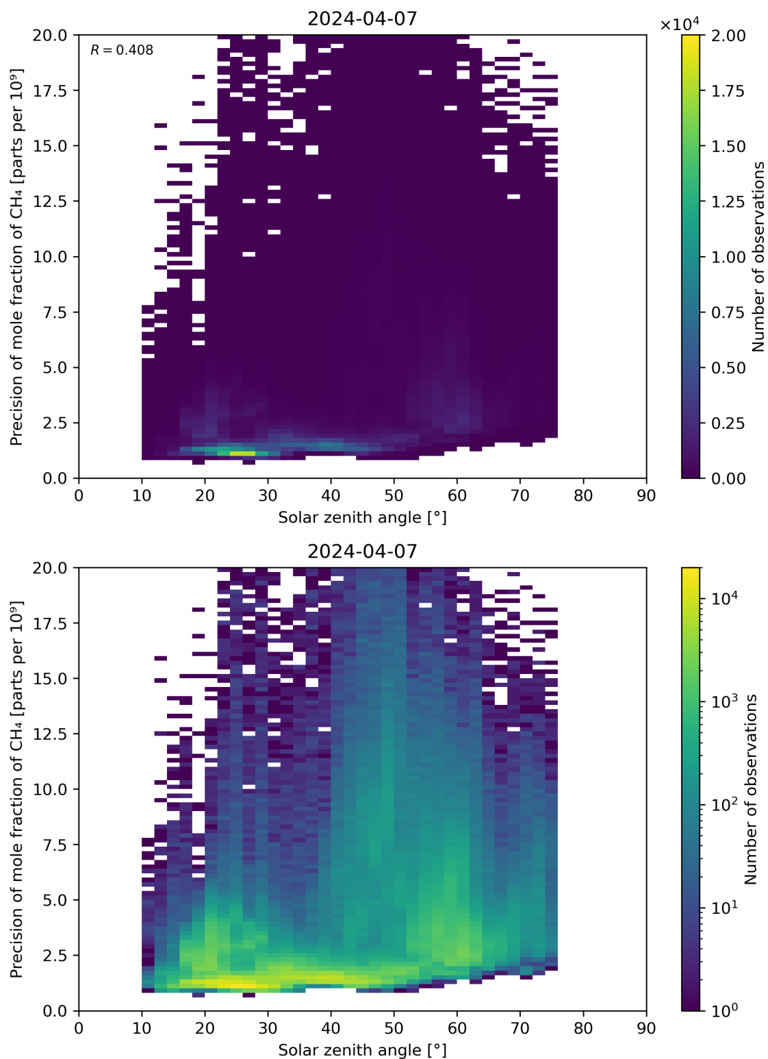
Figure 101: Scatter density plot of “Solar zenith angle” against “Precision of mole fraction of CH 4 ” for 2024-04-06 to 2024-04-08.
