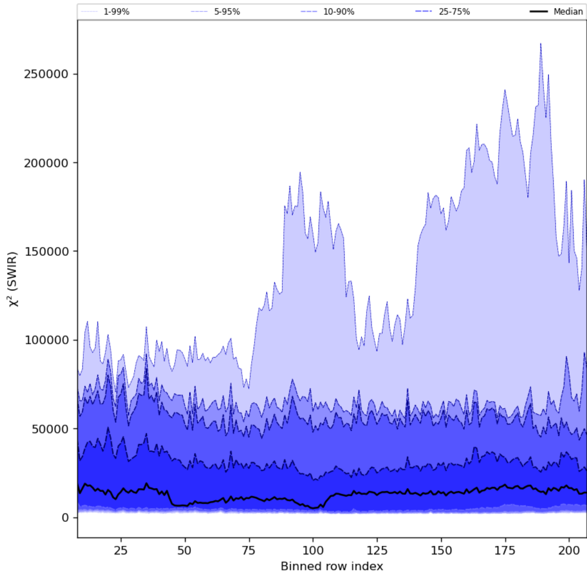
Figure 39: Along track statistics of “ \chi^2 (SWIR)” for 2024-04-06 to 2024-04-08
