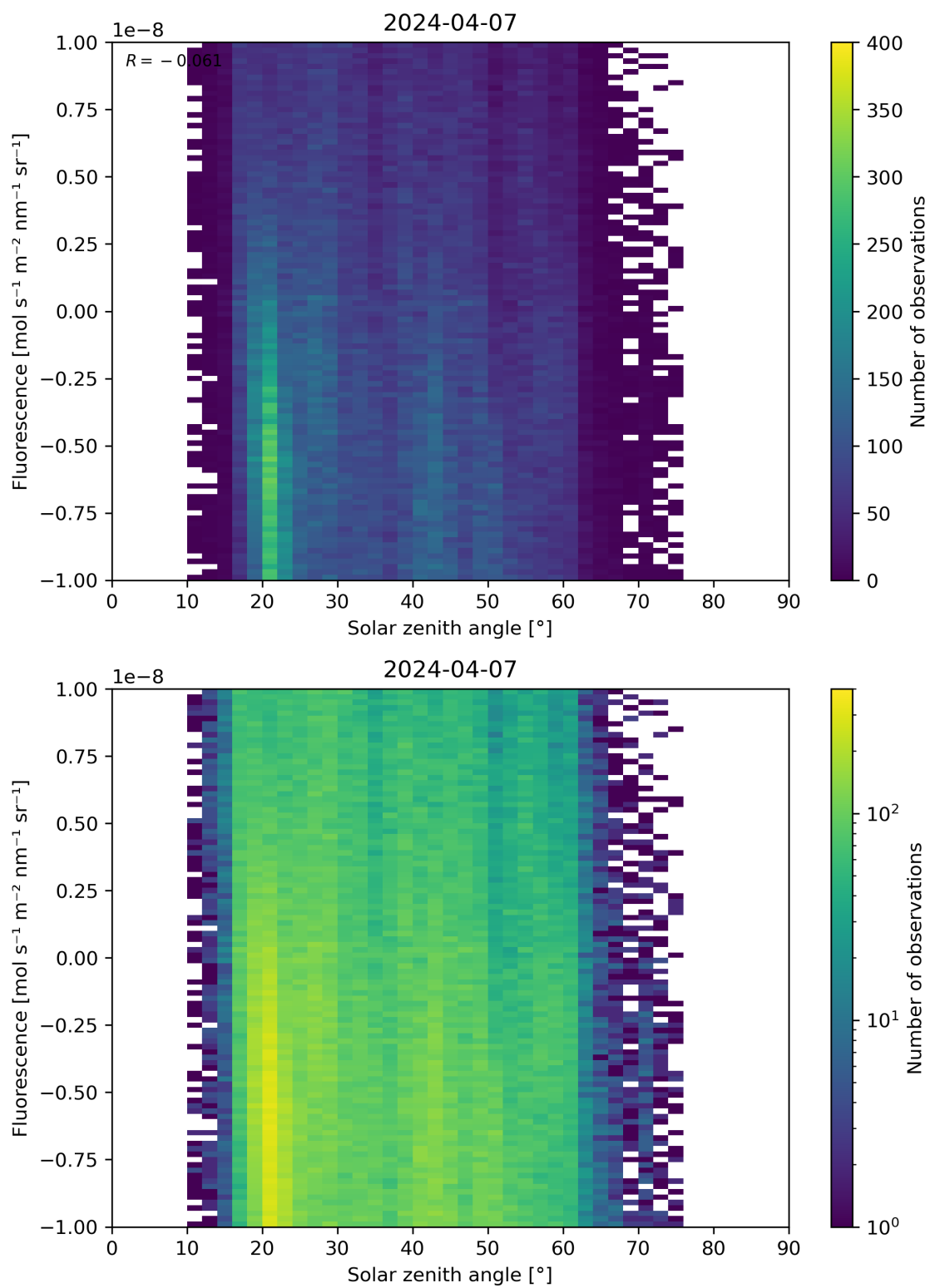
Figure 97: Scatter density plot of “Solar zenith angle” against “Fluorescence” for 2024-04-06 to 2024-04-08.
