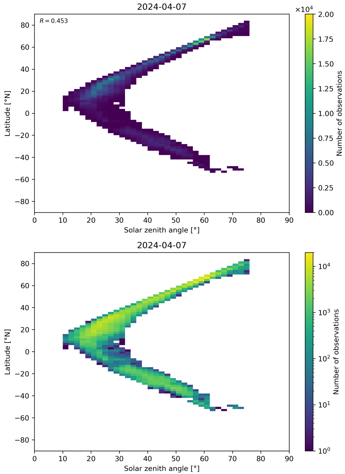
Figure 98: Scatter density plot of “Solar zenith angle” against “Latitude” for 2024-04-06 to 2024-04-08.
