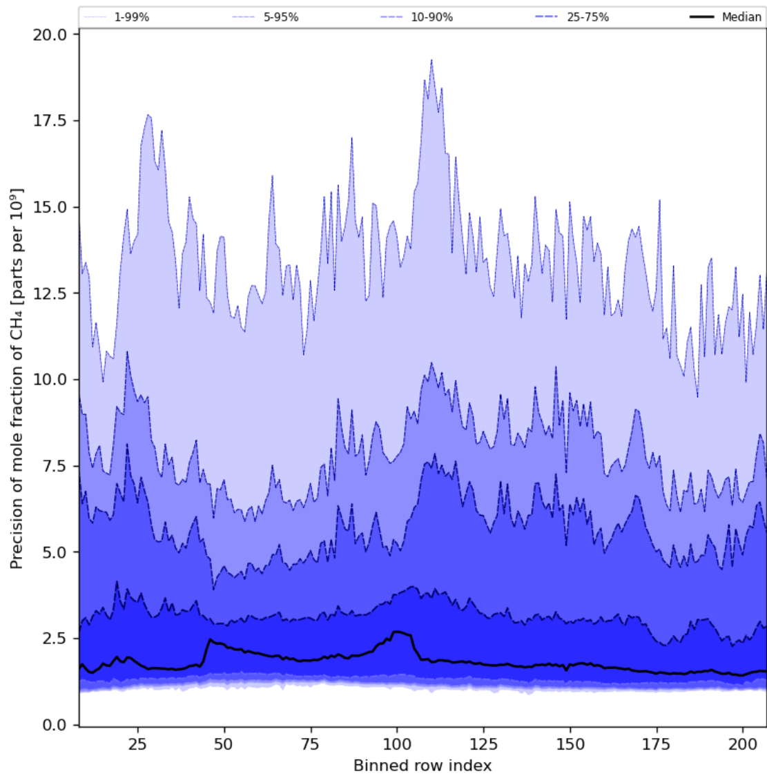
Figure 35: Along track statistics of “Precision of mole fraction of CH 4 ” for 2024-04-06 to 2024-04-08
