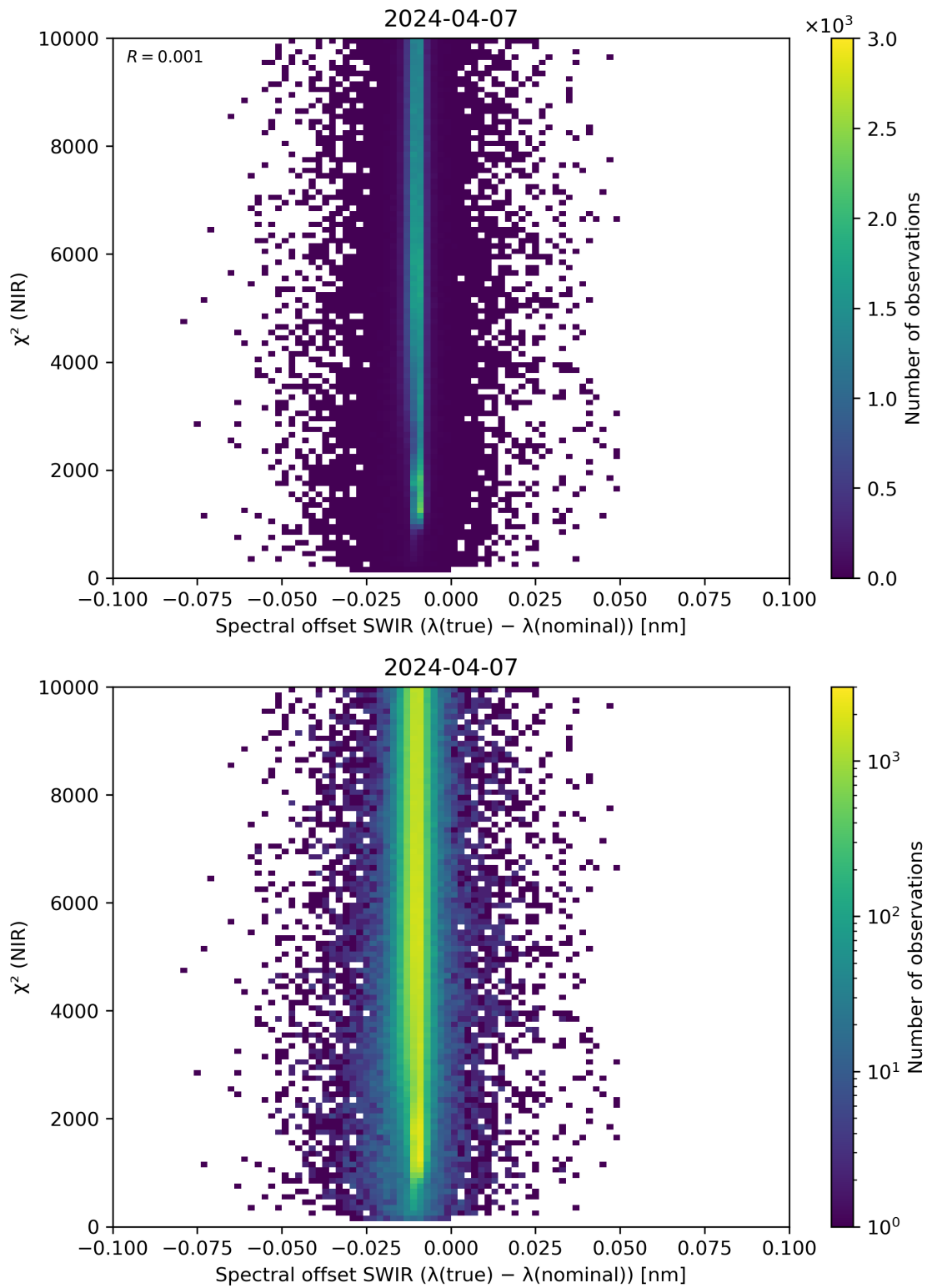
Figure 117: Scatter density plot of “Spectral offset SWIR ( \lambda(\text{true}) - \lambda(\text{nominal}) )” against “ \chi^2 (NIR)” for 2024-04-06 to 2024-04-08.
