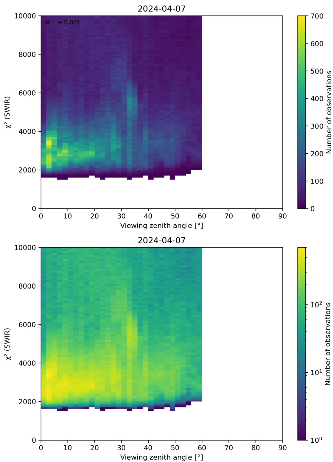
Figure 106: Scatter density plot of “Viewing zenith angle” against “ \chi^2 (SWIR)” for 2024-04-06 to 2024-04-08.
