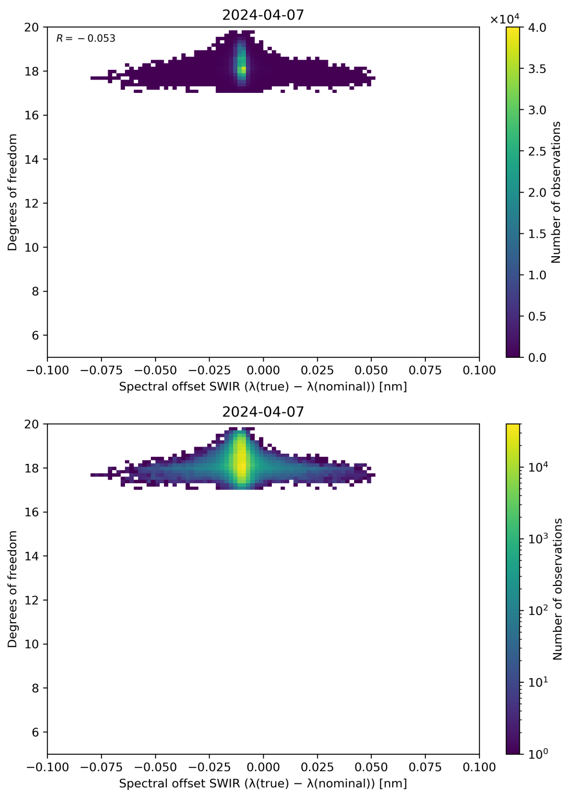
Figure 119: Scatter density plot of “Spectral offset SWIR ( \lambda(\text{true}) - \lambda(\text{nominal}) )” against “Degrees of freedom” for 2024-04-06 to 2024-04-08.
