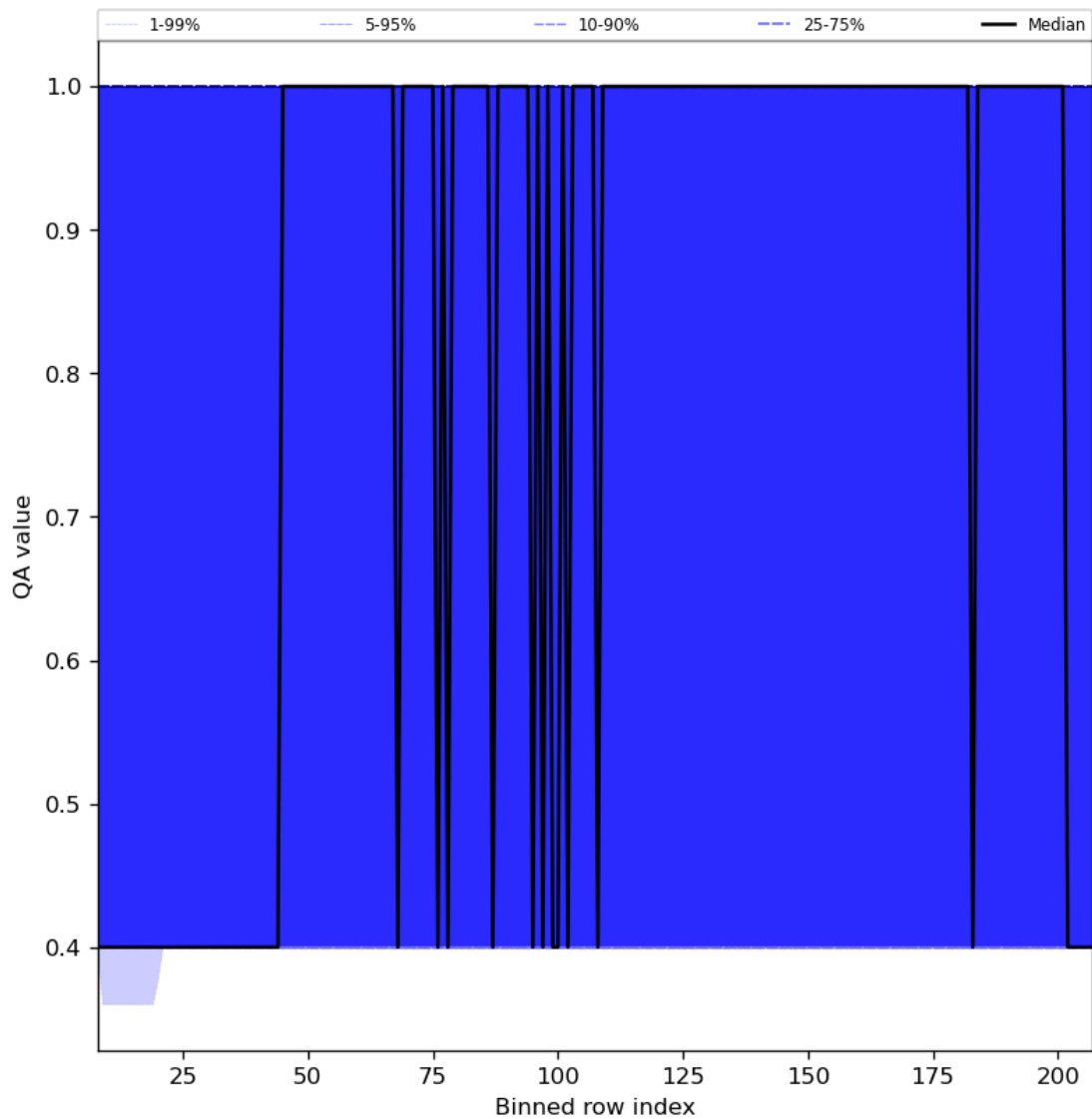
Figure 33: Along track statistics of “QA value” for 2024-04-06 to 2024-04-08
