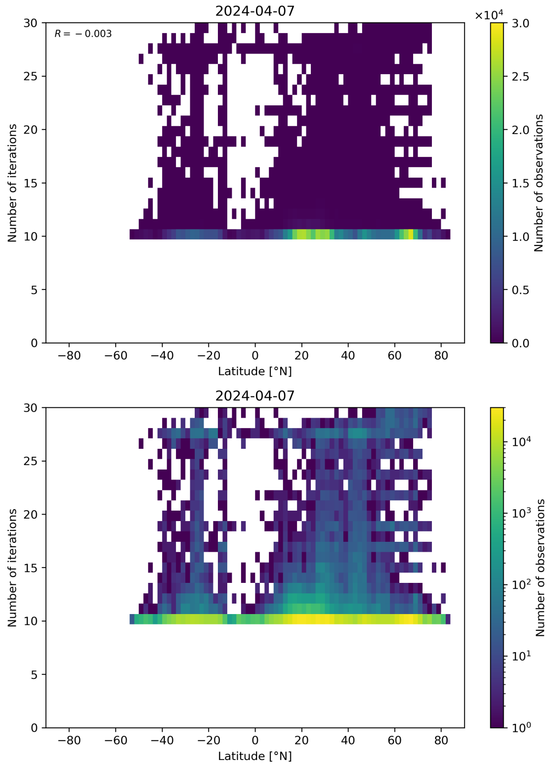
Figure 60: Scatter density plot of “Latitude” against “Number of iterations” for 2024-04-06 to 2024-04-08.
