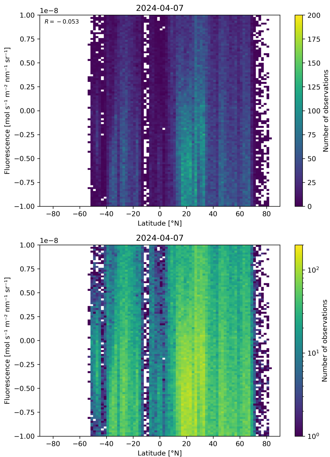
Figure 56: Scatter density plot of “Latitude” against “Fluorescence” for 2024-04-06 to 2024-04-08.
