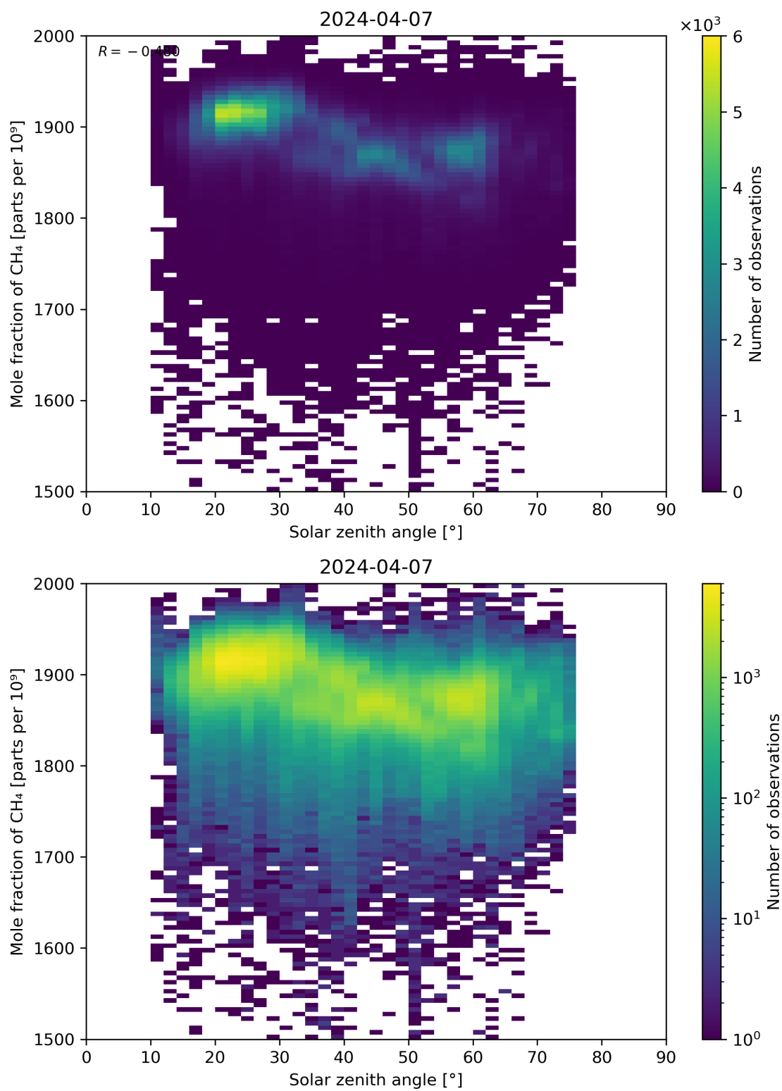
Figure 99: Scatter density plot of “Solar zenith angle” against “Mole fraction of \text{CH}_4 ” for 2024-04-06 to 2024-04-08.
