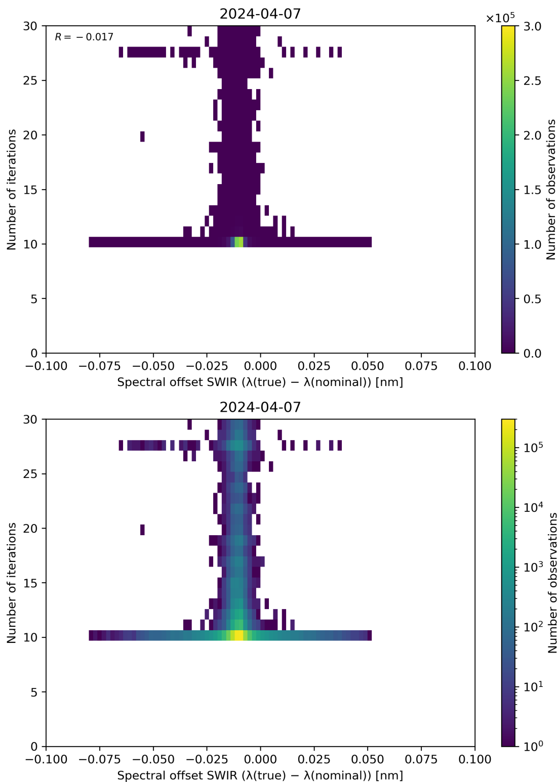
Figure 121: Scatter density plot of “Spectral offset SWIR ( \lambda(\text{true}) - \lambda(\text{nominal}) )” against “Number of iterations” for 2024-04-06 to 2024-04-08.
