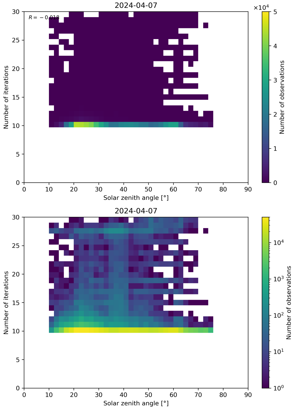
Figure 102: Scatter density plot of “Solar zenith angle” against “Number of iterations” for 2024-04-06 to 2024-04-08.
