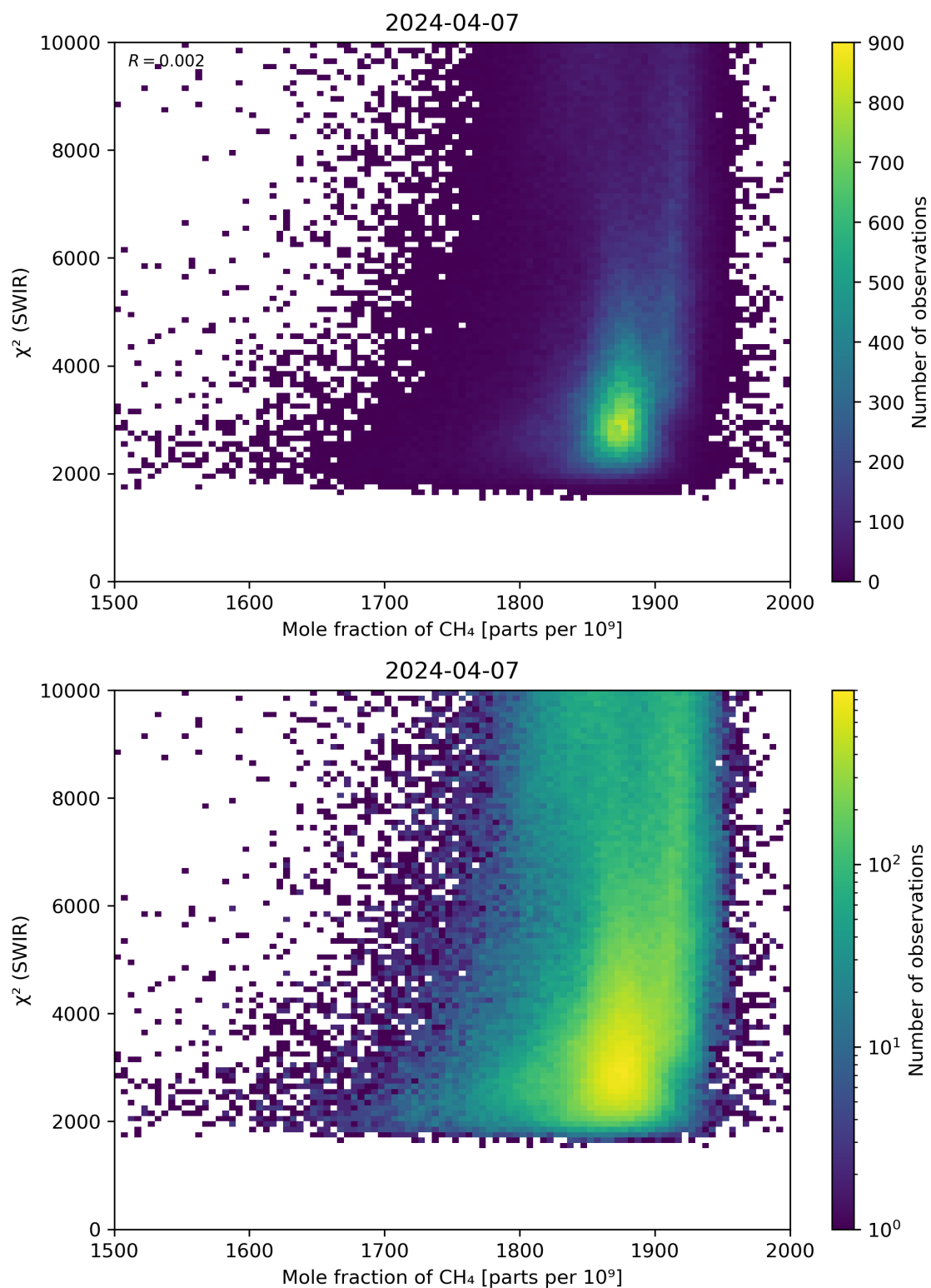
Figure 71: Scatter density plot of “Mole fraction of \text{CH}_4 ” against “ \chi^2 (SWIR)” for 2024-04-06 to 2024-04-08.
