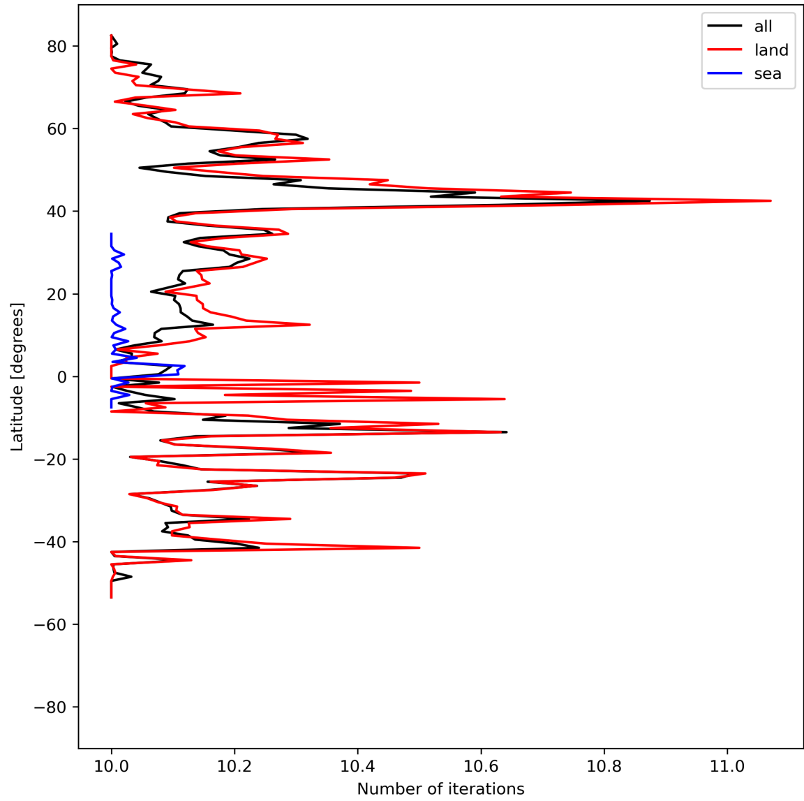
Figure 20: Zonal average of “Number of iterations” for 2024-04-06 to 2024-04-08.
