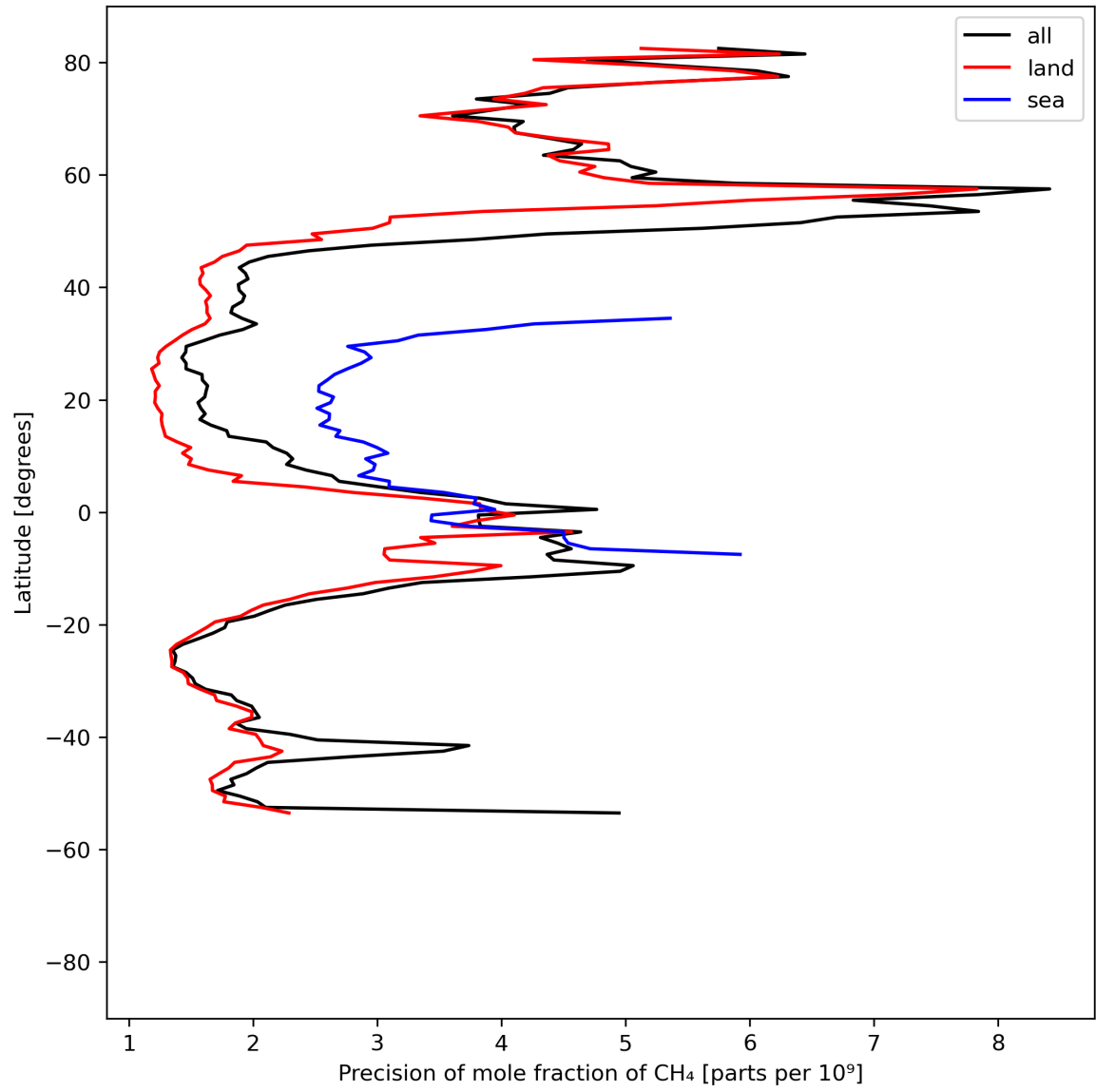
Figure 13: Zonal average of “Precision of mole fraction of CH 4 ” for 2024-04-06 to 2024-04-08.
