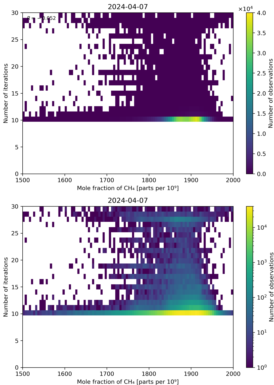
Figure 76: Scatter density plot of “Mole fraction of CH 4 ” against “Number of iterations” for 2024-04-06 to 2024-04-08.
