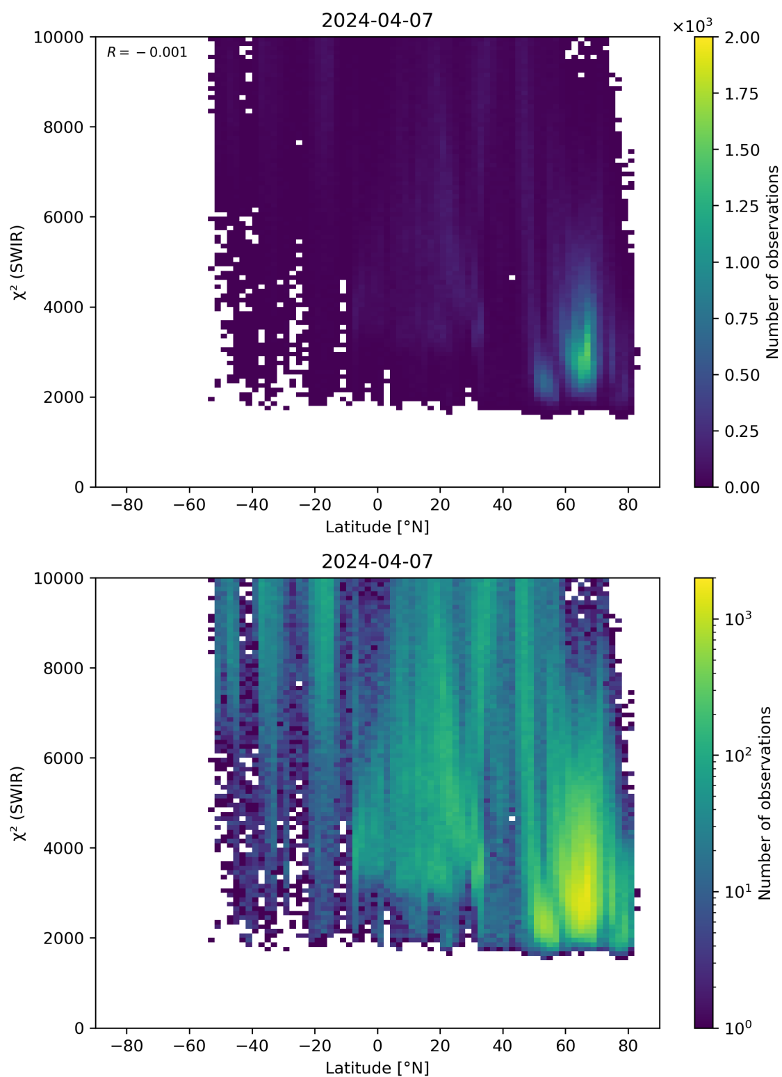
Figure 54: Scatter density plot of “Latitude” against “ \chi^2 (SWIR)” for 2024-04-06 to 2024-04-08.
