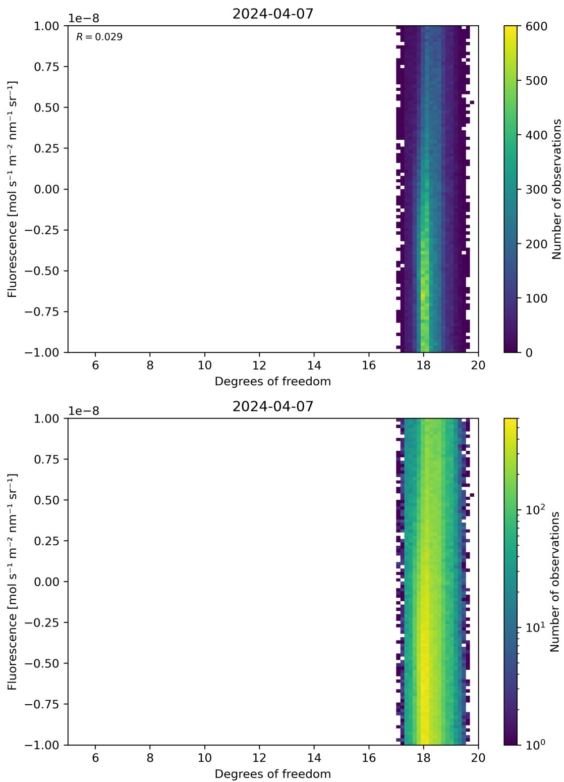
Figure 51: Scatter density plot of “Degrees of freedom” against “Fluorescence” for 2024-04-06 to 2024-04-08.
