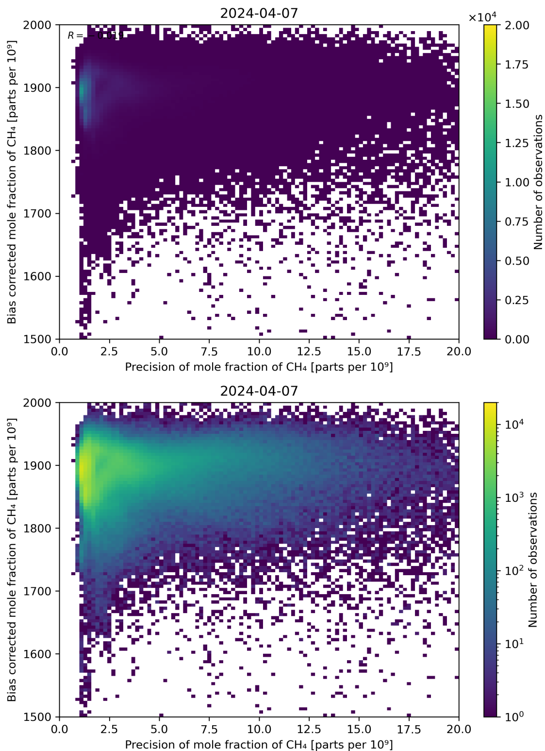
Figure 82: Scatter density plot of “Precision of mole fraction of CH 4 ” against “Bias corrected mole fraction of CH 4 ” for 2024-04-06 to 2024-04-08.
