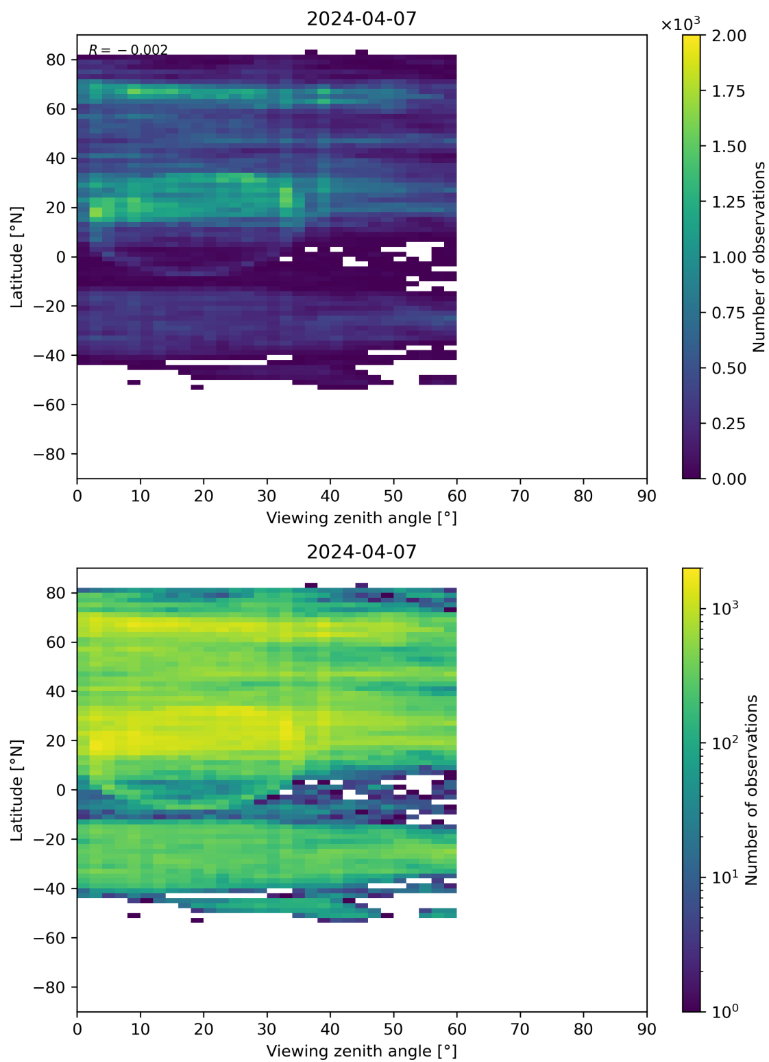
Figure 109: Scatter density plot of “Viewing zenith angle” against “Latitude” for 2024-04-06 to 2024-04-08.
