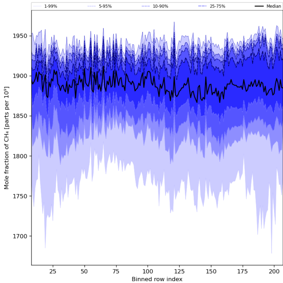
Figure 34: Along track statistics of “Mole fraction of CH 4 ” for 2024-04-06 to 2024-04-08
