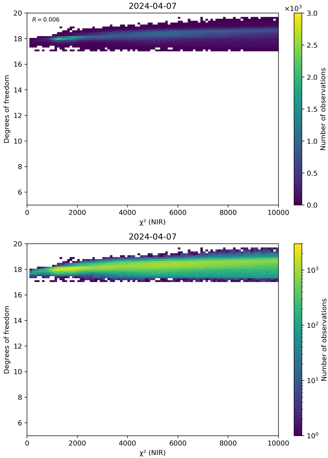
Figure 44: Scatter density plot of “ \chi^2 (NIR)” against “Degrees of freedom” for 2024-04-06 to 2024-04-08.
