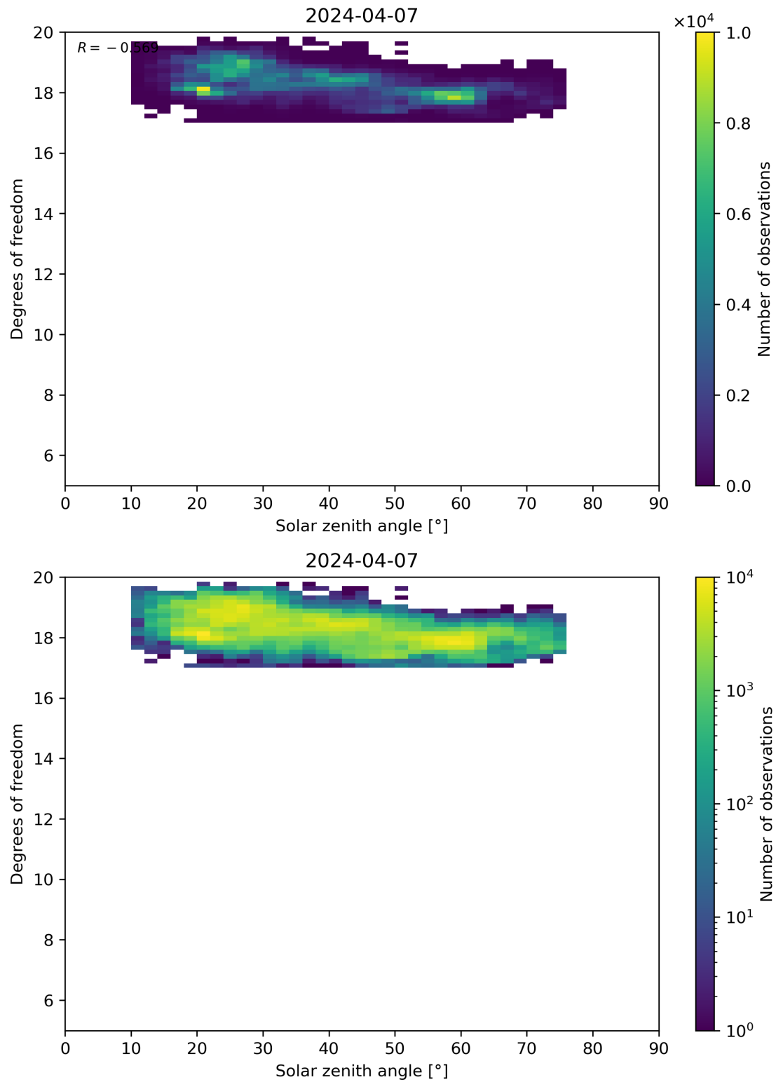
Figure 96: Scatter density plot of “Solar zenith angle” against “Degrees of freedom” for 2024-04-06 to 2024-04-08.
