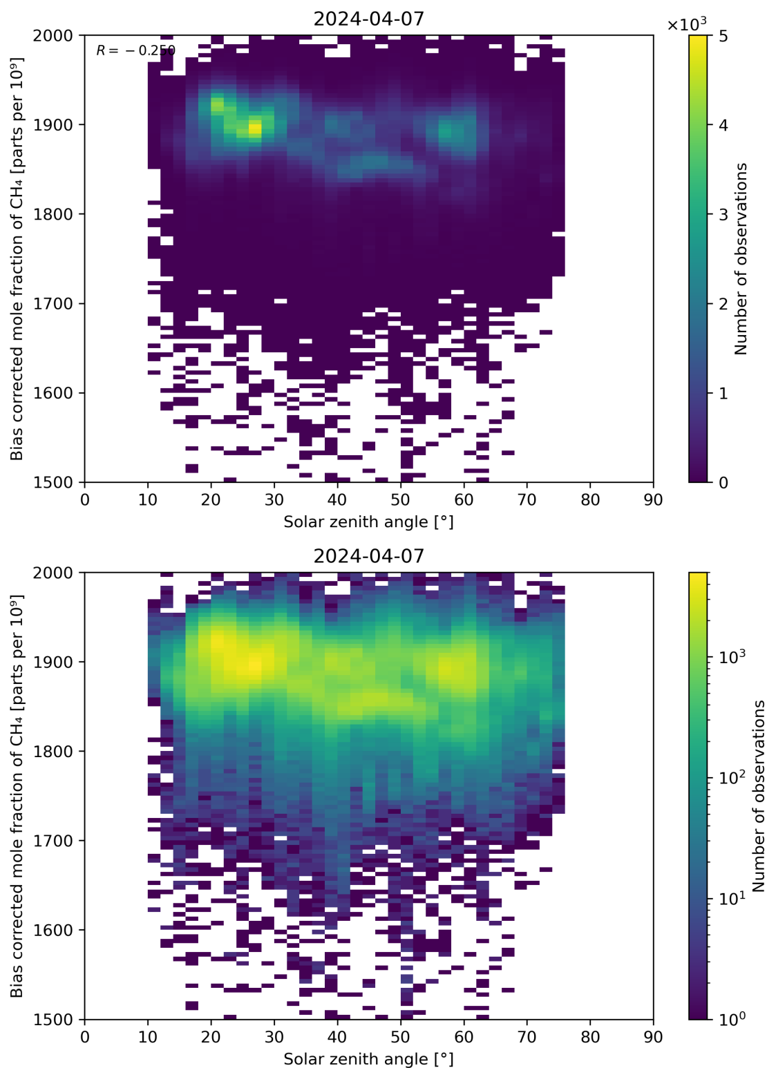
Figure 100: Scatter density plot of “Solar zenith angle” against “Bias corrected mole fraction of CH 4 ” for 2024-04-06 to 2024-04-08.
