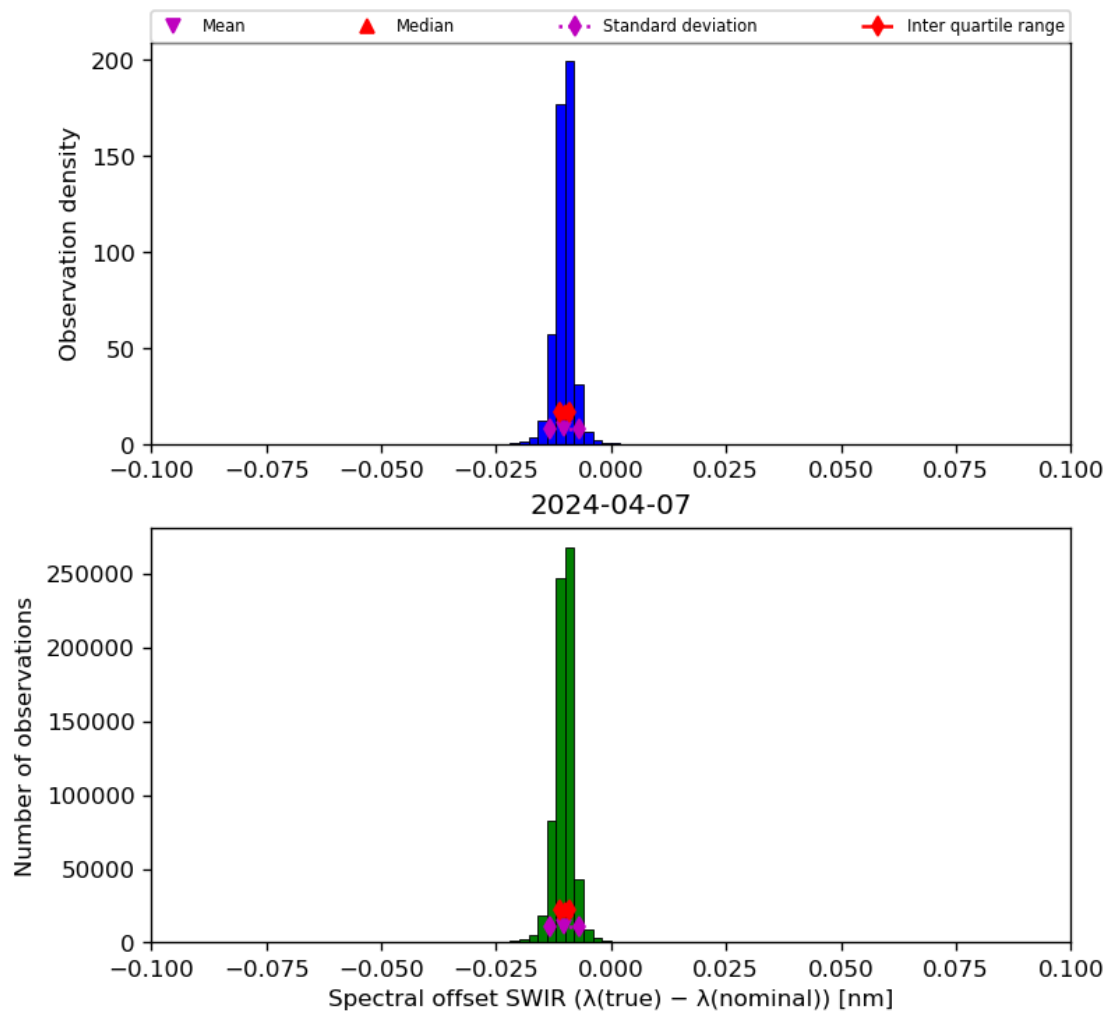
Figure 27: Histogram of “Spectral offset SWIR ( \lambda(\text{true}) - \lambda(\text{nominal}) )” for 2024-04-06 to 2024-04-08
