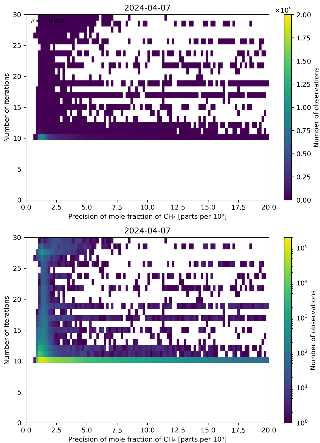
Figure 83: Scatter density plot of “Precision of mole fraction of CH 4 ” against “Number of iterations” for 2024-04-06 to 2024-04-08.
