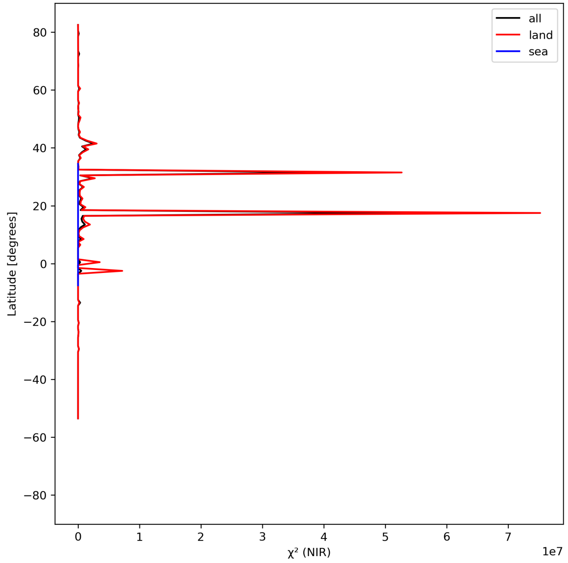
Figure 18: Zonal average of “ \chi^2 (NIR)” for 2024-04-06 to 2024-04-08.
