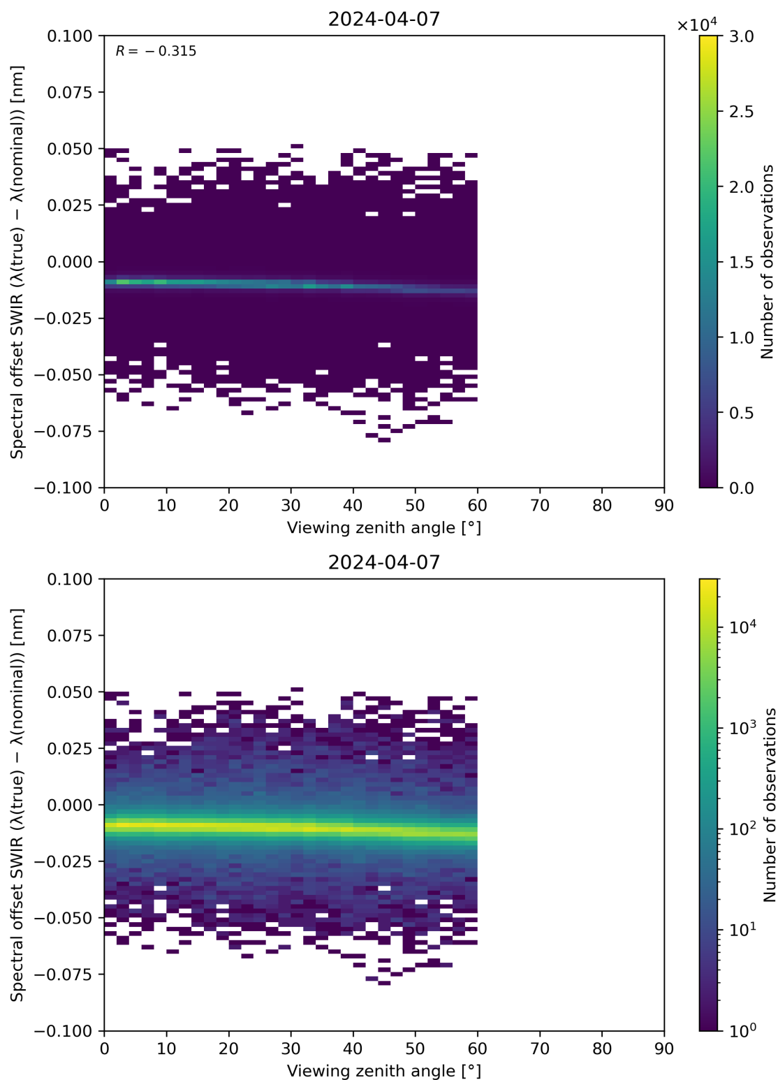
Figure 116: Scatter density plot of “Viewing zenith angle” against “Spectral offset SWIR ( \lambda(\text{true}) - \lambda(\text{nominal}) )” for 2024-04-06 to 2024-04-08.
