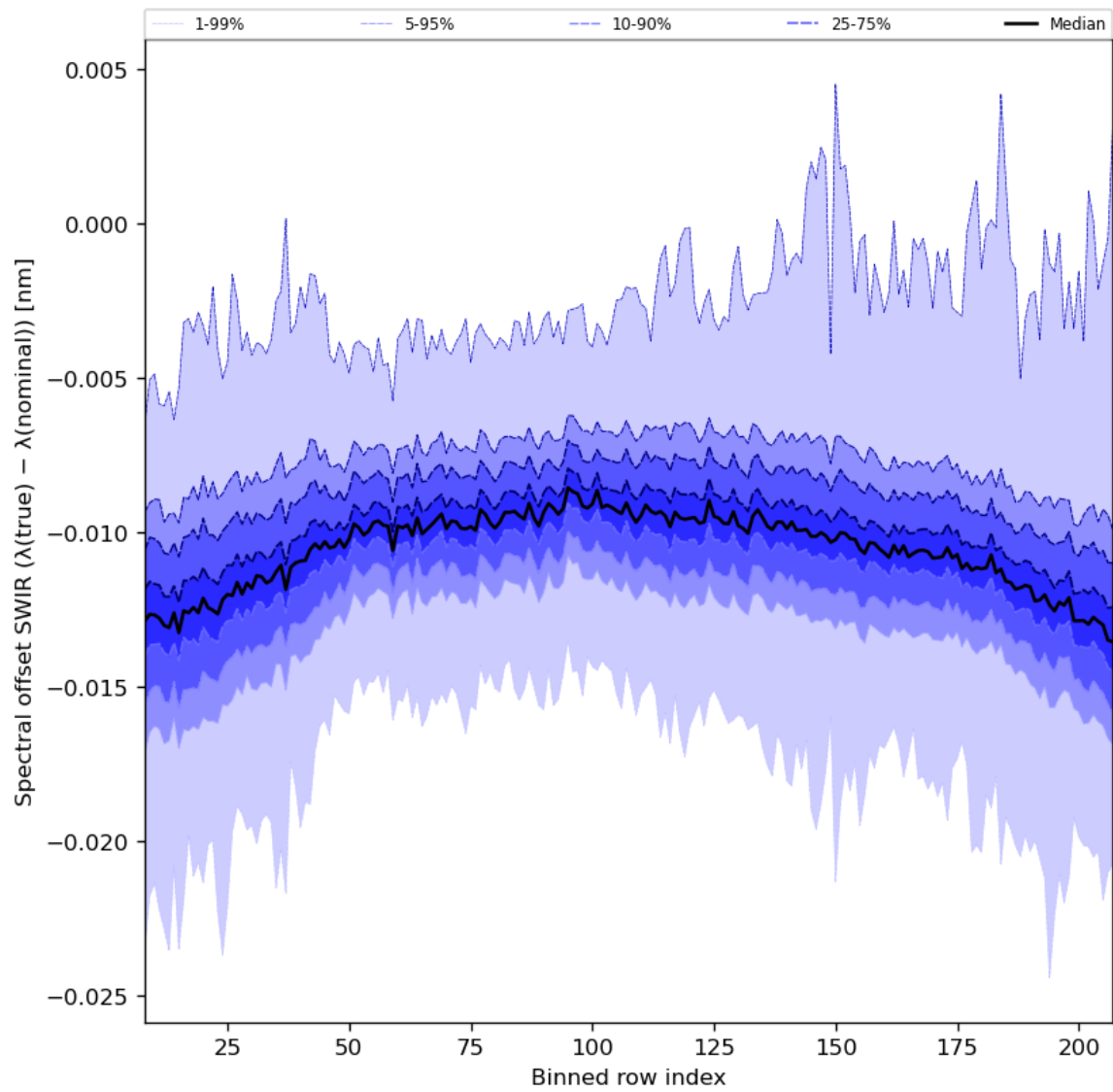
Figure 38: Along track statistics of “Spectral offset SWIR ( \lambda(\text{true}) - \lambda(\text{nominal}) )” for 2024-04-06 to 2024-04-08
