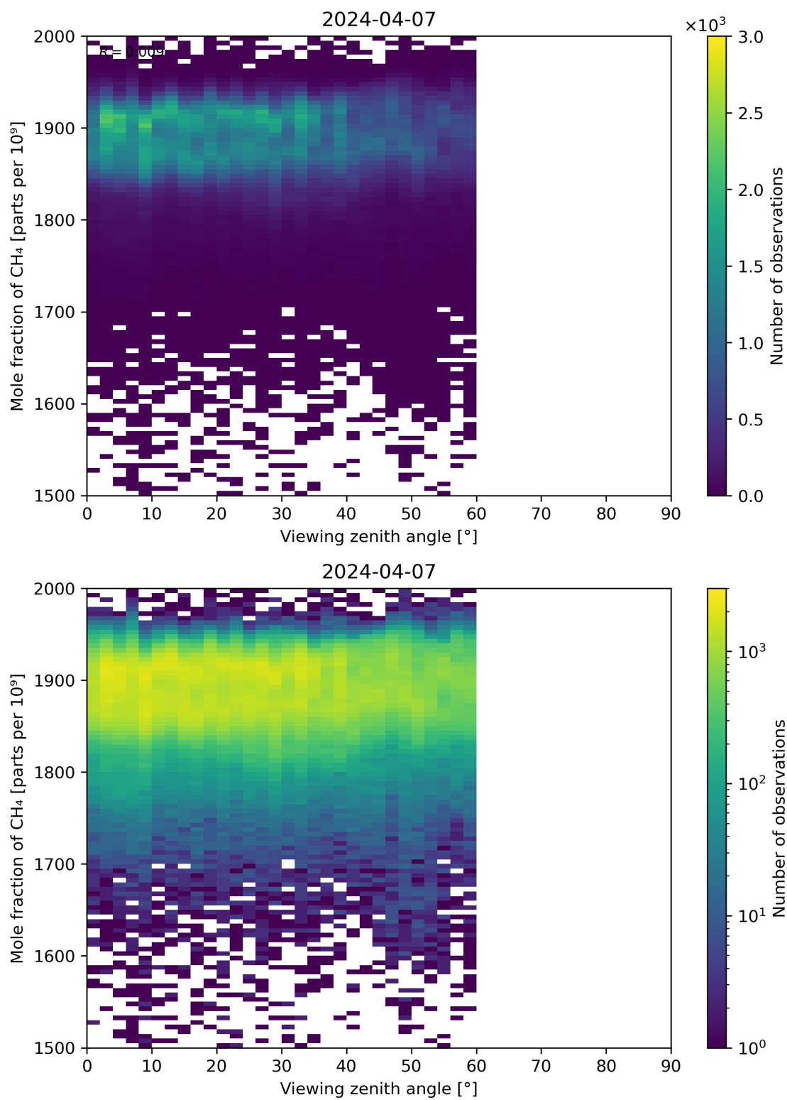
Figure 110: Scatter density plot of “Viewing zenith angle” against “Mole fraction of CH 4 ” for 2024-04-06 to 2024-04-08.
