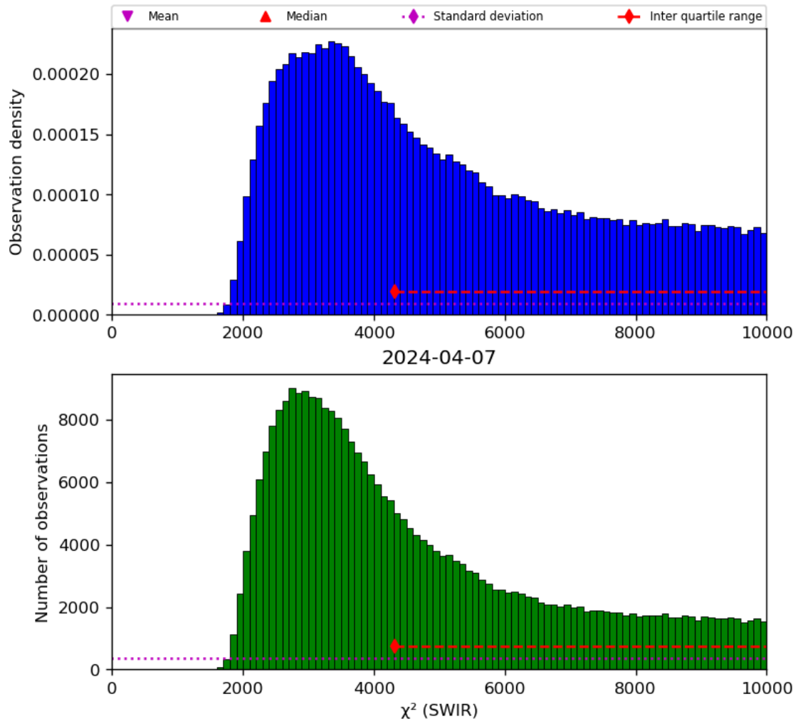
Figure 28: Histogram of “ \chi^2 (SWIR)” for 2024-04-06 to 2024-04-08
