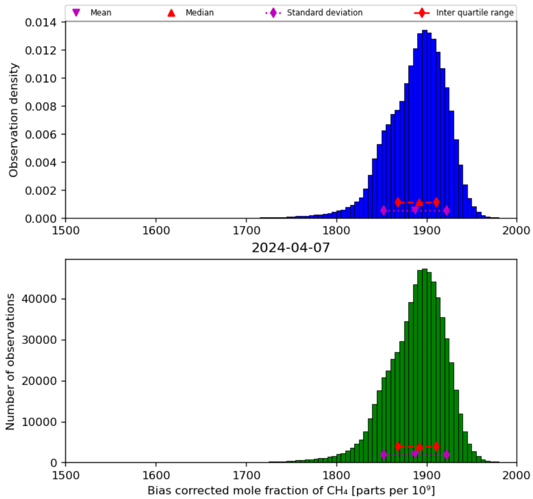
Figure 25: Histogram of “Bias corrected mole fraction of CH 4 ” for 2024-04-06 to 2024-04-08
