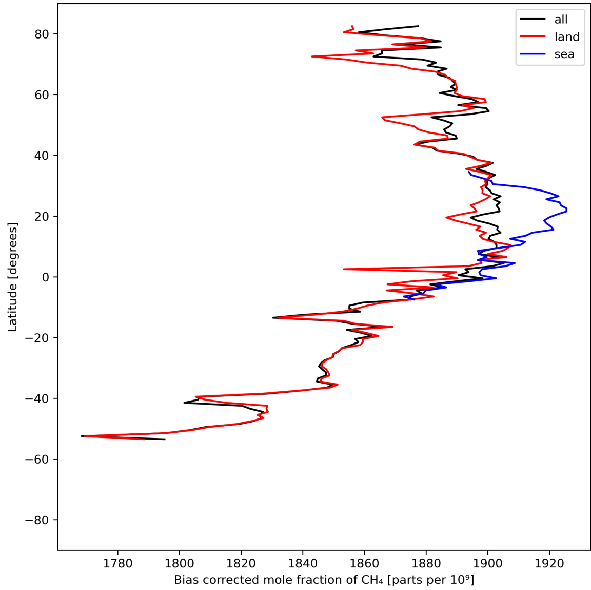
Figure 14: Zonal average of “Bias corrected mole fraction of CH 4 ” for 2024-04-06 to 2024-04-08.
