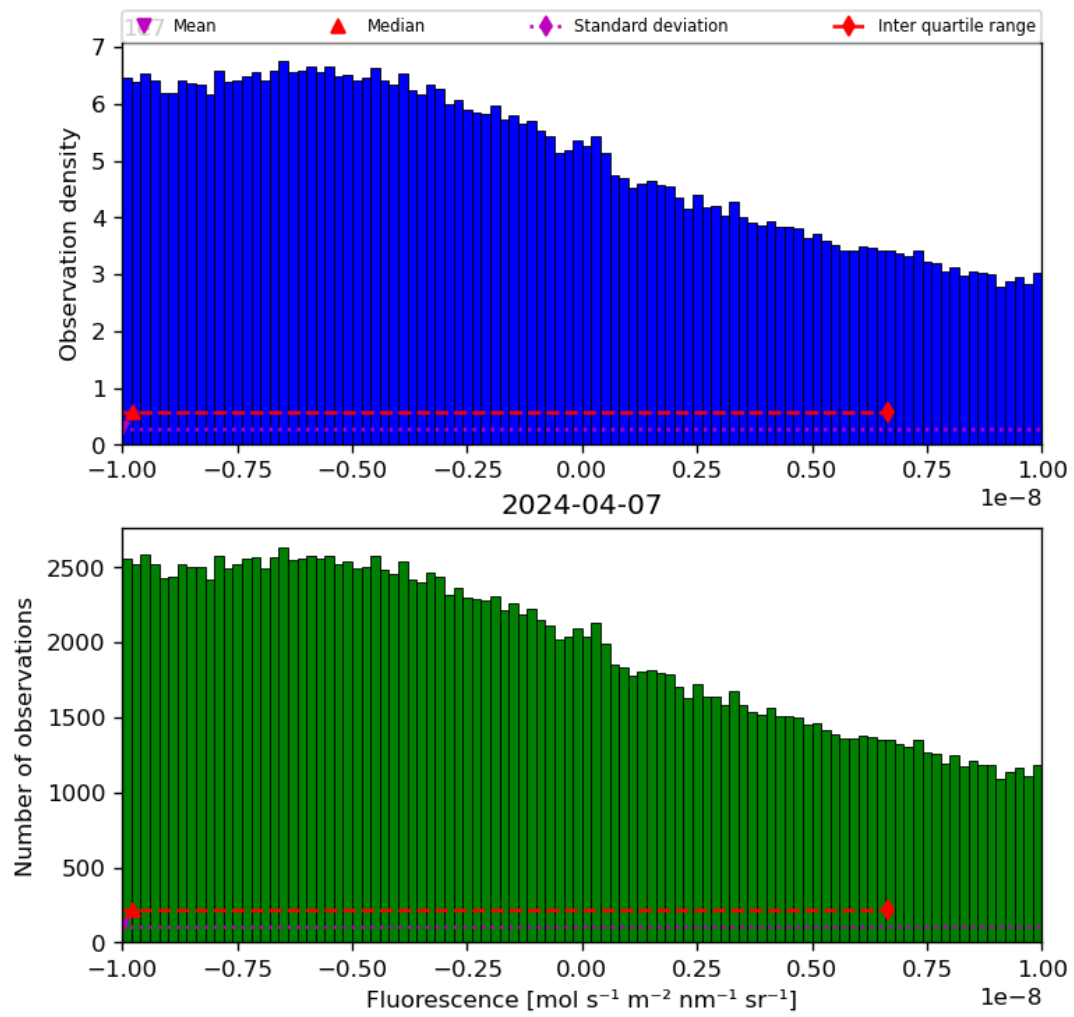
Figure 32: Histogram of “Fluorescence” for 2024-04-06 to 2024-04-08
