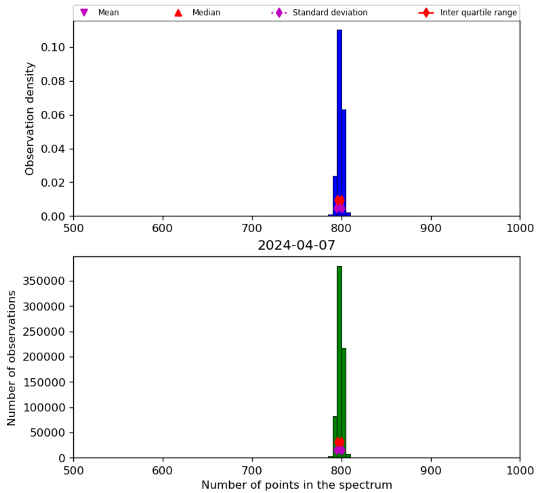
Figure 26: Histogram of “Number of points in the spectrum” for 2024-04-06 to 2024-04-08
