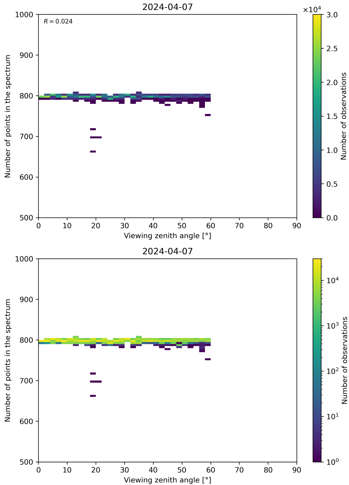
Figure 114: Scatter density plot of “Viewing zenith angle” against “Number of points in the spectrum” for 2024-04-06 to 2024-04-08.
