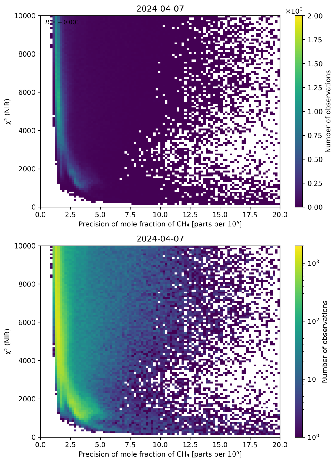
Figure 78: Scatter density plot of “Precision of mole fraction of \text{CH}_4 ” against “ \chi^2 (NIR)” for 2024-04-06 to 2024-04-08.
