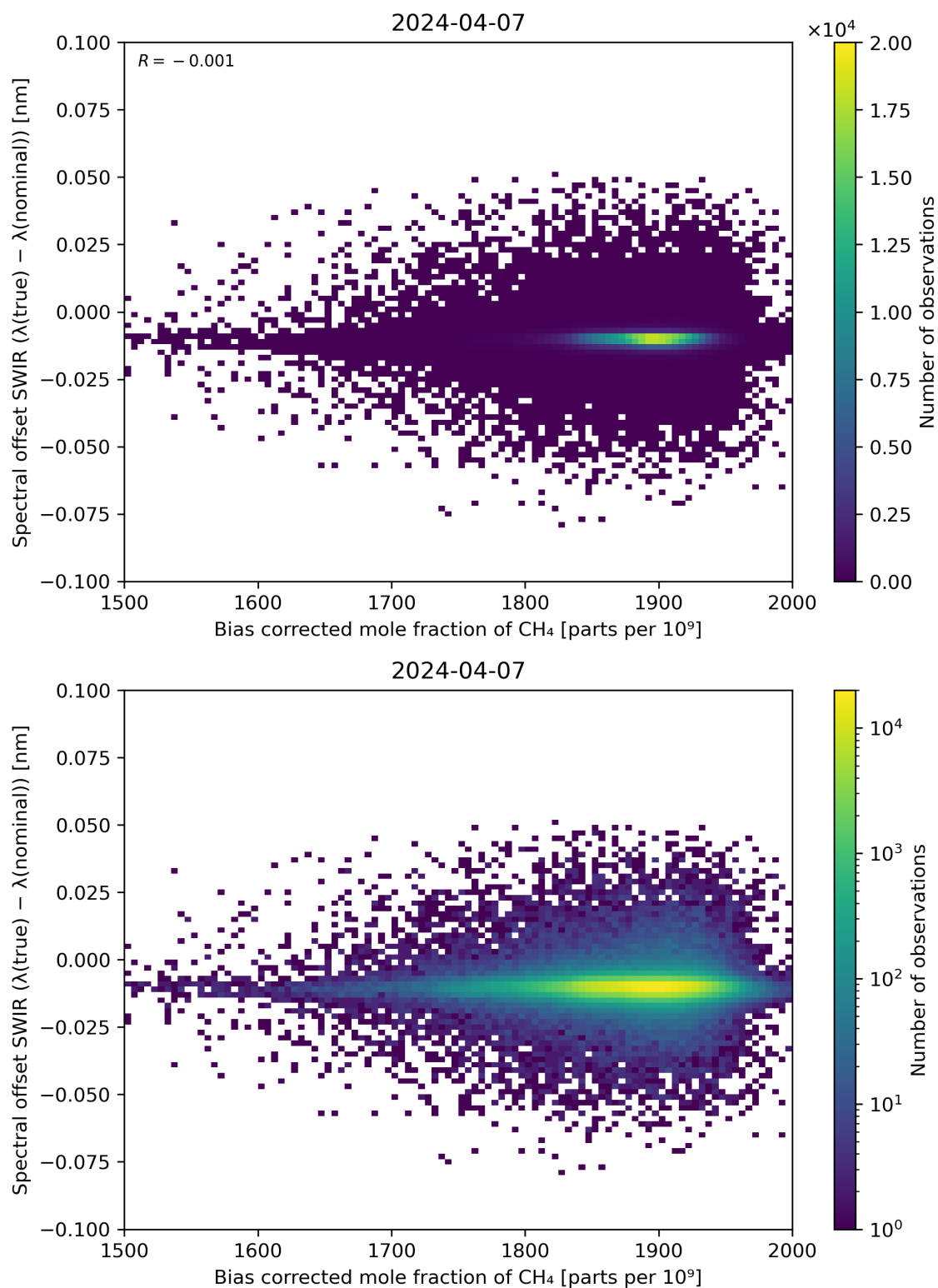
Figure 69: Scatter density plot of “Bias corrected mole fraction of \text{CH}_4 ” against “Spectral offset SWIR ( \lambda(\text{true}) - \lambda(\text{nominal}) )” for 2024-04-06 to 2024-04-08.
