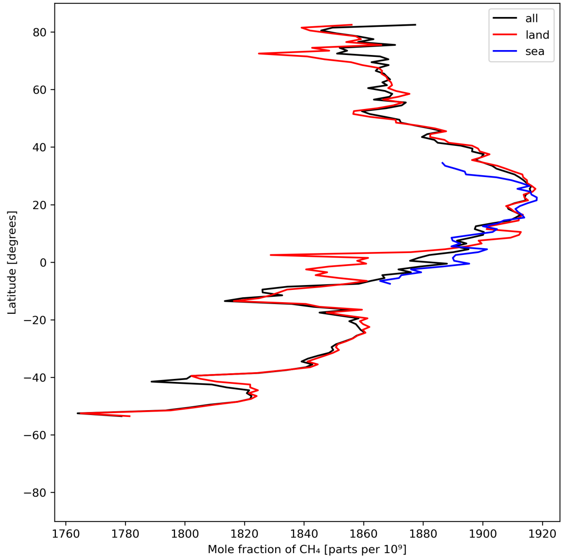
Figure 12: Zonal average of “Mole fraction of \text{CH}_4 ” for 2024-04-06 to 2024-04-08.
