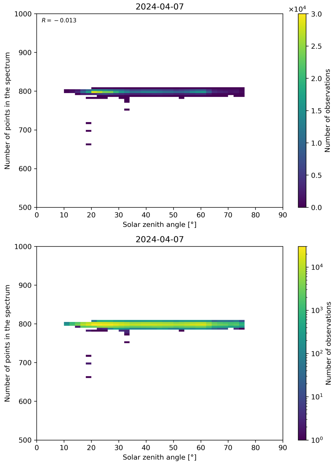
Figure 103: Scatter density plot of “Solar zenith angle” against “Number of points in the spectrum” for 2024-04-06 to 2024-04-08.
