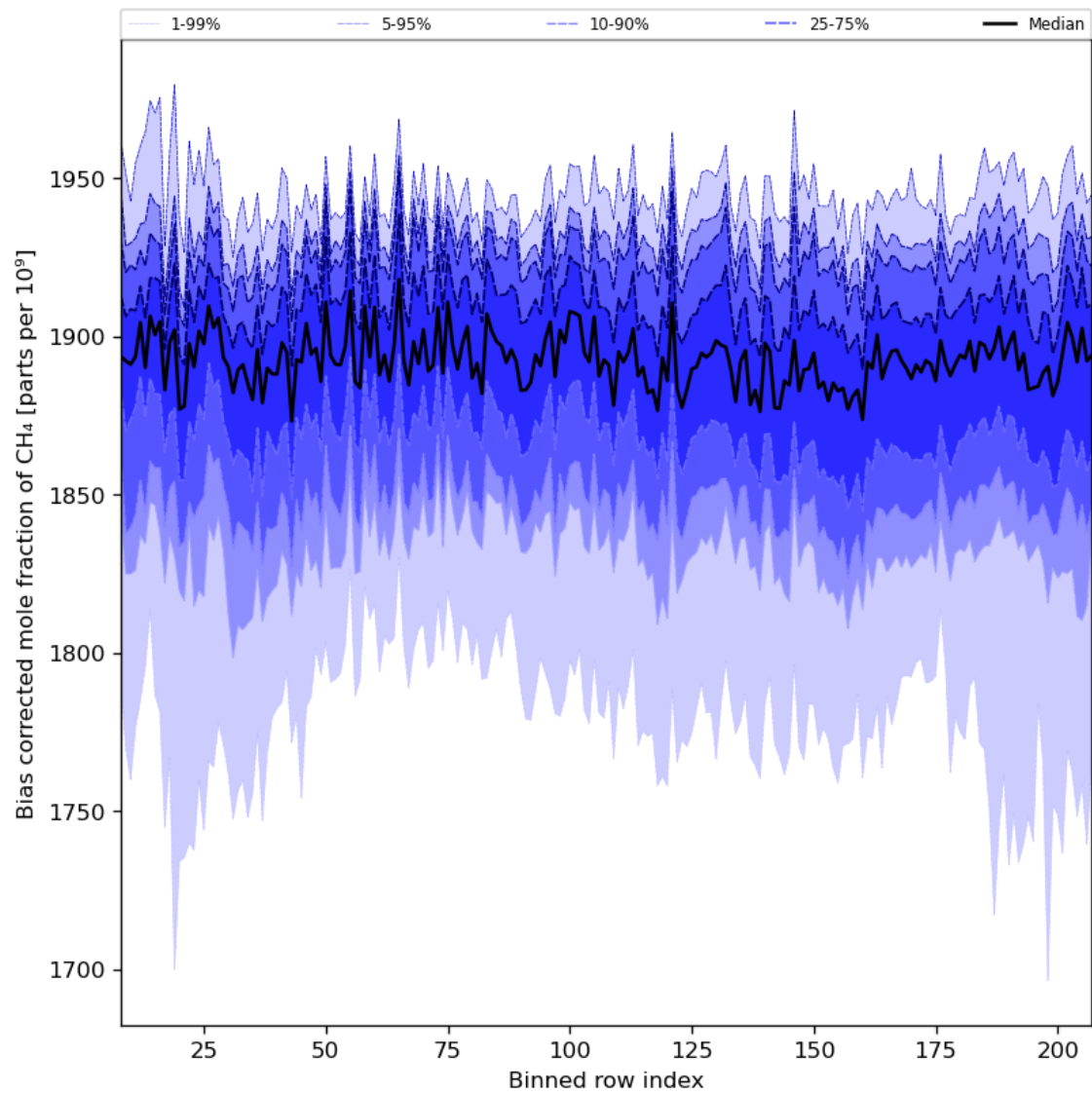
Figure 36: Along track statistics of “Bias corrected mole fraction of CH 4 ” for 2024-04-06 to 2024-04-08
