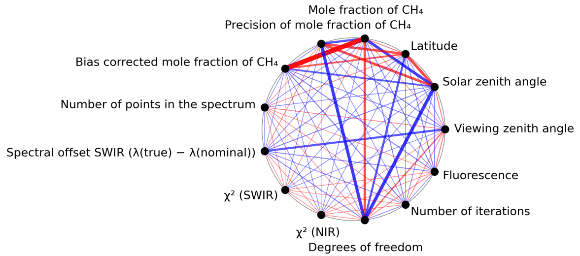
Figure 1: Map of correlation graph for 2024-04-06 to 2024-04-08.
