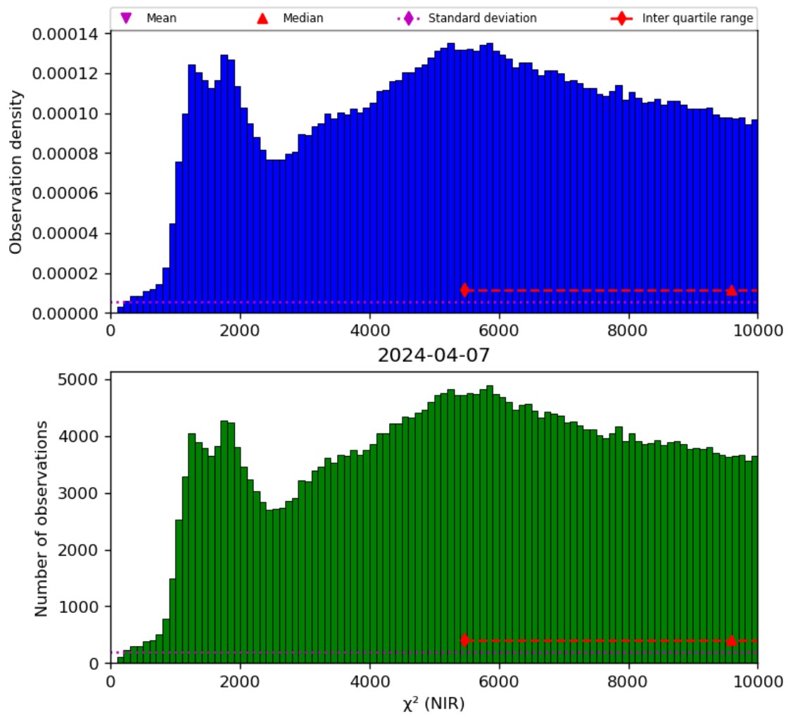
Figure 29: Histogram of “ \chi^2 (NIR)” for 2024-04-06 to 2024-04-08
