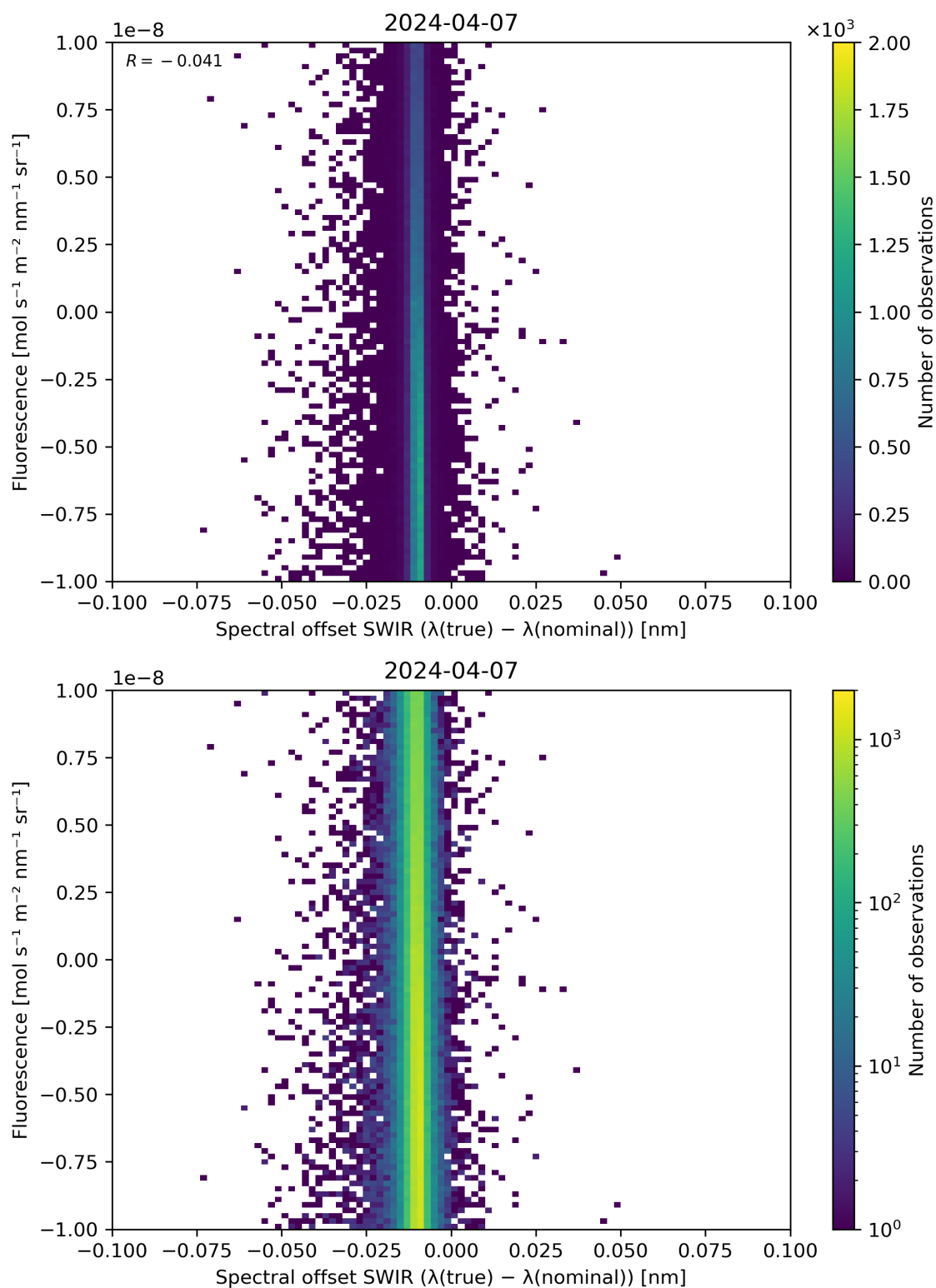
Figure 120: Scatter density plot of “Spectral offset SWIR ( \lambda(\text{true}) - \lambda(\text{nominal}) )” against “Fluorescence” for 2024-04-06 to 2024-04-08.
