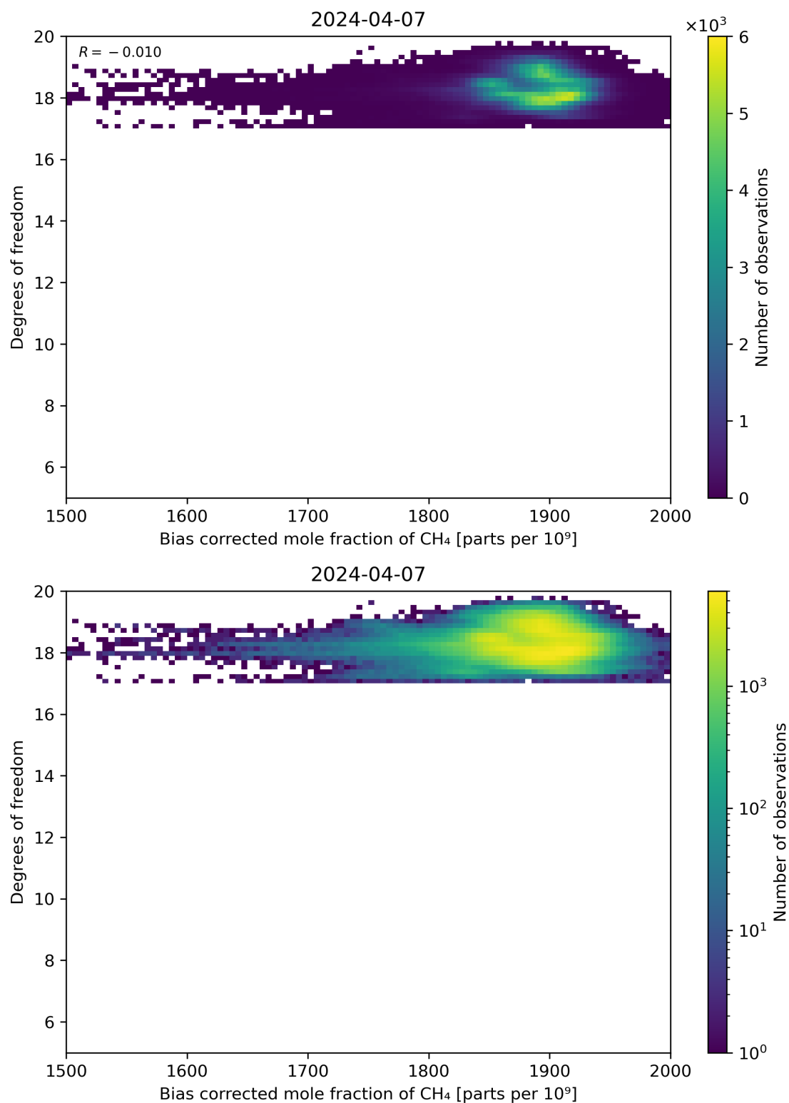
Figure 65: Scatter density plot of “Bias corrected mole fraction of CH 4 ” against “Degrees of freedom” for 2024-04-06 to 2024-04-08.
