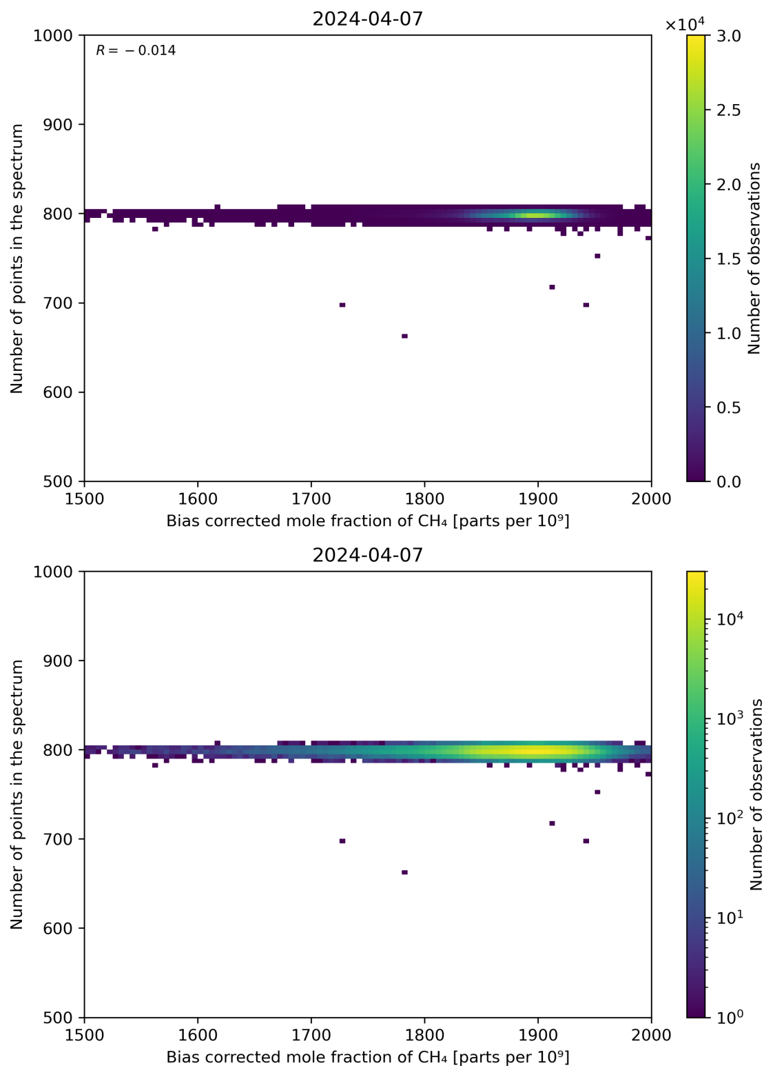
Figure 68: Scatter density plot of “Bias corrected mole fraction of CH 4 ” against “Number of points in the spectrum” for 2024-04-06 to 2024-04-08.
