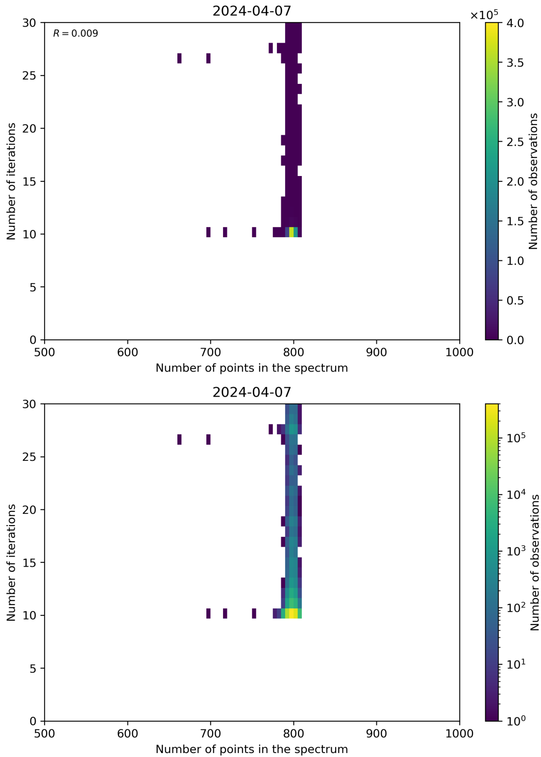
Figure 92: Scatter density plot of “Number of points in the spectrum” against “Number of iterations” for 2024-04-06 to 2024-04-08.
