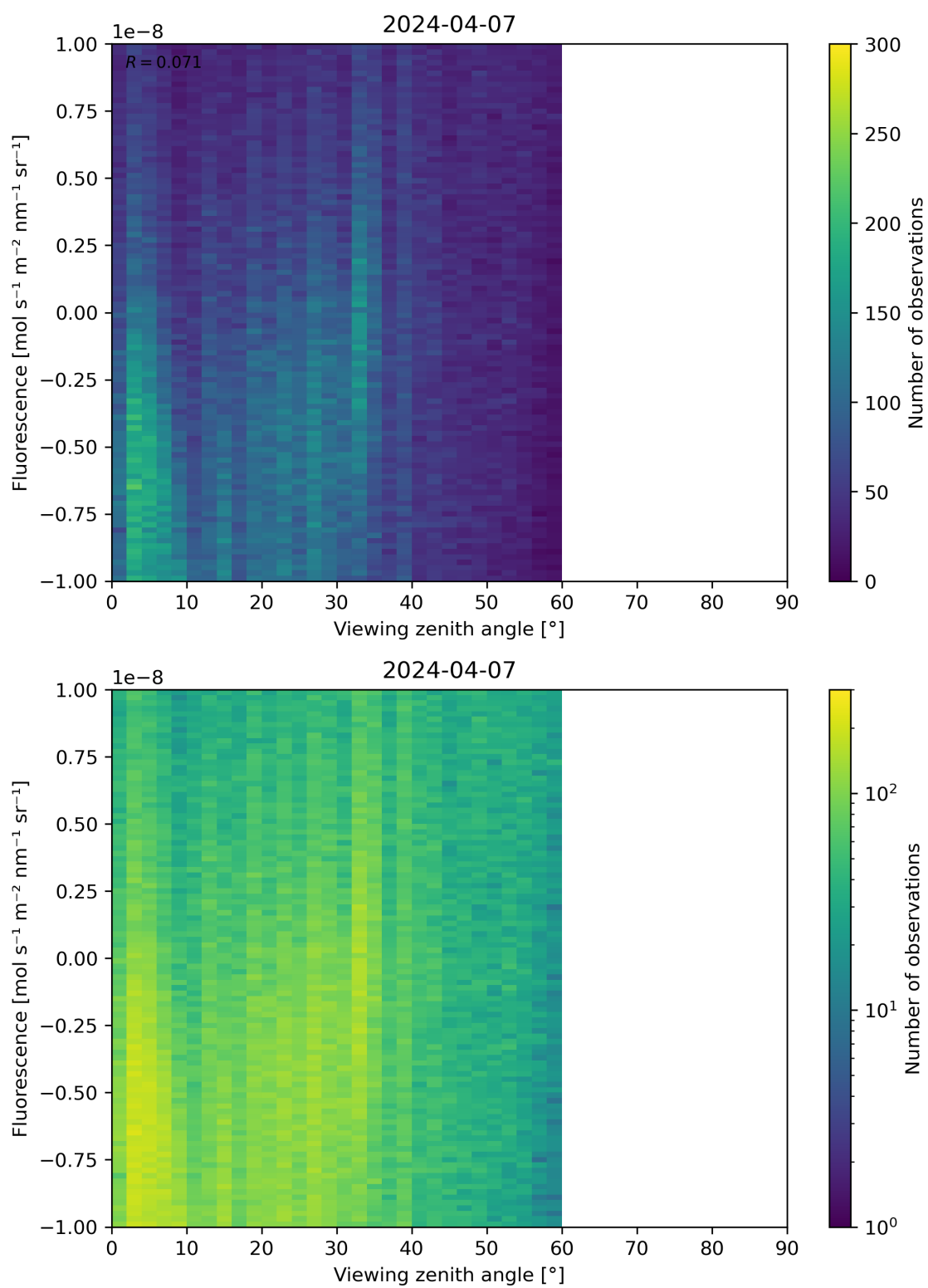
Figure 108: Scatter density plot of “Viewing zenith angle” against “Fluorescence” for 2024-04-06 to 2024-04-08.
