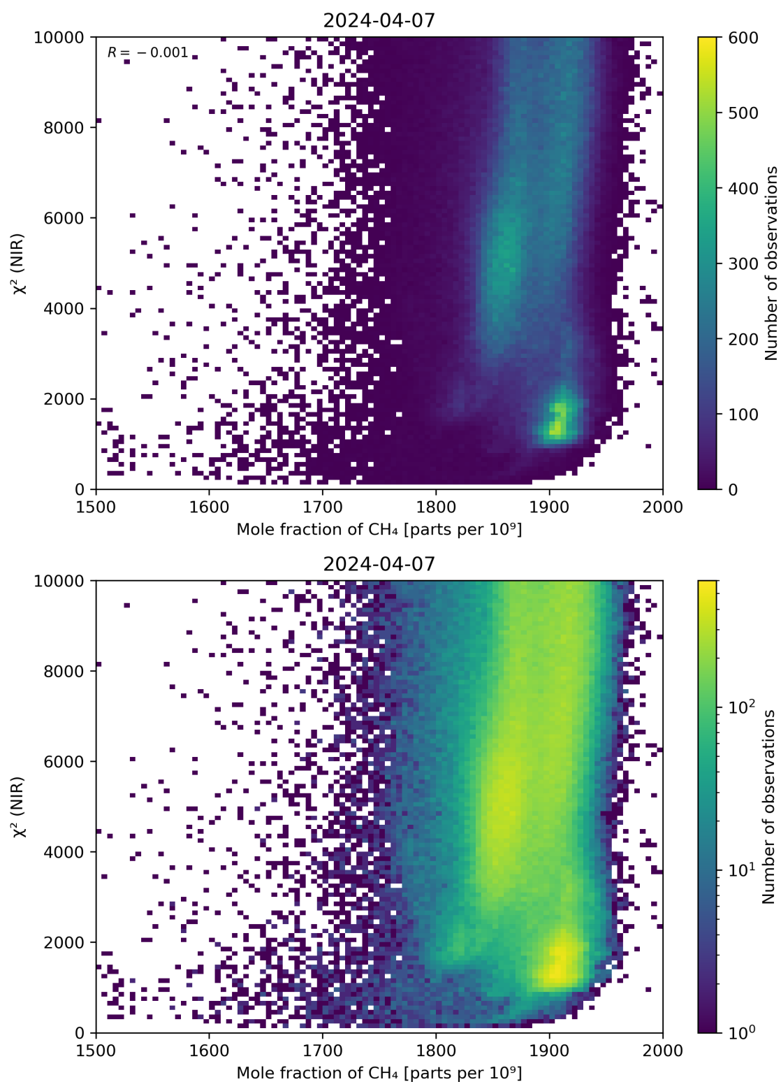
Figure 70: Scatter density plot of “Mole fraction of CH 4 ” against “ \chi^2 (NIR)” for 2024-04-06 to 2024-04-08.
