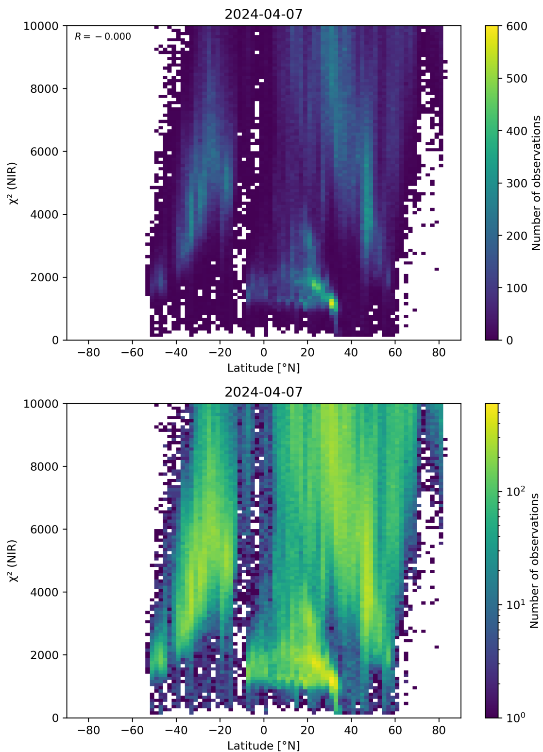
Figure 53: Scatter density plot of “Latitude” against “ \chi^2 (NIR)” for 2024-04-06 to 2024-04-08.
