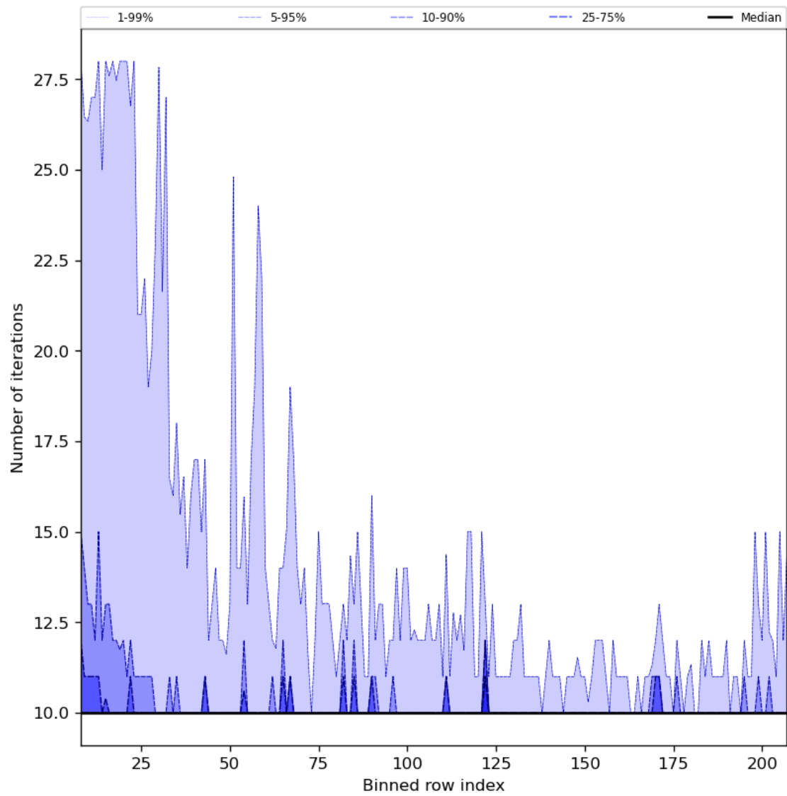
Figure 42: Along track statistics of “Number of iterations” for 2024-04-06 to 2024-04-08
