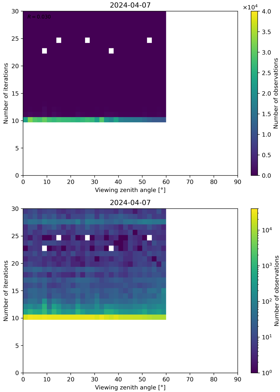
Figure 113: Scatter density plot of “Viewing zenith angle” against “Number of iterations” for 2024-04-06 to 2024-04-08.
