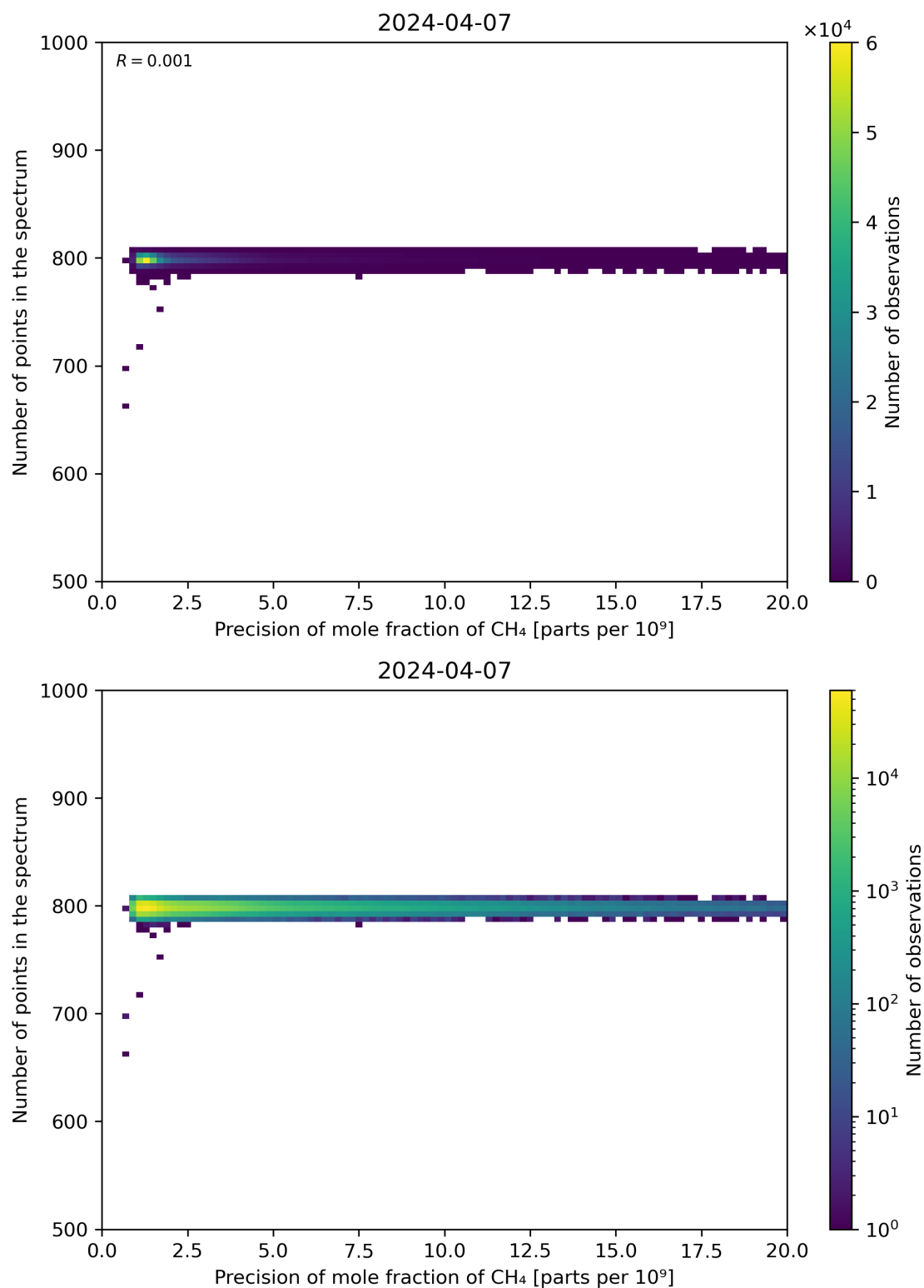
Figure 84: Scatter density plot of “Precision of mole fraction of CH 4 ” against “Number of points in the spectrum” for 2024-04-06 to 2024-04-08.
