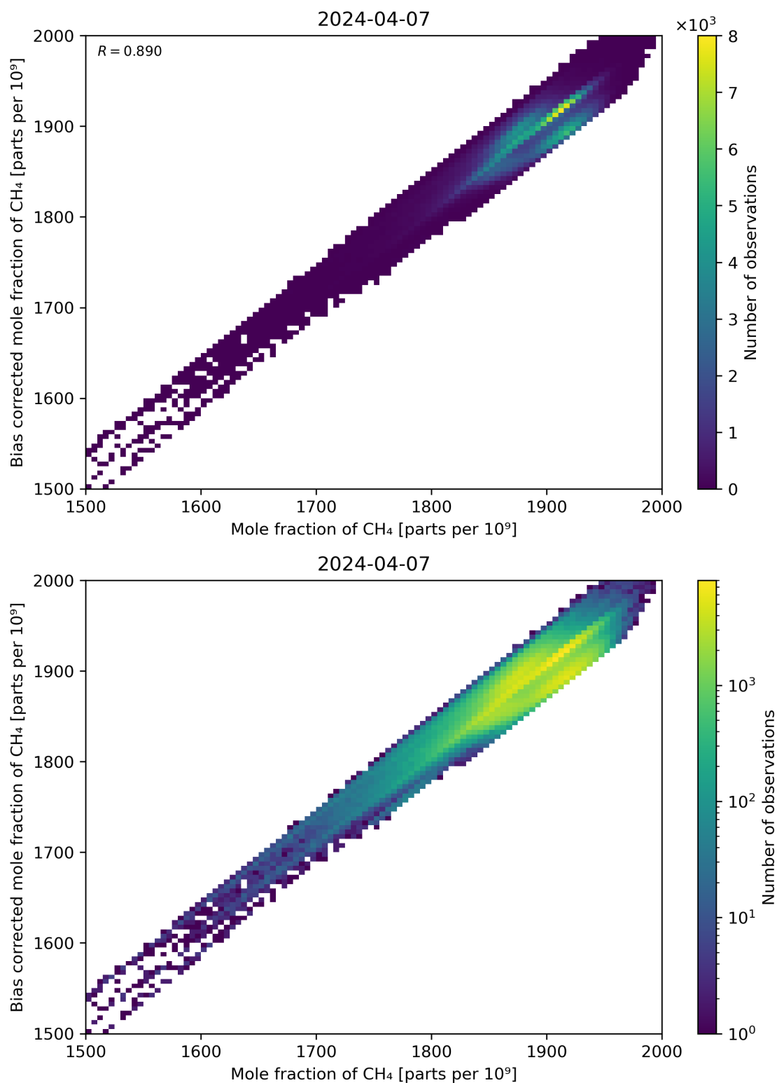
Figure 74: Scatter density plot of “Mole fraction of CH 4 ” against “Bias corrected mole fraction of CH 4 ” for 2024-04-06 to 2024-04-08.
