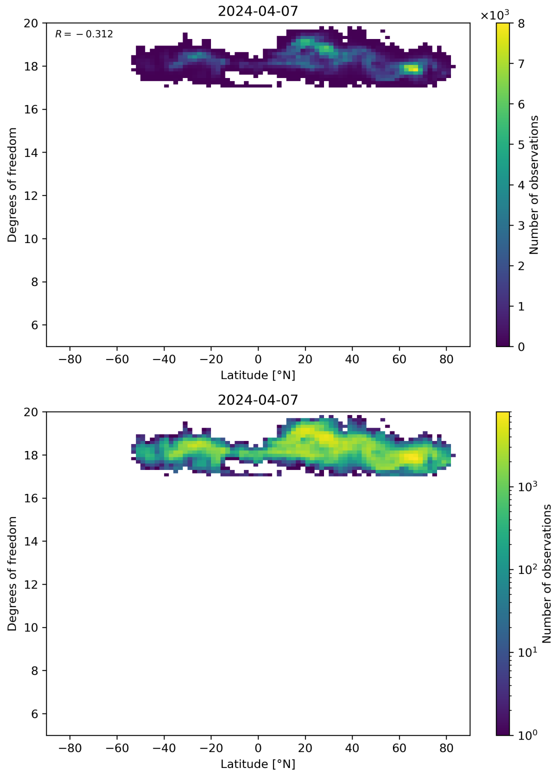
Figure 55: Scatter density plot of “Latitude” against “Degrees of freedom” for 2024-04-06 to 2024-04-08.
