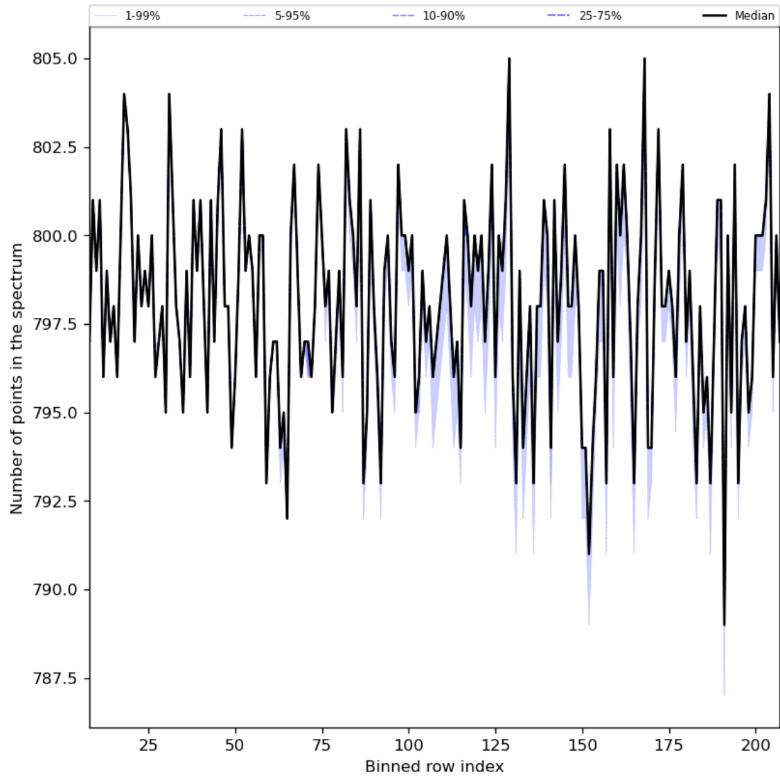
Figure 37: Along track statistics of “Number of points in the spectrum” for 2024-04-06 to 2024-04-08
