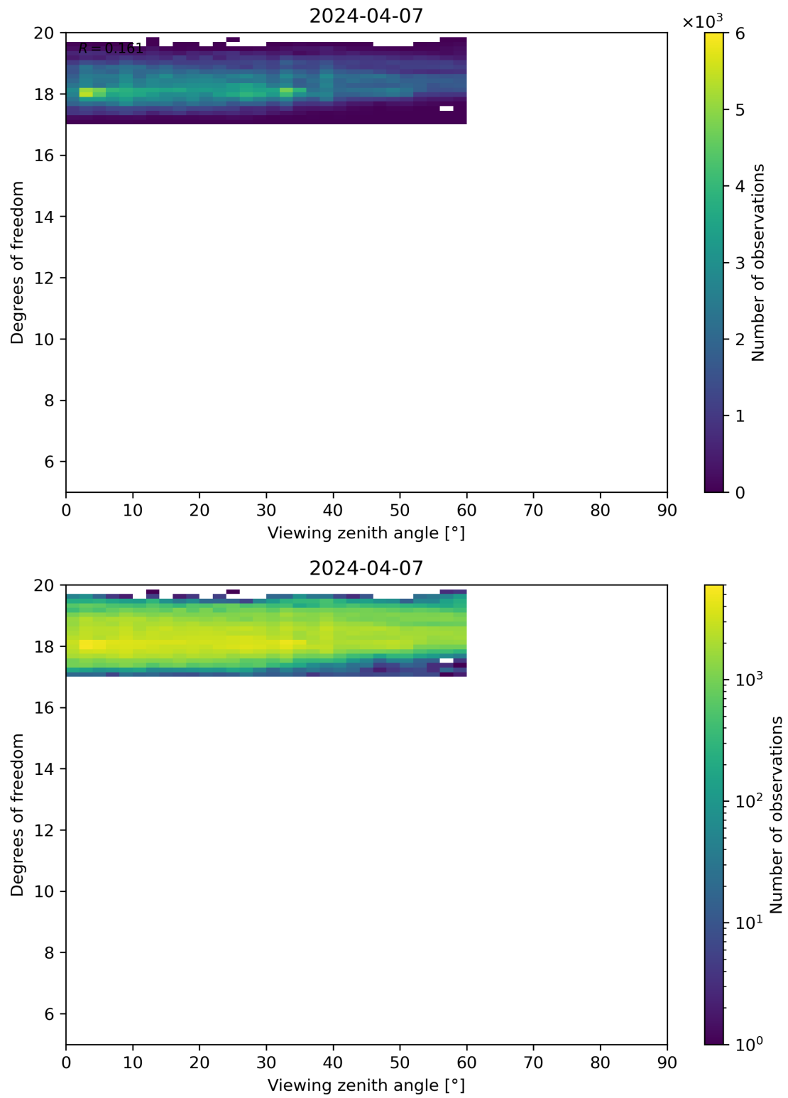
Figure 107: Scatter density plot of “Viewing zenith angle” against “Degrees of freedom” for 2024-04-06 to 2024-04-08.
