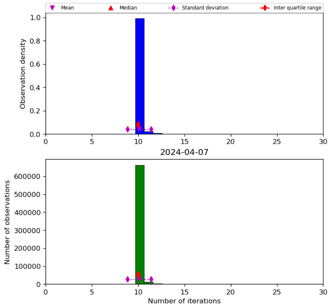
Figure 31: Histogram of “Number of iterations” for 2024-04-06 to 2024-04-08
