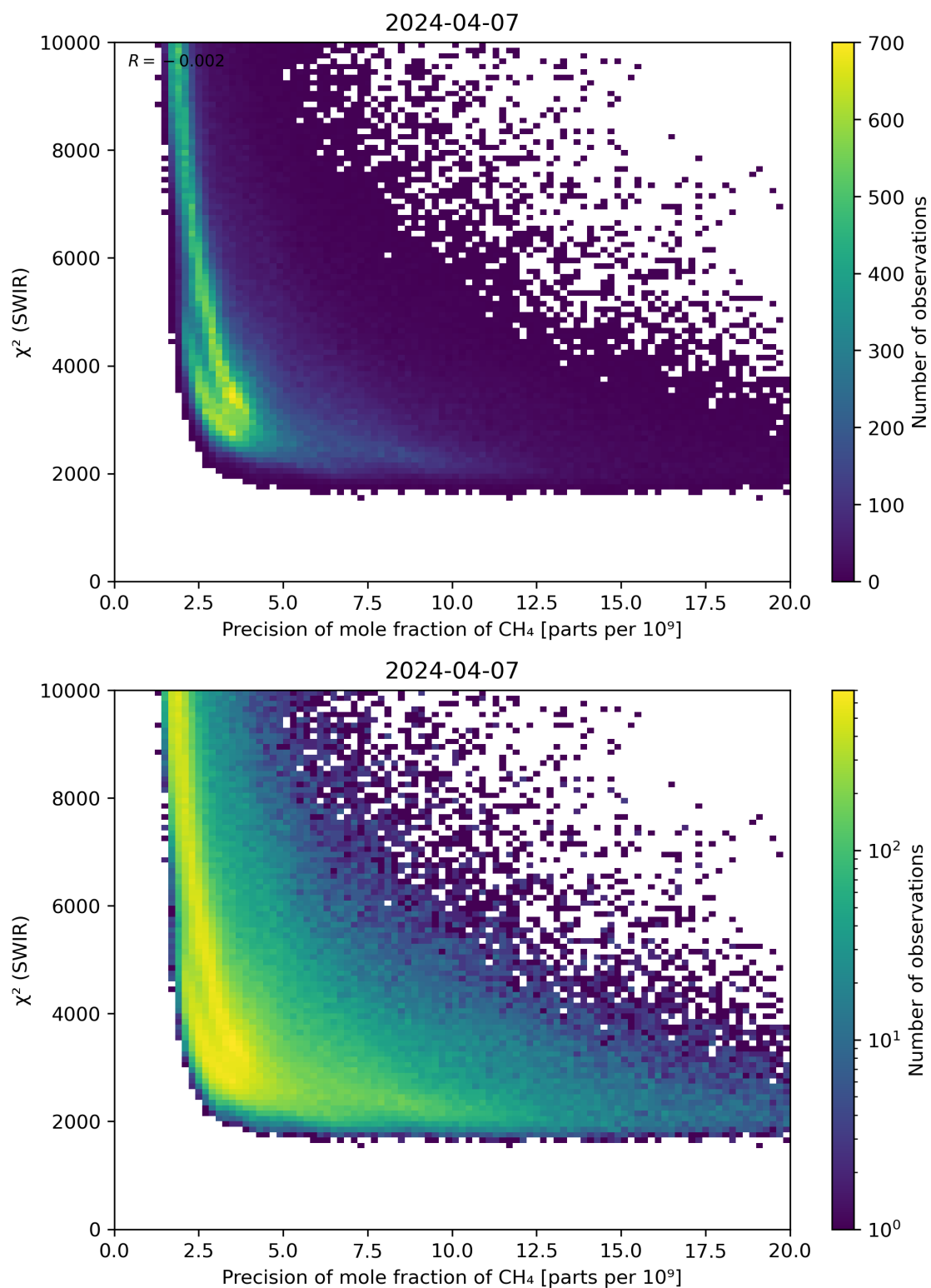
Figure 79: Scatter density plot of “Precision of mole fraction of \text{CH}_4 ” against “ \chi^2 (SWIR)” for 2024-04-06 to 2024-04-08.
