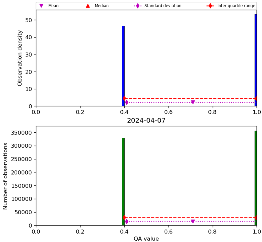
Figure 22: Histogram of “QA value” for 2024-04-06 to 2024-04-08
