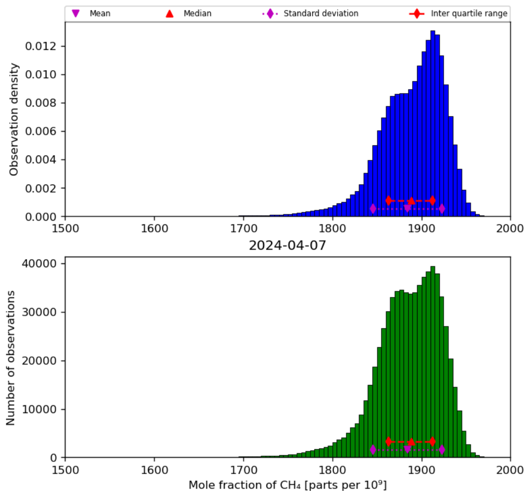
Figure 23: Histogram of “Mole fraction of CH 4 ” for 2024-04-06 to 2024-04-08
