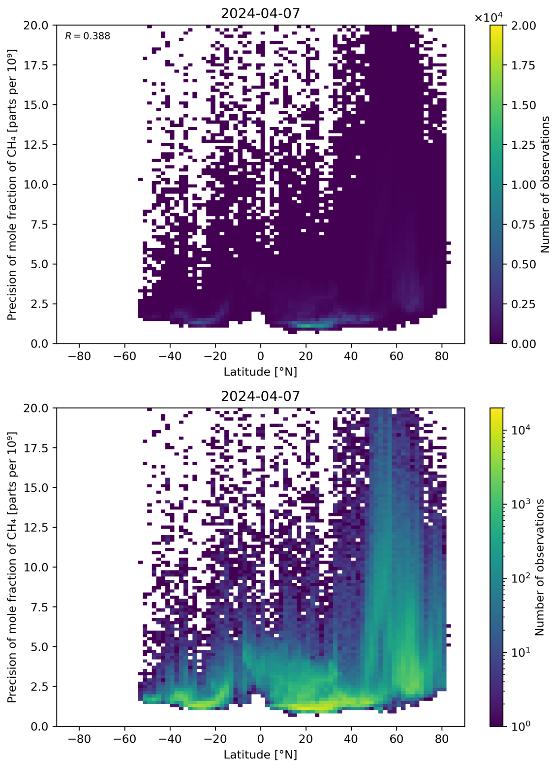
Figure 59: Scatter density plot of “Latitude” against “Precision of mole fraction of \text{CH}_4 ” for 2024-04-06 to 2024-04-08.
