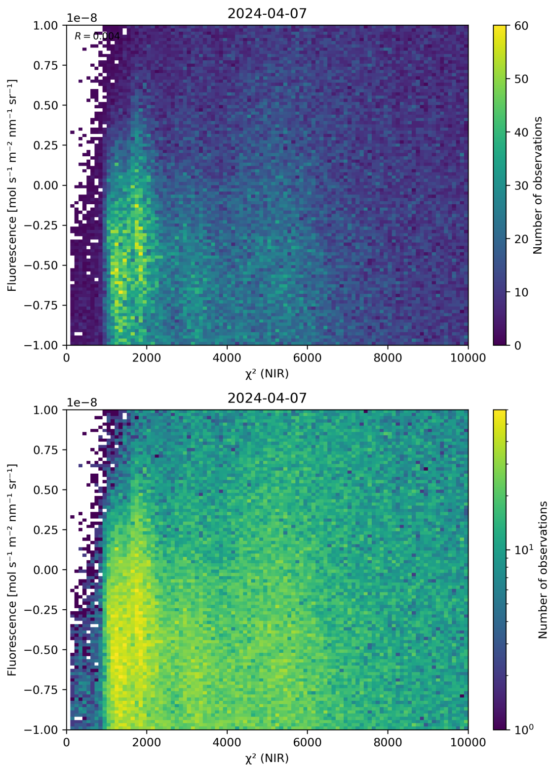
Figure 45: Scatter density plot of “ \chi^2 (NIR)” against “Fluorescence” for 2024-04-06 to 2024-04-08.
