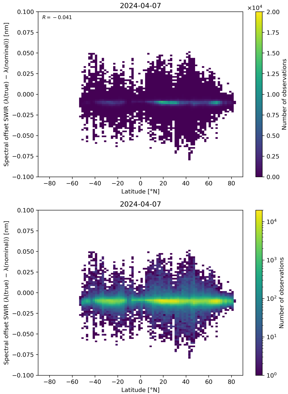
Figure 62: Scatter density plot of “Latitude” against “Spectral offset SWIR ( \lambda(\text{true}) - \lambda(\text{nominal}) )” for 2024-04-06 to 2024-04-08.
