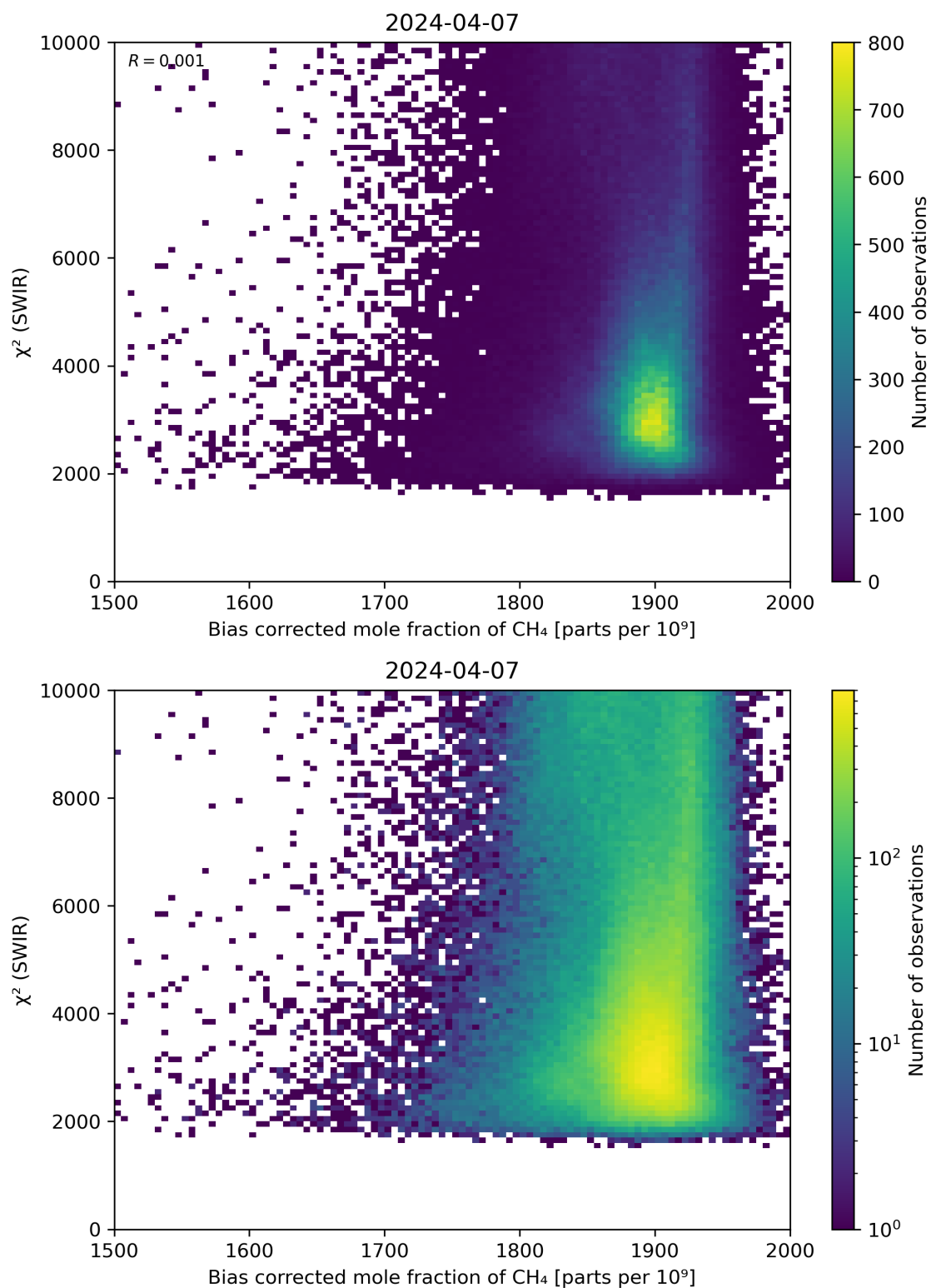
Figure 64: Scatter density plot of “Bias corrected mole fraction of CH 4 ” against “ \chi^2 (SWIR)” for 2024-04-06 to 2024-04-08.
