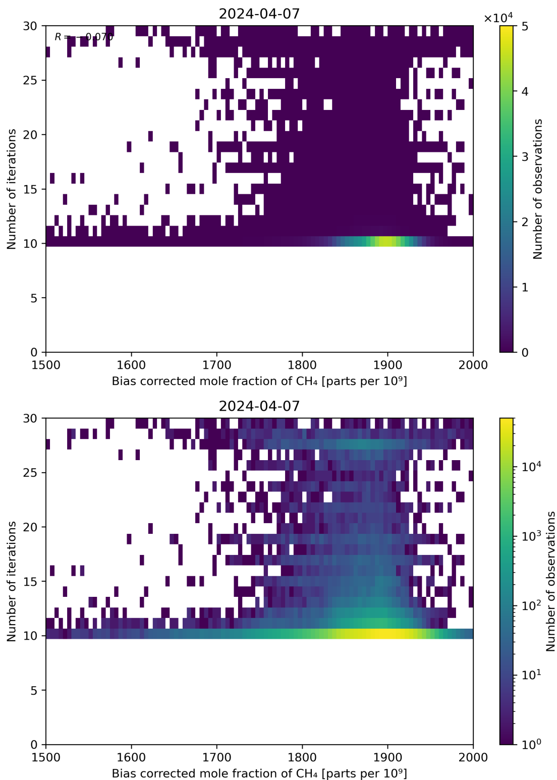
Figure 67: Scatter density plot of “Bias corrected mole fraction of CH 4 ” against “Number of iterations” for 2024-04-06 to 2024-04-08.
