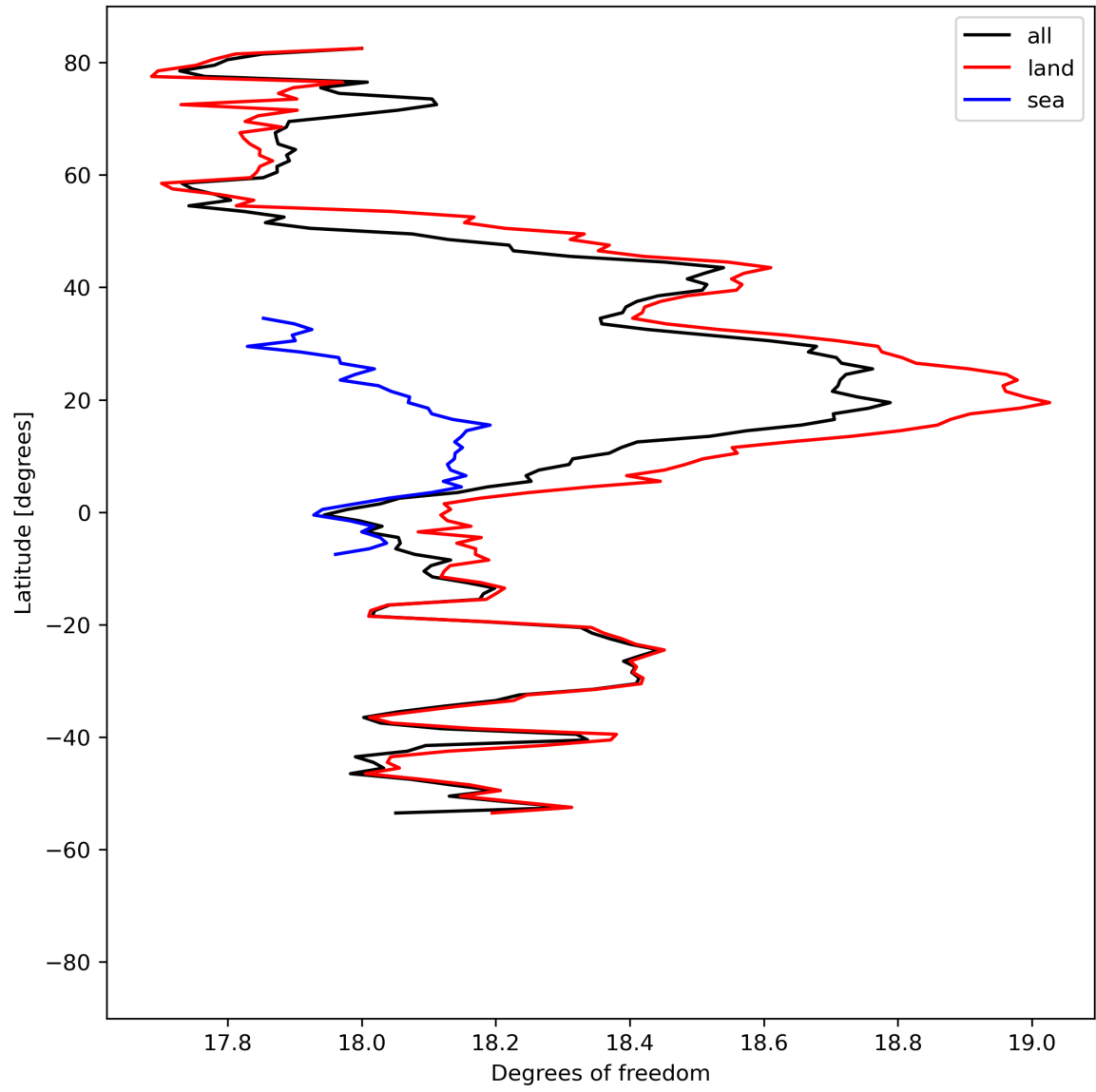
Figure 19: Zonal average of “Degrees of freedom” for 2024-04-06 to 2024-04-08.
