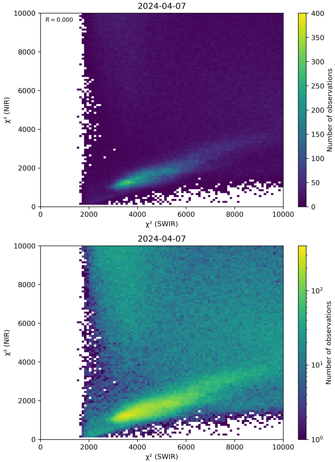
Figure 47: Scatter density plot of “ \chi^2 (SWIR)” against “ \chi^2 (NIR)” for 2024-04-06 to 2024-04-08.
