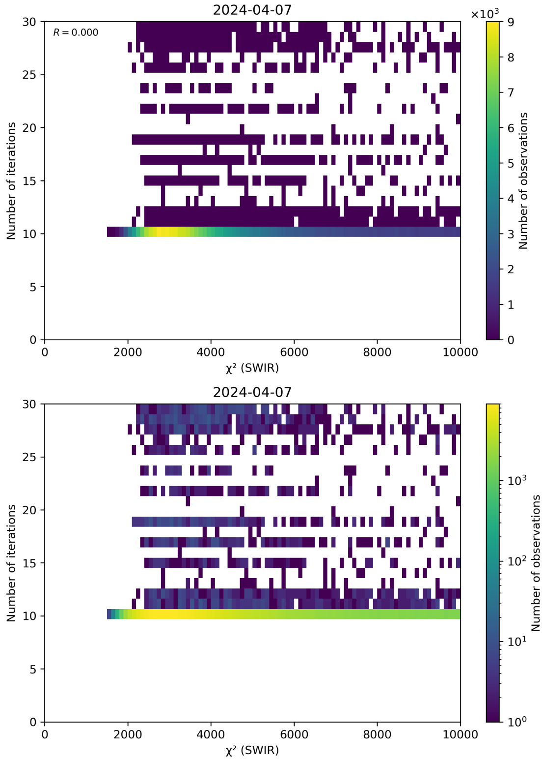
Figure 50: Scatter density plot of “ \chi^2 (SWIR)” against “Number of iterations” for 2024-04-06 to 2024-04-08.
