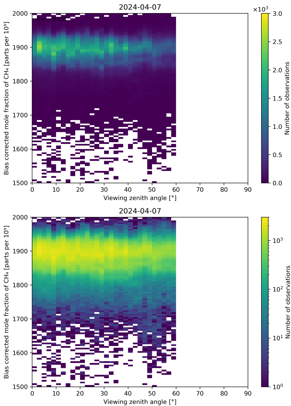
Figure 111: Scatter density plot of “Viewing zenith angle” against “Bias corrected mole fraction of CH 4 ” for 2024-04-06 to 2024-04-08.
