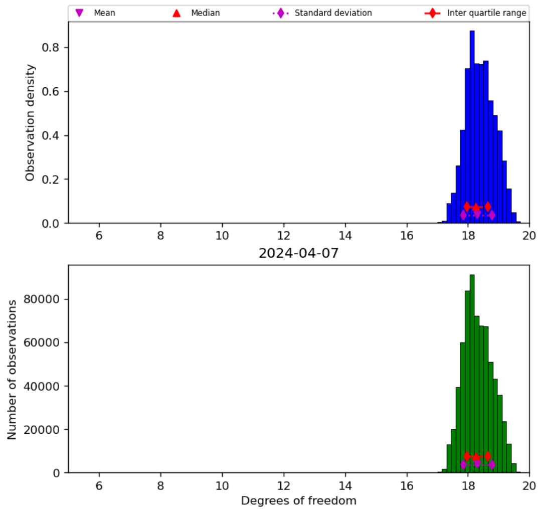
Figure 30: Histogram of “Degrees of freedom” for 2024-04-06 to 2024-04-08
