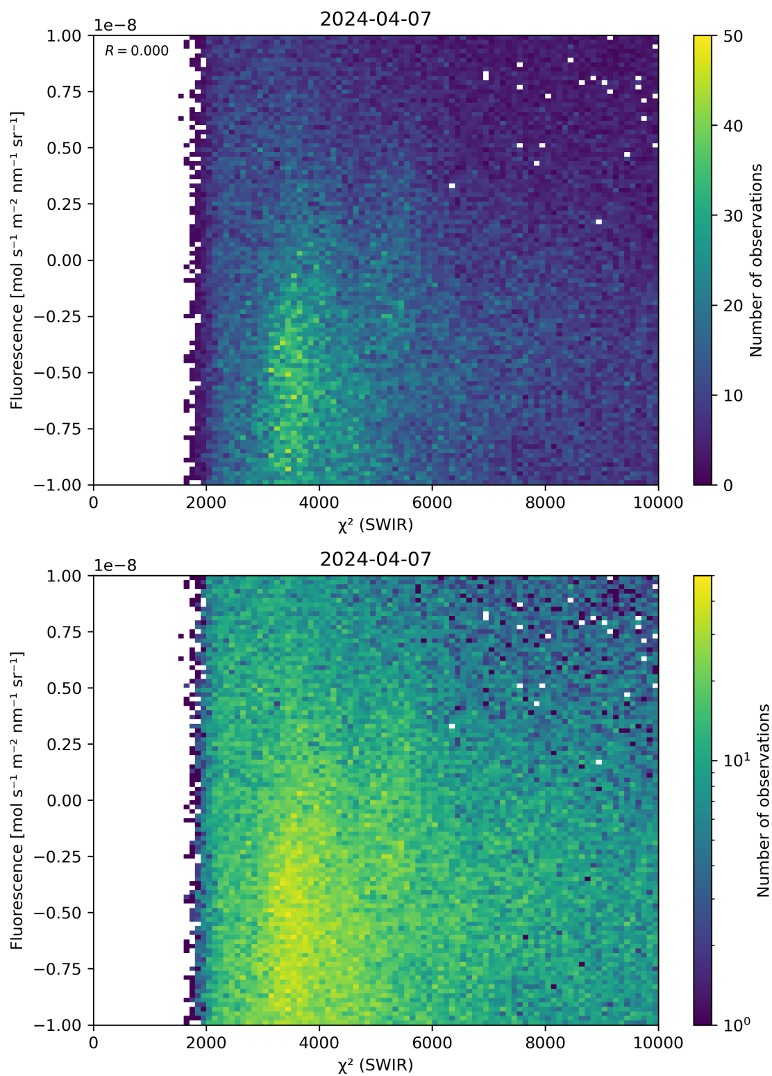
Figure 49: Scatter density plot of “ \chi^2 (SWIR)” against “Fluorescence” for 2024-04-06 to 2024-04-08.
