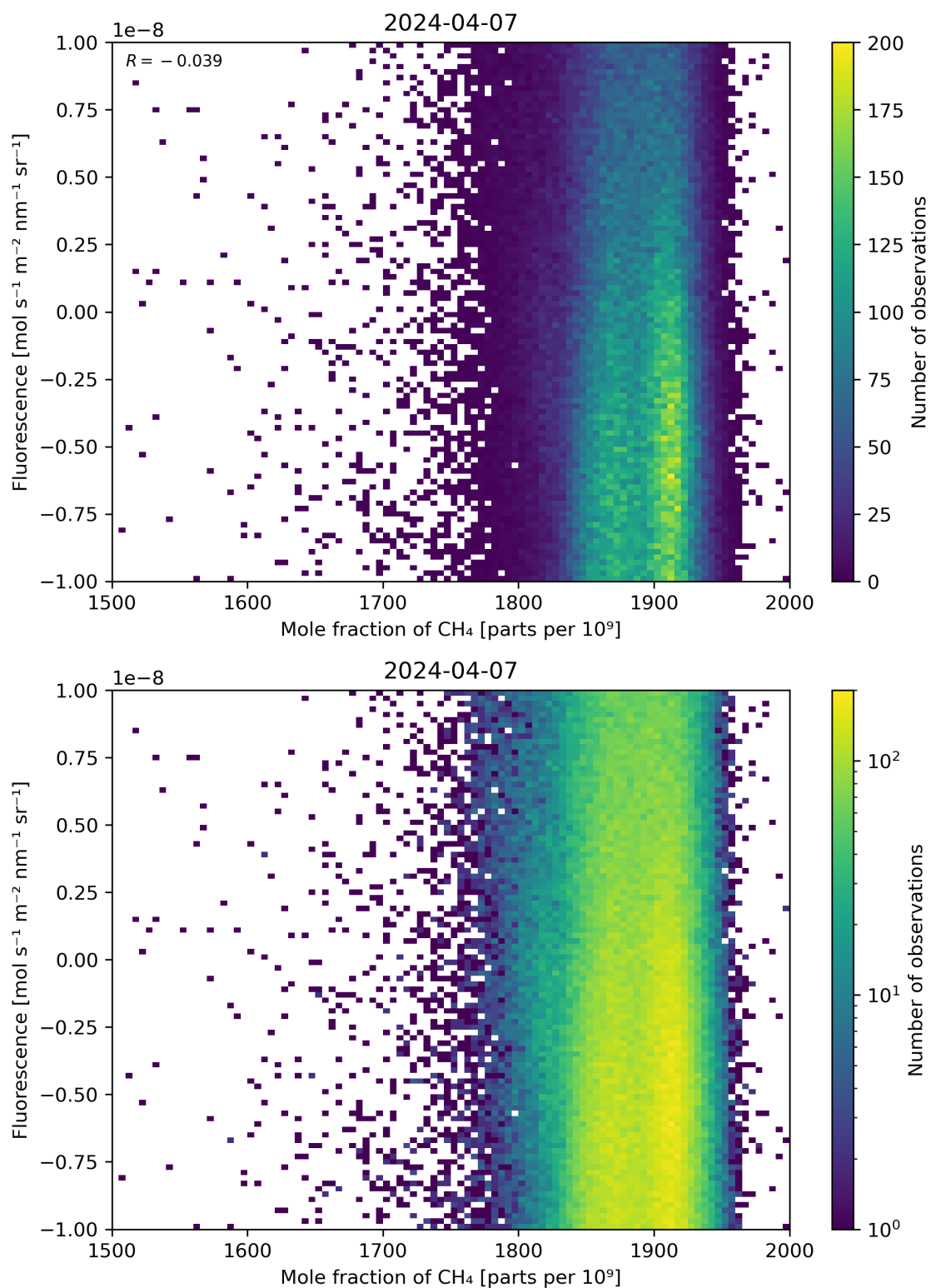
Figure 73: Scatter density plot of “Mole fraction of \text{CH}_4 ” against “Fluorescence” for 2024-04-06 to 2024-04-08.
