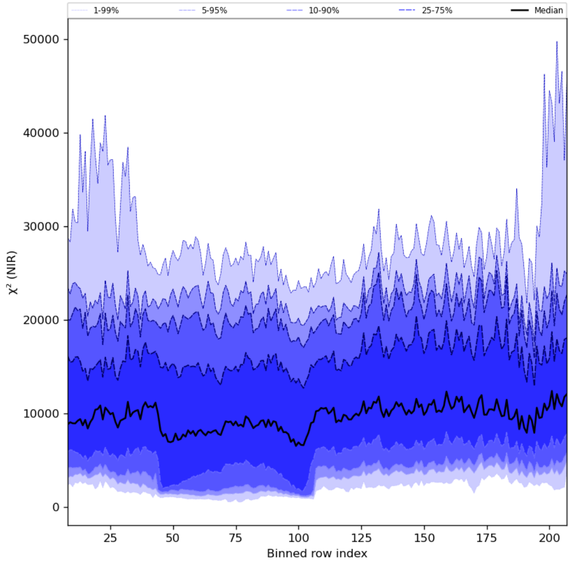
Figure 40: Along track statistics of “ \chi^2 (NIR)” for 2024-04-06 to 2024-04-08
