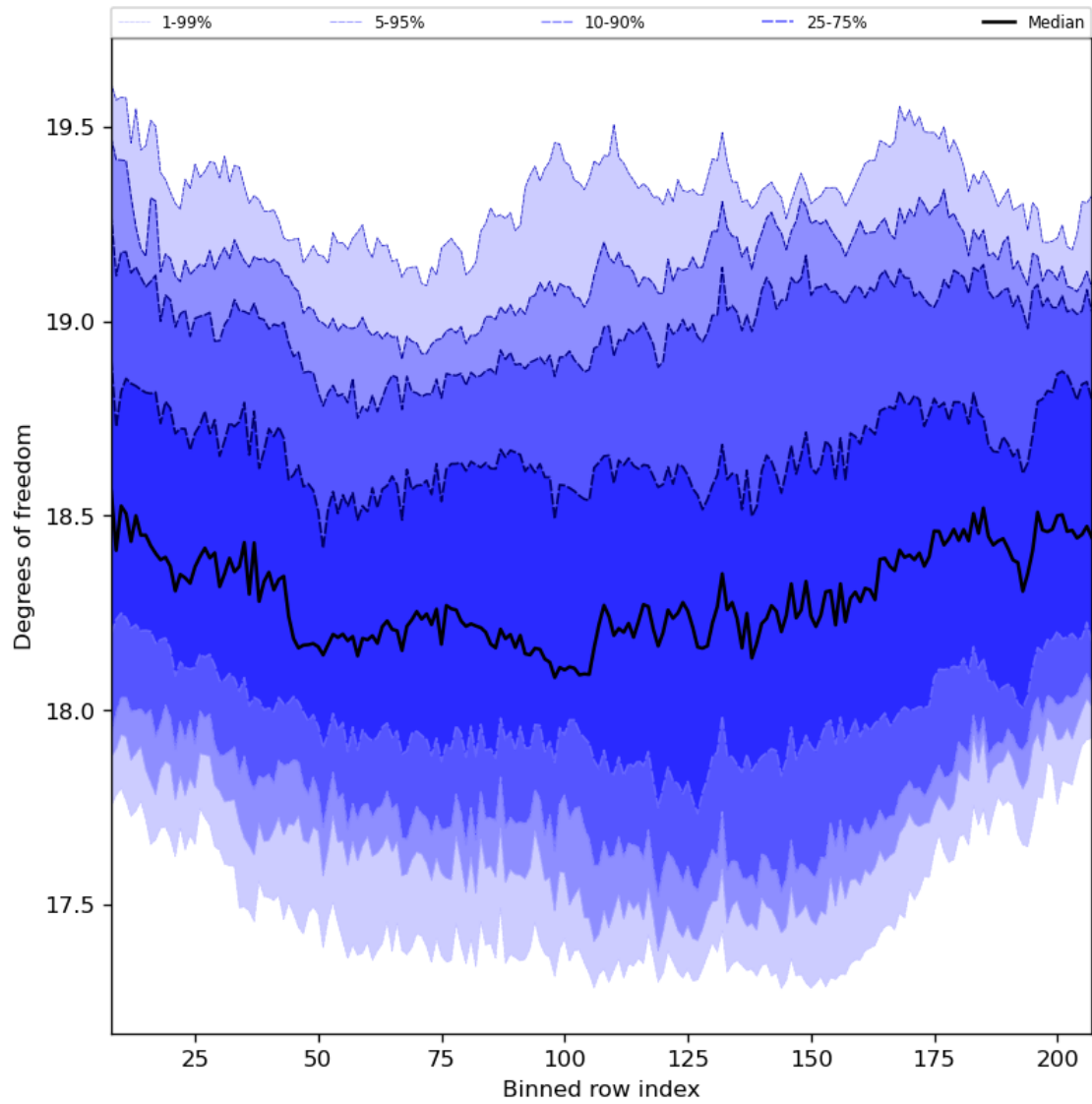
Figure 41: Along track statistics of “Degrees of freedom” for 2024-04-06 to 2024-04-08
