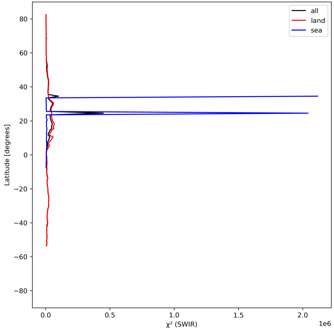
Figure 17: Zonal average of “ \chi^2 (SWIR)” for 2024-04-06 to 2024-04-08.
