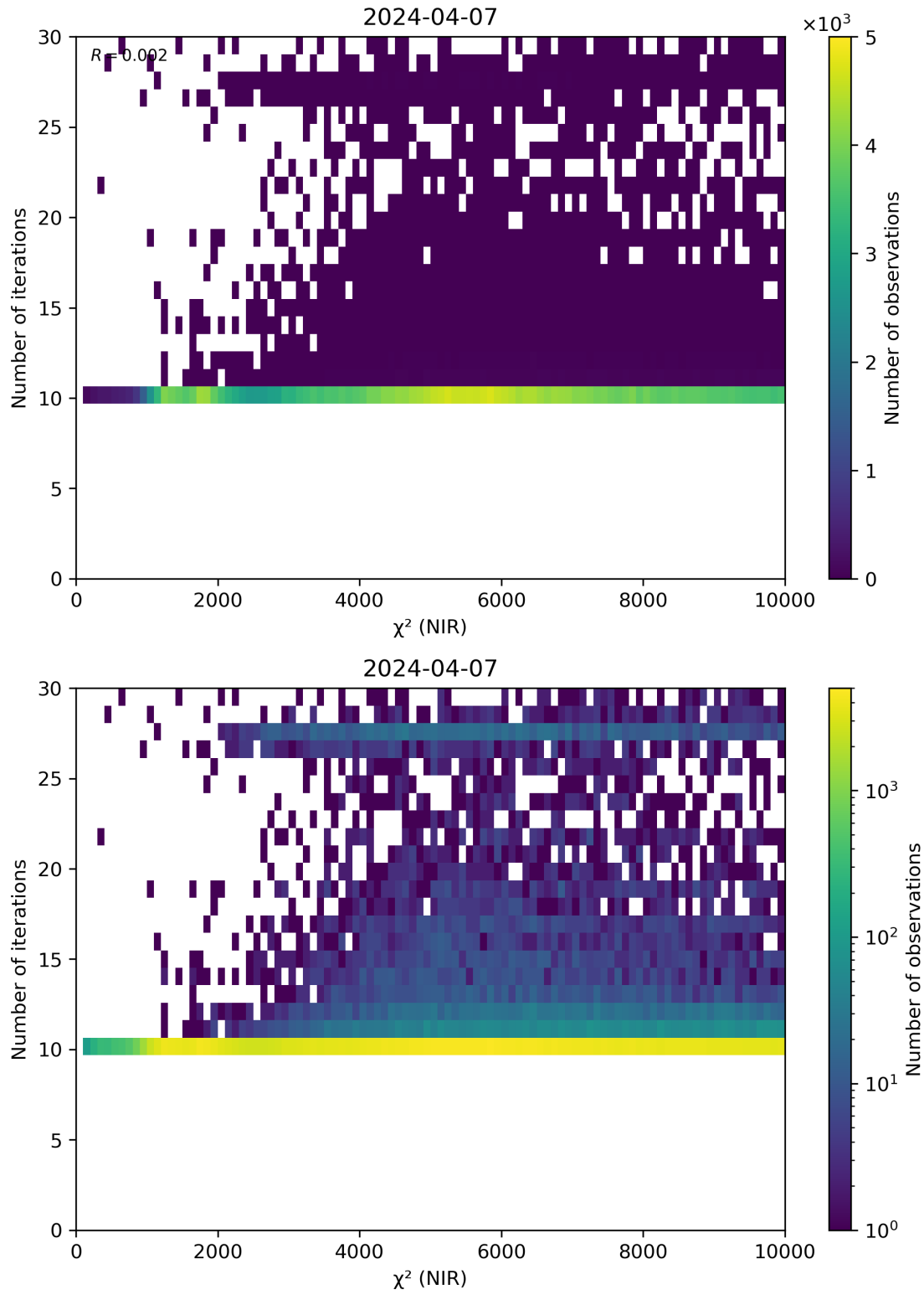
Figure 46: Scatter density plot of “ \chi^2 (NIR)” against “Number of iterations” for 2024-04-06 to 2024-04-08.
