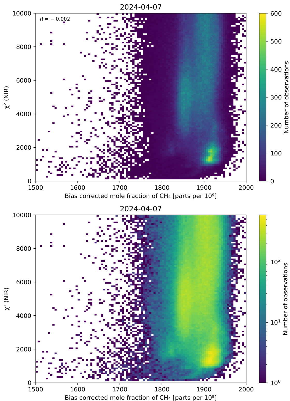
Figure 63: Scatter density plot of “Bias corrected mole fraction of CH 4 ” against “ \chi^2 (NIR)” for 2024-04-06 to 2024-04-08.
