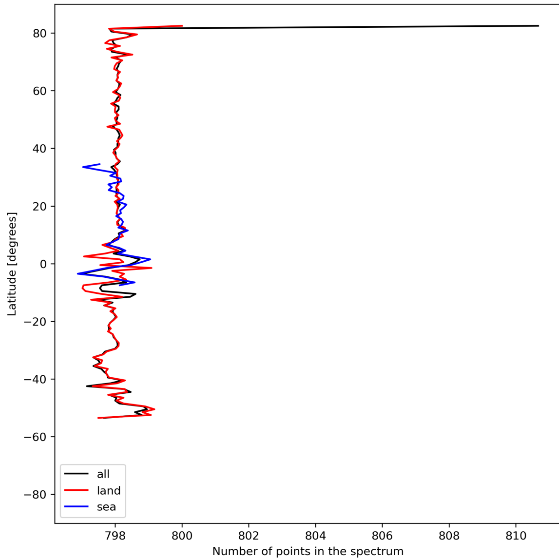
Figure 15: Zonal average of “Number of points in the spectrum” for 2024-04-06 to 2024-04-08.
