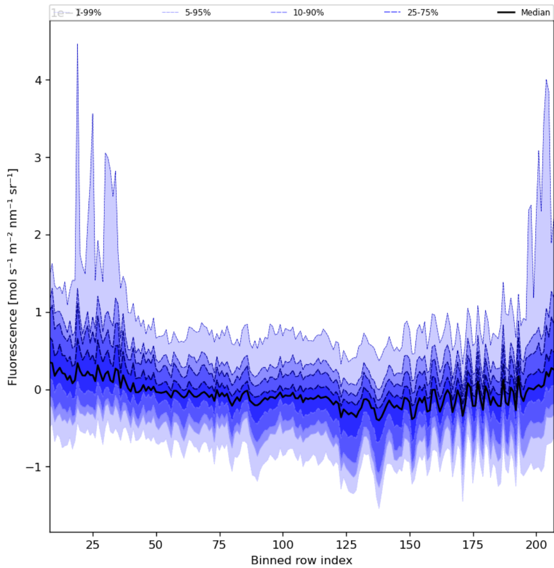
Figure 43: Along track statistics of “Fluorescence” for 2024-04-06 to 2024-04-08
