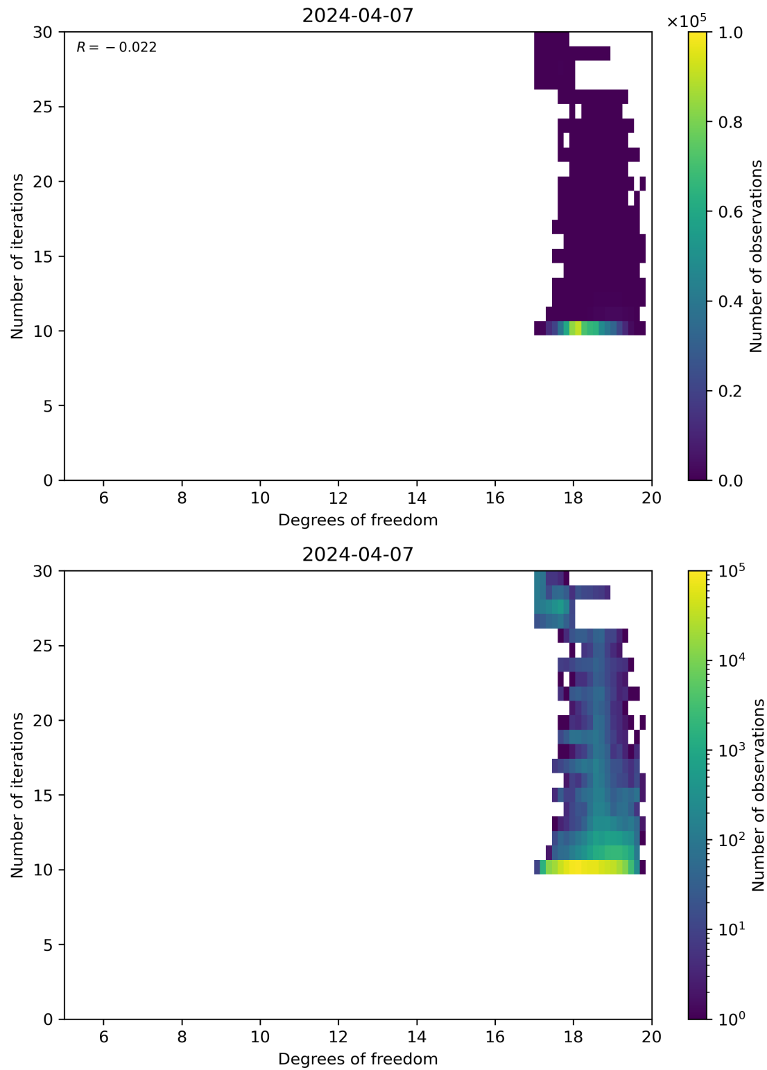
Figure 52: Scatter density plot of “Degrees of freedom” against “Number of iterations” for 2024-04-06 to 2024-04-08.
