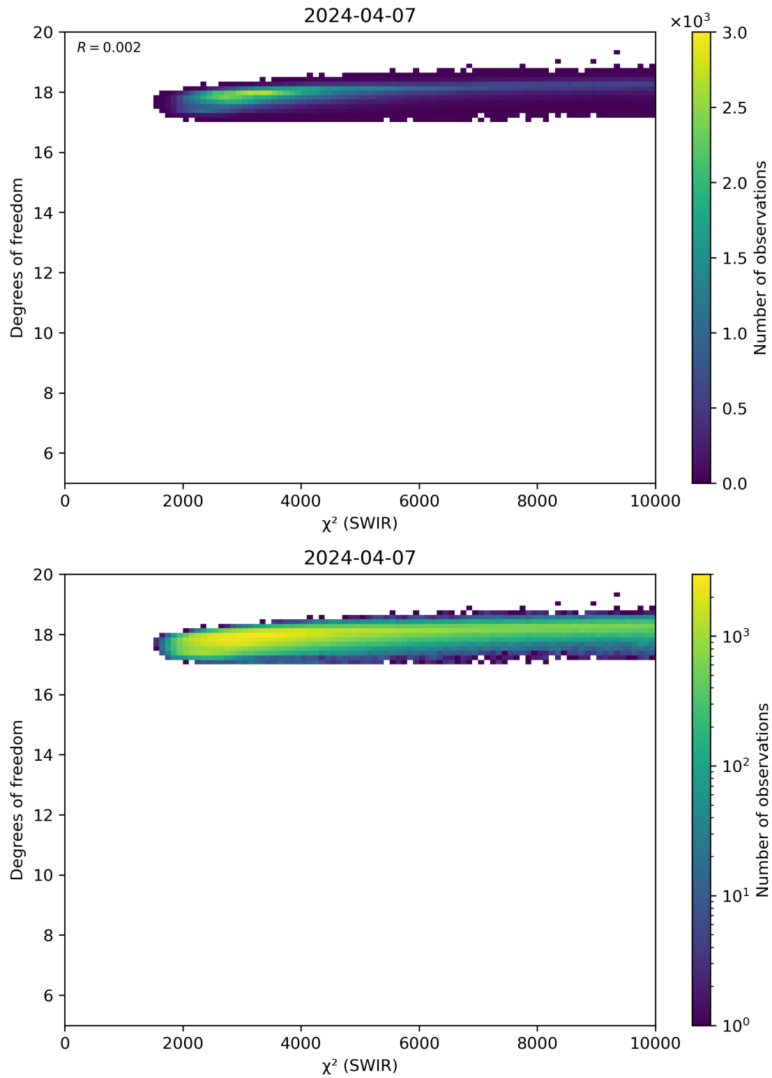
Figure 48: Scatter density plot of “ \chi^2 (SWIR)” against “Degrees of freedom” for 2024-04-06 to 2024-04-08.
