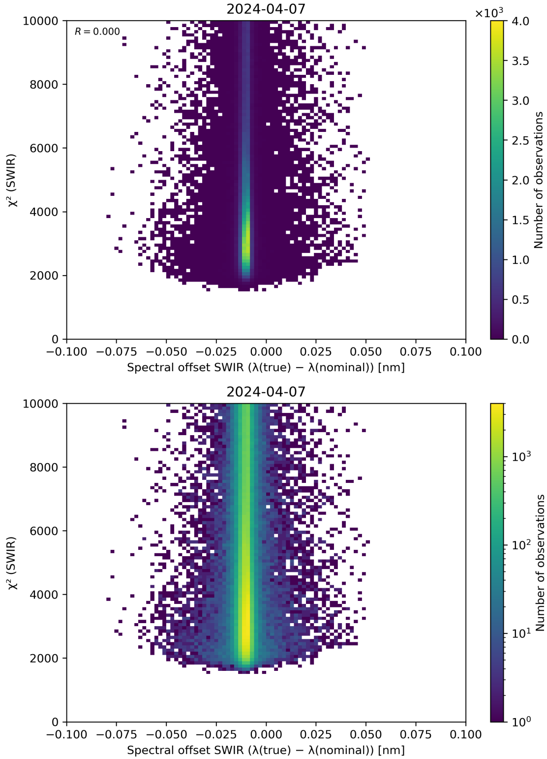
Figure 118: Scatter density plot of “Spectral offset SWIR ( \lambda(\text{true}) - \lambda(\text{nominal}) )” against “ \chi^2 (SWIR)” for 2024-04-06 to 2024-04-08.
