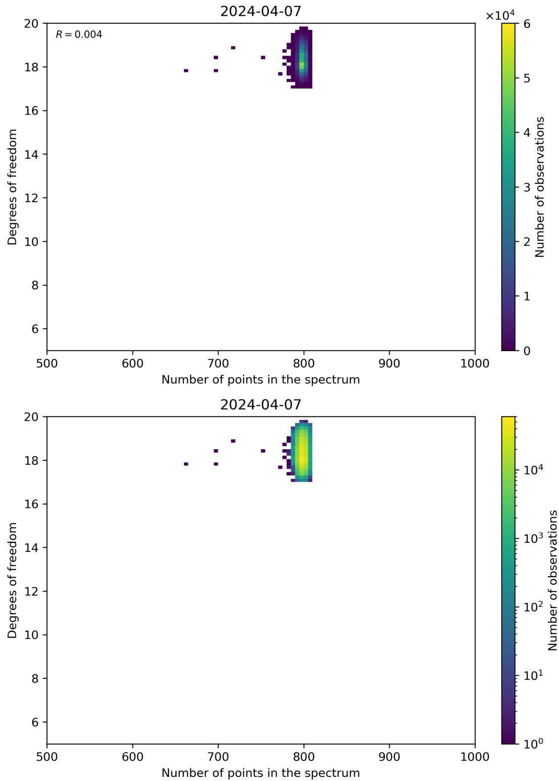
Figure 90: Scatter density plot of “Number of points in the spectrum” against “Degrees of freedom” for 2024-04-06 to 2024-04-08.
