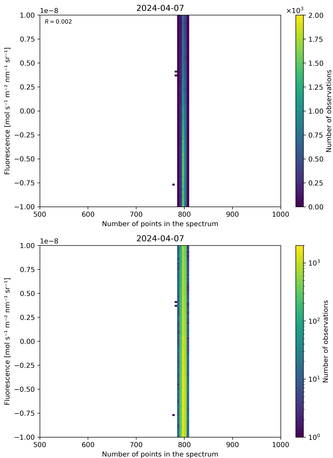
Figure 91: Scatter density plot of “Number of points in the spectrum” against “Fluorescence” for 2024-04-06 to 2024-04-08.
