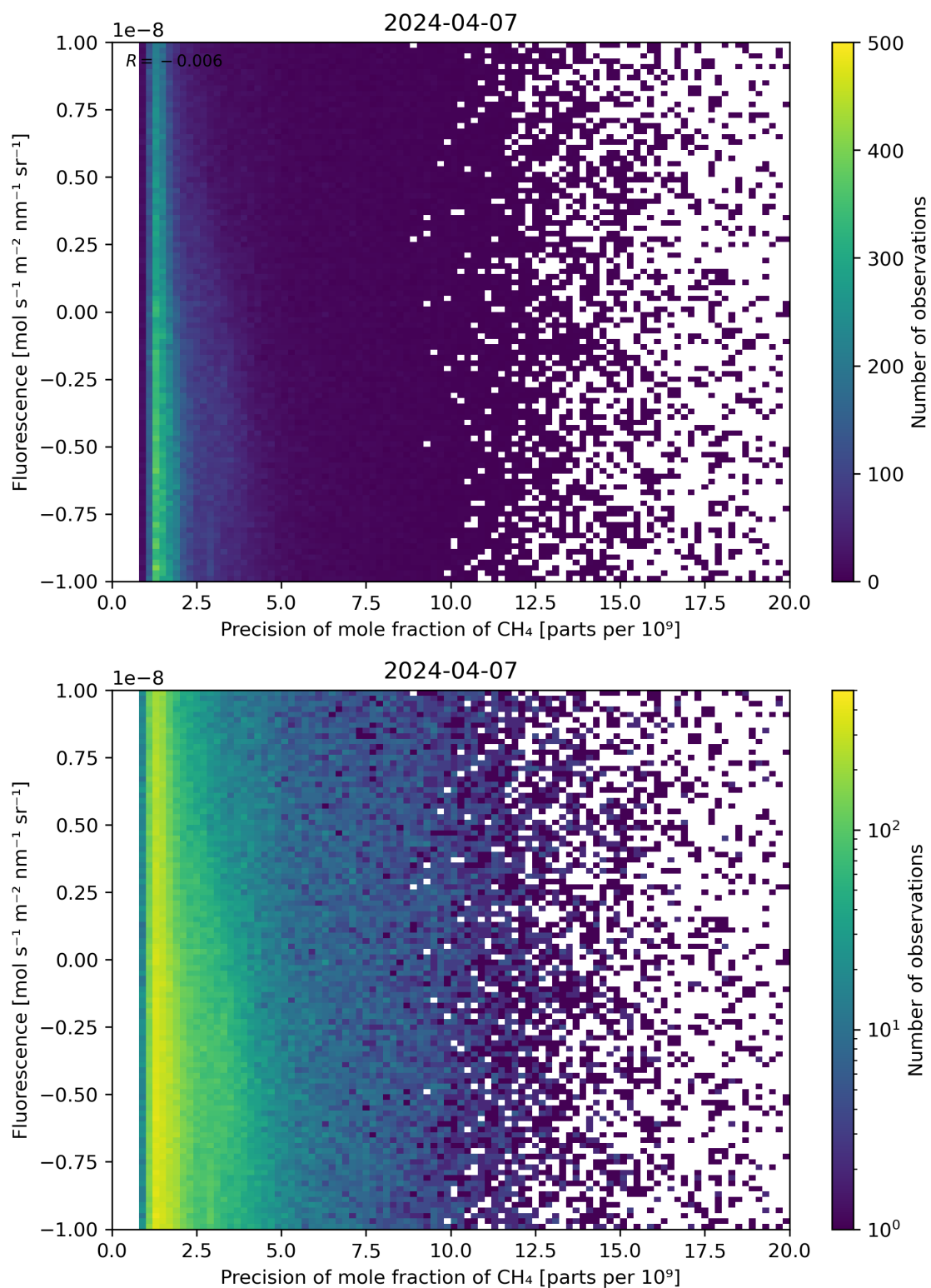
Figure 81: Scatter density plot of “Precision of mole fraction of CH 4 ” against “Fluorescence” for 2024-04-06 to 2024-04-08.
