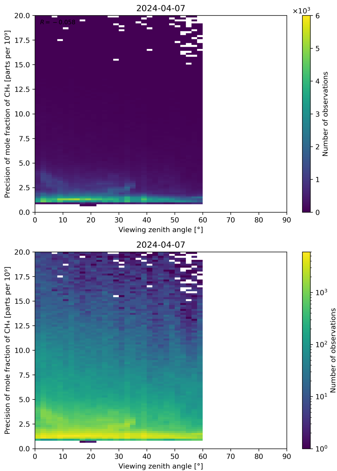
Figure 112: Scatter density plot of “Viewing zenith angle” against “Precision of mole fraction of CH 4 ” for 2024-04-06 to 2024-04-08.
