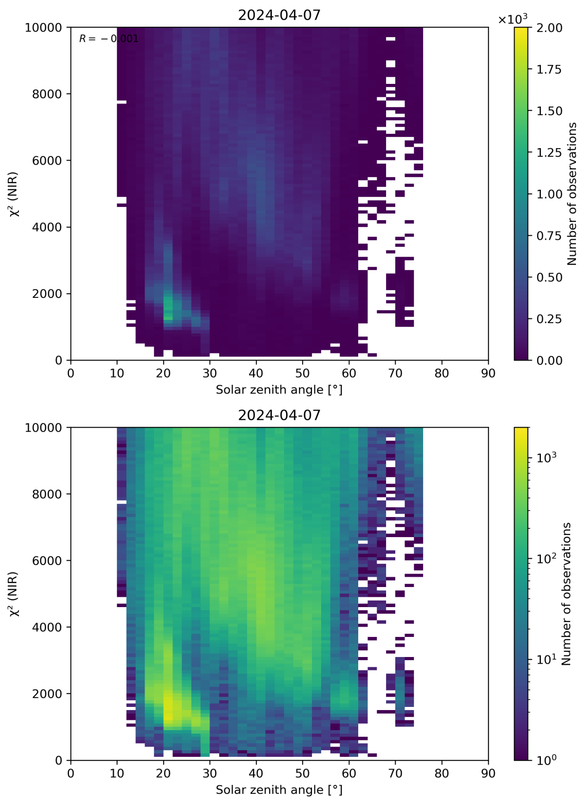
Figure 94: Scatter density plot of “Solar zenith angle” against “ \chi^2 (NIR)” for 2024-04-06 to 2024-04-08.
