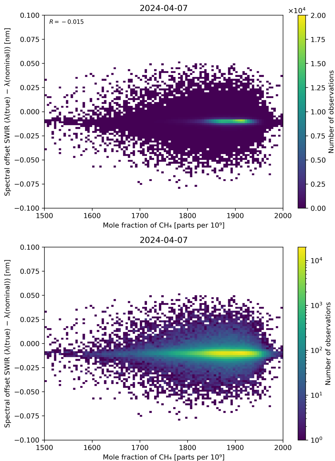
Figure 86: Scatter density plot of “Mole fraction of CH 4 ” against “Spectral offset SWIR ( \lambda(\text{true}) - \lambda(\text{nominal}) )” for 2024-04-06 to 2024-04-08.
