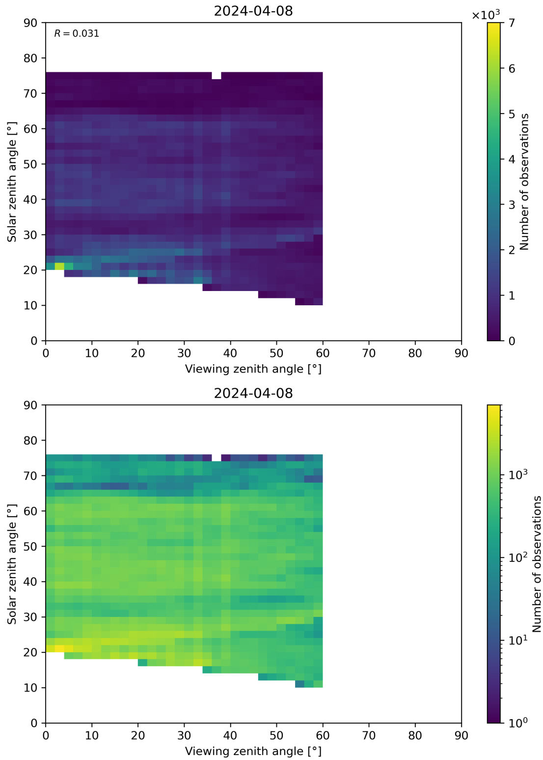
Figure 115: Scatter density plot of “Viewing zenith angle” against “Solar zenith angle” for 2024-04-07 to 2024-04-09.
