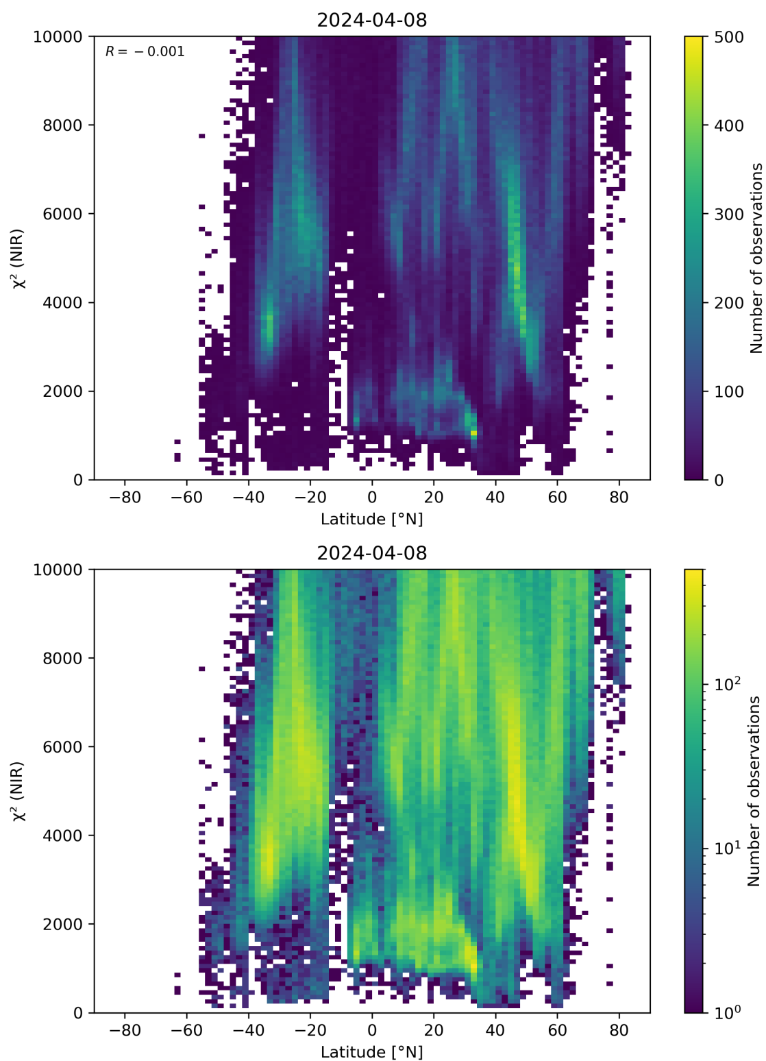
Figure 53: Scatter density plot of “Latitude” against “ \chi^2 (NIR)” for 2024-04-07 to 2024-04-09.
