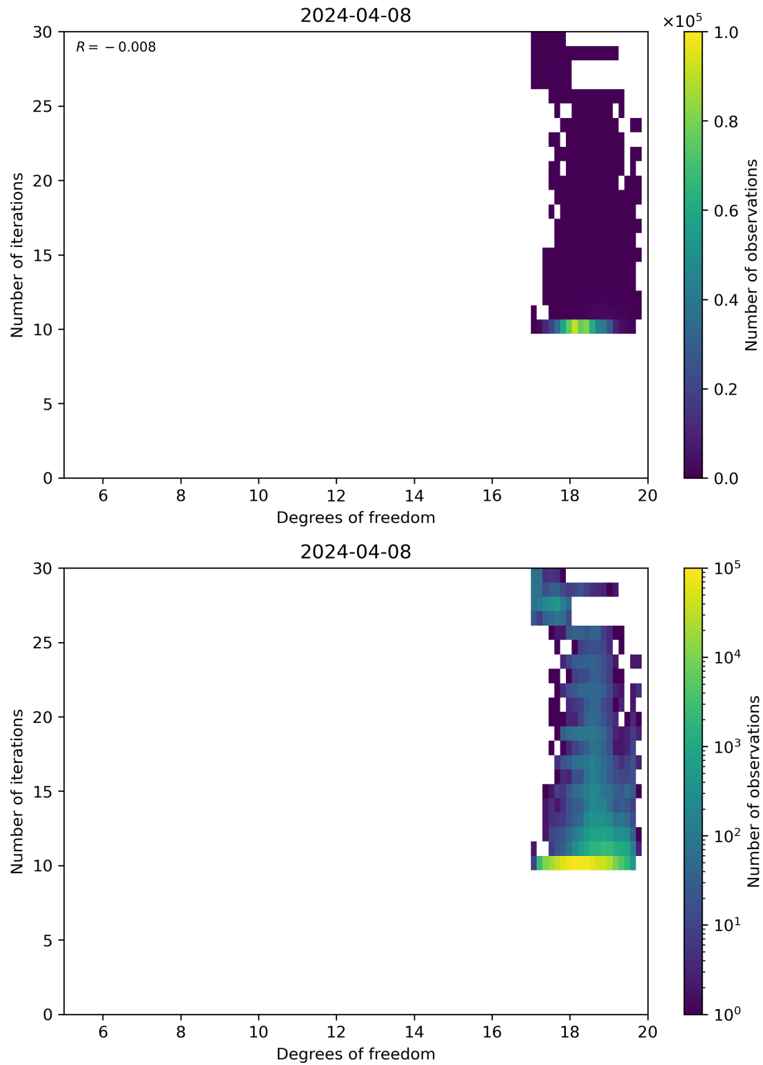
Figure 52: Scatter density plot of “Degrees of freedom” against “Number of iterations” for 2024-04-07 to 2024-04-09.
