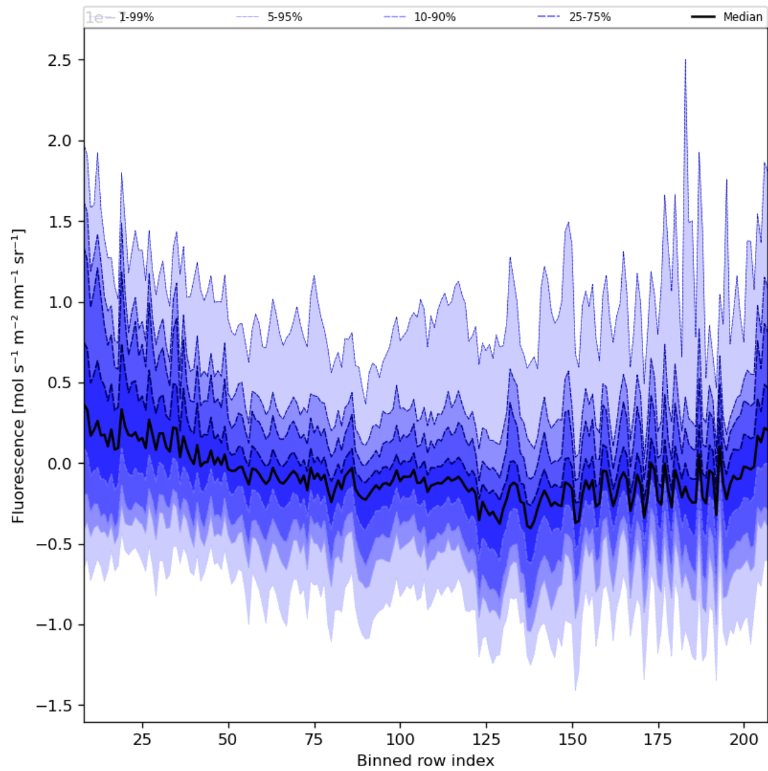
Figure 43: Along track statistics of “Fluorescence” for 2024-04-07 to 2024-04-09
