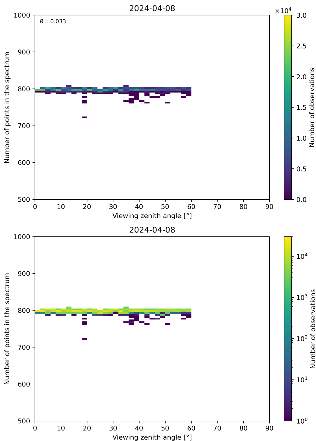
Figure 114: Scatter density plot of “Viewing zenith angle” against “Number of points in the spectrum” for 2024-04-07 to 2024-04-09.
