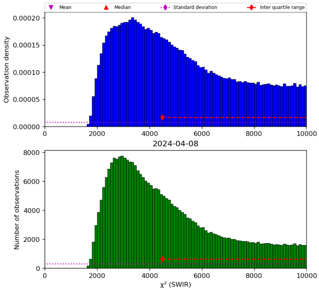
Figure 28: Histogram of “ \chi^2 (SWIR)” for 2024-04-07 to 2024-04-09
