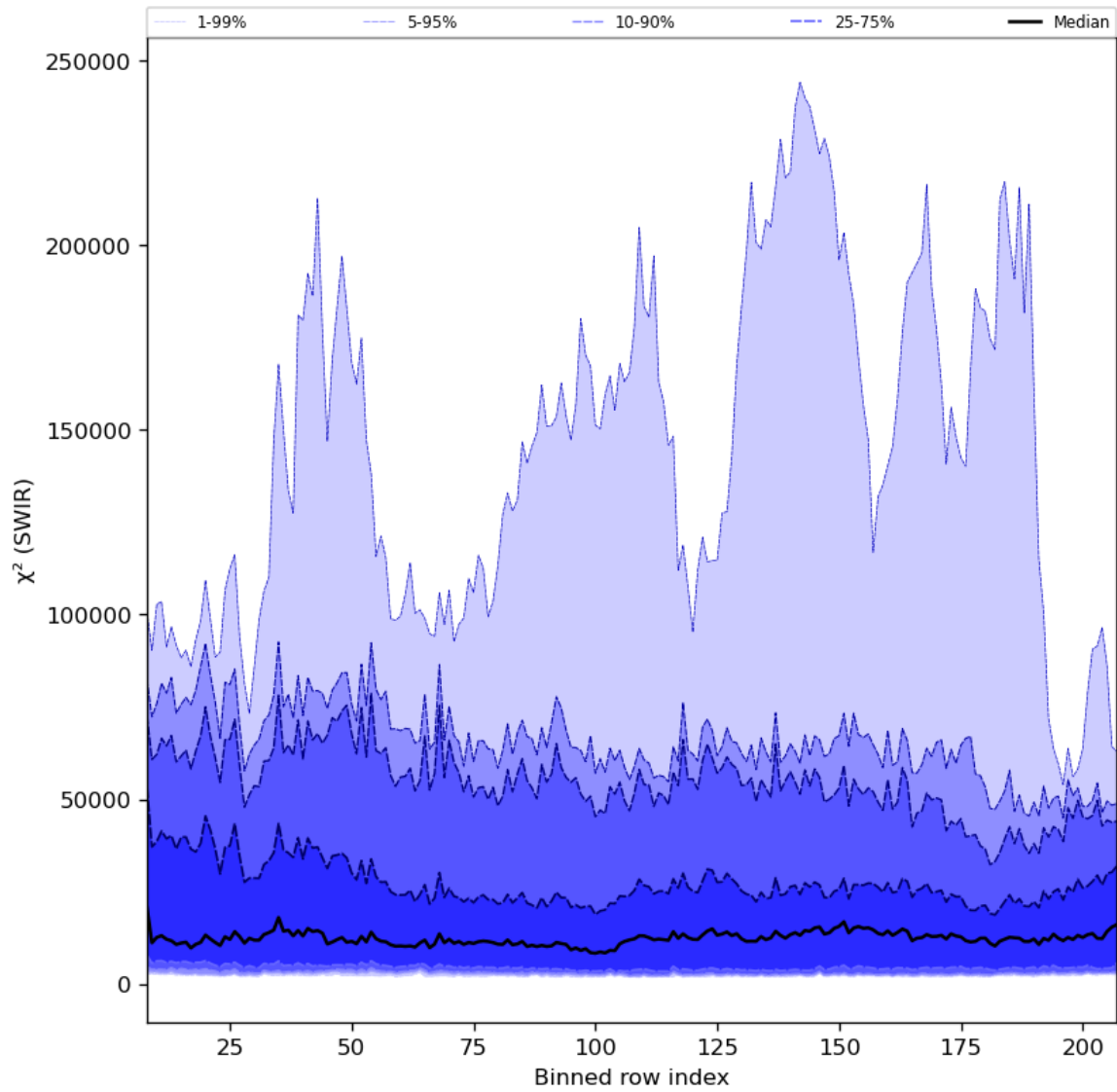
Figure 39: Along track statistics of " \chi^2 (SWIR)" for 2024-04-07 to 2024-04-09
