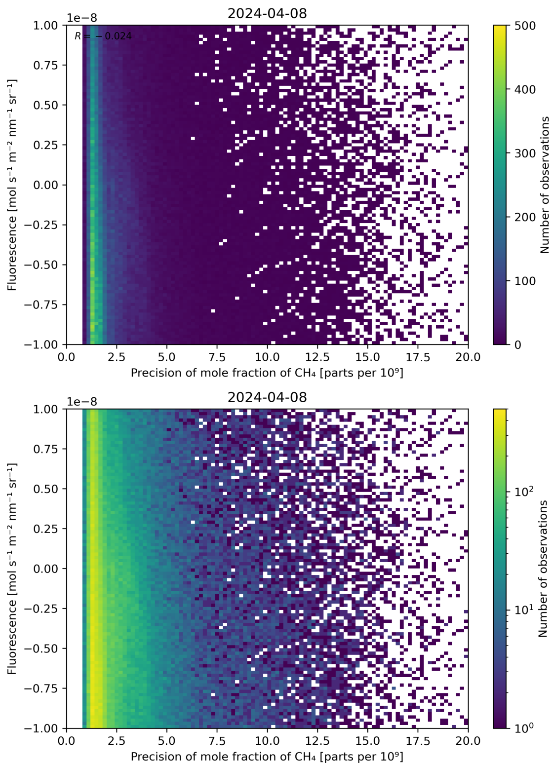
Figure 81: Scatter density plot of “Precision of mole fraction of \text{CH}_4 ” against “Fluorescence” for 2024-04-07 to 2024-04-09.
