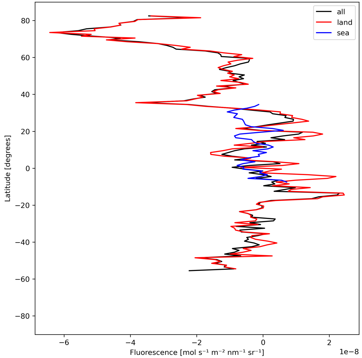
Figure 21: Zonal average of “Fluorescence” for 2024-04-07 to 2024-04-09.
