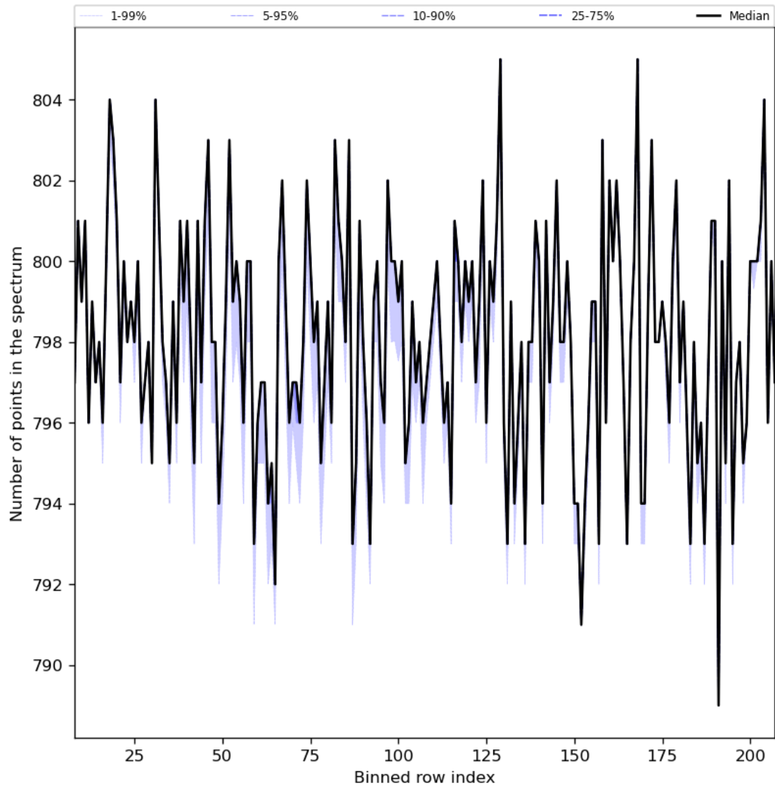
Figure 37: Along track statistics of “Number of points in the spectrum” for 2024-04-07 to 2024-04-09
