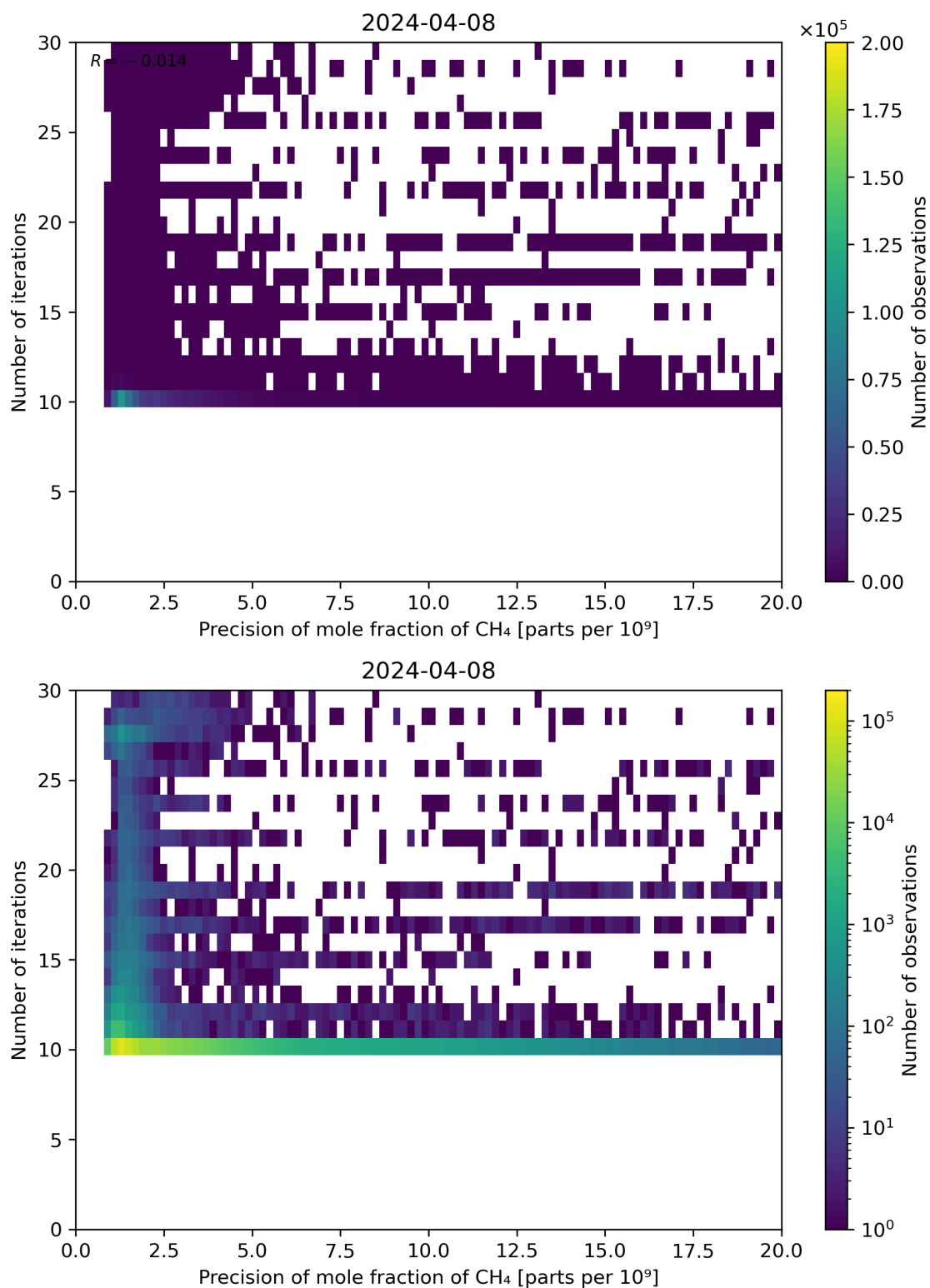
Figure 83: Scatter density plot of “Precision of mole fraction of CH 4 ” against “Number of iterations” for 2024-04-07 to 2024-04-09.
