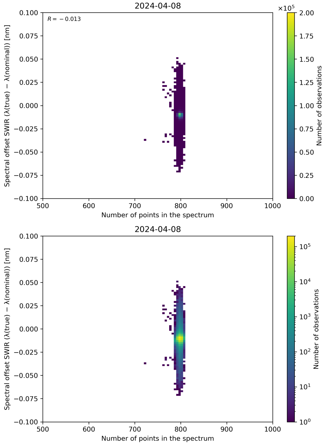
Figure 93: Scatter density plot of “Number of points in the spectrum” against “Spectral offset SWIR ( \lambda(\text{true}) - \lambda(\text{nominal}) )” for 2024-04-07 to 2024-04-09.
