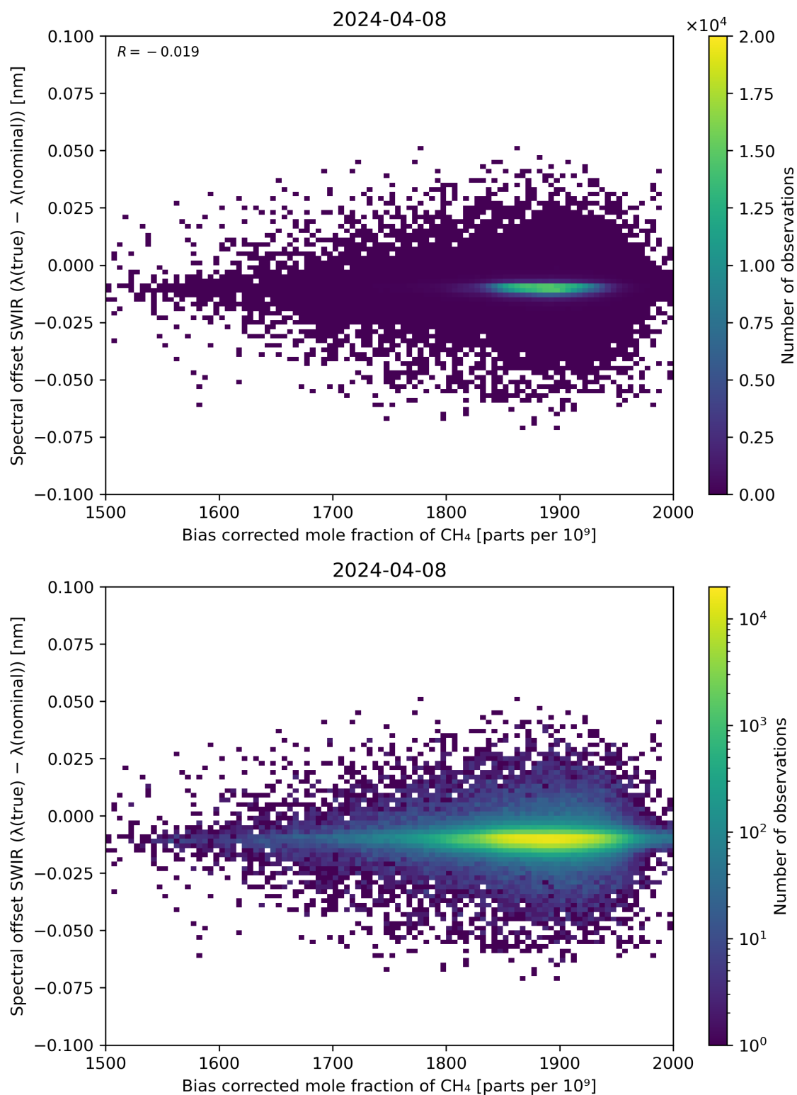
Figure 69: Scatter density plot of “Bias corrected mole fraction of \text{CH}_4 ” against “Spectral offset SWIR ( \lambda(\text{true}) - \lambda(\text{nominal}) )” for 2024-04-07 to 2024-04-09.
