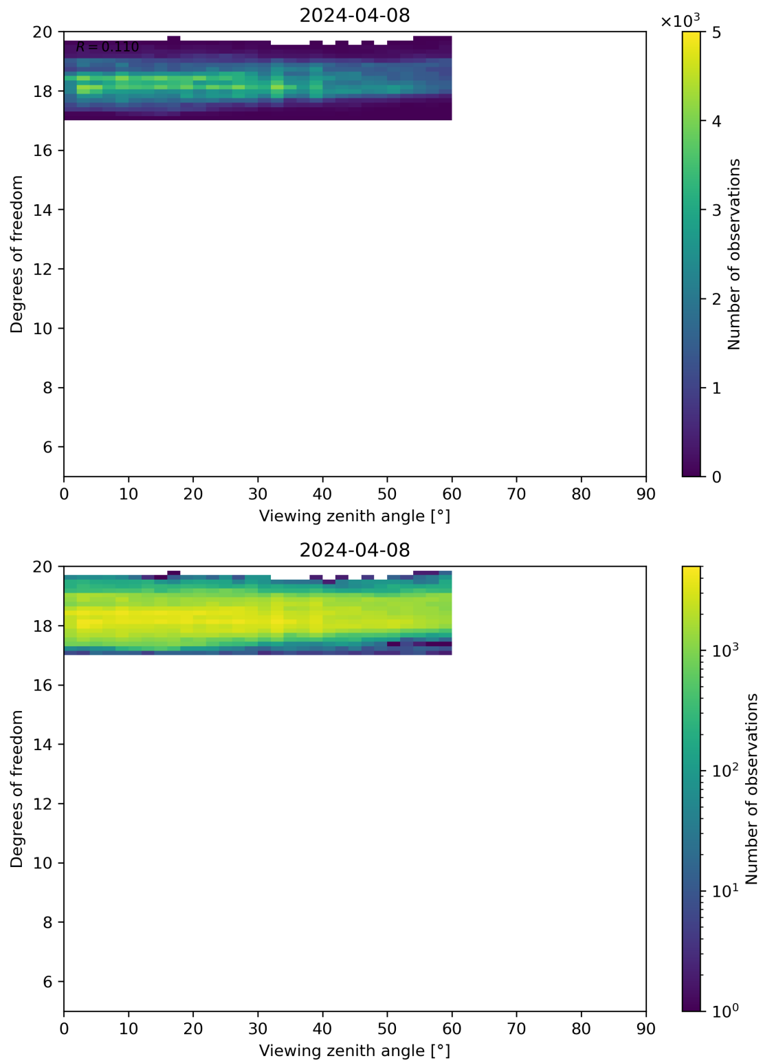
Figure 107: Scatter density plot of “Viewing zenith angle” against “Degrees of freedom” for 2024-04-07 to 2024-04-09.
