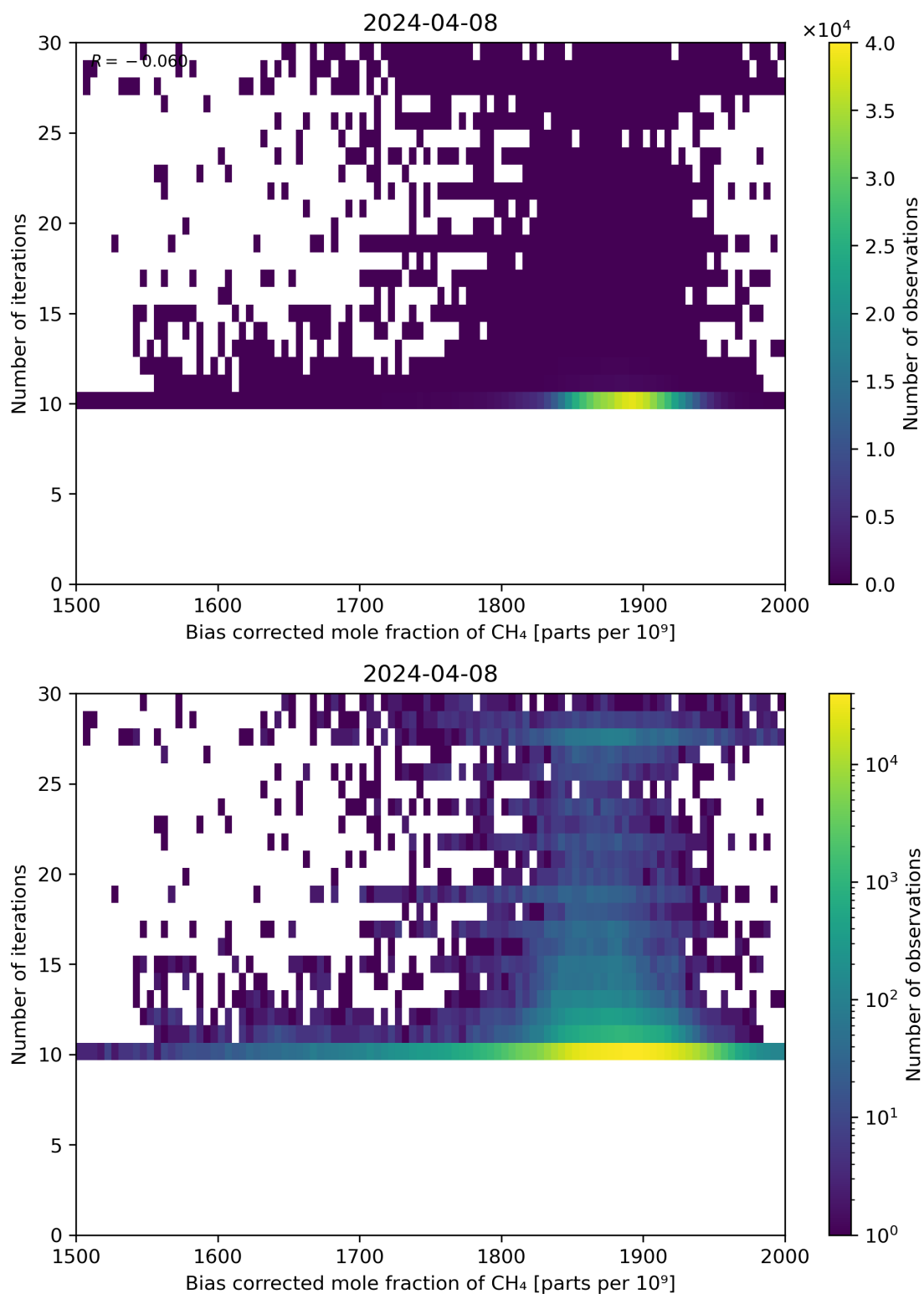
Figure 67: Scatter density plot of “Bias corrected mole fraction of \text{CH}_4 ” against “Number of iterations” for 2024-04-07 to 2024-04-09.
