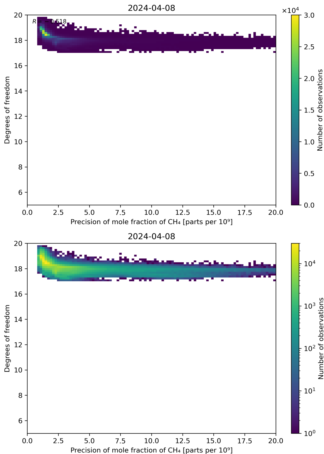
Figure 80: Scatter density plot of “Precision of mole fraction of CH 4 ” against “Degrees of freedom” for 2024-04-07 to 2024-04-09.
