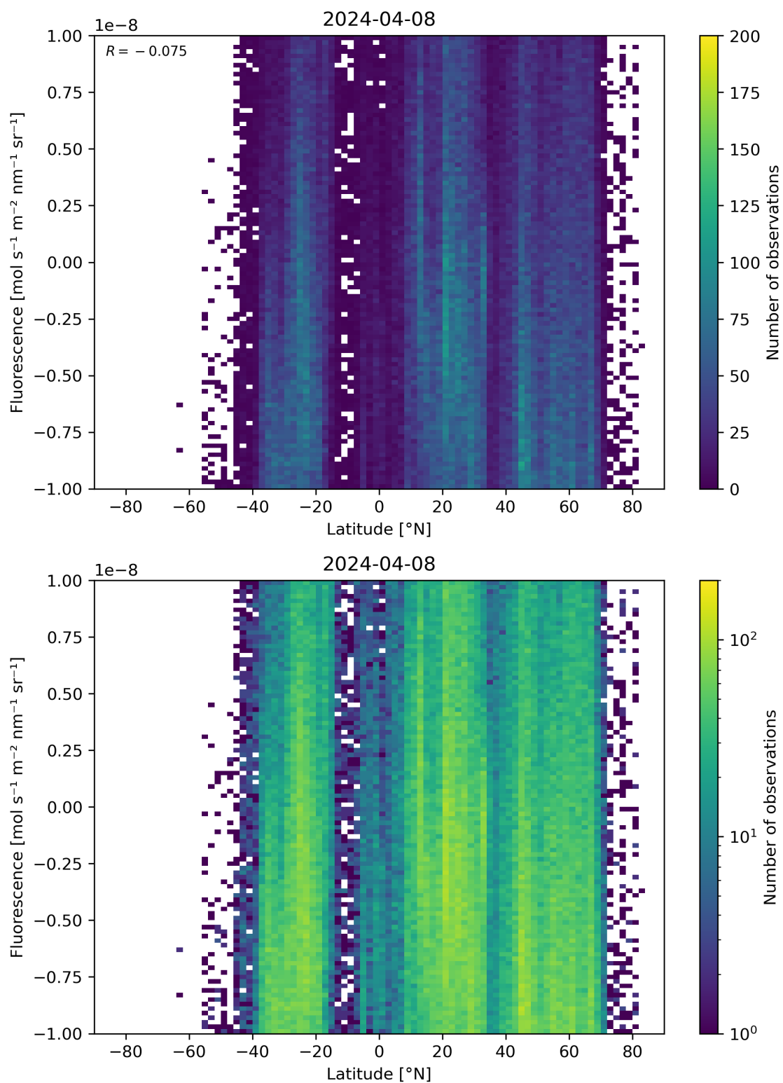
Figure 56: Scatter density plot of “Latitude” against “Fluorescence” for 2024-04-07 to 2024-04-09.
