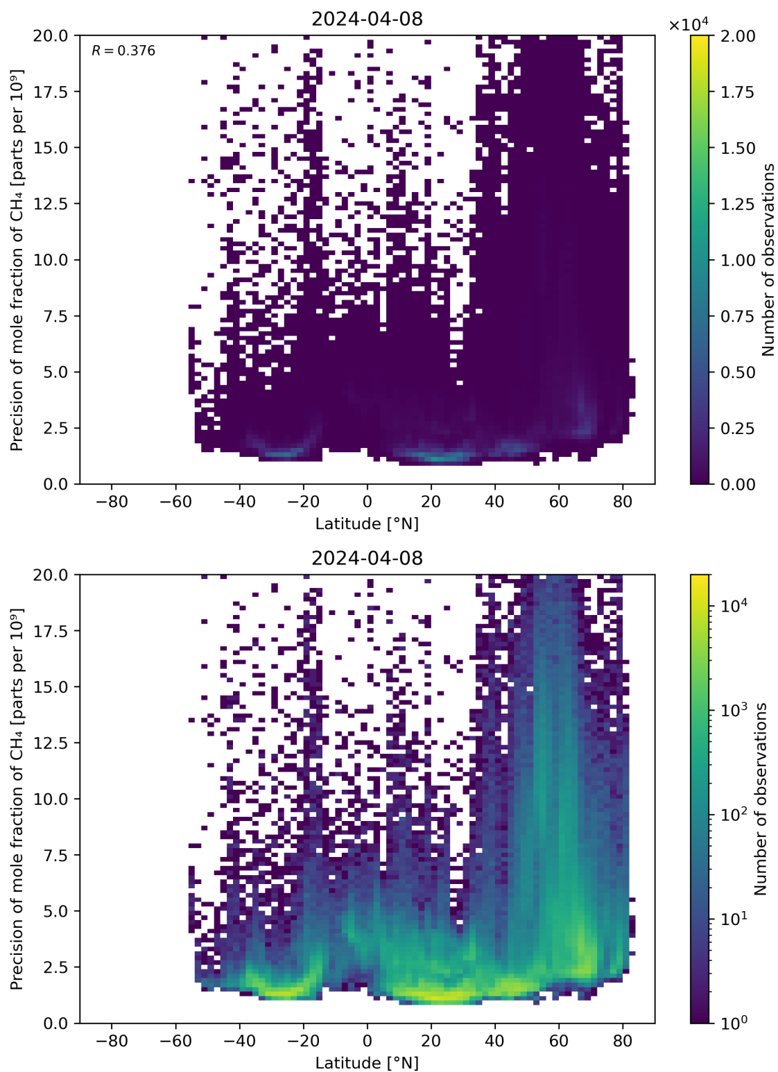
Figure 59: Scatter density plot of “Latitude” against “Precision of mole fraction of \text{CH}_4 ” for 2024-04-07 to 2024-04-09.
