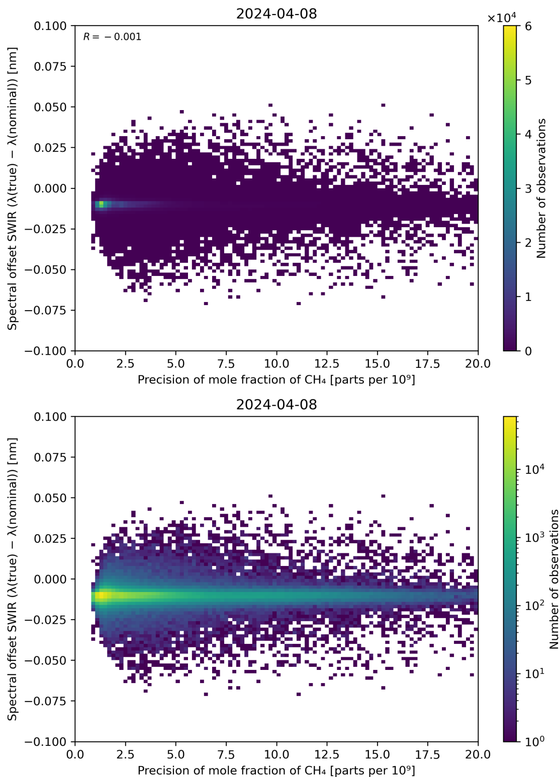
Figure 85: Scatter density plot of “Precision of mole fraction of \text{CH}_4 ” against “Spectral offset SWIR ( \lambda(\text{true}) - \lambda(\text{nominal}) )” for 2024-04-07 to 2024-04-09.
