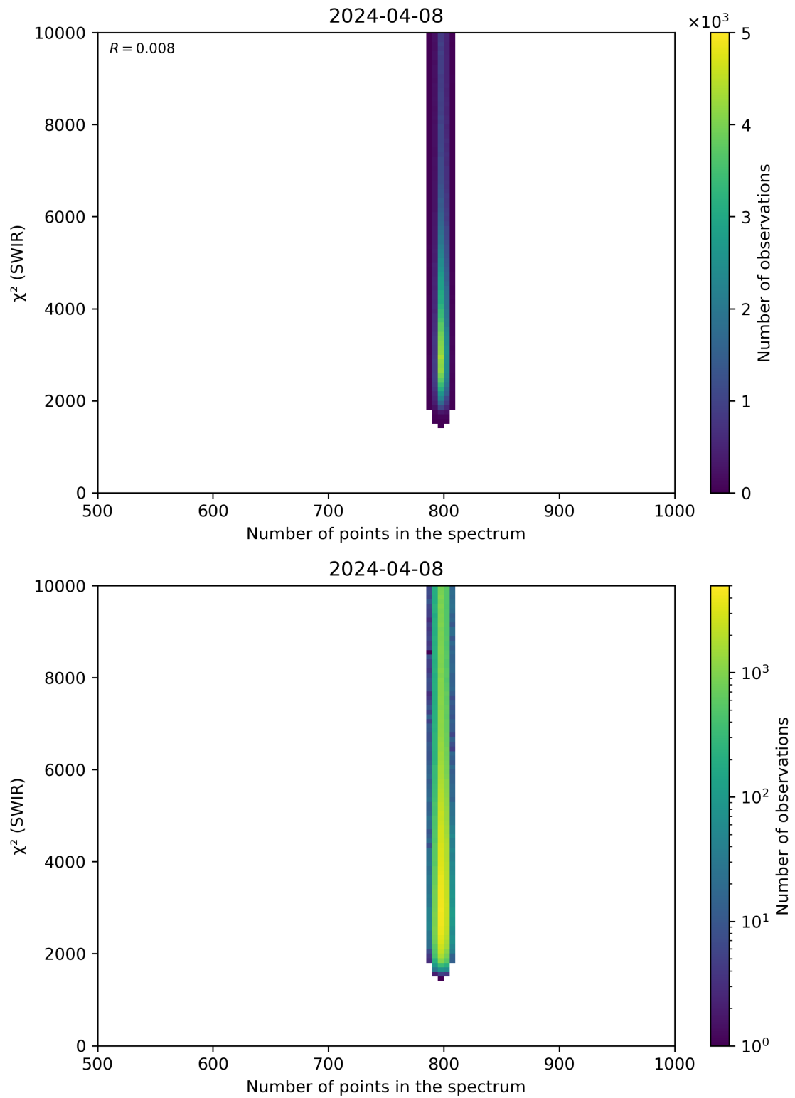
Figure 89: Scatter density plot of “Number of points in the spectrum” against “ \chi^2 (SWIR)” for 2024-04-07 to 2024-04-09.
