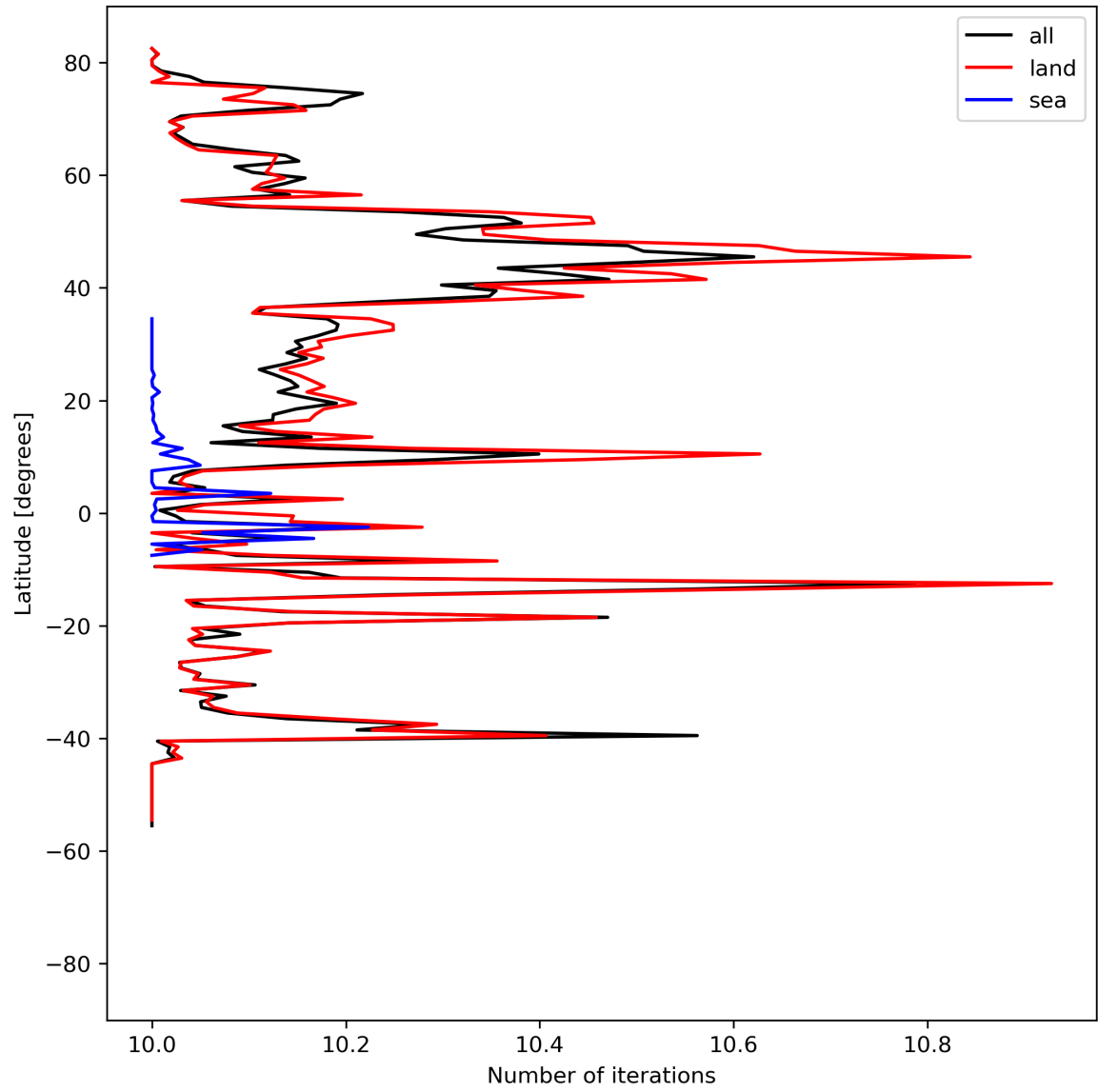
Figure 20: Zonal average of “Number of iterations” for 2024-04-07 to 2024-04-09.
