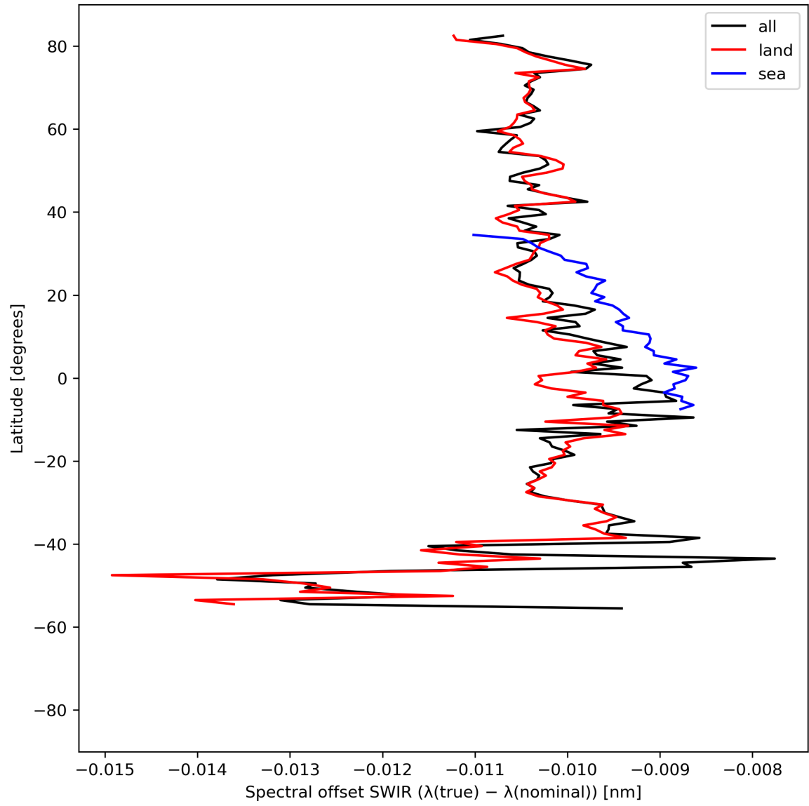
Figure 16: Zonal average of “Spectral offset SWIR ( \lambda(\text{true}) - \lambda(\text{nominal}) )” for 2024-04-07 to 2024-04-09.
