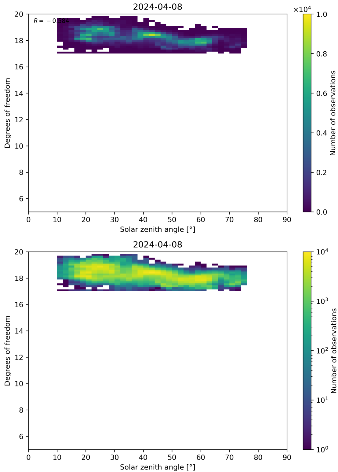
Figure 96: Scatter density plot of “Solar zenith angle” against “Degrees of freedom” for 2024-04-07 to 2024-04-09.
