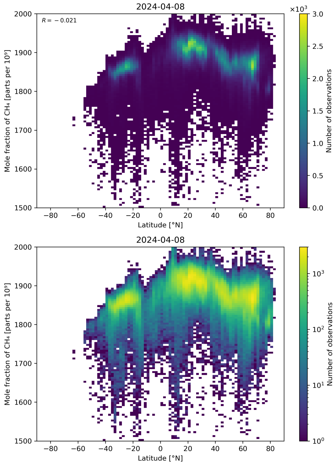
Figure 57: Scatter density plot of “Latitude” against “Mole fraction of CH 4 ” for 2024-04-07 to 2024-04-09.
