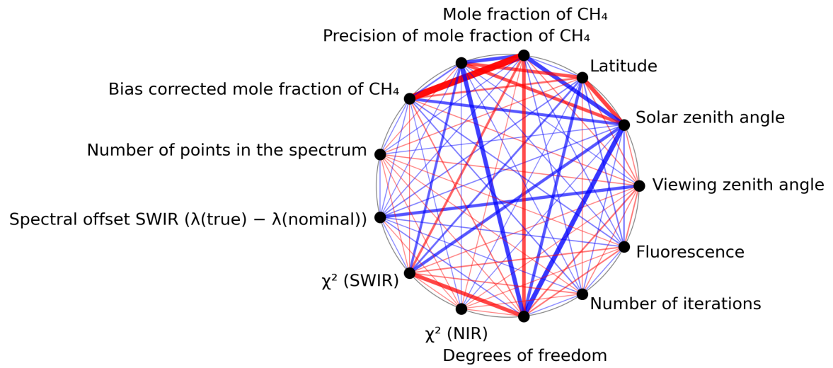
Figure 1: Map of correlation graph for 2024-04-07 to 2024-04-09.
