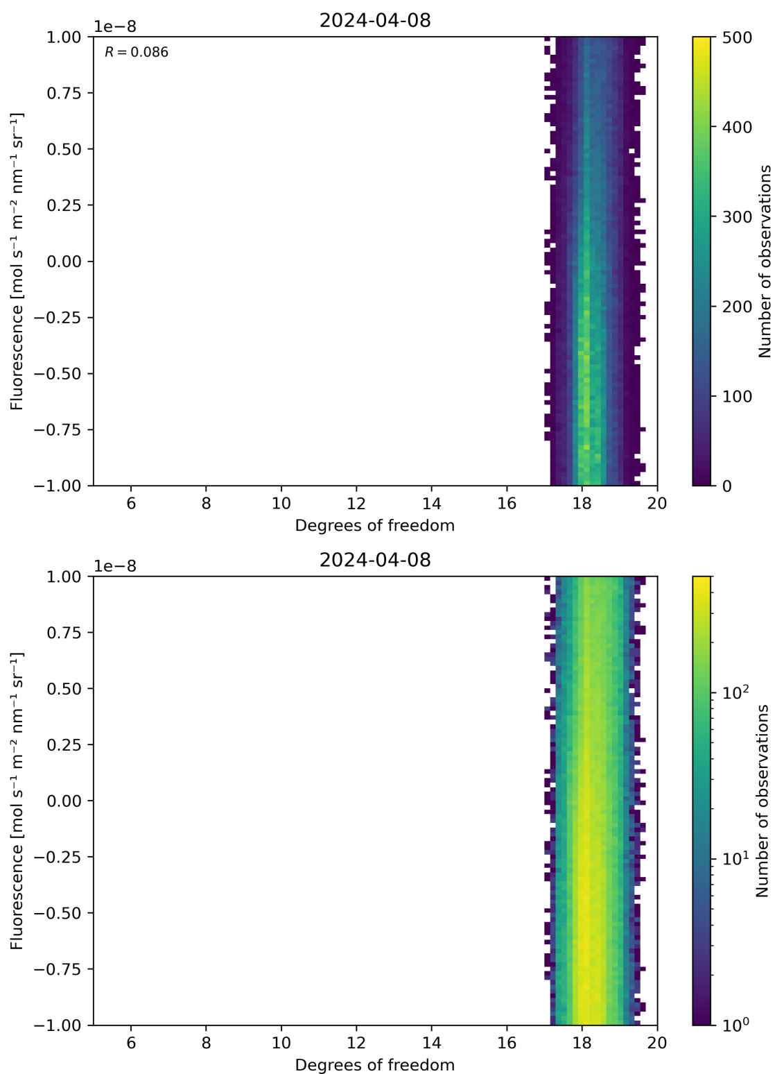
Figure 51: Scatter density plot of “Degrees of freedom” against “Fluorescence” for 2024-04-07 to 2024-04-09.
