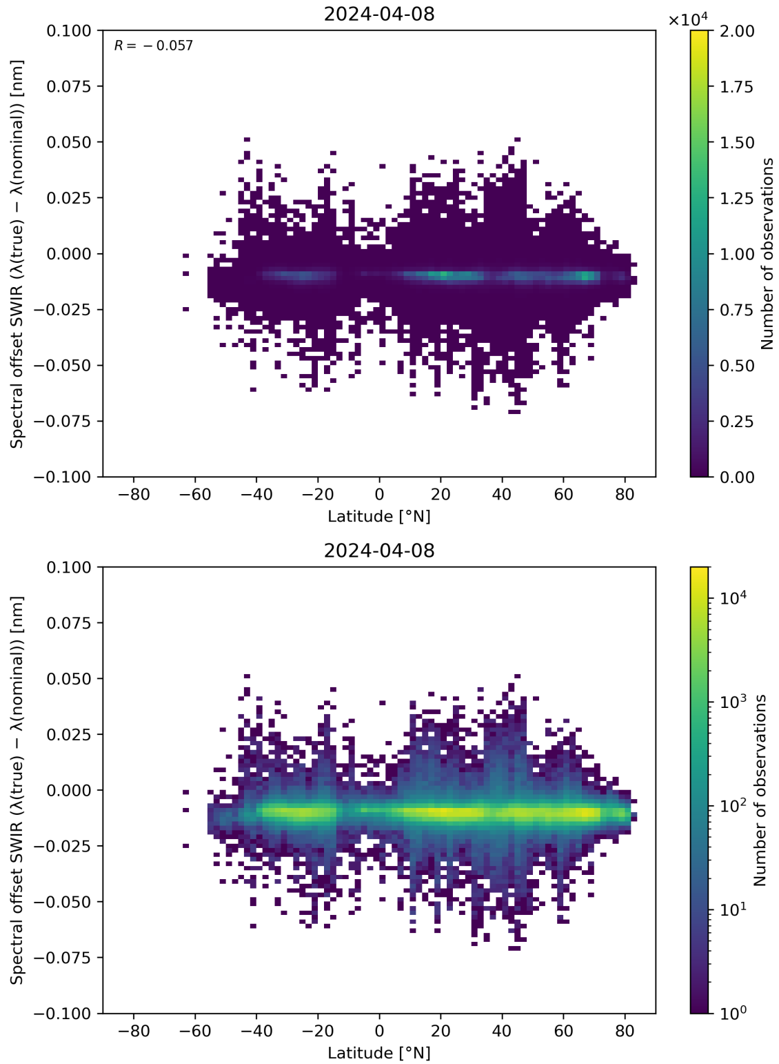
Figure 62: Scatter density plot of “Latitude” against “Spectral offset SWIR ( \lambda(\text{true}) - \lambda(\text{nominal}) )” for 2024-04-07 to 2024-04-09.
