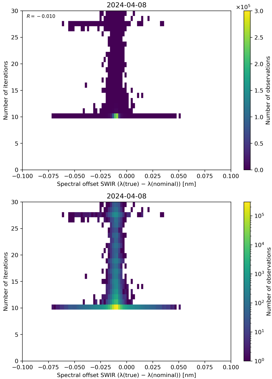
Figure 121: Scatter density plot of “Spectral offset SWIR ( \lambda(\text{true}) - \lambda(\text{nominal}) )” against “Number of iterations” for 2024-04-07 to 2024-04-09.
