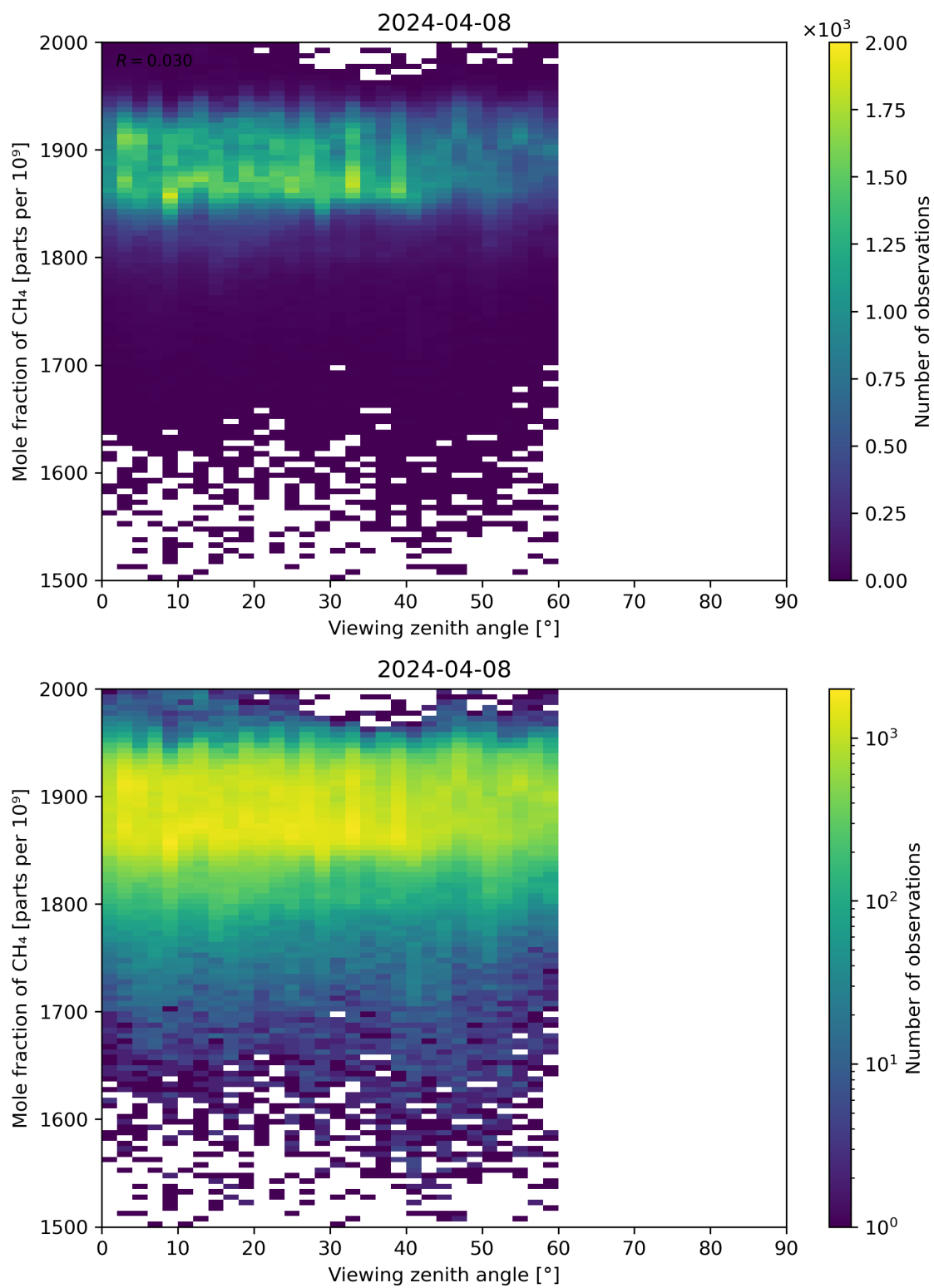
Figure 110: Scatter density plot of “Viewing zenith angle” against “Mole fraction of CH 4 ” for 2024-04-07 to 2024-04-09.
