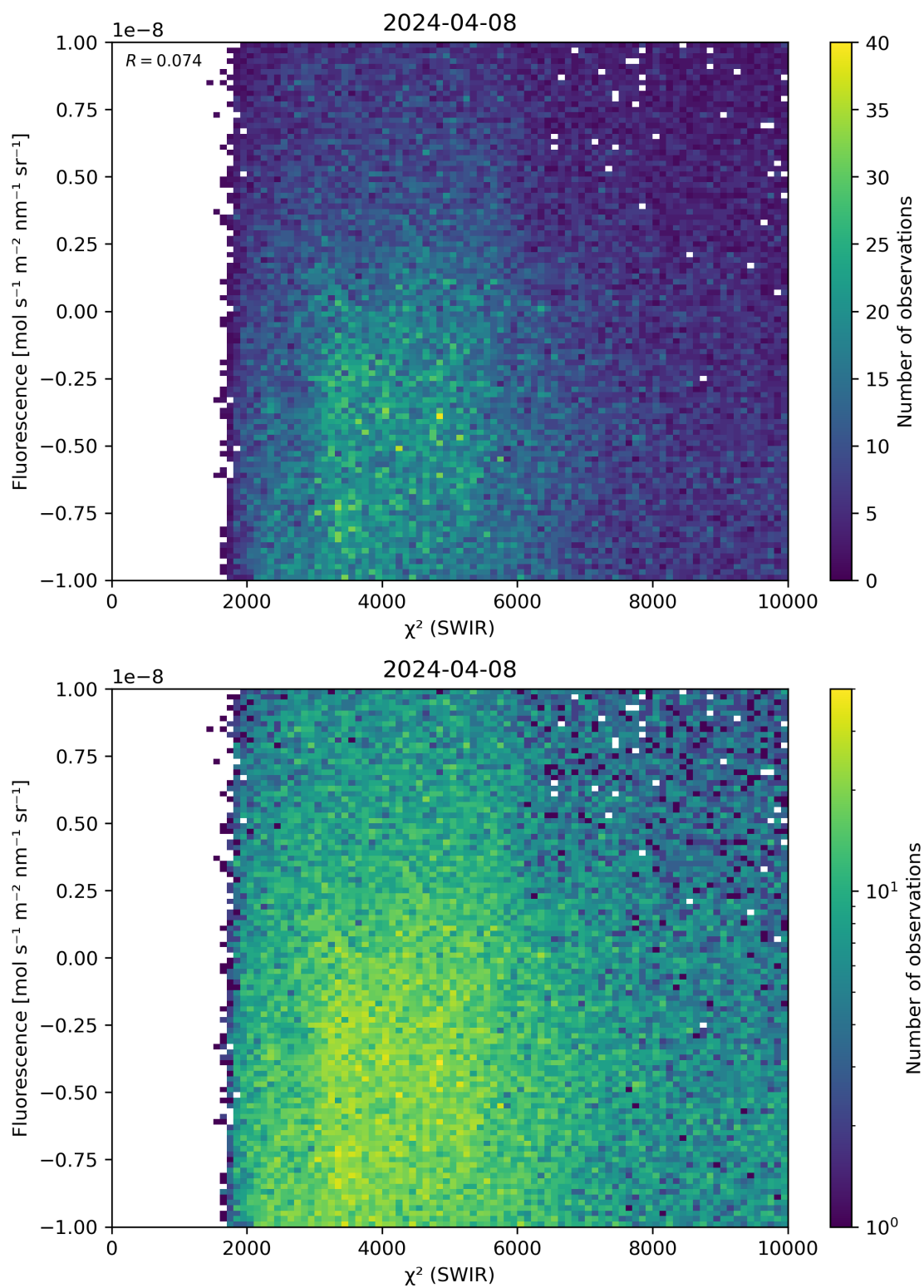
Figure 49: Scatter density plot of “ \chi^2 (SWIR)” against “Fluorescence” for 2024-04-07 to 2024-04-09.
