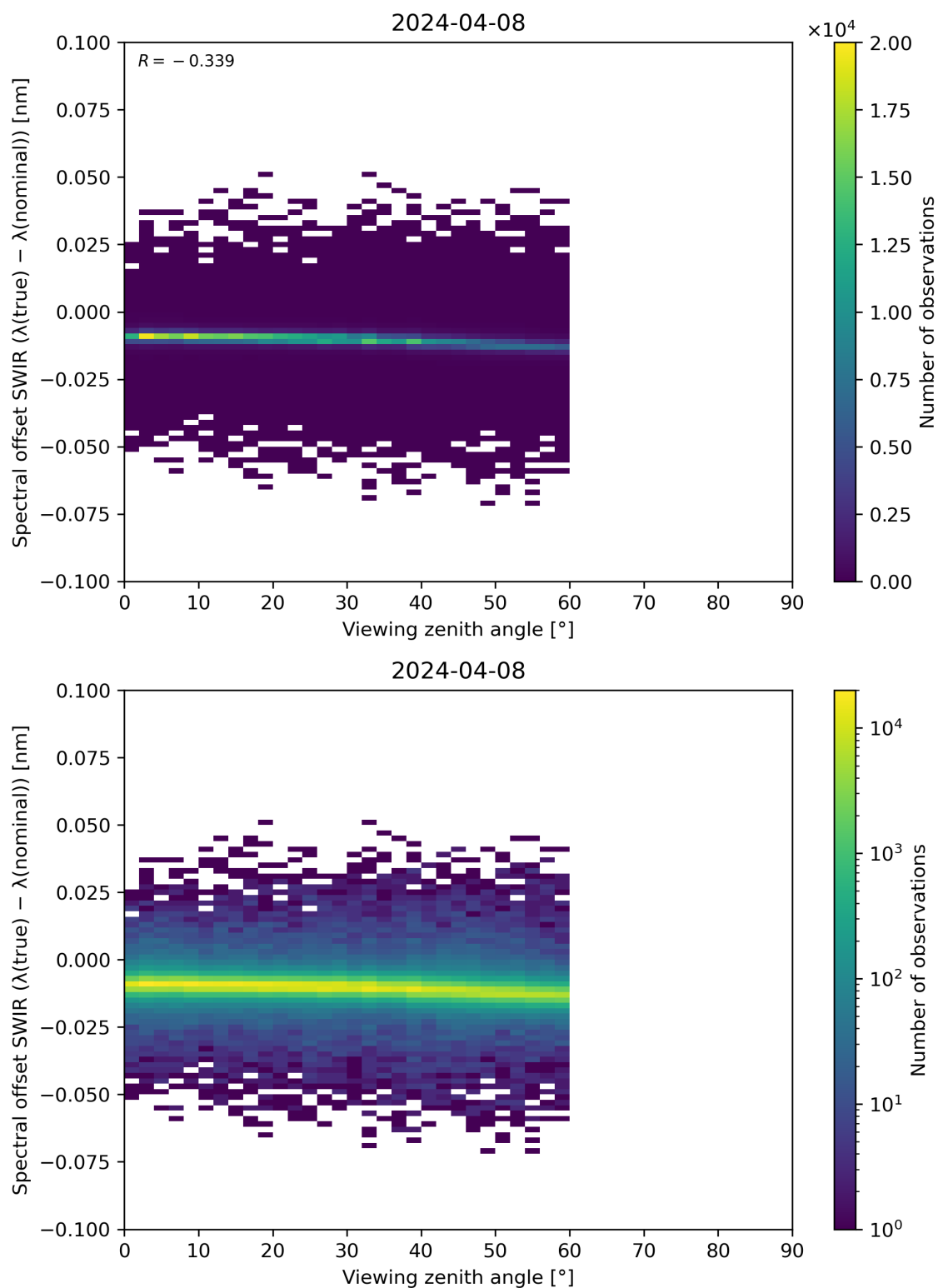
Figure 116: Scatter density plot of “Viewing zenith angle” against “Spectral offset SWIR ( \lambda(\text{true}) - \lambda(\text{nominal}) )” for 2024-04-07 to 2024-04-09.
