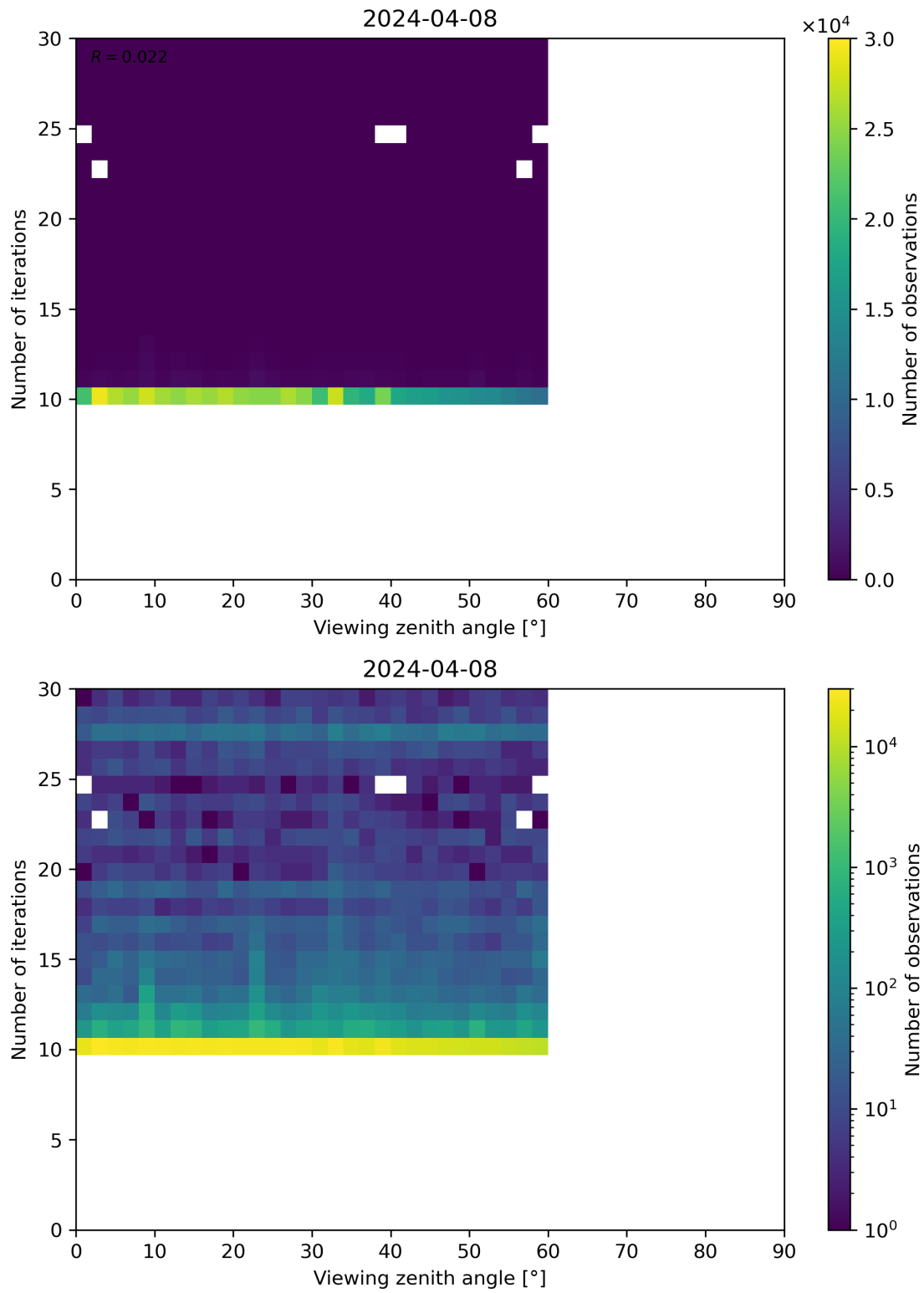
Figure 113: Scatter density plot of “Viewing zenith angle” against “Number of iterations” for 2024-04-07 to 2024-04-09.
