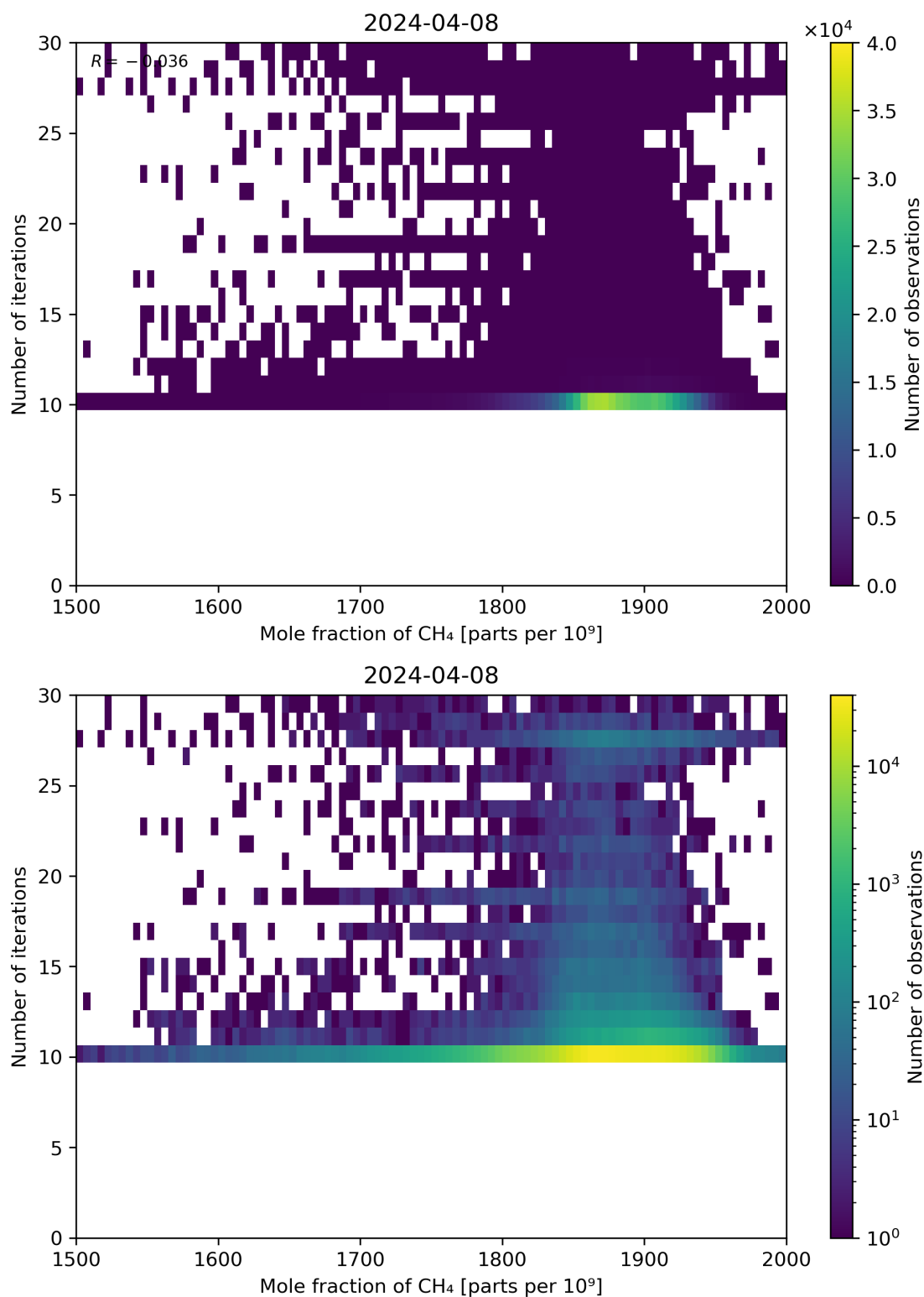
Figure 76: Scatter density plot of “Mole fraction of CH 4 ” against “Number of iterations” for 2024-04-07 to 2024-04-09.
