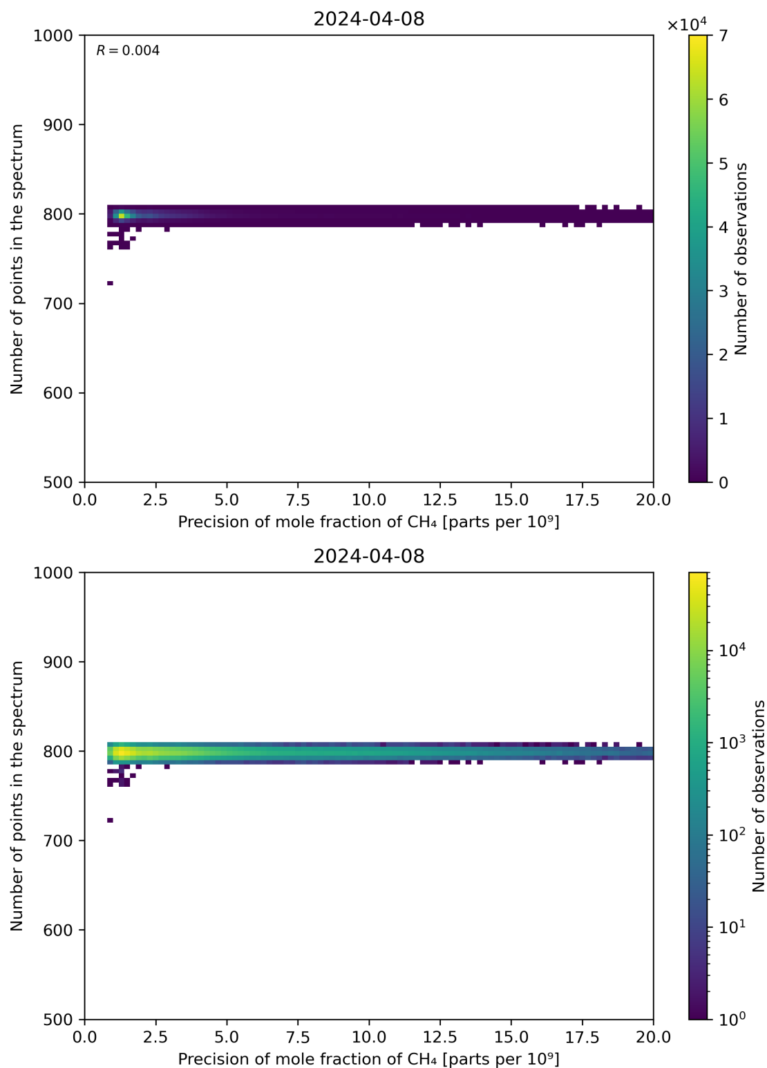
Figure 84: Scatter density plot of “Precision of mole fraction of CH 4 ” against “Number of points in the spectrum” for 2024-04-07 to 2024-04-09.
