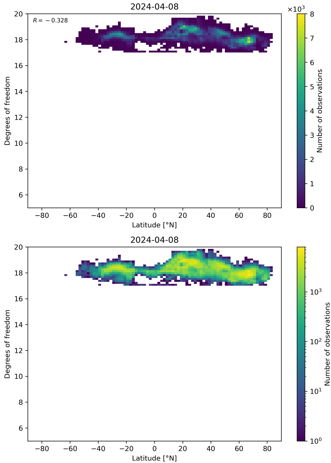
Figure 55: Scatter density plot of “Latitude” against “Degrees of freedom” for 2024-04-07 to 2024-04-09.
