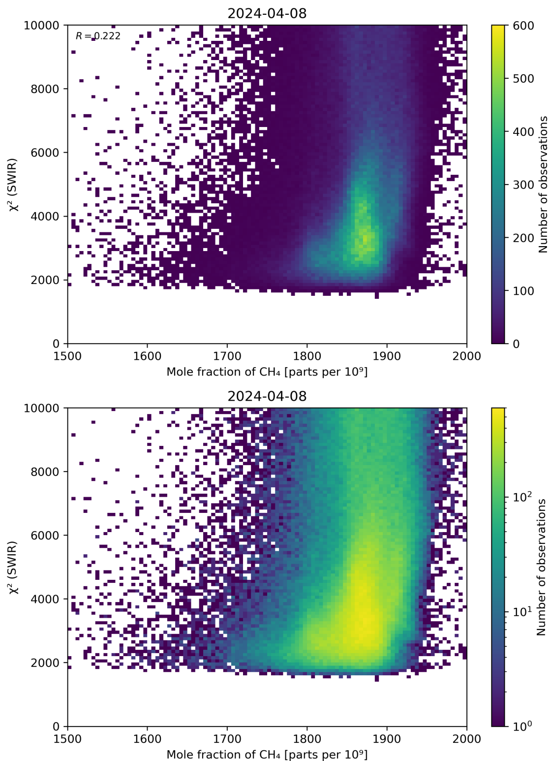
Figure 71: Scatter density plot of “Mole fraction of \text{CH}_4 ” against “ \chi^2 (SWIR)” for 2024-04-07 to 2024-04-09.
