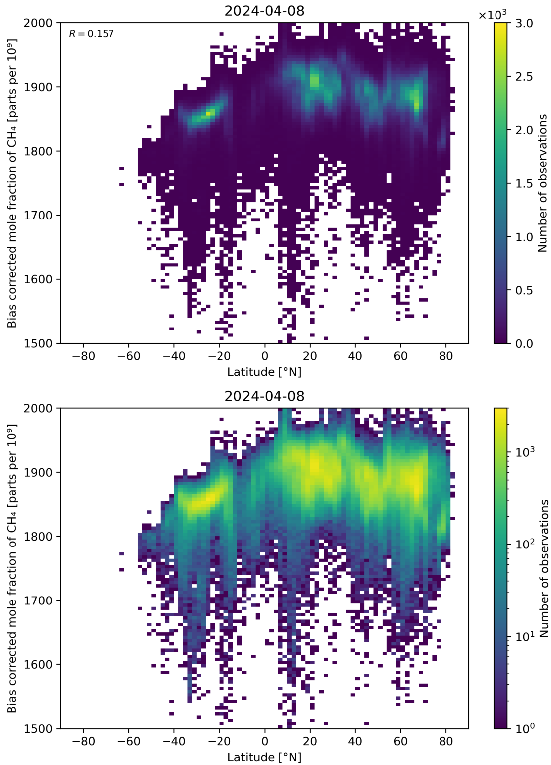
Figure 58: Scatter density plot of “Latitude” against “Bias corrected mole fraction of CH 4 ” for 2024-04-07 to 2024-04-09.
