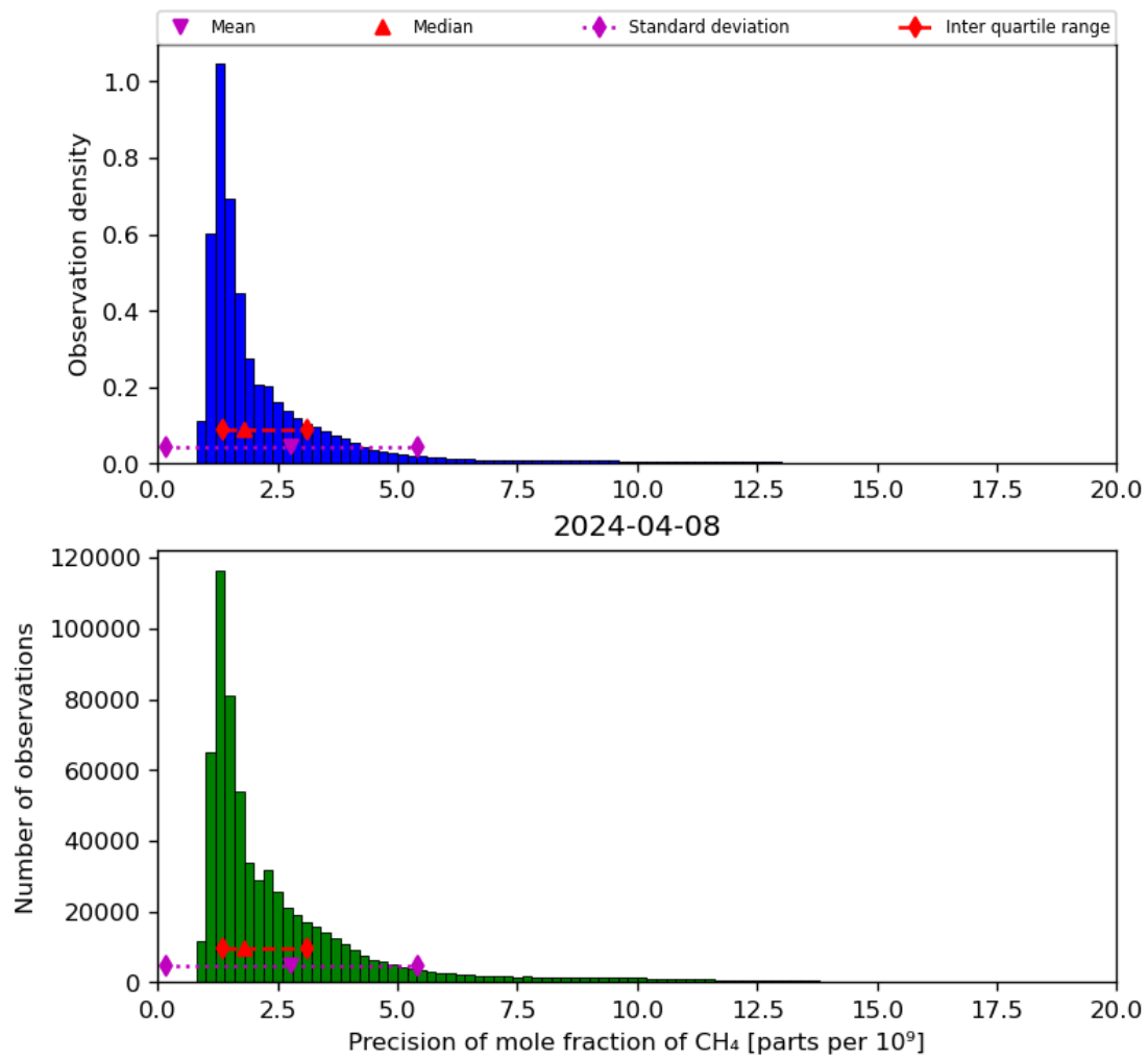
Figure 24: Histogram of “Precision of mole fraction of CH 4 ” for 2024-04-07 to 2024-04-09
