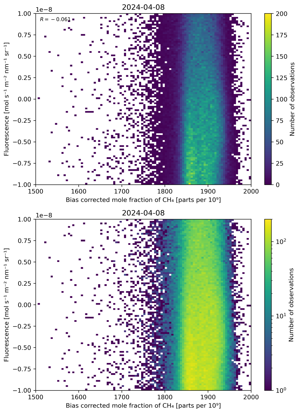
Figure 66: Scatter density plot of “Bias corrected mole fraction of \text{CH}_4 ” against “Fluorescence” for 2024-04-07 to 2024-04-09.
