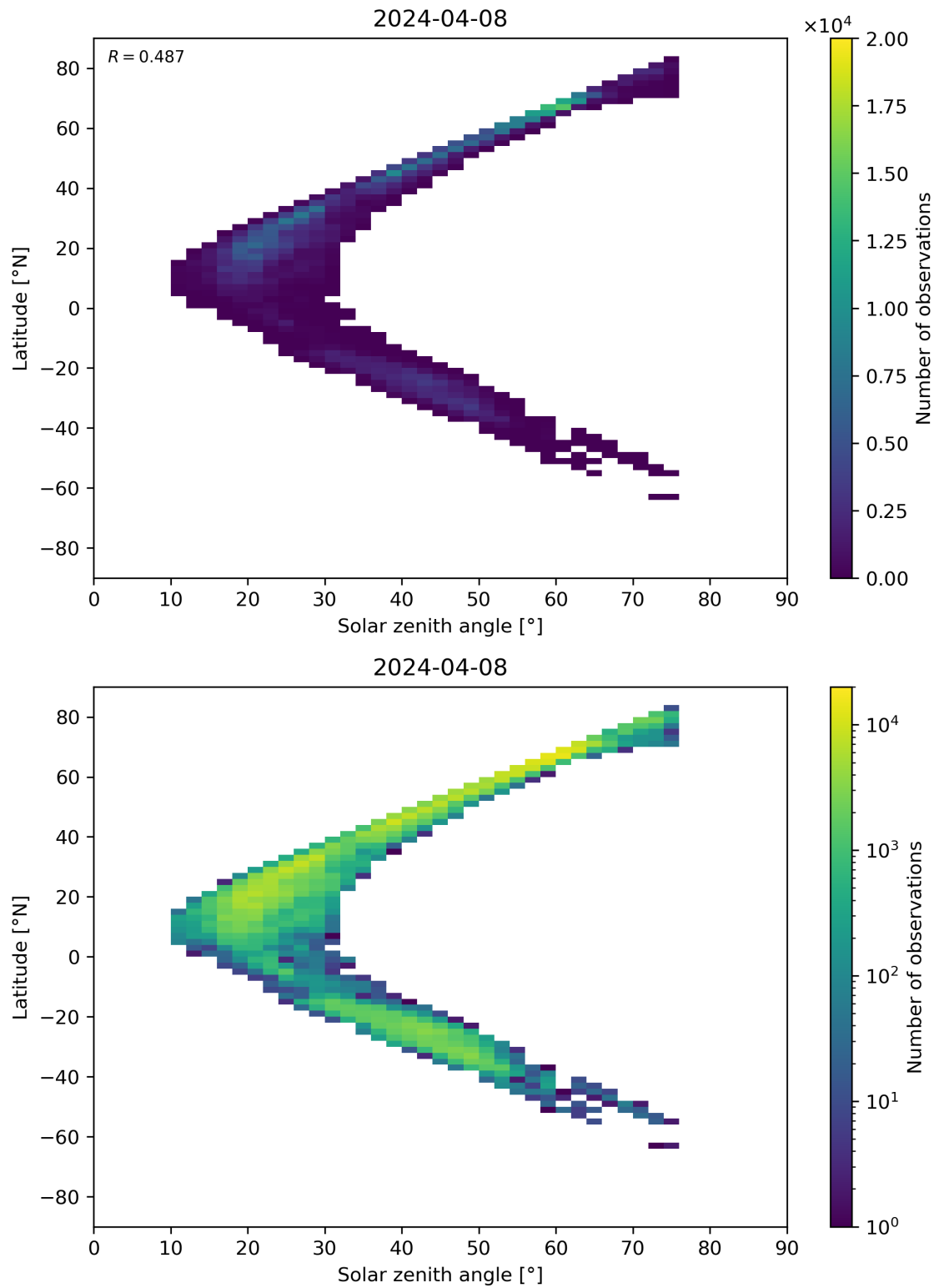
Figure 98: Scatter density plot of “Solar zenith angle” against “Latitude” for 2024-04-07 to 2024-04-09.
