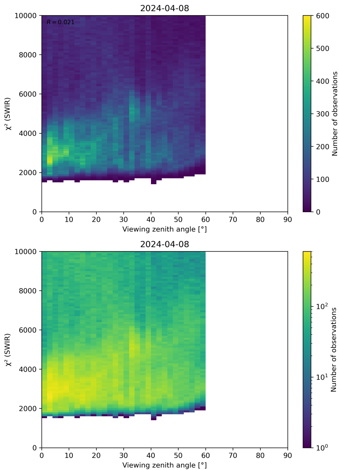
Figure 106: Scatter density plot of “Viewing zenith angle” against “ \chi^2 (SWIR)” for 2024-04-07 to 2024-04-09.
