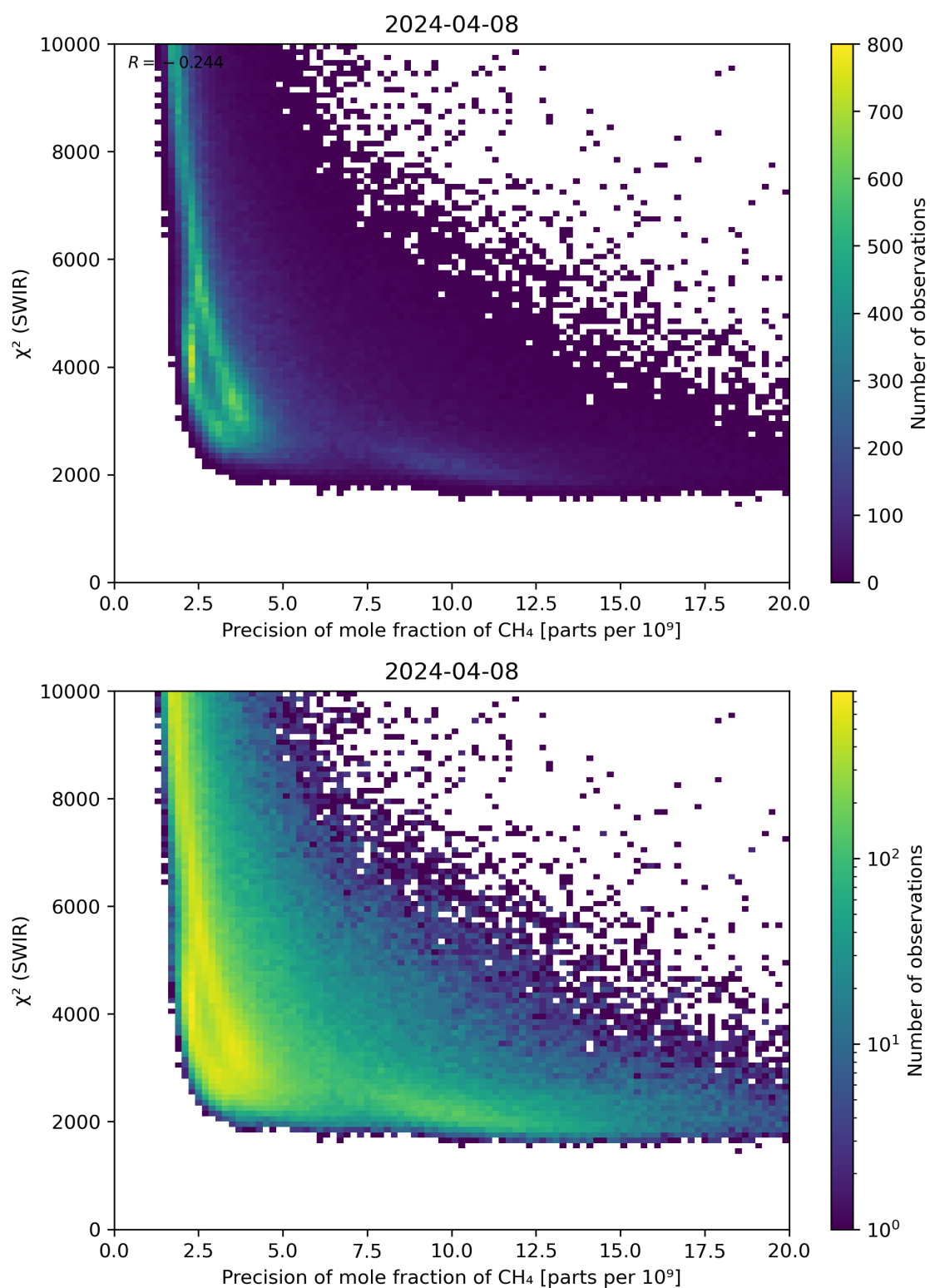
Figure 79: Scatter density plot of “Precision of mole fraction of CH 4 ” against “ \chi^2 (SWIR)” for 2024-04-07 to 2024-04-09.
