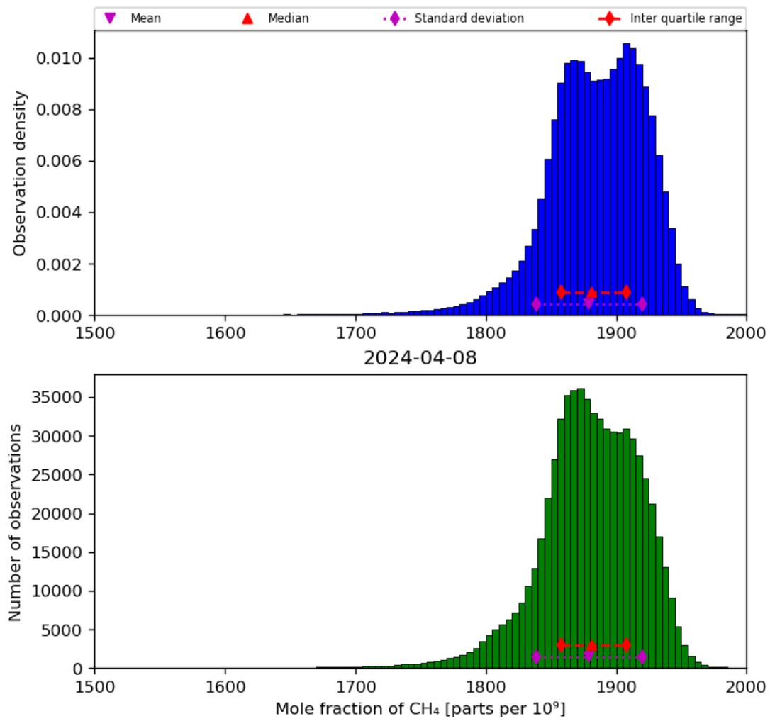
Figure 23: Histogram of “Mole fraction of CH 4 ” for 2024-04-07 to 2024-04-09
