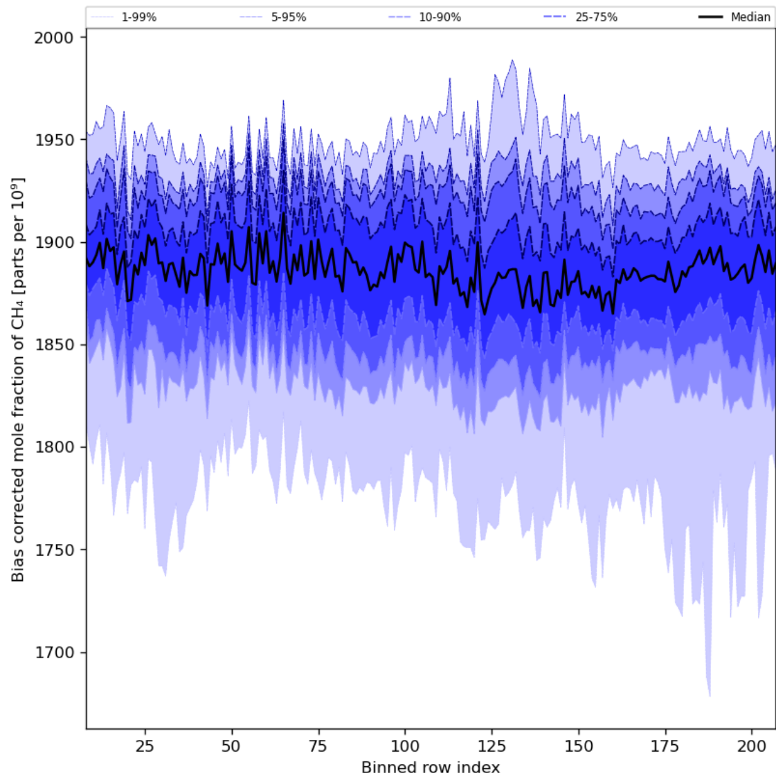
Figure 36: Along track statistics of “Bias corrected mole fraction of CH 4 ” for 2024-04-07 to 2024-04-09
