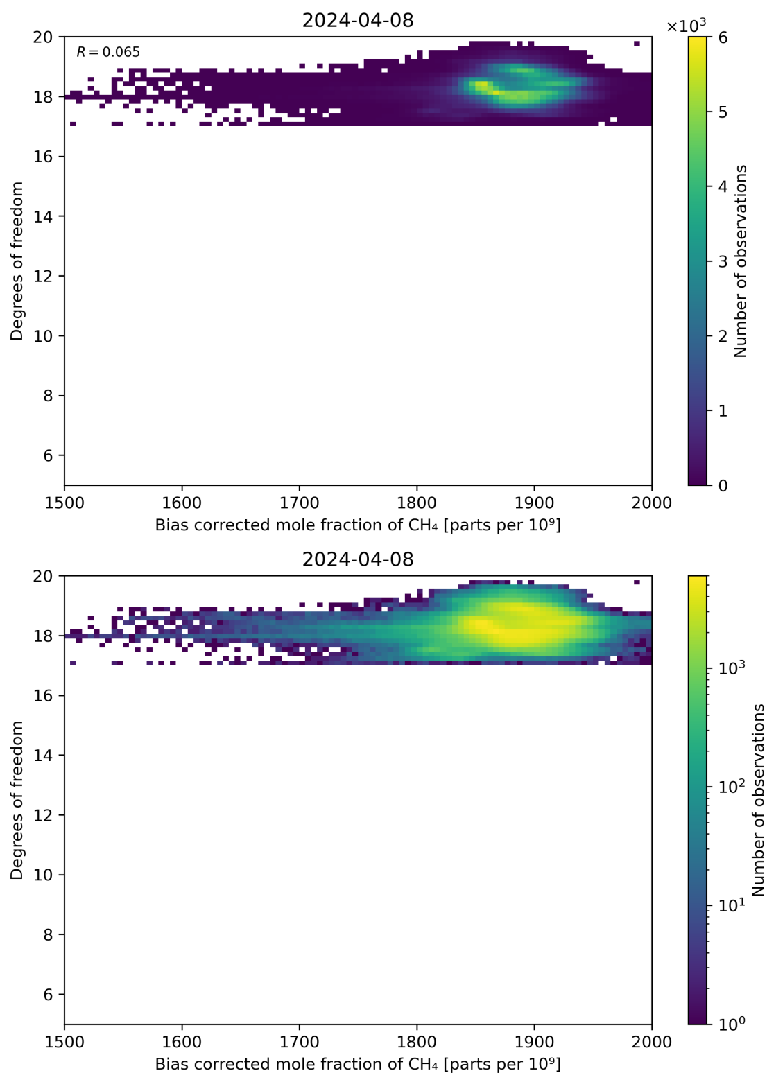
Figure 65: Scatter density plot of “Bias corrected mole fraction of CH 4 ” against “Degrees of freedom” for 2024-04-07 to 2024-04-09.
