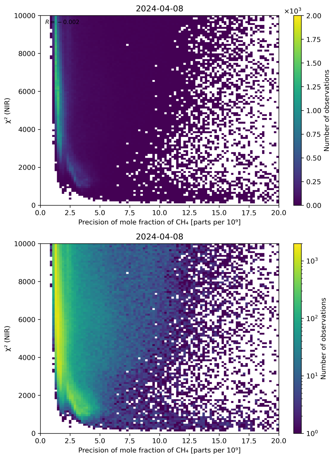
Figure 78: Scatter density plot of “Precision of mole fraction of CH 4 ” against “ \chi^2 (NIR)” for 2024-04-07 to 2024-04-09.
