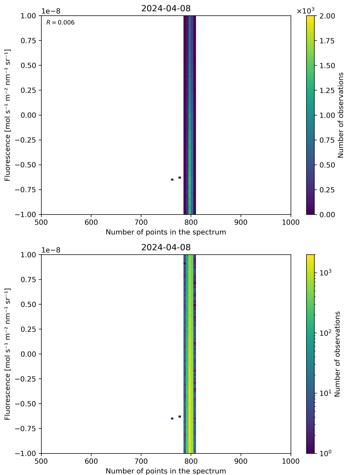
Figure 91: Scatter density plot of “Number of points in the spectrum” against “Fluorescence” for 2024-04-07 to 2024-04-09.
