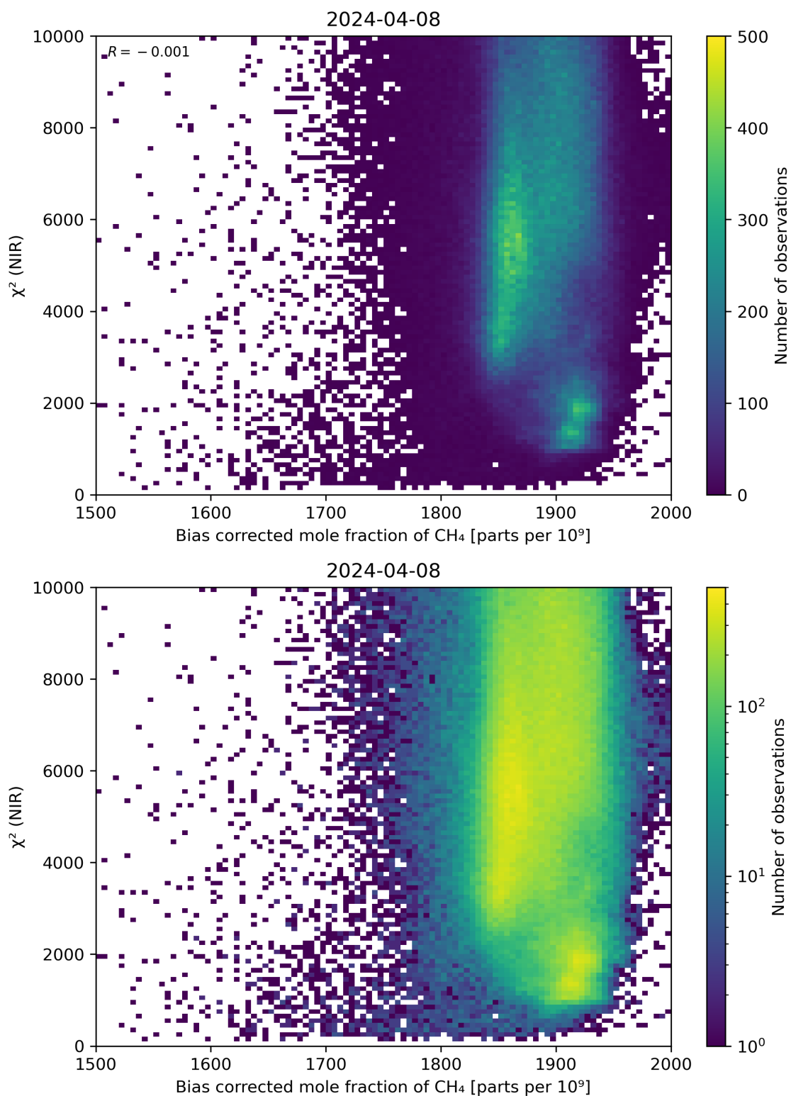
Figure 63: Scatter density plot of “Bias corrected mole fraction of CH 4 ” against “ \chi^2 (NIR)” for 2024-04-07 to 2024-04-09.
