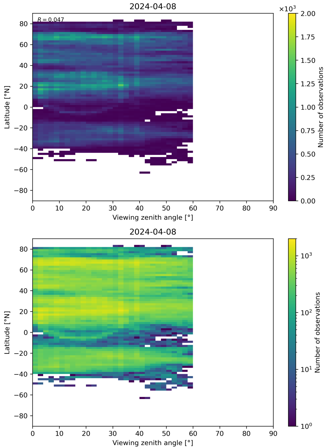
Figure 109: Scatter density plot of “Viewing zenith angle” against “Latitude” for 2024-04-07 to 2024-04-09.
