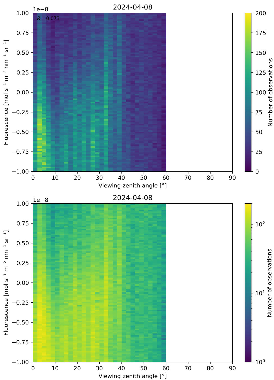
Figure 108: Scatter density plot of “Viewing zenith angle” against “Fluorescence” for 2024-04-07 to 2024-04-09.
