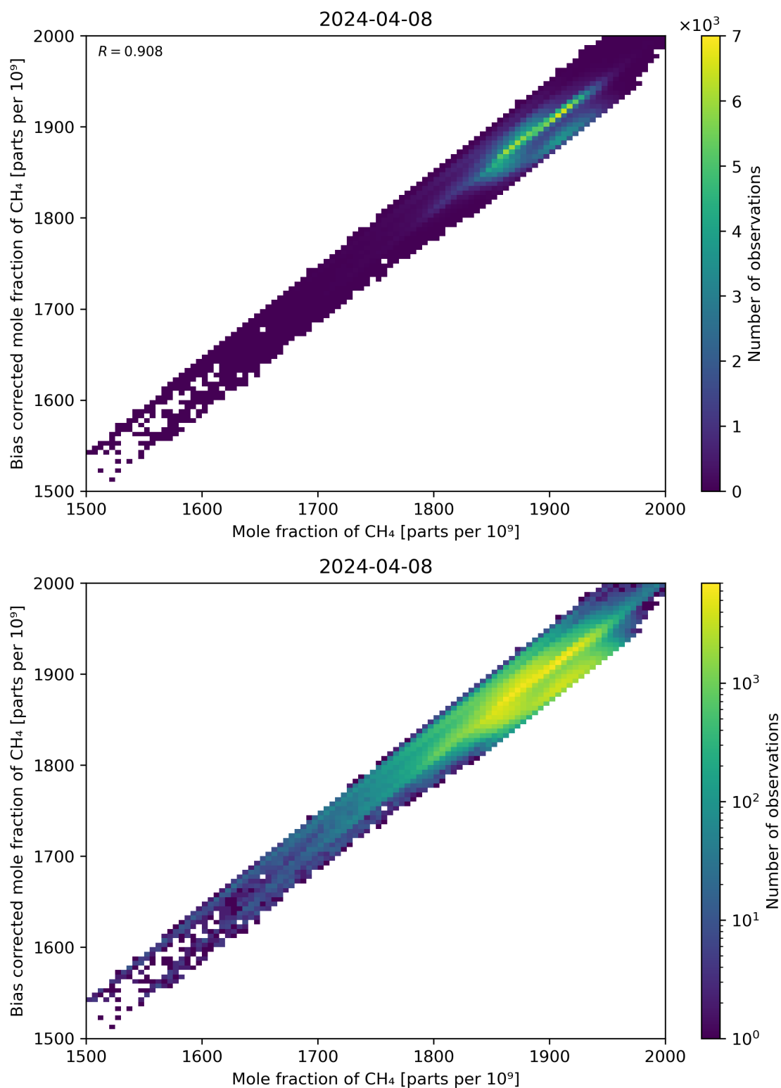
Figure 74: Scatter density plot of “Mole fraction of CH 4 ” against “Bias corrected mole fraction of CH 4 ” for 2024-04-07 to 2024-04-09.
