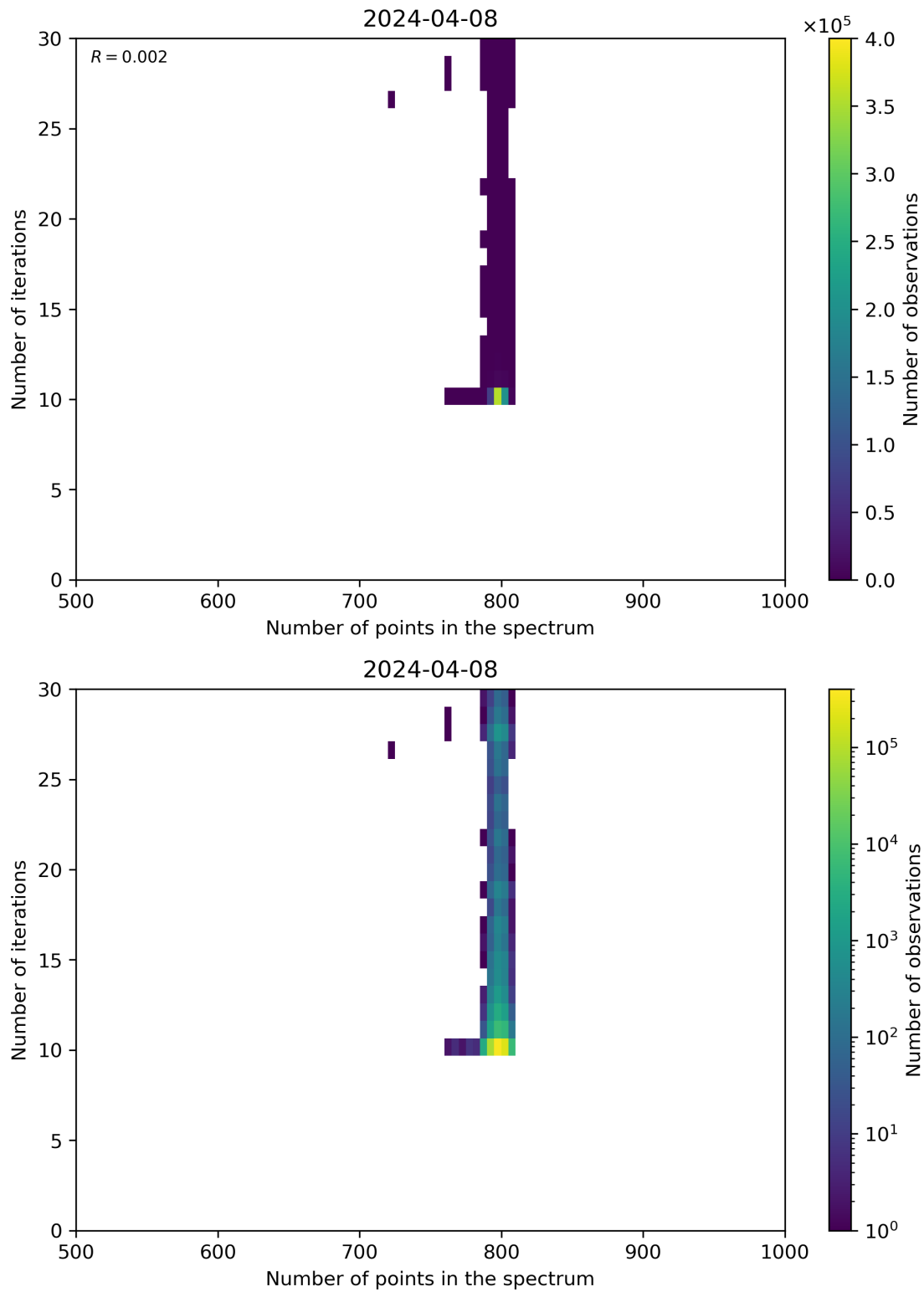
Figure 92: Scatter density plot of “Number of points in the spectrum” against “Number of iterations” for 2024-04-07 to 2024-04-09.
