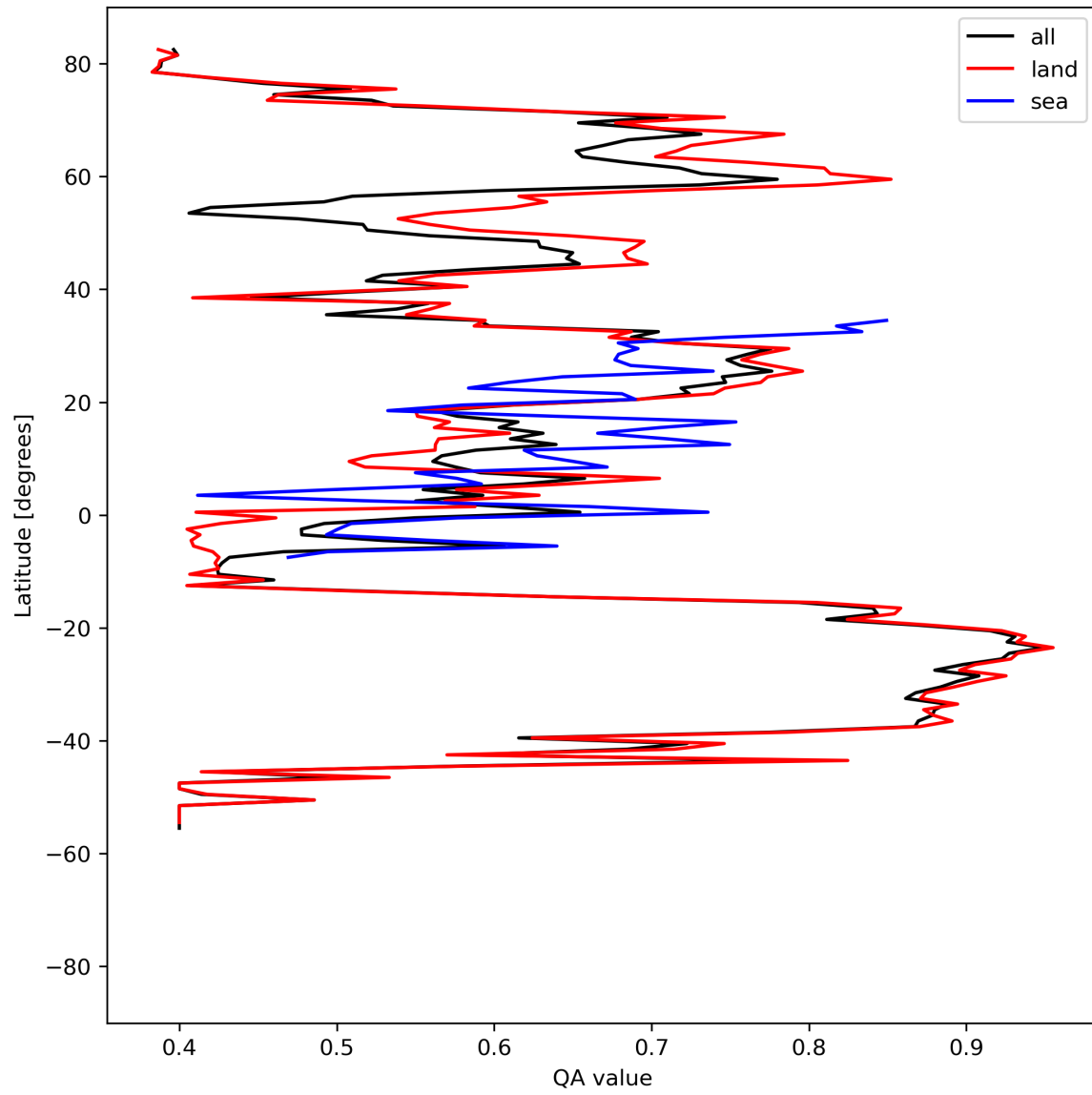
Figure 11: Zonal average of “QA value” for 2024-04-07 to 2024-04-09.
