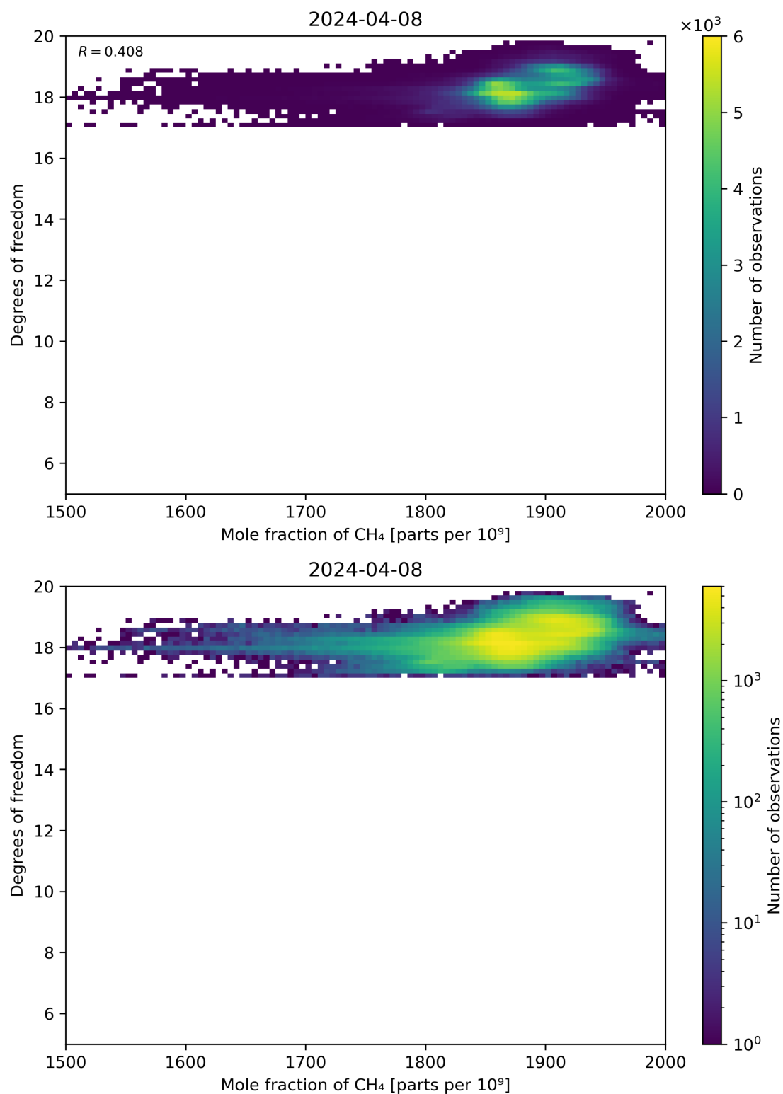
Figure 72: Scatter density plot of “Mole fraction of CH 4 ” against “Degrees of freedom” for 2024-04-07 to 2024-04-09.
