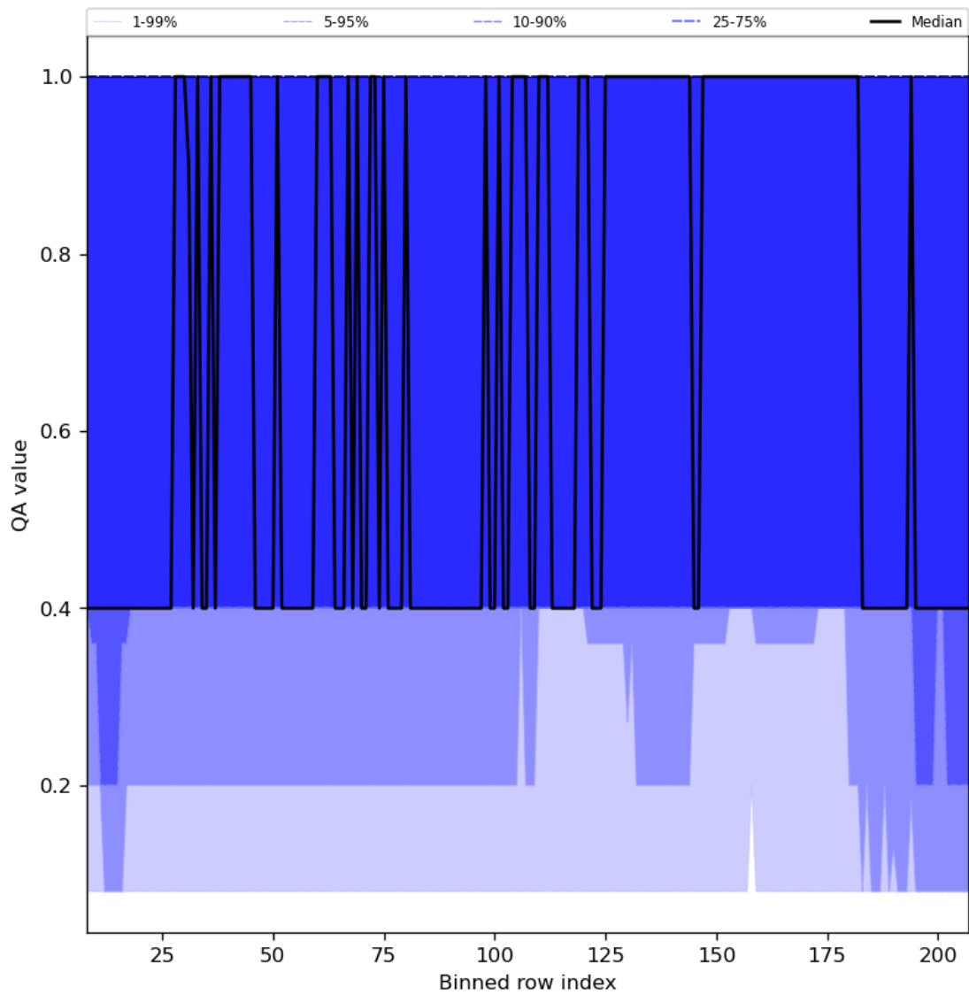
Figure 33: Along track statistics of “QA value” for 2024-04-07 to 2024-04-09
