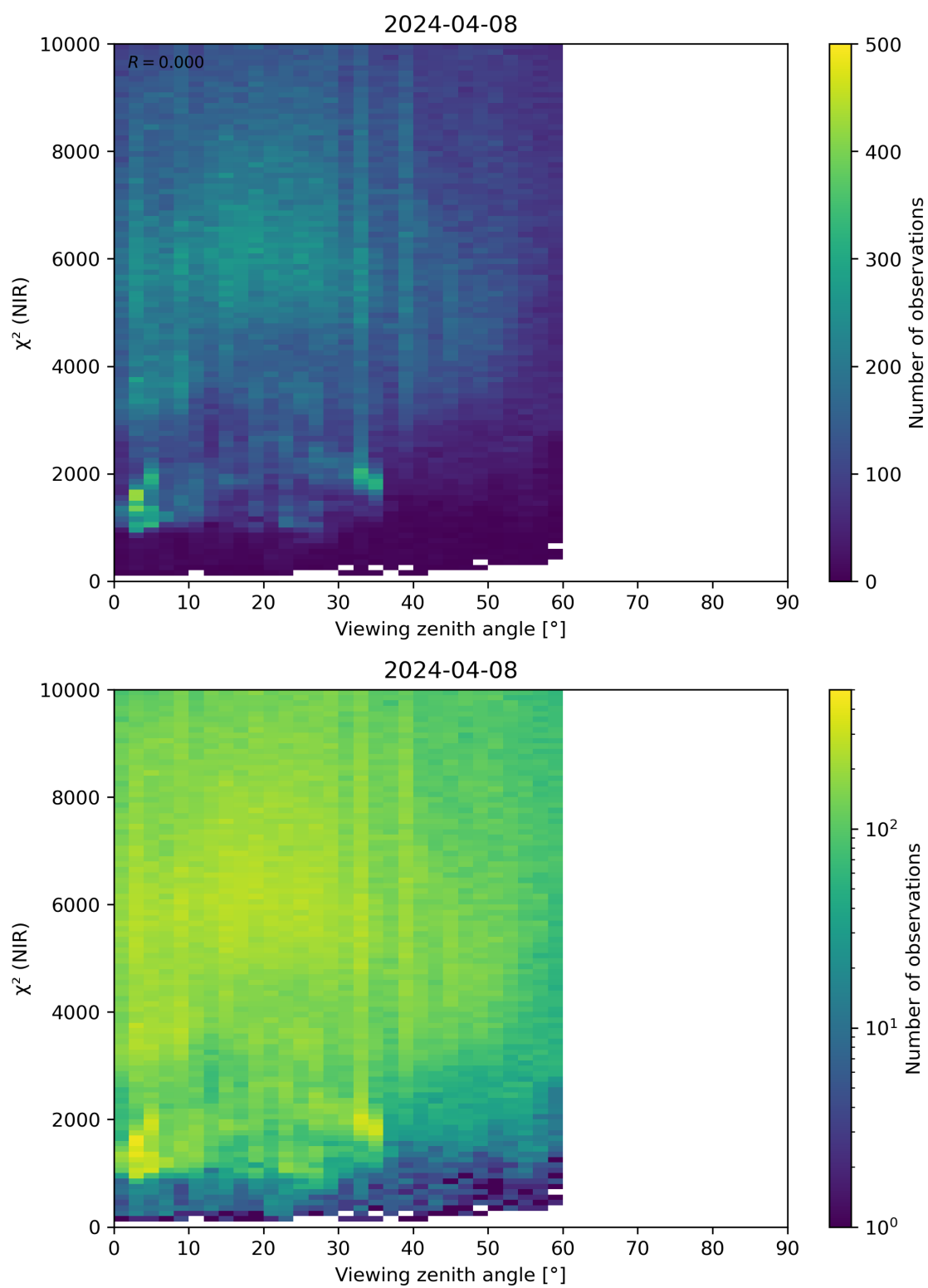
Figure 105: Scatter density plot of “Viewing zenith angle” against “ \chi^2 (NIR)” for 2024-04-07 to 2024-04-09.
