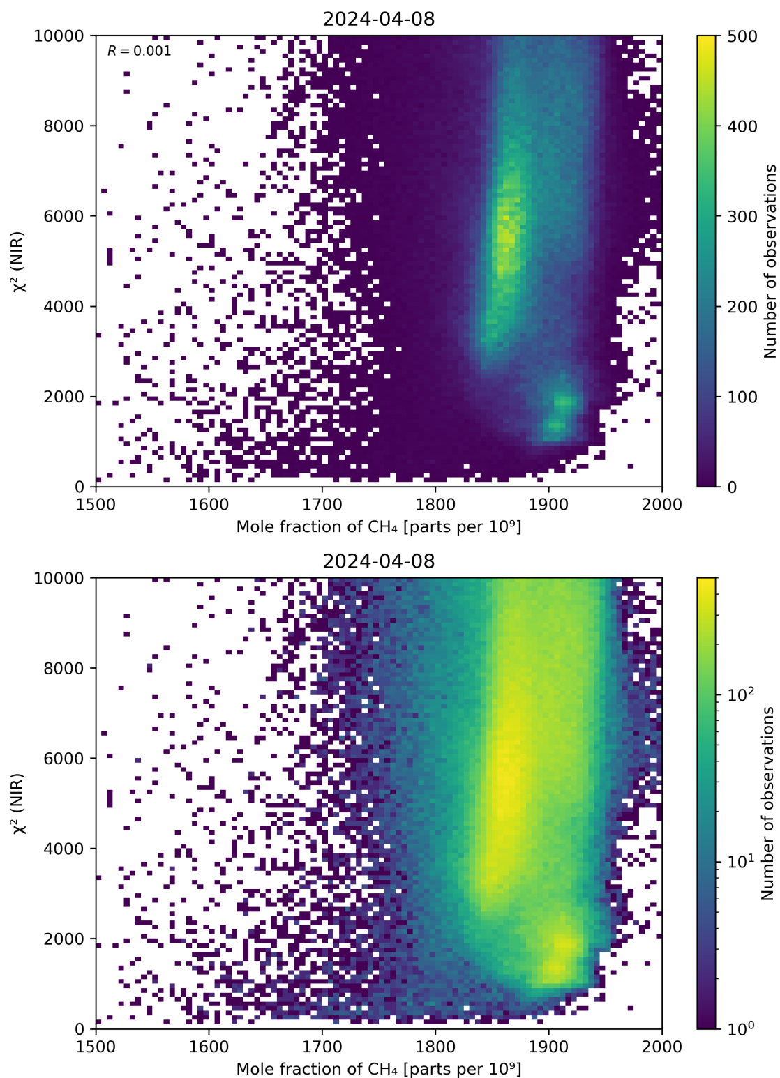
Figure 70: Scatter density plot of “Mole fraction of \text{CH}_4 ” against “ \chi^2 (NIR)” for 2024-04-07 to 2024-04-09.
