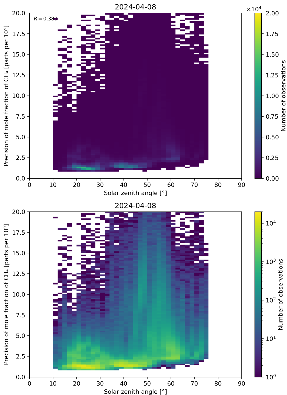
Figure 101: Scatter density plot of “Solar zenith angle” against “Precision of mole fraction of CH 4 ” for 2024-04-07 to 2024-04-09.
