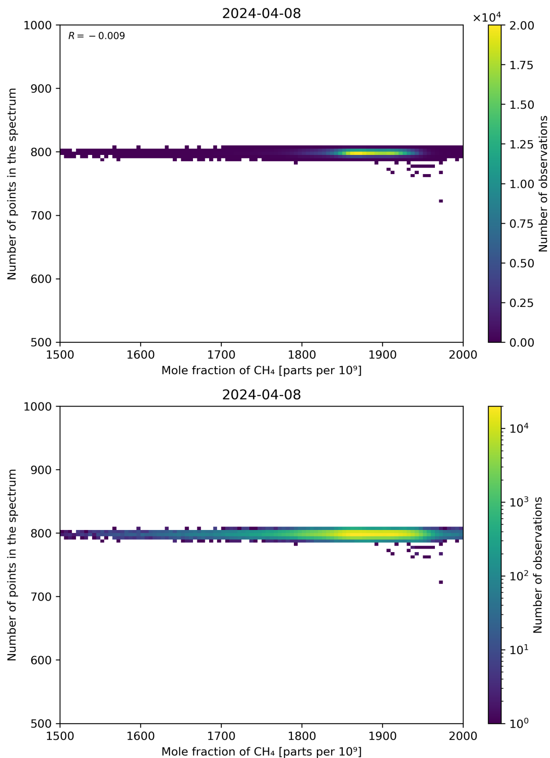
Figure 77: Scatter density plot of “Mole fraction of CH 4 ” against “Number of points in the spectrum” for 2024-04-07 to 2024-04-09.
