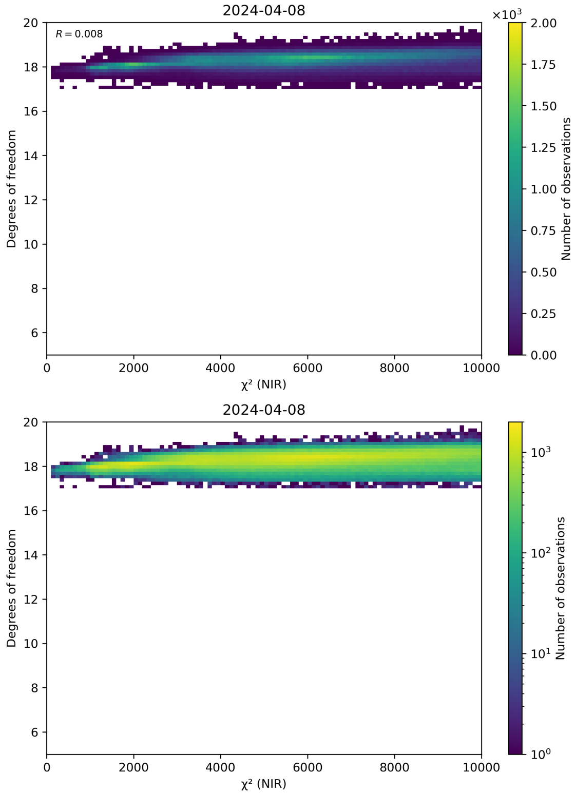
Figure 44: Scatter density plot of “ \chi^2 (NIR)” against “Degrees of freedom” for 2024-04-07 to 2024-04-09.
