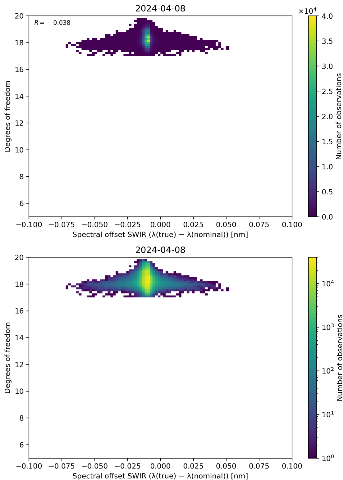
Figure 119: Scatter density plot of “Spectral offset SWIR ( \lambda(\text{true}) - \lambda(\text{nominal}) )” against “Degrees of freedom” for 2024-04-07 to 2024-04-09.
