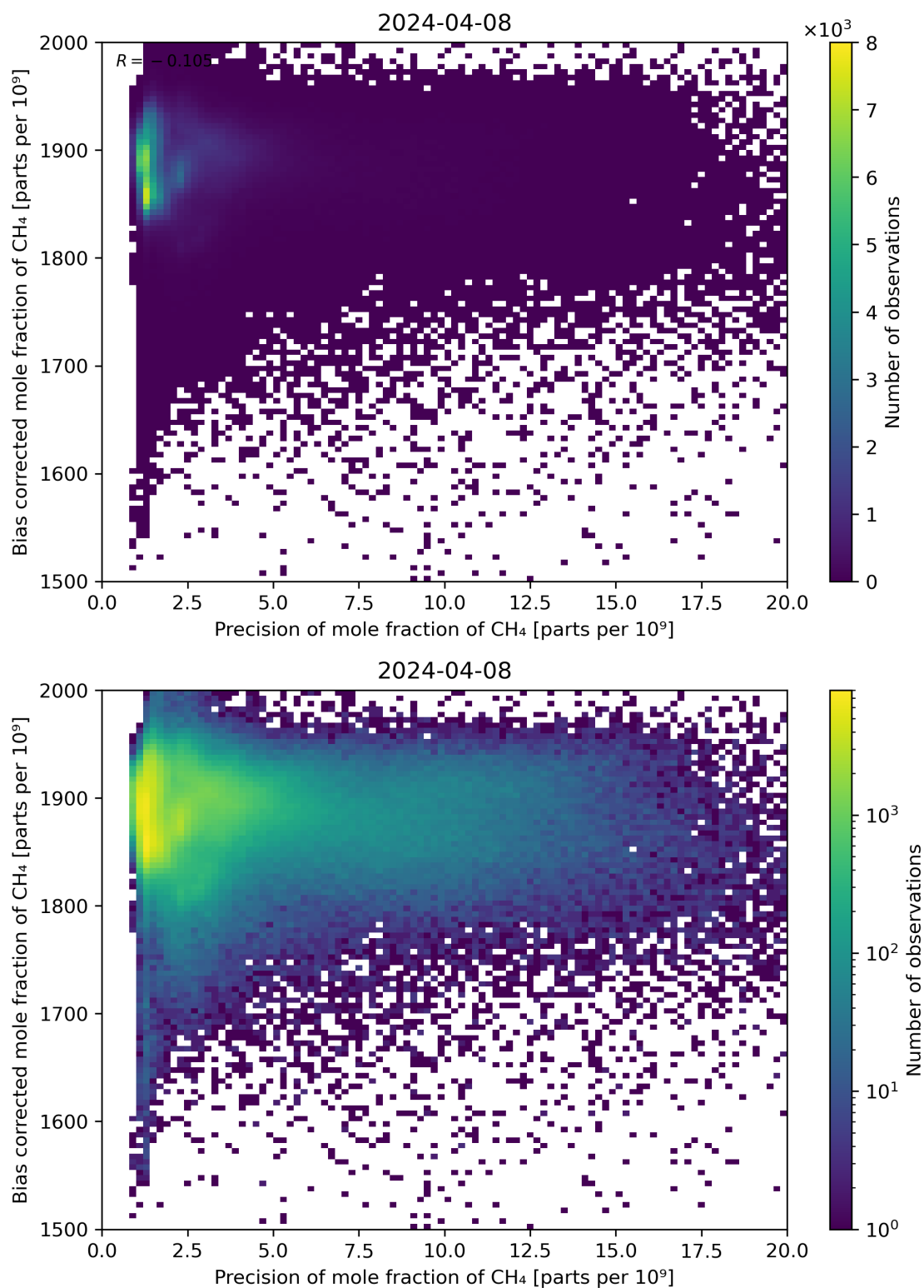
Figure 82: Scatter density plot of “Precision of mole fraction of CH 4 ” against “Bias corrected mole fraction of CH 4 ” for 2024-04-07 to 2024-04-09.
