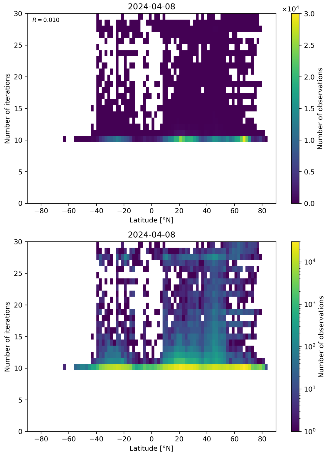
Figure 60: Scatter density plot of “Latitude” against “Number of iterations” for 2024-04-07 to 2024-04-09.
