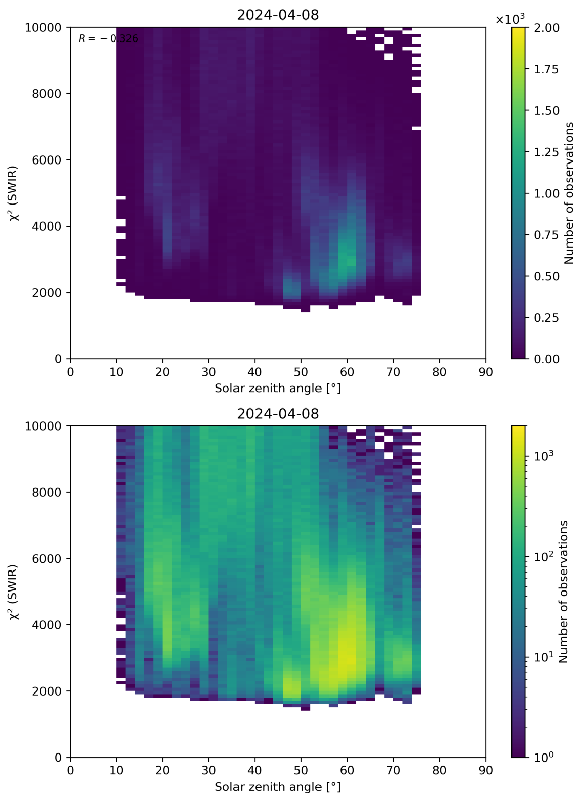
Figure 95: Scatter density plot of “Solar zenith angle” against “ \chi^2 (SWIR)” for 2024-04-07 to 2024-04-09.
