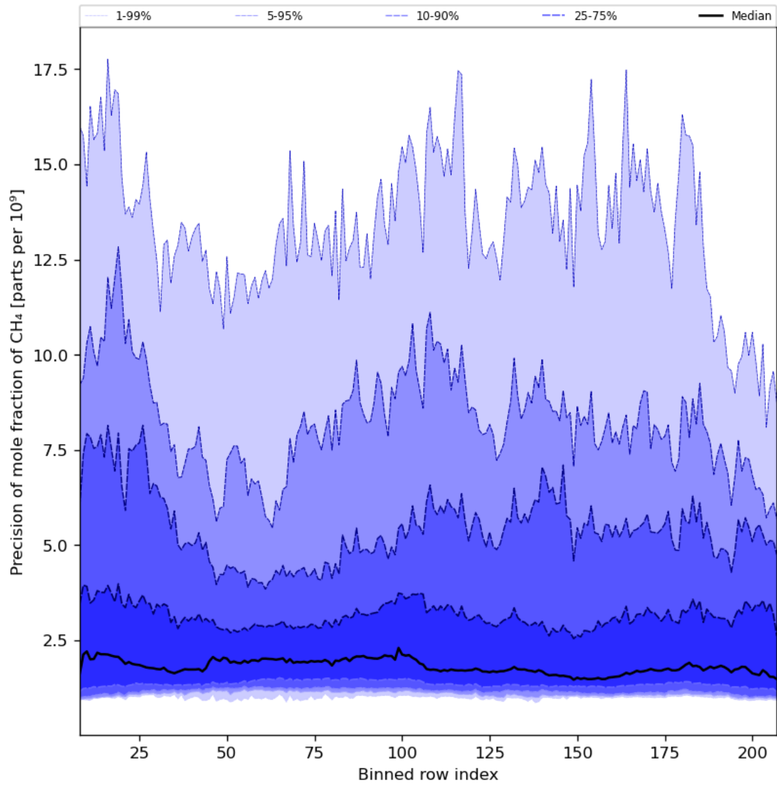
Figure 35: Along track statistics of “Precision of mole fraction of CH 4 ” for 2024-04-07 to 2024-04-09
