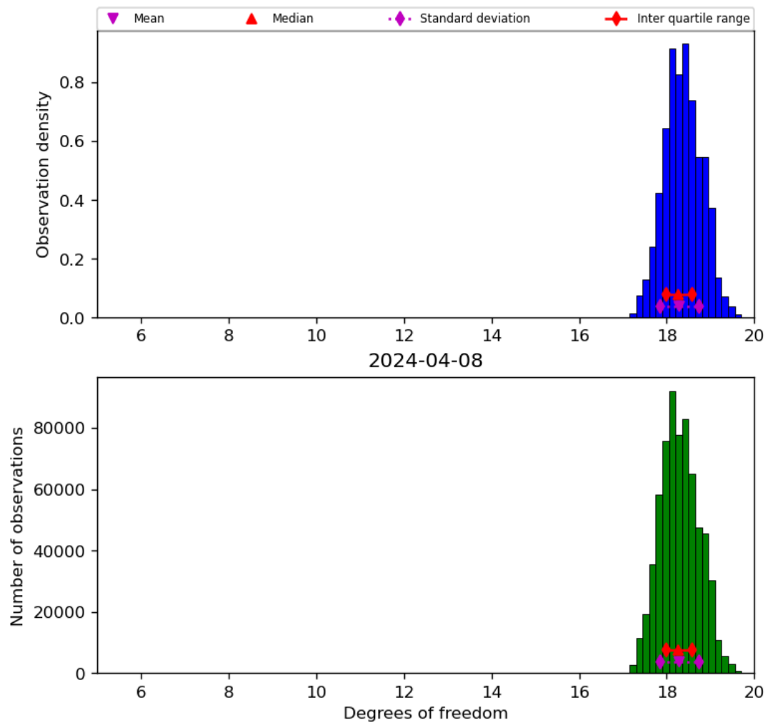
Figure 30: Histogram of “Degrees of freedom” for 2024-04-07 to 2024-04-09
