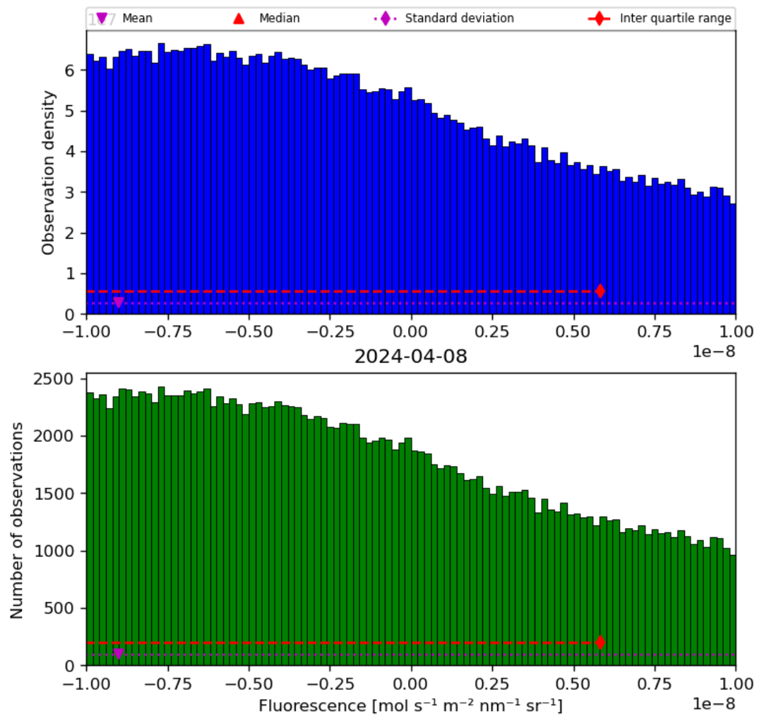
Figure 32: Histogram of “Fluorescence” for 2024-04-07 to 2024-04-09
