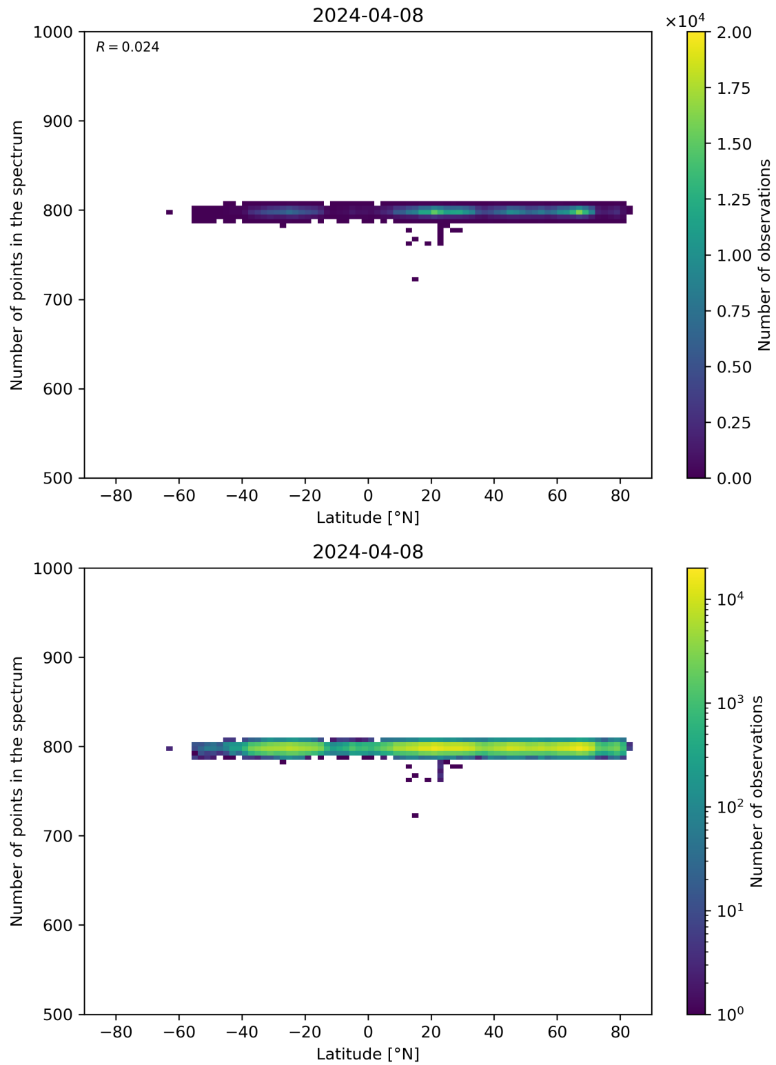
Figure 61: Scatter density plot of “Latitude” against “Number of points in the spectrum” for 2024-04-07 to 2024-04-09.
