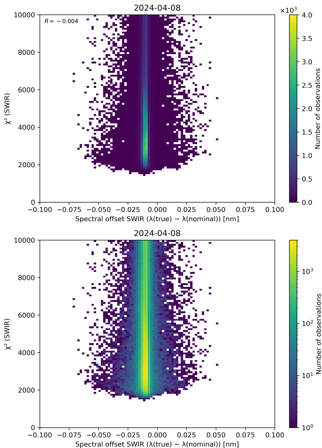
Figure 118: Scatter density plot of “Spectral offset SWIR ( \lambda(\text{true}) - \lambda(\text{nominal}) )” against “ \chi^2 (SWIR)” for 2024-04-07 to 2024-04-09.
