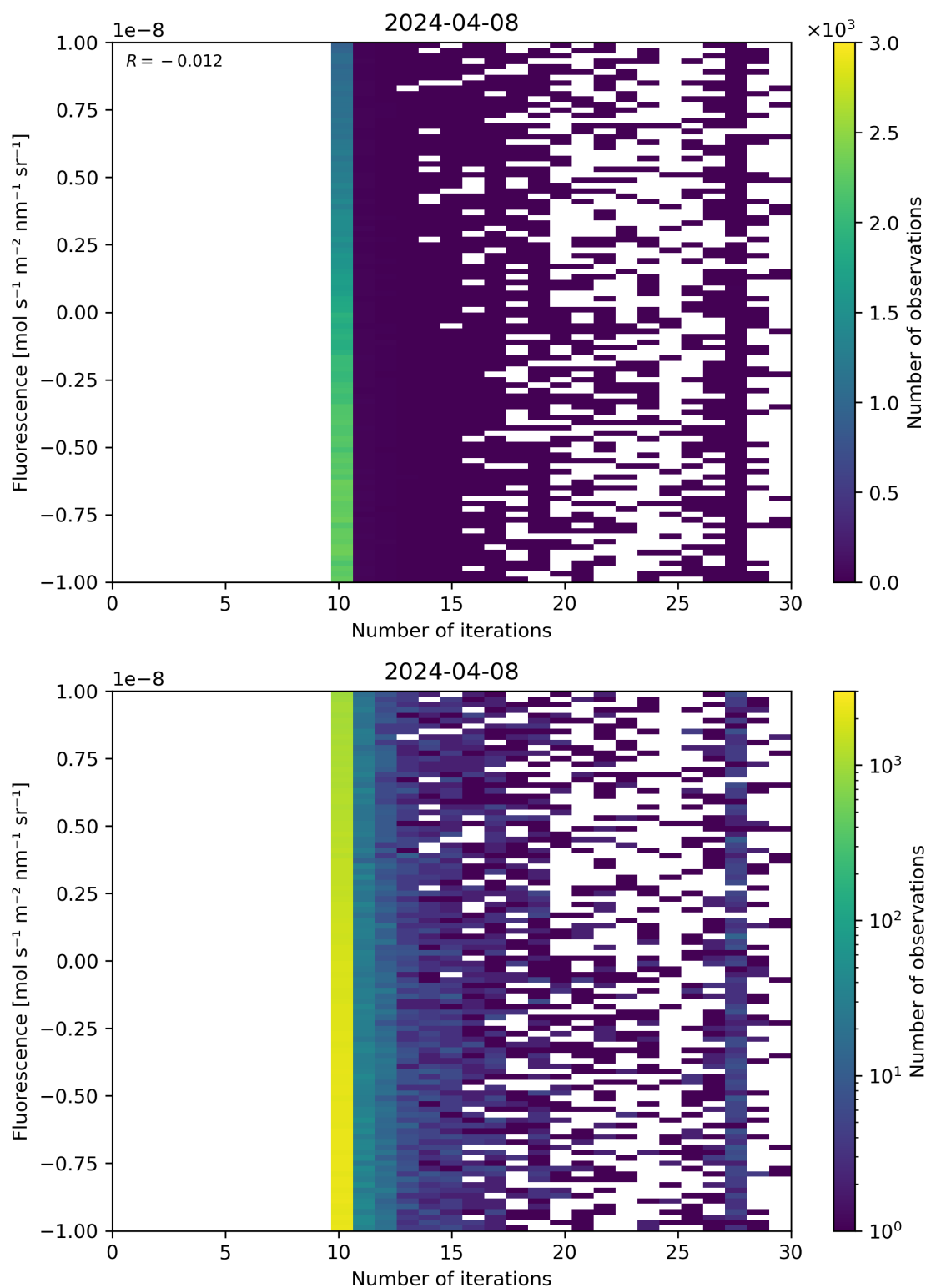
Figure 87: Scatter density plot of “Number of iterations” against “Fluorescence” for 2024-04-07 to 2024-04-09.
