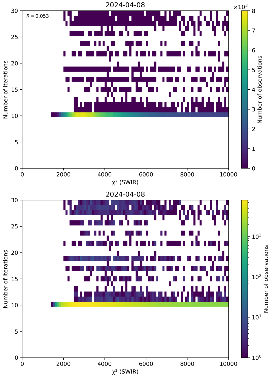
Figure 50: Scatter density plot of “ \chi^2 (SWIR)” against “Number of iterations” for 2024-04-07 to 2024-04-09.
