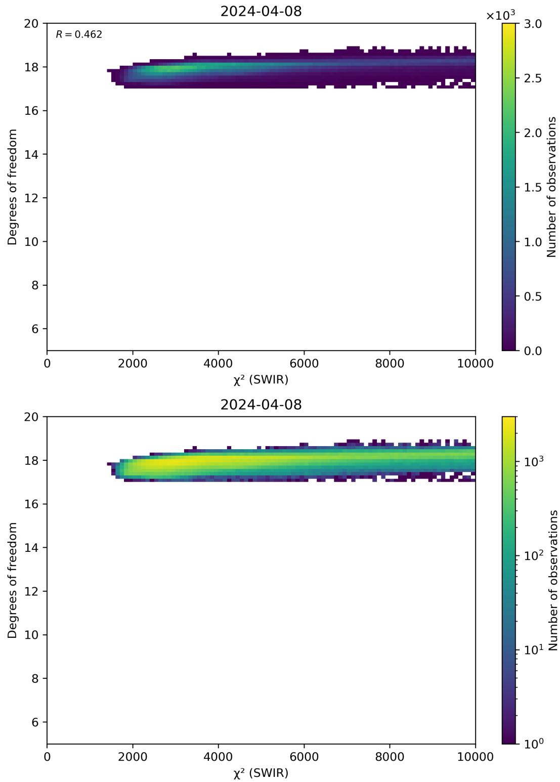
Figure 48: Scatter density plot of “ \chi^2 (SWIR)” against “Degrees of freedom” for 2024-04-07 to 2024-04-09.
