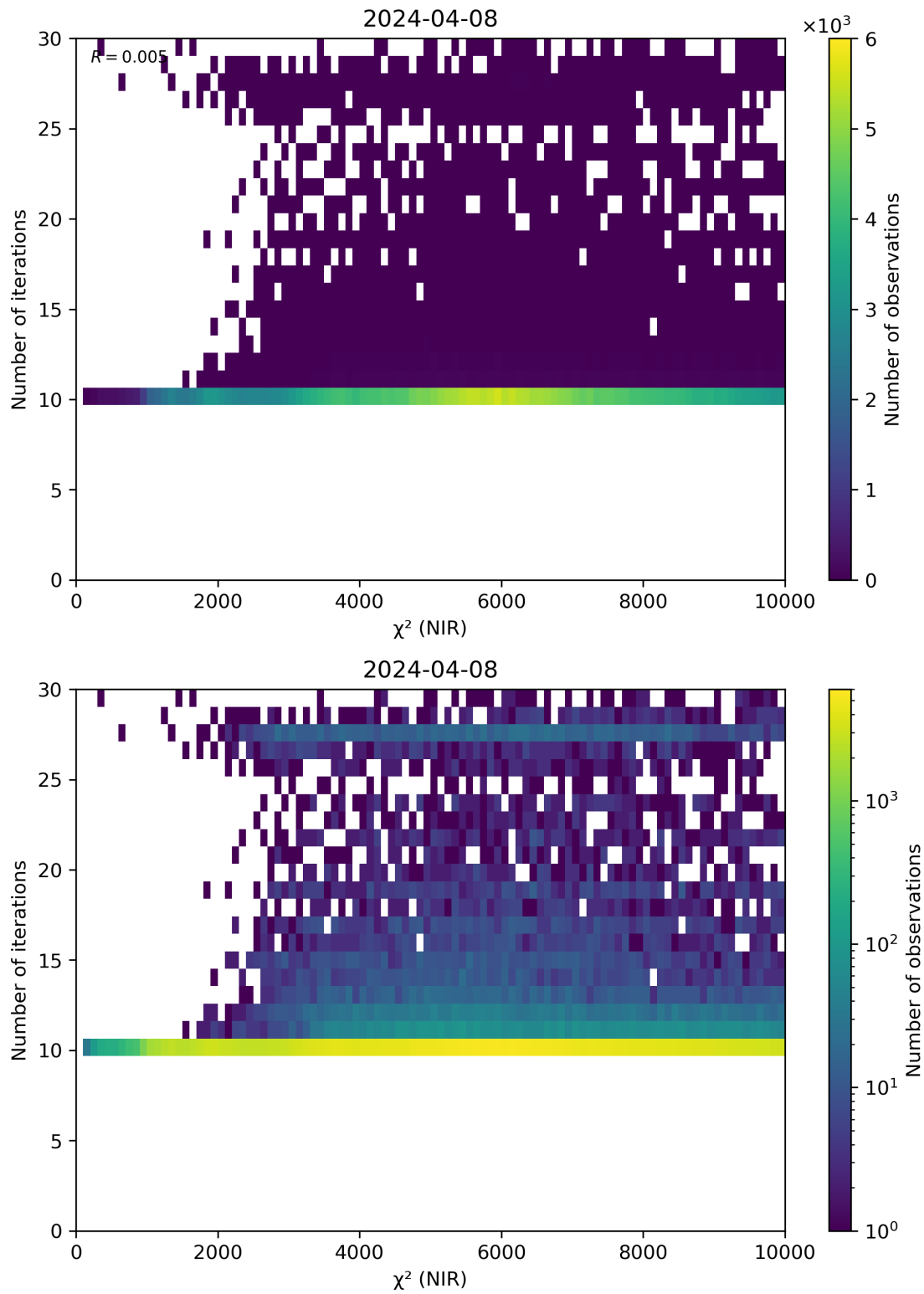
Figure 46: Scatter density plot of “ \chi^2 (NIR)” against “Number of iterations” for 2024-04-07 to 2024-04-09.
