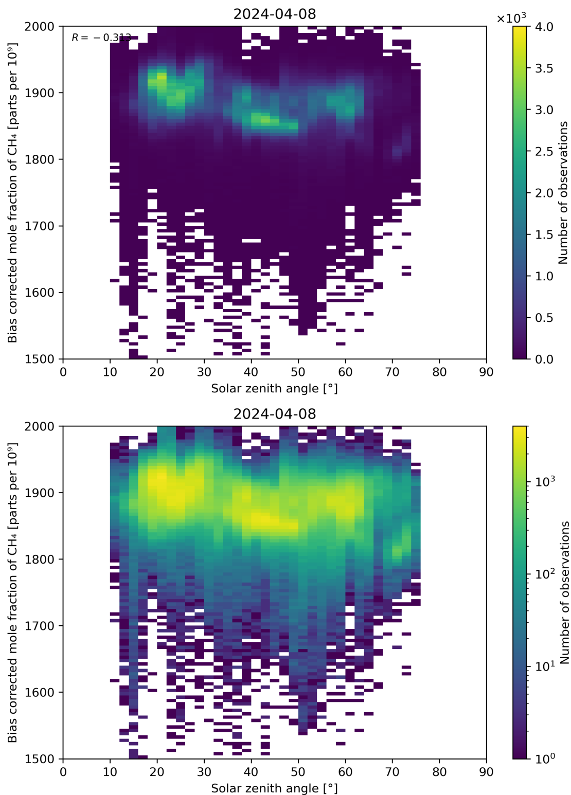
Figure 100: Scatter density plot of “Solar zenith angle” against “Bias corrected mole fraction of \text{CH}_4 ” for 2024-04-07 to 2024-04-09.
