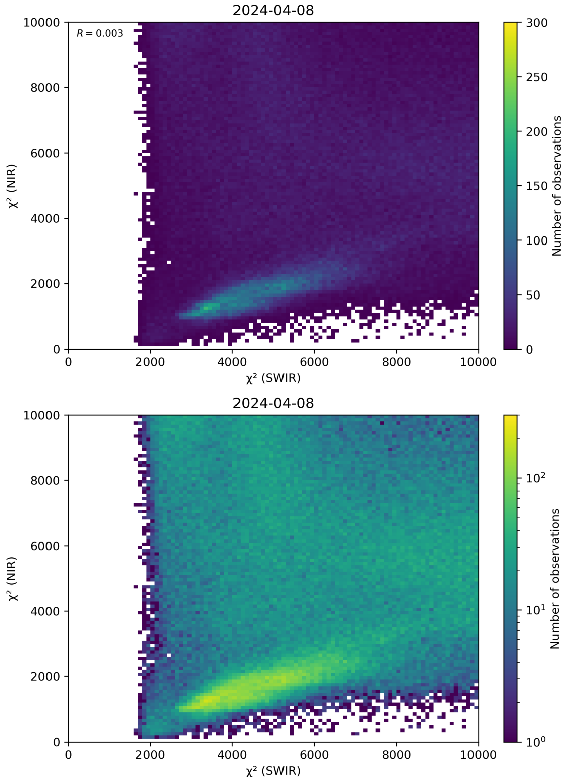
Figure 47: Scatter density plot of “ \chi^2 (SWIR)” against “ \chi^2 (NIR)” for 2024-04-07 to 2024-04-09.
