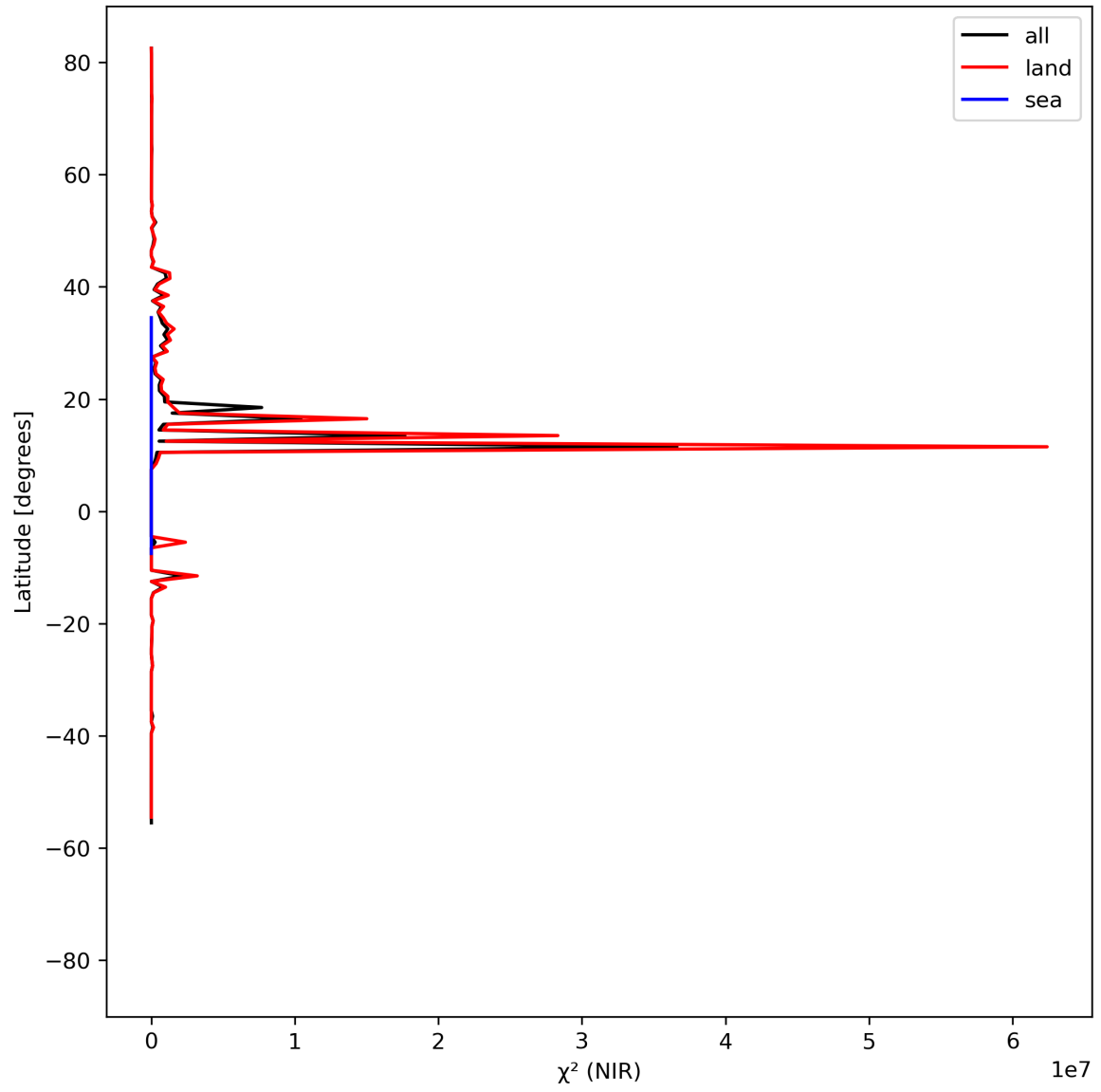
Figure 18: Zonal average of “ \chi^2 (NIR)” for 2024-04-07 to 2024-04-09.
