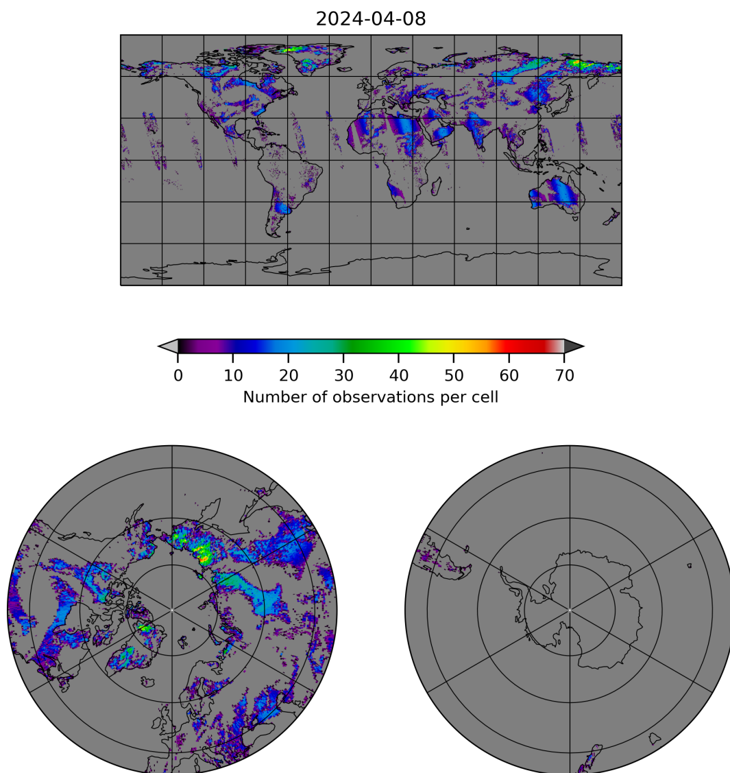
Figure 10: Map of the number of observations for 2024-04-07 to 2024-04-09
