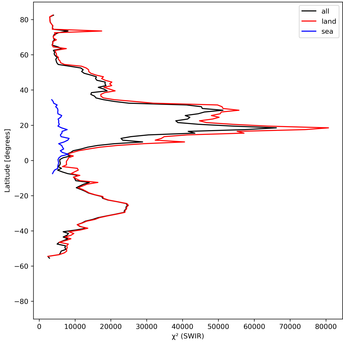
Figure 17: Zonal average of “ \chi^2 (SWIR)” for 2024-04-07 to 2024-04-09.
