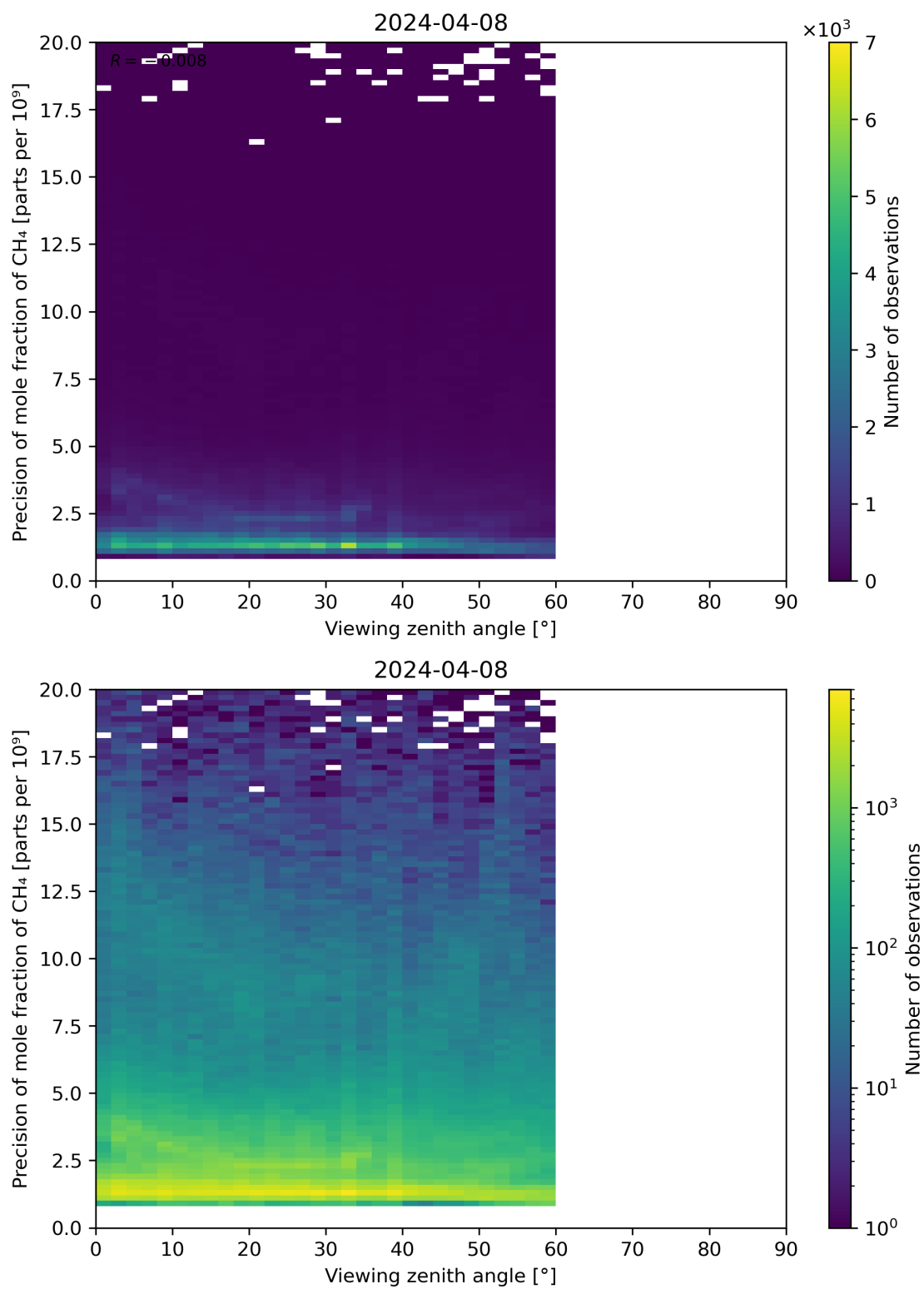
Figure 112: Scatter density plot of “Viewing zenith angle” against “Precision of mole fraction of CH 4 ” for 2024-04-07 to 2024-04-09.
