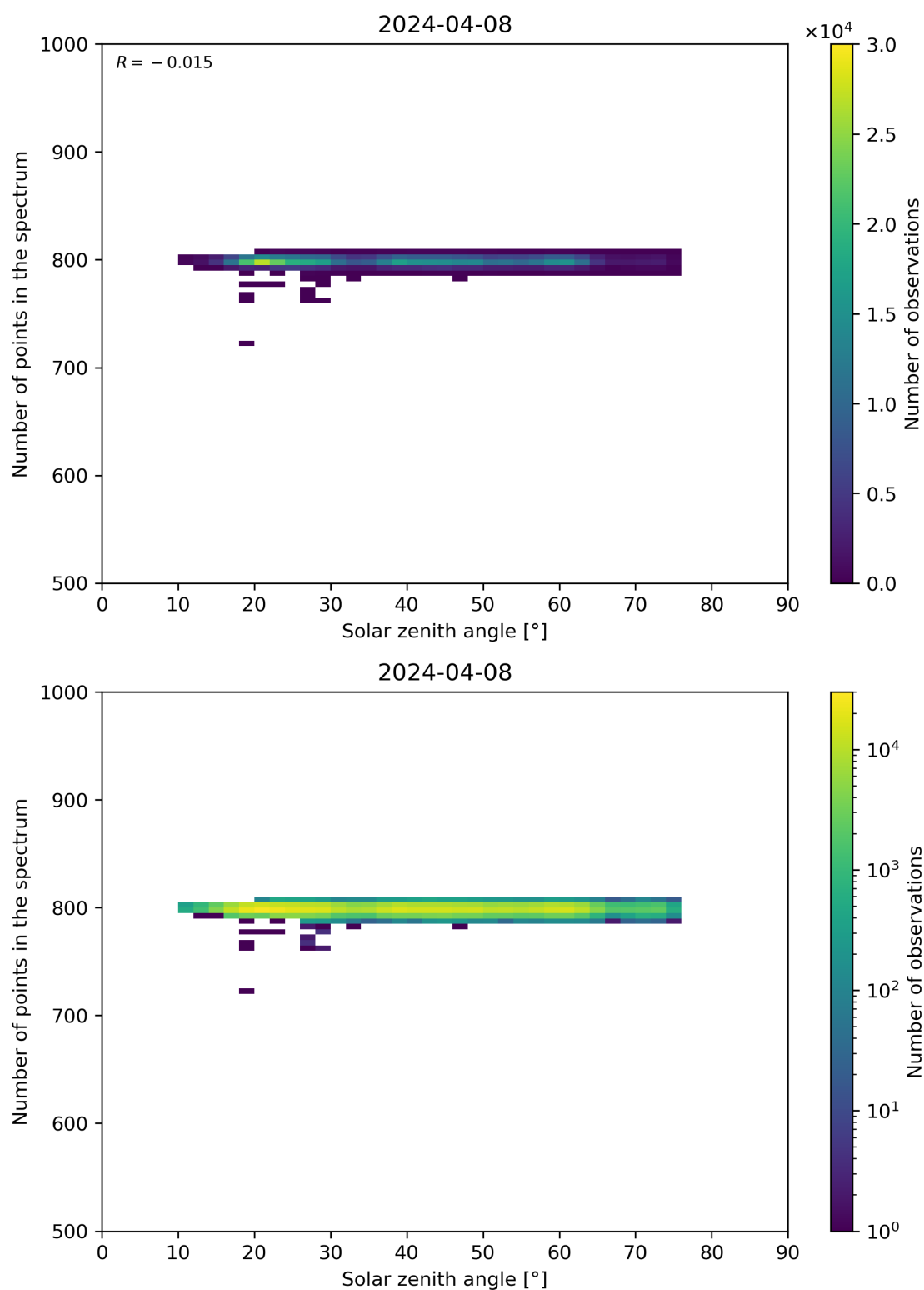
Figure 103: Scatter density plot of “Solar zenith angle” against “Number of points in the spectrum” for 2024-04-07 to 2024-04-09.
