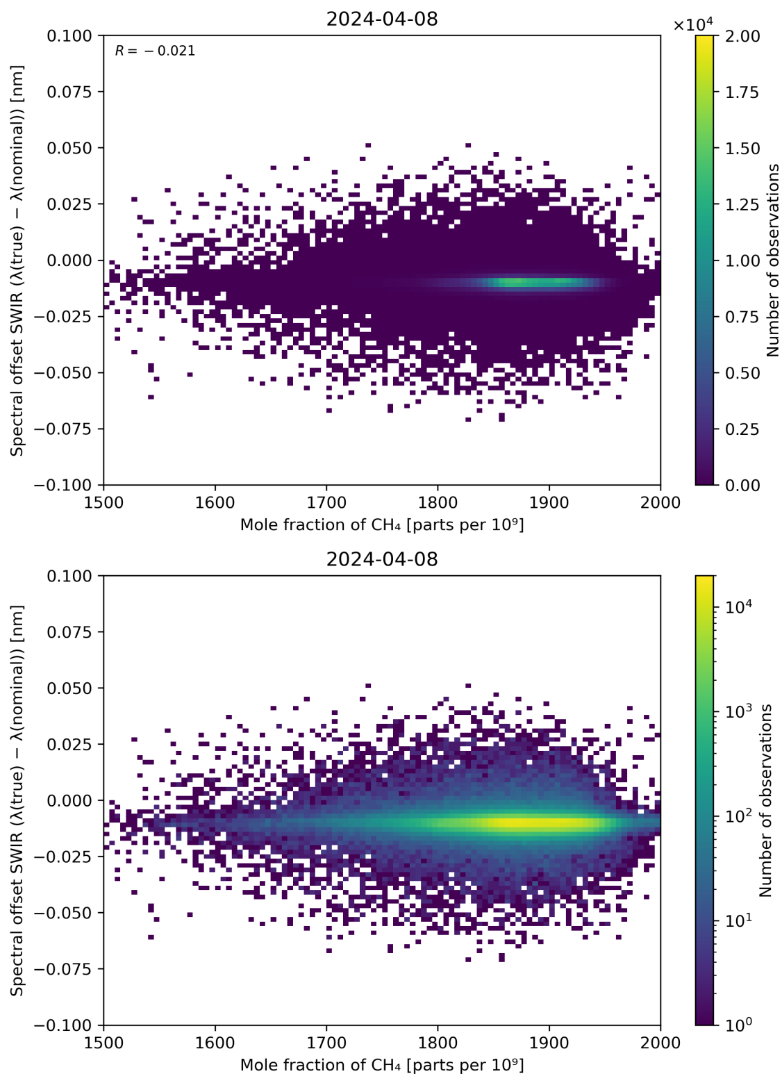
Figure 86: Scatter density plot of “Mole fraction of CH 4 ” against “Spectral offset SWIR ( \lambda(\text{true}) - \lambda(\text{nominal}) )” for 2024-04-07 to 2024-04-09.
