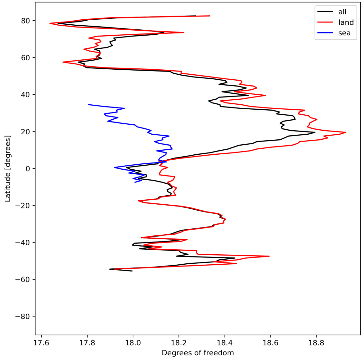
Figure 19: Zonal average of “Degrees of freedom” for 2024-04-07 to 2024-04-09.
