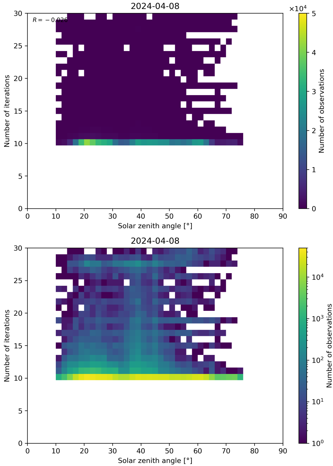
Figure 102: Scatter density plot of “Solar zenith angle” against “Number of iterations” for 2024-04-07 to 2024-04-09.
