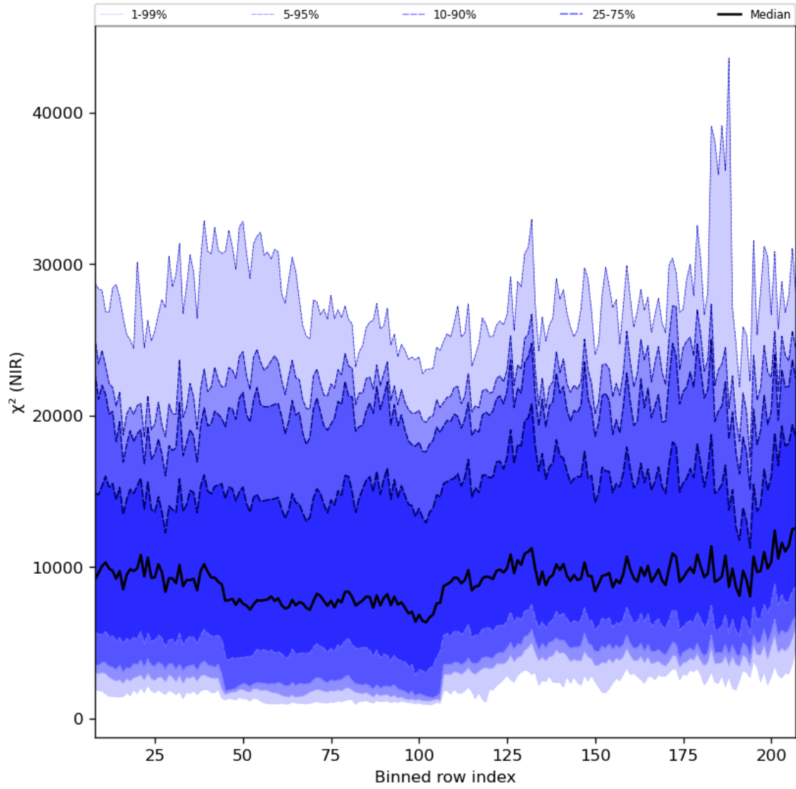
Figure 40: Along track statistics of “ \chi^2 (NIR)” for 2024-04-07 to 2024-04-09
