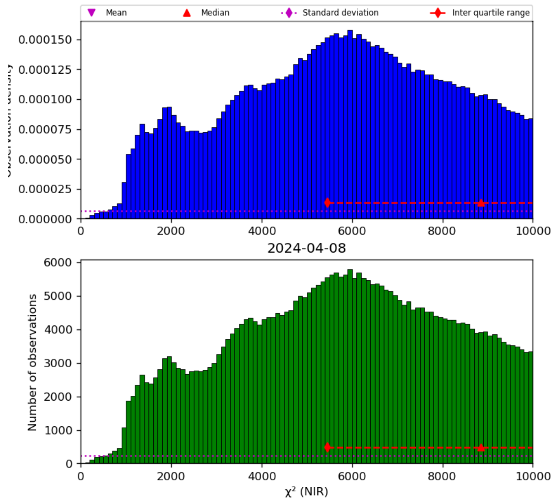
Figure 29: Histogram of “ \chi^2 (NIR)” for 2024-04-07 to 2024-04-09
