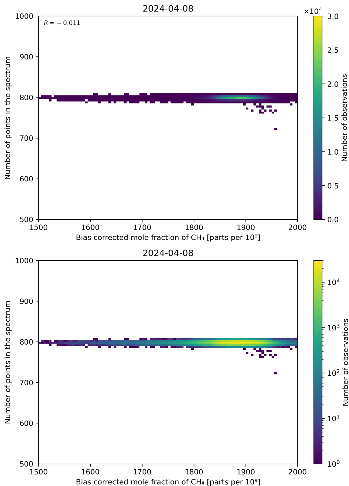
Figure 68: Scatter density plot of “Bias corrected mole fraction of CH 4 ” against “Number of points in the spectrum” for 2024-04-07 to 2024-04-09.
