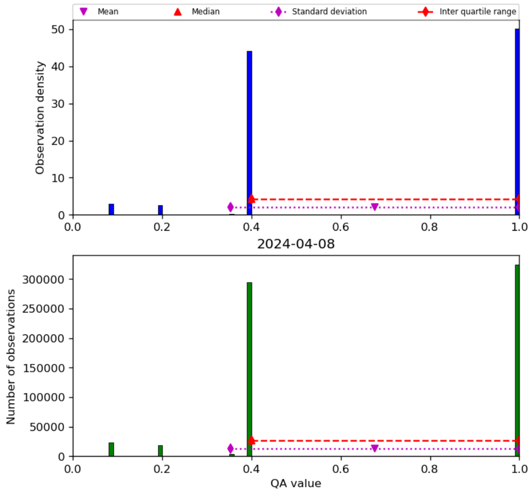
Figure 22: Histogram of “QA value” for 2024-04-07 to 2024-04-09
