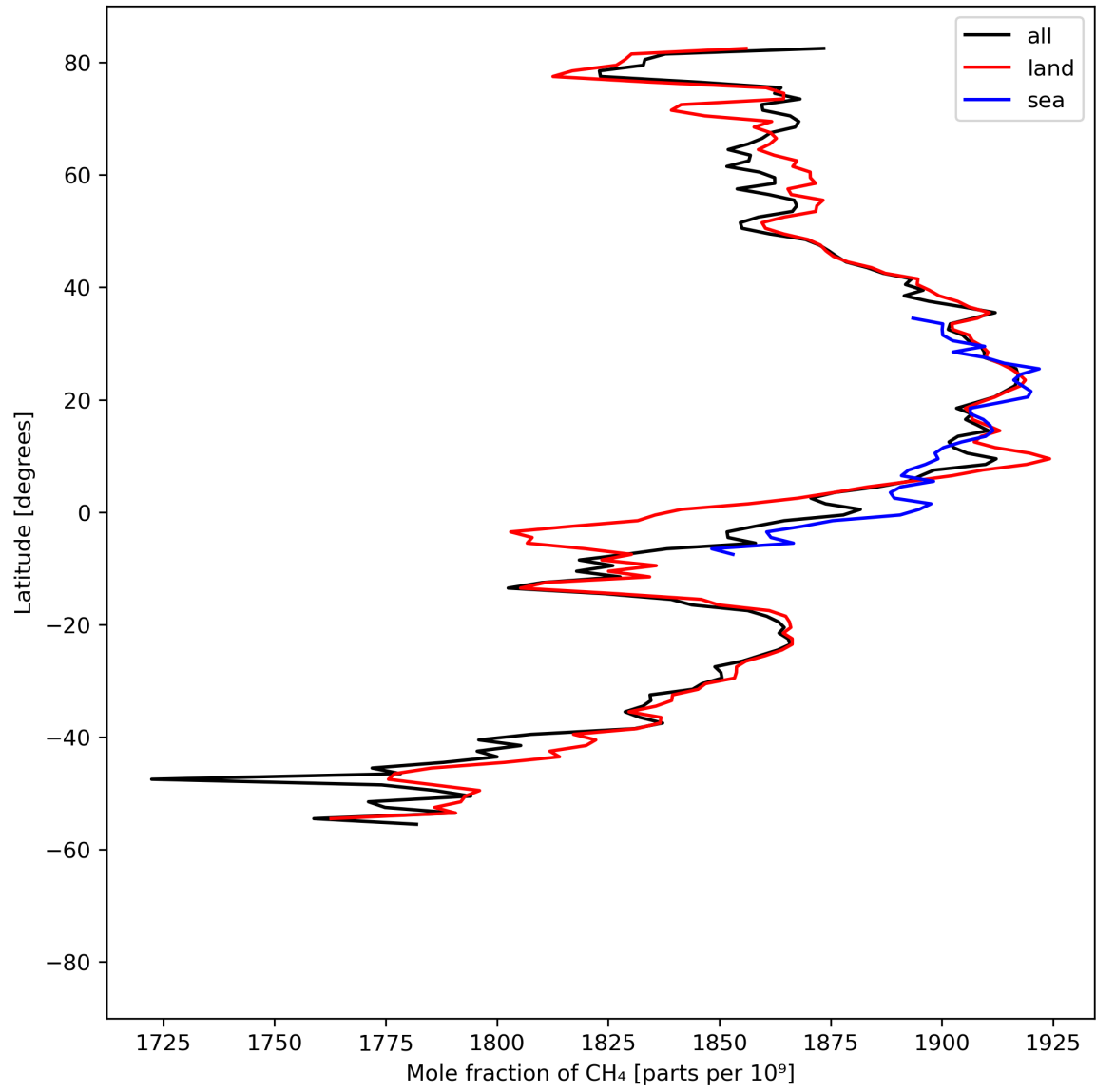
Figure 12: Zonal average of “Mole fraction of \text{CH}_4 ” for 2024-04-07 to 2024-04-09.
