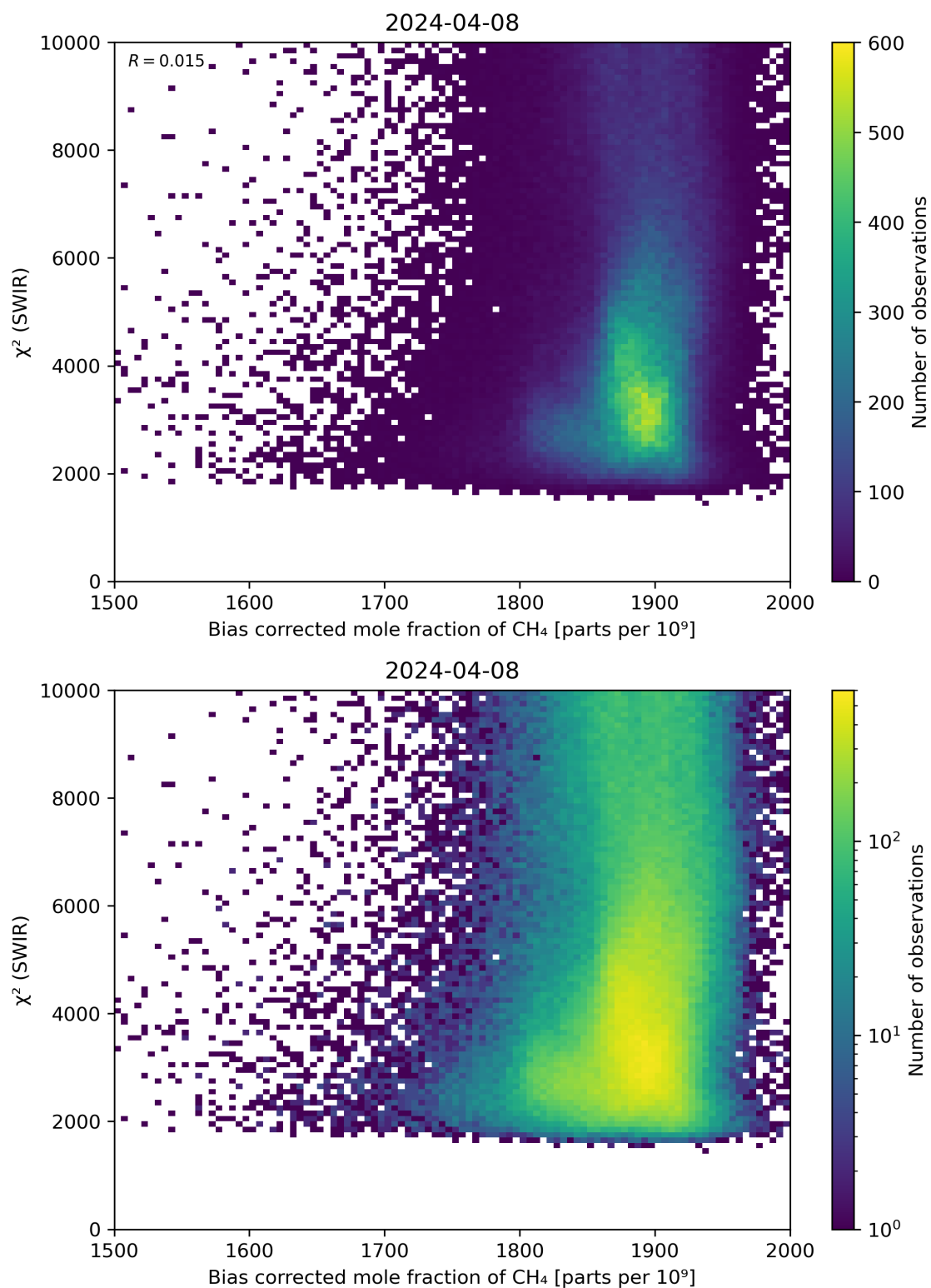
Figure 64: Scatter density plot of “Bias corrected mole fraction of CH 4 ” against “ \chi^2 (SWIR)” for 2024-04-07 to 2024-04-09.
