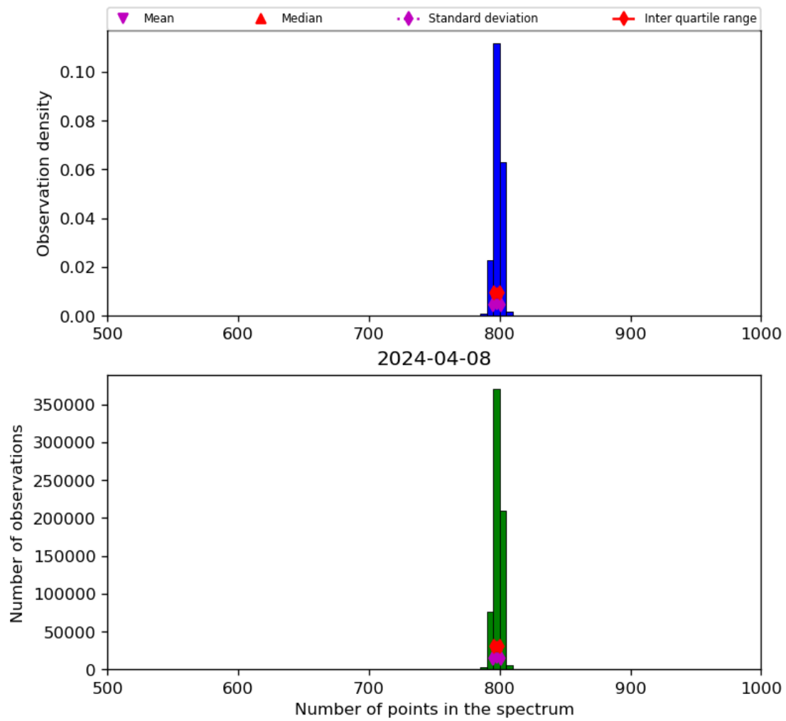
Figure 26: Histogram of “Number of points in the spectrum” for 2024-04-07 to 2024-04-09
