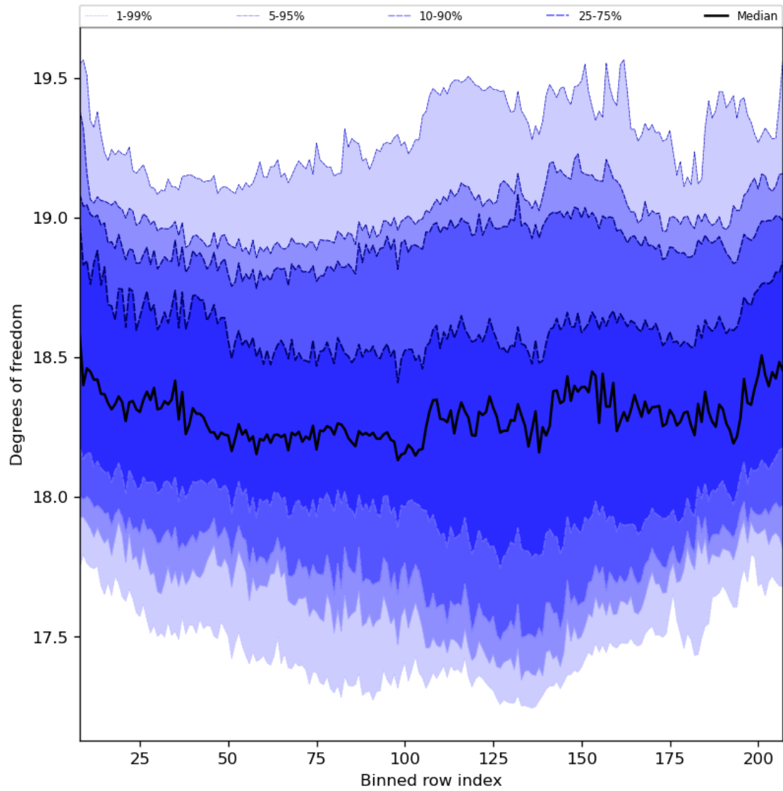
Figure 41: Along track statistics of “Degrees of freedom” for 2024-04-07 to 2024-04-09
