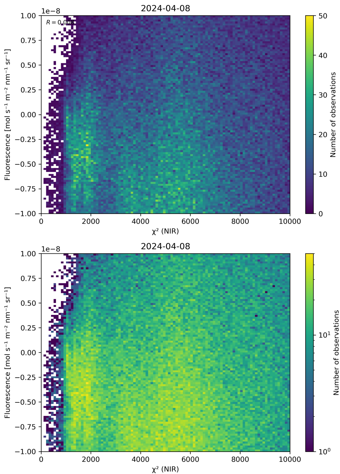
Figure 45: Scatter density plot of “ \chi^2 (NIR)” against “Fluorescence” for 2024-04-07 to 2024-04-09.
