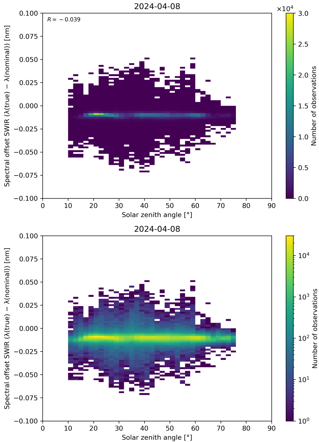
Figure 104: Scatter density plot of “Solar zenith angle” against “Spectral offset SWIR ( \lambda(\text{true}) - \lambda(\text{nominal}) )” for 2024-04-07 to 2024-04-09.
