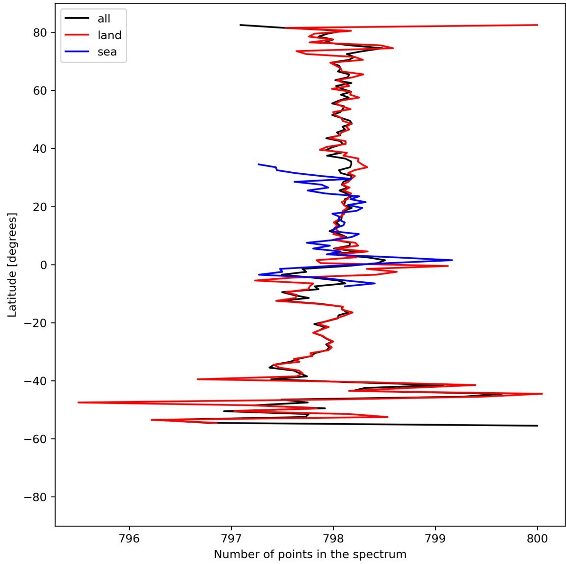
Figure 15: Zonal average of “Number of points in the spectrum” for 2024-04-07 to 2024-04-09.
