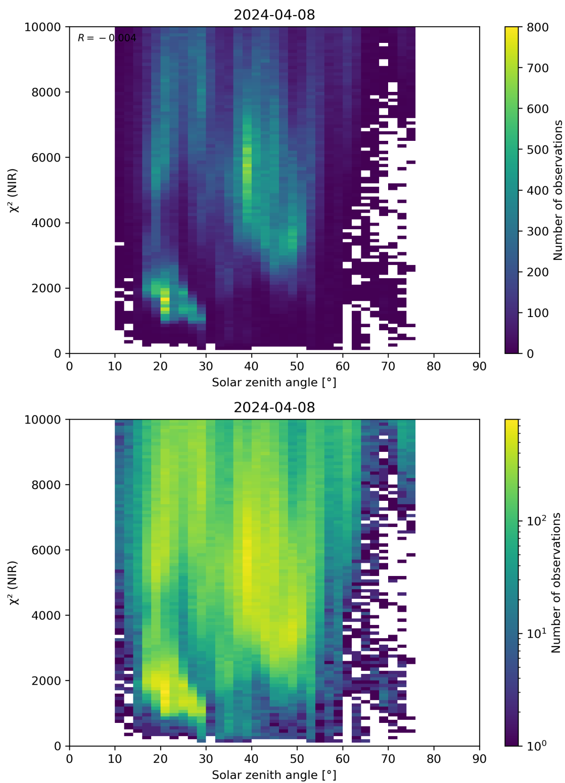
Figure 94: Scatter density plot of “Solar zenith angle” against “ \chi^2 (NIR)” for 2024-04-07 to 2024-04-09.
