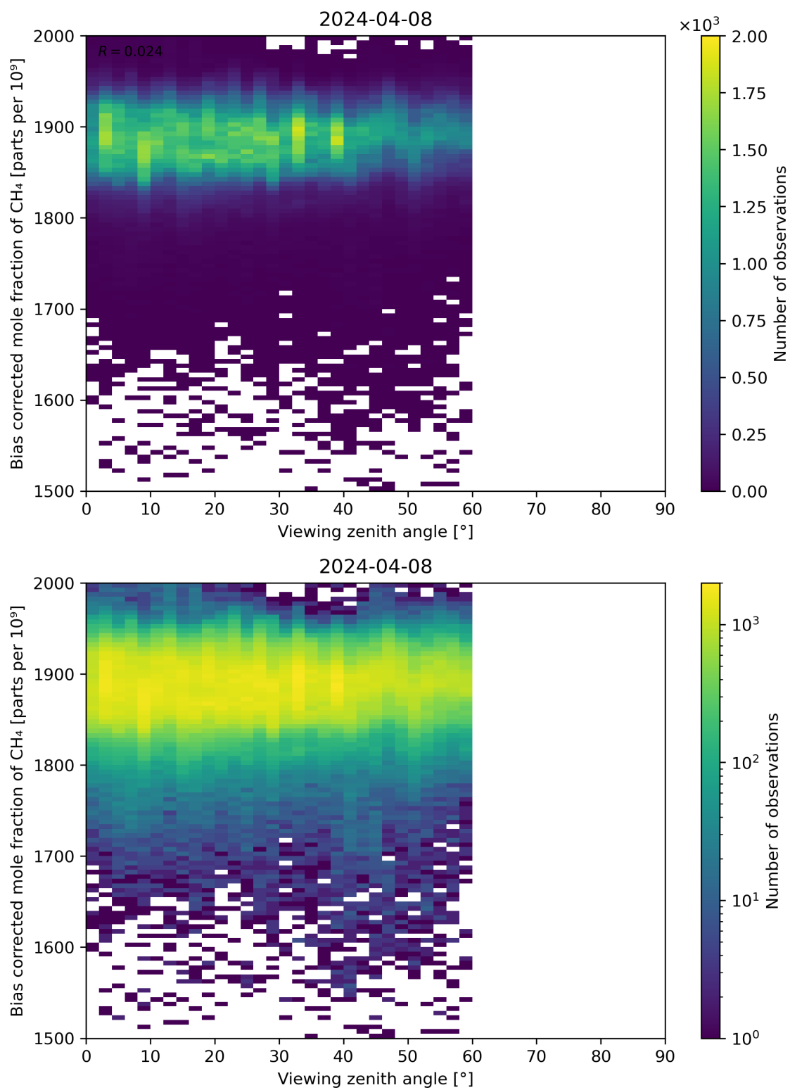
Figure 111: Scatter density plot of “Viewing zenith angle” against “Bias corrected mole fraction of CH 4 ” for 2024-04-07 to 2024-04-09.
