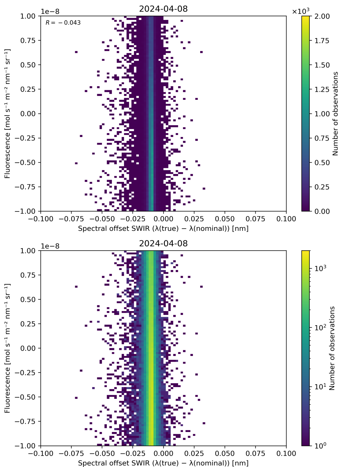
Figure 120: Scatter density plot of “Spectral offset SWIR ( \lambda(\text{true}) - \lambda(\text{nominal}) )” against “Fluorescence” for 2024-04-07 to 2024-04-09.
