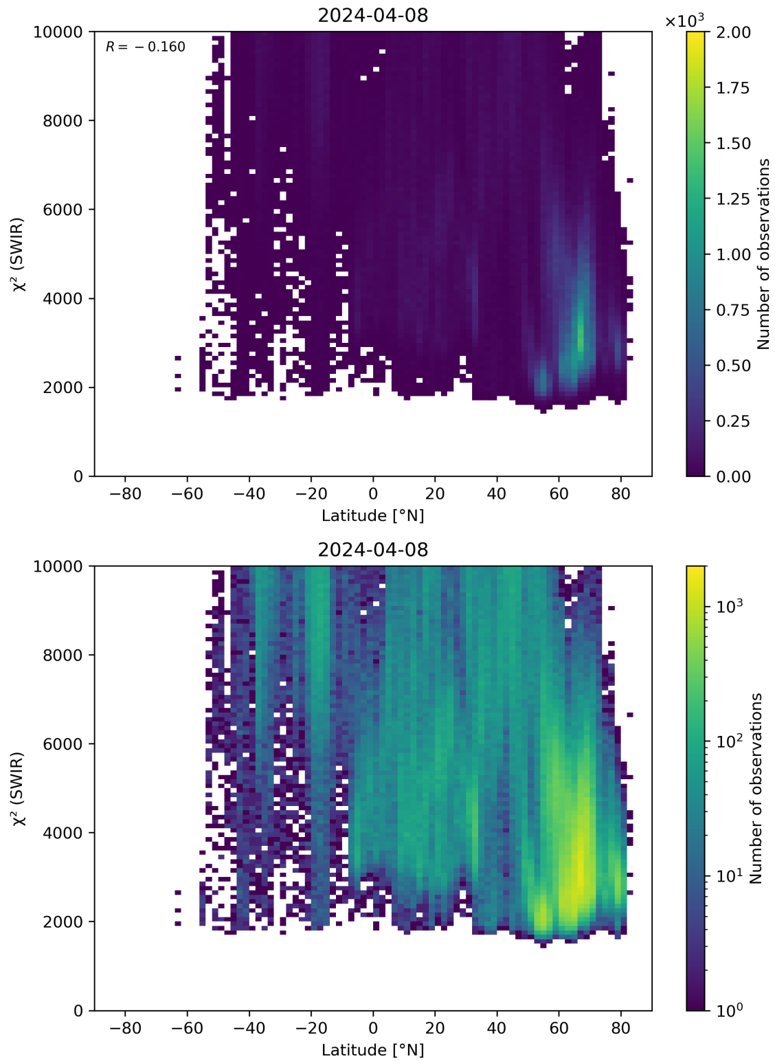
Figure 54: Scatter density plot of “Latitude” against “ \chi^2 (SWIR)” for 2024-04-07 to 2024-04-09.
