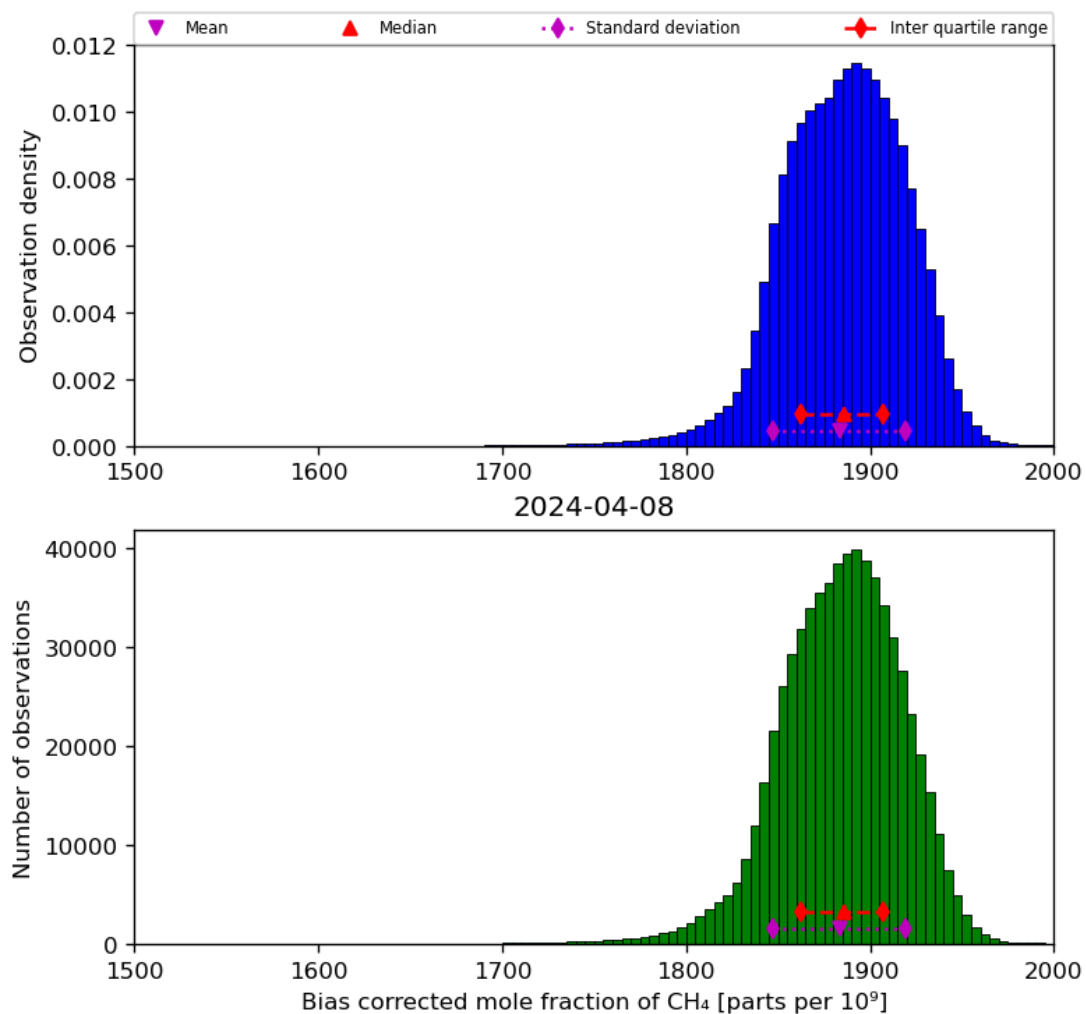
Figure 25: Histogram of “Bias corrected mole fraction of CH 4 ” for 2024-04-07 to 2024-04-09
