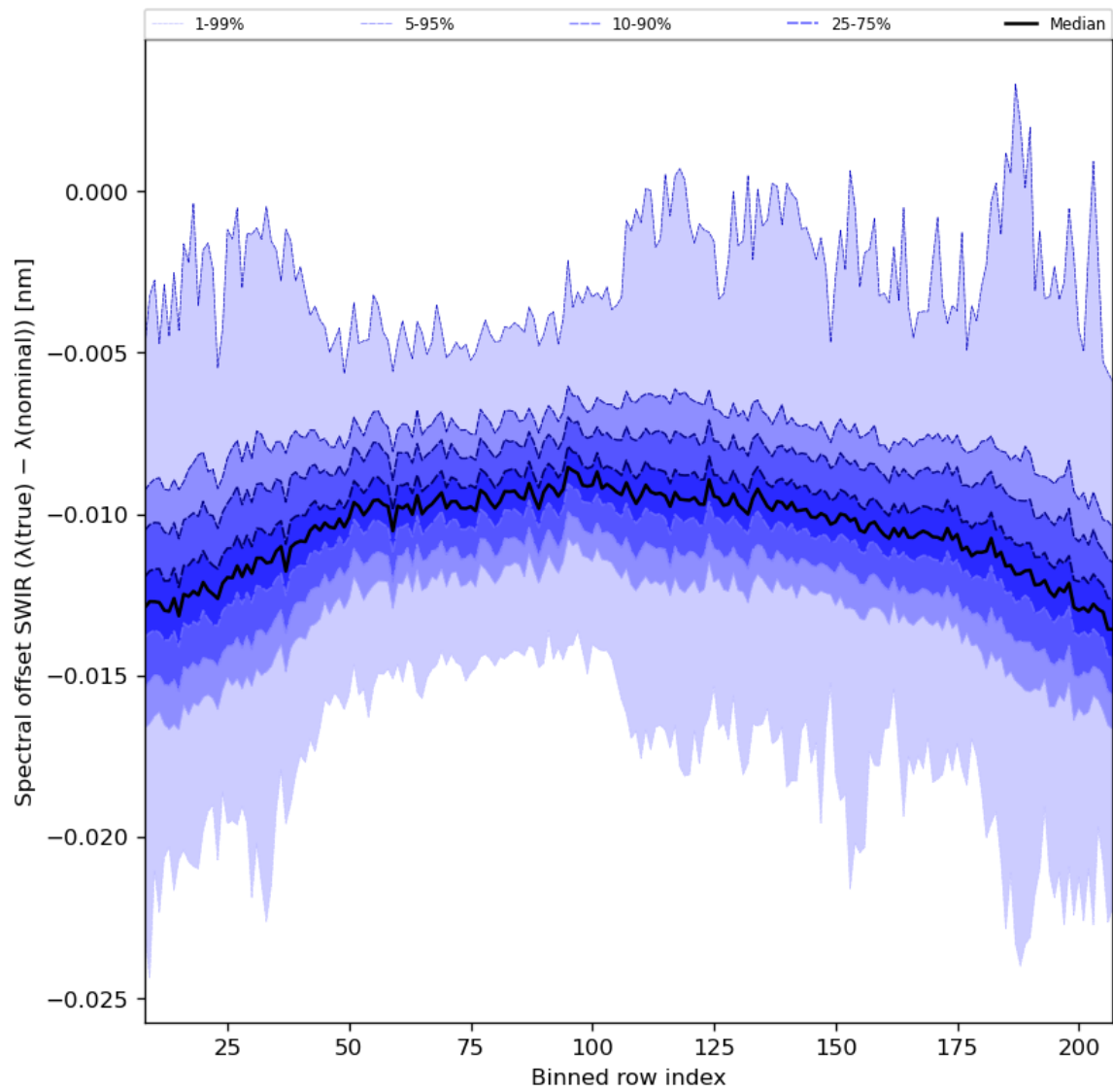
Figure 38: Along track statistics of “Spectral offset SWIR ( \lambda(\text{true}) - \lambda(\text{nominal}) )” for 2024-04-07 to 2024-04-09
