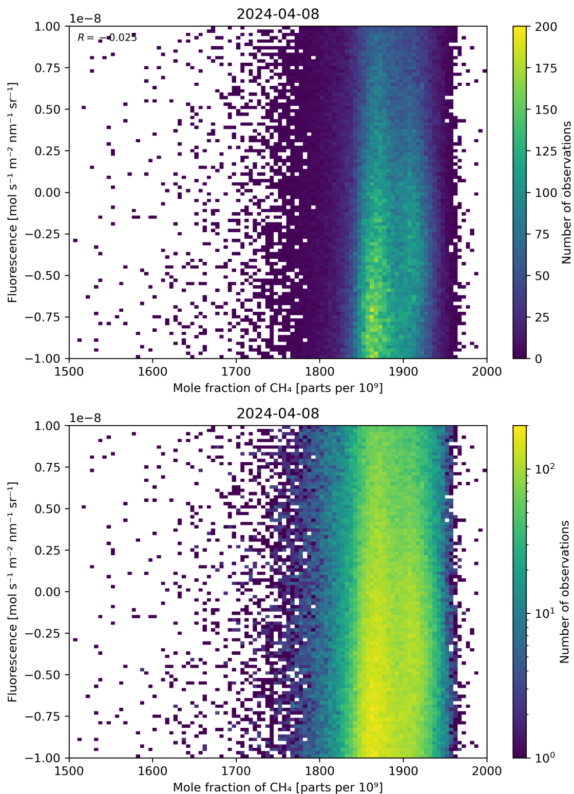
Figure 73: Scatter density plot of “Mole fraction of \text{CH}_4 ” against “Fluorescence” for 2024-04-07 to 2024-04-09.
