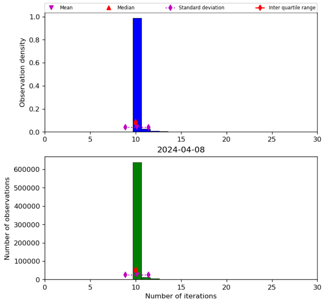
Figure 31: Histogram of “Number of iterations” for 2024-04-07 to 2024-04-09
