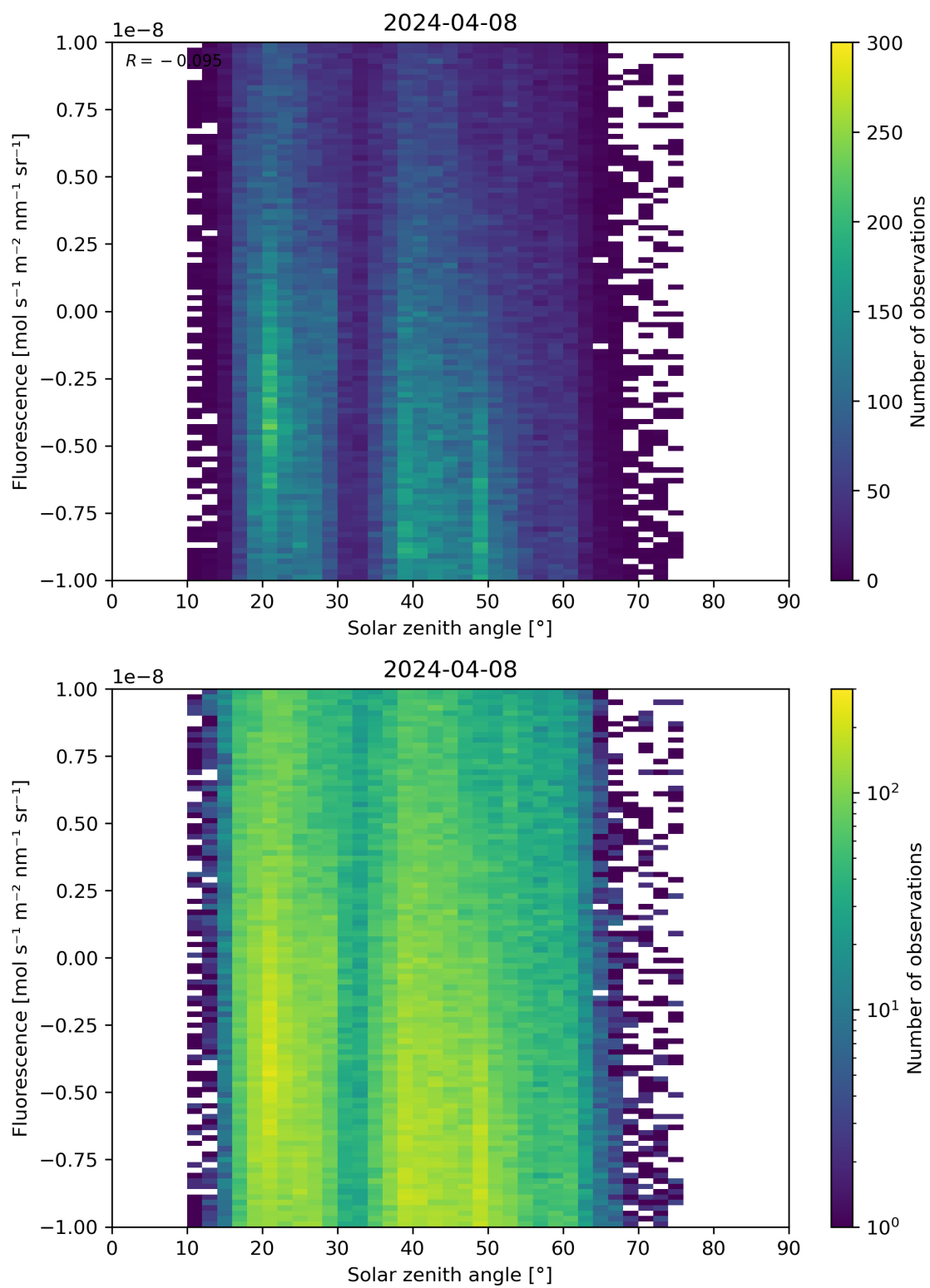
Figure 97: Scatter density plot of “Solar zenith angle” against “Fluorescence” for 2024-04-07 to 2024-04-09.
