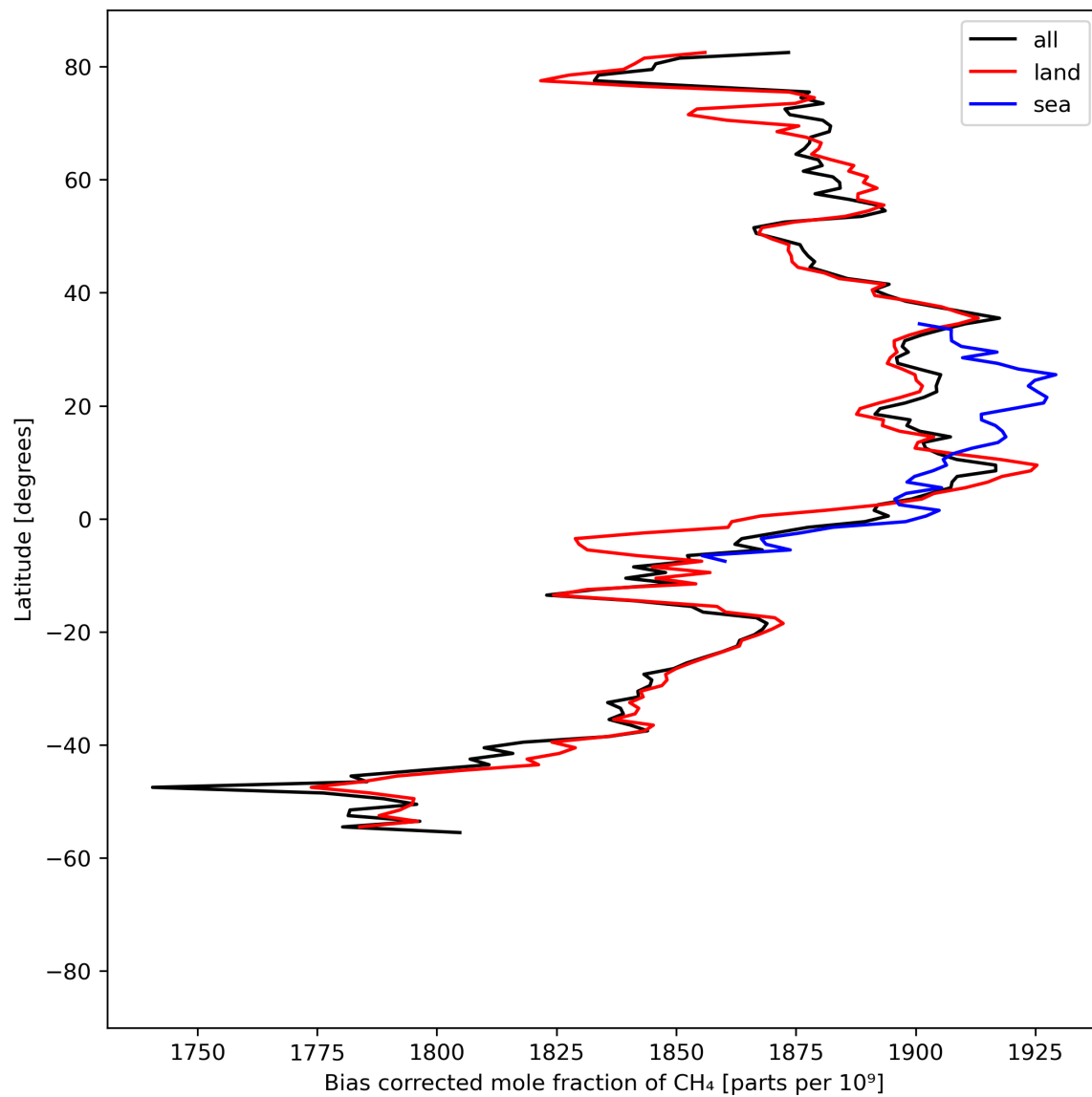
Figure 14: Zonal average of “Bias corrected mole fraction of CH 4 ” for 2024-04-07 to 2024-04-09.
