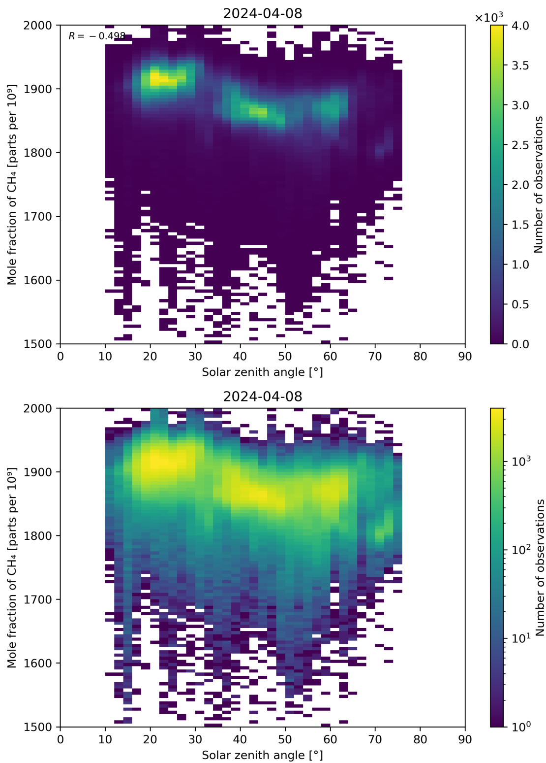
Figure 99: Scatter density plot of “Solar zenith angle” against “Mole fraction of CH 4 ” for 2024-04-07 to 2024-04-09.
