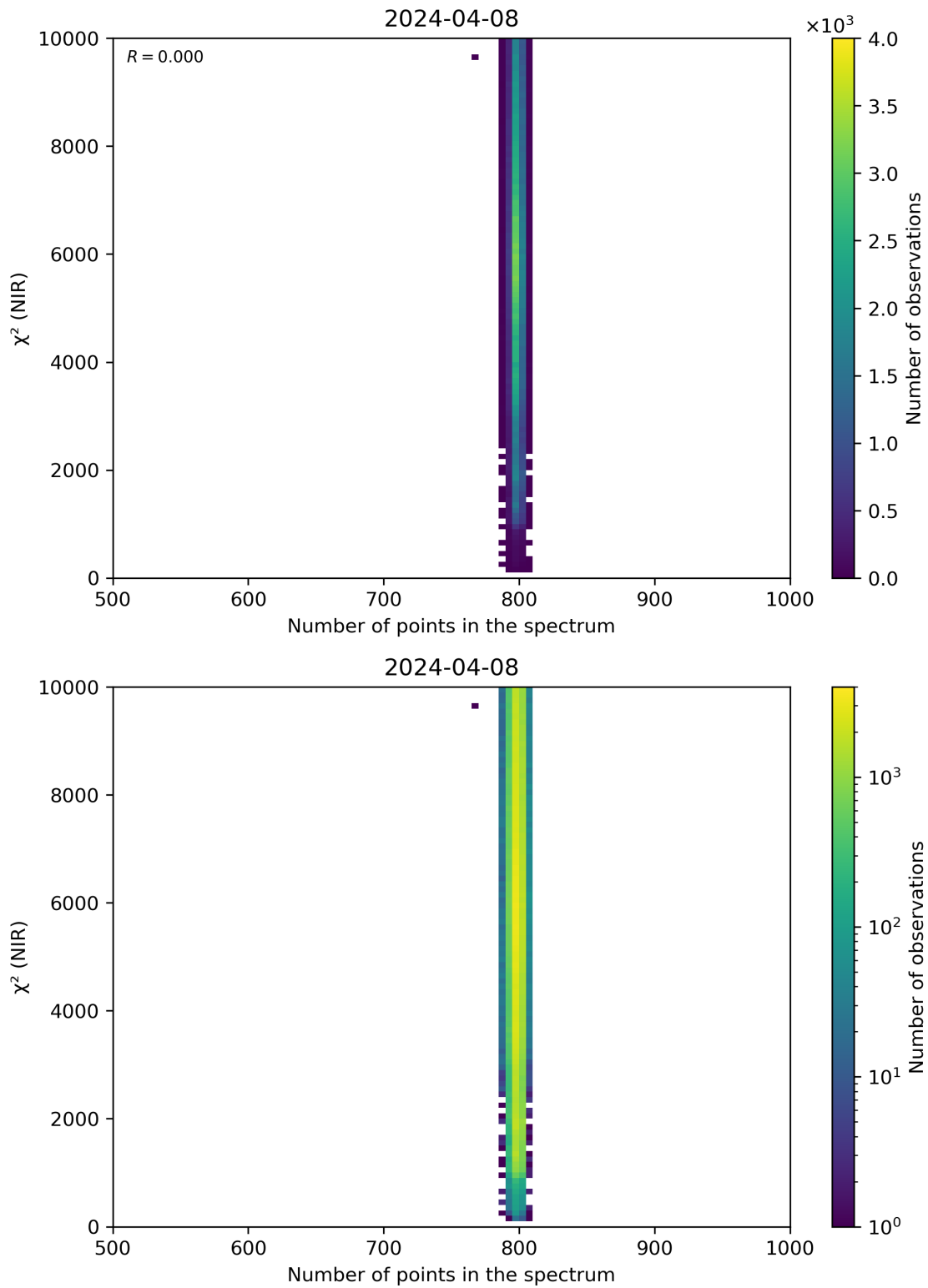
Figure 88: Scatter density plot of “Number of points in the spectrum” against “ \chi^2 (NIR)” for 2024-04-07 to 2024-04-09.
