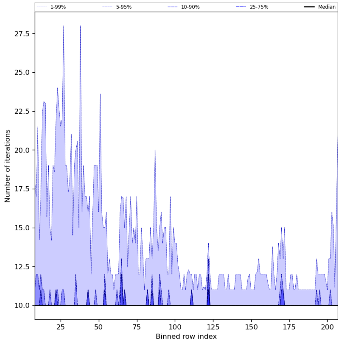
Figure 42: Along track statistics of “Number of iterations” for 2024-04-07 to 2024-04-09
