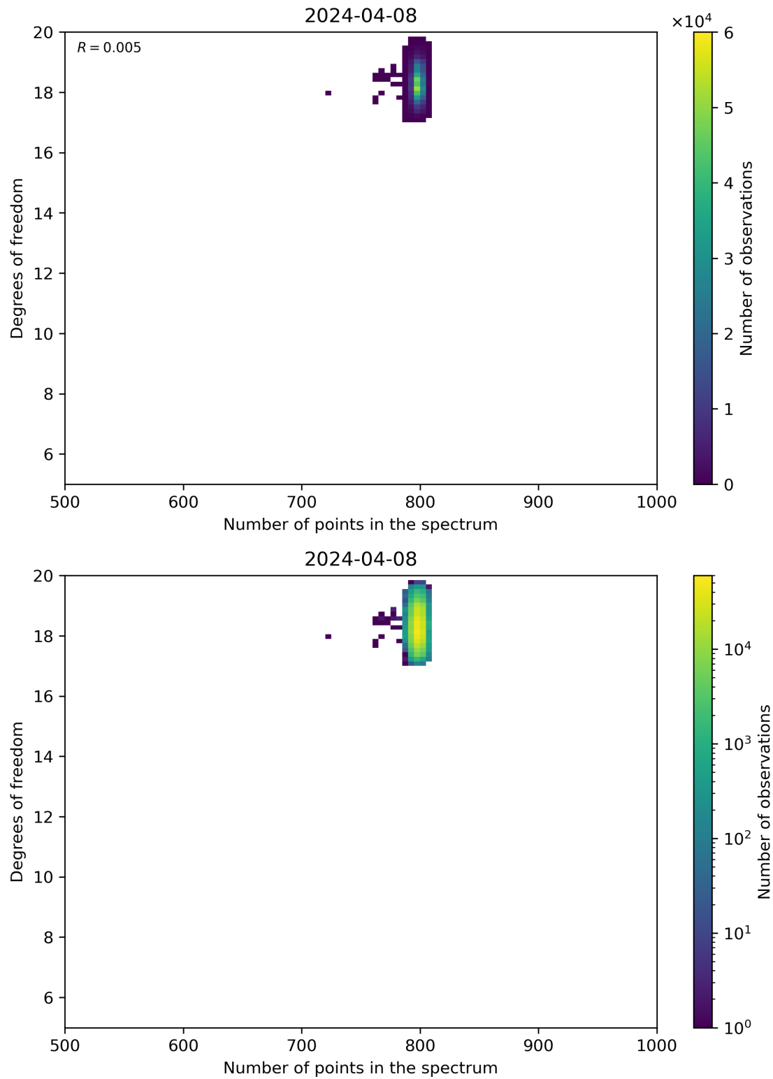
Figure 90: Scatter density plot of “Number of points in the spectrum” against “Degrees of freedom” for 2024-04-07 to 2024-04-09.
