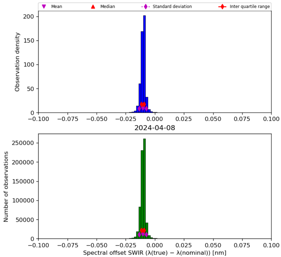
Figure 27: Histogram of “Spectral offset SWIR ( \lambda(\text{true}) - \lambda(\text{nominal}) )” for 2024-04-07 to 2024-04-09
