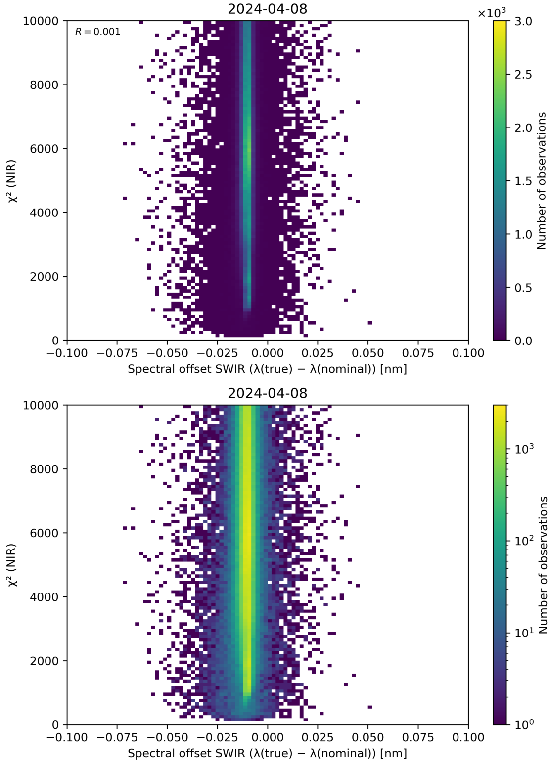
Figure 117: Scatter density plot of “Spectral offset SWIR ( \lambda(\text{true}) - \lambda(\text{nominal}) )” against “ \chi^2 (NIR)” for 2024-04-07 to 2024-04-09.
