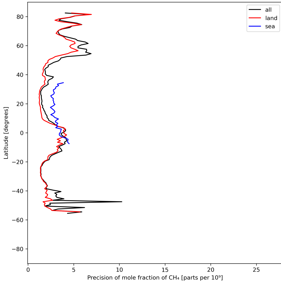
Figure 13: Zonal average of “Precision of mole fraction of CH 4 ” for 2024-04-07 to 2024-04-09.
