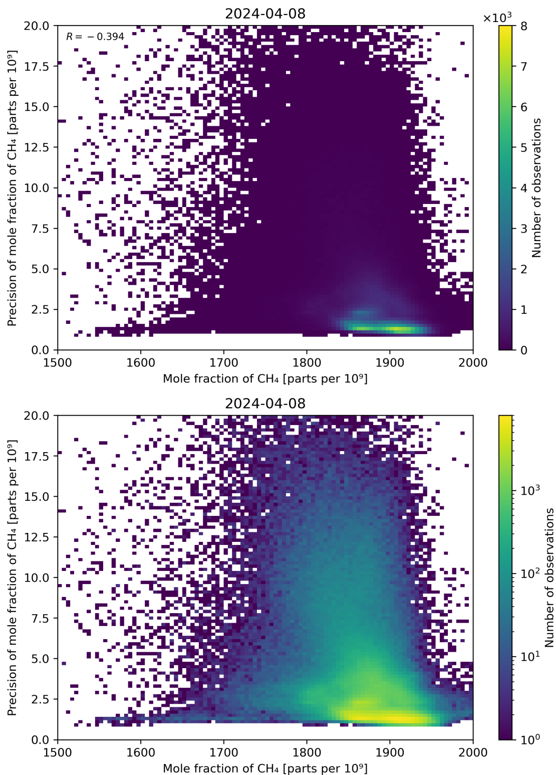
Figure 75: Scatter density plot of “Mole fraction of CH 4 ” against “Precision of mole fraction of CH 4 ” for 2024-04-07 to 2024-04-09.
