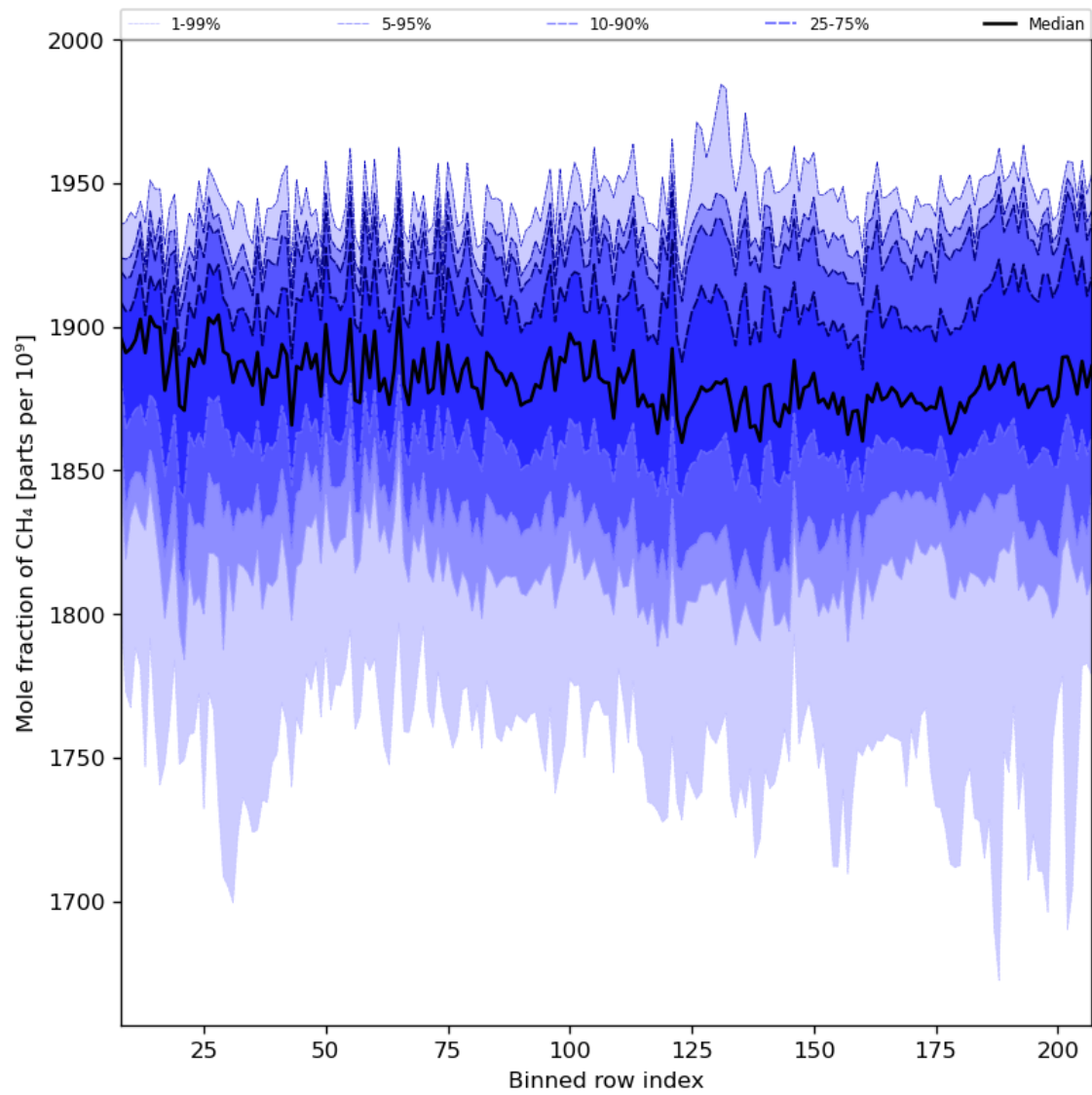
Figure 34: Along track statistics of “Mole fraction of CH 4 ” for 2024-04-07 to 2024-04-09
