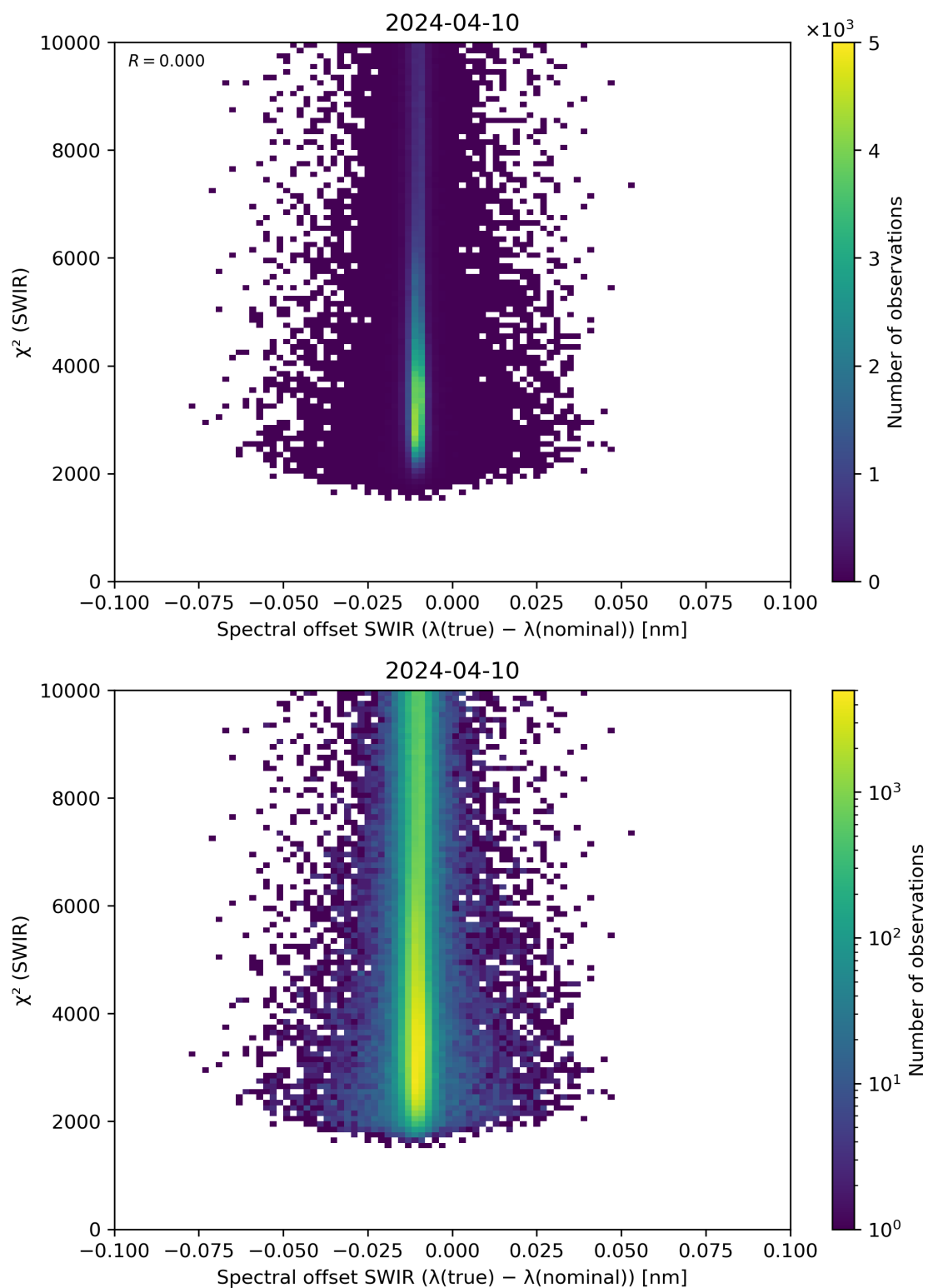
Figure 118: Scatter density plot of “Spectral offset SWIR ( \lambda(\text{true}) - \lambda(\text{nominal}) )” against “ \chi^2 (SWIR)” for 2024-04-10 to 2024-04-11.
