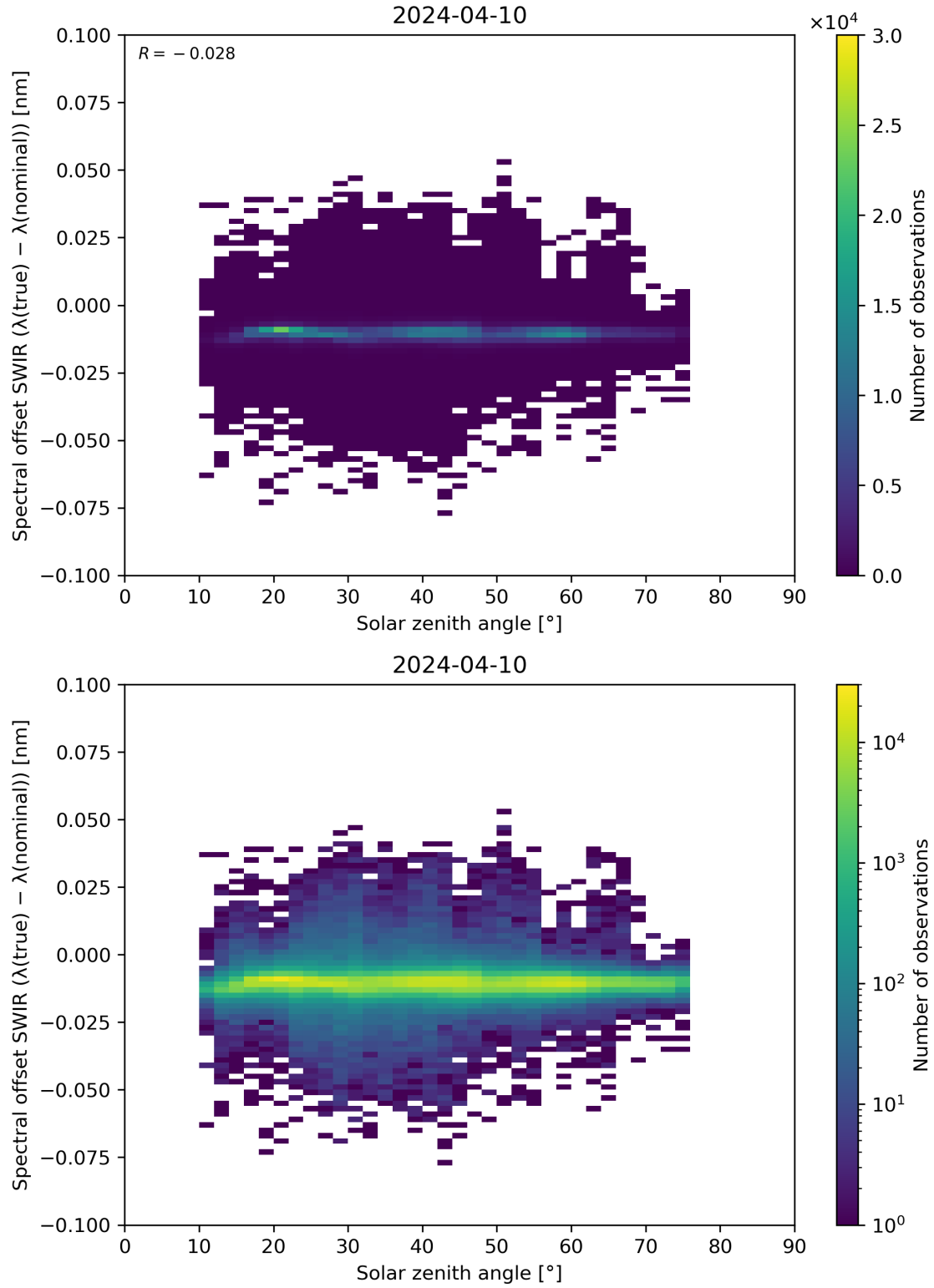
Figure 104: Scatter density plot of “Solar zenith angle” against “Spectral offset SWIR ( \lambda(\text{true}) - \lambda(\text{nominal}) )” for 2024-04-10 to 2024-04-11.
