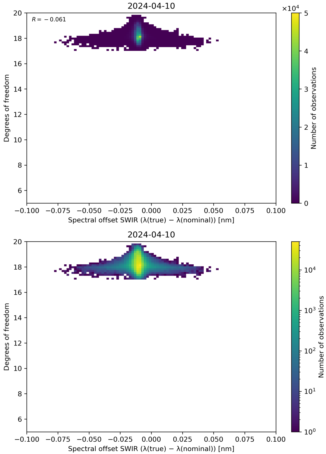
Figure 119: Scatter density plot of “Spectral offset SWIR ( \lambda(\text{true}) - \lambda(\text{nominal}) )” against “Degrees of freedom” for 2024-04-10 to 2024-04-11.
