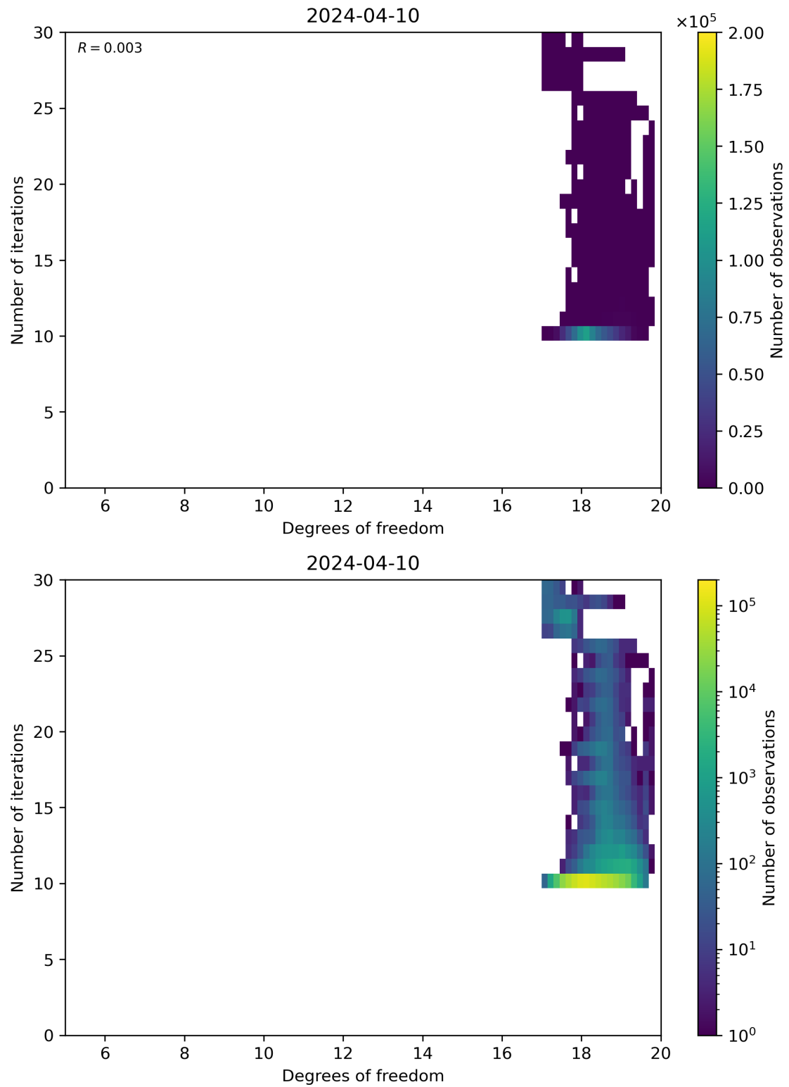
Figure 52: Scatter density plot of “Degrees of freedom” against “Number of iterations” for 2024-04-10 to 2024-04-11.
