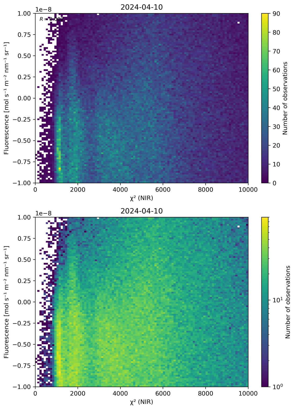
Figure 45: Scatter density plot of “ \chi^2 (NIR)” against “Fluorescence” for 2024-04-10 to 2024-04-11.
