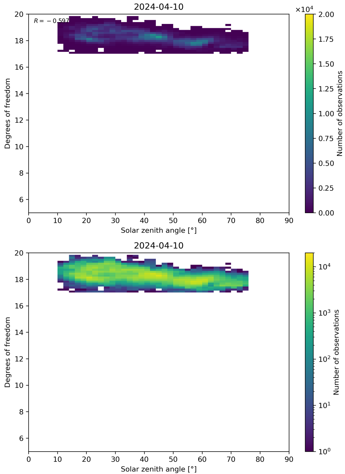
Figure 96: Scatter density plot of “Solar zenith angle” against “Degrees of freedom” for 2024-04-10 to 2024-04-11.
