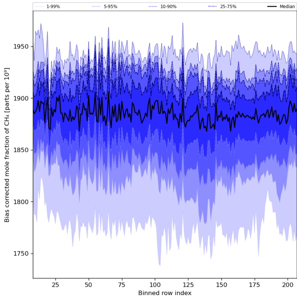
Figure 36: Along track statistics of “Bias corrected mole fraction of CH 4 ” for 2024-04-10 to 2024-04-11
