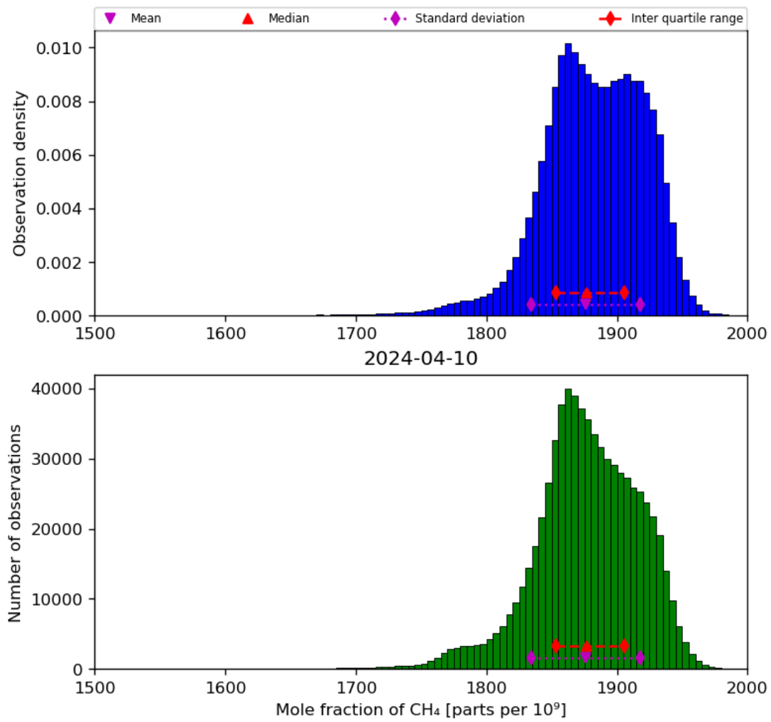
Figure 23: Histogram of “Mole fraction of CH 4 ” for 2024-04-10 to 2024-04-11
