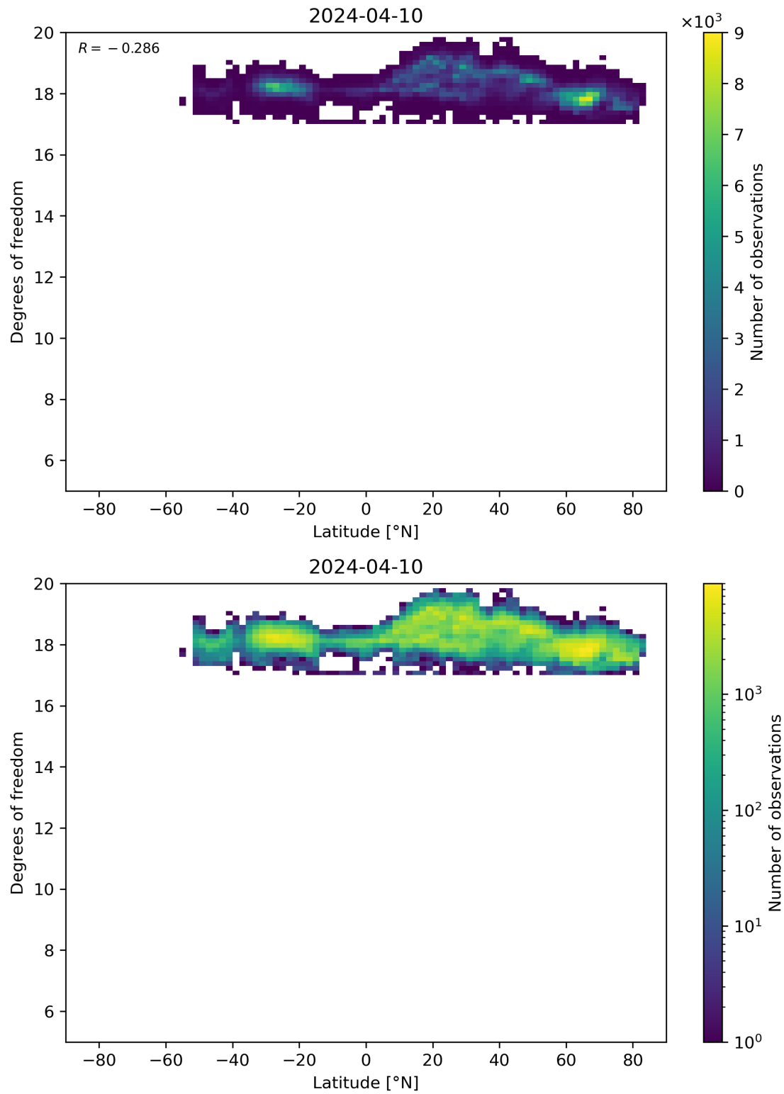
Figure 55: Scatter density plot of “Latitude” against “Degrees of freedom” for 2024-04-10 to 2024-04-11.
