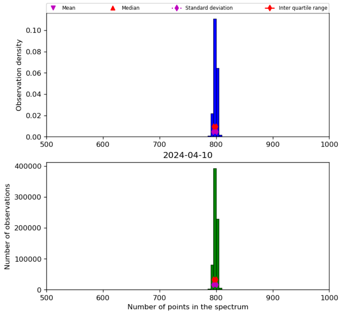
Figure 26: Histogram of “Number of points in the spectrum” for 2024-04-10 to 2024-04-11
