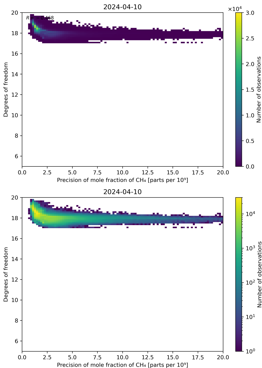
Figure 80: Scatter density plot of “Precision of mole fraction of CH 4 ” against “Degrees of freedom” for 2024-04-10 to 2024-04-11.
