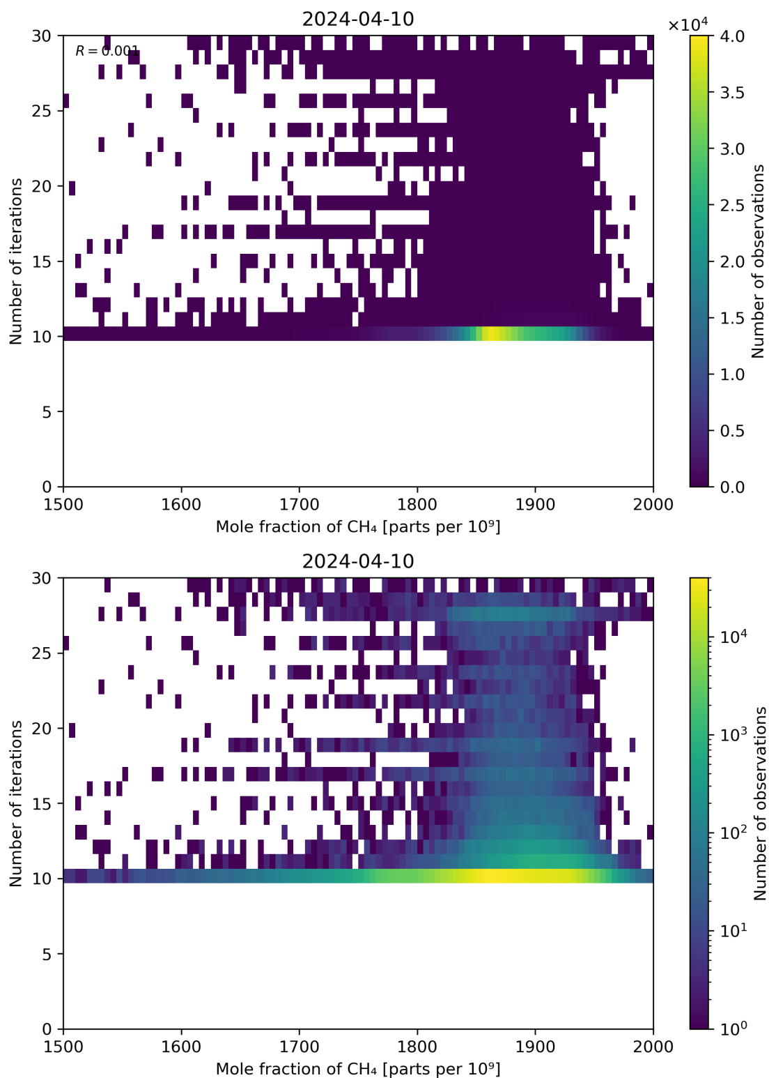
Figure 76: Scatter density plot of “Mole fraction of CH 4 ” against “Number of iterations” for 2024-04-10 to 2024-04-11.
