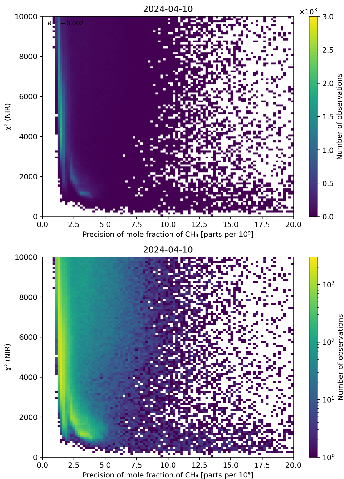
Figure 78: Scatter density plot of “Precision of mole fraction of \text{CH}_4 ” against “ \chi^2 (NIR)” for 2024-04-10 to 2024-04-11.
