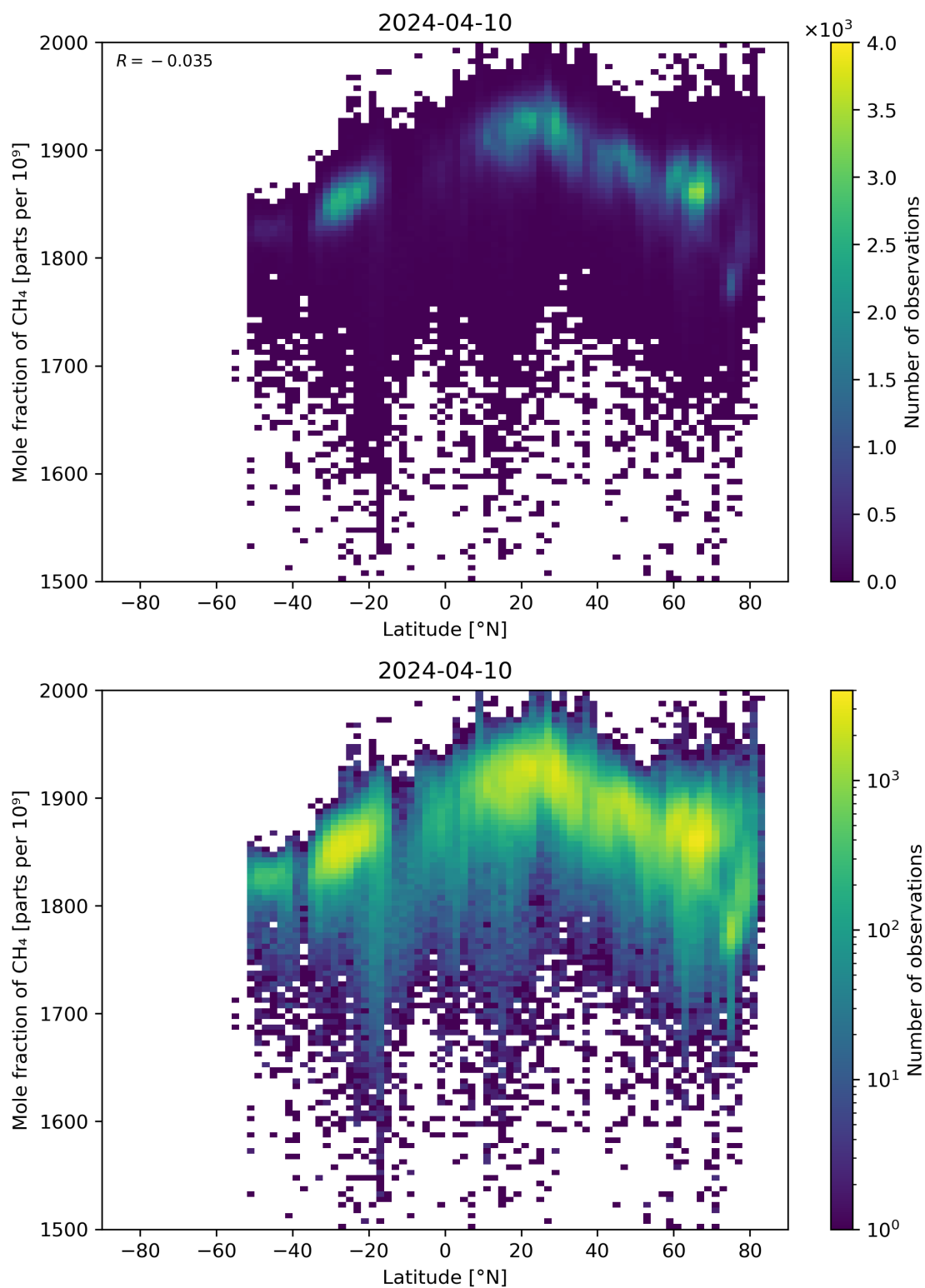
Figure 57: Scatter density plot of “Latitude” against “Mole fraction of CH 4 ” for 2024-04-10 to 2024-04-11.
