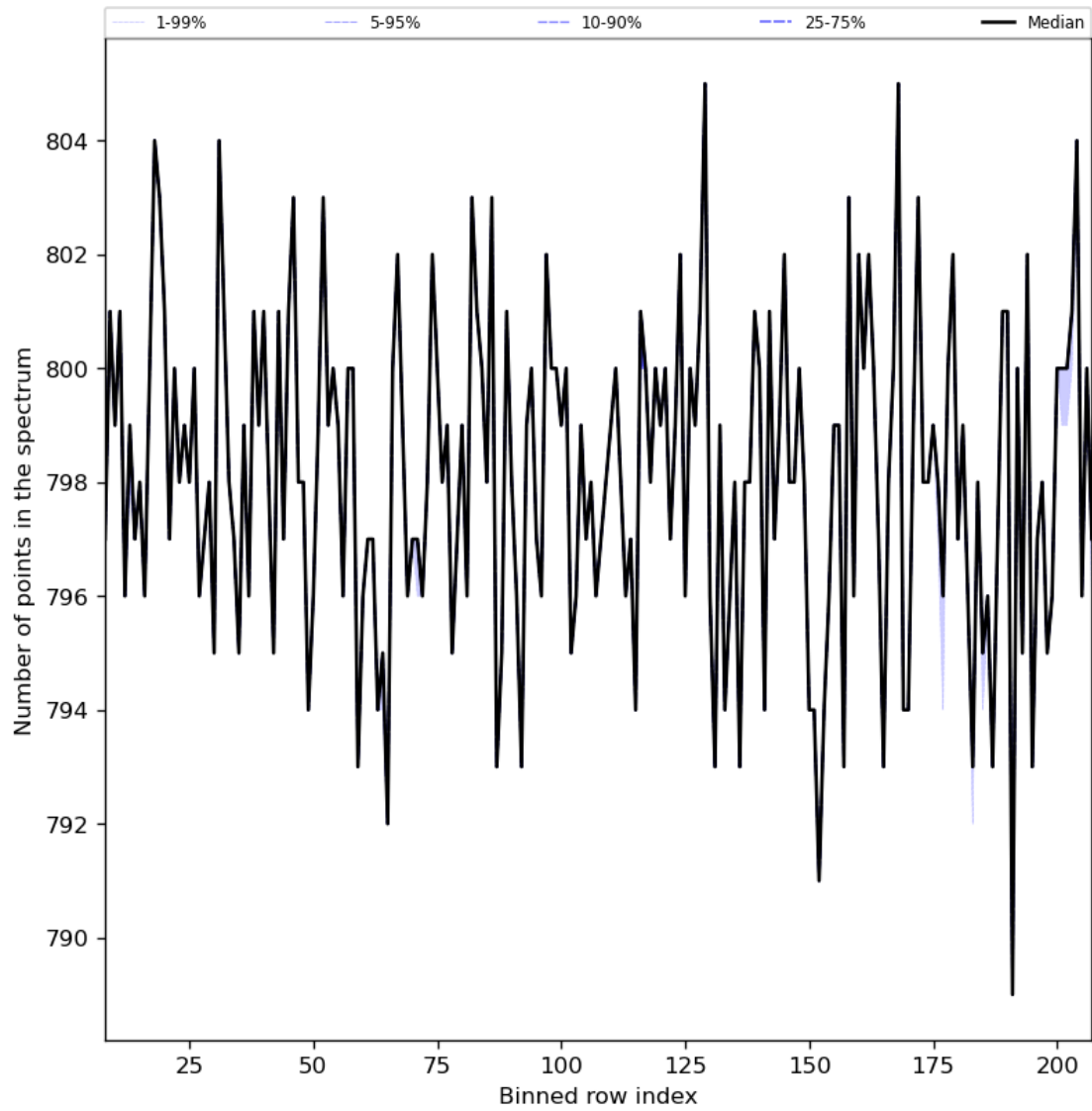
Figure 37: Along track statistics of “Number of points in the spectrum” for 2024-04-10 to 2024-04-11
