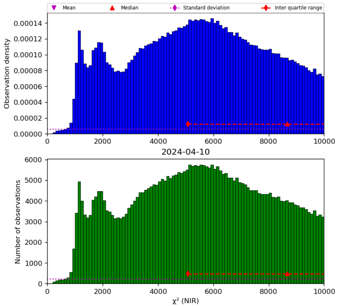
Figure 29: Histogram of “ \chi^2 (NIR)” for 2024-04-10 to 2024-04-11
