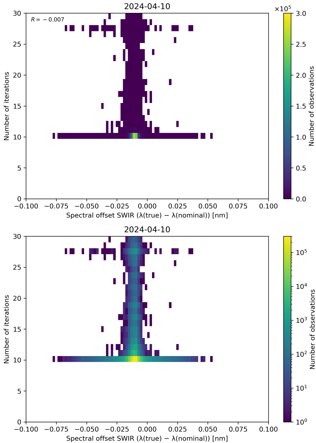
Figure 121: Scatter density plot of “Spectral offset SWIR ( \lambda(\text{true}) - \lambda(\text{nominal}) )” against “Number of iterations” for 2024-04-10 to 2024-04-11.
