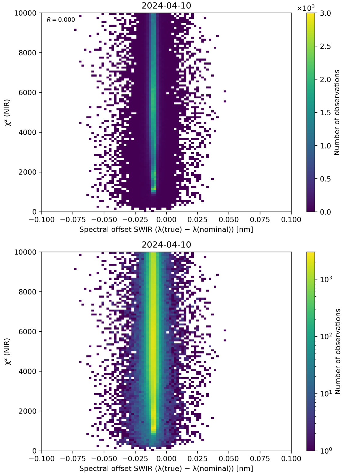
Figure 117: Scatter density plot of “Spectral offset SWIR ( \lambda(\text{true}) - \lambda(\text{nominal}) )” against “ \chi^2 (NIR)” for 2024-04-10 to 2024-04-11.
