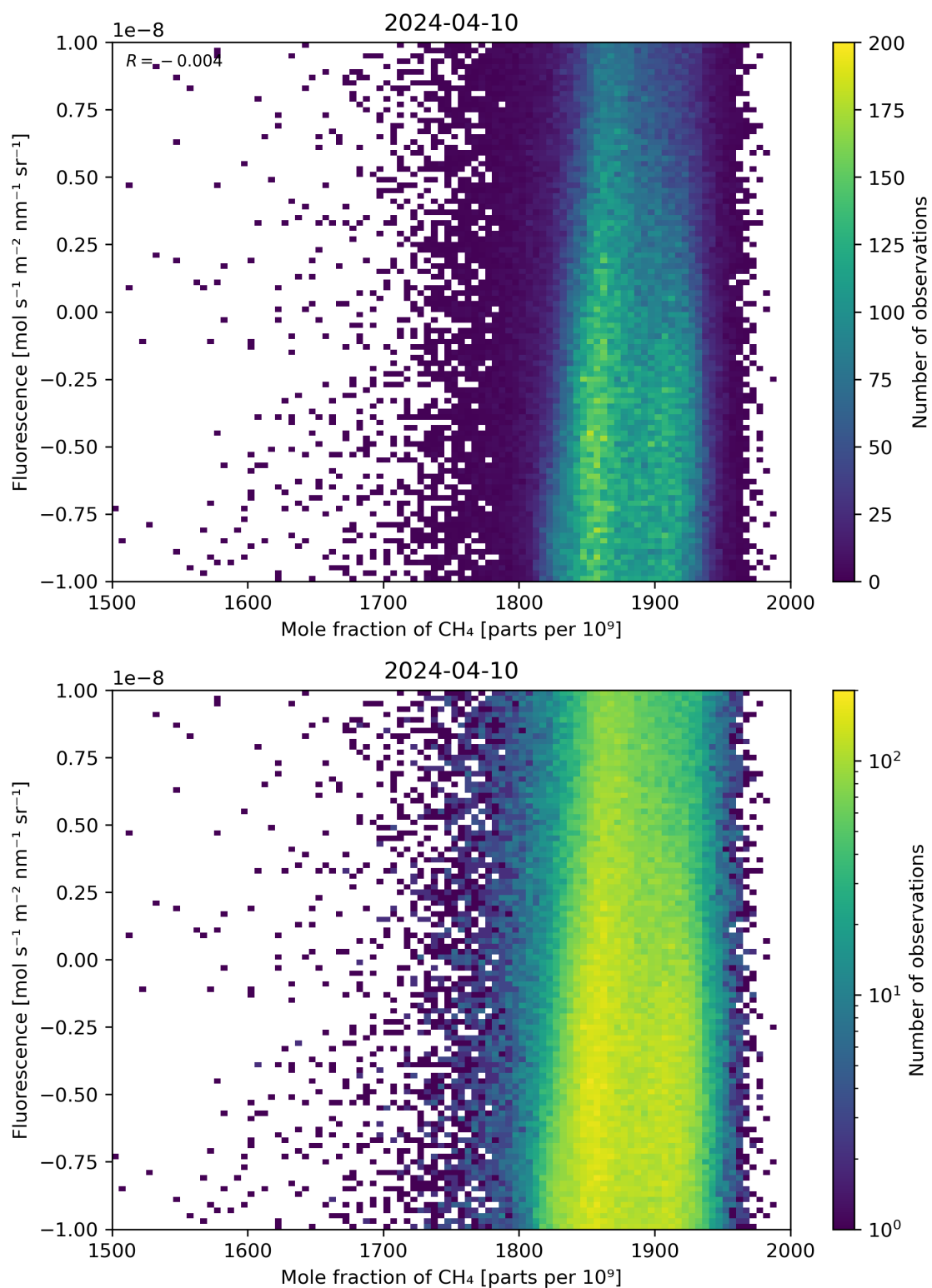
Figure 73: Scatter density plot of “Mole fraction of \text{CH}_4 ” against “Fluorescence” for 2024-04-10 to 2024-04-11.
