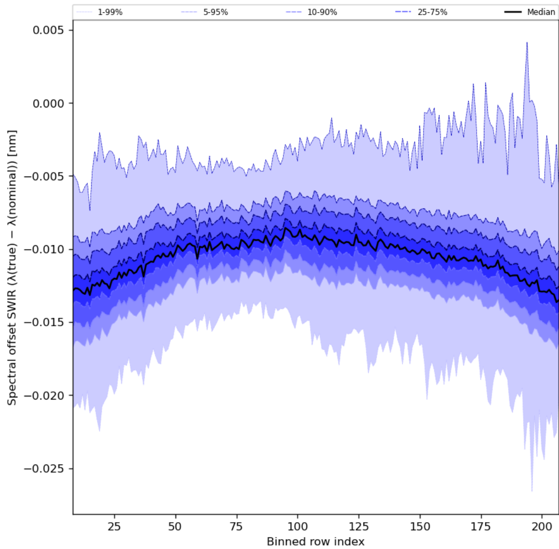
Figure 38: Along track statistics of “Spectral offset SWIR ( \lambda(\text{true}) - \lambda(\text{nominal}) )” for 2024-04-10 to 2024-04-11
