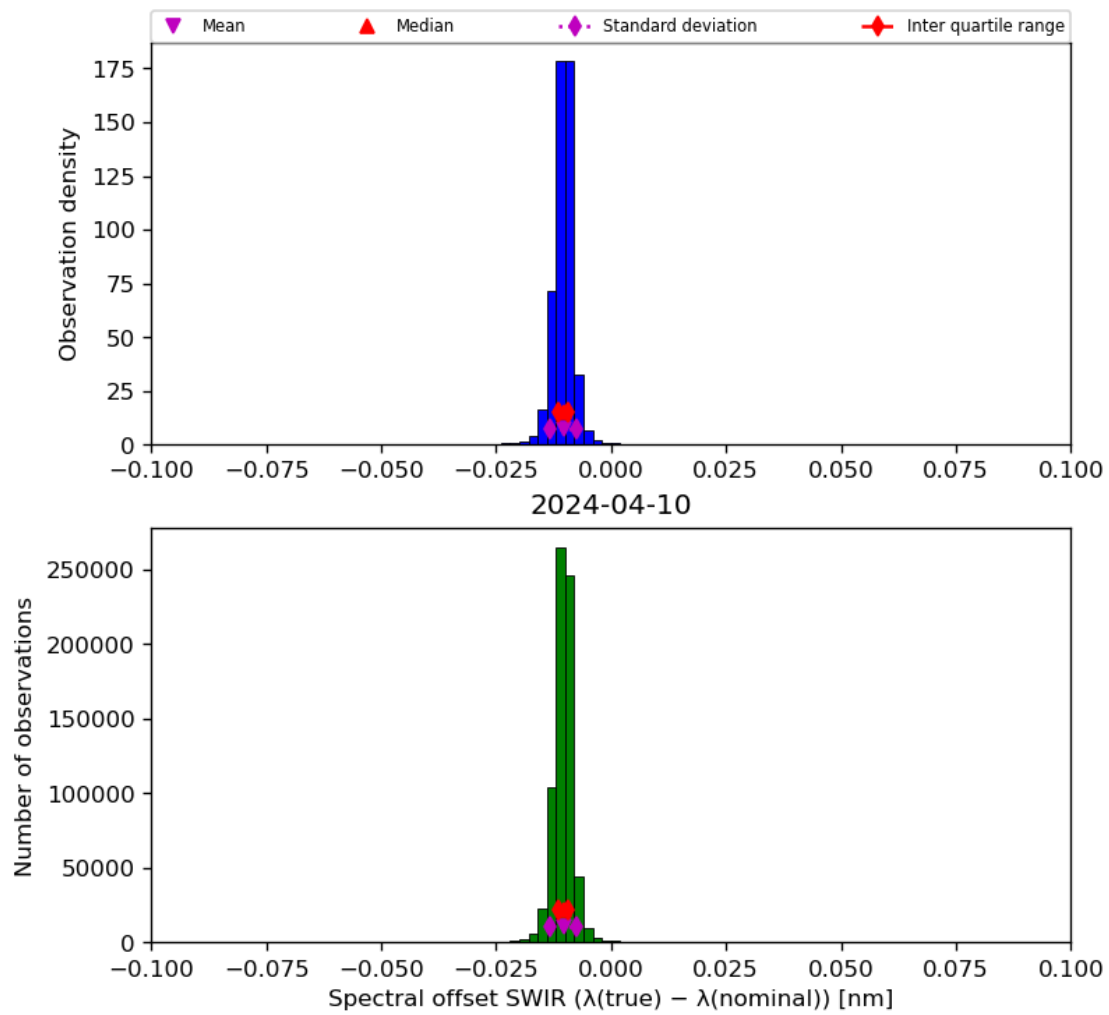
Figure 27: Histogram of “Spectral offset SWIR ( \lambda(\text{true}) - \lambda(\text{nominal}) )” for 2024-04-10 to 2024-04-11
