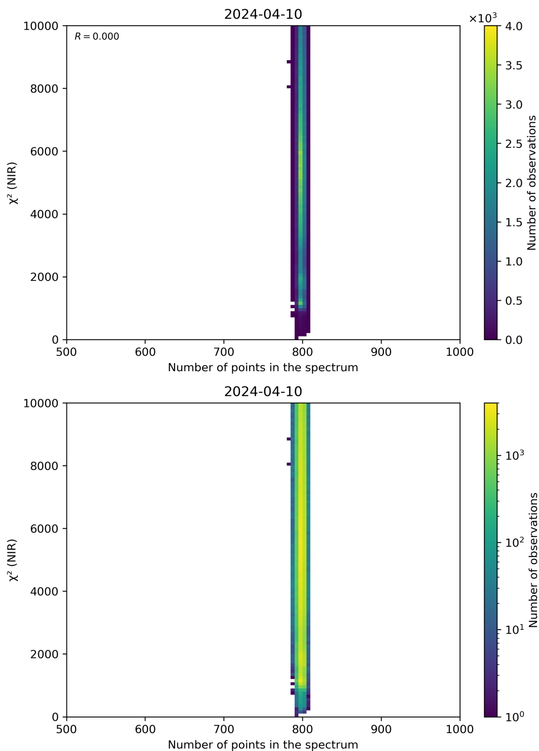
Figure 88: Scatter density plot of “Number of points in the spectrum” against “ \chi^2 (NIR)” for 2024-04-10 to 2024-04-11.
