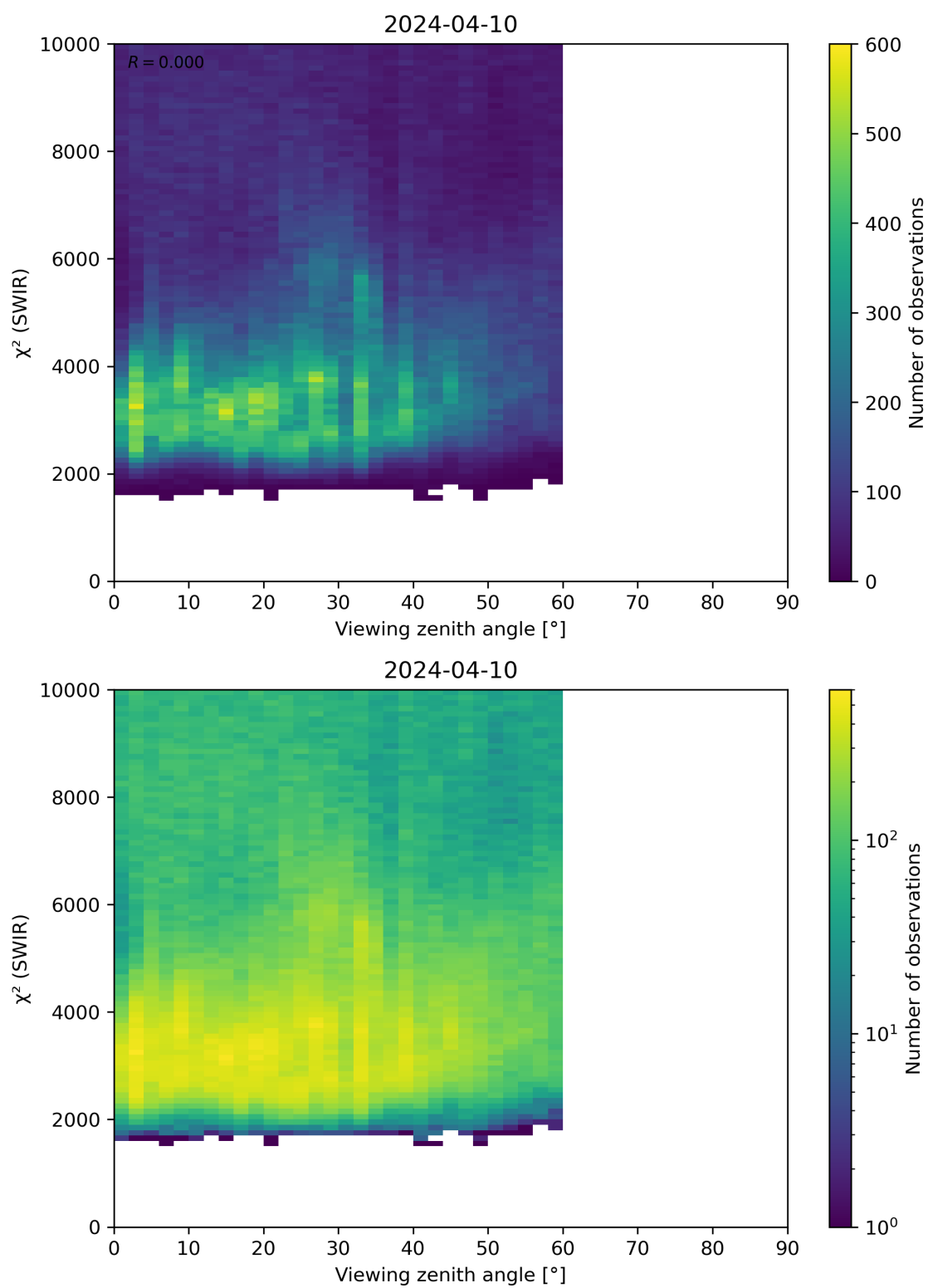
Figure 106: Scatter density plot of “Viewing zenith angle” against “ \chi^2 (SWIR)” for 2024-04-10 to 2024-04-11.
