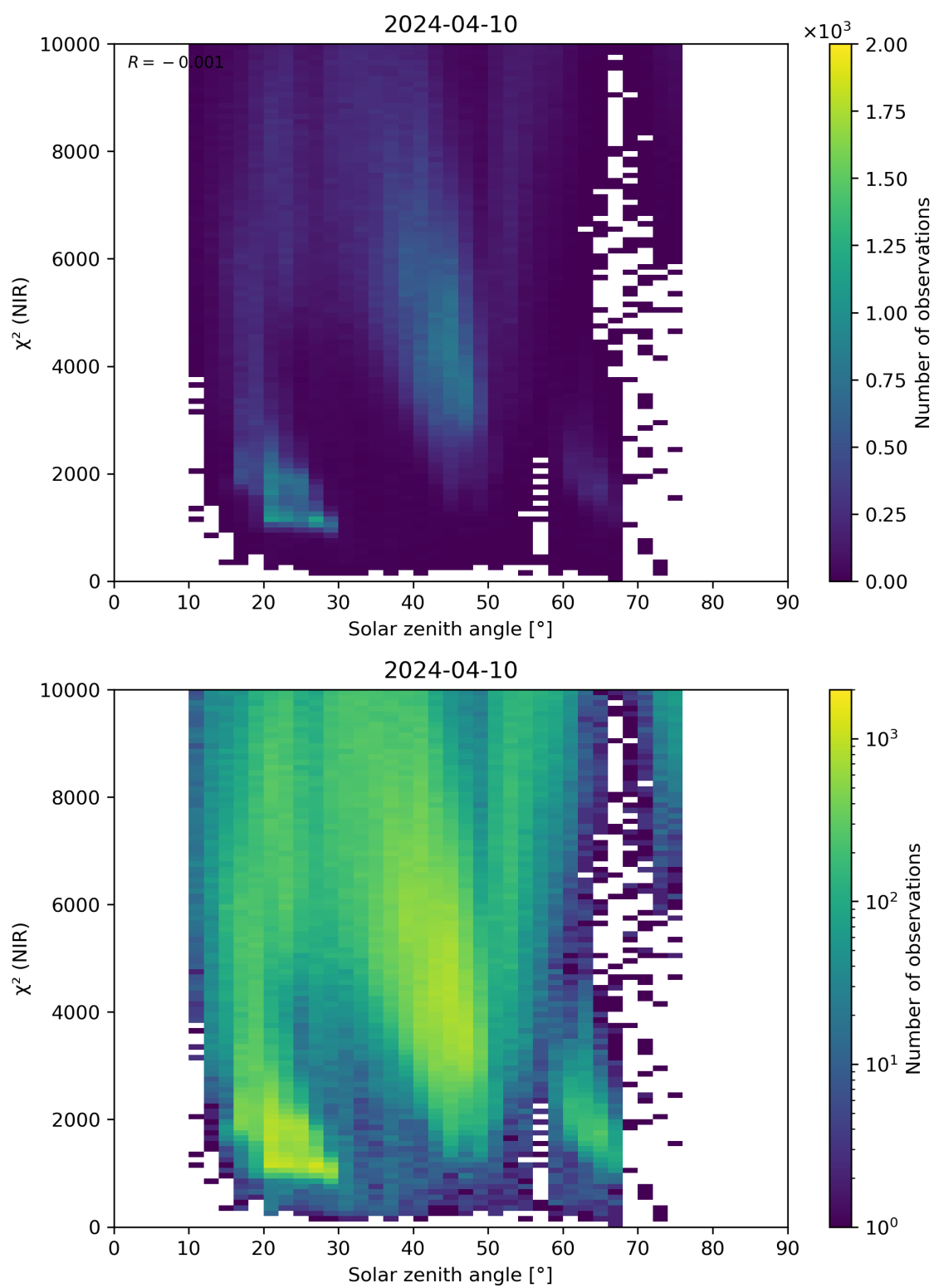
Figure 94: Scatter density plot of “Solar zenith angle” against “ \chi^2 (NIR)” for 2024-04-10 to 2024-04-11.
