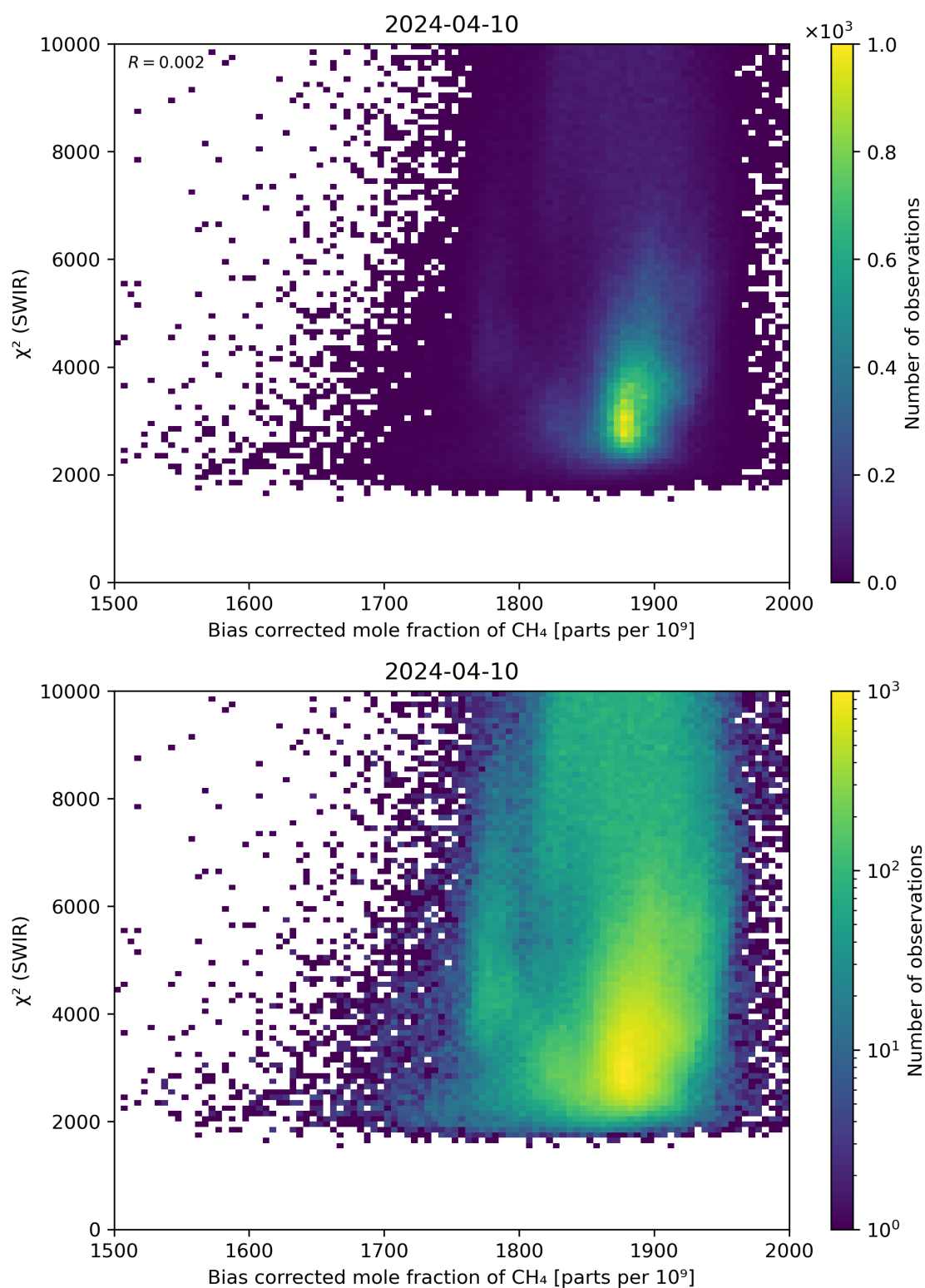
Figure 64: Scatter density plot of “Bias corrected mole fraction of CH 4 ” against “ \chi^2 (SWIR)” for 2024-04-10 to 2024-04-11.
