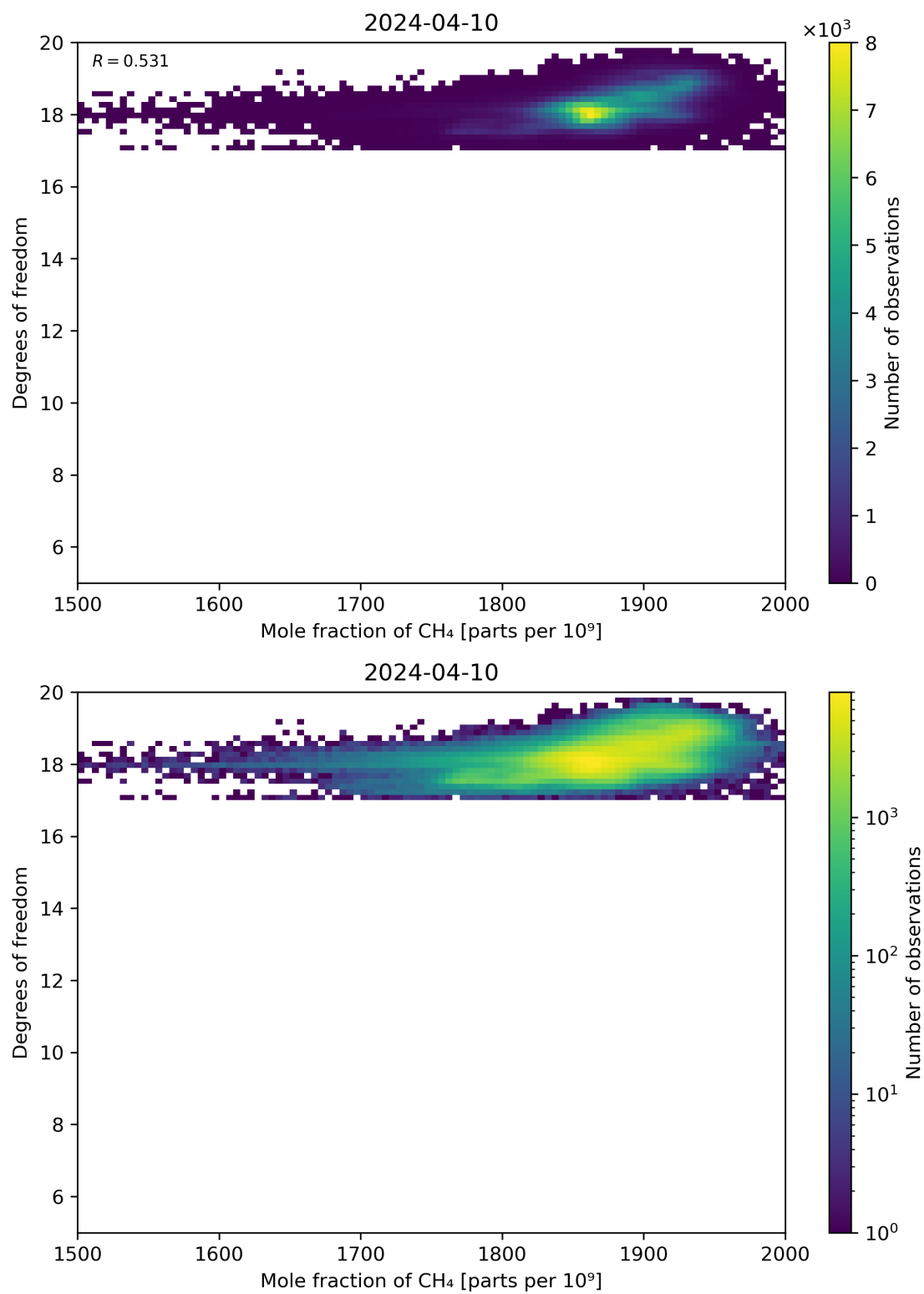
Figure 72: Scatter density plot of “Mole fraction of CH 4 ” against “Degrees of freedom” for 2024-04-10 to 2024-04-11.
