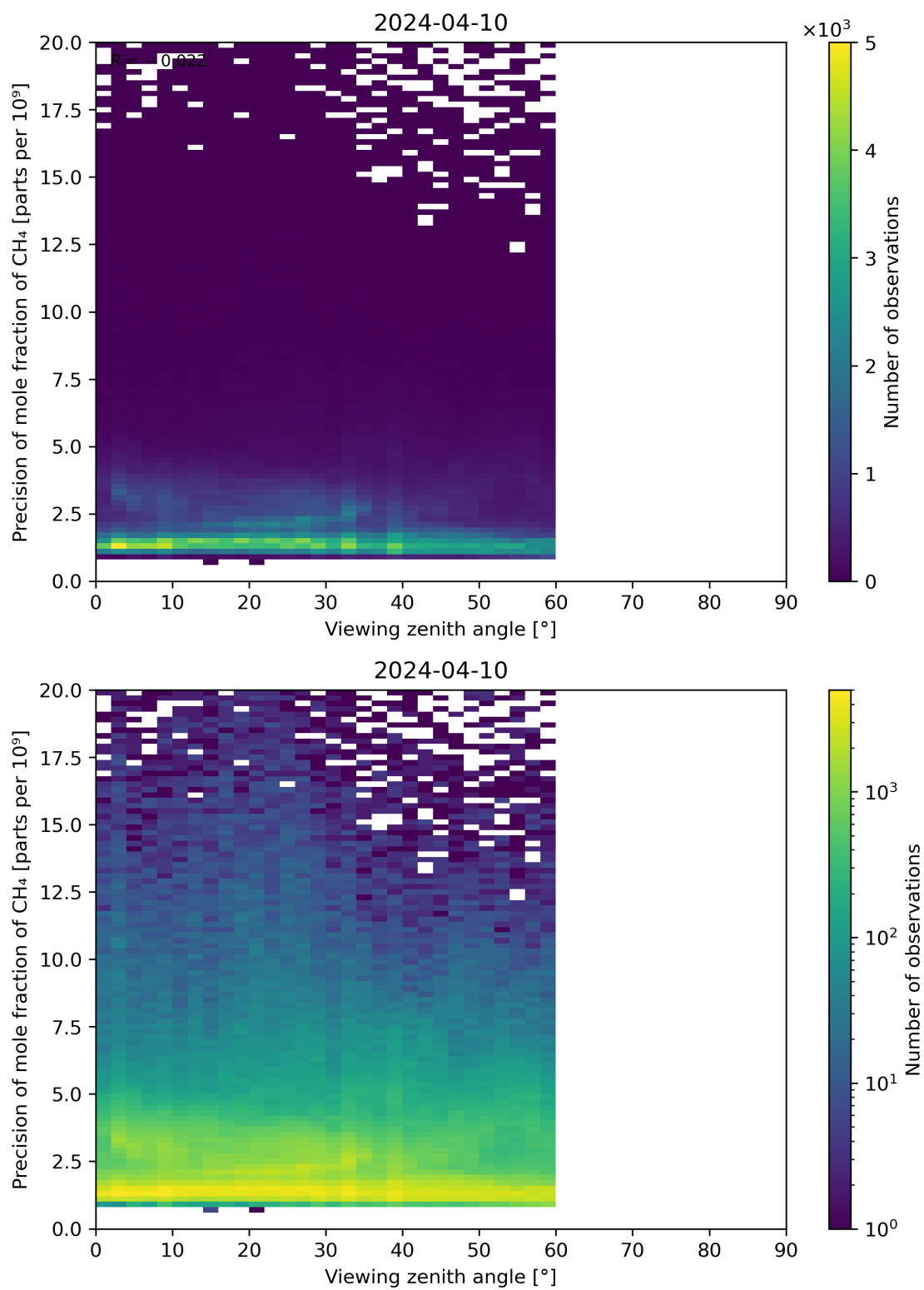
Figure 112: Scatter density plot of “Viewing zenith angle” against “Precision of mole fraction of CH 4 ” for 2024-04-10 to 2024-04-11.
