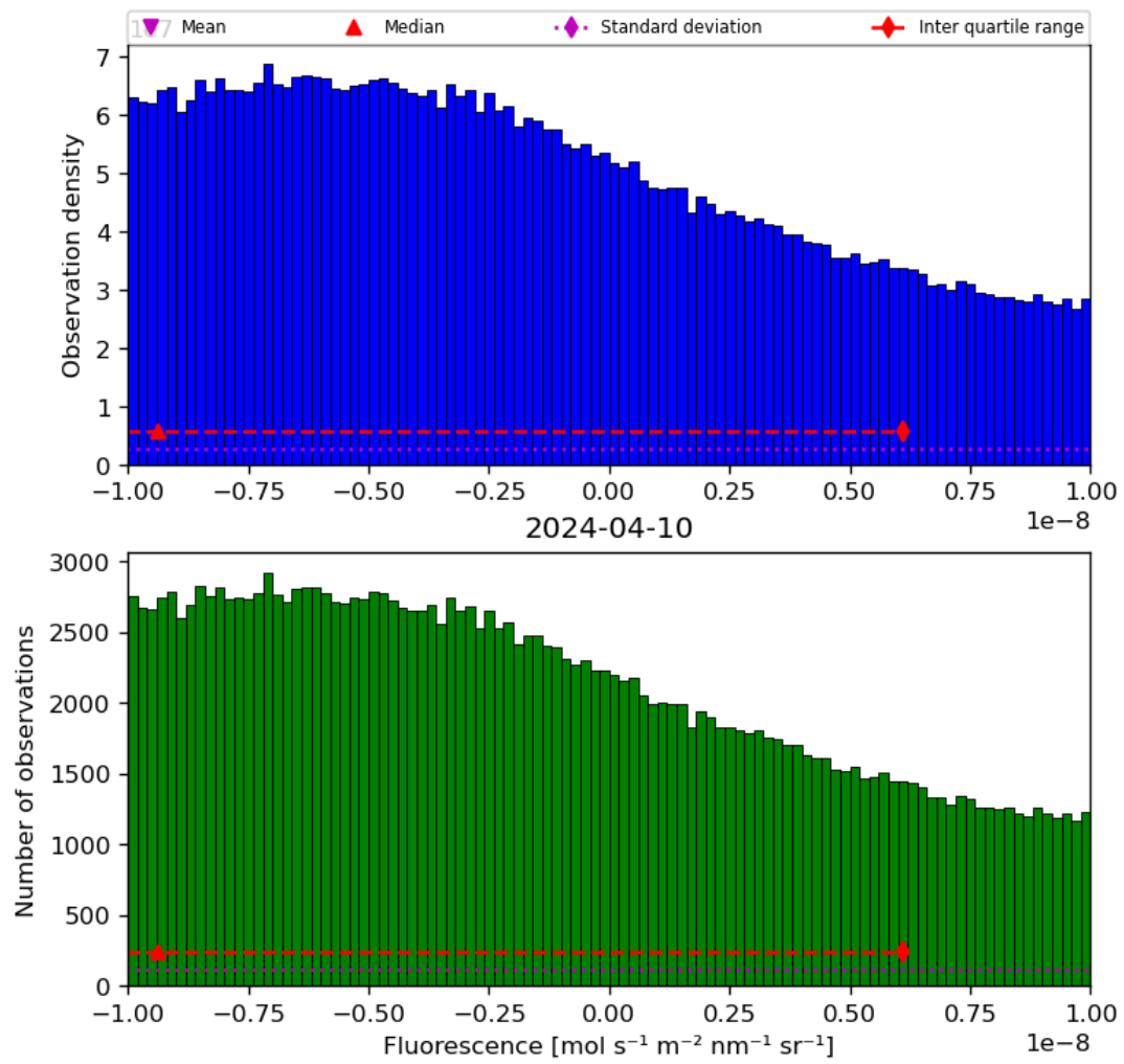
Figure 32: Histogram of “Fluorescence” for 2024-04-10 to 2024-04-11
