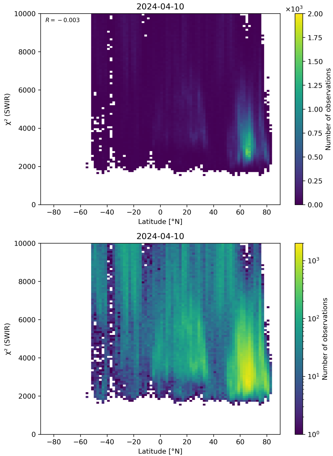
Figure 54: Scatter density plot of “Latitude” against “ \chi^2 (SWIR)” for 2024-04-10 to 2024-04-11.
