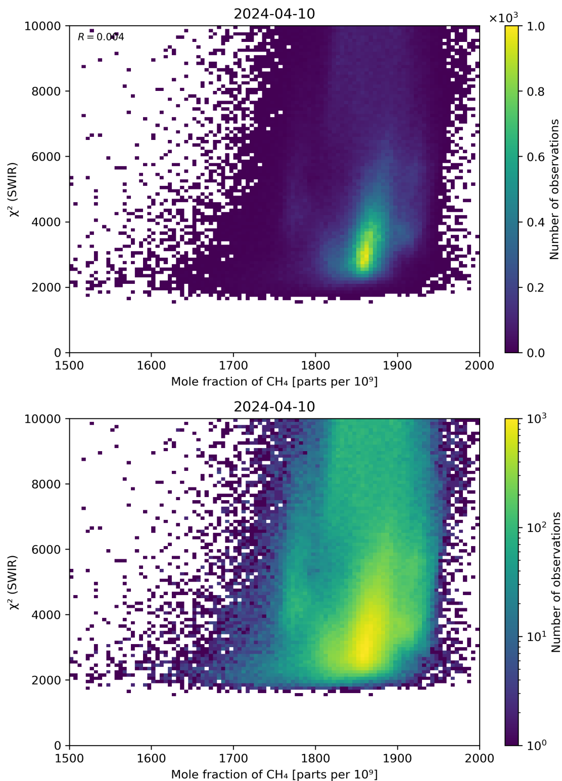
Figure 71: Scatter density plot of “Mole fraction of \text{CH}_4 ” against “ \chi^2 (SWIR)” for 2024-04-10 to 2024-04-11.
