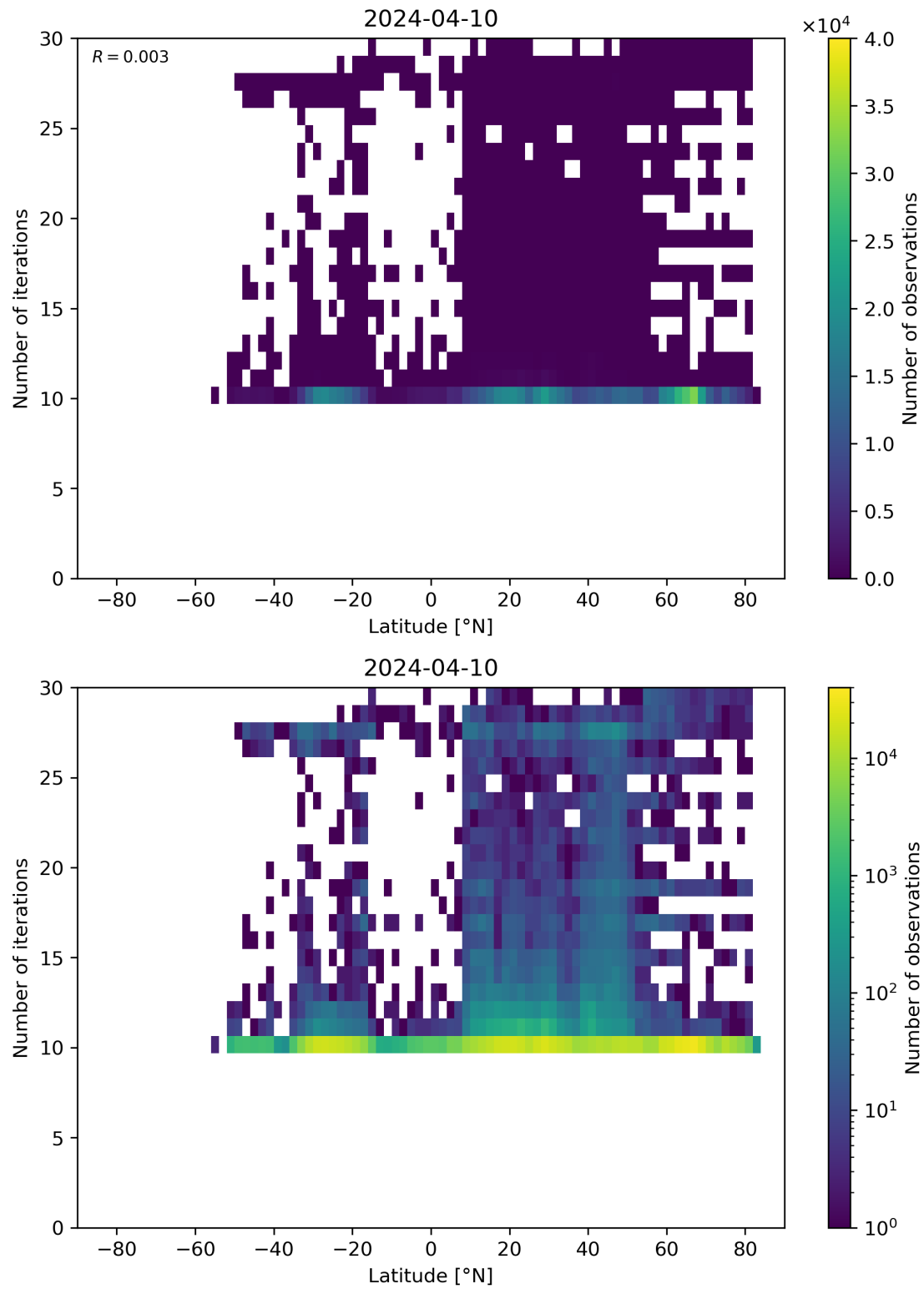
Figure 60: Scatter density plot of “Latitude” against “Number of iterations” for 2024-04-10 to 2024-04-11.
