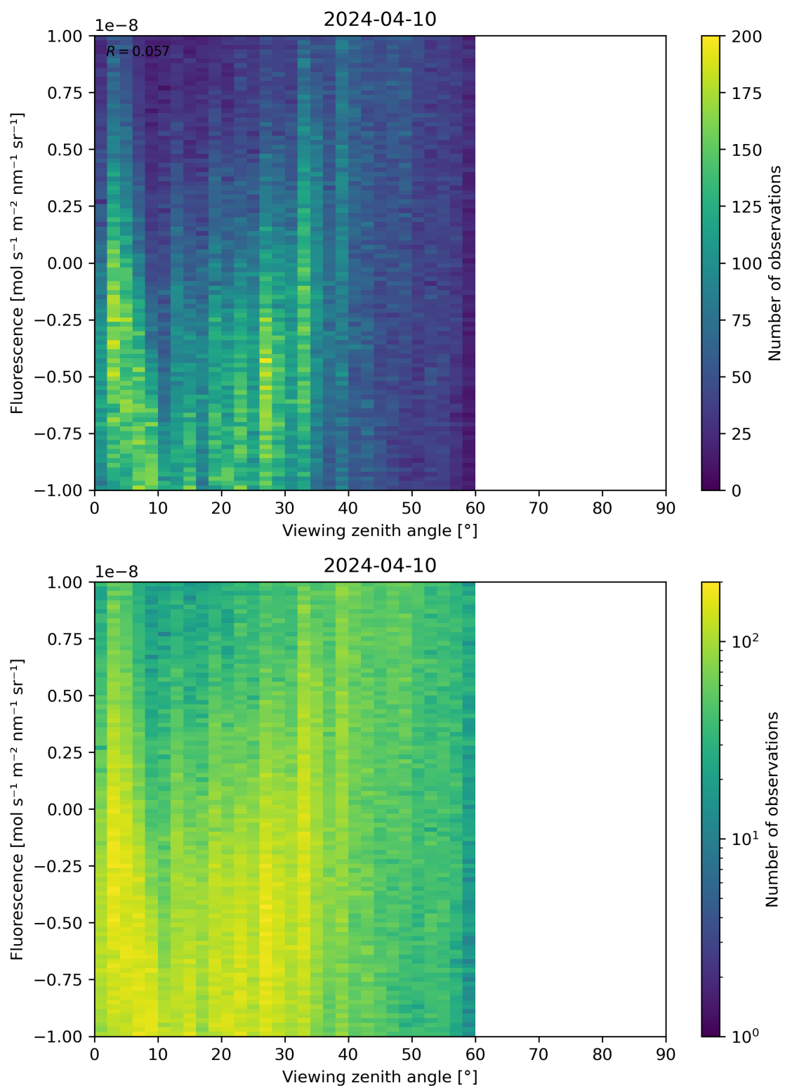
Figure 108: Scatter density plot of “Viewing zenith angle” against “Fluorescence” for 2024-04-10 to 2024-04-11.
