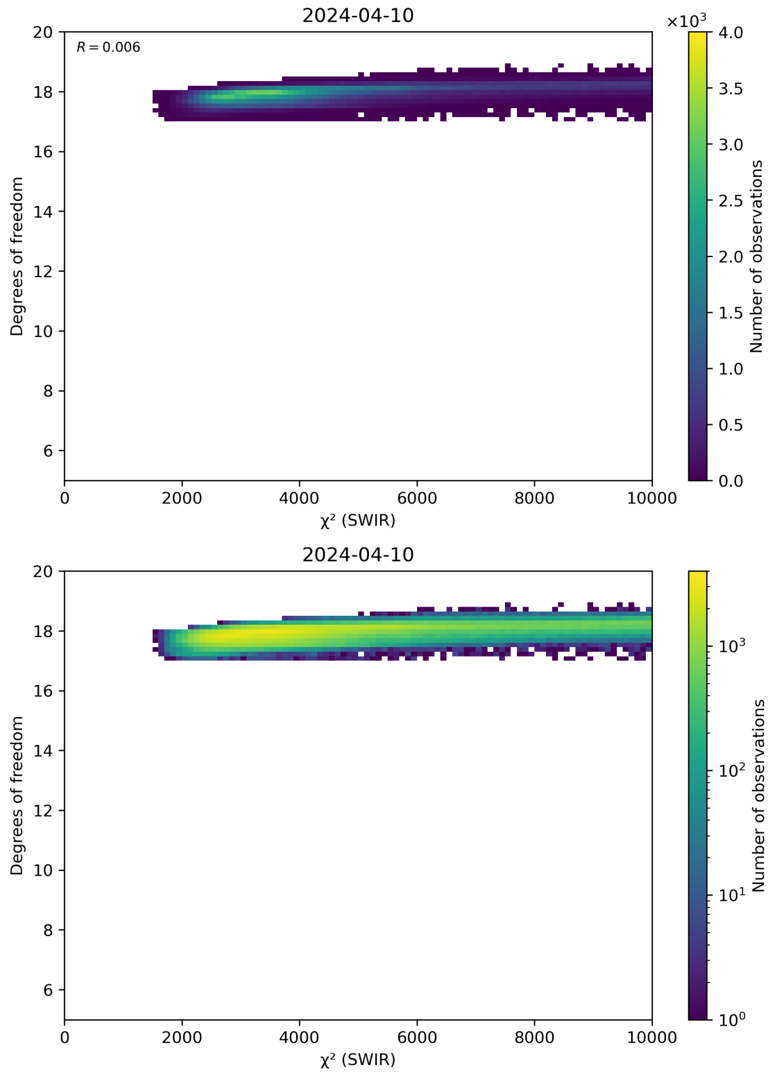
Figure 48: Scatter density plot of “ \chi^2 (SWIR)” against “Degrees of freedom” for 2024-04-10 to 2024-04-11.
