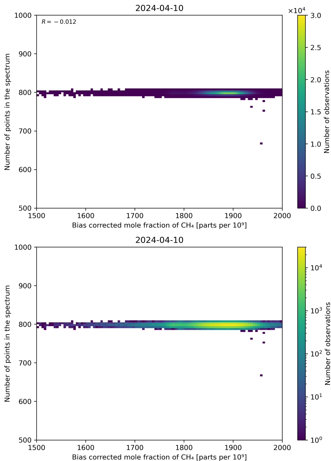
Figure 68: Scatter density plot of “Bias corrected mole fraction of CH 4 ” against “Number of points in the spectrum” for 2024-04-10 to 2024-04-11.
