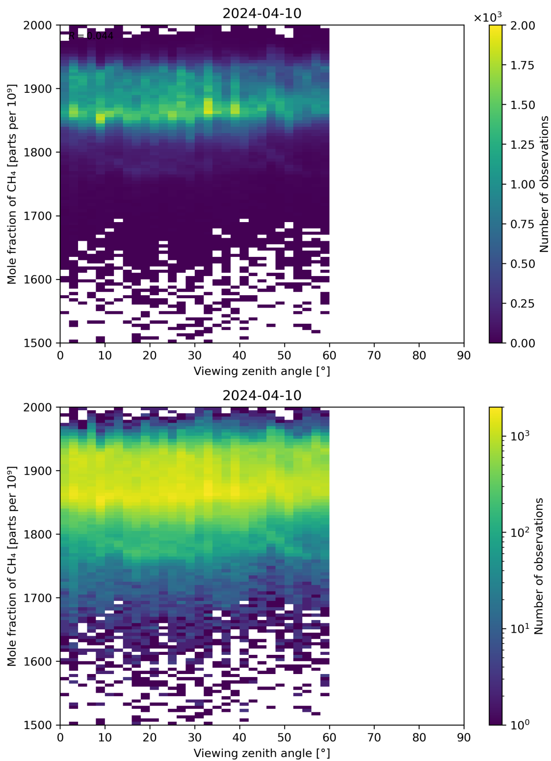
Figure 110: Scatter density plot of “Viewing zenith angle” against “Mole fraction of CH 4 ” for 2024-04-10 to 2024-04-11.
