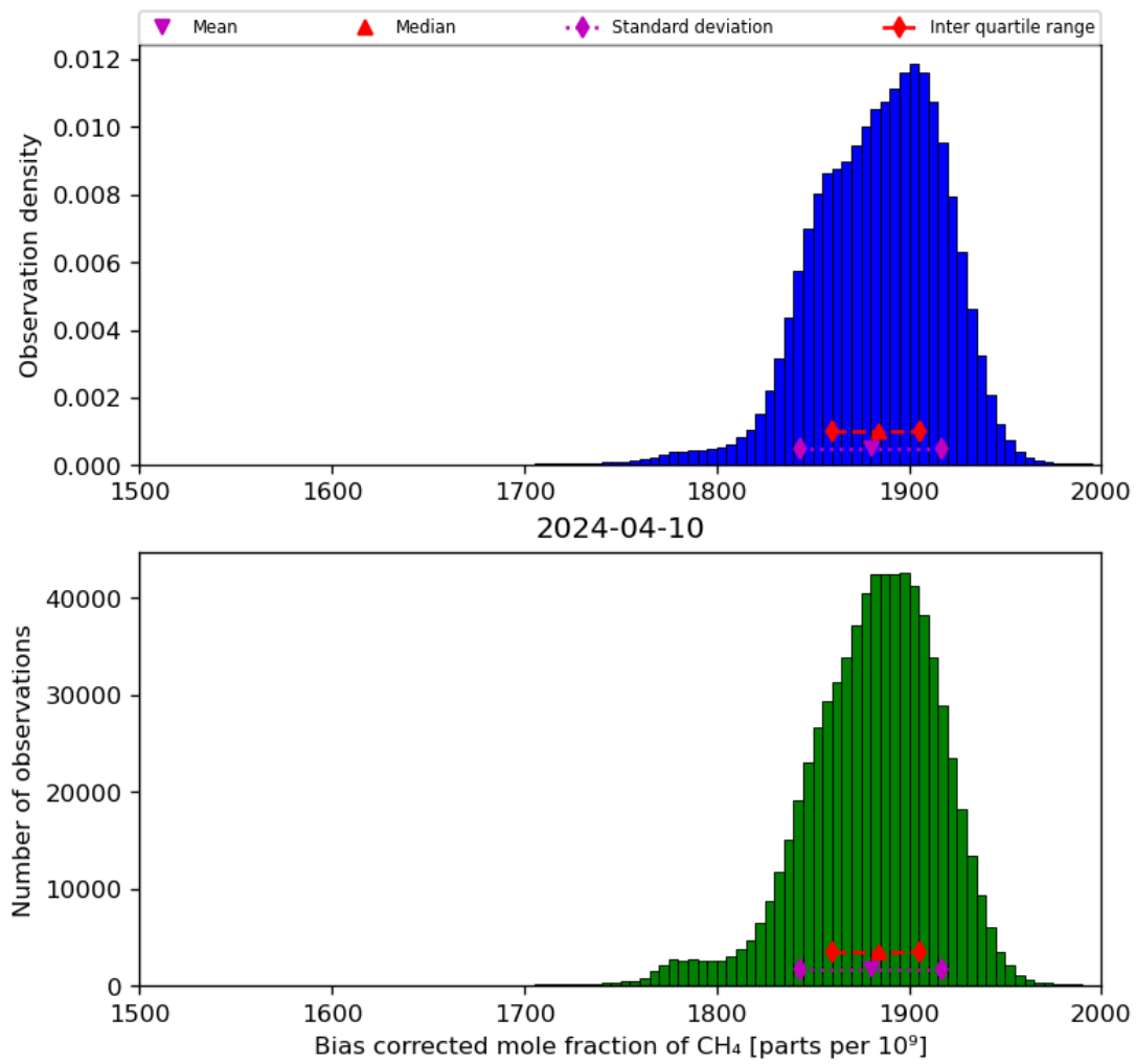
Figure 25: Histogram of “Bias corrected mole fraction of CH 4 ” for 2024-04-10 to 2024-04-11
