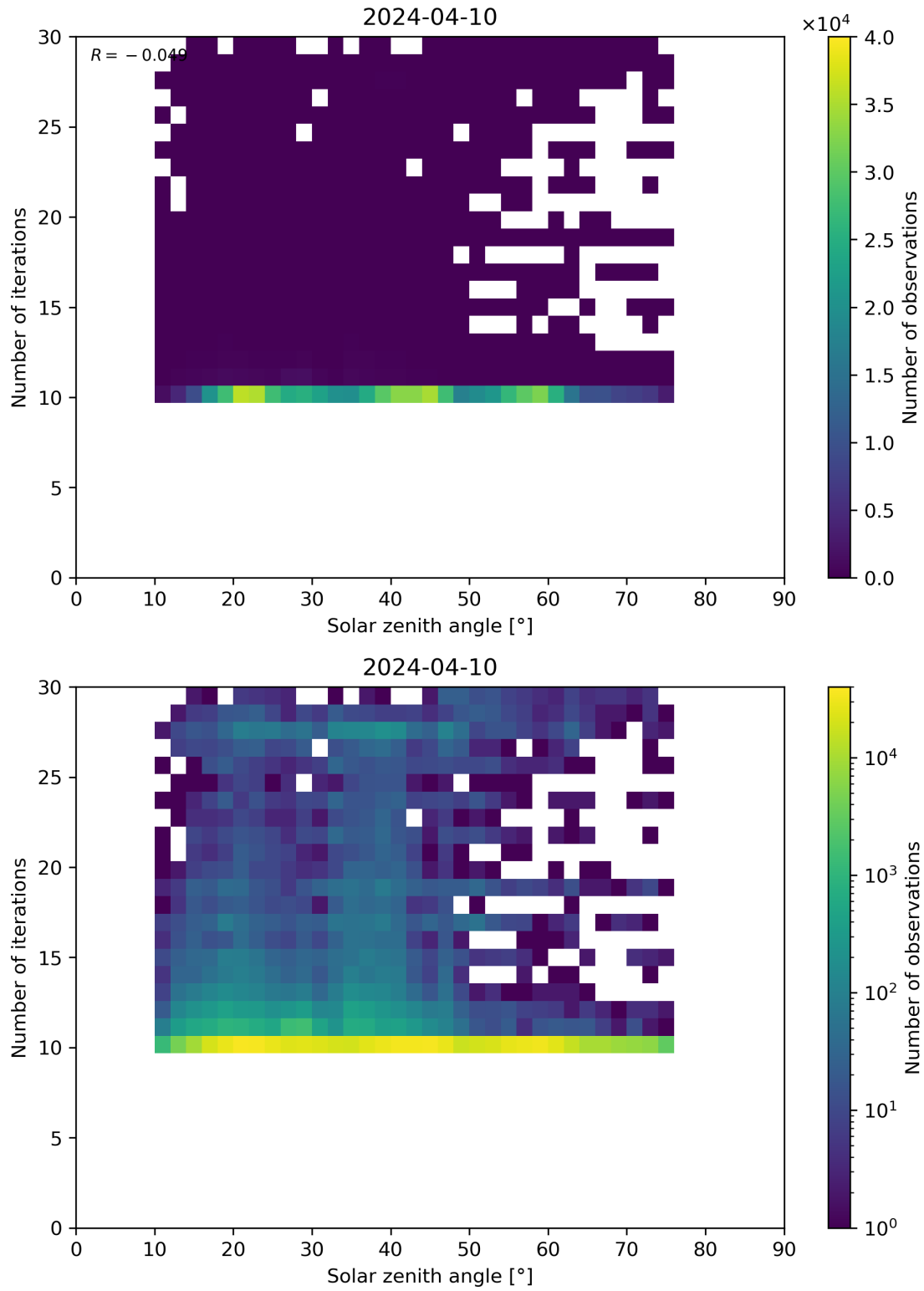
Figure 102: Scatter density plot of “Solar zenith angle” against “Number of iterations” for 2024-04-10 to 2024-04-11.
