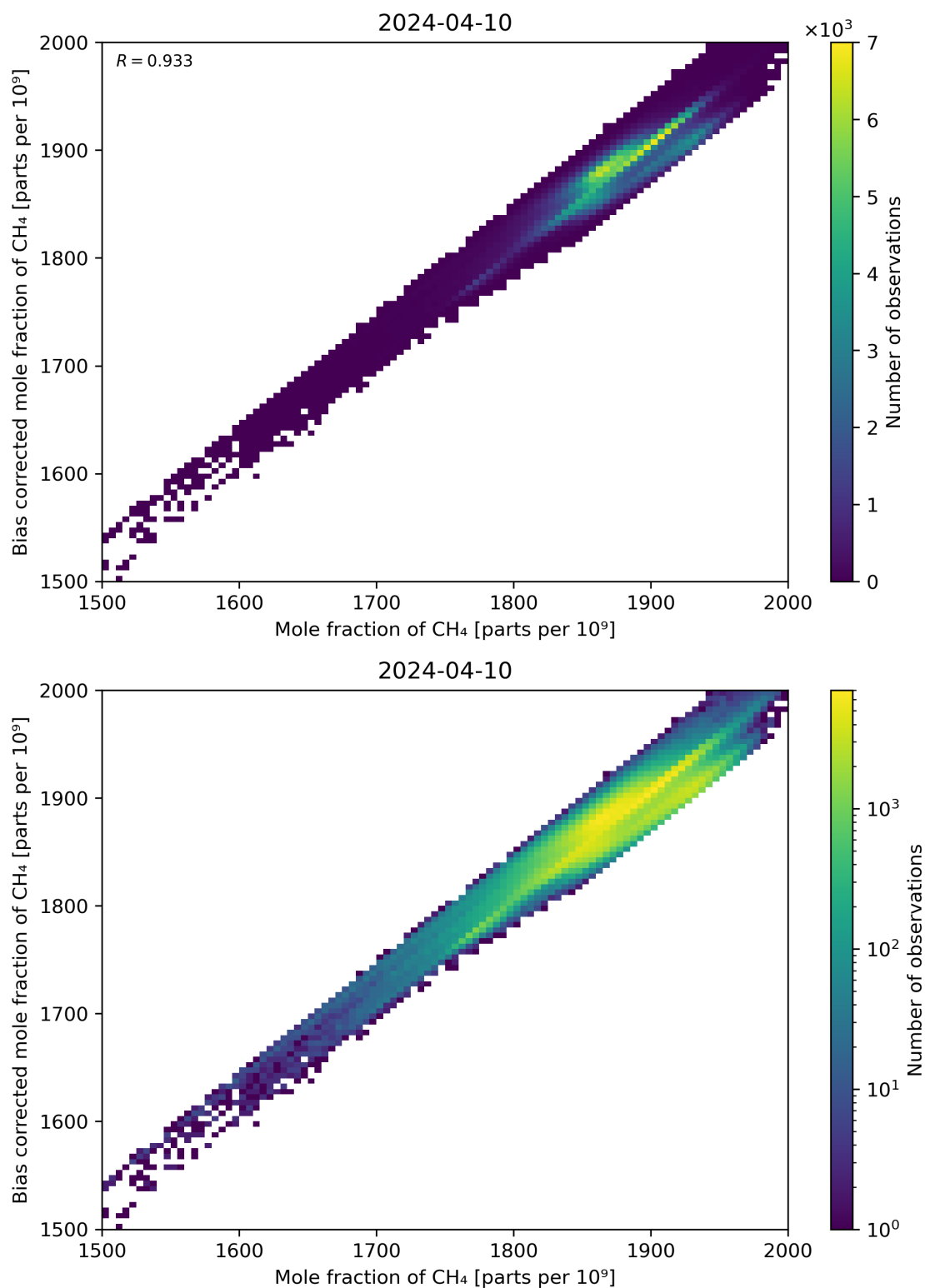
Figure 74: Scatter density plot of “Mole fraction of CH 4 ” against “Bias corrected mole fraction of CH 4 ” for 2024-04-10 to 2024-04-11.
