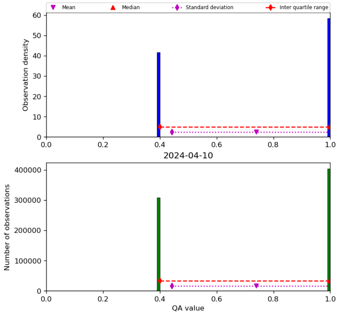
Figure 22: Histogram of “QA value” for 2024-04-10 to 2024-04-11
