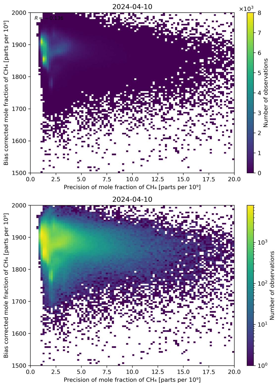
Figure 82: Scatter density plot of “Precision of mole fraction of CH 4 ” against “Bias corrected mole fraction of CH 4 ” for 2024-04-10 to 2024-04-11.
