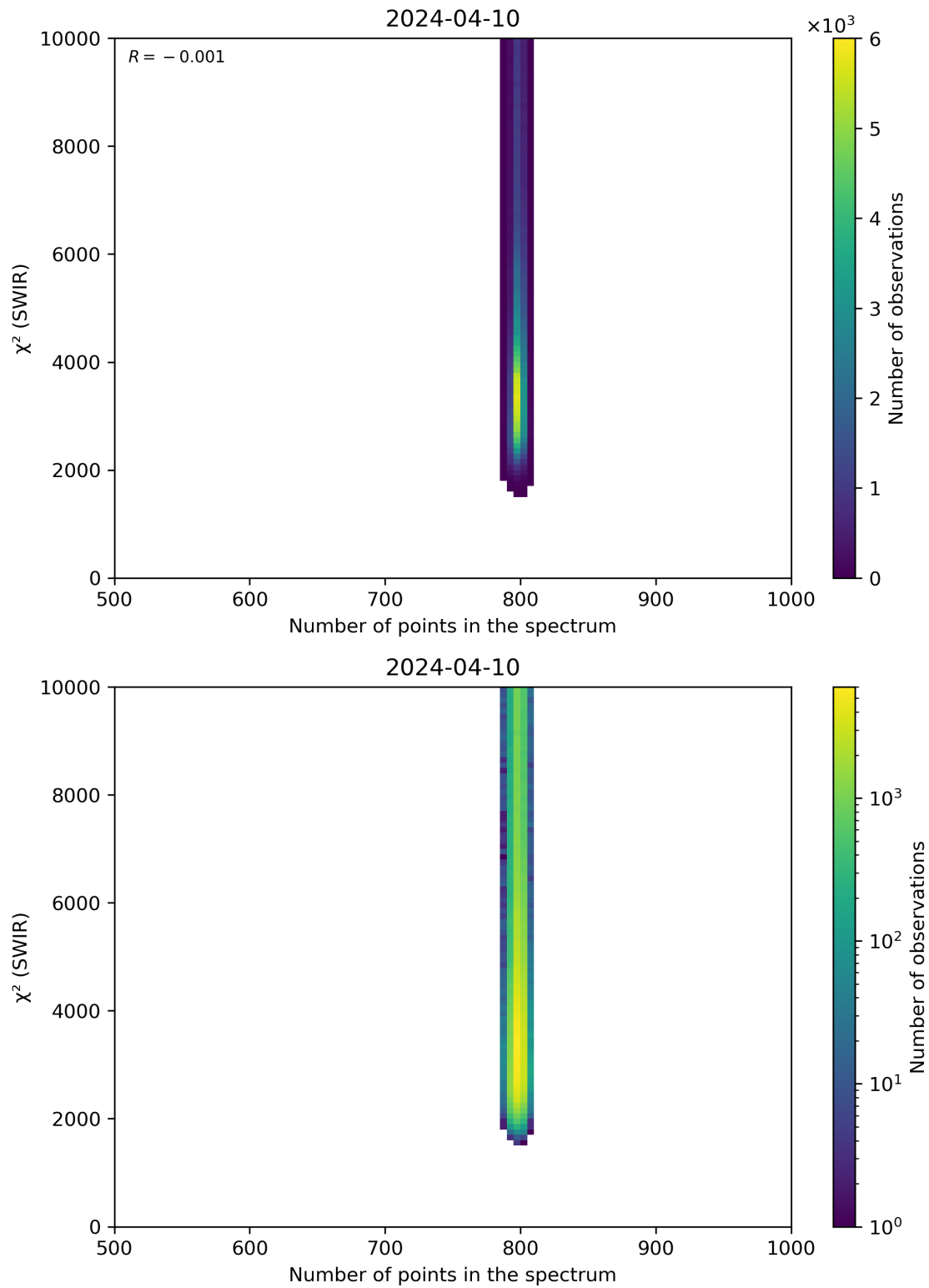
Figure 89: Scatter density plot of “Number of points in the spectrum” against “ \chi^2 (SWIR)” for 2024-04-10 to 2024-04-11.
