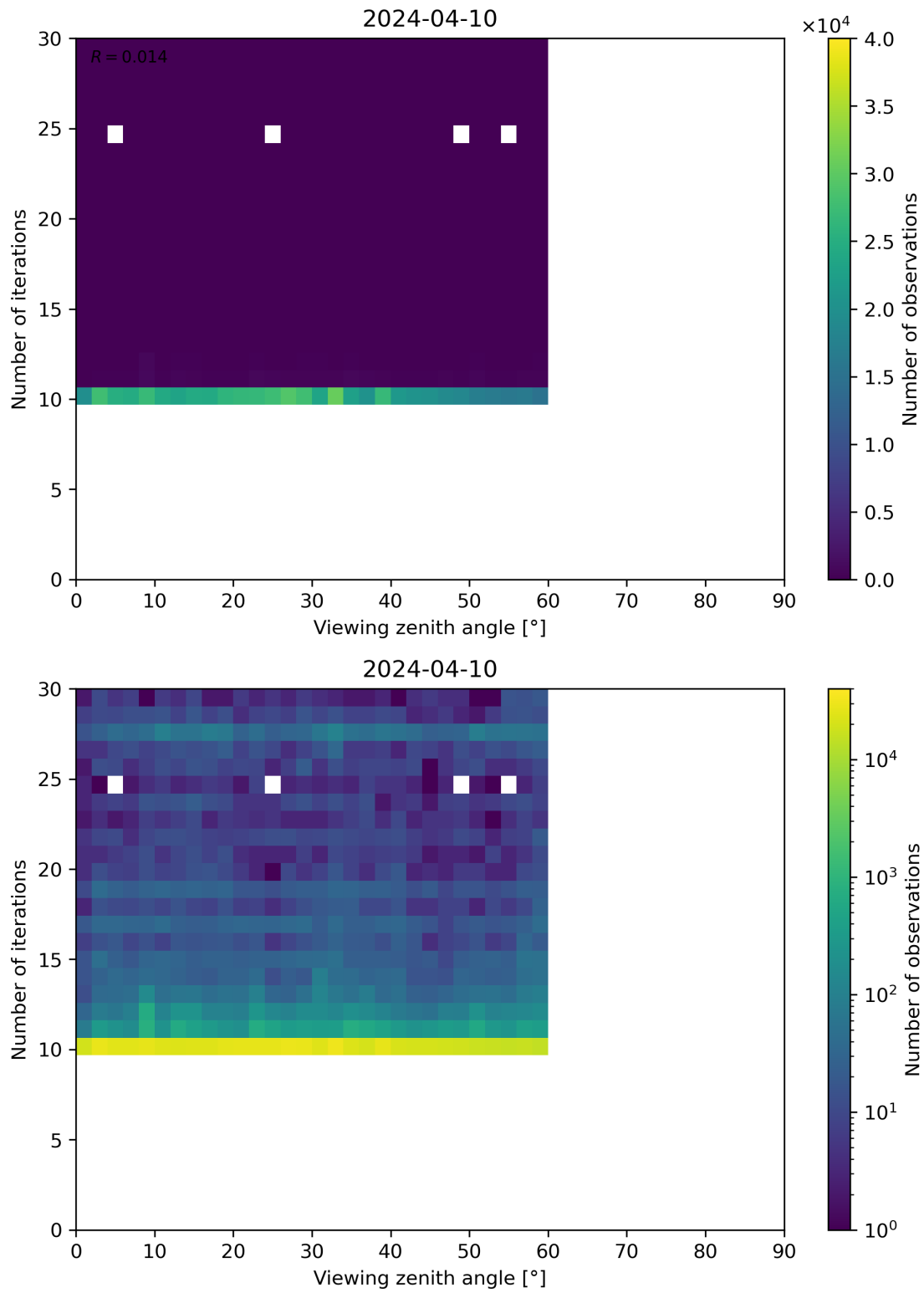
Figure 113: Scatter density plot of “Viewing zenith angle” against “Number of iterations” for 2024-04-10 to 2024-04-11.
