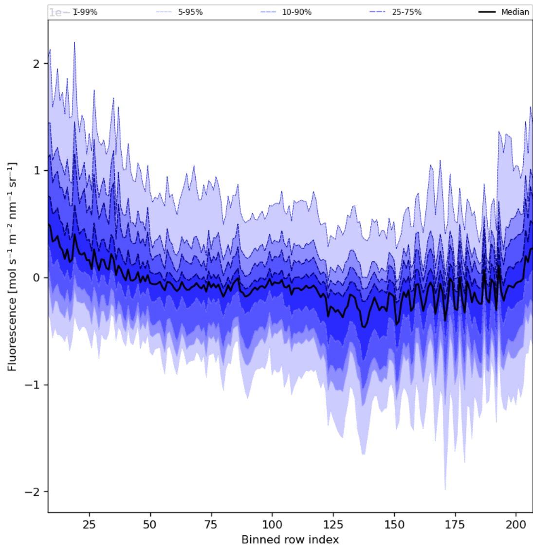
Figure 43: Along track statistics of “Fluorescence” for 2024-04-10 to 2024-04-11
