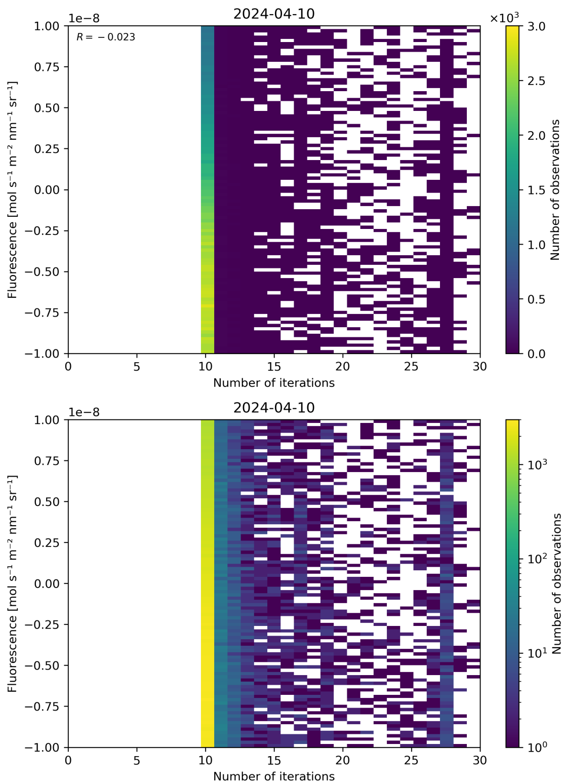
Figure 87: Scatter density plot of “Number of iterations” against “Fluorescence” for 2024-04-10 to 2024-04-11.
