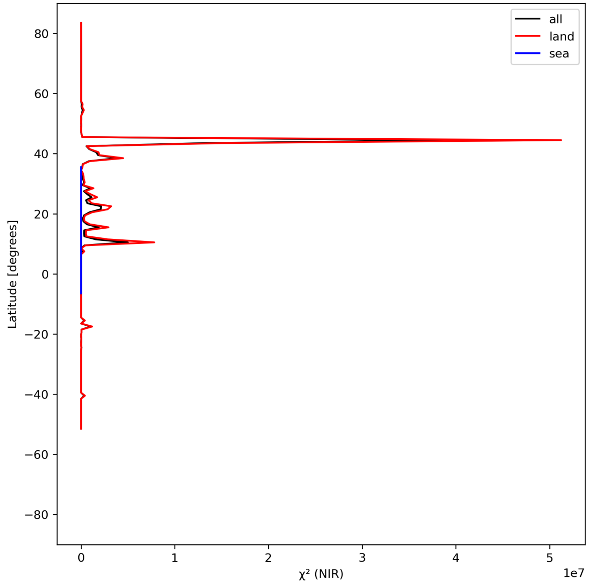
Figure 18: Zonal average of “ \chi^2 (NIR)” for 2024-04-10 to 2024-04-11.
