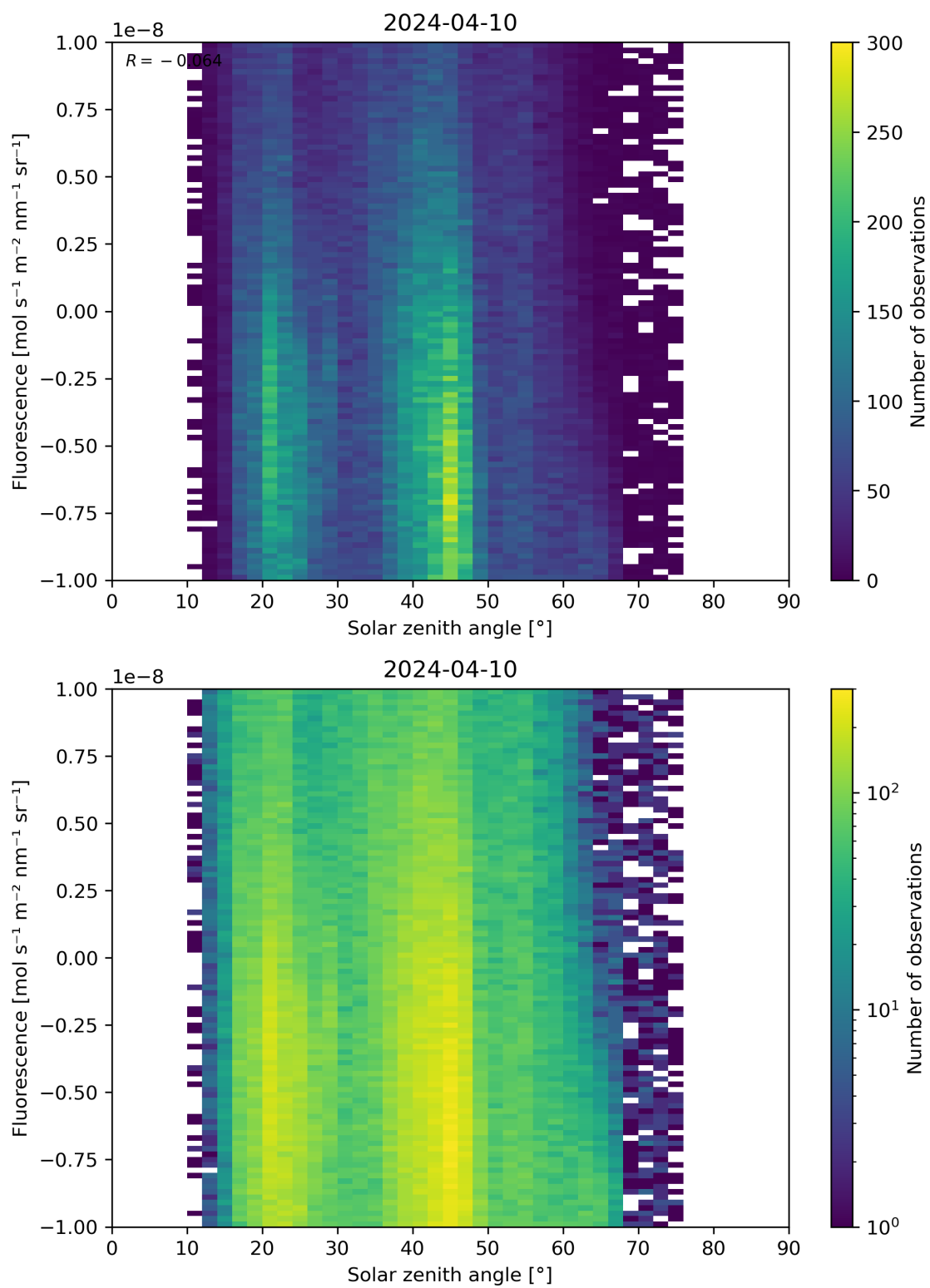
Figure 97: Scatter density plot of “Solar zenith angle” against “Fluorescence” for 2024-04-10 to 2024-04-11.
