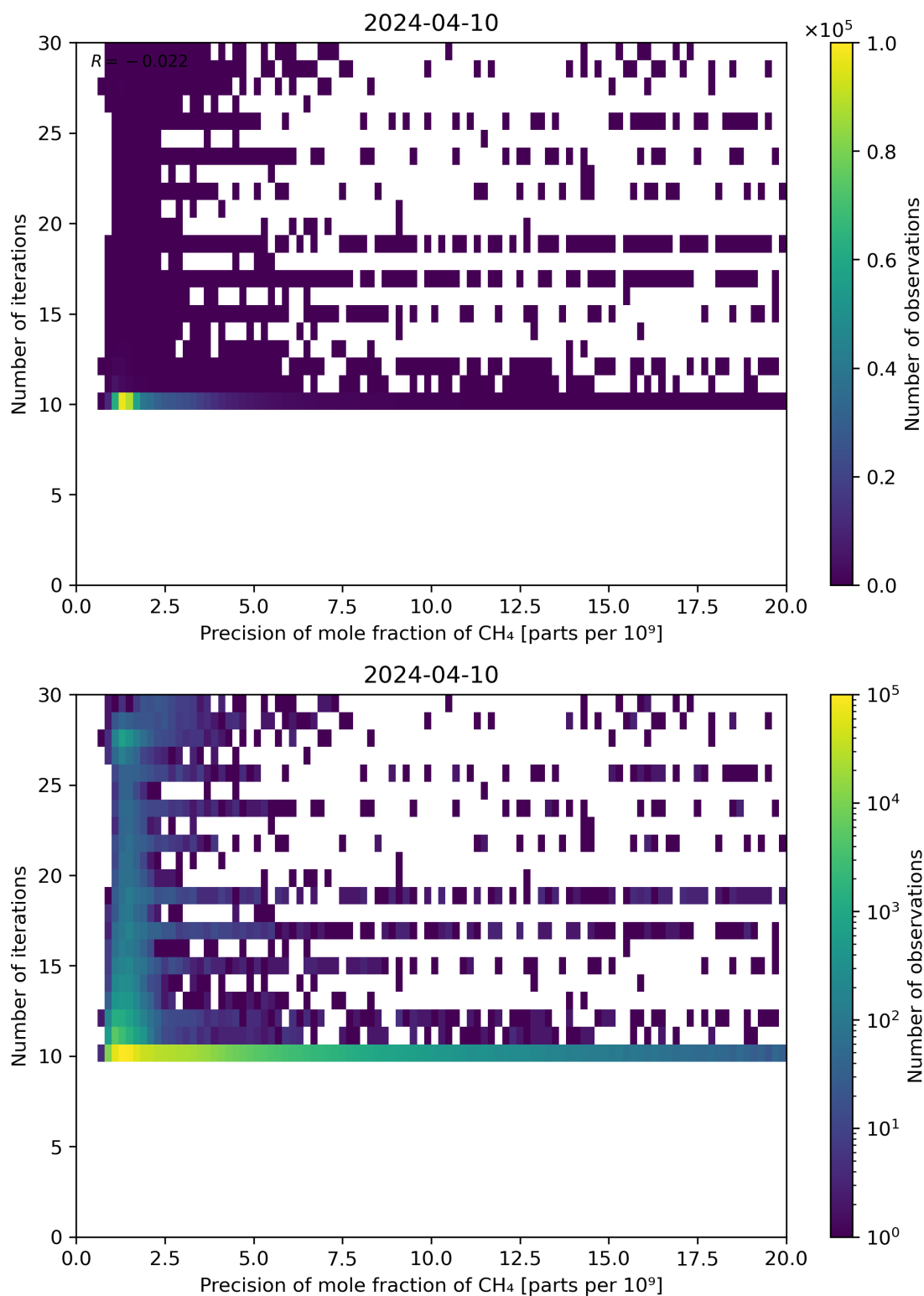
Figure 83: Scatter density plot of “Precision of mole fraction of CH 4 ” against “Number of iterations” for 2024-04-10 to 2024-04-11.
