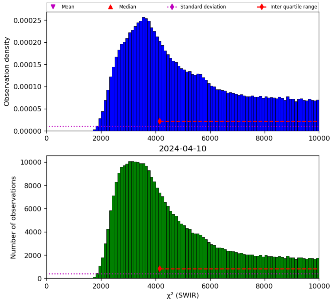
Figure 28: Histogram of “ \chi^2 (SWIR)” for 2024-04-10 to 2024-04-11
