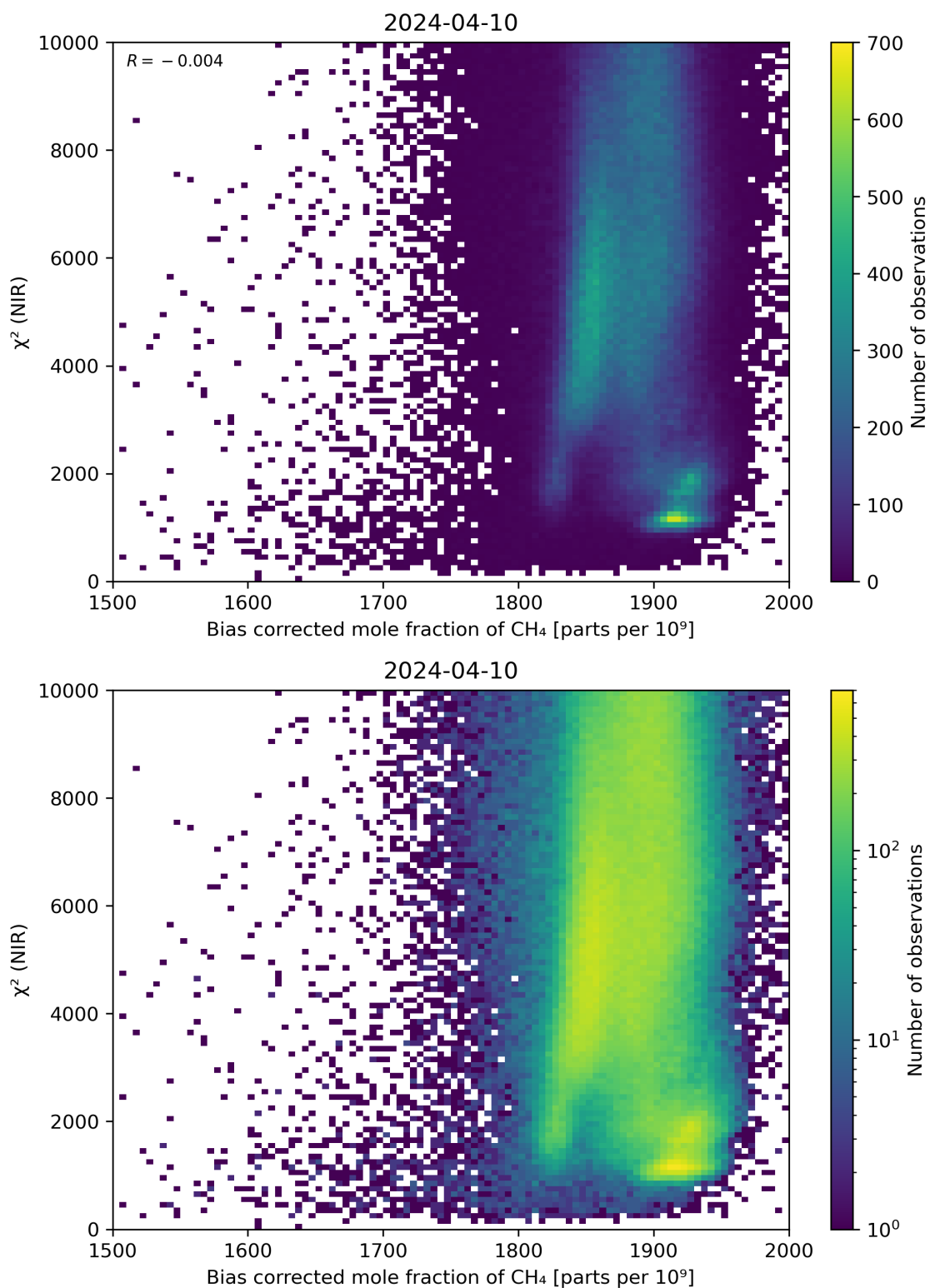
Figure 63: Scatter density plot of “Bias corrected mole fraction of CH 4 ” against “ \chi^2 (NIR)” for 2024-04-10 to 2024-04-11.
