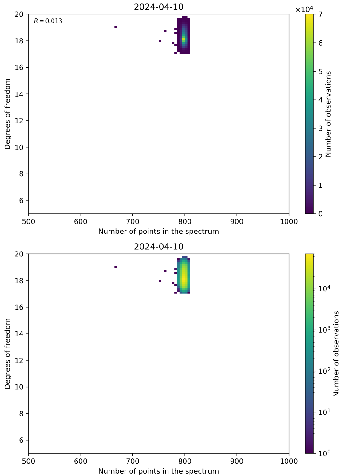
Figure 90: Scatter density plot of “Number of points in the spectrum” against “Degrees of freedom” for 2024-04-10 to 2024-04-11.
