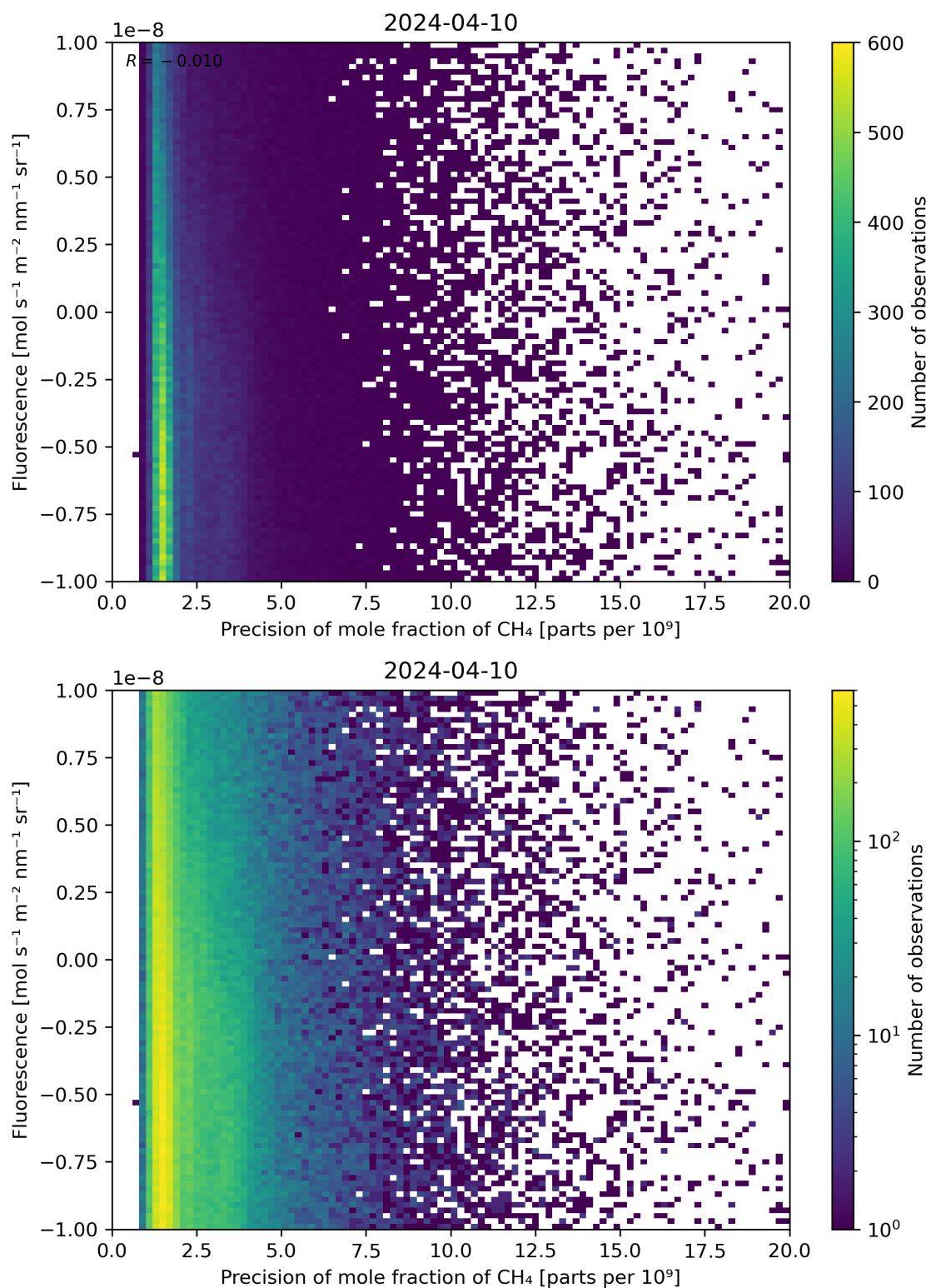
Figure 81: Scatter density plot of “Precision of mole fraction of \text{CH}_4 ” against “Fluorescence” for 2024-04-10 to 2024-04-11.
