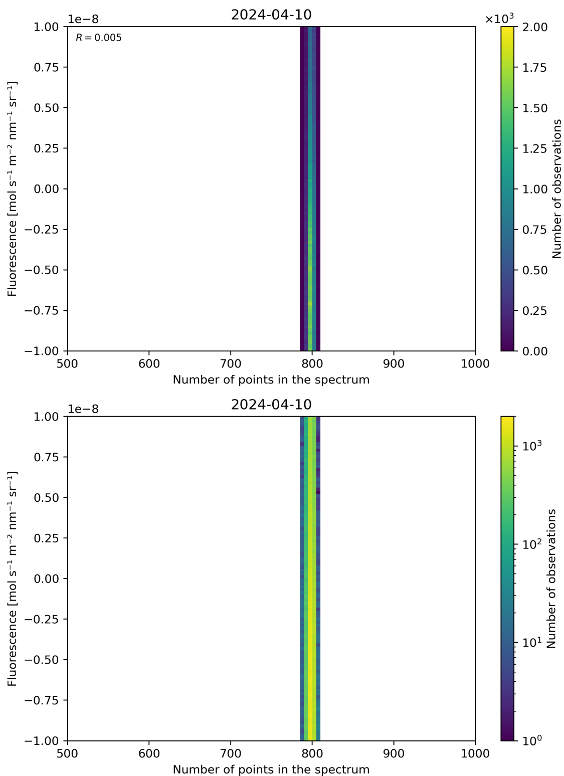
Figure 91: Scatter density plot of “Number of points in the spectrum” against “Fluorescence” for 2024-04-10 to 2024-04-11.
