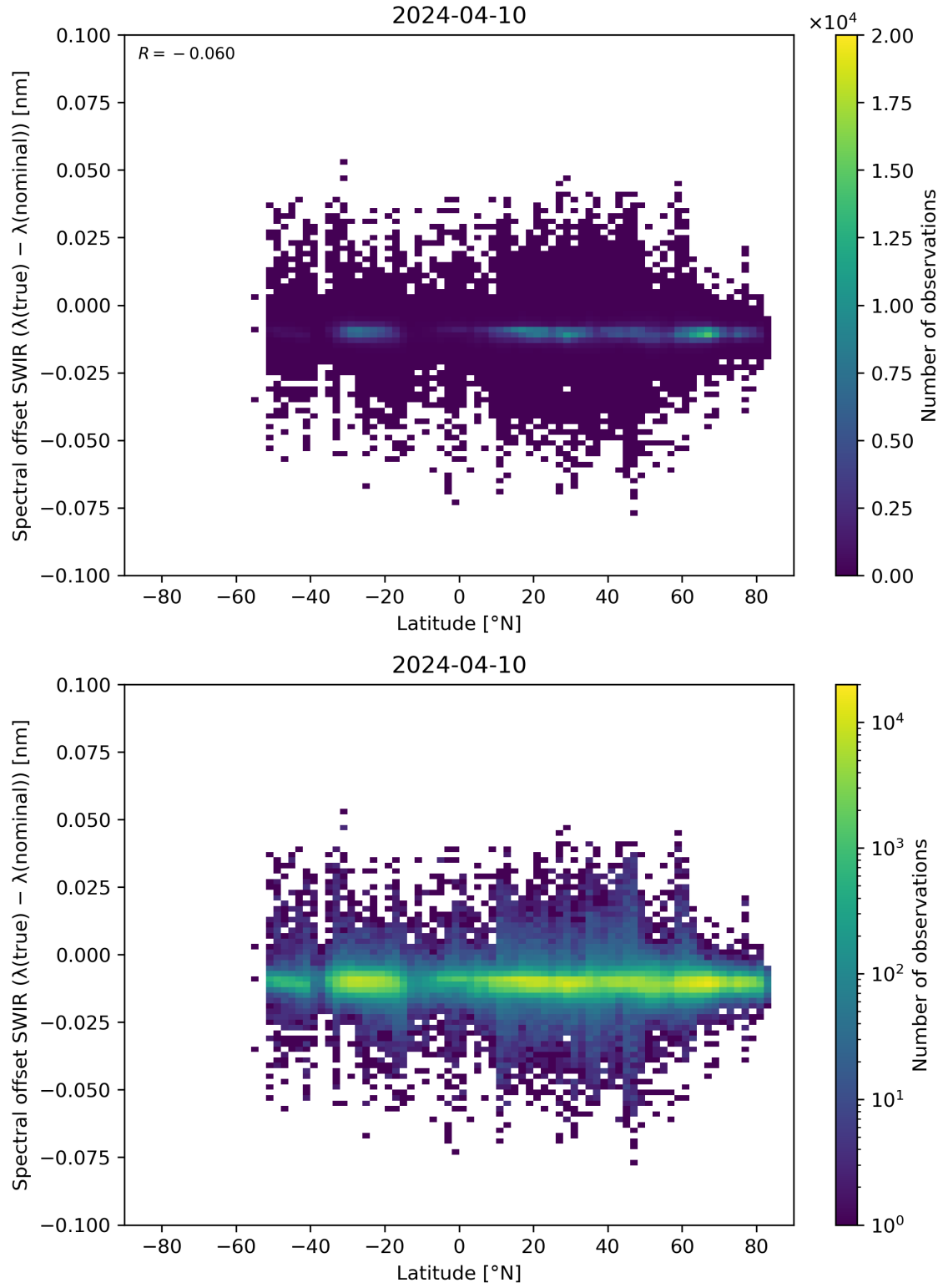
Figure 62: Scatter density plot of “Latitude” against “Spectral offset SWIR ( \lambda(\text{true}) - \lambda(\text{nominal}) )” for 2024-04-10 to 2024-04-11.
