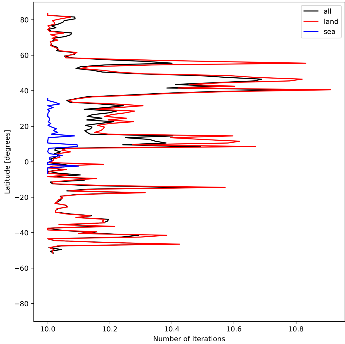
Figure 20: Zonal average of “Number of iterations” for 2024-04-10 to 2024-04-11.
