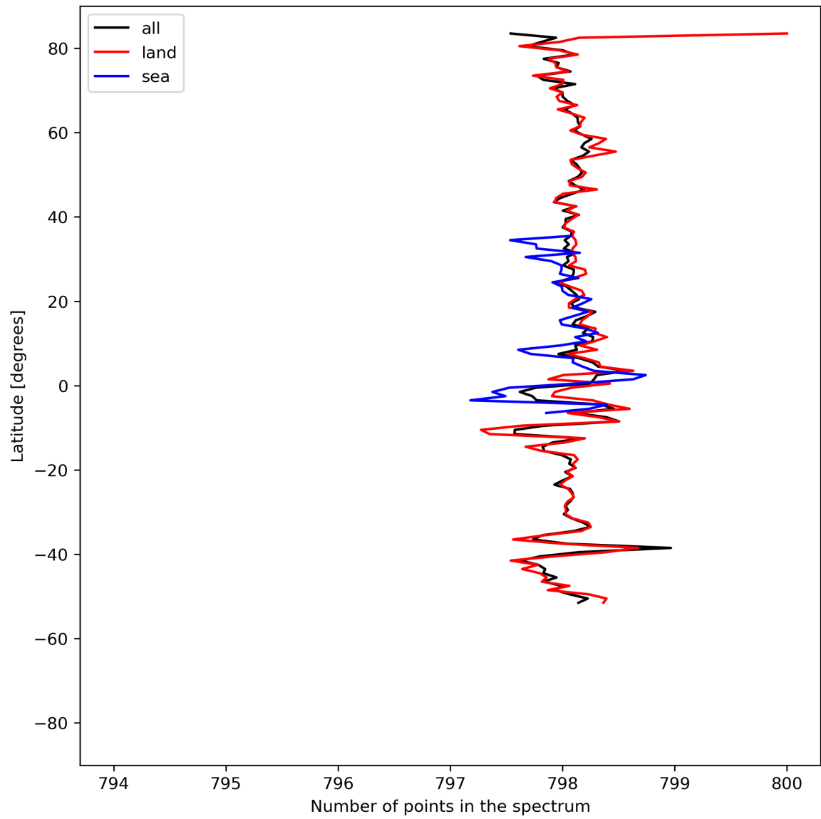
Figure 15: Zonal average of “Number of points in the spectrum” for 2024-04-10 to 2024-04-11.
