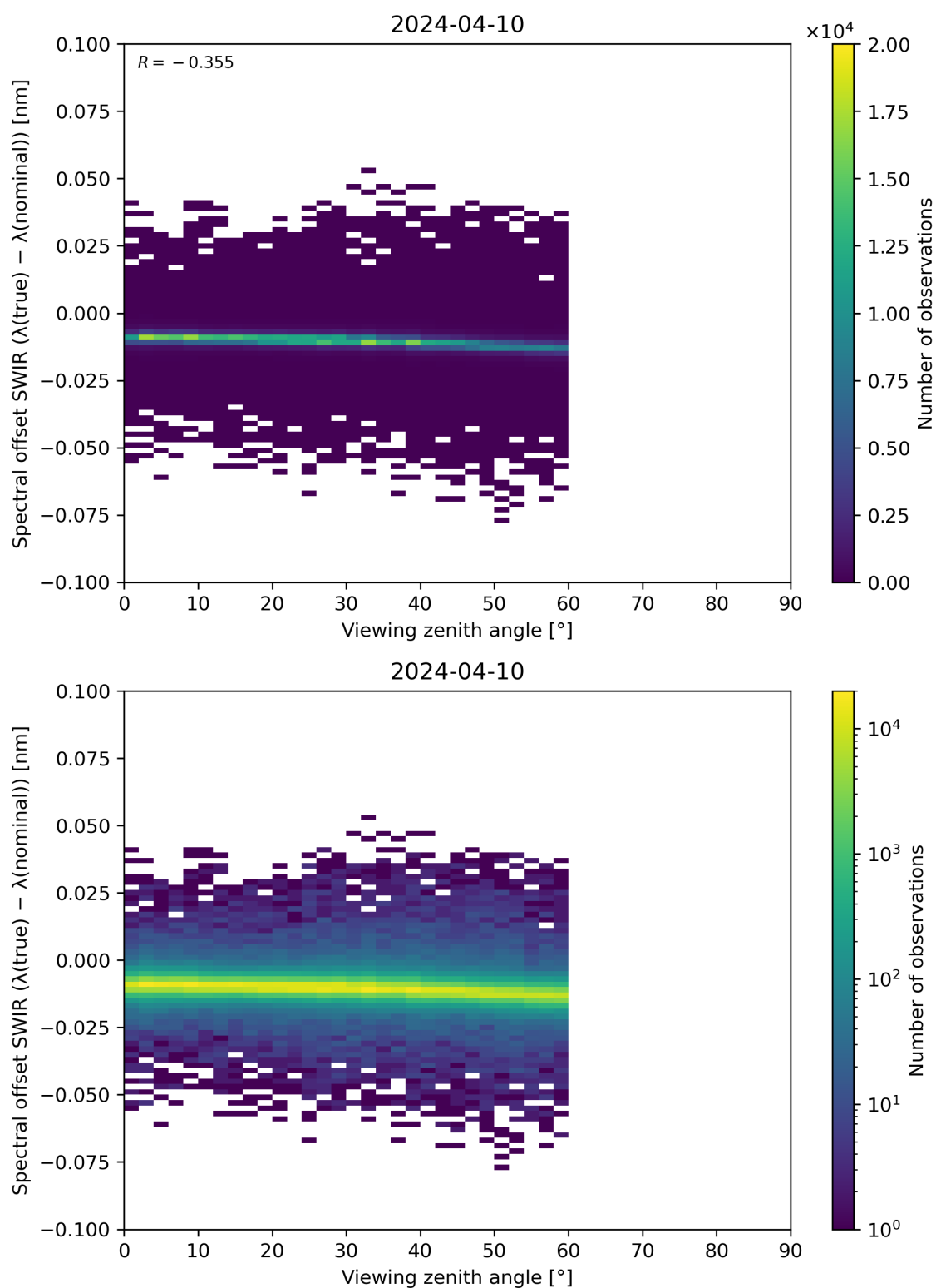
Figure 116: Scatter density plot of “Viewing zenith angle” against “Spectral offset SWIR ( \lambda(\text{true}) - \lambda(\text{nominal}) )” for 2024-04-10 to 2024-04-11.
