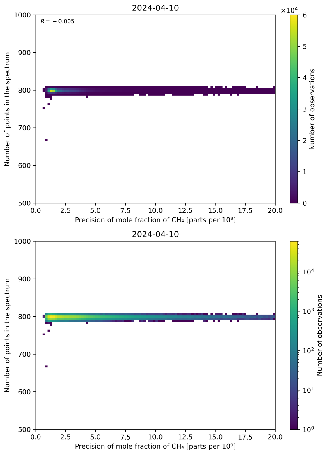
Figure 84: Scatter density plot of “Precision of mole fraction of CH 4 ” against “Number of points in the spectrum” for 2024-04-10 to 2024-04-11.
