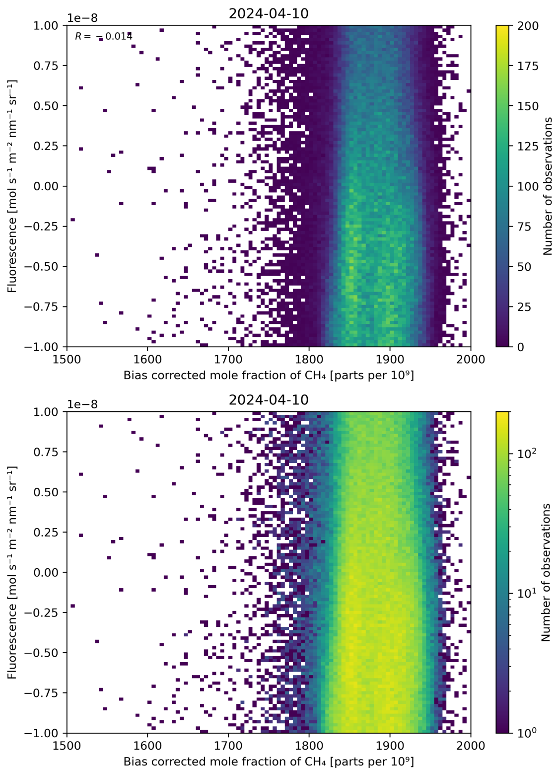
Figure 66: Scatter density plot of “Bias corrected mole fraction of \text{CH}_4 ” against “Fluorescence” for 2024-04-10 to 2024-04-11.
