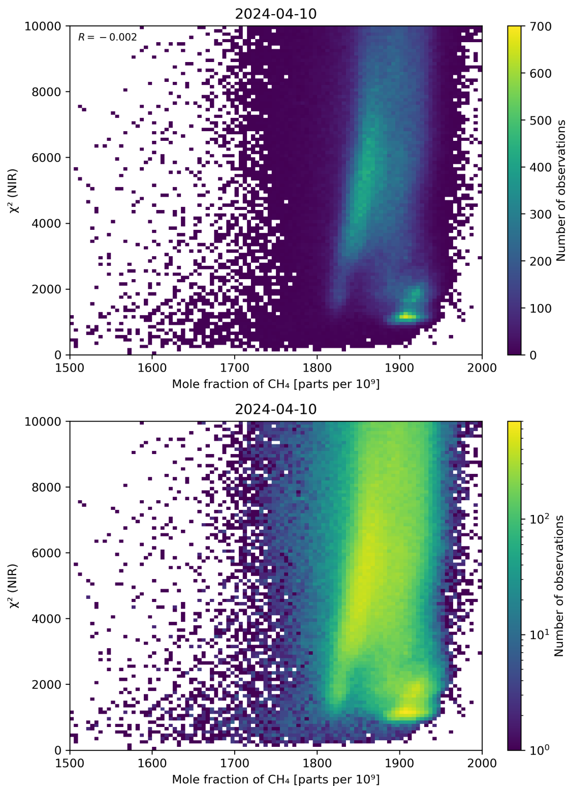
Figure 70: Scatter density plot of “Mole fraction of CH 4 ” against “ \chi^2 (NIR)” for 2024-04-10 to 2024-04-11.
