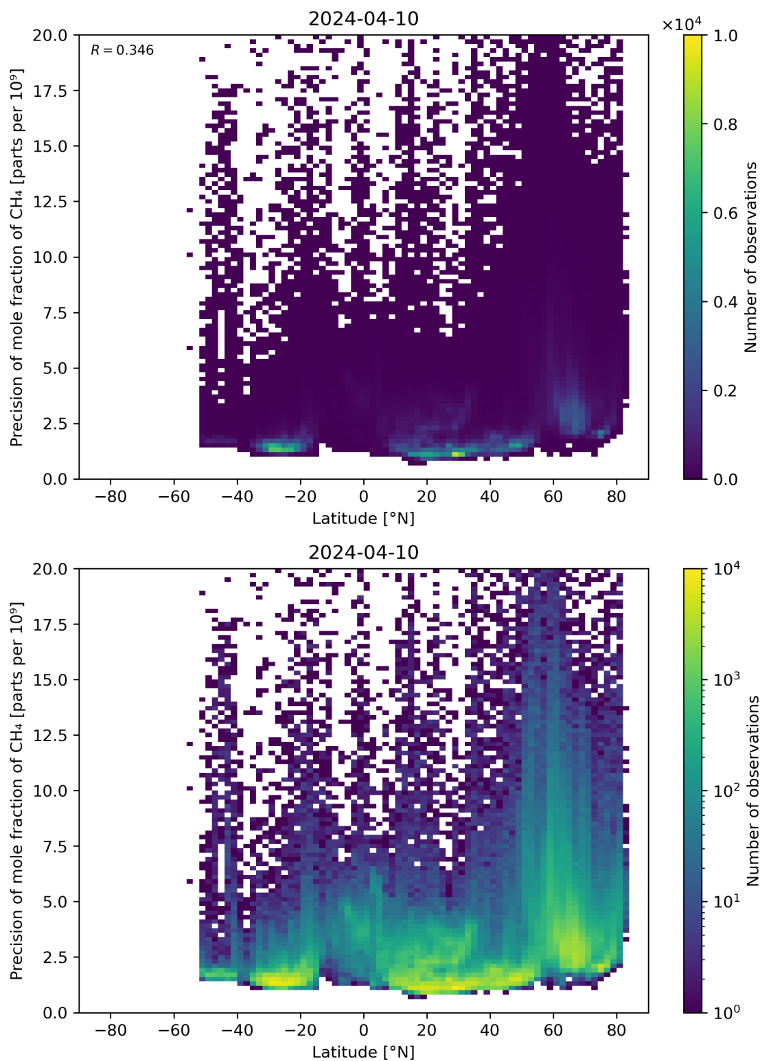
Figure 59: Scatter density plot of “Latitude” against “Precision of mole fraction of \text{CH}_4 ” for 2024-04-10 to 2024-04-11.
