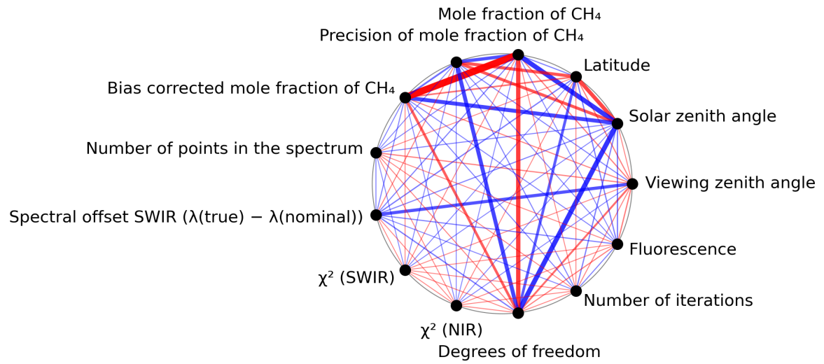
Figure 1: Map of correlation graph for 2024-04-10 to 2024-04-11.
