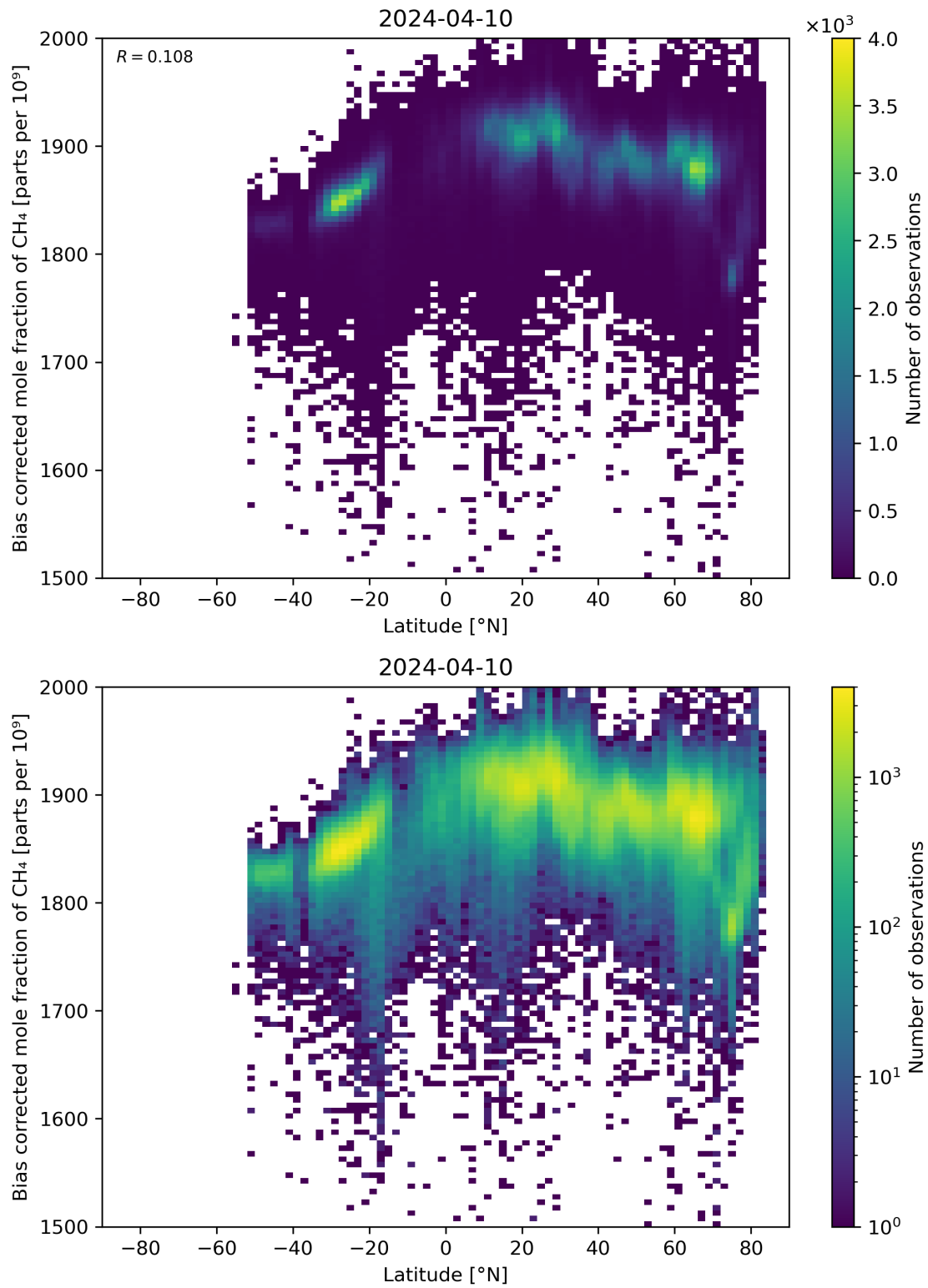
Figure 58: Scatter density plot of “Latitude” against “Bias corrected mole fraction of \text{CH}_4 ” for 2024-04-10 to 2024-04-11.
