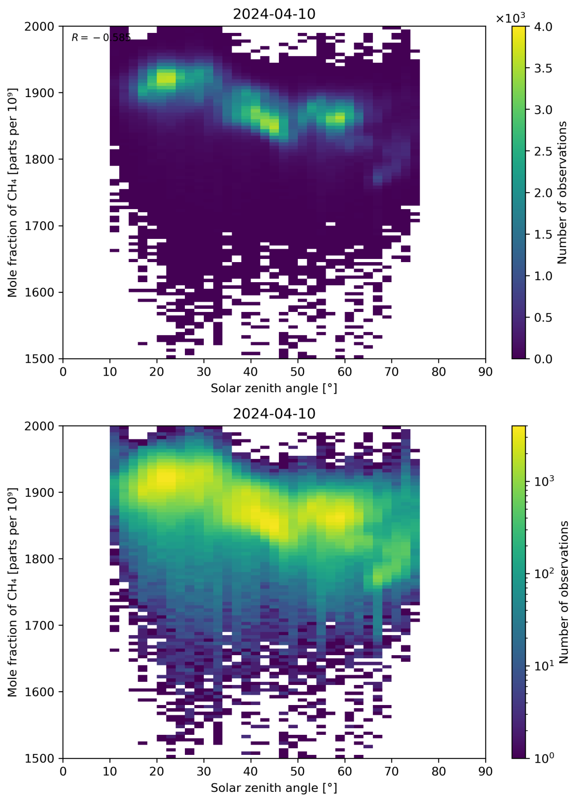
Figure 99: Scatter density plot of “Solar zenith angle” against “Mole fraction of CH 4 ” for 2024-04-10 to 2024-04-11.
