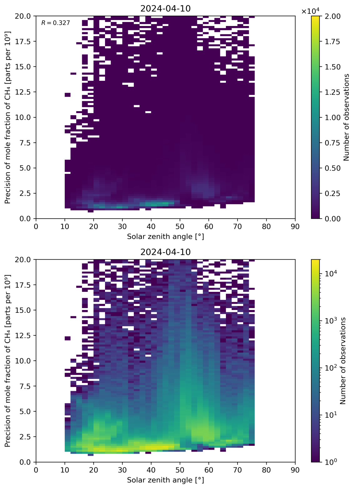
Figure 101: Scatter density plot of “Solar zenith angle” against “Precision of mole fraction of CH 4 ” for 2024-04-10 to 2024-04-11.
