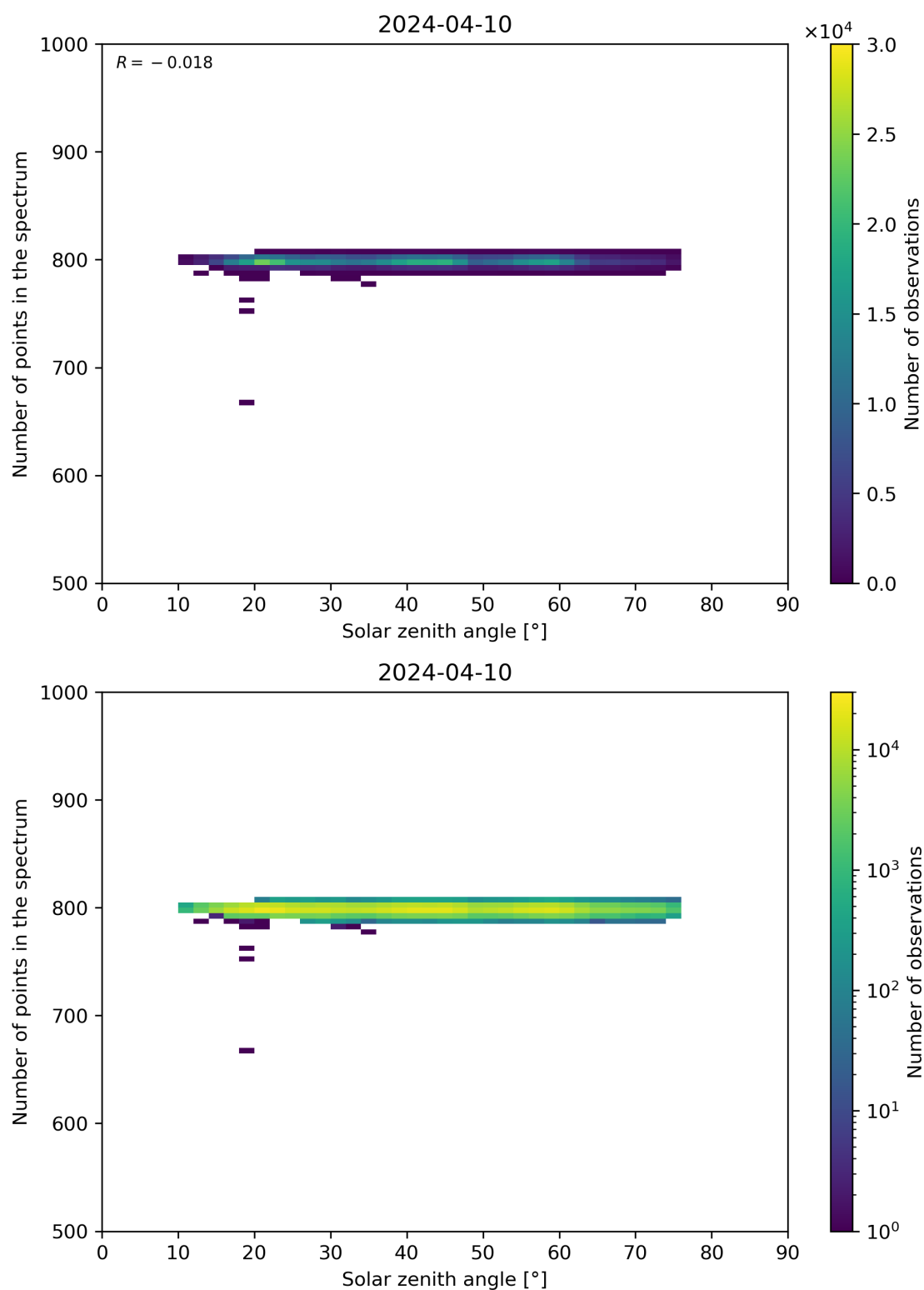
Figure 103: Scatter density plot of “Solar zenith angle” against “Number of points in the spectrum” for 2024-04-10 to 2024-04-11.
