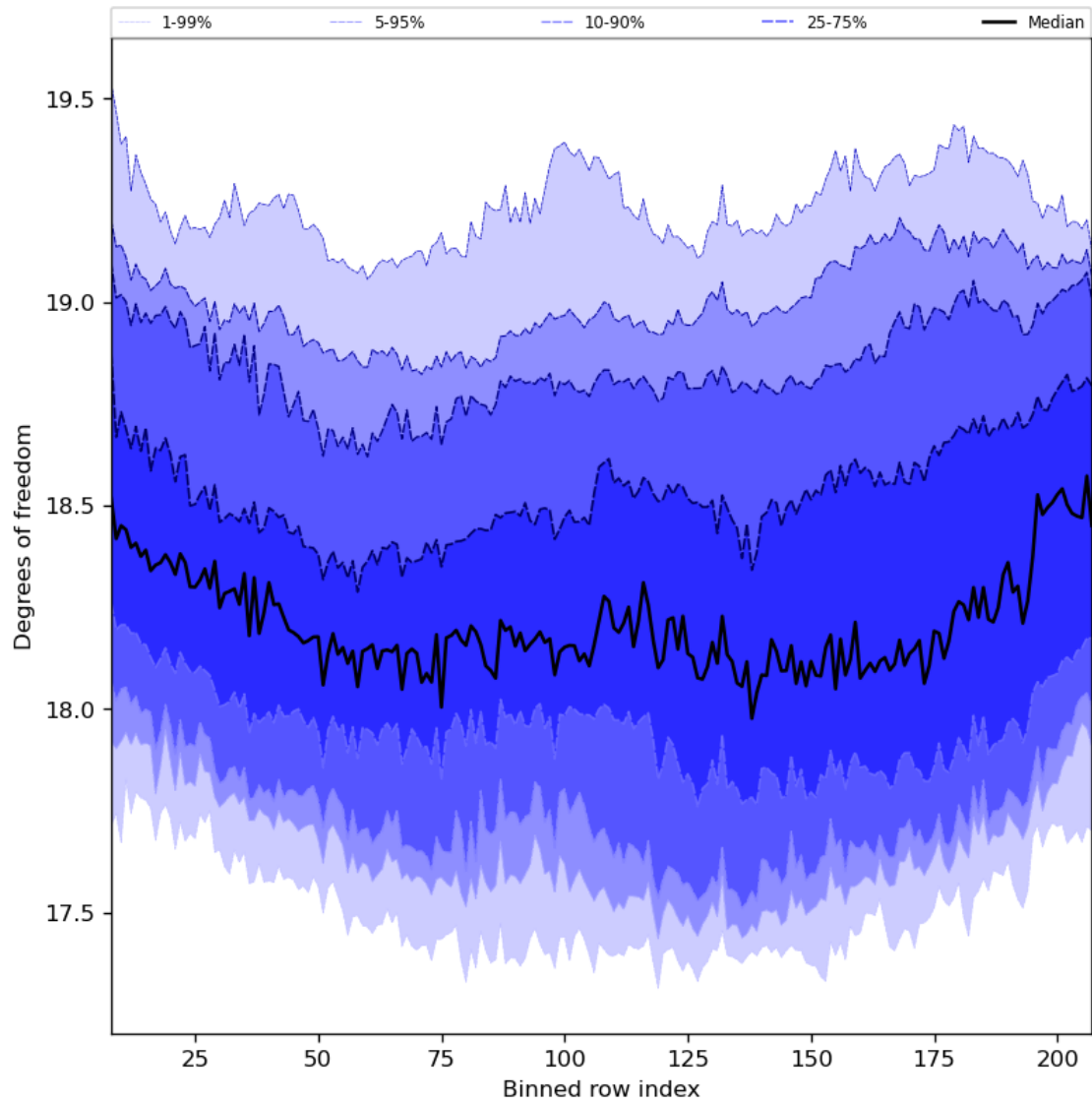
Figure 41: Along track statistics of “Degrees of freedom” for 2024-04-10 to 2024-04-11
