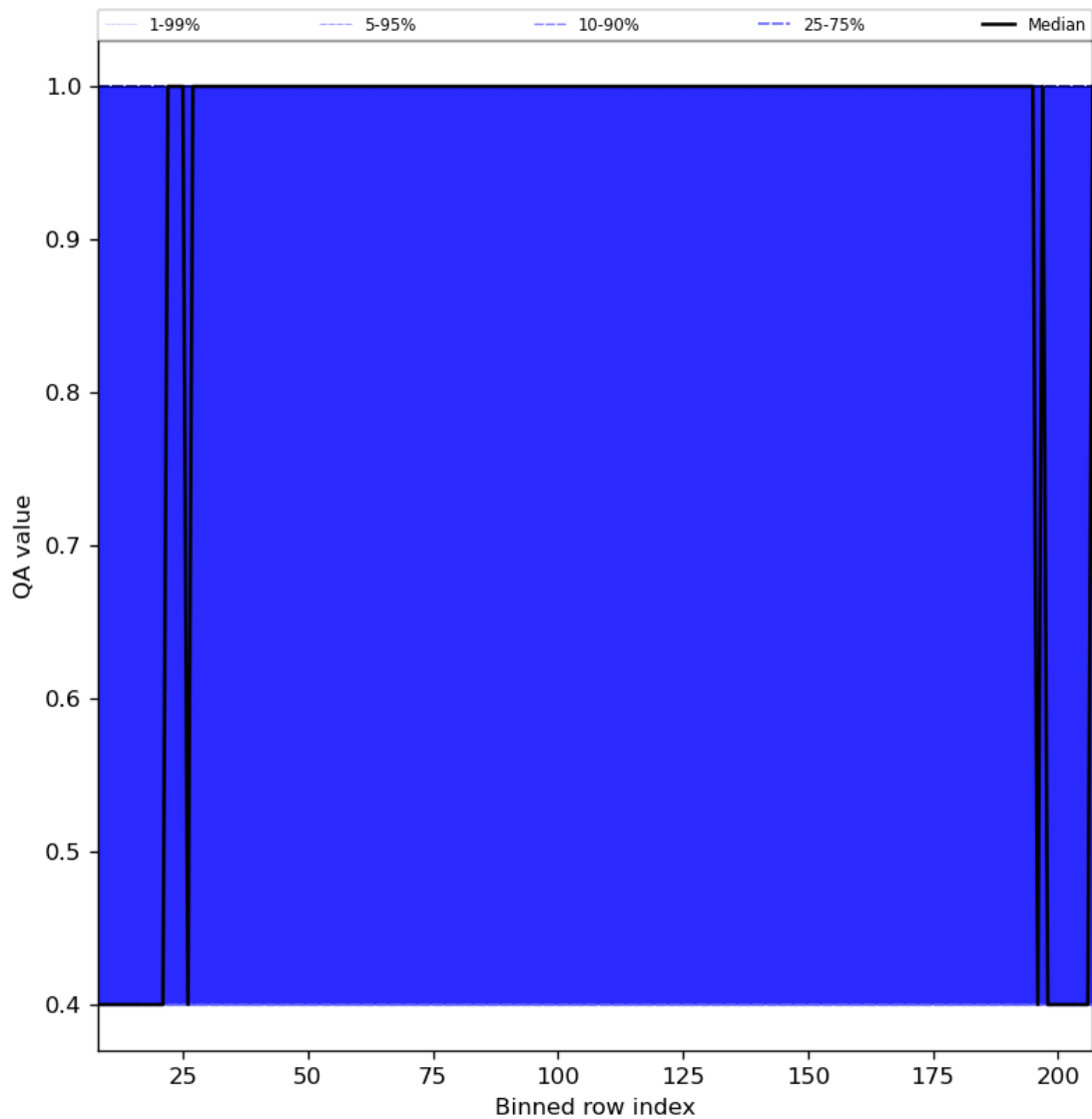
Figure 33: Along track statistics of “QA value” for 2024-04-10 to 2024-04-11
