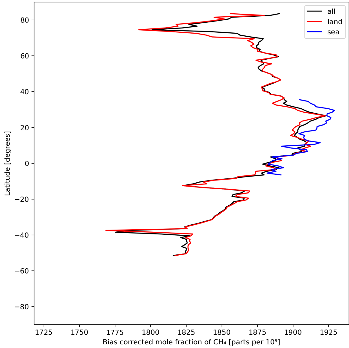
Figure 14: Zonal average of “Bias corrected mole fraction of CH 4 ” for 2024-04-10 to 2024-04-11.
