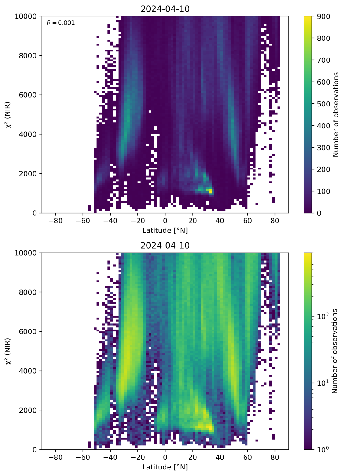
Figure 53: Scatter density plot of “Latitude” against “ \chi^2 (NIR)” for 2024-04-10 to 2024-04-11.
