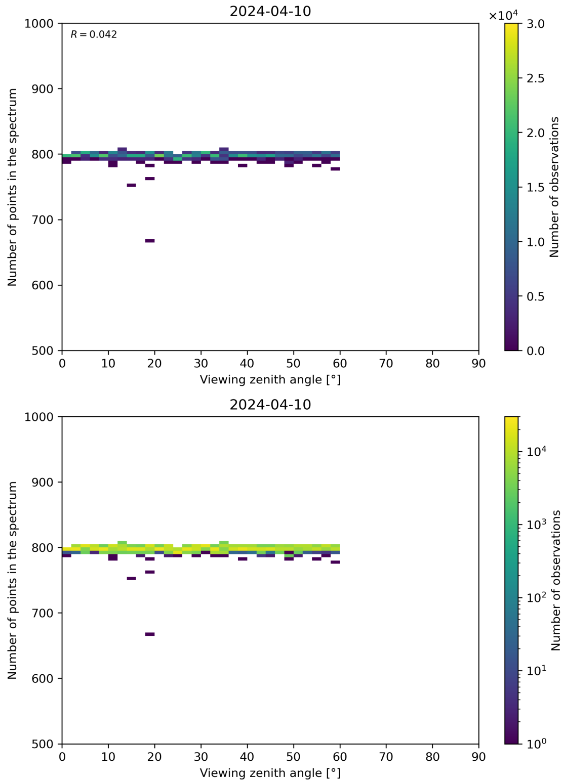
Figure 114: Scatter density plot of “Viewing zenith angle” against “Number of points in the spectrum” for 2024-04-10 to 2024-04-11.
