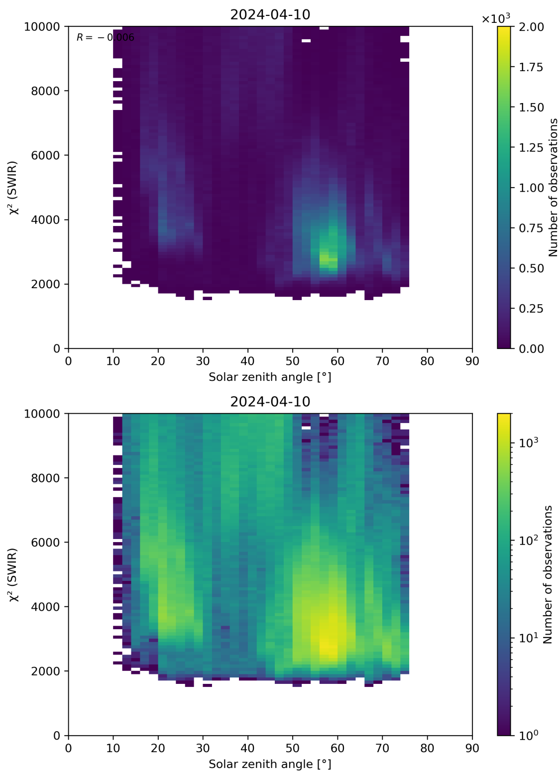
Figure 95: Scatter density plot of “Solar zenith angle” against “ \chi^2 (SWIR)” for 2024-04-10 to 2024-04-11.
