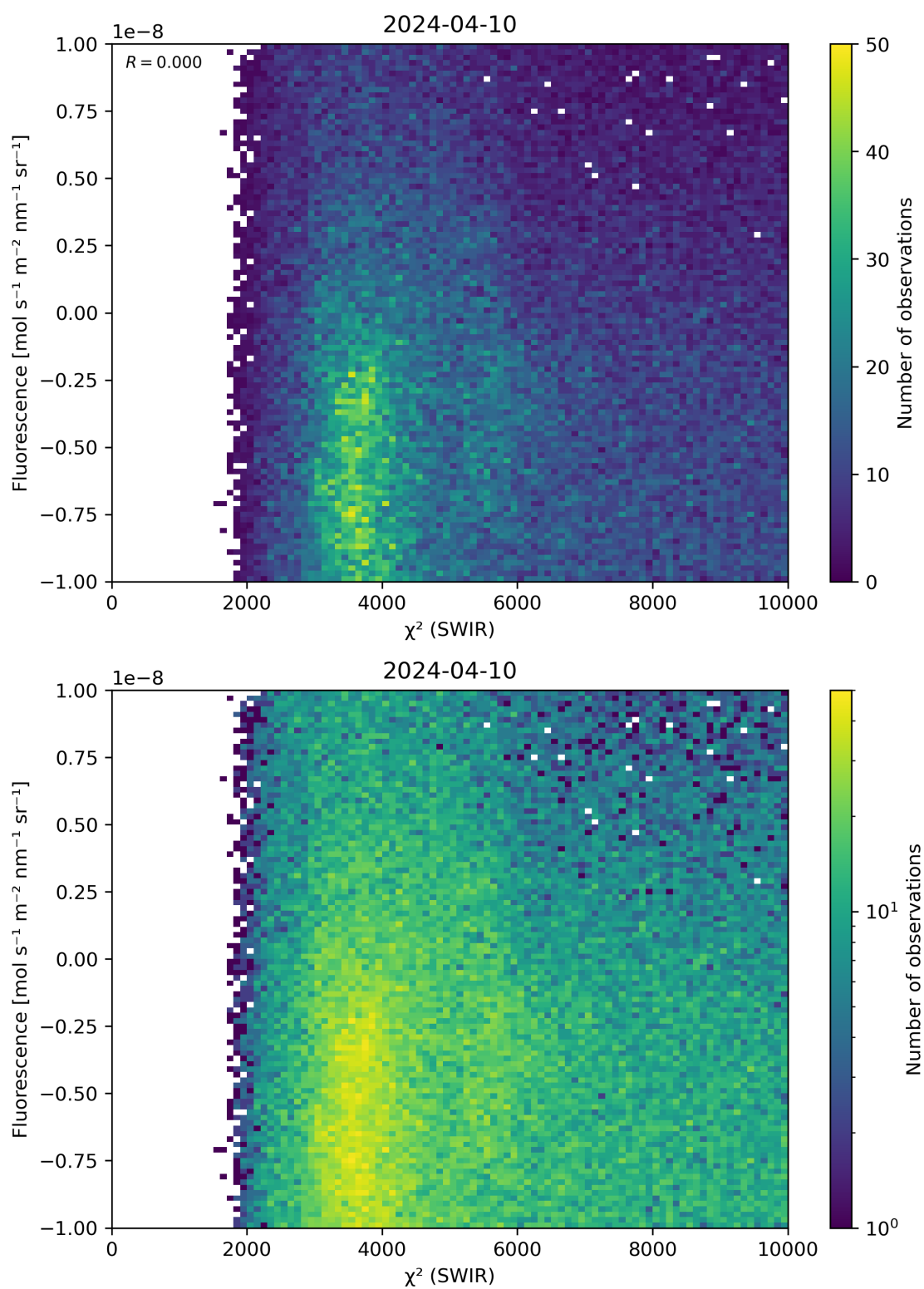
Figure 49: Scatter density plot of “ \chi^2 (SWIR)” against “Fluorescence” for 2024-04-10 to 2024-04-11.
