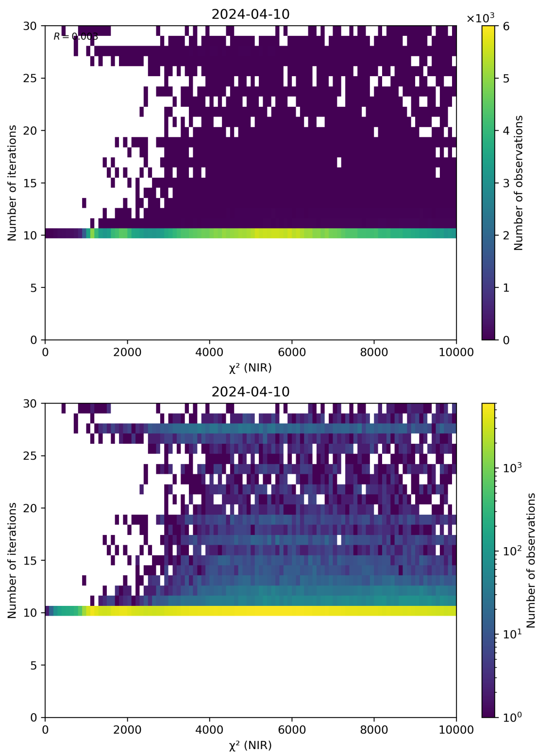
Figure 46: Scatter density plot of “ \chi^2 (NIR)” against “Number of iterations” for 2024-04-10 to 2024-04-11.
