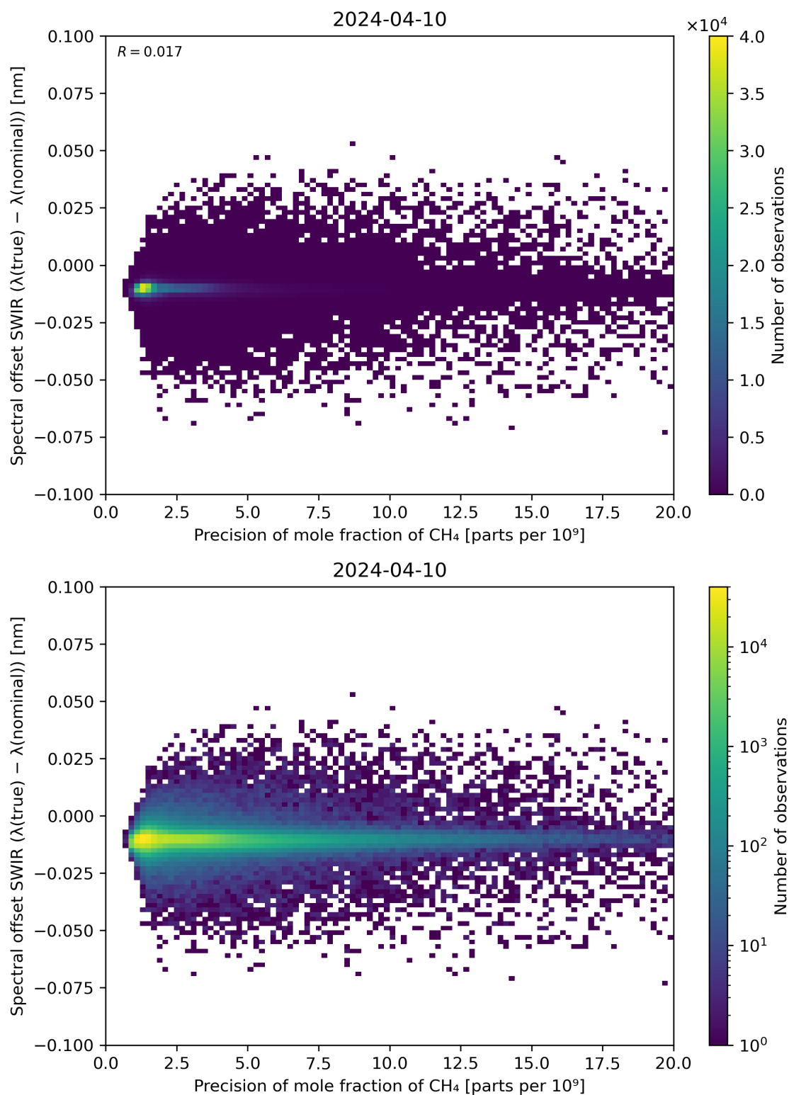
Figure 85: Scatter density plot of “Precision of mole fraction of \text{CH}_4 ” against “Spectral offset SWIR ( \lambda(\text{true}) - \lambda(\text{nominal}) )” for 2024-04-10 to 2024-04-11.
