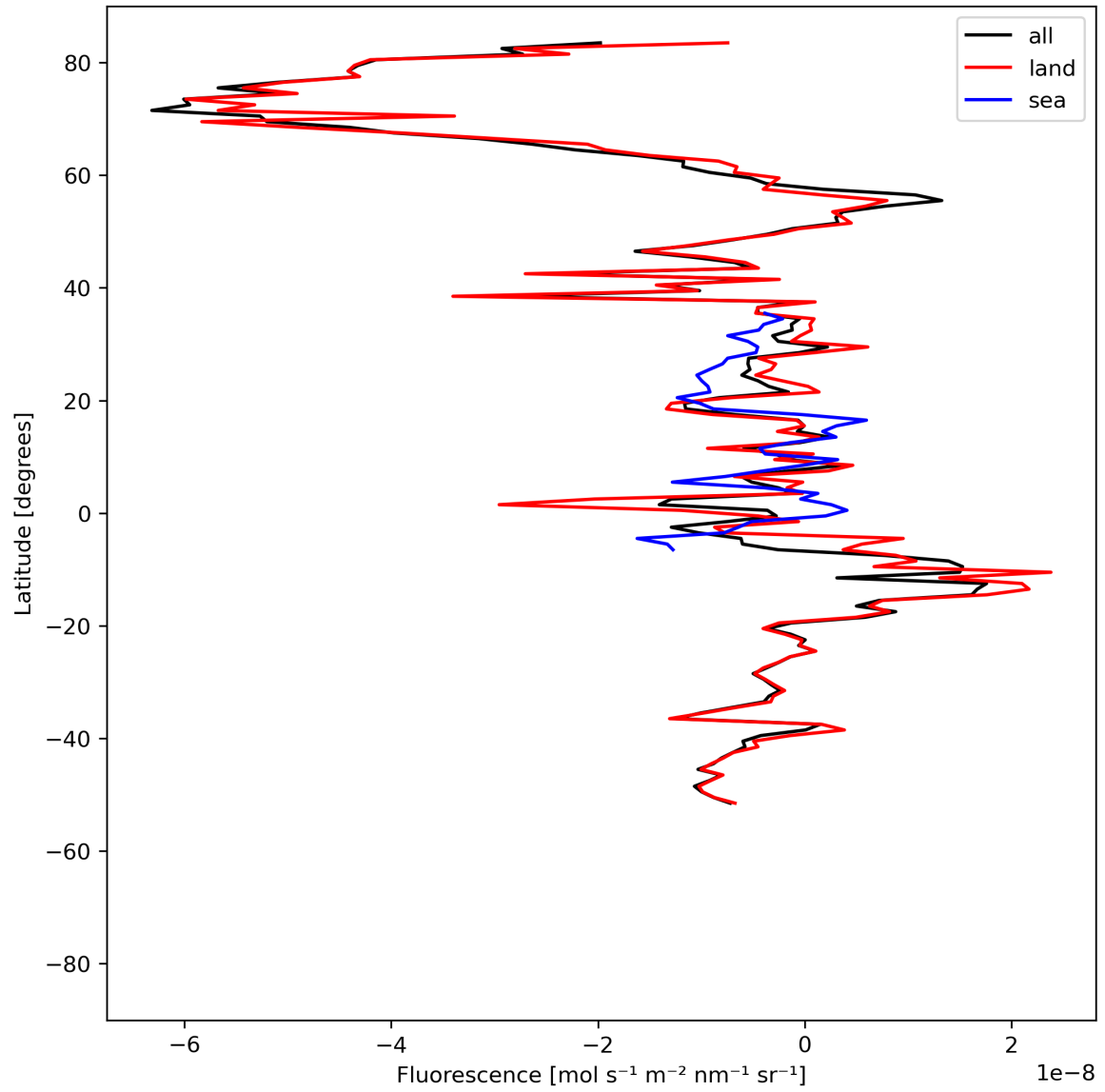
Figure 21: Zonal average of “Fluorescence” for 2024-04-10 to 2024-04-11.
