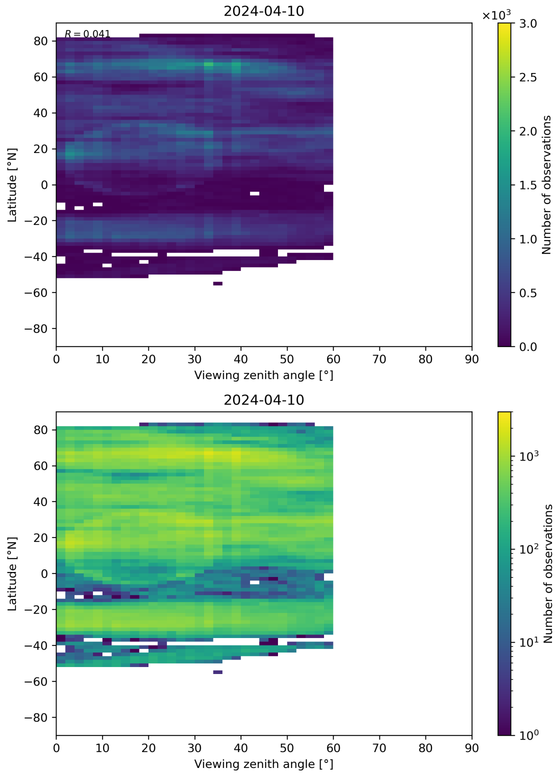
Figure 109: Scatter density plot of “Viewing zenith angle” against “Latitude” for 2024-04-10 to 2024-04-11.
