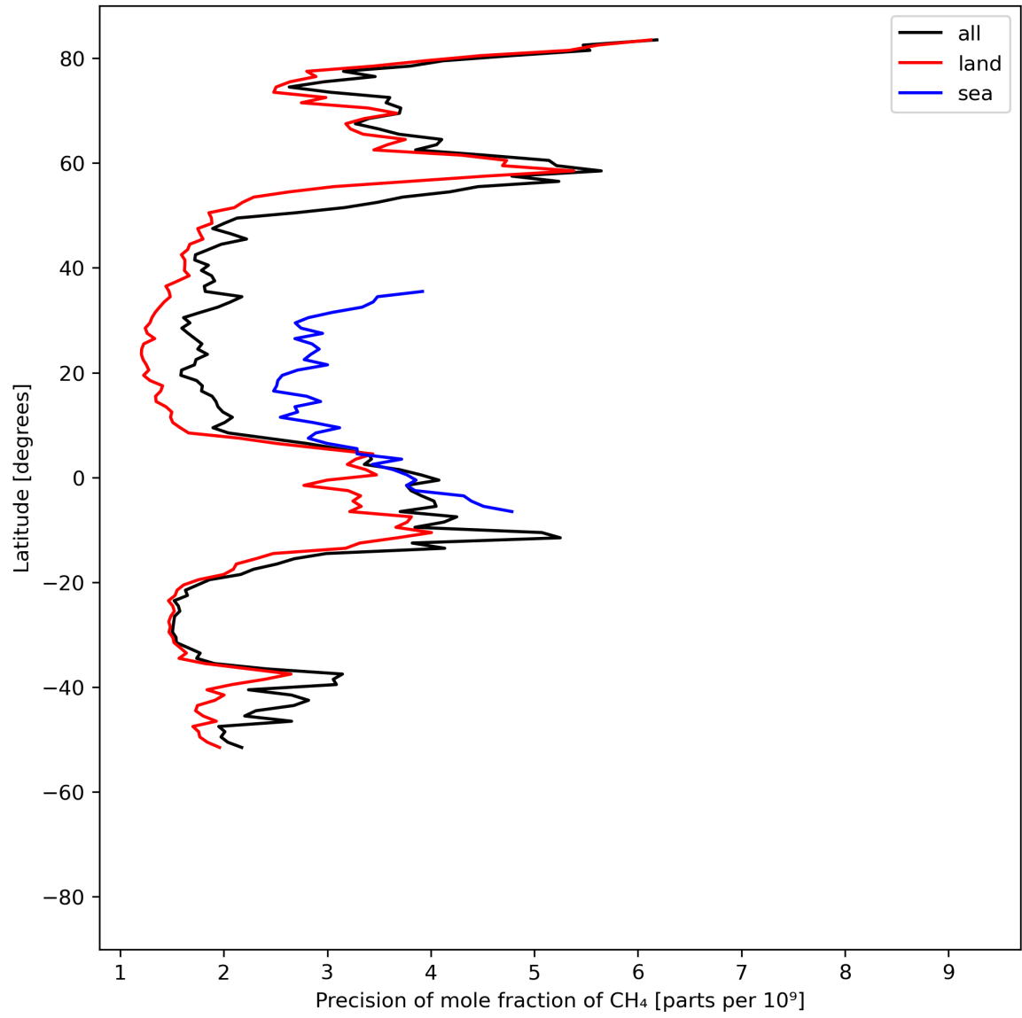
Figure 13: Zonal average of “Precision of mole fraction of CH 4 ” for 2024-04-10 to 2024-04-11.
