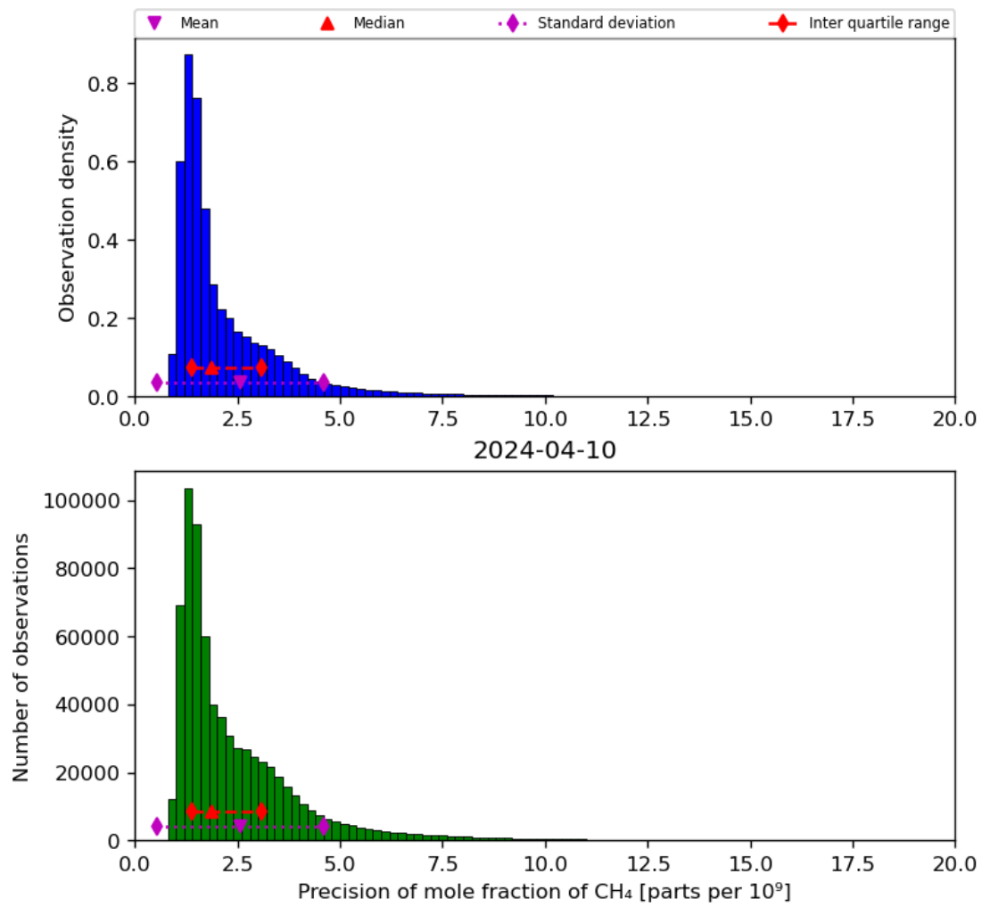
Figure 24: Histogram of “Precision of mole fraction of CH 4 ” for 2024-04-10 to 2024-04-11
