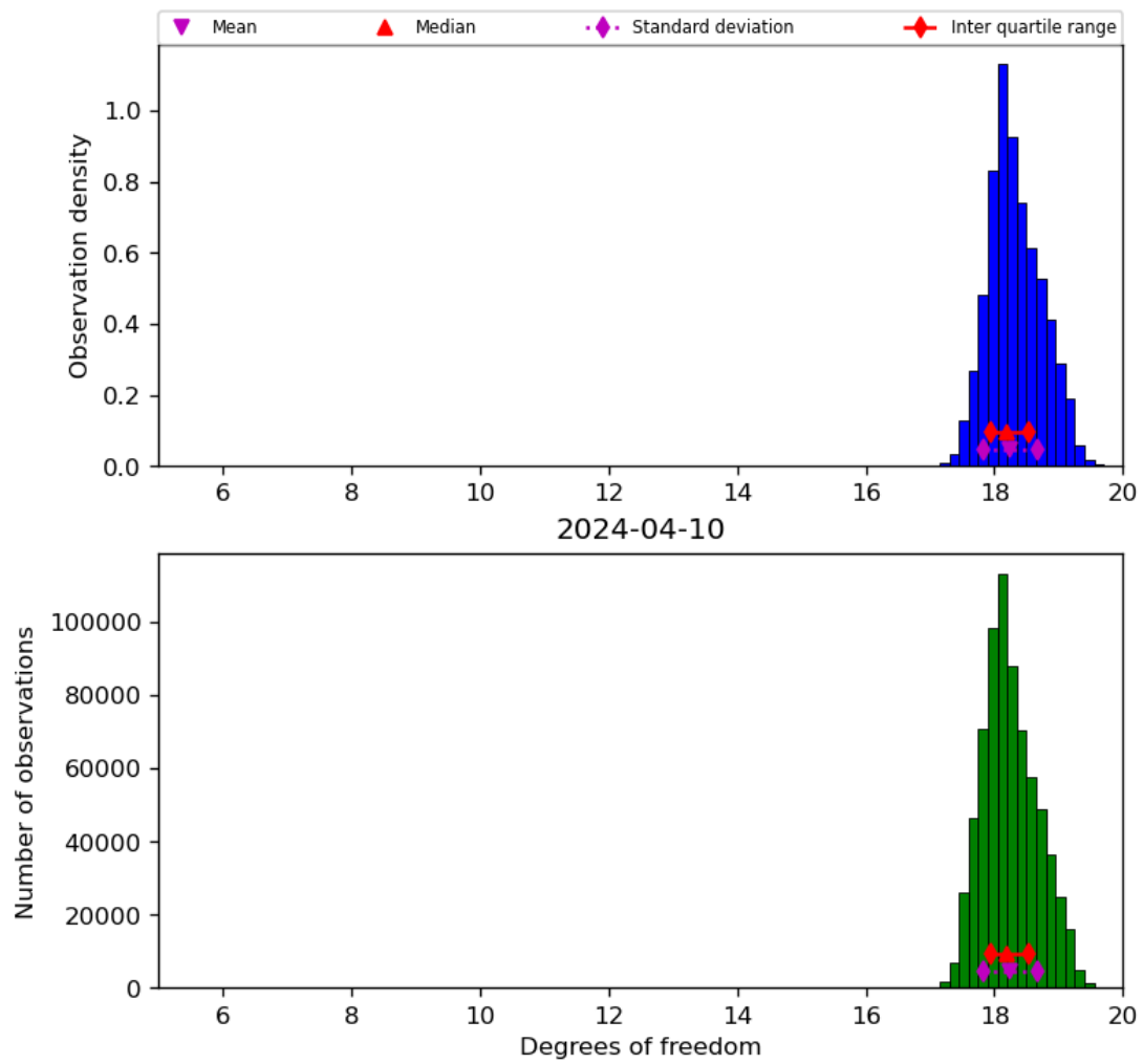
Figure 30: Histogram of “Degrees of freedom” for 2024-04-10 to 2024-04-11
