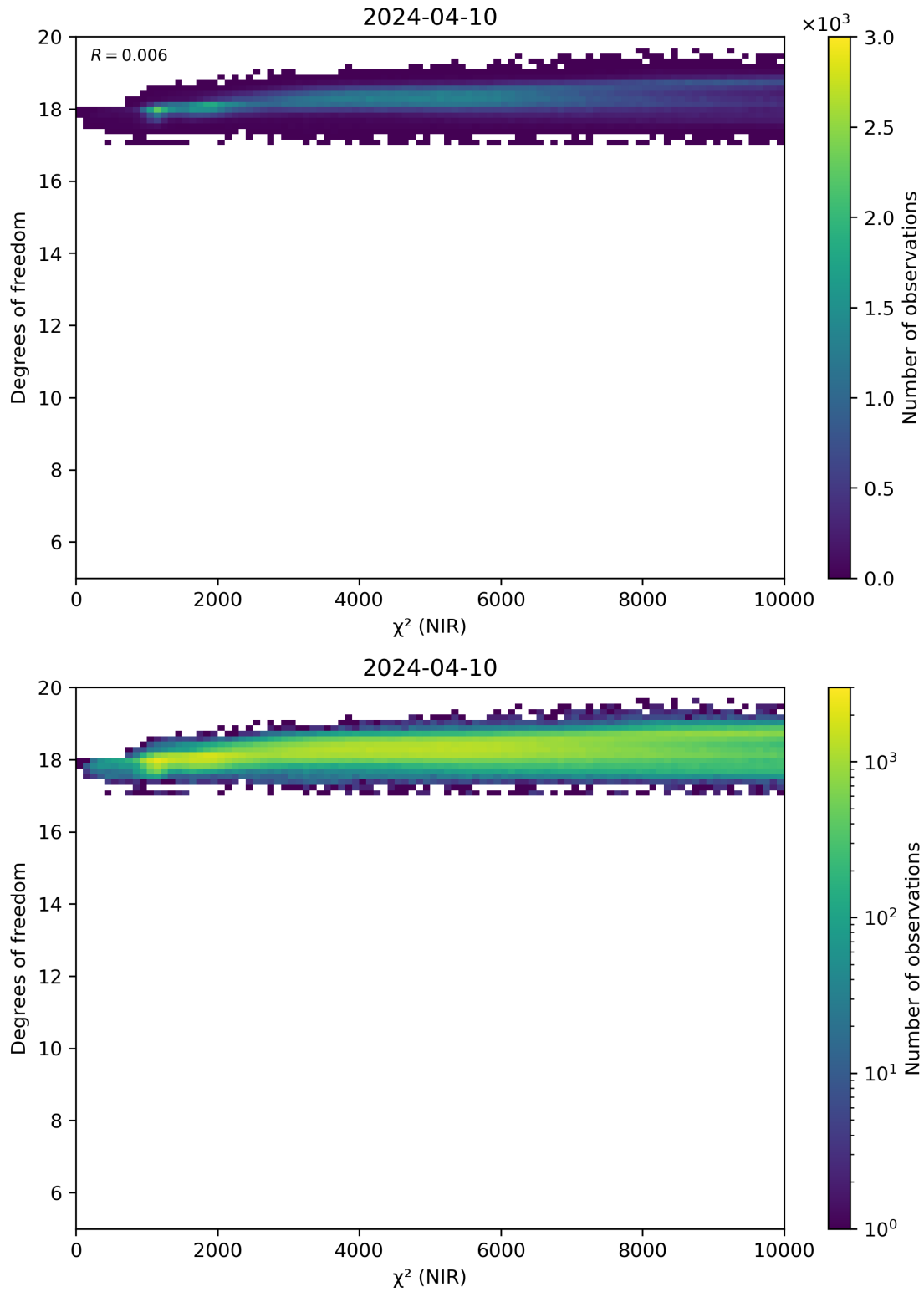
Figure 44: Scatter density plot of “ \chi^2 (NIR)” against “Degrees of freedom” for 2024-04-10 to 2024-04-11.
