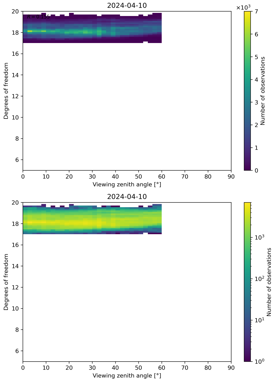
Figure 107: Scatter density plot of “Viewing zenith angle” against “Degrees of freedom” for 2024-04-10 to 2024-04-11.
