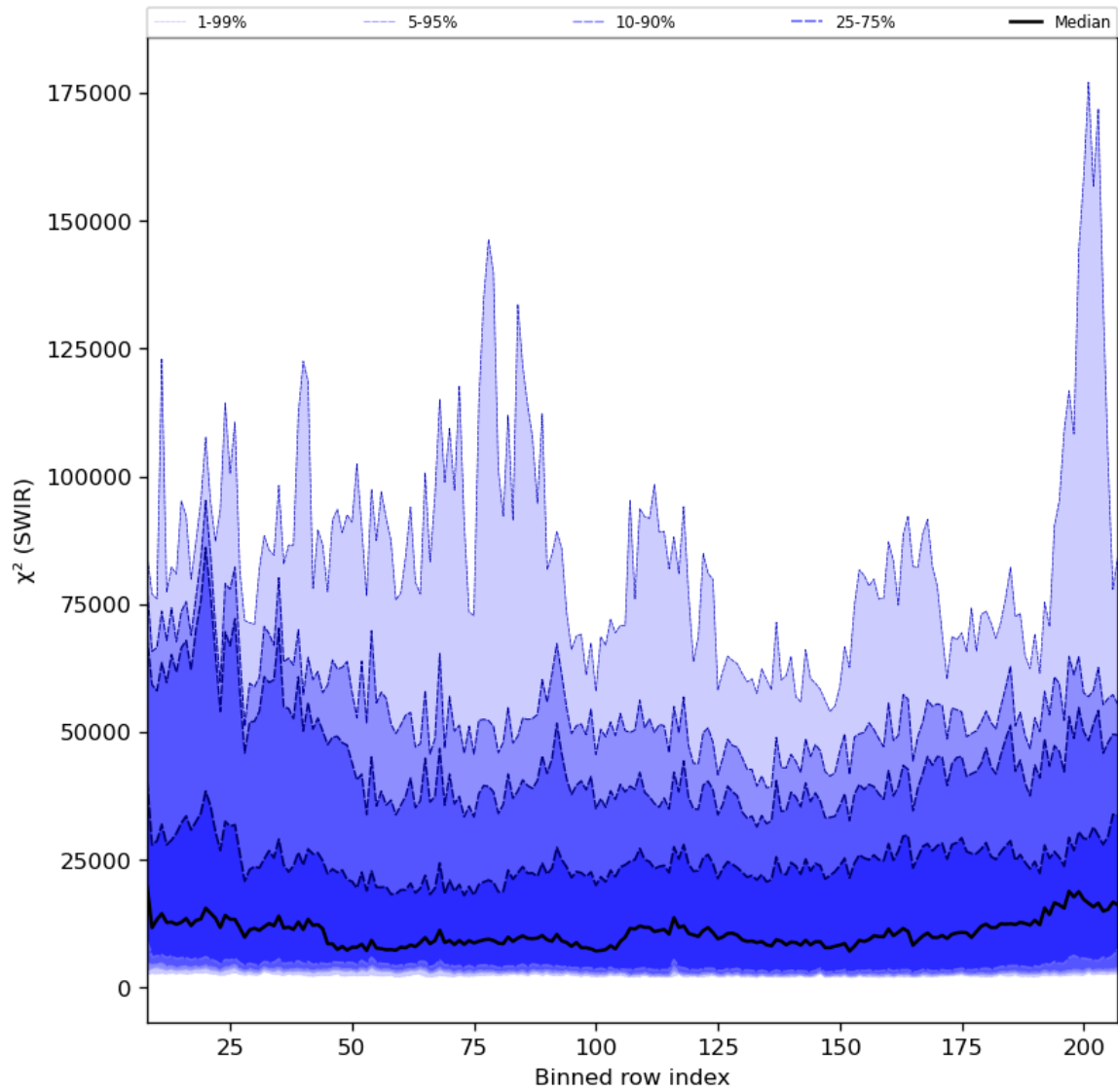
Figure 39: Along track statistics of " \chi^2 (SWIR)" for 2024-04-10 to 2024-04-11
