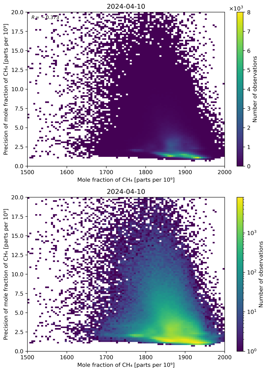
Figure 75: Scatter density plot of “Mole fraction of CH 4 ” against “Precision of mole fraction of CH 4 ” for 2024-04-10 to 2024-04-11.
