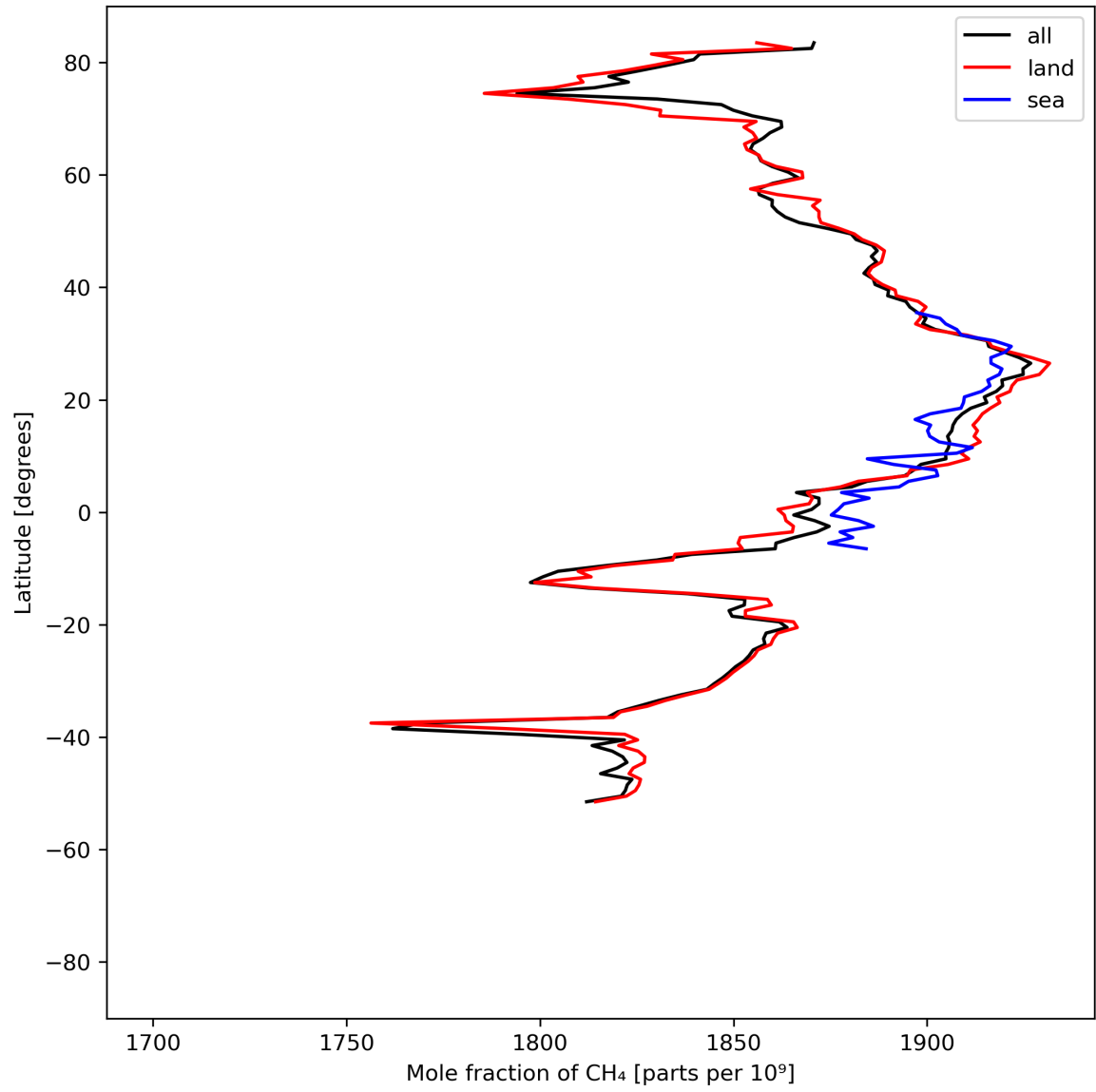
Figure 12: Zonal average of “Mole fraction of \text{CH}_4 ” for 2024-04-10 to 2024-04-11.
