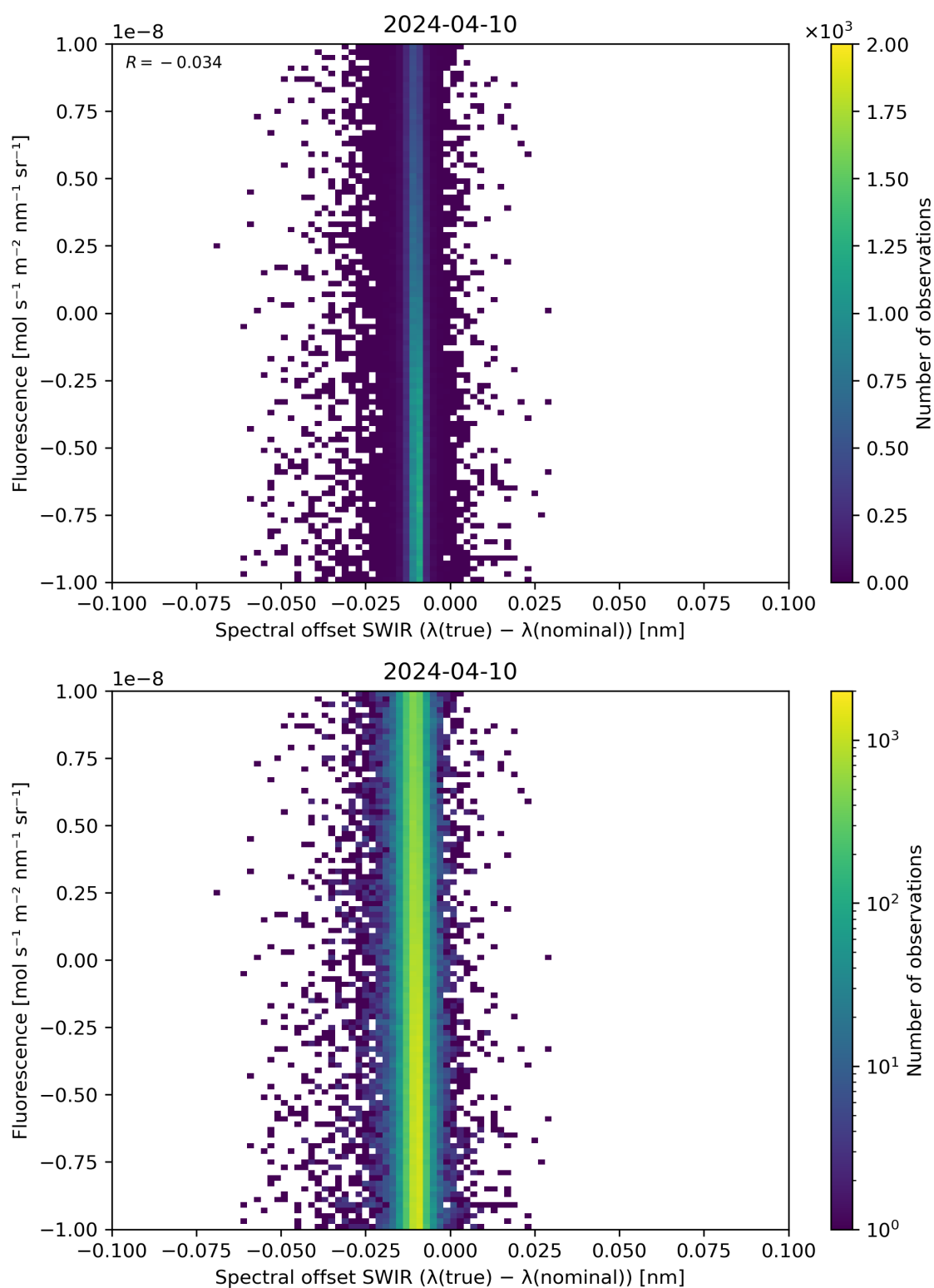
Figure 120: Scatter density plot of “Spectral offset SWIR ( \lambda(\text{true}) - \lambda(\text{nominal}) )” against “Fluorescence” for 2024-04-10 to 2024-04-11.
