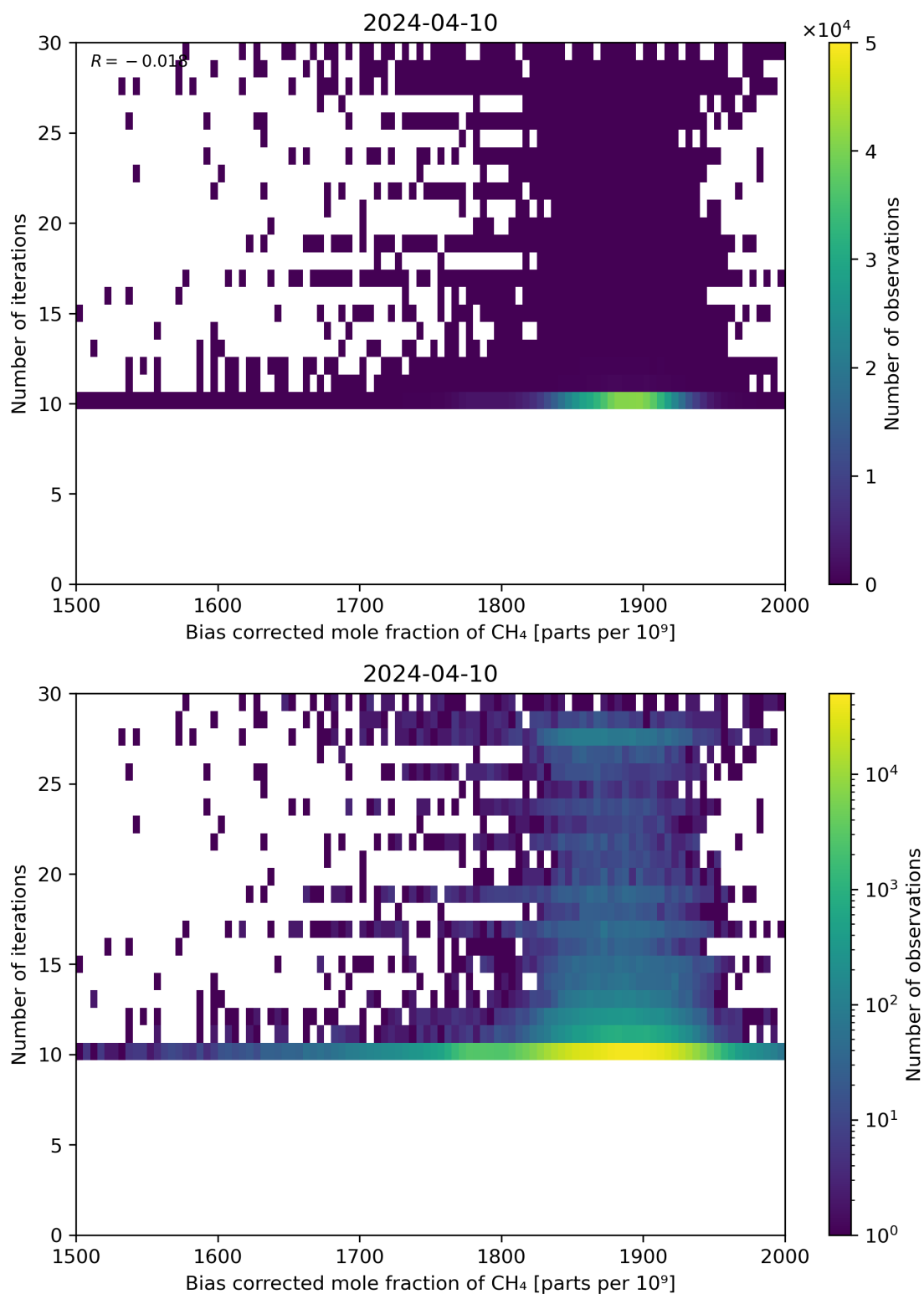
Figure 67: Scatter density plot of “Bias corrected mole fraction of CH 4 ” against “Number of iterations” for 2024-04-10 to 2024-04-11.
