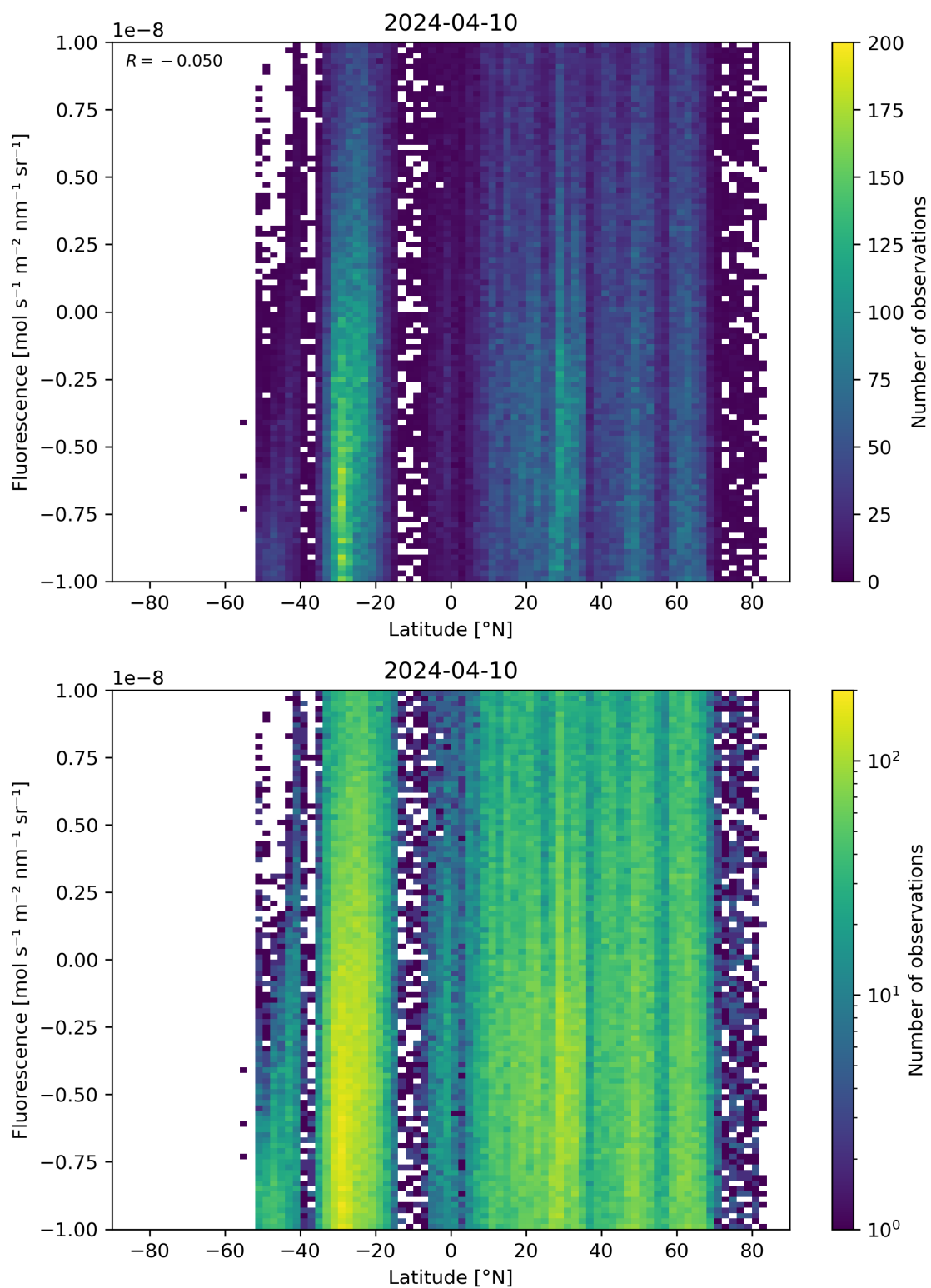
Figure 56: Scatter density plot of “Latitude” against “Fluorescence” for 2024-04-10 to 2024-04-11.
