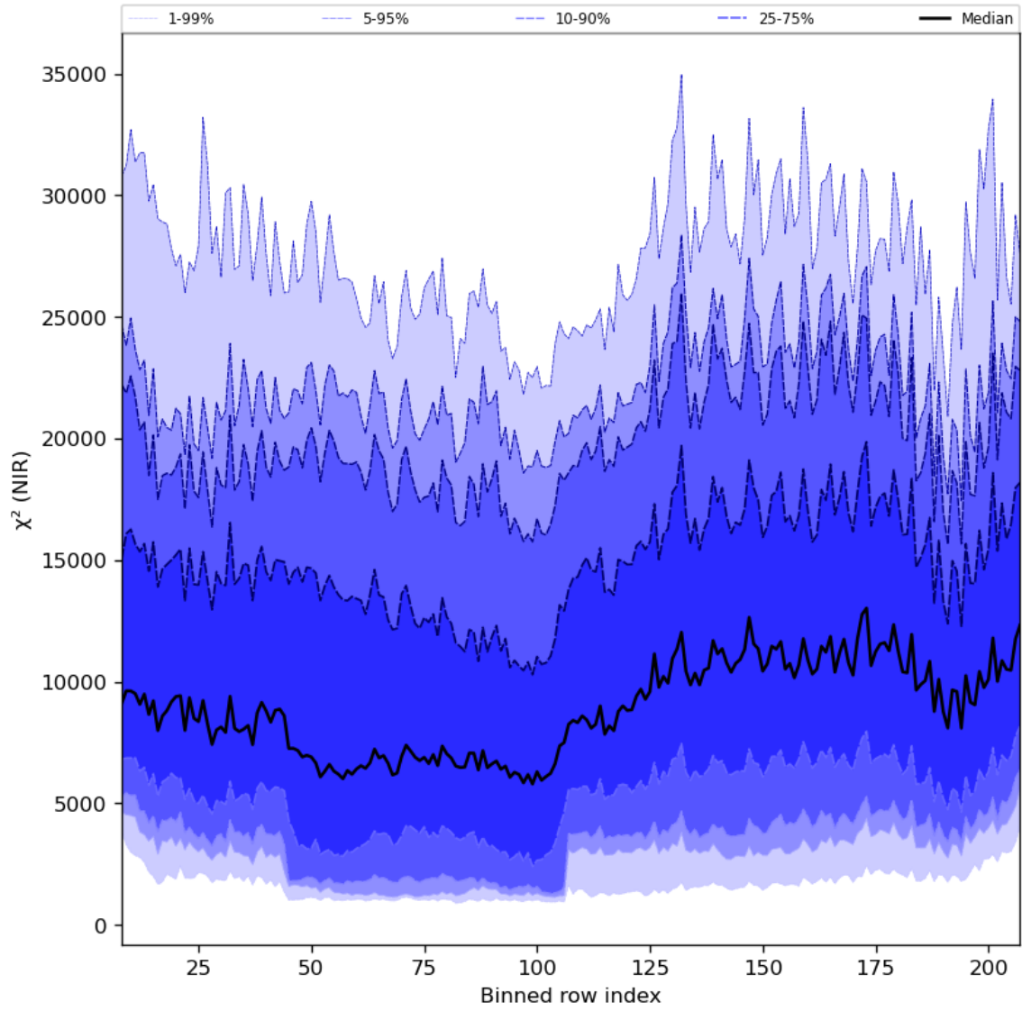
Figure 40: Along track statistics of " \chi^2 (NIR)" for 2024-04-10 to 2024-04-11
