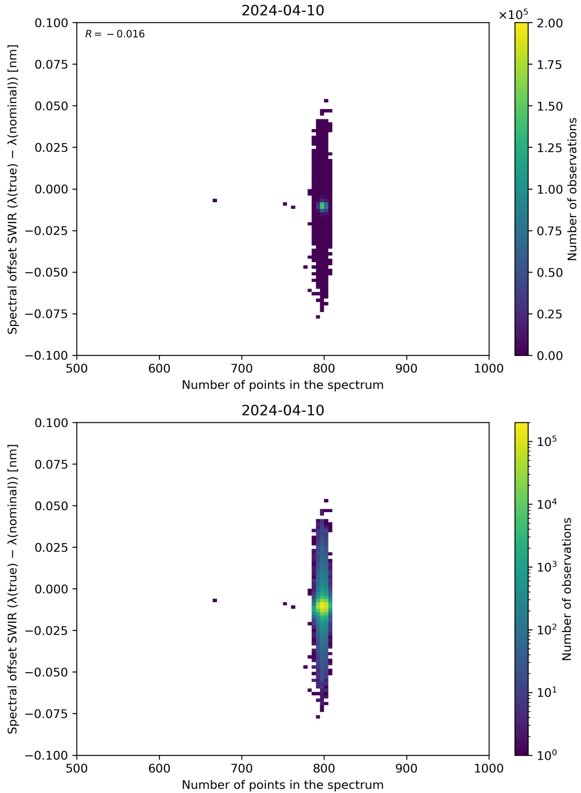
Figure 93: Scatter density plot of “Number of points in the spectrum” against “Spectral offset SWIR ( \lambda(\text{true}) - \lambda(\text{nominal}) )” for 2024-04-10 to 2024-04-11.
