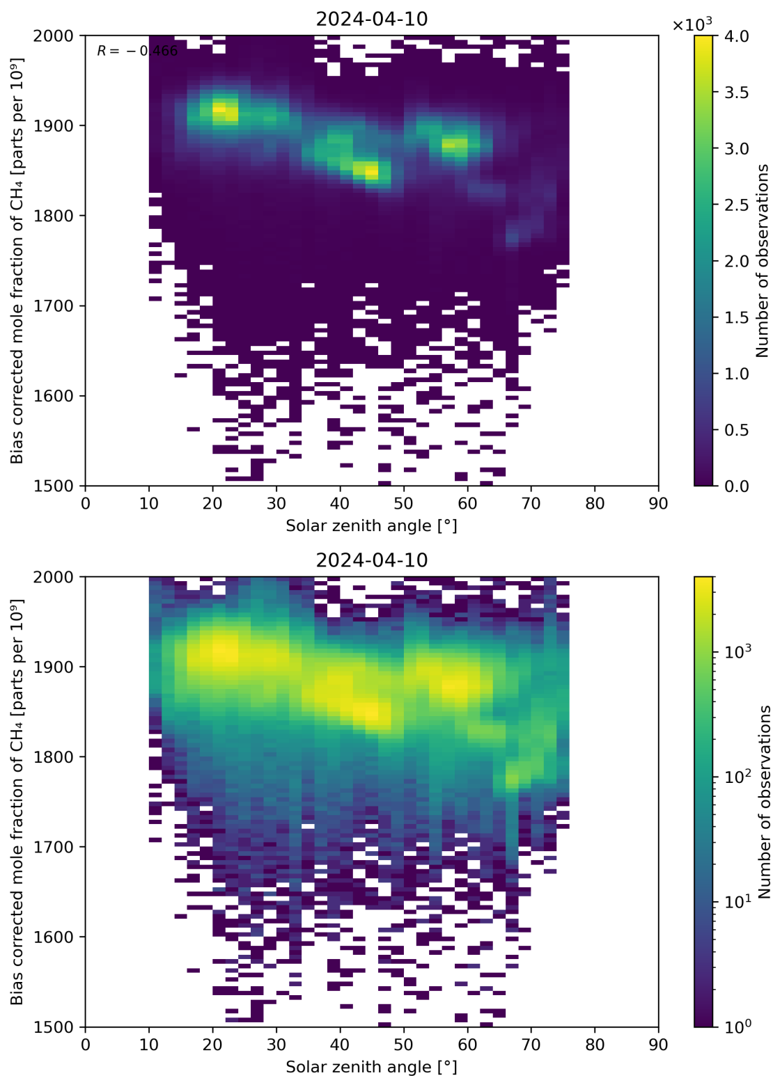
Figure 100: Scatter density plot of “Solar zenith angle” against “Bias corrected mole fraction of CH 4 ” for 2024-04-10 to 2024-04-11.
