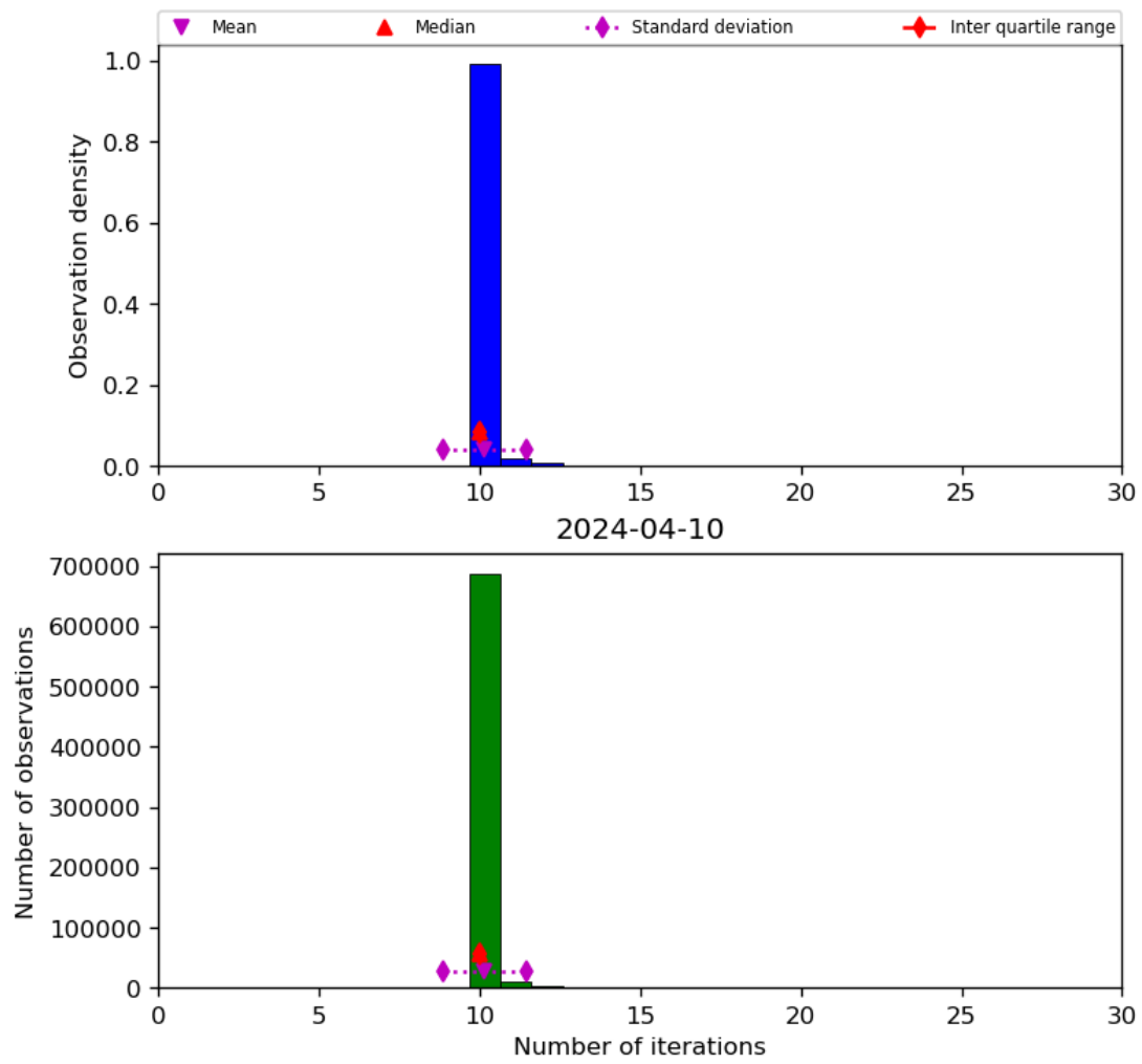
Figure 31: Histogram of “Number of iterations” for 2024-04-10 to 2024-04-11
