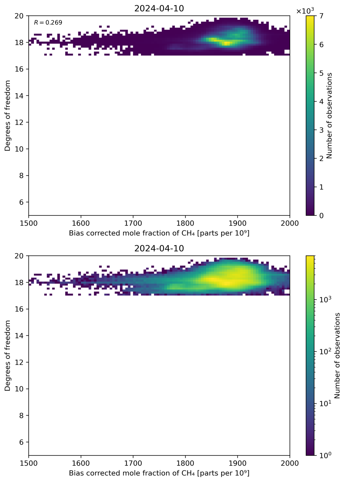
Figure 65: Scatter density plot of “Bias corrected mole fraction of CH 4 ” against “Degrees of freedom” for 2024-04-10 to 2024-04-11.
