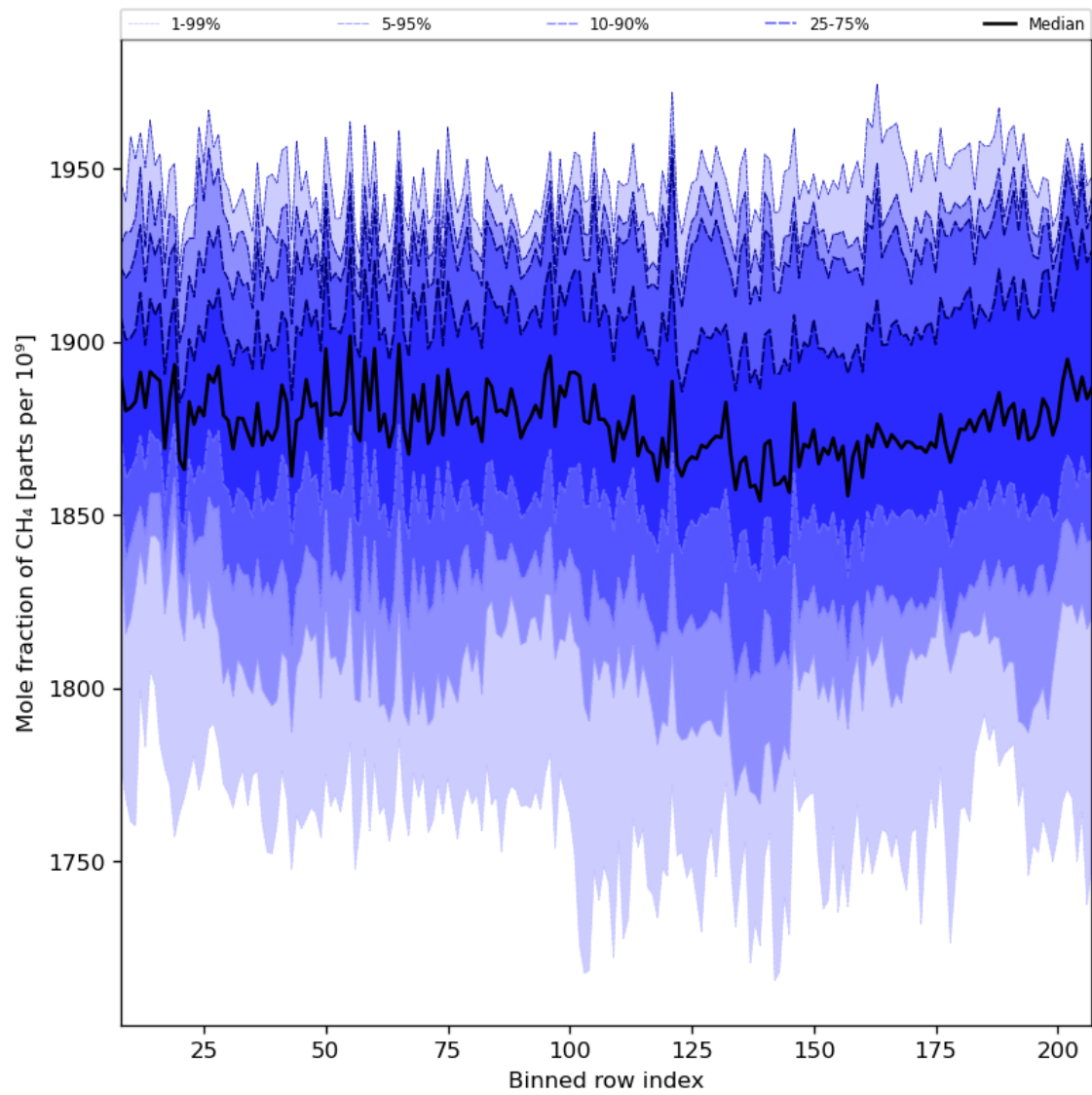
Figure 34: Along track statistics of “Mole fraction of CH 4 ” for 2024-04-10 to 2024-04-11
