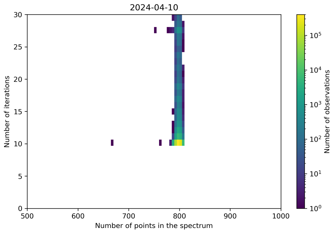
Figure 92: Scatter density plot of “Number of points in the spectrum” against “Number of iterations” for 2024-04-10 to 2024-04-11.
