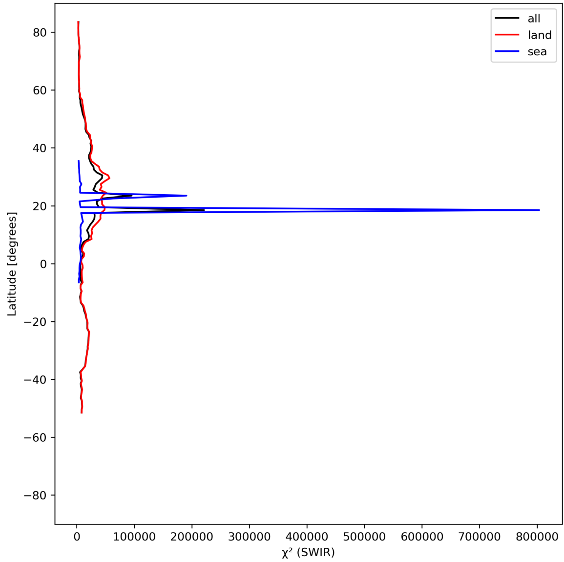
Figure 17: Zonal average of “ \chi^2 (SWIR)” for 2024-04-10 to 2024-04-11.
