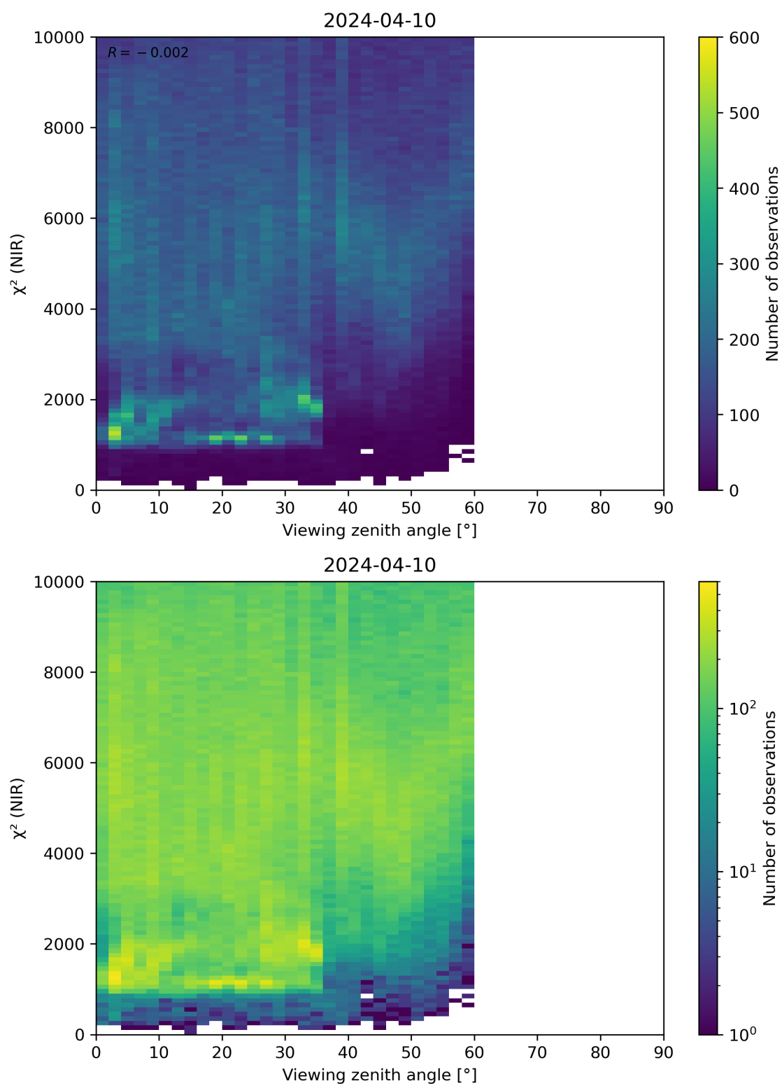
Figure 105: Scatter density plot of “Viewing zenith angle” against “ \chi^2 (NIR)” for 2024-04-10 to 2024-04-11.
