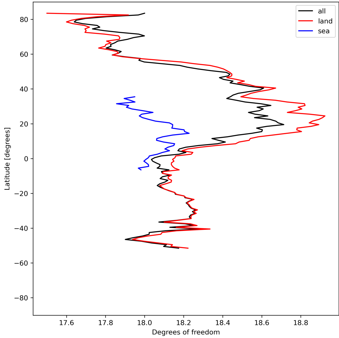
Figure 19: Zonal average of “Degrees of freedom” for 2024-04-10 to 2024-04-11.
