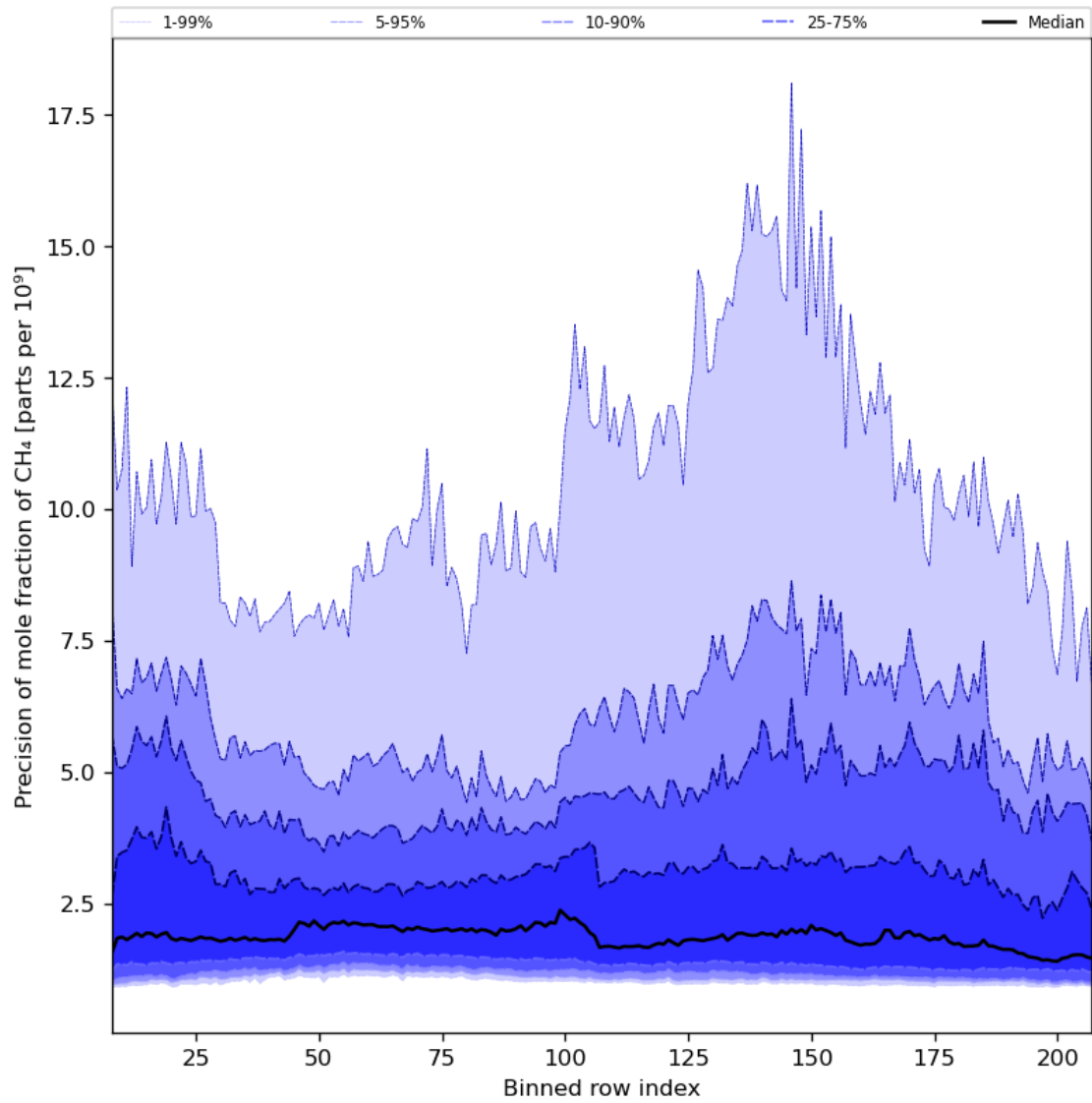
Figure 35: Along track statistics of “Precision of mole fraction of CH 4 ” for 2024-04-10 to 2024-04-11
