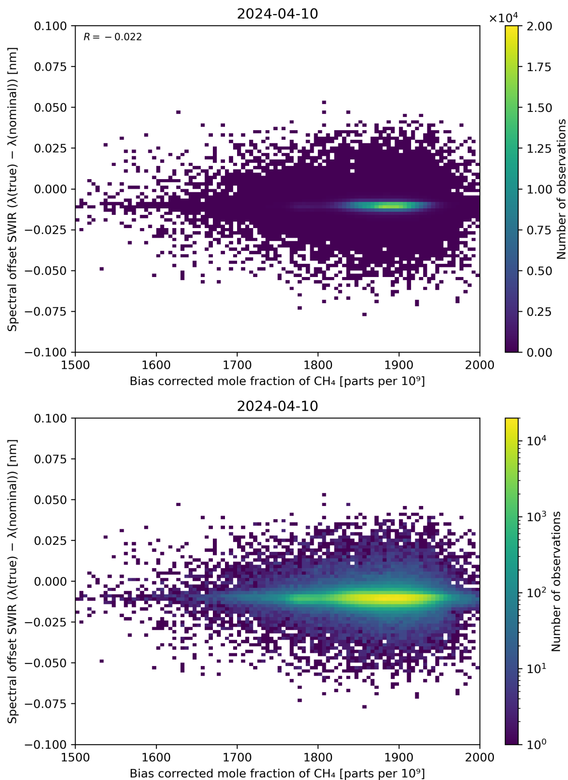
Figure 69: Scatter density plot of “Bias corrected mole fraction of \text{CH}_4 ” against “Spectral offset SWIR ( \lambda(\text{true}) - \lambda(\text{nominal}) )” for 2024-04-10 to 2024-04-11.
