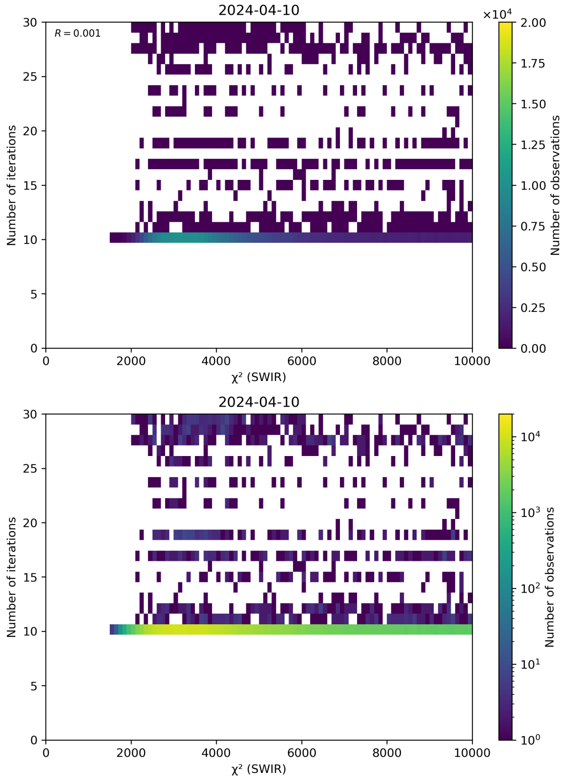
Figure 50: Scatter density plot of “ \chi^2 (SWIR)” against “Number of iterations” for 2024-04-10 to 2024-04-11.
