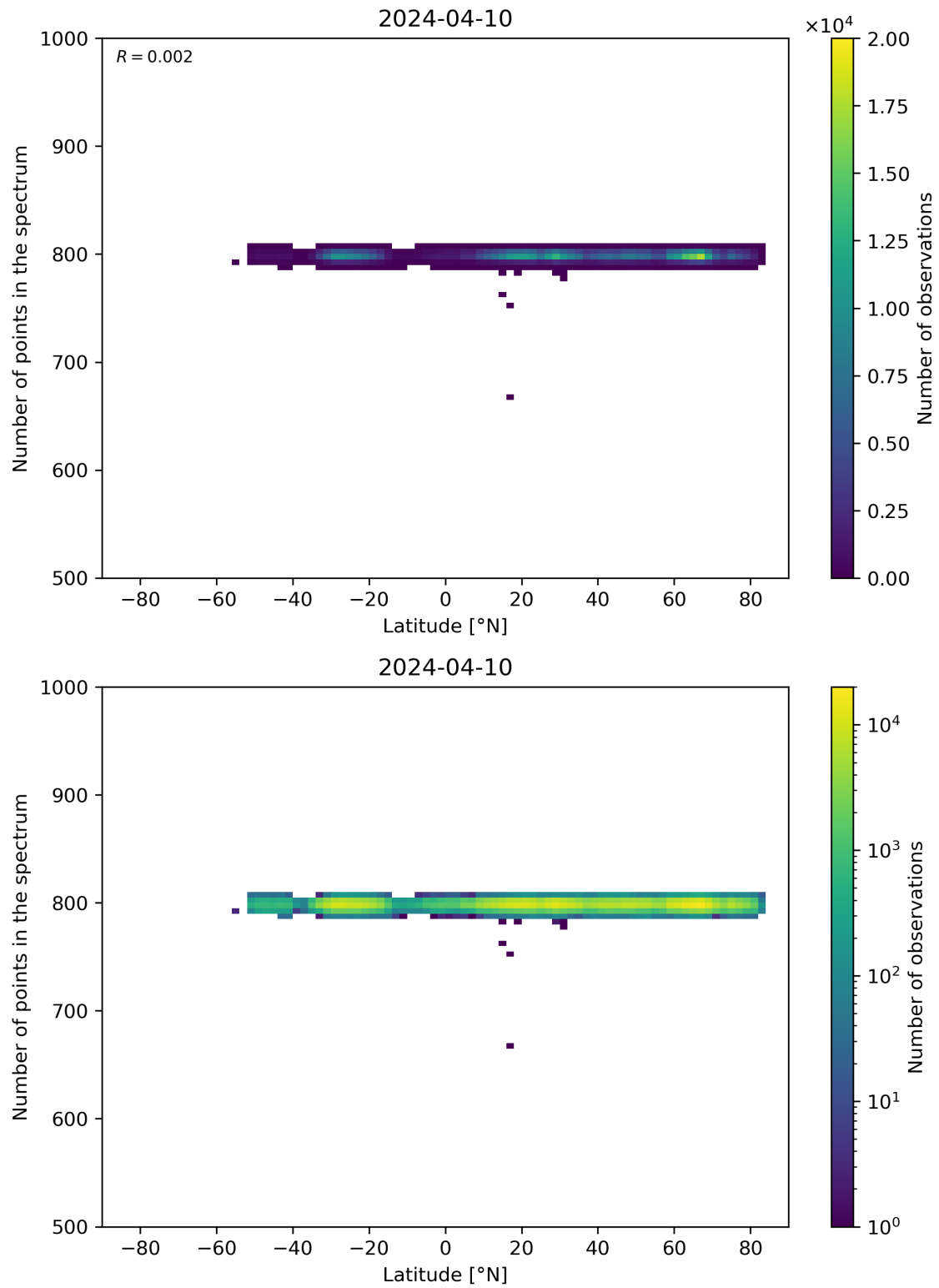
Figure 61: Scatter density plot of “Latitude” against “Number of points in the spectrum” for 2024-04-10 to 2024-04-11.
