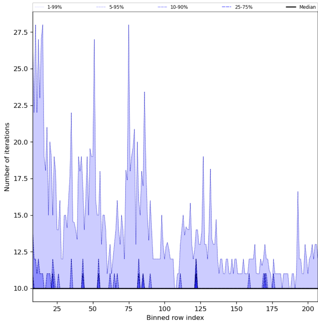
Figure 42: Along track statistics of “Number of iterations” for 2024-04-10 to 2024-04-11
