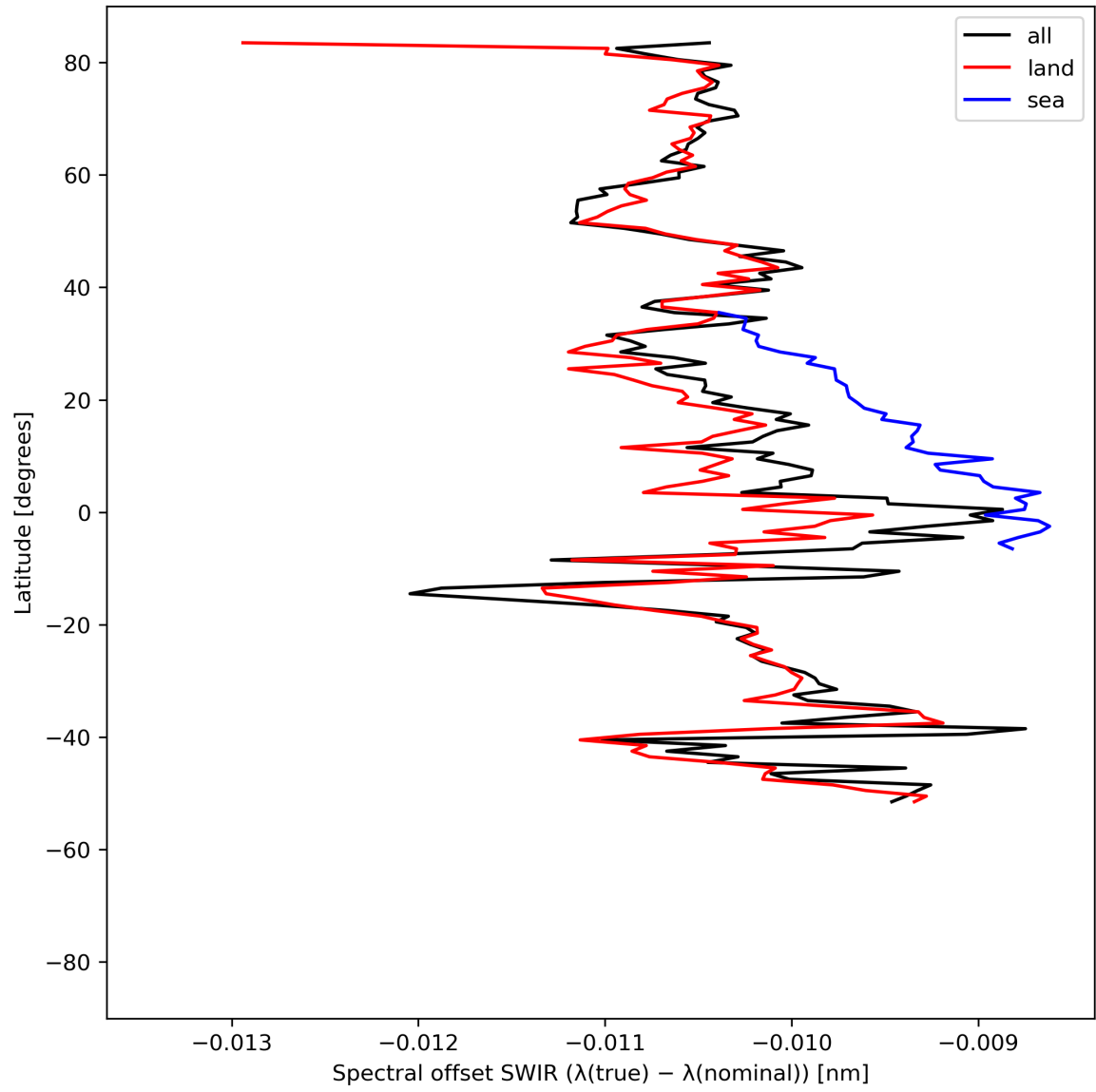
Figure 16: Zonal average of “Spectral offset SWIR ( \lambda(\text{true}) - \lambda(\text{nominal}) )” for 2024-04-10 to 2024-04-11.
