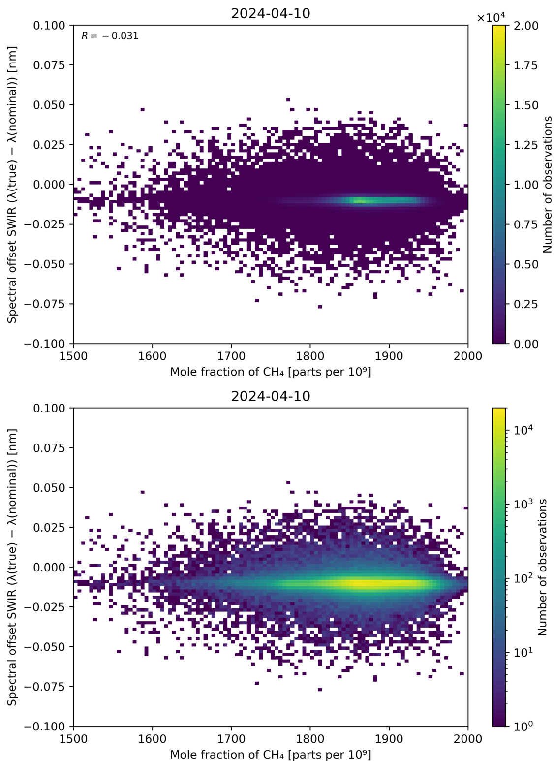
Figure 86: Scatter density plot of “Mole fraction of CH 4 ” against “Spectral offset SWIR ( \lambda(\text{true}) - \lambda(\text{nominal}) )” for 2024-04-10 to 2024-04-11.
