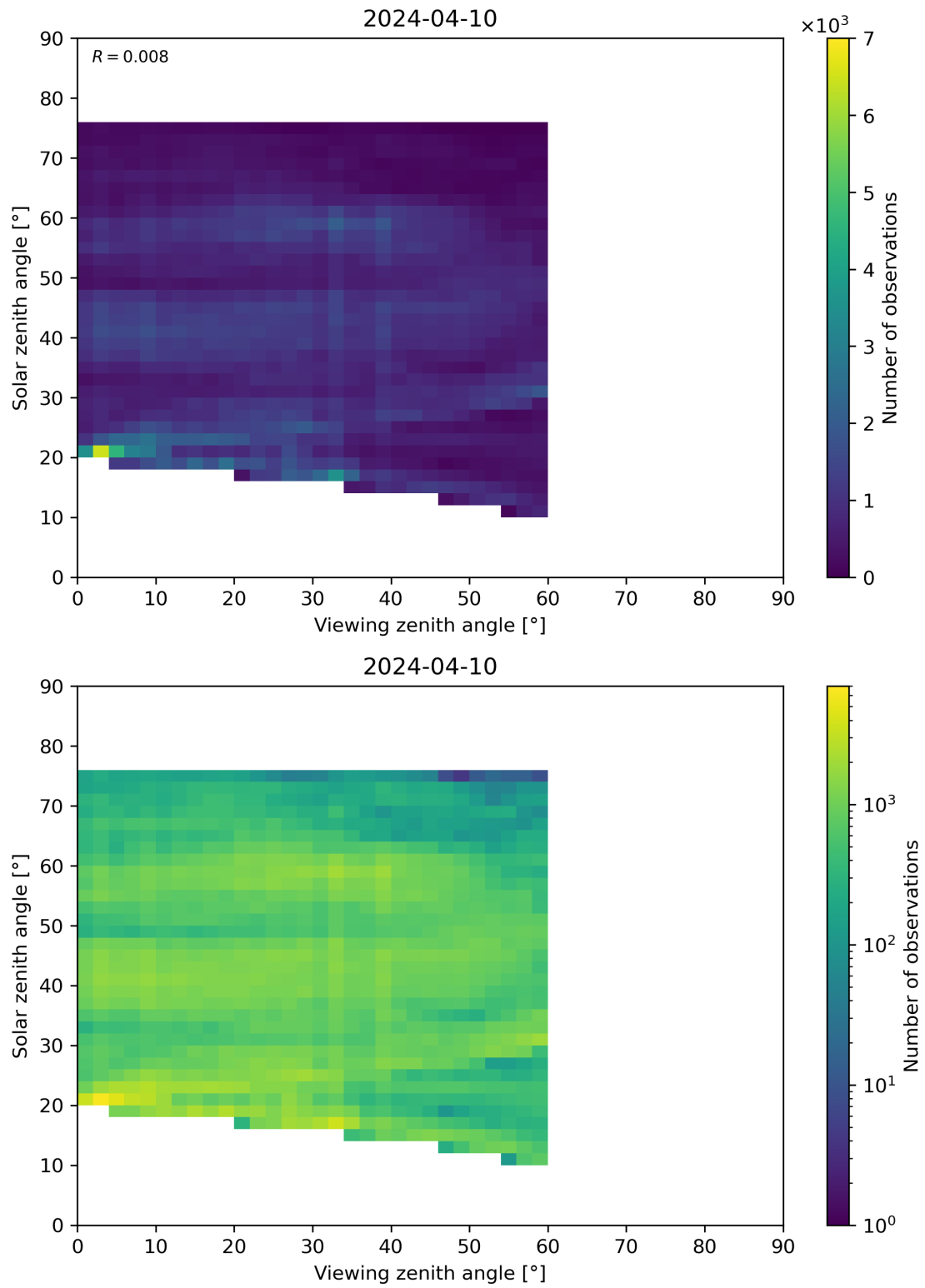
Figure 115: Scatter density plot of “Viewing zenith angle” against “Solar zenith angle” for 2024-04-10 to 2024-04-11.
