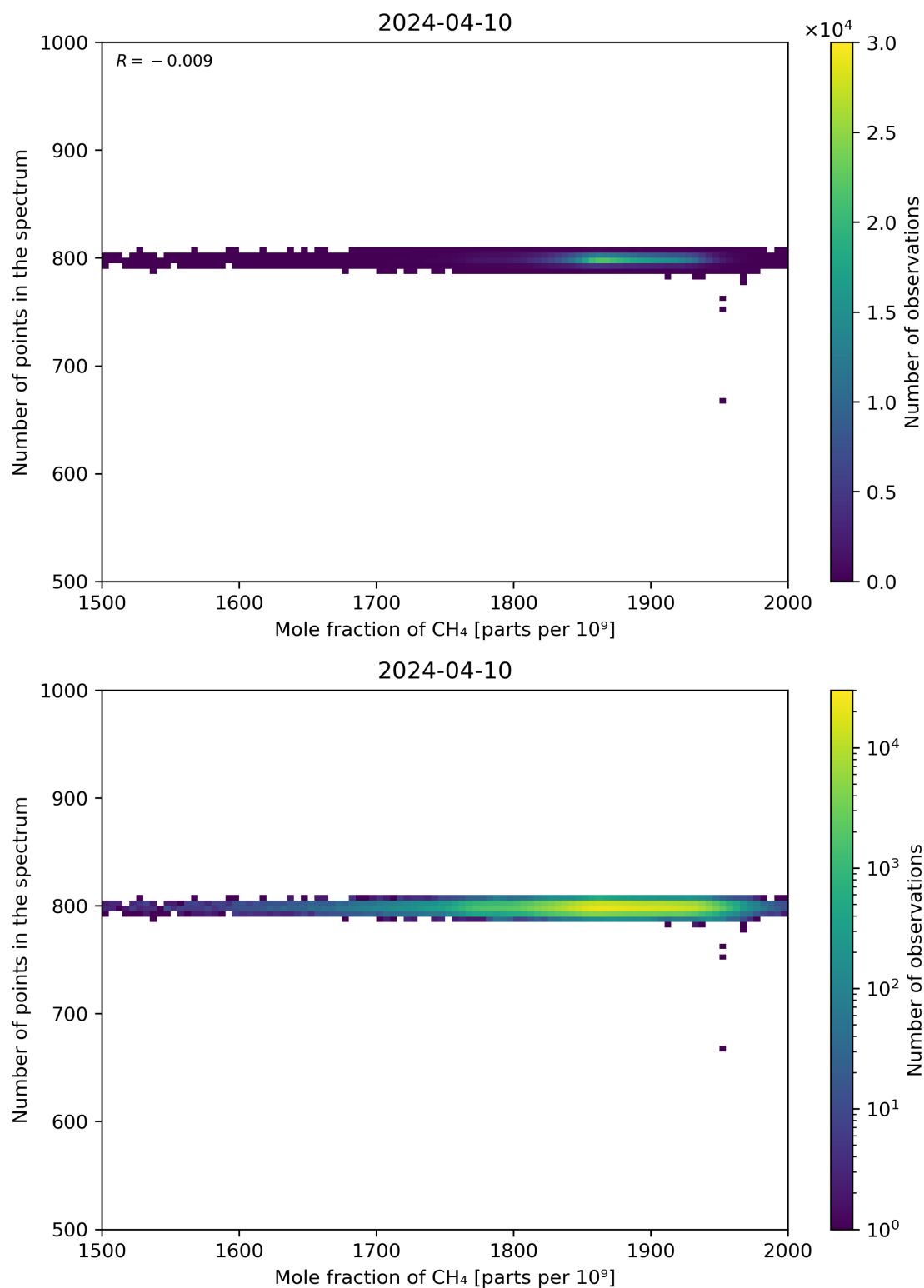
Figure 77: Scatter density plot of “Mole fraction of CH 4 ” against “Number of points in the spectrum” for 2024-04-10 to 2024-04-11.
