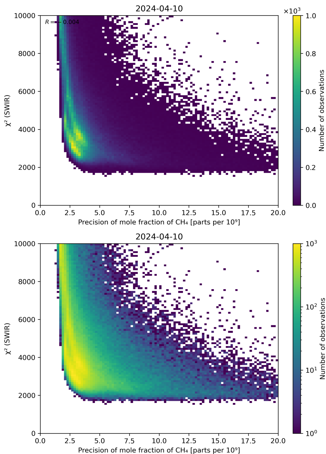
Figure 79: Scatter density plot of “Precision of mole fraction of \text{CH}_4 ” against “ \chi^2 (SWIR)” for 2024-04-10 to 2024-04-11.
