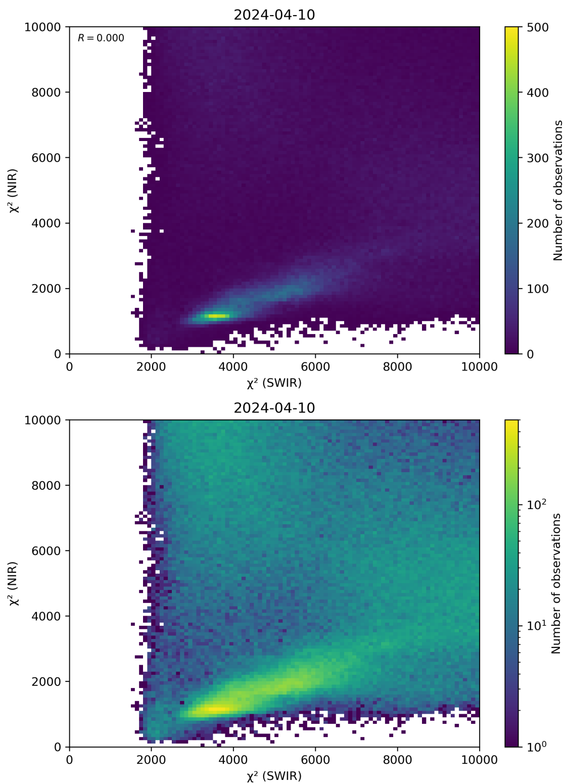
Figure 47: Scatter density plot of “ \chi^2 (SWIR)” against “ \chi^2 (NIR)” for 2024-04-10 to 2024-04-11.
