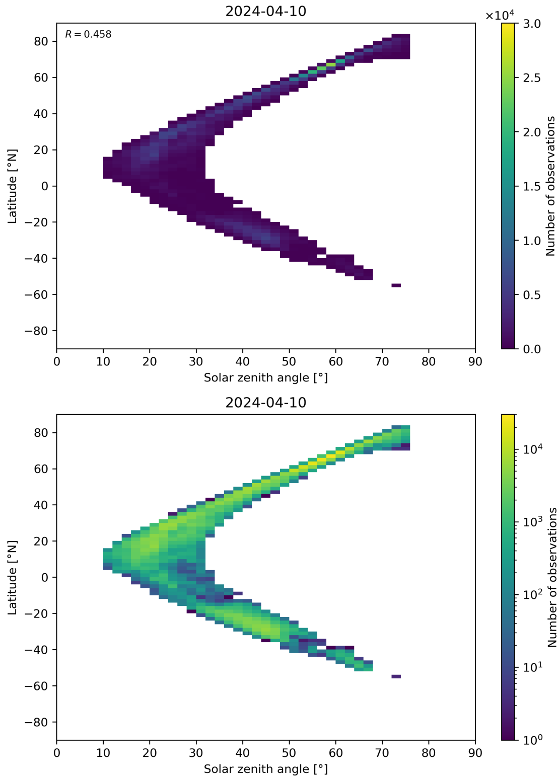
Figure 98: Scatter density plot of “Solar zenith angle” against “Latitude” for 2024-04-10 to 2024-04-11.
