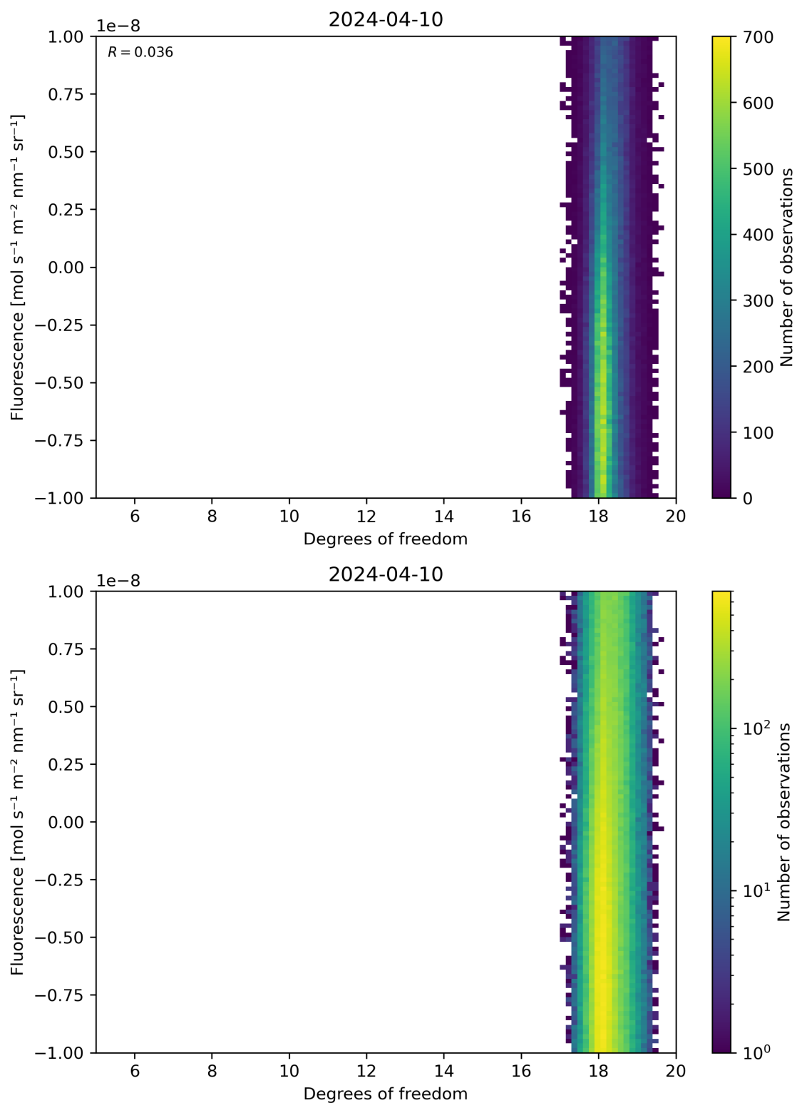
Figure 51: Scatter density plot of “Degrees of freedom” against “Fluorescence” for 2024-04-10 to 2024-04-11.
