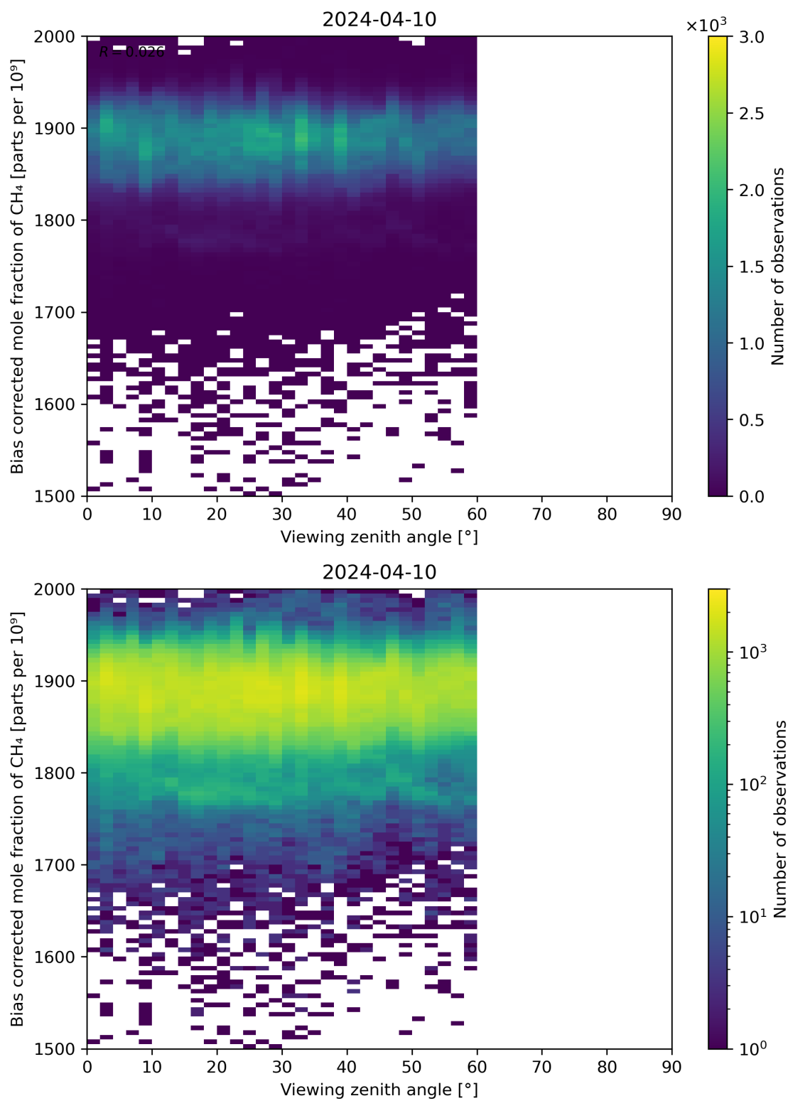
Figure 111: Scatter density plot of “Viewing zenith angle” against “Bias corrected mole fraction of CH 4 ” for 2024-04-10 to 2024-04-11.
