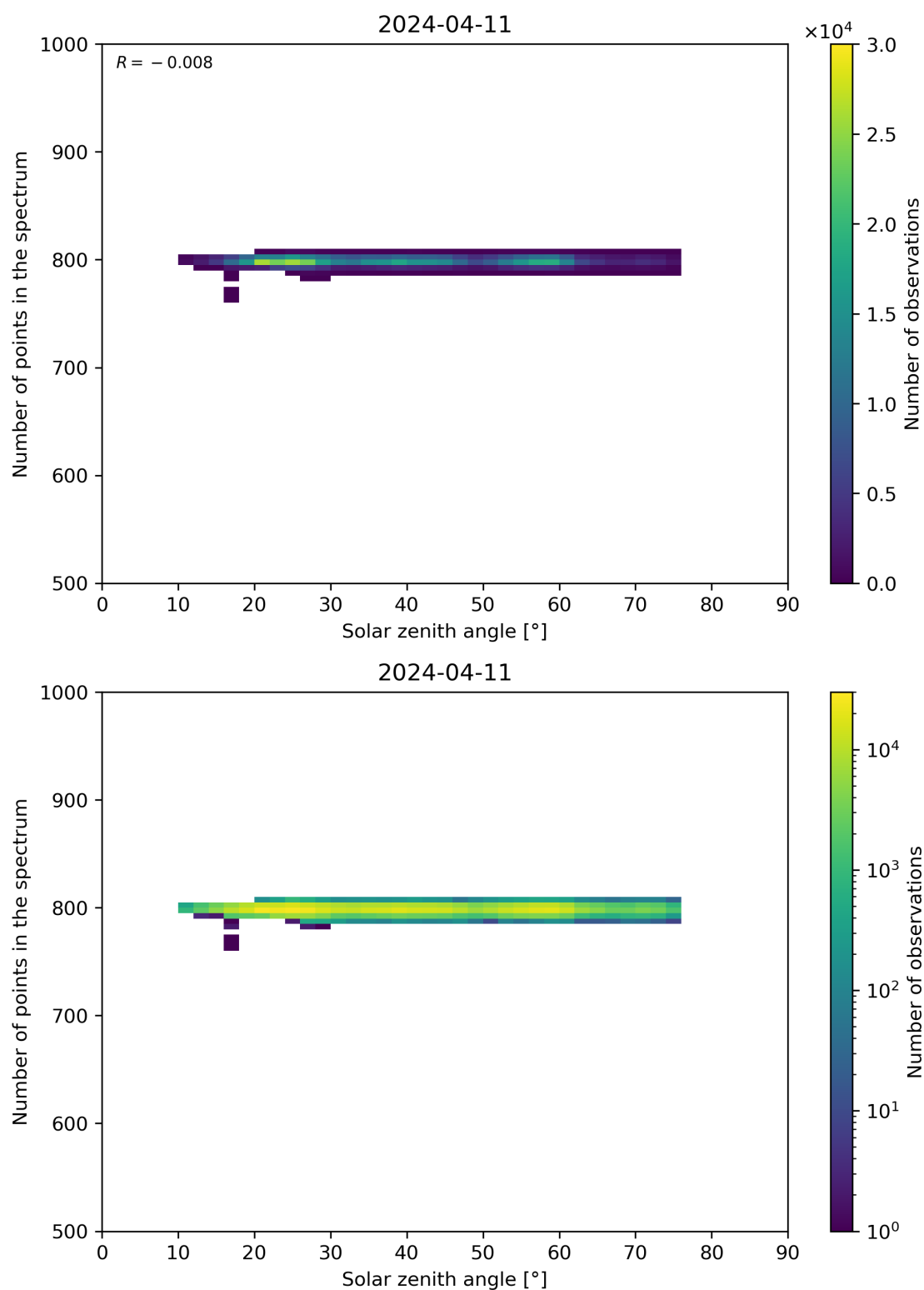
Figure 103: Scatter density plot of “Solar zenith angle” against “Number of points in the spectrum” for 2024-04-10 to 2024-04-12.
