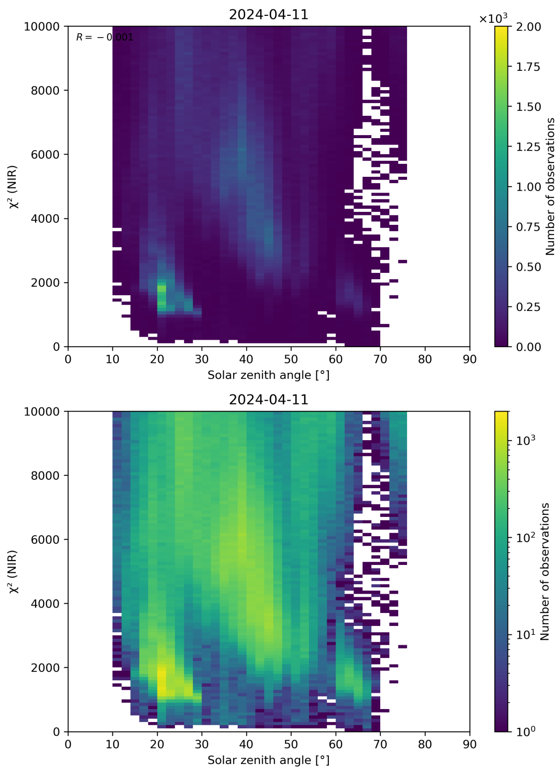
Figure 94: Scatter density plot of “Solar zenith angle” against “ \chi^2 (NIR)” for 2024-04-10 to 2024-04-12.
