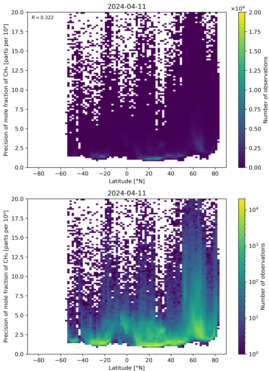
Figure 59: Scatter density plot of “Latitude” against “Precision of mole fraction of CH 4 ” for 2024-04-10 to 2024-04-12.
