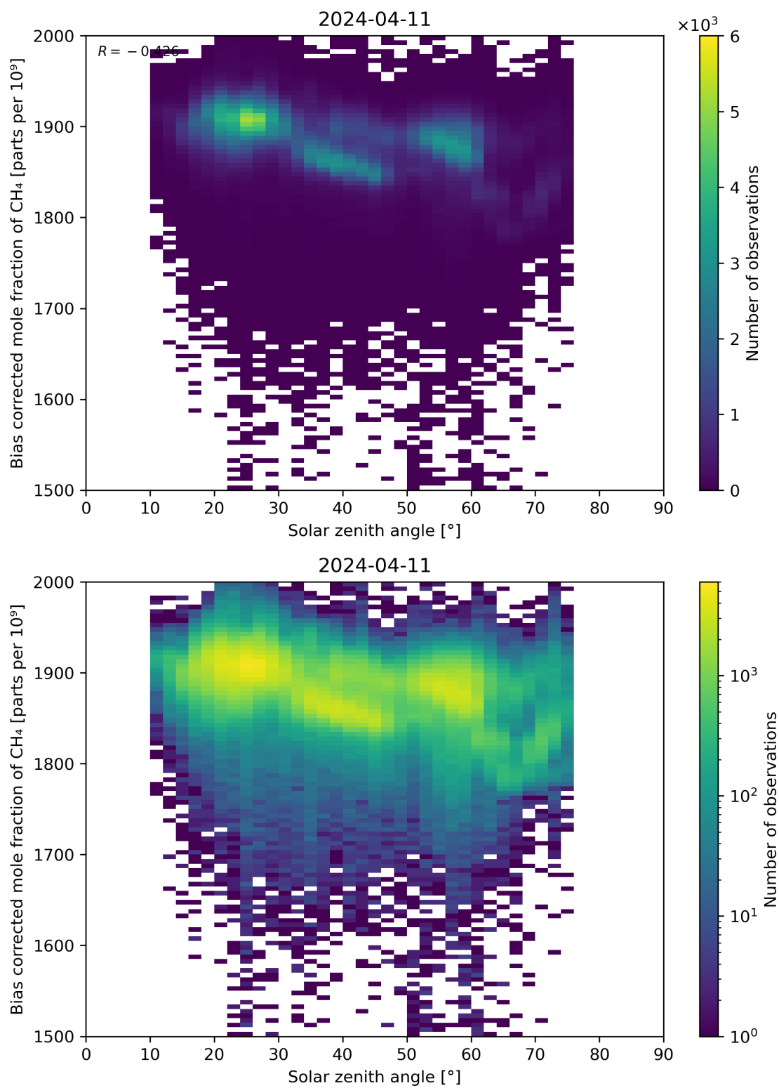
Figure 100: Scatter density plot of “Solar zenith angle” against “Bias corrected mole fraction of CH 4 ” for 2024-04-10 to 2024-04-12.
