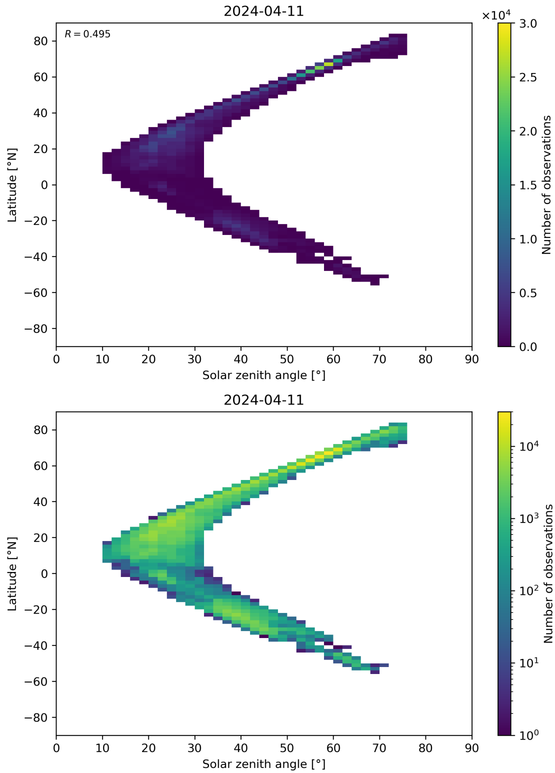
Figure 98: Scatter density plot of “Solar zenith angle” against “Latitude” for 2024-04-10 to 2024-04-12.
