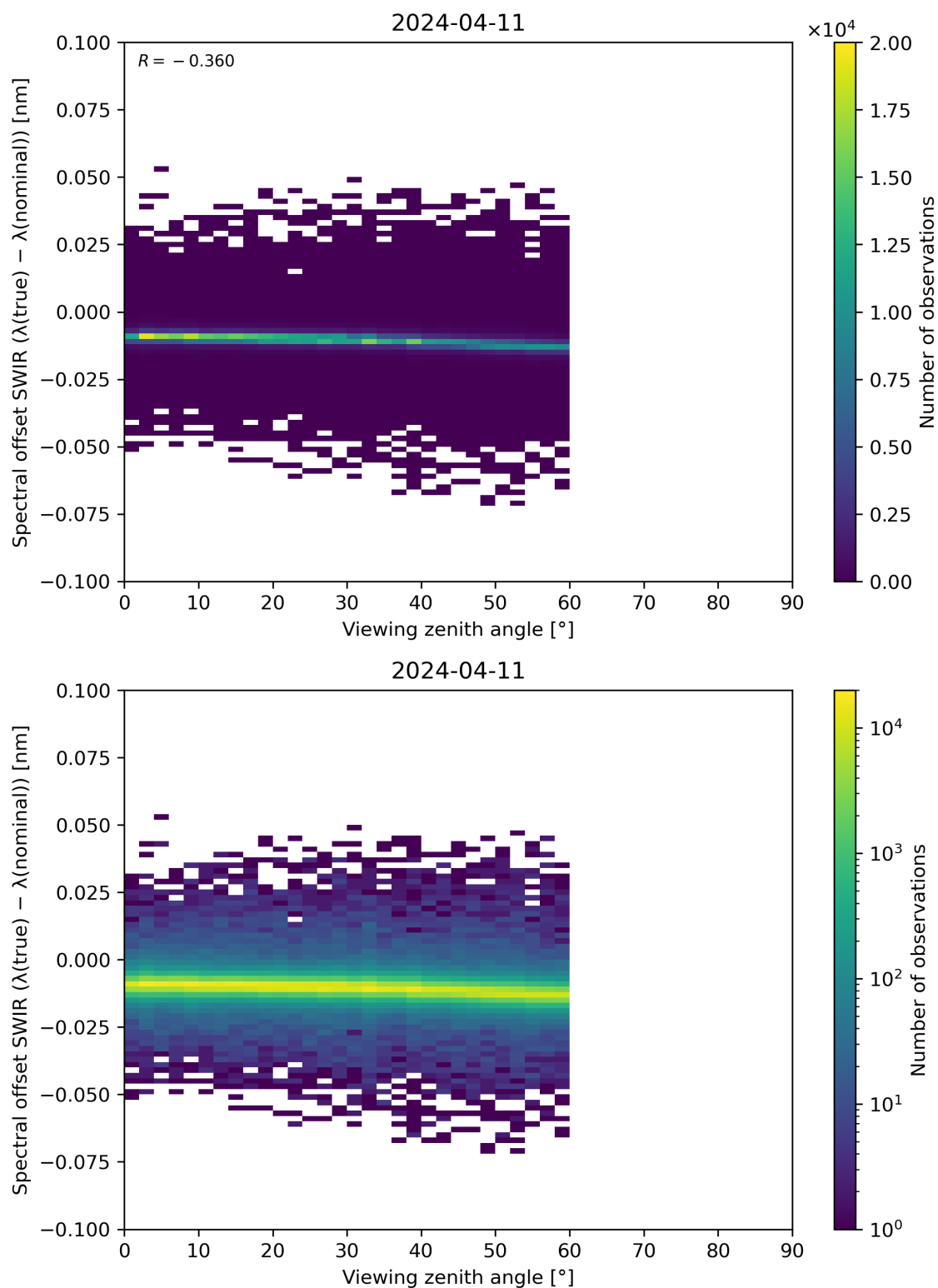
Figure 116: Scatter density plot of “Viewing zenith angle” against “Spectral offset SWIR ( \lambda(\text{true}) - \lambda(\text{nominal}) )” for 2024-04-10 to 2024-04-12.
