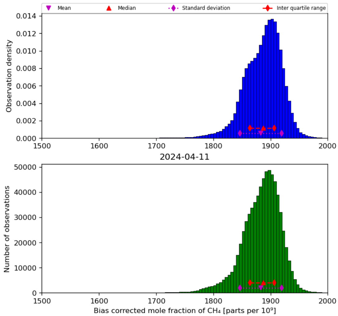
Figure 25: Histogram of “Bias corrected mole fraction of CH 4 ” for 2024-04-10 to 2024-04-12
