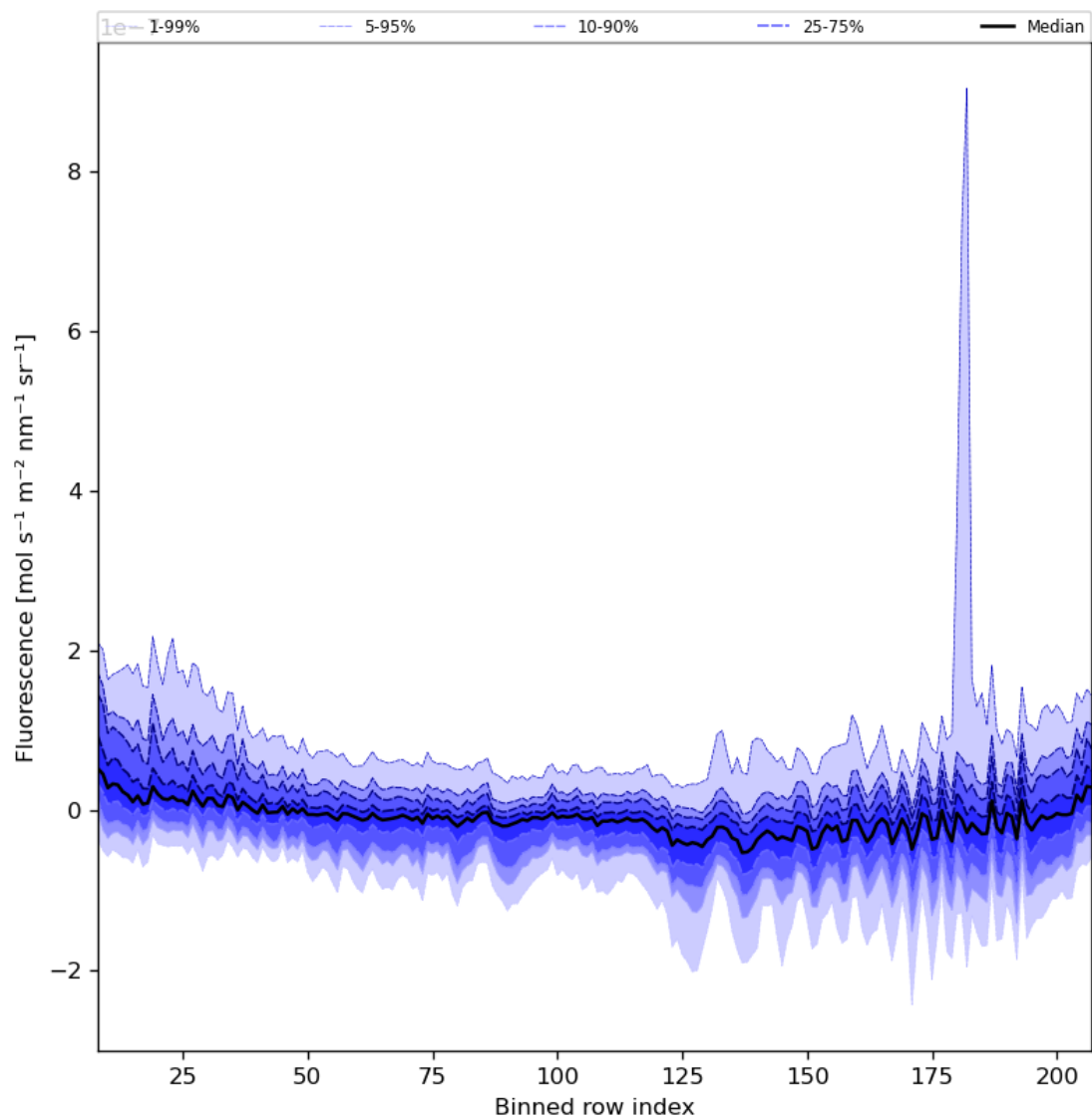
Figure 43: Along track statistics of “Fluorescence” for 2024-04-10 to 2024-04-12
