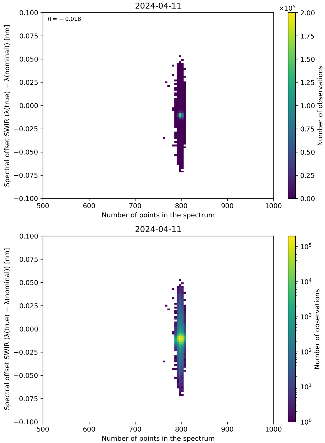
Figure 93: Scatter density plot of “Number of points in the spectrum” against “Spectral offset SWIR ( \lambda(\text{true}) - \lambda(\text{nominal}) )” for 2024-04-10 to 2024-04-12.
