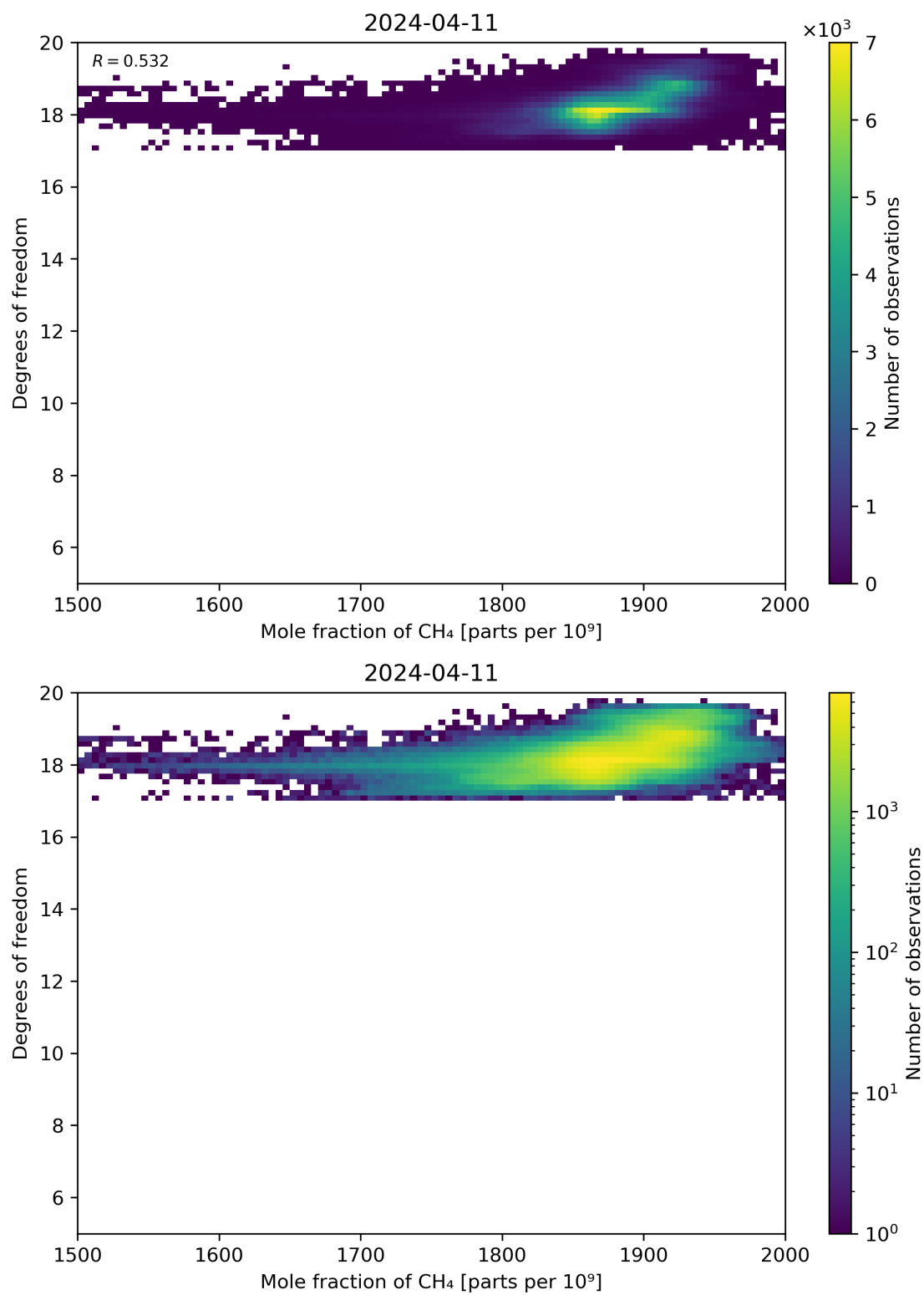
Figure 72: Scatter density plot of “Mole fraction of CH 4 ” against “Degrees of freedom” for 2024-04-10 to 2024-04-12.
