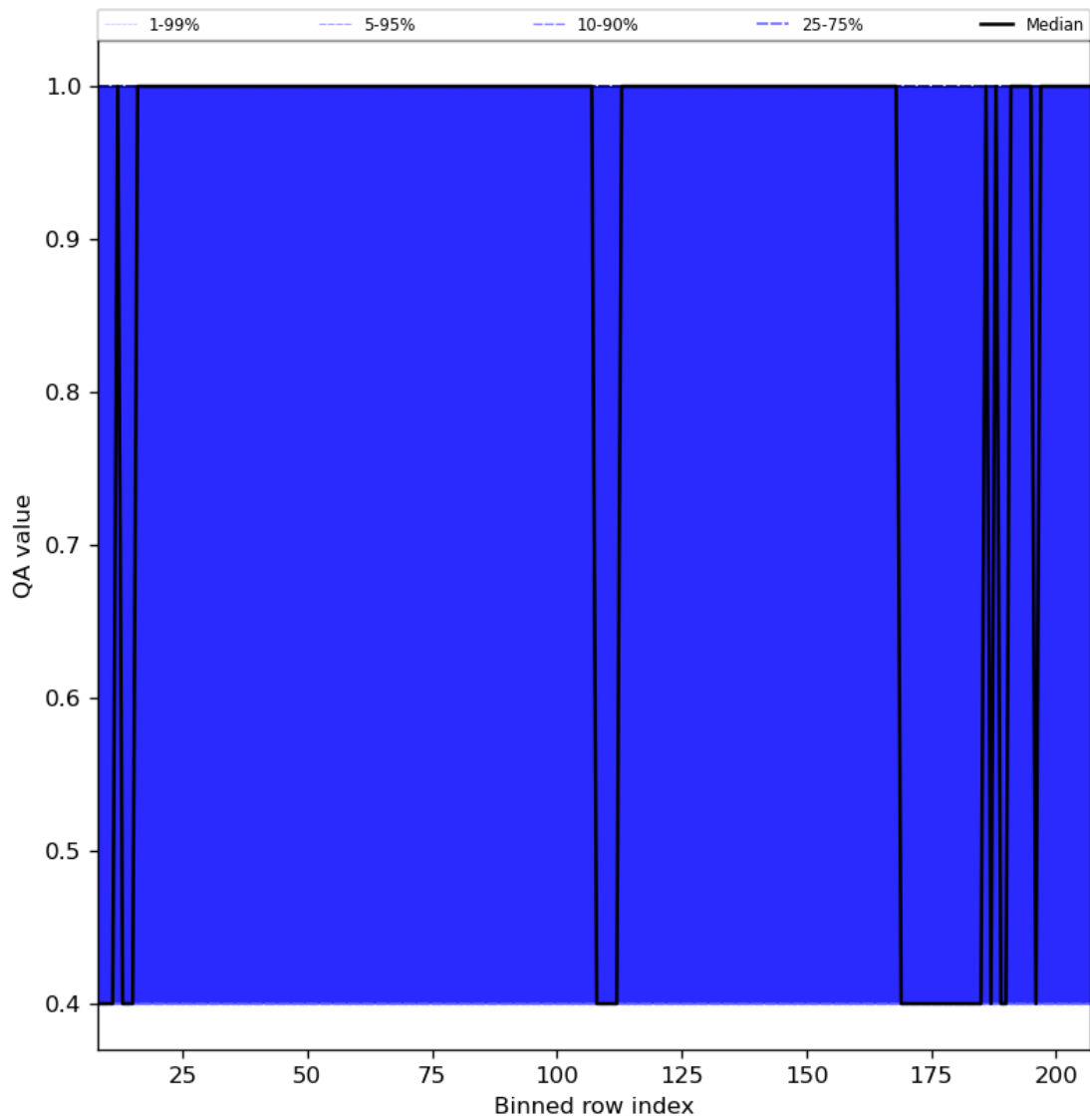
Figure 33: Along track statistics of “QA value” for 2024-04-10 to 2024-04-12
