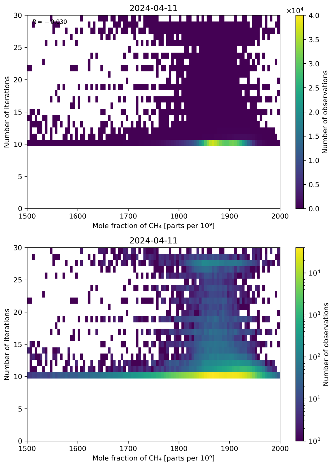
Figure 76: Scatter density plot of “Mole fraction of CH 4 ” against “Number of iterations” for 2024-04-10 to 2024-04-12.
