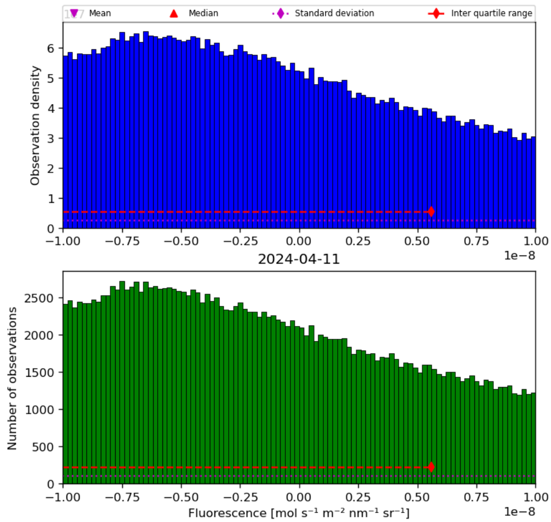
Figure 32: Histogram of “Fluorescence” for 2024-04-10 to 2024-04-12
