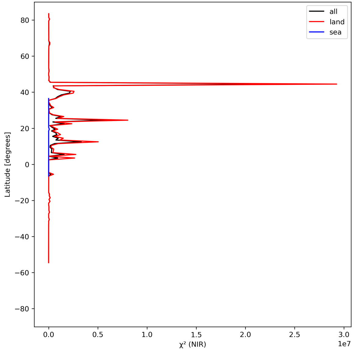
Figure 18: Zonal average of “ \chi^2 (NIR)” for 2024-04-10 to 2024-04-12.
