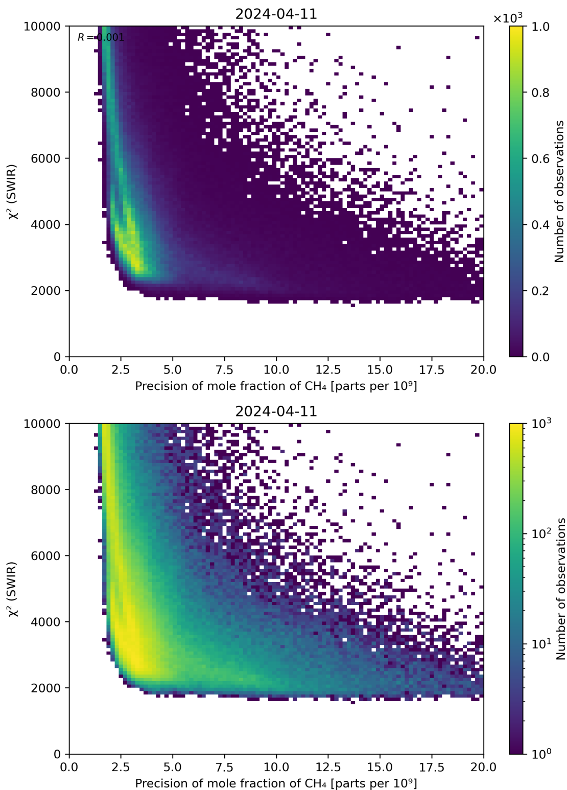
Figure 79: Scatter density plot of “Precision of mole fraction of \text{CH}_4 ” against “ \chi^2 (SWIR)” for 2024-04-10 to 2024-04-12.
