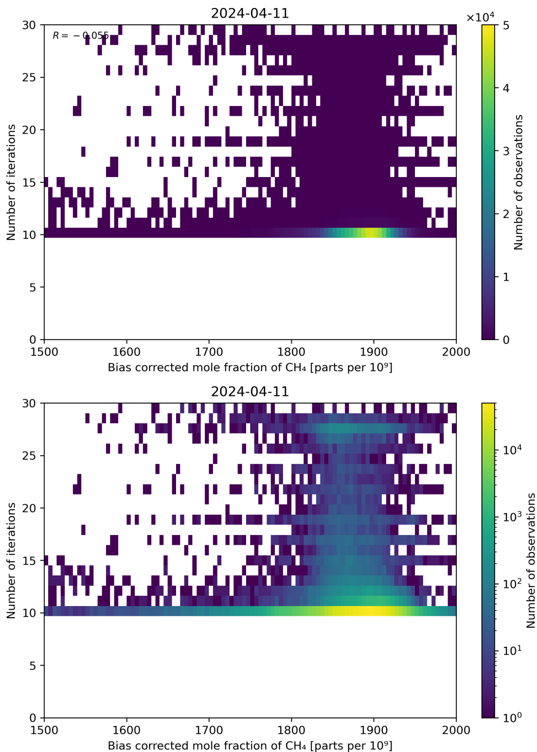
Figure 67: Scatter density plot of “Bias corrected mole fraction of CH 4 ” against “Number of iterations” for 2024-04-10 to 2024-04-12.
