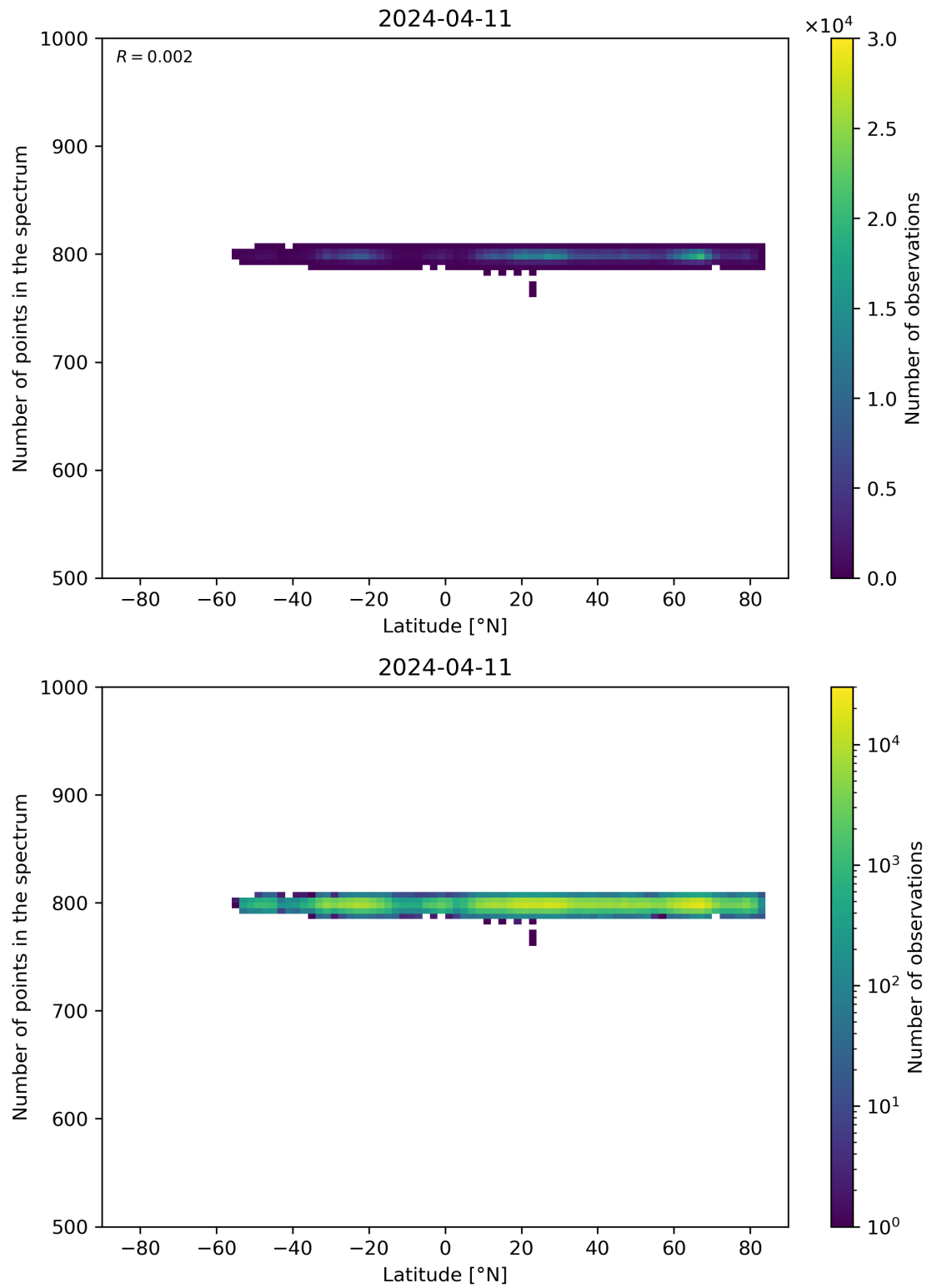
Figure 61: Scatter density plot of “Latitude” against “Number of points in the spectrum” for 2024-04-10 to 2024-04-12.
