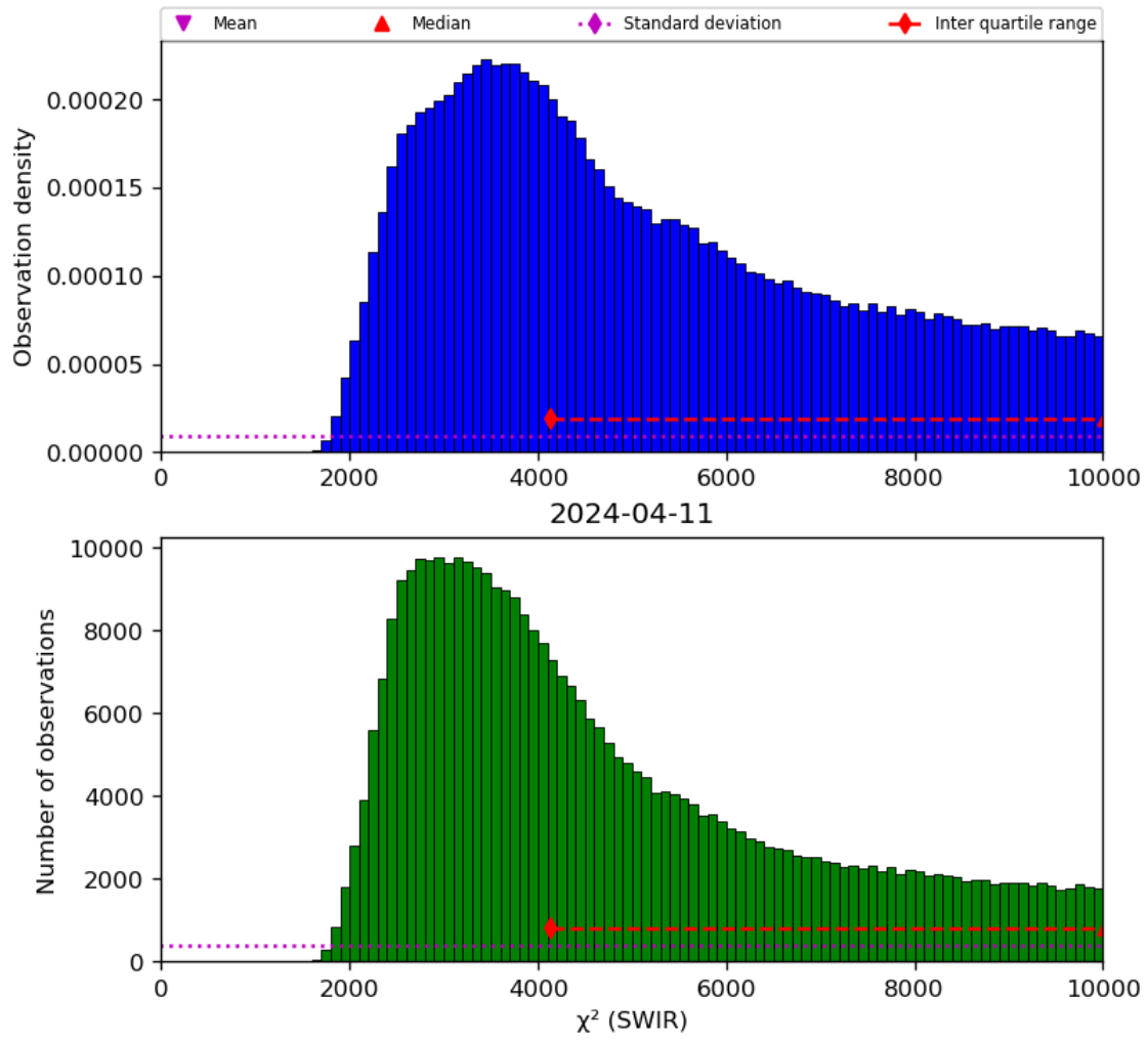
Figure 28: Histogram of “ \chi^2 (SWIR)” for 2024-04-10 to 2024-04-12
