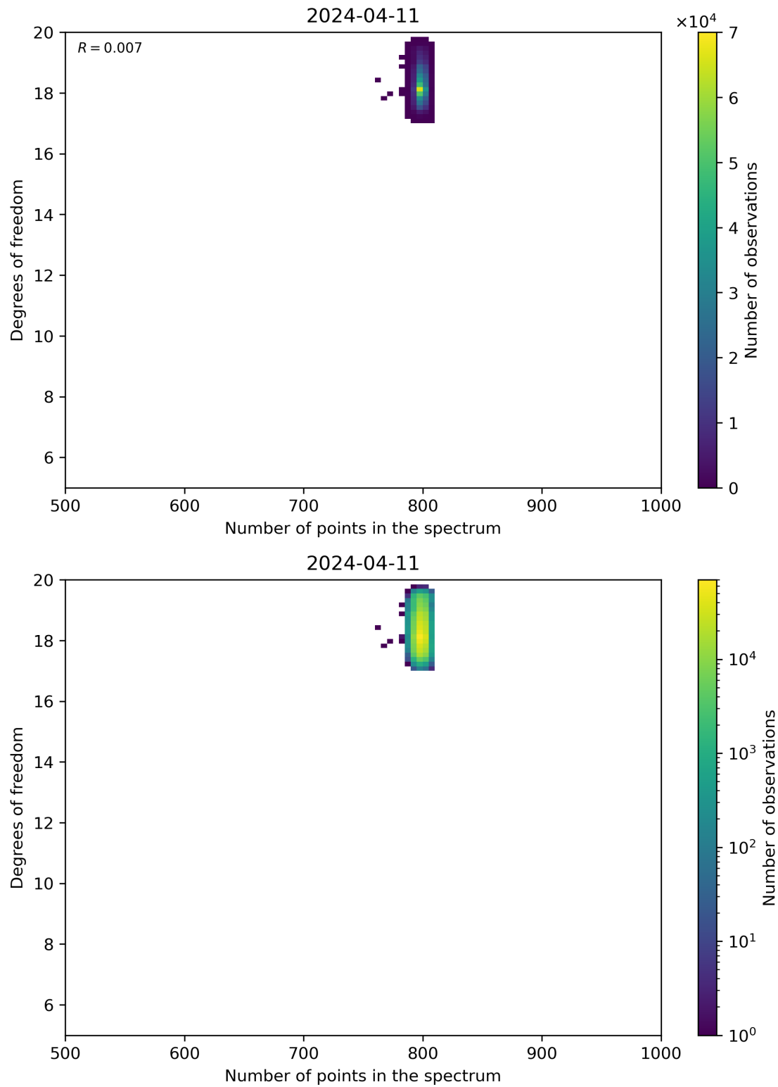
Figure 90: Scatter density plot of “Number of points in the spectrum” against “Degrees of freedom” for 2024-04-10 to 2024-04-12.
