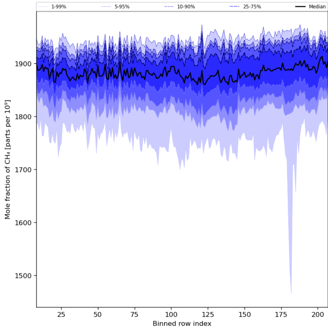
Figure 34: Along track statistics of “Mole fraction of CH 4 ” for 2024-04-10 to 2024-04-12
