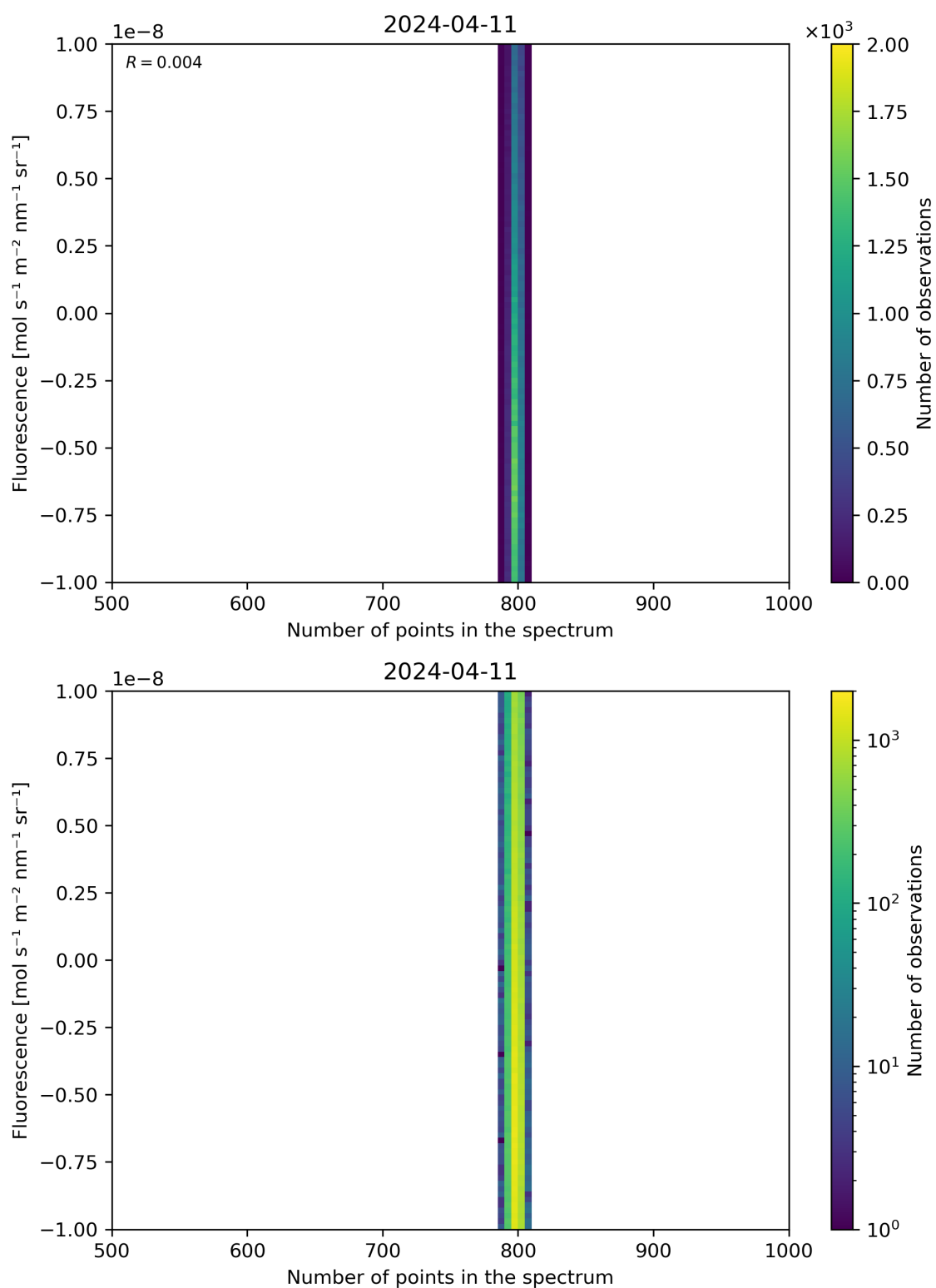
Figure 91: Scatter density plot of “Number of points in the spectrum” against “Fluorescence” for 2024-04-10 to 2024-04-12.
