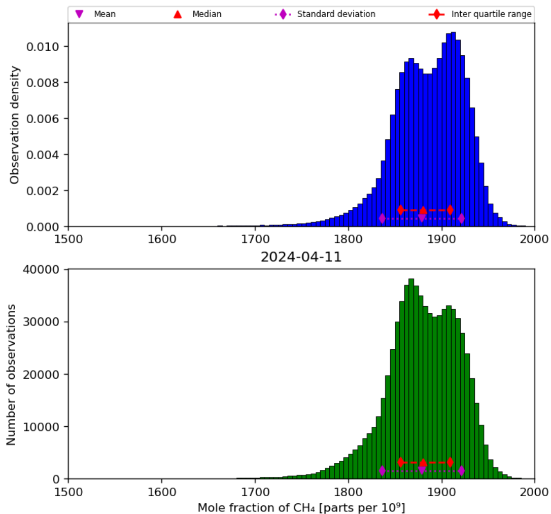
Figure 23: Histogram of “Mole fraction of CH 4 ” for 2024-04-10 to 2024-04-12
