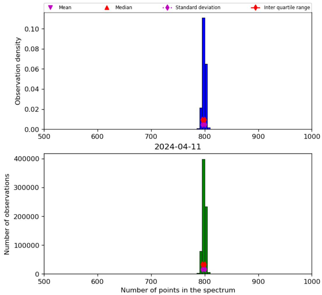
Figure 26: Histogram of “Number of points in the spectrum” for 2024-04-10 to 2024-04-12
