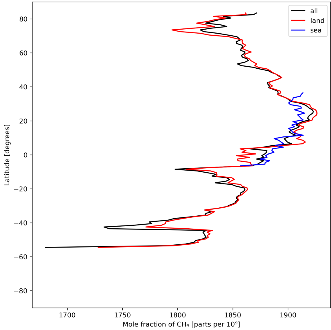
Figure 12: Zonal average of “Mole fraction of \text{CH}_4 ” for 2024-04-10 to 2024-04-12.
