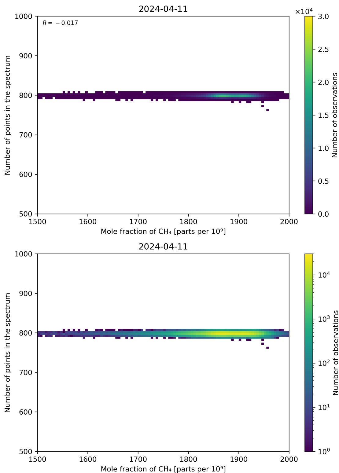
Figure 77: Scatter density plot of “Mole fraction of CH 4 ” against “Number of points in the spectrum” for 2024-04-10 to 2024-04-12.
