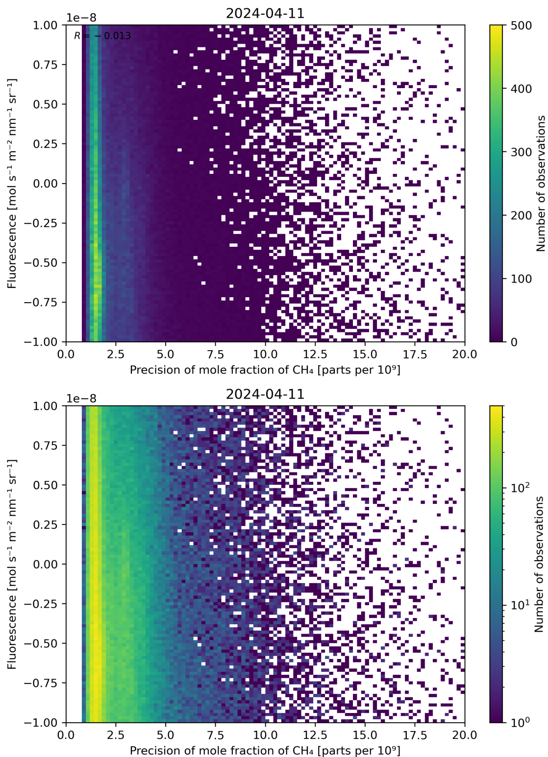
Figure 81: Scatter density plot of “Precision of mole fraction of CH 4 ” against “Fluorescence” for 2024-04-10 to 2024-04-12.
