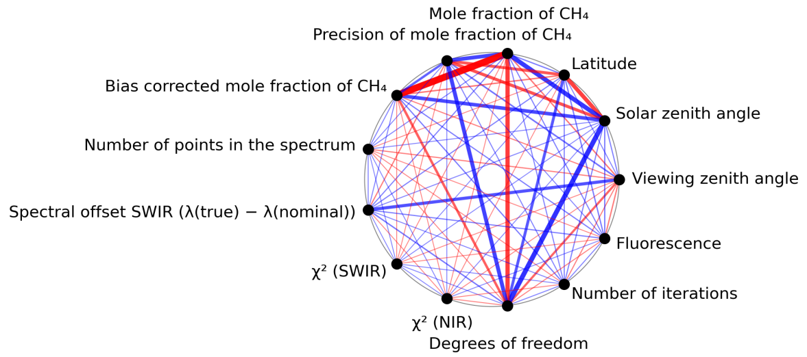
Figure 1: Map of correlation graph for 2024-04-10 to 2024-04-12.
