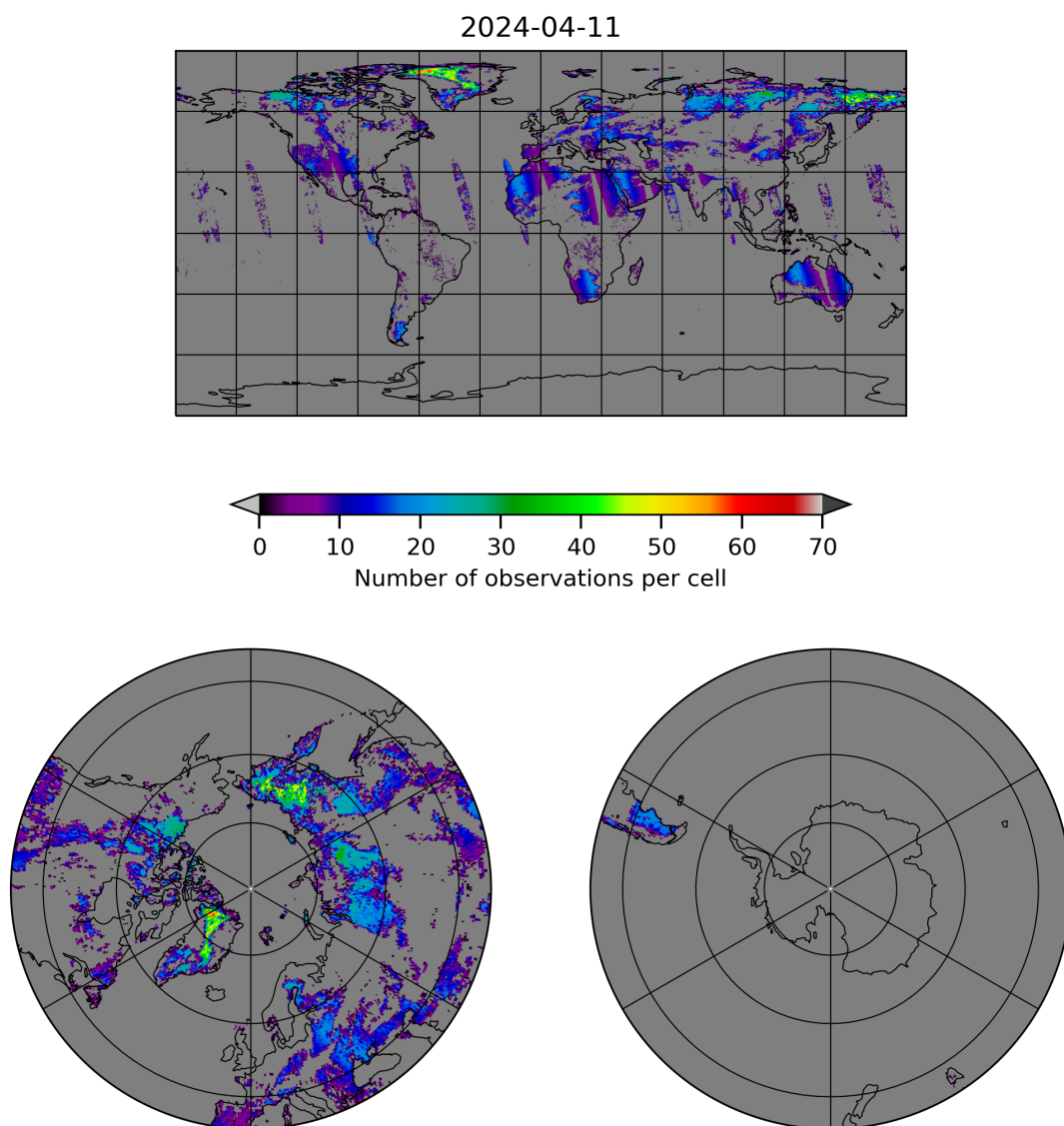
Figure 10: Map of the number of observations for 2024-04-10 to 2024-04-12
