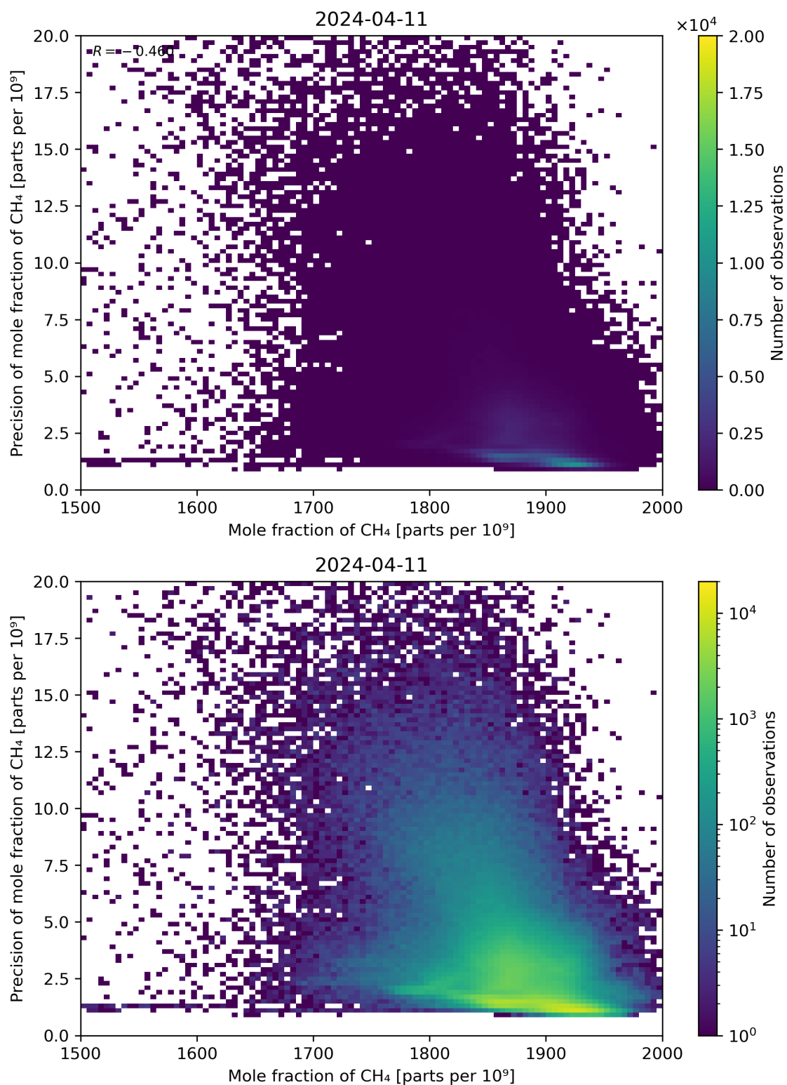
Figure 75: Scatter density plot of “Mole fraction of CH 4 ” against “Precision of mole fraction of CH 4 ” for 2024-04-10 to 2024-04-12.
