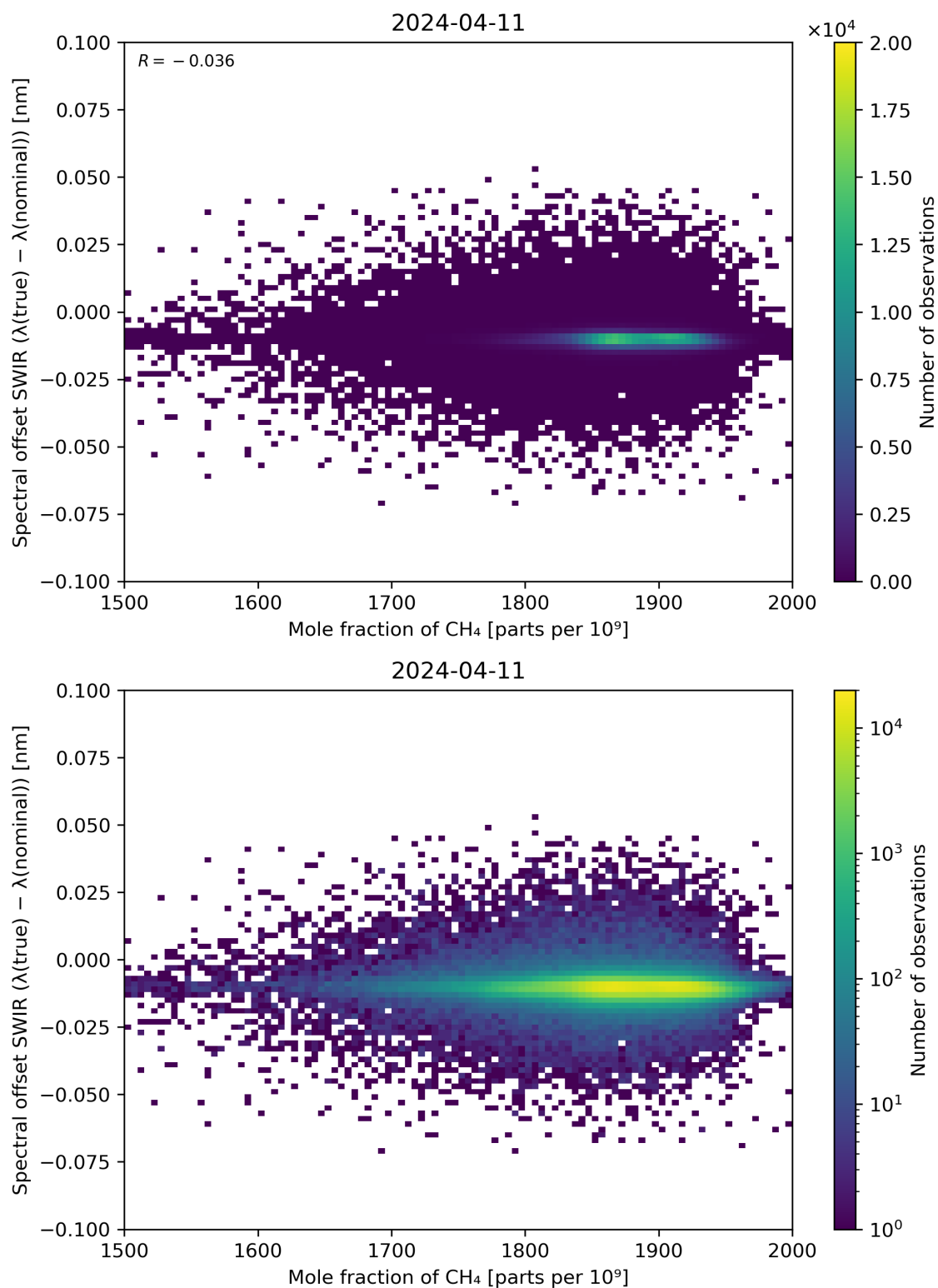
Figure 86: Scatter density plot of “Mole fraction of CH 4 ” against “Spectral offset SWIR ( \lambda(\text{true}) - \lambda(\text{nominal}) )” for 2024-04-10 to 2024-04-12.
