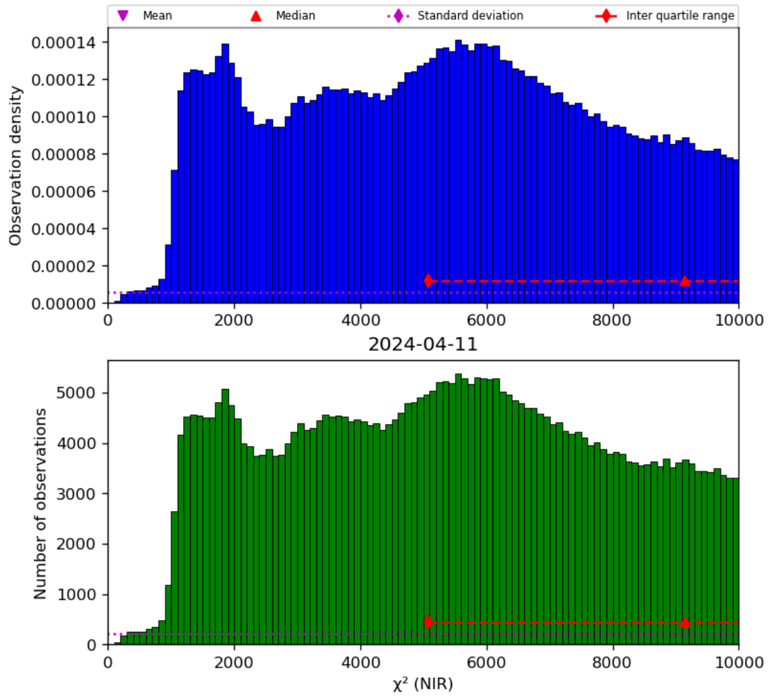
Figure 29: Histogram of " \chi^2 (NIR)" for 2024-04-10 to 2024-04-12
