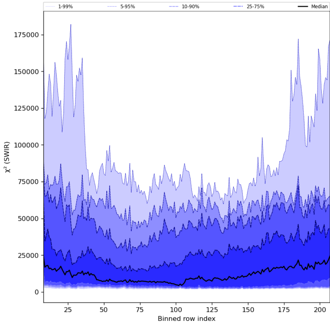
Figure 39: Along track statistics of “ \chi^2 (SWIR)” for 2024-04-10 to 2024-04-12
