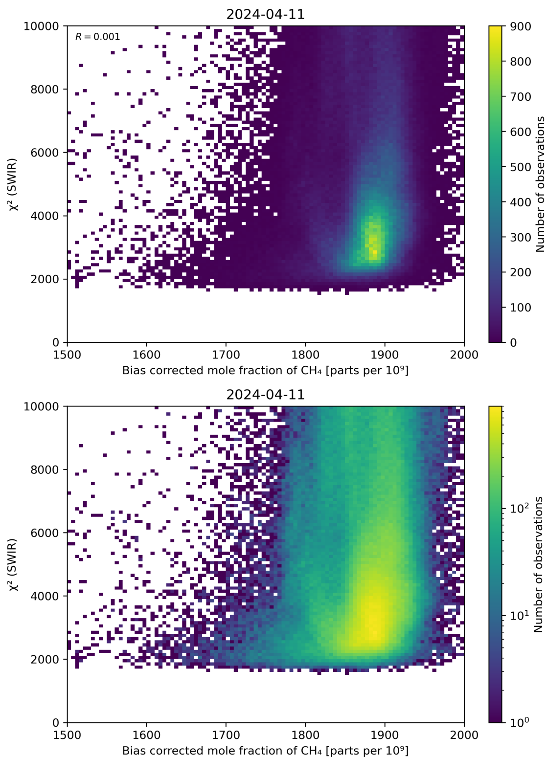
Figure 64: Scatter density plot of “Bias corrected mole fraction of CH 4 ” against “ \chi^2 (SWIR)” for 2024-04-10 to 2024-04-12.
