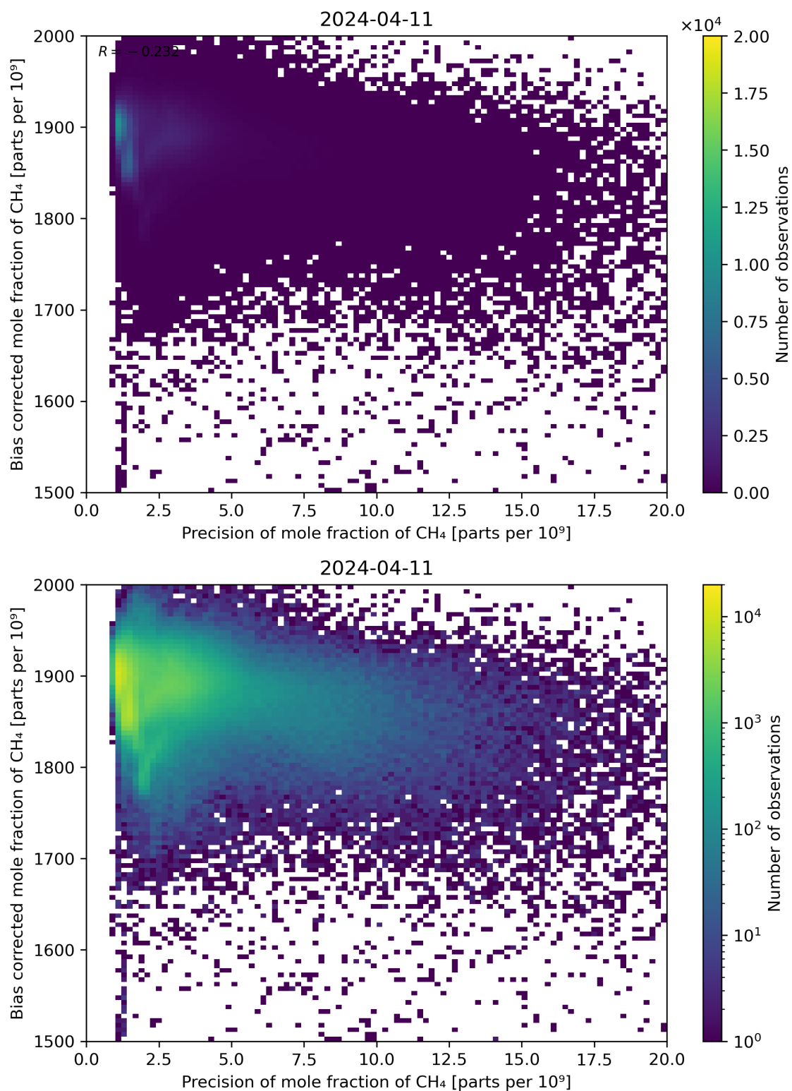
Figure 82: Scatter density plot of “Precision of mole fraction of CH 4 ” against “Bias corrected mole fraction of CH 4 ” for 2024-04-10 to 2024-04-12.
