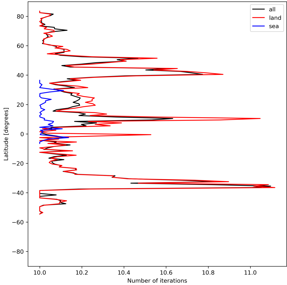
Figure 20: Zonal average of “Number of iterations” for 2024-04-10 to 2024-04-12.
