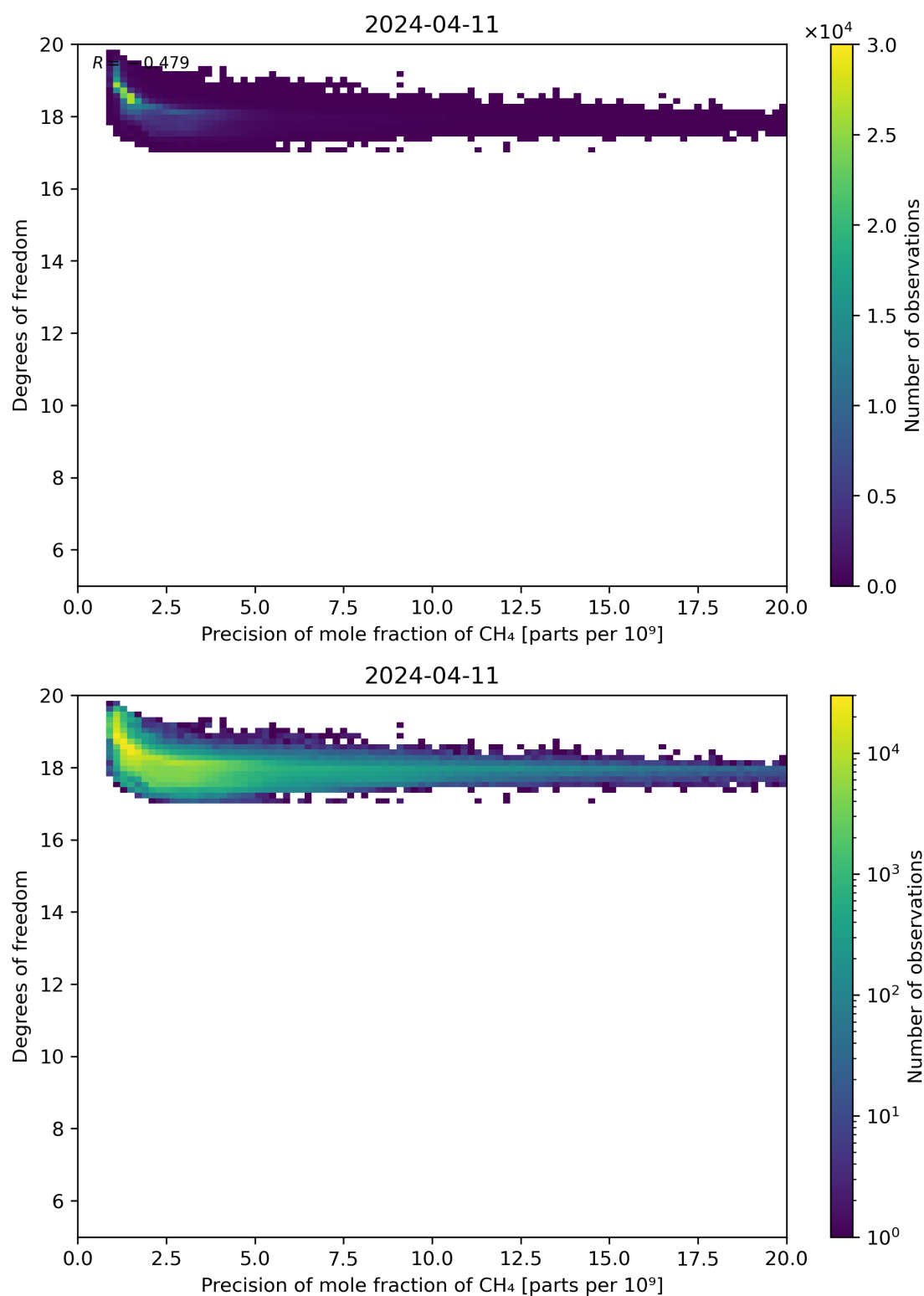
Figure 80: Scatter density plot of “Precision of mole fraction of CH 4 ” against “Degrees of freedom” for 2024-04-10 to 2024-04-12.
