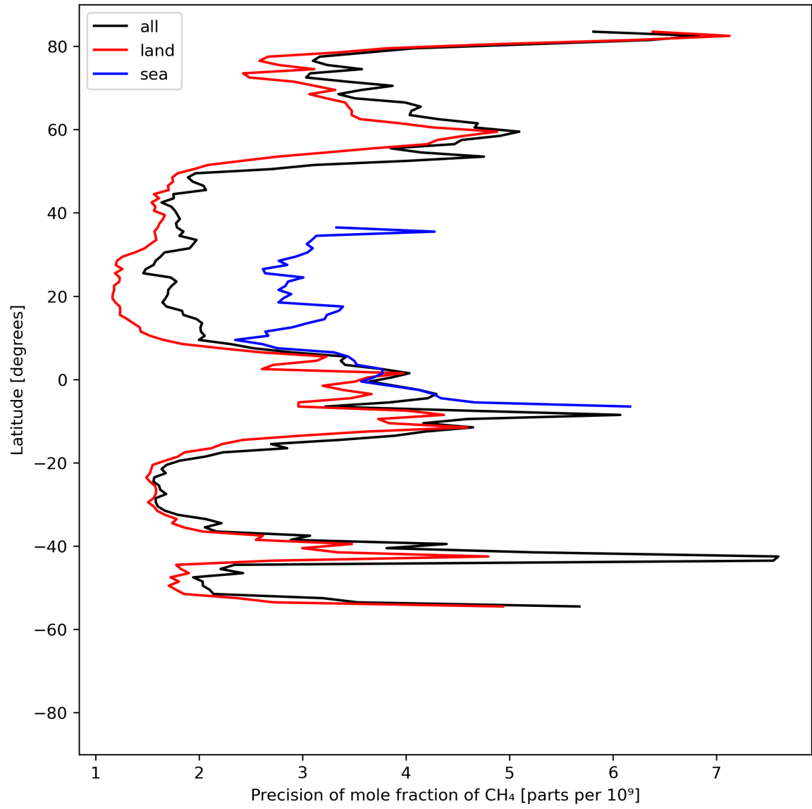
Figure 13: Zonal average of “Precision of mole fraction of CH 4 ” for 2024-04-10 to 2024-04-12.
