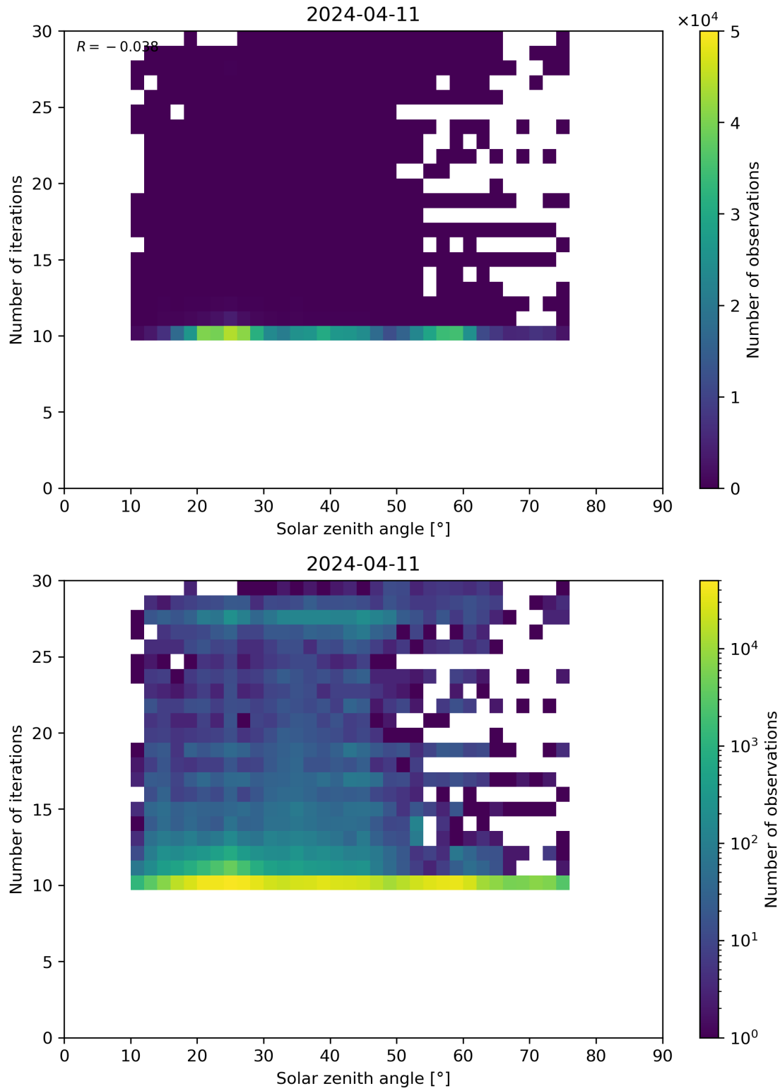
Figure 102: Scatter density plot of “Solar zenith angle” against “Number of iterations” for 2024-04-10 to 2024-04-12.
