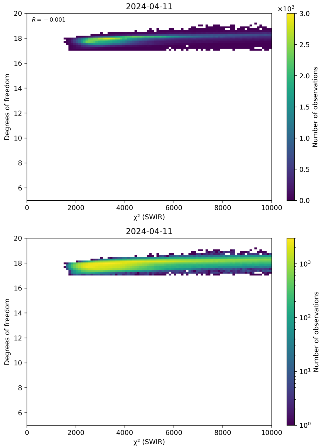
Figure 48: Scatter density plot of “ \chi^2 (SWIR)” against “Degrees of freedom” for 2024-04-10 to 2024-04-12.
