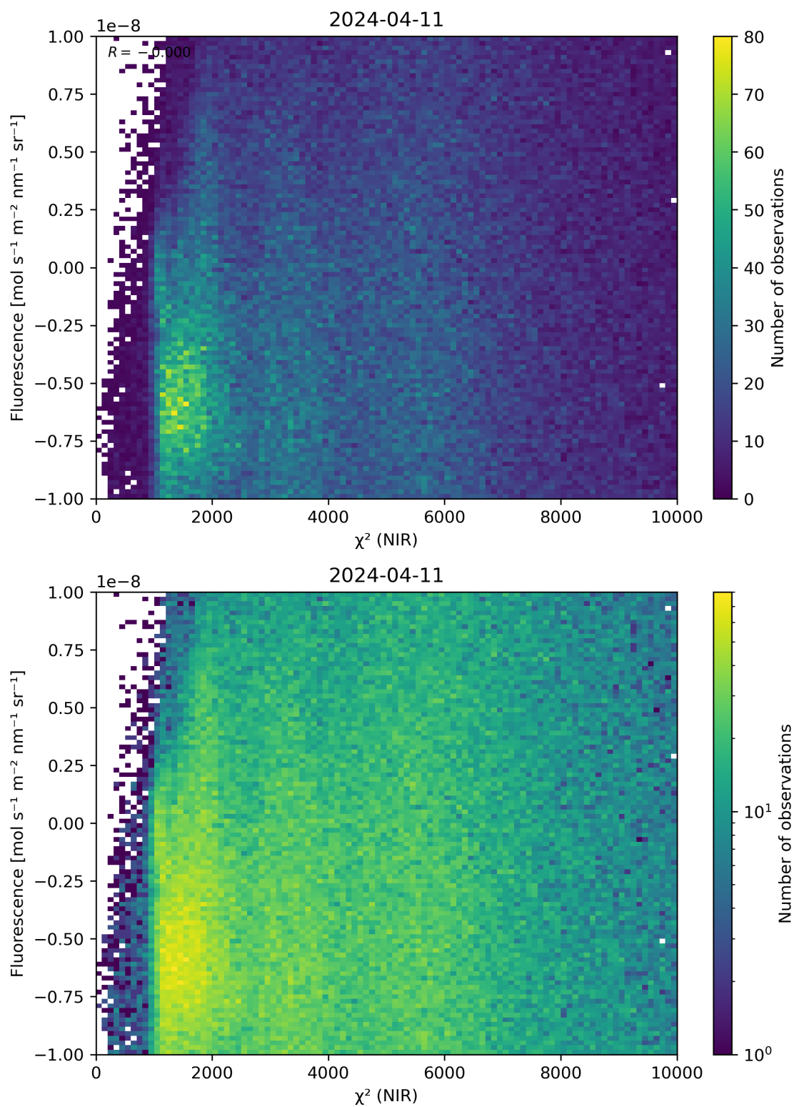
Figure 45: Scatter density plot of “ \chi^2 (NIR)” against “Fluorescence” for 2024-04-10 to 2024-04-12.
