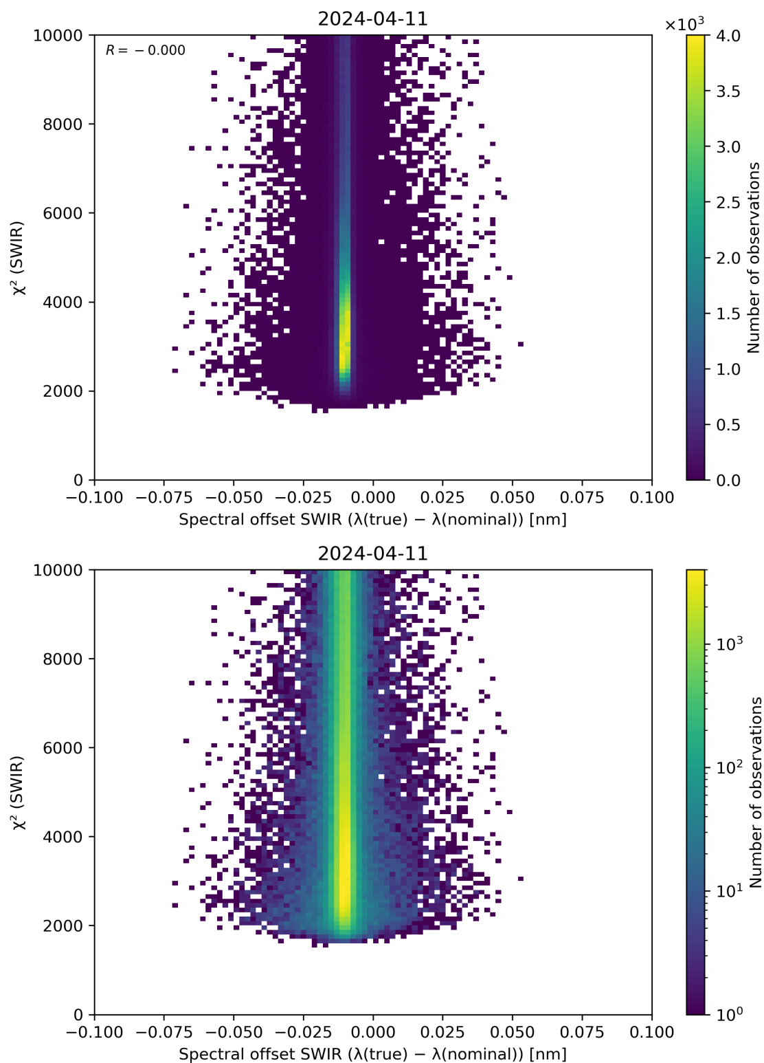
Figure 118: Scatter density plot of “Spectral offset SWIR ( \lambda(\text{true}) - \lambda(\text{nominal}) )” against “ \chi^2 (SWIR)” for 2024-04-10 to 2024-04-12.
