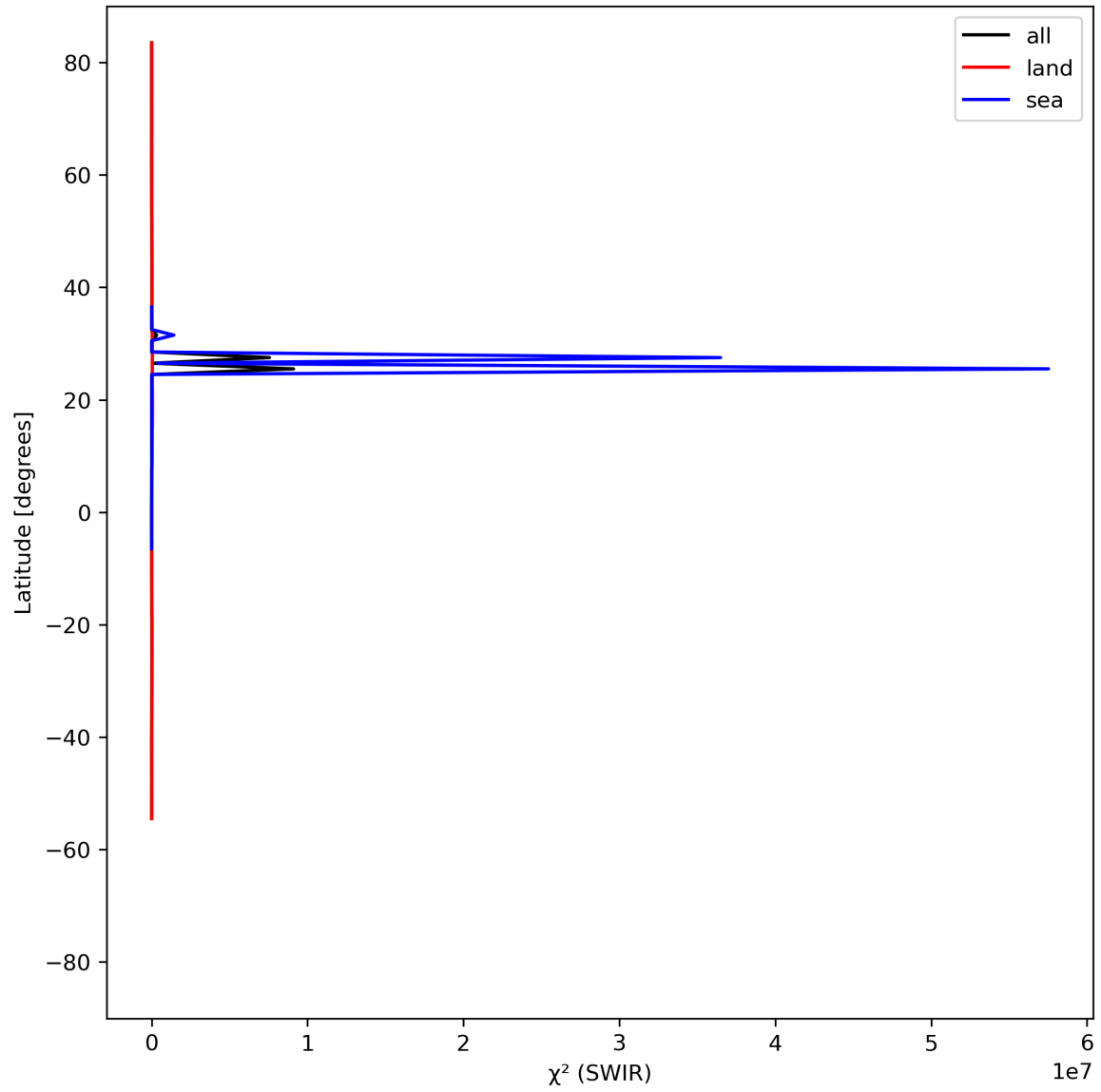
Figure 17: Zonal average of “ \chi^2 (SWIR)” for 2024-04-10 to 2024-04-12.
