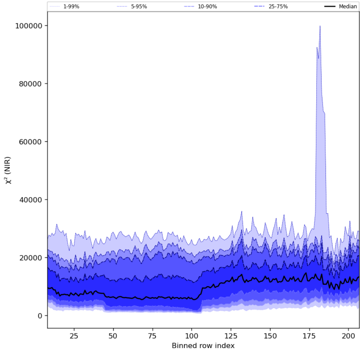
Figure 40: Along track statistics of “ \chi^2 (NIR)” for 2024-04-10 to 2024-04-12
