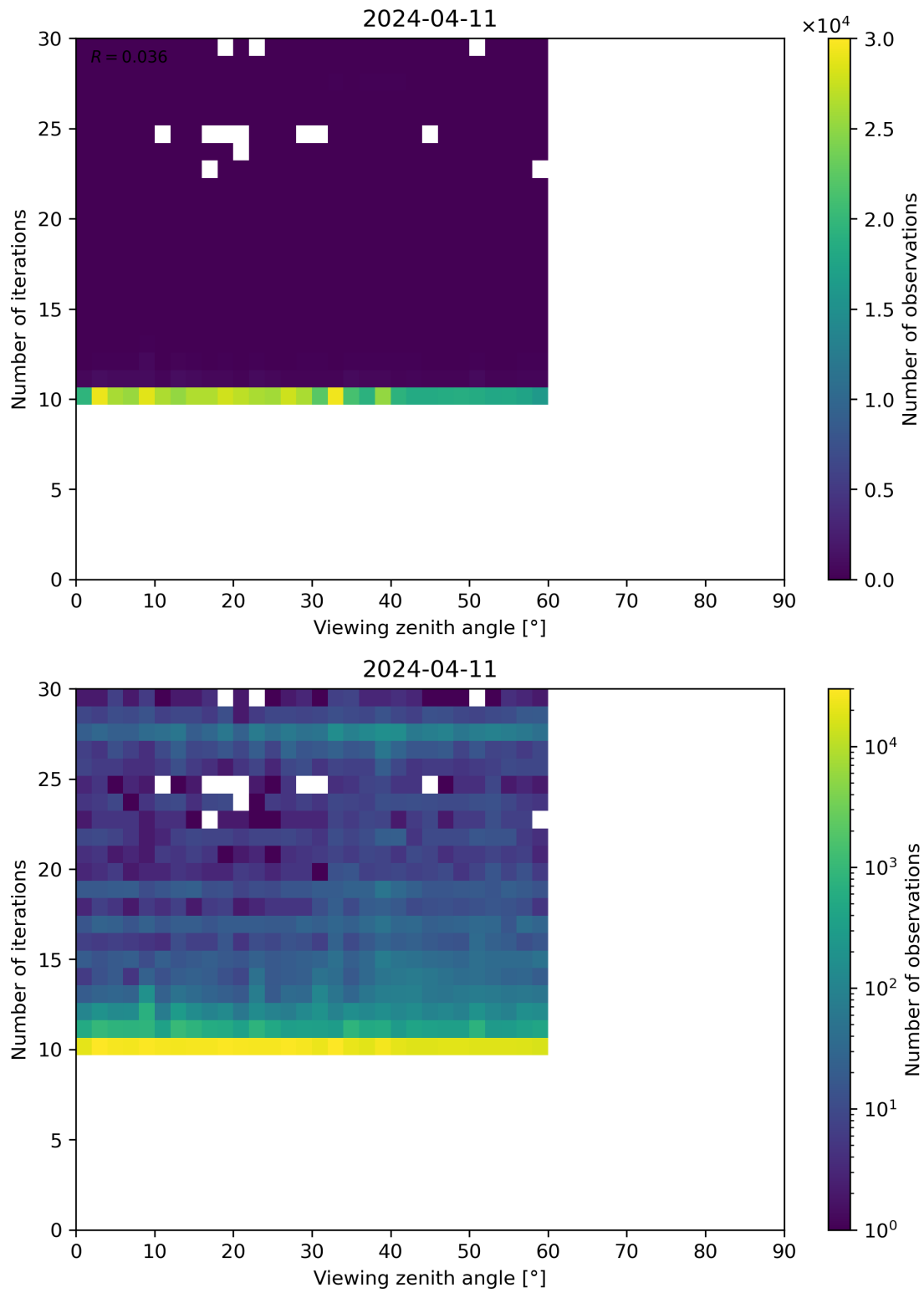
Figure 113: Scatter density plot of “Viewing zenith angle” against “Number of iterations” for 2024-04-10 to 2024-04-12.
