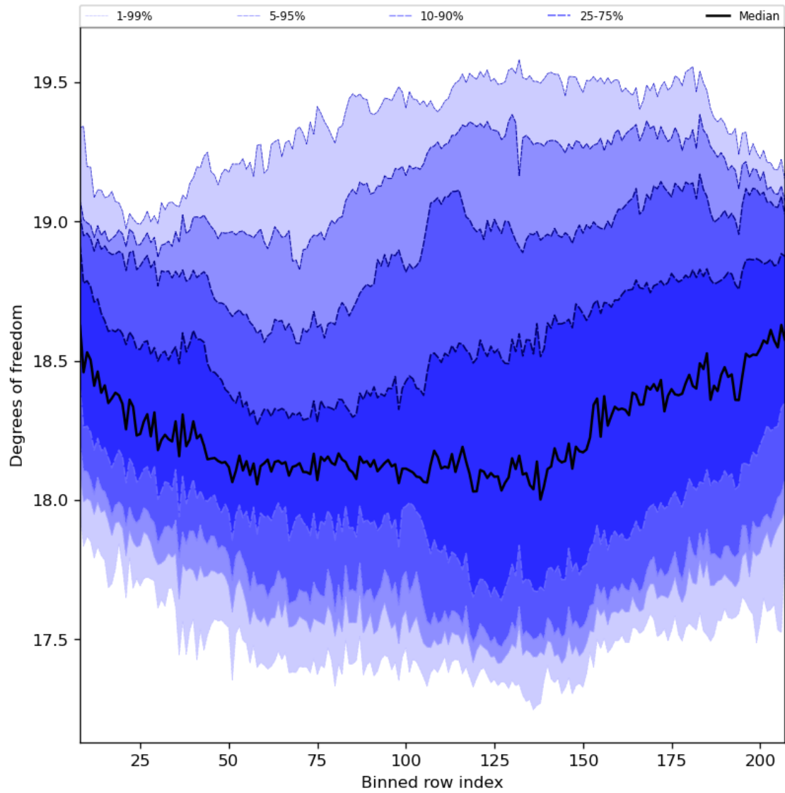
Figure 41: Along track statistics of “Degrees of freedom” for 2024-04-10 to 2024-04-12
