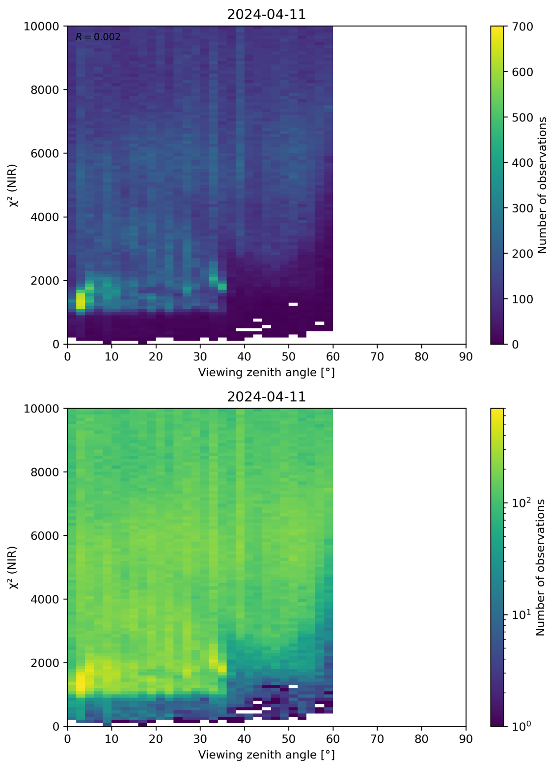
Figure 105: Scatter density plot of “Viewing zenith angle” against “ \chi^2 (NIR)” for 2024-04-10 to 2024-04-12.
