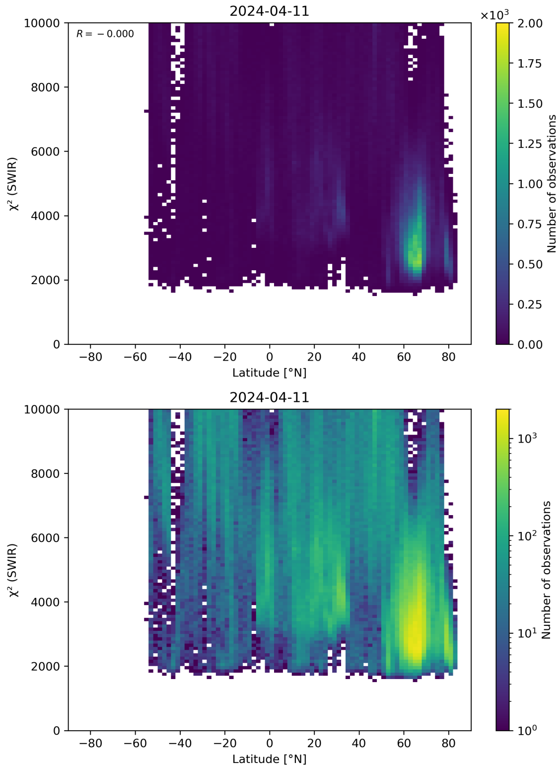
Figure 54: Scatter density plot of “Latitude” against “ \chi^2 (SWIR)” for 2024-04-10 to 2024-04-12.
