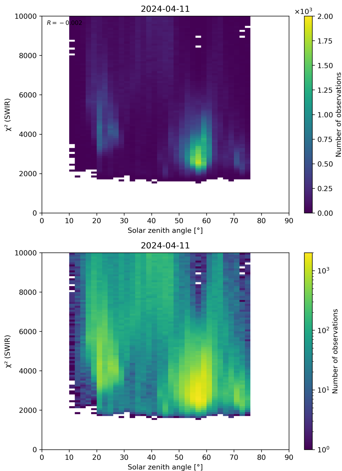
Figure 95: Scatter density plot of “Solar zenith angle” against “ \chi^2 (SWIR)” for 2024-04-10 to 2024-04-12.
