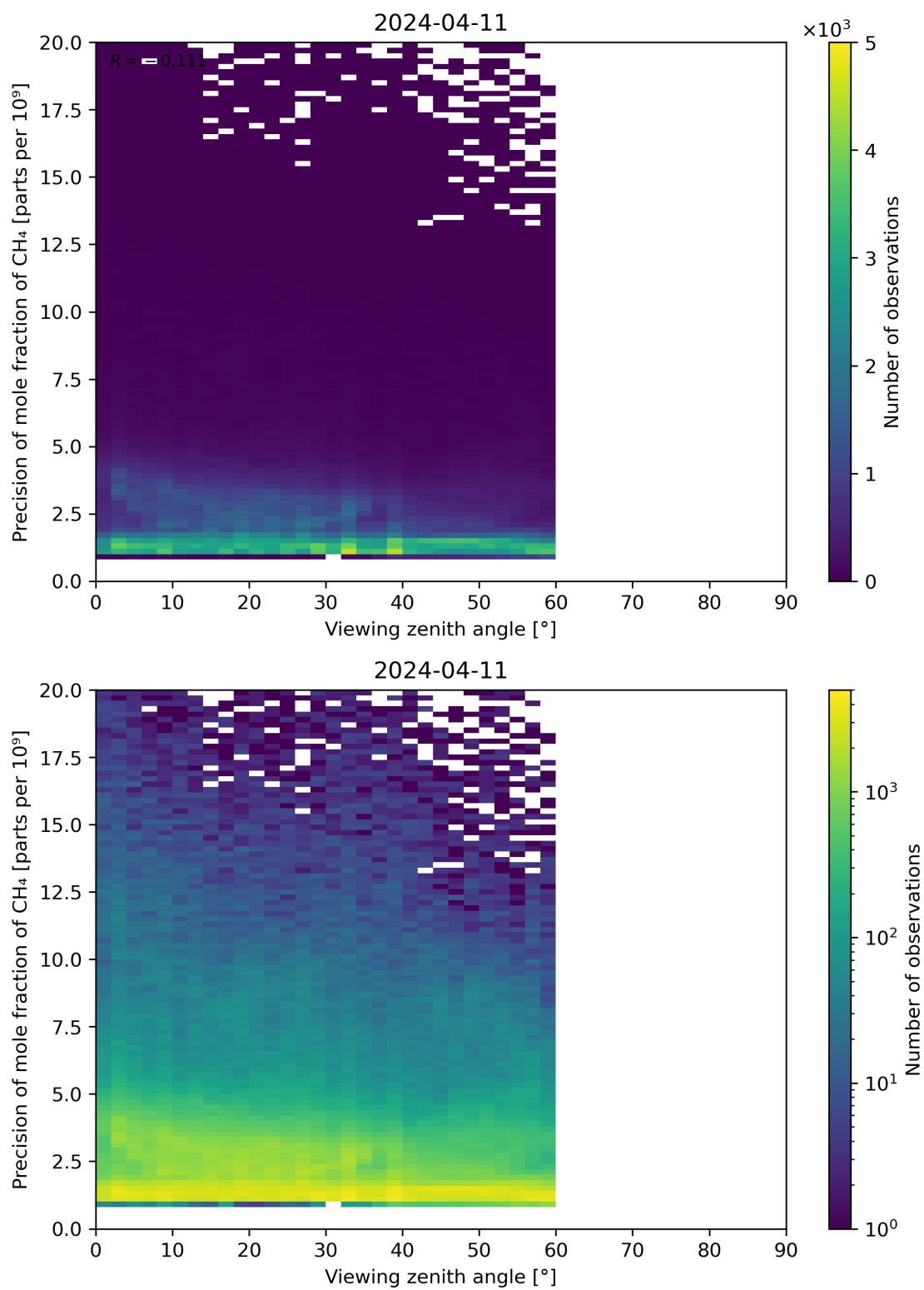
Figure 112: Scatter density plot of “Viewing zenith angle” against “Precision of mole fraction of CH 4 ” for 2024-04-10 to 2024-04-12.
