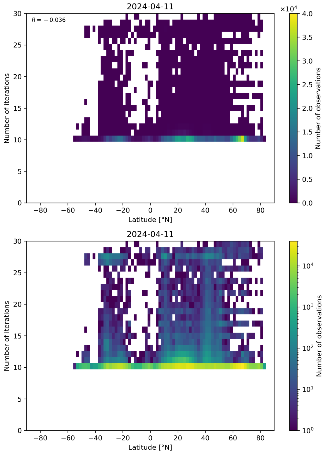
Figure 60: Scatter density plot of “Latitude” against “Number of iterations” for 2024-04-10 to 2024-04-12.
