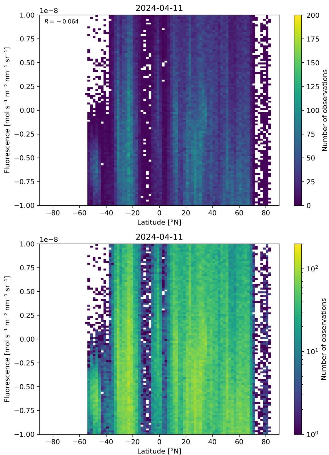
Figure 56: Scatter density plot of “Latitude” against “Fluorescence” for 2024-04-10 to 2024-04-12.
