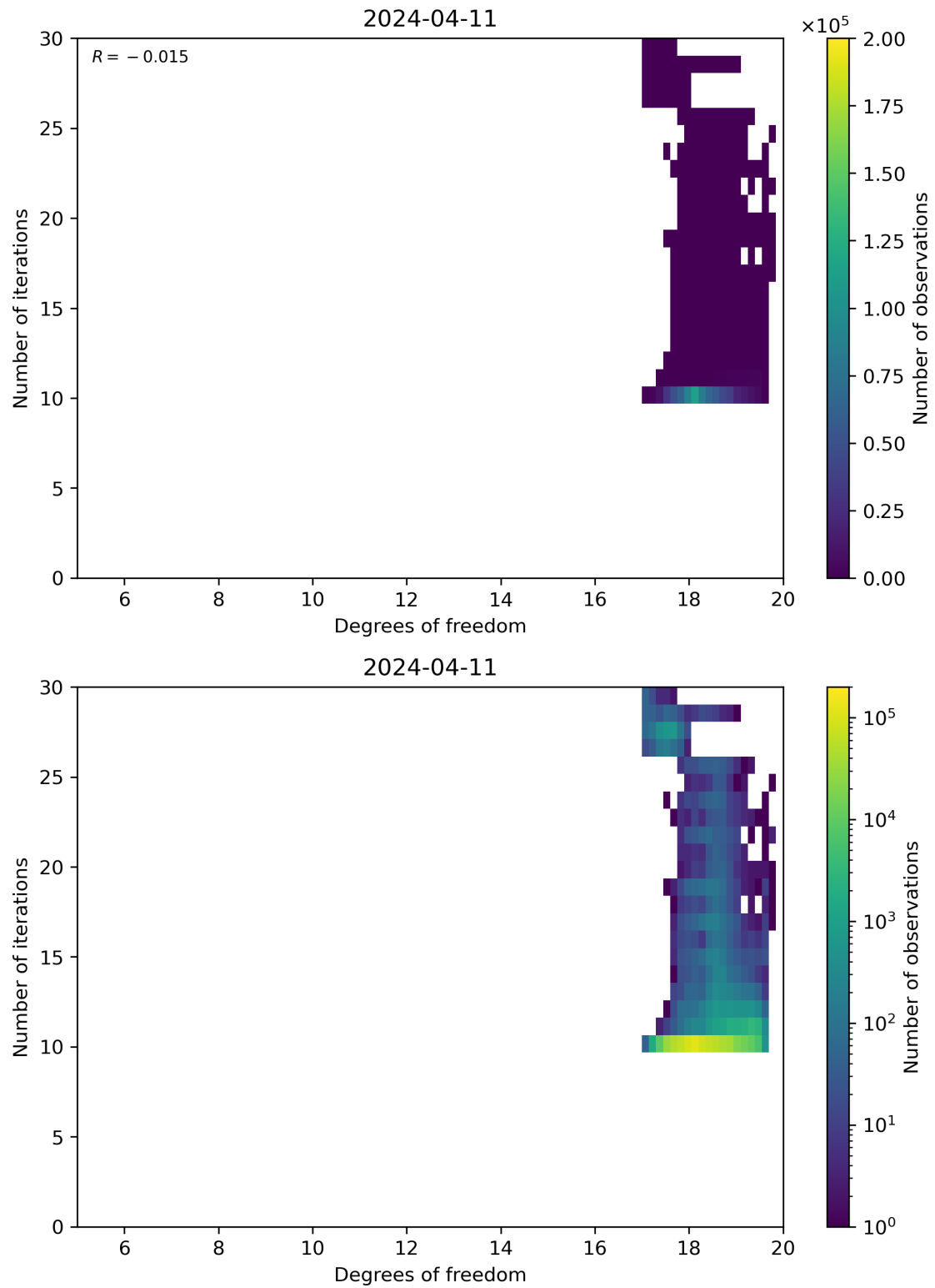
Figure 52: Scatter density plot of “Degrees of freedom” against “Number of iterations” for 2024-04-10 to 2024-04-12.
