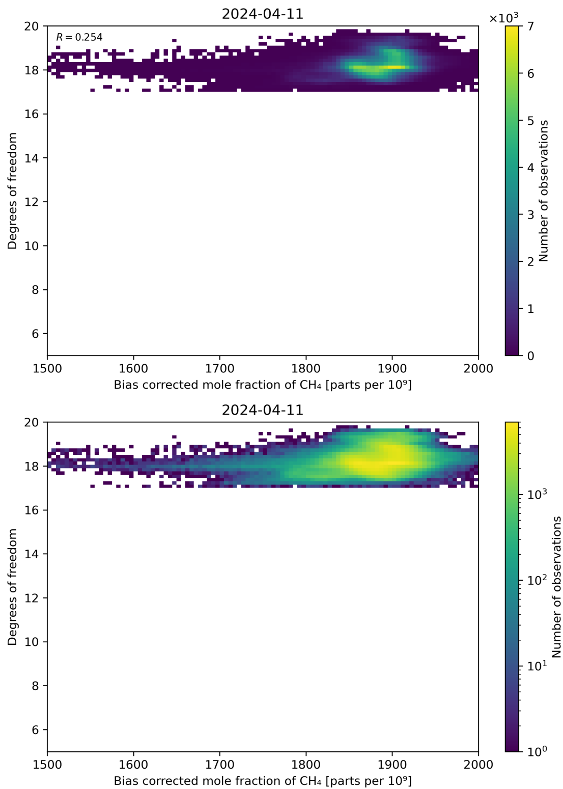
Figure 65: Scatter density plot of “Bias corrected mole fraction of CH 4 ” against “Degrees of freedom” for 2024-04-10 to 2024-04-12.
