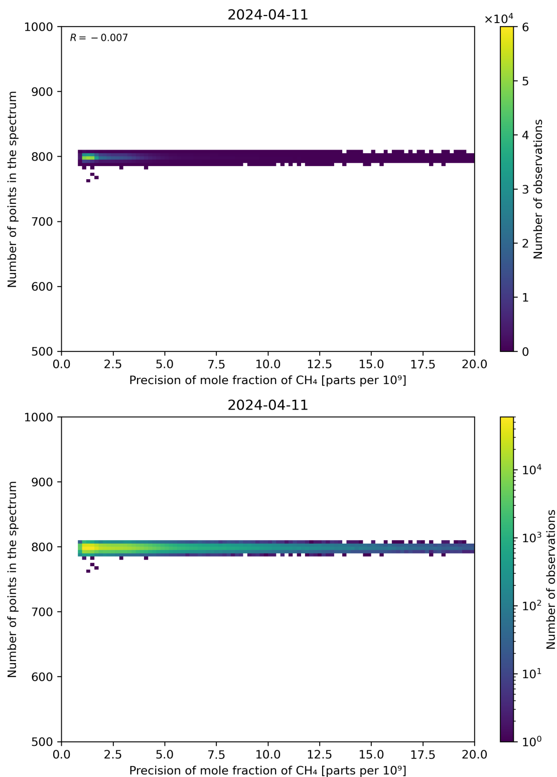
Figure 84: Scatter density plot of “Precision of mole fraction of CH 4 ” against “Number of points in the spectrum” for 2024-04-10 to 2024-04-12.
