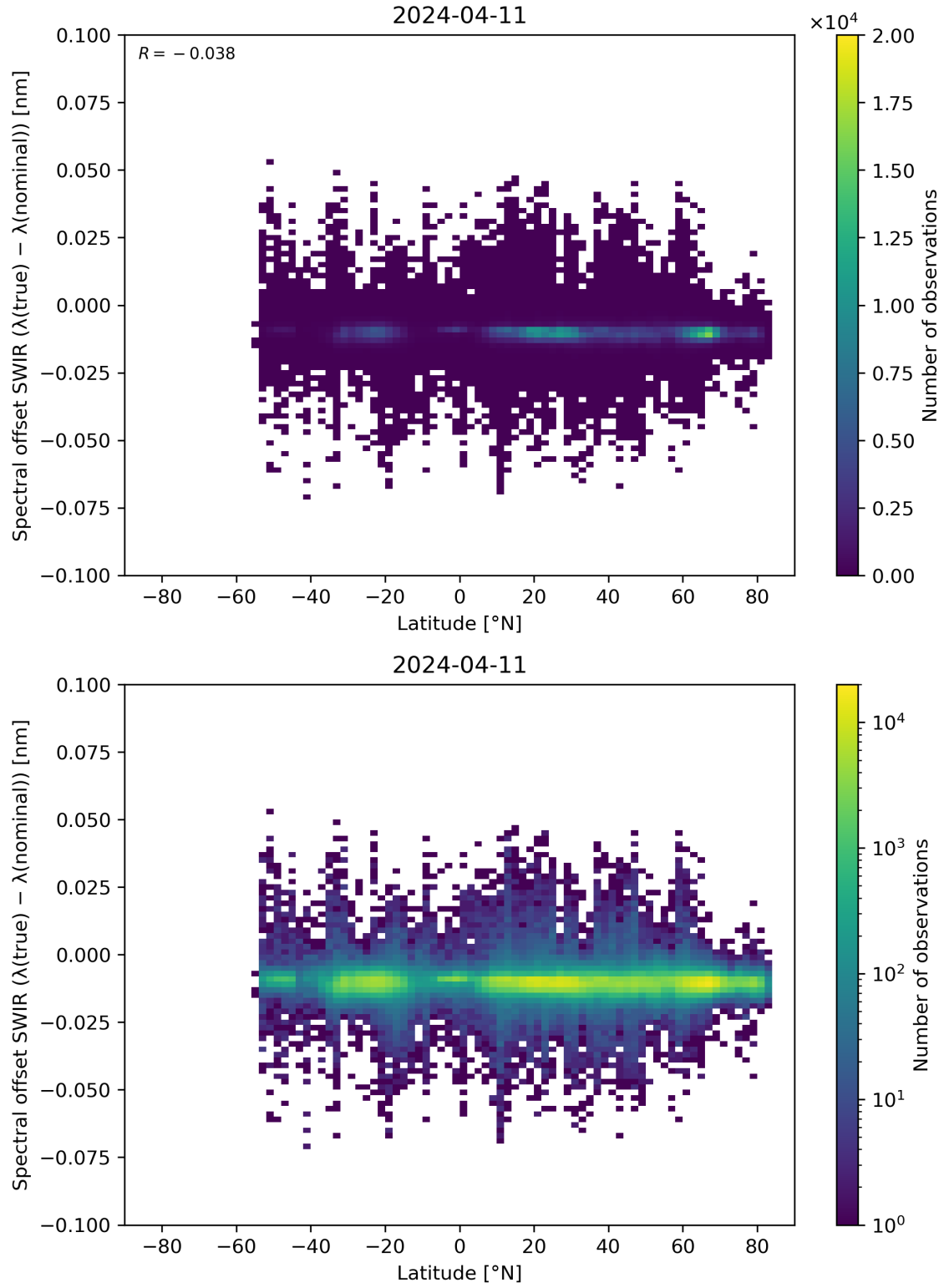
Figure 62: Scatter density plot of “Latitude” against “Spectral offset SWIR ( \lambda(\text{true}) - \lambda(\text{nominal}) )” for 2024-04-10 to 2024-04-12.
