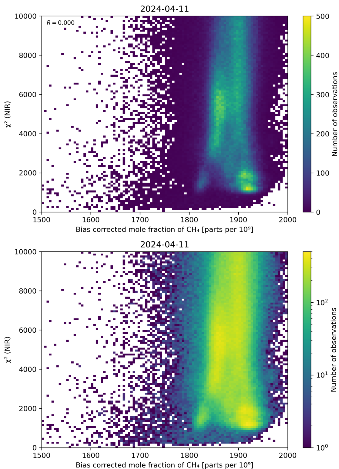
Figure 63: Scatter density plot of “Bias corrected mole fraction of CH 4 ” against “ \chi^2 (NIR)” for 2024-04-10 to 2024-04-12.
