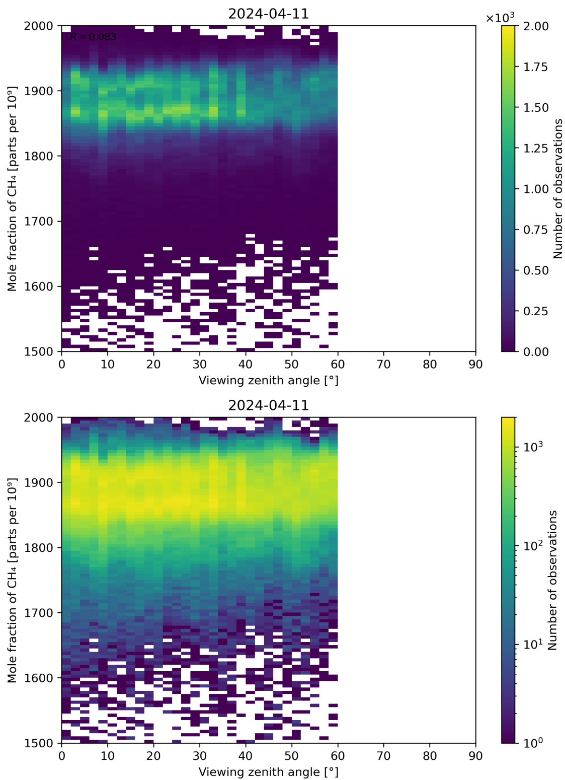
Figure 110: Scatter density plot of “Viewing zenith angle” against “Mole fraction of CH 4 ” for 2024-04-10 to 2024-04-12.
