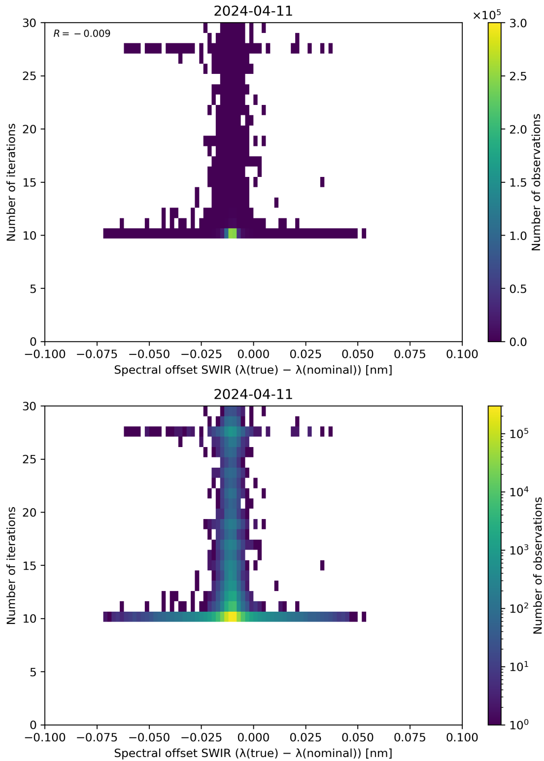
Figure 121: Scatter density plot of “Spectral offset SWIR ( \lambda(\text{true}) - \lambda(\text{nominal}) )” against “Number of iterations” for 2024-04-10 to 2024-04-12.
