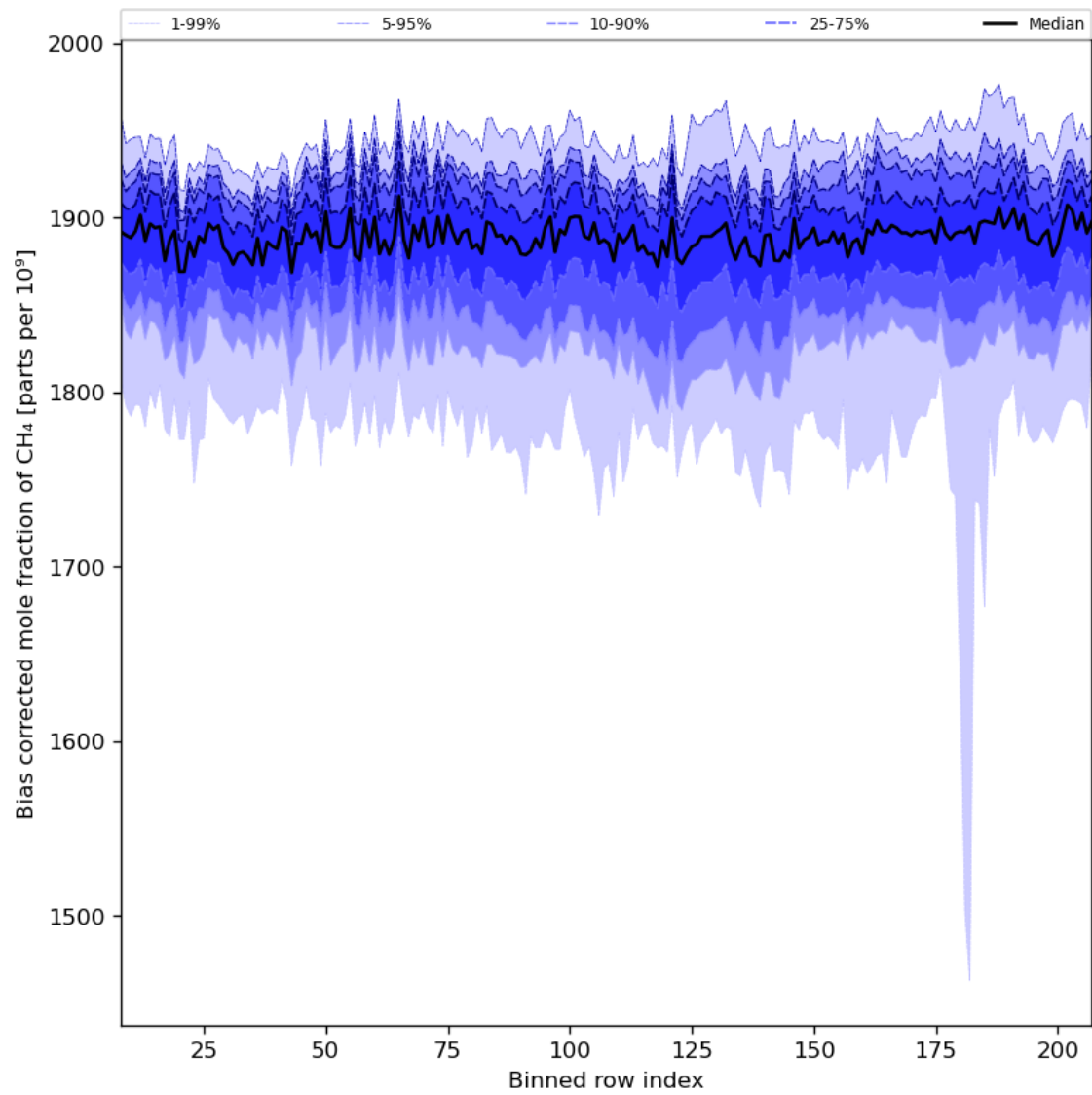
Figure 36: Along track statistics of “Bias corrected mole fraction of CH 4 ” for 2024-04-10 to 2024-04-12
