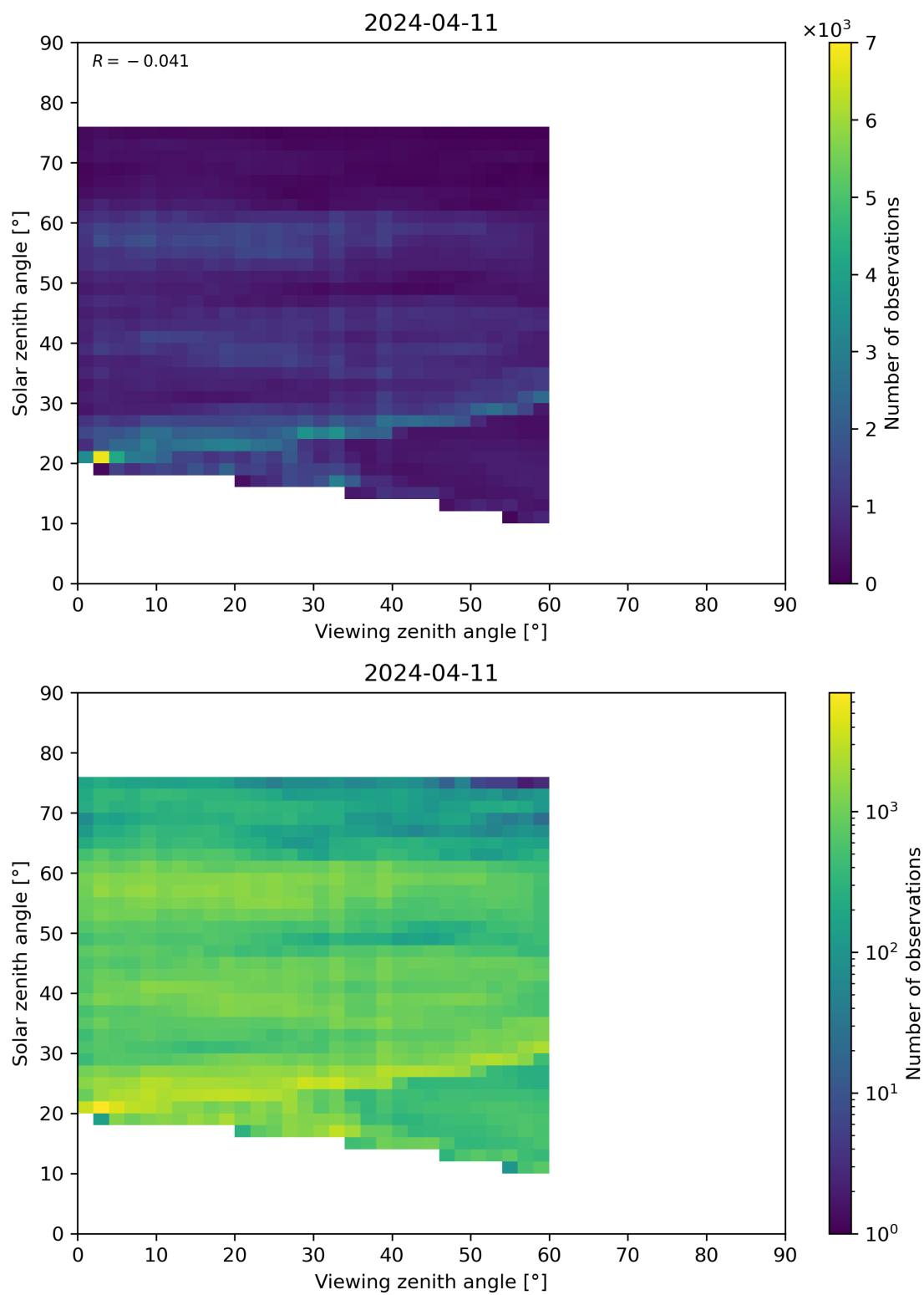
Figure 115: Scatter density plot of “Viewing zenith angle” against “Solar zenith angle” for 2024-04-10 to 2024-04-12.
