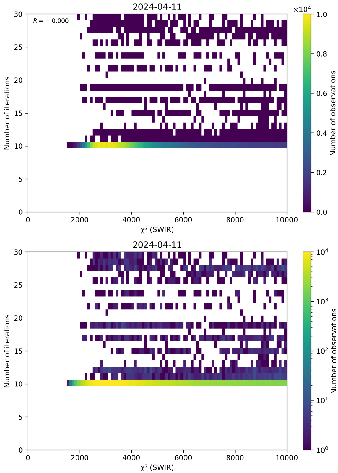
Figure 50: Scatter density plot of “ \chi^2 (SWIR)” against “Number of iterations” for 2024-04-10 to 2024-04-12.
