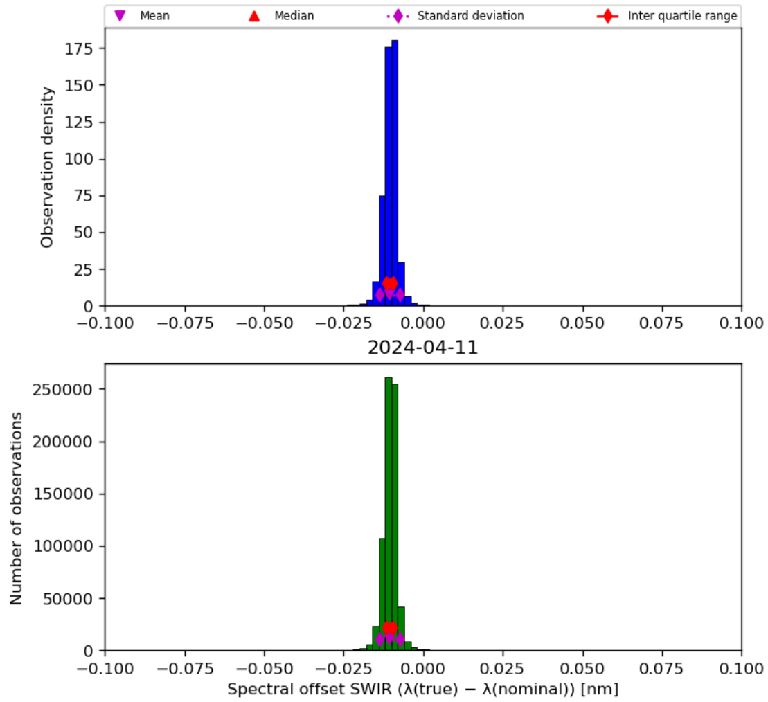
Figure 27: Histogram of “Spectral offset SWIR ( \lambda(\text{true}) - \lambda(\text{nominal}) )” for 2024-04-10 to 2024-04-12
