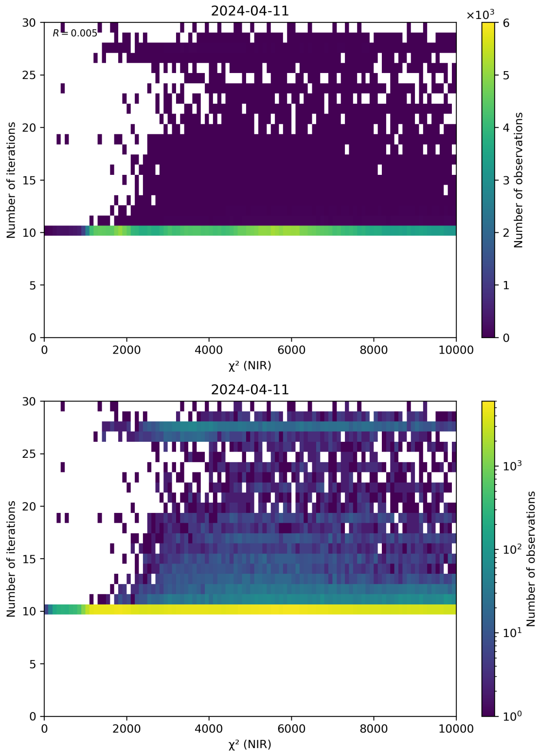
Figure 46: Scatter density plot of “ \chi^2 (NIR)” against “Number of iterations” for 2024-04-10 to 2024-04-12.
