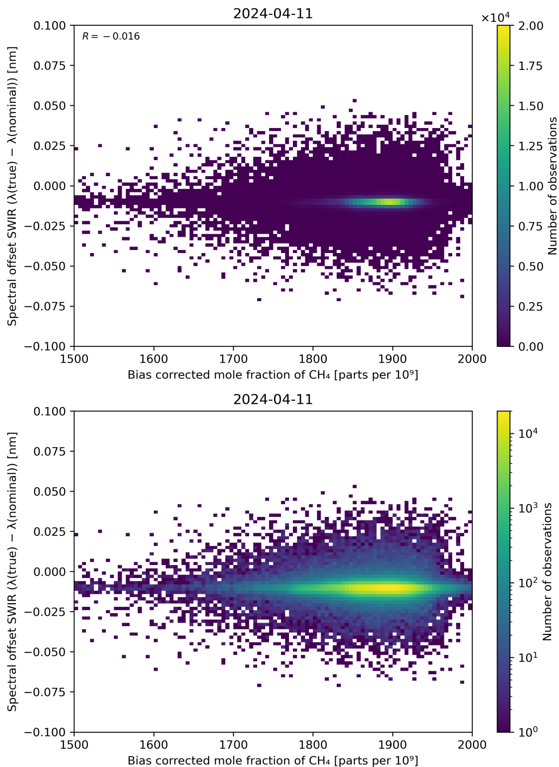
Figure 69: Scatter density plot of “Bias corrected mole fraction of \text{CH}_4 ” against “Spectral offset SWIR ( \lambda(\text{true}) - \lambda(\text{nominal}) )” for 2024-04-10 to 2024-04-12.
