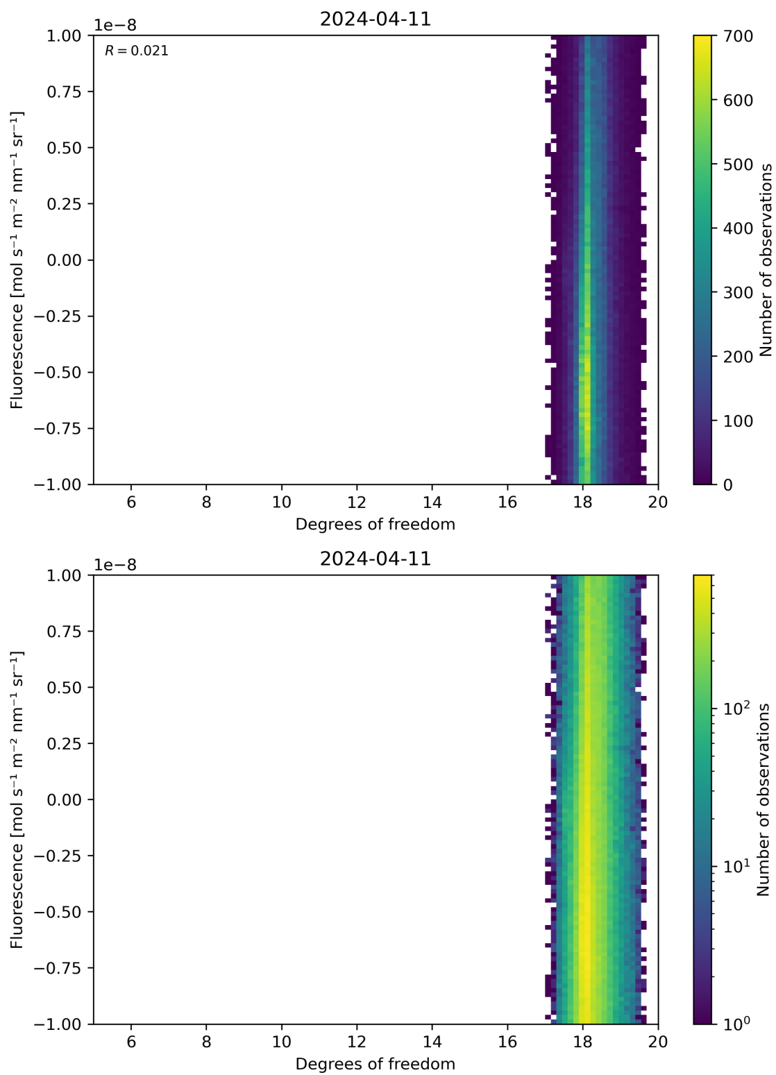
Figure 51: Scatter density plot of “Degrees of freedom” against “Fluorescence” for 2024-04-10 to 2024-04-12.
