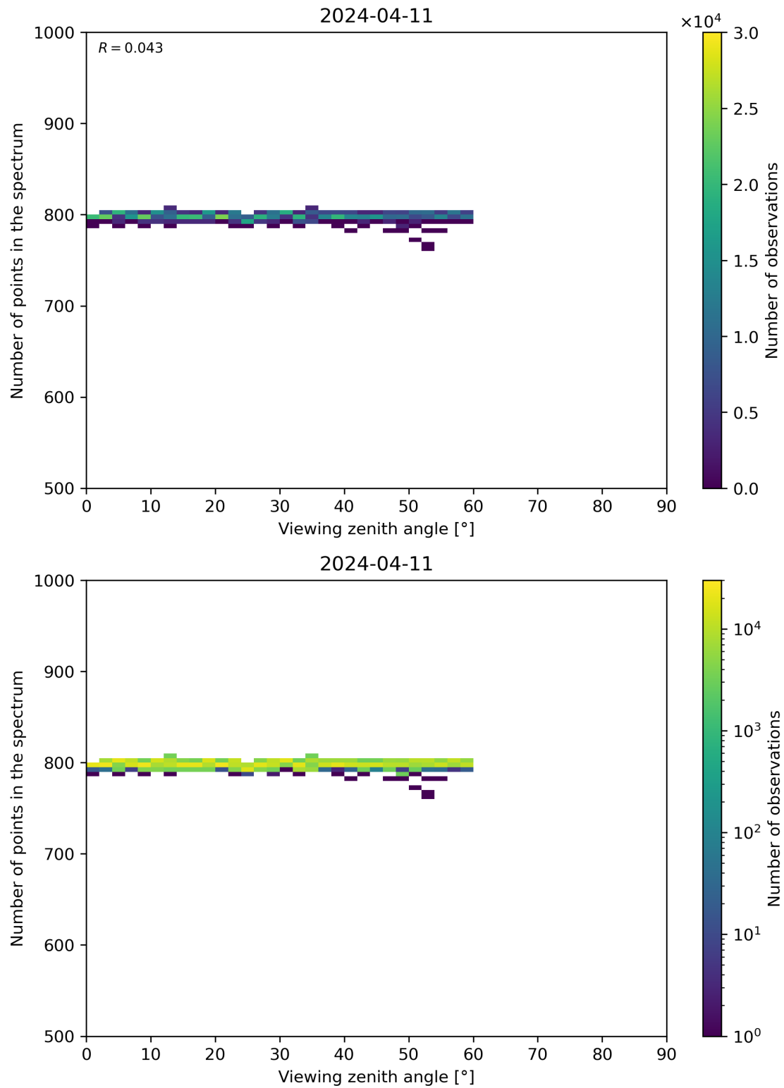
Figure 114: Scatter density plot of “Viewing zenith angle” against “Number of points in the spectrum” for 2024-04-10 to 2024-04-12.
