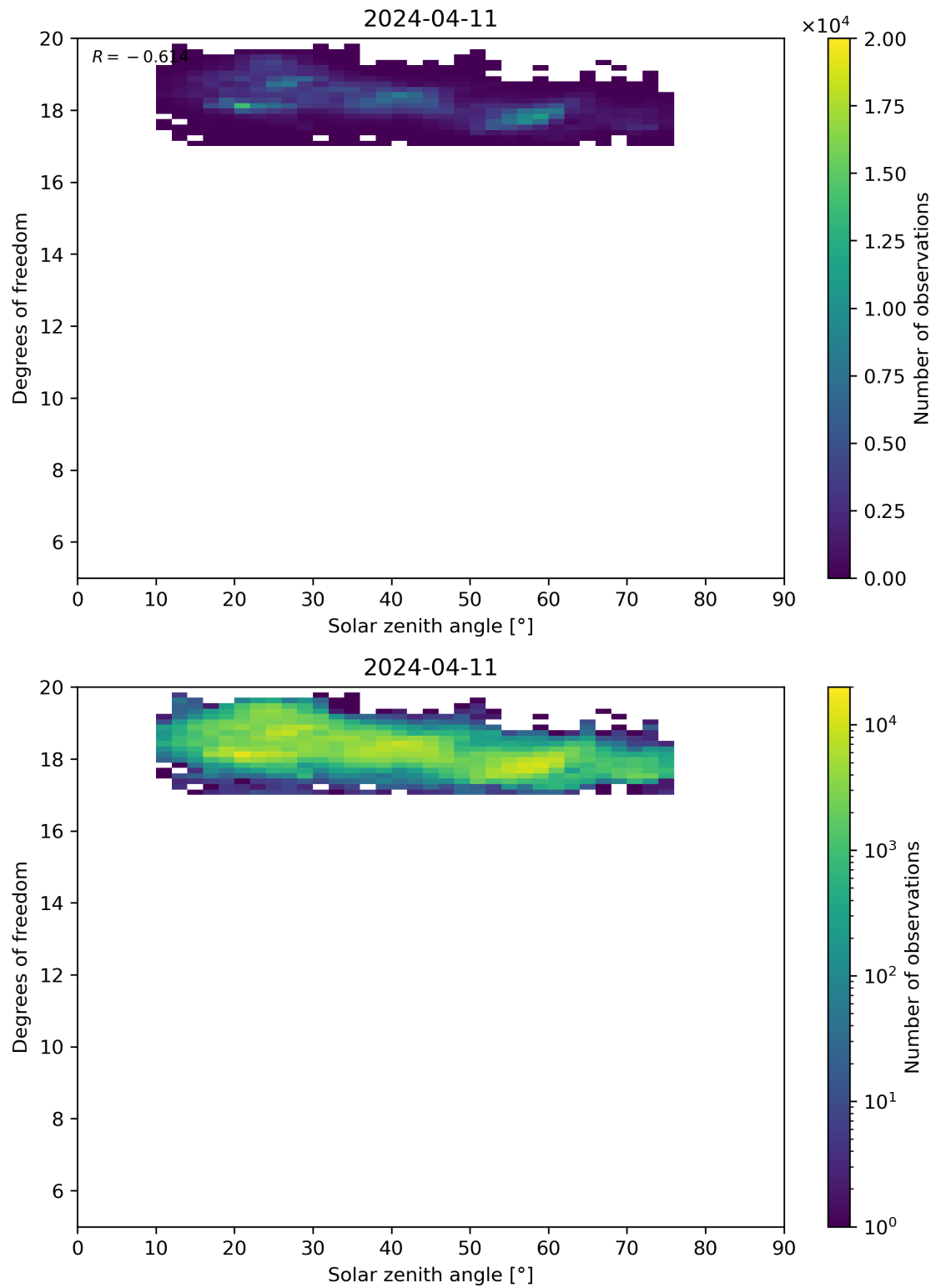
Figure 96: Scatter density plot of “Solar zenith angle” against “Degrees of freedom” for 2024-04-10 to 2024-04-12.
