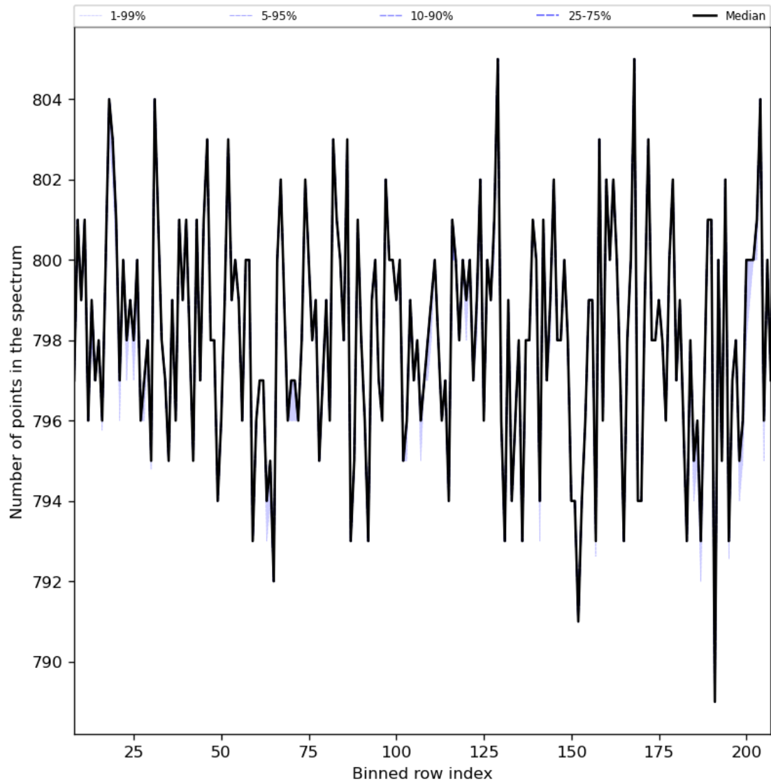
Figure 37: Along track statistics of “Number of points in the spectrum” for 2024-04-10 to 2024-04-12
