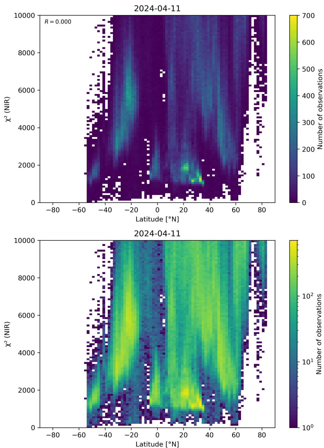
Figure 53: Scatter density plot of “Latitude” against “ \chi^2 (NIR)” for 2024-04-10 to 2024-04-12.
