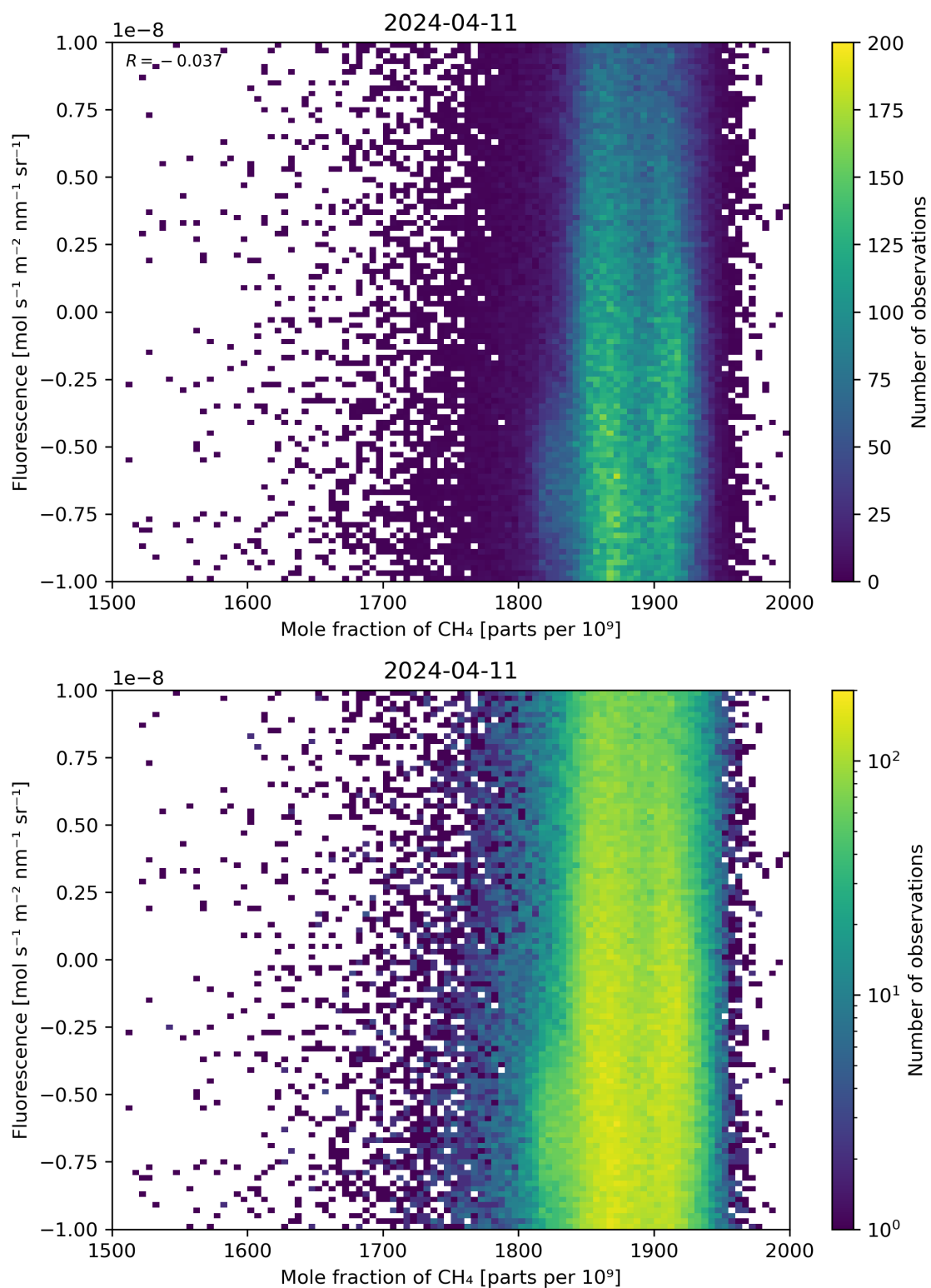
Figure 73: Scatter density plot of “Mole fraction of \text{CH}_4 ” against “Fluorescence” for 2024-04-10 to 2024-04-12.
