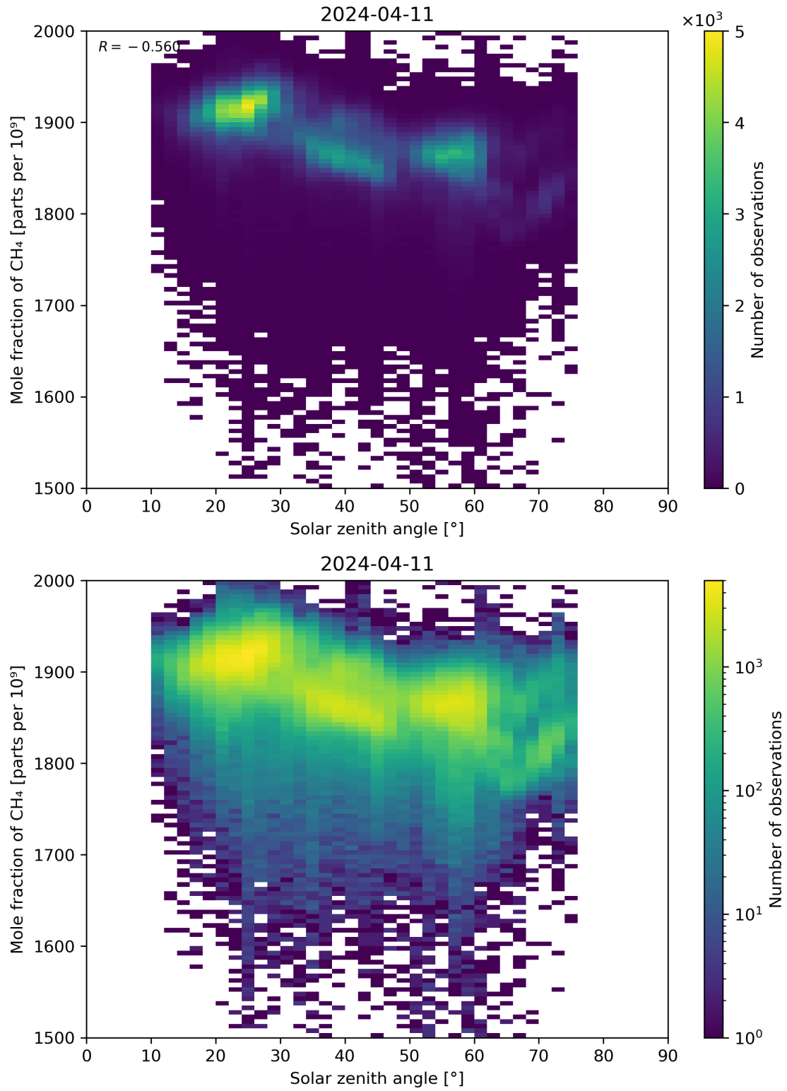
Figure 99: Scatter density plot of “Solar zenith angle” against “Mole fraction of CH 4 ” for 2024-04-10 to 2024-04-12.
