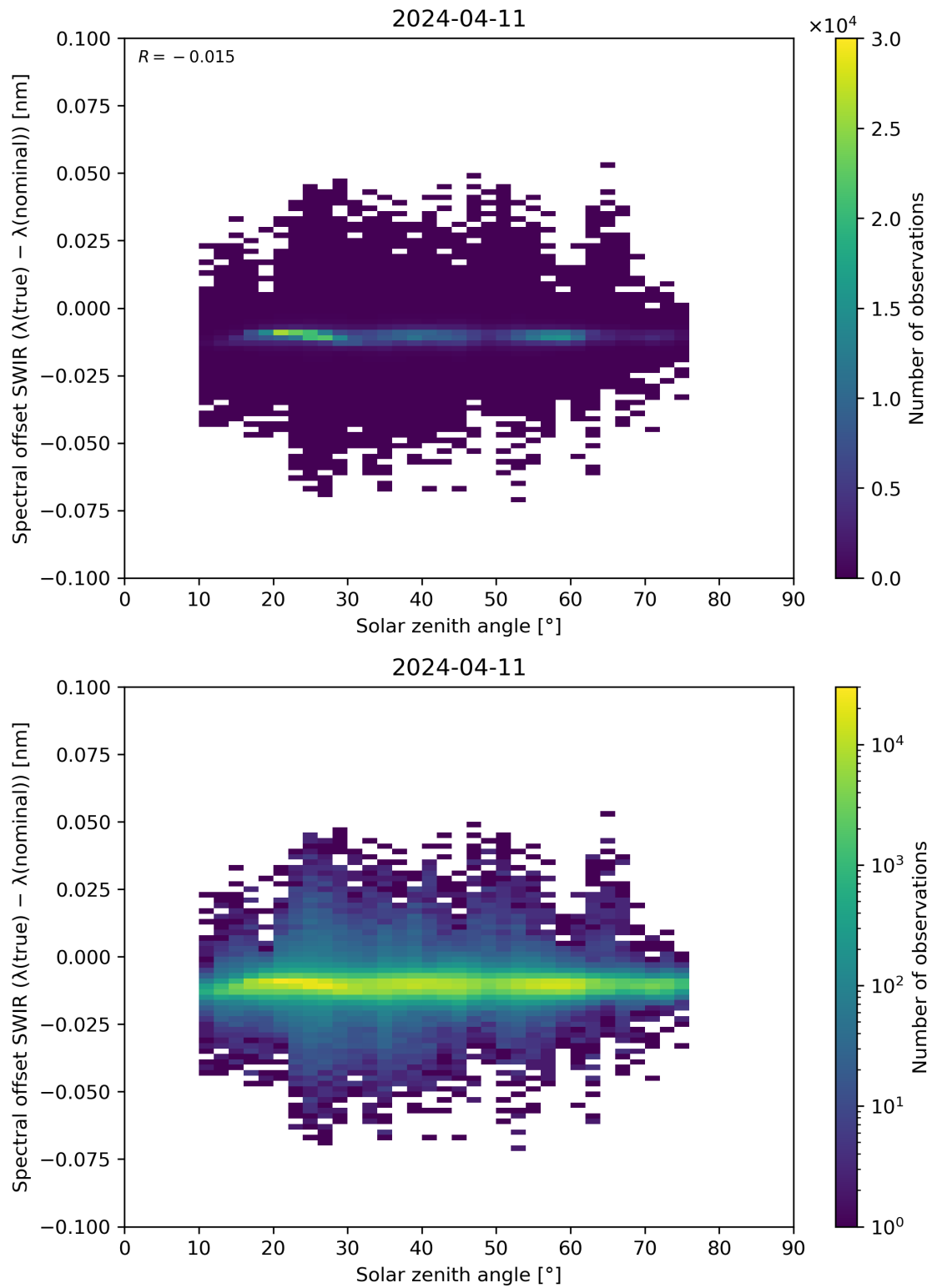
Figure 104: Scatter density plot of “Solar zenith angle” against “Spectral offset SWIR ( \lambda(\text{true}) - \lambda(\text{nominal}) )” for 2024-04-10 to 2024-04-12.
