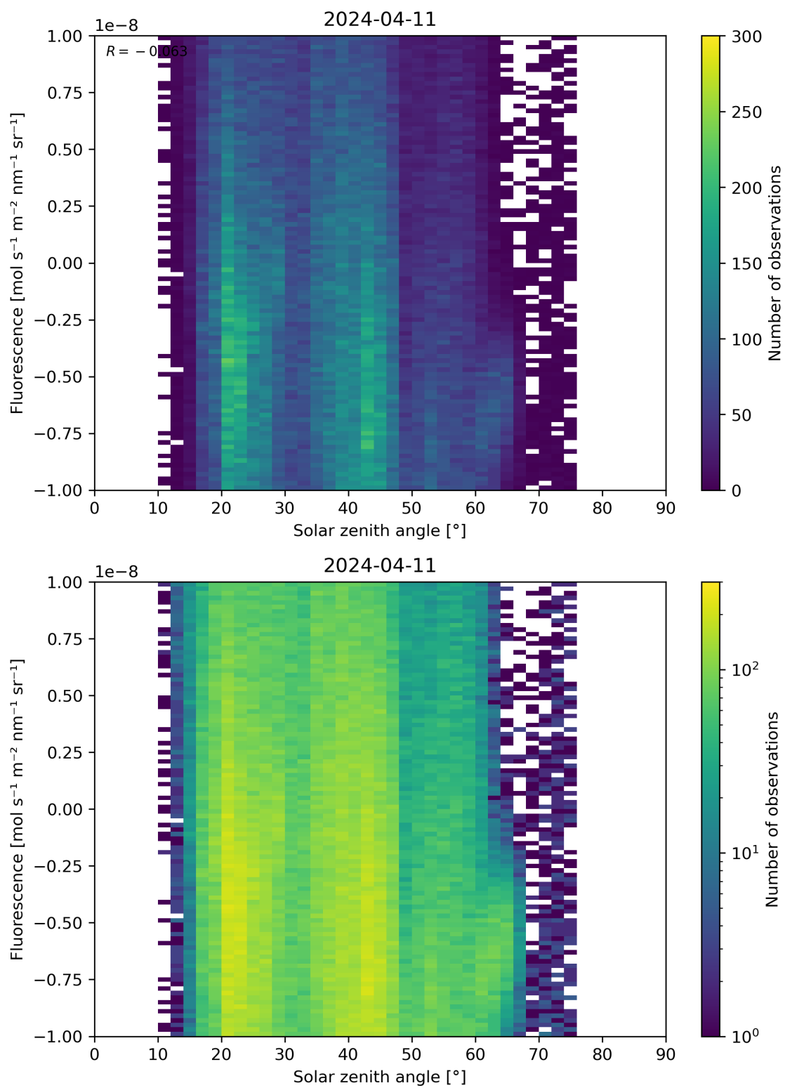
Figure 97: Scatter density plot of “Solar zenith angle” against “Fluorescence” for 2024-04-10 to 2024-04-12.
