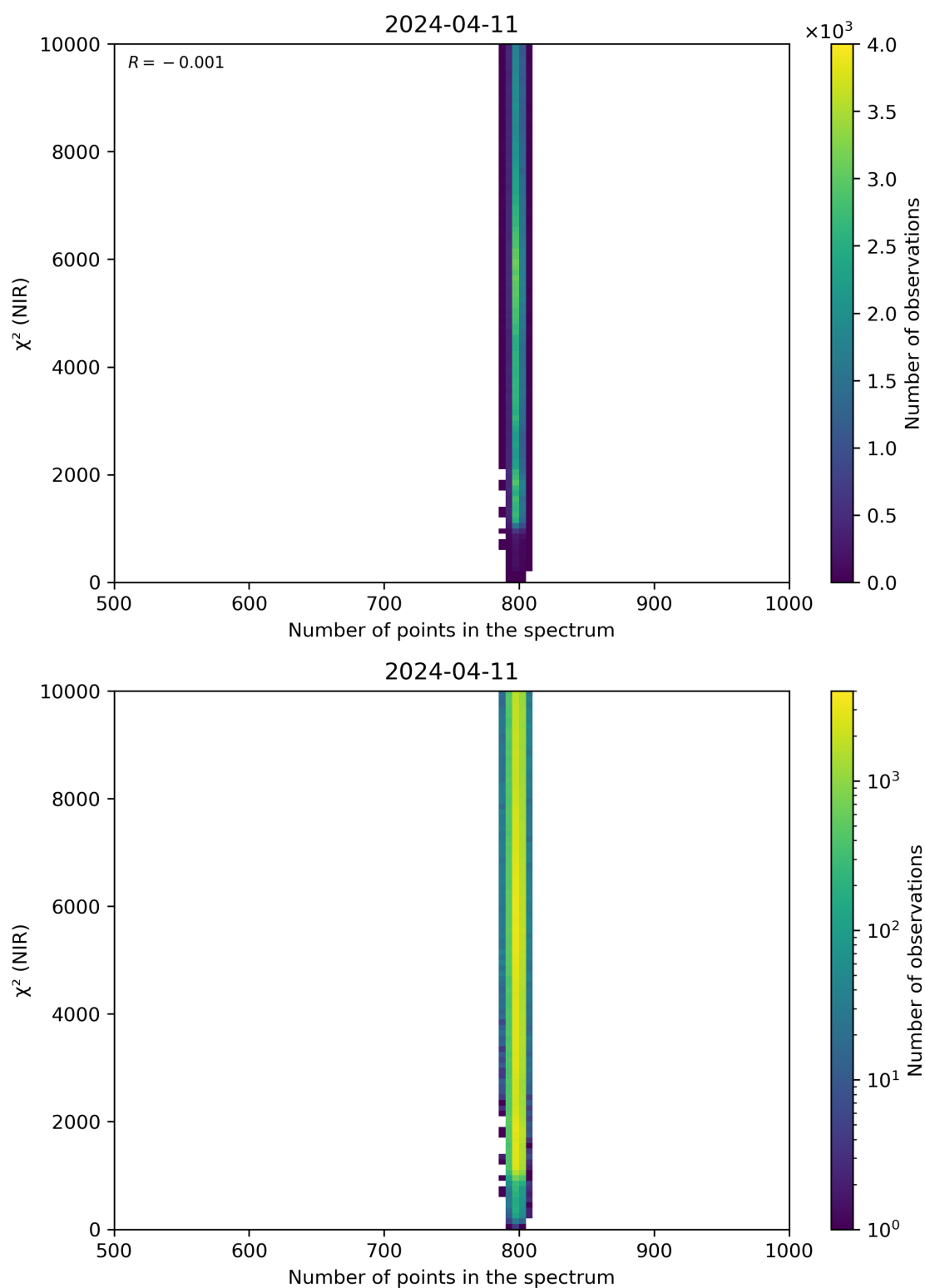
Figure 88: Scatter density plot of “Number of points in the spectrum” against “ \chi^2 (NIR)” for 2024-04-10 to 2024-04-12.
