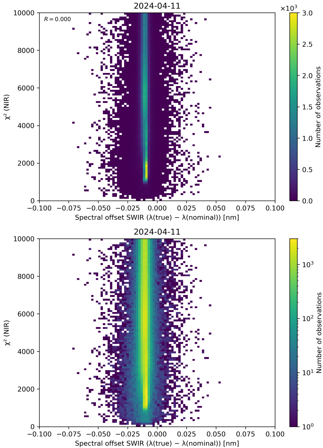
Figure 117: Scatter density plot of “Spectral offset SWIR ( \lambda(\text{true}) - \lambda(\text{nominal}) )” against “ \chi^2 (NIR)” for 2024-04-10 to 2024-04-12.
