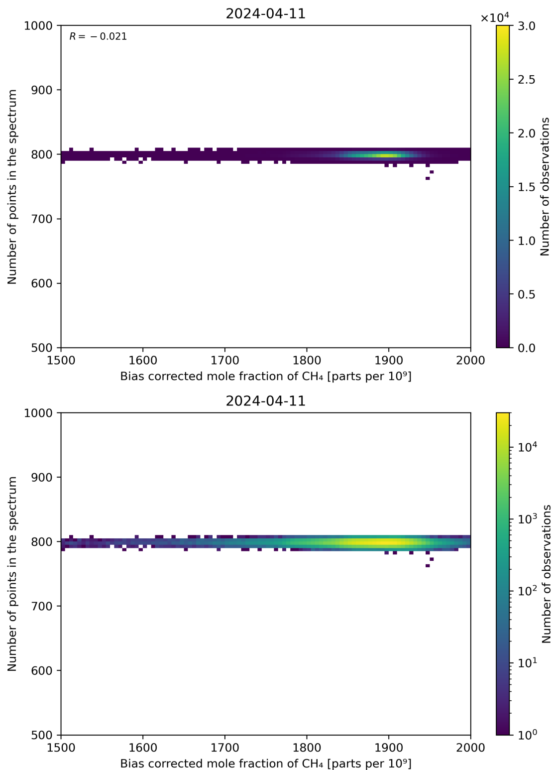
Figure 68: Scatter density plot of “Bias corrected mole fraction of CH 4 ” against “Number of points in the spectrum” for 2024-04-10 to 2024-04-12.
