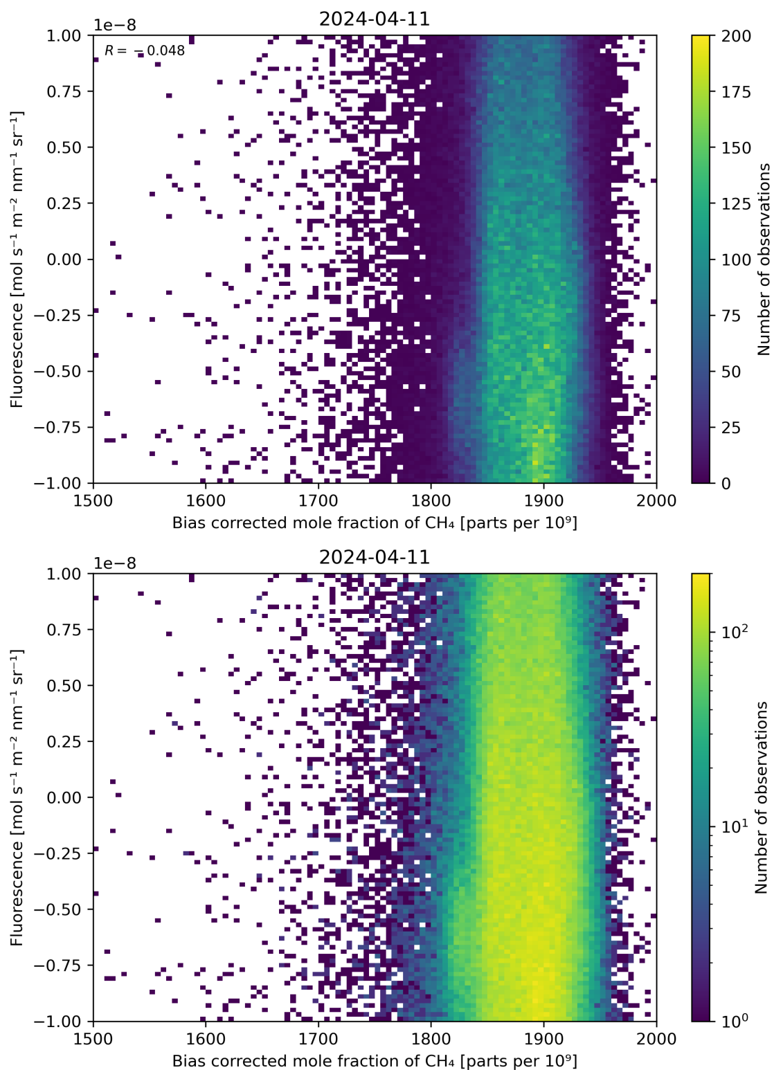
Figure 66: Scatter density plot of “Bias corrected mole fraction of \text{CH}_4 ” against “Fluorescence” for 2024-04-10 to 2024-04-12.
