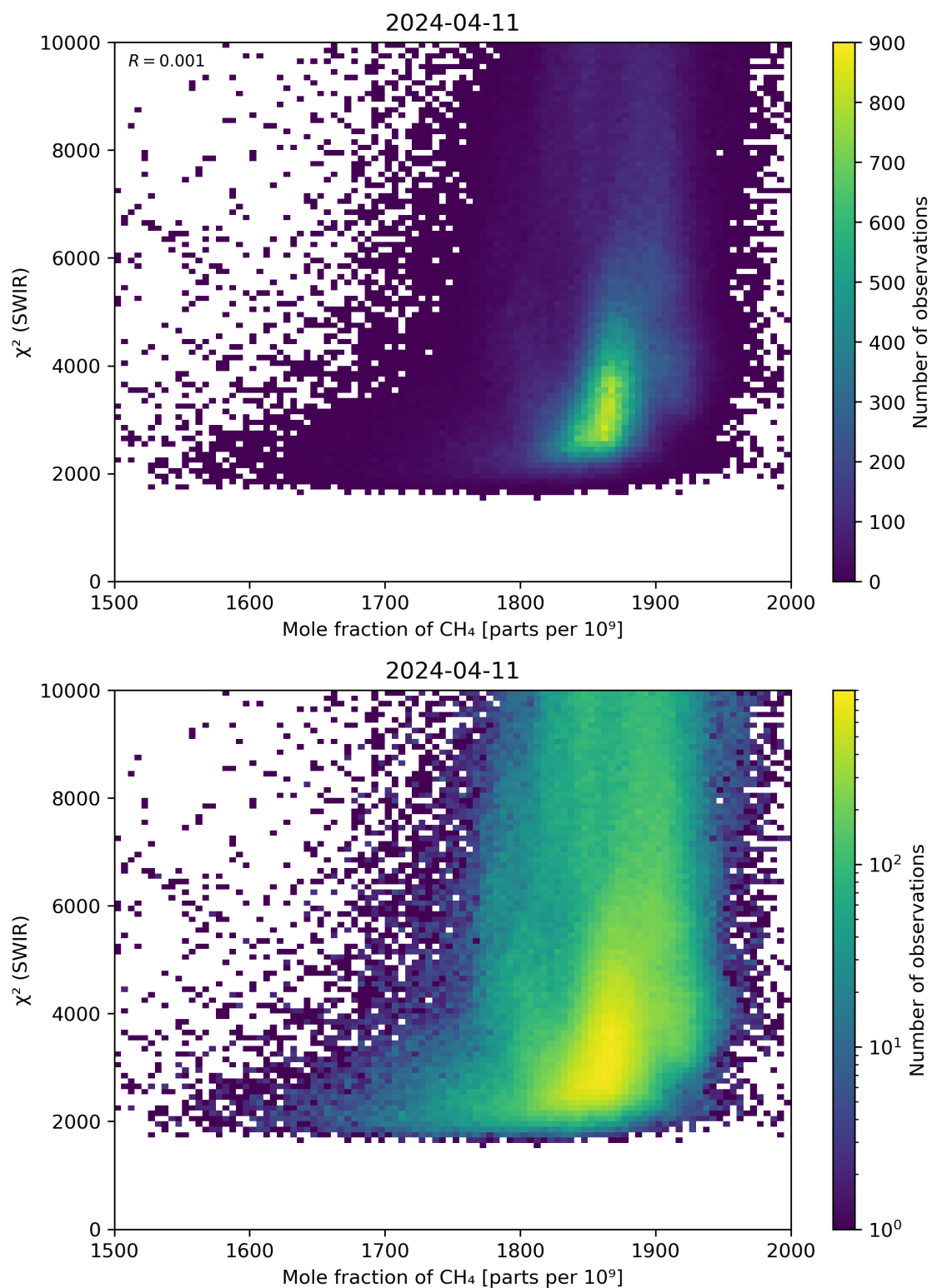
Figure 71: Scatter density plot of “Mole fraction of \text{CH}_4 ” against “ \chi^2 (SWIR)” for 2024-04-10 to 2024-04-12.
