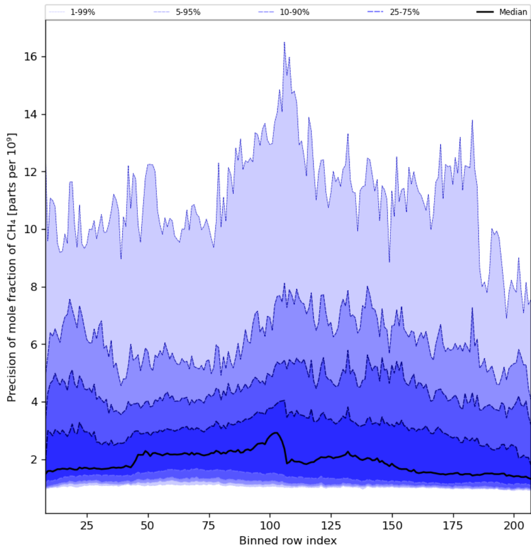
Figure 35: Along track statistics of “Precision of mole fraction of CH 4 ” for 2024-04-10 to 2024-04-12
