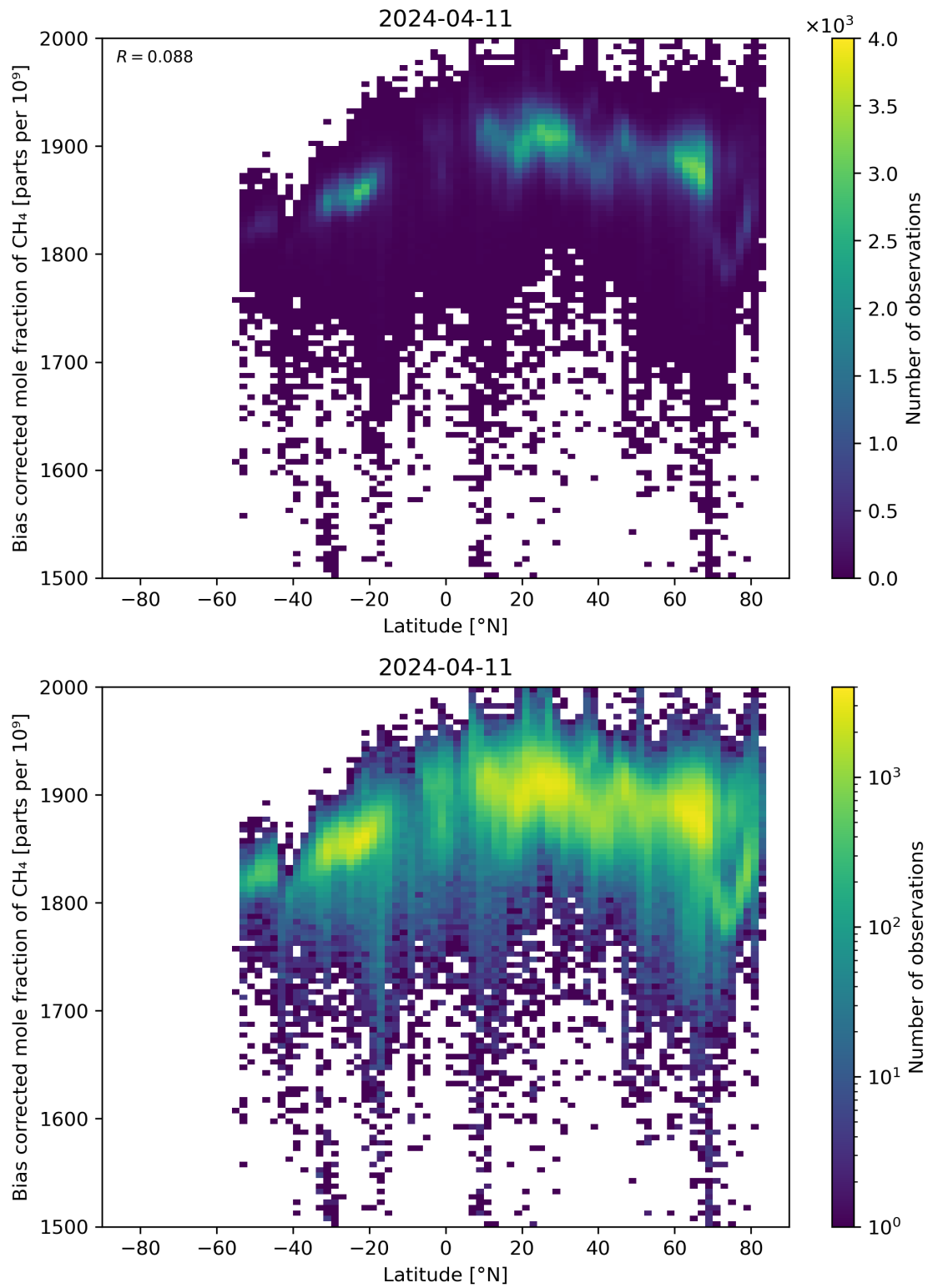
Figure 58: Scatter density plot of “Latitude” against “Bias corrected mole fraction of \text{CH}_4 ” for 2024-04-10 to 2024-04-12.
