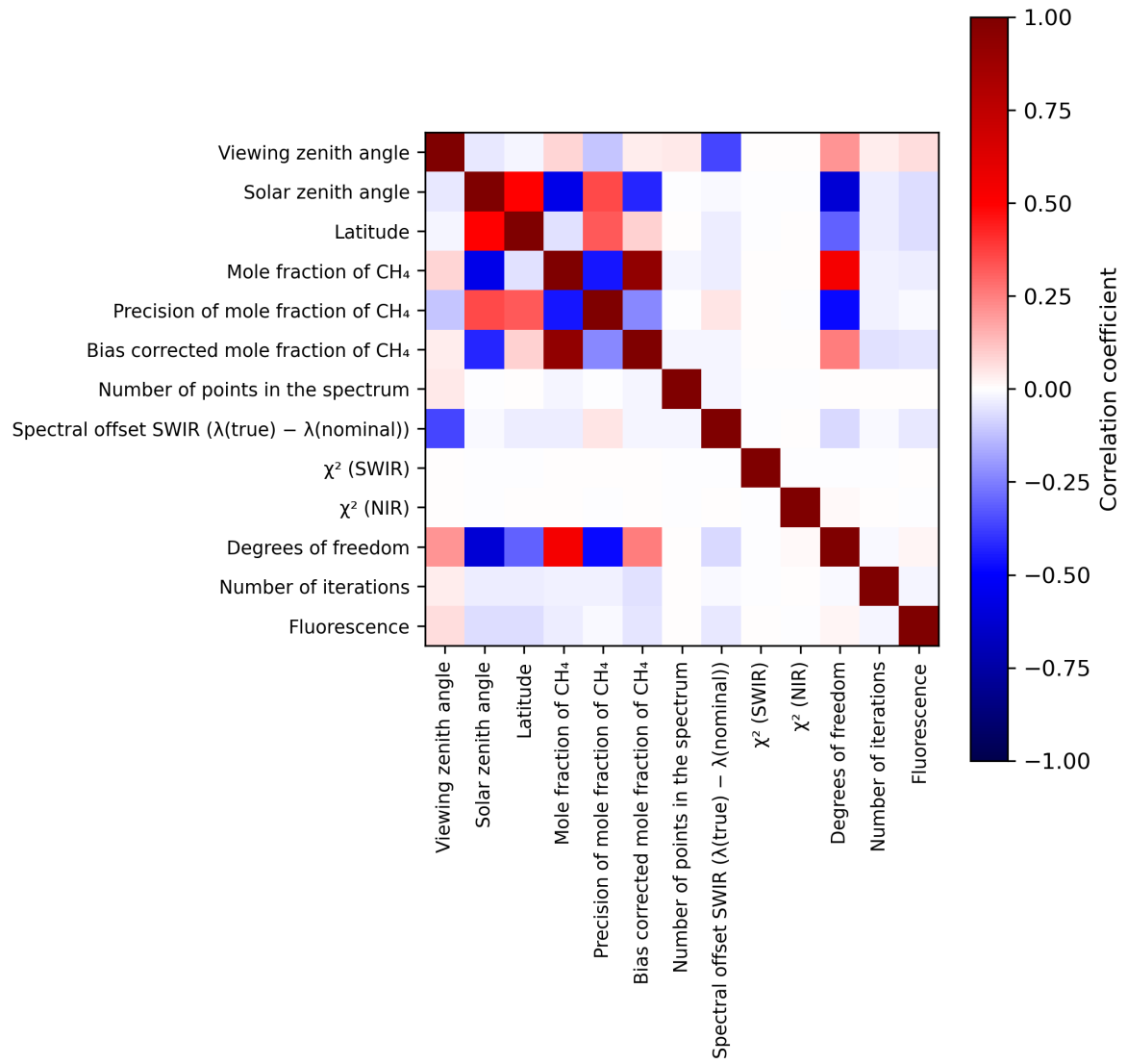
Figure 2: Map of correlation matrix for 2024-04-10 to 2024-04-12.
