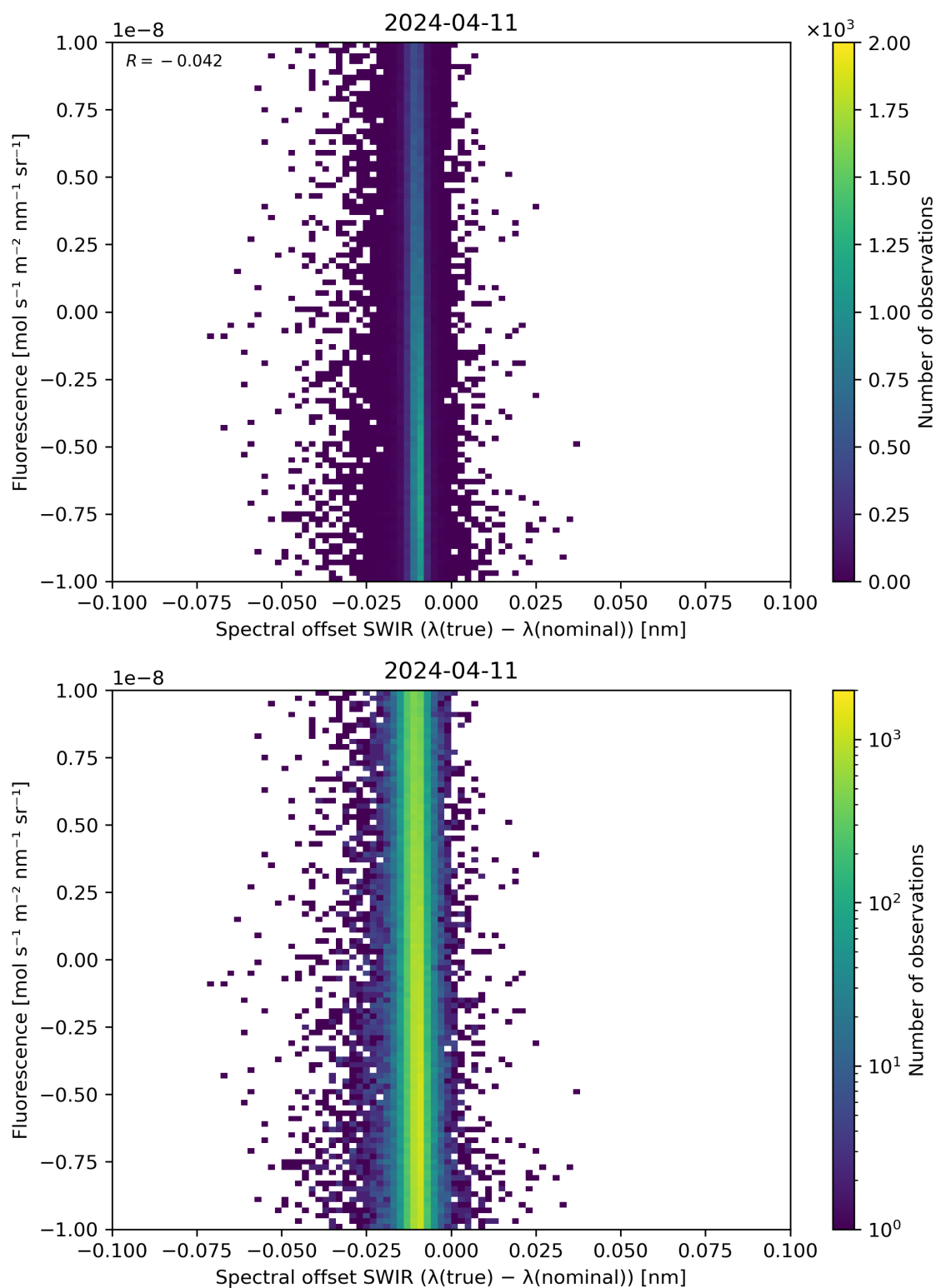
Figure 120: Scatter density plot of “Spectral offset SWIR ( \lambda(\text{true}) - \lambda(\text{nominal}) )” against “Fluorescence” for 2024-04-10 to 2024-04-12.
