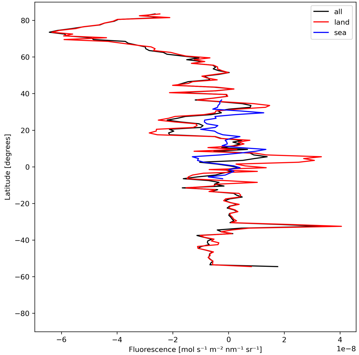
Figure 21: Zonal average of “Fluorescence” for 2024-04-10 to 2024-04-12.
