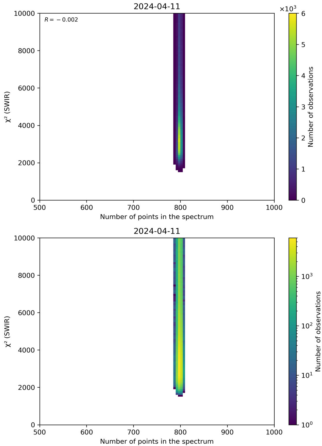
Figure 89: Scatter density plot of “Number of points in the spectrum” against “ \chi^2 (SWIR)” for 2024-04-10 to 2024-04-12.
