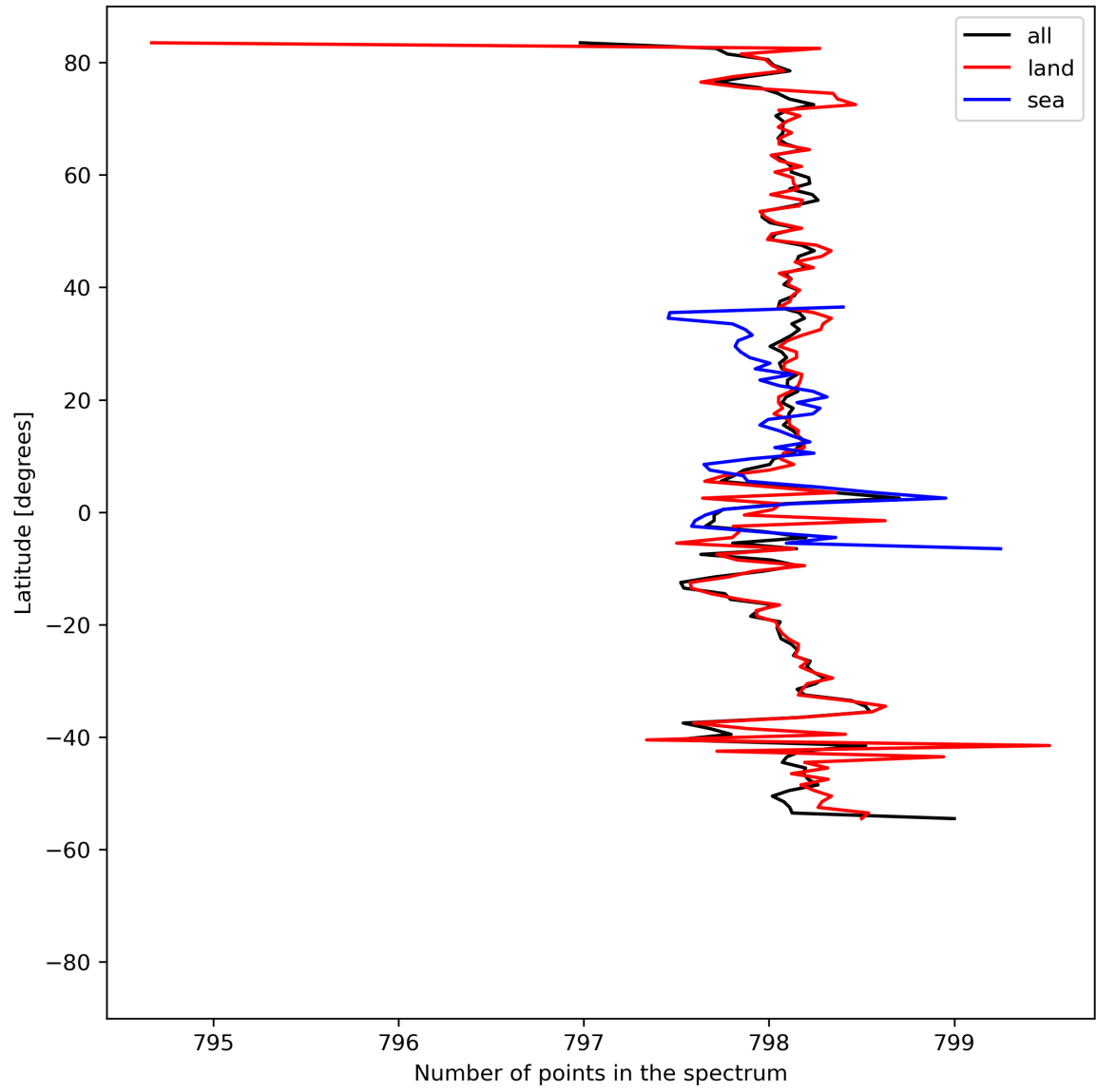
Figure 15: Zonal average of “Number of points in the spectrum” for 2024-04-10 to 2024-04-12.
