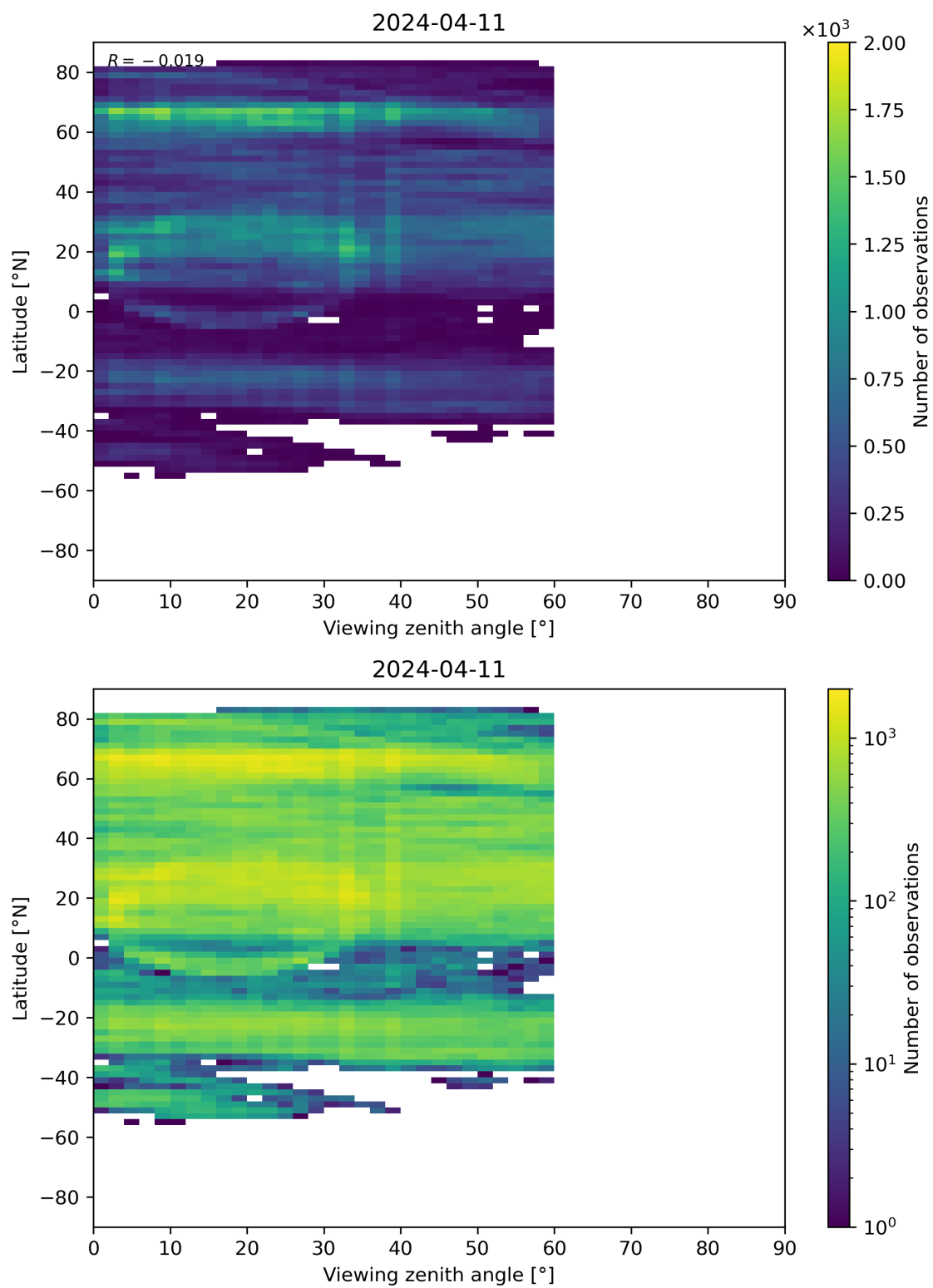
Figure 109: Scatter density plot of “Viewing zenith angle” against “Latitude” for 2024-04-10 to 2024-04-12.
