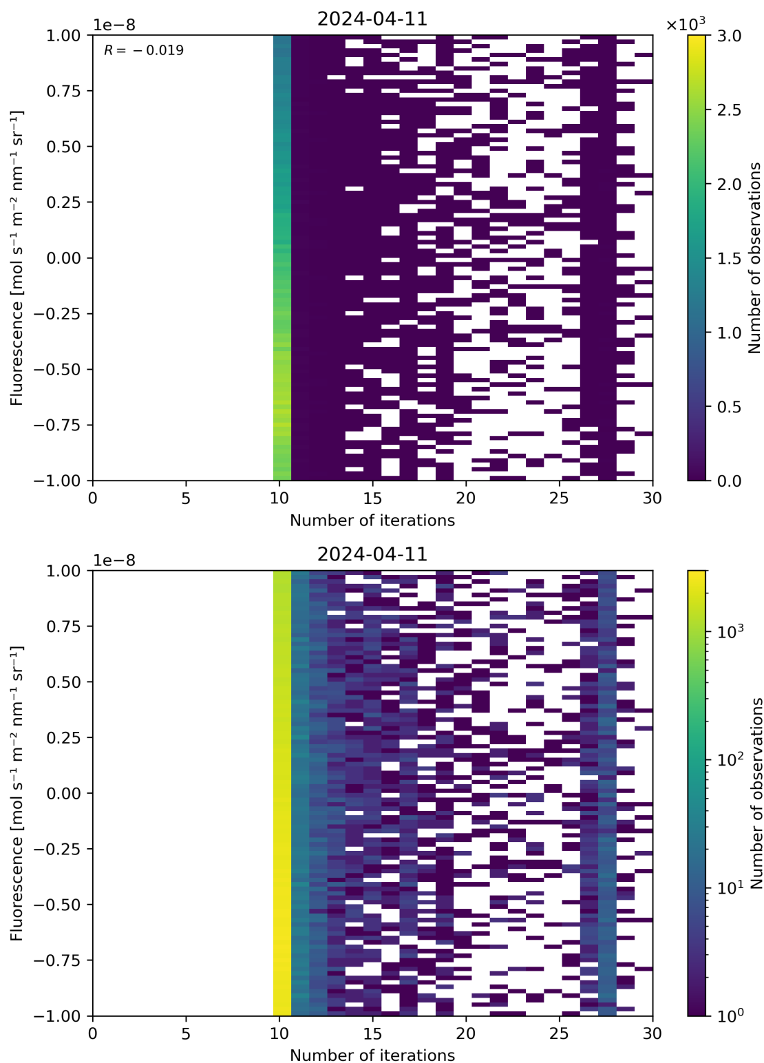
Figure 87: Scatter density plot of “Number of iterations” against “Fluorescence” for 2024-04-10 to 2024-04-12.
