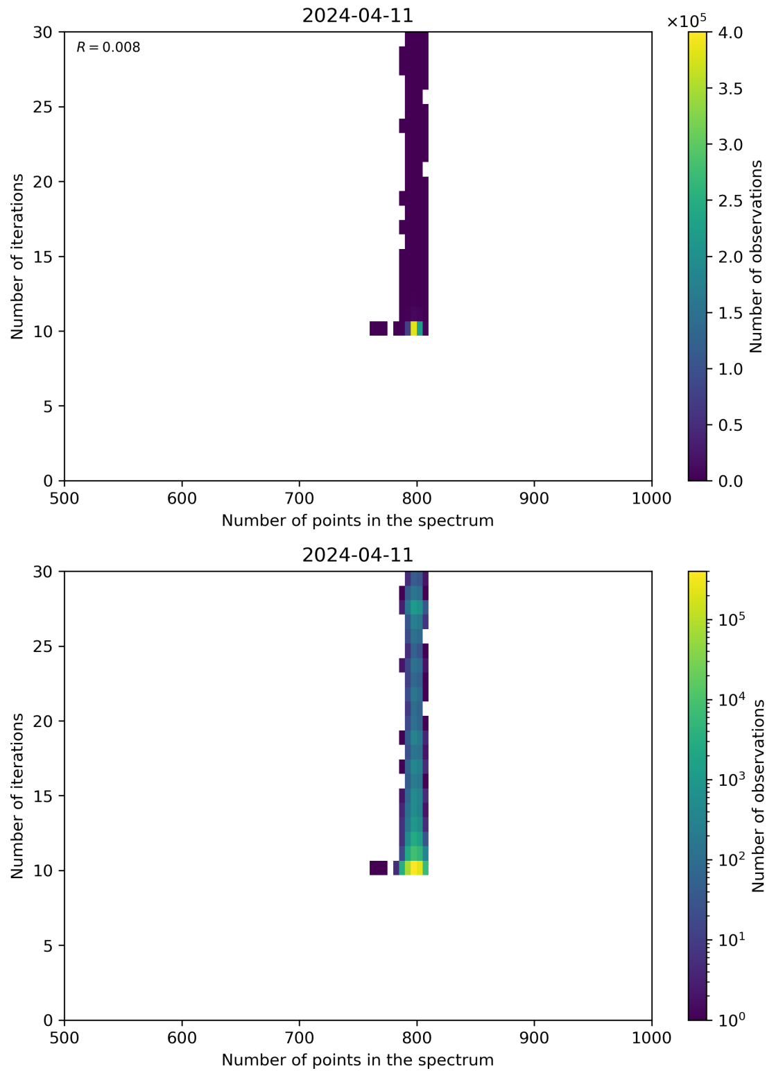
Figure 92: Scatter density plot of “Number of points in the spectrum” against “Number of iterations” for 2024-04-10 to 2024-04-12.
