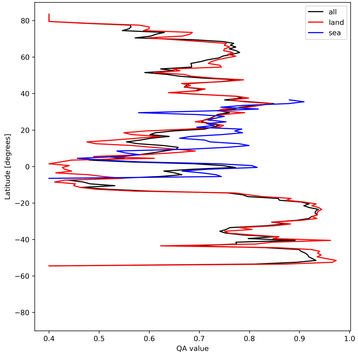
Figure 11: Zonal average of “QA value” for 2024-04-10 to 2024-04-12.
