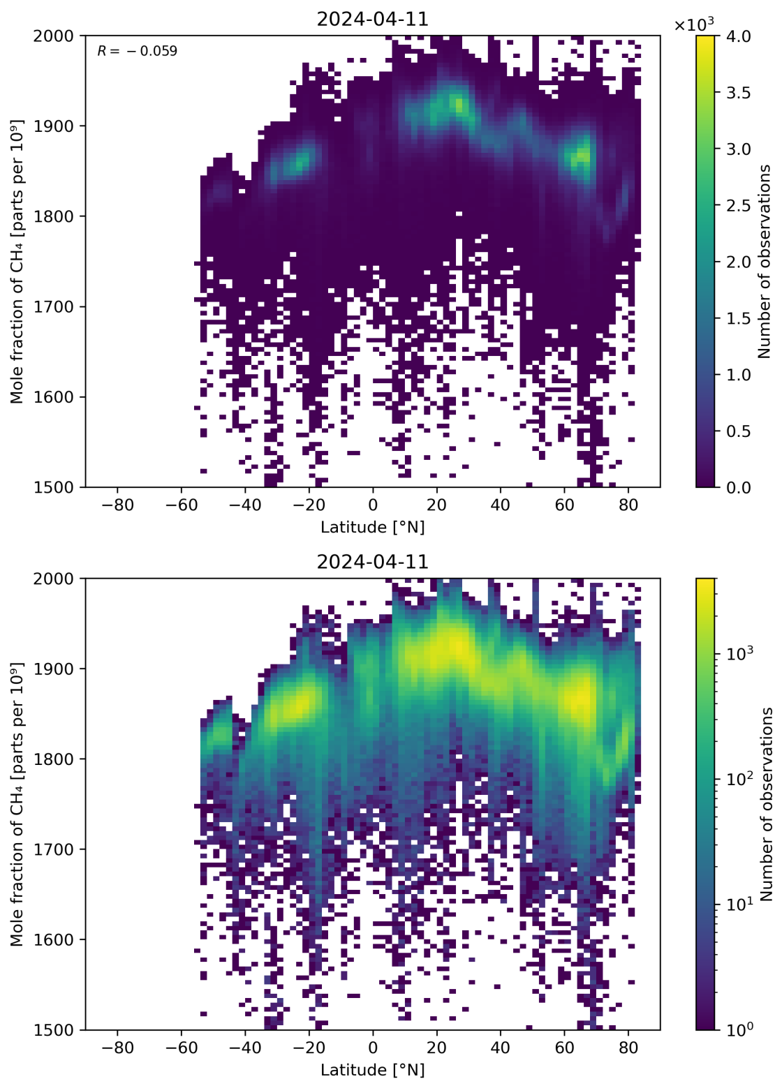
Figure 57: Scatter density plot of “Latitude” against “Mole fraction of CH 4 ” for 2024-04-10 to 2024-04-12.
