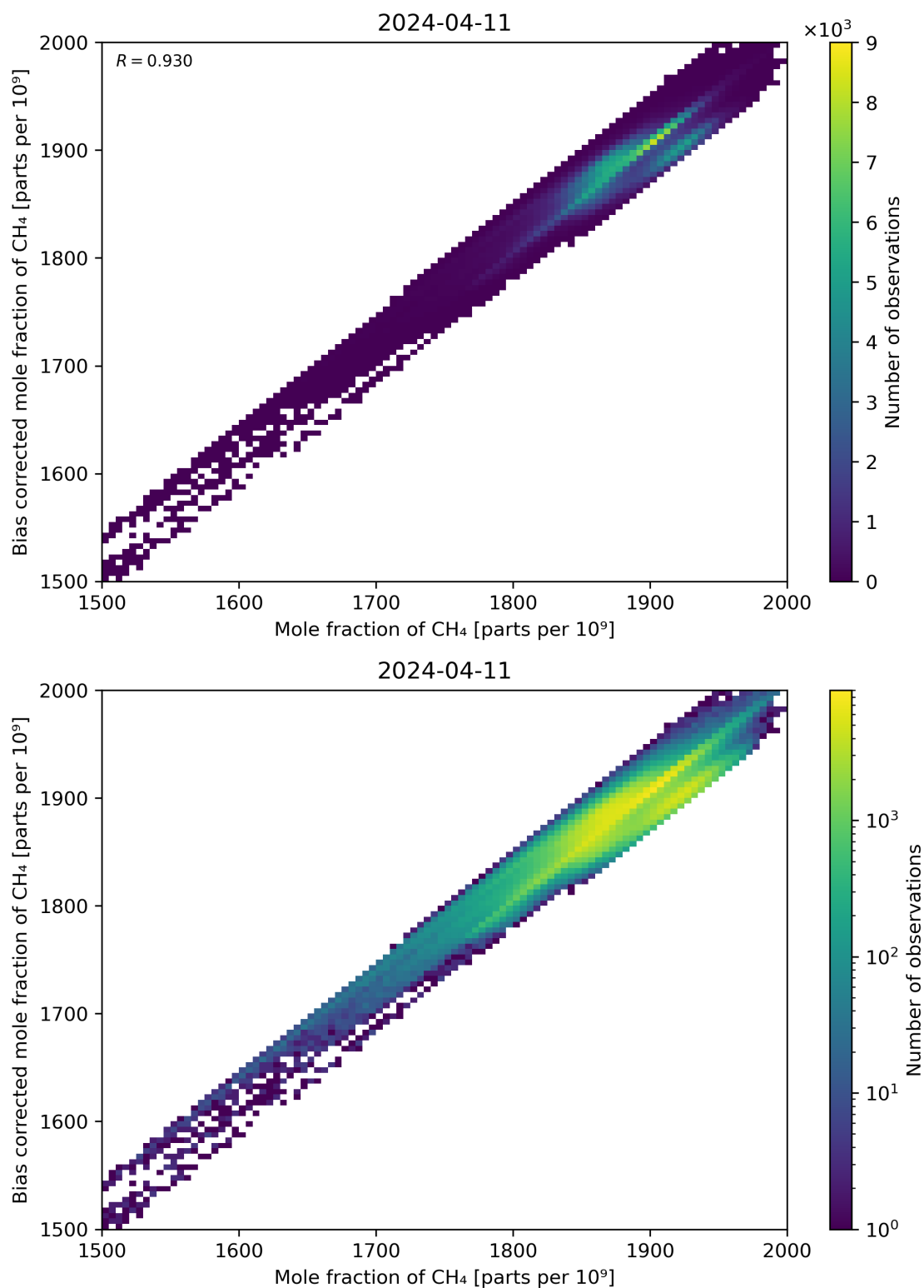
Figure 74: Scatter density plot of “Mole fraction of CH 4 ” against “Bias corrected mole fraction of CH 4 ” for 2024-04-10 to 2024-04-12.
