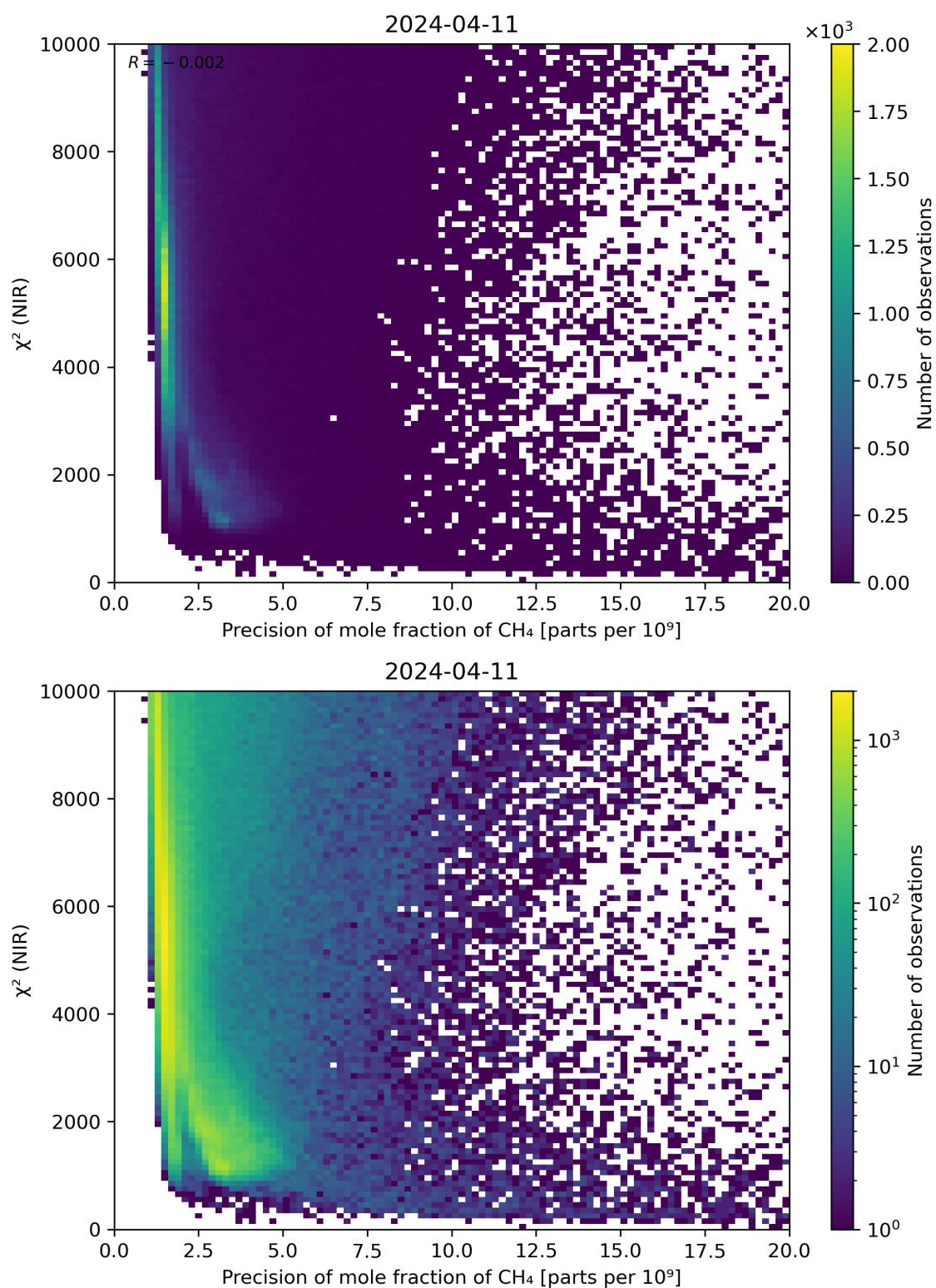
Figure 78: Scatter density plot of “Precision of mole fraction of CH 4 ” against “ \chi^2 (NIR)” for 2024-04-10 to 2024-04-12.
