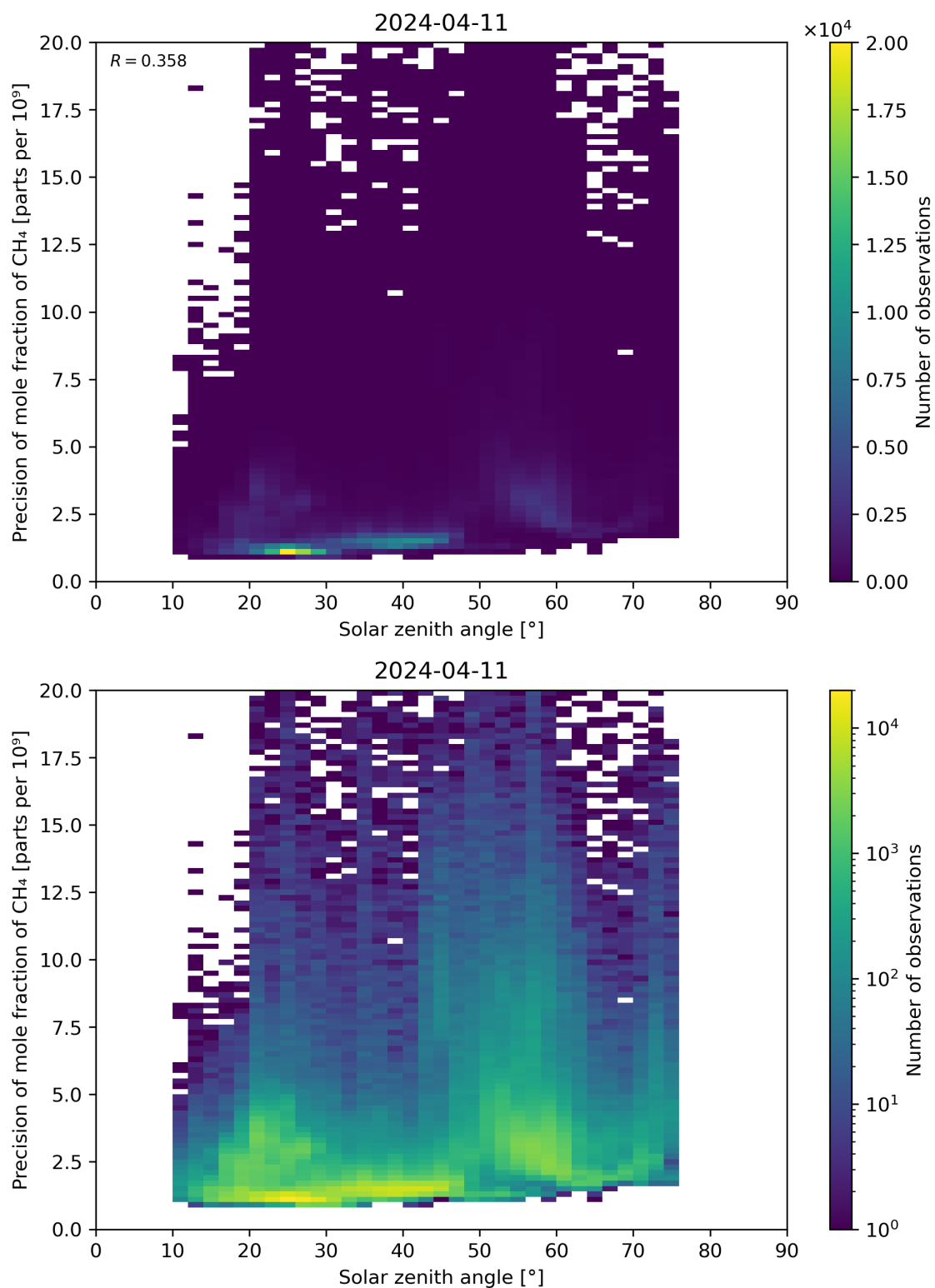
Figure 101: Scatter density plot of “Solar zenith angle” against “Precision of mole fraction of CH 4 ” for 2024-04-10 to 2024-04-12.
