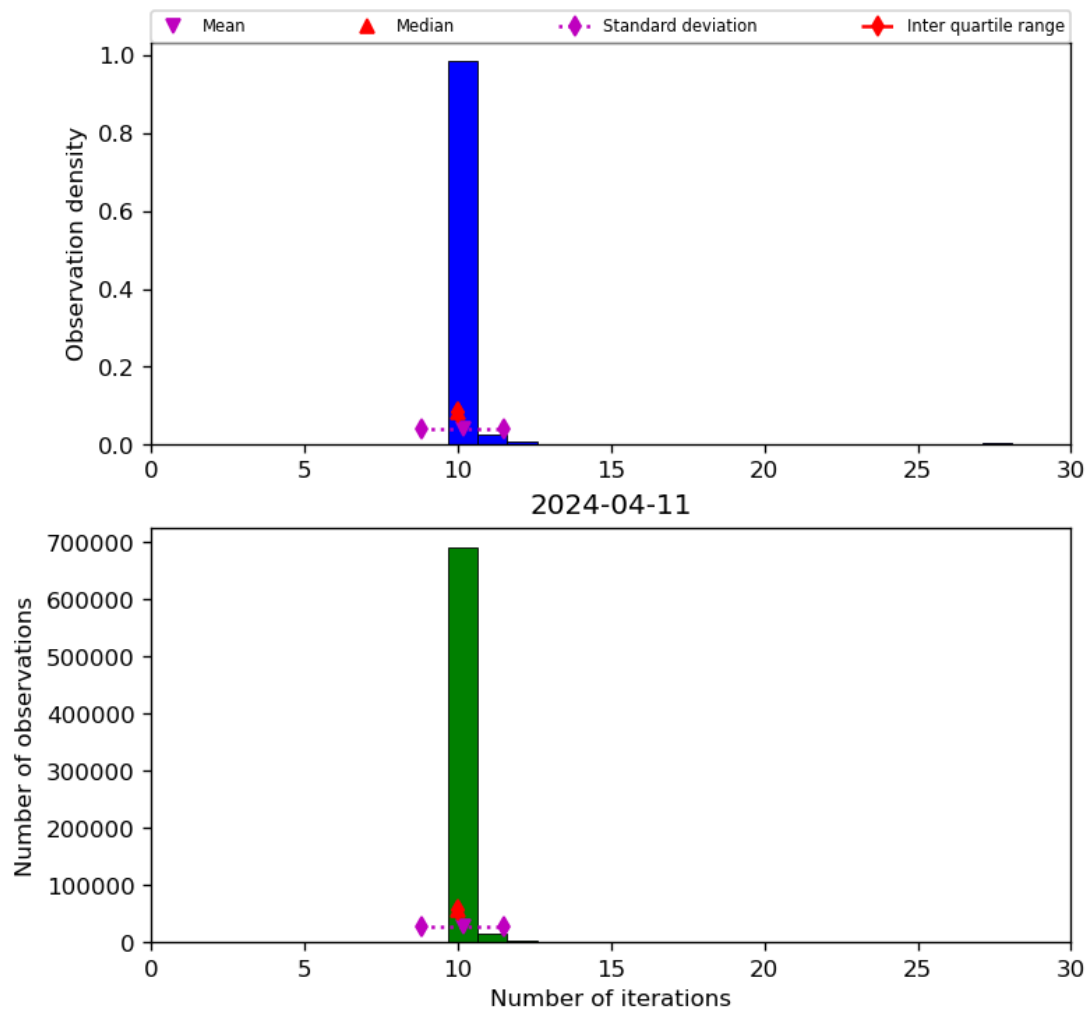
Figure 31: Histogram of “Number of iterations” for 2024-04-10 to 2024-04-12
