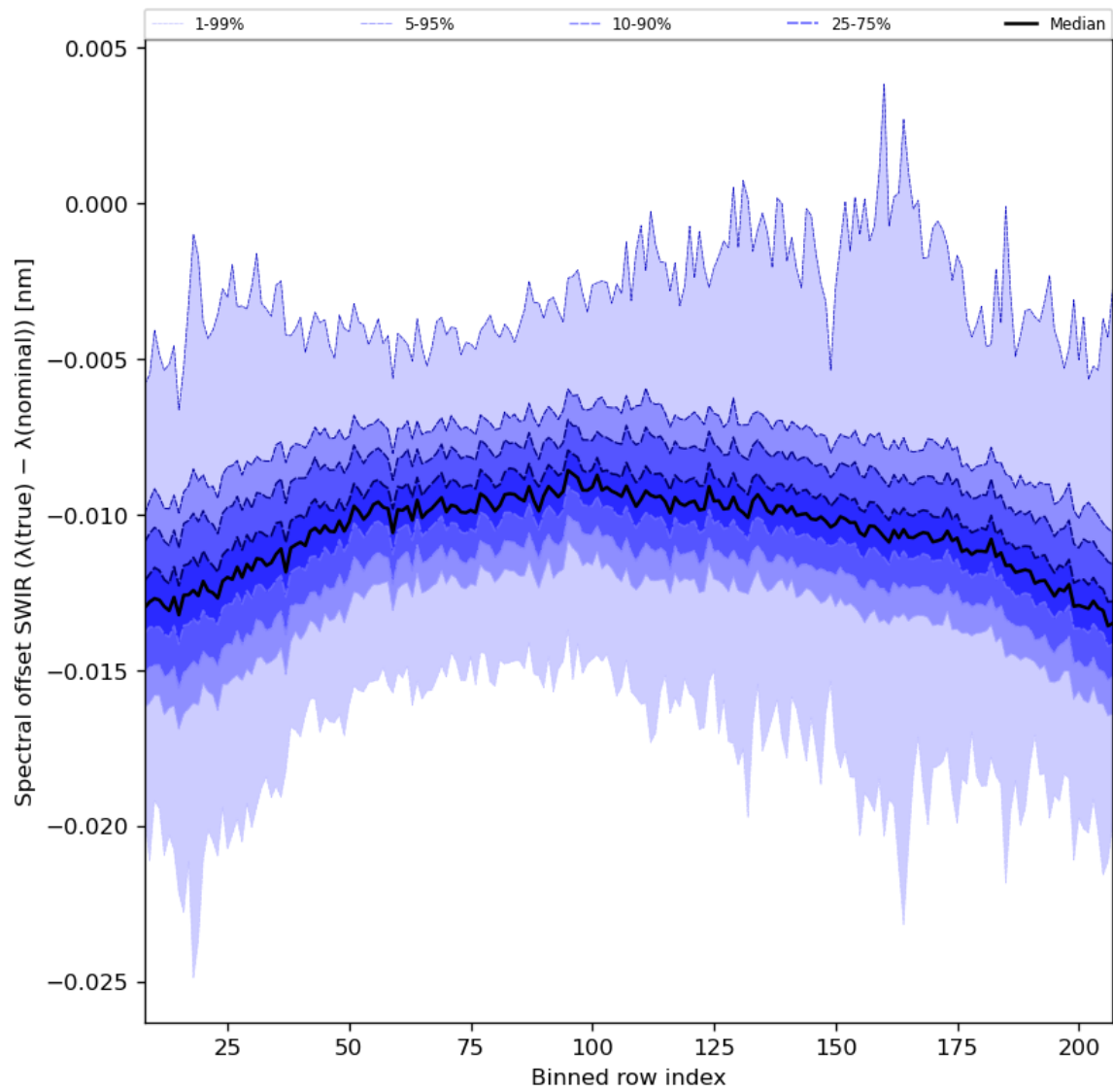
Figure 38: Along track statistics of “Spectral offset SWIR ( \lambda(\text{true}) - \lambda(\text{nominal}) )” for 2024-04-10 to 2024-04-12
