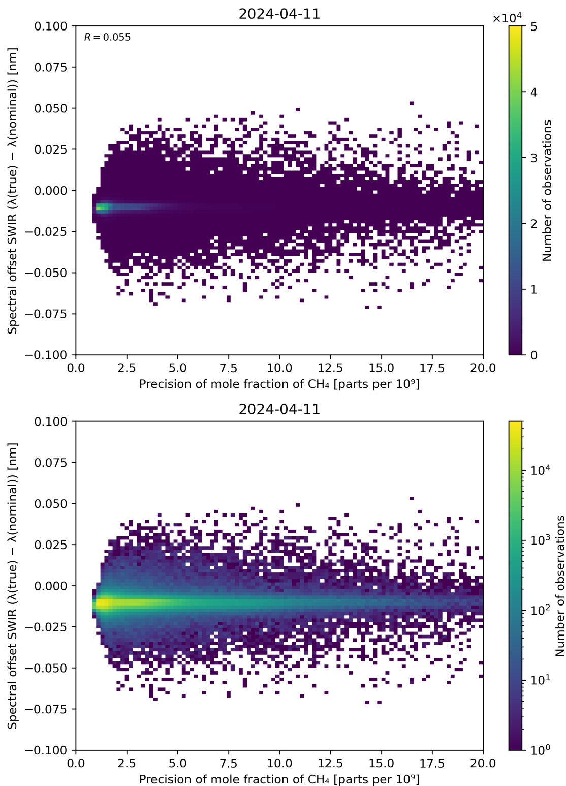
Figure 85: Scatter density plot of “Precision of mole fraction of \text{CH}_4 ” against “Spectral offset SWIR ( \lambda(\text{true}) - \lambda(\text{nominal}) )” for 2024-04-10 to 2024-04-12.
