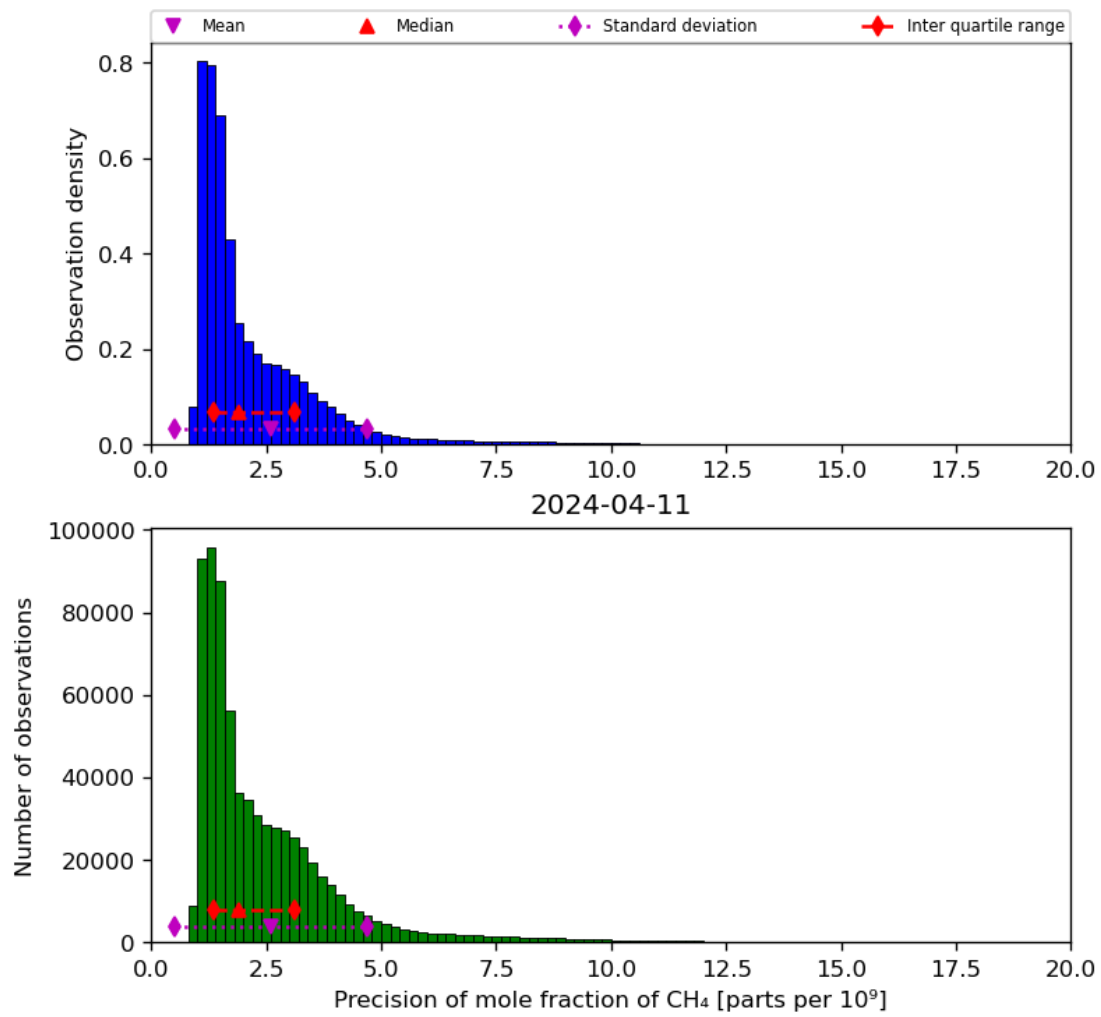
Figure 24: Histogram of “Precision of mole fraction of CH 4 ” for 2024-04-10 to 2024-04-12
