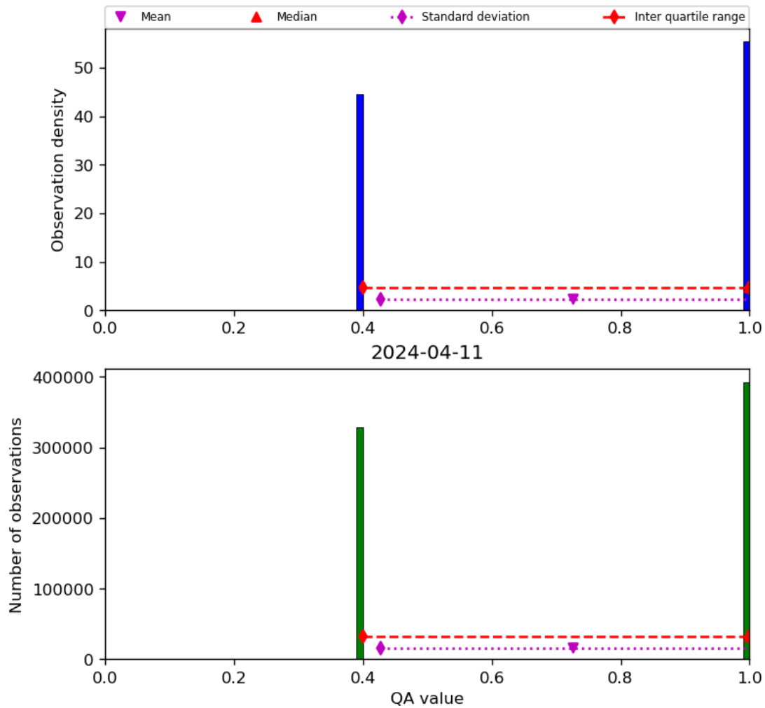
Figure 22: Histogram of “QA value” for 2024-04-10 to 2024-04-12
