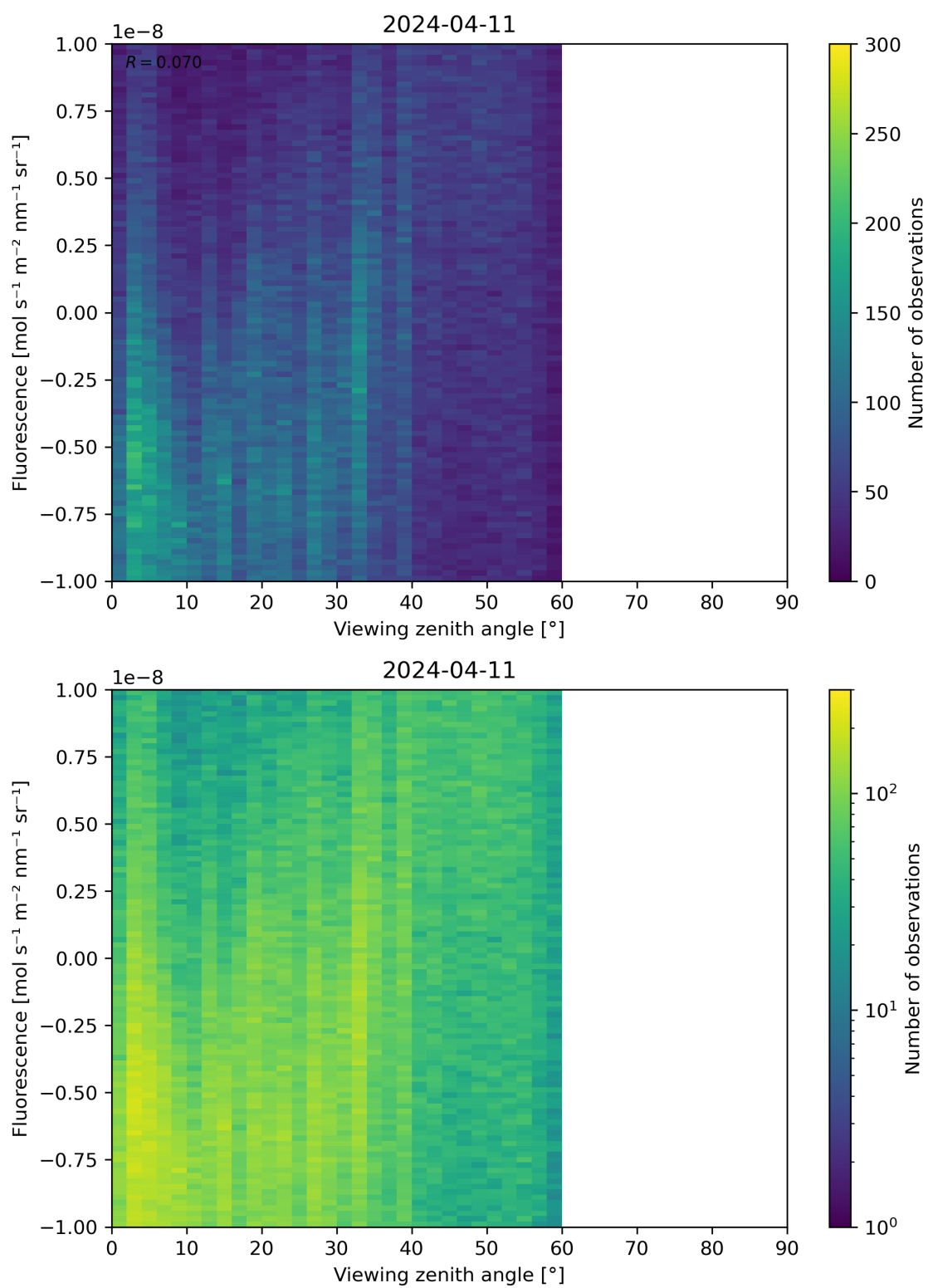
Figure 108: Scatter density plot of “Viewing zenith angle” against “Fluorescence” for 2024-04-10 to 2024-04-12.
