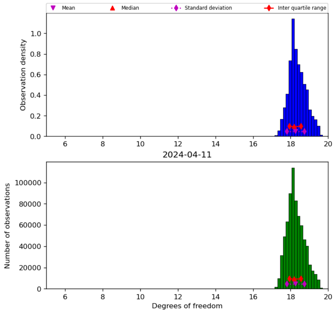
Figure 30: Histogram of "Degrees of freedom" for 2024-04-10 to 2024-04-12
