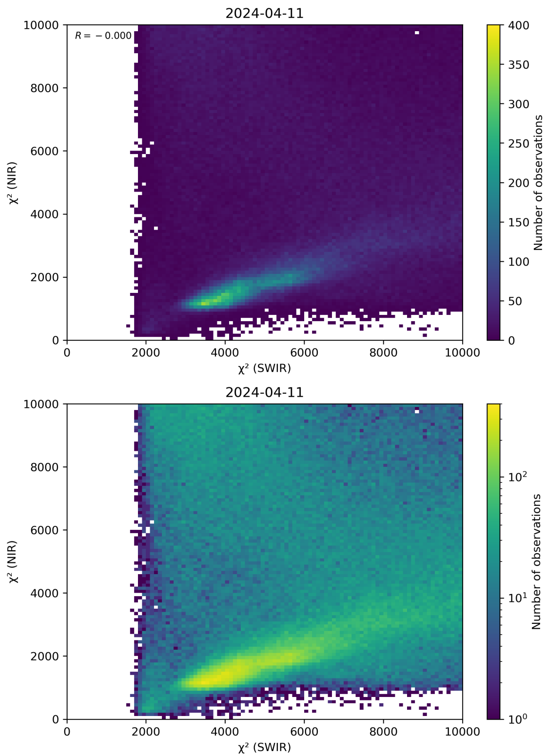
Figure 47: Scatter density plot of “ \chi^2 (SWIR)” against “ \chi^2 (NIR)” for 2024-04-10 to 2024-04-12.
