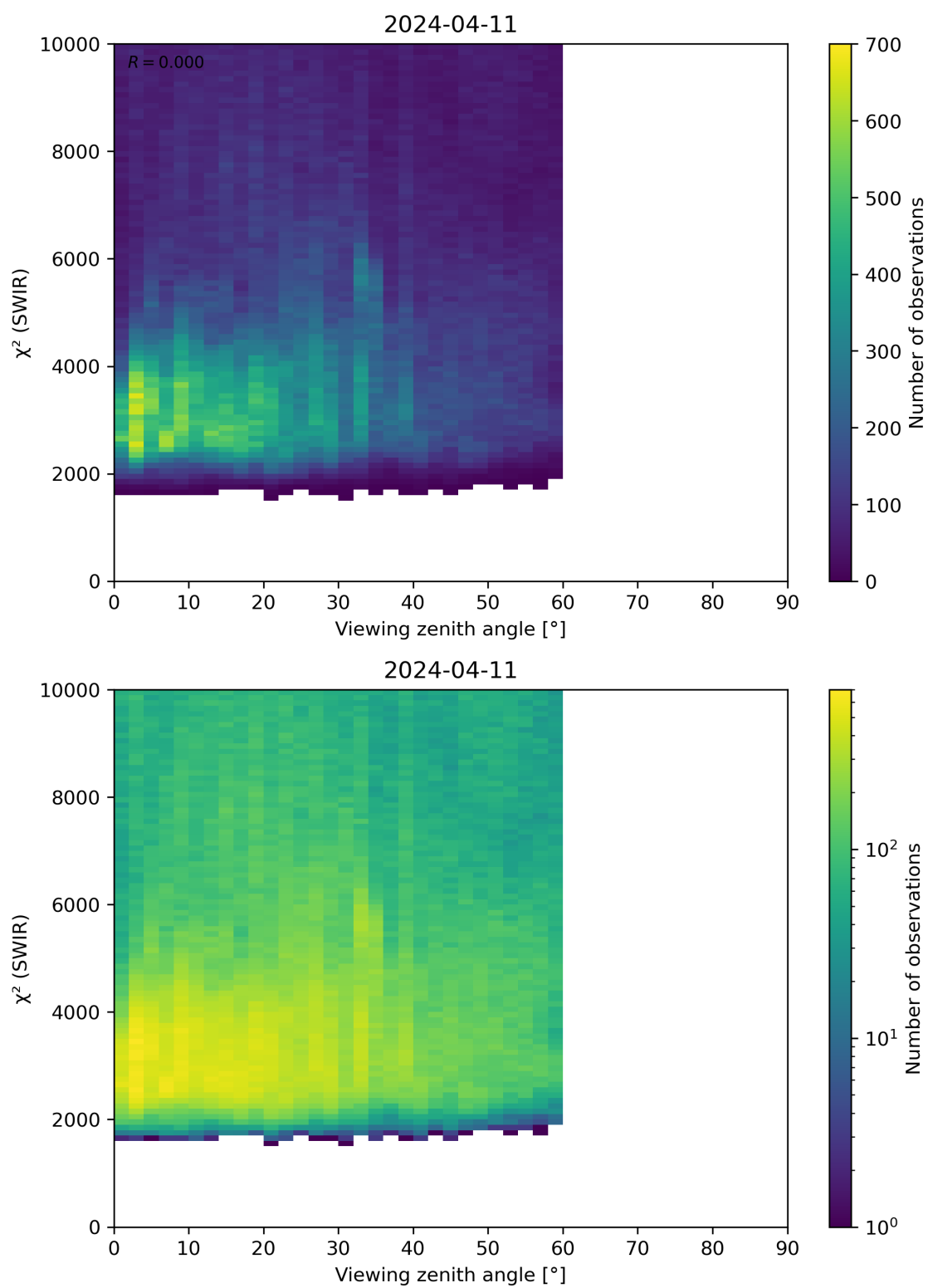
Figure 106: Scatter density plot of “Viewing zenith angle” against “ \chi^2 (SWIR)” for 2024-04-10 to 2024-04-12.
