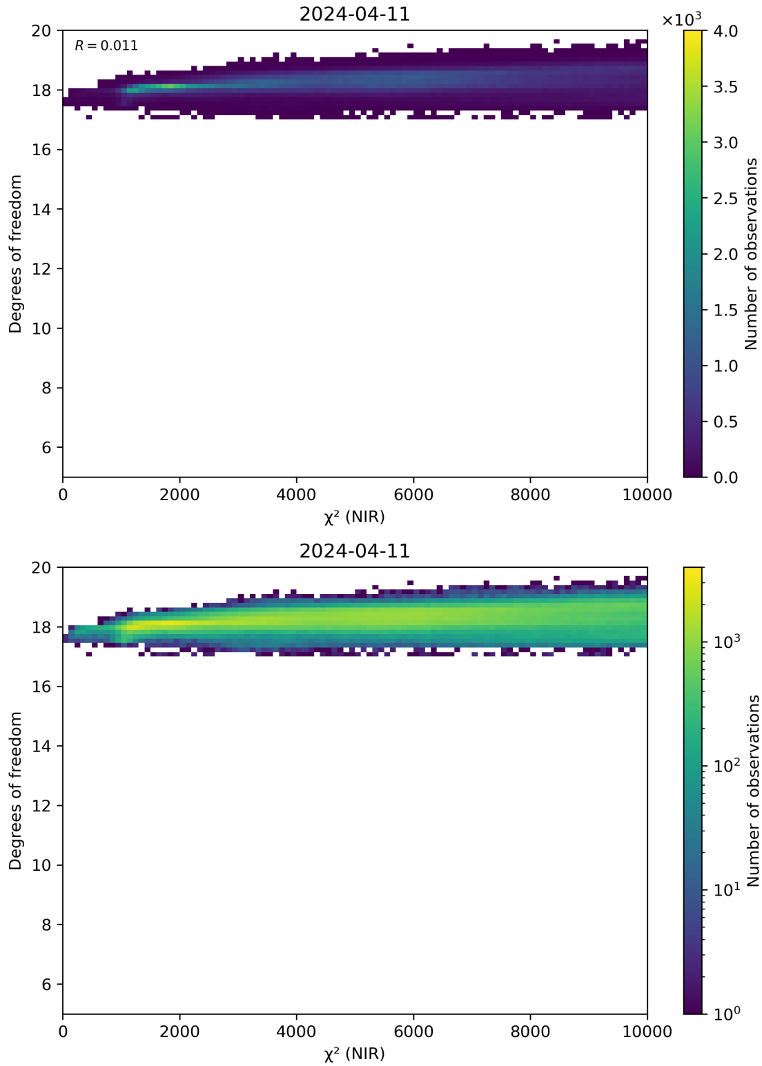
Figure 44: Scatter density plot of “ \chi^2 (NIR)” against “Degrees of freedom” for 2024-04-10 to 2024-04-12.
