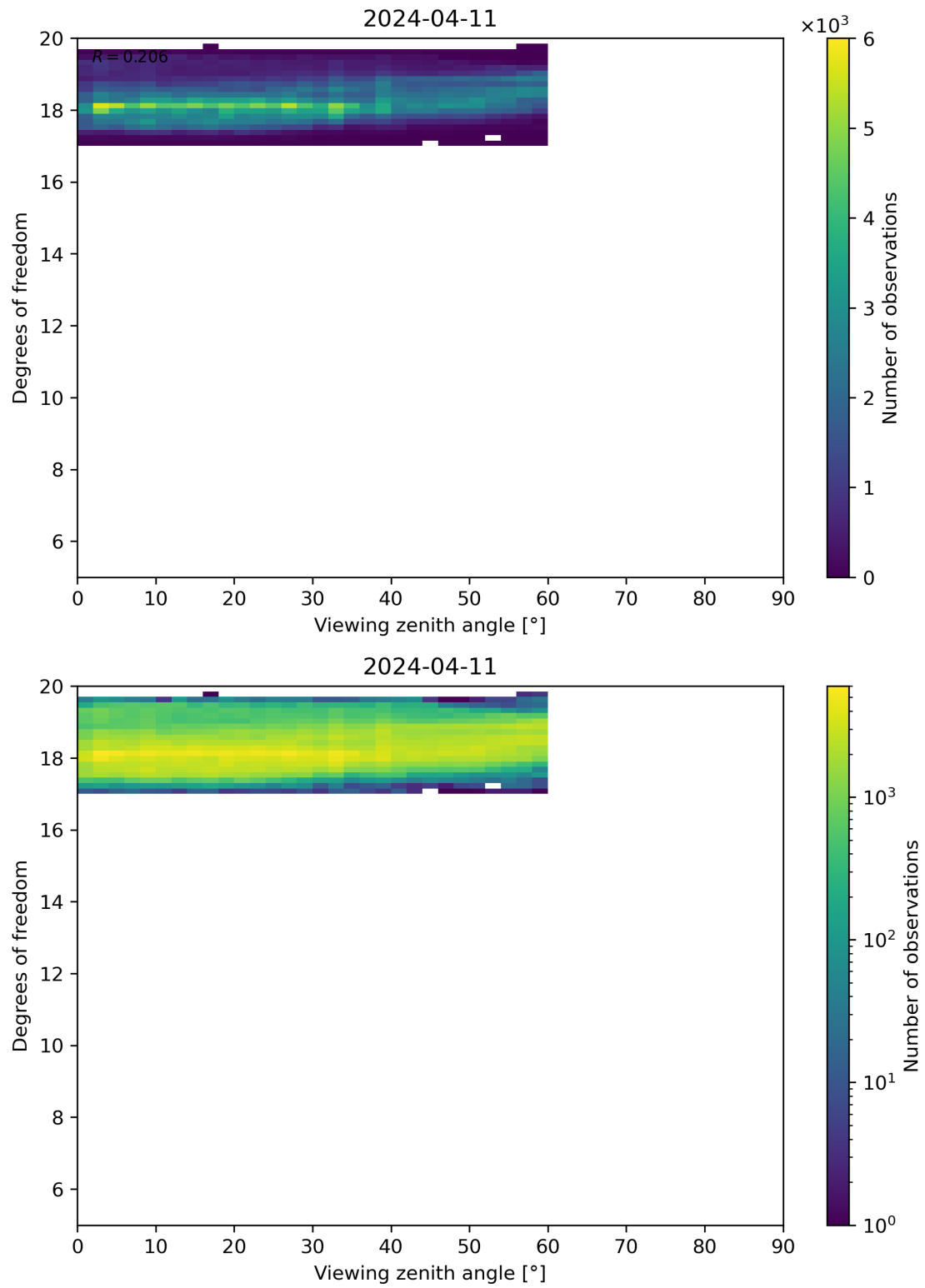
Figure 107: Scatter density plot of “Viewing zenith angle” against “Degrees of freedom” for 2024-04-10 to 2024-04-12.
