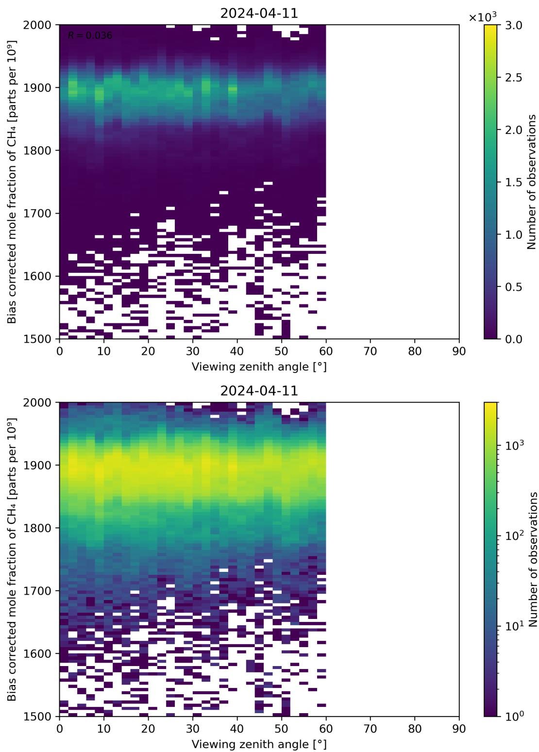
Figure 111: Scatter density plot of “Viewing zenith angle” against “Bias corrected mole fraction of CH 4 ” for 2024-04-10 to 2024-04-12.
