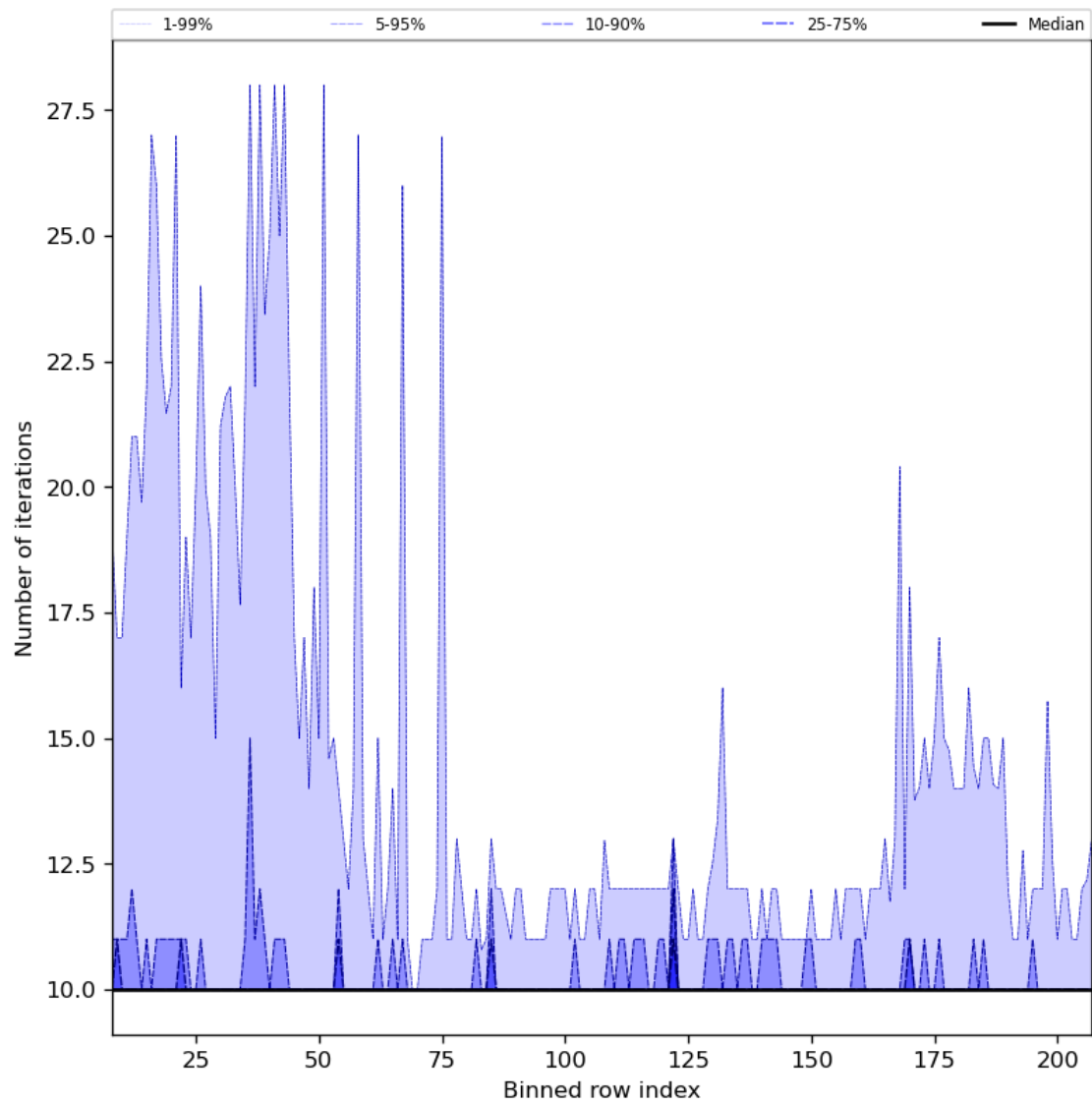
Figure 42: Along track statistics of “Number of iterations” for 2024-04-10 to 2024-04-12
