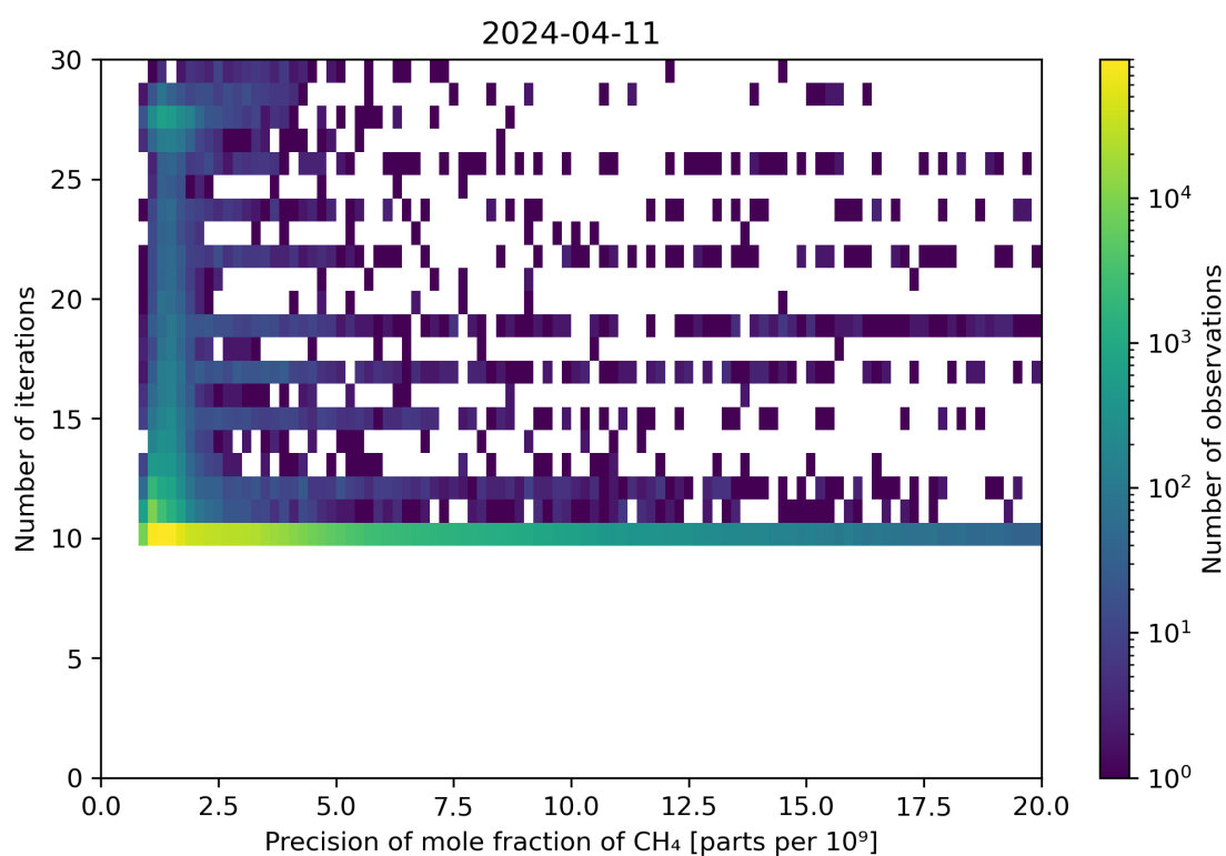
Figure 83: Scatter density plot of “Precision of mole fraction of CH 4 ” against “Number of iterations” for 2024-04-10 to 2024-04-12.
