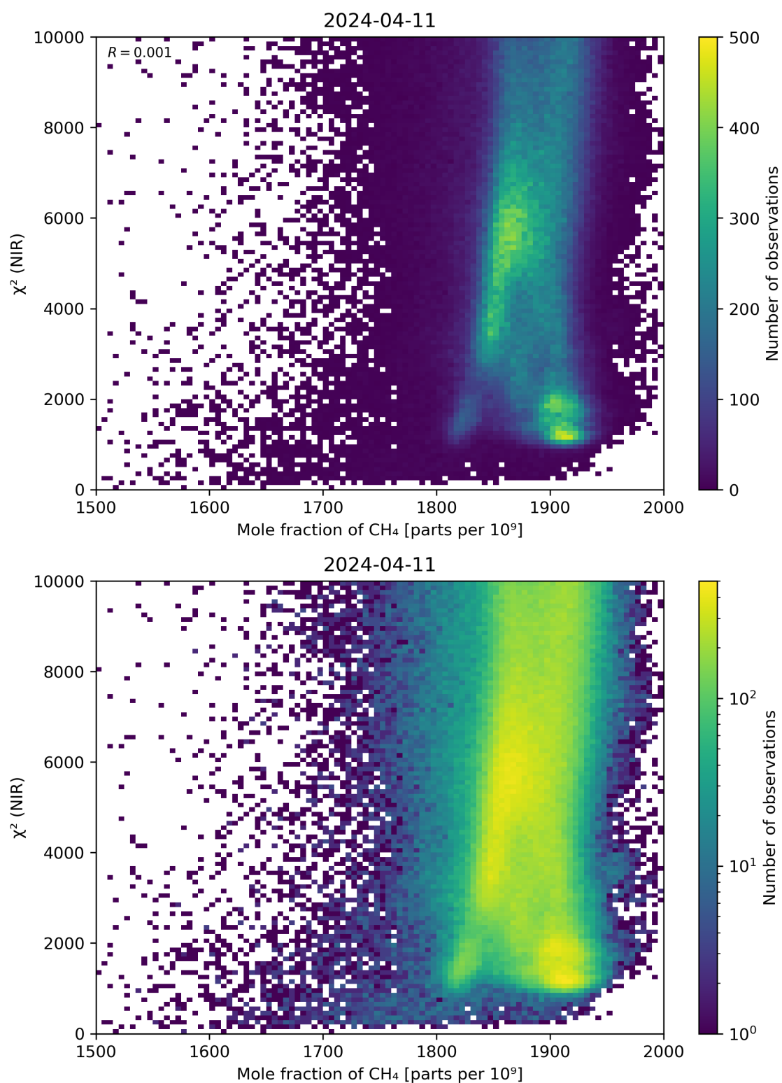
Figure 70: Scatter density plot of “Mole fraction of CH 4 ” against “ \chi^2 (NIR)” for 2024-04-10 to 2024-04-12.
