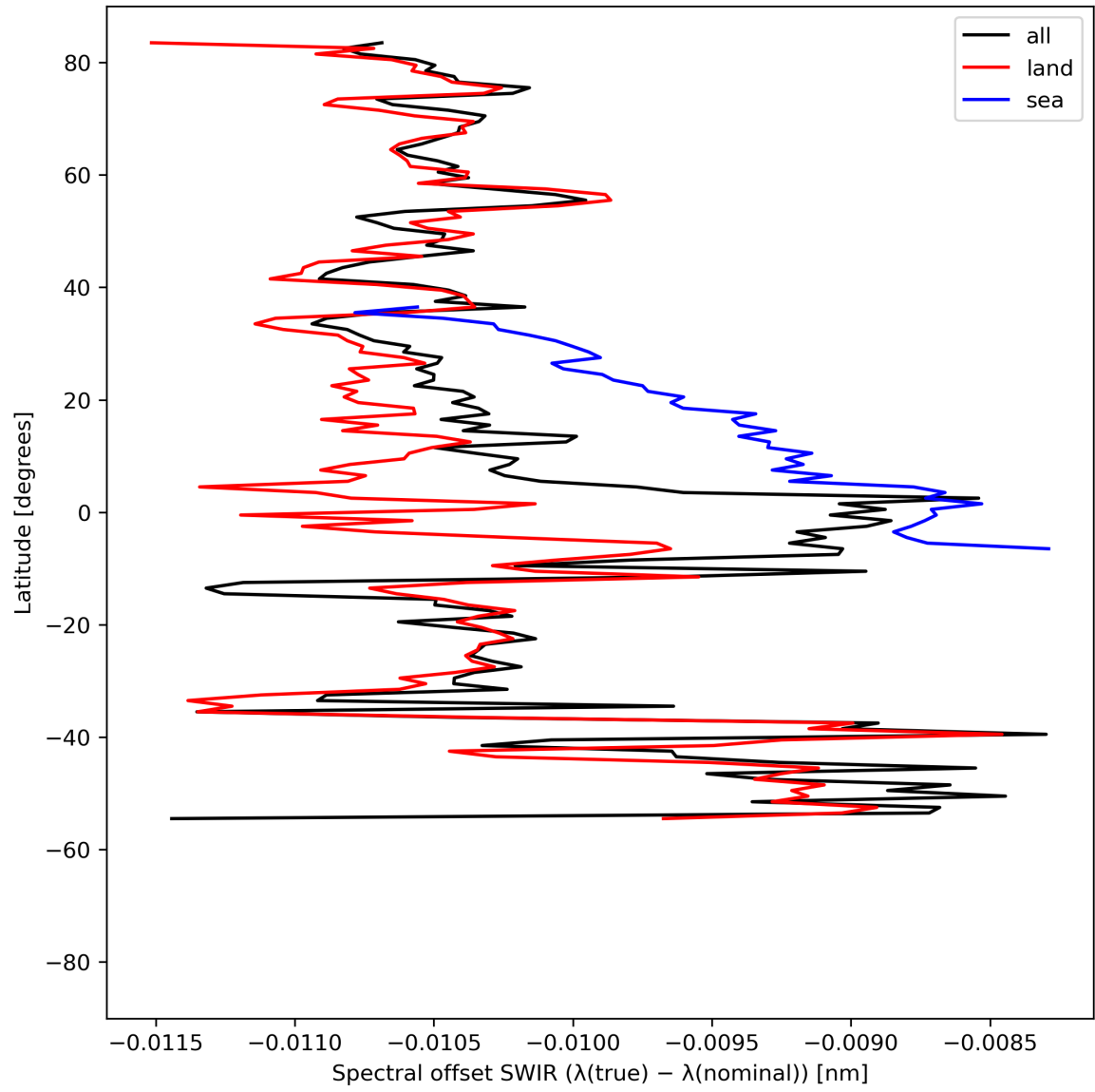
Figure 16: Zonal average of “Spectral offset SWIR ( \lambda(\text{true}) - \lambda(\text{nominal}) )” for 2024-04-10 to 2024-04-12.
