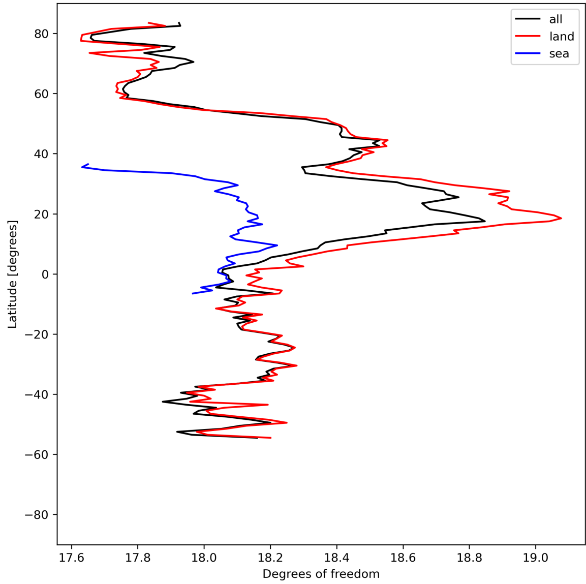
Figure 19: Zonal average of “Degrees of freedom” for 2024-04-10 to 2024-04-12.
