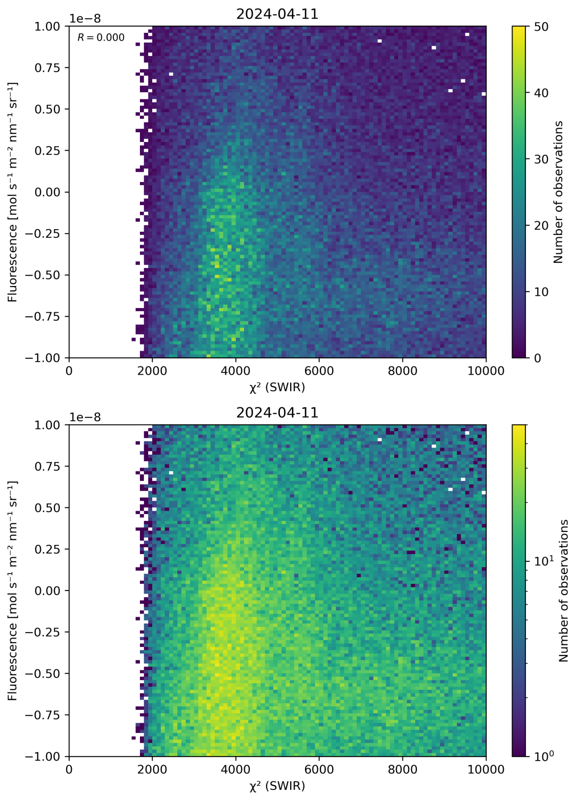
Figure 49: Scatter density plot of “ \chi^2 (SWIR)” against “Fluorescence” for 2024-04-10 to 2024-04-12.
