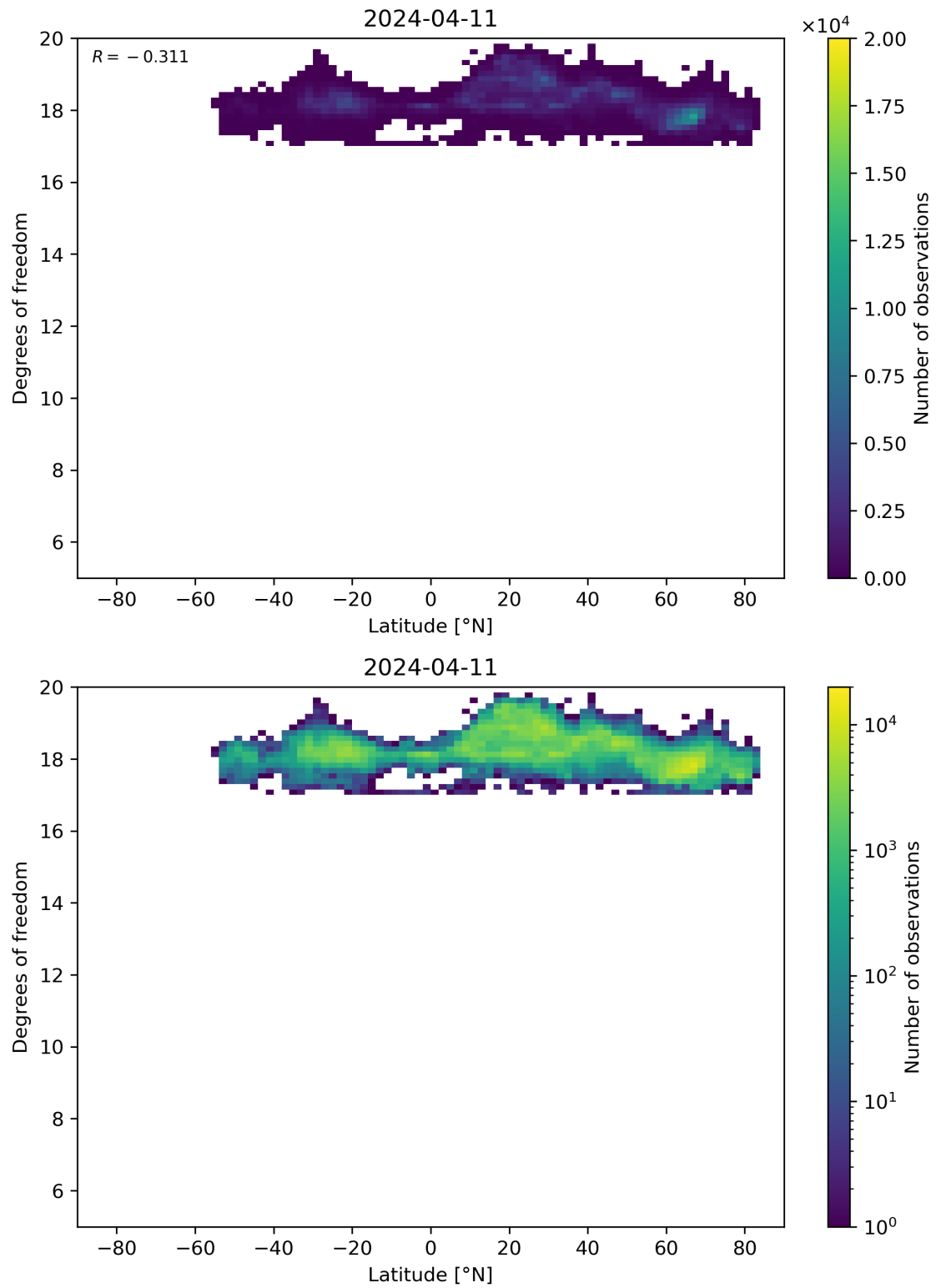
Figure 55: Scatter density plot of “Latitude” against “Degrees of freedom” for 2024-04-10 to 2024-04-12.
