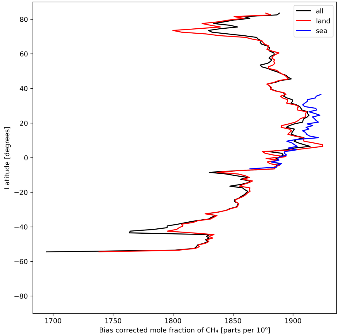
Figure 14: Zonal average of “Bias corrected mole fraction of \text{CH}_4 ” for 2024-04-10 to 2024-04-12.
