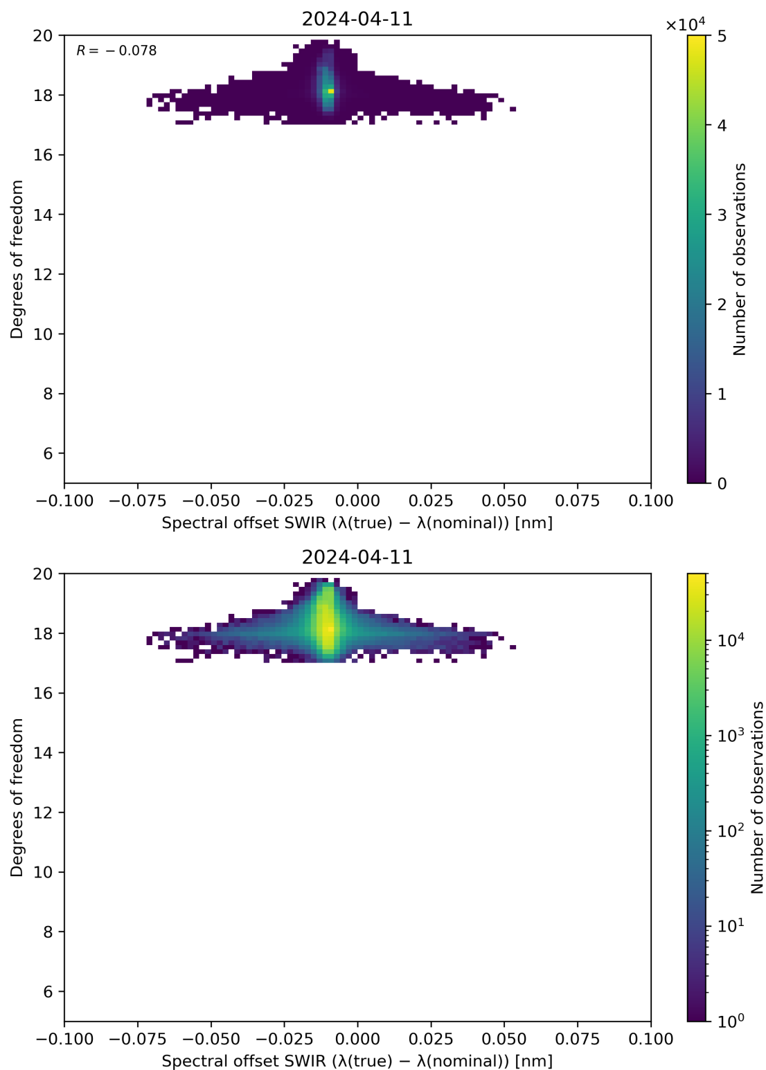
Figure 119: Scatter density plot of “Spectral offset SWIR ( \lambda(\text{true}) - \lambda(\text{nominal}) )” against “Degrees of freedom” for 2024-04-10 to 2024-04-12.
