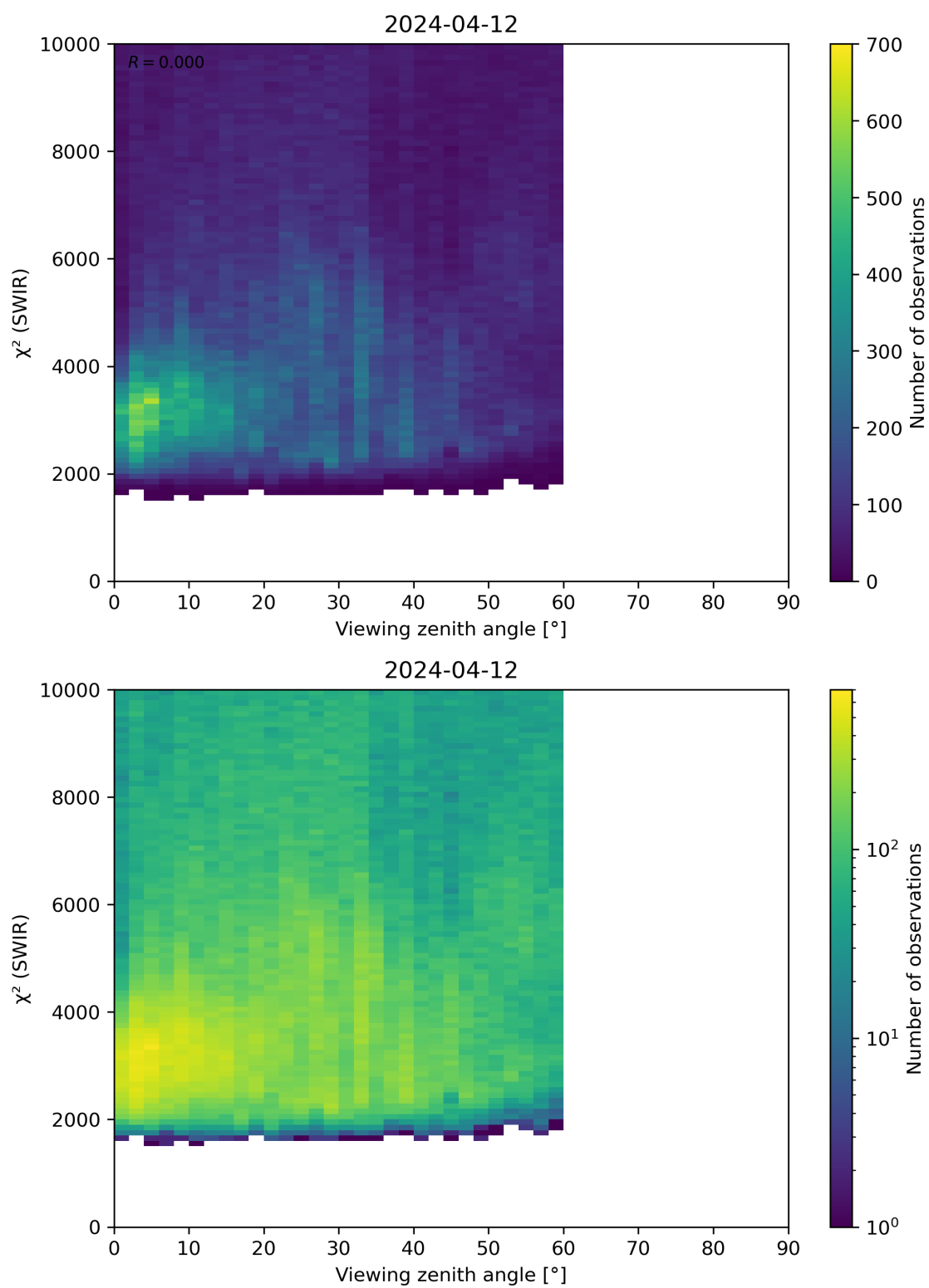
Figure 106: Scatter density plot of “Viewing zenith angle” against “ \chi^2 (SWIR)” for 2024-04-11 to 2024-04-13.
