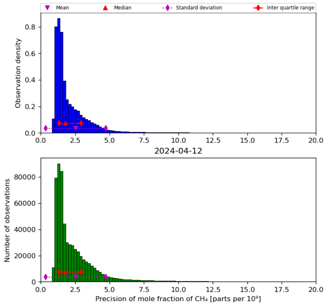
Figure 24: Histogram of “Precision of mole fraction of CH 4 ” for 2024-04-11 to 2024-04-13
