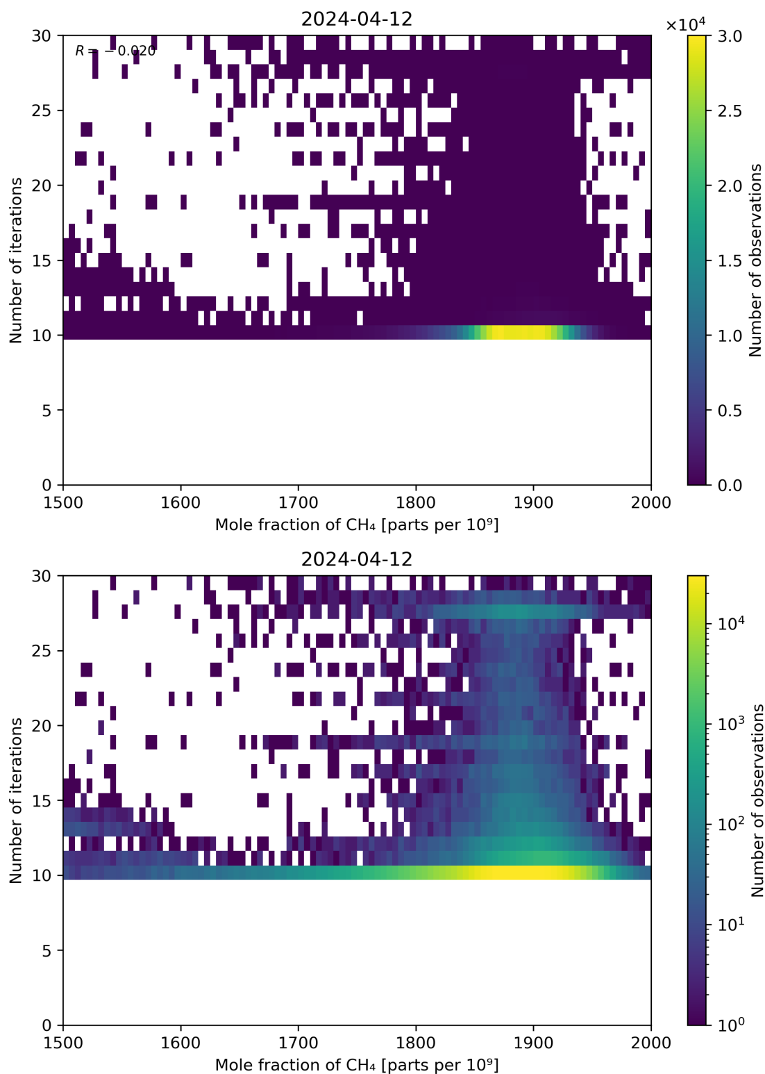
Figure 76: Scatter density plot of “Mole fraction of CH 4 ” against “Number of iterations” for 2024-04-11 to 2024-04-13.
