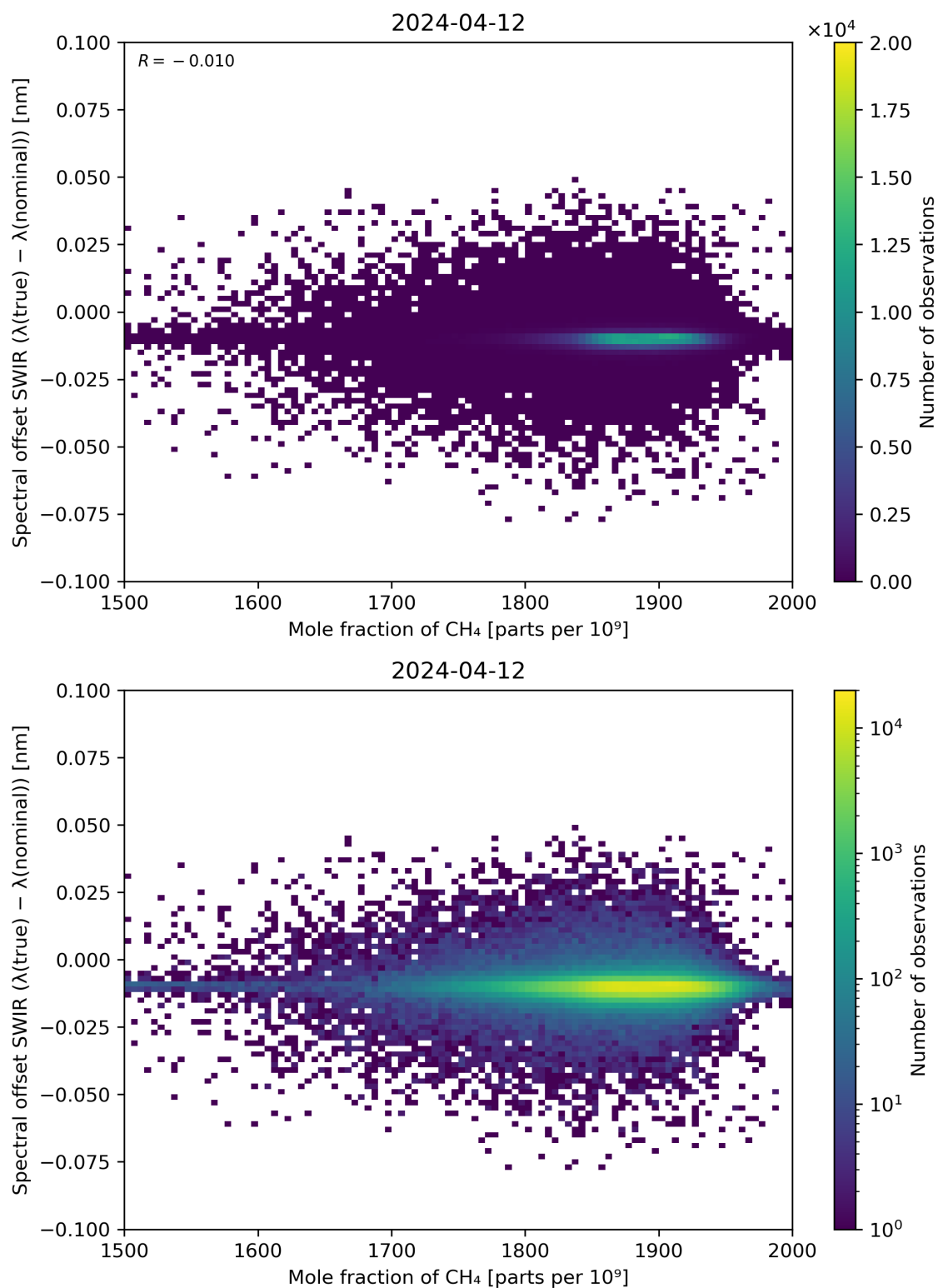
Figure 86: Scatter density plot of “Mole fraction of CH 4 ” against “Spectral offset SWIR ( \lambda(\text{true}) - \lambda(\text{nominal}) )” for 2024-04-11 to 2024-04-13.
