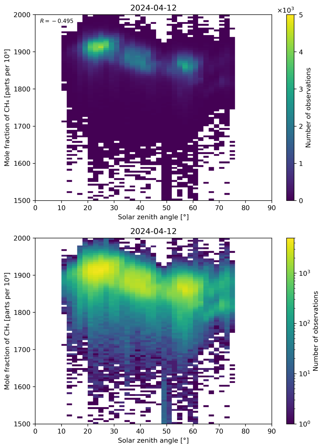
Figure 99: Scatter density plot of “Solar zenith angle” against “Mole fraction of CH 4 ” for 2024-04-11 to 2024-04-13.
