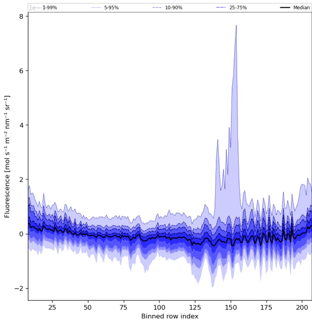
Figure 43: Along track statistics of “Fluorescence” for 2024-04-11 to 2024-04-13
