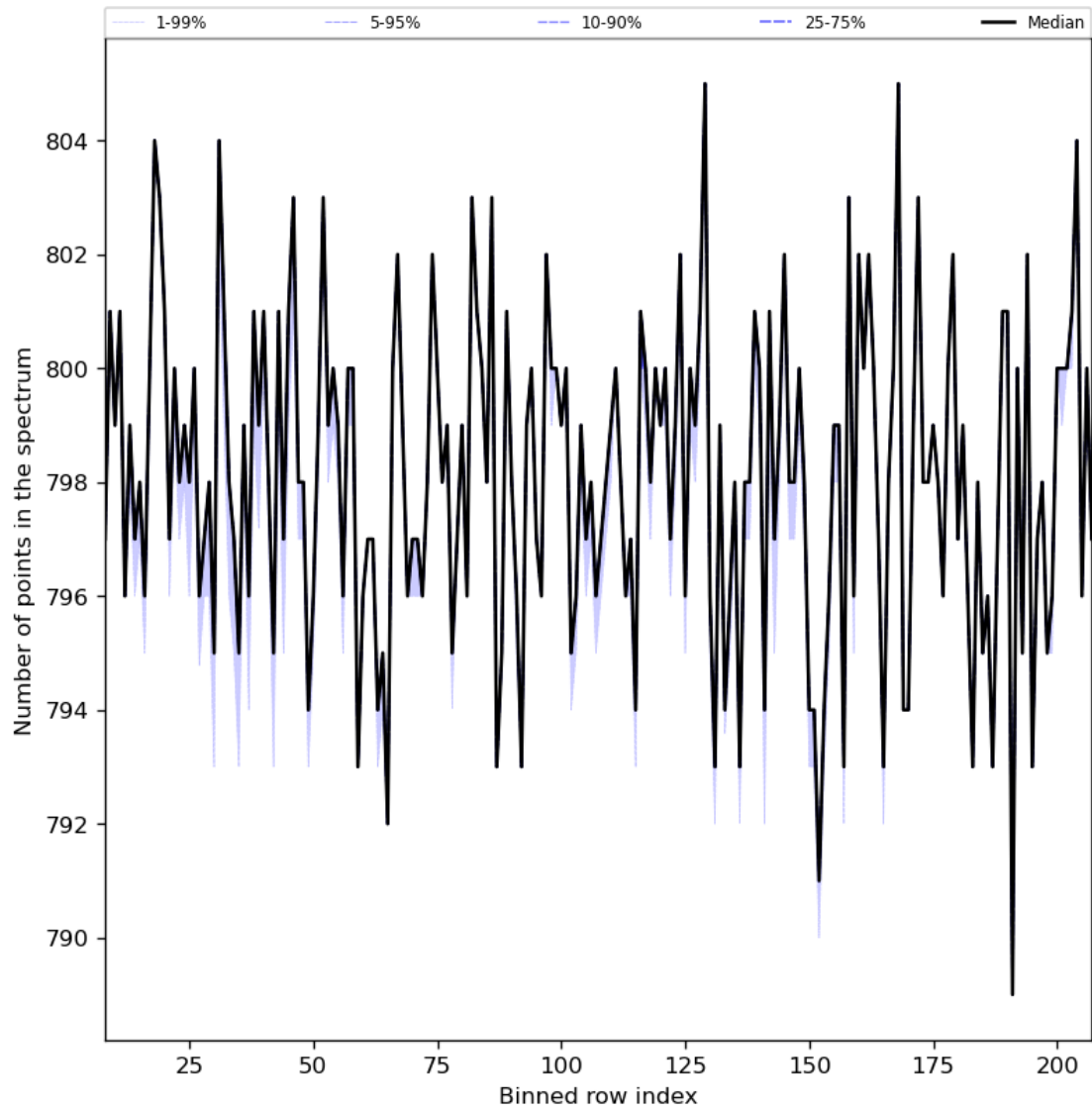
Figure 37: Along track statistics of “Number of points in the spectrum” for 2024-04-11 to 2024-04-13
