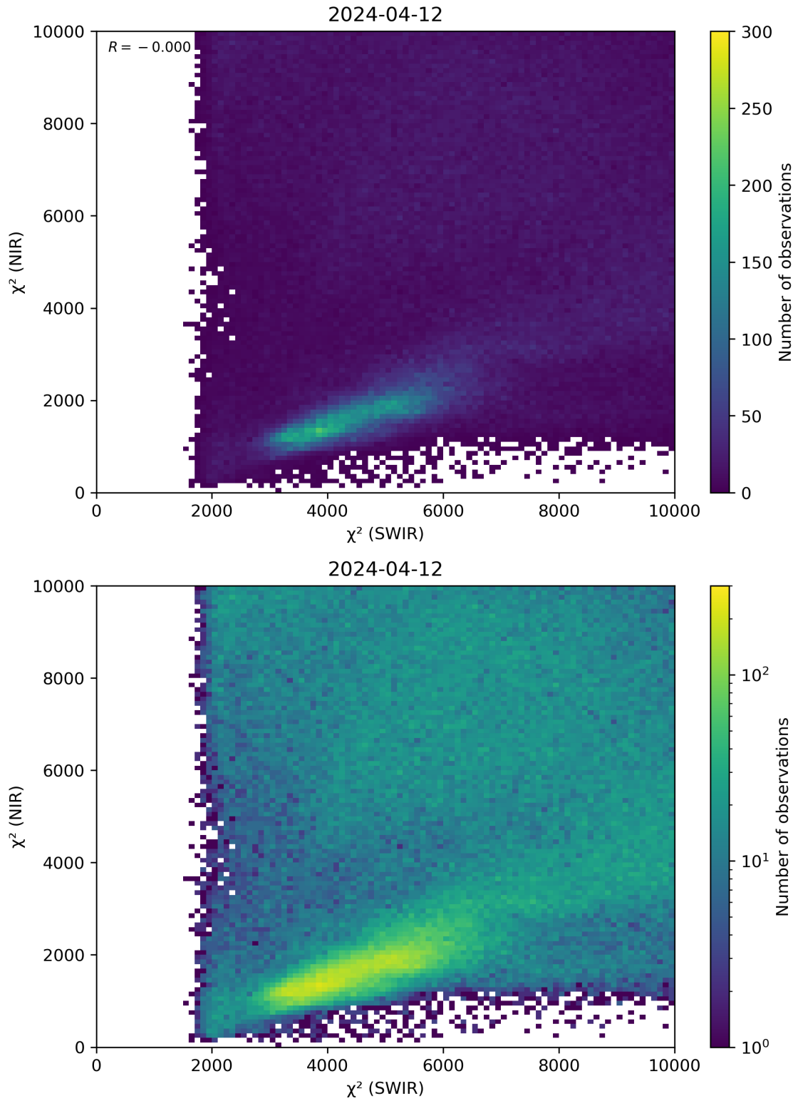
Figure 47: Scatter density plot of “ \chi^2 (SWIR)” against “ \chi^2 (NIR)” for 2024-04-11 to 2024-04-13.
