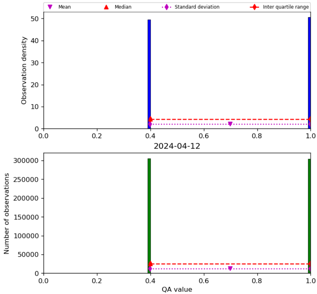
Figure 22: Histogram of “QA value” for 2024-04-11 to 2024-04-13
