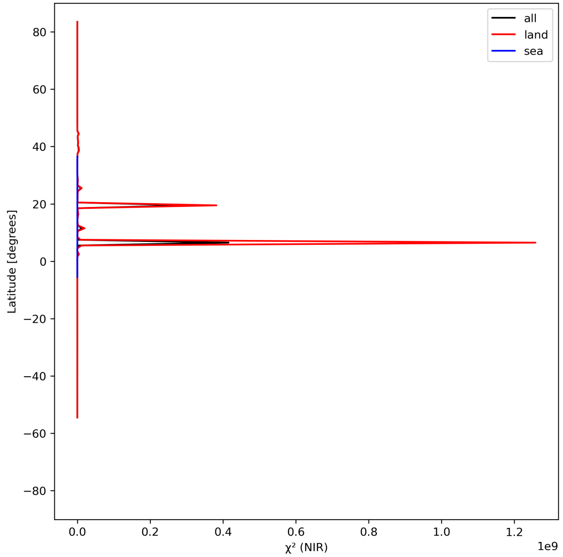
Figure 18: Zonal average of “ \chi^2 (NIR)” for 2024-04-11 to 2024-04-13.
