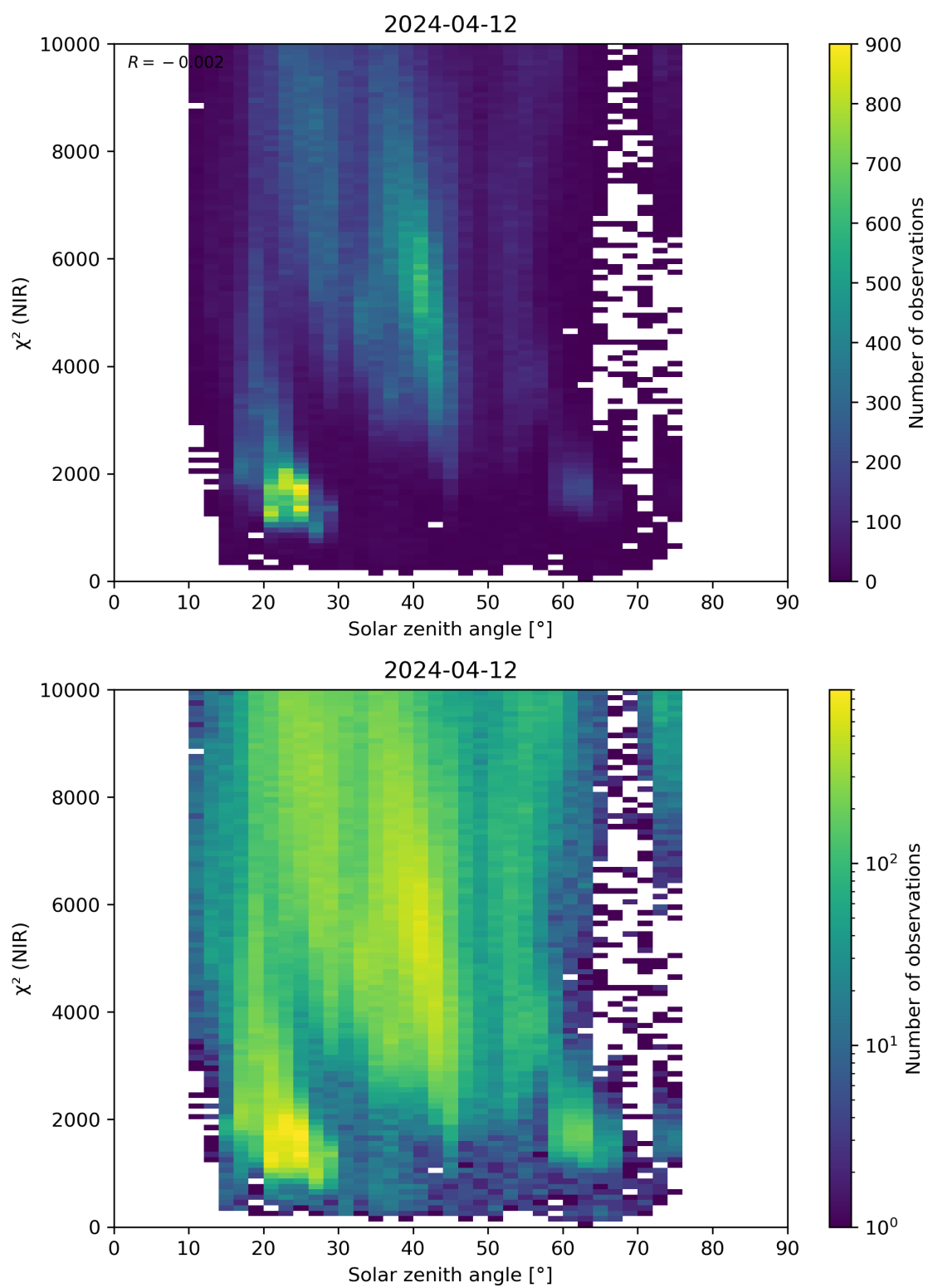
Figure 94: Scatter density plot of “Solar zenith angle” against “ \chi^2 (NIR)” for 2024-04-11 to 2024-04-13.
