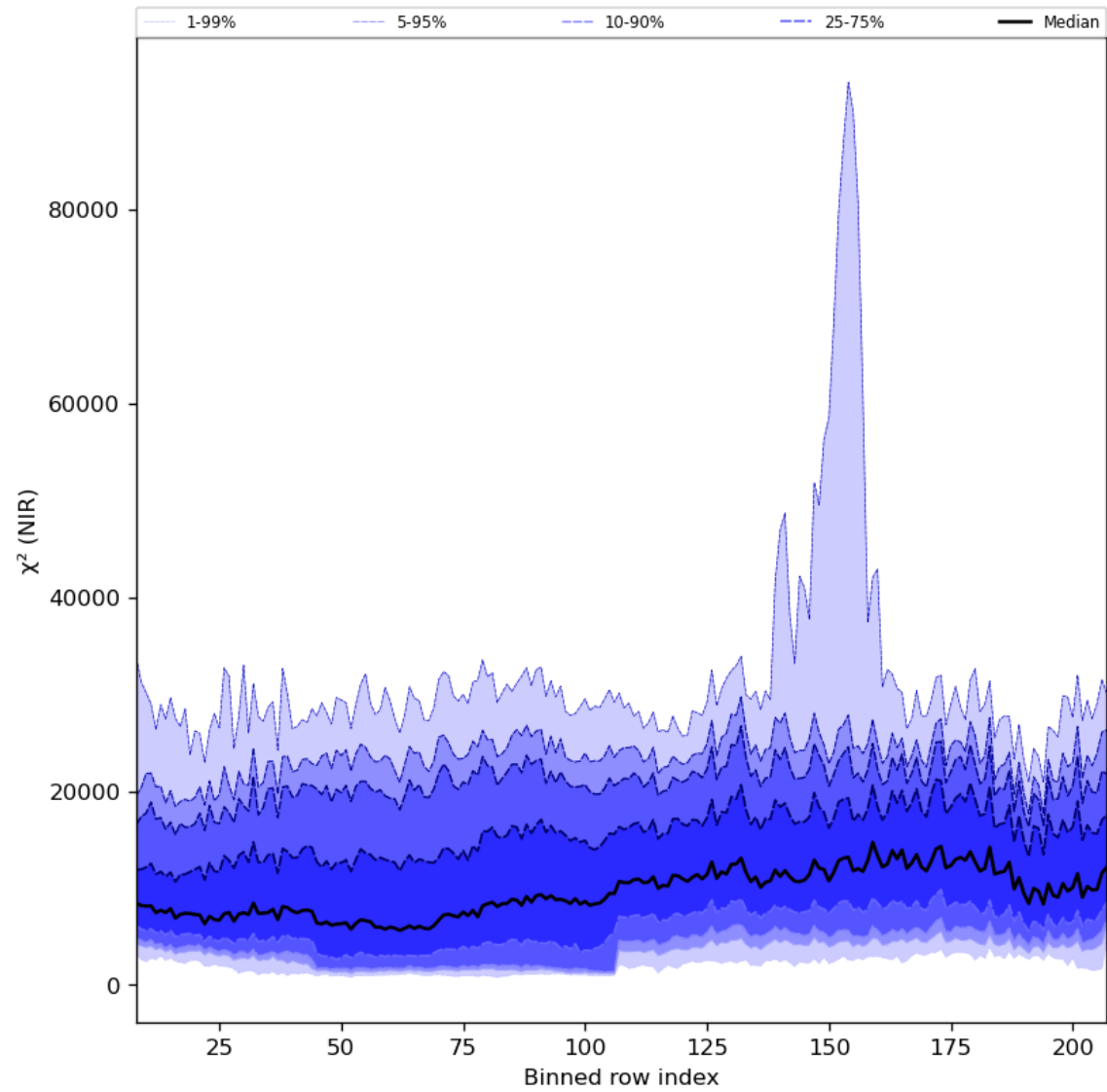
Figure 40: Along track statistics of “ \chi^2 (NIR)” for 2024-04-11 to 2024-04-13
