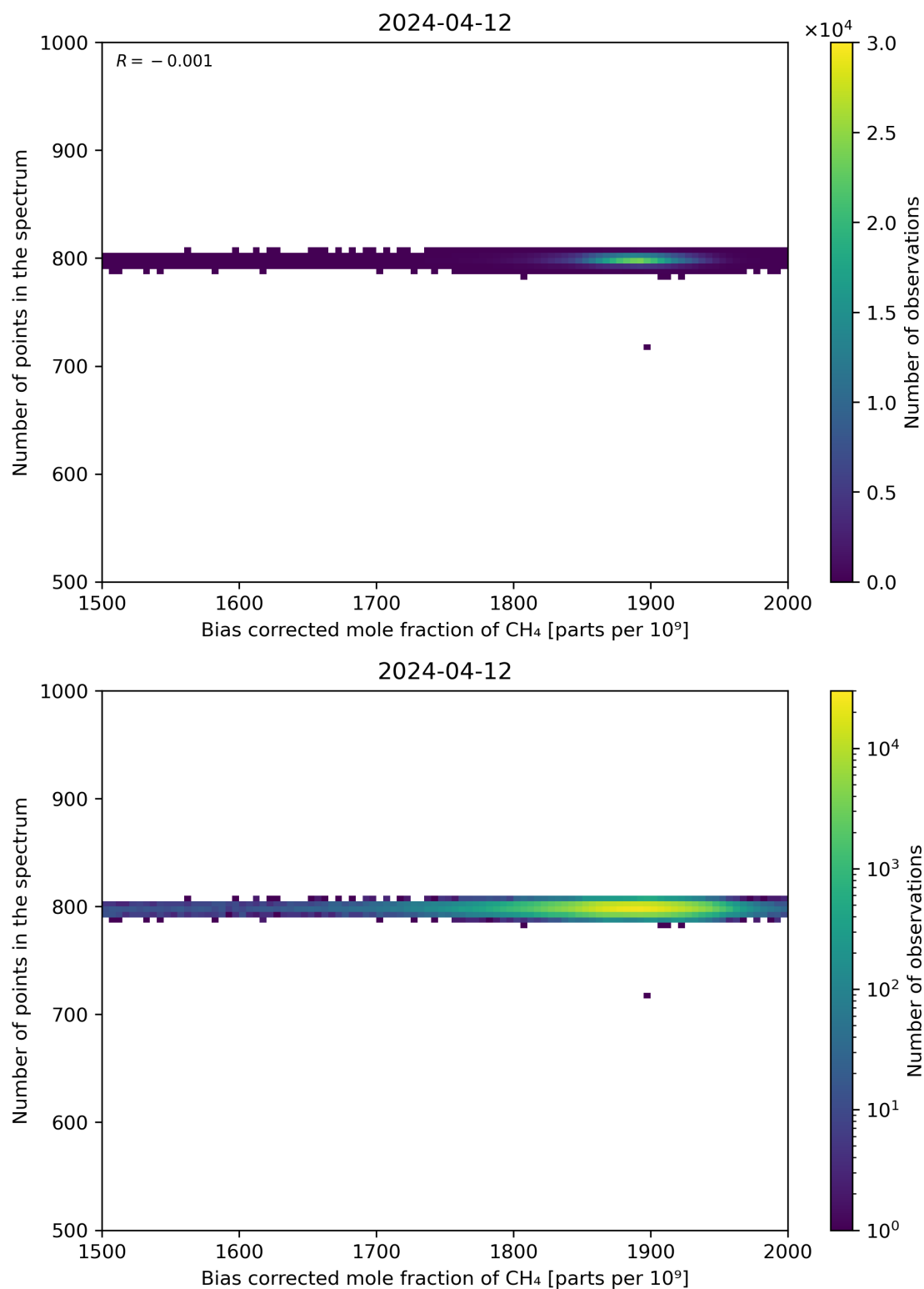
Figure 68: Scatter density plot of “Bias corrected mole fraction of CH 4 ” against “Number of points in the spectrum” for 2024-04-11 to 2024-04-13.
