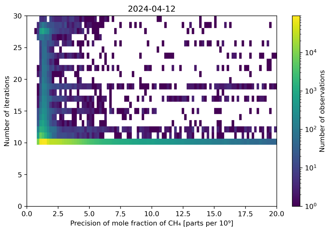
Figure 83: Scatter density plot of “Precision of mole fraction of \text{CH}_4 ” against “Number of iterations” for 2024-04-11 to 2024-04-13.
