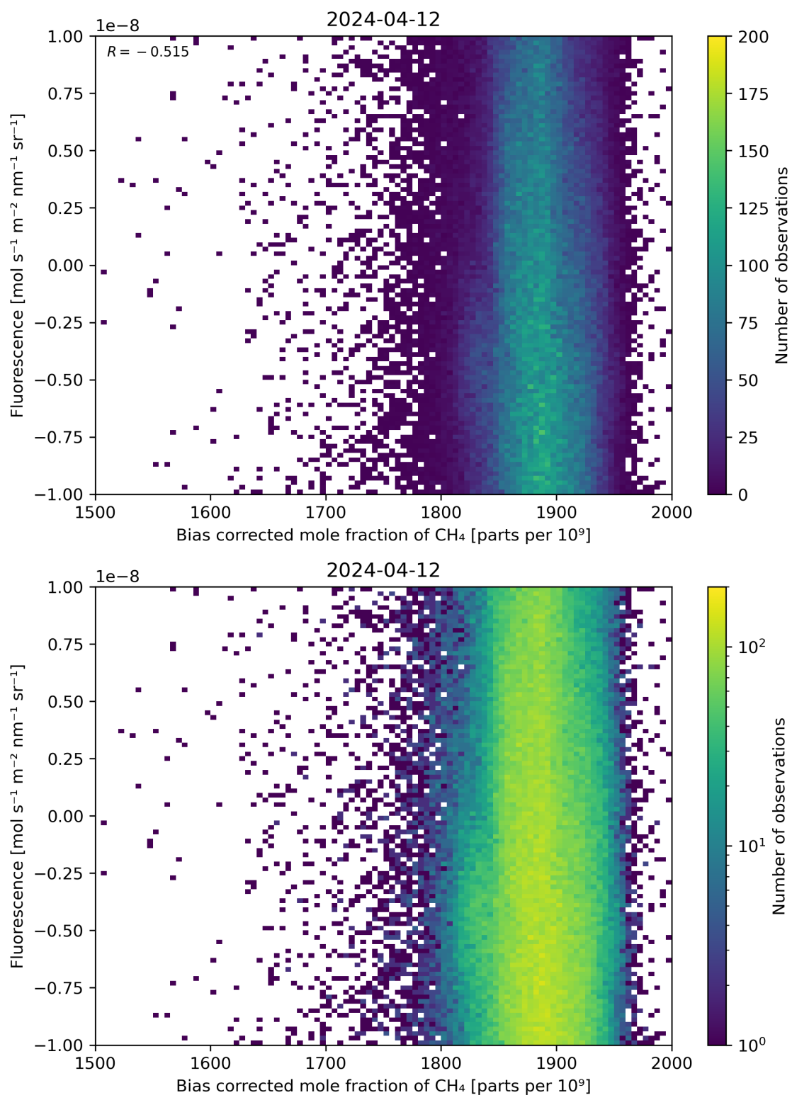
Figure 66: Scatter density plot of “Bias corrected mole fraction of \text{CH}_4 ” against “Fluorescence” for 2024-04-11 to 2024-04-13.
