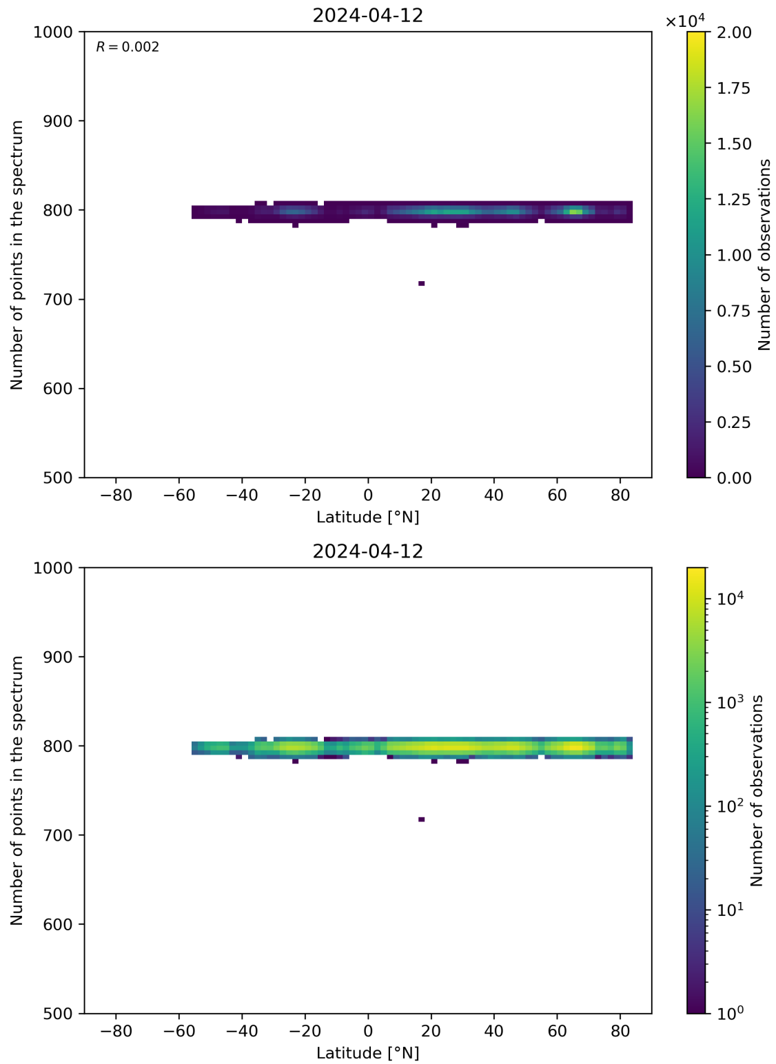
Figure 61: Scatter density plot of “Latitude” against “Number of points in the spectrum” for 2024-04-11 to 2024-04-13.
