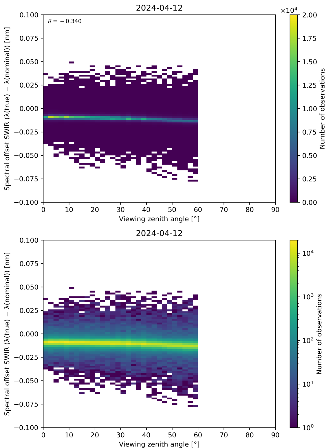
Figure 116: Scatter density plot of “Viewing zenith angle” against “Spectral offset SWIR ( \lambda(\text{true}) - \lambda(\text{nominal}) )” for 2024-04-11 to 2024-04-13.
