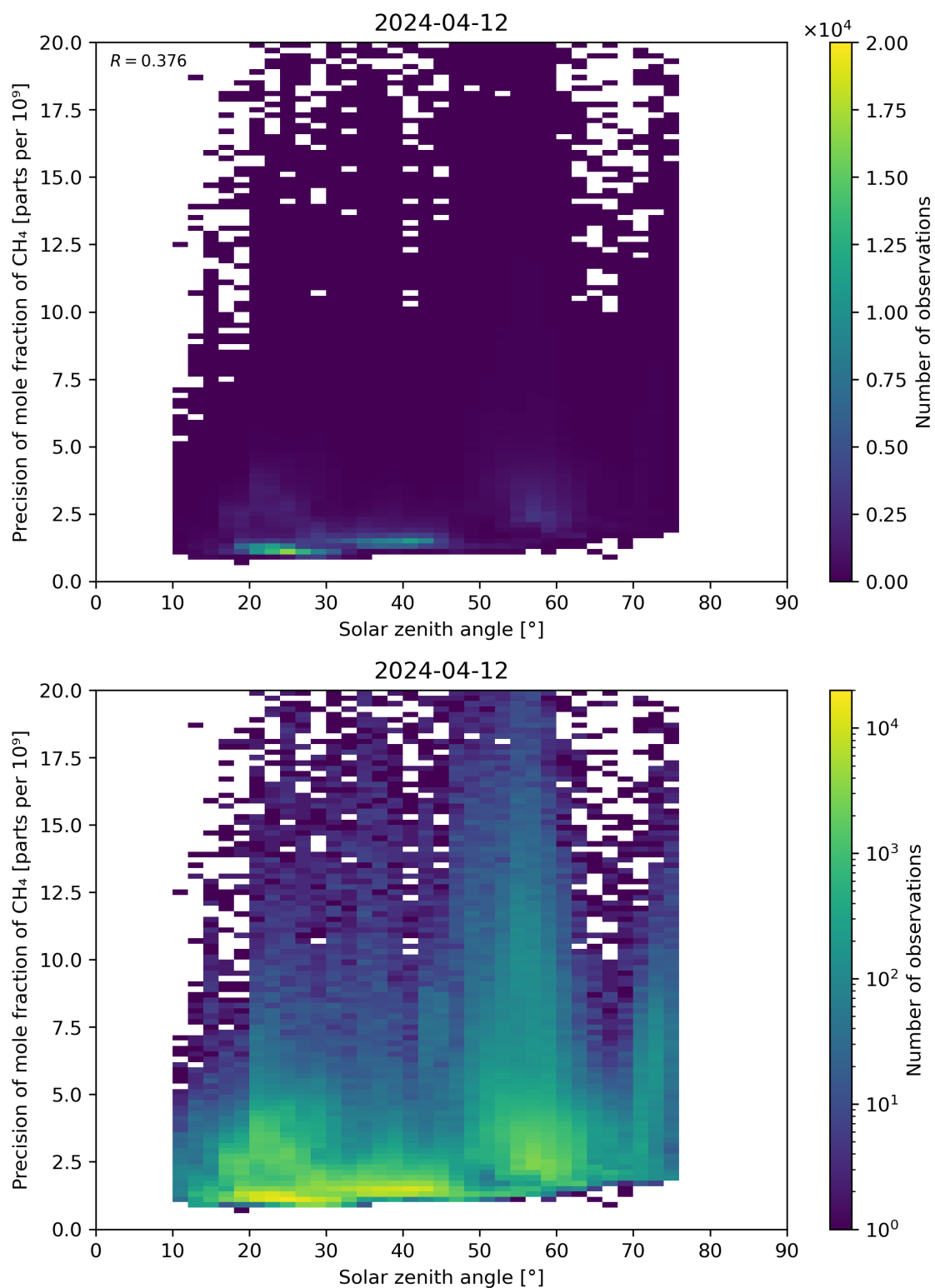
Figure 101: Scatter density plot of “Solar zenith angle” against “Precision of mole fraction of CH 4 ” for 2024-04-11 to 2024-04-13.
