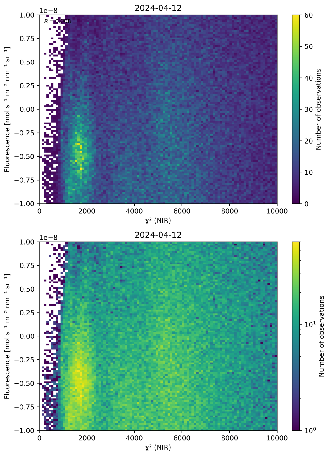
Figure 45: Scatter density plot of “ \chi^2 (NIR)” against “Fluorescence” for 2024-04-11 to 2024-04-13.
