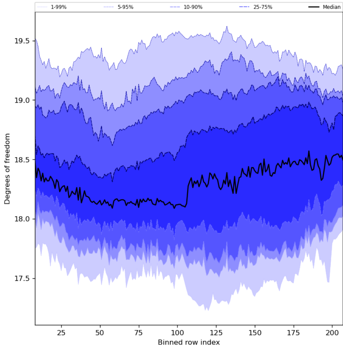
Figure 41: Along track statistics of “Degrees of freedom” for 2024-04-11 to 2024-04-13
