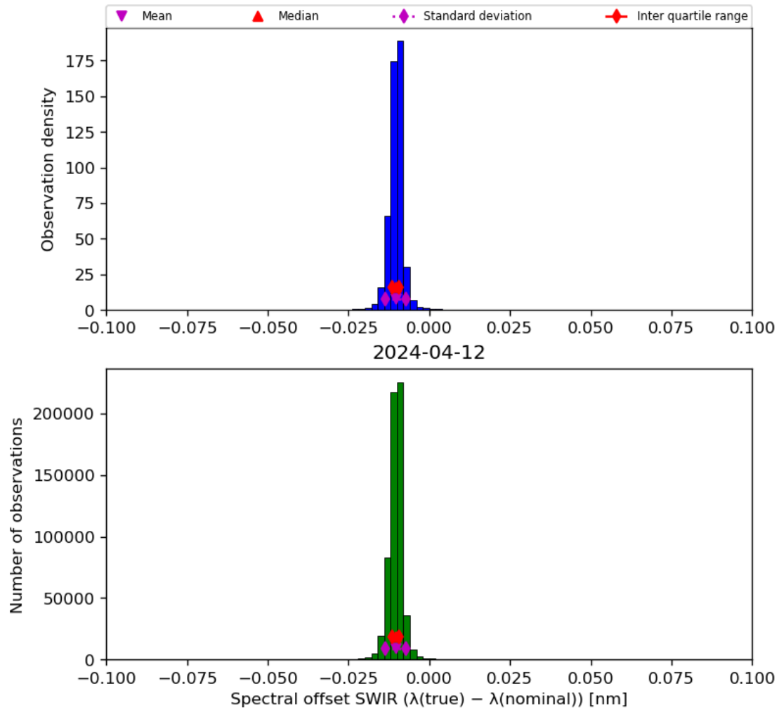
Figure 27: Histogram of “Spectral offset SWIR ( \lambda(\text{true}) - \lambda(\text{nominal}) )” for 2024-04-11 to 2024-04-13
