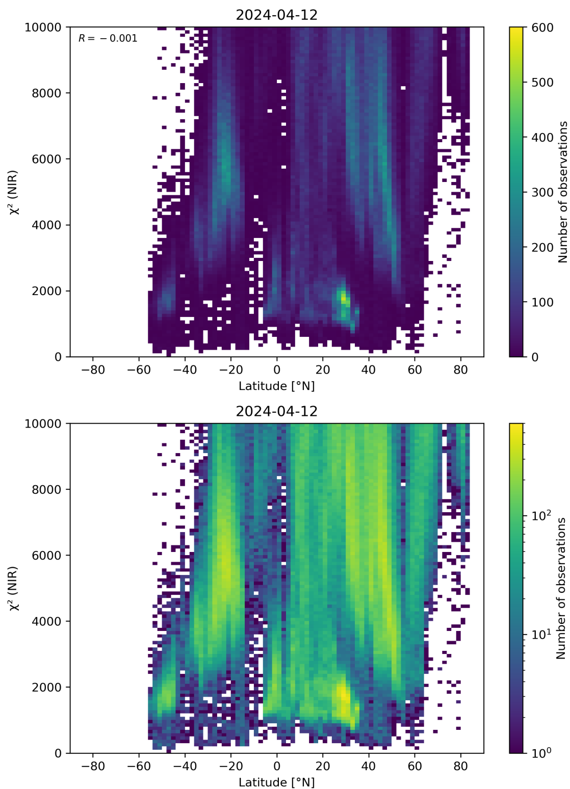
Figure 53: Scatter density plot of “Latitude” against “ \chi^2 (NIR)” for 2024-04-11 to 2024-04-13.
