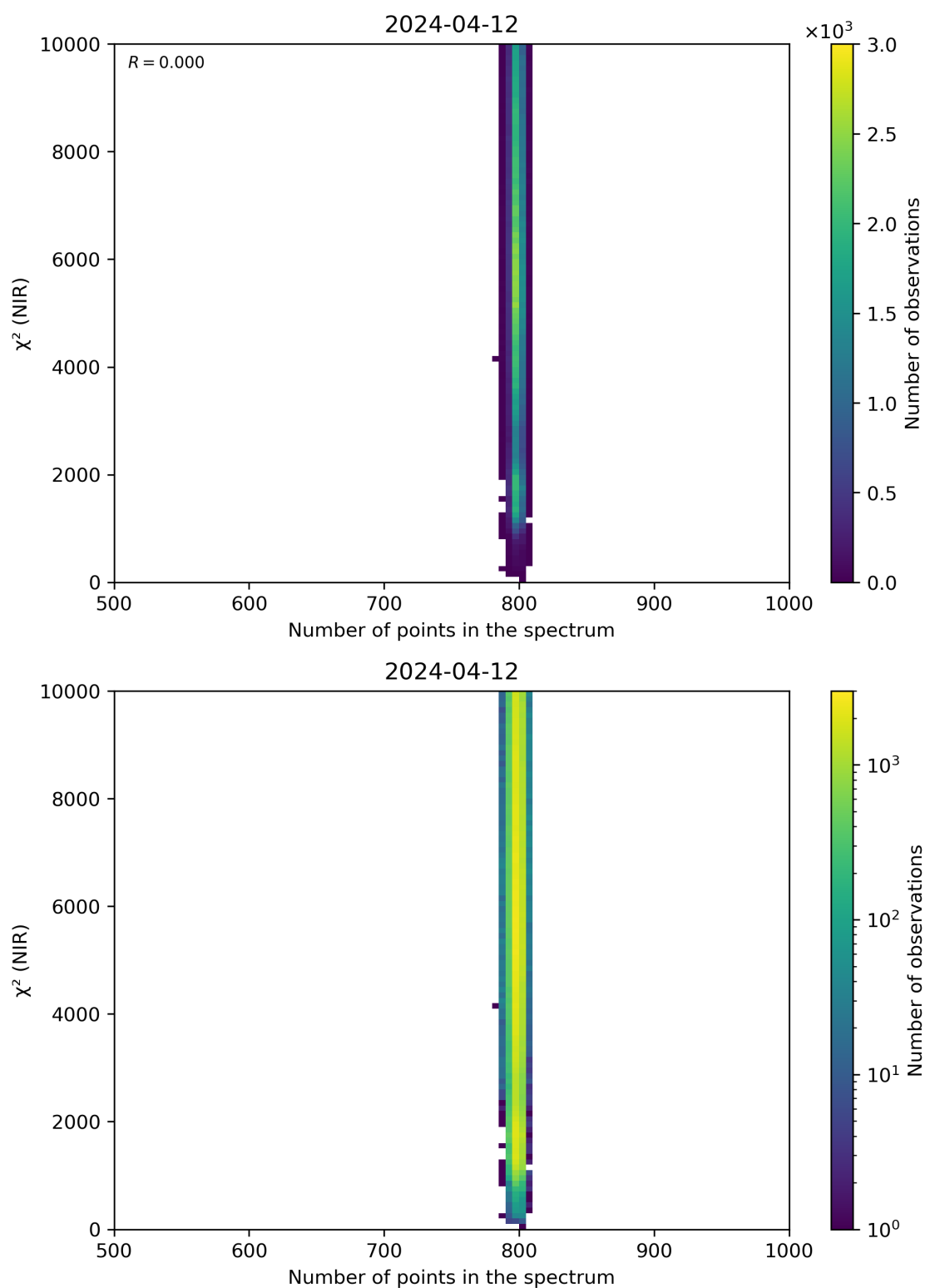
Figure 88: Scatter density plot of “Number of points in the spectrum” against “ \chi^2 (NIR)” for 2024-04-11 to 2024-04-13.
