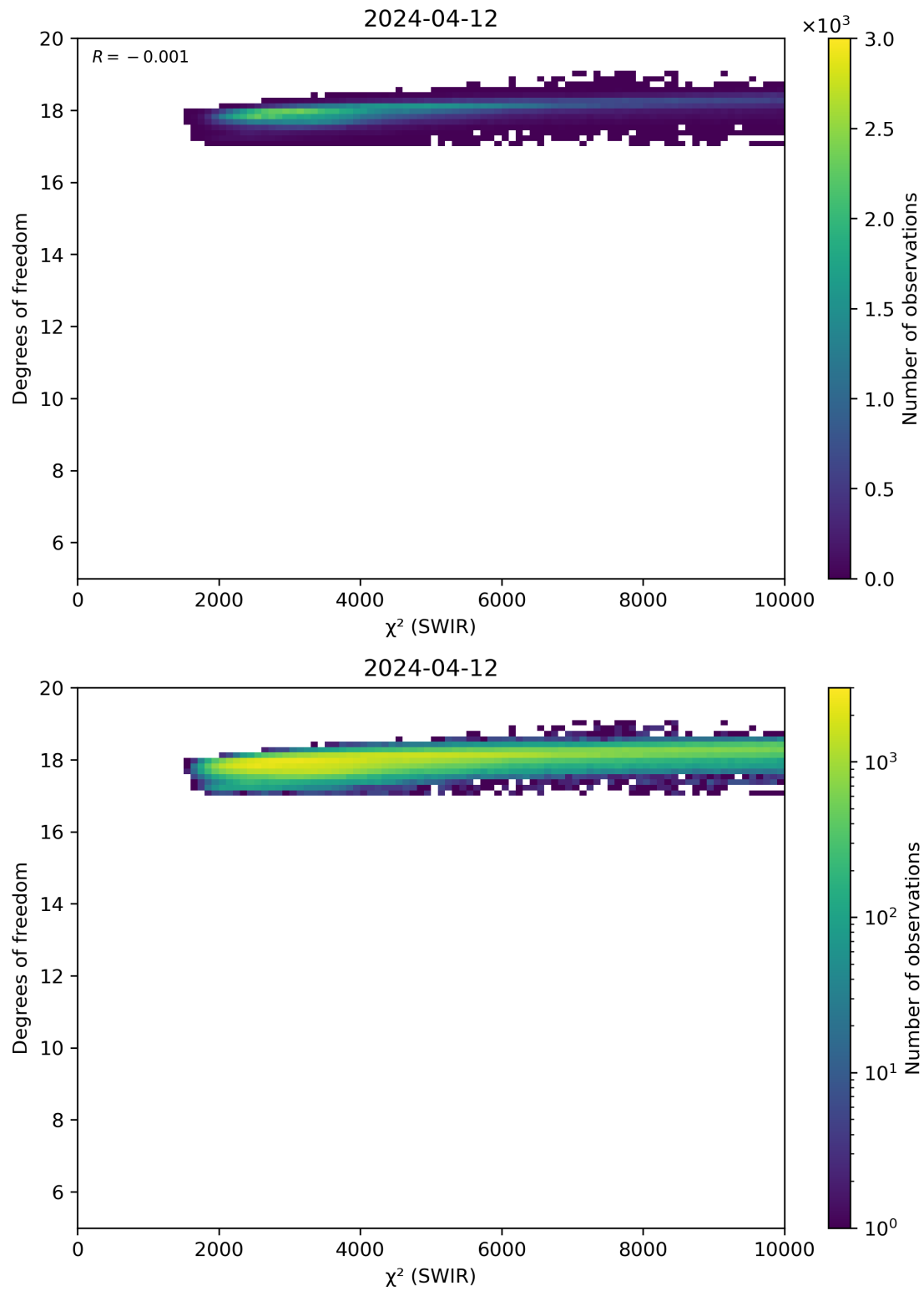
Figure 48: Scatter density plot of “ \chi^2 (SWIR)” against “Degrees of freedom” for 2024-04-11 to 2024-04-13.
