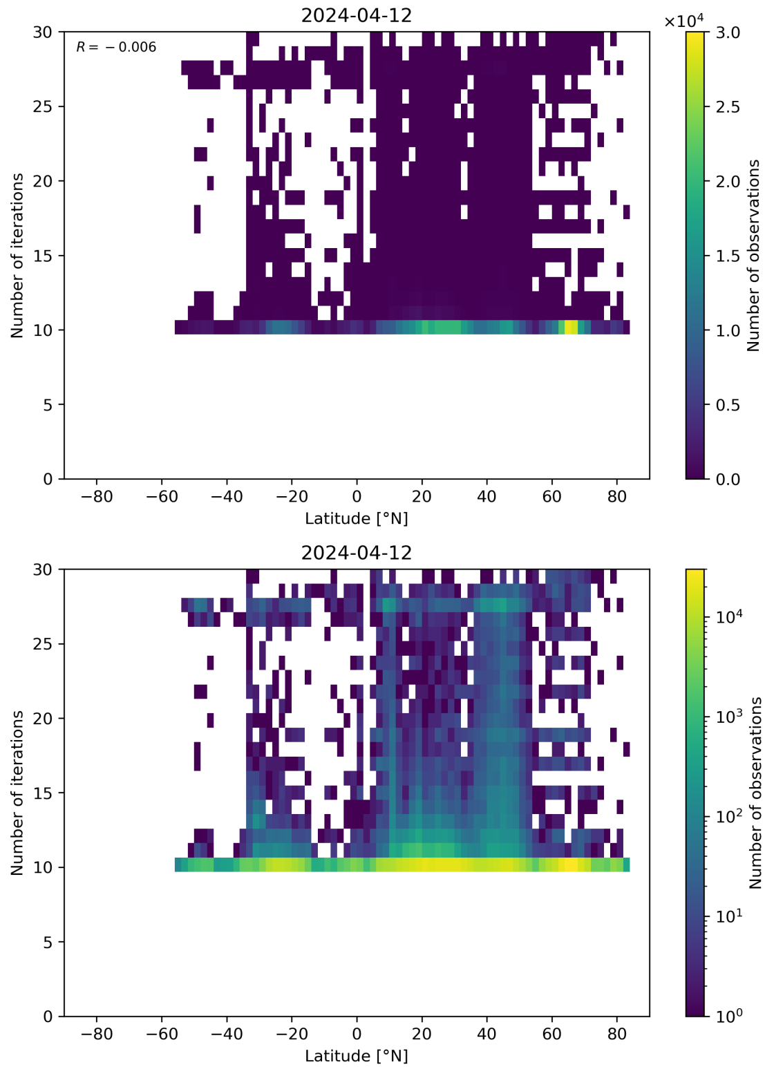
Figure 60: Scatter density plot of “Latitude” against “Number of iterations” for 2024-04-11 to 2024-04-13.
