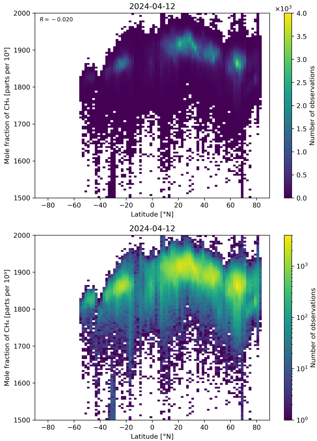
Figure 57: Scatter density plot of “Latitude” against “Mole fraction of CH 4 ” for 2024-04-11 to 2024-04-13.
