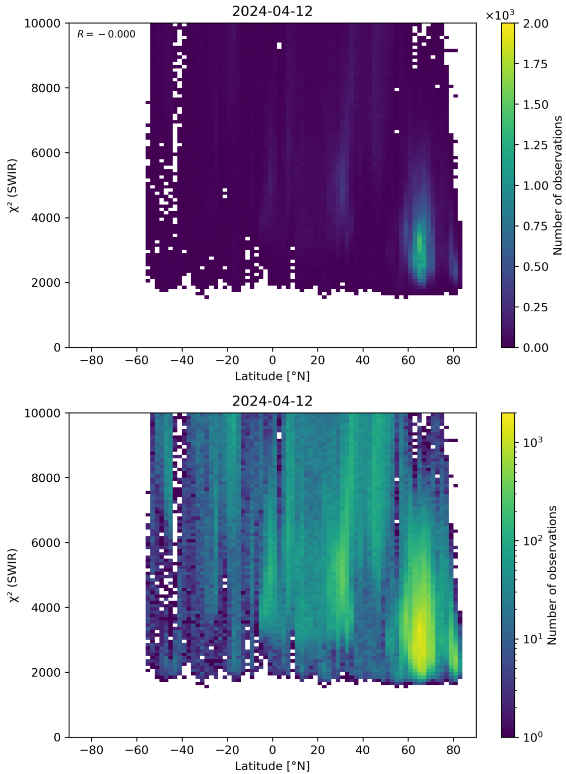
Figure 54: Scatter density plot of “Latitude” against “ \chi^2 (SWIR)” for 2024-04-11 to 2024-04-13.
