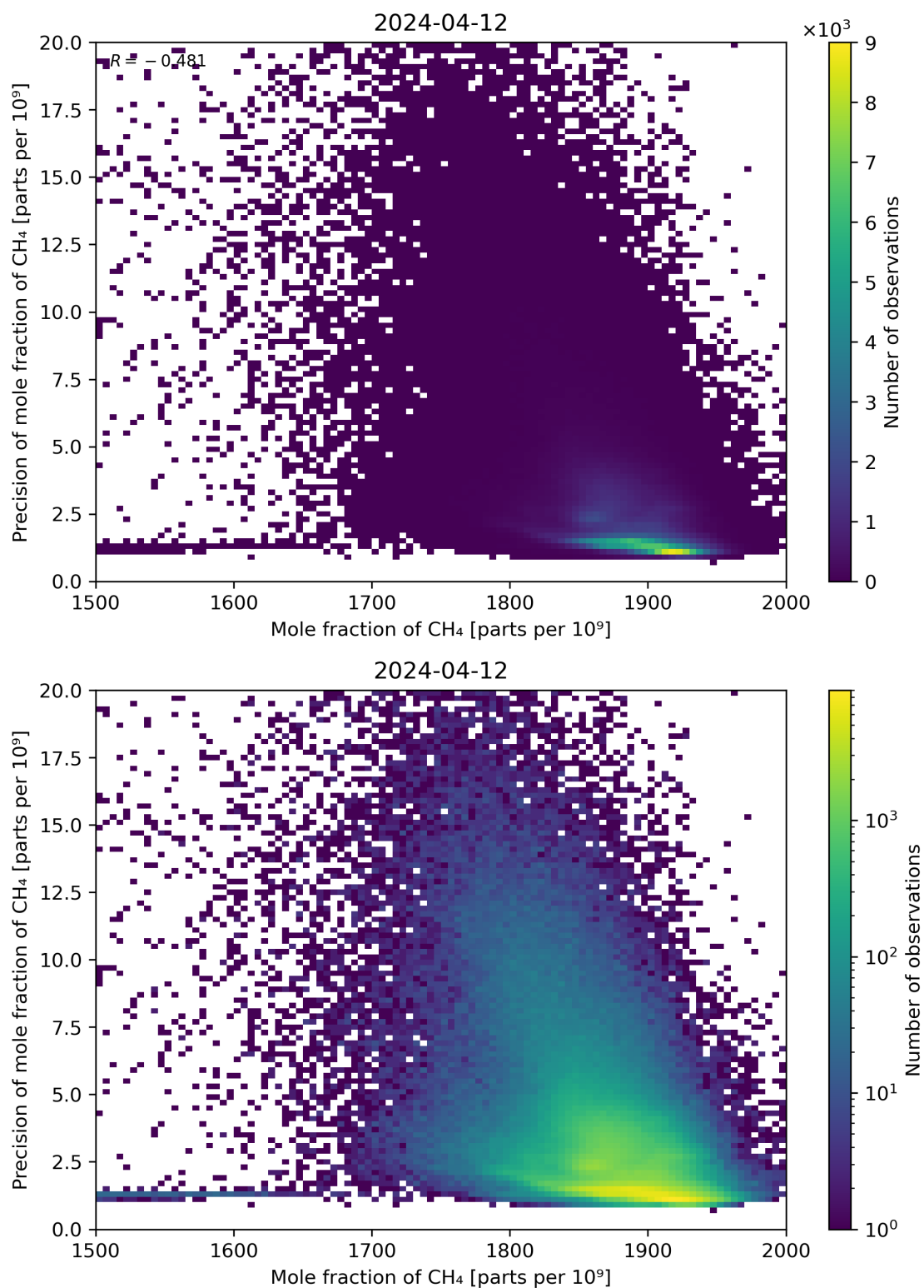
Figure 75: Scatter density plot of “Mole fraction of CH 4 ” against “Precision of mole fraction of CH 4 ” for 2024-04-11 to 2024-04-13.
