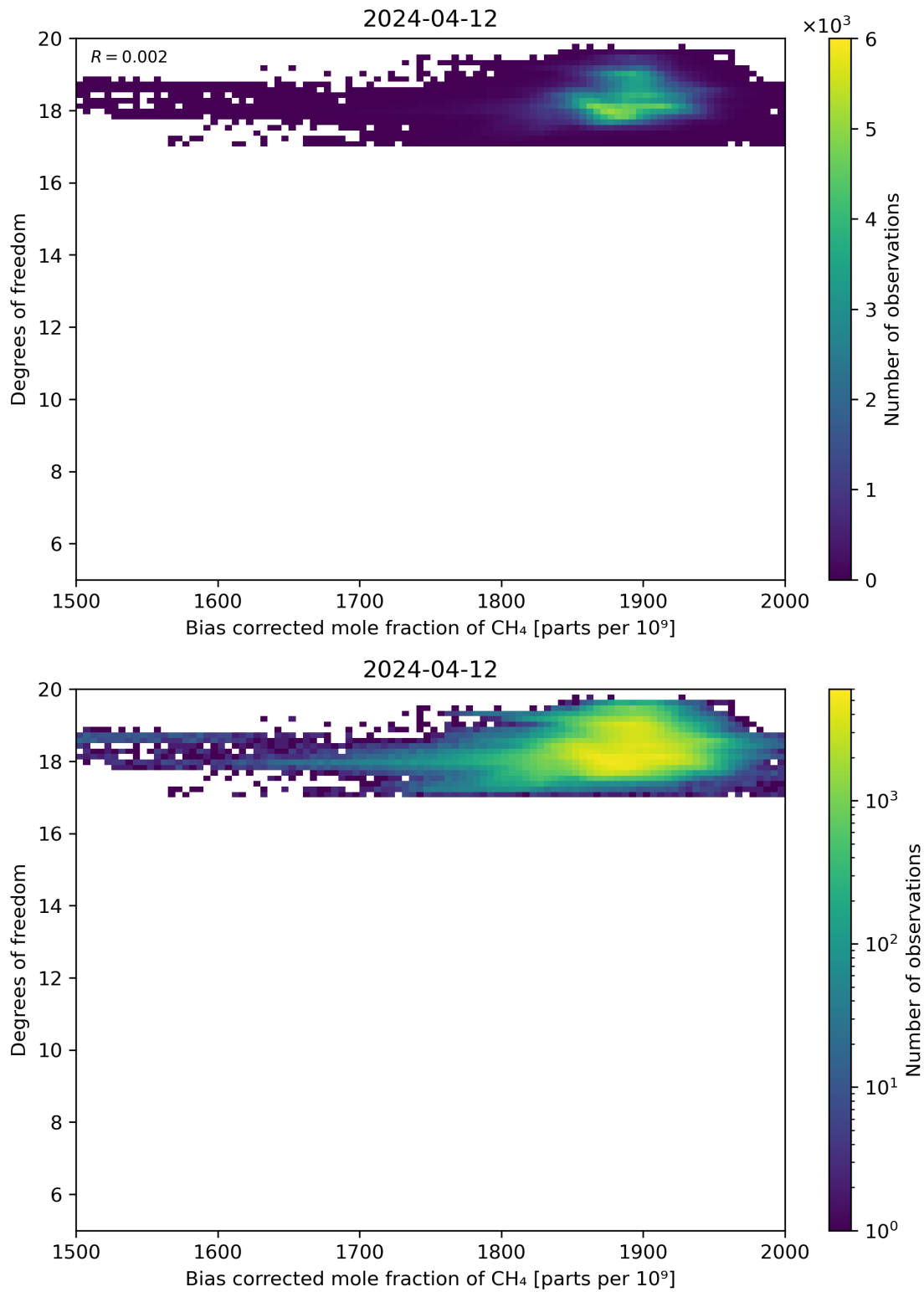
Figure 65: Scatter density plot of “Bias corrected mole fraction of CH 4 ” against “Degrees of freedom” for 2024-04-11 to 2024-04-13.
