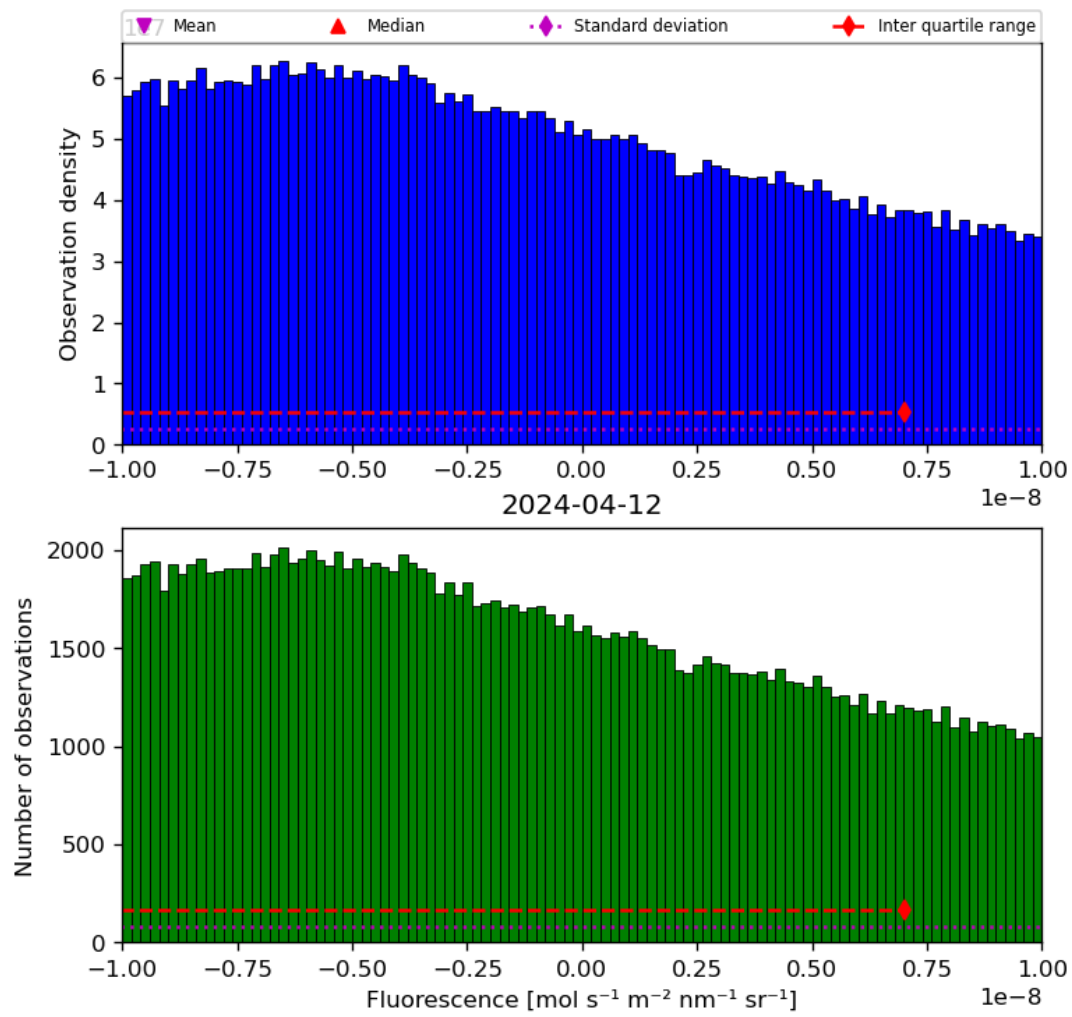
Figure 32: Histogram of “Fluorescence” for 2024-04-11 to 2024-04-13
