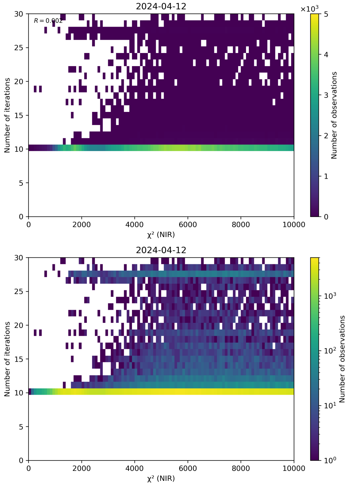
Figure 46: Scatter density plot of “ \chi^2 (NIR)” against “Number of iterations” for 2024-04-11 to 2024-04-13.
