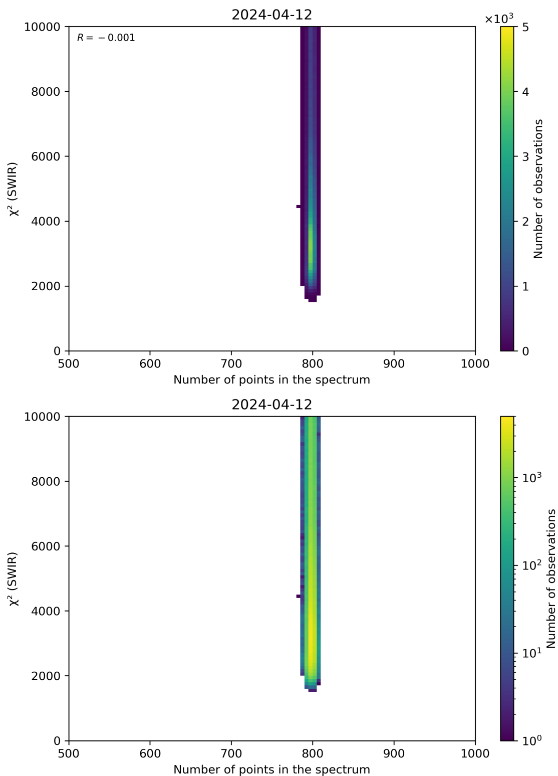
Figure 89: Scatter density plot of “Number of points in the spectrum” against “ \chi^2 (SWIR)” for 2024-04-11 to 2024-04-13.
