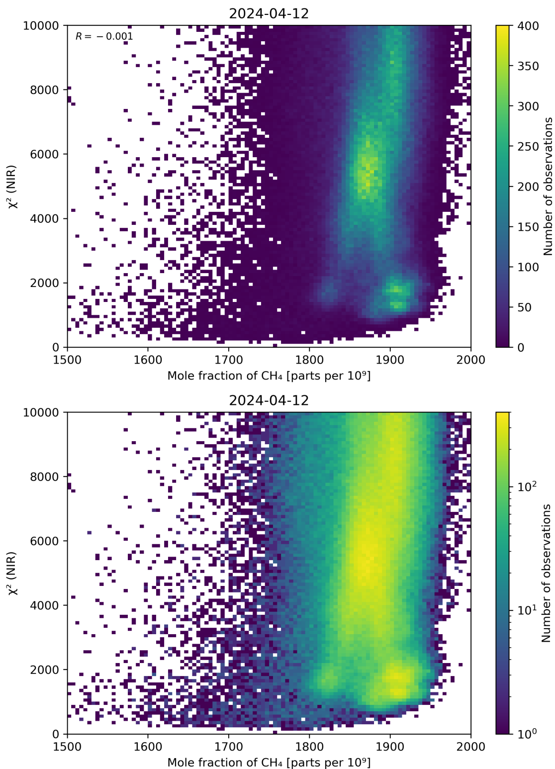
Figure 70: Scatter density plot of “Mole fraction of CH 4 ” against “ \chi^2 (NIR)” for 2024-04-11 to 2024-04-13.
