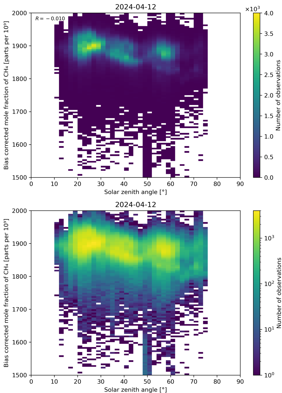
Figure 100: Scatter density plot of “Solar zenith angle” against “Bias corrected mole fraction of CH 4 ” for 2024-04-11 to 2024-04-13.
