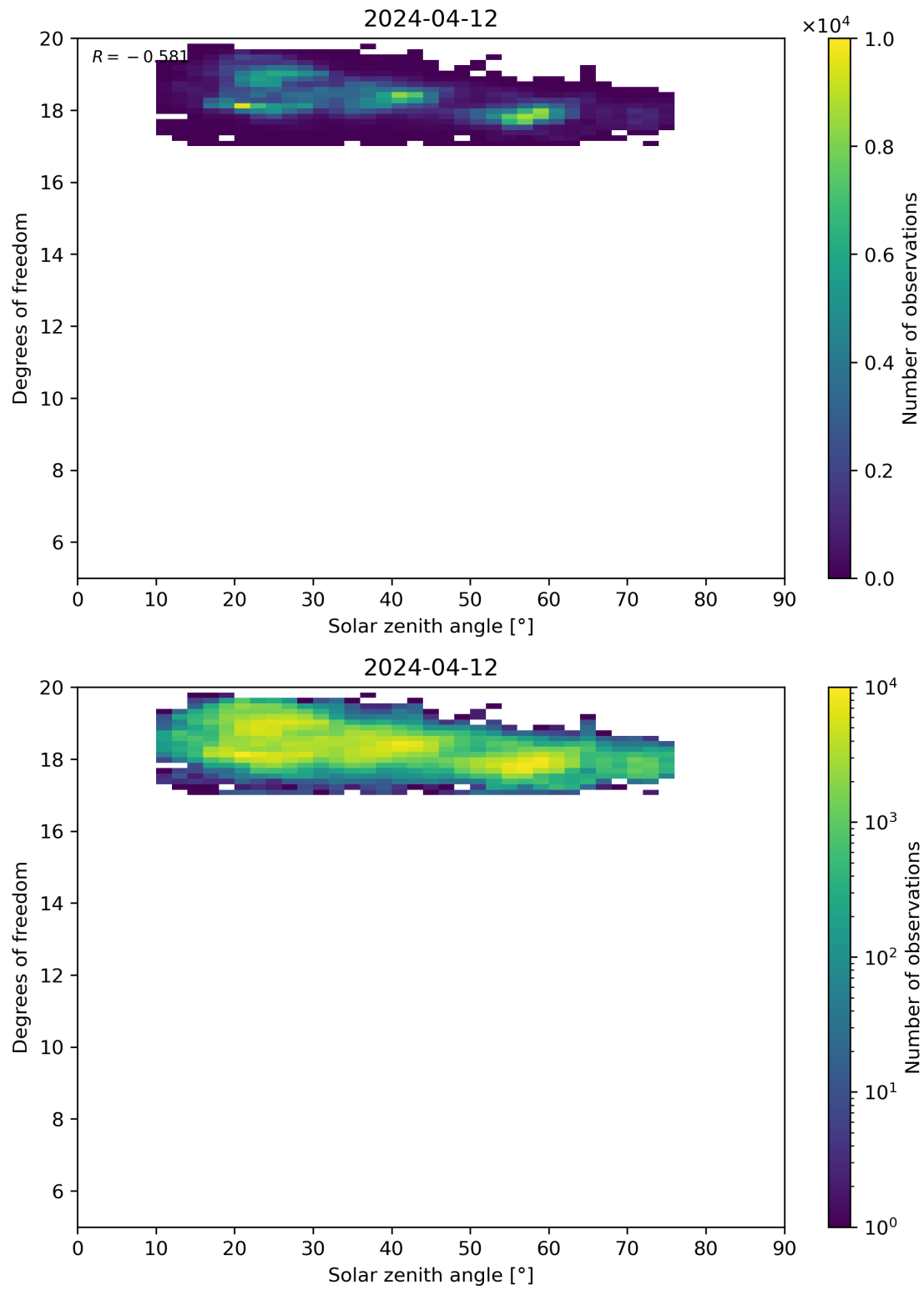
Figure 96: Scatter density plot of “Solar zenith angle” against “Degrees of freedom” for 2024-04-11 to 2024-04-13.
