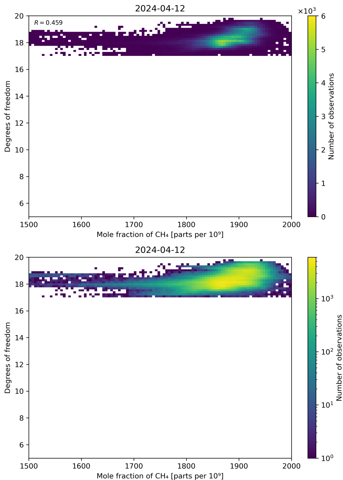
Figure 72: Scatter density plot of “Mole fraction of CH 4 ” against “Degrees of freedom” for 2024-04-11 to 2024-04-13.
