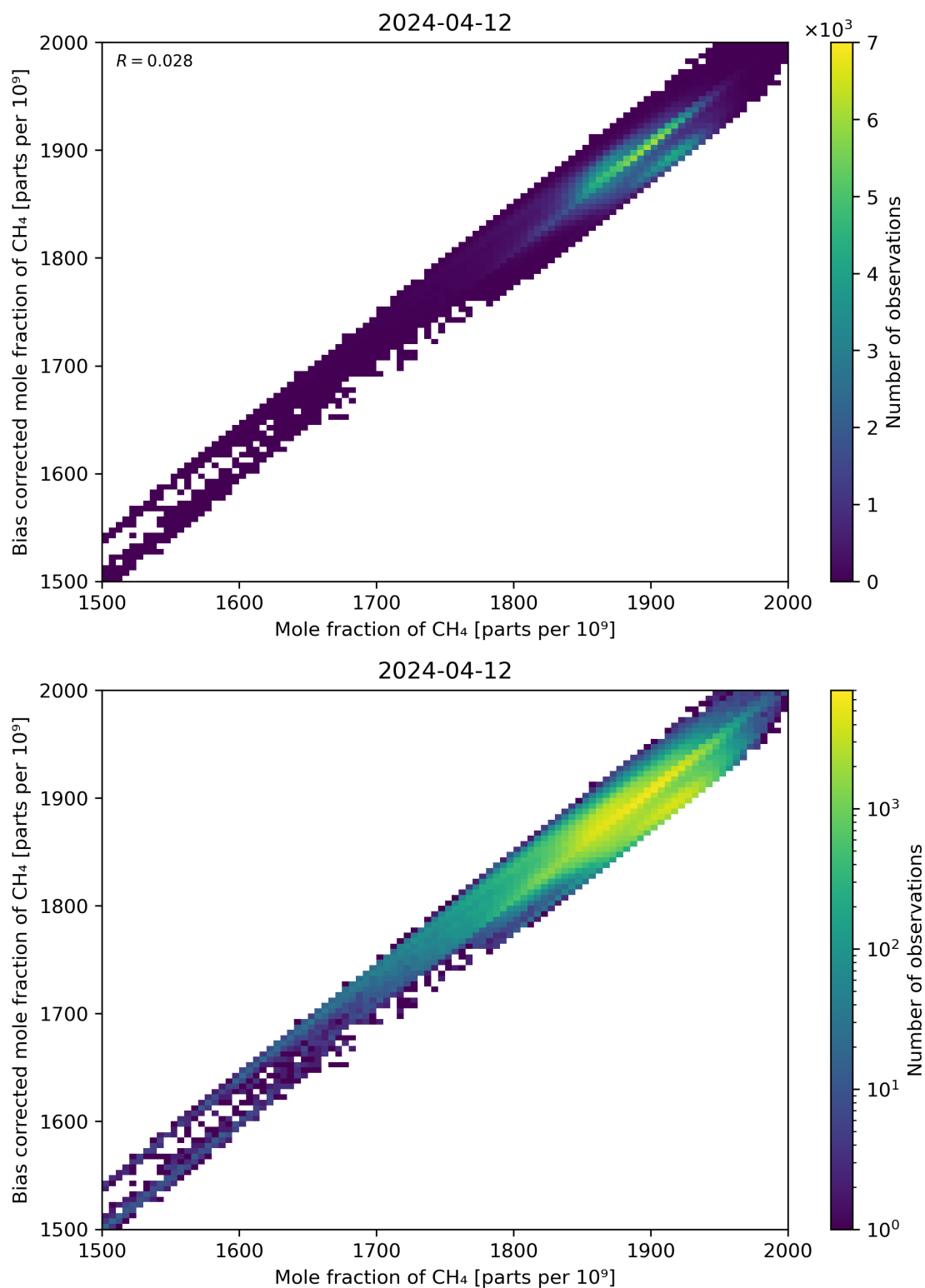
Figure 74: Scatter density plot of “Mole fraction of CH 4 ” against “Bias corrected mole fraction of CH 4 ” for 2024-04-11 to 2024-04-13.
