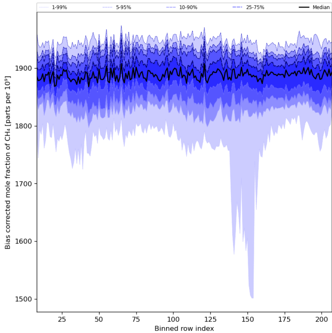
Figure 36: Along track statistics of “Bias corrected mole fraction of CH 4 ” for 2024-04-11 to 2024-04-13
