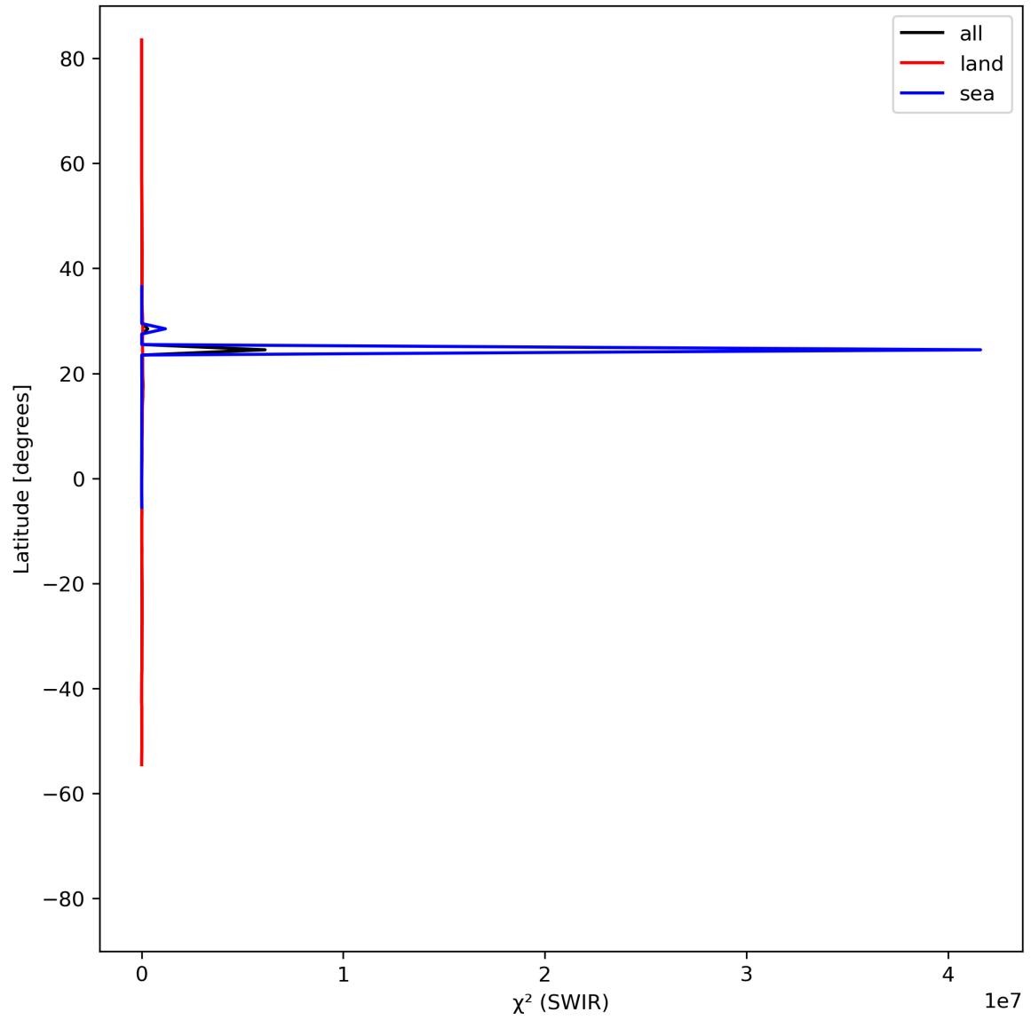
Figure 17: Zonal average of “ \chi^2 (SWIR)” for 2024-04-11 to 2024-04-13.
