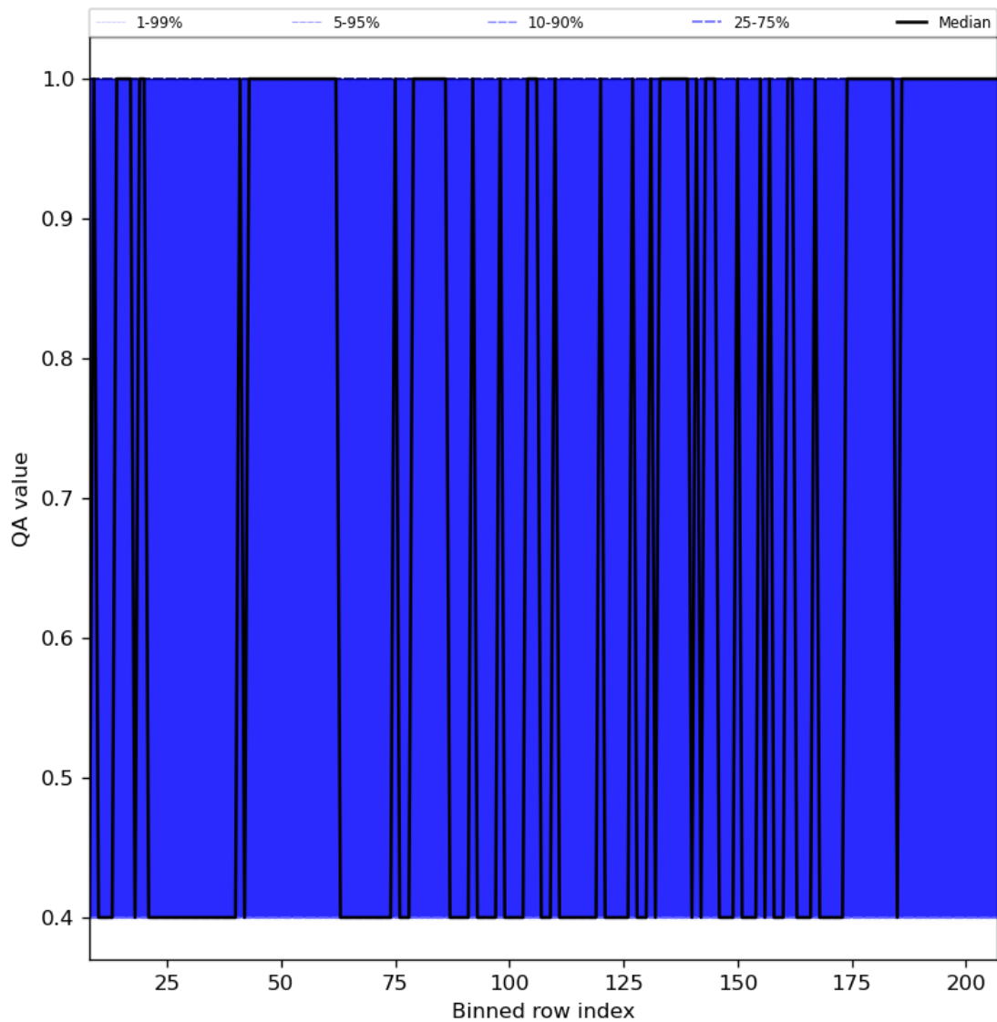
Figure 33: Along track statistics of “QA value” for 2024-04-11 to 2024-04-13
