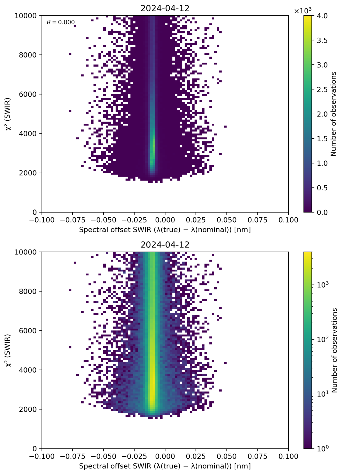
Figure 118: Scatter density plot of “Spectral offset SWIR ( \lambda(\text{true}) - \lambda(\text{nominal}) )” against “ \chi^2 (SWIR)” for 2024-04-11 to 2024-04-13.
