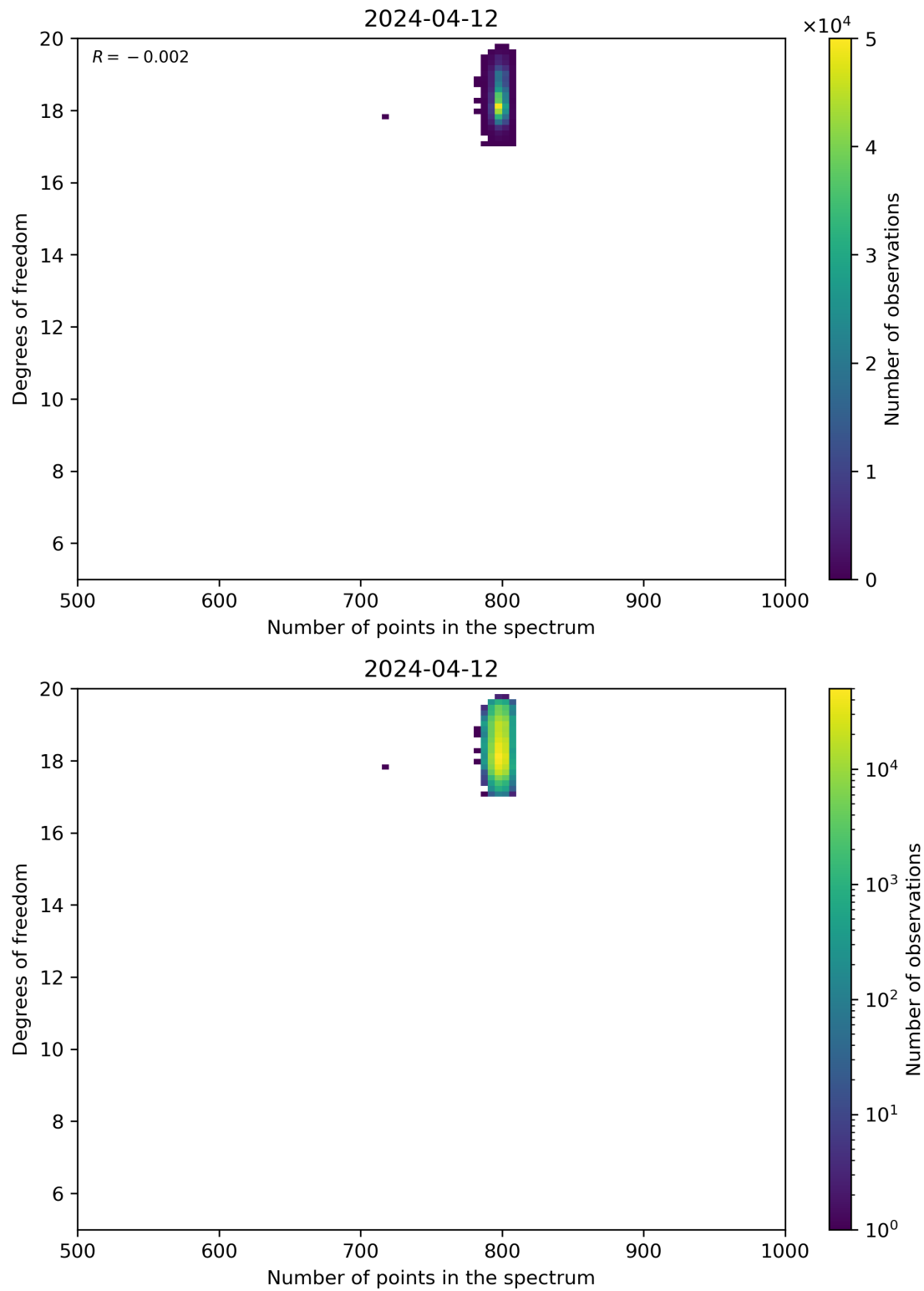
Figure 90: Scatter density plot of “Number of points in the spectrum” against “Degrees of freedom” for 2024-04-11 to 2024-04-13.
