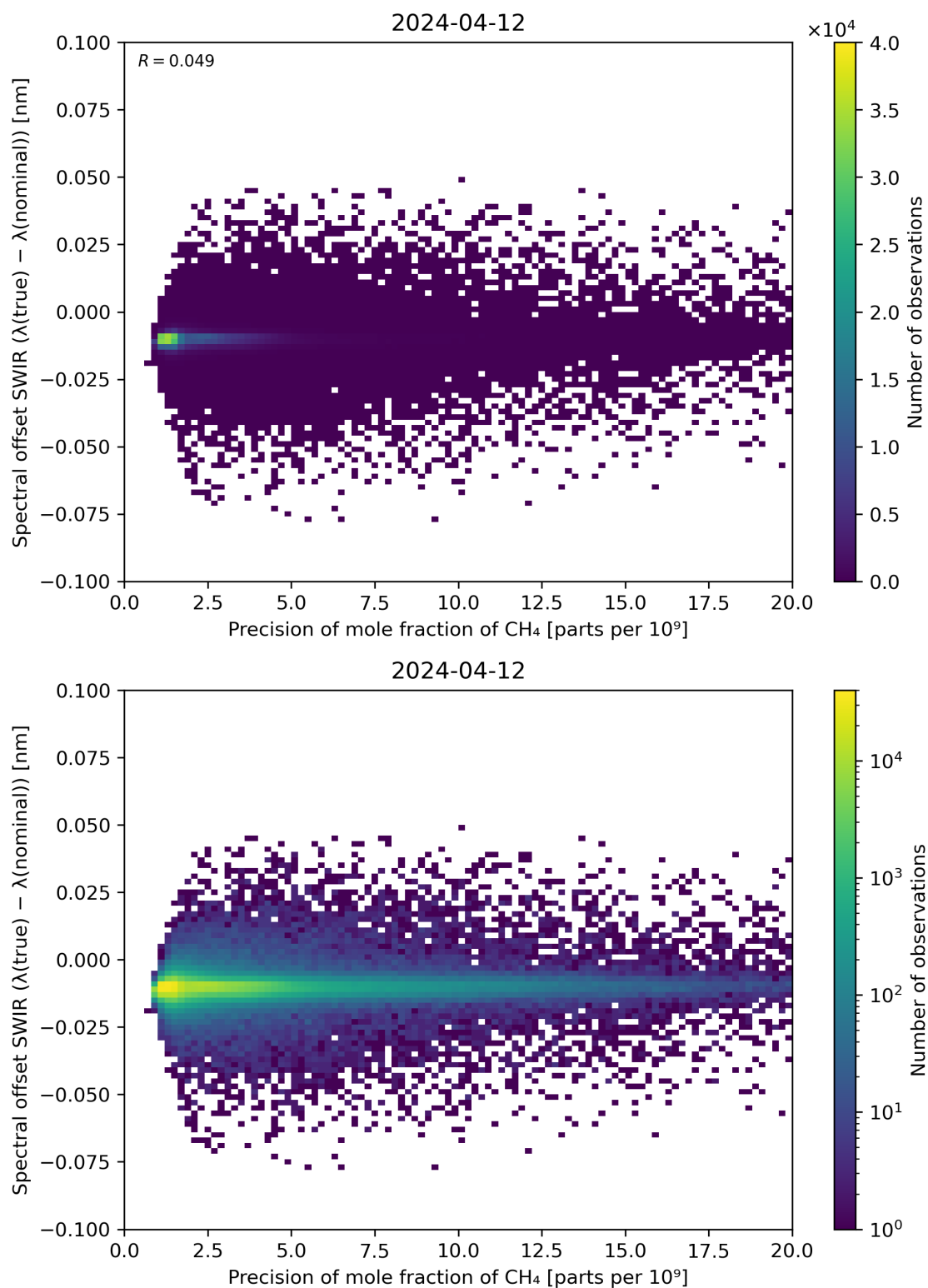
Figure 85: Scatter density plot of “Precision of mole fraction of \text{CH}_4 ” against “Spectral offset SWIR ( \lambda(\text{true}) - \lambda(\text{nominal}) )” for 2024-04-11 to 2024-04-13.
