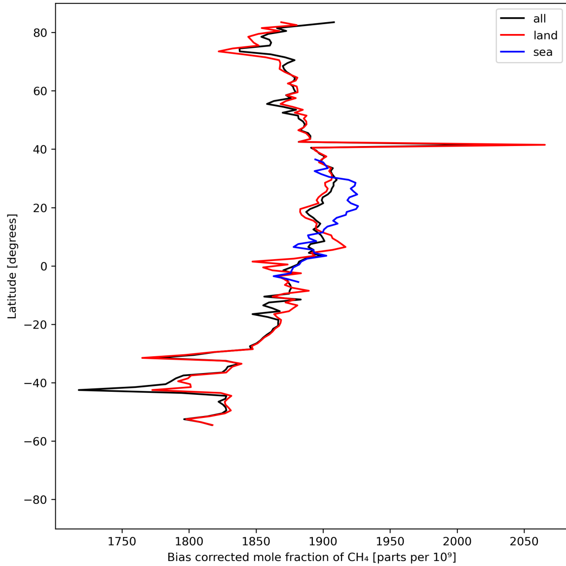
Figure 14: Zonal average of “Bias corrected mole fraction of CH 4 ” for 2024-04-11 to 2024-04-13.
