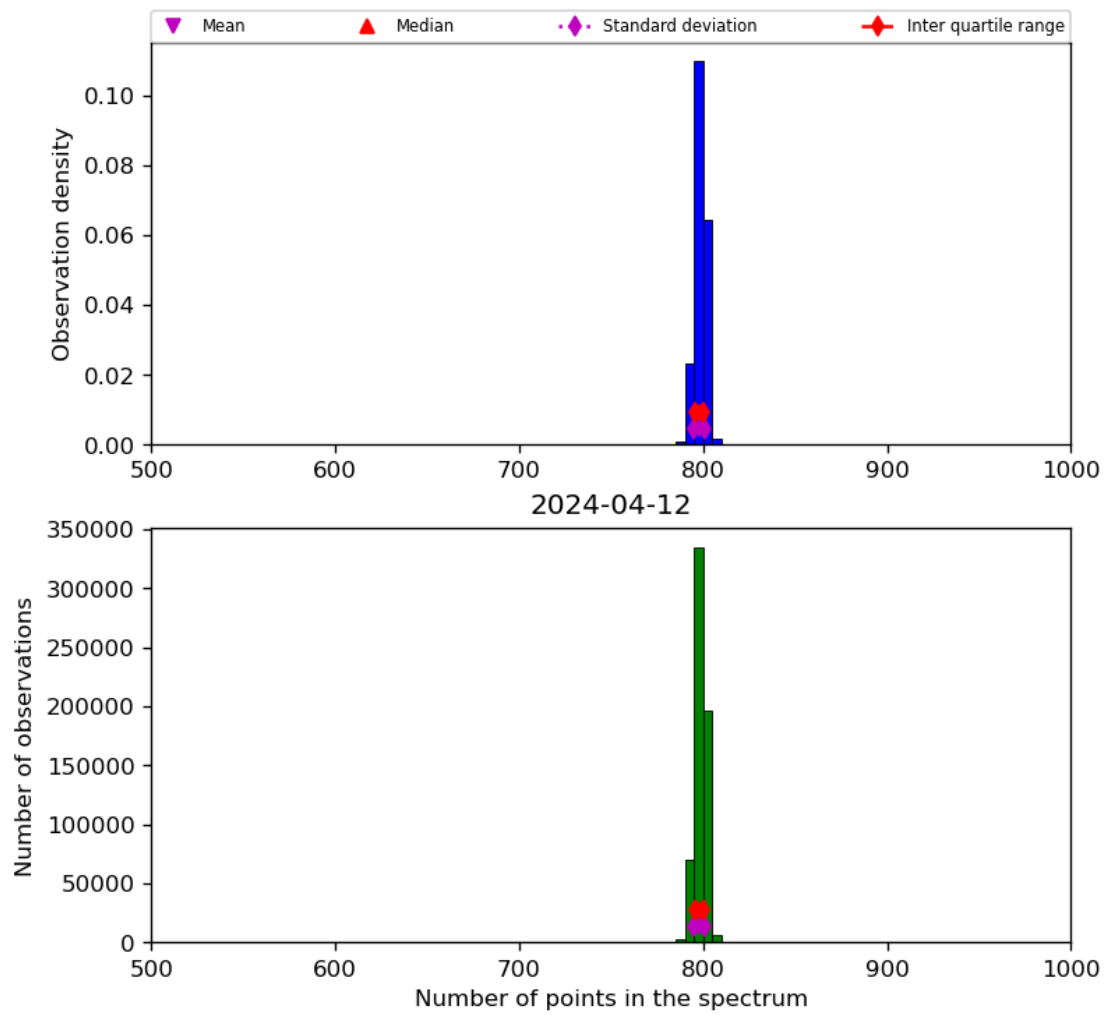
Figure 26: Histogram of “Number of points in the spectrum” for 2024-04-11 to 2024-04-13
