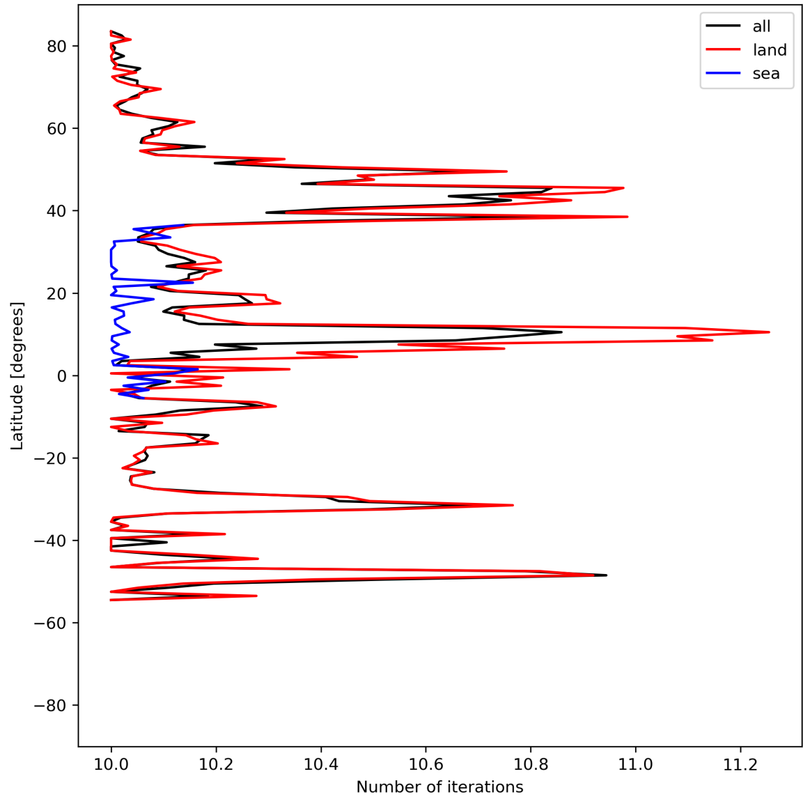
Figure 20: Zonal average of “Number of iterations” for 2024-04-11 to 2024-04-13.
