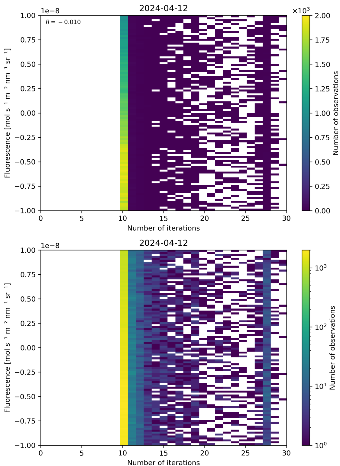
Figure 87: Scatter density plot of “Number of iterations” against “Fluorescence” for 2024-04-11 to 2024-04-13.
