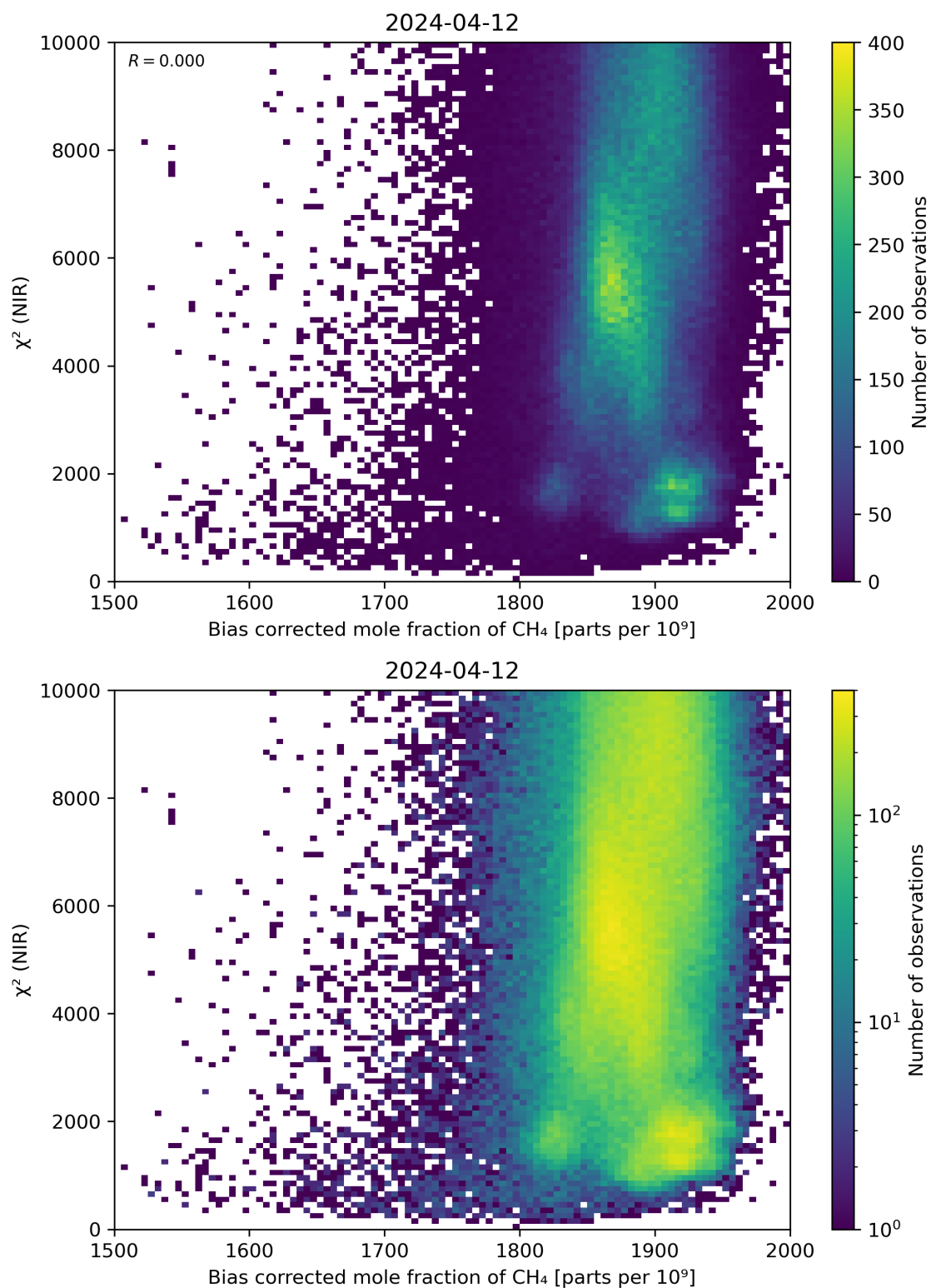
Figure 63: Scatter density plot of “Bias corrected mole fraction of CH 4 ” against “ \chi^2 (NIR)” for 2024-04-11 to 2024-04-13.
