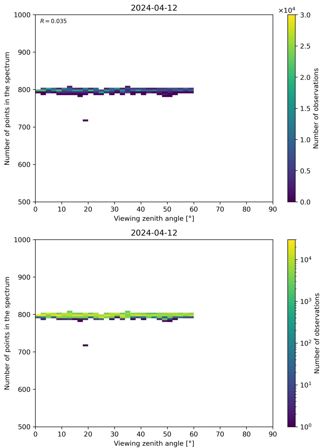
Figure 114: Scatter density plot of “Viewing zenith angle” against “Number of points in the spectrum” for 2024-04-11 to 2024-04-13.
