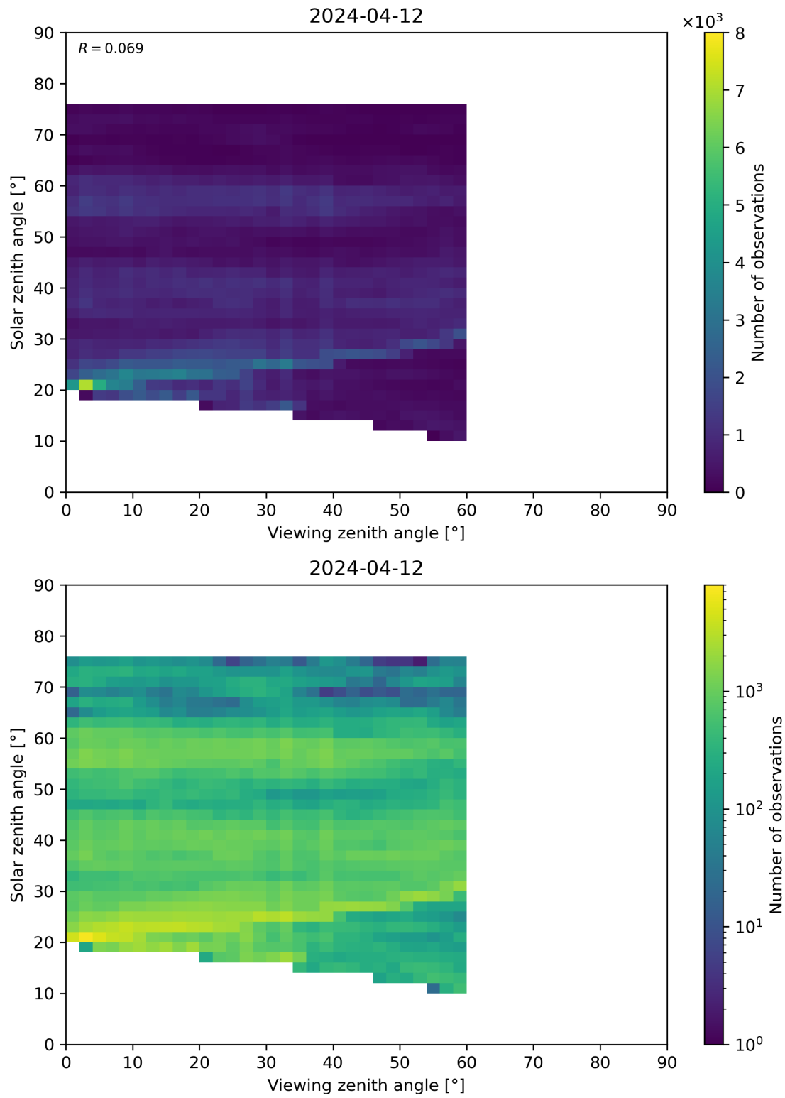
Figure 115: Scatter density plot of “Viewing zenith angle” against “Solar zenith angle” for 2024-04-11 to 2024-04-13.
