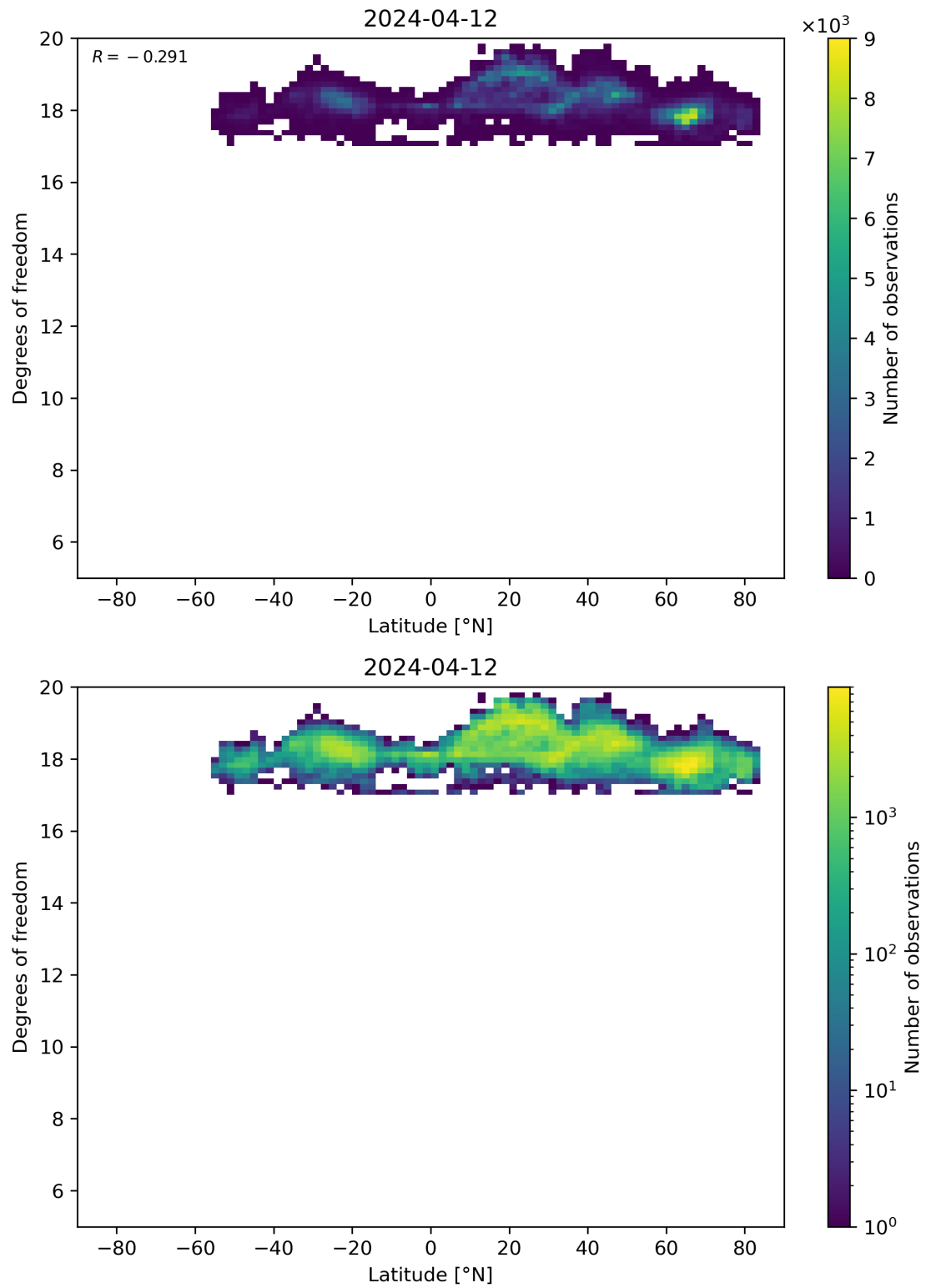
Figure 55: Scatter density plot of “Latitude” against “Degrees of freedom” for 2024-04-11 to 2024-04-13.
