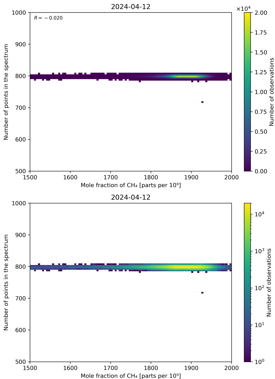
Figure 77: Scatter density plot of “Mole fraction of CH 4 ” against “Number of points in the spectrum” for 2024-04-11 to 2024-04-13.
