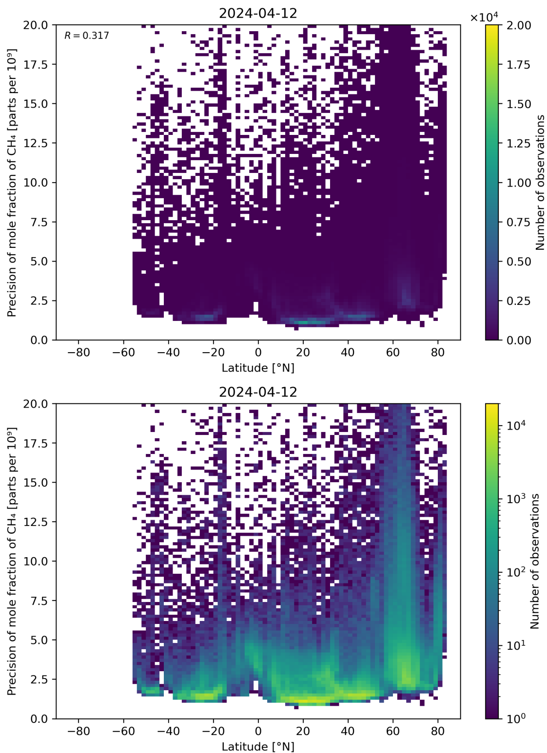
Figure 59: Scatter density plot of “Latitude” against “Precision of mole fraction of \text{CH}_4 ” for 2024-04-11 to 2024-04-13.
