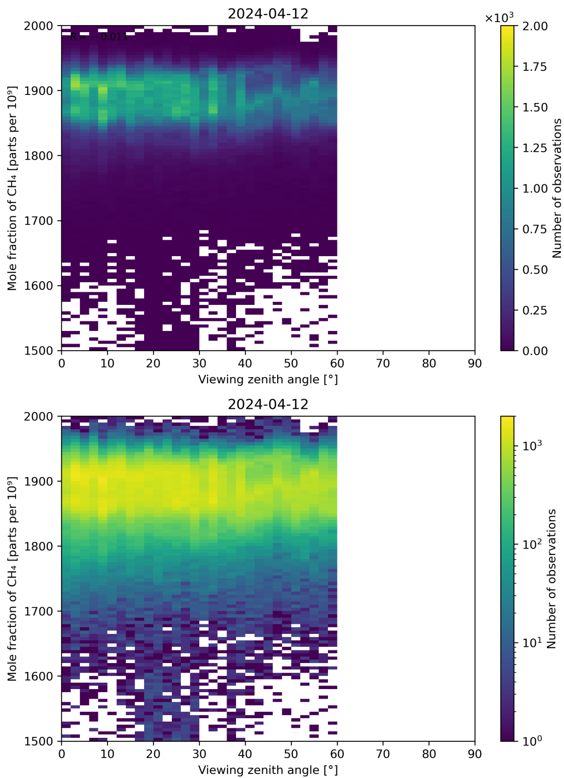
Figure 110: Scatter density plot of “Viewing zenith angle” against “Mole fraction of CH 4 ” for 2024-04-11 to 2024-04-13.
