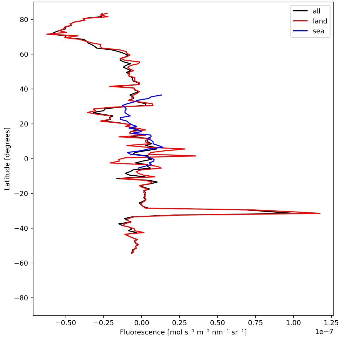
Figure 21: Zonal average of “Fluorescence” for 2024-04-11 to 2024-04-13.
