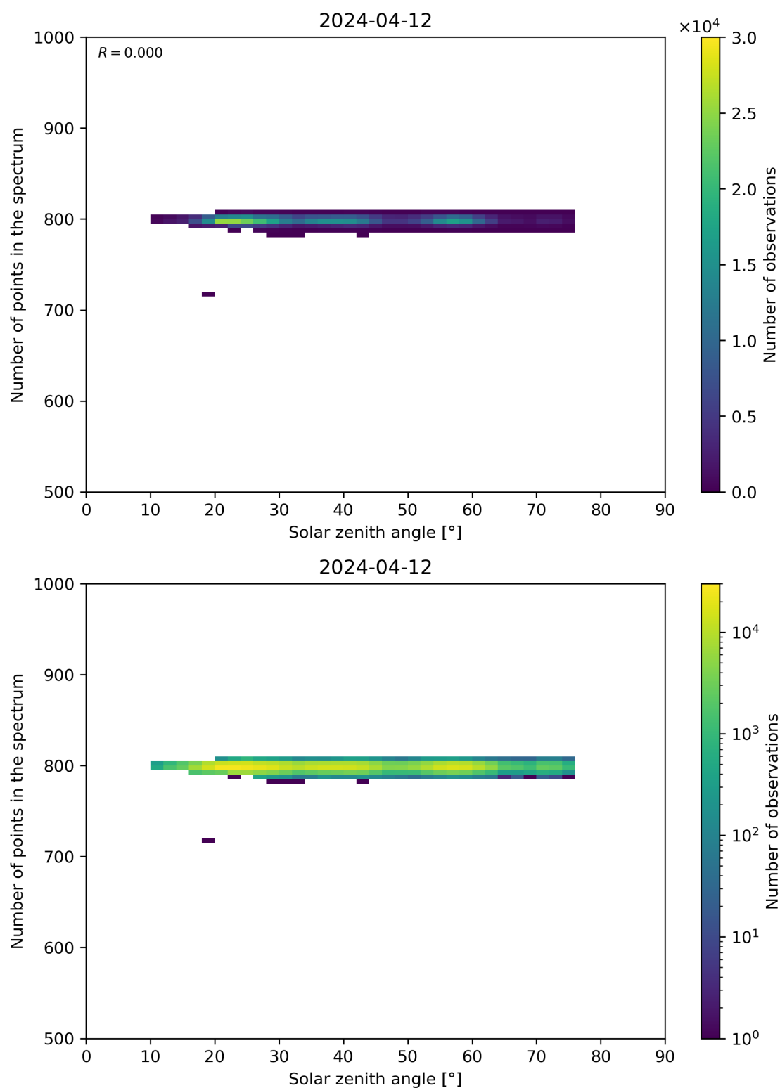
Figure 103: Scatter density plot of “Solar zenith angle” against “Number of points in the spectrum” for 2024-04-11 to 2024-04-13.
