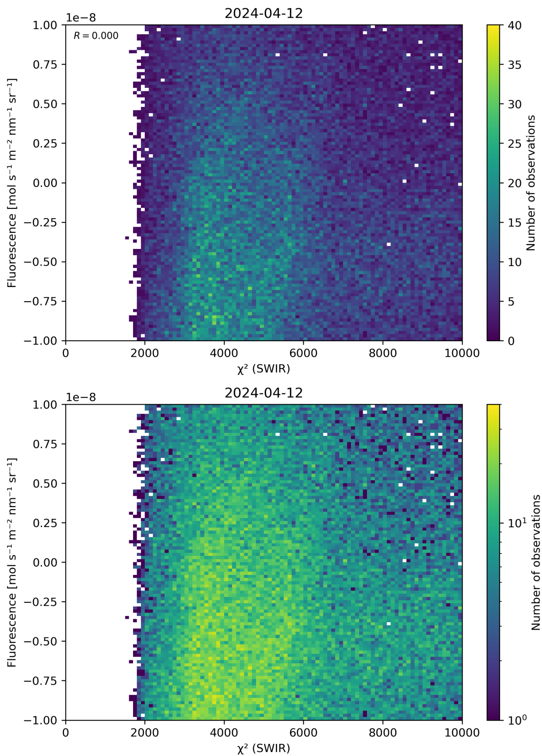
Figure 49: Scatter density plot of “ \chi^2 (SWIR)” against “Fluorescence” for 2024-04-11 to 2024-04-13.
