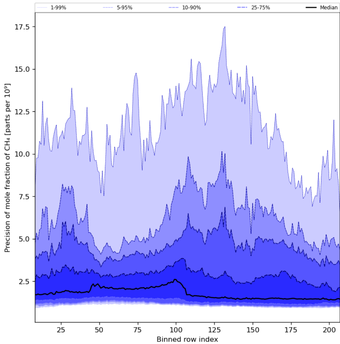
Figure 35: Along track statistics of “Precision of mole fraction of CH 4 ” for 2024-04-11 to 2024-04-13
