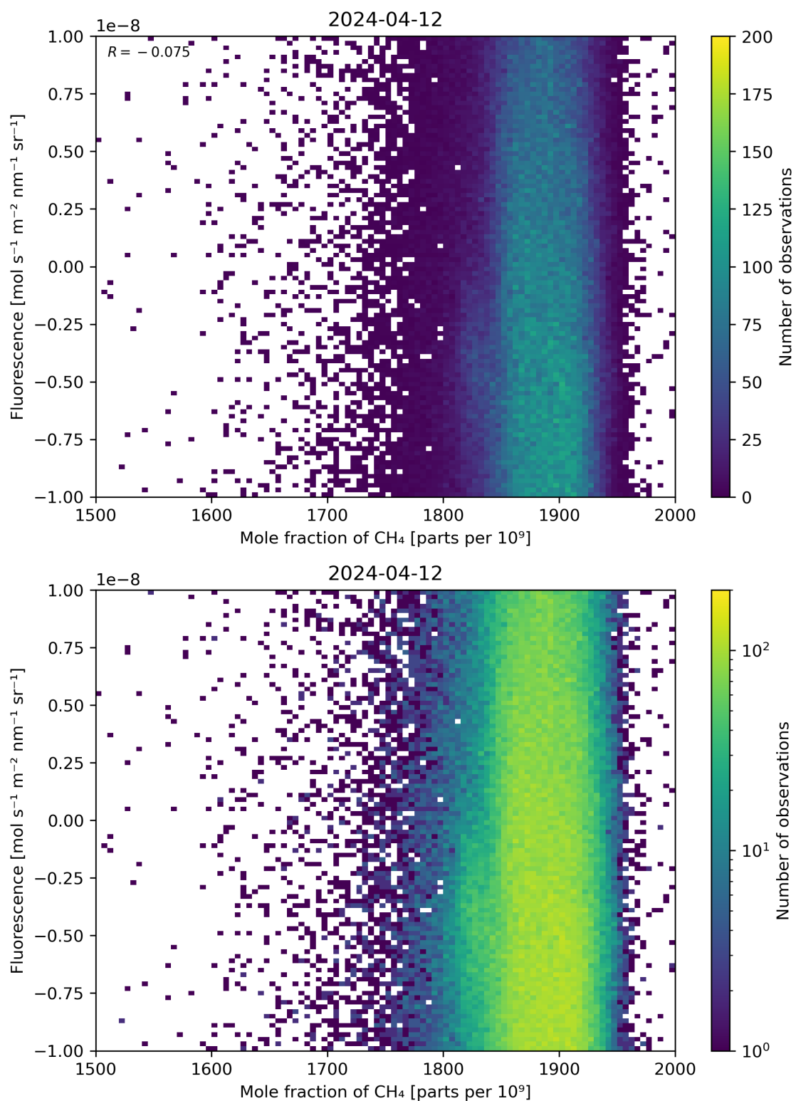
Figure 73: Scatter density plot of “Mole fraction of \text{CH}_4 ” against “Fluorescence” for 2024-04-11 to 2024-04-13.
