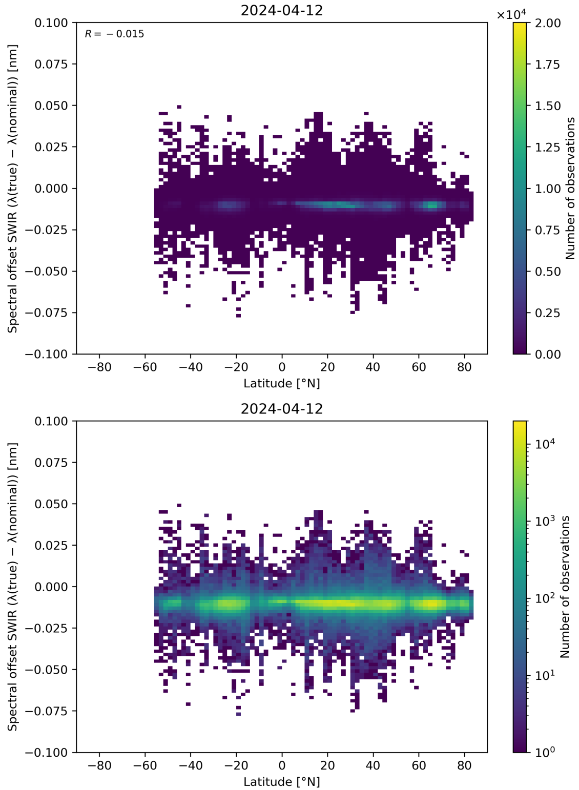
Figure 62: Scatter density plot of “Latitude” against “Spectral offset SWIR ( \lambda(\text{true}) - \lambda(\text{nominal}) )” for 2024-04-11 to 2024-04-13.
