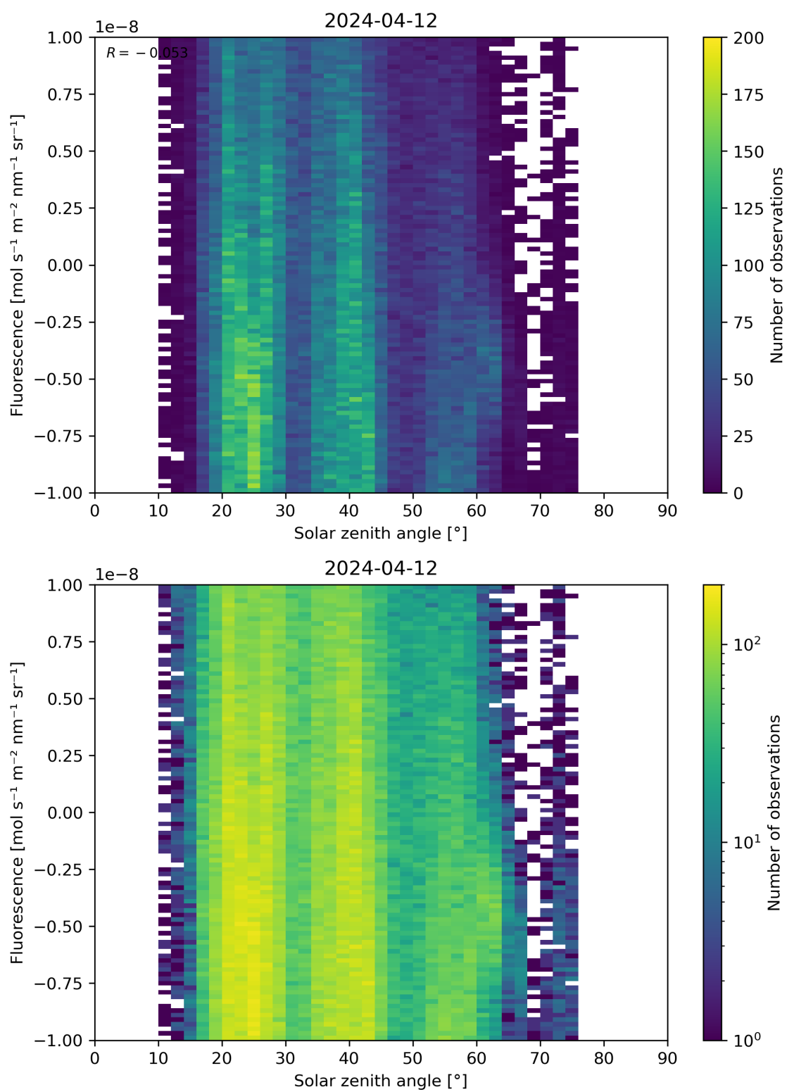
Figure 97: Scatter density plot of “Solar zenith angle” against “Fluorescence” for 2024-04-11 to 2024-04-13.
