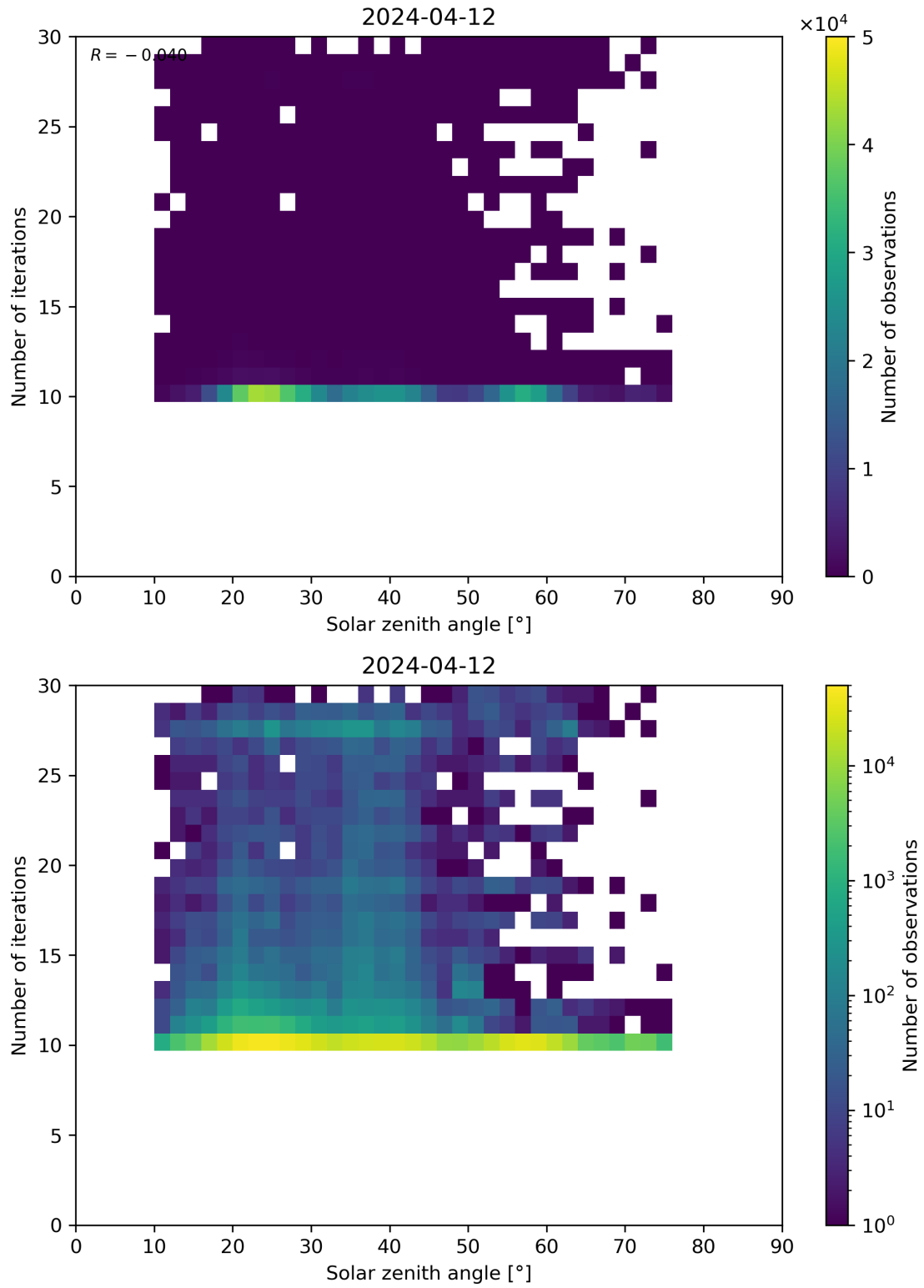
Figure 102: Scatter density plot of “Solar zenith angle” against “Number of iterations” for 2024-04-11 to 2024-04-13.
