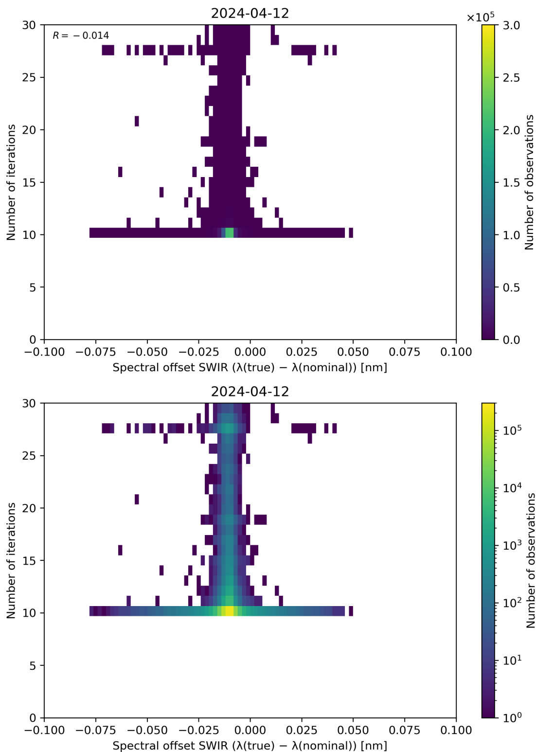
Figure 121: Scatter density plot of “Spectral offset SWIR ( \lambda(\text{true}) - \lambda(\text{nominal}) )” against “Number of iterations” for 2024-04-11 to 2024-04-13.
