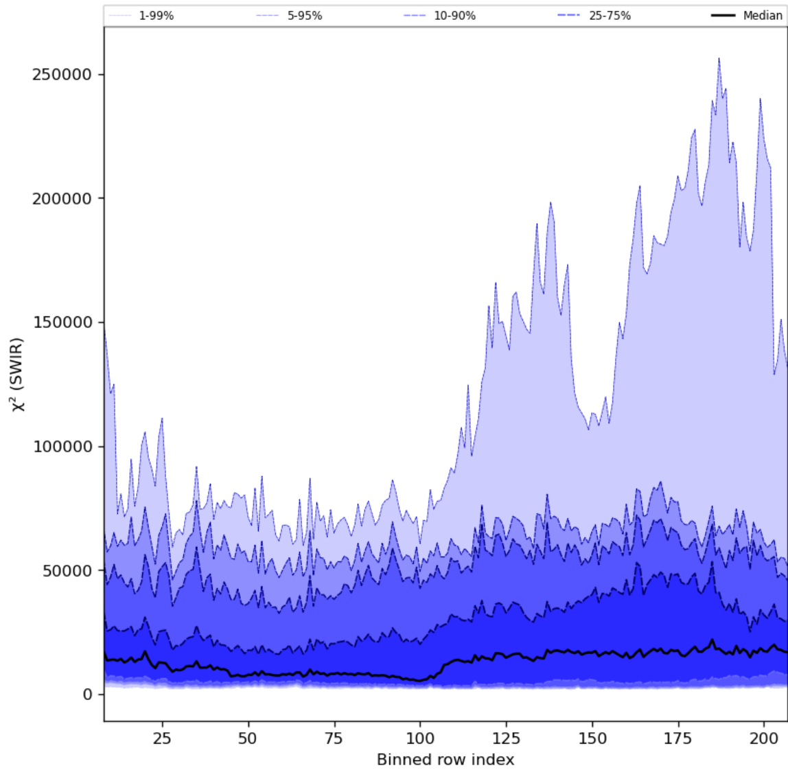
Figure 39: Along track statistics of “ \chi^2 (SWIR)” for 2024-04-11 to 2024-04-13
