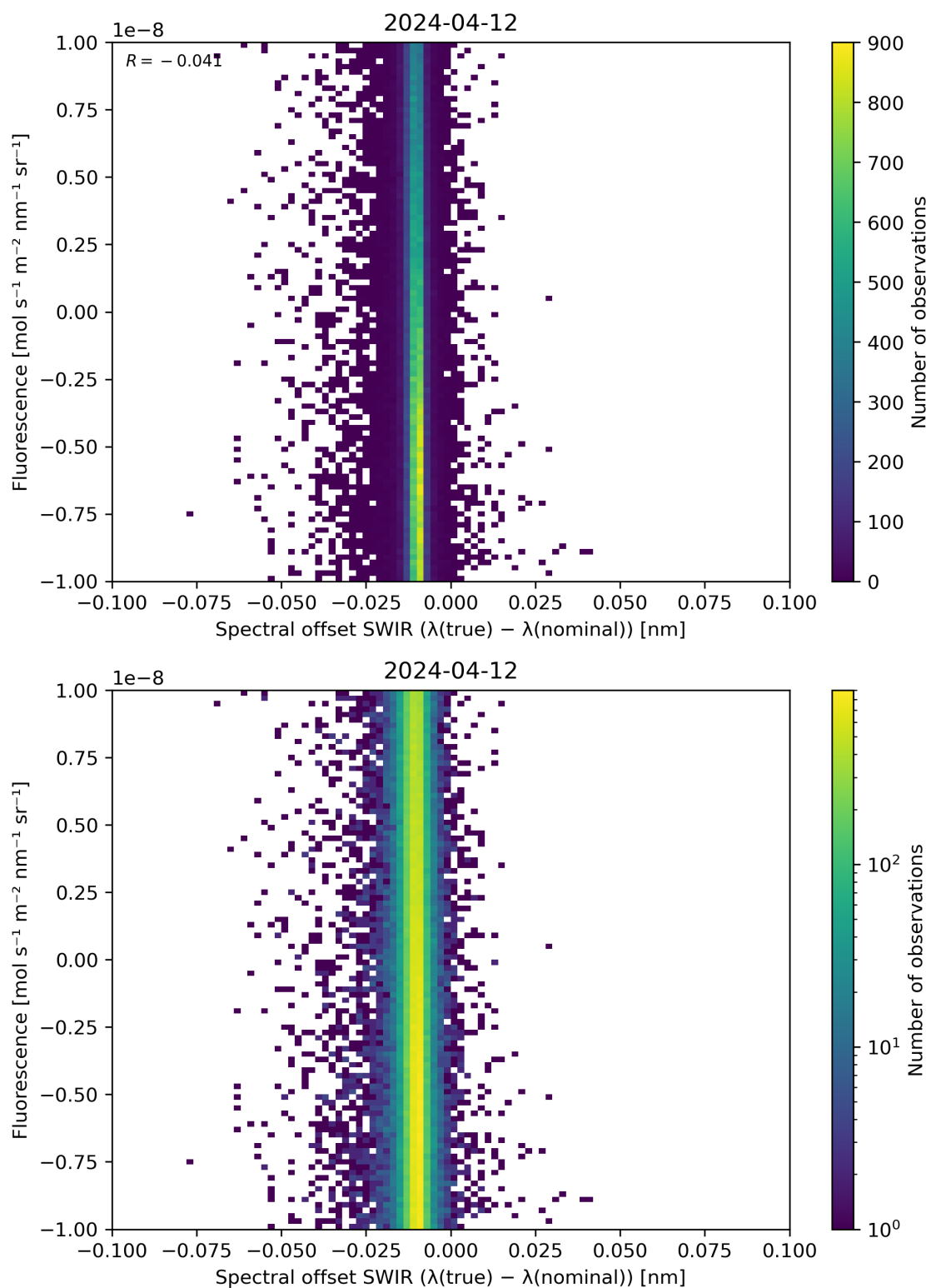
Figure 120: Scatter density plot of “Spectral offset SWIR ( \lambda(\text{true}) - \lambda(\text{nominal}) )” against “Fluorescence” for 2024-04-11 to 2024-04-13.
