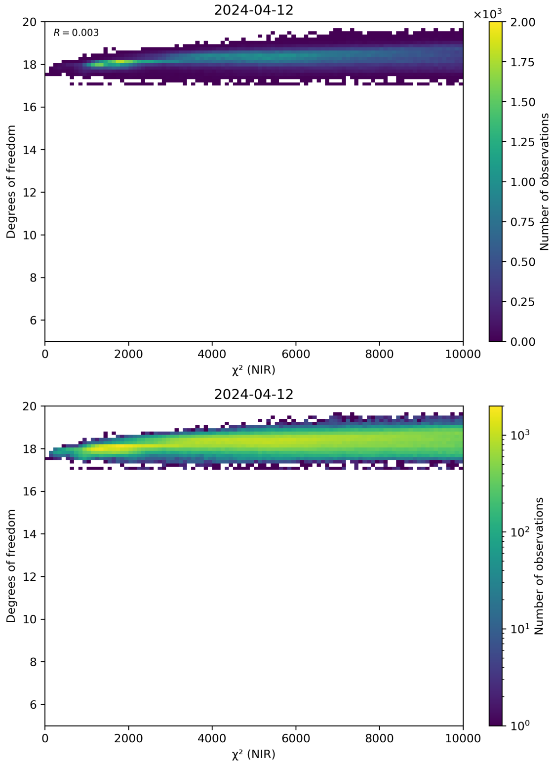
Figure 44: Scatter density plot of “ \chi^2 (NIR)” against “Degrees of freedom” for 2024-04-11 to 2024-04-13.
