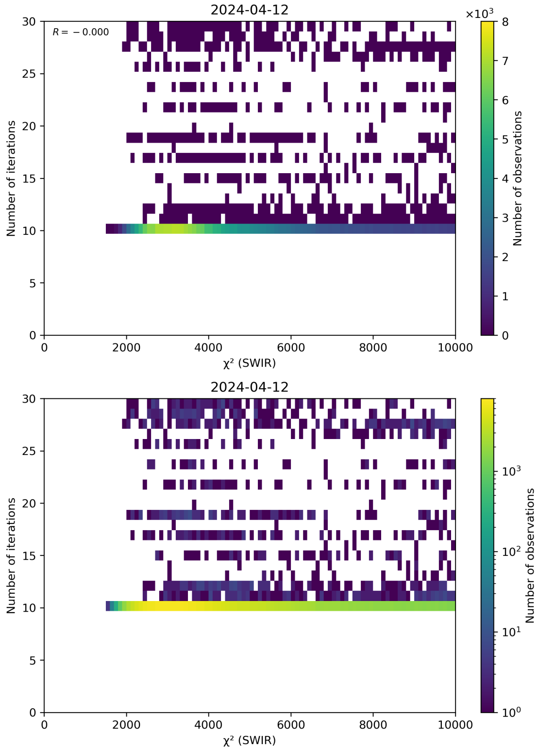
Figure 50: Scatter density plot of “ \chi^2 (SWIR)” against “Number of iterations” for 2024-04-11 to 2024-04-13.
