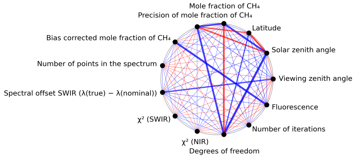
Figure 1: Map of correlation graph for 2024-04-11 to 2024-04-13.
