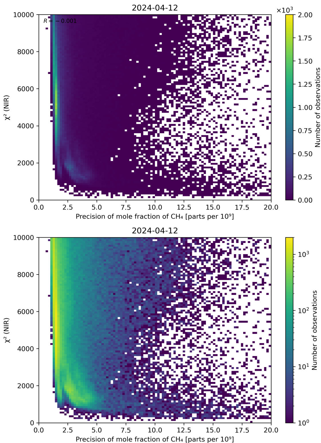
Figure 78: Scatter density plot of “Precision of mole fraction of CH 4 ” against “ \chi^2 (NIR)” for 2024-04-11 to 2024-04-13.
