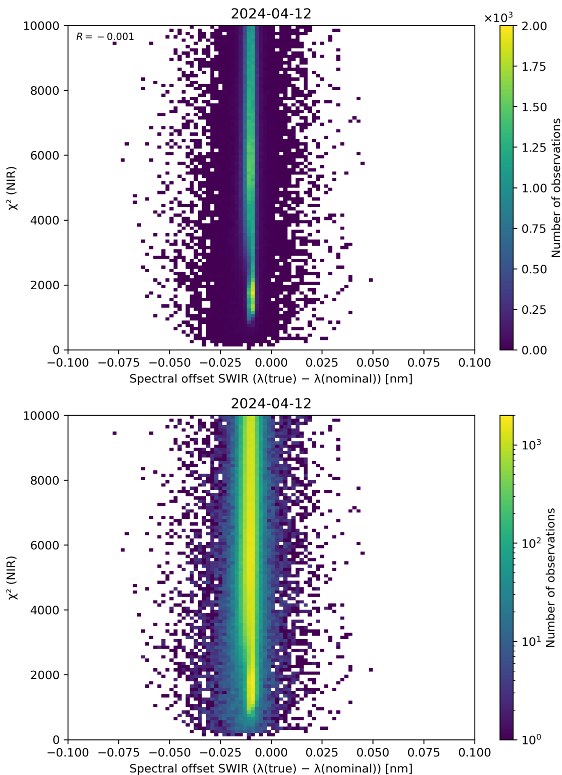
Figure 117: Scatter density plot of “Spectral offset SWIR ( \lambda(\text{true}) - \lambda(\text{nominal}) )” against “ \chi^2 (NIR)” for 2024-04-11 to 2024-04-13.
