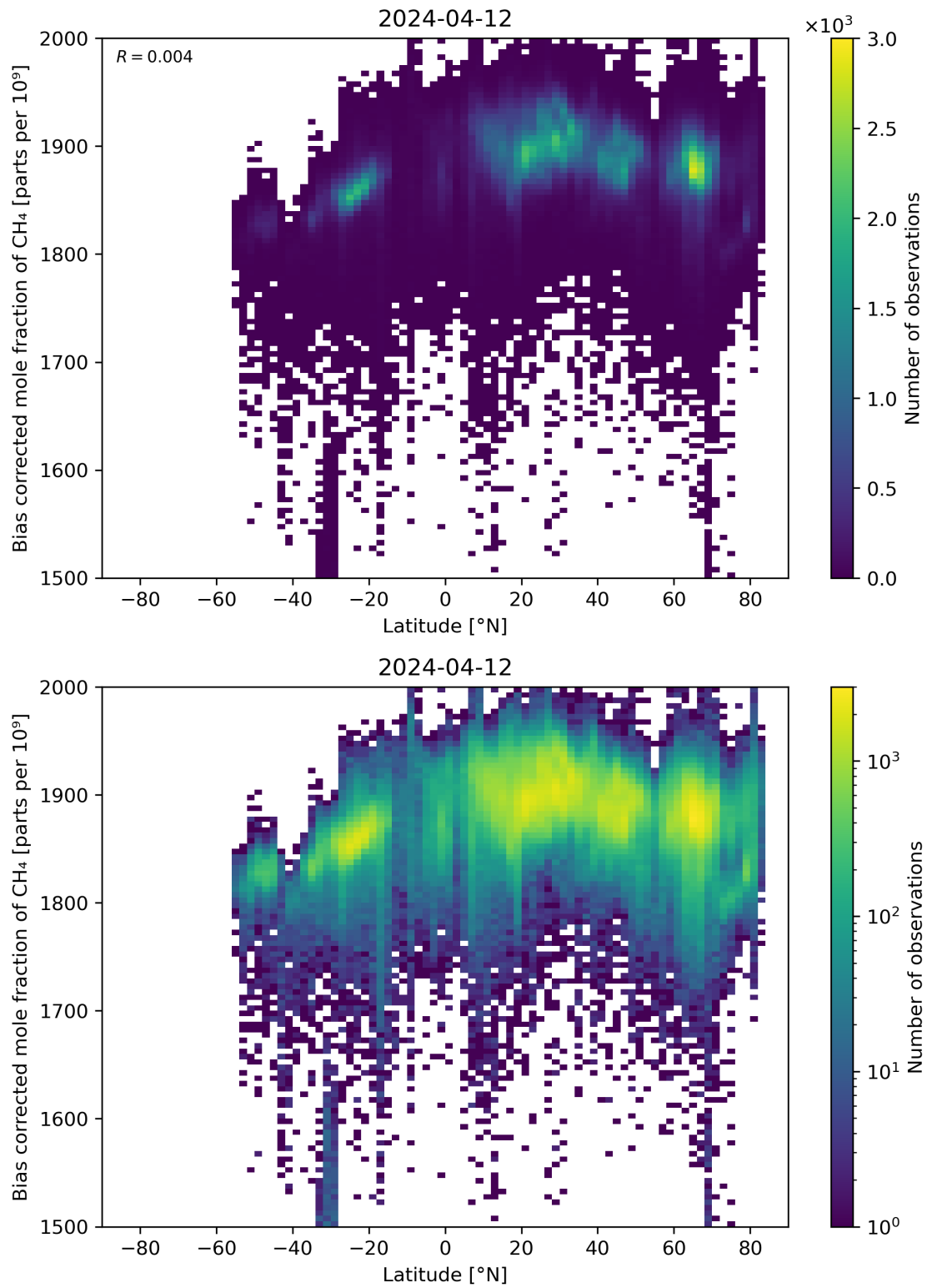
Figure 58: Scatter density plot of “Latitude” against “Bias corrected mole fraction of CH 4 ” for 2024-04-11 to 2024-04-13.
