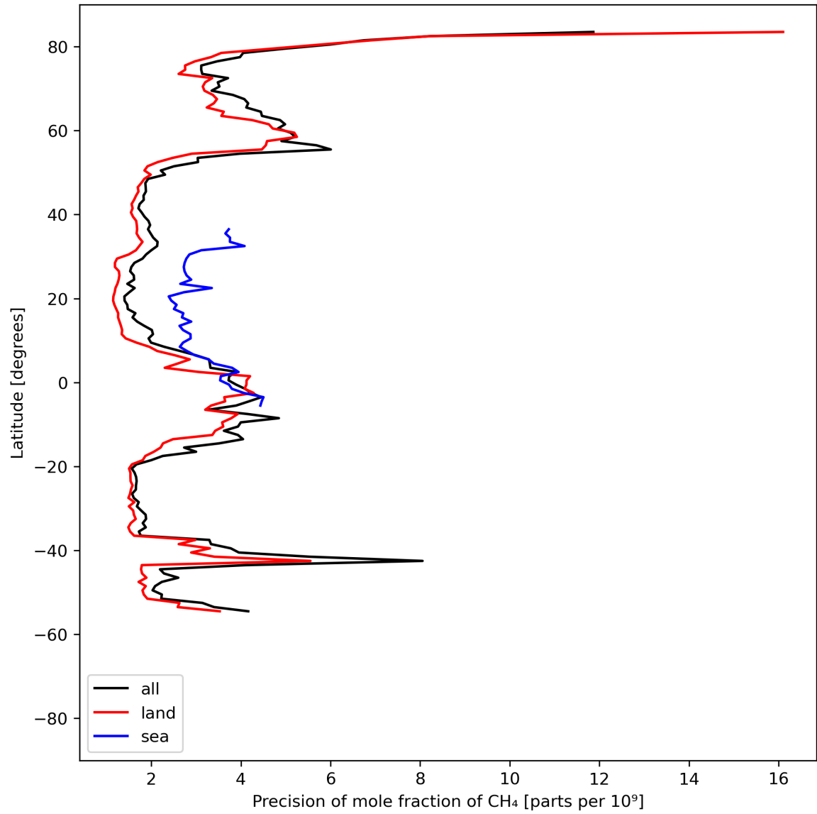
Figure 13: Zonal average of “Precision of mole fraction of CH 4 ” for 2024-04-11 to 2024-04-13.
