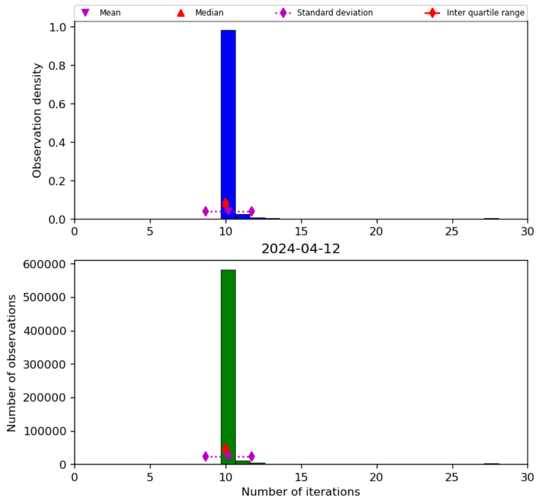
Figure 31: Histogram of “Number of iterations” for 2024-04-11 to 2024-04-13
