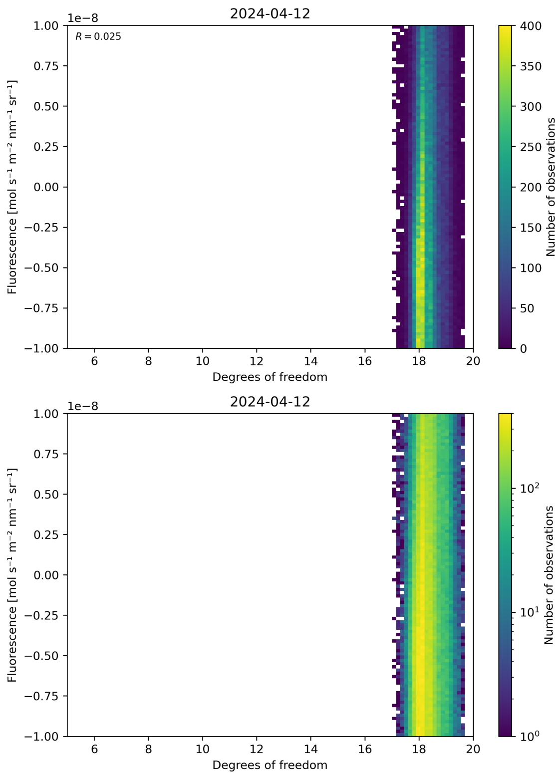
Figure 51: Scatter density plot of “Degrees of freedom” against “Fluorescence” for 2024-04-11 to 2024-04-13.
