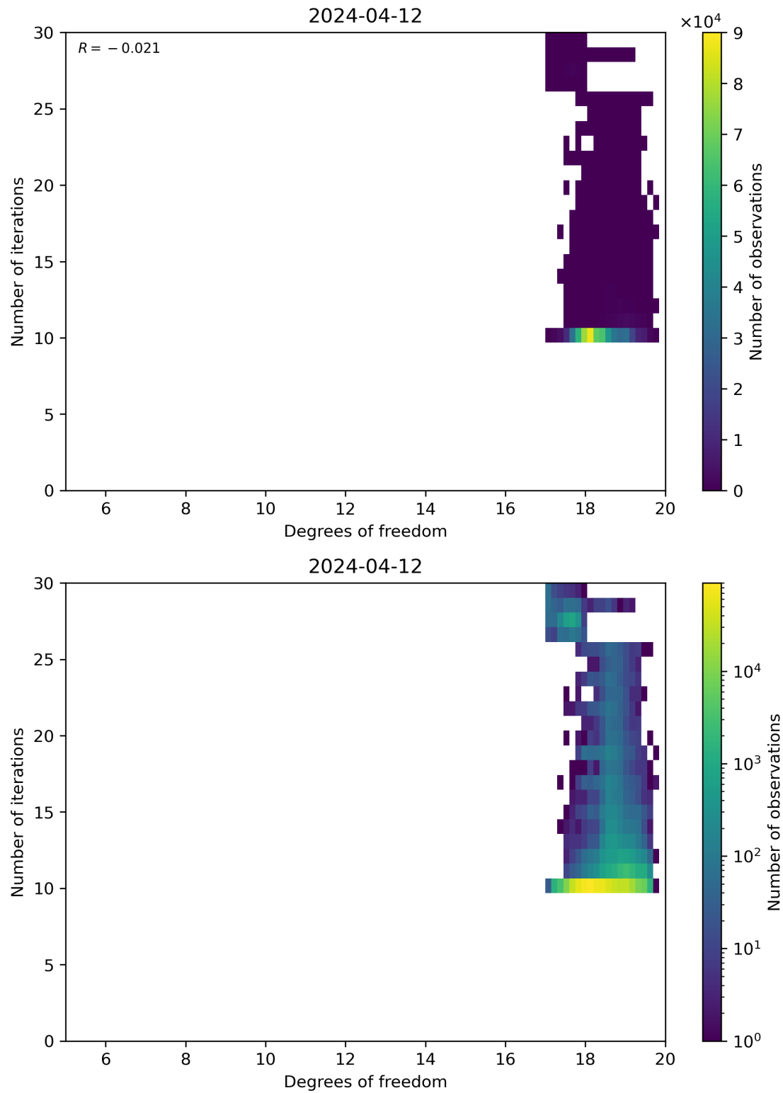
Figure 52: Scatter density plot of “Degrees of freedom” against “Number of iterations” for 2024-04-11 to 2024-04-13.
