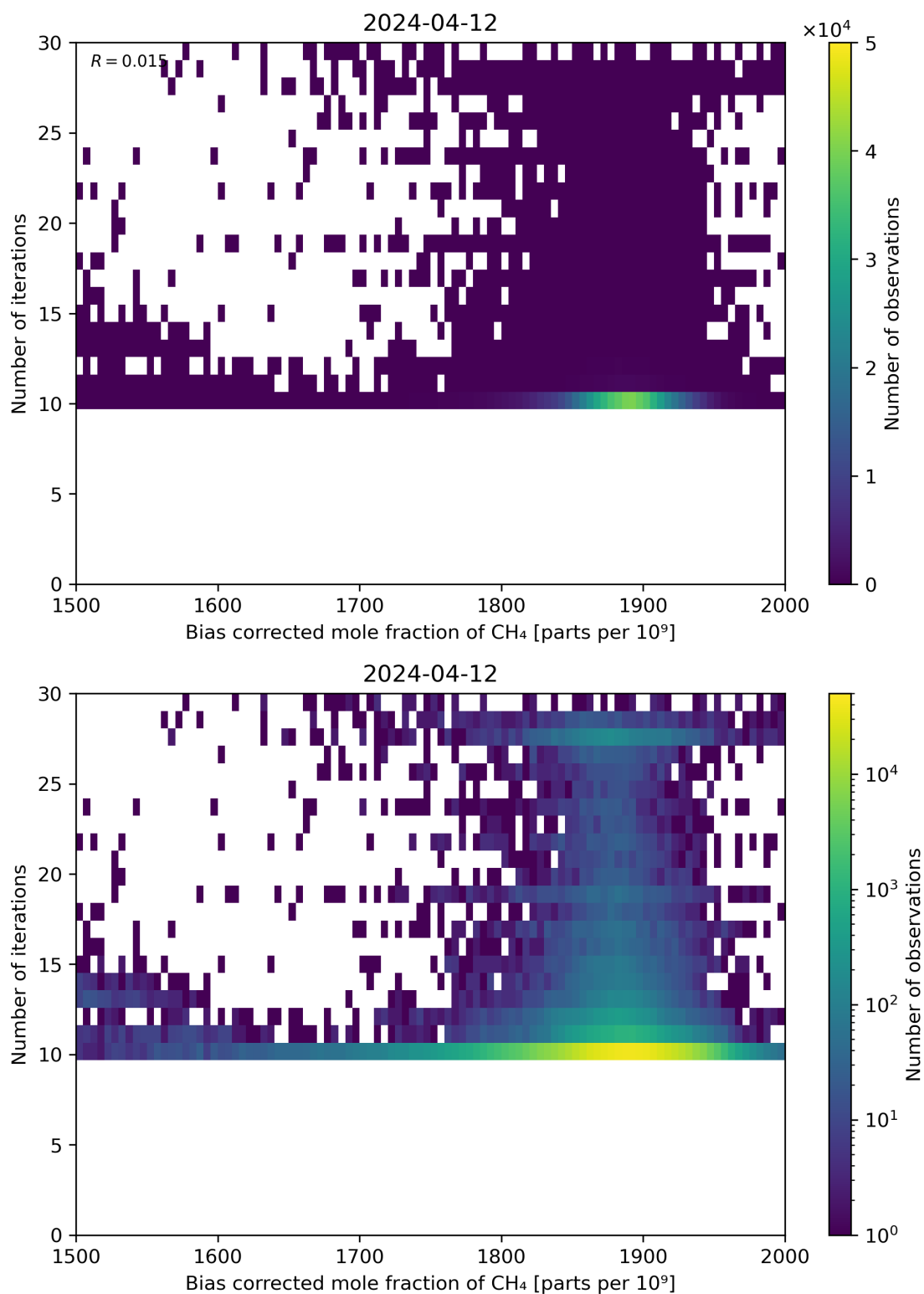
Figure 67: Scatter density plot of “Bias corrected mole fraction of \text{CH}_4 ” against “Number of iterations” for 2024-04-11 to 2024-04-13.
