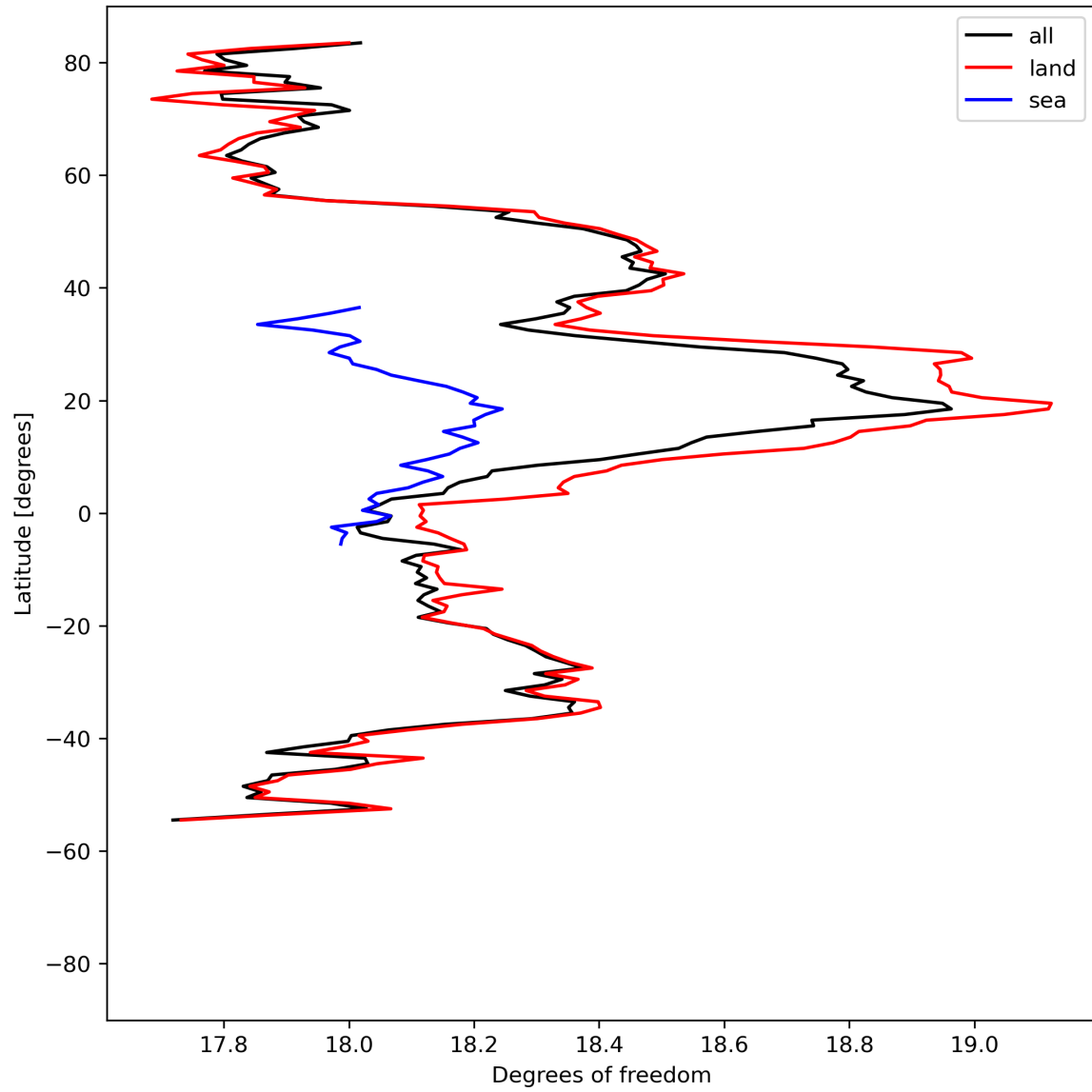
Figure 19: Zonal average of “Degrees of freedom” for 2024-04-11 to 2024-04-13.
