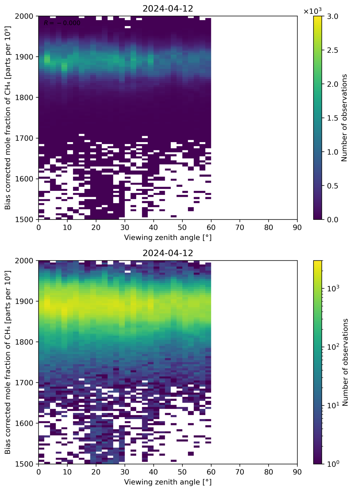
Figure 111: Scatter density plot of “Viewing zenith angle” against “Bias corrected mole fraction of CH 4 ” for 2024-04-11 to 2024-04-13.
