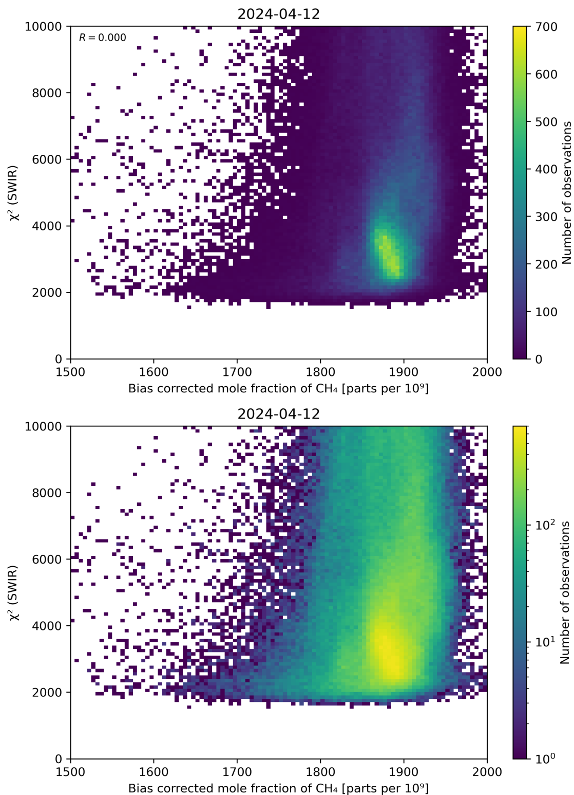
Figure 64: Scatter density plot of “Bias corrected mole fraction of CH 4 ” against “ \chi^2 (SWIR)” for 2024-04-11 to 2024-04-13.
