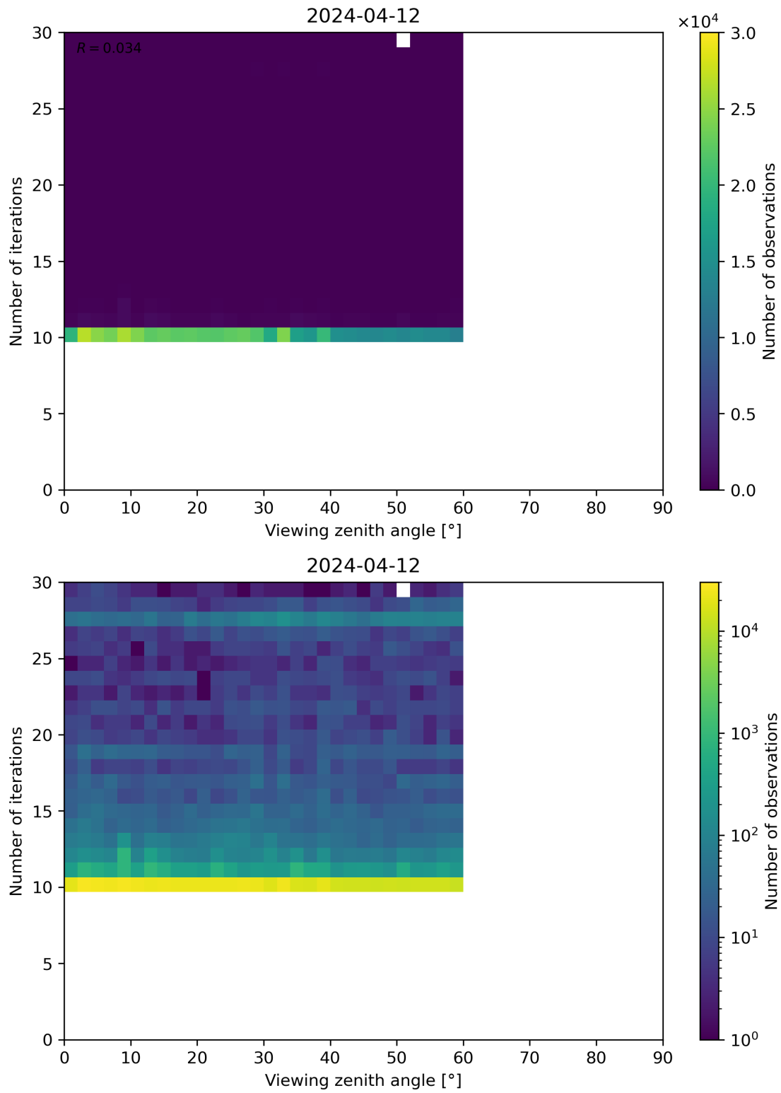
Figure 113: Scatter density plot of “Viewing zenith angle” against “Number of iterations” for 2024-04-11 to 2024-04-13.
