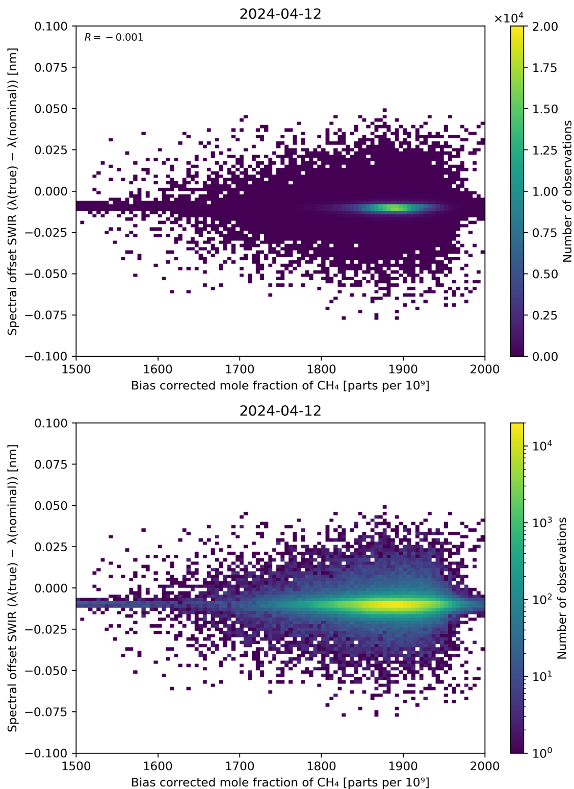
Figure 69: Scatter density plot of “Bias corrected mole fraction of \text{CH}_4 ” against “Spectral offset SWIR ( \lambda(\text{true}) - \lambda(\text{nominal}) )” for 2024-04-11 to 2024-04-13.
