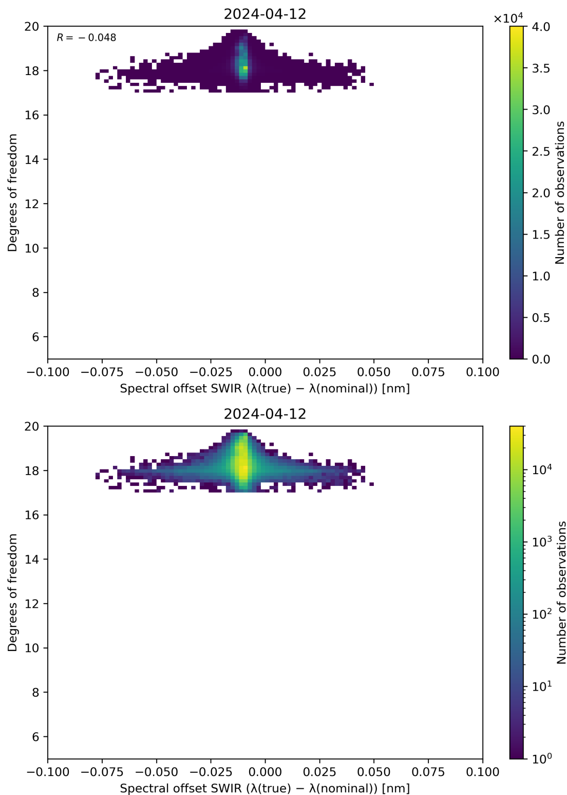
Figure 119: Scatter density plot of “Spectral offset SWIR ( \lambda(\text{true}) - \lambda(\text{nominal}) )” against “Degrees of freedom” for 2024-04-11 to 2024-04-13.
