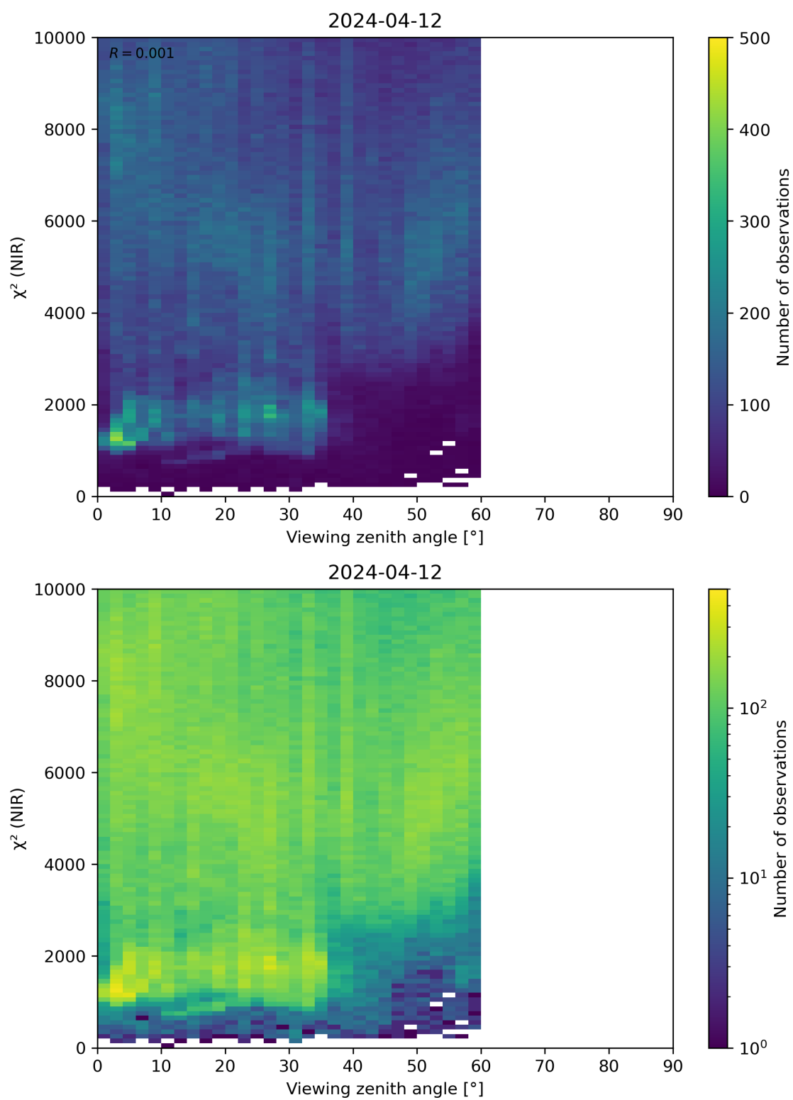
Figure 105: Scatter density plot of “Viewing zenith angle” against “ \chi^2 (NIR)” for 2024-04-11 to 2024-04-13.
