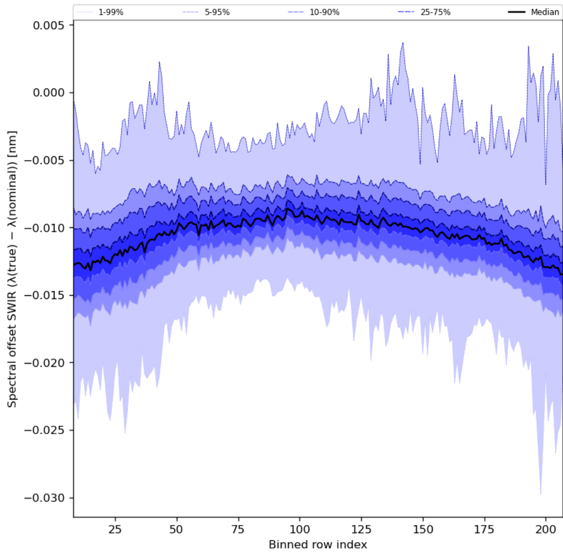
Figure 38: Along track statistics of “Spectral offset SWIR ( \lambda(\text{true}) - \lambda(\text{nominal}) )” for 2024-04-11 to 2024-04-13
