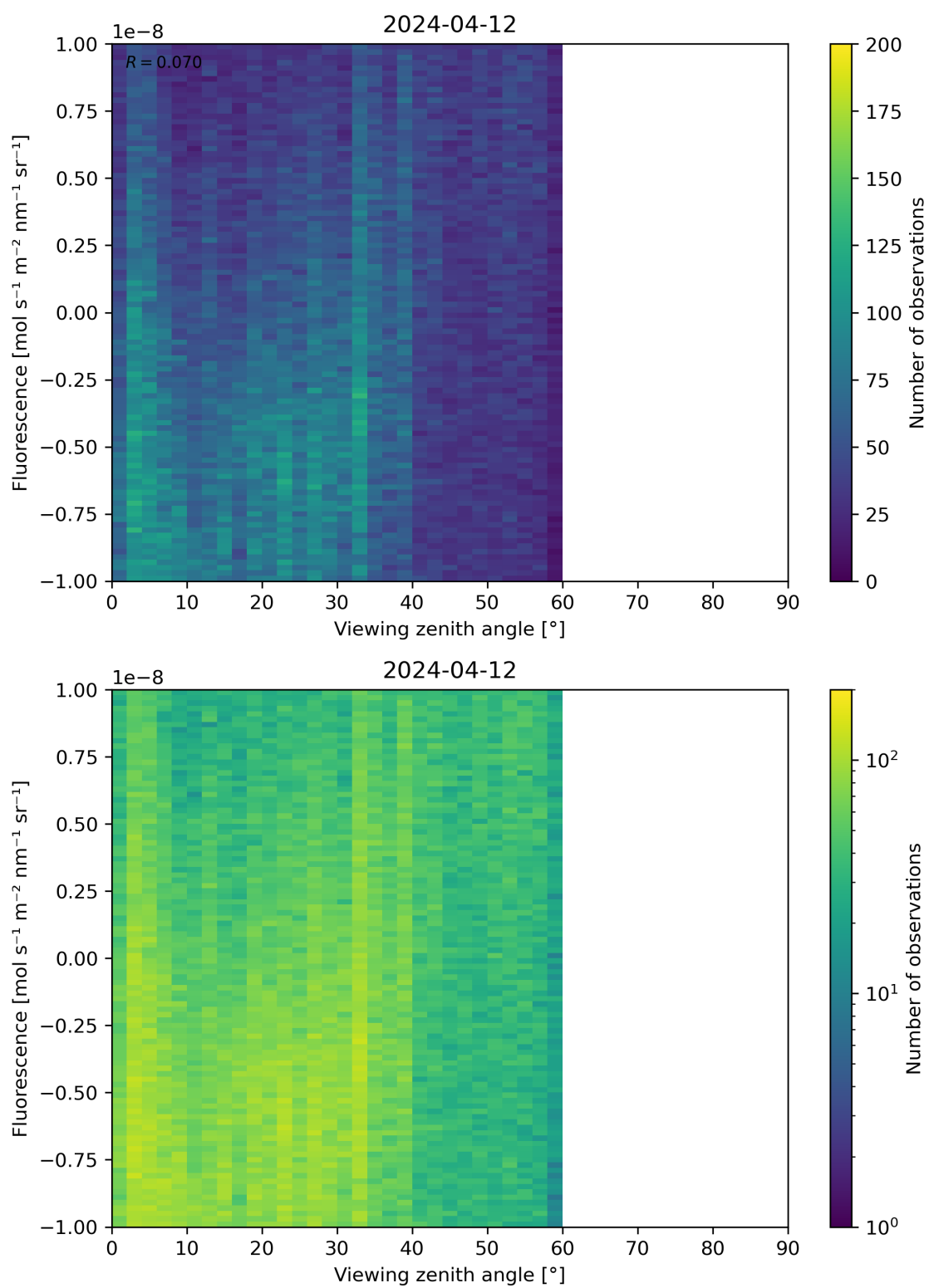
Figure 108: Scatter density plot of “Viewing zenith angle” against “Fluorescence” for 2024-04-11 to 2024-04-13.
