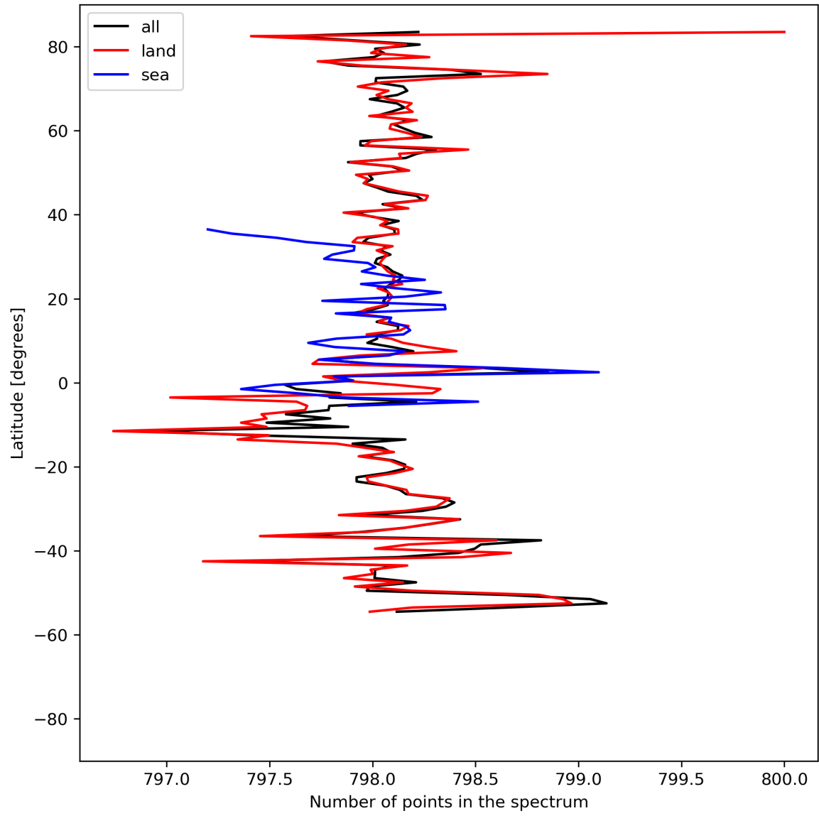
Figure 15: Zonal average of “Number of points in the spectrum” for 2024-04-11 to 2024-04-13.
