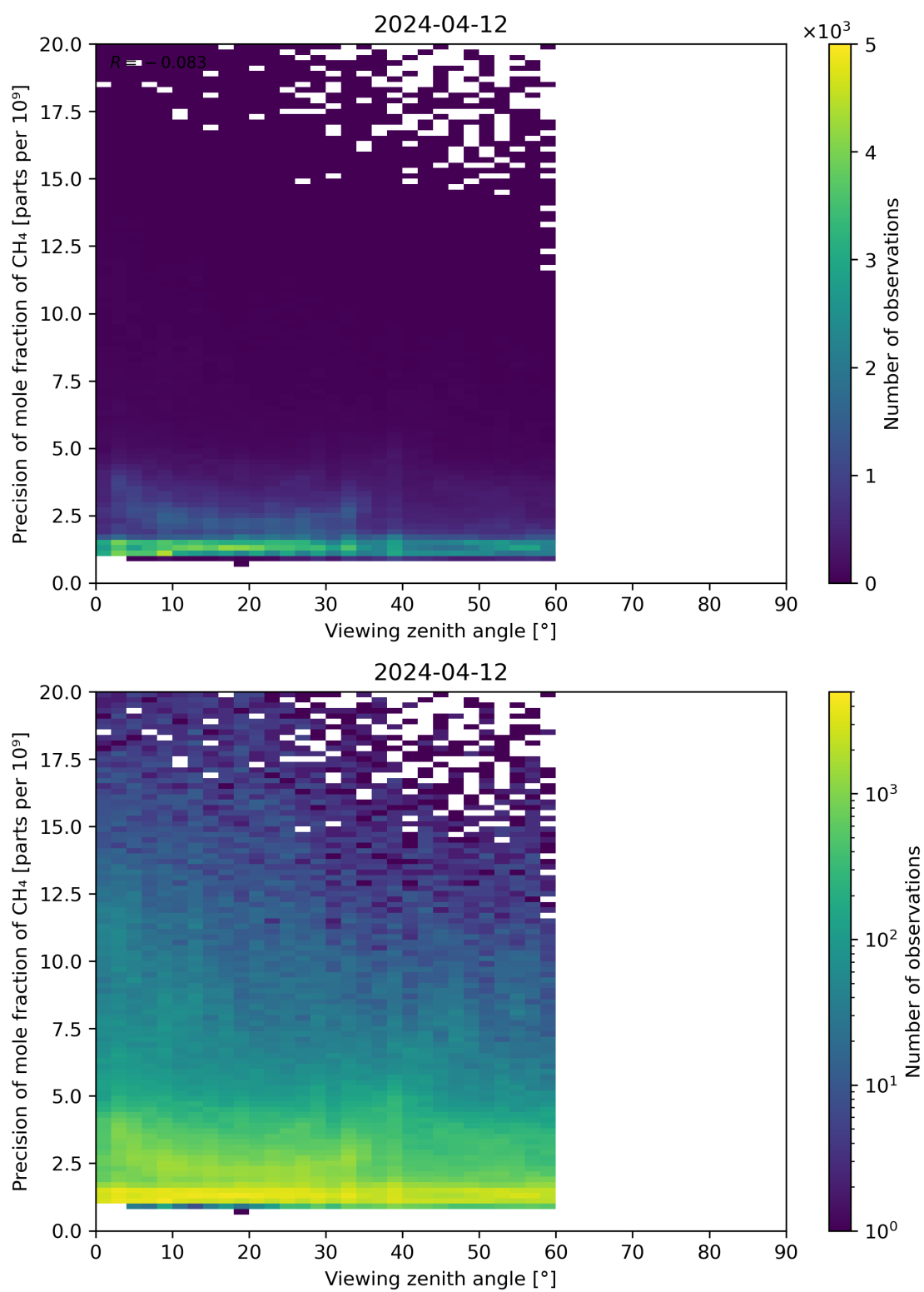
Figure 112: Scatter density plot of “Viewing zenith angle” against “Precision of mole fraction of CH 4 ” for 2024-04-11 to 2024-04-13.
