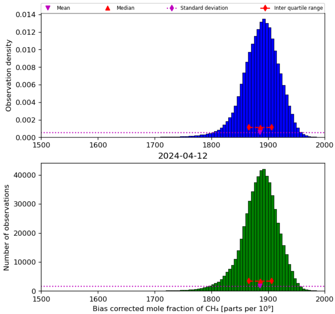
Figure 25: Histogram of “Bias corrected mole fraction of CH 4 ” for 2024-04-11 to 2024-04-13
