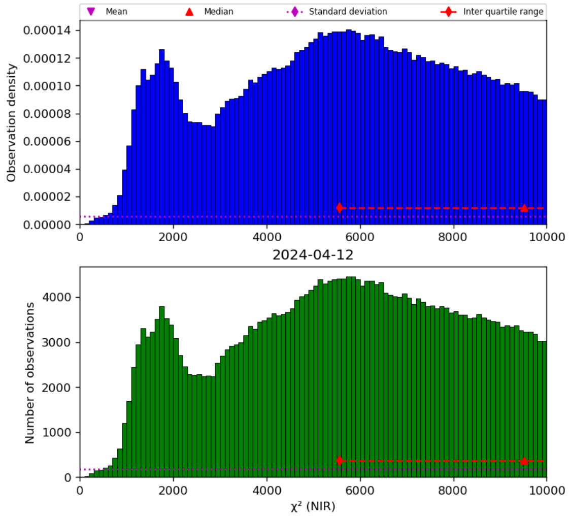
Figure 29: Histogram of “ \chi^2 (NIR)” for 2024-04-11 to 2024-04-13
