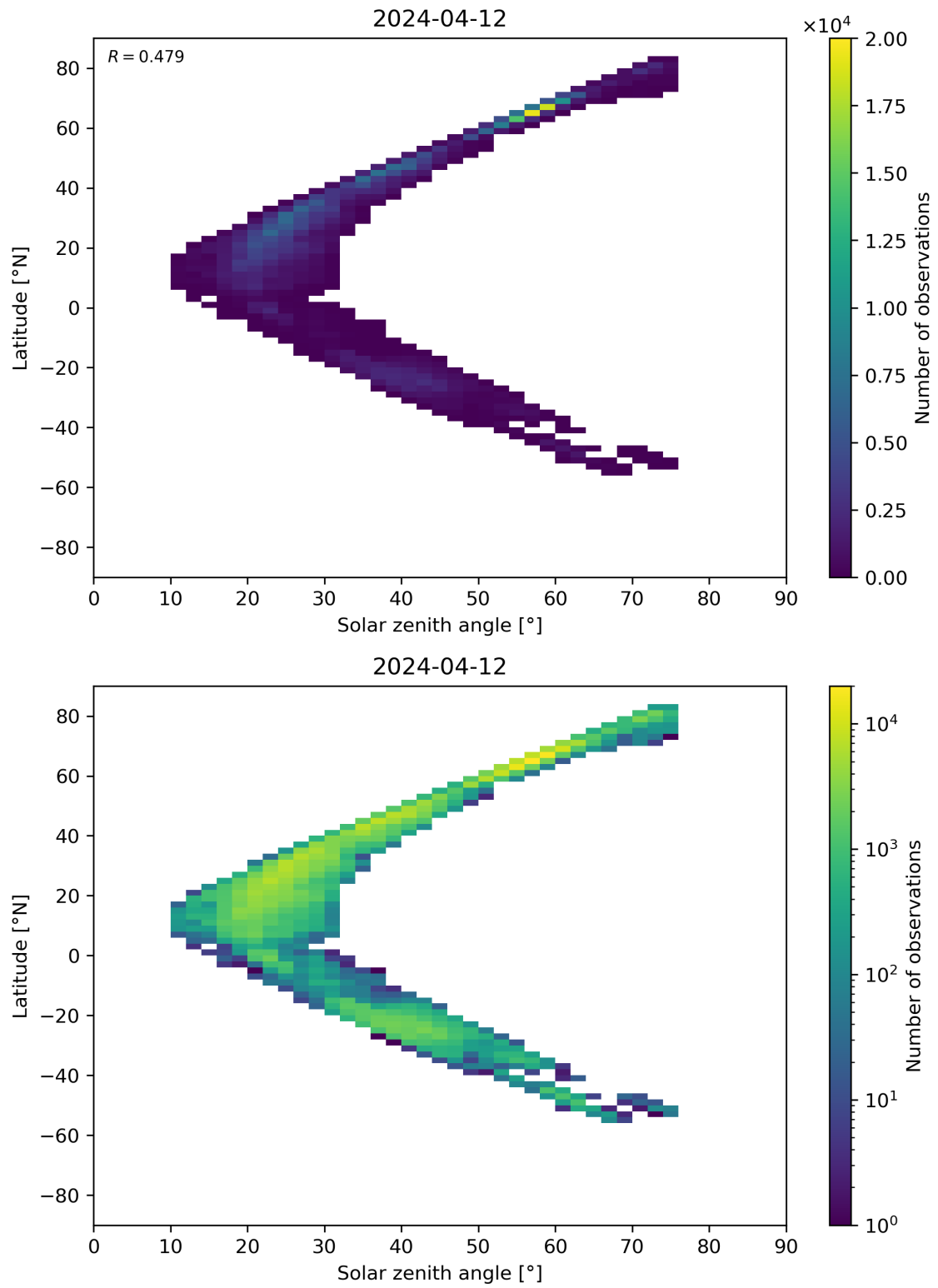
Figure 98: Scatter density plot of “Solar zenith angle” against “Latitude” for 2024-04-11 to 2024-04-13.
