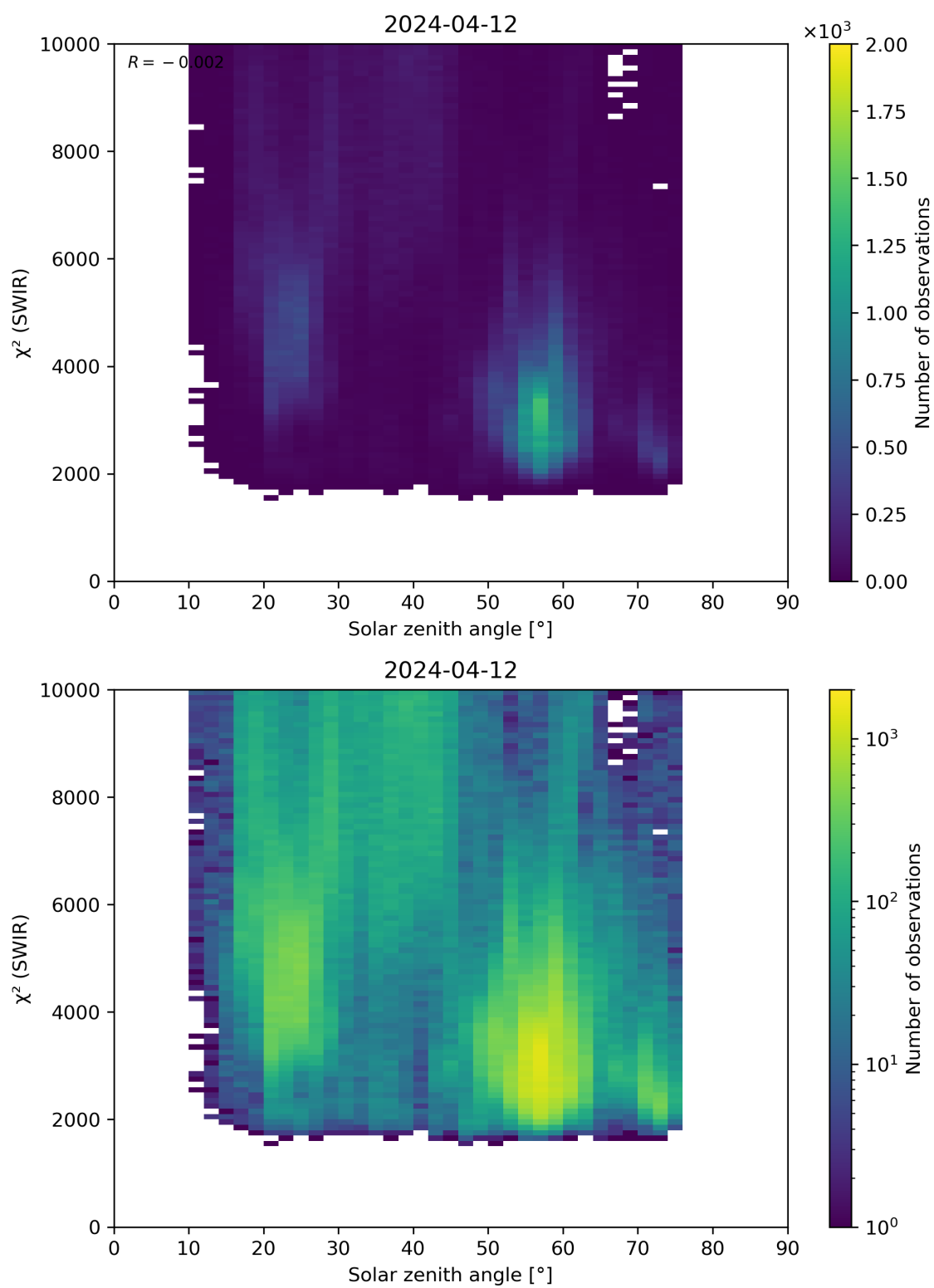
Figure 95: Scatter density plot of “Solar zenith angle” against “ \chi^2 (SWIR)” for 2024-04-11 to 2024-04-13.
