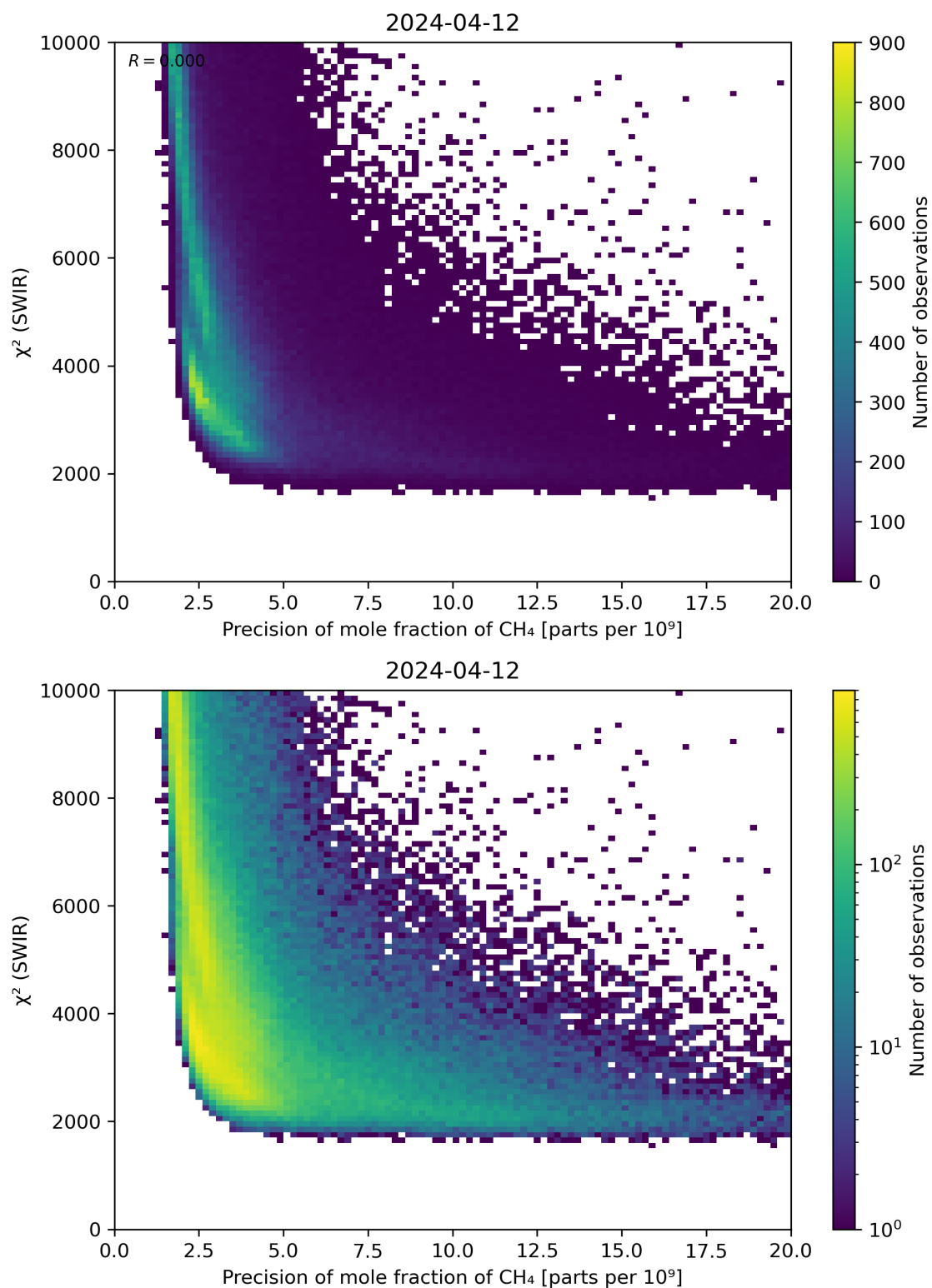
Figure 79: Scatter density plot of “Precision of mole fraction of \text{CH}_4 ” against “ \chi^2 (SWIR)” for 2024-04-11 to 2024-04-13.
