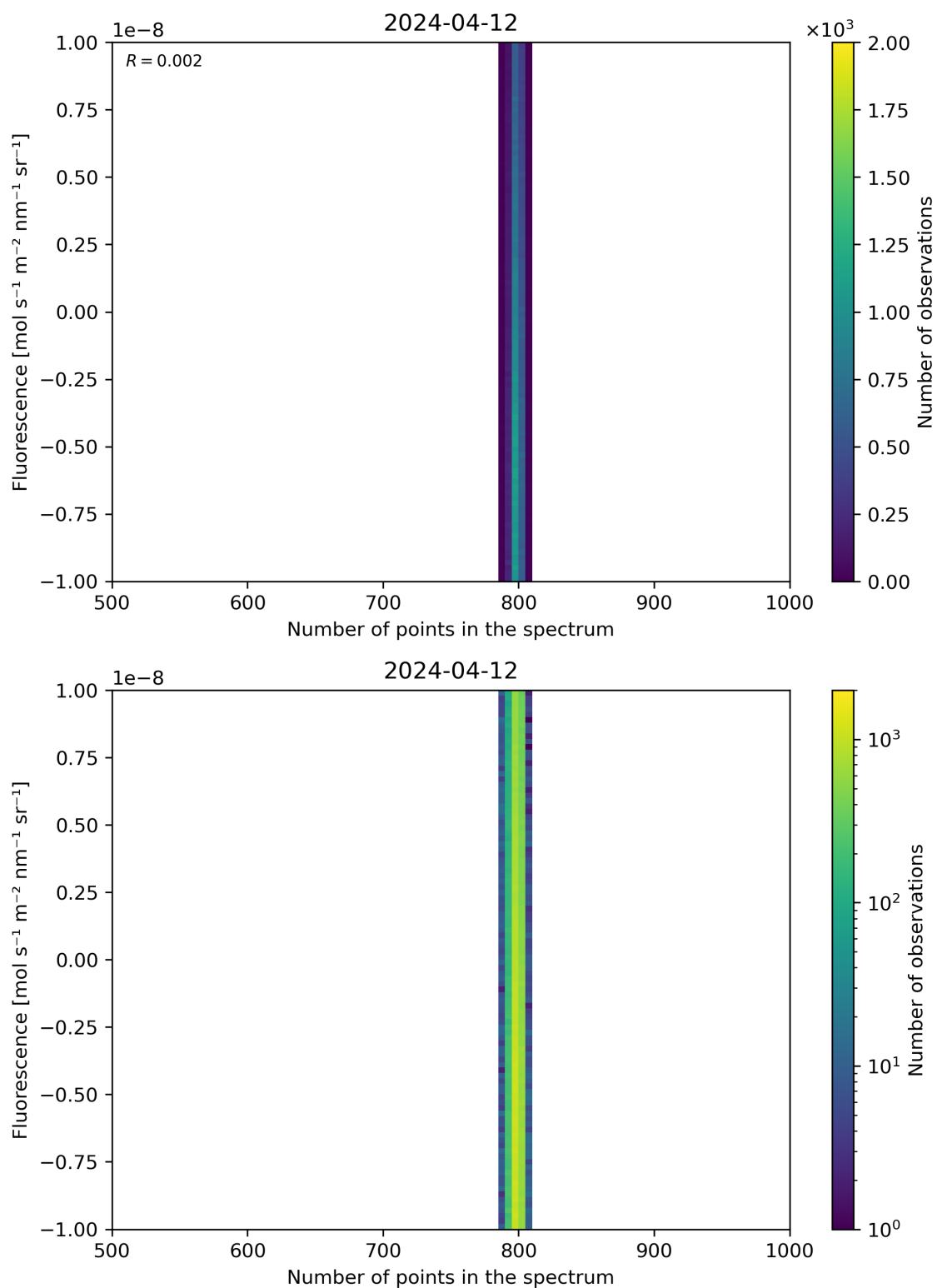
Figure 91: Scatter density plot of “Number of points in the spectrum” against “Fluorescence” for 2024-04-11 to 2024-04-13.
