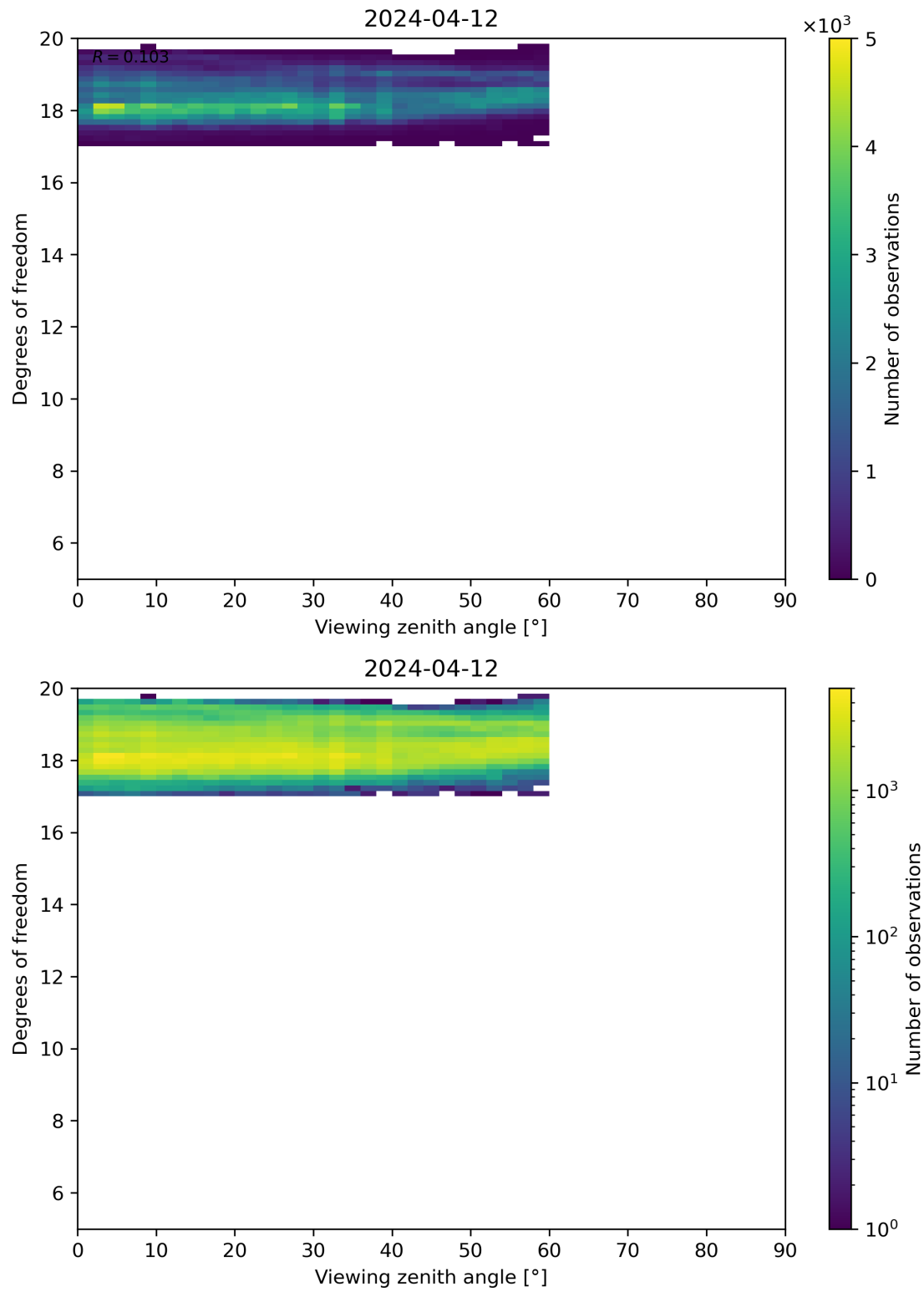
Figure 107: Scatter density plot of “Viewing zenith angle” against “Degrees of freedom” for 2024-04-11 to 2024-04-13.
