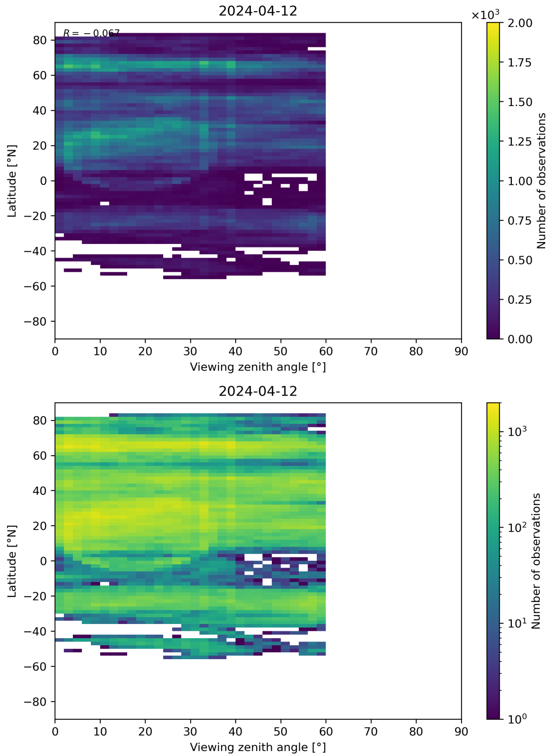
Figure 109: Scatter density plot of “Viewing zenith angle” against “Latitude” for 2024-04-11 to 2024-04-13.
