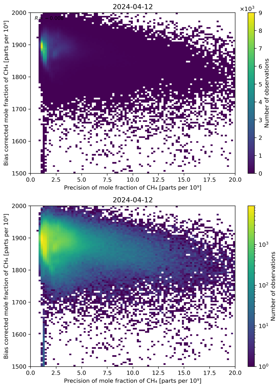
Figure 82: Scatter density plot of “Precision of mole fraction of CH 4 ” against “Bias corrected mole fraction of CH 4 ” for 2024-04-11 to 2024-04-13.
