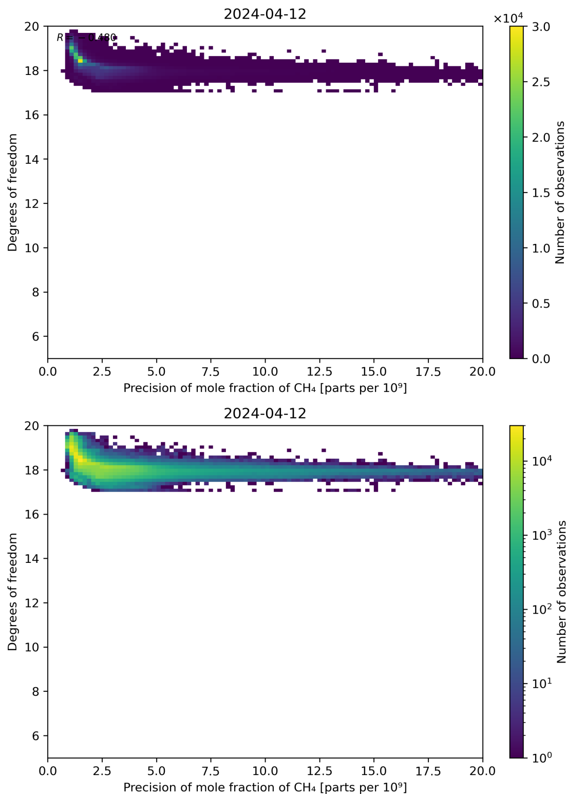
Figure 80: Scatter density plot of “Precision of mole fraction of CH 4 ” against “Degrees of freedom” for 2024-04-11 to 2024-04-13.
