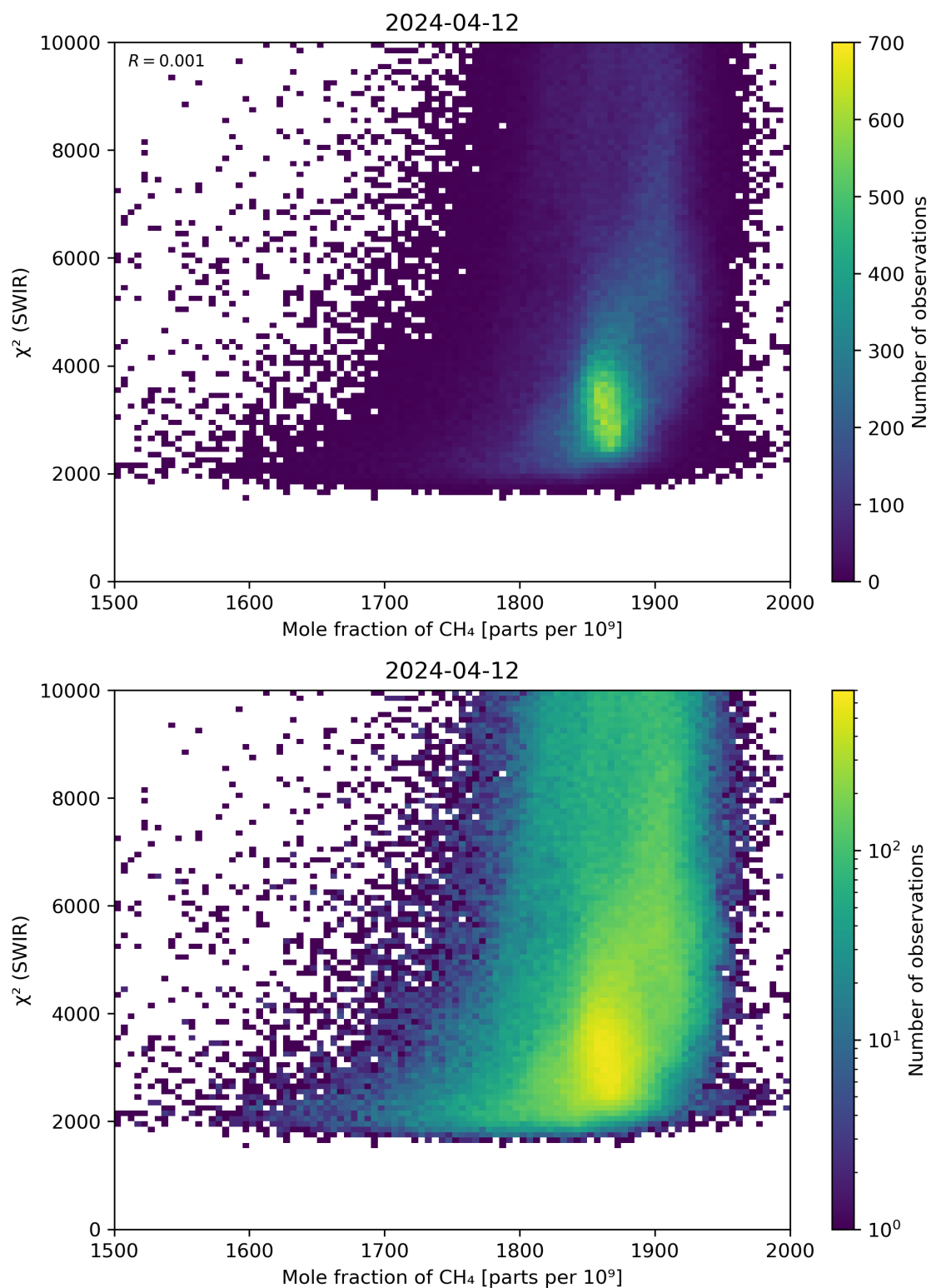
Figure 71: Scatter density plot of “Mole fraction of \text{CH}_4 ” against “ \chi^2 (SWIR)” for 2024-04-11 to 2024-04-13.
