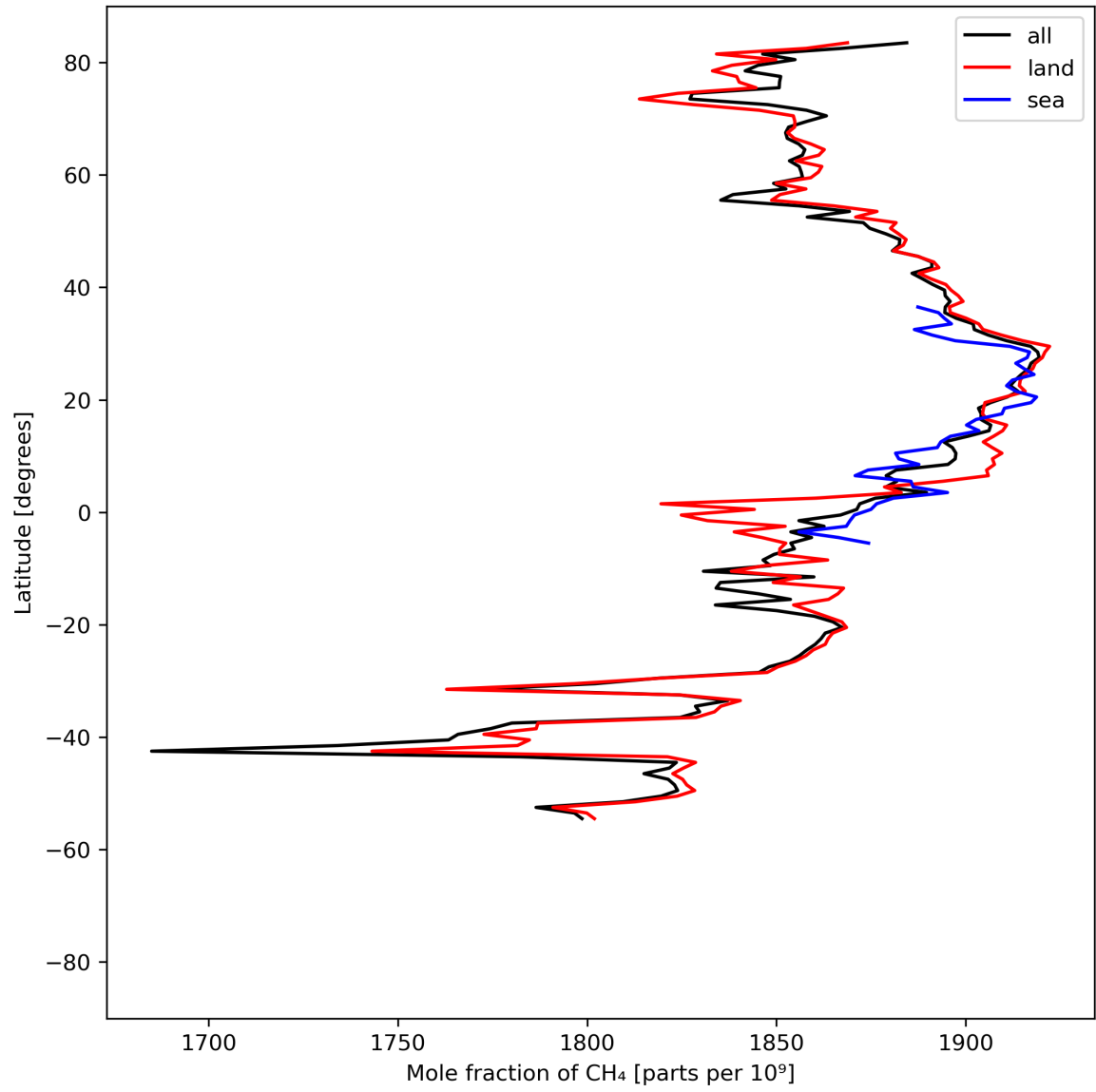
Figure 12: Zonal average of “Mole fraction of \text{CH}_4 ” for 2024-04-11 to 2024-04-13.
