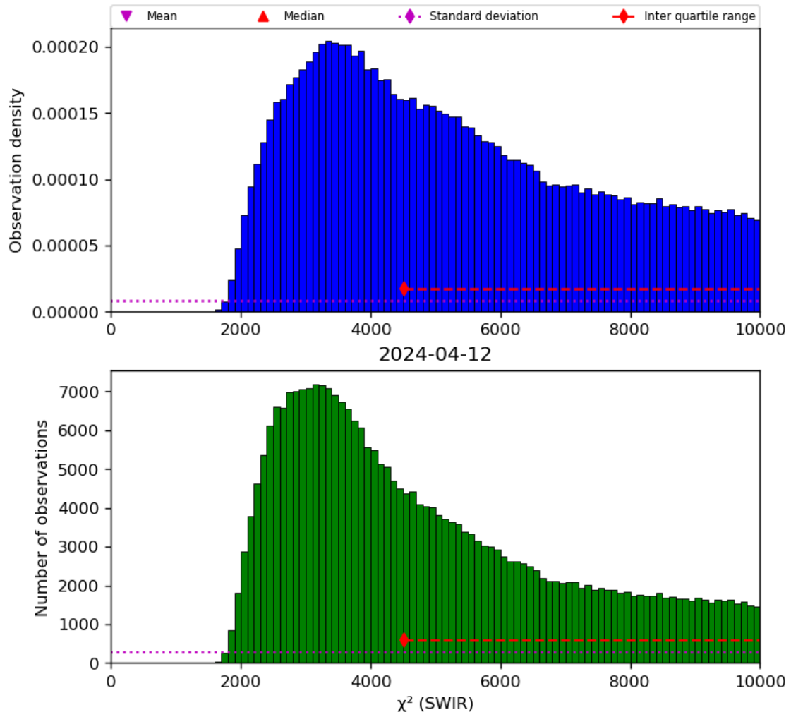
Figure 28: Histogram of “ \chi^2 (SWIR)” for 2024-04-11 to 2024-04-13
