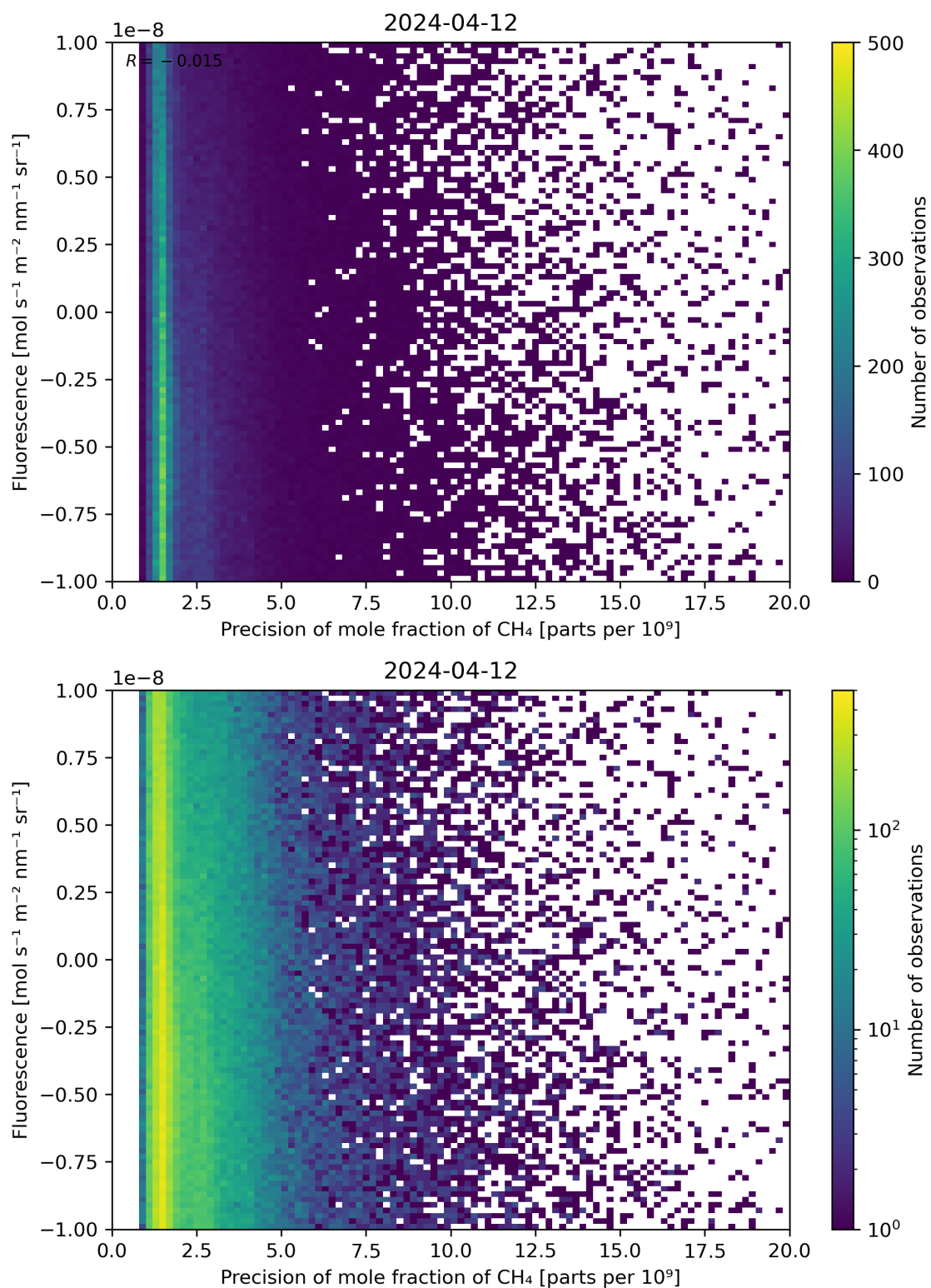
Figure 81: Scatter density plot of “Precision of mole fraction of \text{CH}_4 ” against “Fluorescence” for 2024-04-11 to 2024-04-13.
