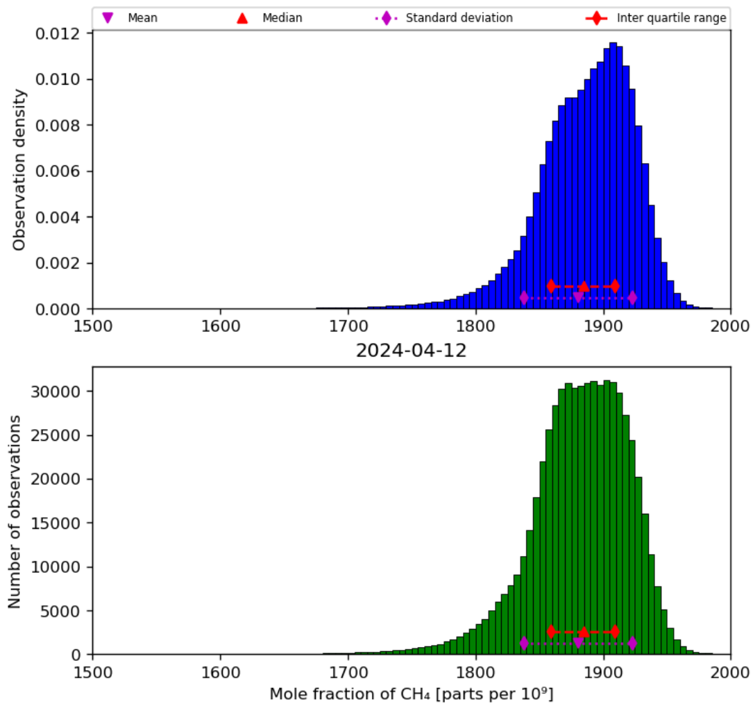
Figure 23: Histogram of “Mole fraction of CH 4 ” for 2024-04-11 to 2024-04-13
