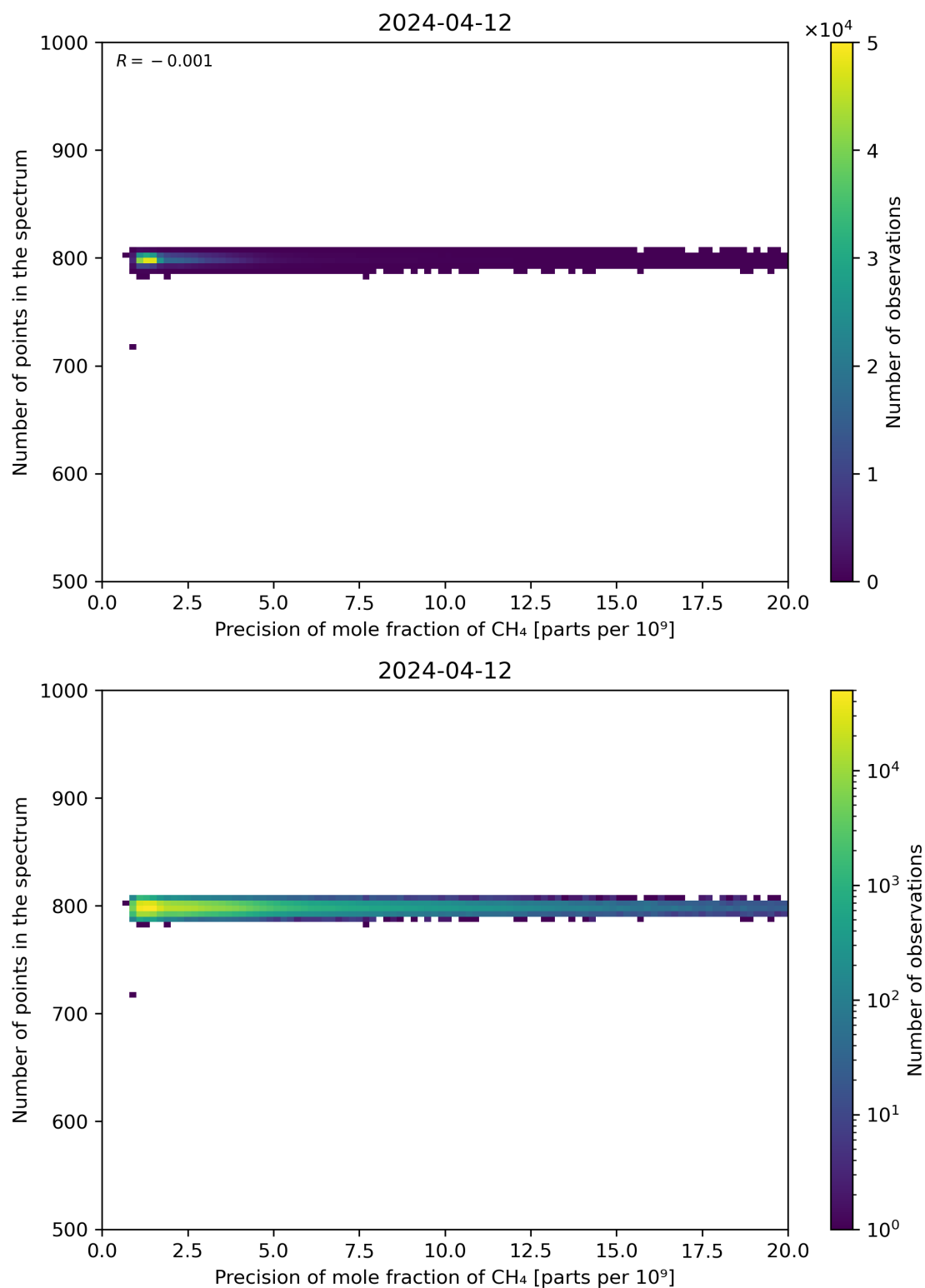
Figure 84: Scatter density plot of “Precision of mole fraction of CH 4 ” against “Number of points in the spectrum” for 2024-04-11 to 2024-04-13.
