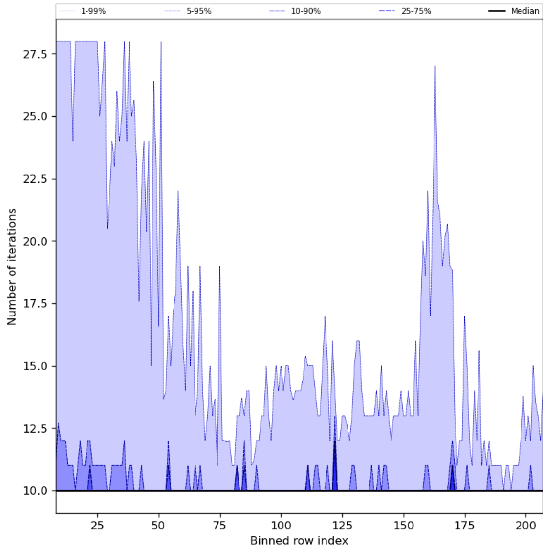
Figure 42: Along track statistics of “Number of iterations” for 2024-04-11 to 2024-04-13
