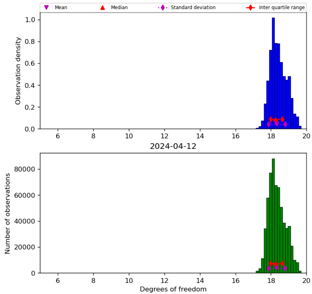
Figure 30: Histogram of “Degrees of freedom” for 2024-04-11 to 2024-04-13
