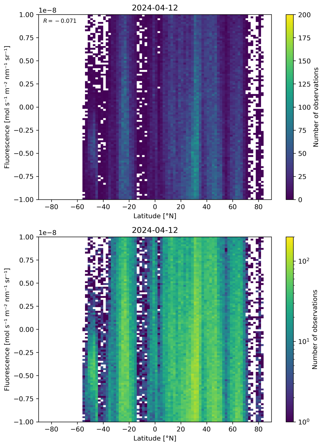
Figure 56: Scatter density plot of “Latitude” against “Fluorescence” for 2024-04-11 to 2024-04-13.
