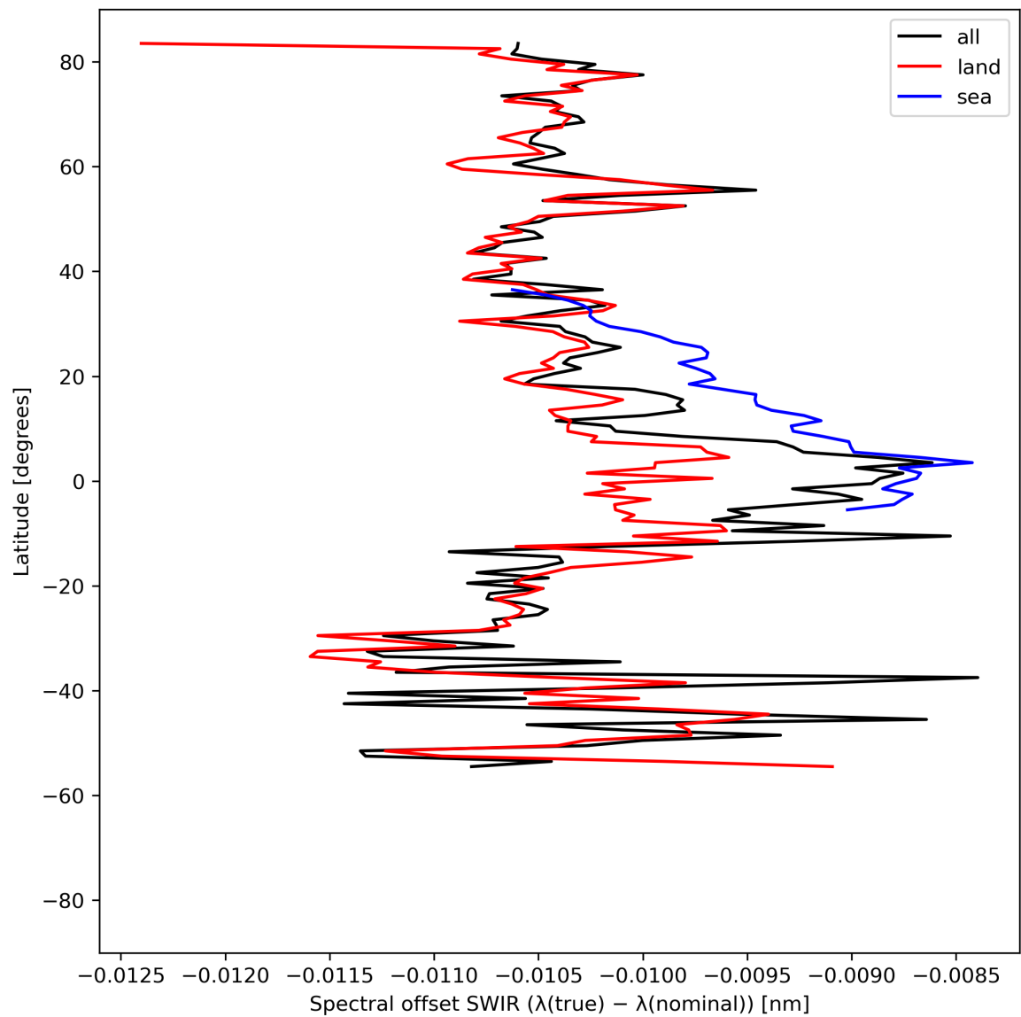
Figure 16: Zonal average of “Spectral offset SWIR ( \lambda(\text{true}) - \lambda(\text{nominal}) )” for 2024-04-11 to 2024-04-13.
