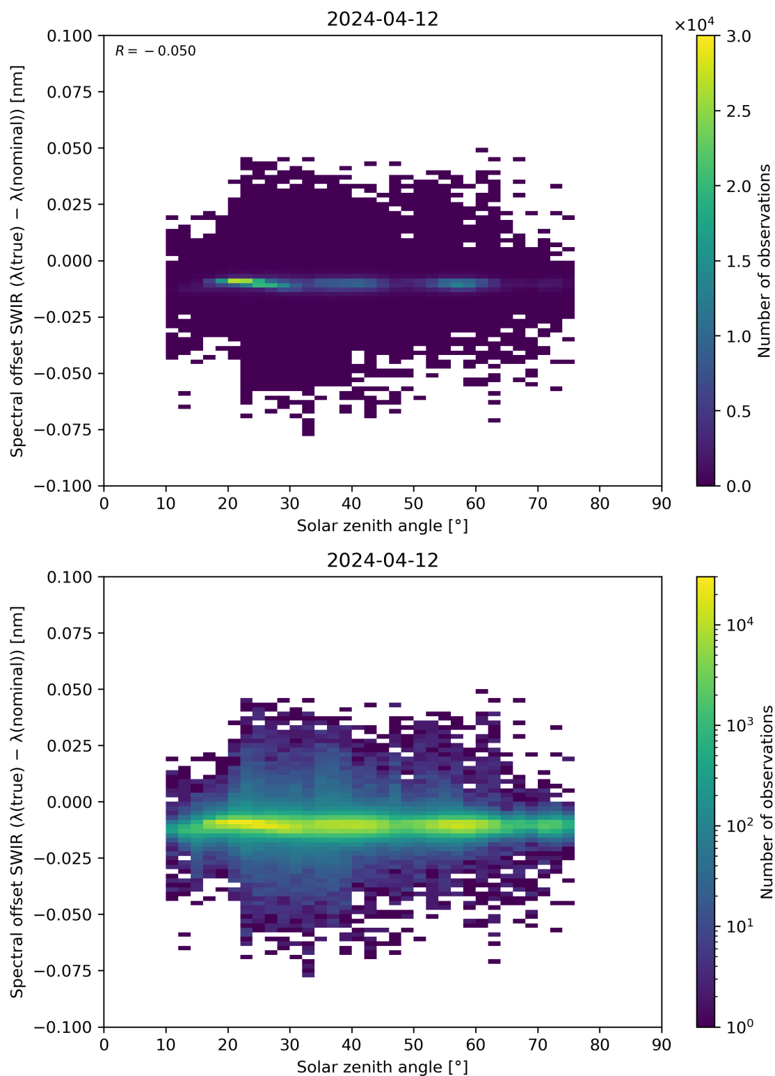
Figure 104: Scatter density plot of “Solar zenith angle” against “Spectral offset SWIR ( \lambda(\text{true}) - \lambda(\text{nominal}) )” for 2024-04-11 to 2024-04-13.
