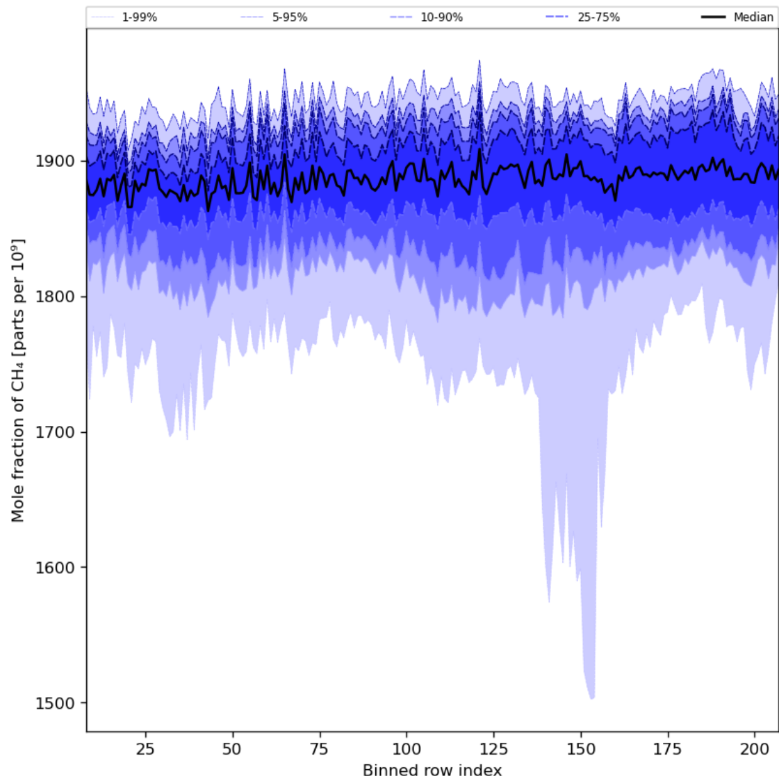
Figure 34: Along track statistics of “Mole fraction of CH 4 ” for 2024-04-11 to 2024-04-13
