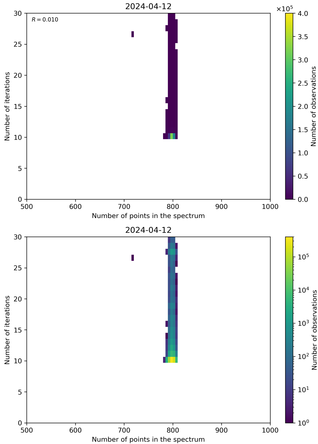
Figure 92: Scatter density plot of “Number of points in the spectrum” against “Number of iterations” for 2024-04-11 to 2024-04-13.
