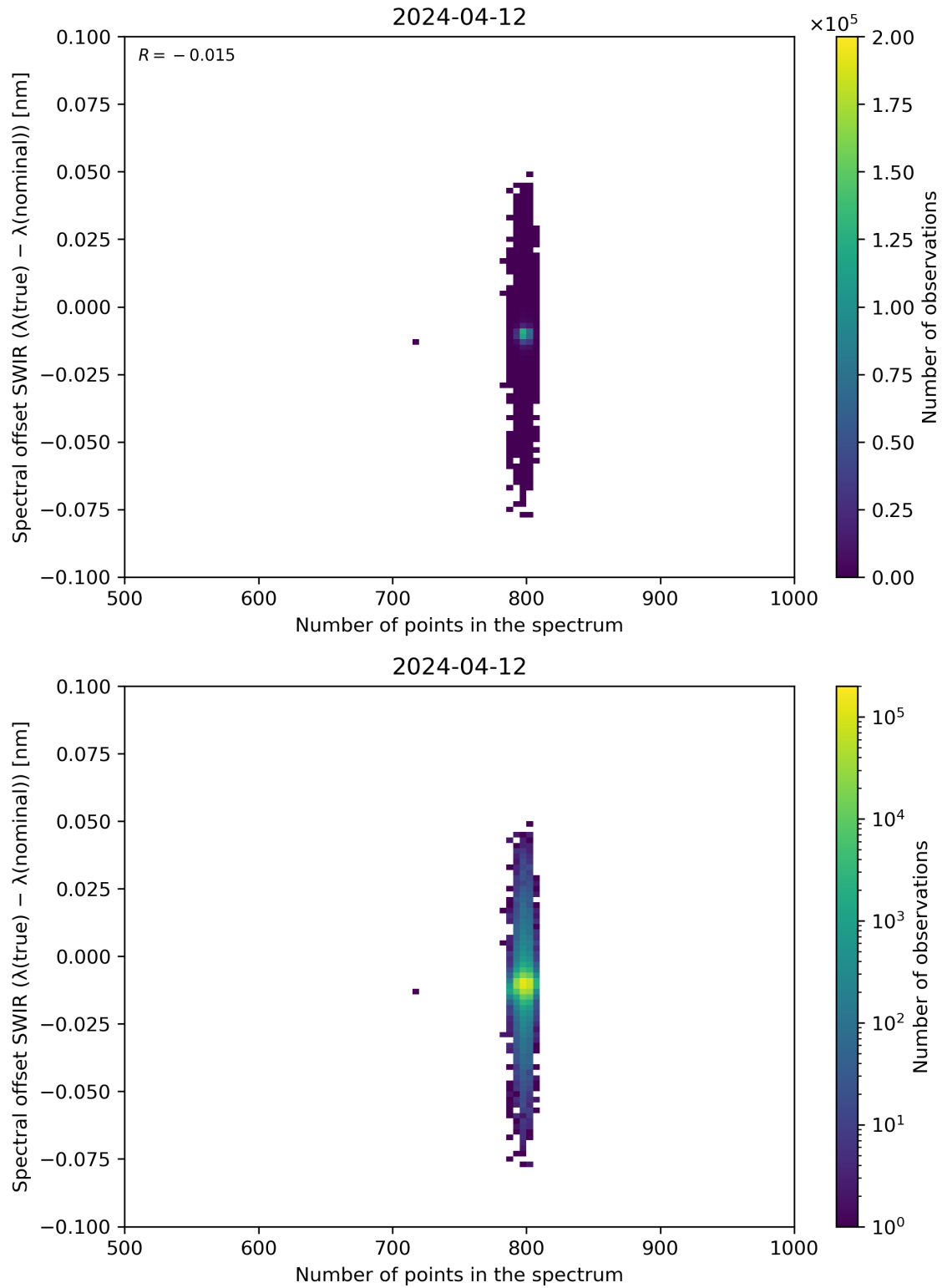
Figure 93: Scatter density plot of “Number of points in the spectrum” against “Spectral offset SWIR ( \lambda(\text{true}) - \lambda(\text{nominal}) )” for 2024-04-11 to 2024-04-13.
