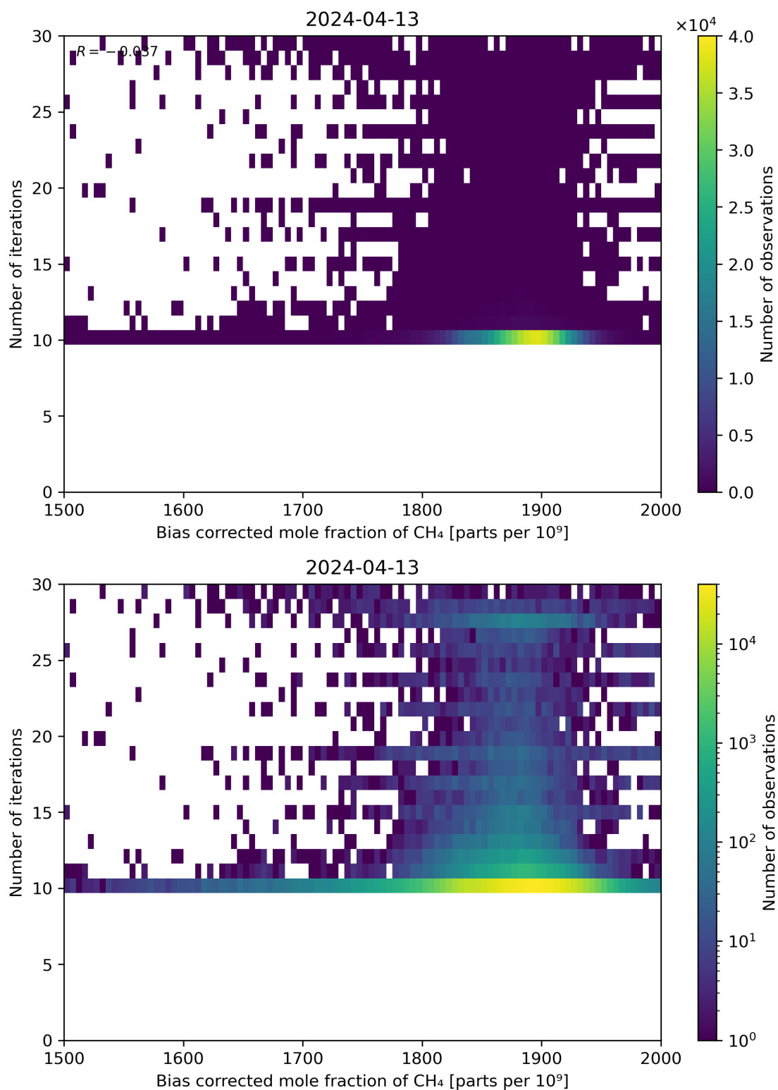
Figure 67: Scatter density plot of “Bias corrected mole fraction of \text{CH}_4 ” against “Number of iterations” for 2024-04-12 to 2024-04-14.
