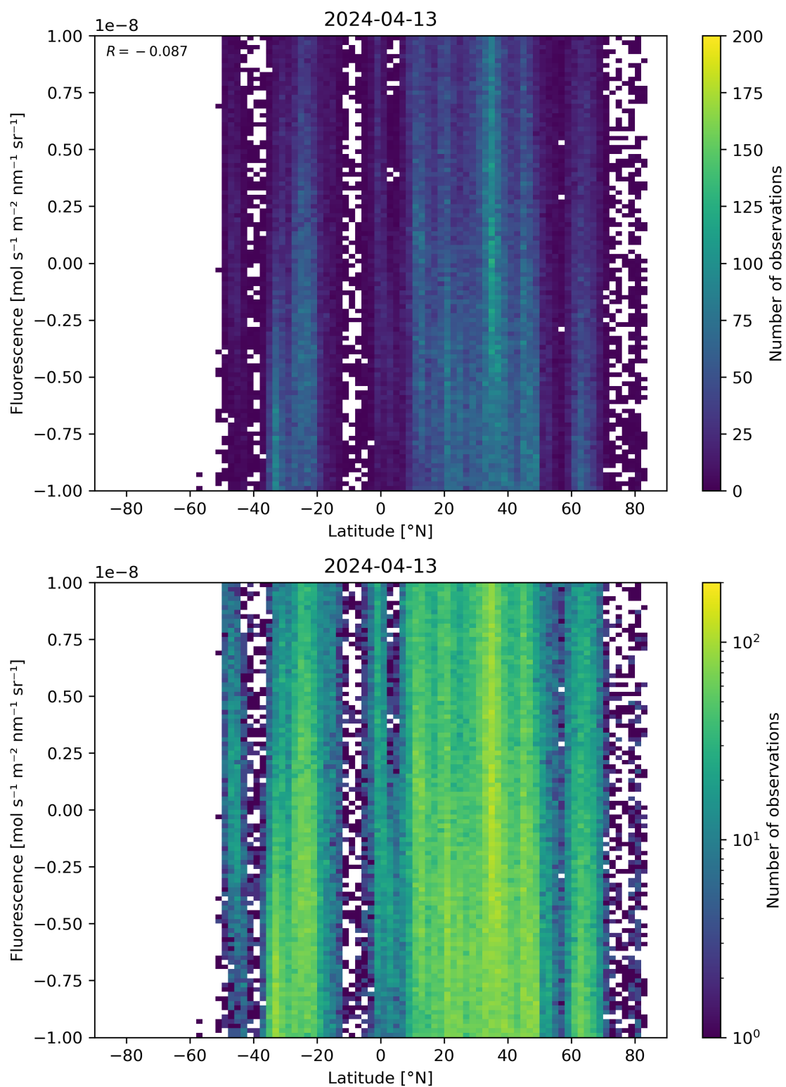
Figure 56: Scatter density plot of “Latitude” against “Fluorescence” for 2024-04-12 to 2024-04-14.
