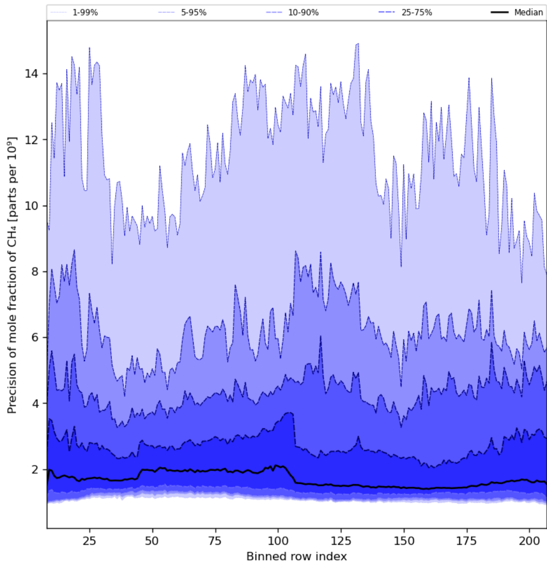
Figure 35: Along track statistics of “Precision of mole fraction of CH 4 ” for 2024-04-12 to 2024-04-14
