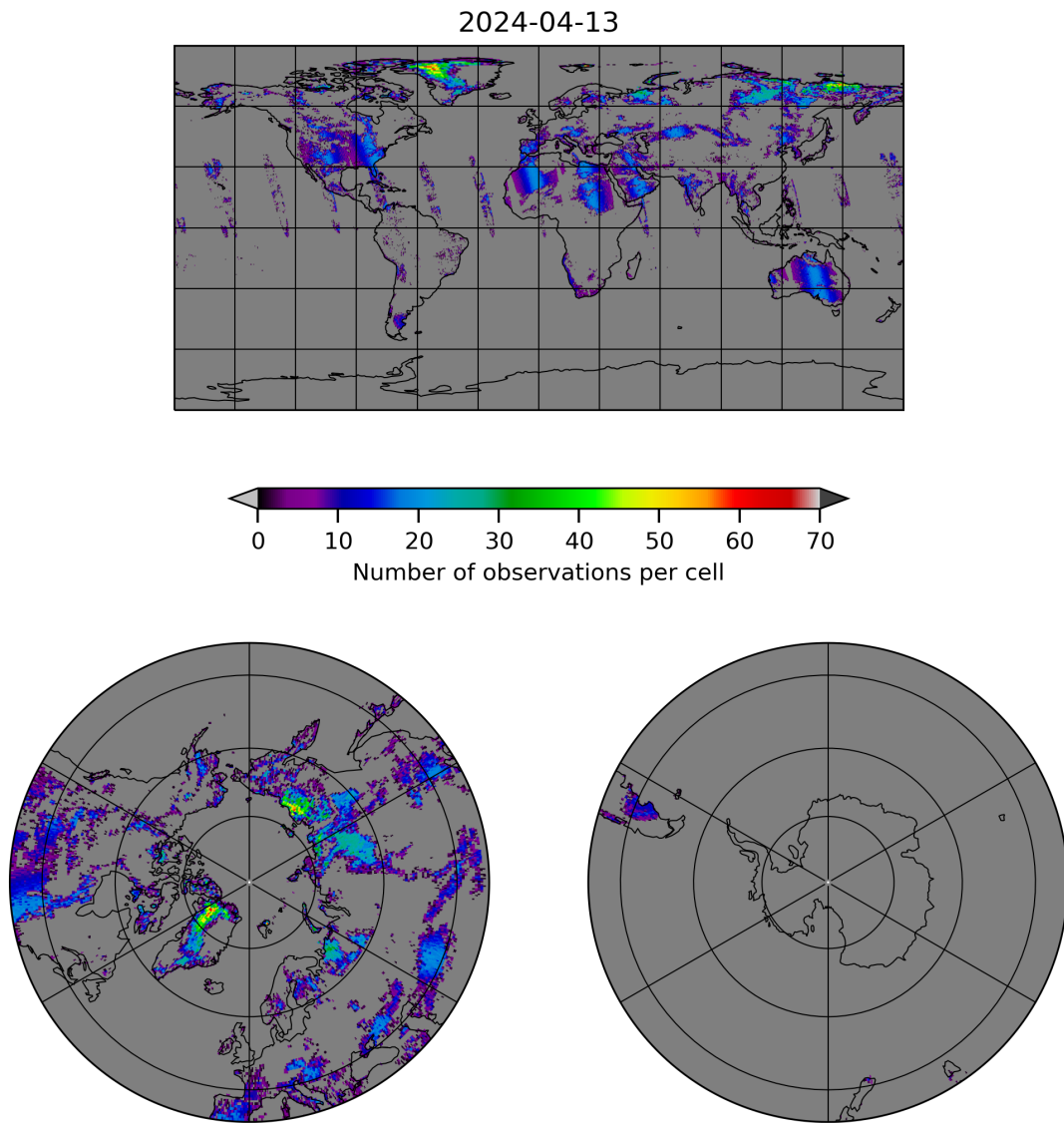
Figure 10: Map of the number of observations for 2024-04-12 to 2024-04-14
