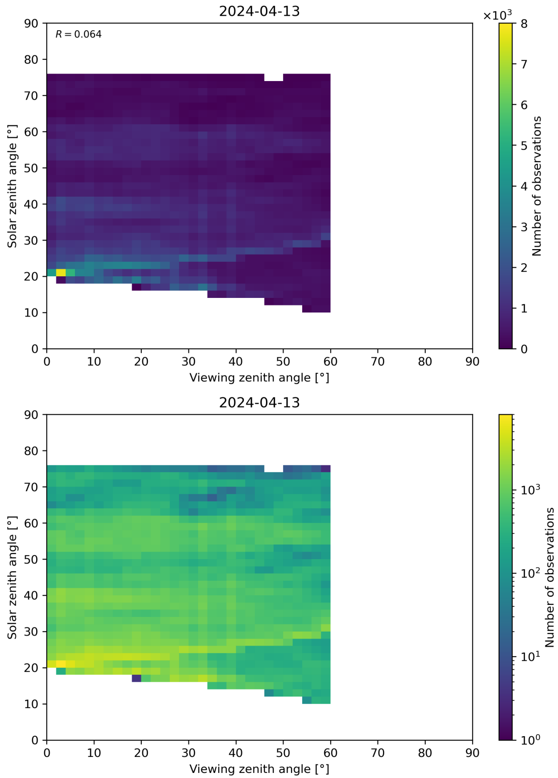
Figure 115: Scatter density plot of “Viewing zenith angle” against “Solar zenith angle” for 2024-04-12 to 2024-04-14.
