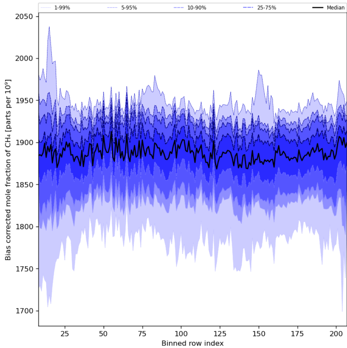
Figure 36: Along track statistics of “Bias corrected mole fraction of CH 4 ” for 2024-04-12 to 2024-04-14
