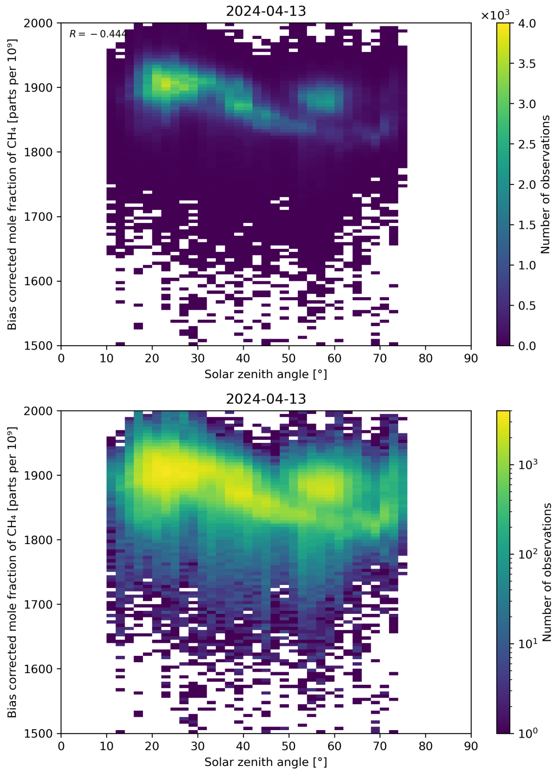
Figure 100: Scatter density plot of “Solar zenith angle” against “Bias corrected mole fraction of CH 4 ” for 2024-04-12 to 2024-04-14.
