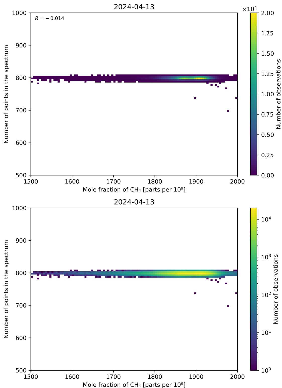
Figure 77: Scatter density plot of “Mole fraction of CH 4 ” against “Number of points in the spectrum” for 2024-04-12 to 2024-04-14.
