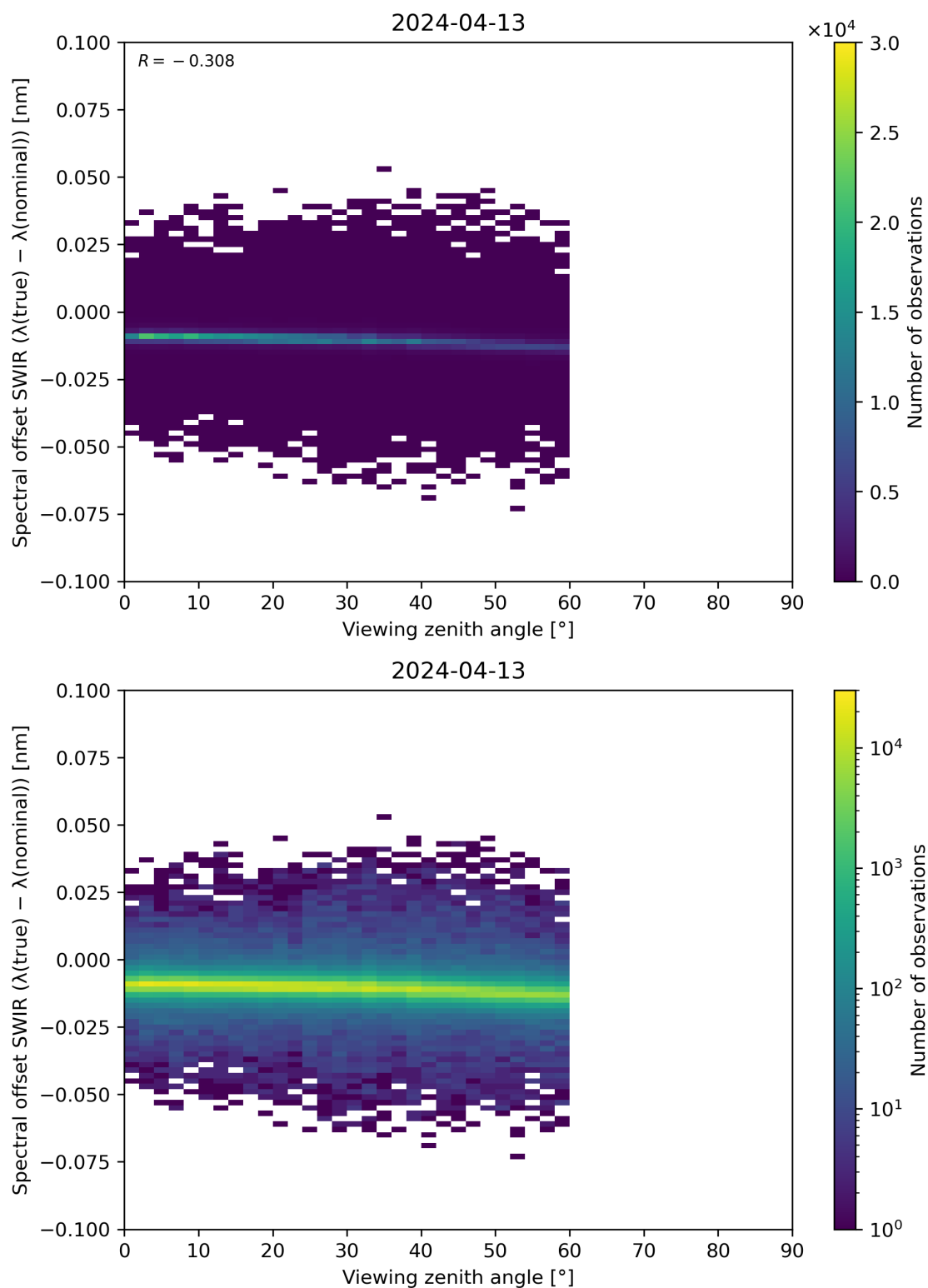
Figure 116: Scatter density plot of “Viewing zenith angle” against “Spectral offset SWIR ( \lambda(\text{true}) - \lambda(\text{nominal}) )” for 2024-04-12 to 2024-04-14.
