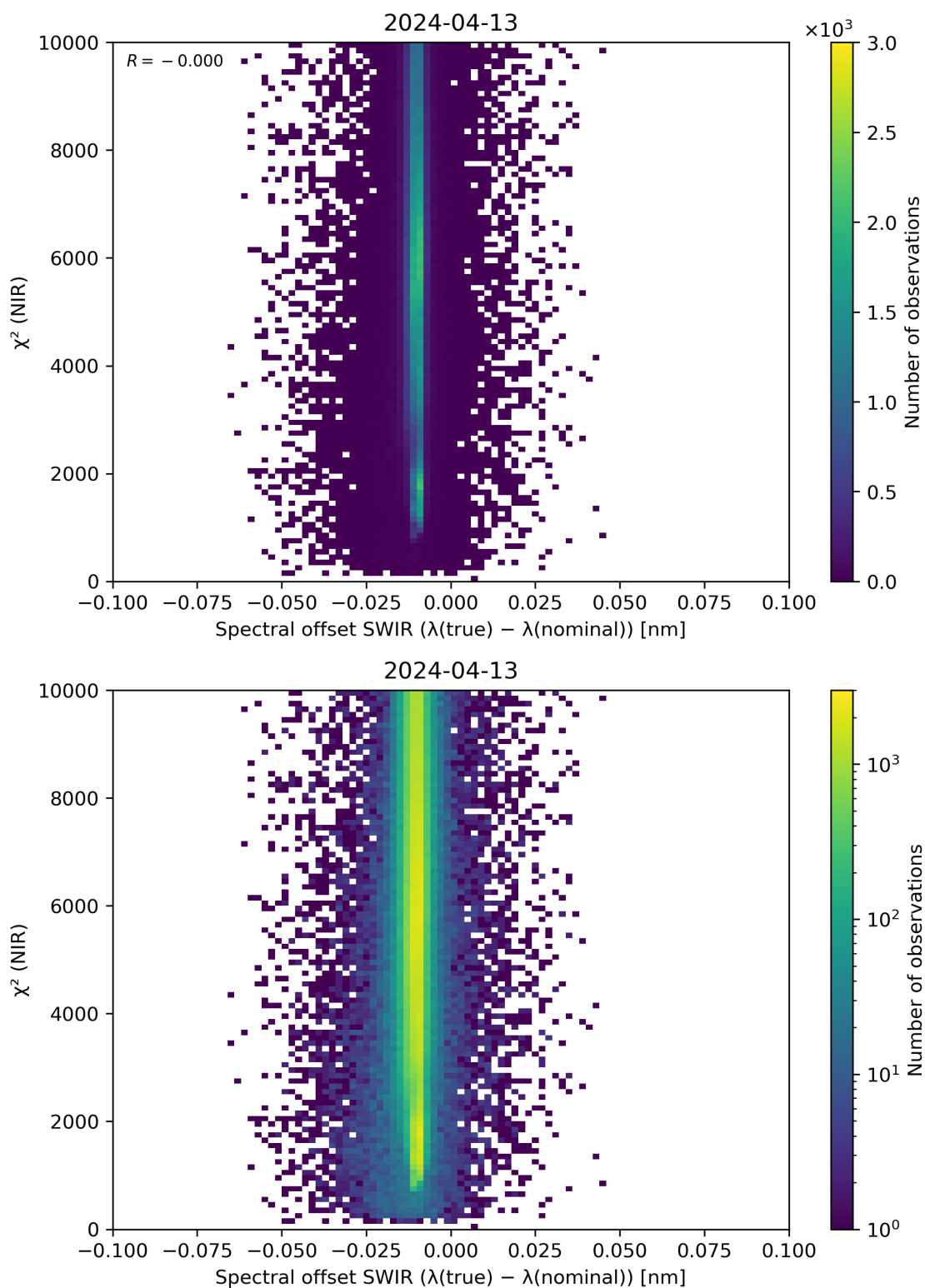
Figure 117: Scatter density plot of “Spectral offset SWIR ( \lambda(\text{true}) - \lambda(\text{nominal}) )” against “ \chi^2 (NIR)” for 2024-04-12 to 2024-04-14.
