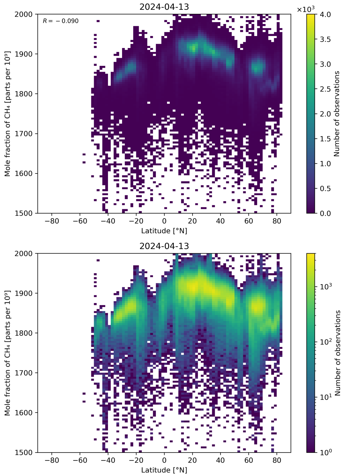
Figure 57: Scatter density plot of “Latitude” against “Mole fraction of \text{CH}_4 ” for 2024-04-12 to 2024-04-14.
