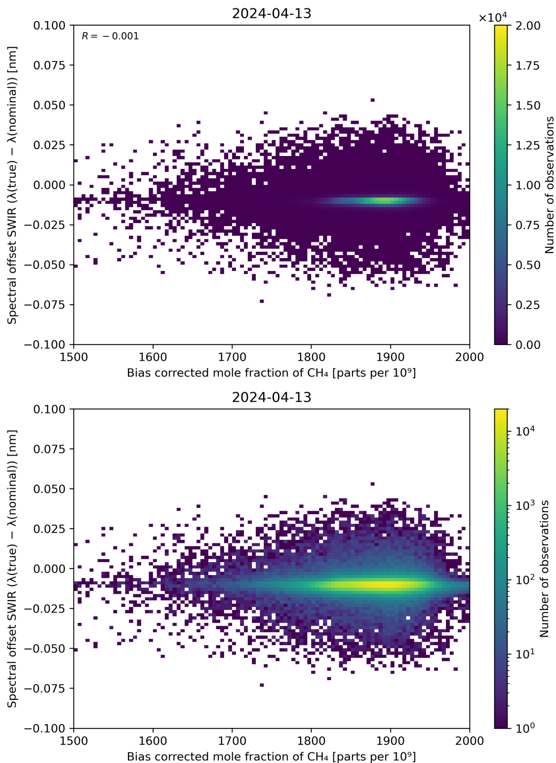
Figure 69: Scatter density plot of “Bias corrected mole fraction of \text{CH}_4 ” against “Spectral offset SWIR ( \lambda(\text{true}) - \lambda(\text{nominal}) )” for 2024-04-12 to 2024-04-14.
