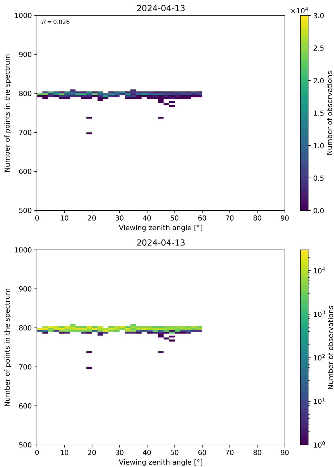
Figure 114: Scatter density plot of “Viewing zenith angle” against “Number of points in the spectrum” for 2024-04-12 to 2024-04-14.
