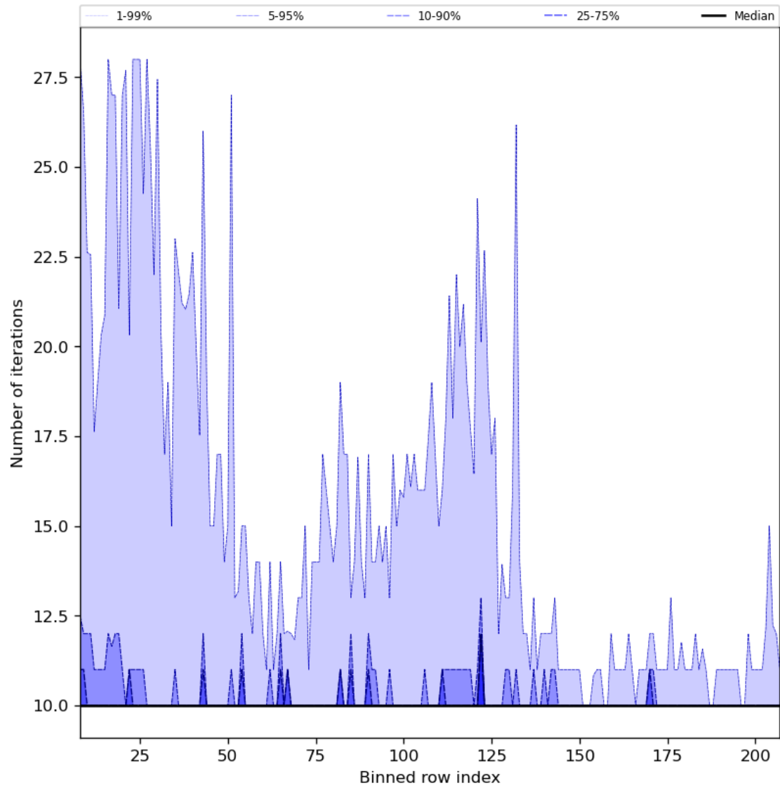
Figure 42: Along track statistics of “Number of iterations” for 2024-04-12 to 2024-04-14
