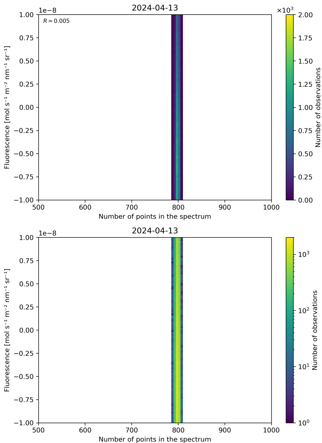
Figure 91: Scatter density plot of “Number of points in the spectrum” against “Fluorescence” for 2024-04-12 to 2024-04-14.
