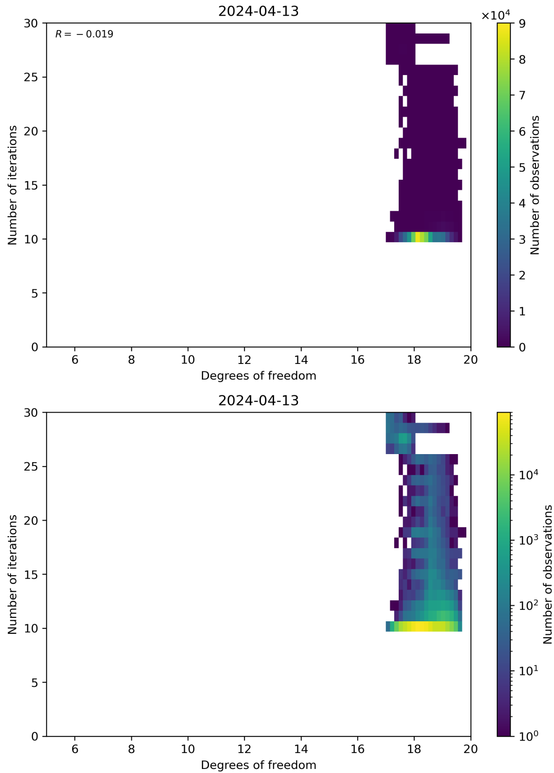
Figure 52: Scatter density plot of “Degrees of freedom” against “Number of iterations” for 2024-04-12 to 2024-04-14.
