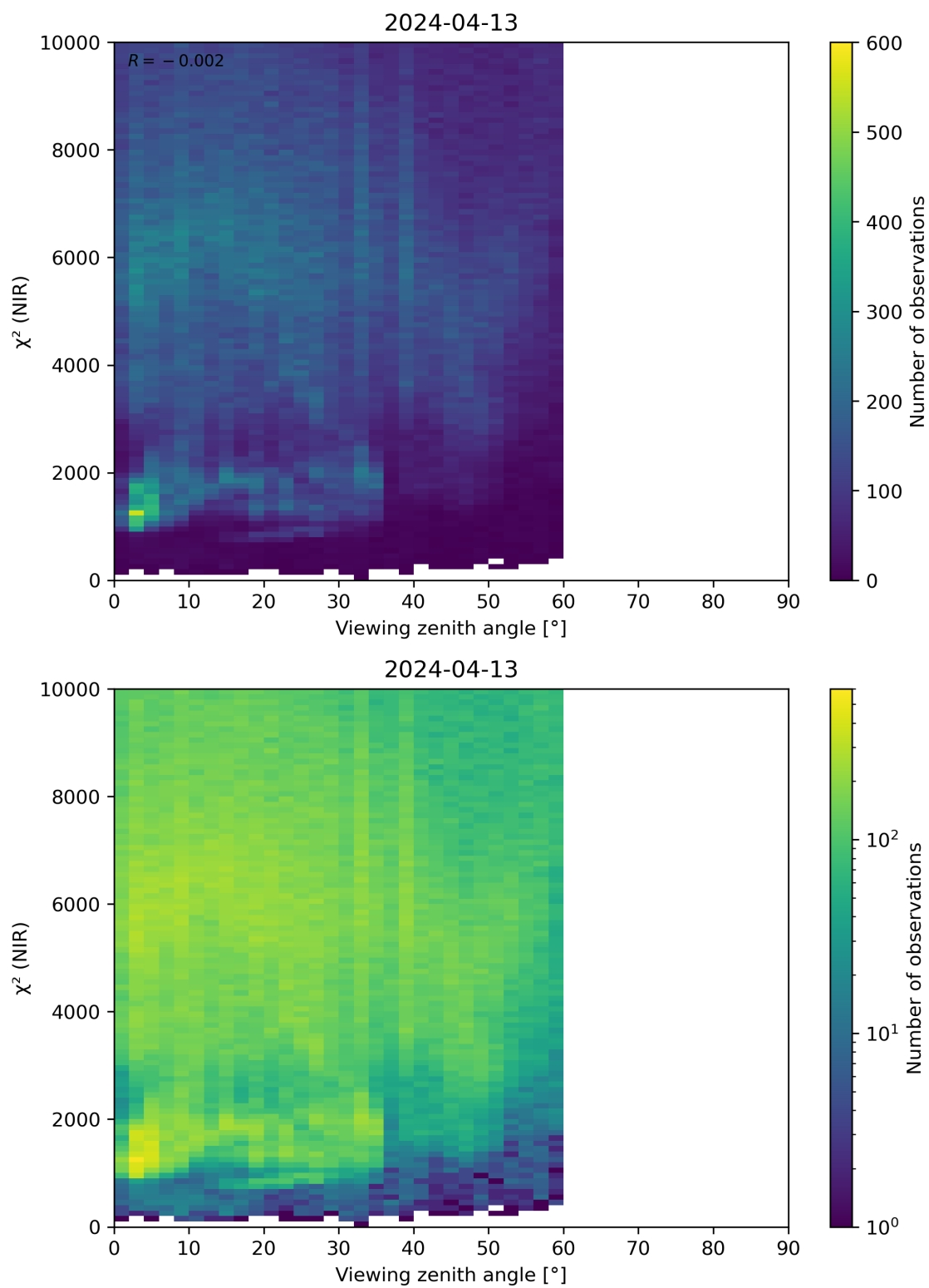
Figure 105: Scatter density plot of “Viewing zenith angle” against “ \chi^2 (NIR)” for 2024-04-12 to 2024-04-14.
