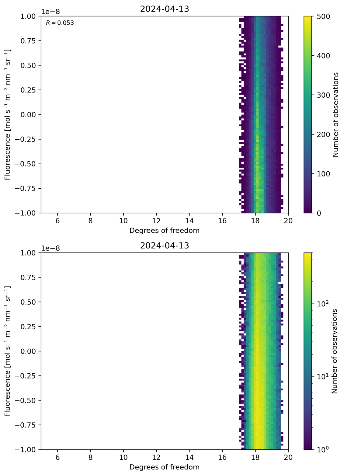
Figure 51: Scatter density plot of “Degrees of freedom” against “Fluorescence” for 2024-04-12 to 2024-04-14.
