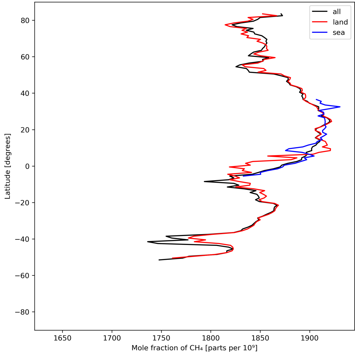
Figure 12: Zonal average of “Mole fraction of \text{CH}_4 ” for 2024-04-12 to 2024-04-14.
