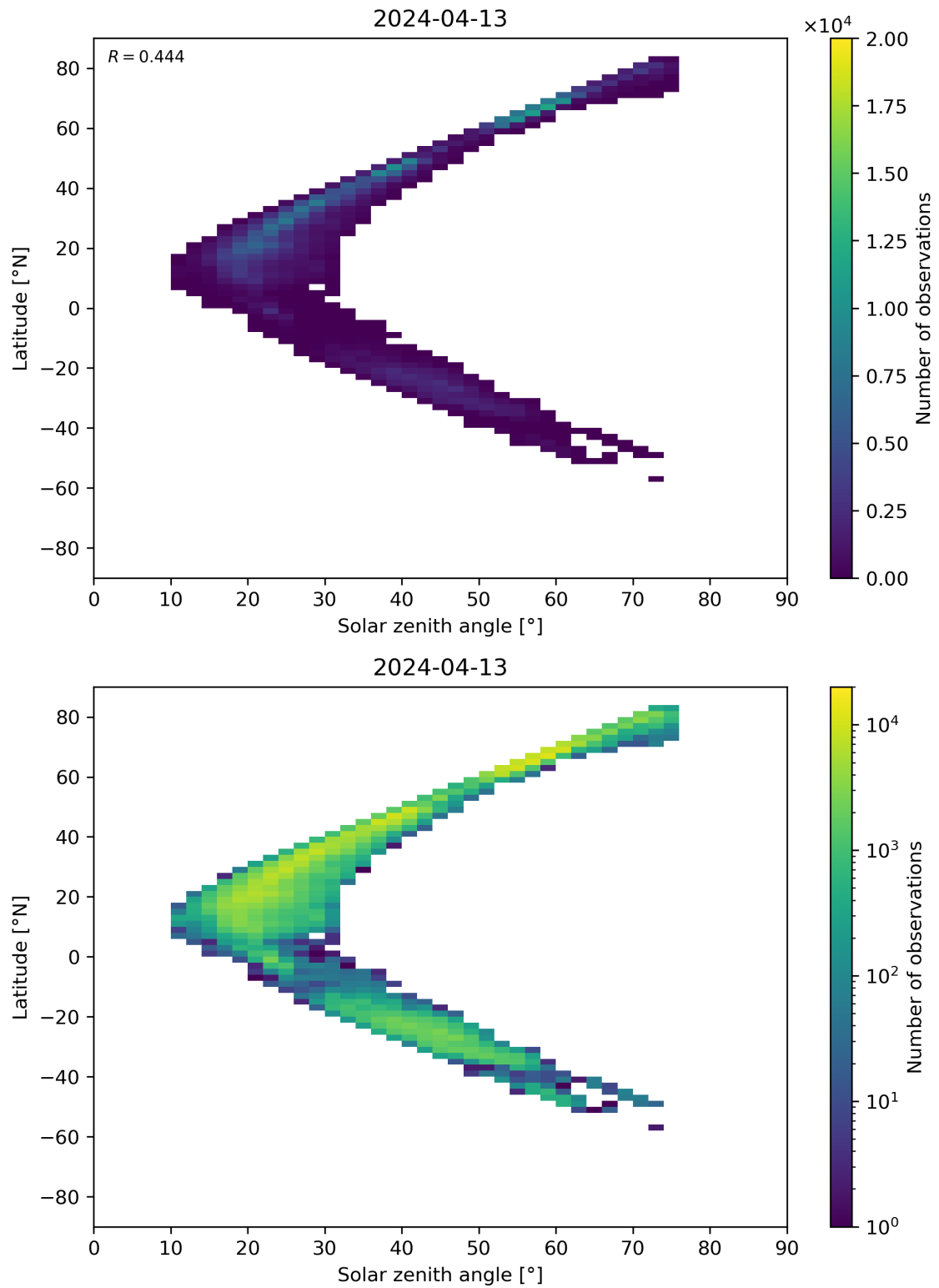
Figure 98: Scatter density plot of “Solar zenith angle” against “Latitude” for 2024-04-12 to 2024-04-14.
