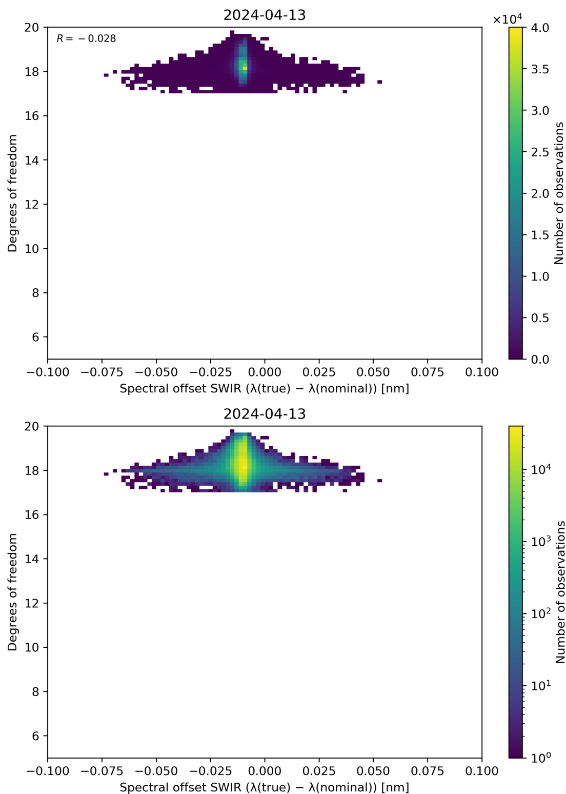
Figure 119: Scatter density plot of “Spectral offset SWIR ( \lambda(\text{true}) - \lambda(\text{nominal}) )” against “Degrees of freedom” for 2024-04-12 to 2024-04-14.
