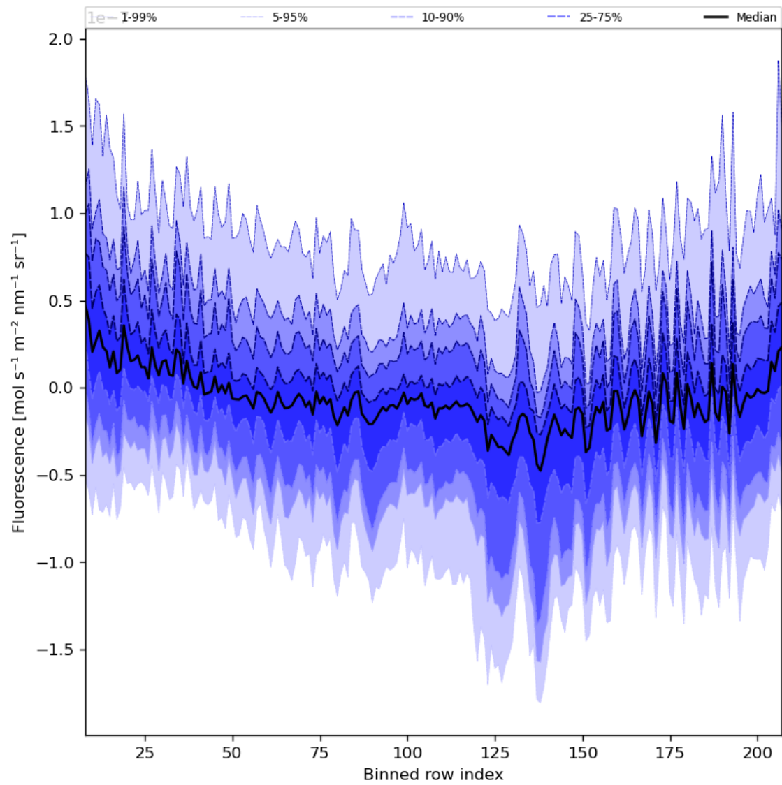
Figure 43: Along track statistics of “Fluorescence” for 2024-04-12 to 2024-04-14
