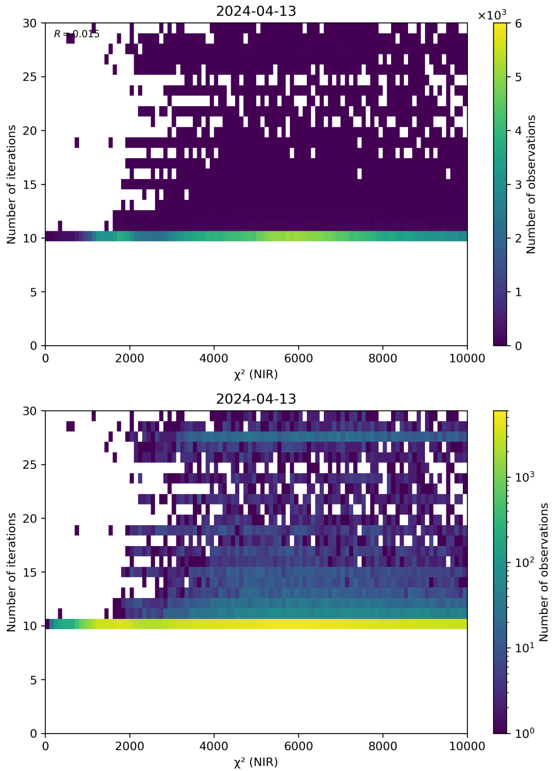
Figure 46: Scatter density plot of “ \chi^2 (NIR)” against “Number of iterations” for 2024-04-12 to 2024-04-14.
