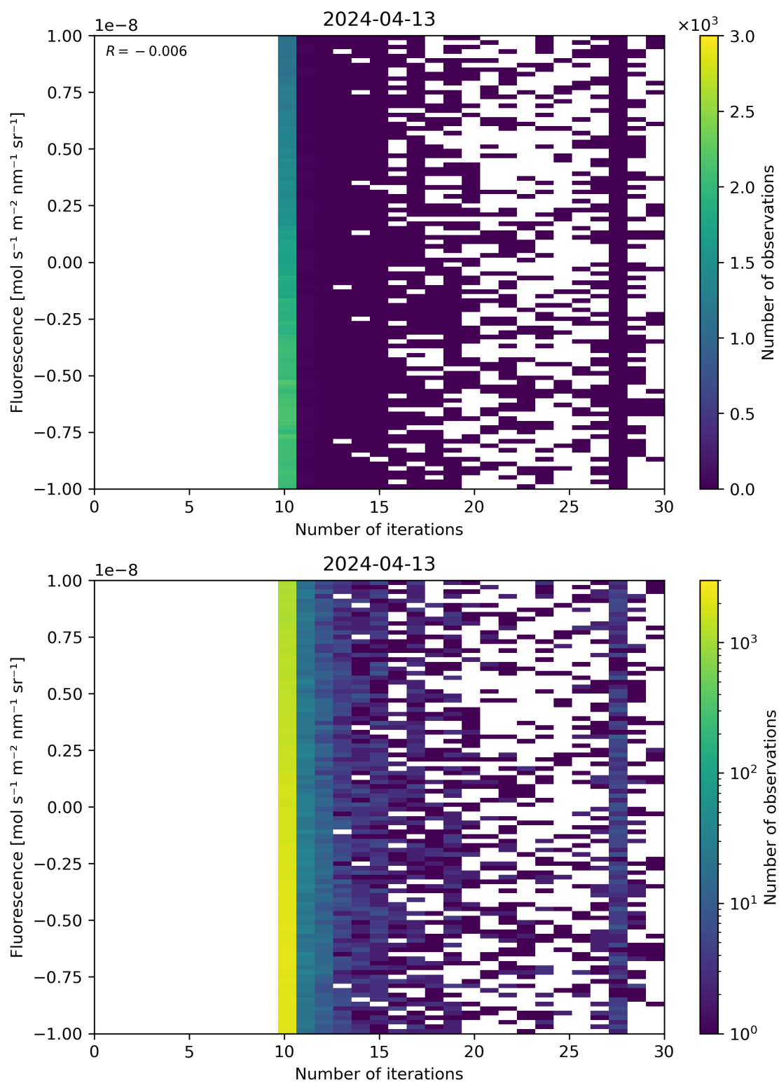
Figure 87: Scatter density plot of “Number of iterations” against “Fluorescence” for 2024-04-12 to 2024-04-14.
