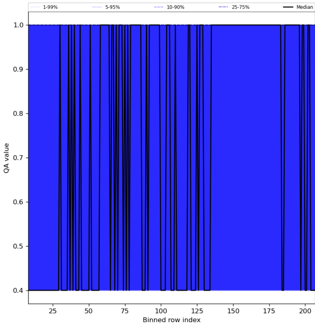
Figure 33: Along track statistics of “QA value” for 2024-04-12 to 2024-04-14
