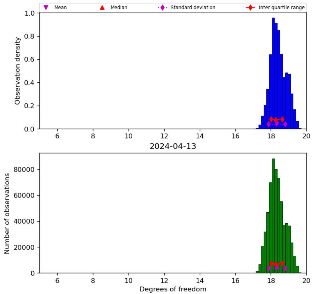
Figure 30: Histogram of “Degrees of freedom” for 2024-04-12 to 2024-04-14
