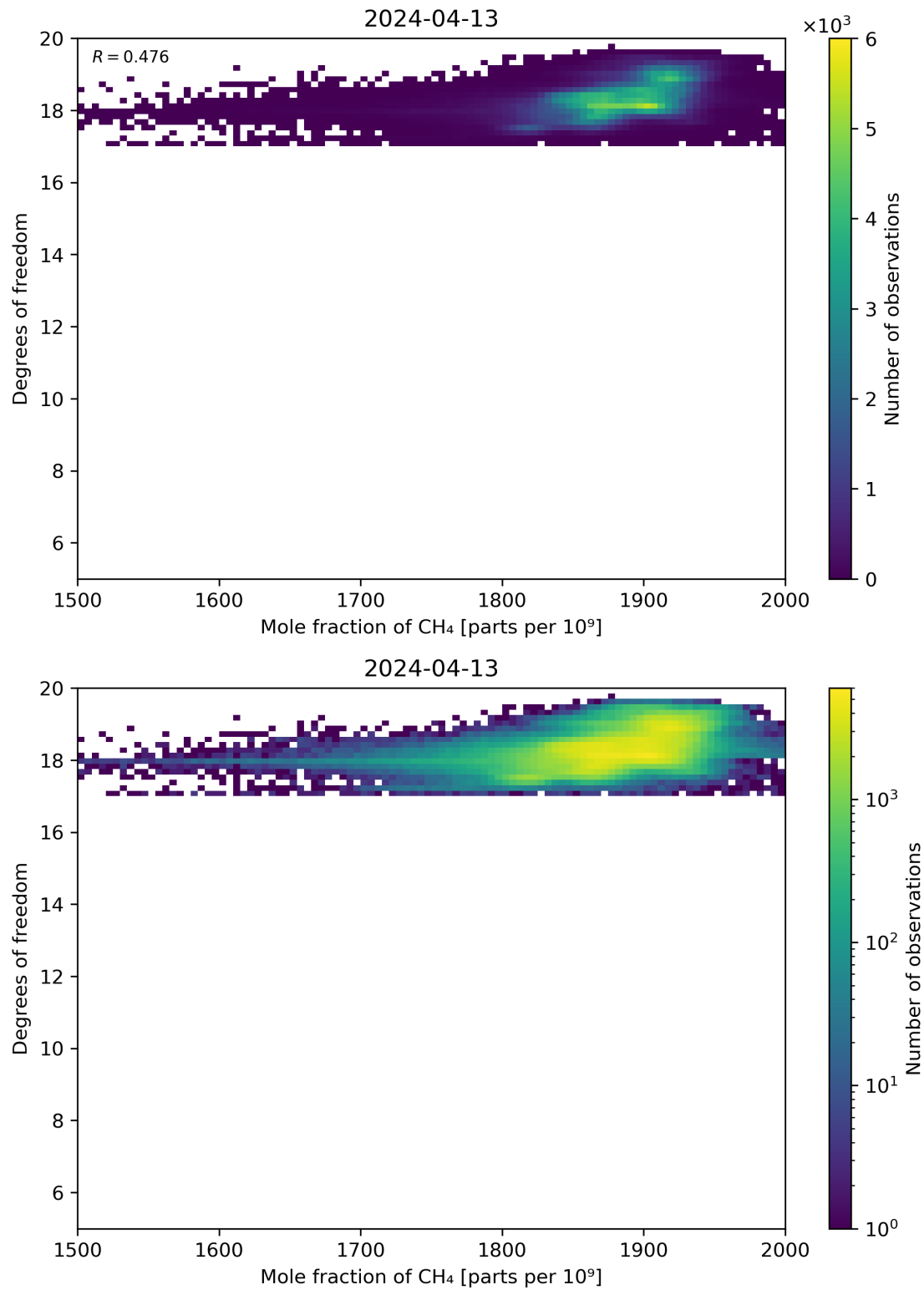
Figure 72: Scatter density plot of “Mole fraction of CH 4 ” against “Degrees of freedom” for 2024-04-12 to 2024-04-14.
