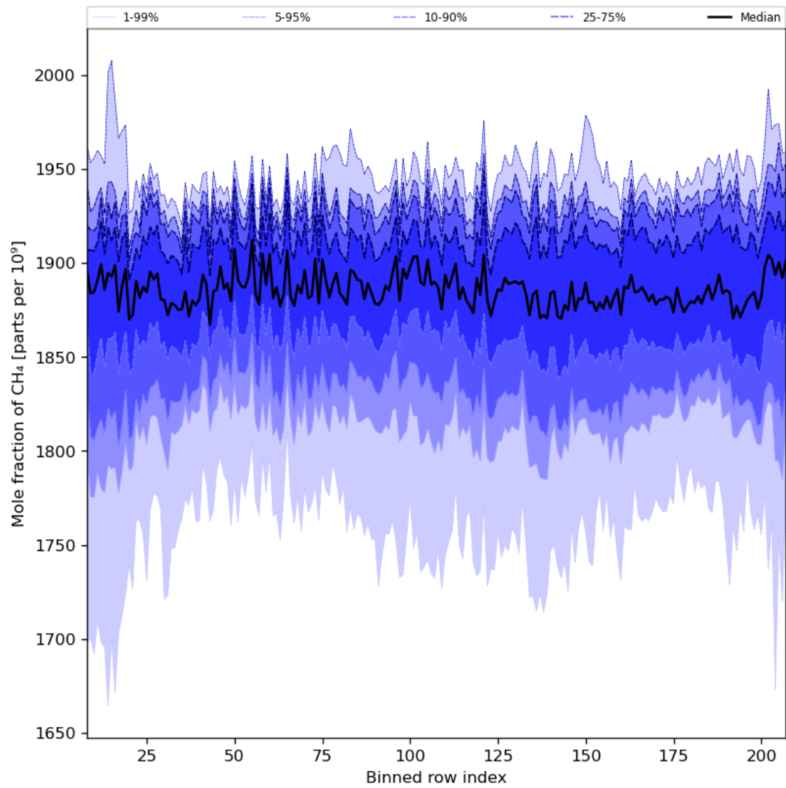
Figure 34: Along track statistics of “Mole fraction of CH 4 ” for 2024-04-12 to 2024-04-14
