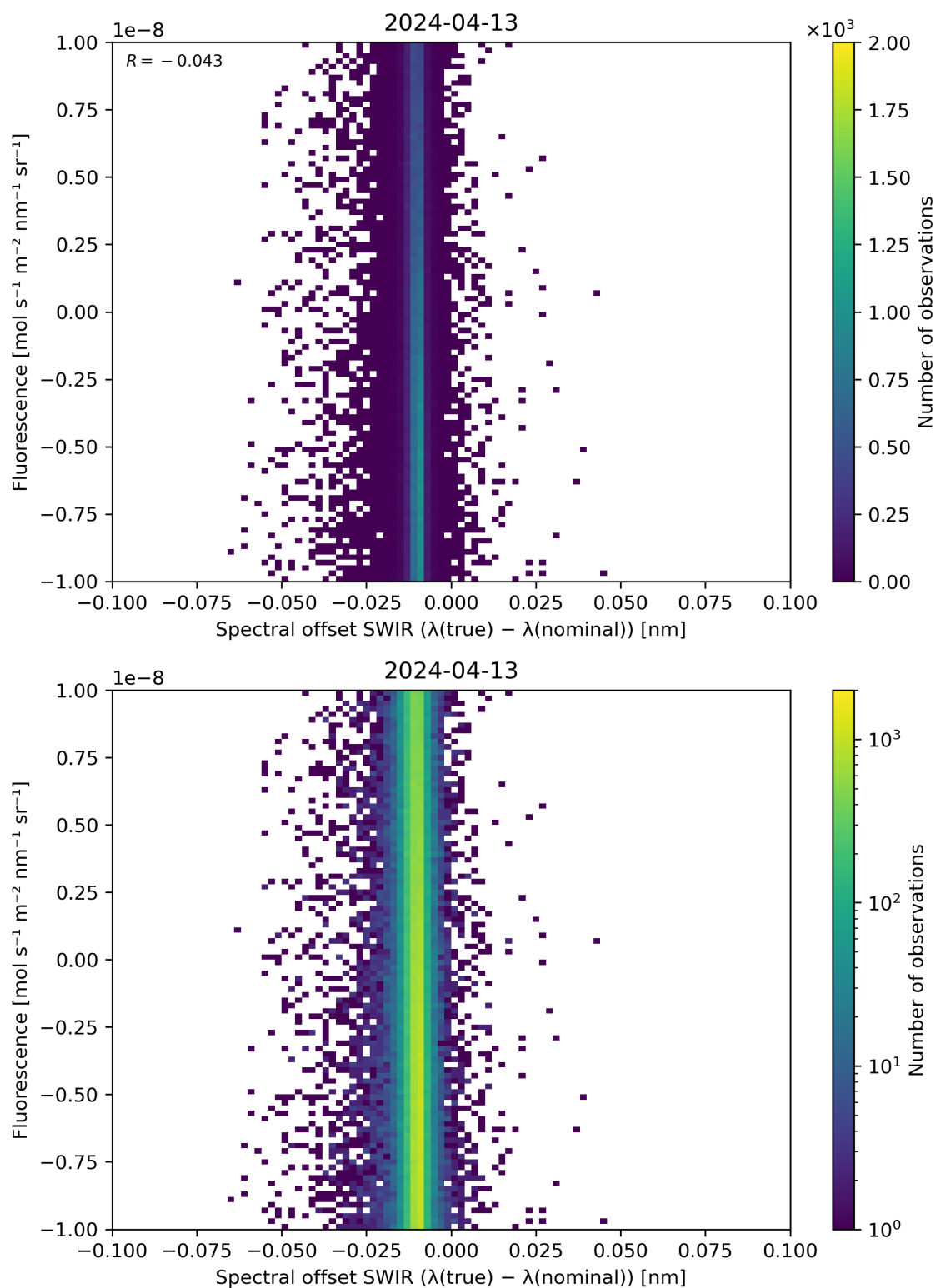
Figure 120: Scatter density plot of “Spectral offset SWIR ( \lambda(\text{true}) - \lambda(\text{nominal}) )” against “Fluorescence” for 2024-04-12 to 2024-04-14.
