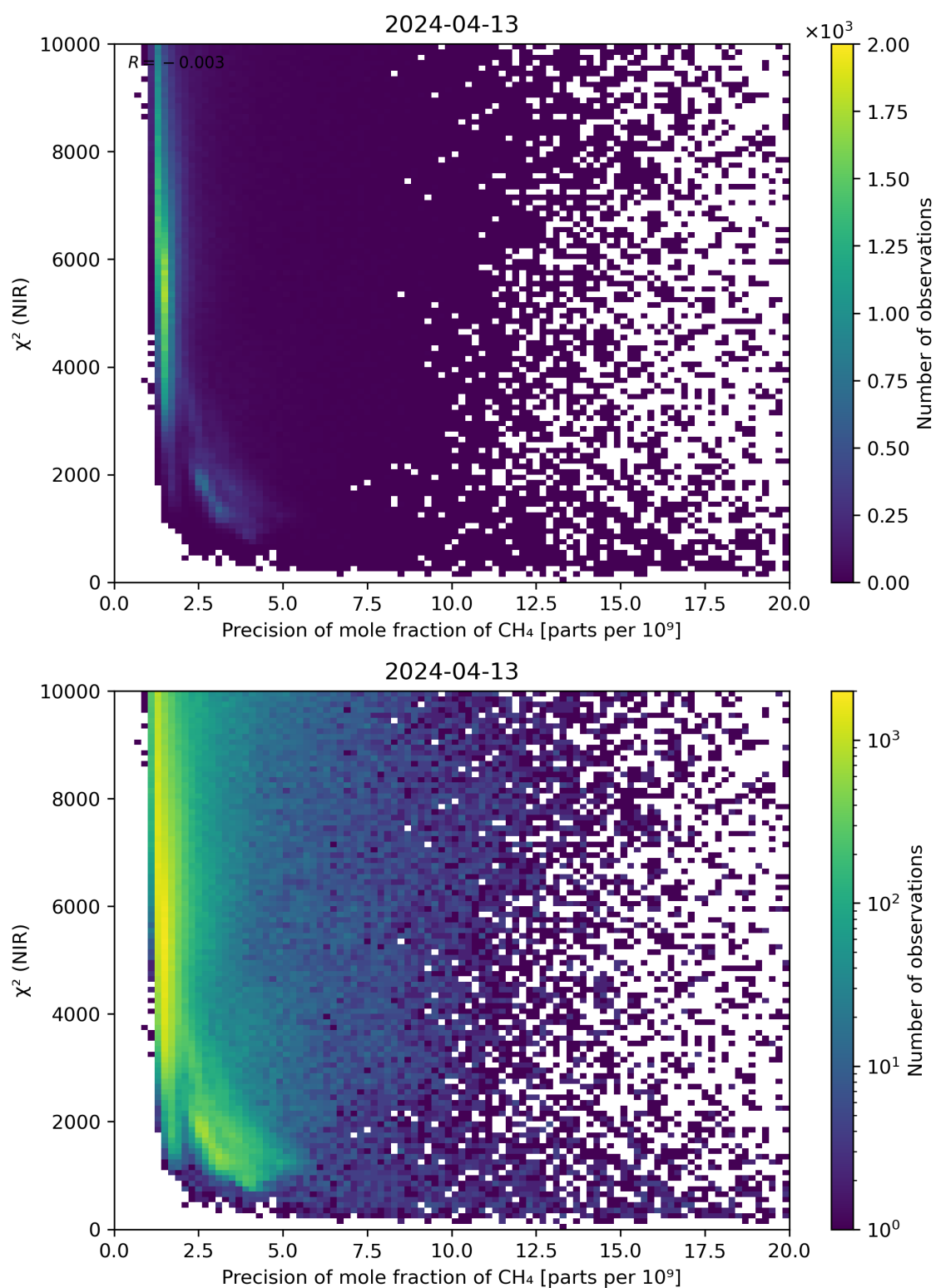
Figure 78: Scatter density plot of “Precision of mole fraction of CH 4 ” against “ \chi^2 (NIR)” for 2024-04-12 to 2024-04-14.
