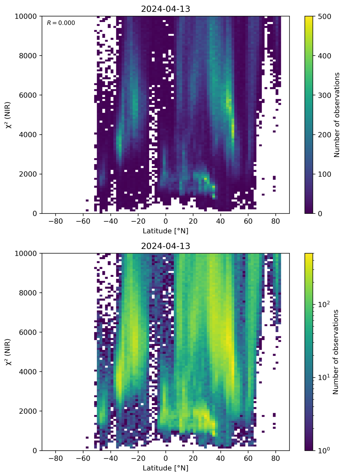
Figure 53: Scatter density plot of “Latitude” against “ \chi^2 (NIR)” for 2024-04-12 to 2024-04-14.
