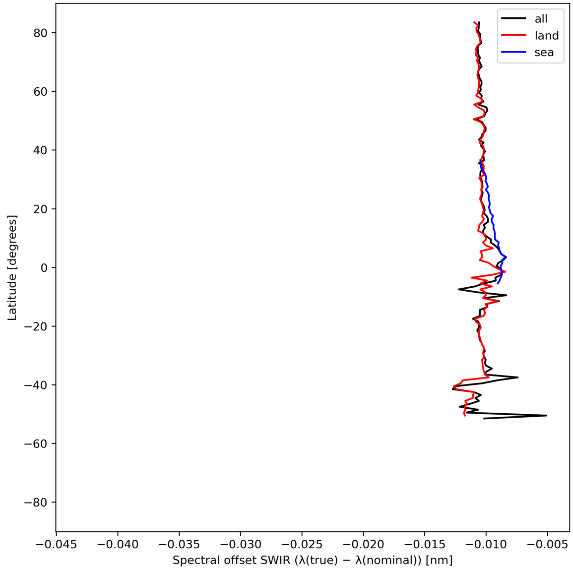
Figure 16: Zonal average of “Spectral offset SWIR ( \lambda(\text{true}) - \lambda(\text{nominal}) )” for 2024-04-12 to 2024-04-14.
