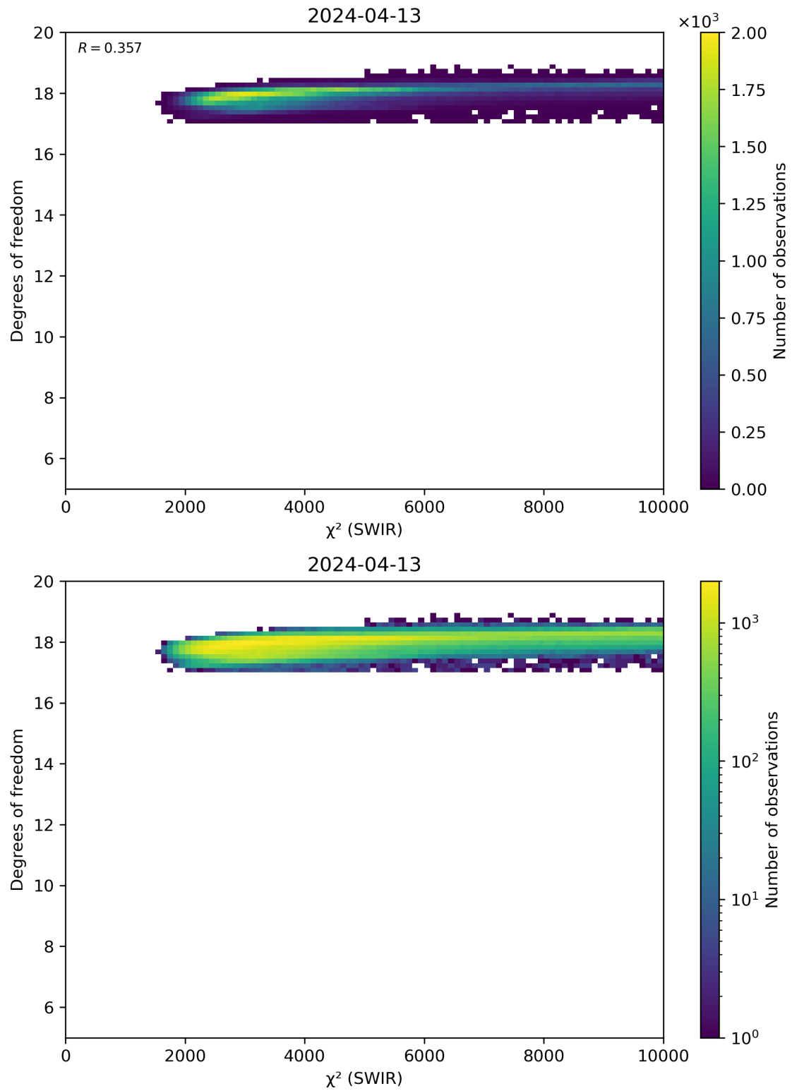
Figure 48: Scatter density plot of “ \chi^2 (SWIR)” against “Degrees of freedom” for 2024-04-12 to 2024-04-14.
