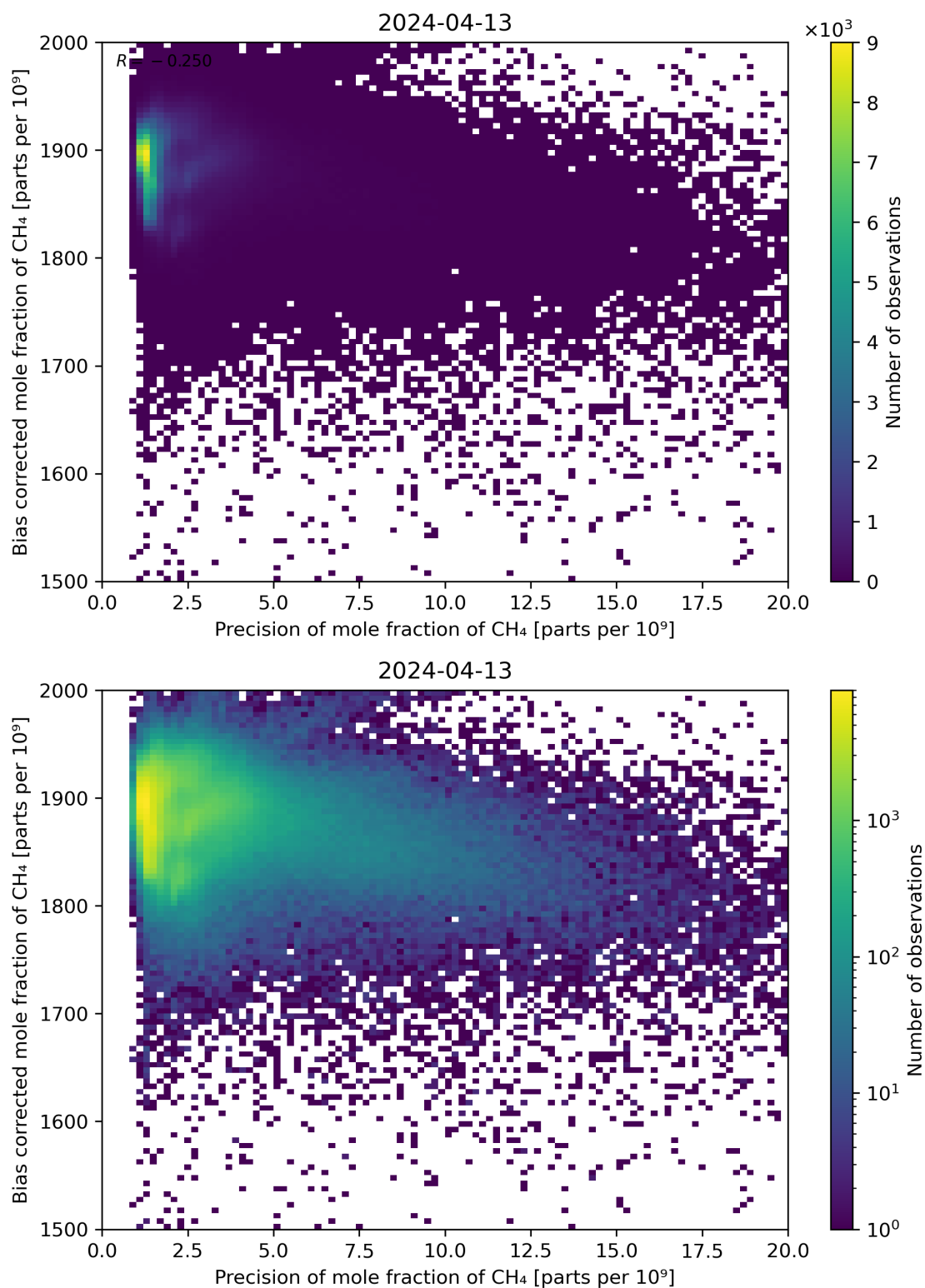
Figure 82: Scatter density plot of “Precision of mole fraction of CH 4 ” against “Bias corrected mole fraction of CH 4 ” for 2024-04-12 to 2024-04-14.
