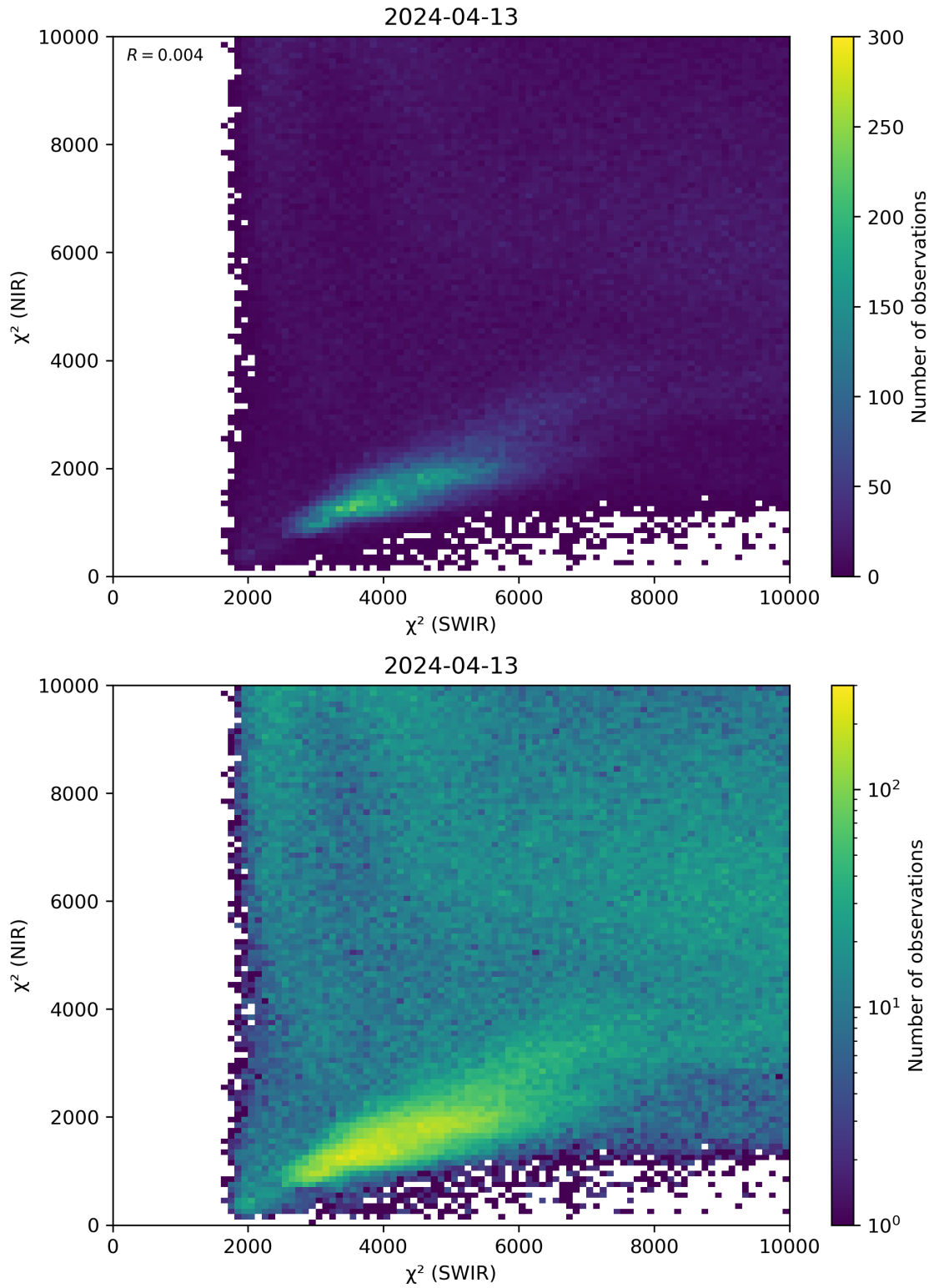
Figure 47: Scatter density plot of “ \chi^2 (SWIR)” against “ \chi^2 (NIR)” for 2024-04-12 to 2024-04-14.
