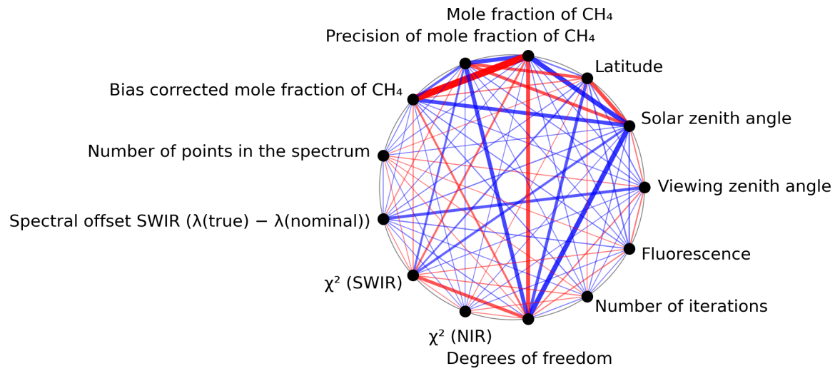
Figure 1: Map of correlation graph for 2024-04-12 to 2024-04-14.
