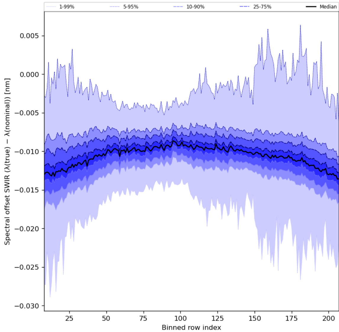
Figure 38: Along track statistics of “Spectral offset SWIR ( \lambda(\text{true}) - \lambda(\text{nominal}) )” for 2024-04-12 to 2024-04-14
