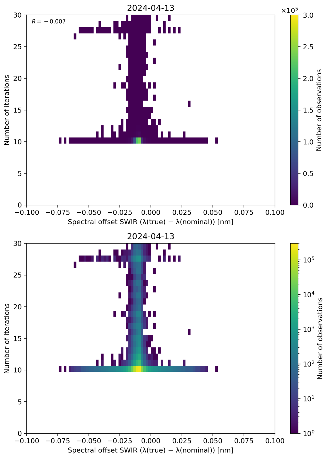
Figure 121: Scatter density plot of “Spectral offset SWIR ( \lambda(\text{true}) - \lambda(\text{nominal}) )” against “Number of iterations” for 2024-04-12 to 2024-04-14.
