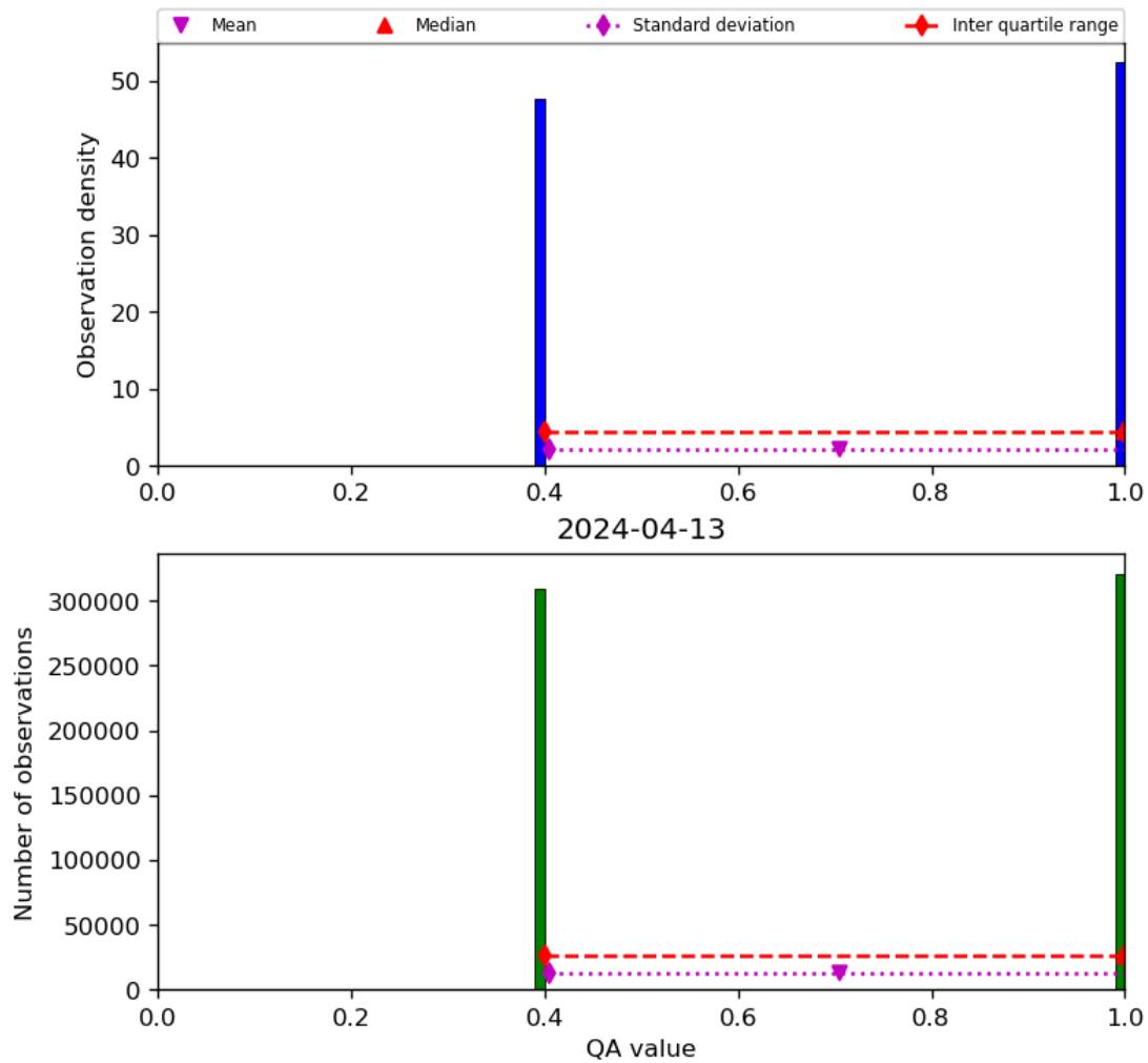
Figure 22: Histogram of “QA value” for 2024-04-12 to 2024-04-14
