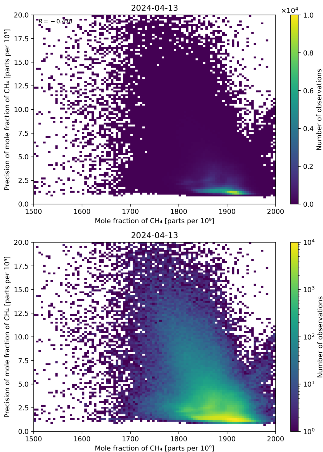
Figure 75: Scatter density plot of “Mole fraction of CH 4 ” against “Precision of mole fraction of CH 4 ” for 2024-04-12 to 2024-04-14.
