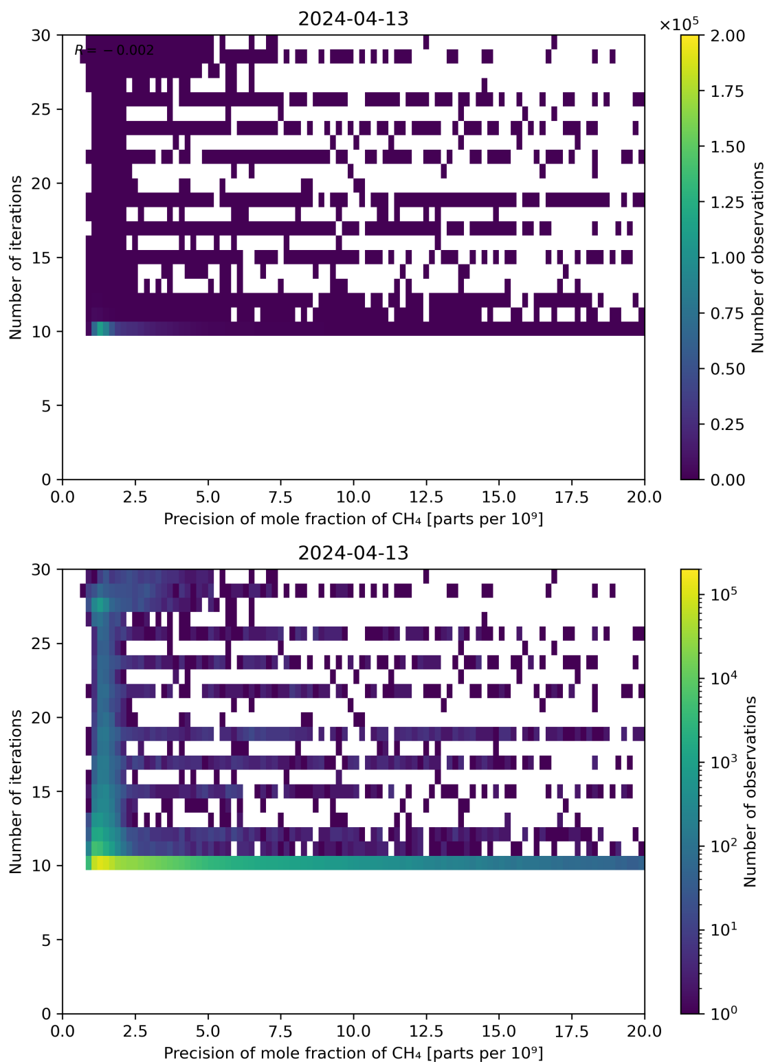
Figure 83: Scatter density plot of “Precision of mole fraction of CH 4 ” against “Number of iterations” for 2024-04-12 to 2024-04-14.
