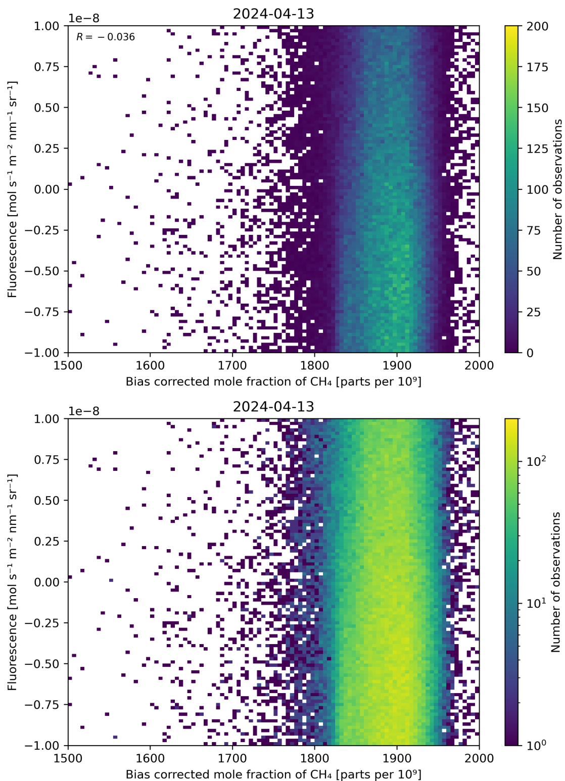
Figure 66: Scatter density plot of “Bias corrected mole fraction of \text{CH}_4 ” against “Fluorescence” for 2024-04-12 to 2024-04-14.
