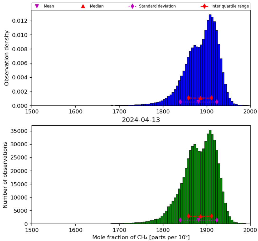
Figure 23: Histogram of “Mole fraction of CH 4 ” for 2024-04-12 to 2024-04-14
