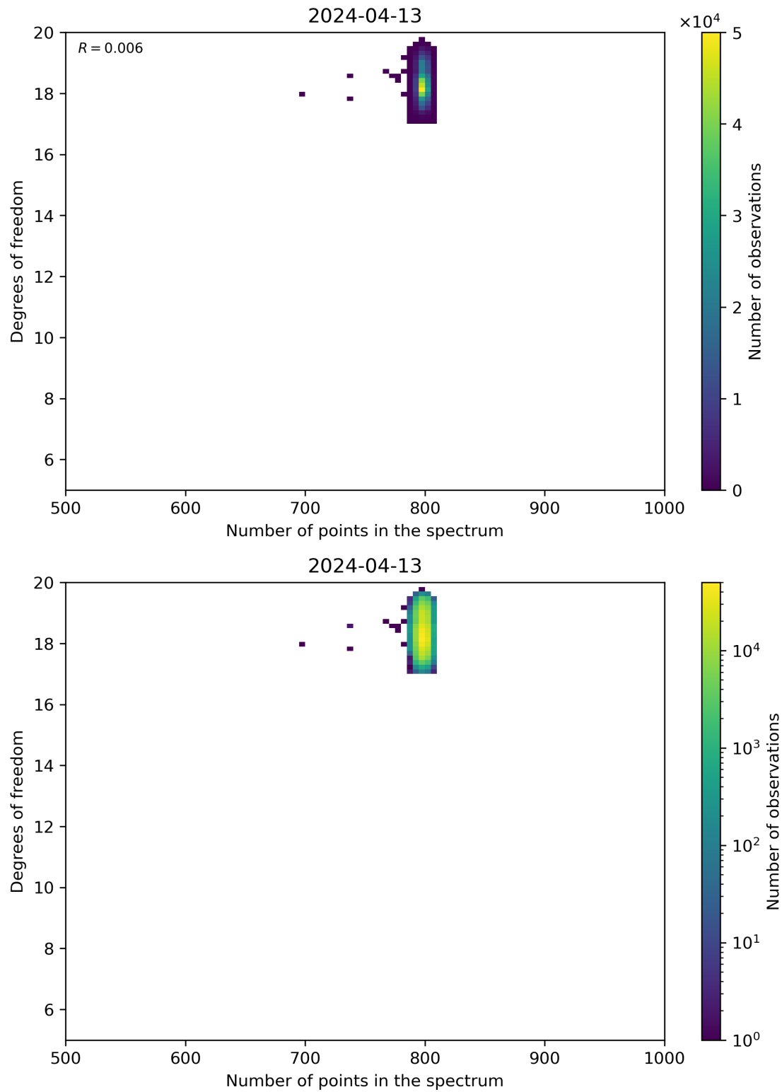
Figure 90: Scatter density plot of “Number of points in the spectrum” against “Degrees of freedom” for 2024-04-12 to 2024-04-14.
