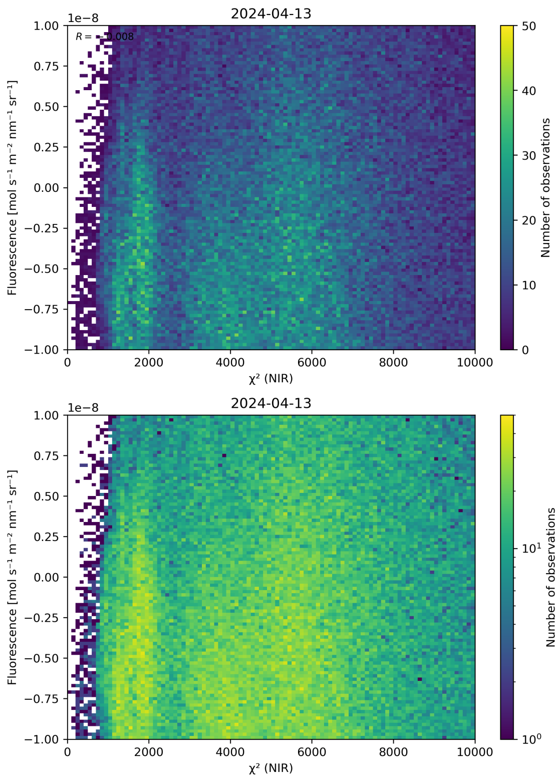
Figure 45: Scatter density plot of “ \chi^2 (NIR)” against “Fluorescence” for 2024-04-12 to 2024-04-14.
