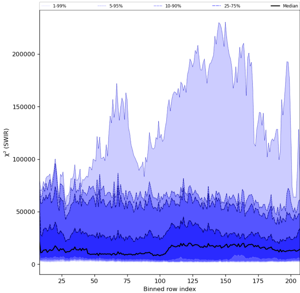
Figure 39: Along track statistics of “ \chi^2 (SWIR)” for 2024-04-12 to 2024-04-14
