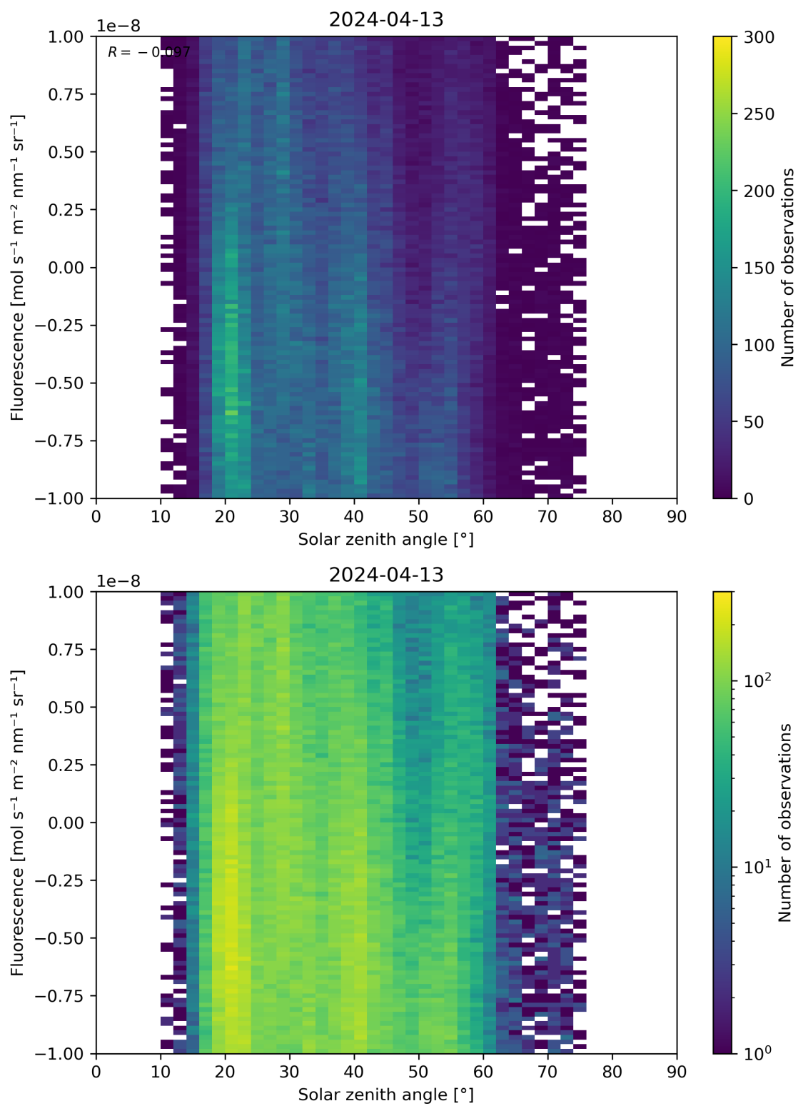
Figure 97: Scatter density plot of “Solar zenith angle” against “Fluorescence” for 2024-04-12 to 2024-04-14.
