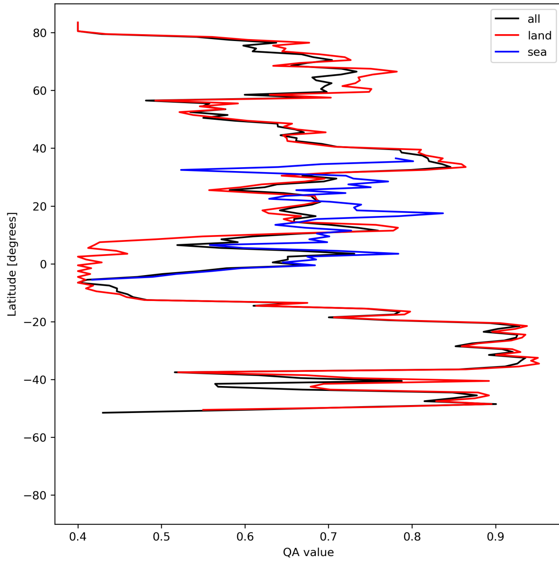
Figure 11: Zonal average of “QA value” for 2024-04-12 to 2024-04-14.
