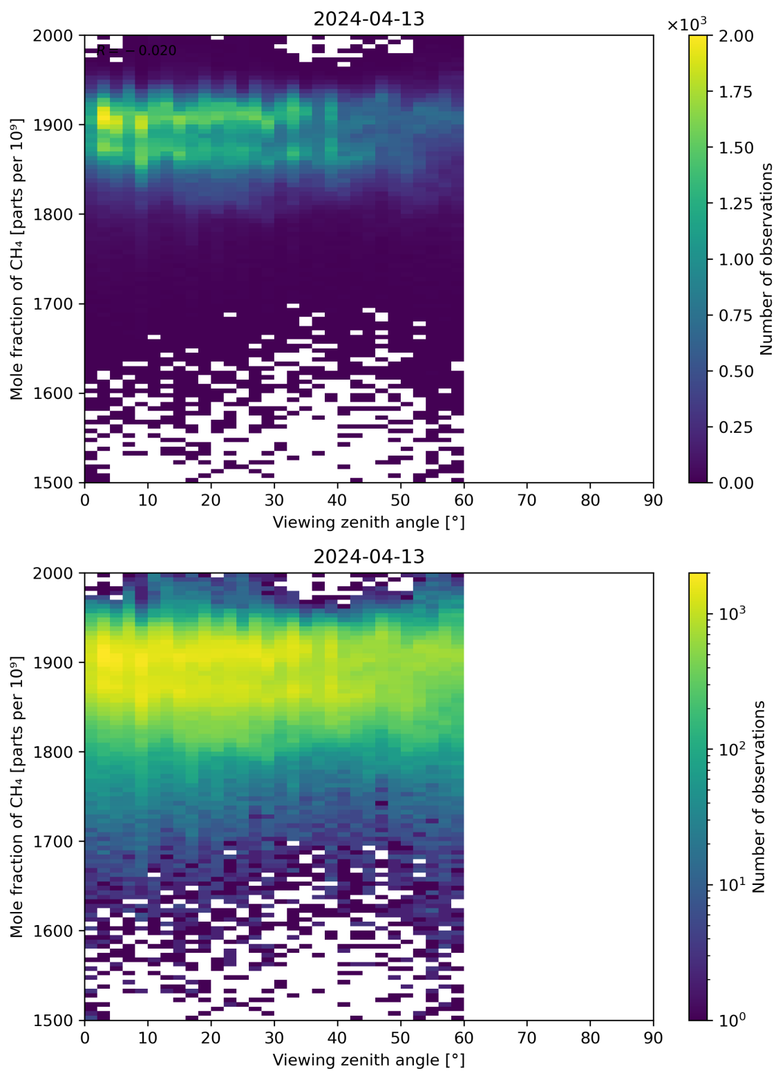
Figure 110: Scatter density plot of “Viewing zenith angle” against “Mole fraction of CH 4 ” for 2024-04-12 to 2024-04-14.
