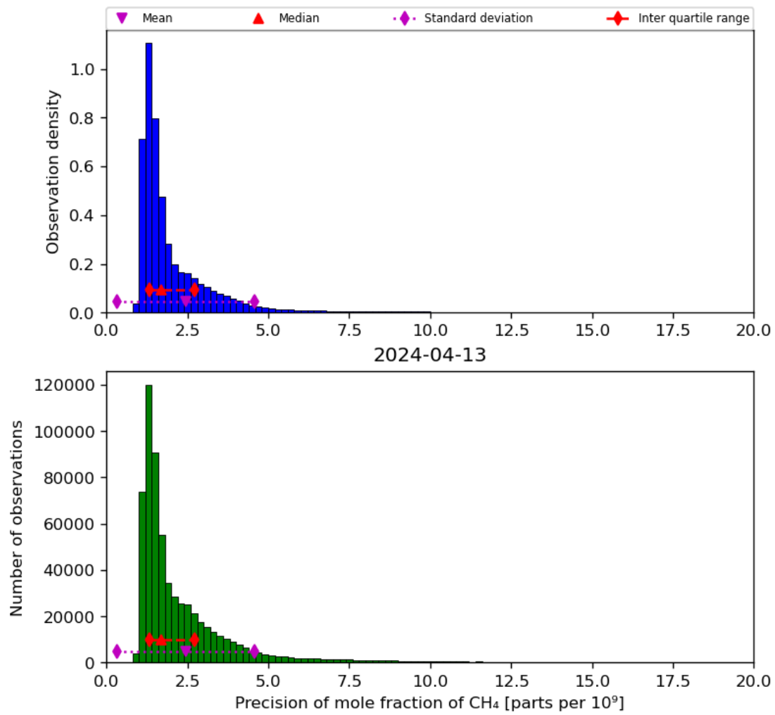
Figure 24: Histogram of “Precision of mole fraction of CH 4 ” for 2024-04-12 to 2024-04-14
