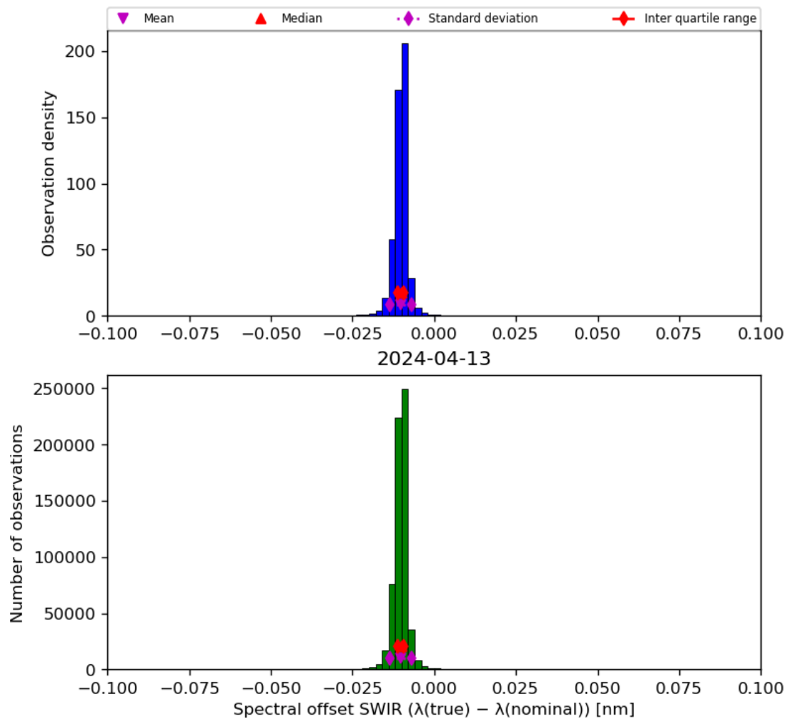
Figure 27: Histogram of “Spectral offset SWIR ( \lambda(\text{true}) - \lambda(\text{nominal}) )” for 2024-04-12 to 2024-04-14
