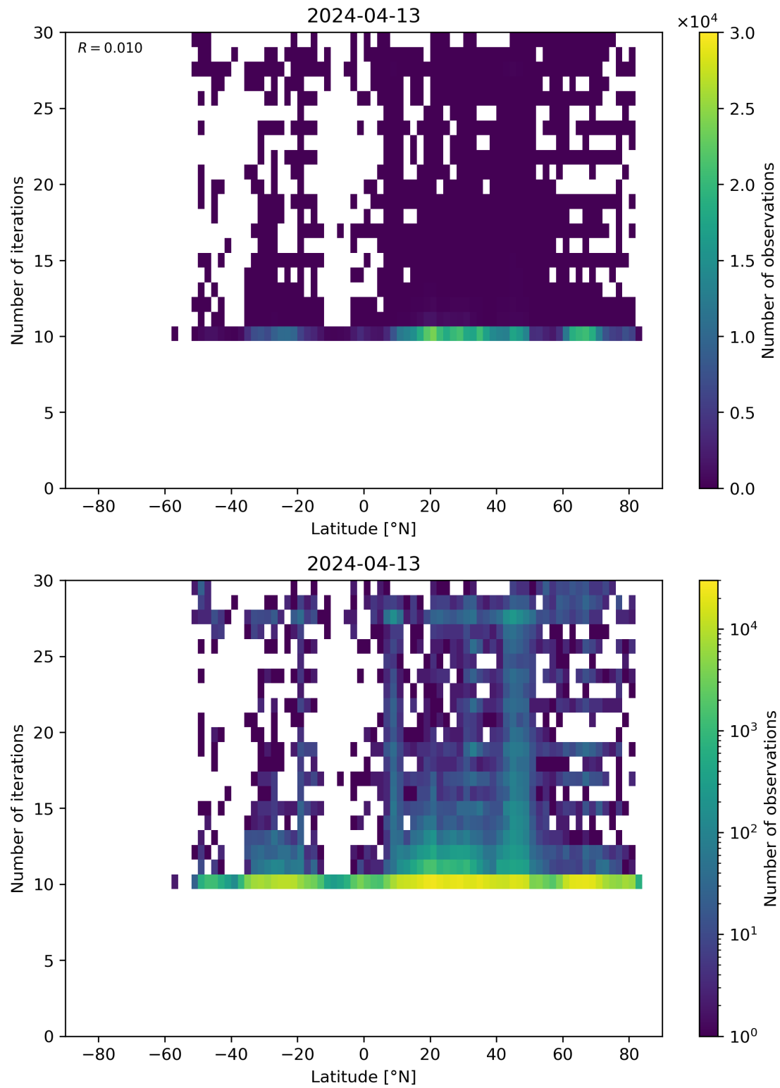
Figure 60: Scatter density plot of “Latitude” against “Number of iterations” for 2024-04-12 to 2024-04-14.
