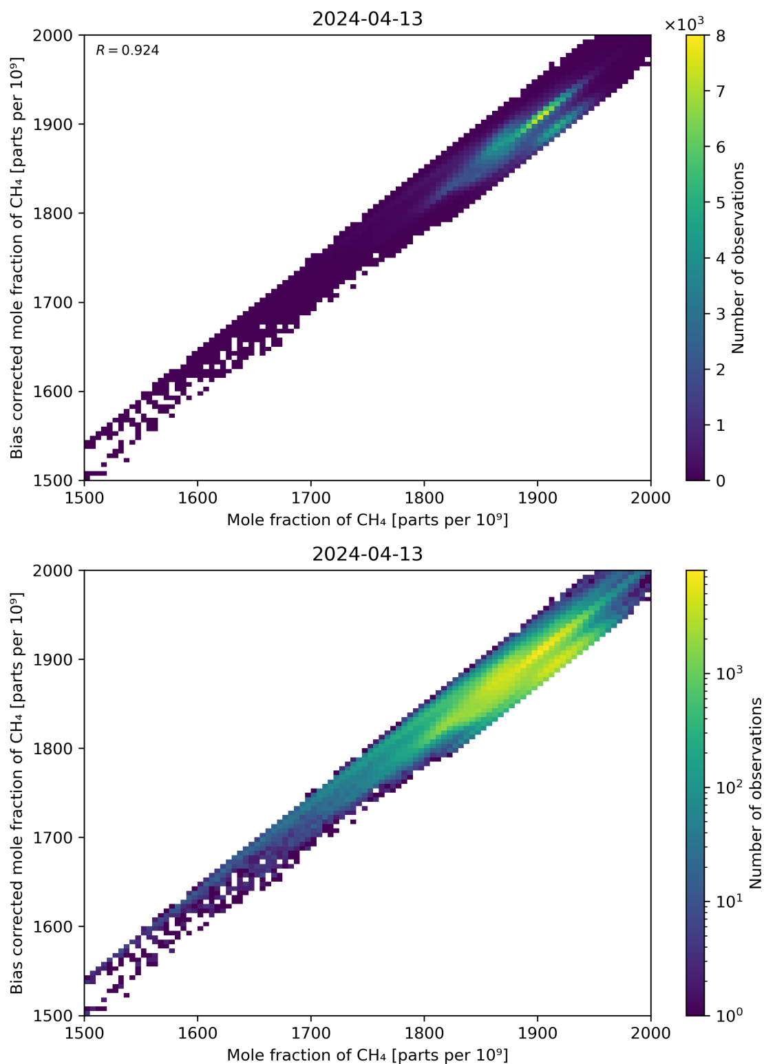
Figure 74: Scatter density plot of “Mole fraction of CH 4 ” against “Bias corrected mole fraction of CH 4 ” for 2024-04-12 to 2024-04-14.
