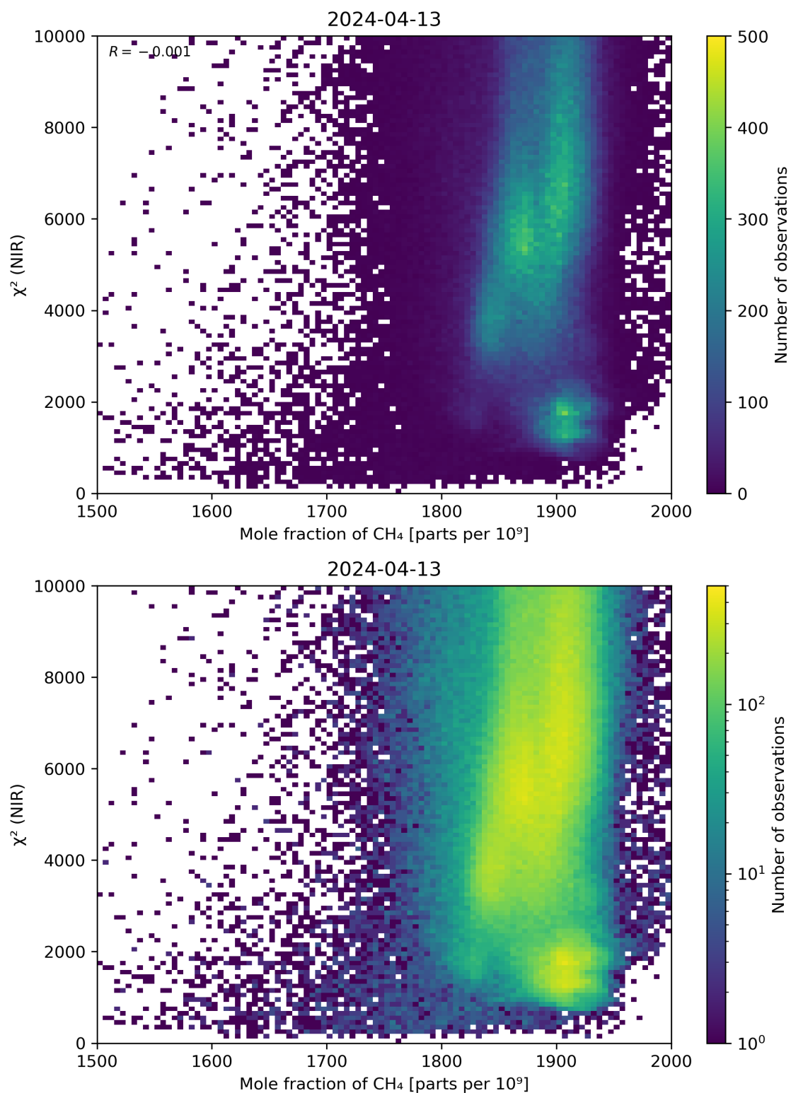
Figure 70: Scatter density plot of “Mole fraction of CH 4 ” against “ \chi^2 (NIR)” for 2024-04-12 to 2024-04-14.
