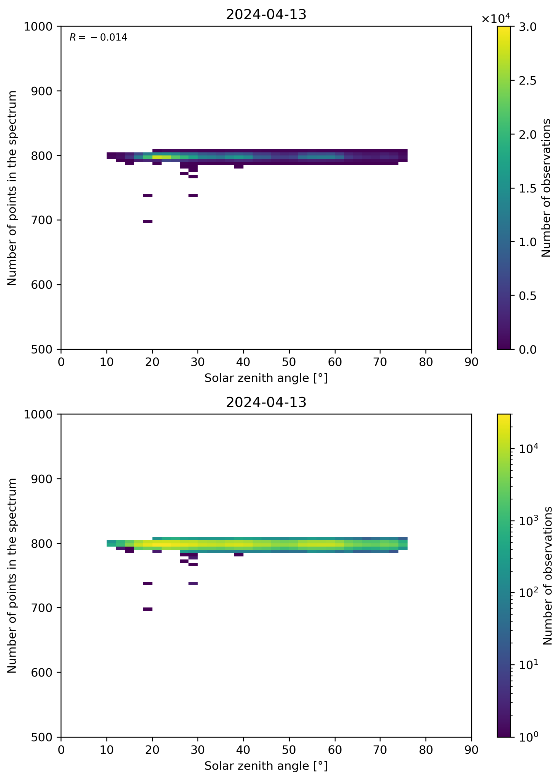
Figure 103: Scatter density plot of “Solar zenith angle” against “Number of points in the spectrum” for 2024-04-12 to 2024-04-14.
