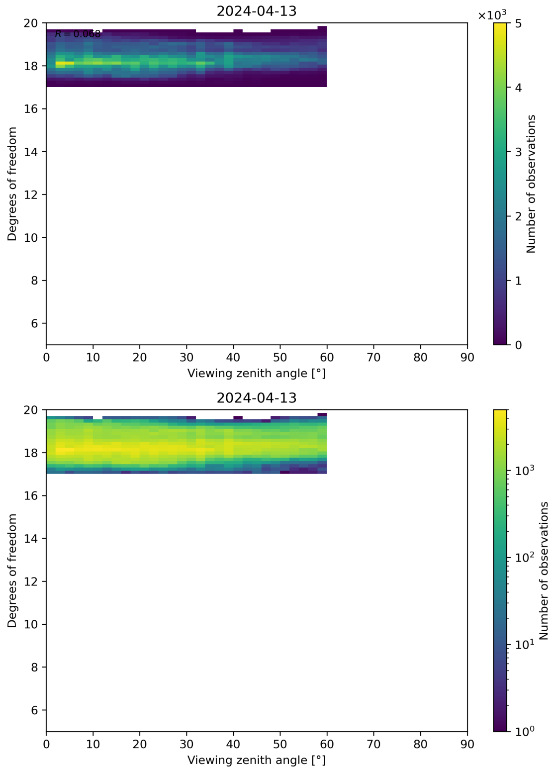
Figure 107: Scatter density plot of “Viewing zenith angle” against “Degrees of freedom” for 2024-04-12 to 2024-04-14.
