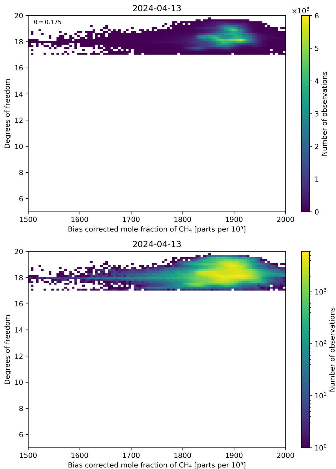
Figure 65: Scatter density plot of “Bias corrected mole fraction of CH 4 ” against “Degrees of freedom” for 2024-04-12 to 2024-04-14.
