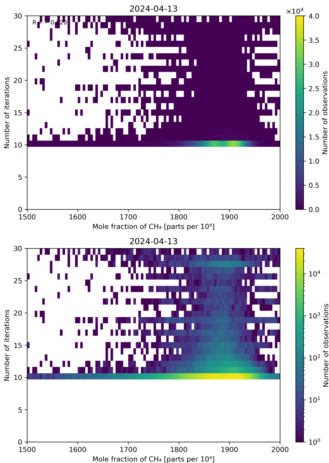
Figure 76: Scatter density plot of “Mole fraction of CH 4 ” against “Number of iterations” for 2024-04-12 to 2024-04-14.
