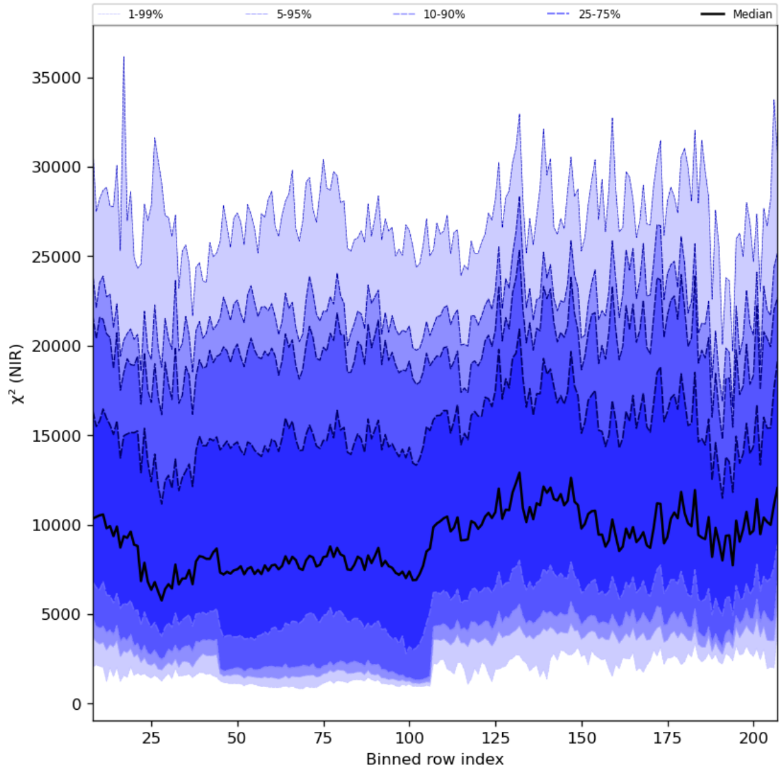
Figure 40: Along track statistics of “ \chi^2 (NIR)” for 2024-04-12 to 2024-04-14
