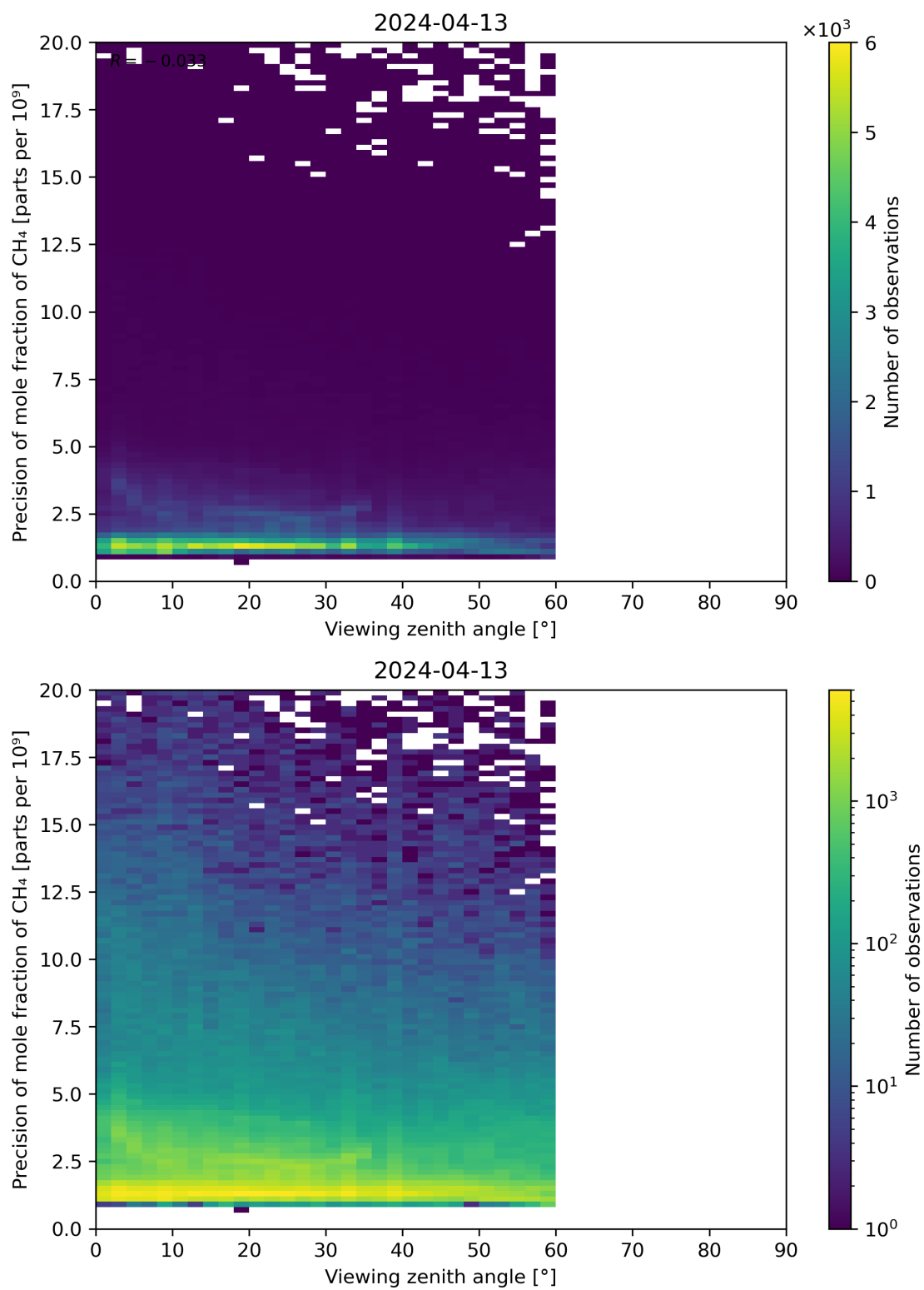
Figure 112: Scatter density plot of “Viewing zenith angle” against “Precision of mole fraction of CH 4 ” for 2024-04-12 to 2024-04-14.
