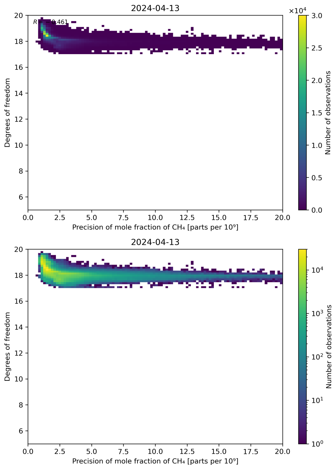
Figure 80: Scatter density plot of “Precision of mole fraction of CH 4 ” against “Degrees of freedom” for 2024-04-12 to 2024-04-14.
