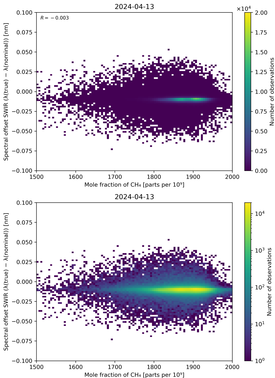
Figure 86: Scatter density plot of “Mole fraction of CH 4 ” against “Spectral offset SWIR ( \lambda(\text{true}) - \lambda(\text{nominal}) )” for 2024-04-12 to 2024-04-14.
