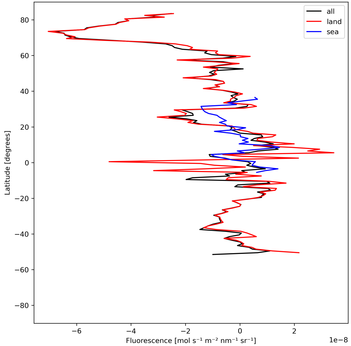
Figure 21: Zonal average of “Fluorescence” for 2024-04-12 to 2024-04-14.
