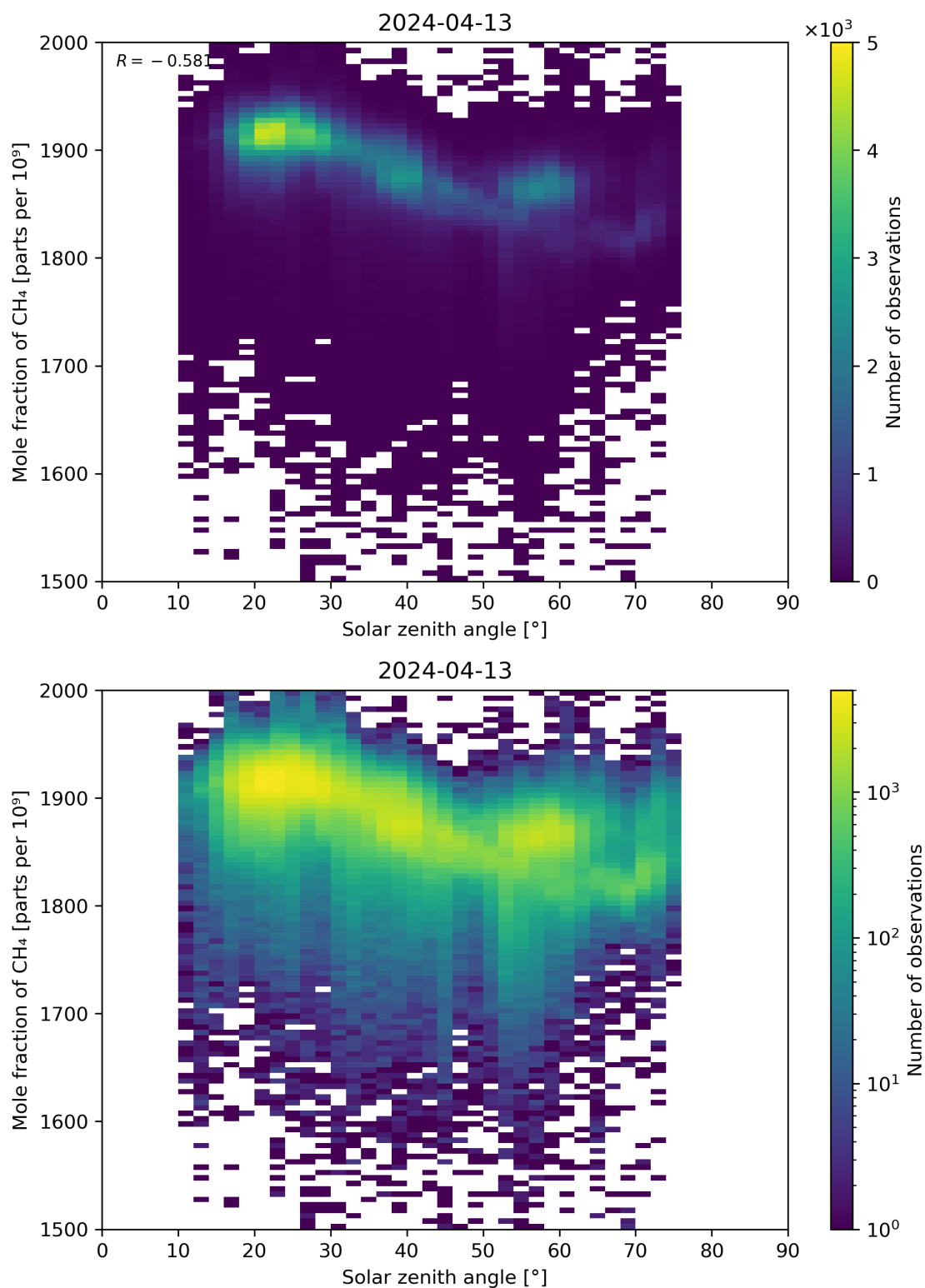
Figure 99: Scatter density plot of “Solar zenith angle” against “Mole fraction of CH 4 ” for 2024-04-12 to 2024-04-14.
