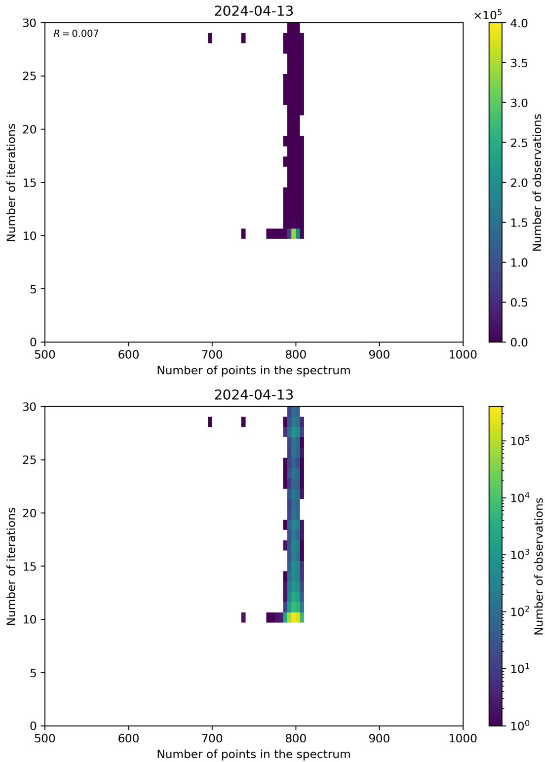
Figure 92: Scatter density plot of “Number of points in the spectrum” against “Number of iterations” for 2024-04-12 to 2024-04-14.
