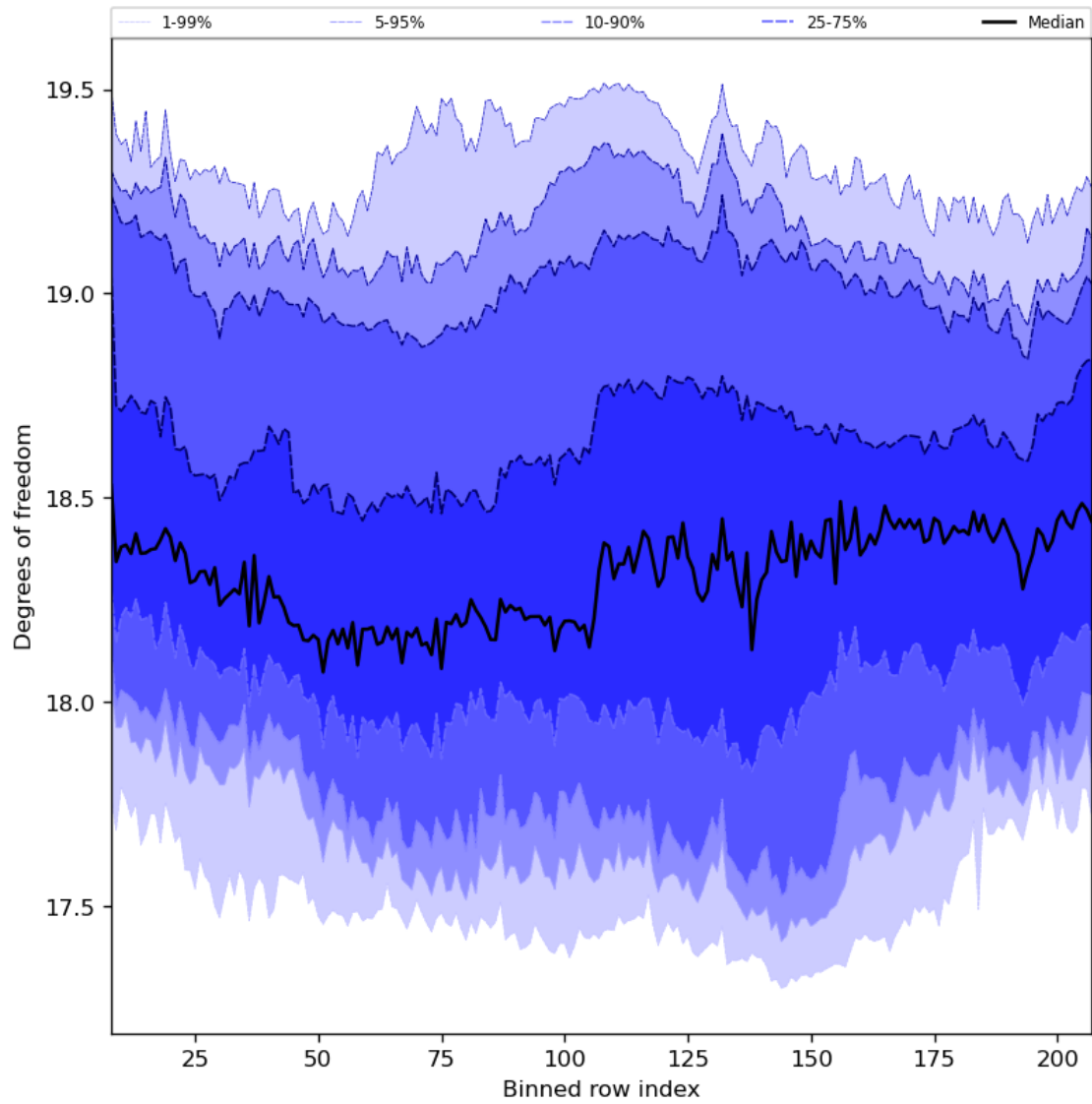
Figure 41: Along track statistics of “Degrees of freedom” for 2024-04-12 to 2024-04-14
