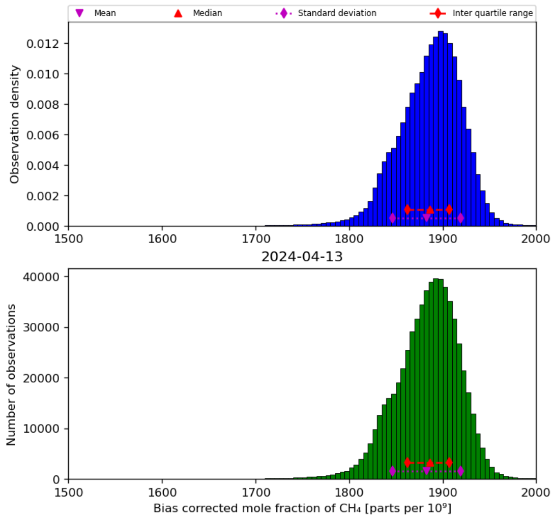
Figure 25: Histogram of “Bias corrected mole fraction of CH 4 ” for 2024-04-12 to 2024-04-14
