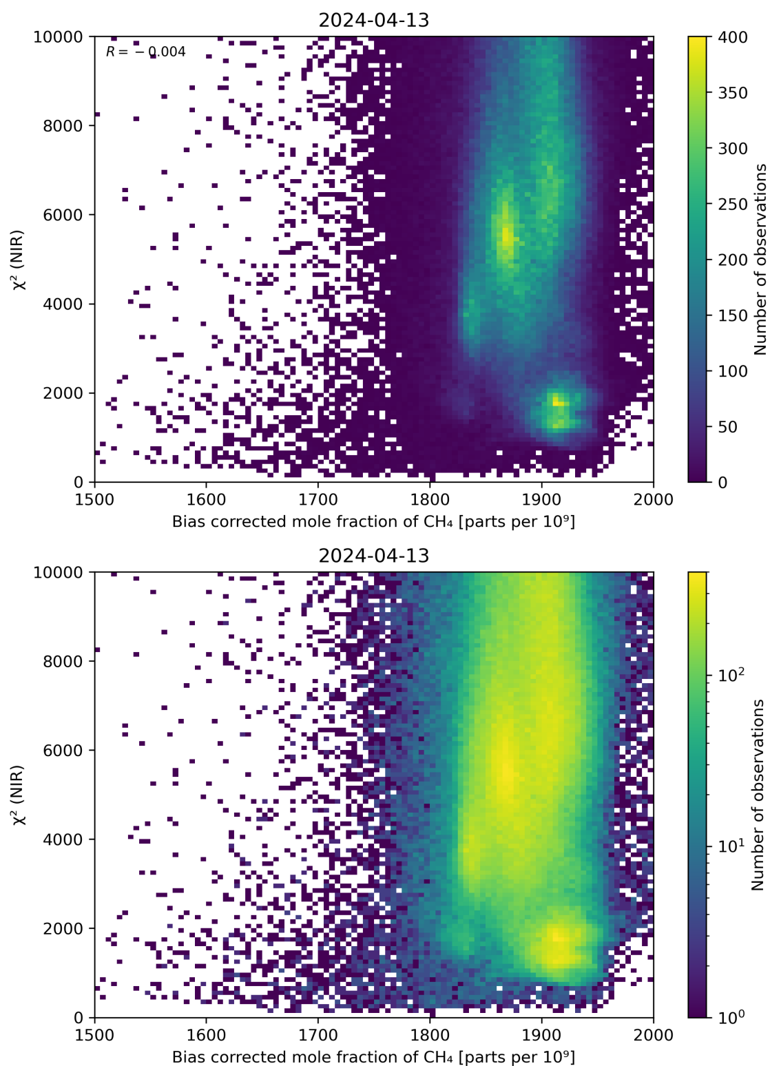
Figure 63: Scatter density plot of “Bias corrected mole fraction of CH 4 ” against “ \chi^2 (NIR)” for 2024-04-12 to 2024-04-14.
