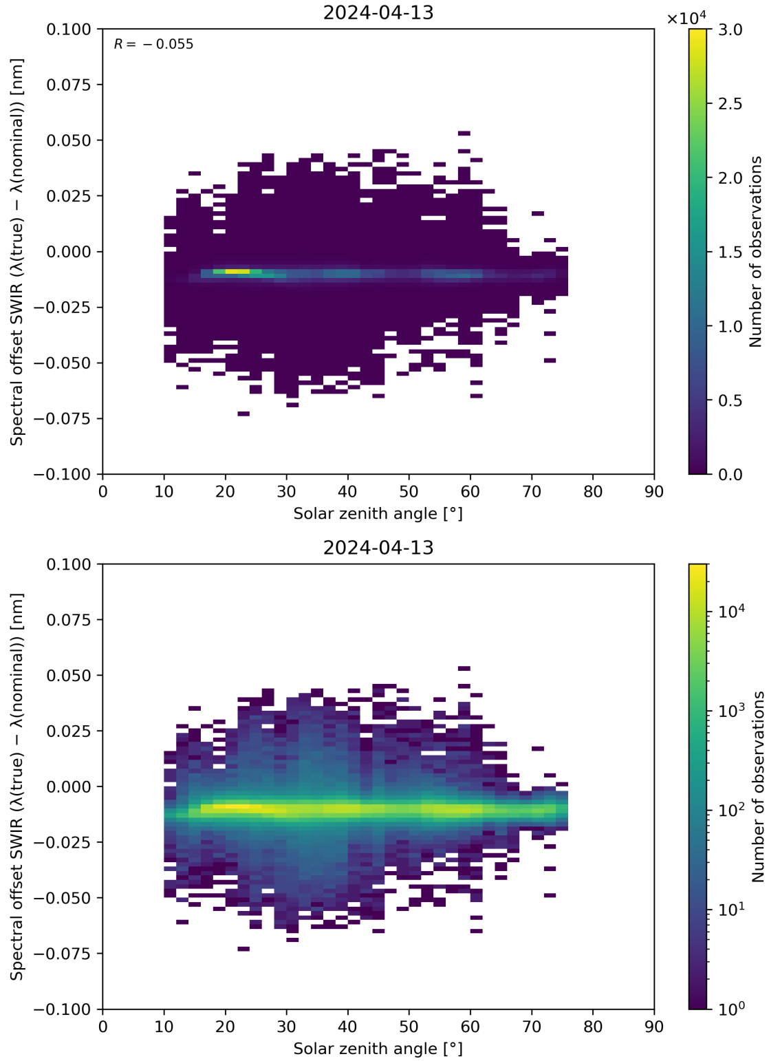
Figure 104: Scatter density plot of “Solar zenith angle” against “Spectral offset SWIR ( \lambda(\text{true}) - \lambda(\text{nominal}) )” for 2024-04-12 to 2024-04-14.
