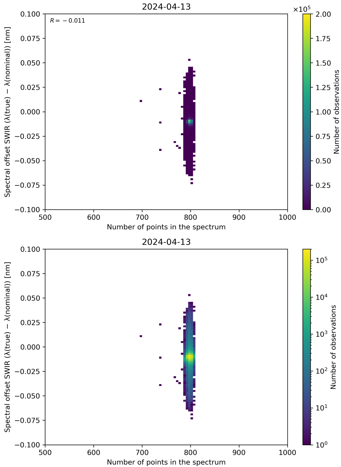
Figure 93: Scatter density plot of “Number of points in the spectrum” against “Spectral offset SWIR ( \lambda(\text{true}) - \lambda(\text{nominal}) )” for 2024-04-12 to 2024-04-14.
