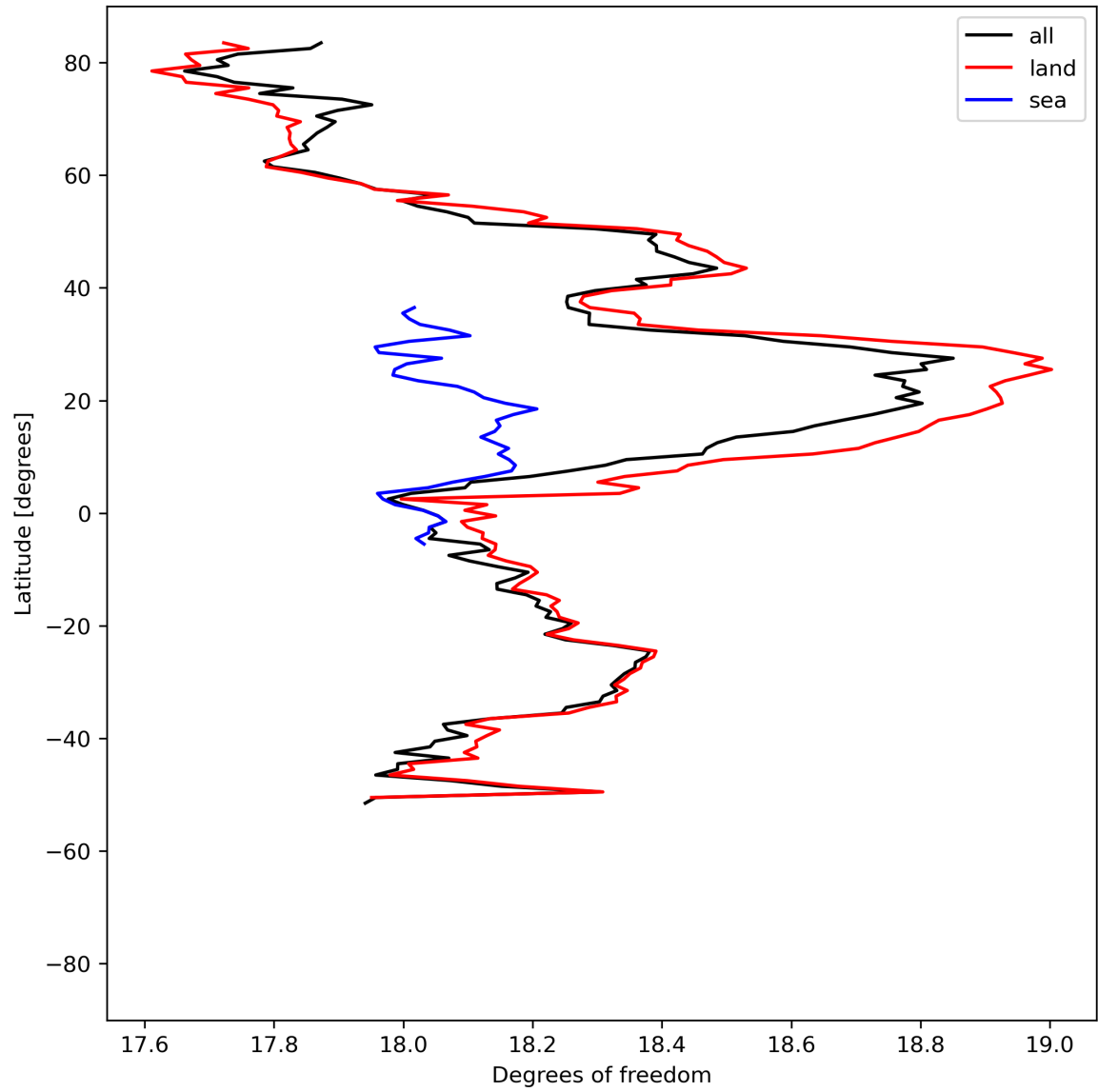
Figure 19: Zonal average of “Degrees of freedom” for 2024-04-12 to 2024-04-14.
