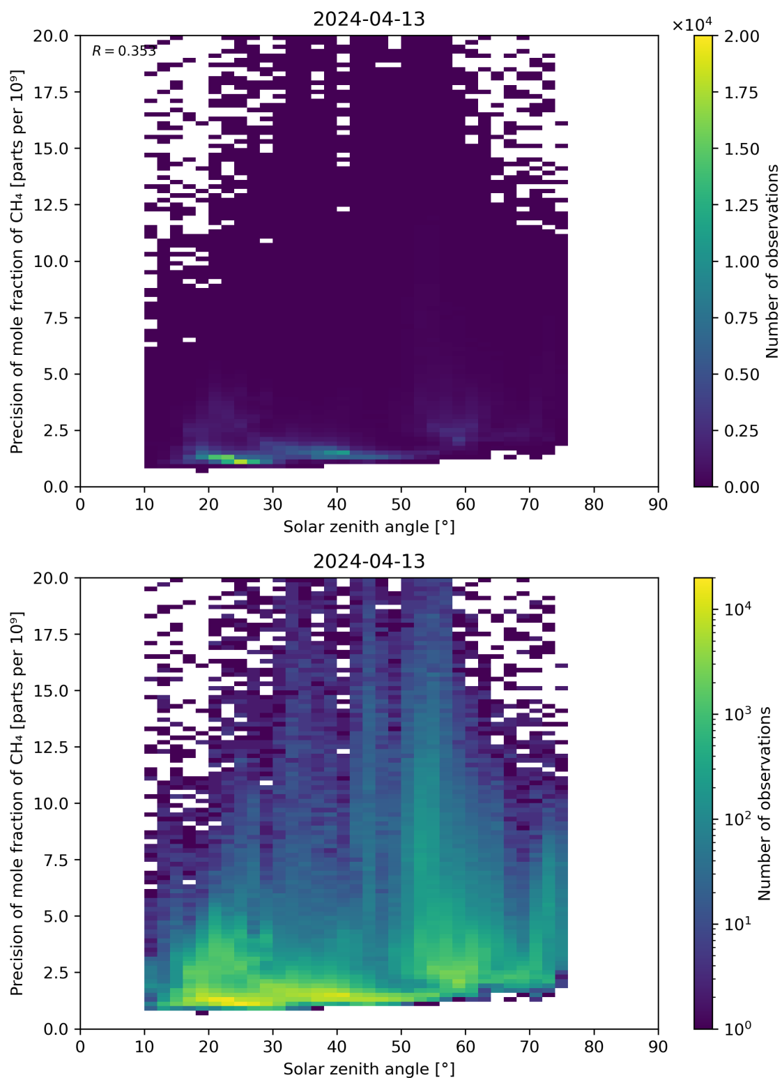
Figure 101: Scatter density plot of “Solar zenith angle” against “Precision of mole fraction of CH 4 ” for 2024-04-12 to 2024-04-14.
