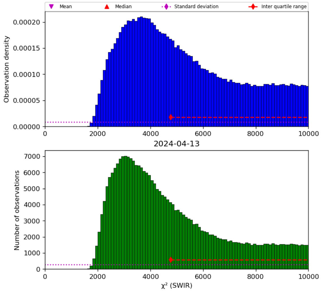
Figure 28: Histogram of “ \chi^2 (SWIR)” for 2024-04-12 to 2024-04-14
