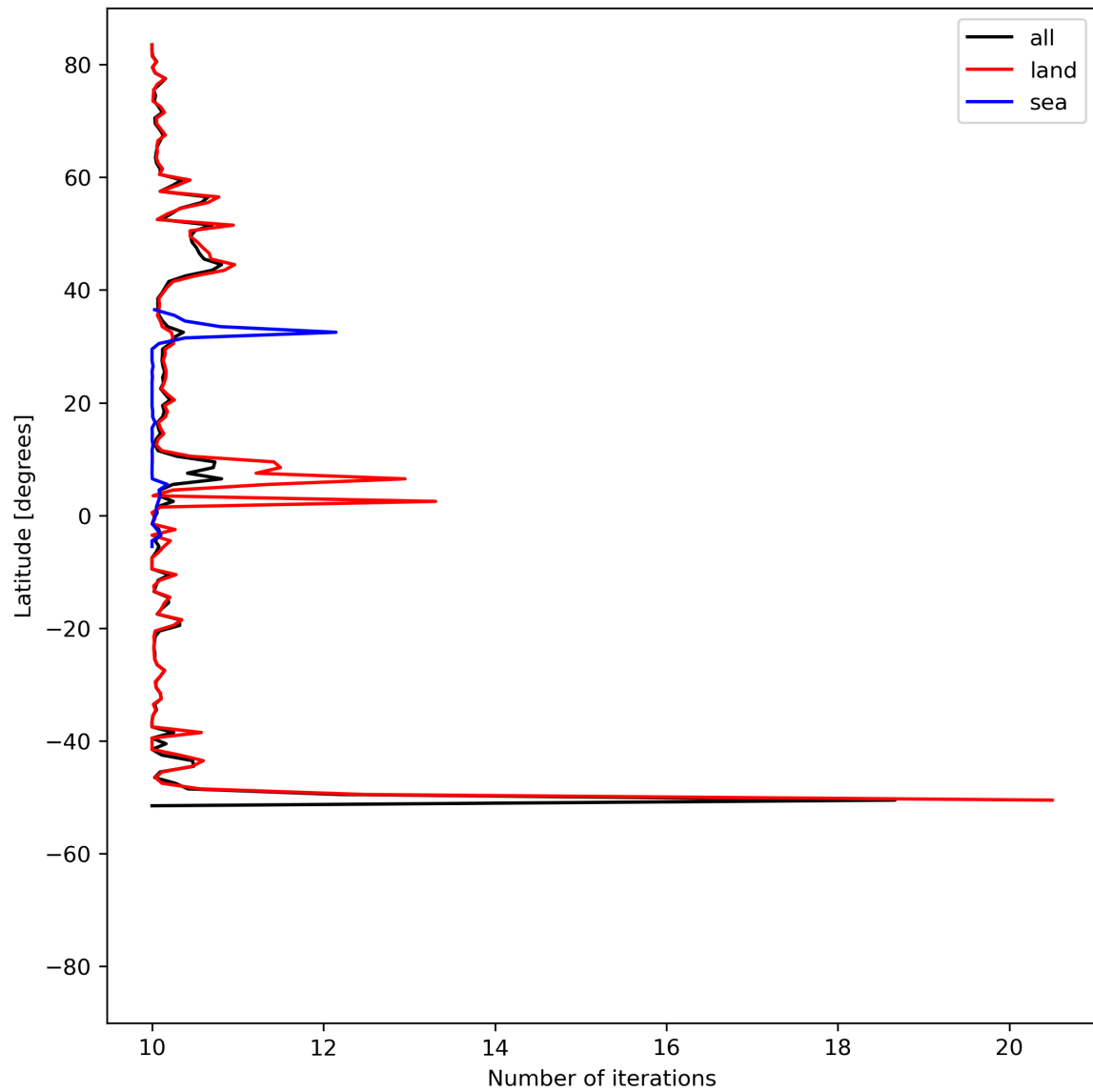
Figure 20: Zonal average of “Number of iterations” for 2024-04-12 to 2024-04-14.
