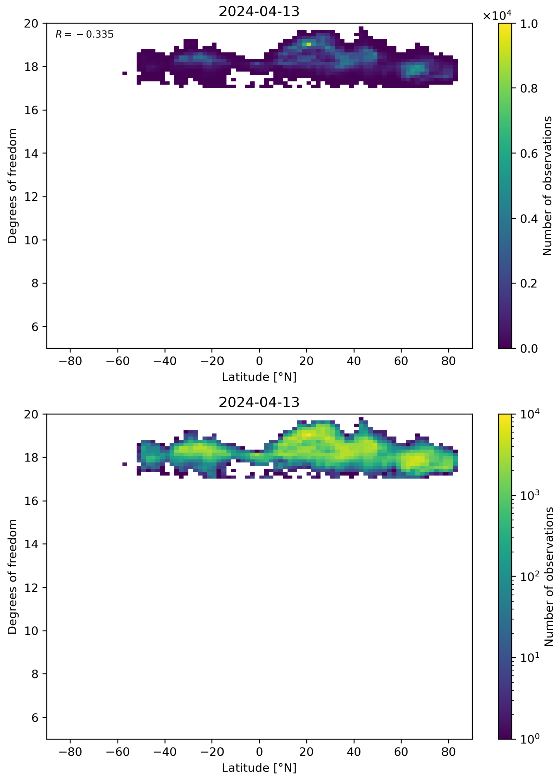
Figure 55: Scatter density plot of “Latitude” against “Degrees of freedom” for 2024-04-12 to 2024-04-14.
