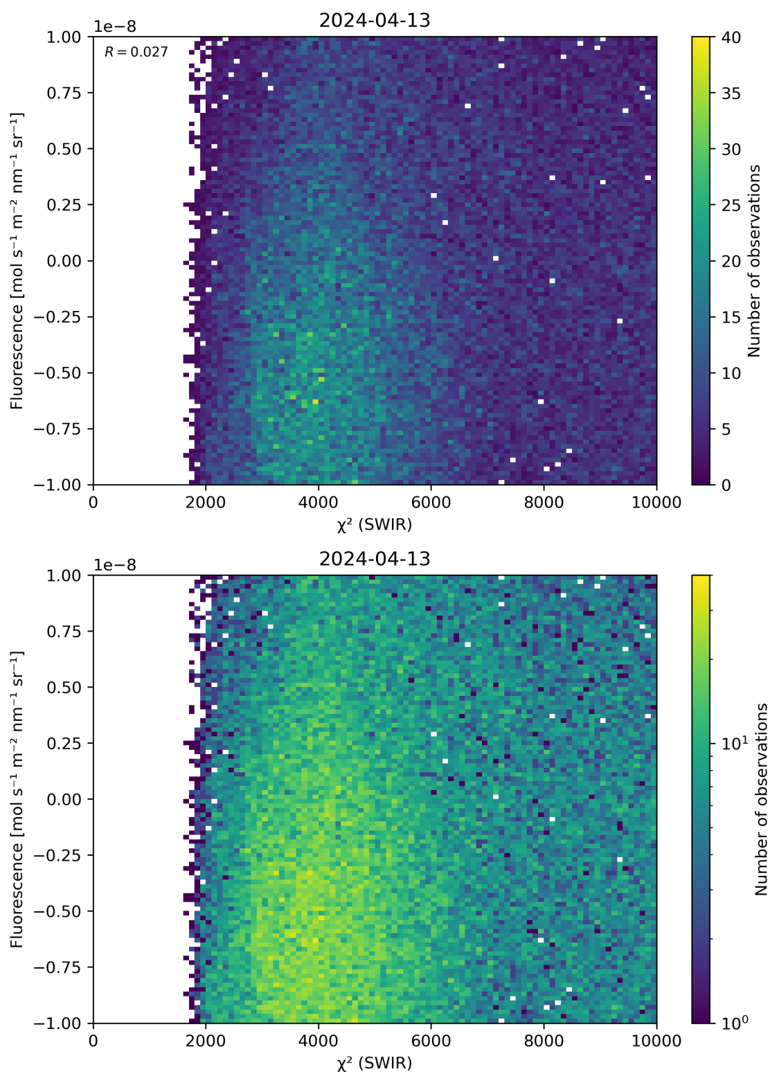
Figure 49: Scatter density plot of “ \chi^2 (SWIR)” against “Fluorescence” for 2024-04-12 to 2024-04-14.
