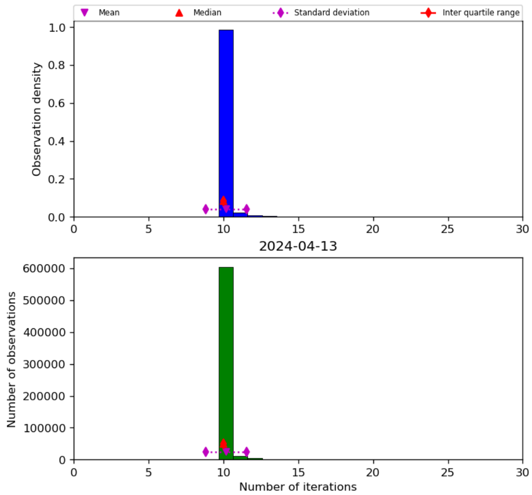
Figure 31: Histogram of “Number of iterations” for 2024-04-12 to 2024-04-14
