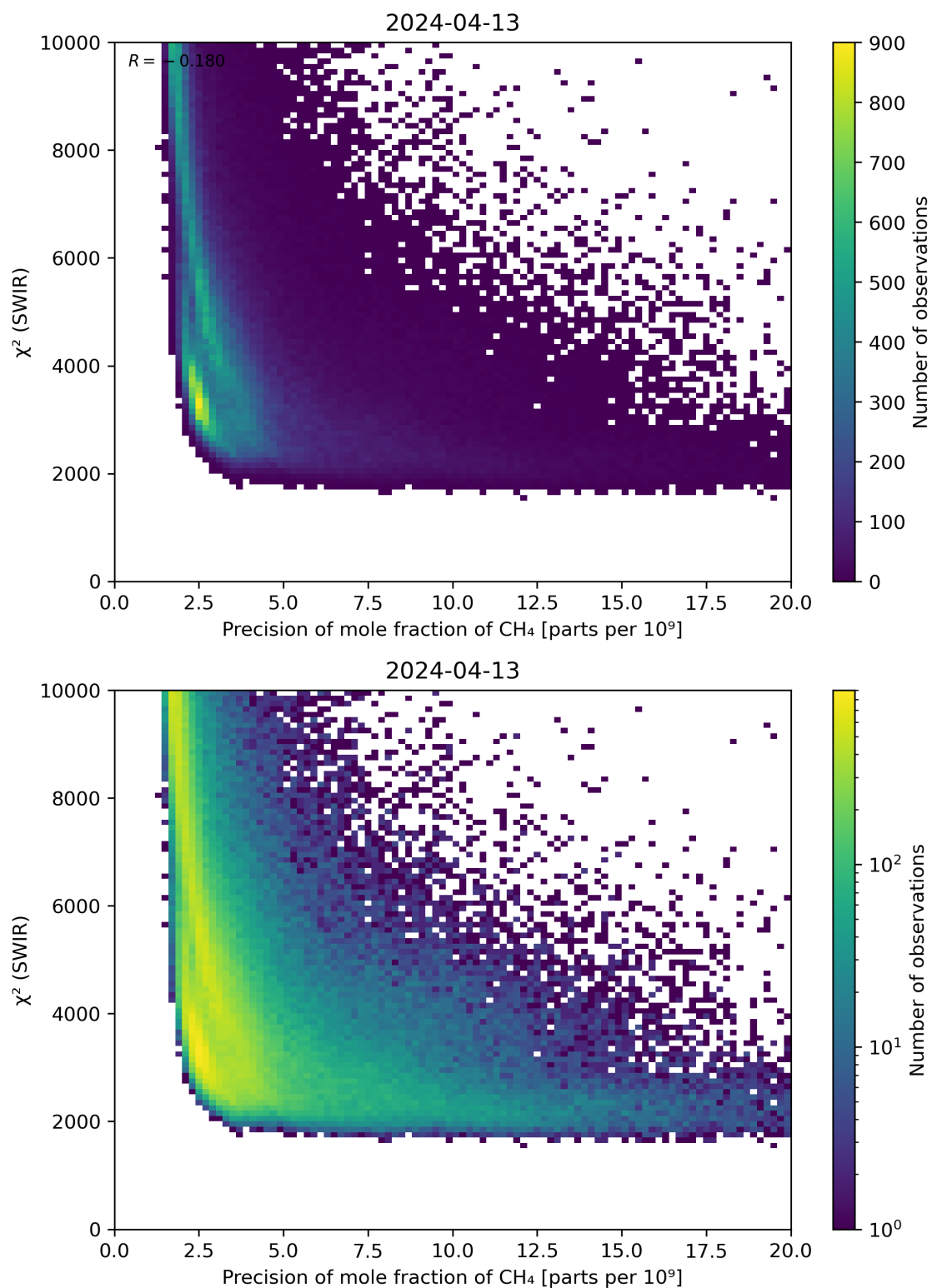
Figure 79: Scatter density plot of “Precision of mole fraction of \text{CH}_4 ” against “ \chi^2 (SWIR)” for 2024-04-12 to 2024-04-14.
