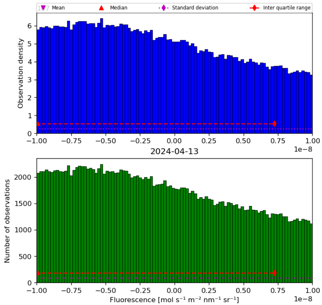
Figure 32: Histogram of “Fluorescence” for 2024-04-12 to 2024-04-14
