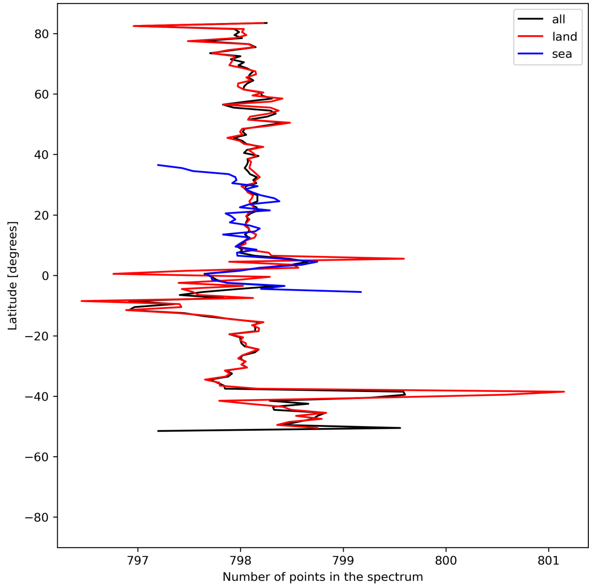
Figure 15: Zonal average of “Number of points in the spectrum” for 2024-04-12 to 2024-04-14.
