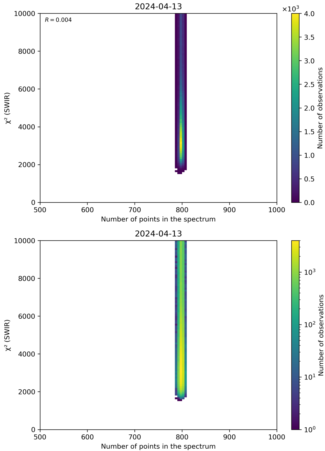
Figure 89: Scatter density plot of “Number of points in the spectrum” against “ \chi^2 (SWIR)” for 2024-04-12 to 2024-04-14.
