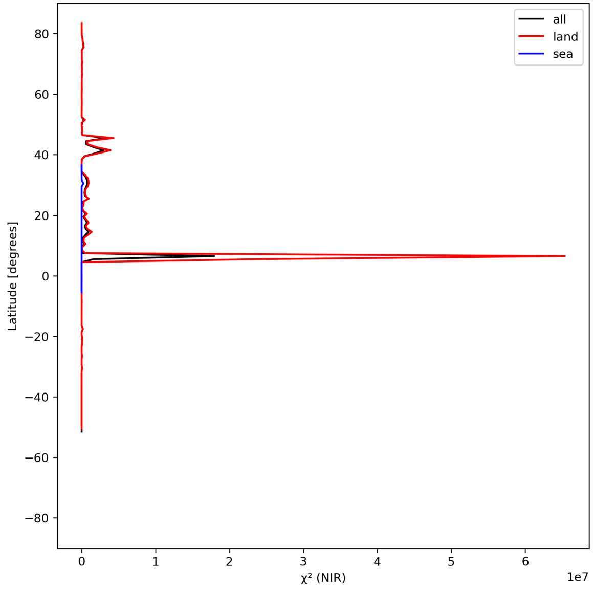
Figure 18: Zonal average of “ \chi^2 (NIR)” for 2024-04-12 to 2024-04-14.
