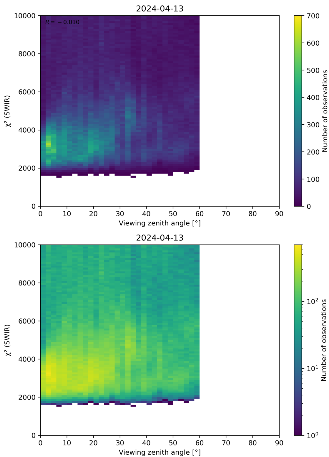
Figure 106: Scatter density plot of “Viewing zenith angle” against “ \chi^2 (SWIR)” for 2024-04-12 to 2024-04-14.
