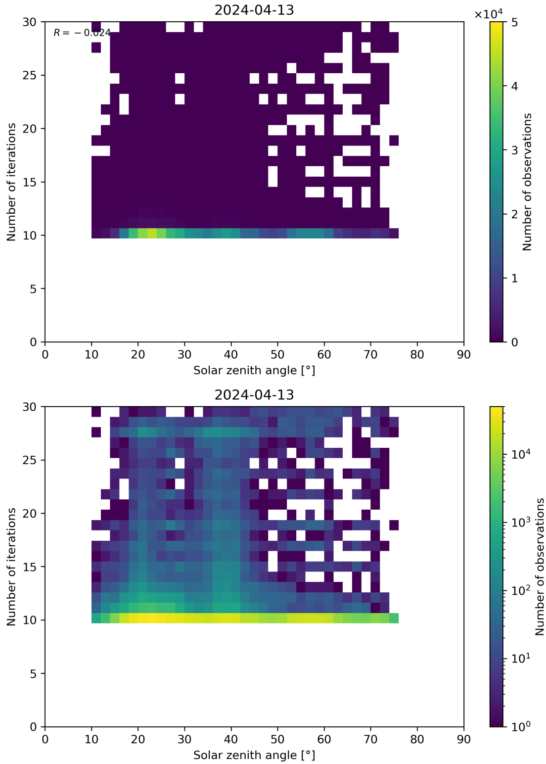
Figure 102: Scatter density plot of “Solar zenith angle” against “Number of iterations” for 2024-04-12 to 2024-04-14.
