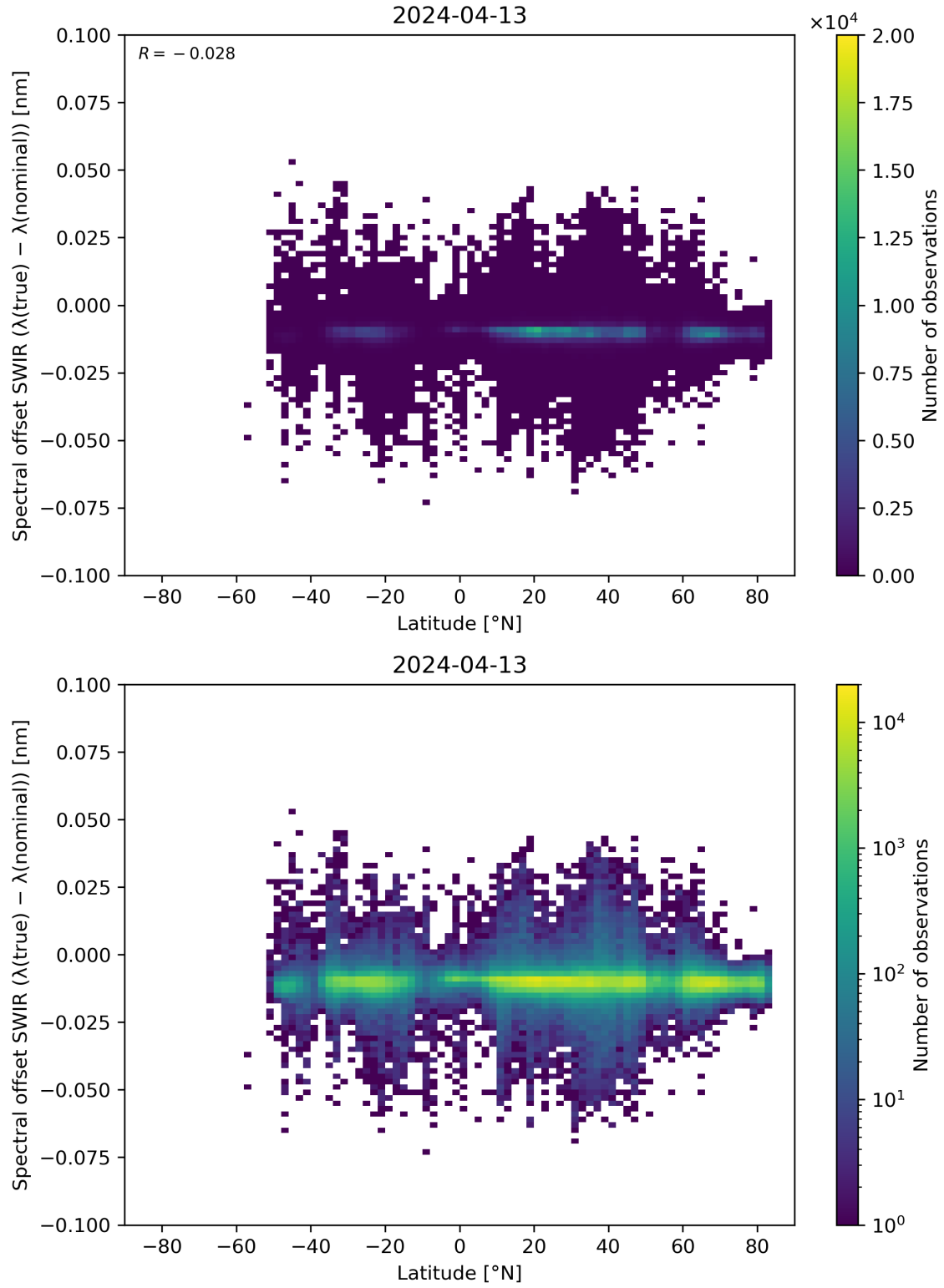
Figure 62: Scatter density plot of “Latitude” against “Spectral offset SWIR ( \lambda(\text{true}) - \lambda(\text{nominal}) )” for 2024-04-12 to 2024-04-14.
