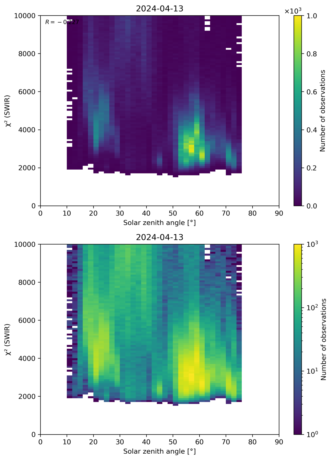
Figure 95: Scatter density plot of “Solar zenith angle” against “ \chi^2 (SWIR)” for 2024-04-12 to 2024-04-14.
