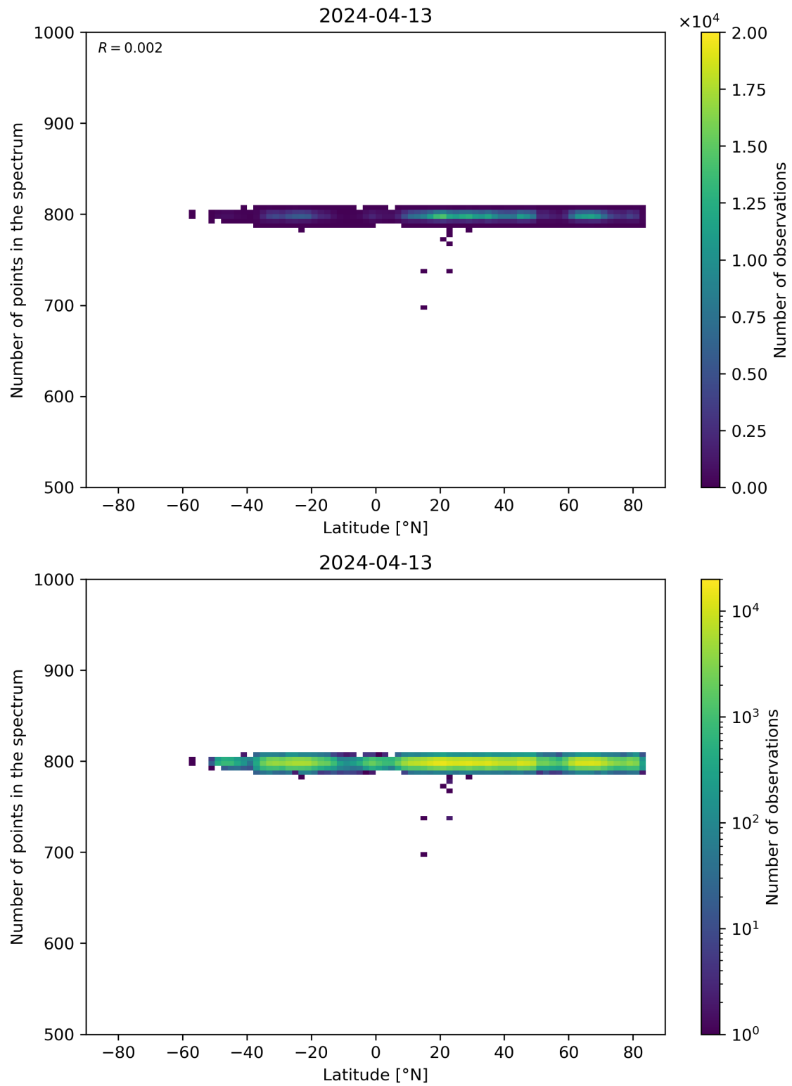
Figure 61: Scatter density plot of “Latitude” against “Number of points in the spectrum” for 2024-04-12 to 2024-04-14.
