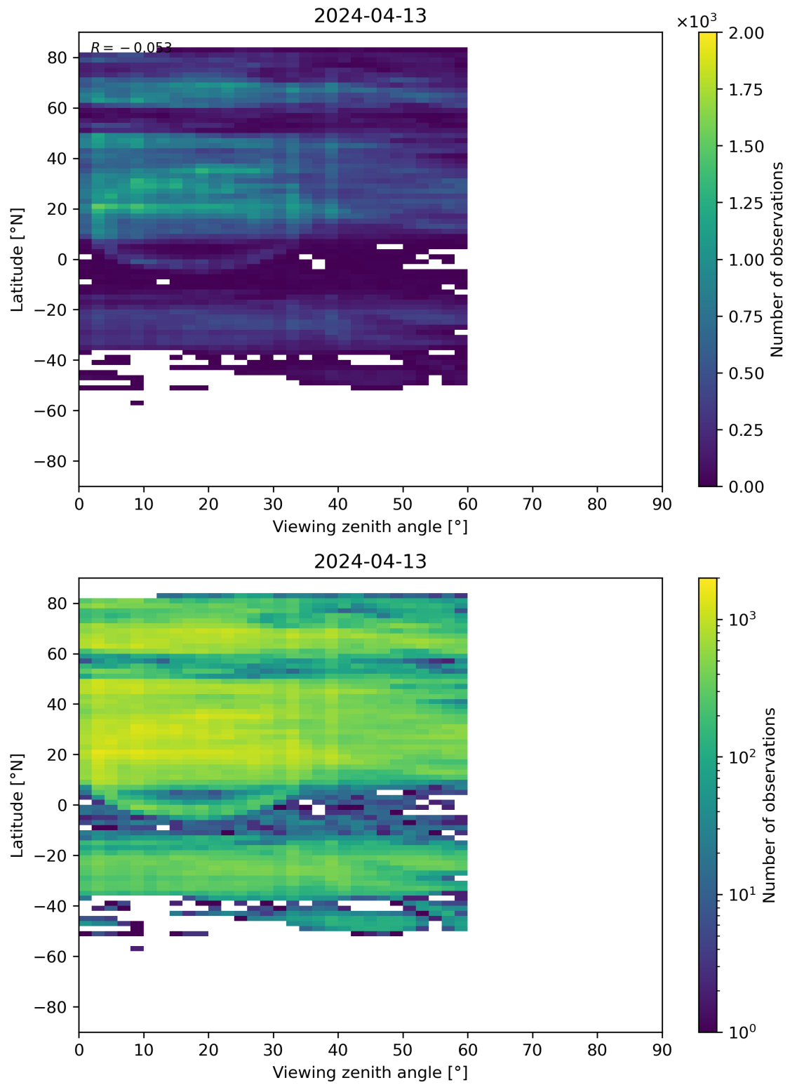
Figure 109: Scatter density plot of “Viewing zenith angle” against “Latitude” for 2024-04-12 to 2024-04-14.
