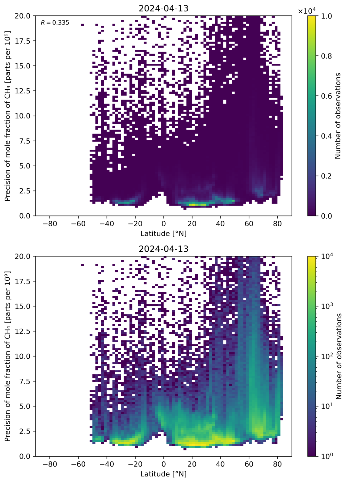
Figure 59: Scatter density plot of “Latitude” against “Precision of mole fraction of \text{CH}_4 ” for 2024-04-12 to 2024-04-14.
