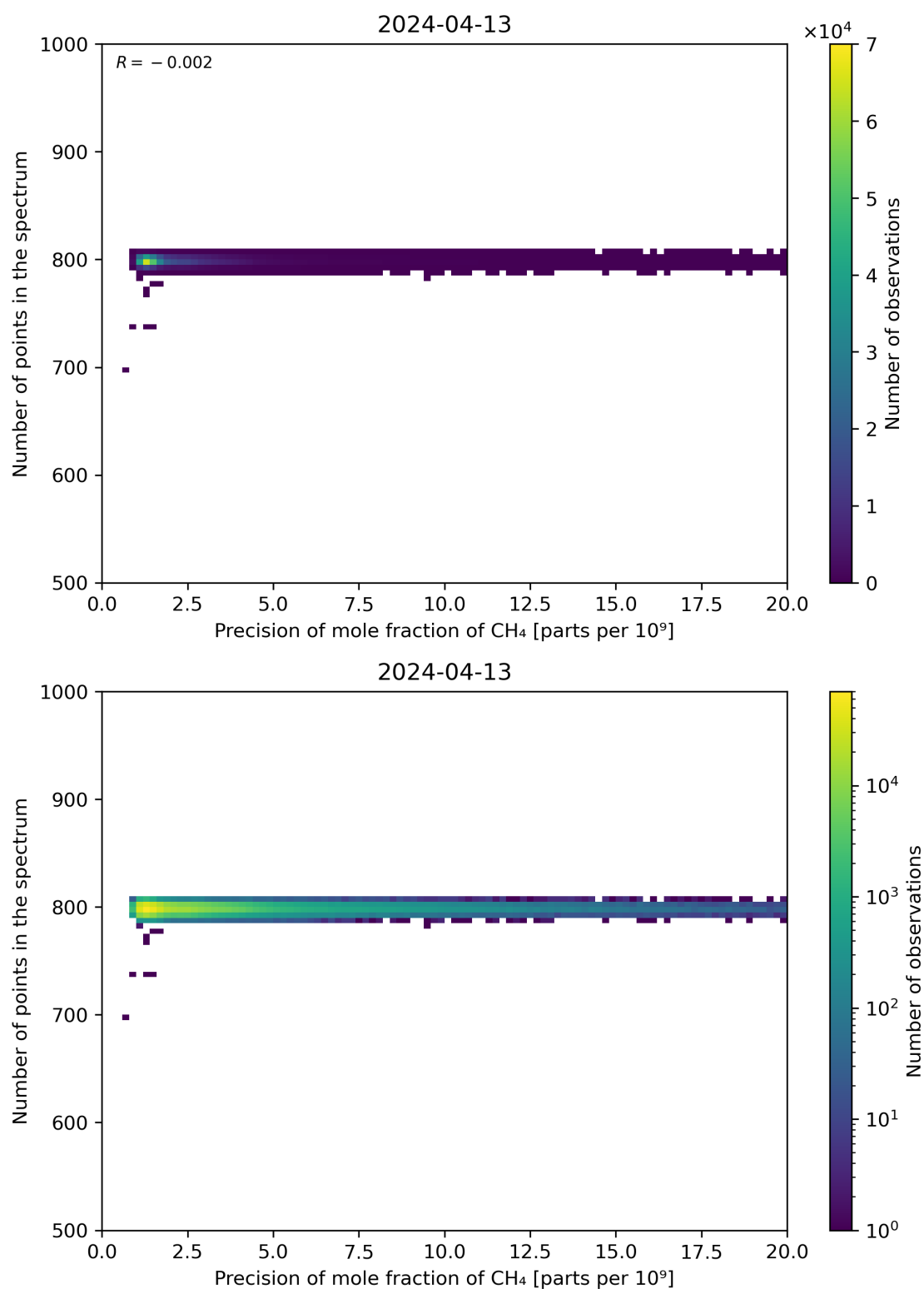
Figure 84: Scatter density plot of “Precision of mole fraction of CH 4 ” against “Number of points in the spectrum” for 2024-04-12 to 2024-04-14.
