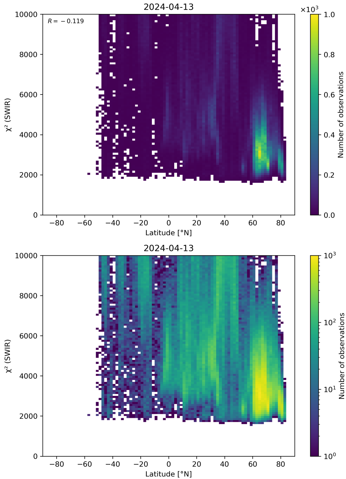
Figure 54: Scatter density plot of “Latitude” against “ \chi^2 (SWIR)” for 2024-04-12 to 2024-04-14.
