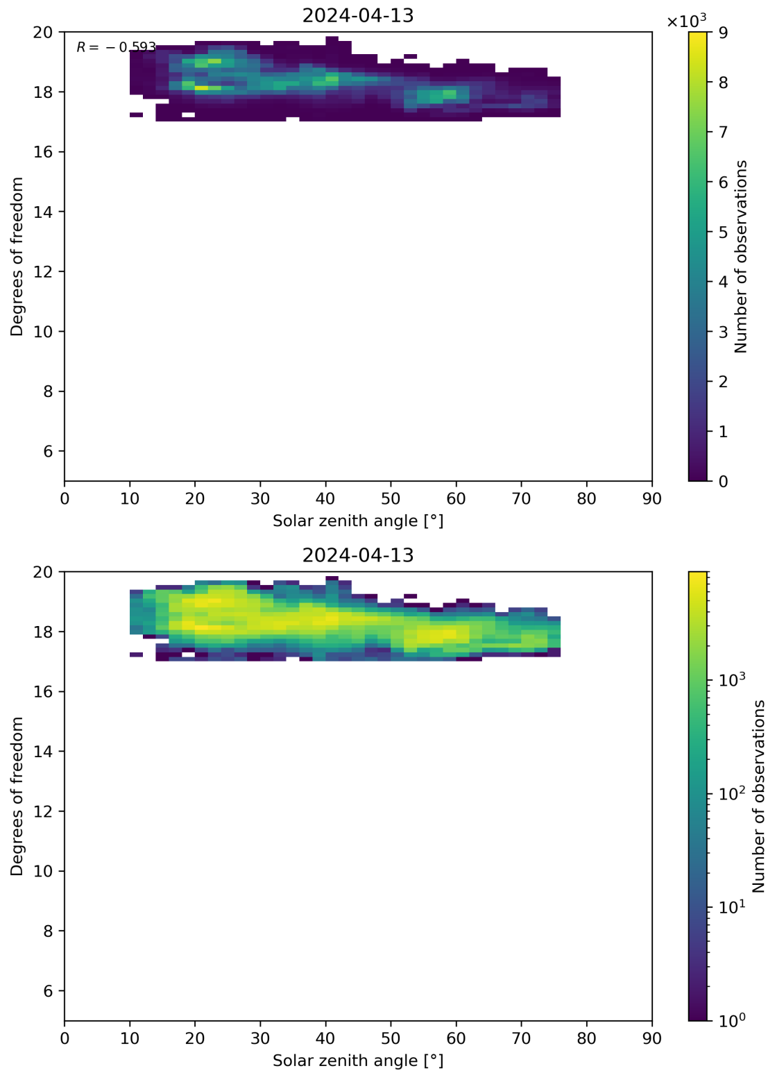
Figure 96: Scatter density plot of “Solar zenith angle” against “Degrees of freedom” for 2024-04-12 to 2024-04-14.
