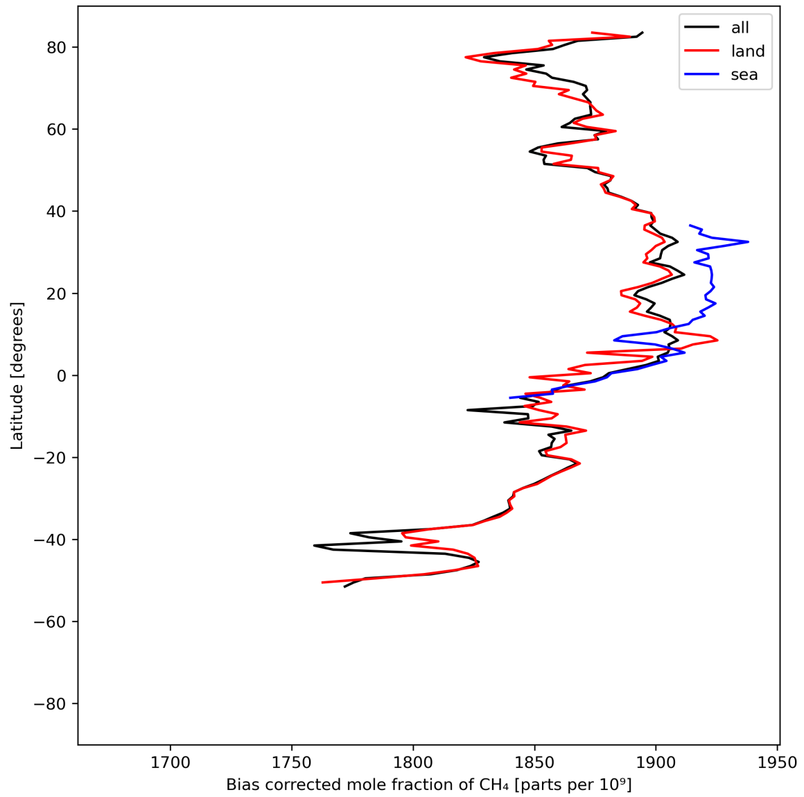
Figure 14: Zonal average of “Bias corrected mole fraction of \text{CH}_4 ” for 2024-04-12 to 2024-04-14.
