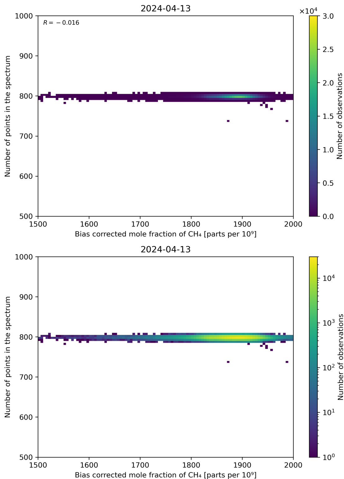
Figure 68: Scatter density plot of “Bias corrected mole fraction of CH 4 ” against “Number of points in the spectrum” for 2024-04-12 to 2024-04-14.
