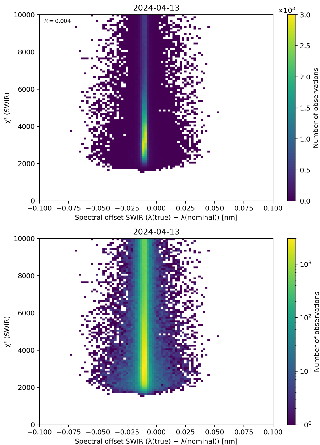
Figure 118: Scatter density plot of “Spectral offset SWIR ( \lambda(\text{true}) - \lambda(\text{nominal}) )” against “ \chi^2 (SWIR)” for 2024-04-12 to 2024-04-14.
