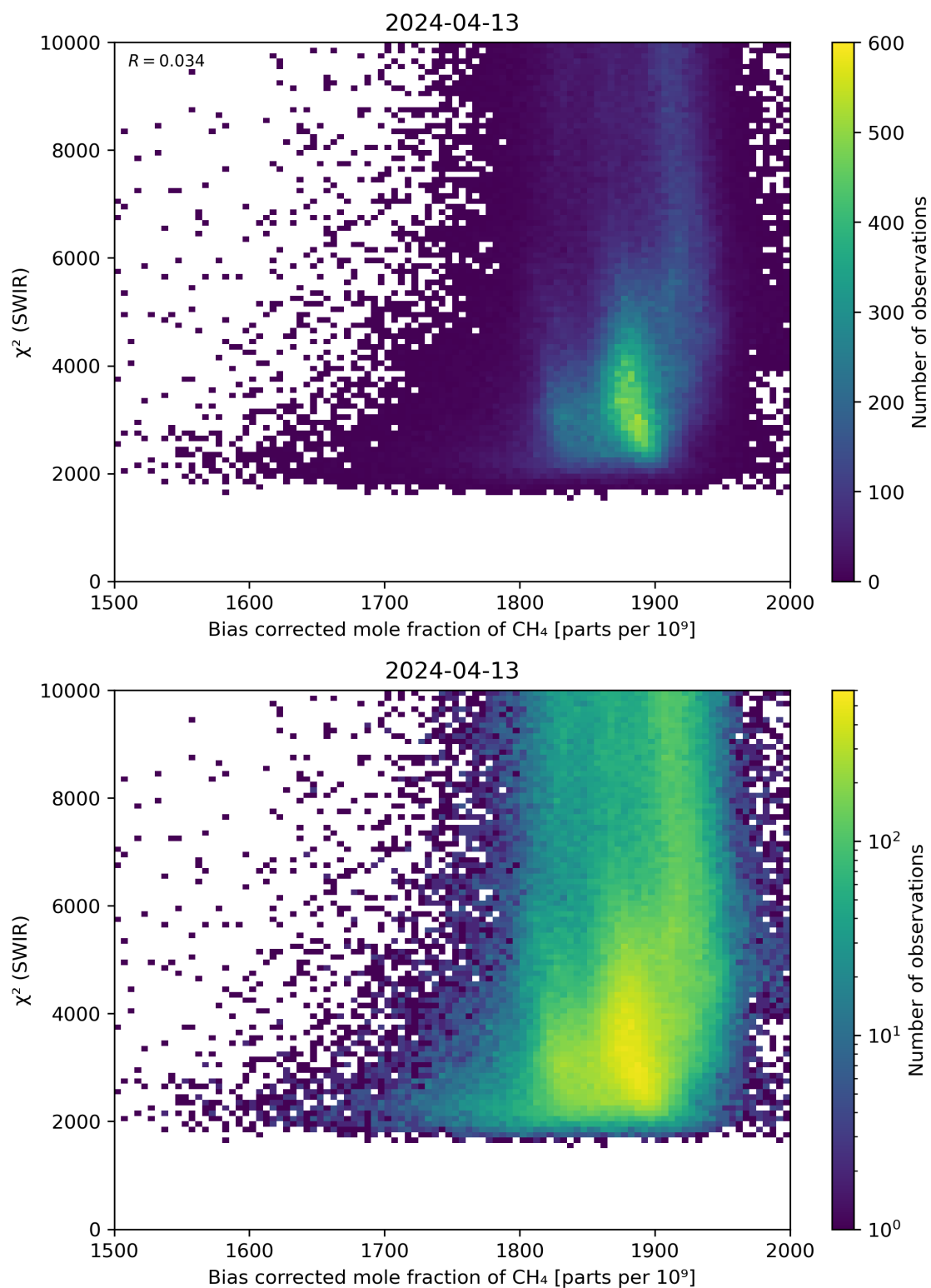
Figure 64: Scatter density plot of “Bias corrected mole fraction of \text{CH}_4 ” against “ \chi^2 (SWIR)” for 2024-04-12 to 2024-04-14.
