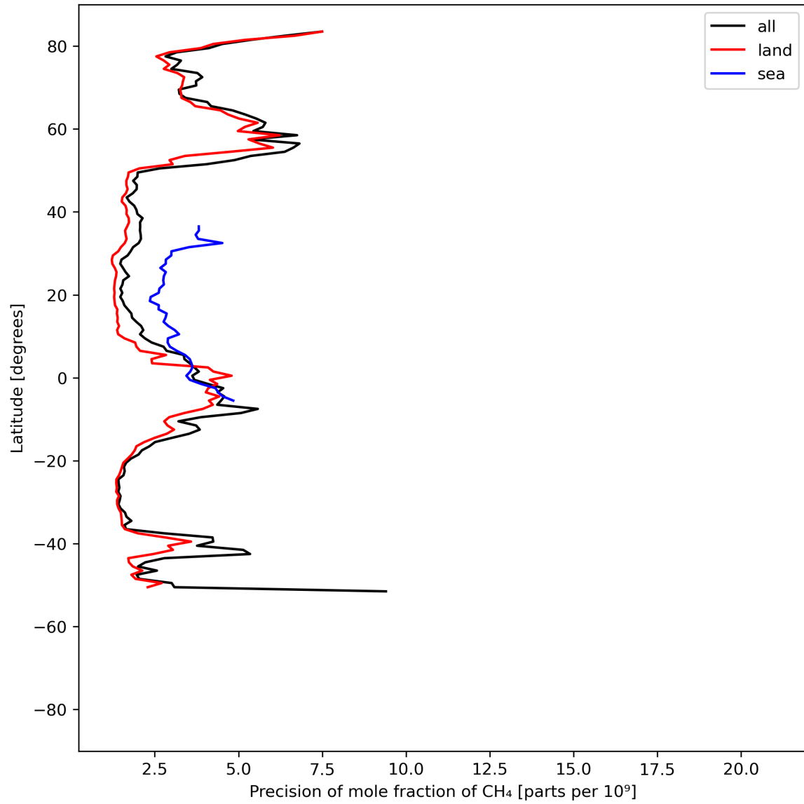
Figure 13: Zonal average of “Precision of mole fraction of CH 4 ” for 2024-04-12 to 2024-04-14.
