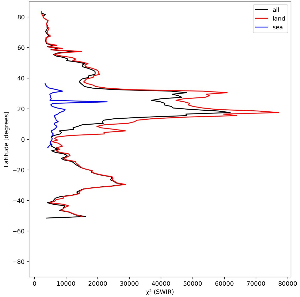
Figure 17: Zonal average of “ \chi^2 (SWIR)” for 2024-04-12 to 2024-04-14.
