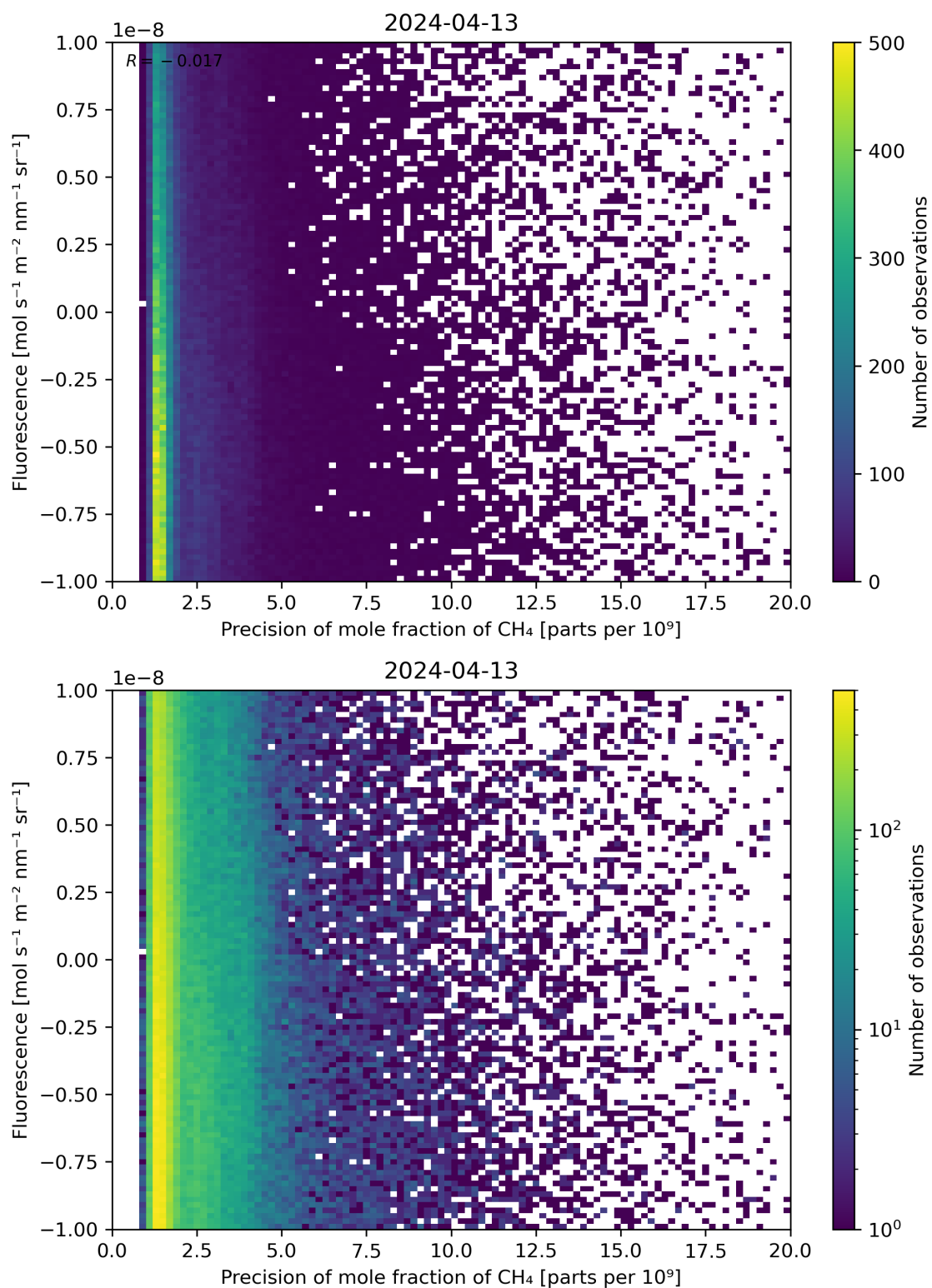
Figure 81: Scatter density plot of “Precision of mole fraction of \text{CH}_4 ” against “Fluorescence” for 2024-04-12 to 2024-04-14.
