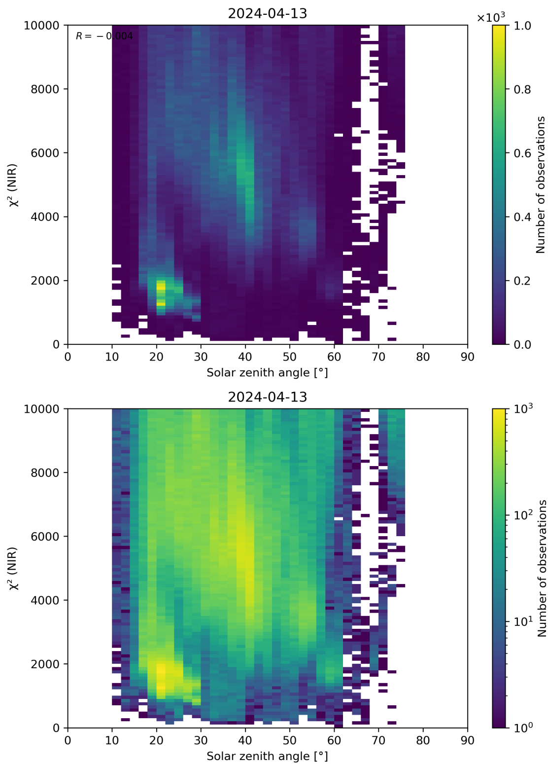
Figure 94: Scatter density plot of “Solar zenith angle” against “ \chi^2 (NIR)” for 2024-04-12 to 2024-04-14.
