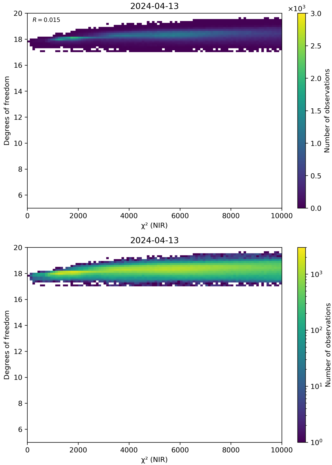
Figure 44: Scatter density plot of “ \chi^2 (NIR)” against “Degrees of freedom” for 2024-04-12 to 2024-04-14.
