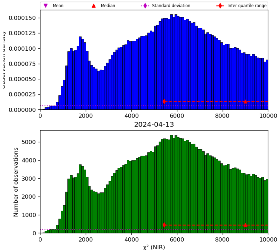
Figure 29: Histogram of “ \chi^2 (NIR)” for 2024-04-12 to 2024-04-14
