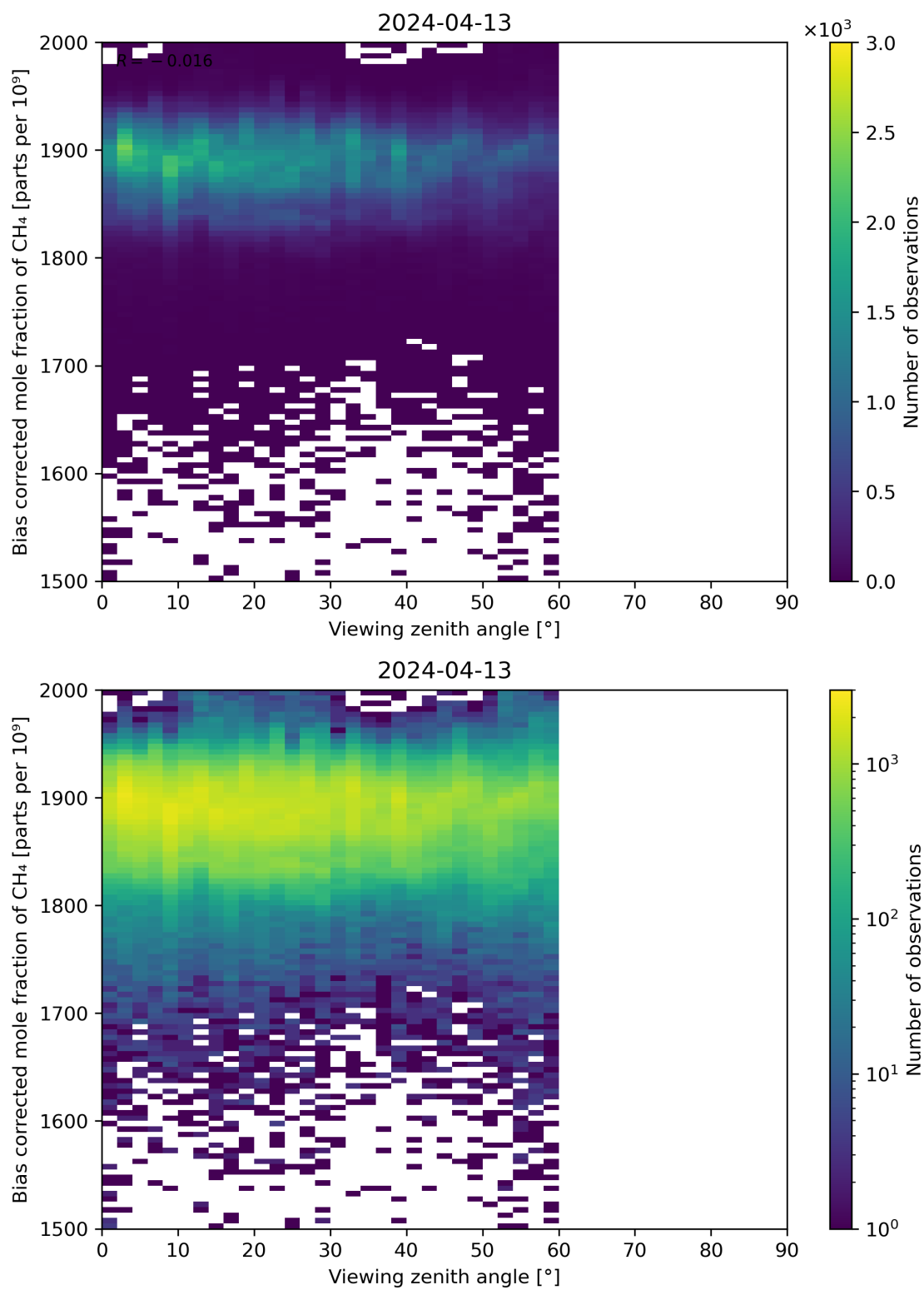
Figure 111: Scatter density plot of “Viewing zenith angle” against “Bias corrected mole fraction of CH 4 ” for 2024-04-12 to 2024-04-14.
