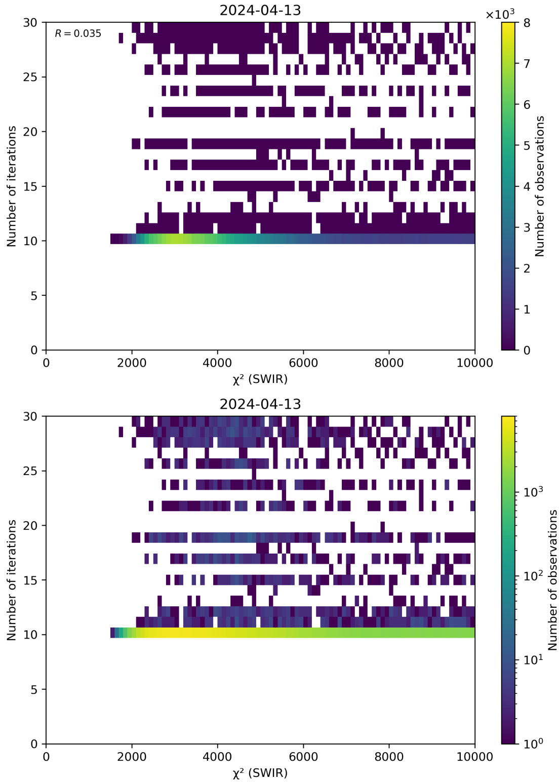
Figure 50: Scatter density plot of “ \chi^2 (SWIR)” against “Number of iterations” for 2024-04-12 to 2024-04-14.
