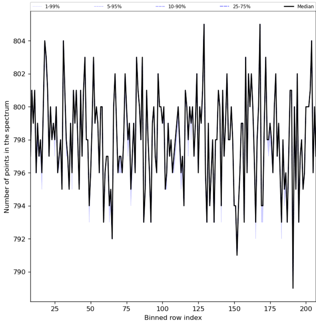
Figure 37: Along track statistics of “Number of points in the spectrum” for 2024-04-12 to 2024-04-14
