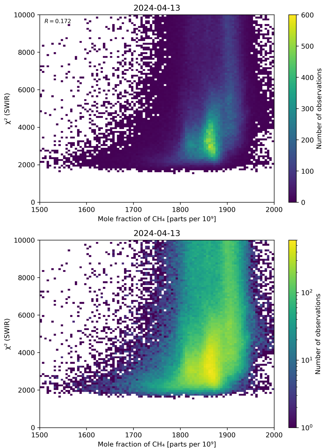
Figure 71: Scatter density plot of “Mole fraction of CH 4 ” against “ \chi^2 (SWIR)” for 2024-04-12 to 2024-04-14.
