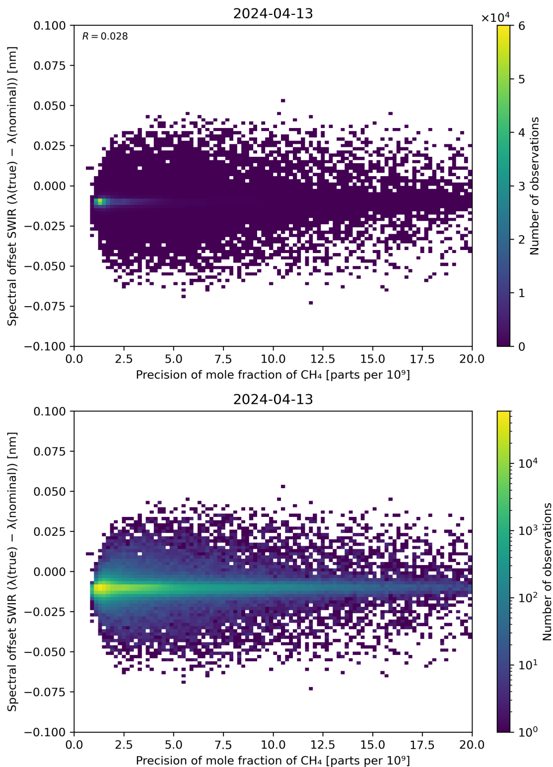
Figure 85: Scatter density plot of “Precision of mole fraction of CH 4 ” against “Spectral offset SWIR ( \lambda(\text{true}) - \lambda(\text{nominal}) )” for 2024-04-12 to 2024-04-14.
