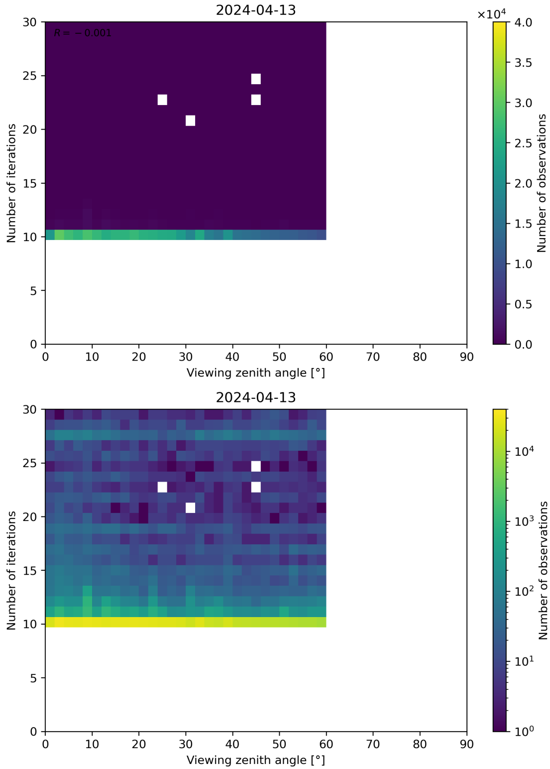
Figure 113: Scatter density plot of “Viewing zenith angle” against “Number of iterations” for 2024-04-12 to 2024-04-14.
