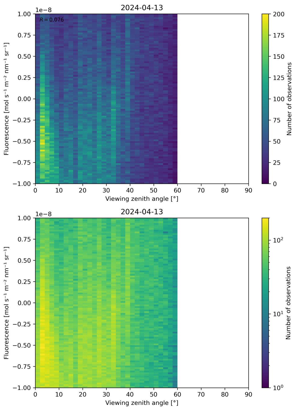
Figure 108: Scatter density plot of “Viewing zenith angle” against “Fluorescence” for 2024-04-12 to 2024-04-14.
