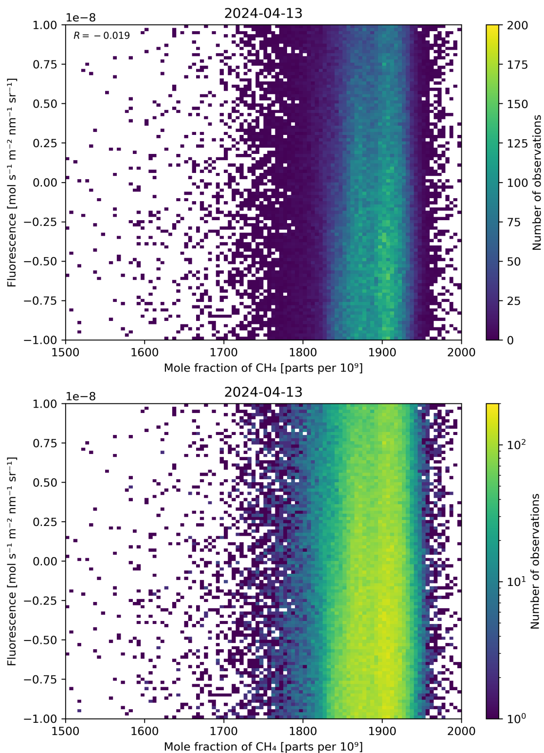
Figure 73: Scatter density plot of “Mole fraction of \text{CH}_4 ” against “Fluorescence” for 2024-04-12 to 2024-04-14.
