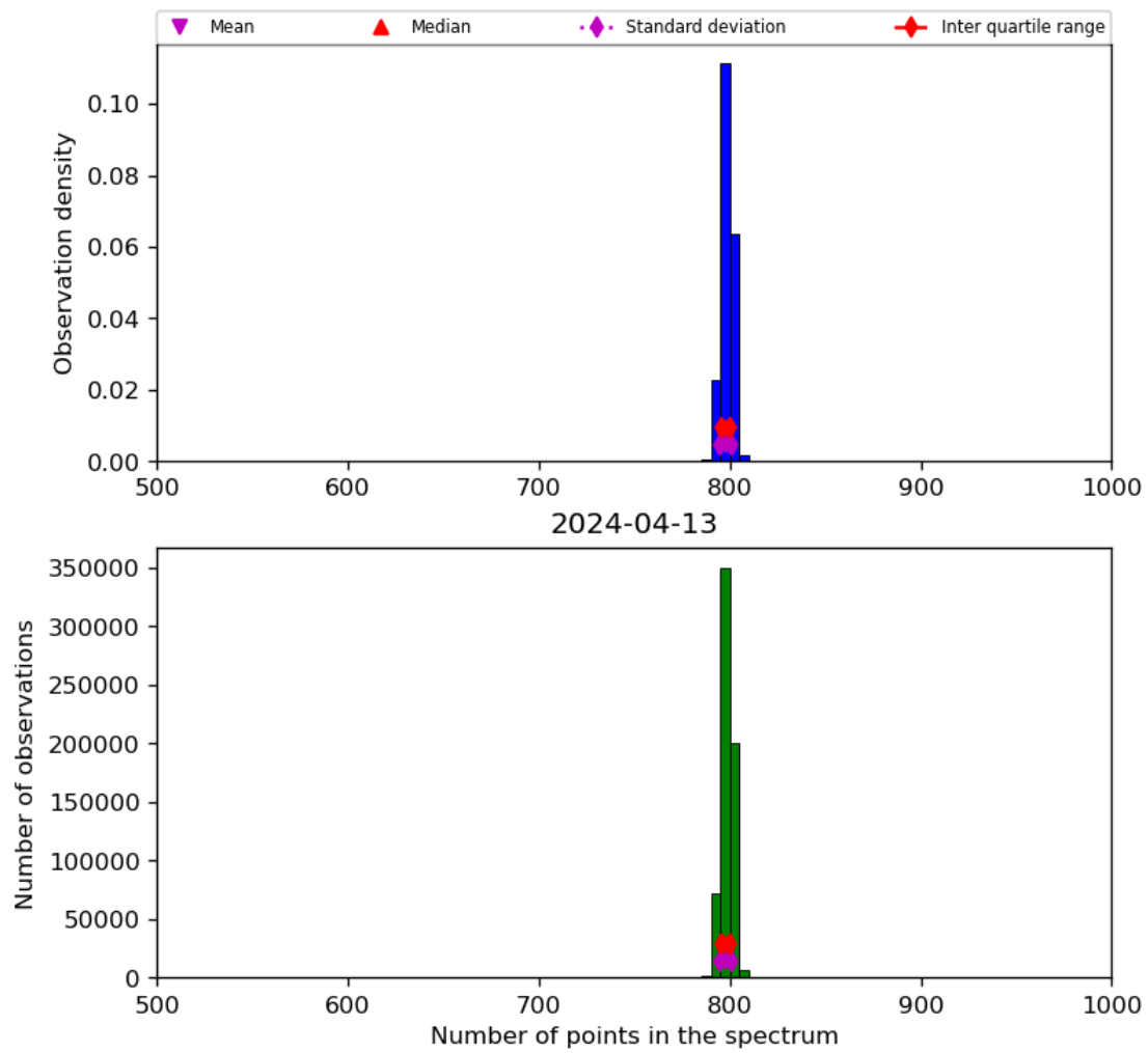
Figure 26: Histogram of “Number of points in the spectrum” for 2024-04-12 to 2024-04-14
