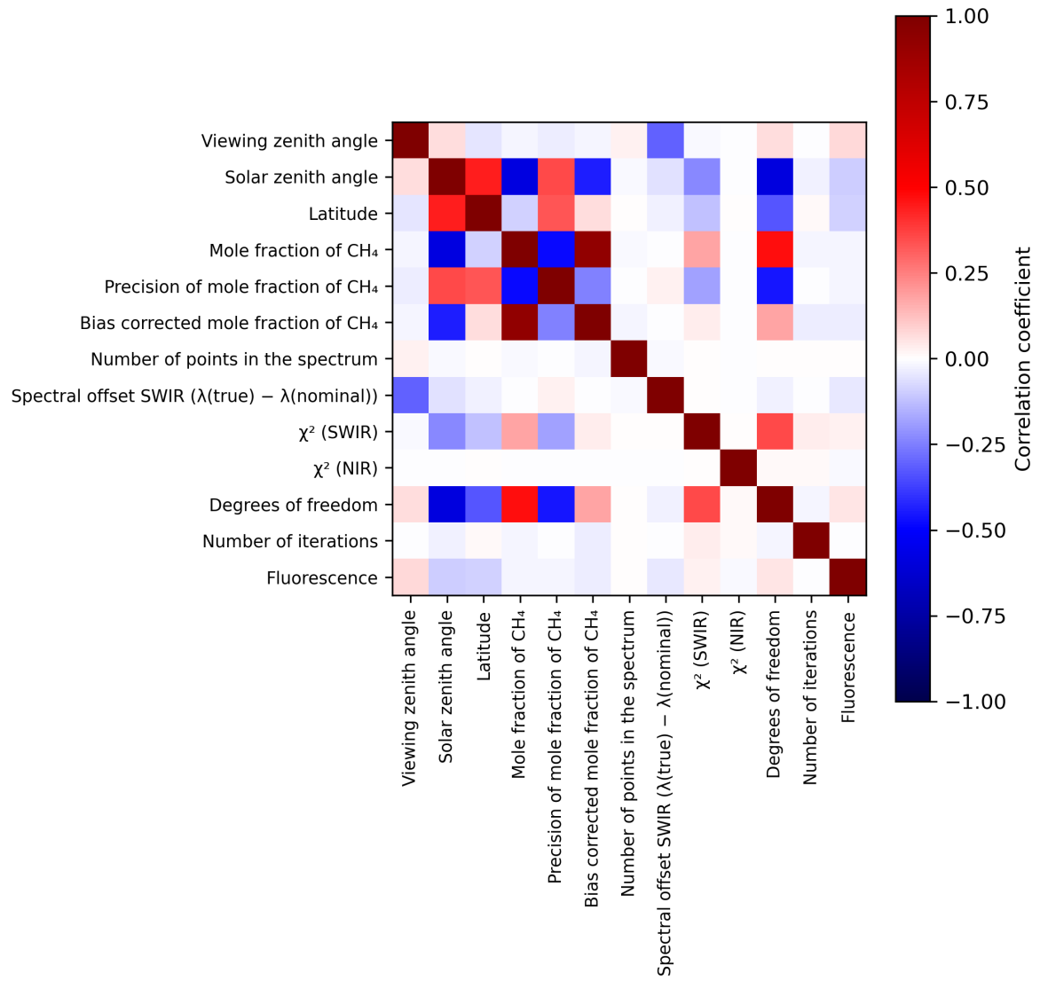
Figure 2: Map of correlation matrix for 2024-04-12 to 2024-04-14.
