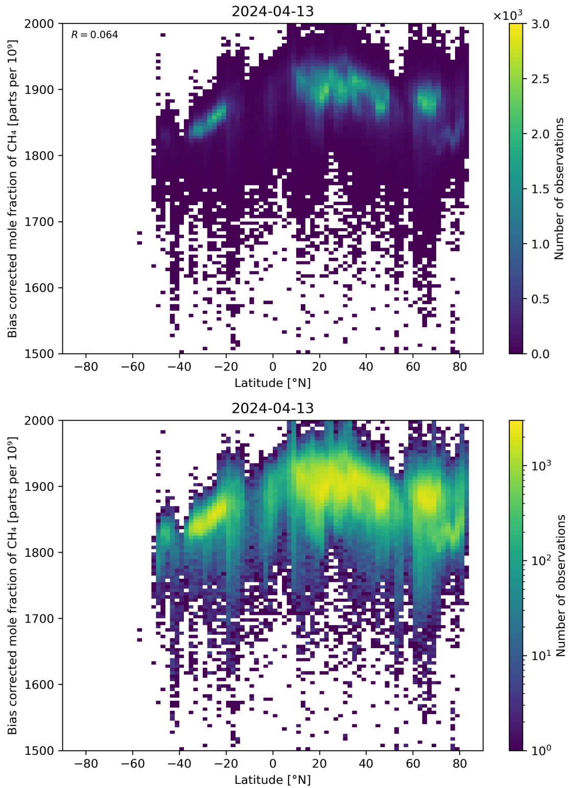
Figure 58: Scatter density plot of “Latitude” against “Bias corrected mole fraction of \text{CH}_4 ” for 2024-04-12 to 2024-04-14.
