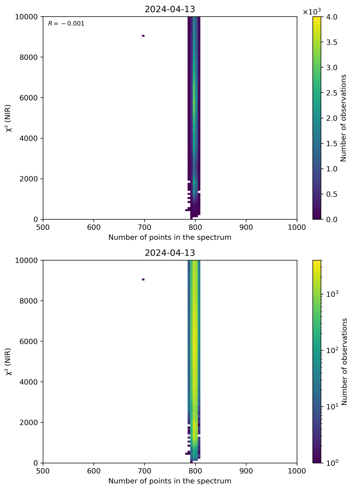
Figure 88: Scatter density plot of “Number of points in the spectrum” against “ \chi^2 (NIR)” for 2024-04-12 to 2024-04-14.
