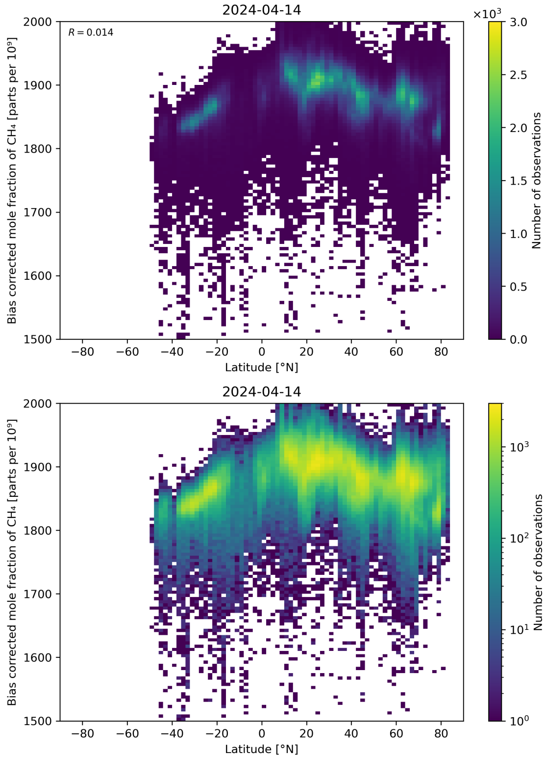
Figure 58: Scatter density plot of “Latitude” against “Bias corrected mole fraction of \text{CH}_4 ” for 2024-04-13 to 2024-04-15.
