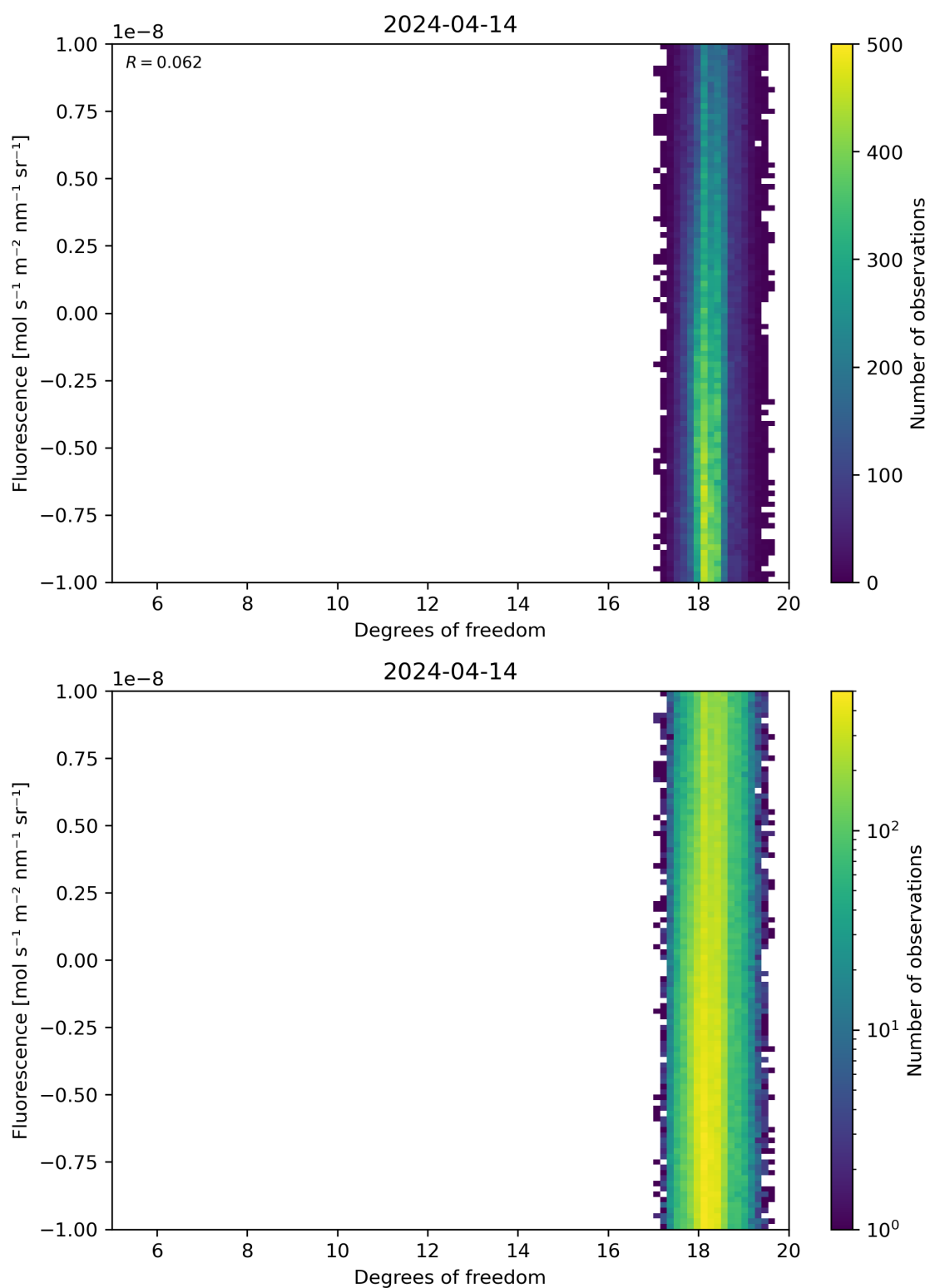
Figure 51: Scatter density plot of “Degrees of freedom” against “Fluorescence” for 2024-04-13 to 2024-04-15.
