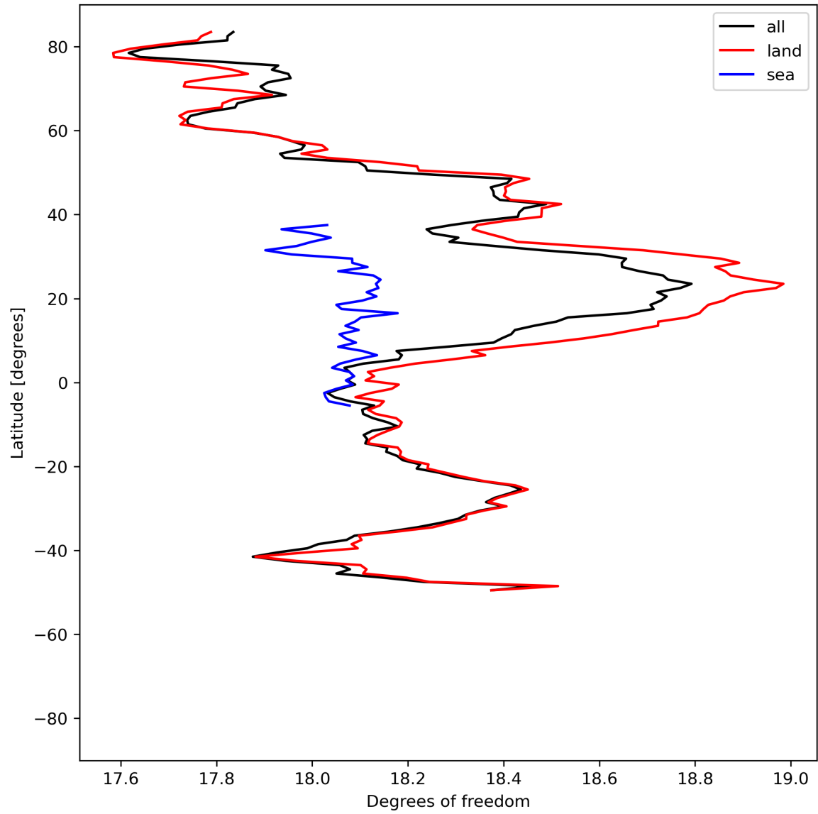
Figure 19: Zonal average of “Degrees of freedom” for 2024-04-13 to 2024-04-15.
