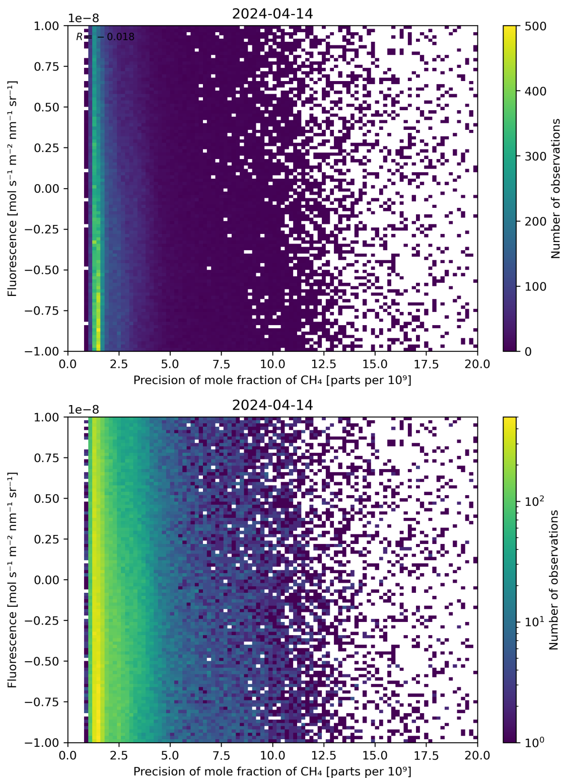
Figure 81: Scatter density plot of “Precision of mole fraction of \text{CH}_4 ” against “Fluorescence” for 2024-04-13 to 2024-04-15.
