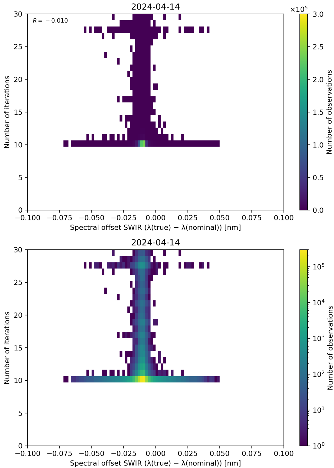
Figure 121: Scatter density plot of “Spectral offset SWIR ( \lambda(\text{true}) - \lambda(\text{nominal}) )” against “Number of iterations” for 2024-04-13 to 2024-04-15.
