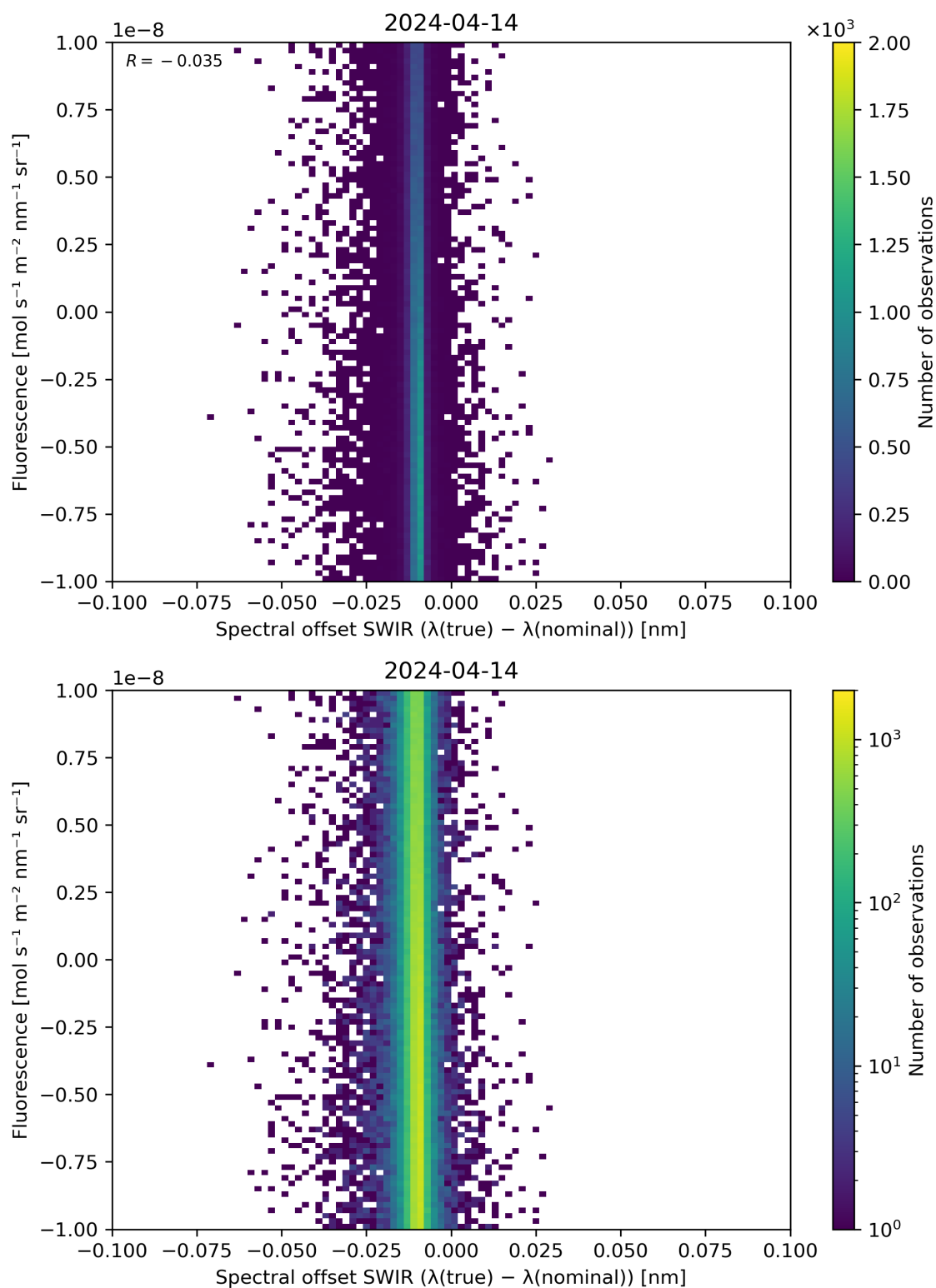
Figure 120: Scatter density plot of “Spectral offset SWIR ( \lambda(\text{true}) - \lambda(\text{nominal}) )” against “Fluorescence” for 2024-04-13 to 2024-04-15.
