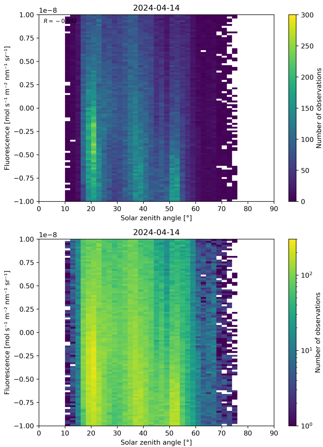
Figure 97: Scatter density plot of “Solar zenith angle” against “Fluorescence” for 2024-04-13 to 2024-04-15.
