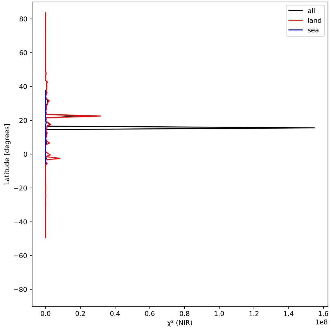
Figure 18: Zonal average of “ \chi^2 (NIR)” for 2024-04-13 to 2024-04-15.
