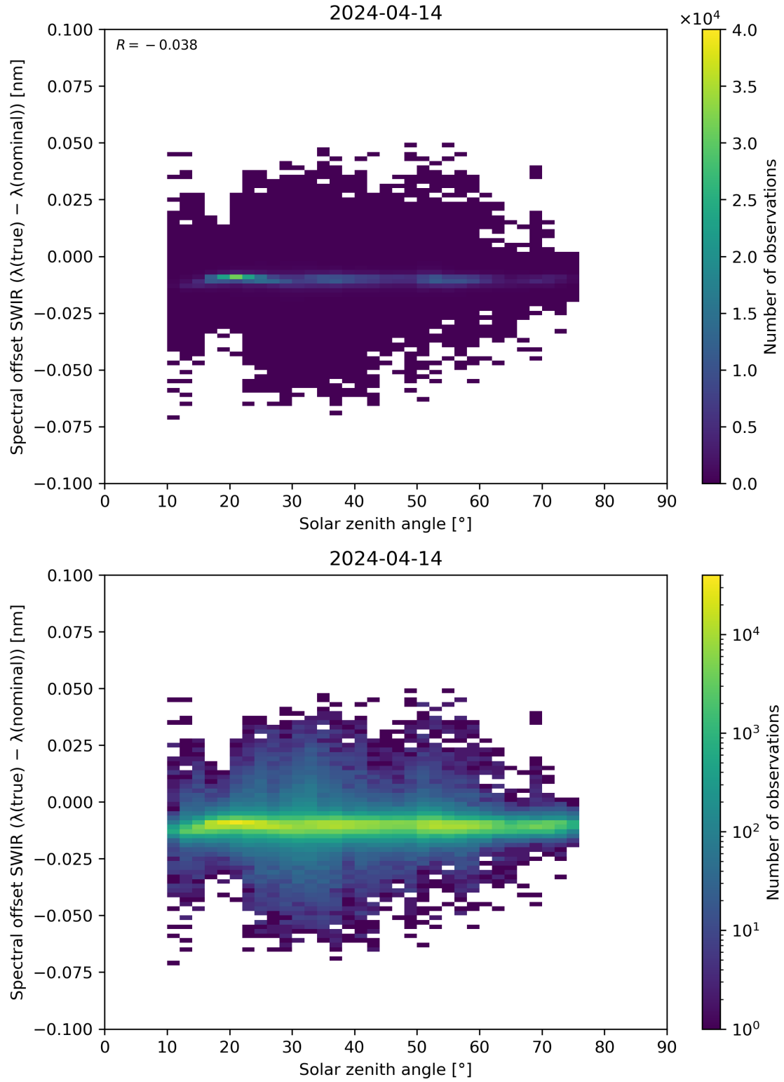
Figure 104: Scatter density plot of “Solar zenith angle” against “Spectral offset SWIR ( \lambda(\text{true}) - \lambda(\text{nominal}) )” for 2024-04-13 to 2024-04-15.
