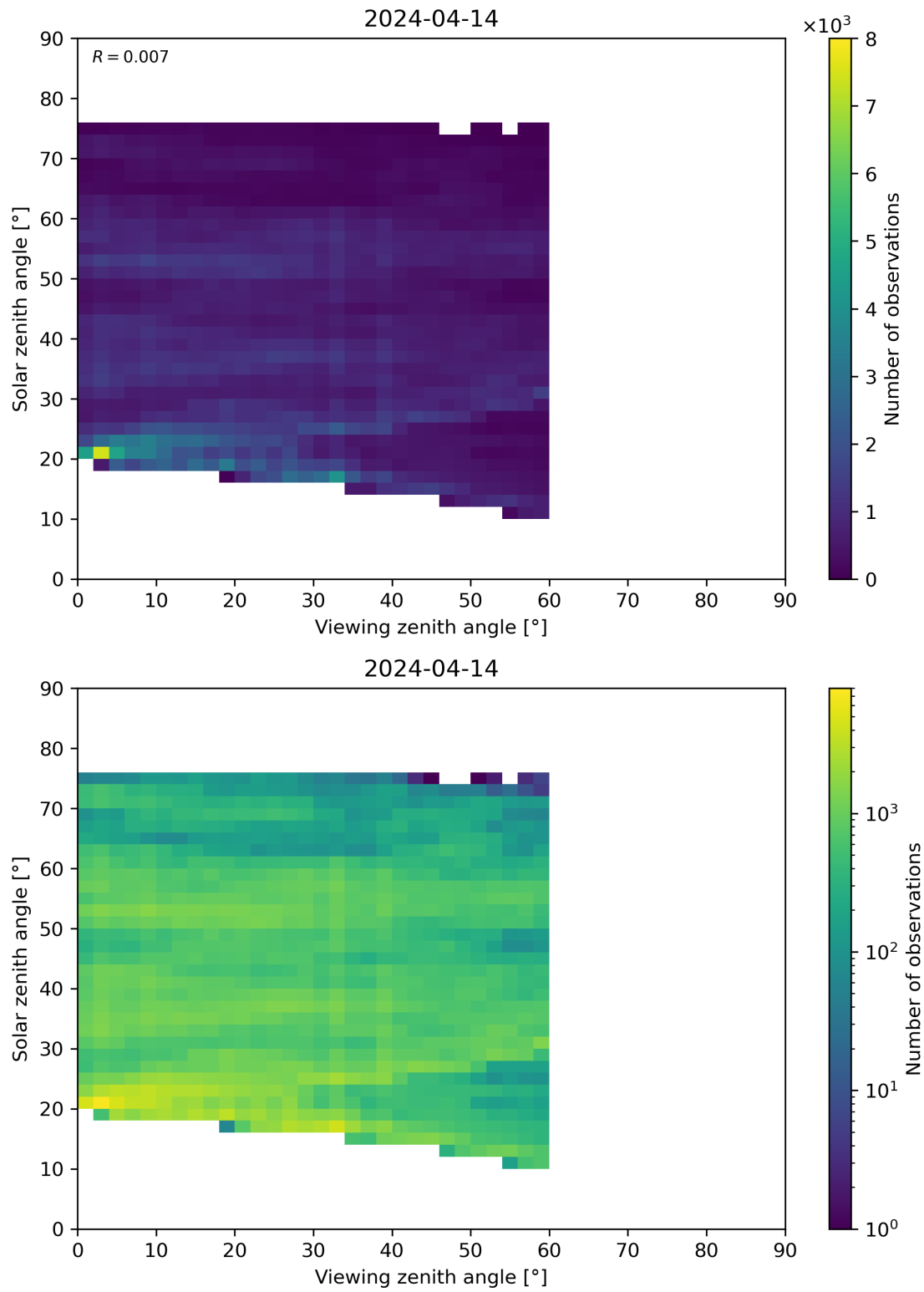
Figure 115: Scatter density plot of “Viewing zenith angle” against “Solar zenith angle” for 2024-04-13 to 2024-04-15.
