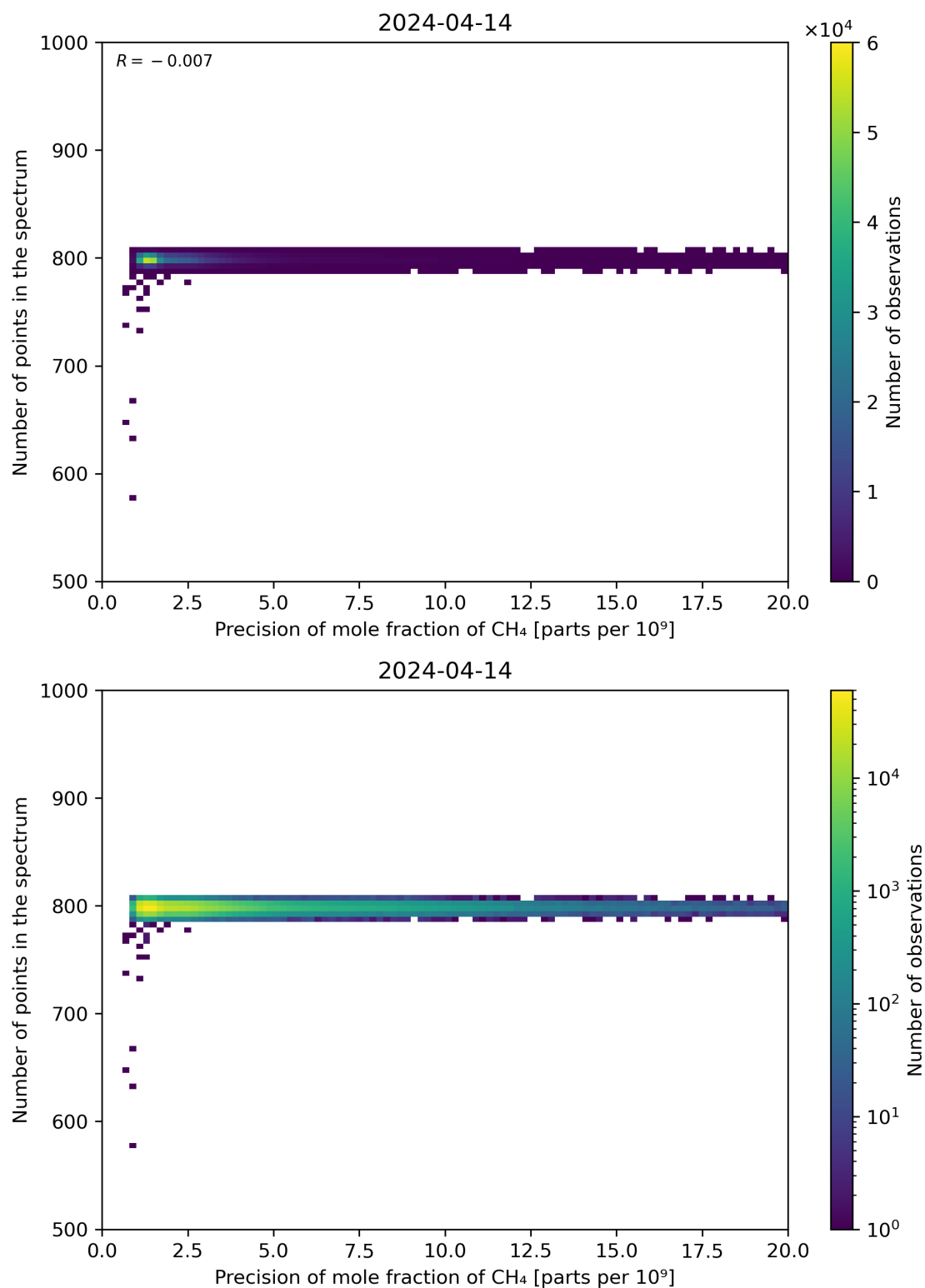
Figure 84: Scatter density plot of “Precision of mole fraction of CH 4 ” against “Number of points in the spectrum” for 2024-04-13 to 2024-04-15.
