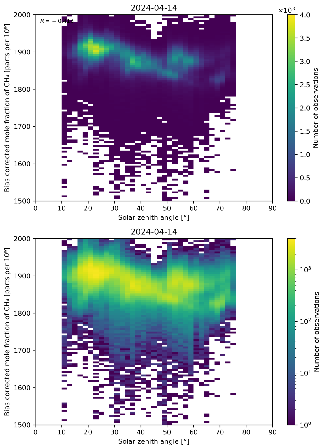
Figure 100: Scatter density plot of “Solar zenith angle” against “Bias corrected mole fraction of \text{CH}_4 ” for 2024-04-13 to 2024-04-15.
