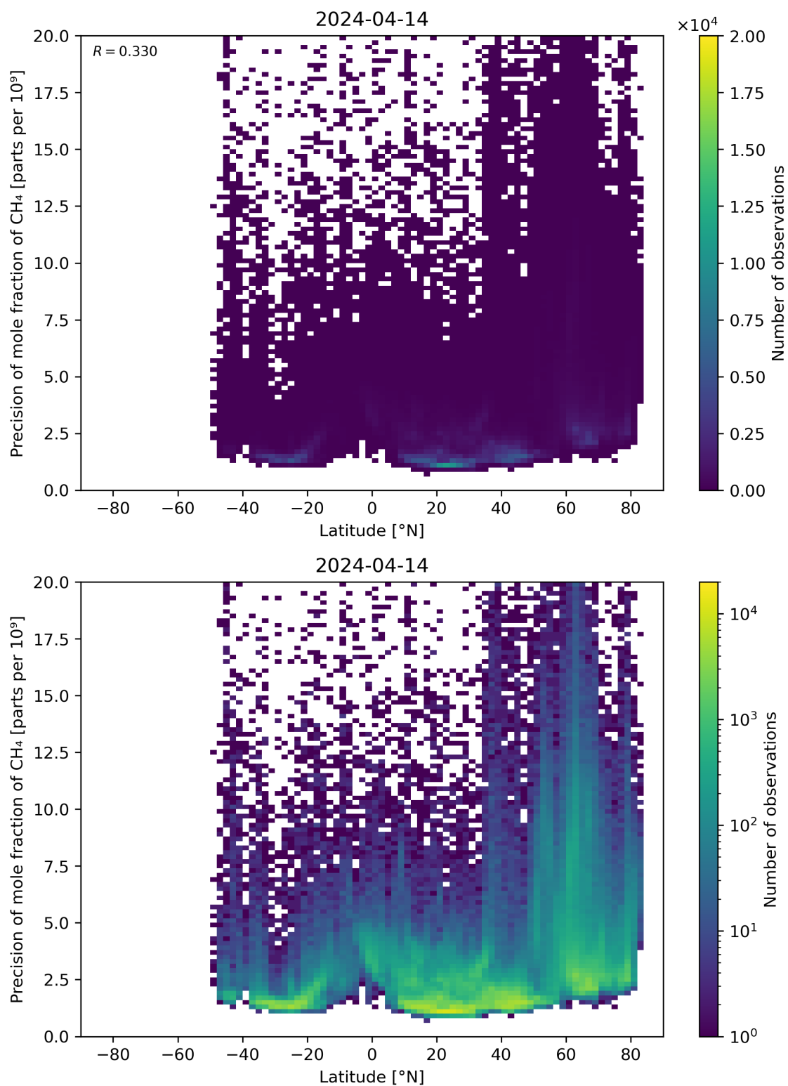
Figure 59: Scatter density plot of “Latitude” against “Precision of mole fraction of \text{CH}_4 ” for 2024-04-13 to 2024-04-15.
