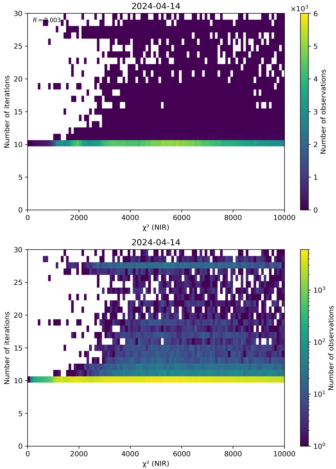
Figure 46: Scatter density plot of “ \chi^2 (NIR)” against “Number of iterations” for 2024-04-13 to 2024-04-15.
