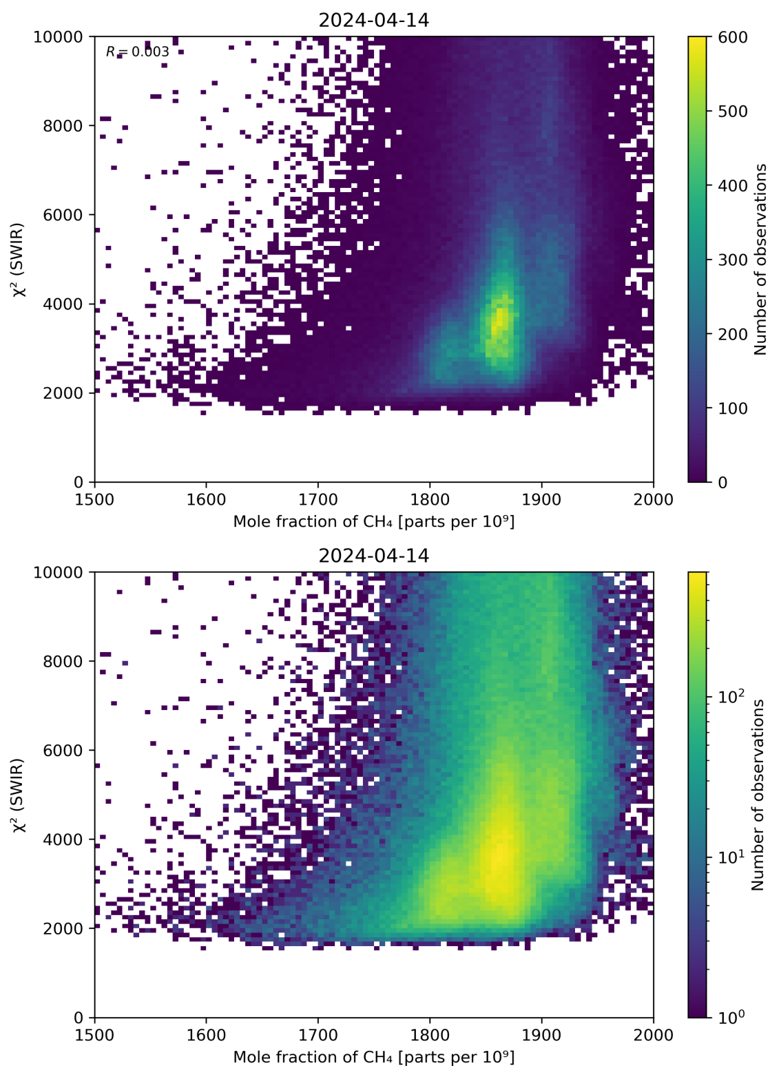
Figure 71: Scatter density plot of “Mole fraction of \text{CH}_4 ” against “ \chi^2 (SWIR)” for 2024-04-13 to 2024-04-15.
