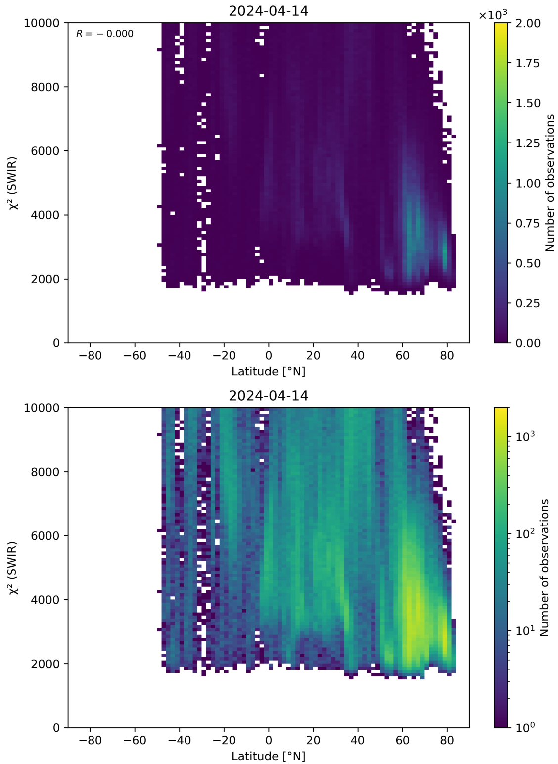
Figure 54: Scatter density plot of “Latitude” against “ \chi^2 (SWIR)” for 2024-04-13 to 2024-04-15.
