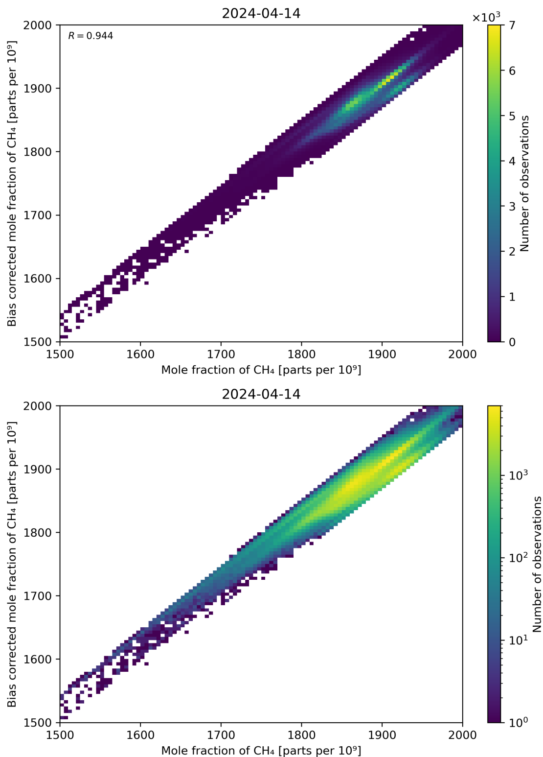
Figure 74: Scatter density plot of “Mole fraction of CH 4 ” against “Bias corrected mole fraction of CH 4 ” for 2024-04-13 to 2024-04-15.
