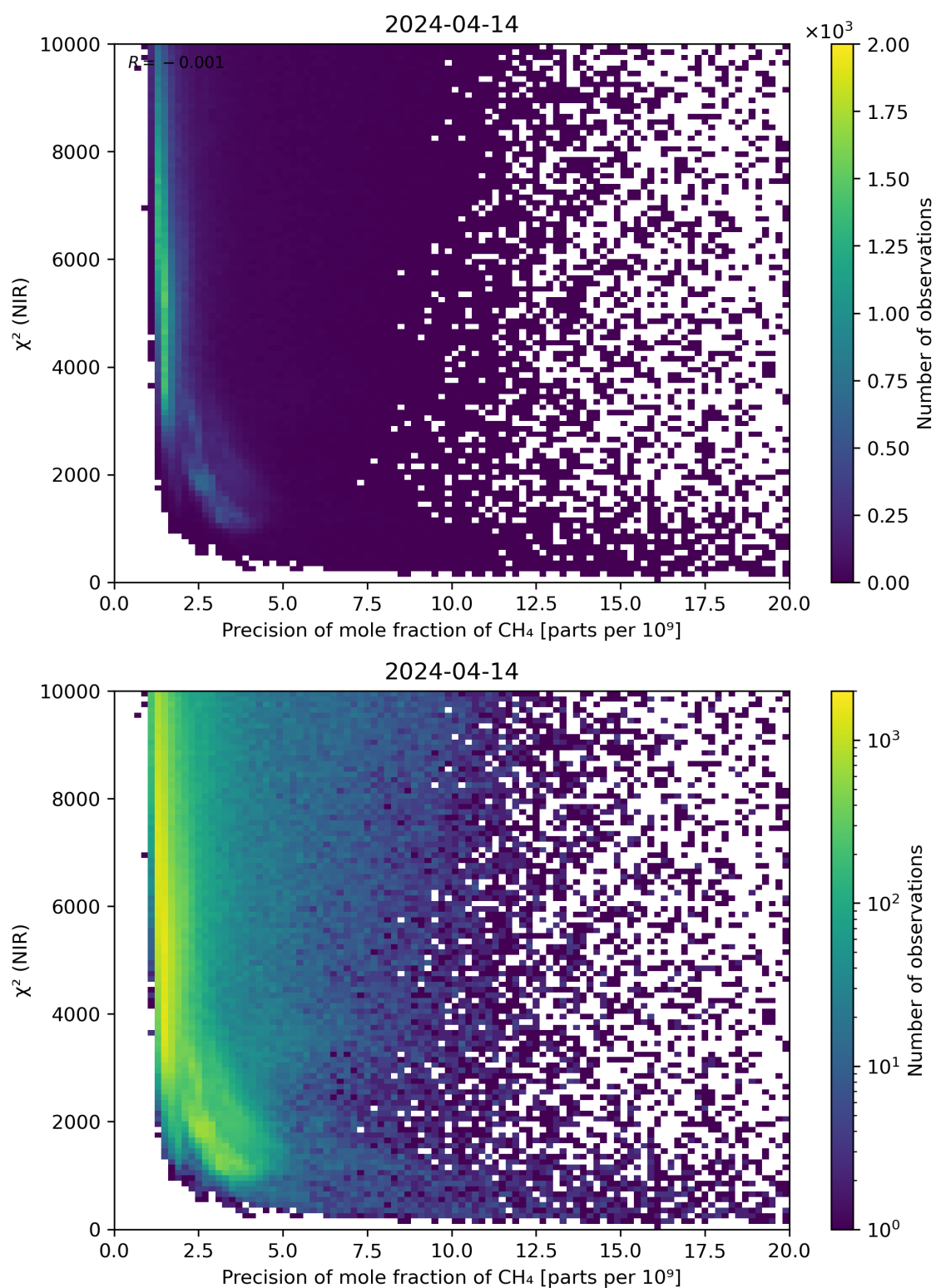
Figure 78: Scatter density plot of “Precision of mole fraction of \text{CH}_4 ” against “ \chi^2 (NIR)” for 2024-04-13 to 2024-04-15.
