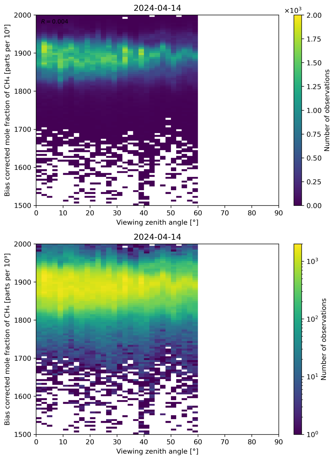
Figure 111: Scatter density plot of “Viewing zenith angle” against “Bias corrected mole fraction of CH 4 ” for 2024-04-13 to 2024-04-15.
