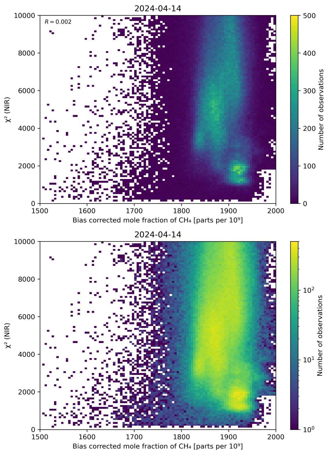
Figure 63: Scatter density plot of “Bias corrected mole fraction of CH 4 ” against “ \chi^2 (NIR)” for 2024-04-13 to 2024-04-15.
