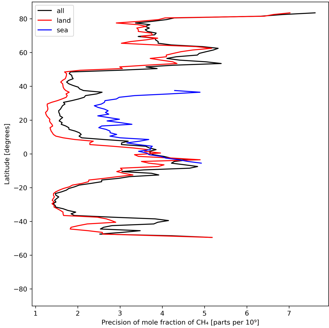
Figure 13: Zonal average of “Precision of mole fraction of CH 4 ” for 2024-04-13 to 2024-04-15.
