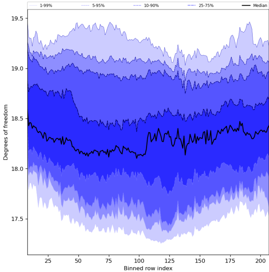
Figure 41: Along track statistics of “Degrees of freedom” for 2024-04-13 to 2024-04-15
