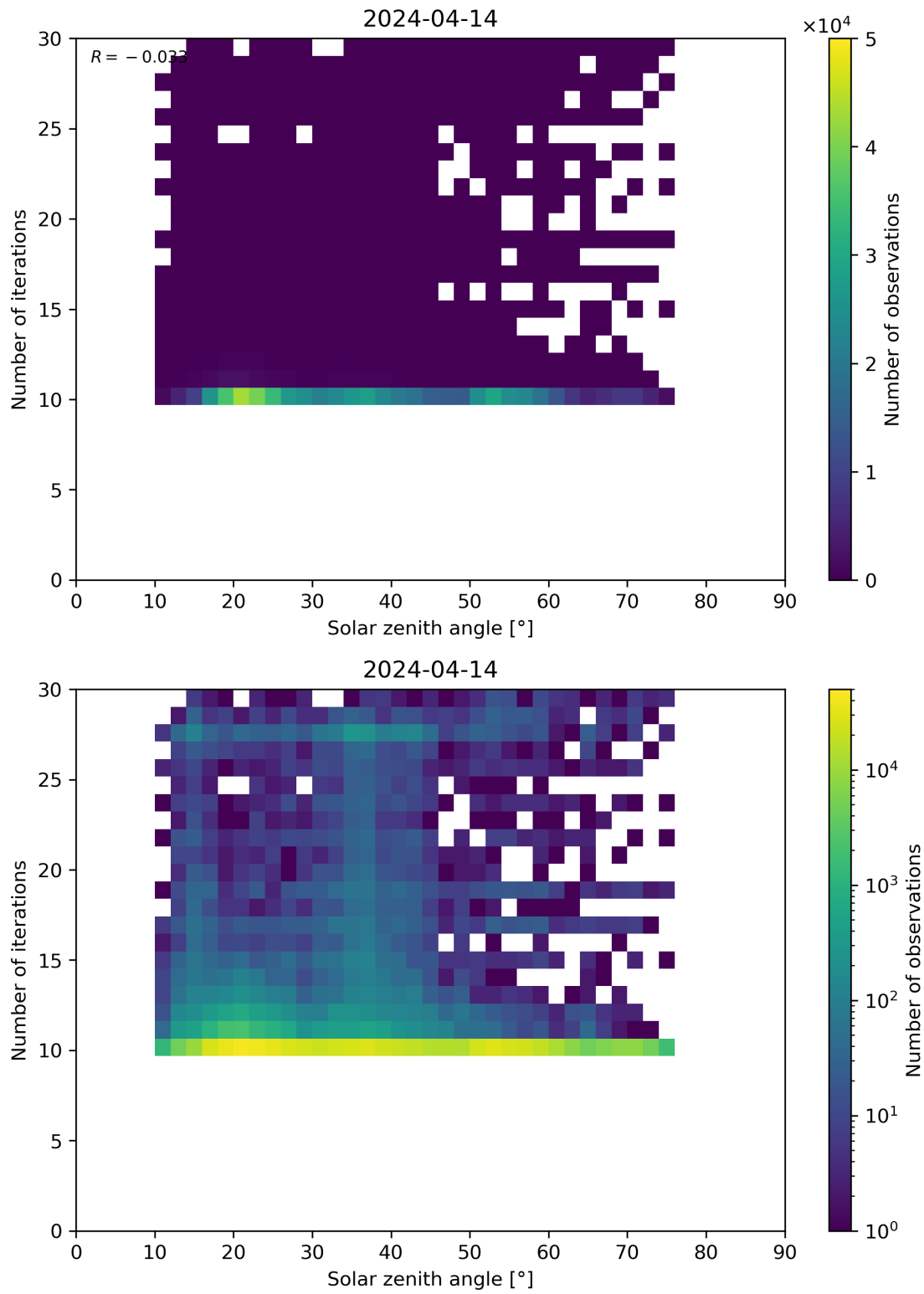
Figure 102: Scatter density plot of “Solar zenith angle” against “Number of iterations” for 2024-04-13 to 2024-04-15.
