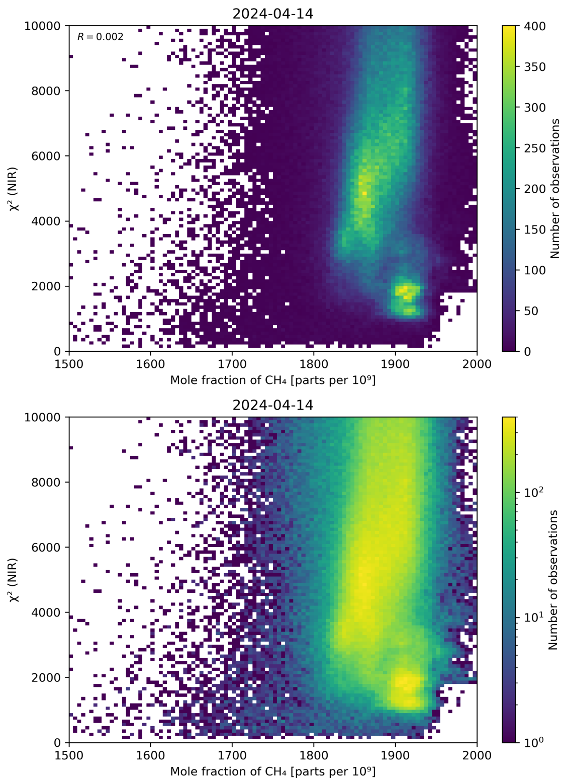
Figure 70: Scatter density plot of “Mole fraction of CH 4 ” against “ \chi^2 (NIR)” for 2024-04-13 to 2024-04-15.
