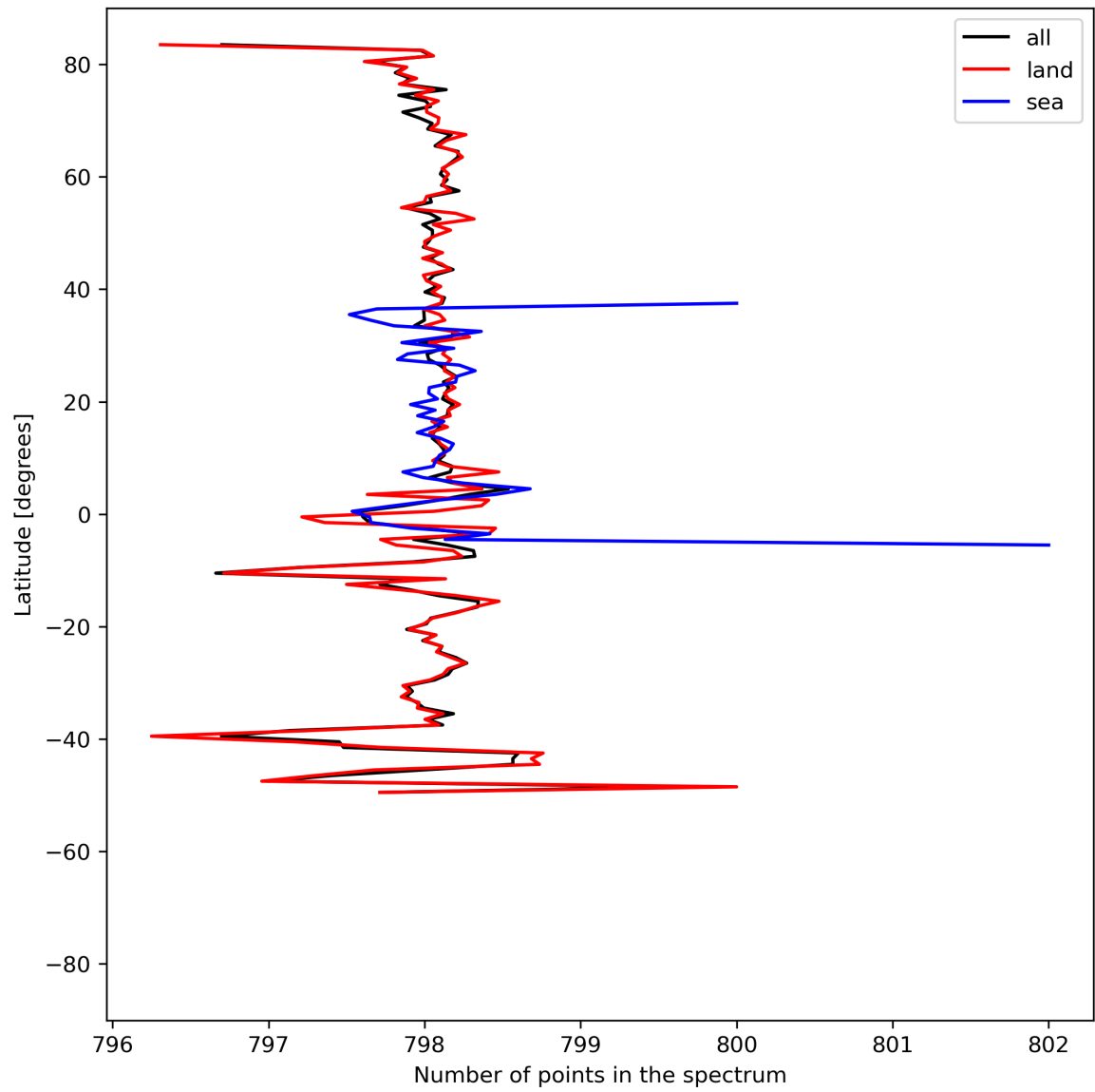
Figure 15: Zonal average of “Number of points in the spectrum” for 2024-04-13 to 2024-04-15.
