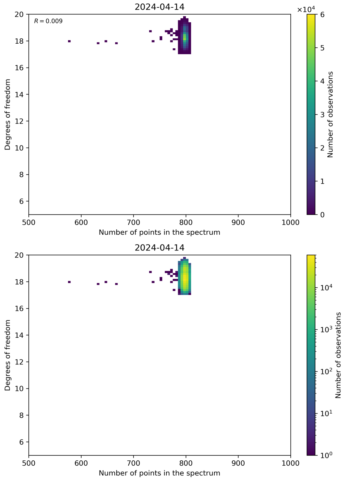
Figure 90: Scatter density plot of “Number of points in the spectrum” against “Degrees of freedom” for 2024-04-13 to 2024-04-15.
