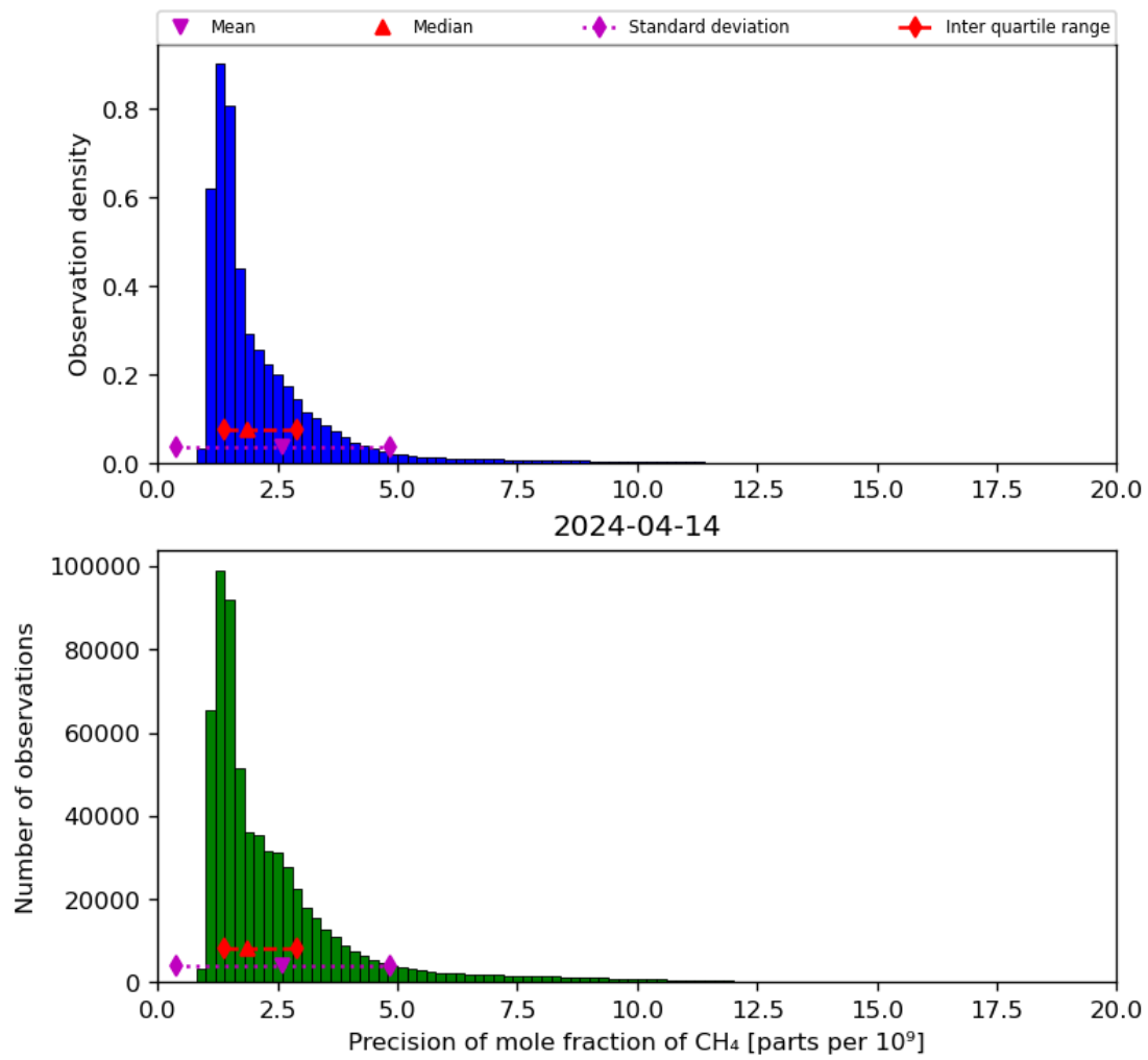
Figure 24: Histogram of “Precision of mole fraction of CH 4 ” for 2024-04-13 to 2024-04-15
