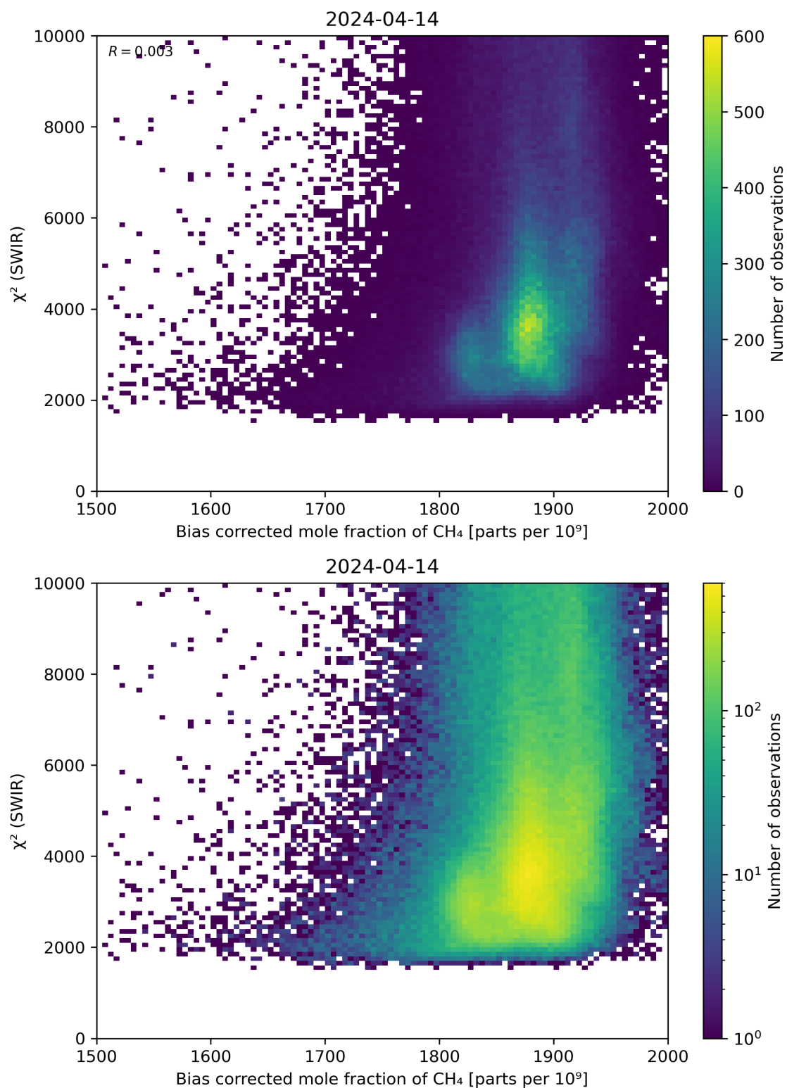
Figure 64: Scatter density plot of “Bias corrected mole fraction of \text{CH}_4 ” against “ \chi^2 (SWIR)” for 2024-04-13 to 2024-04-15.
