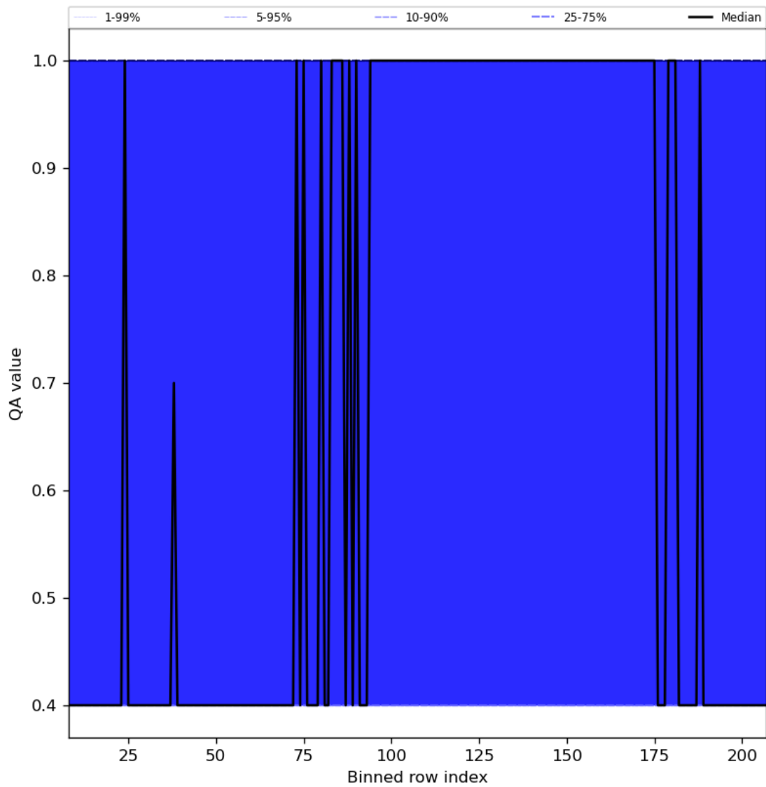
Figure 33: Along track statistics of “QA value” for 2024-04-13 to 2024-04-15
