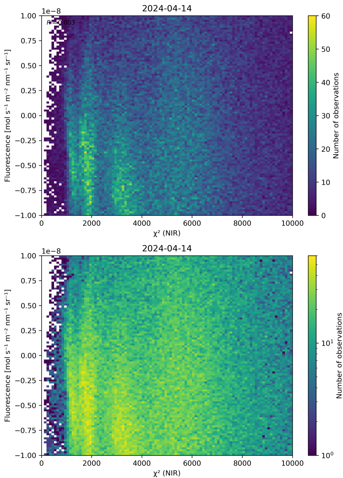
Figure 45: Scatter density plot of “ \chi^2 (NIR)” against “Fluorescence” for 2024-04-13 to 2024-04-15.
