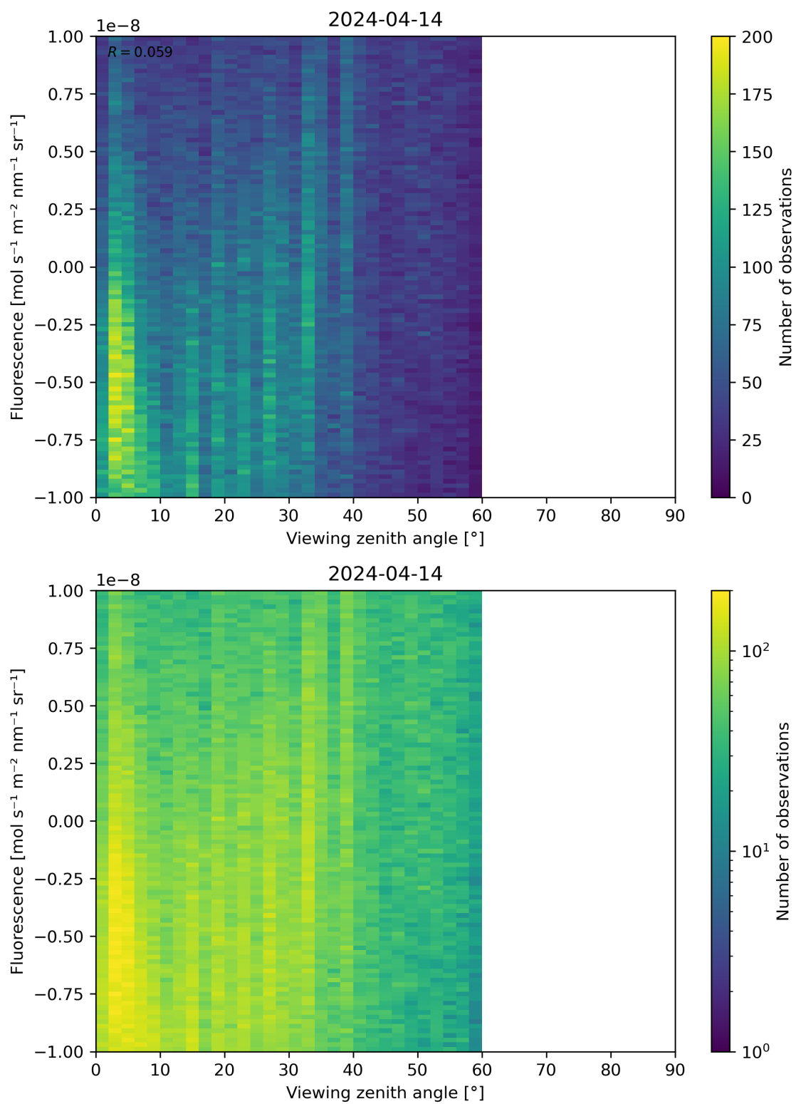
Figure 108: Scatter density plot of “Viewing zenith angle” against “Fluorescence” for 2024-04-13 to 2024-04-15.
