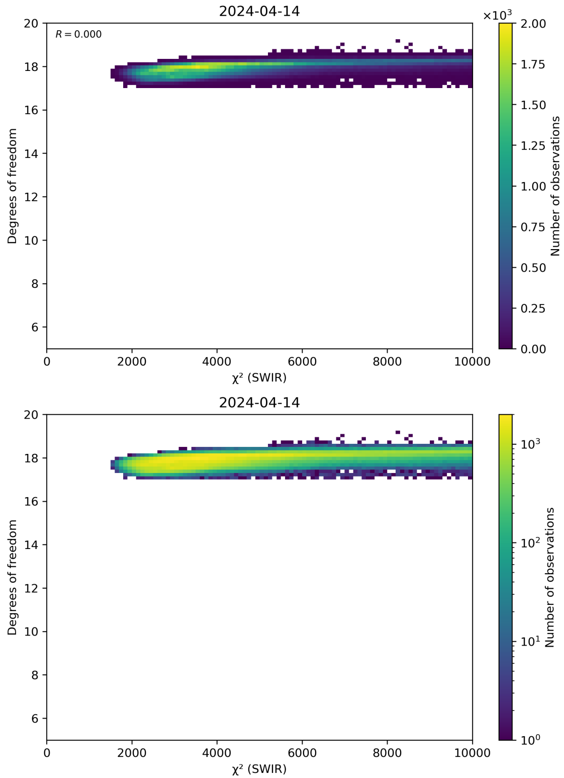
Figure 48: Scatter density plot of “ \chi^2 (SWIR)” against “Degrees of freedom” for 2024-04-13 to 2024-04-15.
