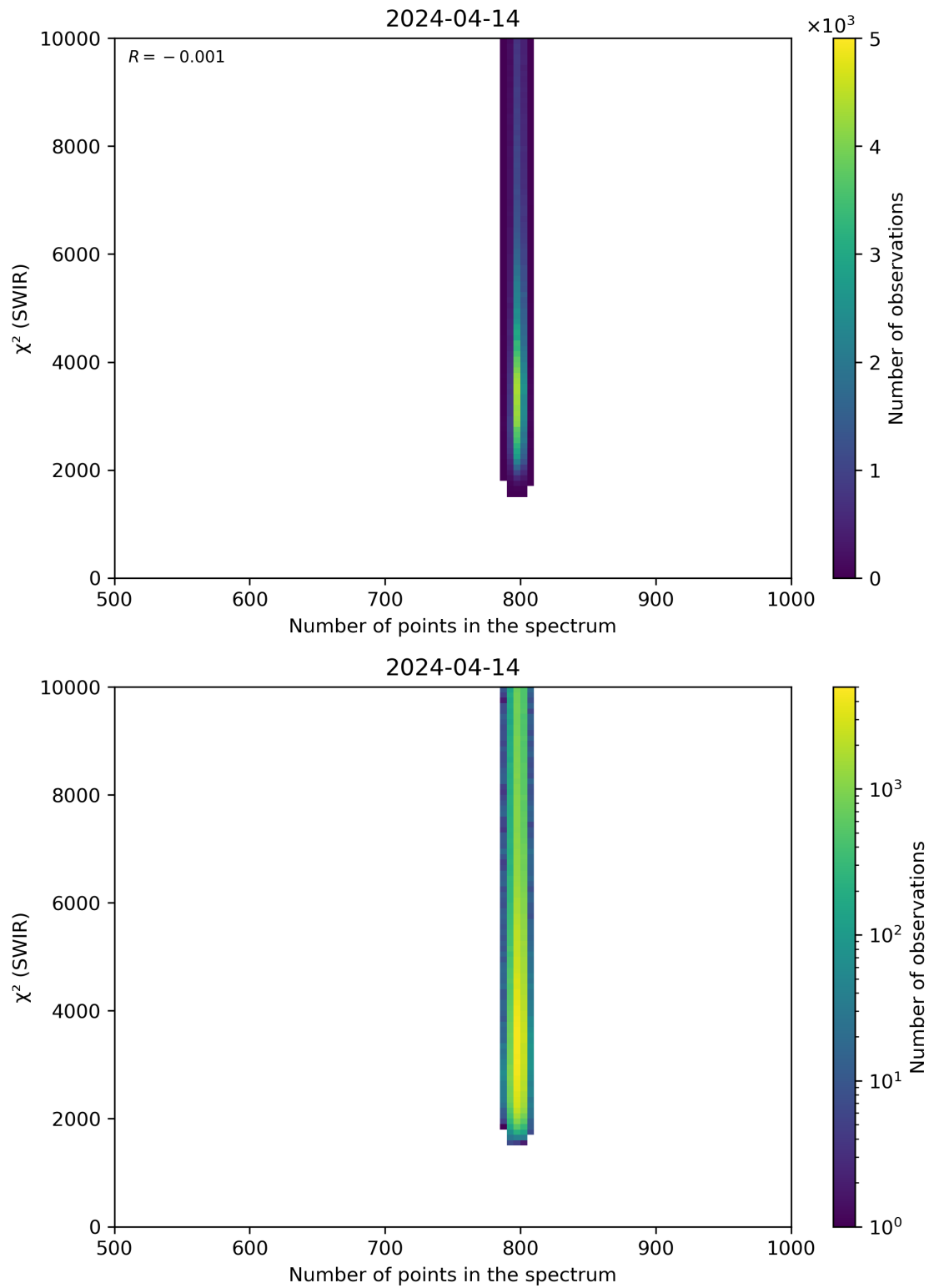
Figure 89: Scatter density plot of “Number of points in the spectrum” against “ \chi^2 (SWIR)” for 2024-04-13 to 2024-04-15.
