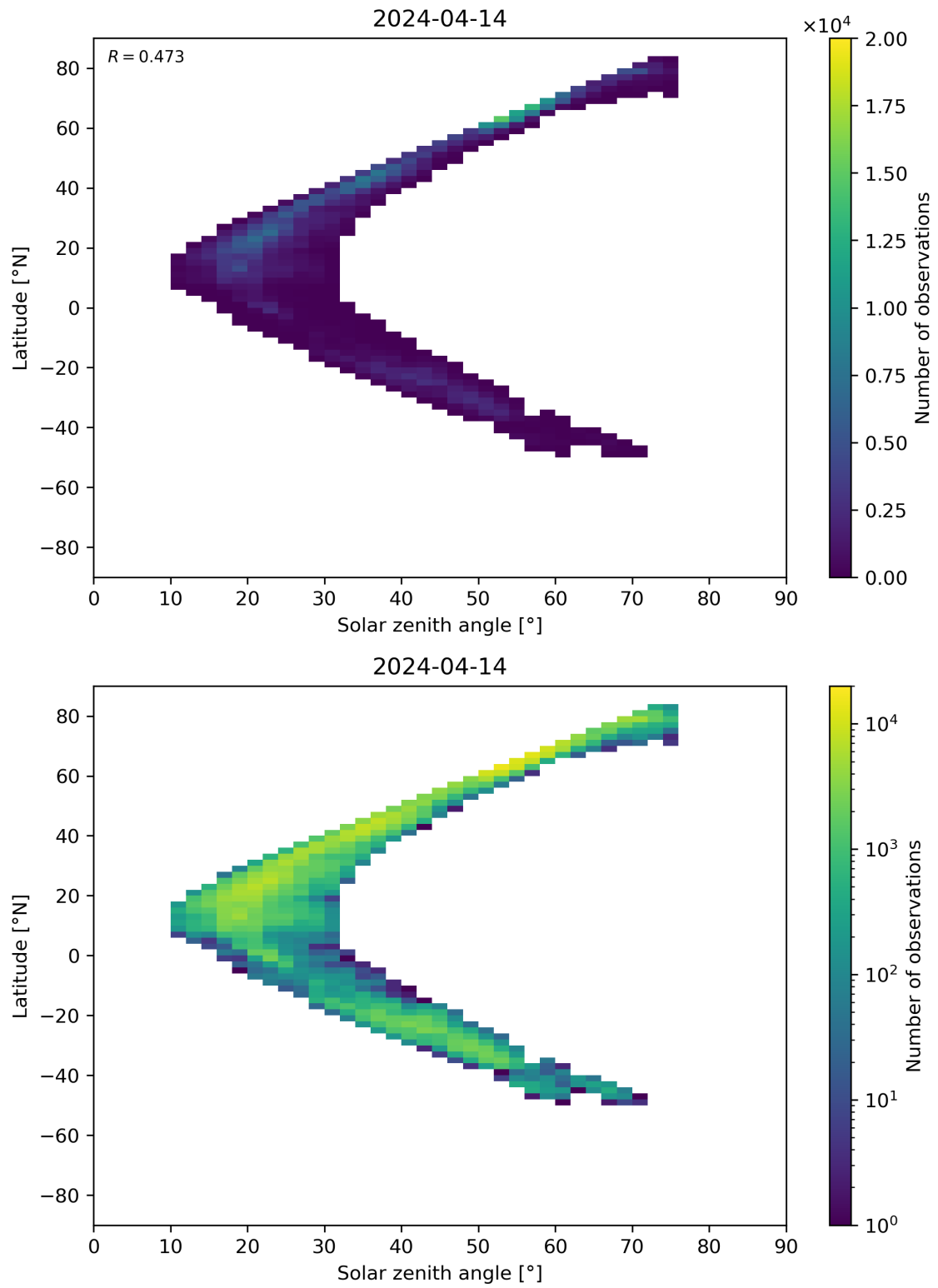
Figure 98: Scatter density plot of “Solar zenith angle” against “Latitude” for 2024-04-13 to 2024-04-15.
