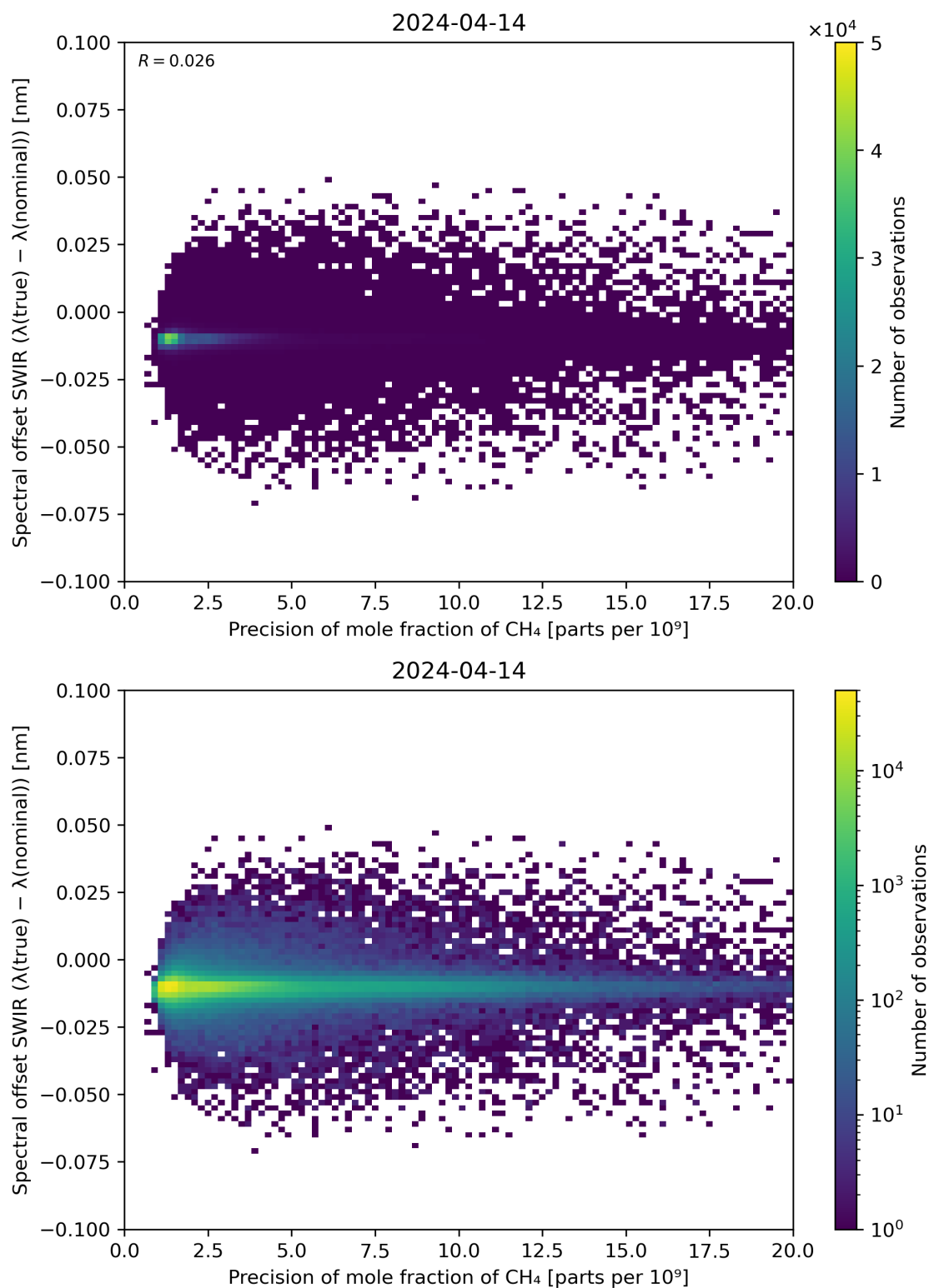
Figure 85: Scatter density plot of “Precision of mole fraction of CH 4 ” against “Spectral offset SWIR ( \lambda(\text{true}) - \lambda(\text{nominal}) )” for 2024-04-13 to 2024-04-15.
