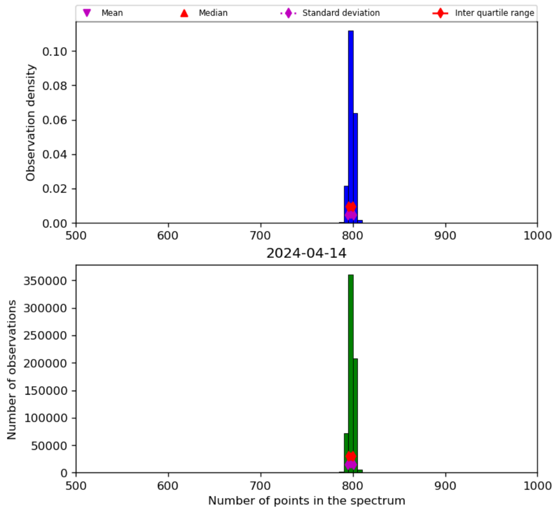
Figure 26: Histogram of “Number of points in the spectrum” for 2024-04-13 to 2024-04-15
