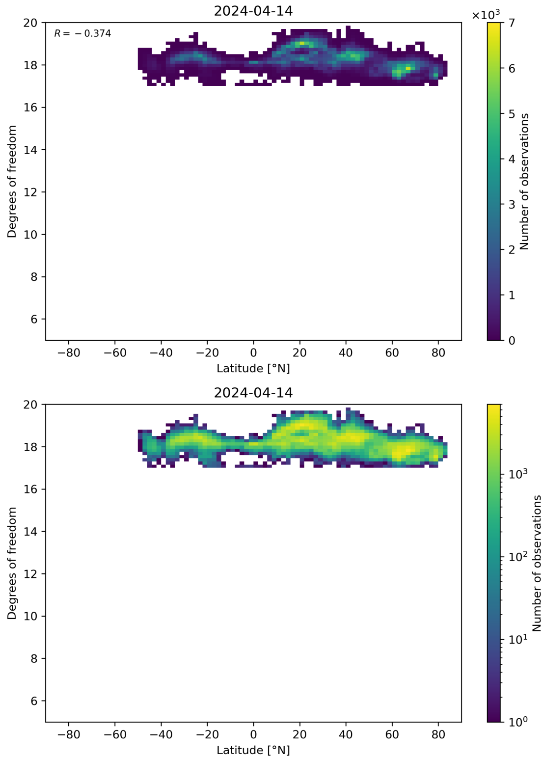
Figure 55: Scatter density plot of “Latitude” against “Degrees of freedom” for 2024-04-13 to 2024-04-15.
