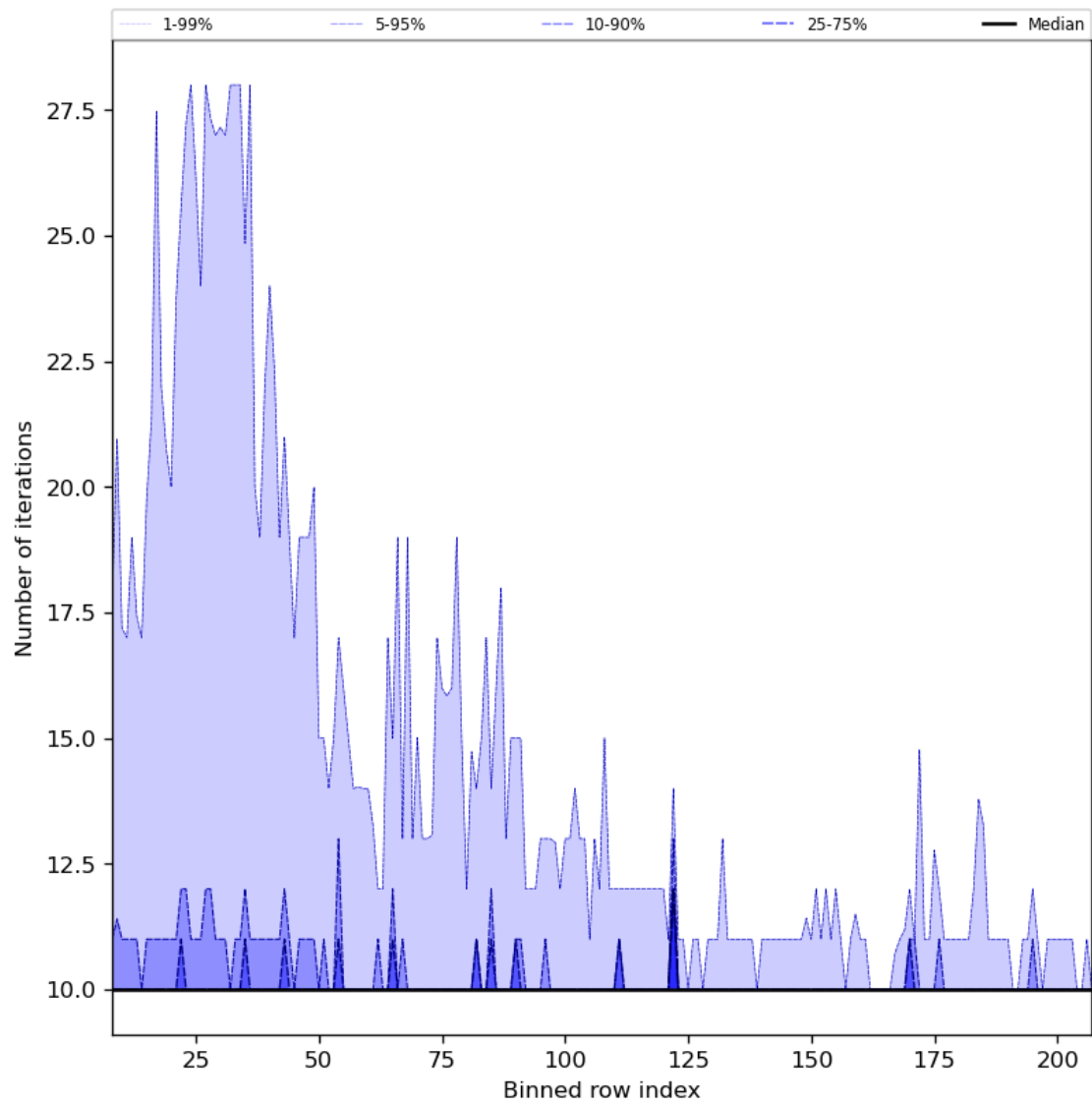
Figure 42: Along track statistics of “Number of iterations” for 2024-04-13 to 2024-04-15
