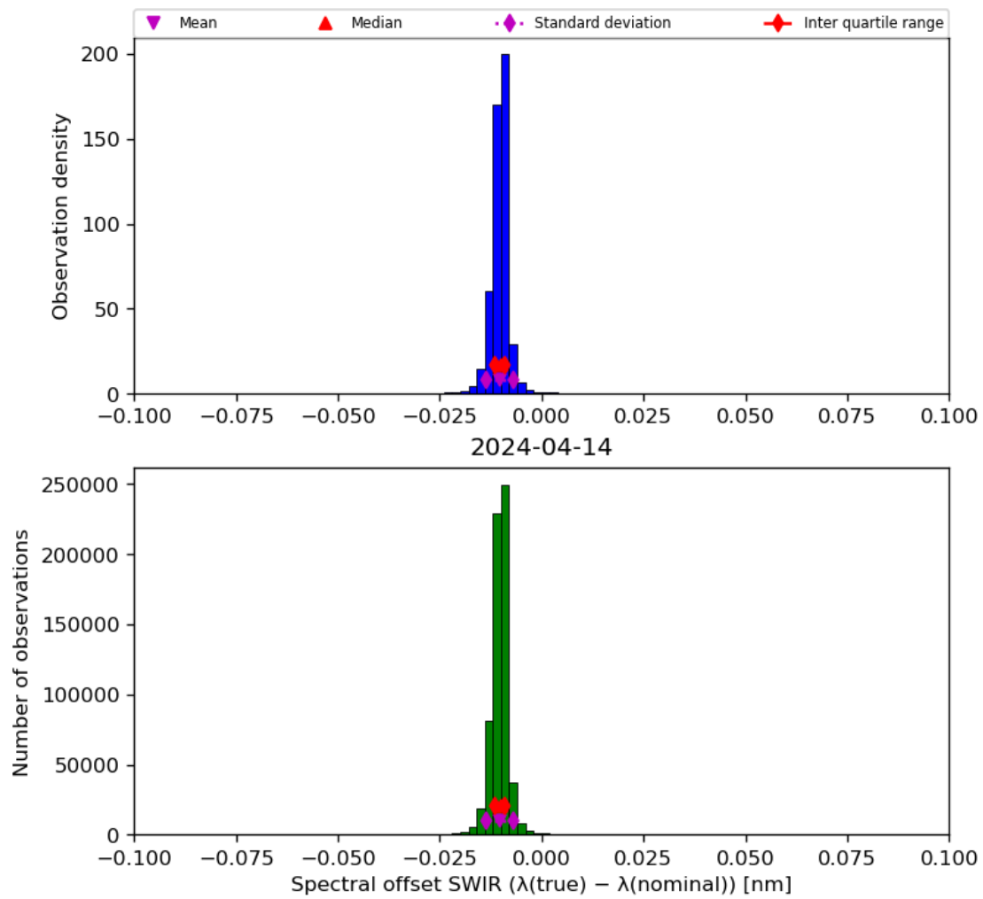
Figure 27: Histogram of “Spectral offset SWIR ( \lambda(\text{true}) - \lambda(\text{nominal}) )” for 2024-04-13 to 2024-04-15
