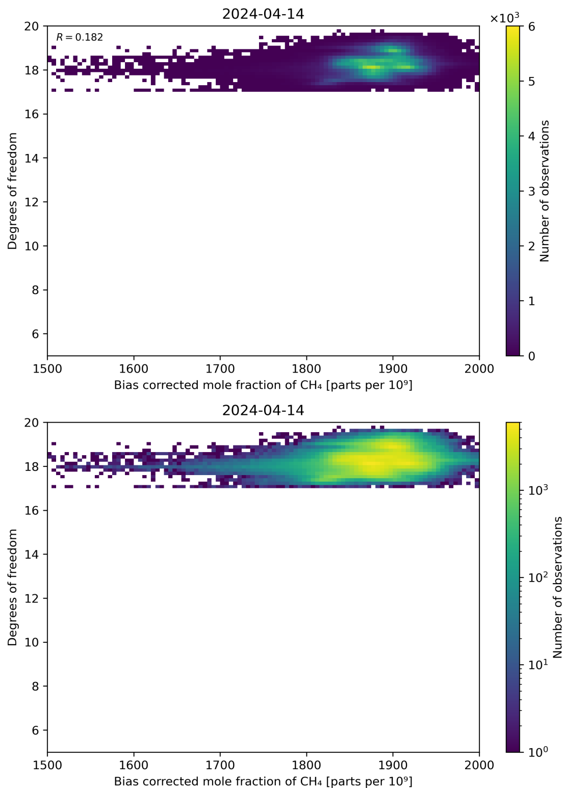
Figure 65: Scatter density plot of “Bias corrected mole fraction of CH 4 ” against “Degrees of freedom” for 2024-04-13 to 2024-04-15.
