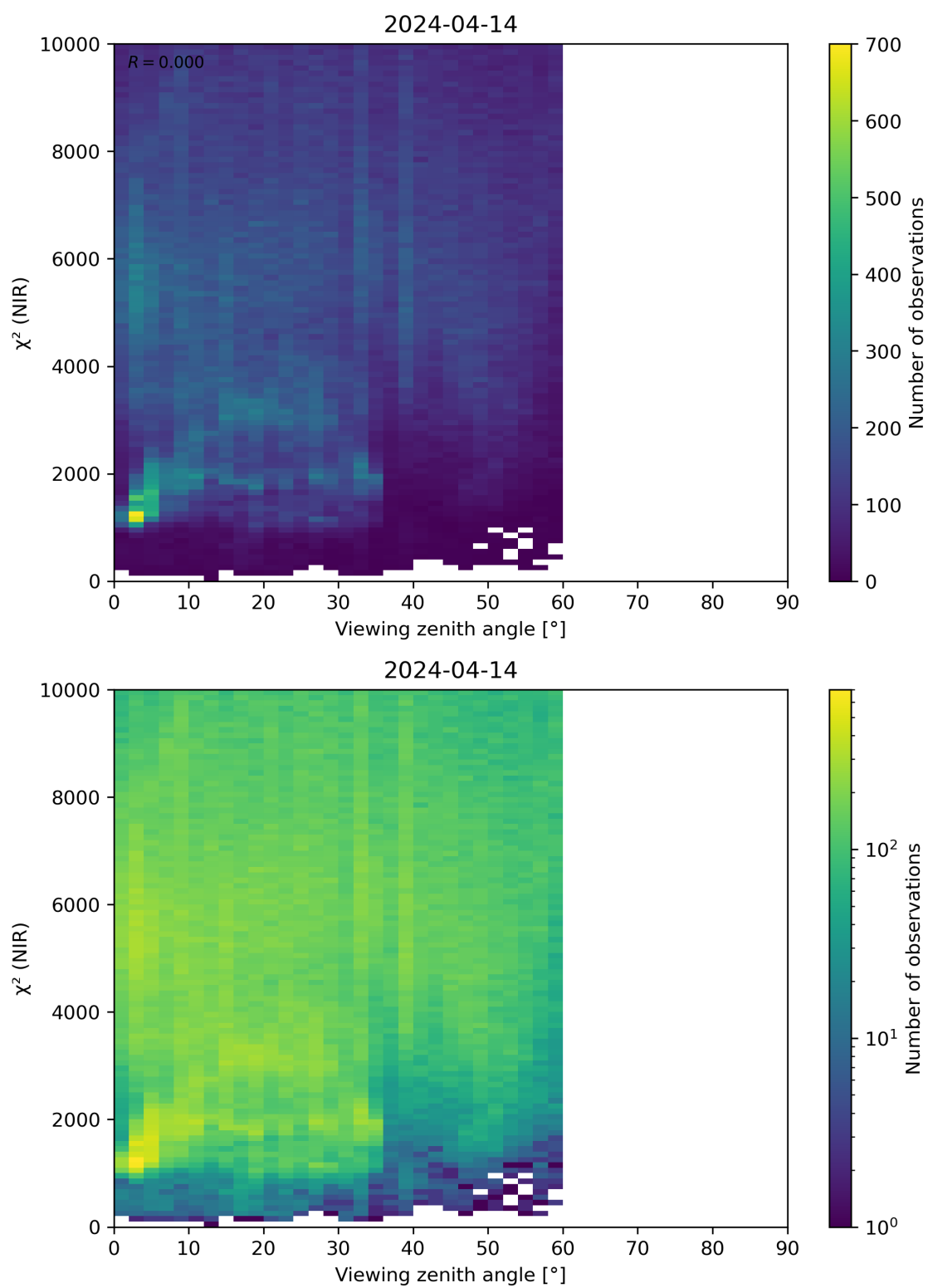
Figure 105: Scatter density plot of “Viewing zenith angle” against “ \chi^2 (NIR)” for 2024-04-13 to 2024-04-15.
