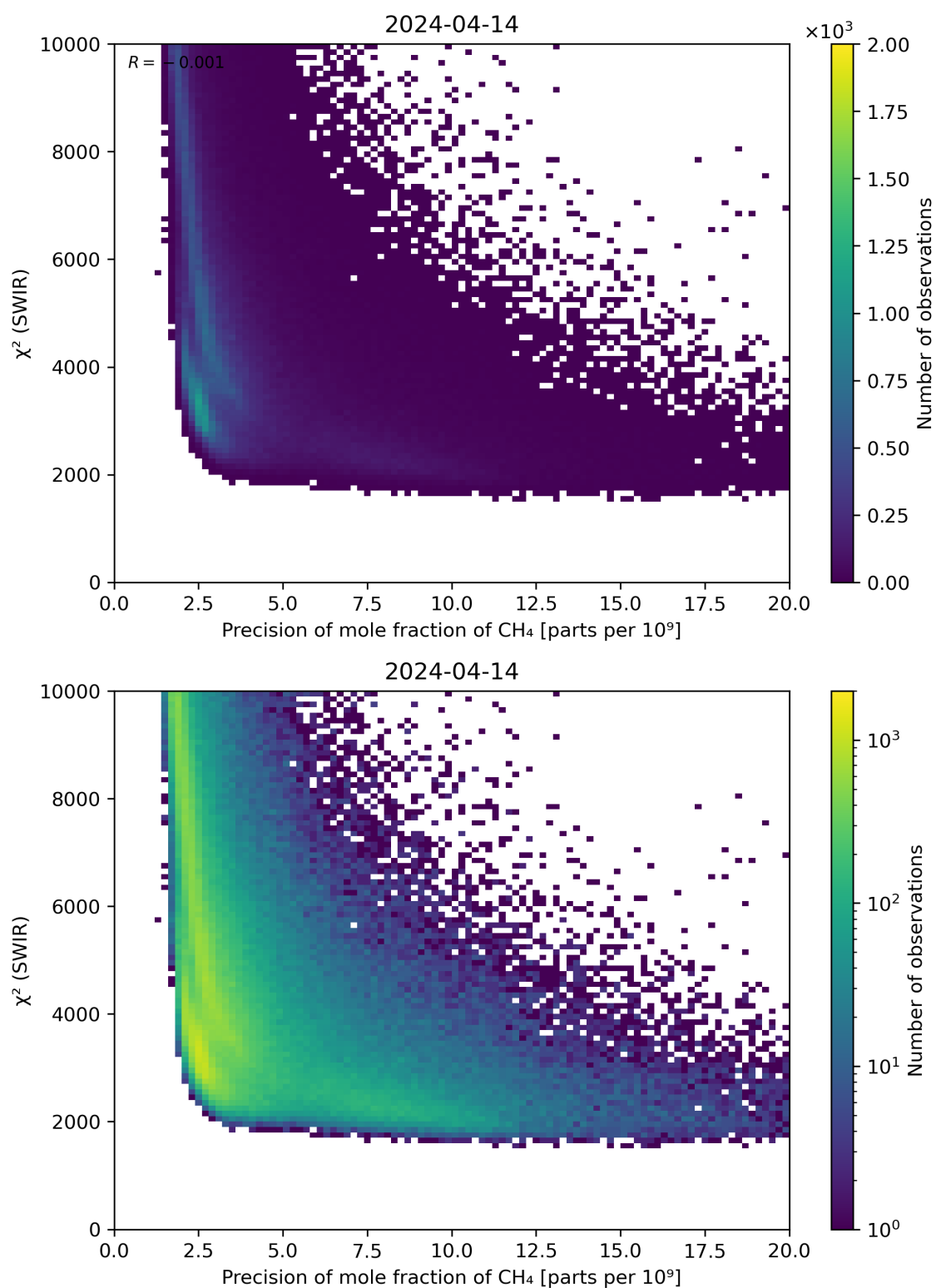
Figure 79: Scatter density plot of “Precision of mole fraction of \text{CH}_4 ” against “ \chi^2 (SWIR)” for 2024-04-13 to 2024-04-15.
