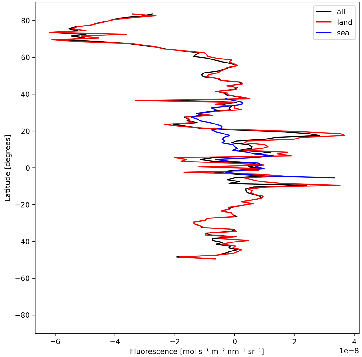
Figure 21: Zonal average of “Fluorescence” for 2024-04-13 to 2024-04-15.
