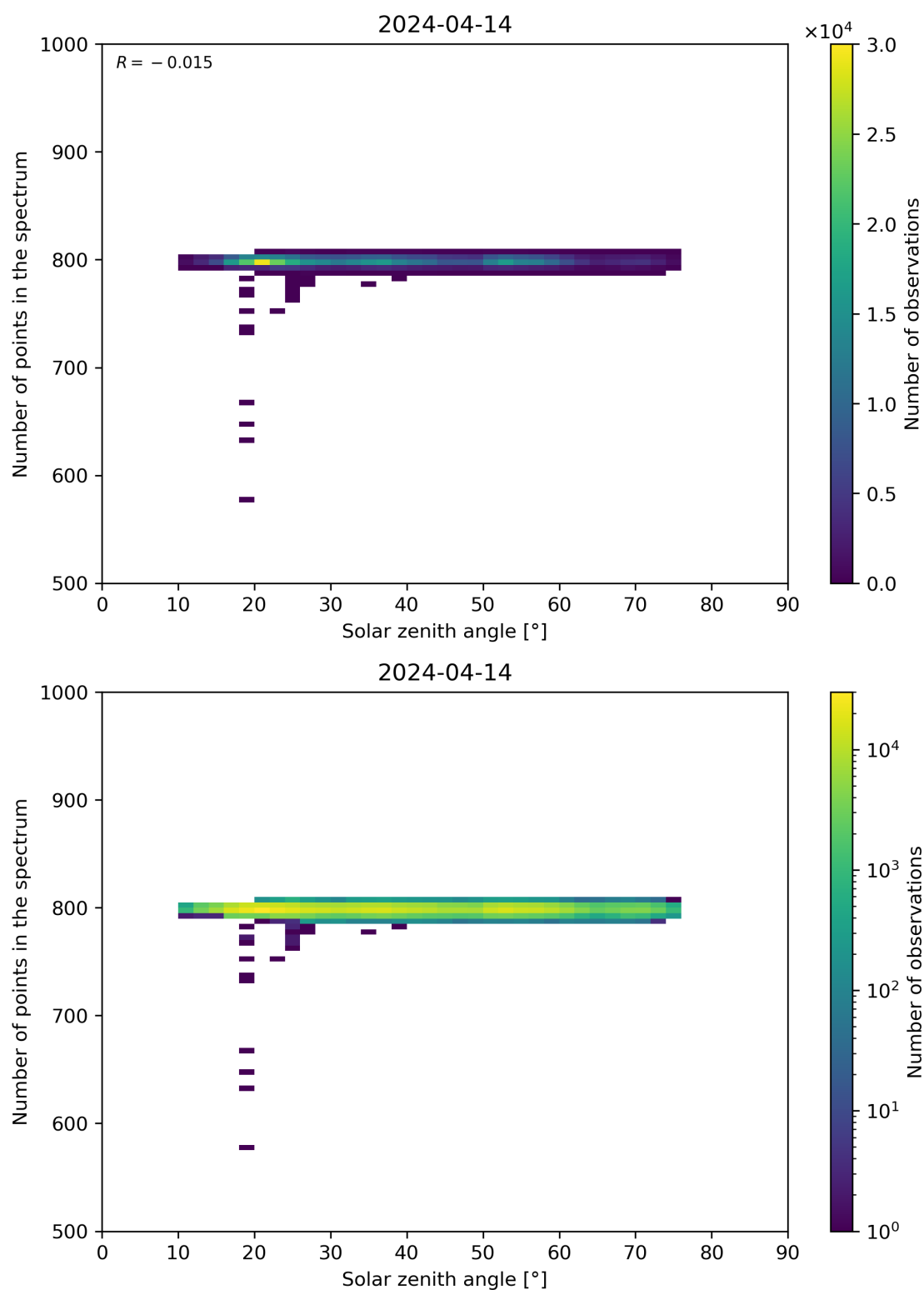
Figure 103: Scatter density plot of “Solar zenith angle” against “Number of points in the spectrum” for 2024-04-13 to 2024-04-15.
