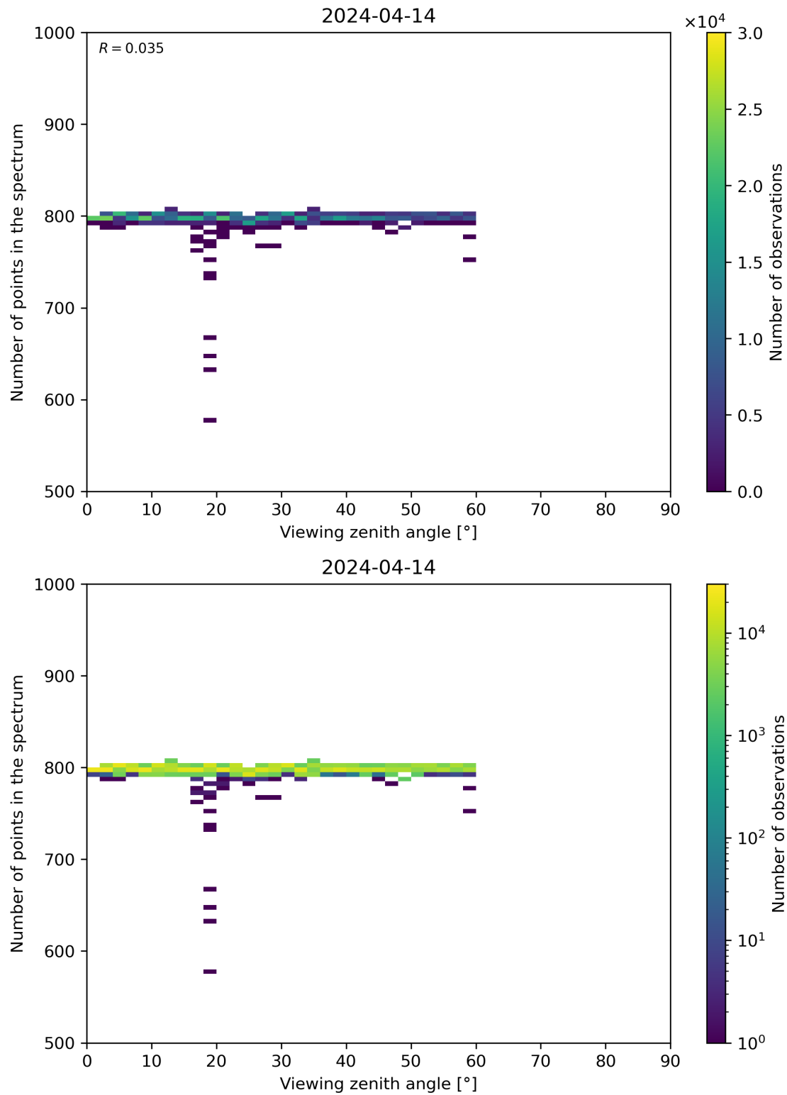
Figure 114: Scatter density plot of “Viewing zenith angle” against “Number of points in the spectrum” for 2024-04-13 to 2024-04-15.
