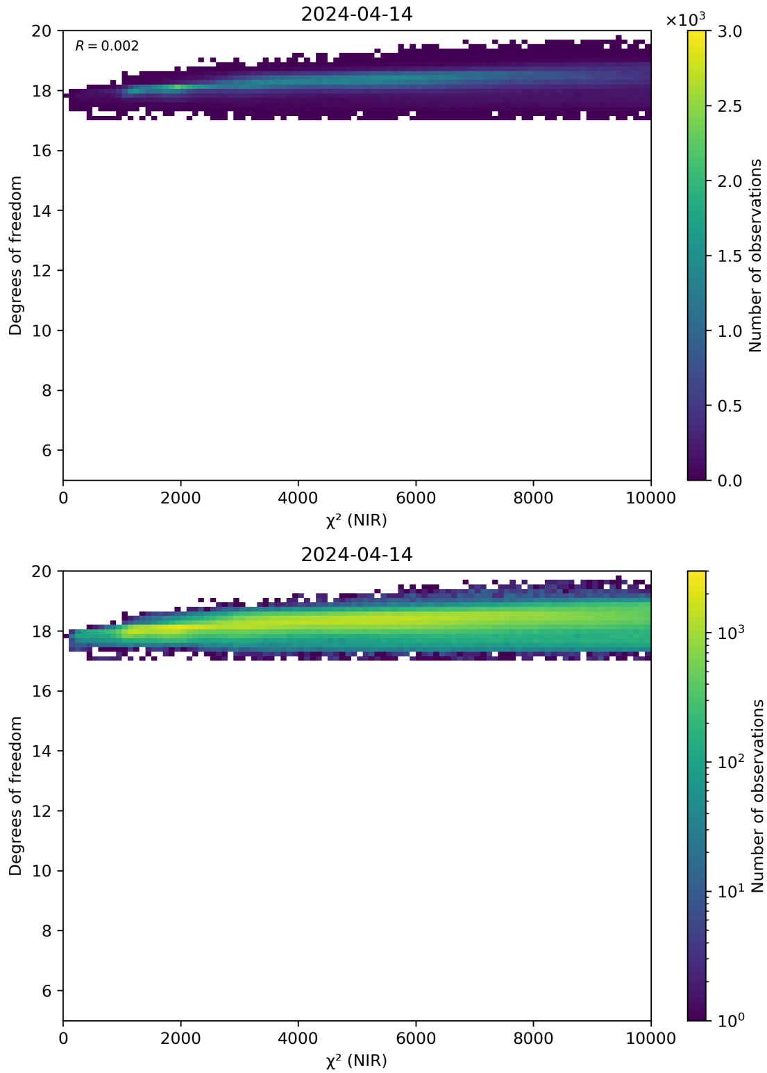
Figure 44: Scatter density plot of “ \chi^2 (NIR)” against “Degrees of freedom” for 2024-04-13 to 2024-04-15.
