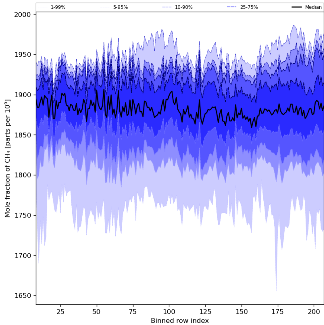
Figure 34: Along track statistics of “Mole fraction of CH 4 ” for 2024-04-13 to 2024-04-15
