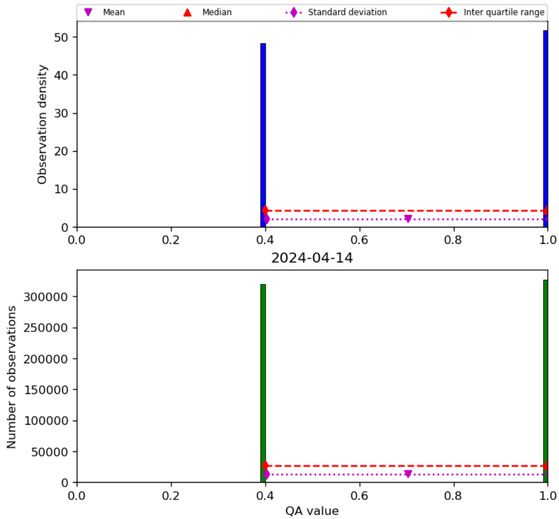
Figure 22: Histogram of “QA value” for 2024-04-13 to 2024-04-15
