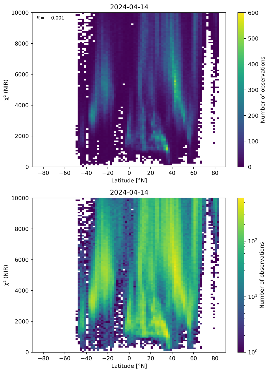
Figure 53: Scatter density plot of “Latitude” against “ \chi^2 (NIR)” for 2024-04-13 to 2024-04-15.
