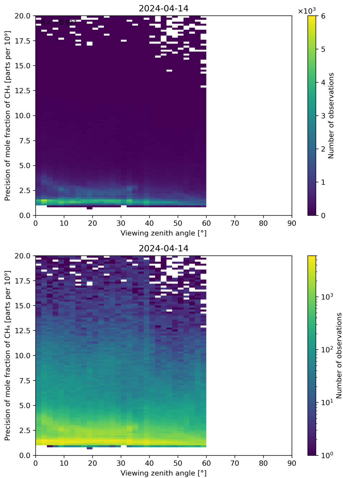
Figure 112: Scatter density plot of “Viewing zenith angle” against “Precision of mole fraction of CH 4 ” for 2024-04-13 to 2024-04-15.
