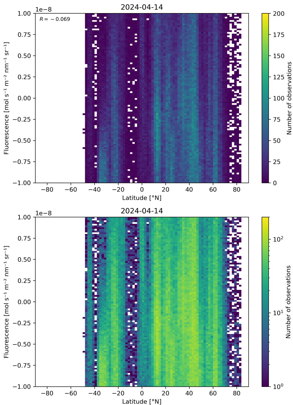
Figure 56: Scatter density plot of “Latitude” against “Fluorescence” for 2024-04-13 to 2024-04-15.
