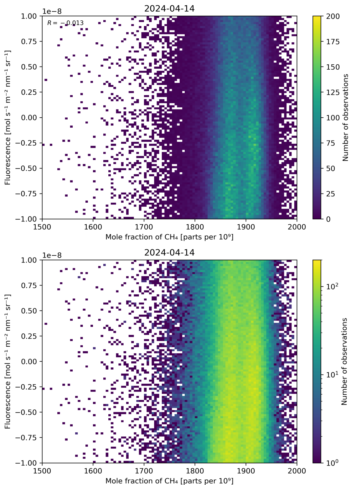
Figure 73: Scatter density plot of “Mole fraction of \text{CH}_4 ” against “Fluorescence” for 2024-04-13 to 2024-04-15.
