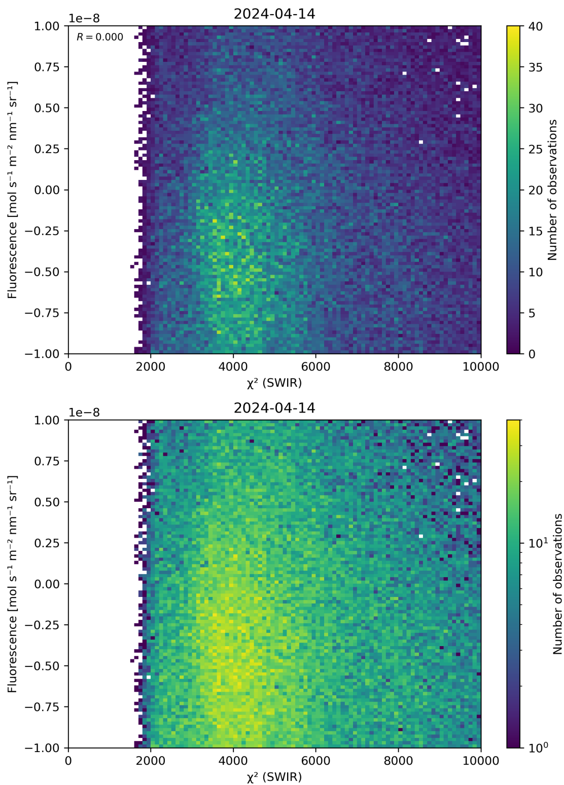
Figure 49: Scatter density plot of “ \chi^2 (SWIR)” against “Fluorescence” for 2024-04-13 to 2024-04-15.
