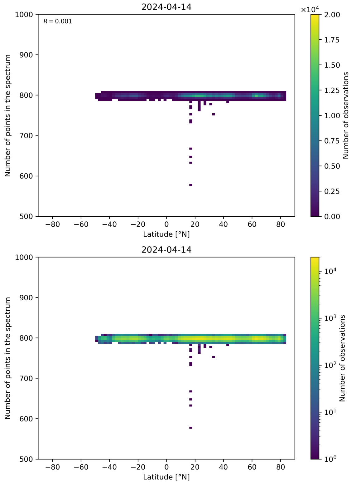
Figure 61: Scatter density plot of “Latitude” against “Number of points in the spectrum” for 2024-04-13 to 2024-04-15.
