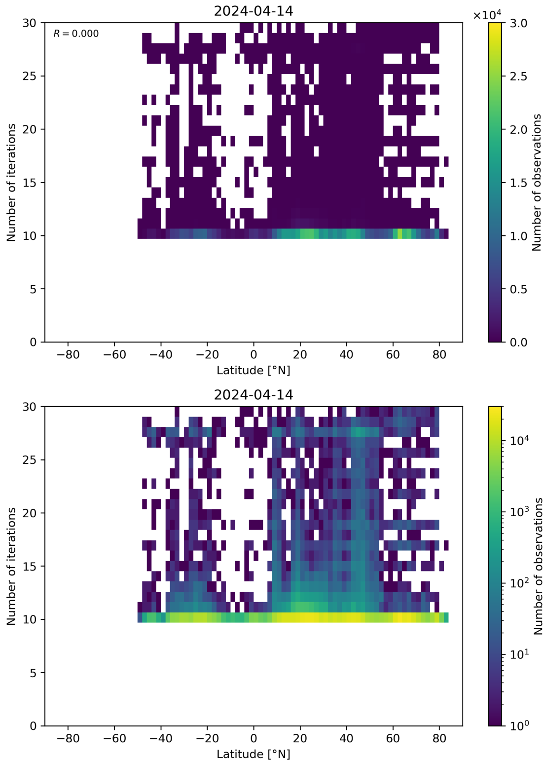
Figure 60: Scatter density plot of “Latitude” against “Number of iterations” for 2024-04-13 to 2024-04-15.
