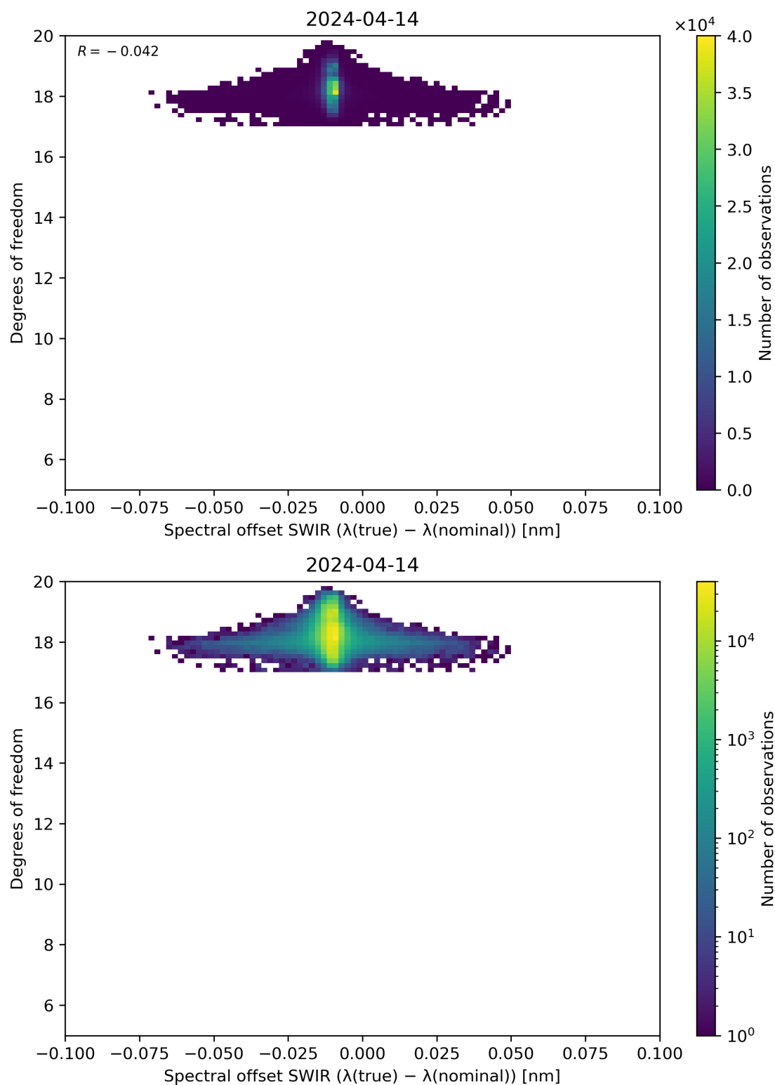
Figure 119: Scatter density plot of “Spectral offset SWIR ( \lambda(\text{true}) - \lambda(\text{nominal}) )” against “Degrees of freedom” for 2024-04-13 to 2024-04-15.
