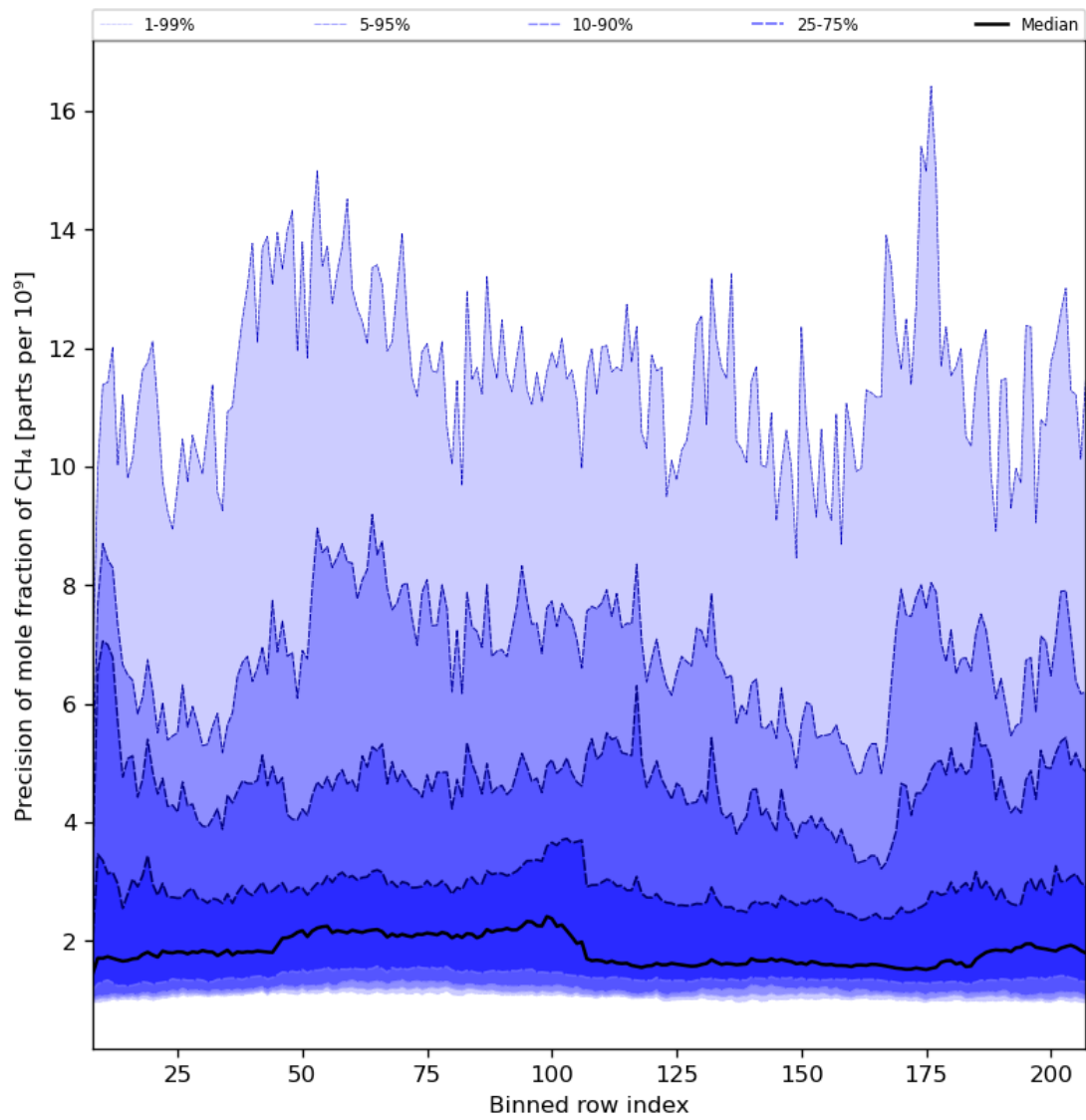
Figure 35: Along track statistics of “Precision of mole fraction of CH 4 ” for 2024-04-13 to 2024-04-15
