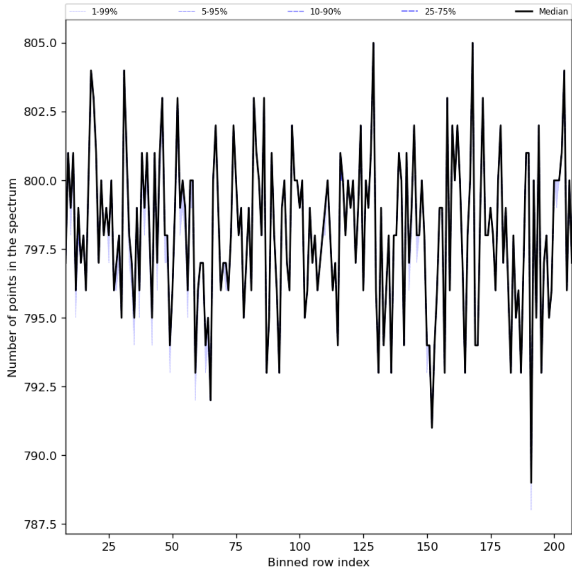
Figure 37: Along track statistics of “Number of points in the spectrum” for 2024-04-13 to 2024-04-15
