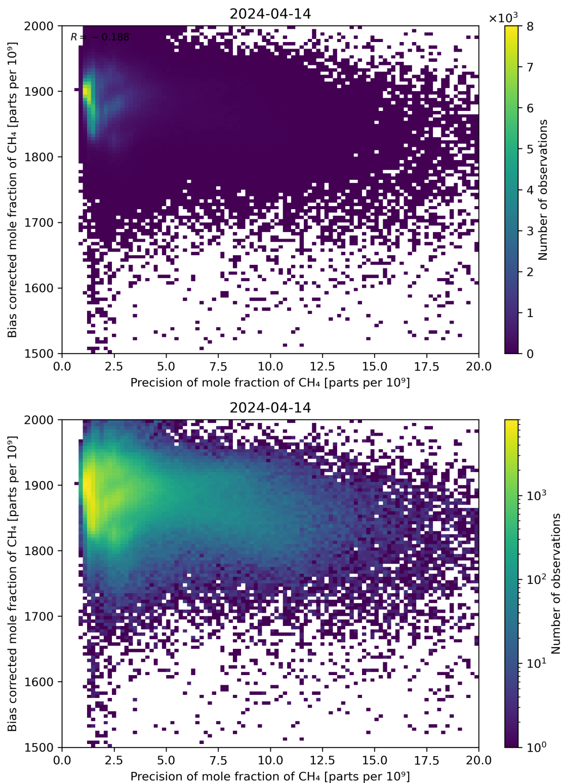
Figure 82: Scatter density plot of “Precision of mole fraction of CH 4 ” against “Bias corrected mole fraction of CH 4 ” for 2024-04-13 to 2024-04-15.
