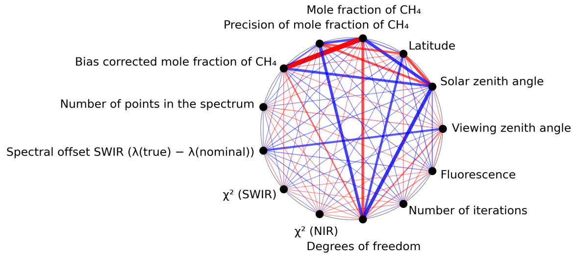
Figure 1: Map of correlation graph for 2024-04-13 to 2024-04-15.
