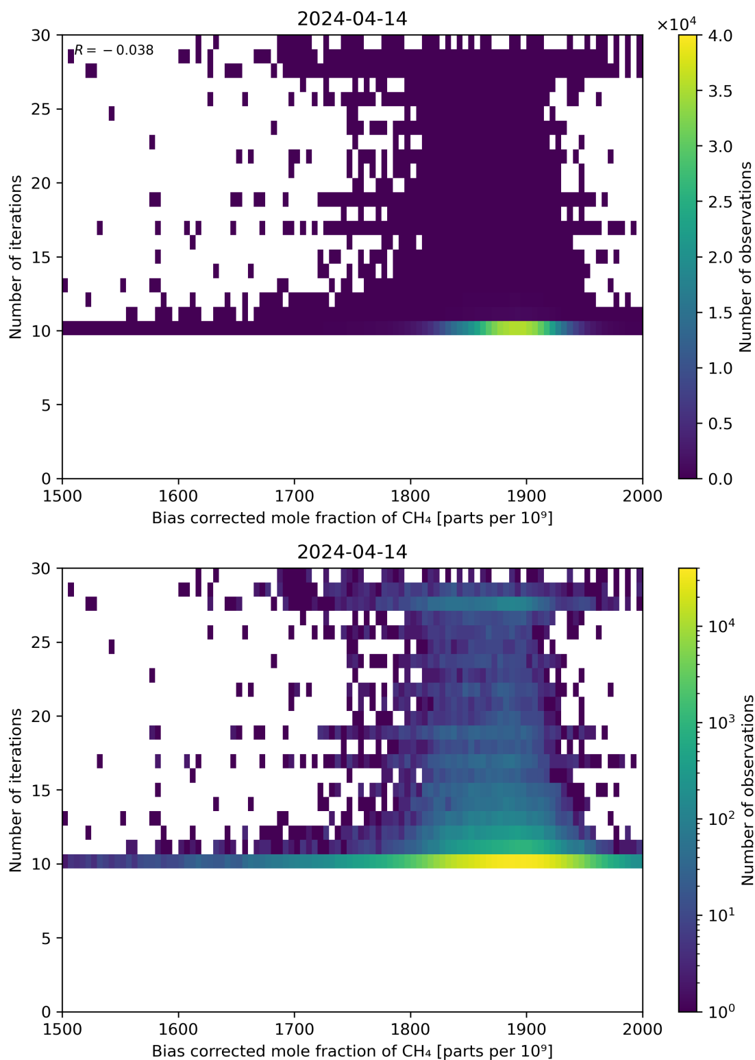
Figure 67: Scatter density plot of “Bias corrected mole fraction of CH 4 ” against “Number of iterations” for 2024-04-13 to 2024-04-15.
