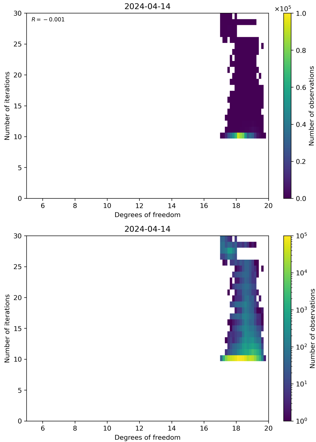
Figure 52: Scatter density plot of “Degrees of freedom” against “Number of iterations” for 2024-04-13 to 2024-04-15.
