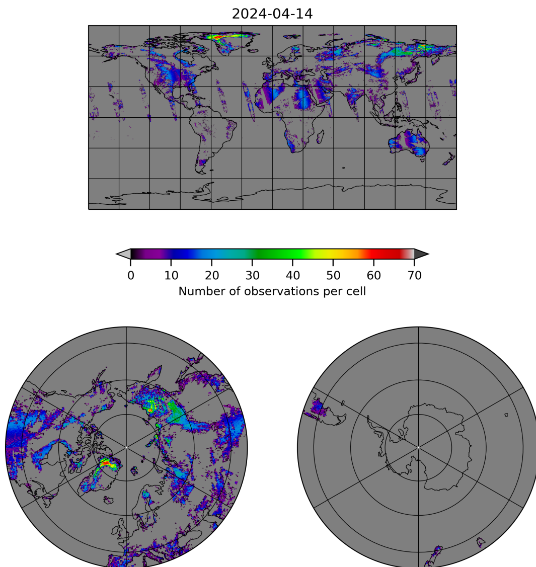
Figure 10: Map of the number of observations for 2024-04-13 to 2024-04-15
