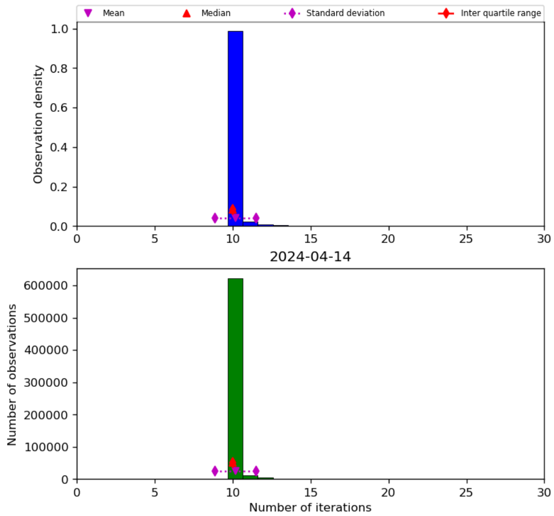
Figure 31: Histogram of “Number of iterations” for 2024-04-13 to 2024-04-15
