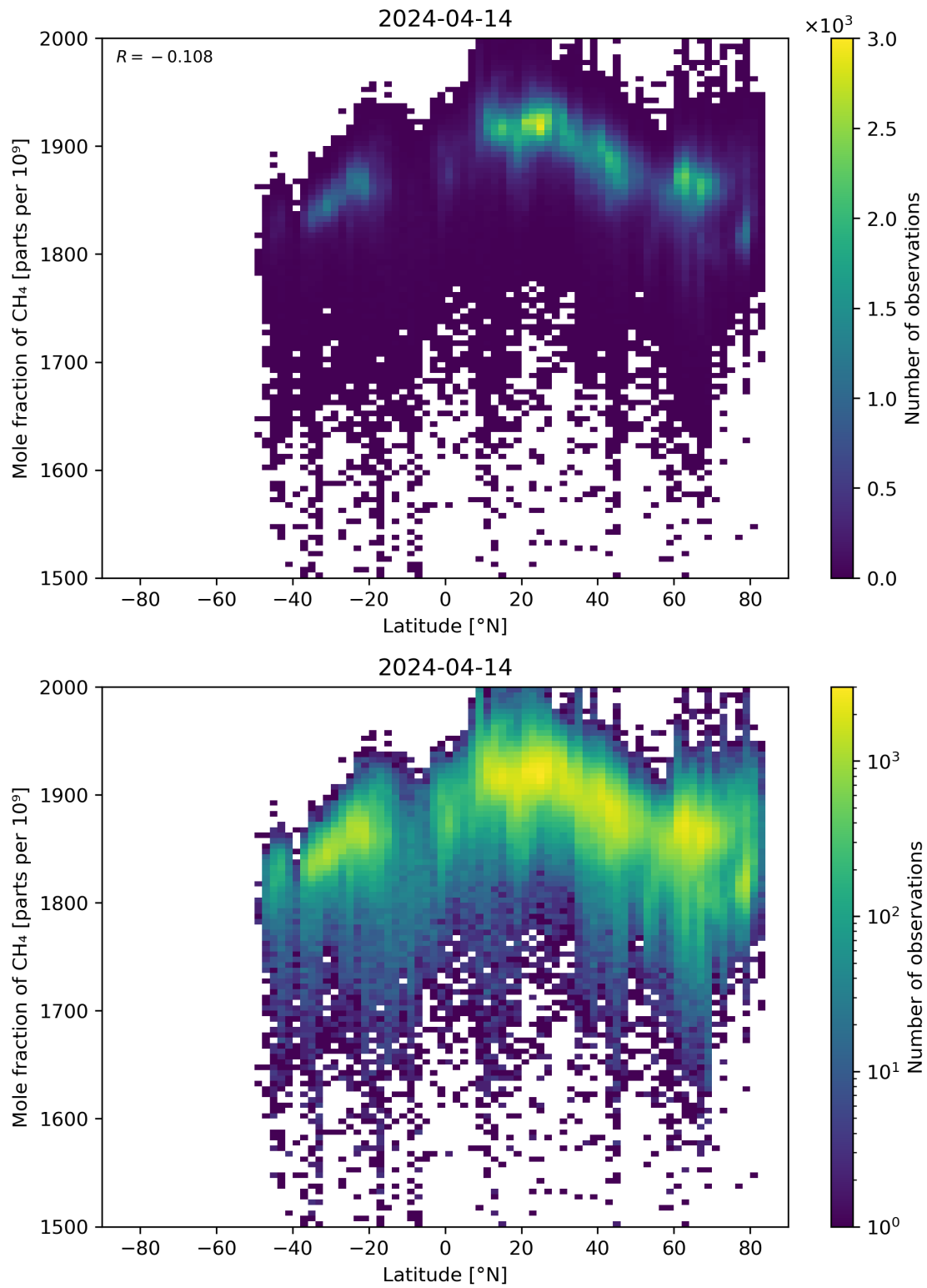
Figure 57: Scatter density plot of “Latitude” against “Mole fraction of CH 4 ” for 2024-04-13 to 2024-04-15.
