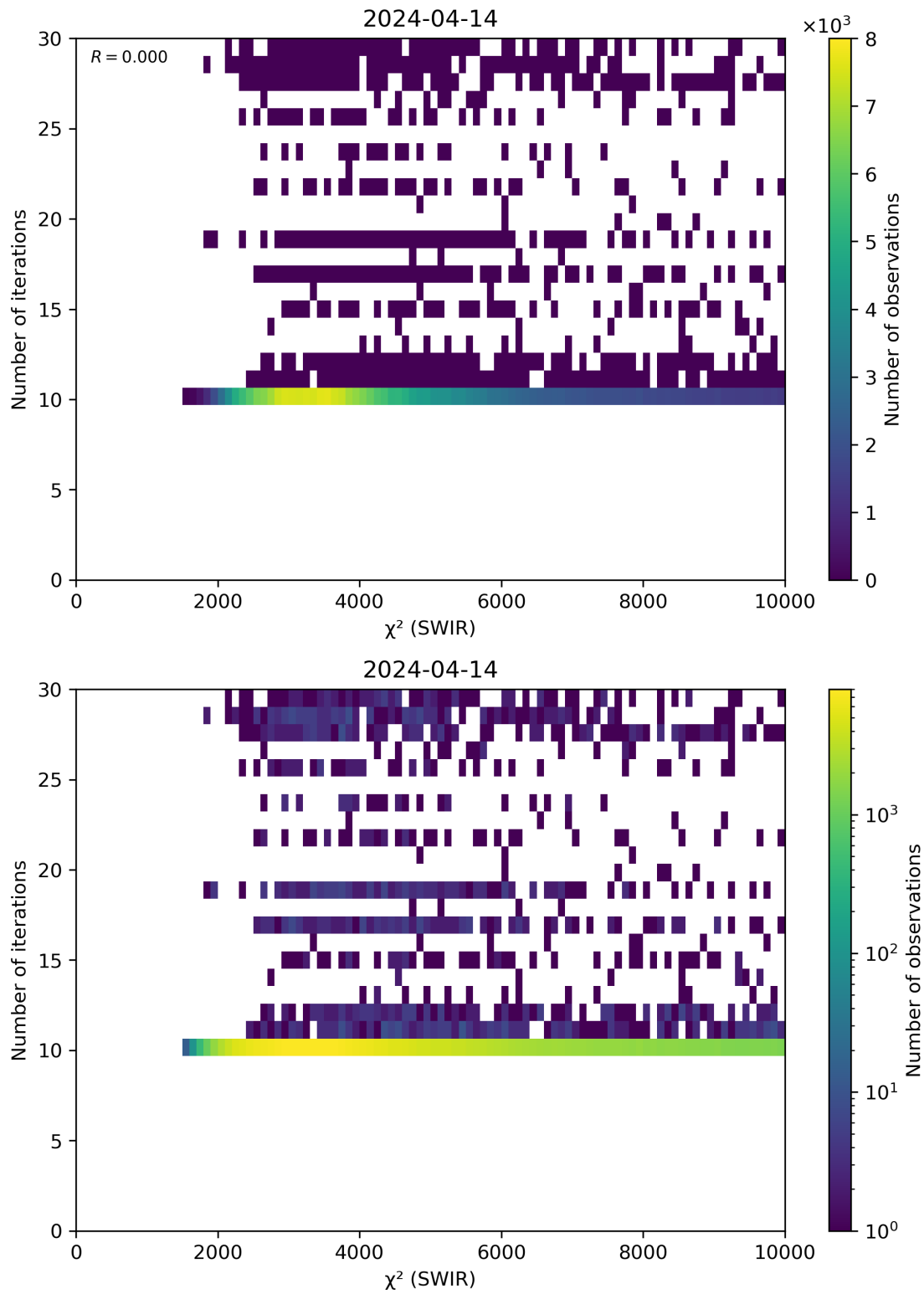
Figure 50: Scatter density plot of “ \chi^2 (SWIR)” against “Number of iterations” for 2024-04-13 to 2024-04-15.
