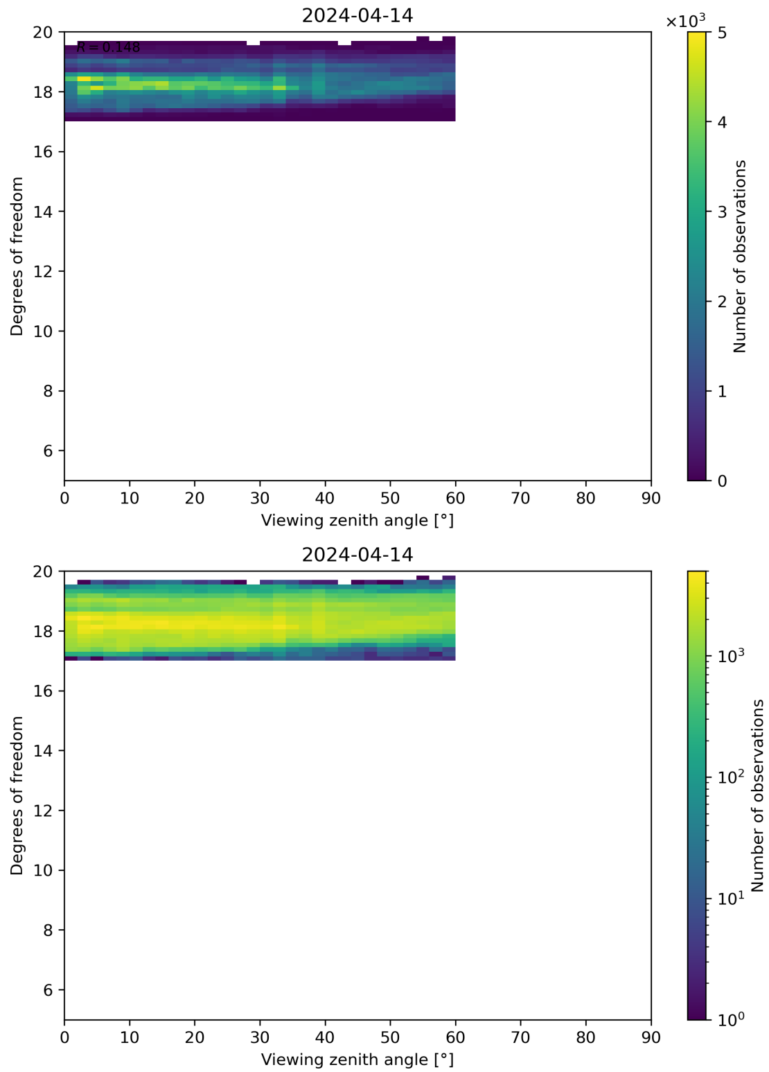
Figure 107: Scatter density plot of “Viewing zenith angle” against “Degrees of freedom” for 2024-04-13 to 2024-04-15.
