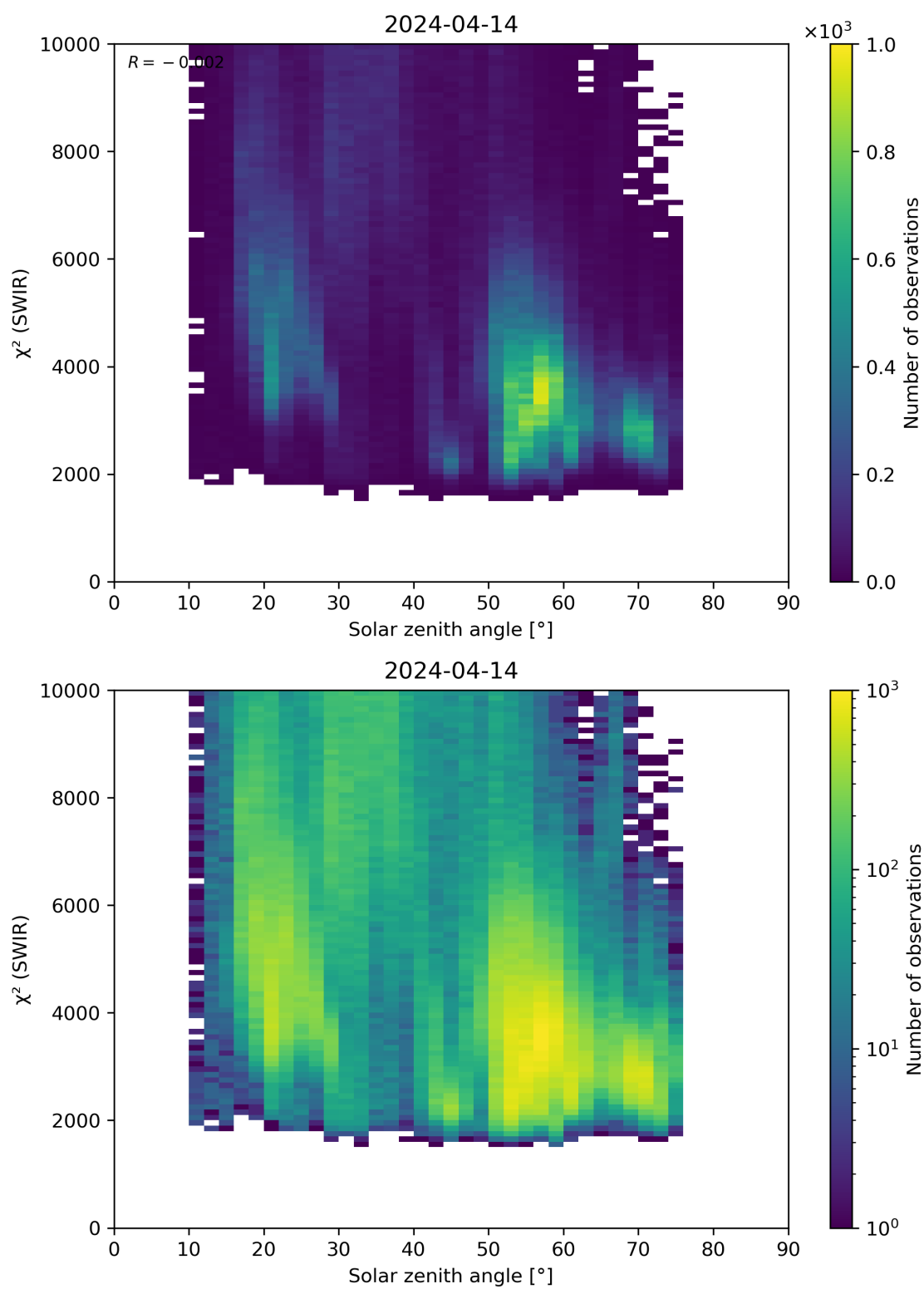
Figure 95: Scatter density plot of “Solar zenith angle” against “ \chi^2 (SWIR)” for 2024-04-13 to 2024-04-15.
