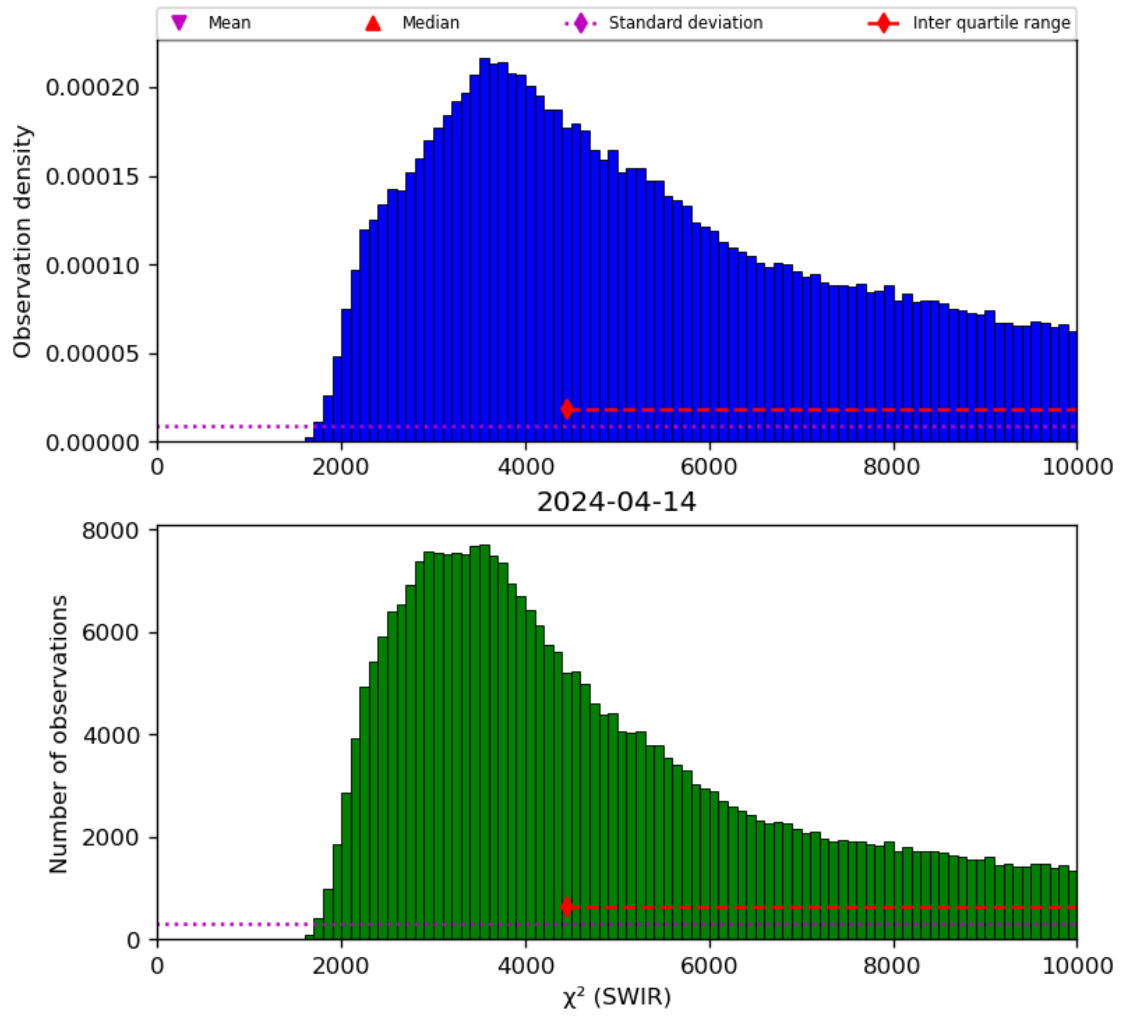
Figure 28: Histogram of “ \chi^2 (SWIR)” for 2024-04-13 to 2024-04-15
