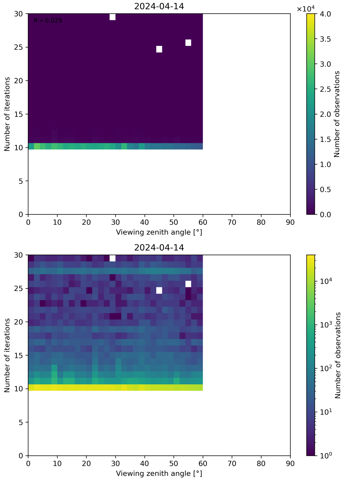
Figure 113: Scatter density plot of “Viewing zenith angle” against “Number of iterations” for 2024-04-13 to 2024-04-15.
