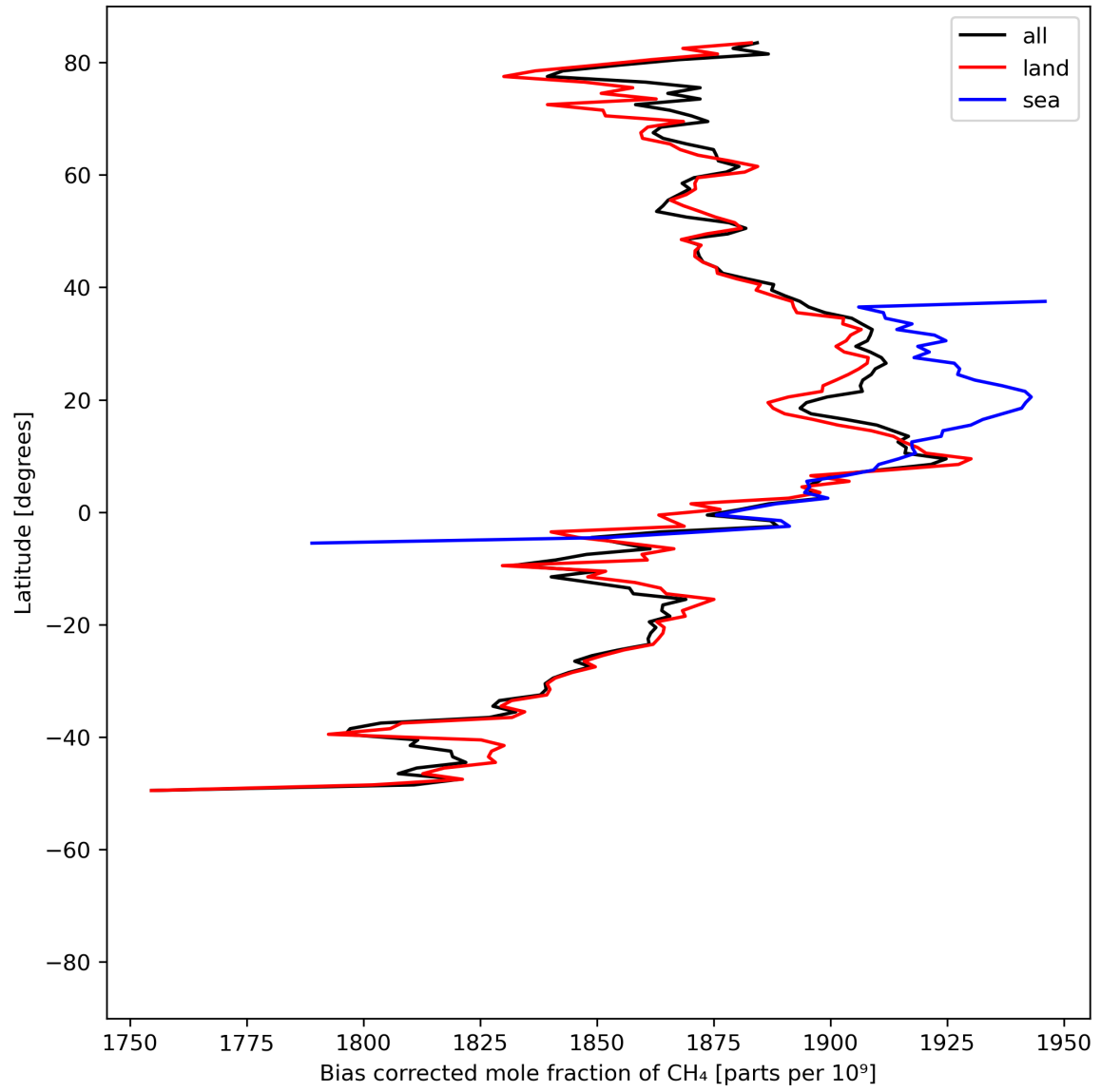
Figure 14: Zonal average of “Bias corrected mole fraction of \text{CH}_4 ” for 2024-04-13 to 2024-04-15.
