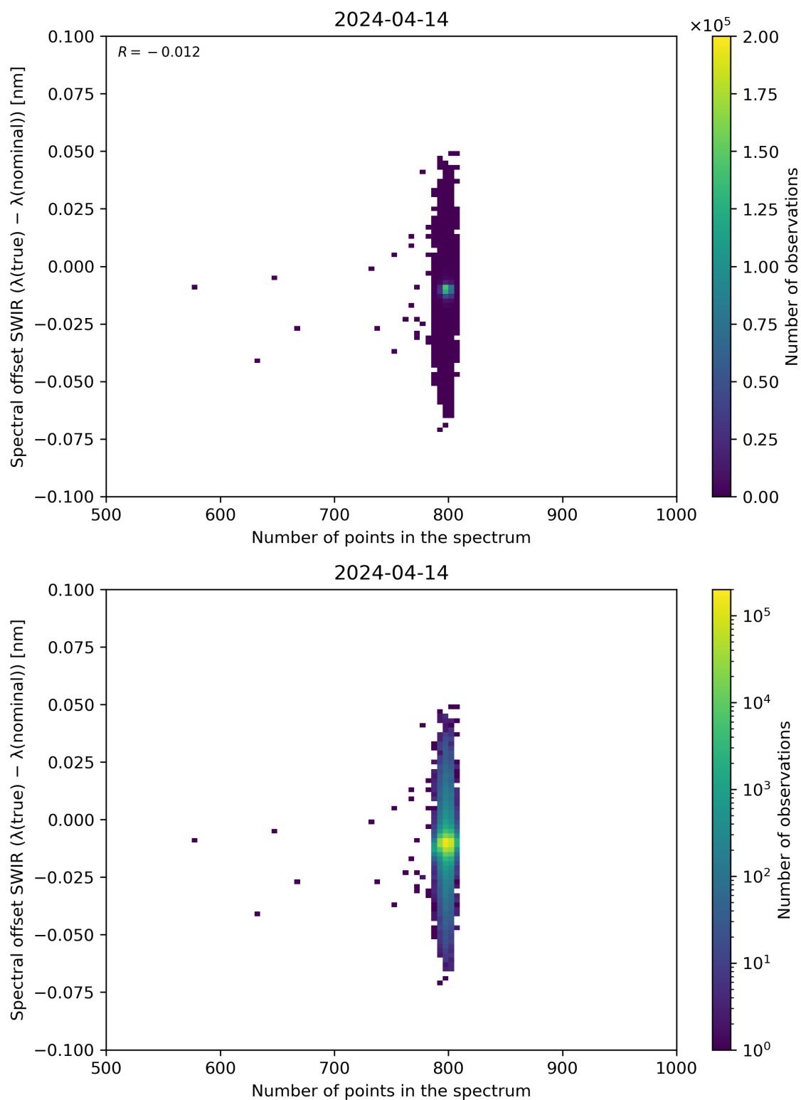
Figure 93: Scatter density plot of “Number of points in the spectrum” against “Spectral offset SWIR ( \lambda(\text{true}) - \lambda(\text{nominal}) )” for 2024-04-13 to 2024-04-15.
