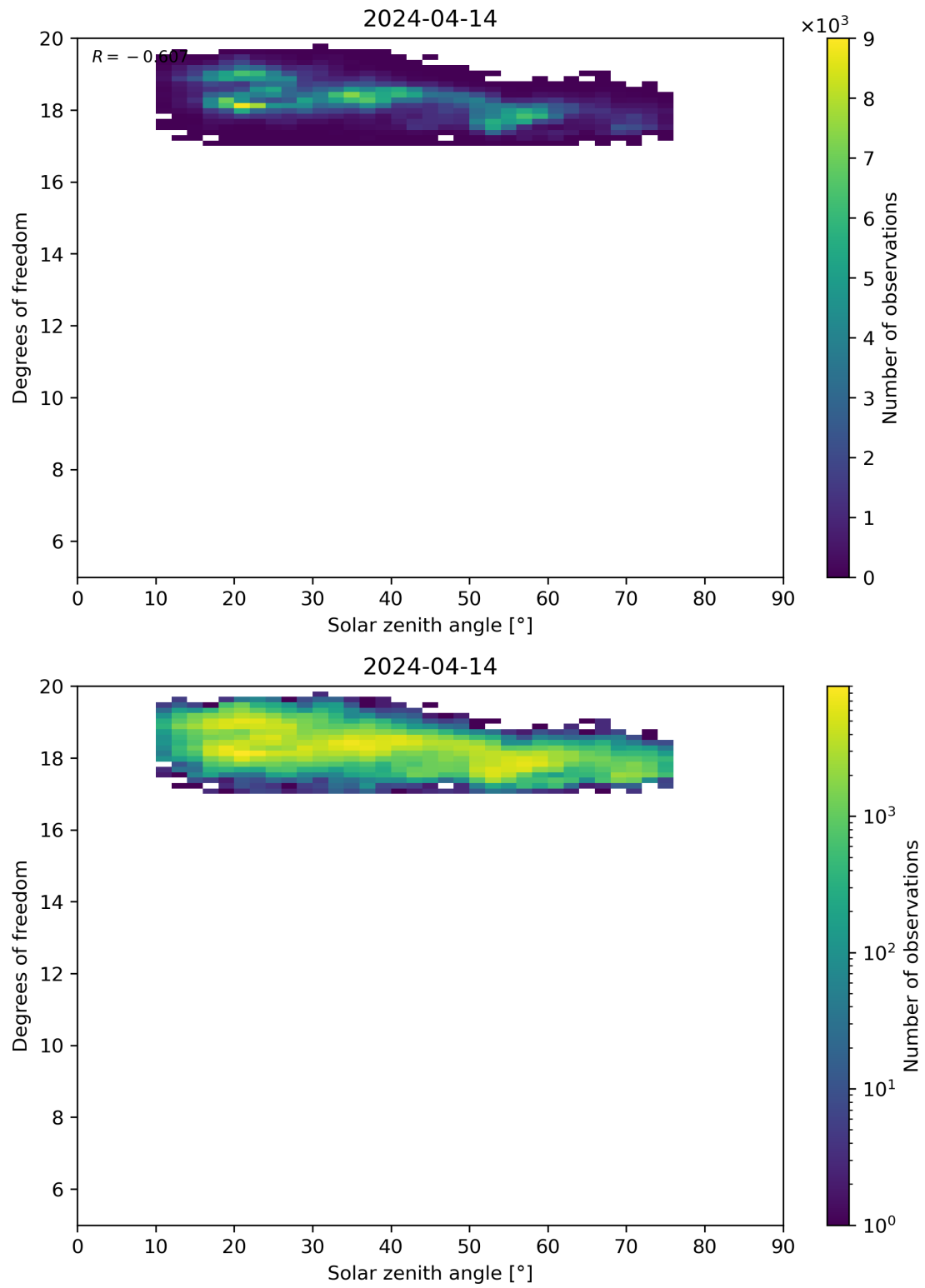
Figure 96: Scatter density plot of “Solar zenith angle” against “Degrees of freedom” for 2024-04-13 to 2024-04-15.
