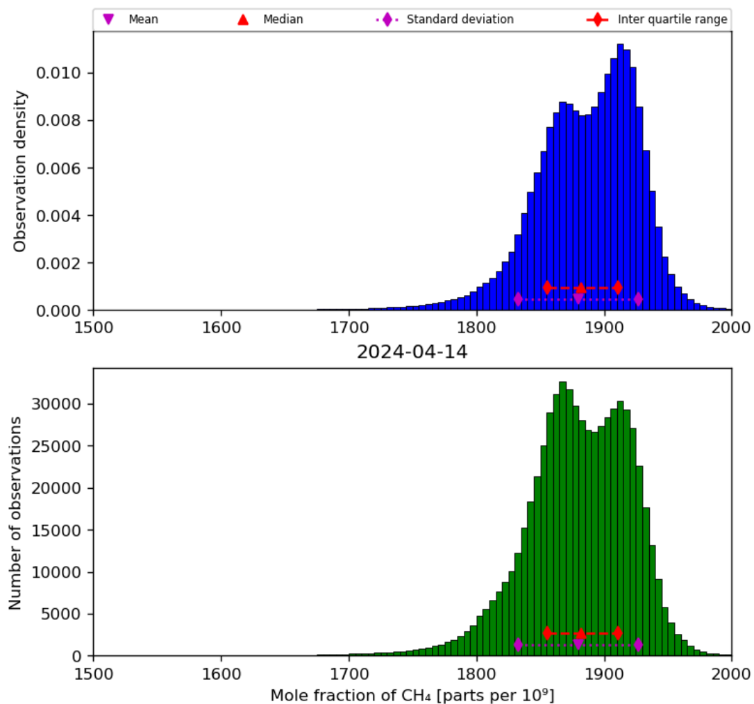
Figure 23: Histogram of “Mole fraction of CH 4 ” for 2024-04-13 to 2024-04-15
