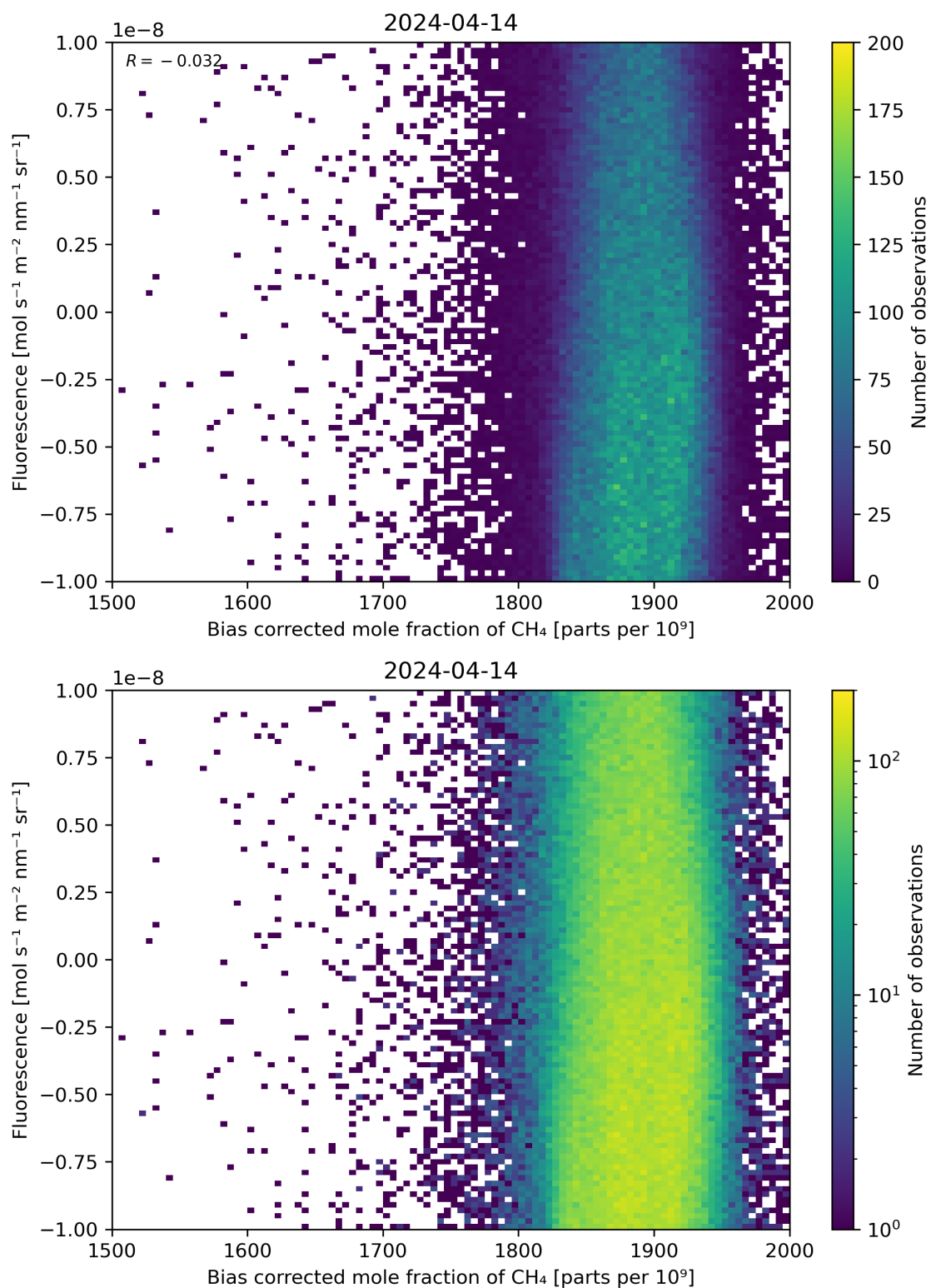
Figure 66: Scatter density plot of “Bias corrected mole fraction of \text{CH}_4 ” against “Fluorescence” for 2024-04-13 to 2024-04-15.
