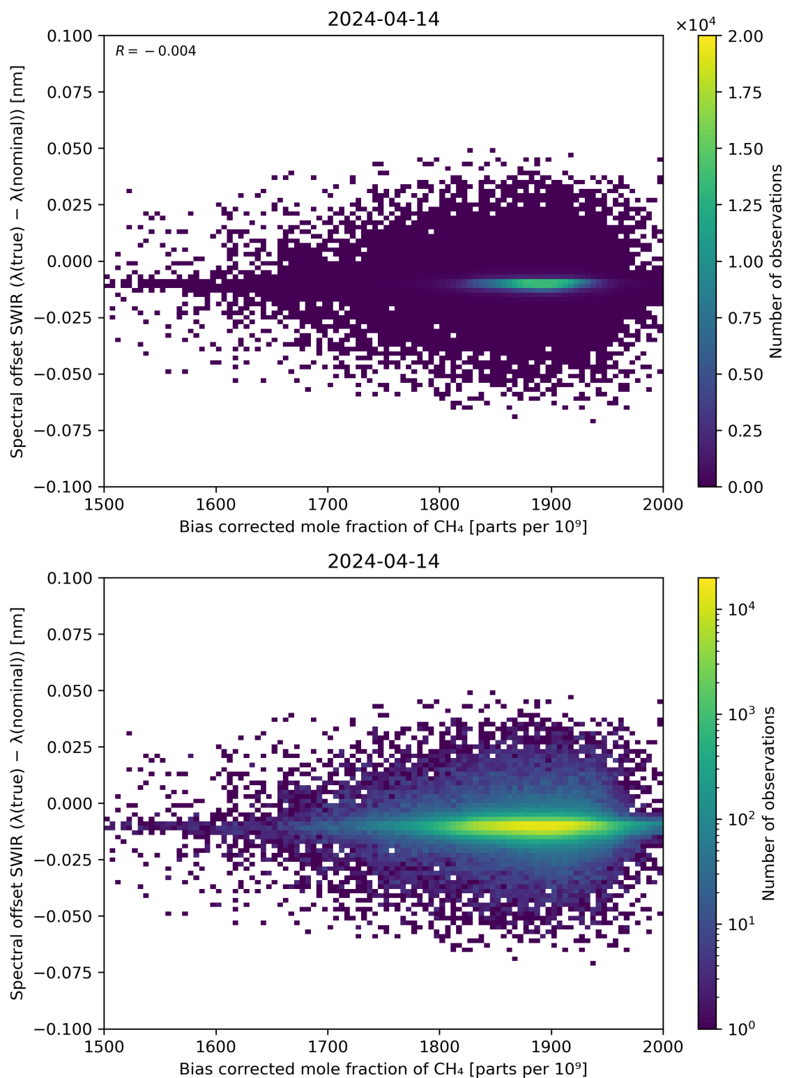
Figure 69: Scatter density plot of “Bias corrected mole fraction of \text{CH}_4 ” against “Spectral offset SWIR ( \lambda(\text{true}) - \lambda(\text{nominal}) )” for 2024-04-13 to 2024-04-15.
