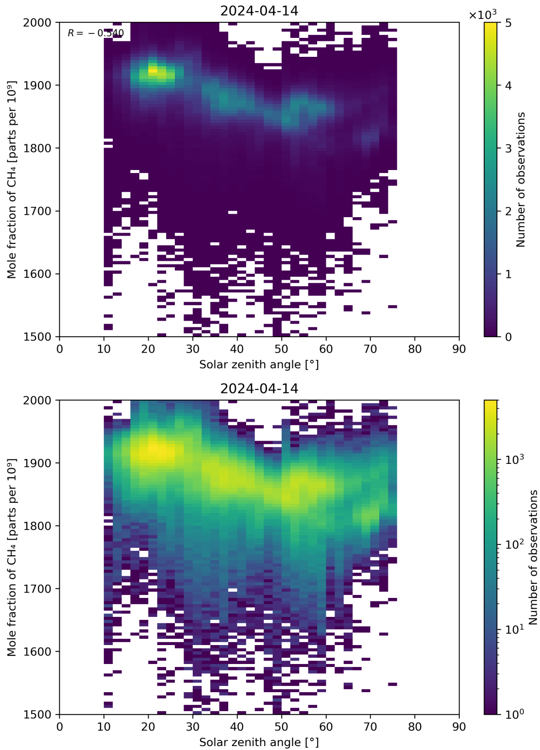
Figure 99: Scatter density plot of “Solar zenith angle” against “Mole fraction of CH 4 ” for 2024-04-13 to 2024-04-15.
