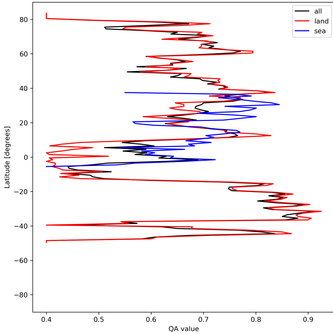
Figure 11: Zonal average of “QA value” for 2024-04-13 to 2024-04-15.
