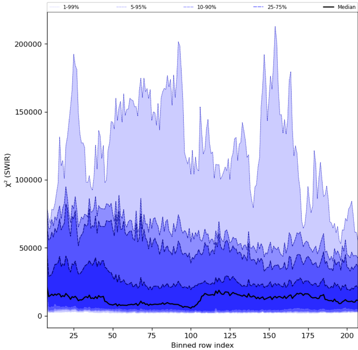
Figure 39: Along track statistics of “ \chi^2 (SWIR)” for 2024-04-13 to 2024-04-15
