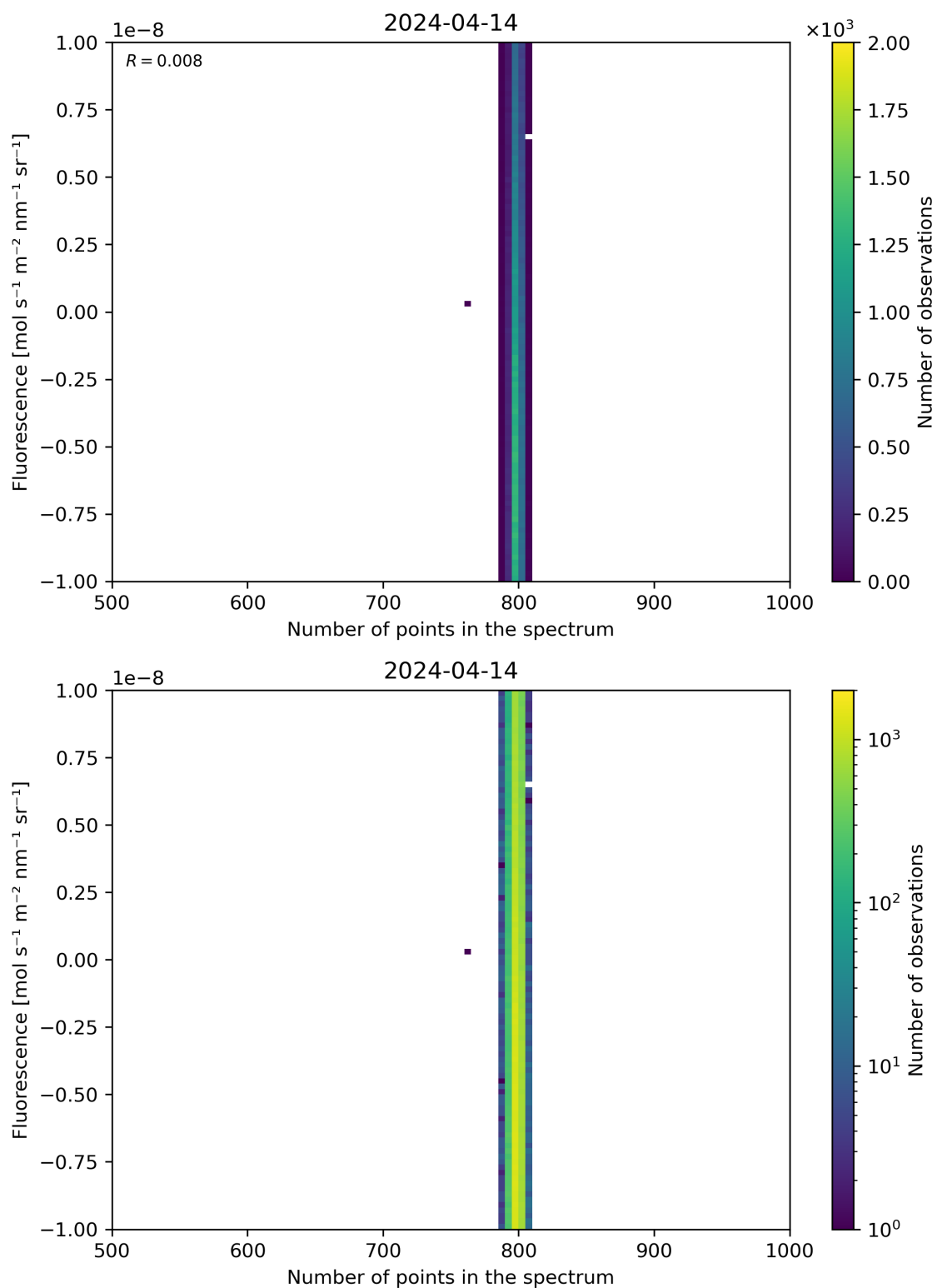
Figure 91: Scatter density plot of “Number of points in the spectrum” against “Fluorescence” for 2024-04-13 to 2024-04-15.
