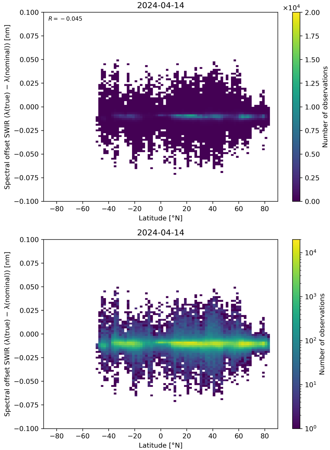
Figure 62: Scatter density plot of “Latitude” against “Spectral offset SWIR ( \lambda(\text{true}) - \lambda(\text{nominal}) )” for 2024-04-13 to 2024-04-15.
