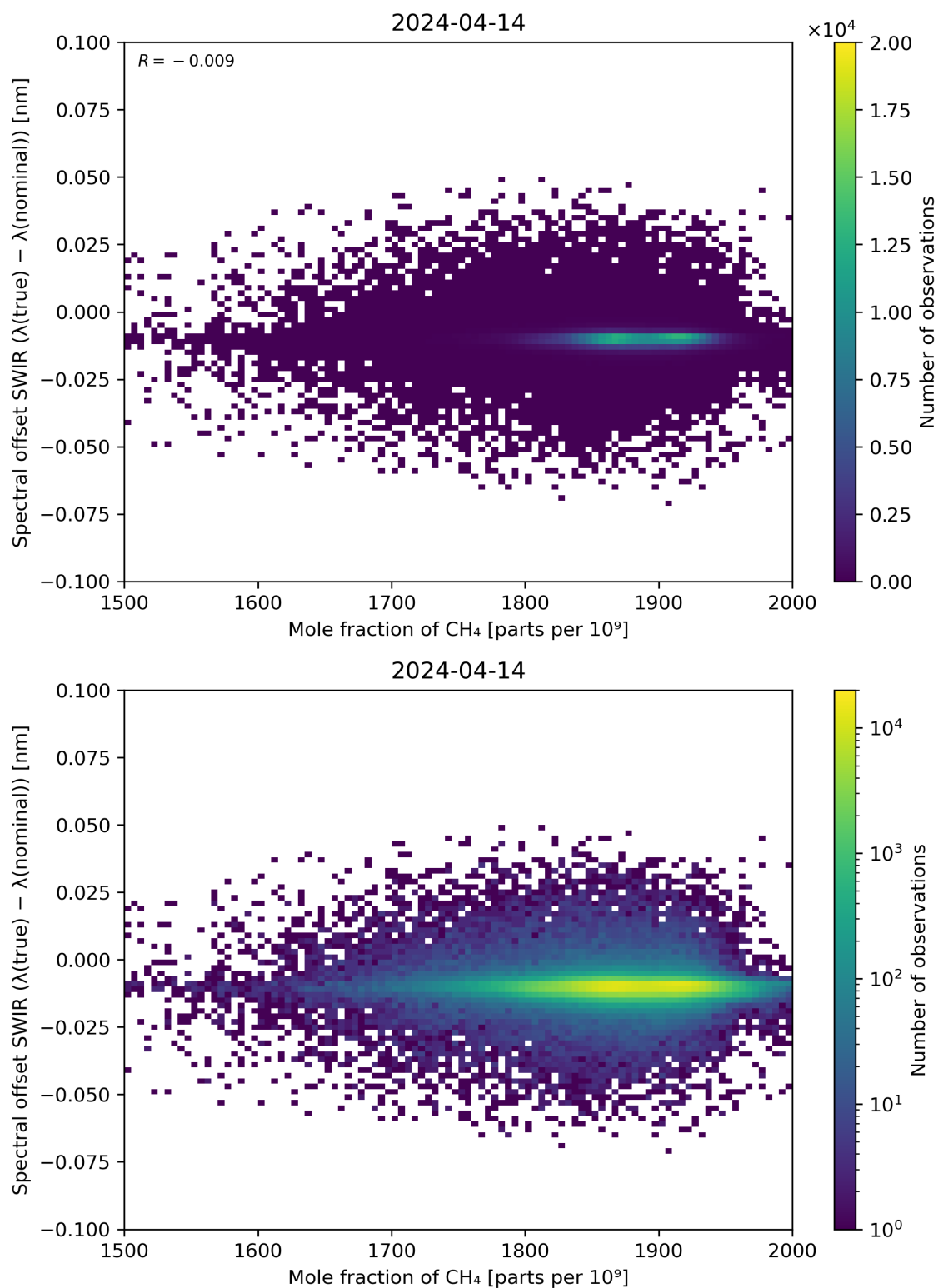
Figure 86: Scatter density plot of “Mole fraction of CH 4 ” against “Spectral offset SWIR ( \lambda(\text{true}) - \lambda(\text{nominal}) )” for 2024-04-13 to 2024-04-15.
