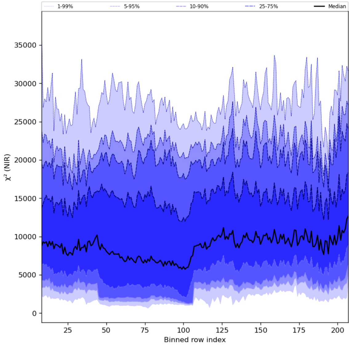
Figure 40: Along track statistics of “ \chi^2 (NIR)” for 2024-04-13 to 2024-04-15
