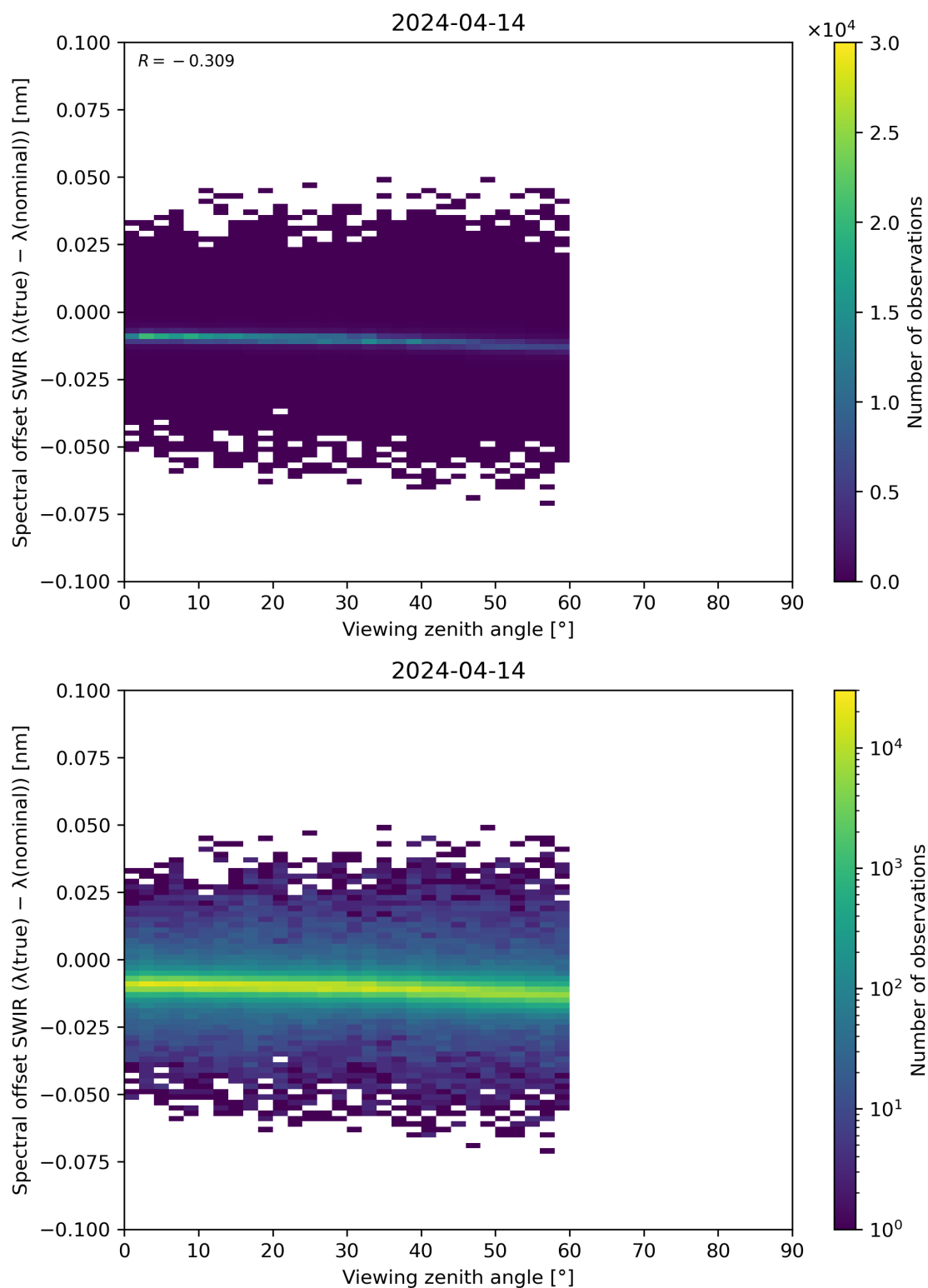
Figure 116: Scatter density plot of “Viewing zenith angle” against “Spectral offset SWIR ( \lambda(\text{true}) - \lambda(\text{nominal}) )” for 2024-04-13 to 2024-04-15.
