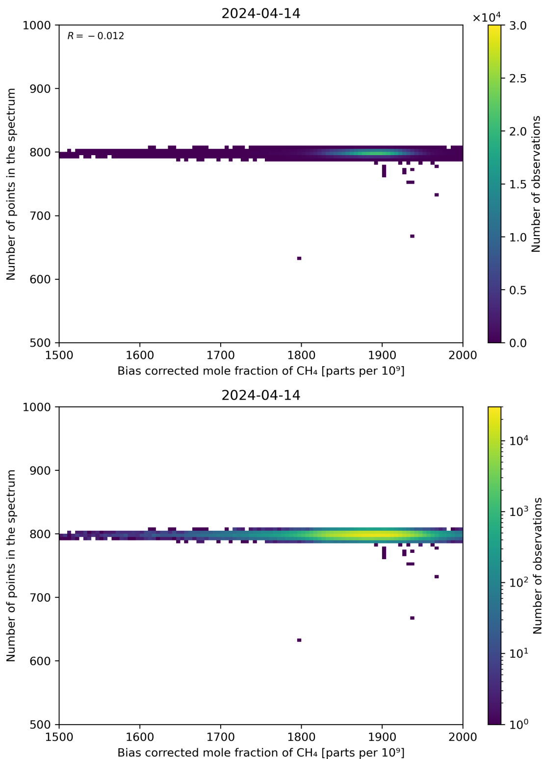
Figure 68: Scatter density plot of “Bias corrected mole fraction of CH 4 ” against “Number of points in the spectrum” for 2024-04-13 to 2024-04-15.
