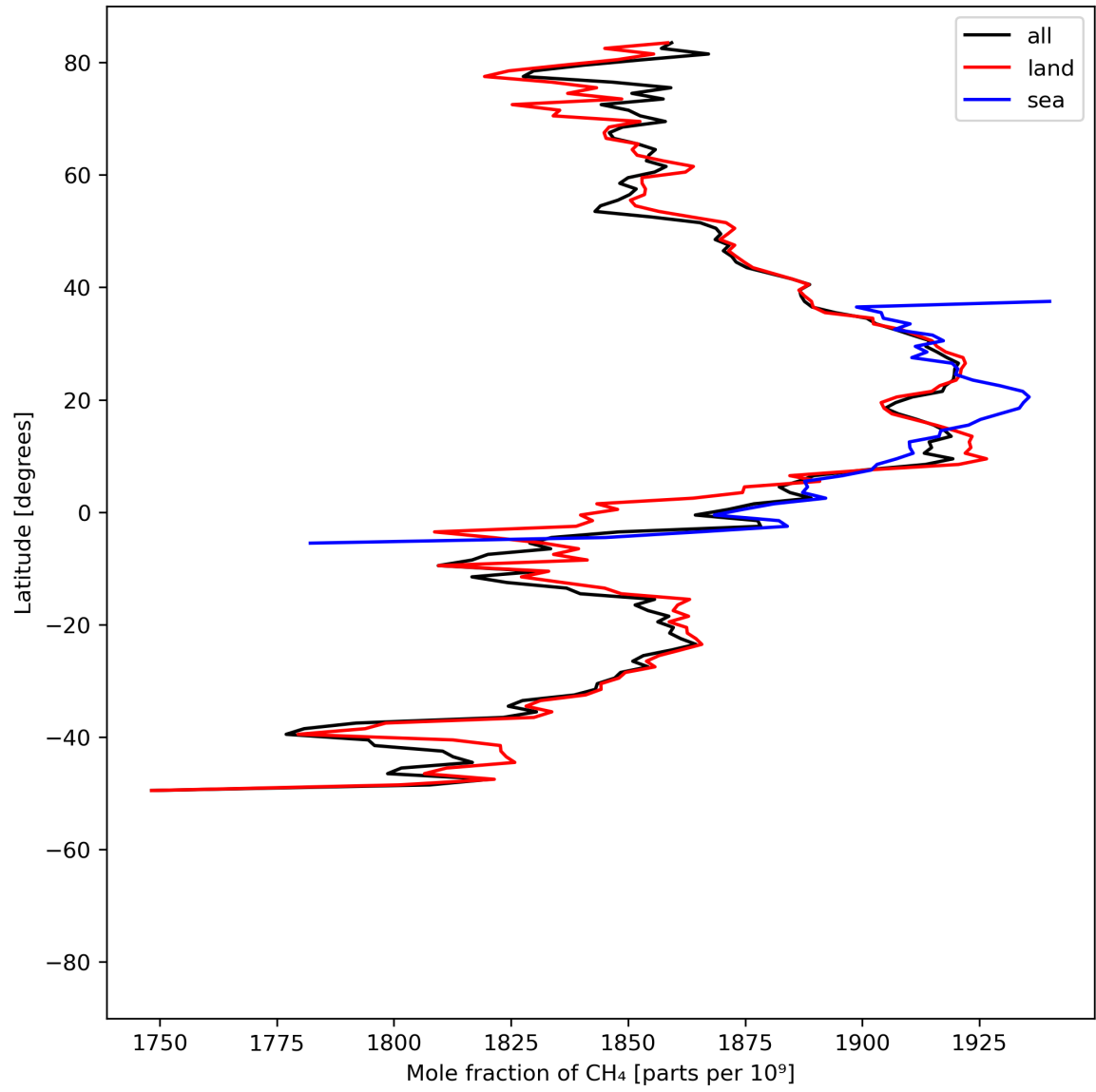
Figure 12: Zonal average of “Mole fraction of \text{CH}_4 ” for 2024-04-13 to 2024-04-15.
