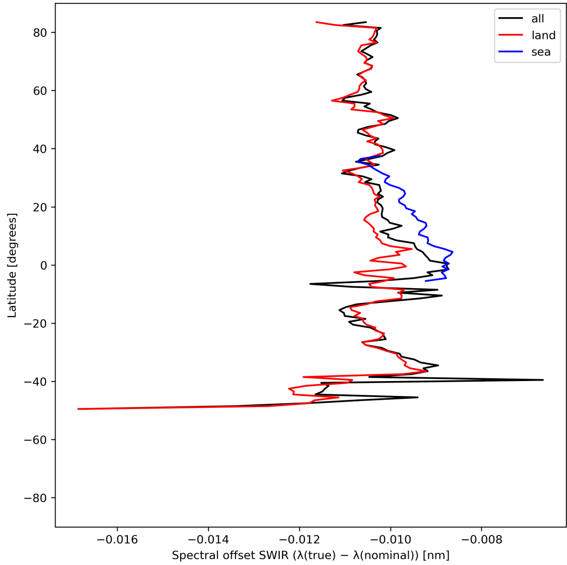
Figure 16: Zonal average of “Spectral offset SWIR ( \lambda(\text{true}) - \lambda(\text{nominal}) )” for 2024-04-13 to 2024-04-15.
