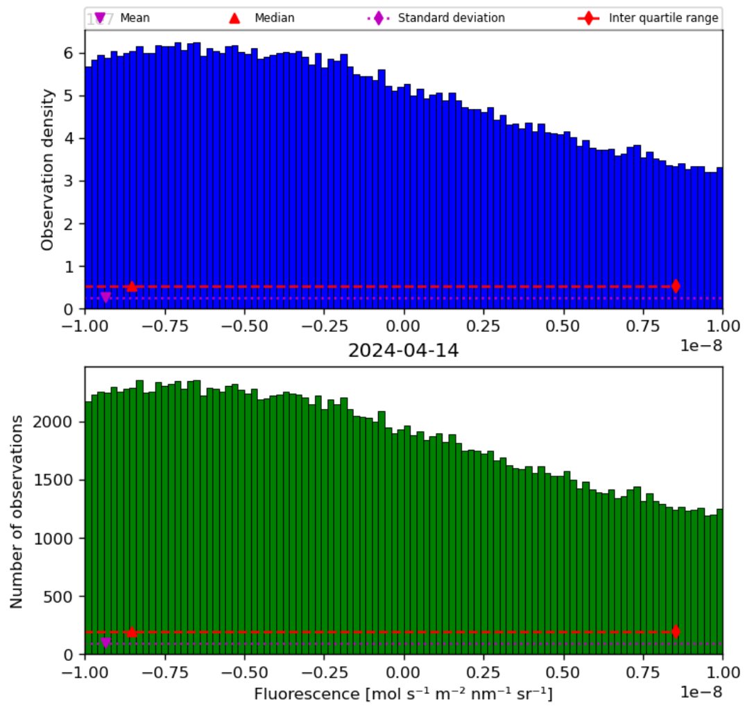
Figure 32: Histogram of “Fluorescence” for 2024-04-13 to 2024-04-15
