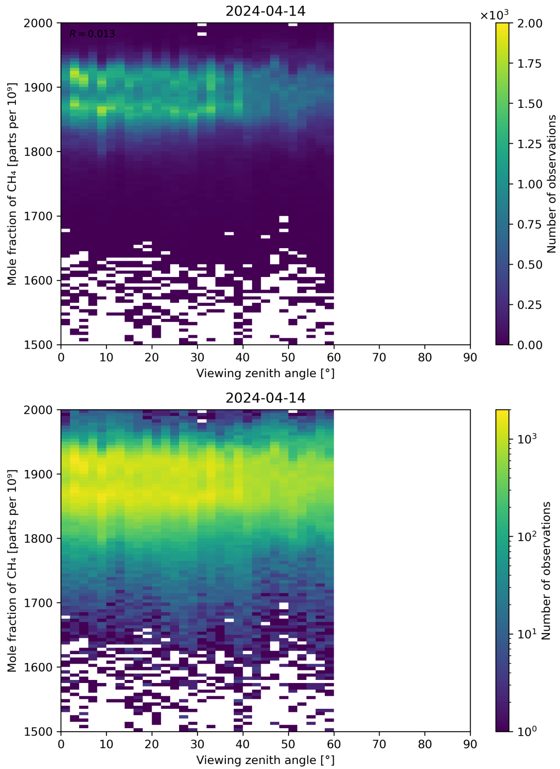
Figure 110: Scatter density plot of “Viewing zenith angle” against “Mole fraction of CH 4 ” for 2024-04-13 to 2024-04-15.
