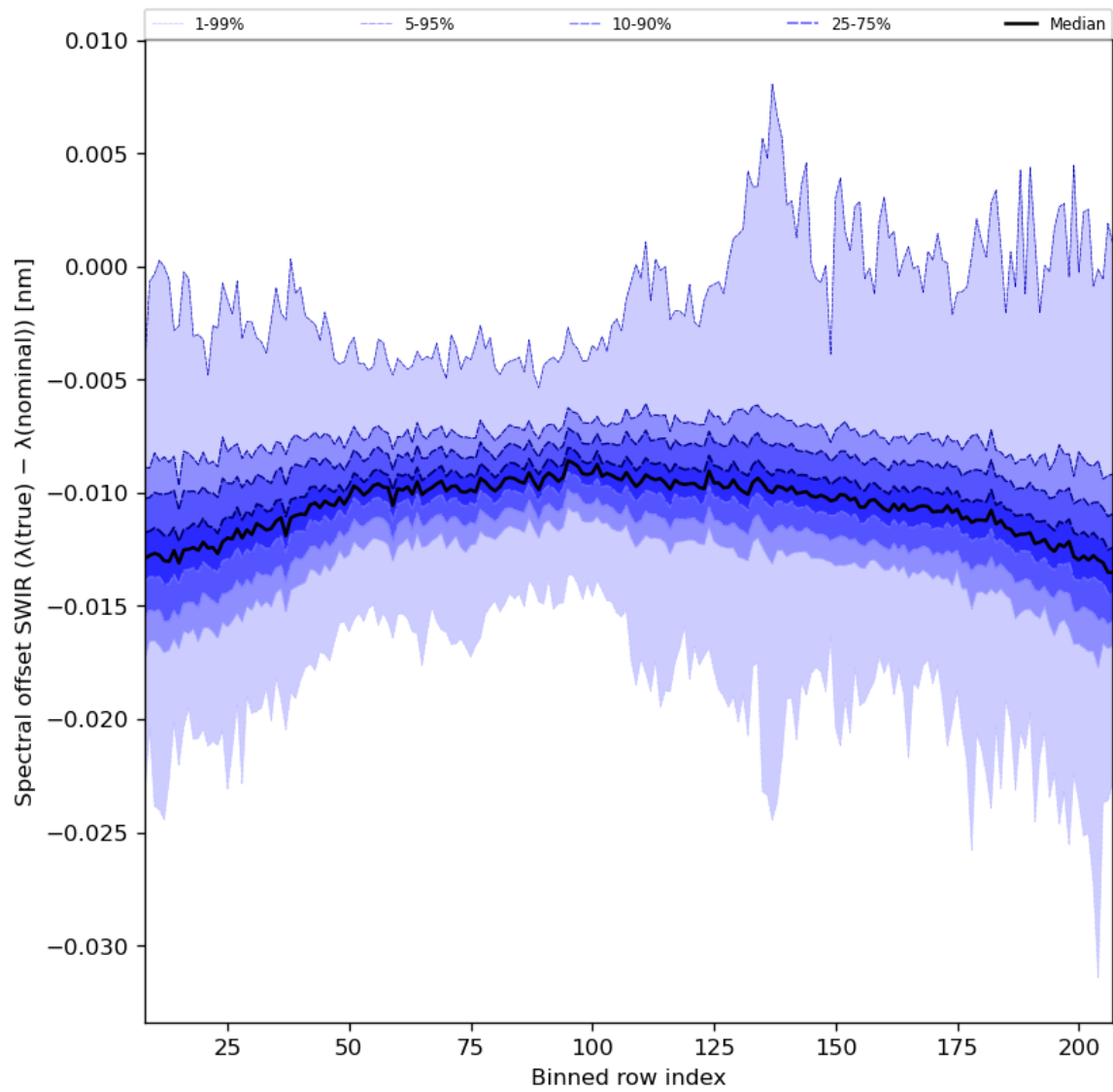
Figure 38: Along track statistics of “Spectral offset SWIR ( \lambda(\text{true}) - \lambda(\text{nominal}) )” for 2024-04-13 to 2024-04-15
