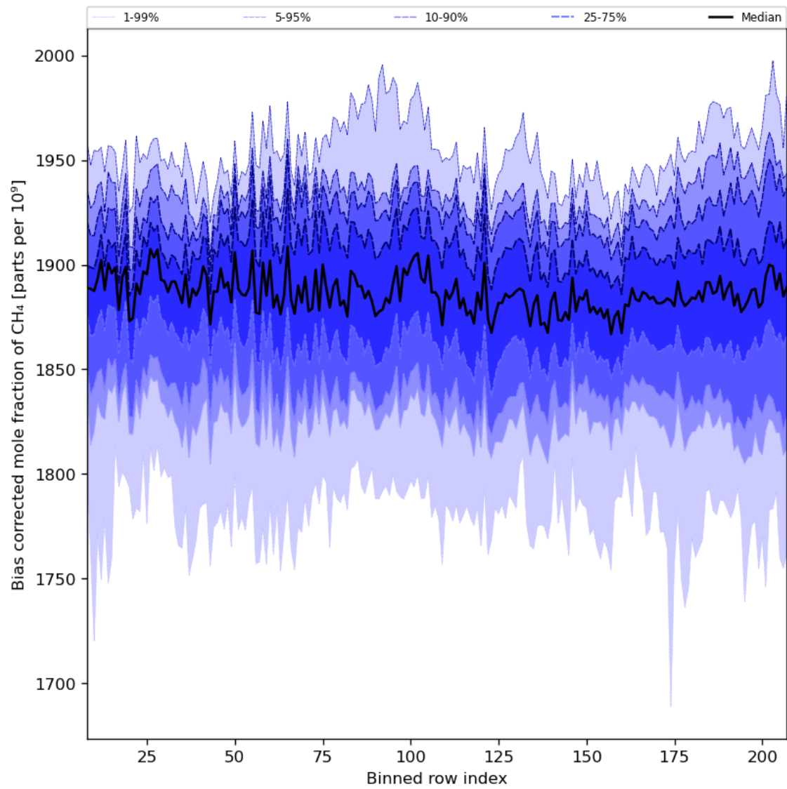
Figure 36: Along track statistics of “Bias corrected mole fraction of CH 4 ” for 2024-04-13 to 2024-04-15
