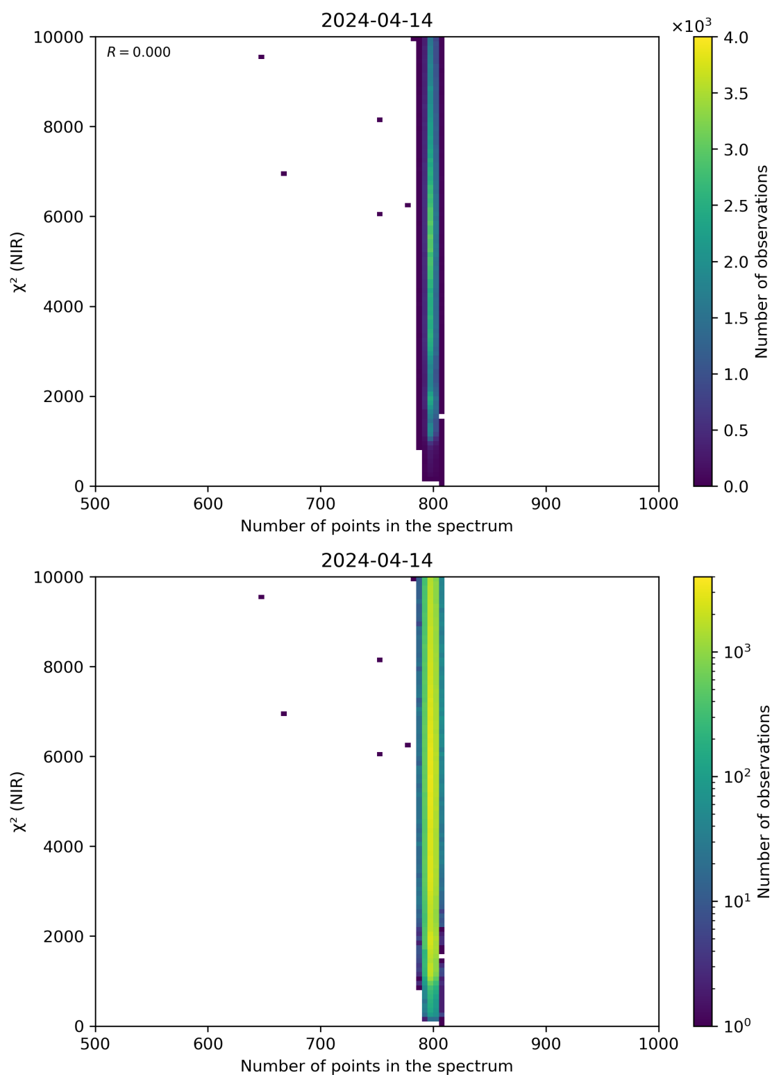
Figure 88: Scatter density plot of “Number of points in the spectrum” against “ \chi^2 (NIR)” for 2024-04-13 to 2024-04-15.
