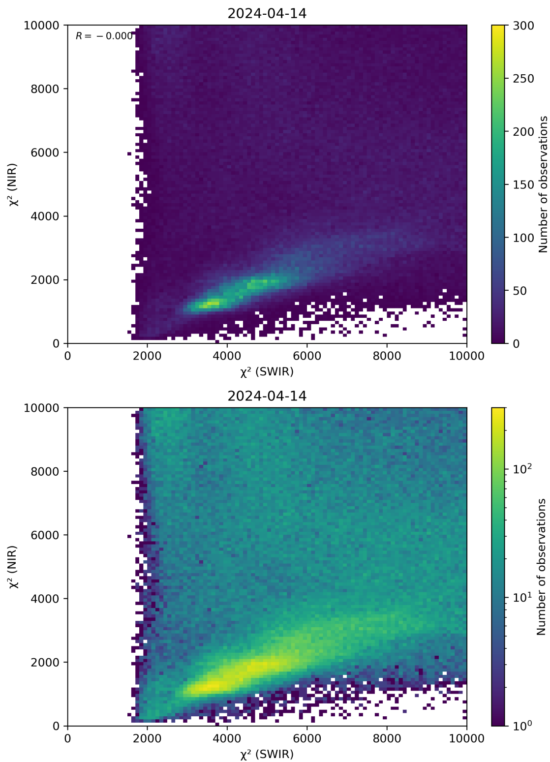
Figure 47: Scatter density plot of “ \chi^2 (SWIR)” against “ \chi^2 (NIR)” for 2024-04-13 to 2024-04-15.
