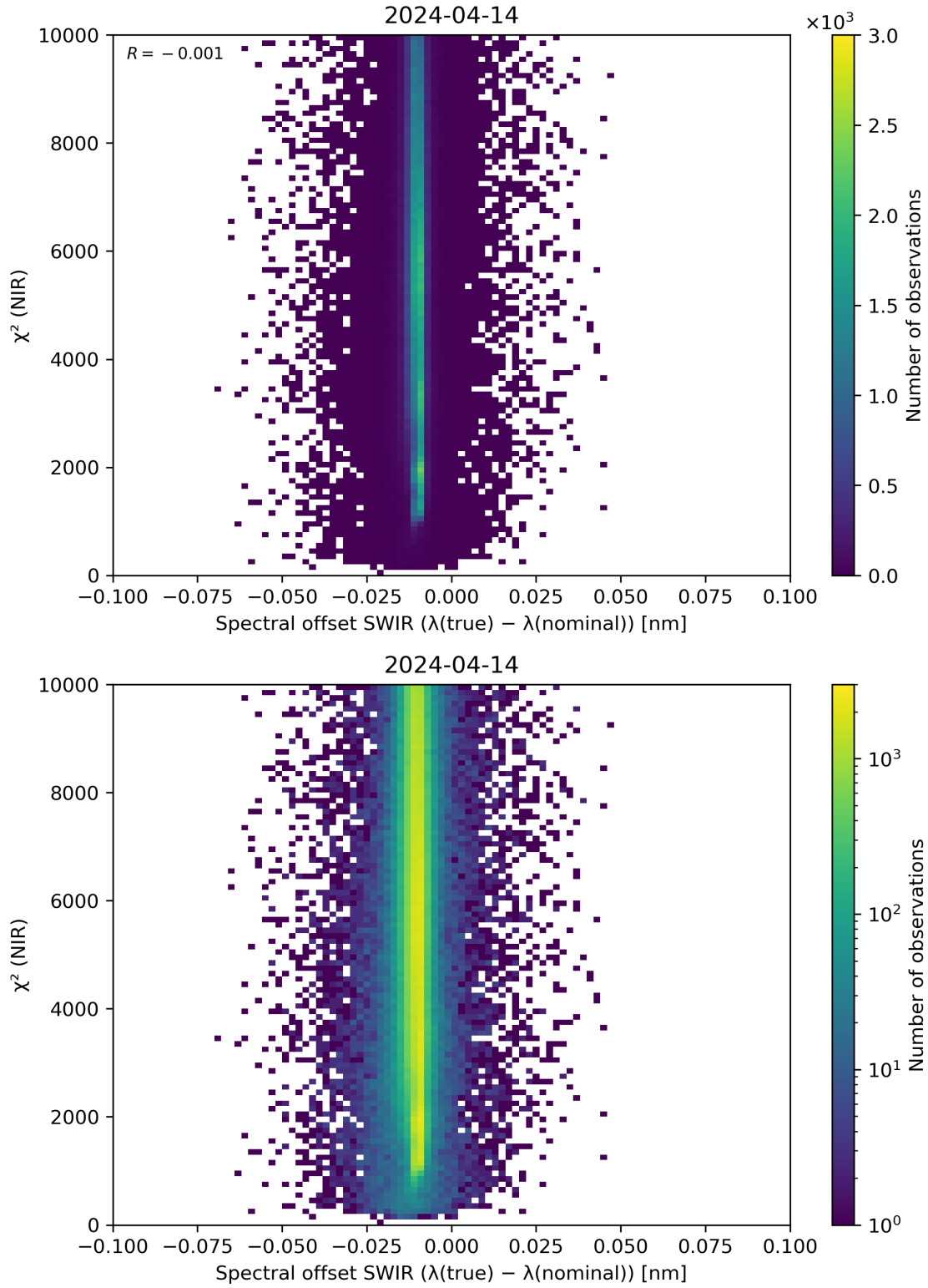
Figure 117: Scatter density plot of “Spectral offset SWIR ( \lambda(\text{true}) - \lambda(\text{nominal}) )” against “ \chi^2 (NIR)” for 2024-04-13 to 2024-04-15.
