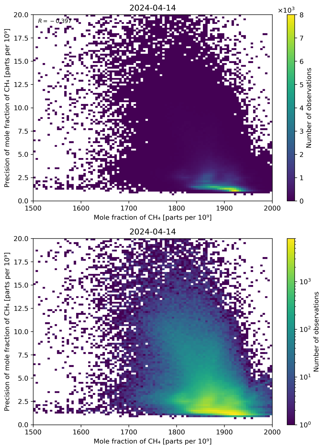
Figure 75: Scatter density plot of “Mole fraction of CH 4 ” against “Precision of mole fraction of CH 4 ” for 2024-04-13 to 2024-04-15.
