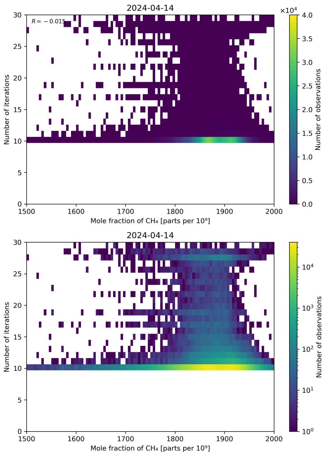
Figure 76: Scatter density plot of “Mole fraction of CH 4 ” against “Number of iterations” for 2024-04-13 to 2024-04-15.
