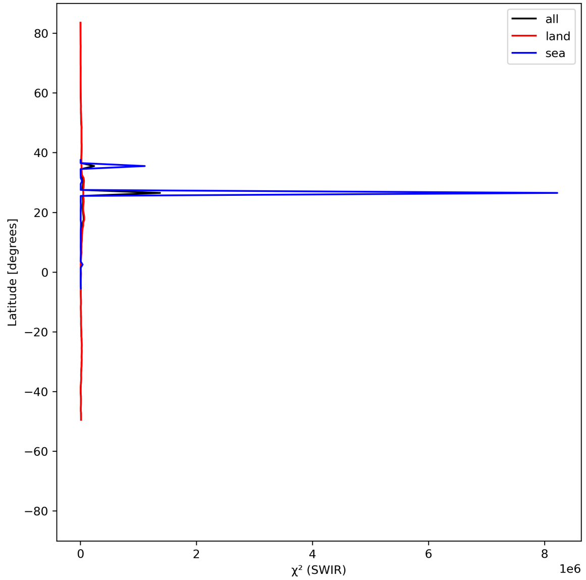
Figure 17: Zonal average of “ \chi^2 (SWIR)” for 2024-04-13 to 2024-04-15.
