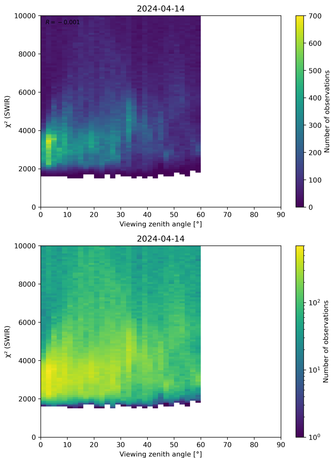
Figure 106: Scatter density plot of “Viewing zenith angle” against “ \chi^2 (SWIR)” for 2024-04-13 to 2024-04-15.
