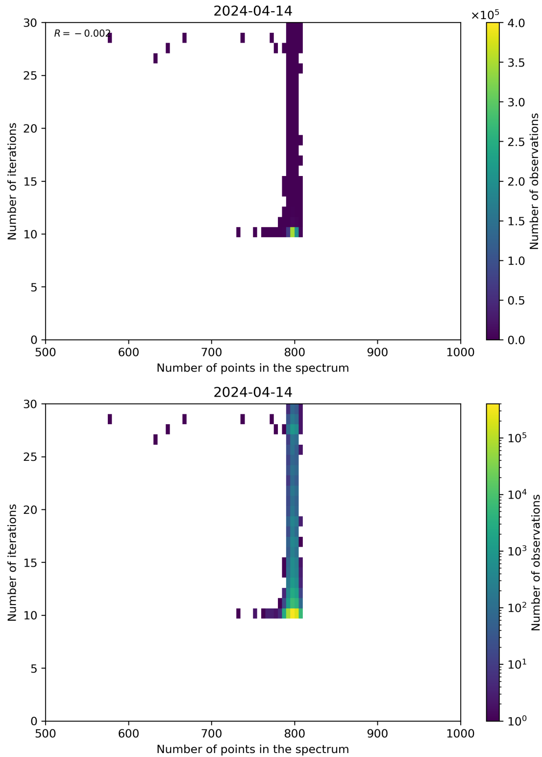
Figure 92: Scatter density plot of “Number of points in the spectrum” against “Number of iterations” for 2024-04-13 to 2024-04-15.
