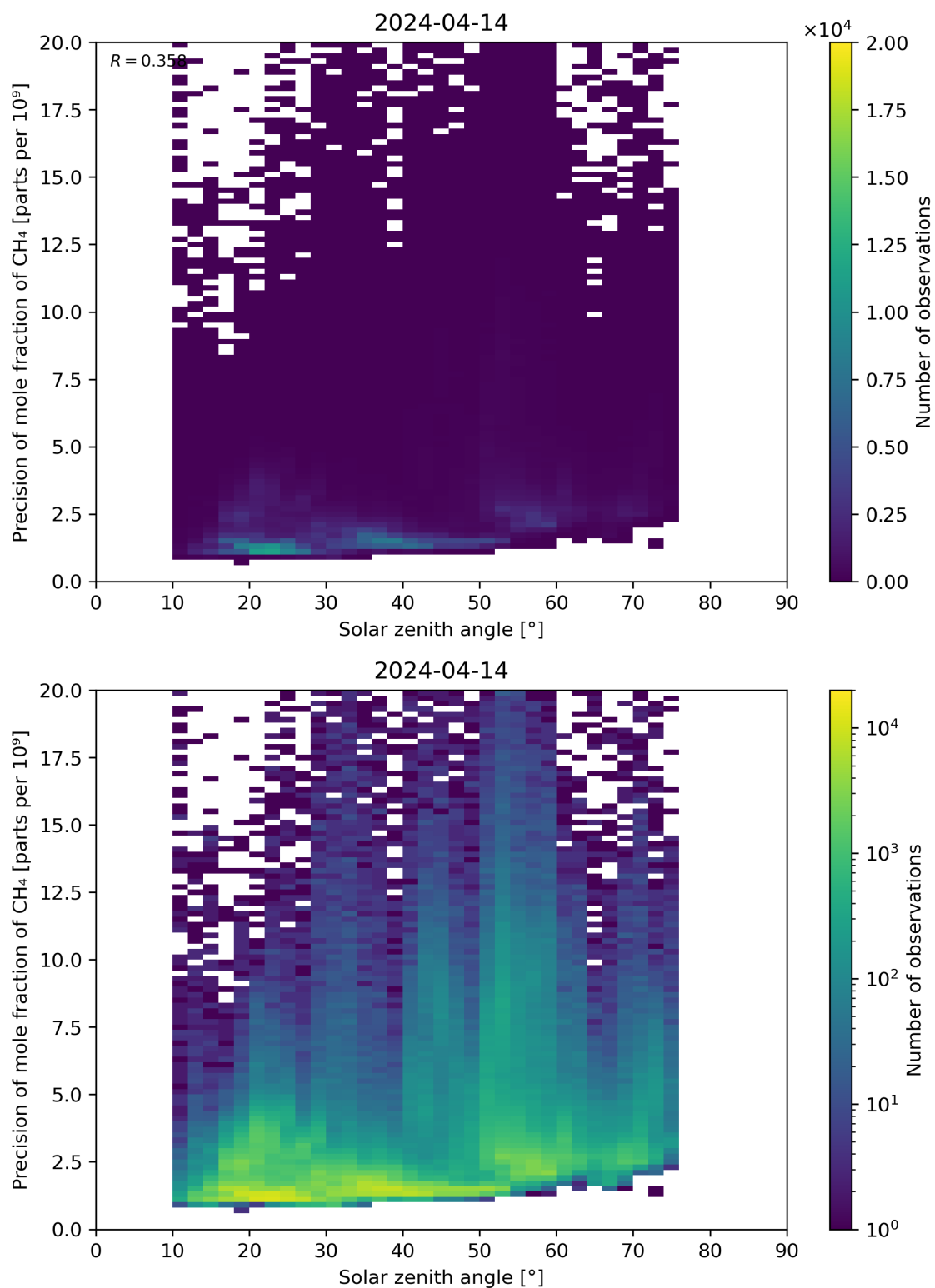
Figure 101: Scatter density plot of “Solar zenith angle” against “Precision of mole fraction of CH 4 ” for 2024-04-13 to 2024-04-15.
