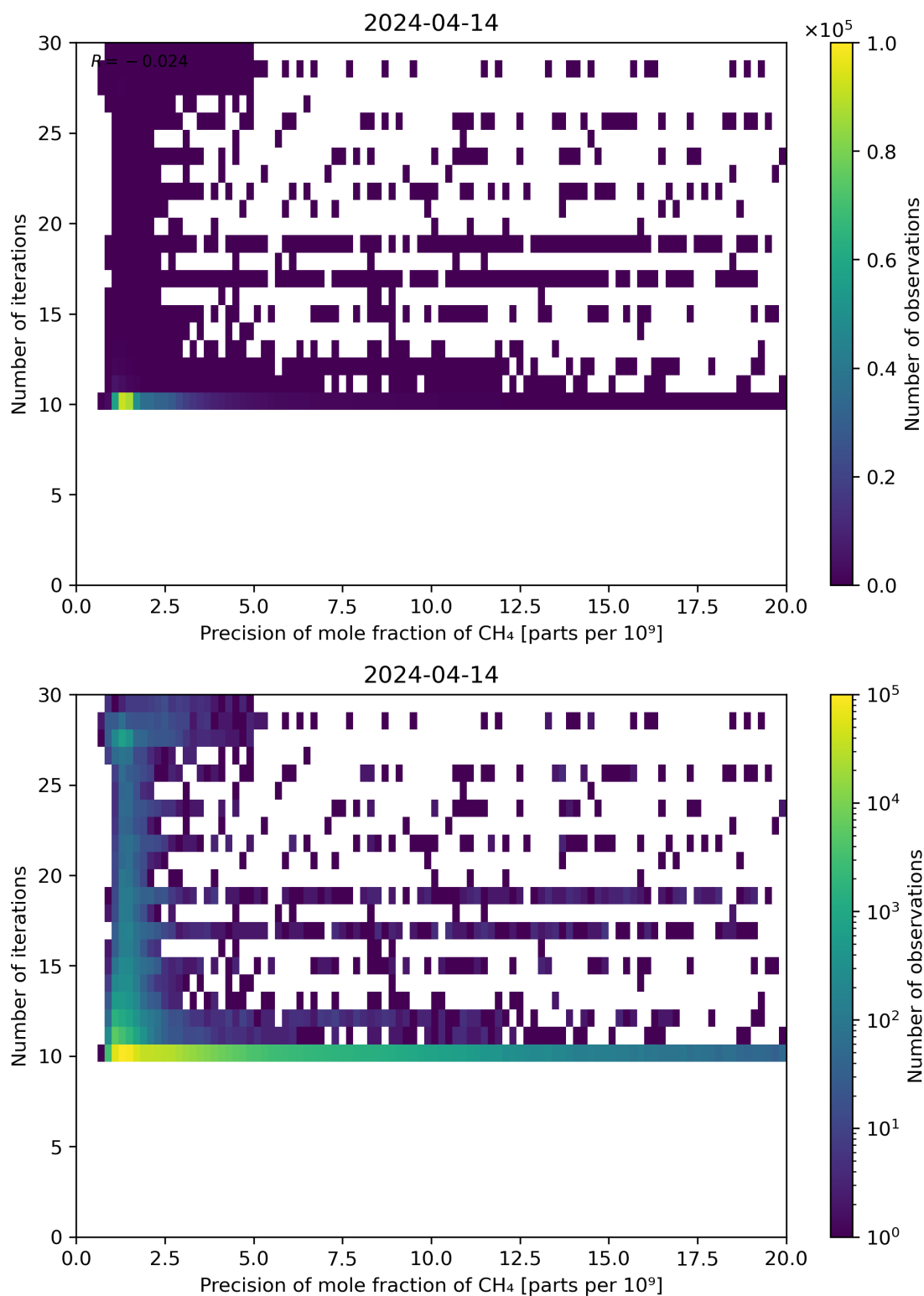
Figure 83: Scatter density plot of “Precision of mole fraction of CH 4 ” against “Number of iterations” for 2024-04-13 to 2024-04-15.
