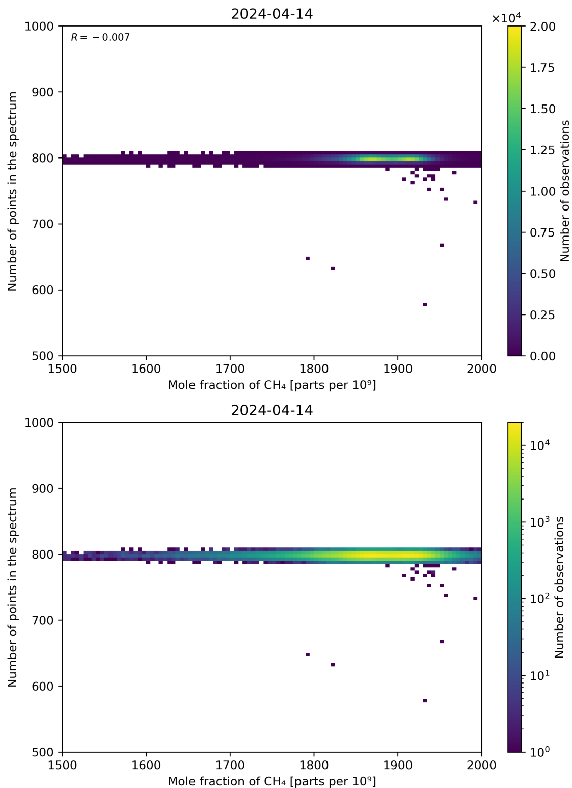
Figure 77: Scatter density plot of “Mole fraction of CH 4 ” against “Number of points in the spectrum” for 2024-04-13 to 2024-04-15.
