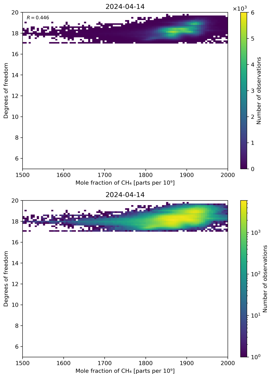
Figure 72: Scatter density plot of “Mole fraction of CH 4 ” against “Degrees of freedom” for 2024-04-13 to 2024-04-15.
