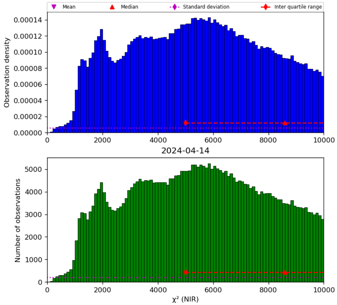
Figure 29: Histogram of “ \chi^2 (NIR)” for 2024-04-13 to 2024-04-15
