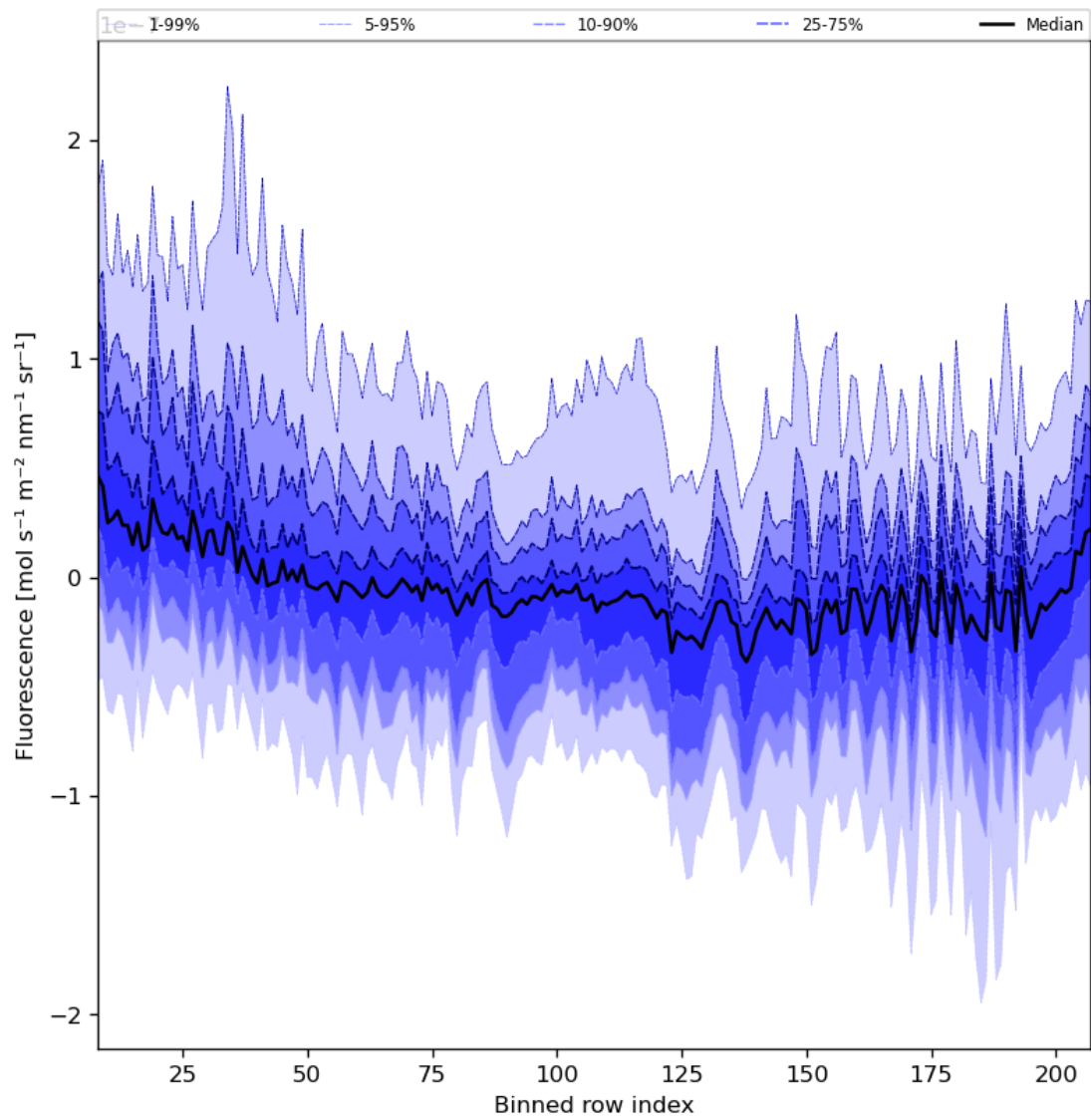
Figure 43: Along track statistics of “Fluorescence” for 2024-04-13 to 2024-04-15
