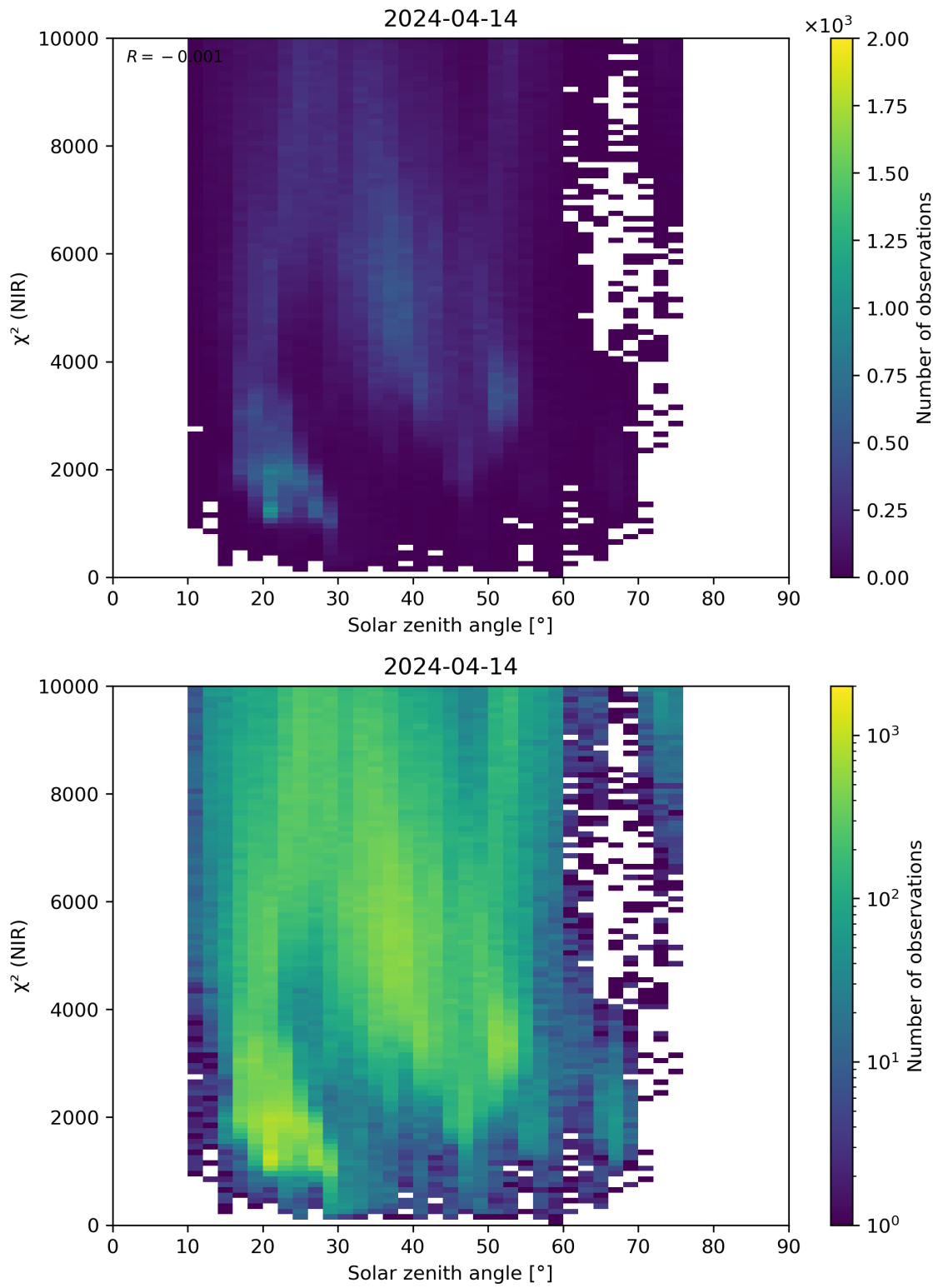
Figure 94: Scatter density plot of “Solar zenith angle” against “ \chi^2 (NIR)” for 2024-04-13 to 2024-04-15.
