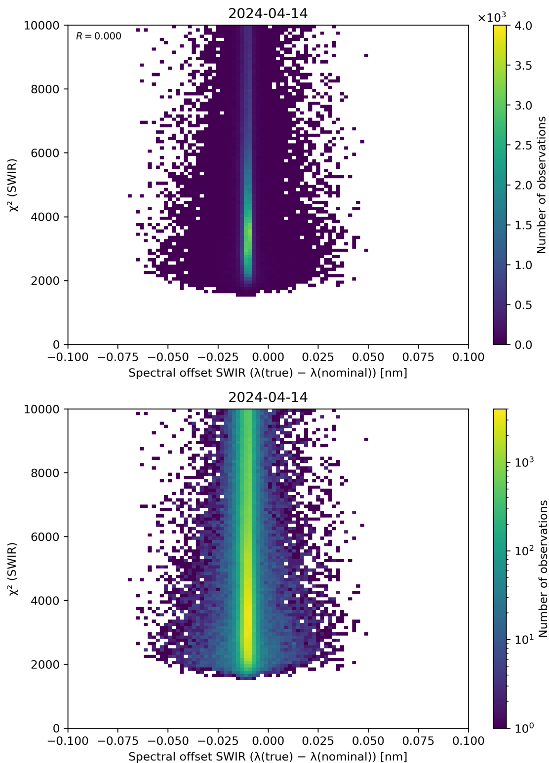
Figure 118: Scatter density plot of “Spectral offset SWIR ( \lambda(\text{true}) - \lambda(\text{nominal}) )” against “ \chi^2 (SWIR)” for 2024-04-13 to 2024-04-15.
