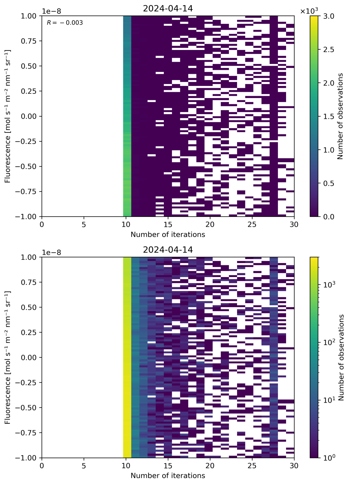
Figure 87: Scatter density plot of “Number of iterations” against “Fluorescence” for 2024-04-13 to 2024-04-15.
