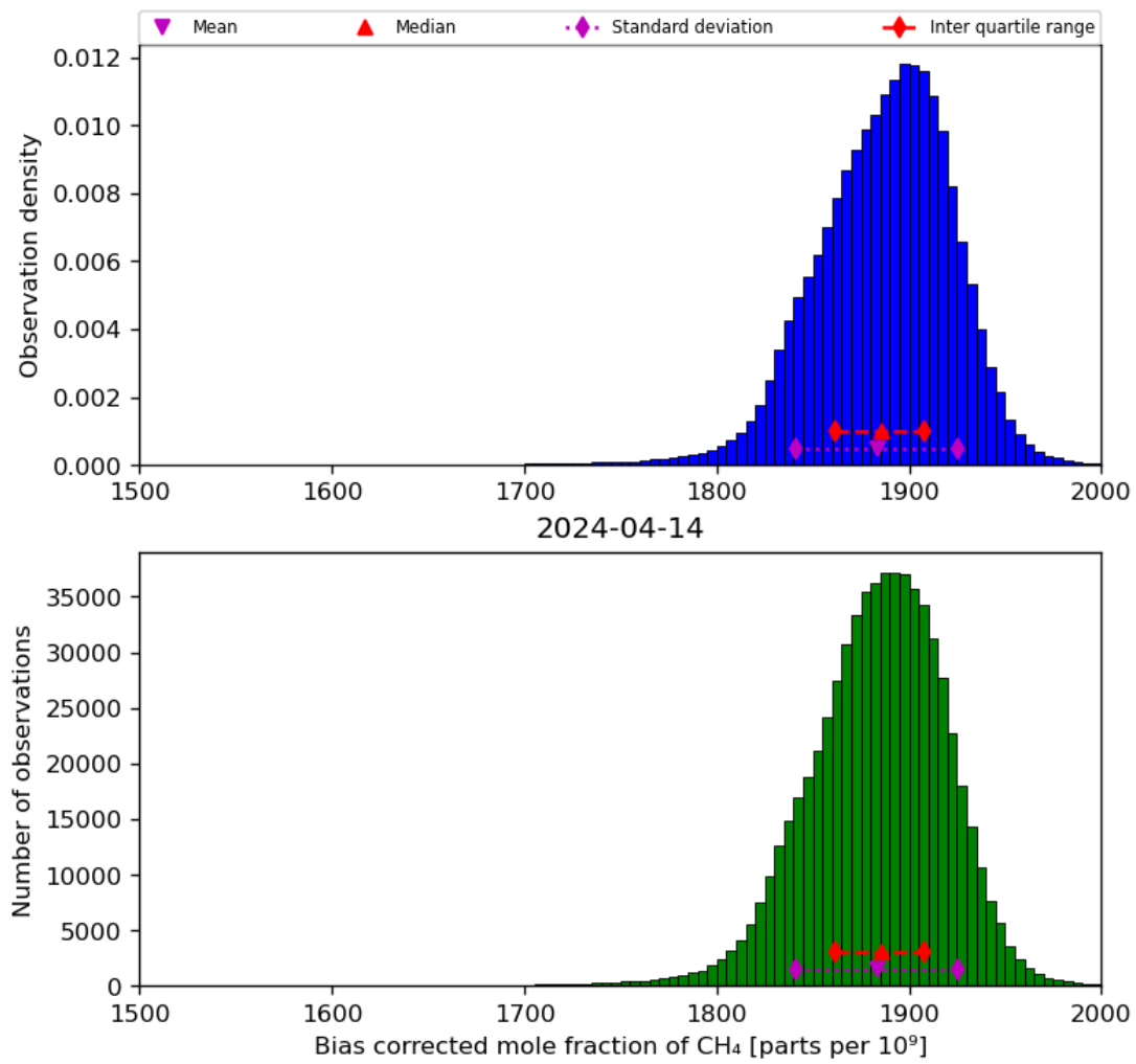
Figure 25: Histogram of “Bias corrected mole fraction of CH 4 ” for 2024-04-13 to 2024-04-15
