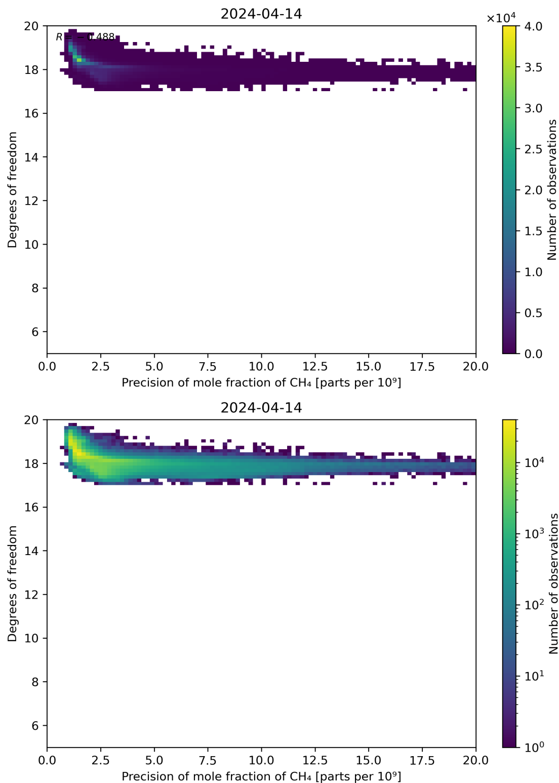
Figure 80: Scatter density plot of “Precision of mole fraction of CH 4 ” against “Degrees of freedom” for 2024-04-13 to 2024-04-15.
