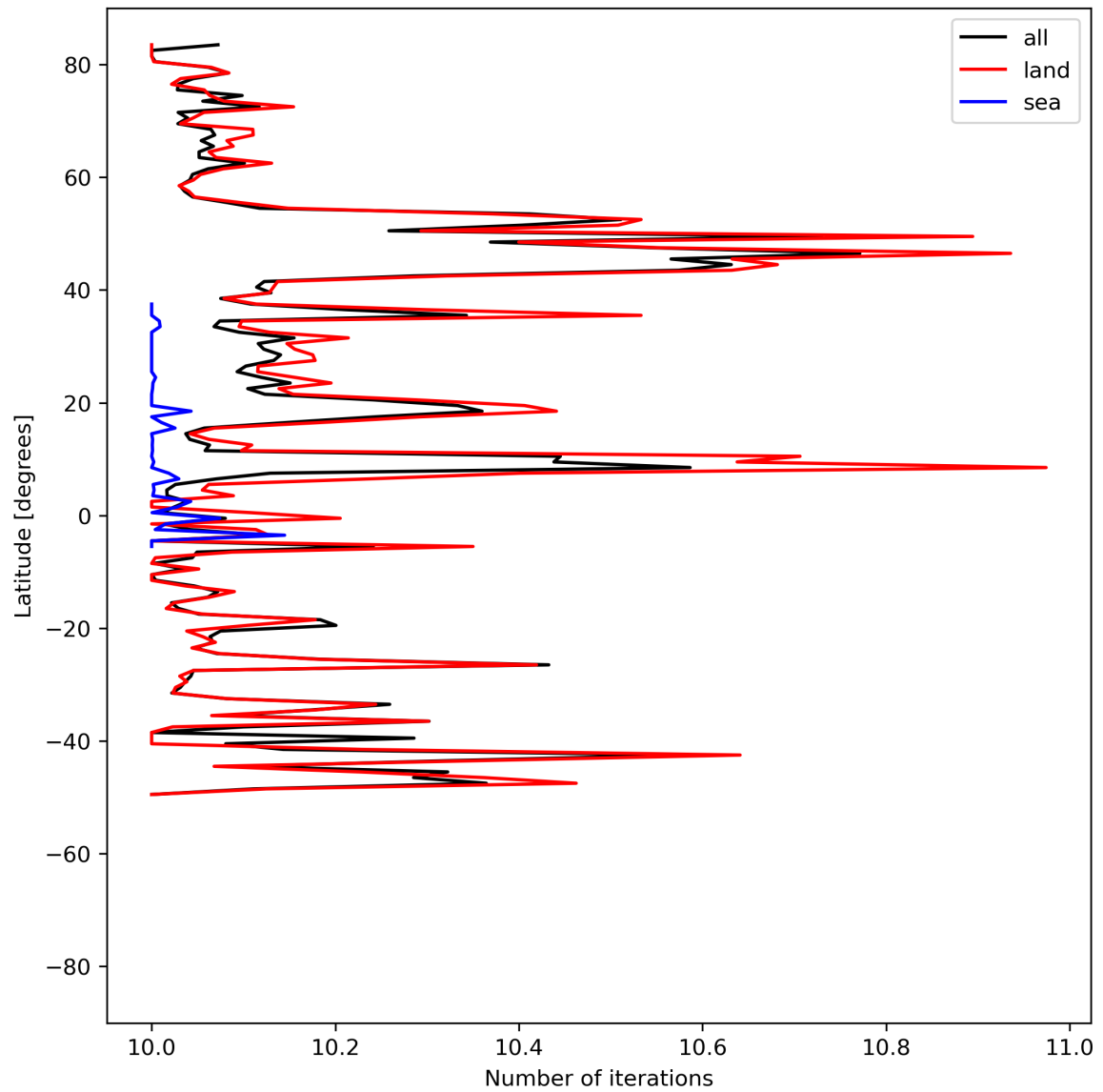
Figure 20: Zonal average of “Number of iterations” for 2024-04-13 to 2024-04-15.
