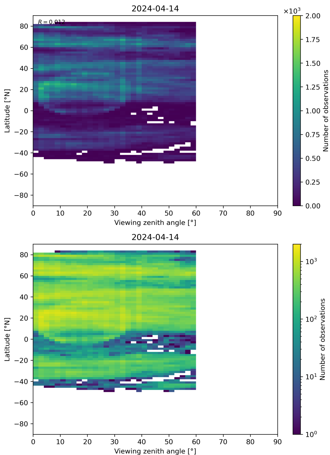
Figure 109: Scatter density plot of “Viewing zenith angle” against “Latitude” for 2024-04-13 to 2024-04-15.
