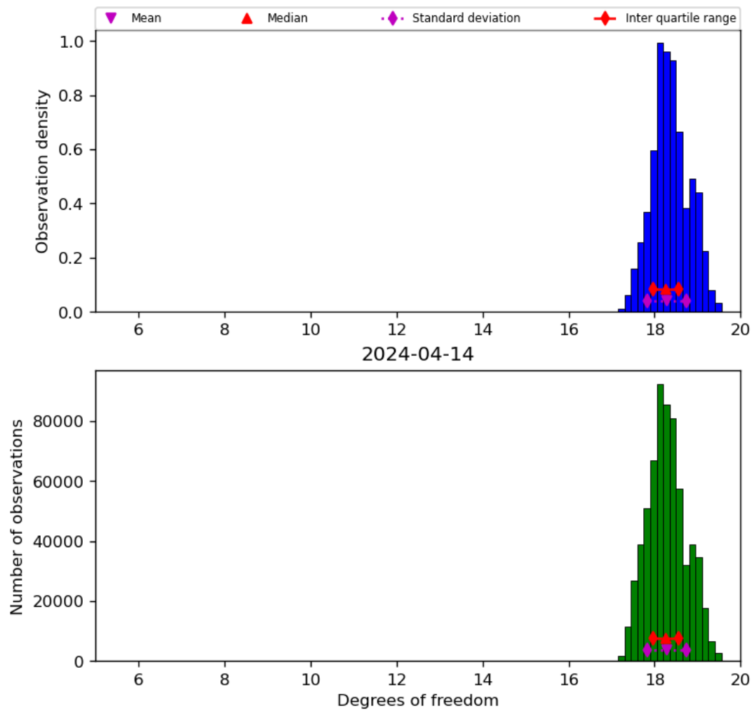
Figure 30: Histogram of “Degrees of freedom” for 2024-04-13 to 2024-04-15
