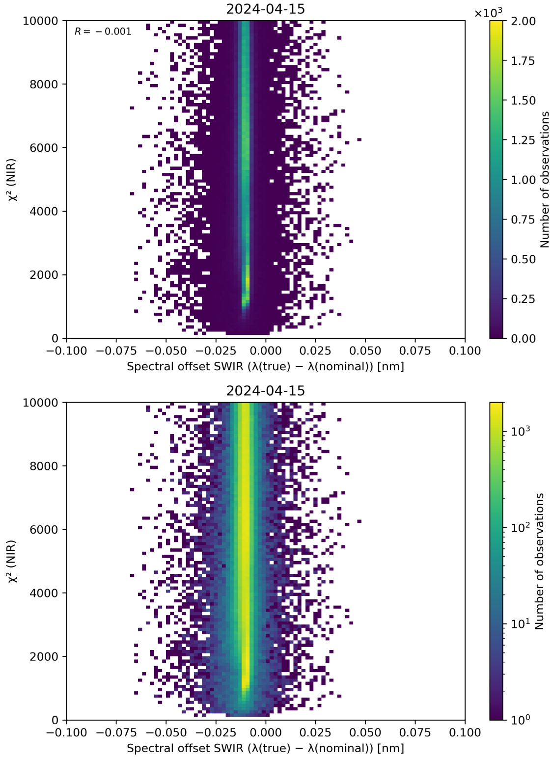
Figure 117: Scatter density plot of “Spectral offset SWIR ( \lambda(\text{true}) - \lambda(\text{nominal}) )” against “ \chi^2 (NIR)” for 2024-04-15 to 2024-04-16.
