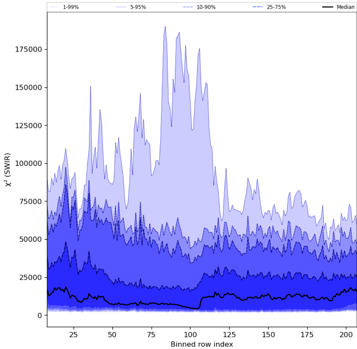
Figure 39: Along track statistics of “ \chi^2 (SWIR)” for 2024-04-15 to 2024-04-16
