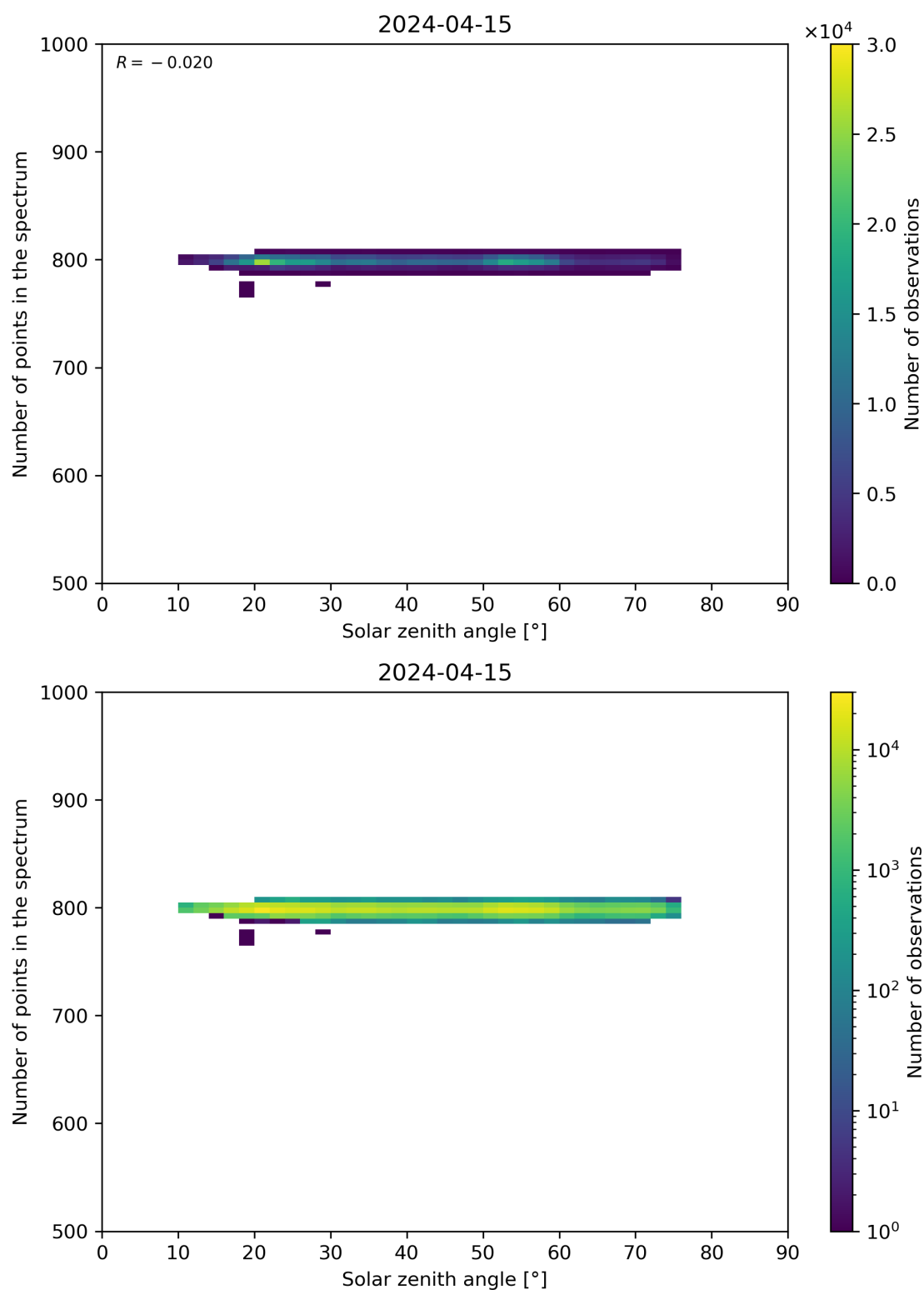
Figure 103: Scatter density plot of “Solar zenith angle” against “Number of points in the spectrum” for 2024-04-15 to 2024-04-16.
