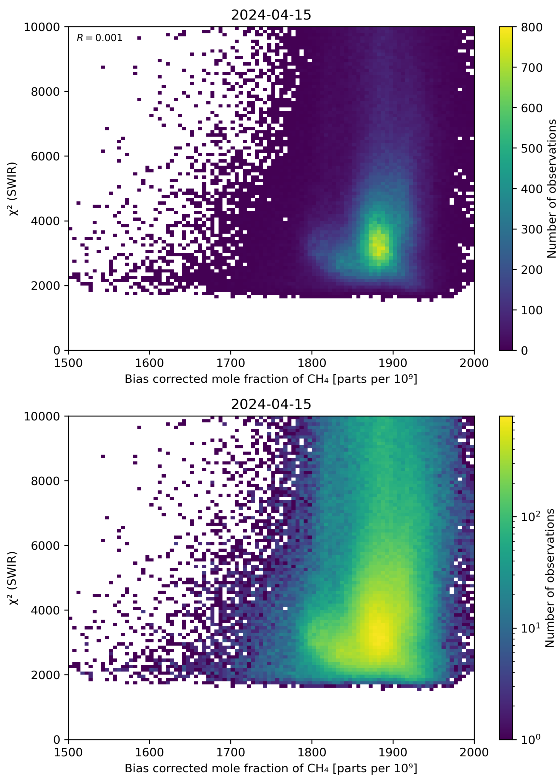
Figure 64: Scatter density plot of “Bias corrected mole fraction of \text{CH}_4 ” against “ \chi^2 (SWIR)” for 2024-04-15 to 2024-04-16.
