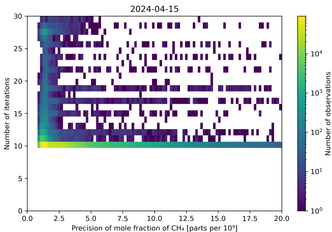
Figure 83: Scatter density plot of “Precision of mole fraction of CH 4 ” against “Number of iterations” for 2024-04-15 to 2024-04-16.
