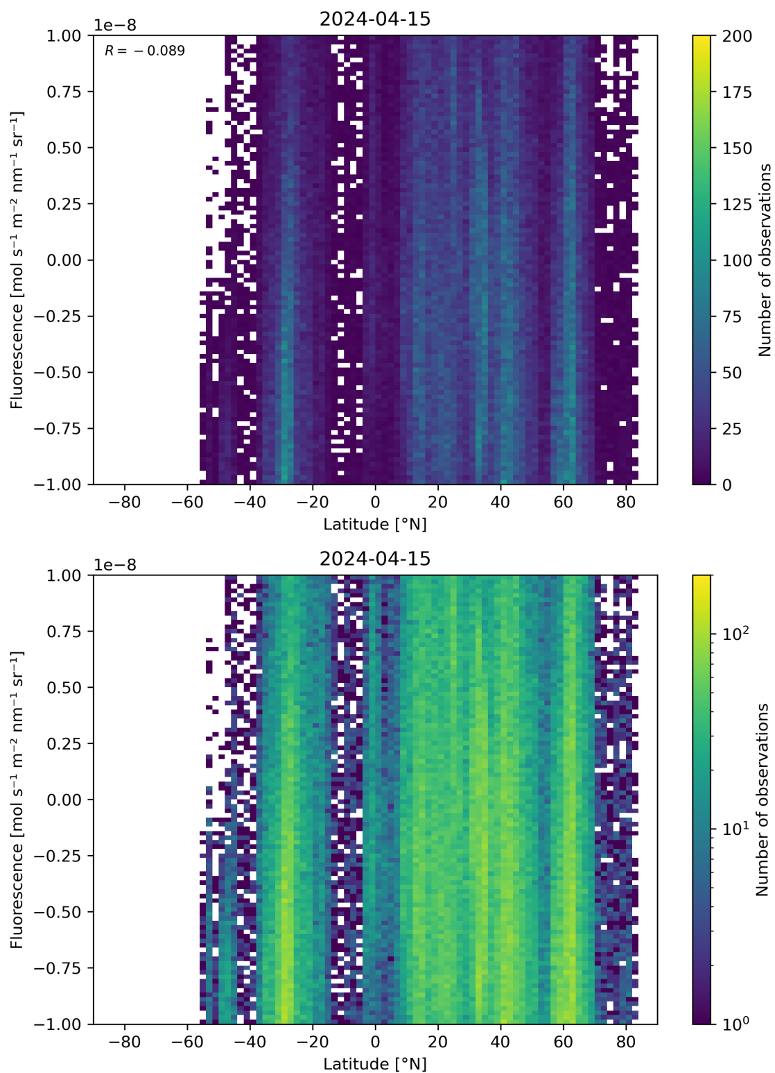
Figure 56: Scatter density plot of “Latitude” against “Fluorescence” for 2024-04-15 to 2024-04-16.
