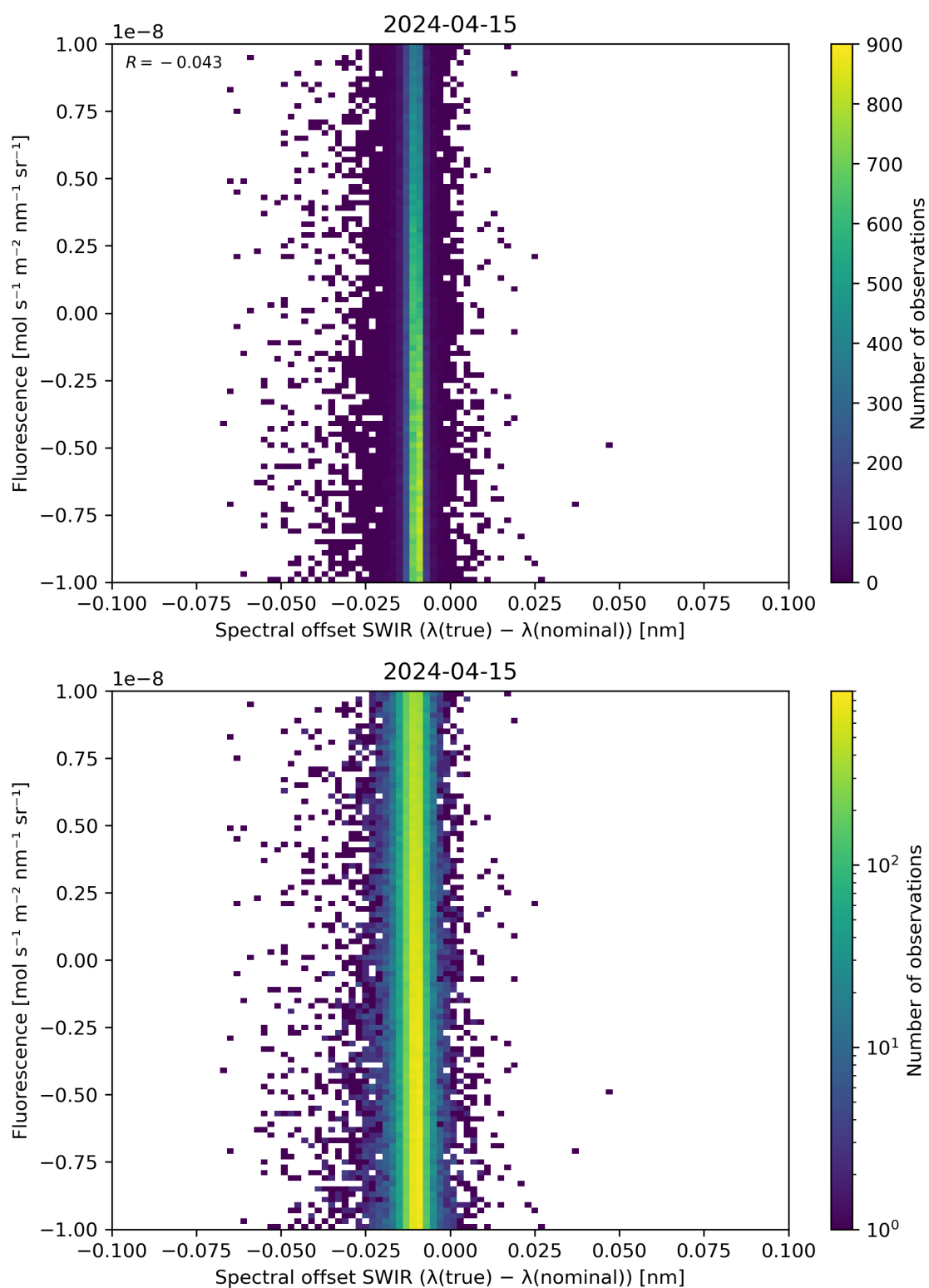
Figure 120: Scatter density plot of “Spectral offset SWIR ( \lambda(\text{true}) - \lambda(\text{nominal}) )” against “Fluorescence” for 2024-04-15 to 2024-04-16.
