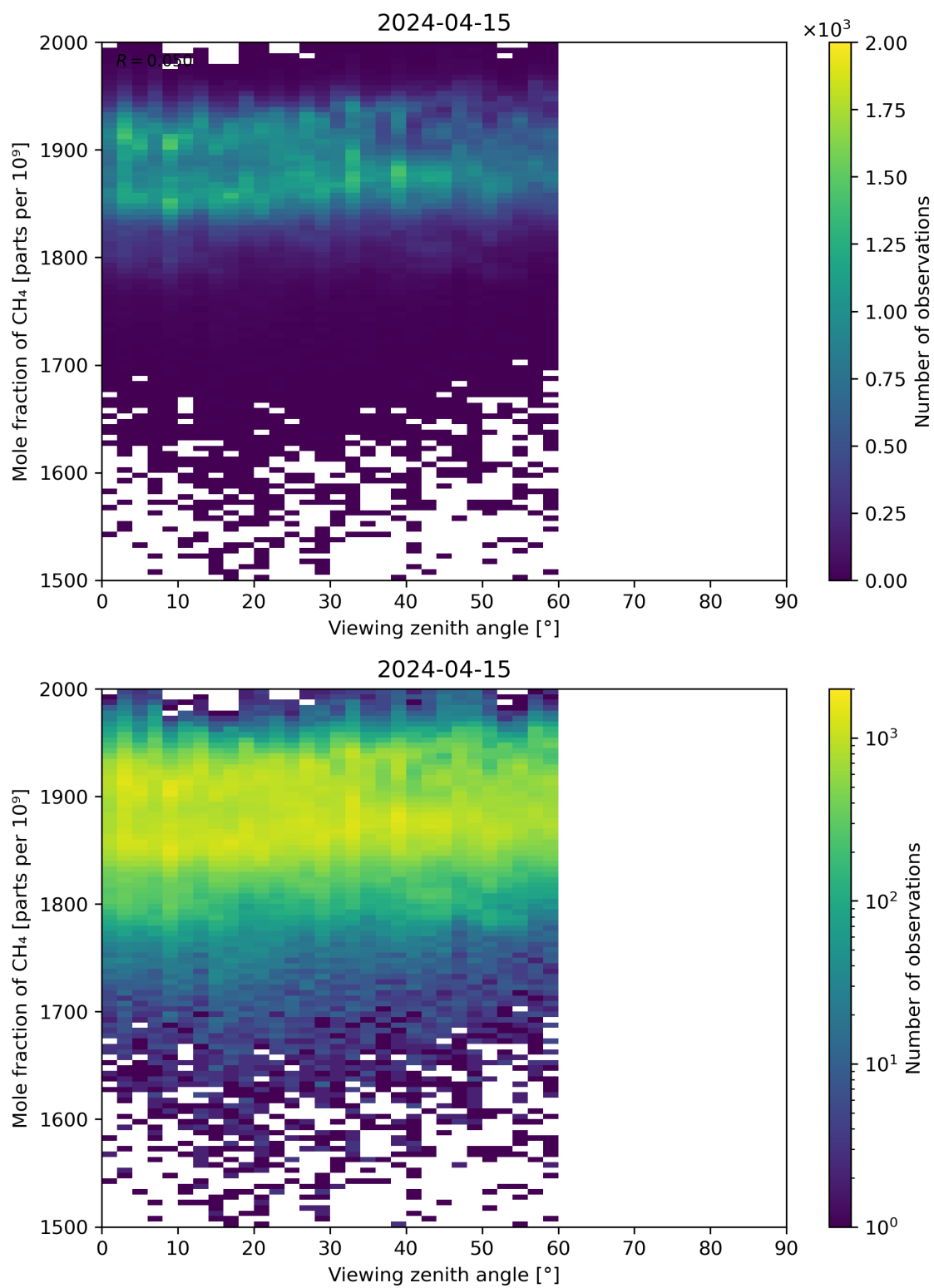
Figure 110: Scatter density plot of “Viewing zenith angle” against “Mole fraction of CH 4 ” for 2024-04-15 to 2024-04-16.
