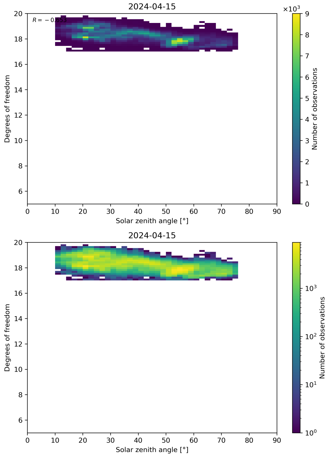
Figure 96: Scatter density plot of “Solar zenith angle” against “Degrees of freedom” for 2024-04-15 to 2024-04-16.
