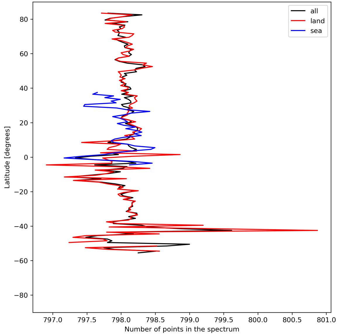
Figure 15: Zonal average of “Number of points in the spectrum” for 2024-04-15 to 2024-04-16.
