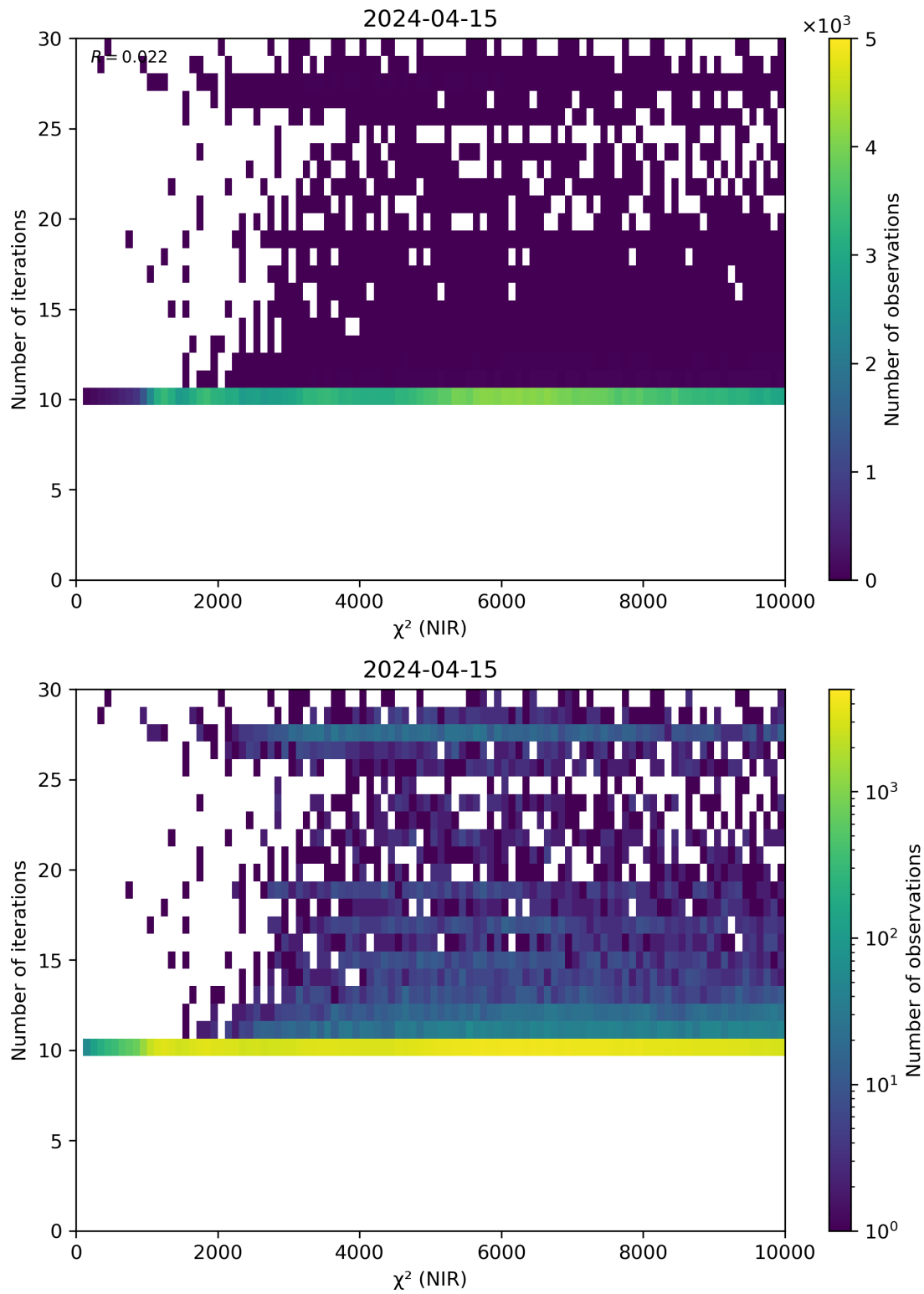
Figure 46: Scatter density plot of “ \chi^2 (NIR)” against “Number of iterations” for 2024-04-15 to 2024-04-16.
