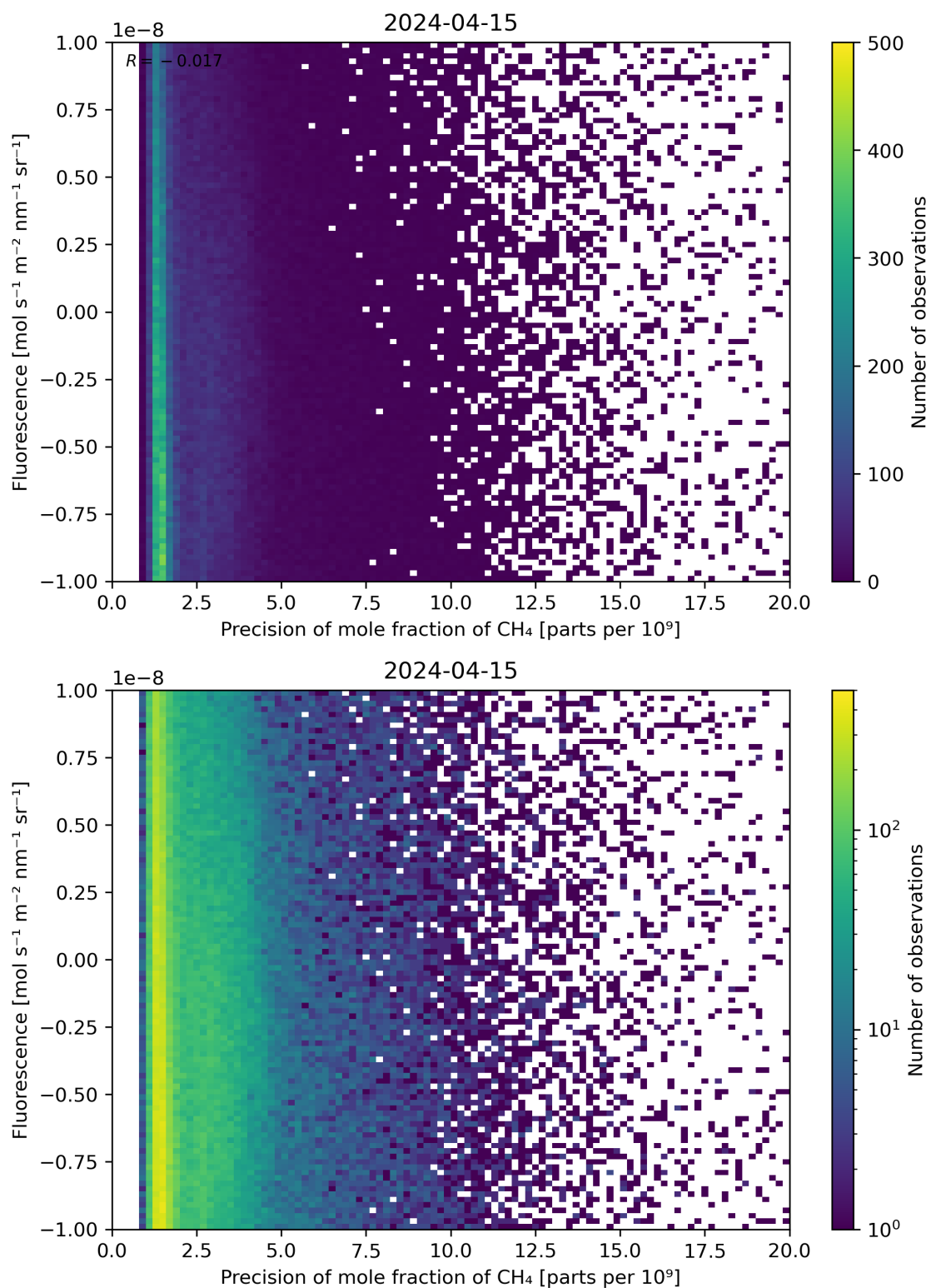
Figure 81: Scatter density plot of “Precision of mole fraction of CH 4 ” against “Fluorescence” for 2024-04-15 to 2024-04-16.
