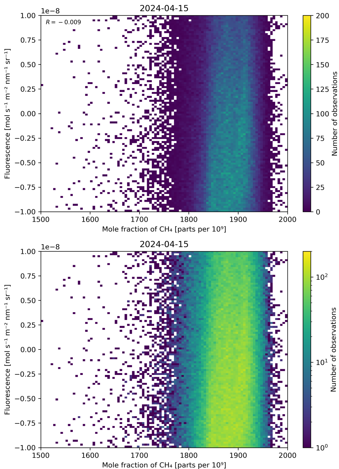
Figure 73: Scatter density plot of “Mole fraction of \text{CH}_4 ” against “Fluorescence” for 2024-04-15 to 2024-04-16.
