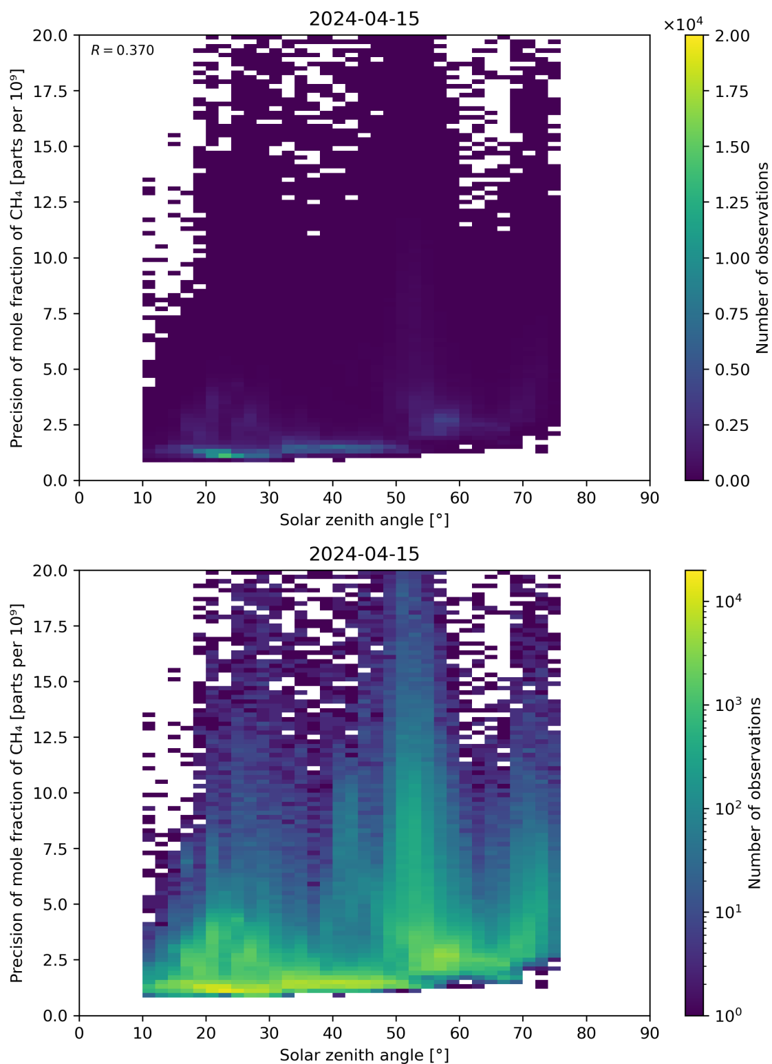
Figure 101: Scatter density plot of “Solar zenith angle” against “Precision of mole fraction of CH 4 ” for 2024-04-15 to 2024-04-16.
