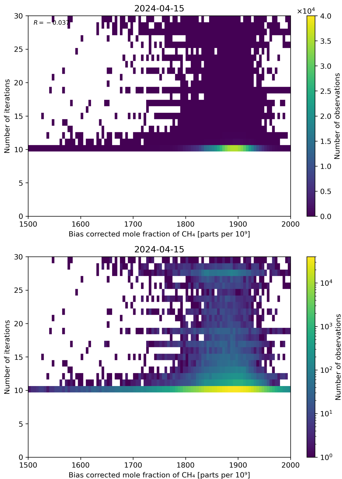
Figure 67: Scatter density plot of “Bias corrected mole fraction of CH 4 ” against “Number of iterations” for 2024-04-15 to 2024-04-16.
