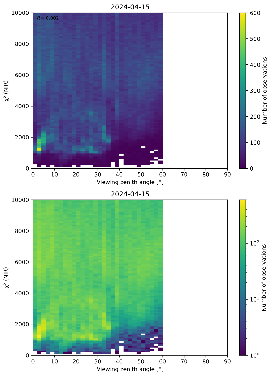
Figure 105: Scatter density plot of “Viewing zenith angle” against “ \chi^2 (NIR)” for 2024-04-15 to 2024-04-16.
