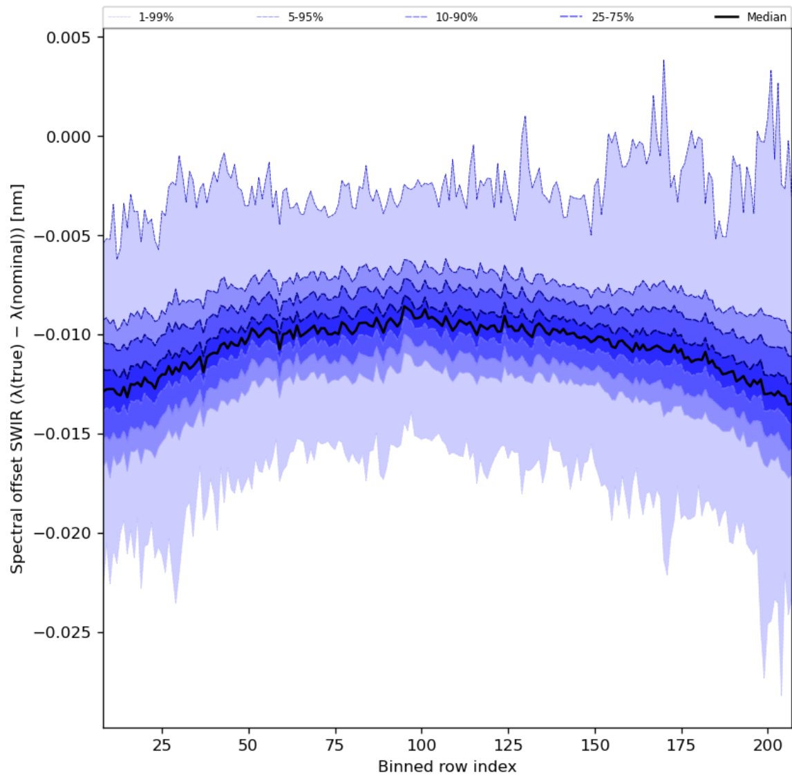
Figure 38: Along track statistics of “Spectral offset SWIR ( \lambda(\text{true}) - \lambda(\text{nominal}) )” for 2024-04-15 to 2024-04-16
