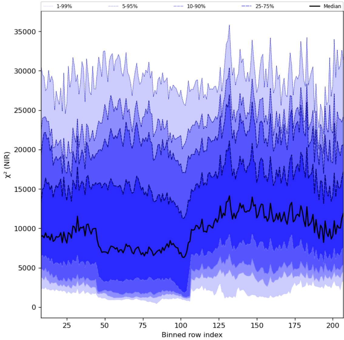
Figure 40: Along track statistics of “ \chi^2 (NIR)” for 2024-04-15 to 2024-04-16
