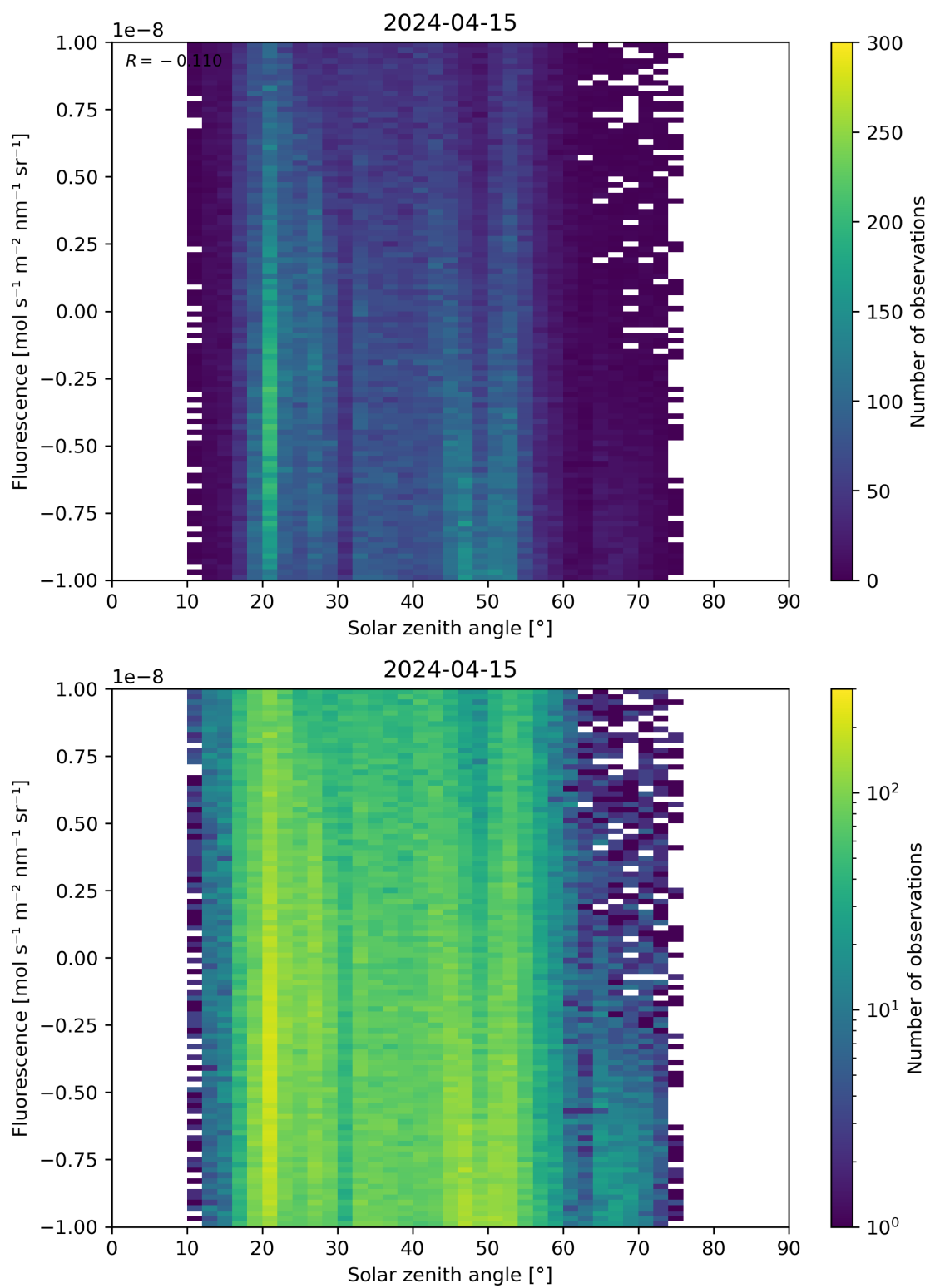
Figure 97: Scatter density plot of “Solar zenith angle” against “Fluorescence” for 2024-04-15 to 2024-04-16.
