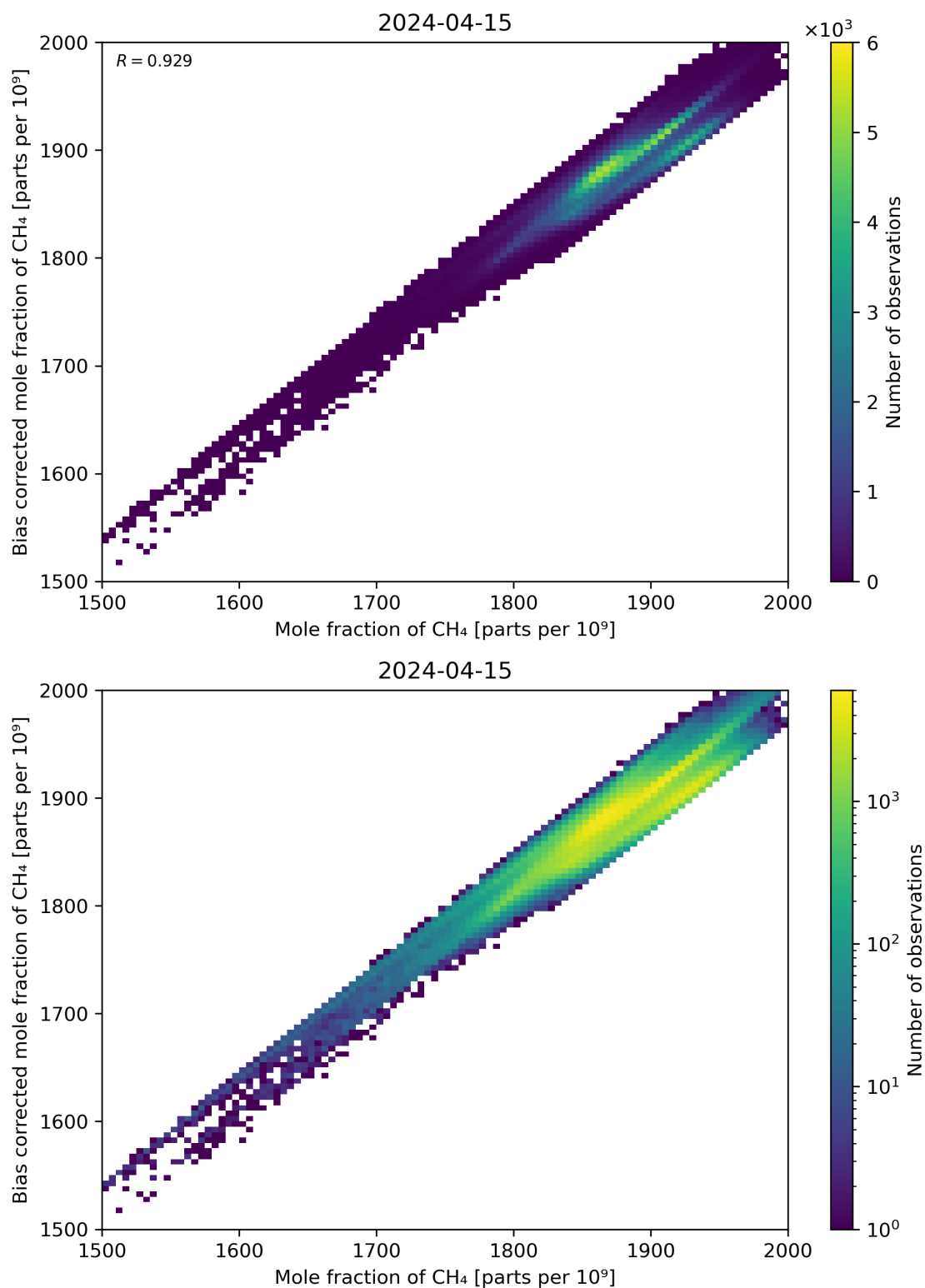
Figure 74: Scatter density plot of “Mole fraction of CH 4 ” against “Bias corrected mole fraction of CH 4 ” for 2024-04-15 to 2024-04-16.
