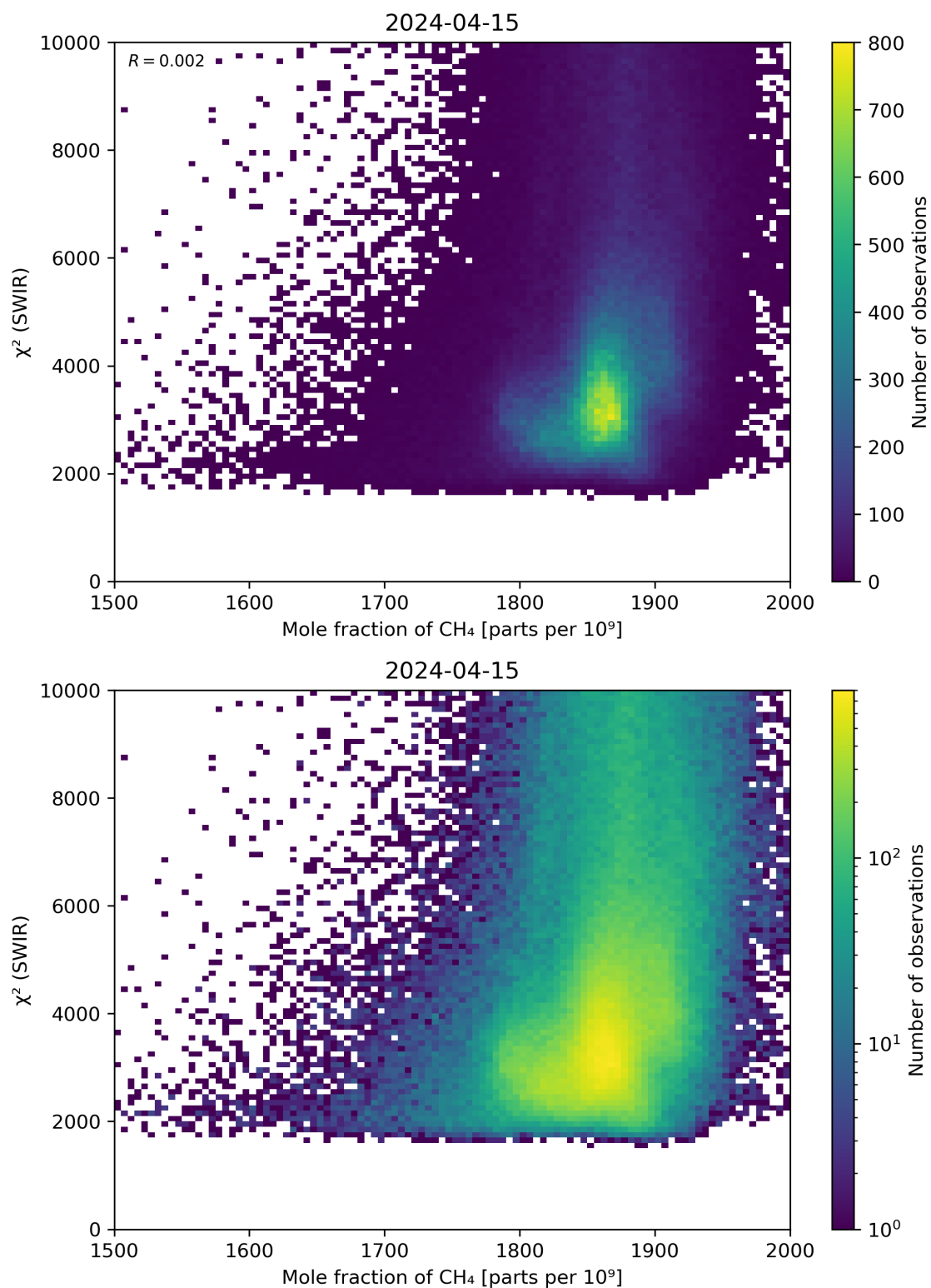
Figure 71: Scatter density plot of “Mole fraction of \text{CH}_4 ” against “ \chi^2 (SWIR)” for 2024-04-15 to 2024-04-16.
