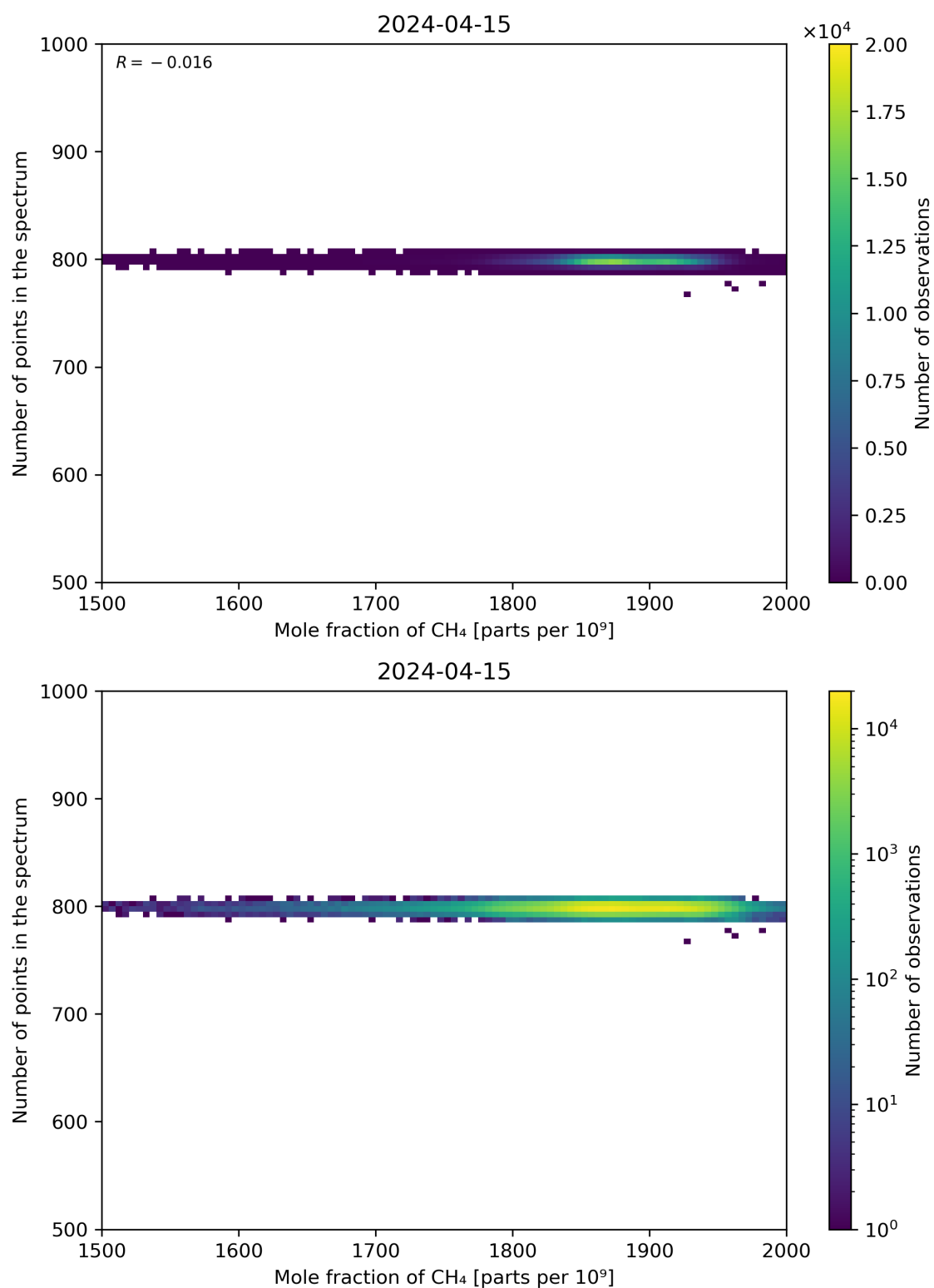
Figure 77: Scatter density plot of “Mole fraction of CH 4 ” against “Number of points in the spectrum” for 2024-04-15 to 2024-04-16.
