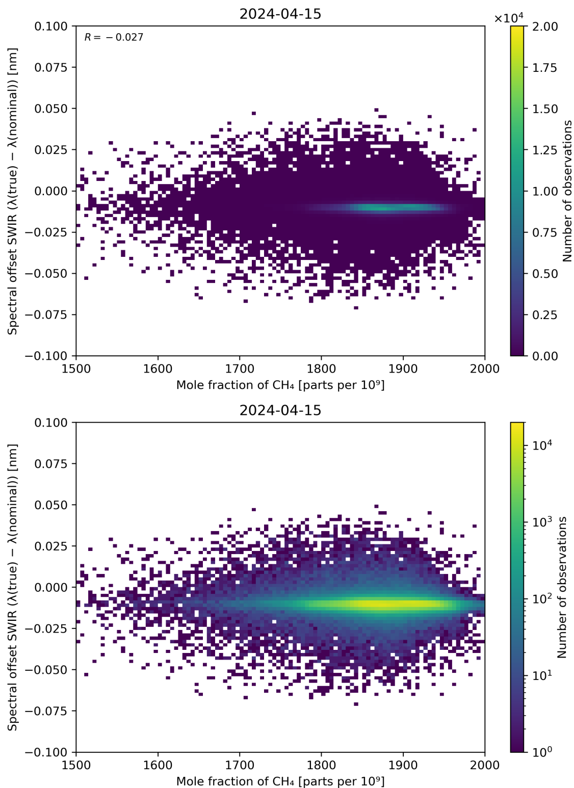
Figure 86: Scatter density plot of “Mole fraction of CH 4 ” against “Spectral offset SWIR ( \lambda(\text{true}) - \lambda(\text{nominal}) )” for 2024-04-15 to 2024-04-16.
