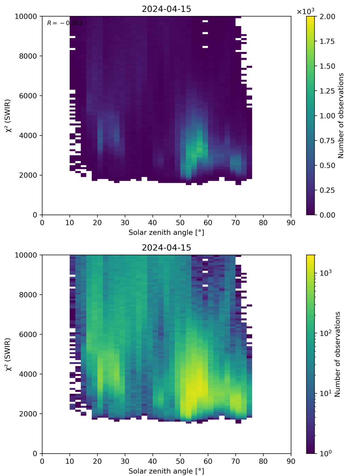
Figure 95: Scatter density plot of “Solar zenith angle” against “ \chi^2 (SWIR)” for 2024-04-15 to 2024-04-16.
