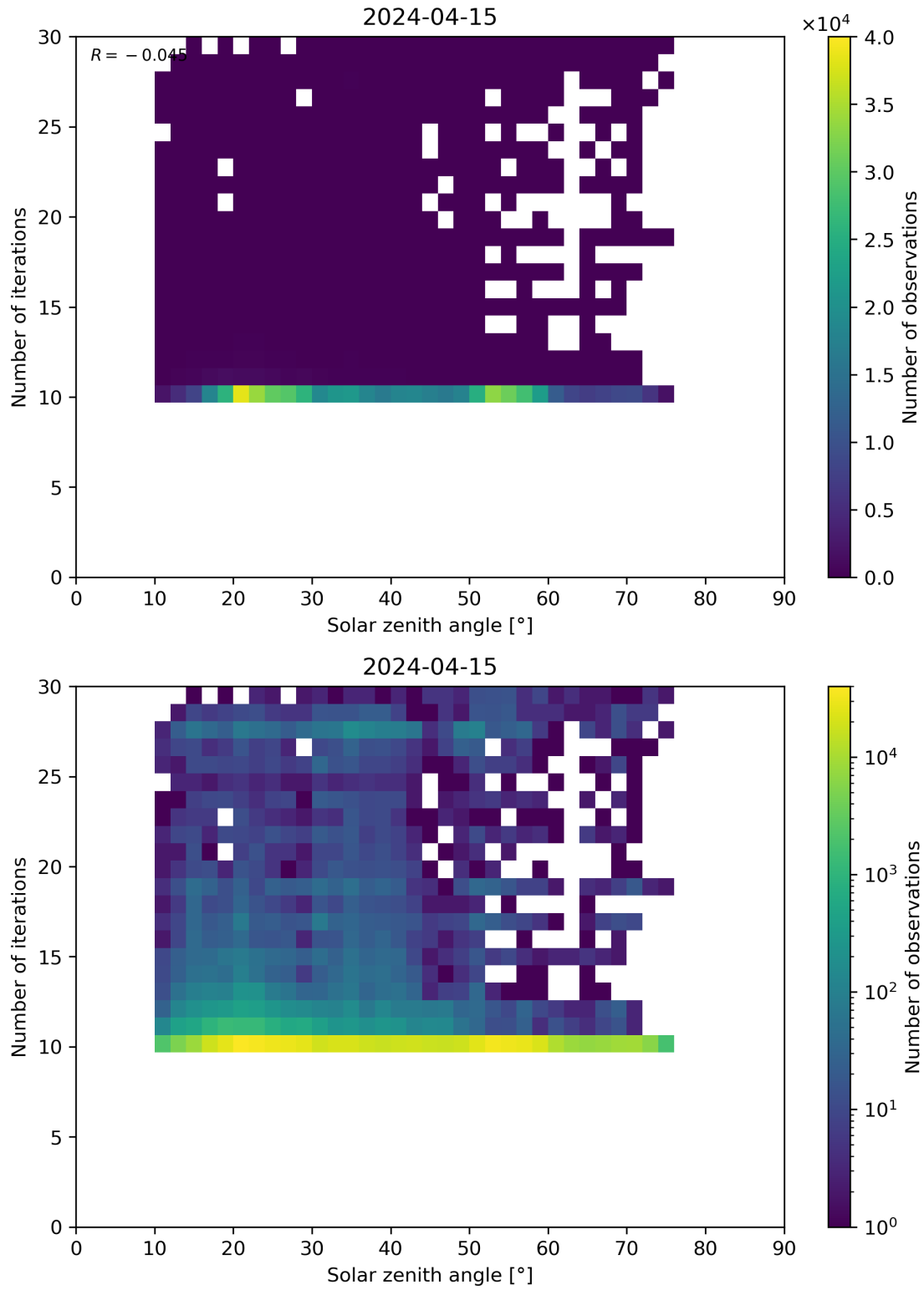
Figure 102: Scatter density plot of “Solar zenith angle” against “Number of iterations” for 2024-04-15 to 2024-04-16.
