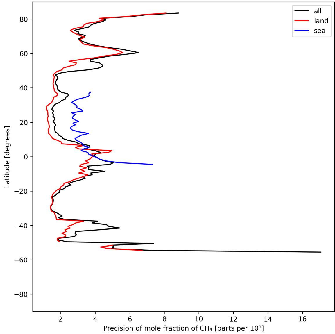
Figure 13: Zonal average of “Precision of mole fraction of CH 4 ” for 2024-04-15 to 2024-04-16.
