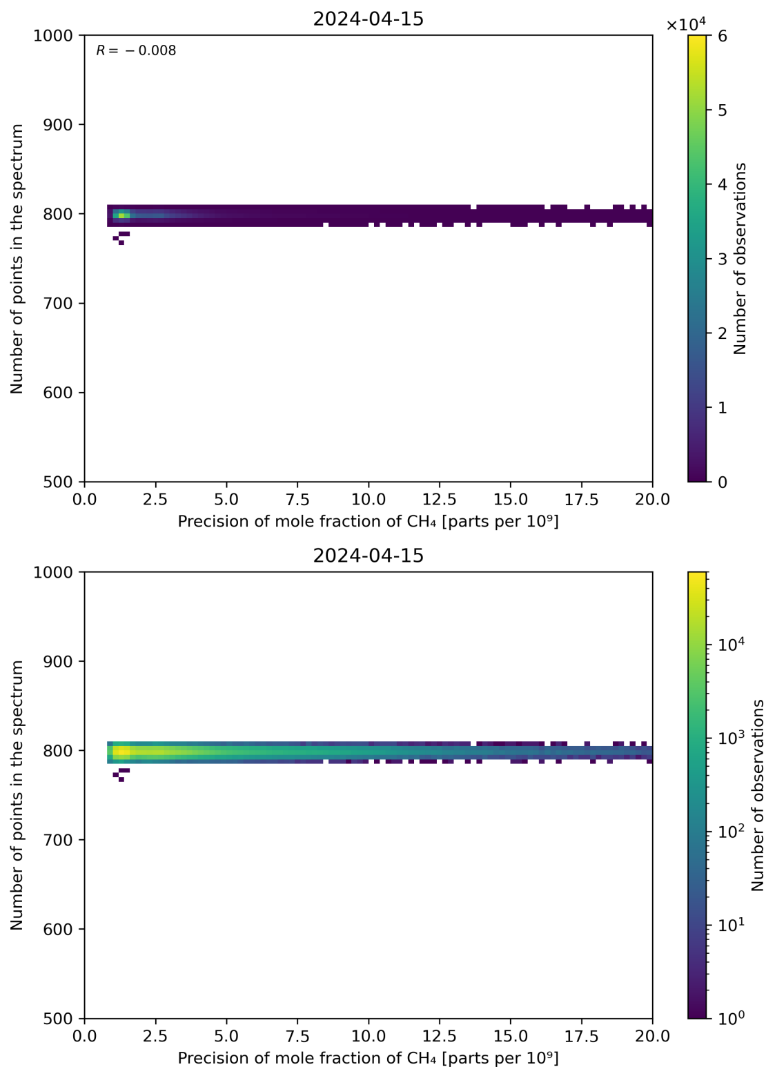
Figure 84: Scatter density plot of “Precision of mole fraction of CH 4 ” against “Number of points in the spectrum” for 2024-04-15 to 2024-04-16.
