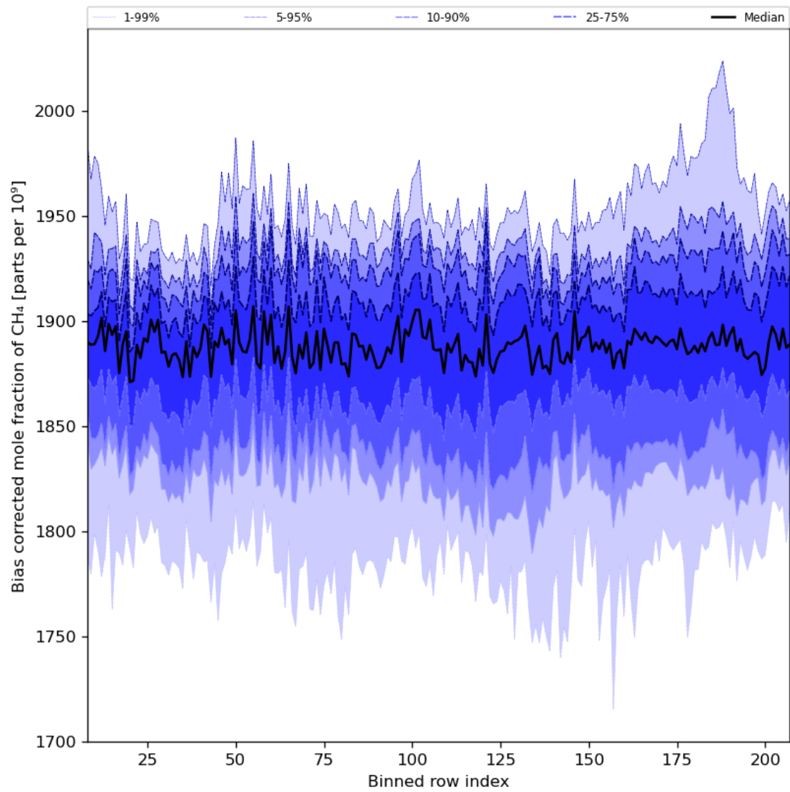
Figure 36: Along track statistics of “Bias corrected mole fraction of CH 4 ” for 2024-04-15 to 2024-04-16
