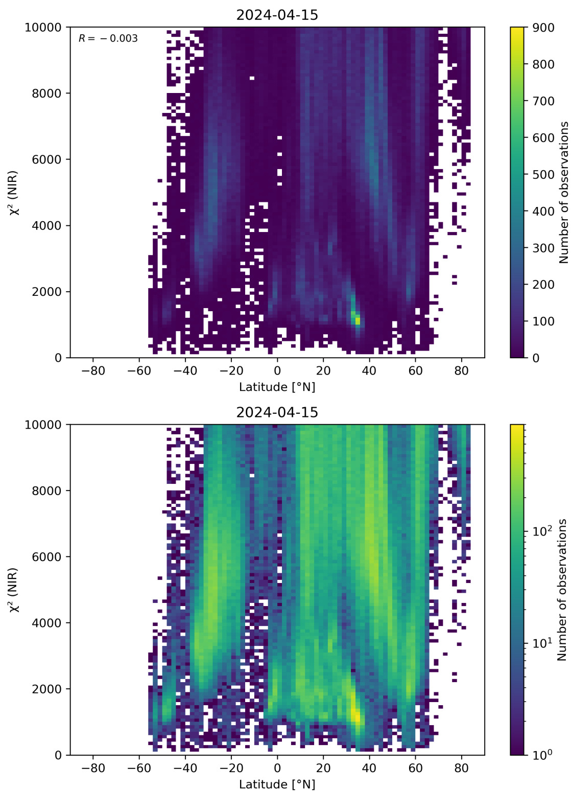
Figure 53: Scatter density plot of “Latitude” against “ \chi^2 (NIR)” for 2024-04-15 to 2024-04-16.
