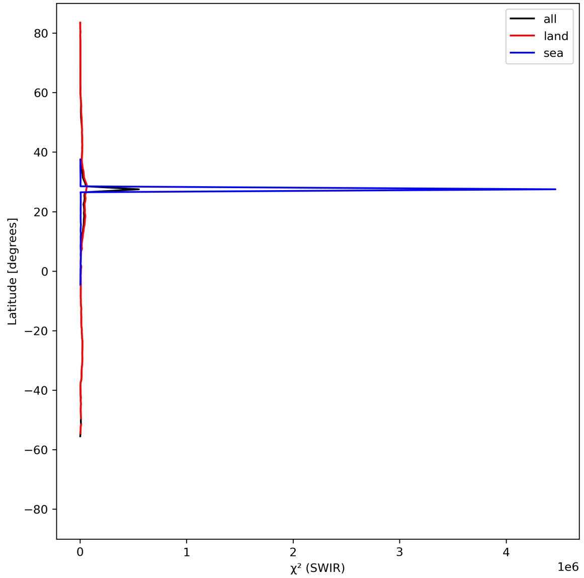
Figure 17: Zonal average of “ \chi^2 (SWIR)” for 2024-04-15 to 2024-04-16.
