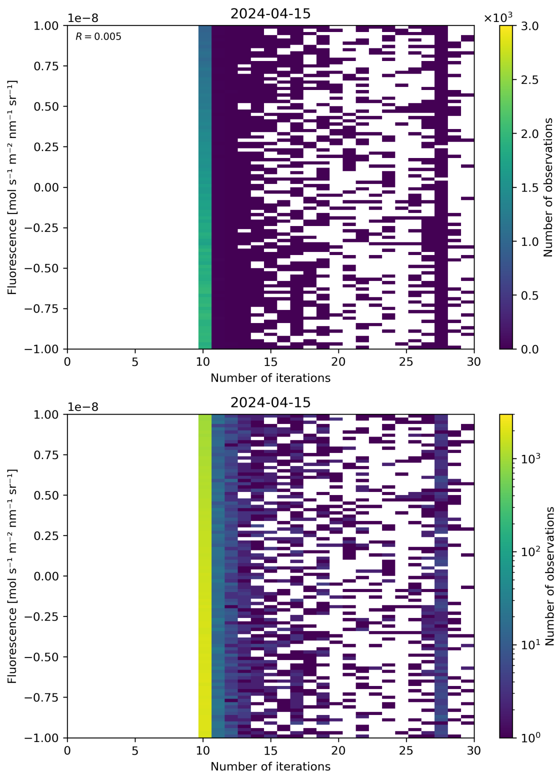
Figure 87: Scatter density plot of “Number of iterations” against “Fluorescence” for 2024-04-15 to 2024-04-16.
