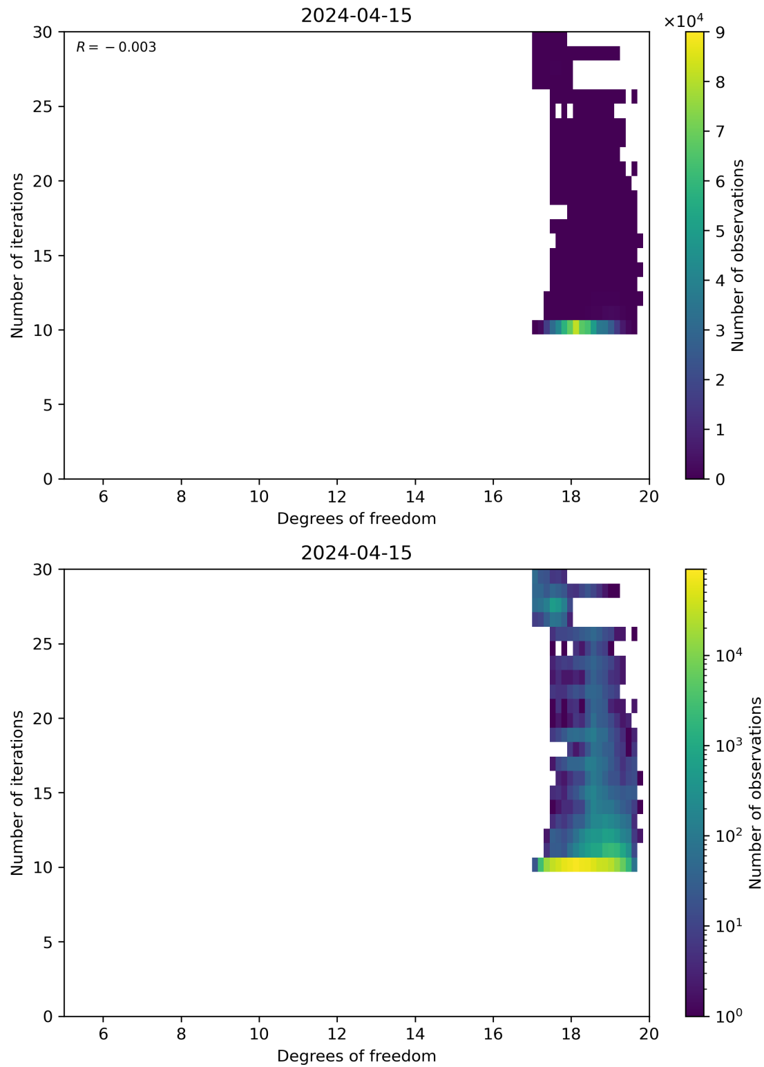
Figure 52: Scatter density plot of “Degrees of freedom” against “Number of iterations” for 2024-04-15 to 2024-04-16.
