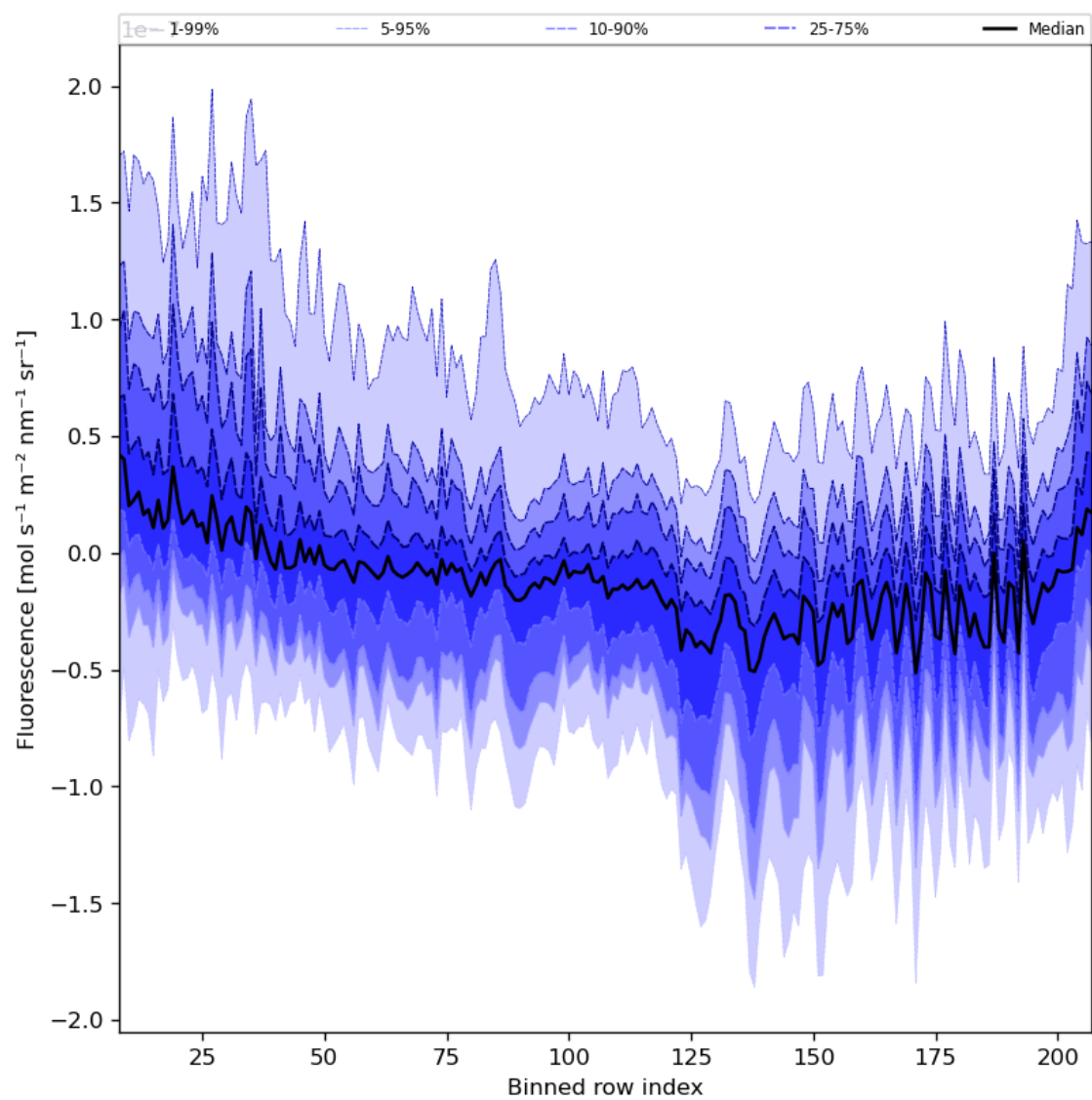
Figure 43: Along track statistics of “Fluorescence” for 2024-04-15 to 2024-04-16
