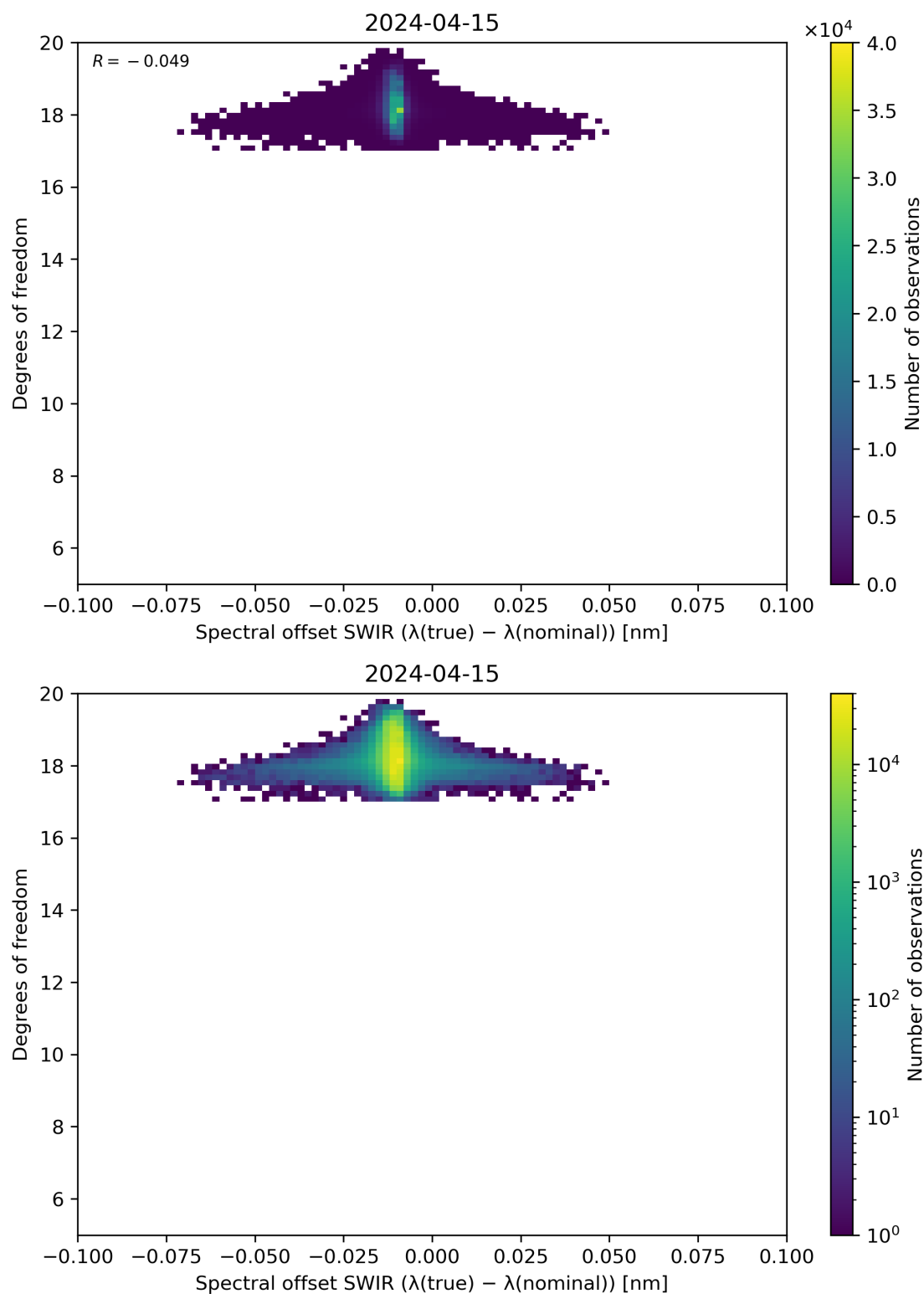
Figure 119: Scatter density plot of “Spectral offset SWIR ( \lambda(\text{true}) - \lambda(\text{nominal}) )” against “Degrees of freedom” for 2024-04-15 to 2024-04-16.
