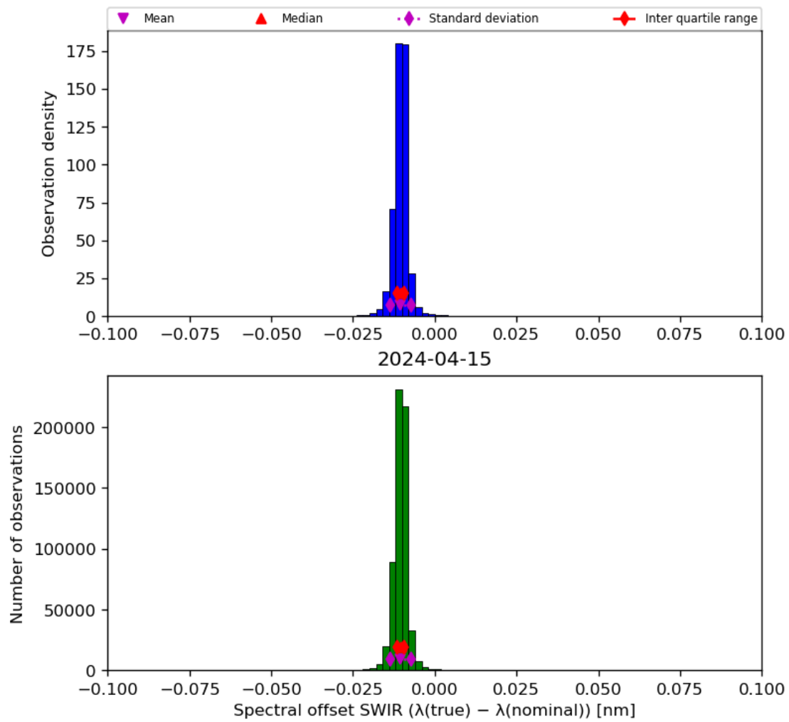
Figure 27: Histogram of “Spectral offset SWIR ( \lambda(\text{true}) - \lambda(\text{nominal}) )” for 2024-04-15 to 2024-04-16
