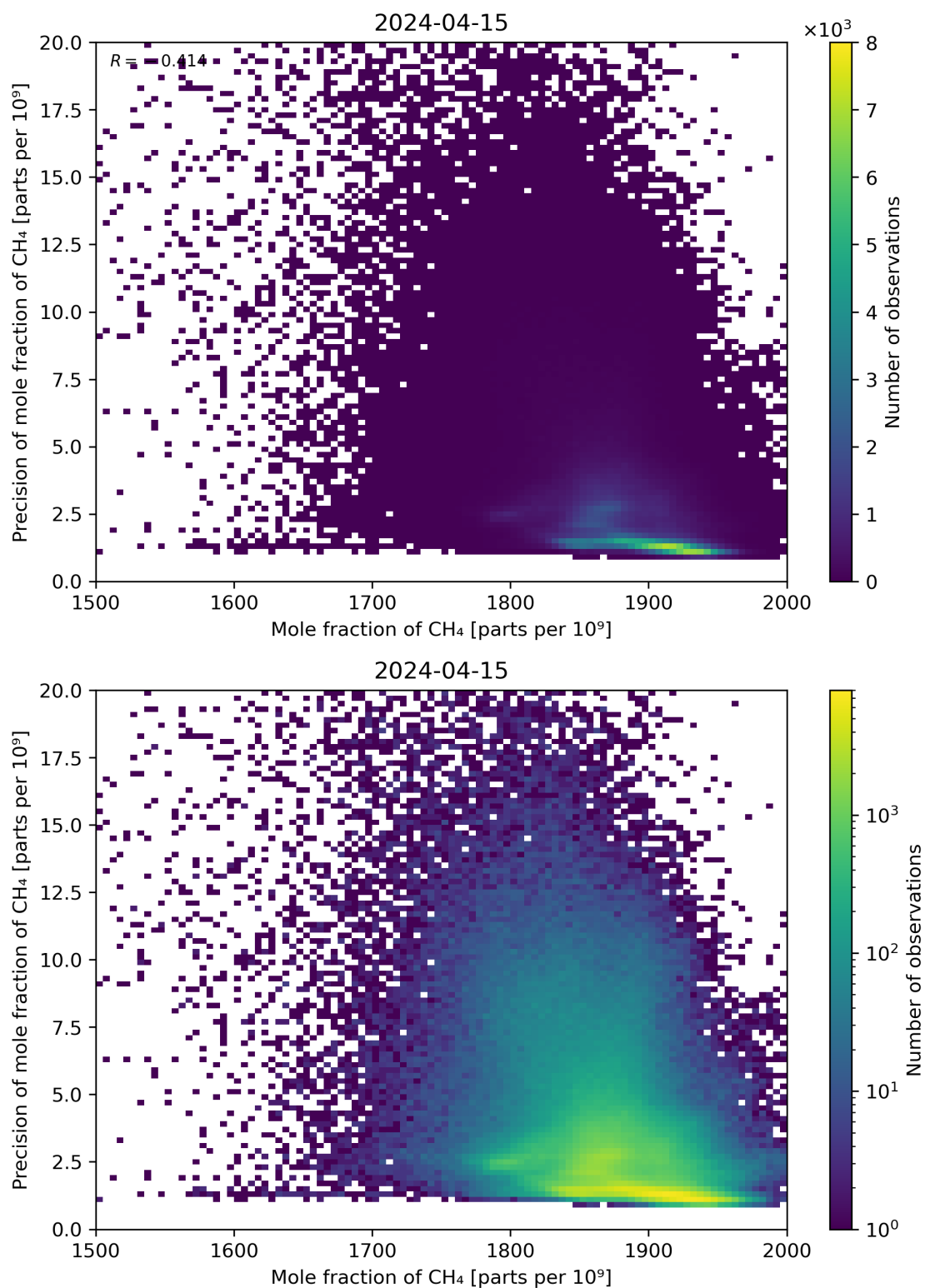
Figure 75: Scatter density plot of “Mole fraction of CH 4 ” against “Precision of mole fraction of CH 4 ” for 2024-04-15 to 2024-04-16.
