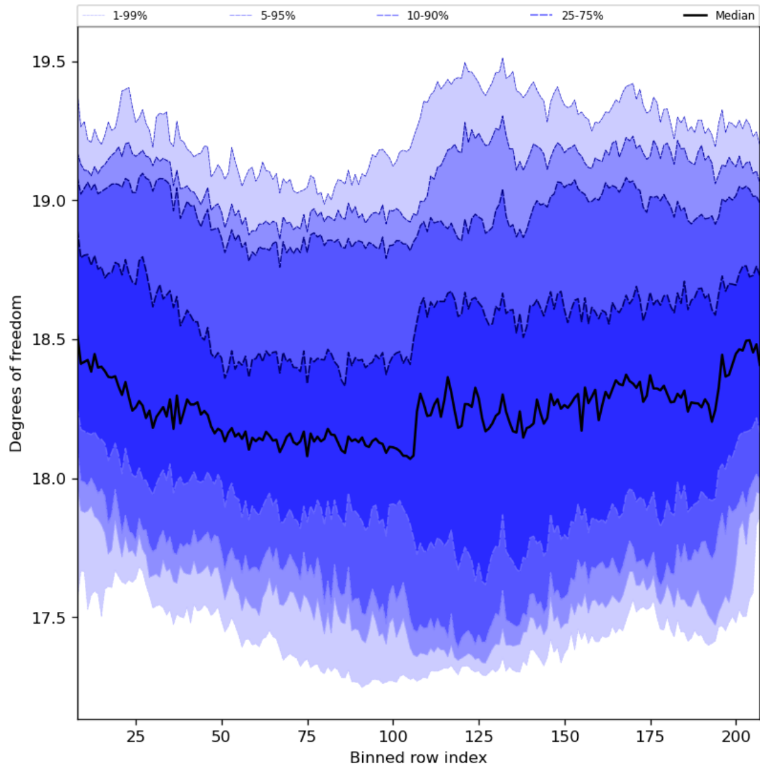
Figure 41: Along track statistics of “Degrees of freedom” for 2024-04-15 to 2024-04-16
