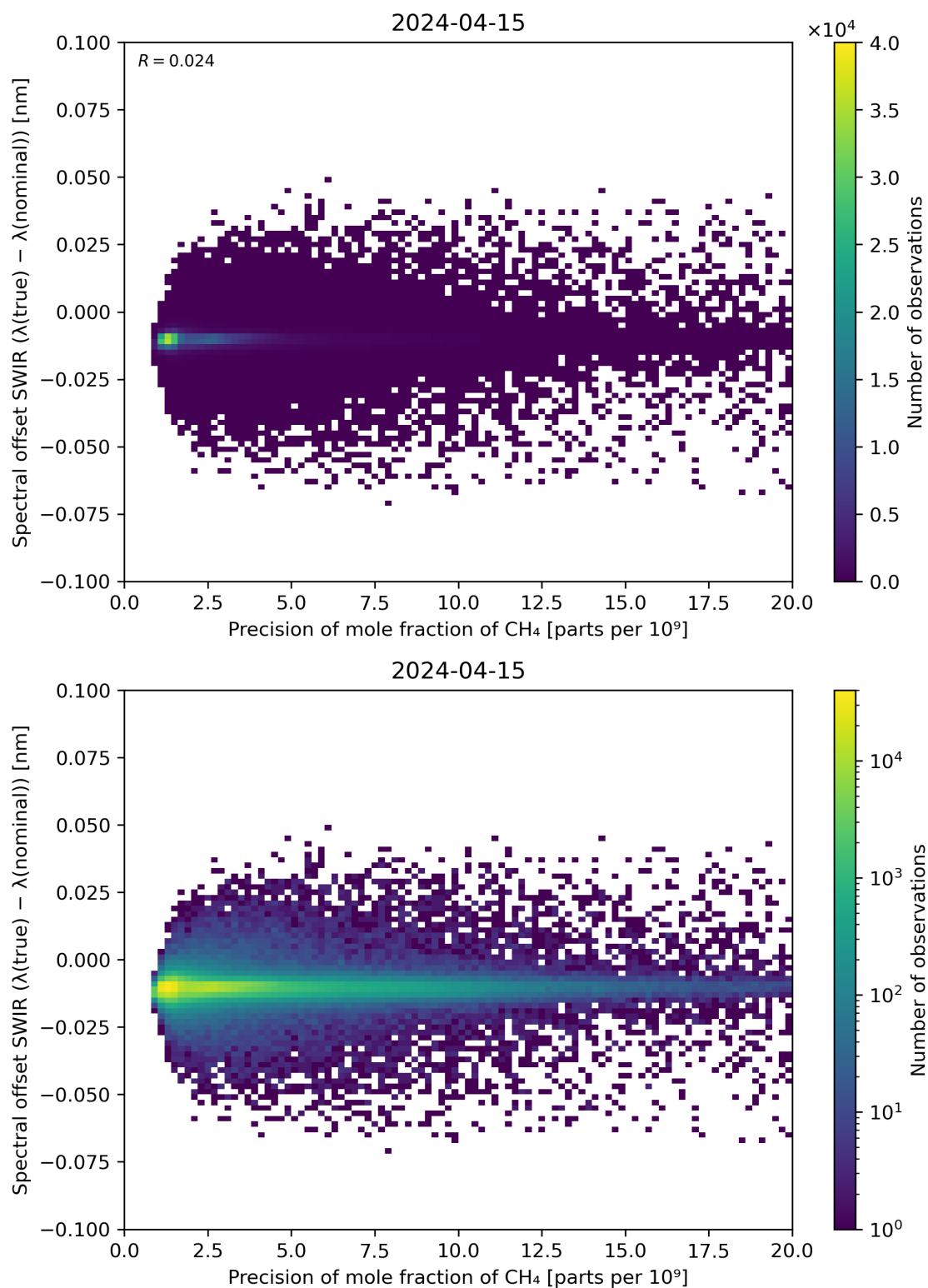
Figure 85: Scatter density plot of “Precision of mole fraction of \text{CH}_4 ” against “Spectral offset SWIR ( \lambda(\text{true}) - \lambda(\text{nominal}) )” for 2024-04-15 to 2024-04-16.
