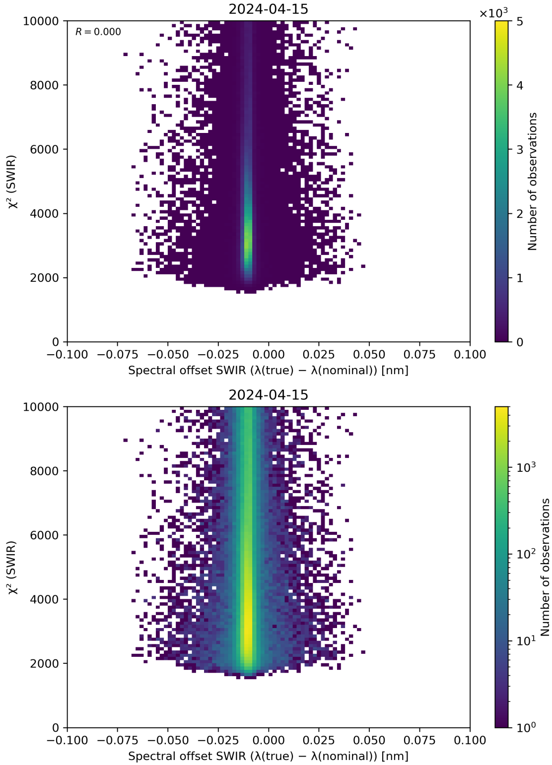
Figure 118: Scatter density plot of “Spectral offset SWIR ( \lambda(\text{true}) - \lambda(\text{nominal}) )” against “ \chi^2 (SWIR)” for 2024-04-15 to 2024-04-16.
