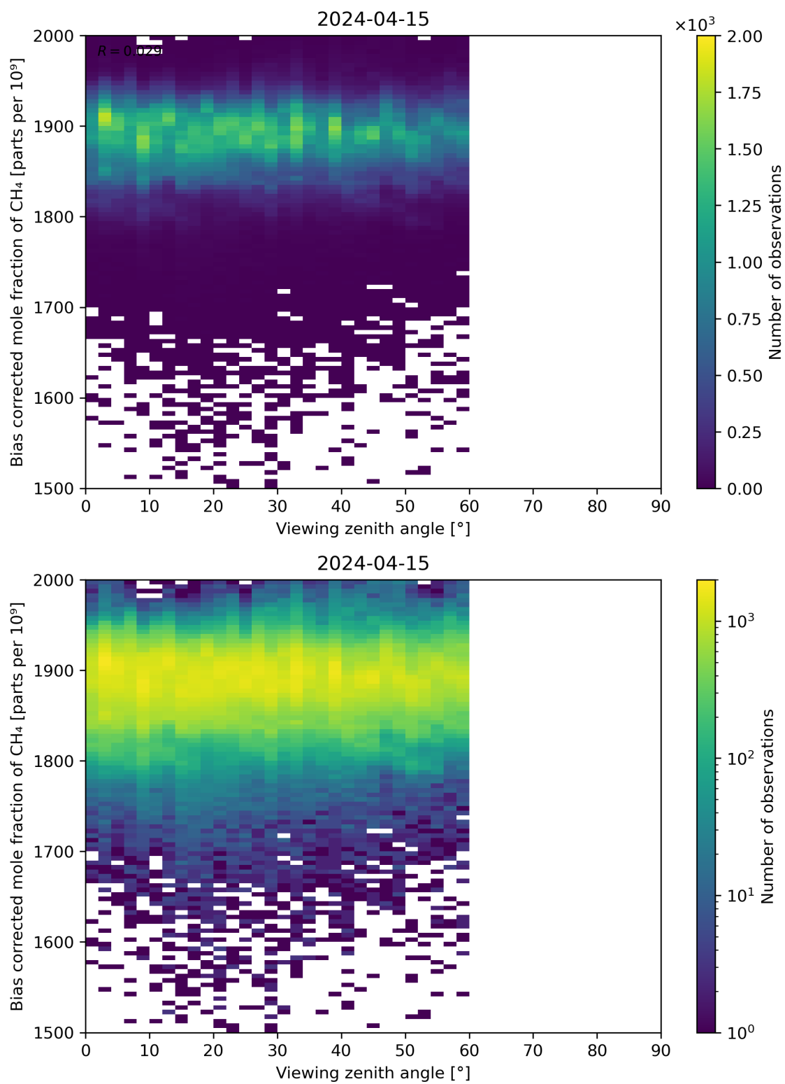
Figure 111: Scatter density plot of “Viewing zenith angle” against “Bias corrected mole fraction of CH 4 ” for 2024-04-15 to 2024-04-16.
