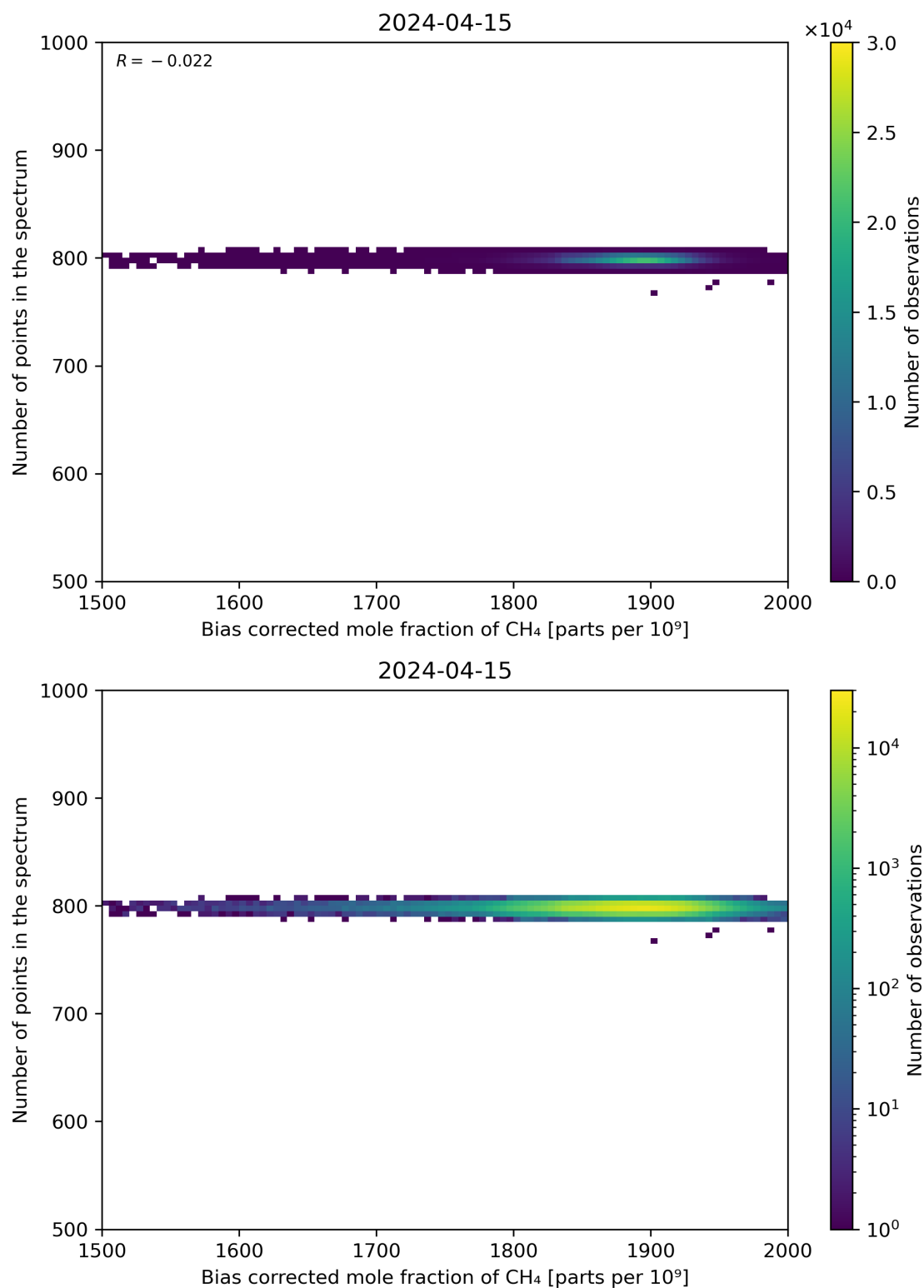
Figure 68: Scatter density plot of “Bias corrected mole fraction of CH 4 ” against “Number of points in the spectrum” for 2024-04-15 to 2024-04-16.
