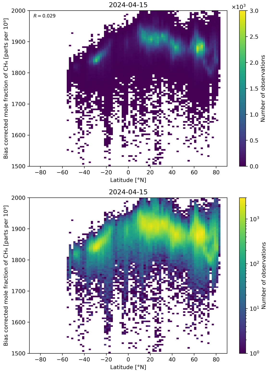
Figure 58: Scatter density plot of “Latitude” against “Bias corrected mole fraction of \text{CH}_4 ” for 2024-04-15 to 2024-04-16.
