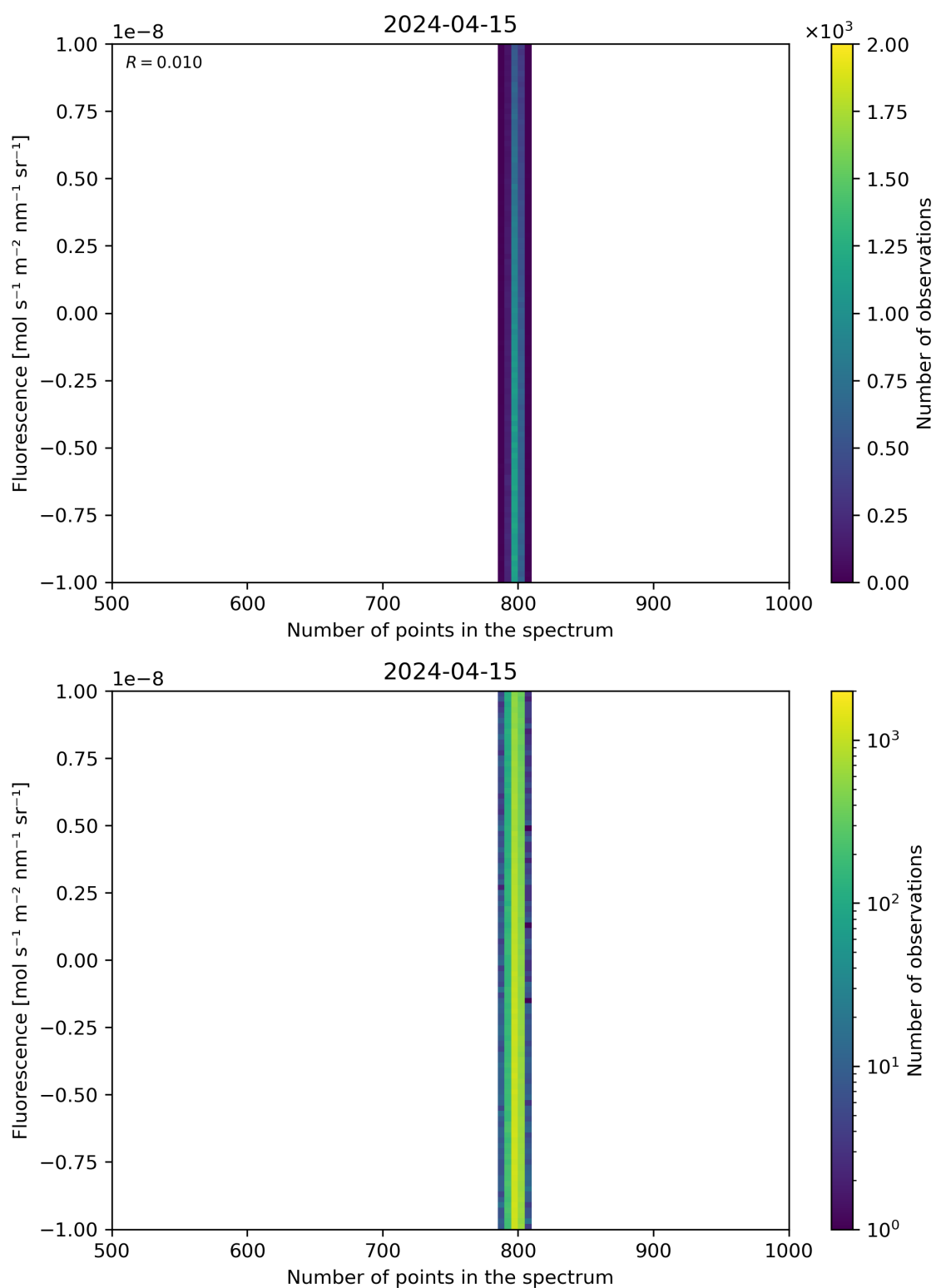
Figure 91: Scatter density plot of “Number of points in the spectrum” against “Fluorescence” for 2024-04-15 to 2024-04-16.
