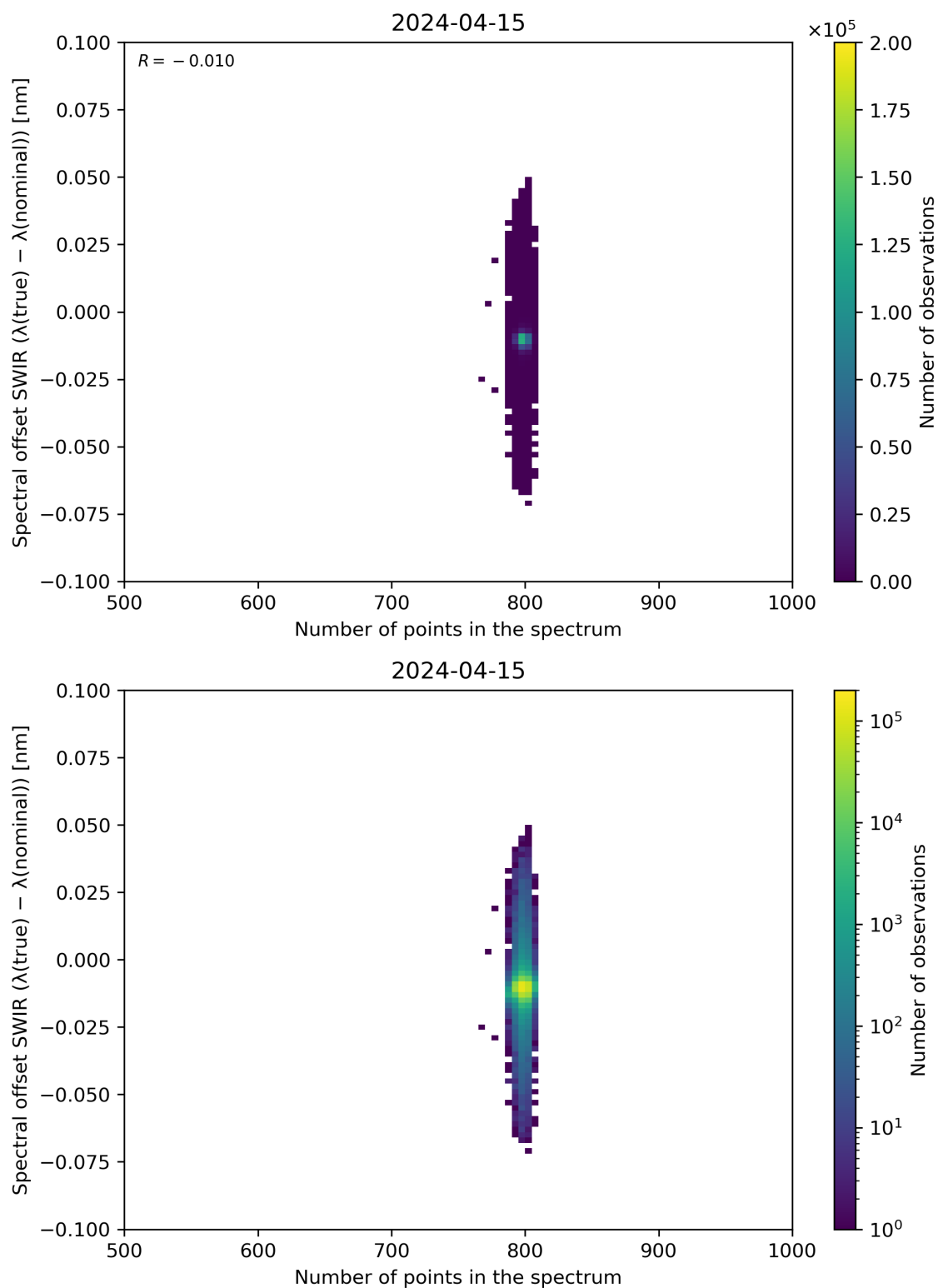
Figure 93: Scatter density plot of “Number of points in the spectrum” against “Spectral offset SWIR ( \lambda(\text{true}) - \lambda(\text{nominal}) )” for 2024-04-15 to 2024-04-16.
