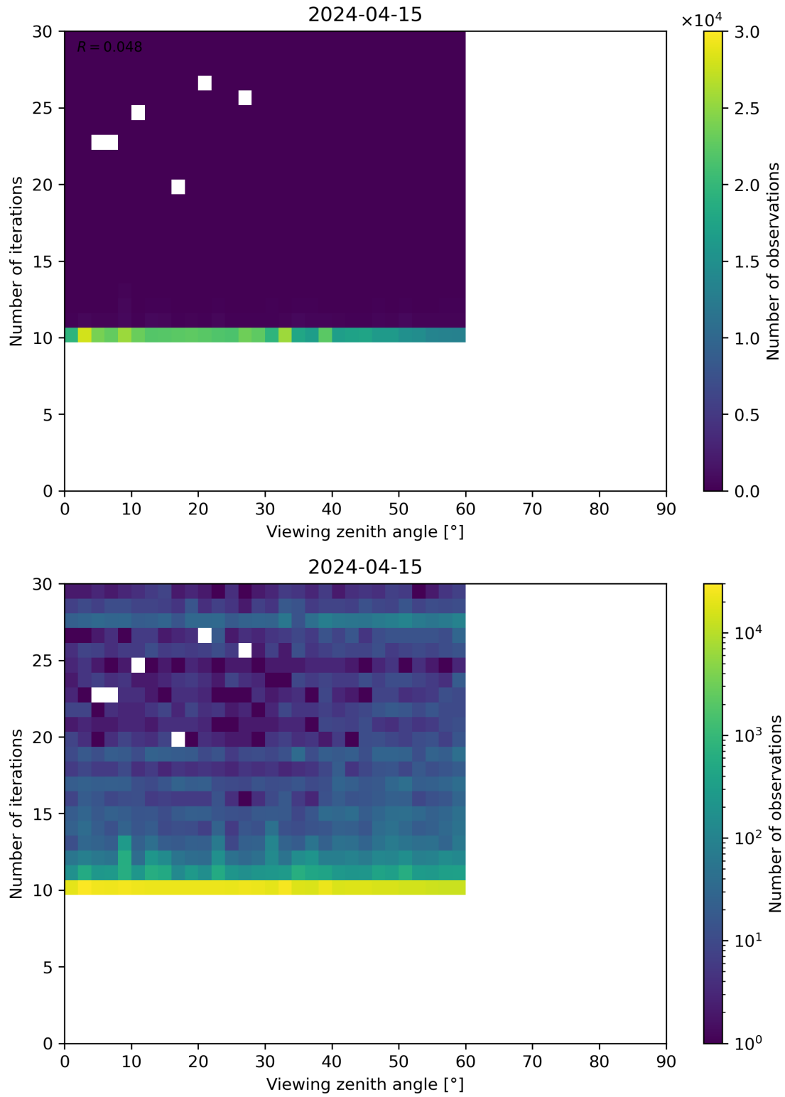
Figure 113: Scatter density plot of “Viewing zenith angle” against “Number of iterations” for 2024-04-15 to 2024-04-16.
