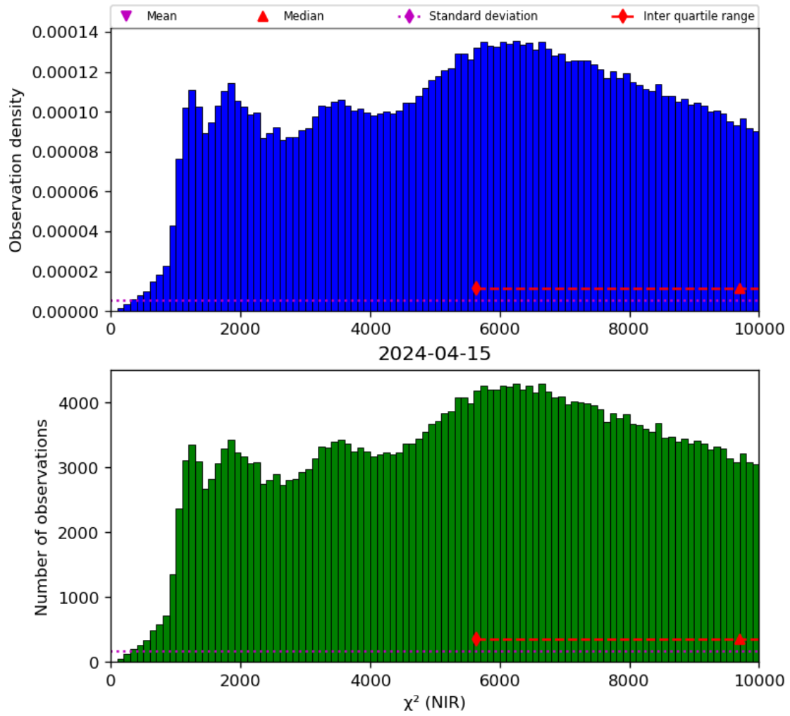
Figure 29: Histogram of “ \chi^2 (NIR)” for 2024-04-15 to 2024-04-16
