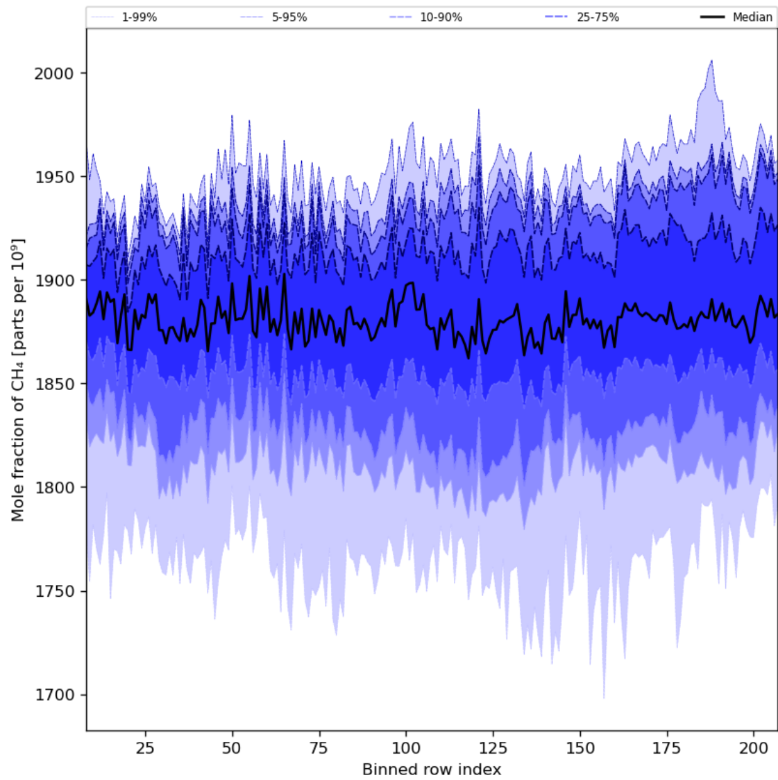
Figure 34: Along track statistics of “Mole fraction of CH 4 ” for 2024-04-15 to 2024-04-16
