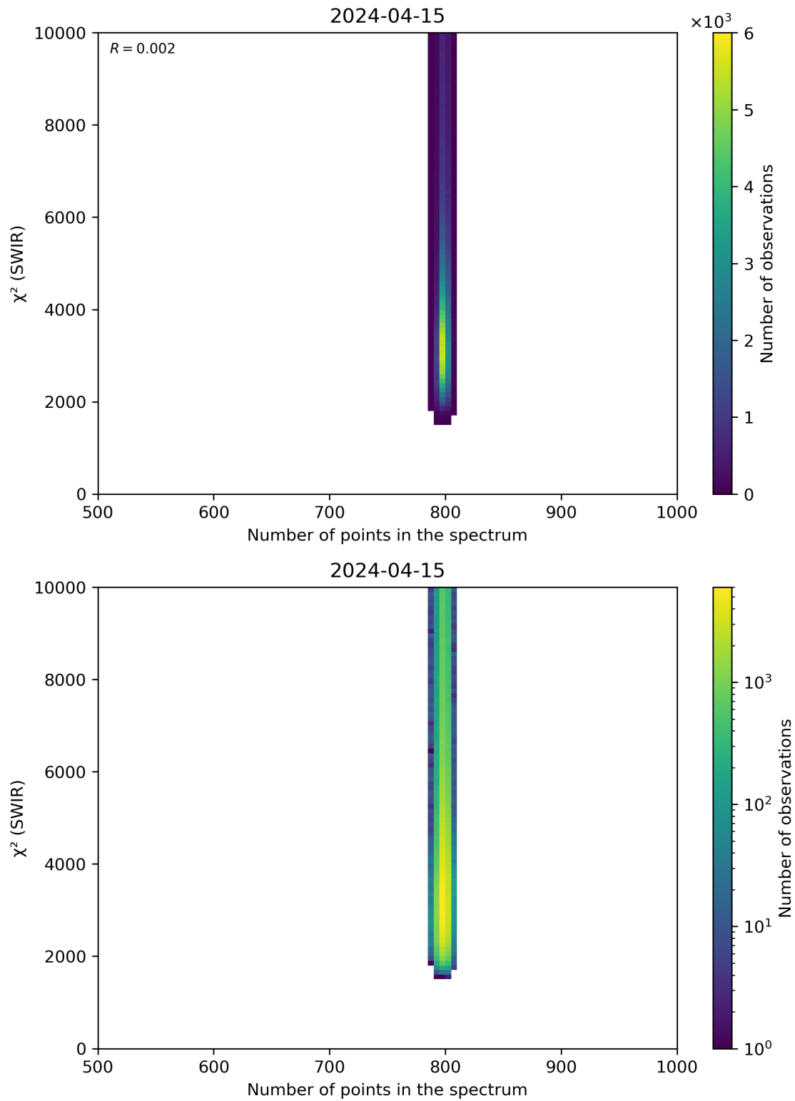
Figure 89: Scatter density plot of “Number of points in the spectrum” against “ \chi^2 (SWIR)” for 2024-04-15 to 2024-04-16.
