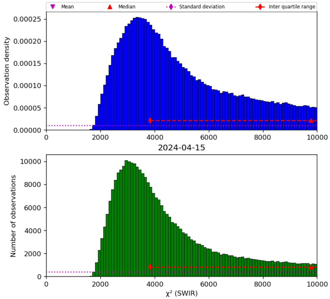
Figure 28: Histogram of “ \chi^2 (SWIR)” for 2024-04-15 to 2024-04-16
