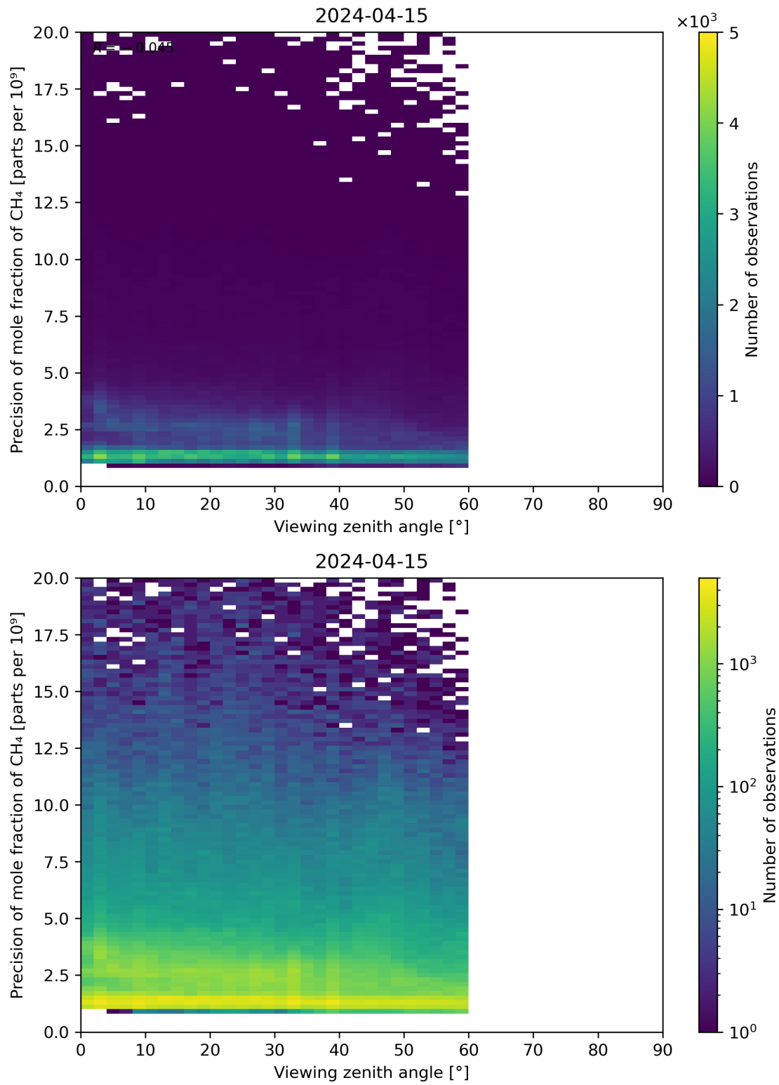
Figure 112: Scatter density plot of “Viewing zenith angle” against “Precision of mole fraction of CH 4 ” for 2024-04-15 to 2024-04-16.
