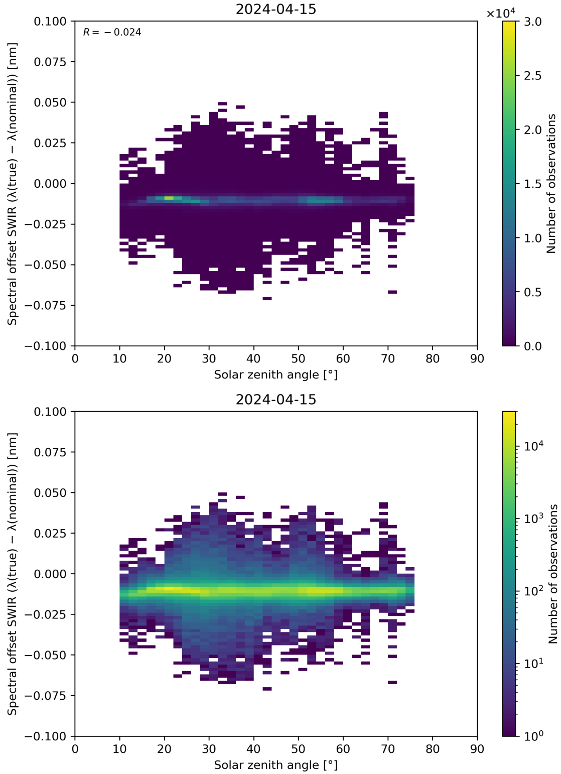
Figure 104: Scatter density plot of “Solar zenith angle” against “Spectral offset SWIR ( \lambda(\text{true}) - \lambda(\text{nominal}) )” for 2024-04-15 to 2024-04-16.
