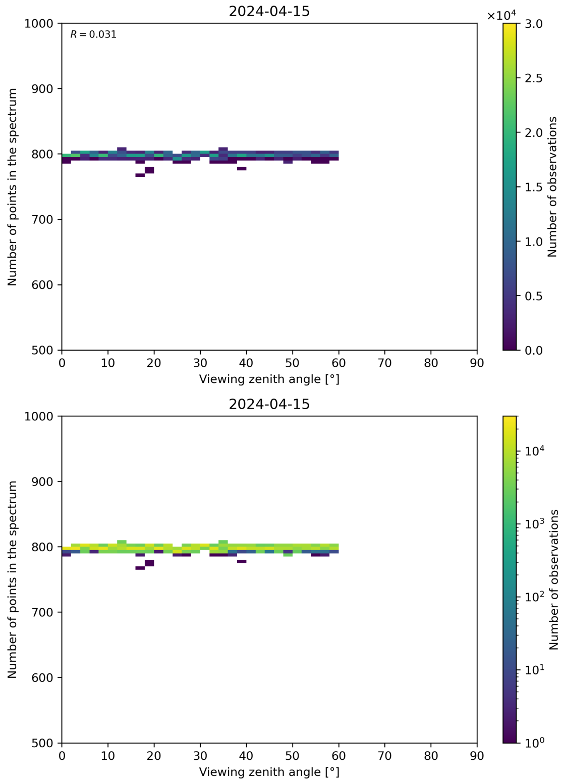
Figure 114: Scatter density plot of “Viewing zenith angle” against “Number of points in the spectrum” for 2024-04-15 to 2024-04-16.
