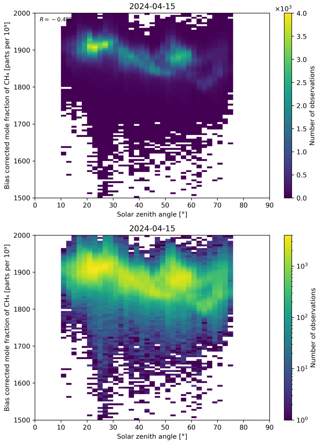
Figure 100: Scatter density plot of “Solar zenith angle” against “Bias corrected mole fraction of CH 4 ” for 2024-04-15 to 2024-04-16.
