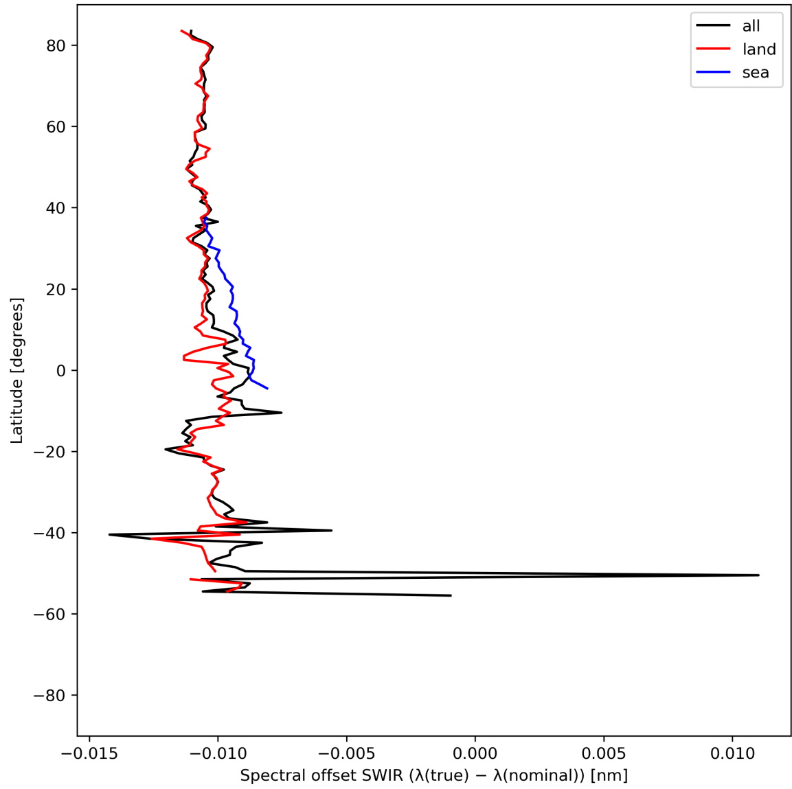
Figure 16: Zonal average of “Spectral offset SWIR ( \lambda(\text{true}) - \lambda(\text{nominal}) )” for 2024-04-15 to 2024-04-16.
