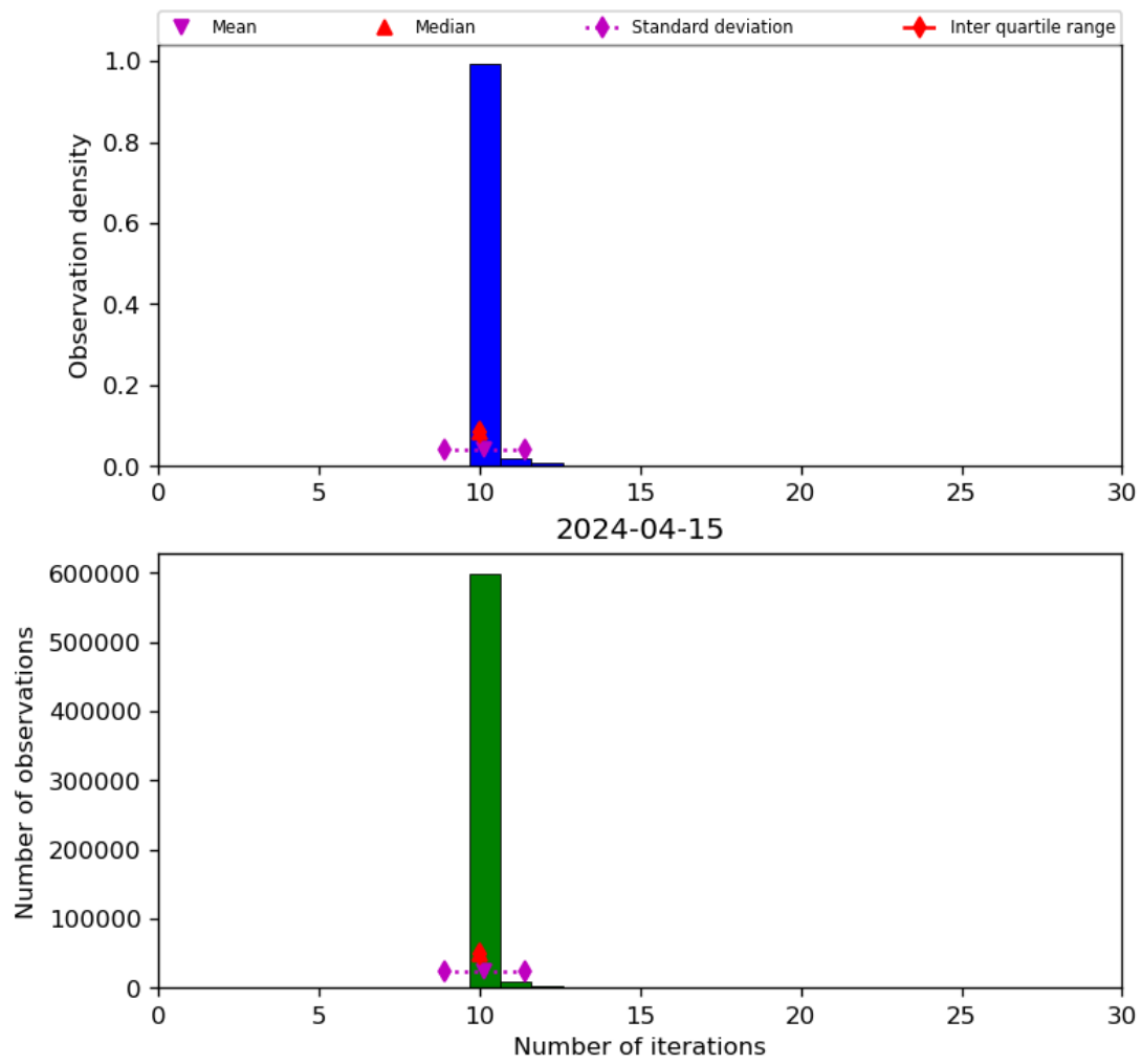
Figure 31: Histogram of “Number of iterations” for 2024-04-15 to 2024-04-16
