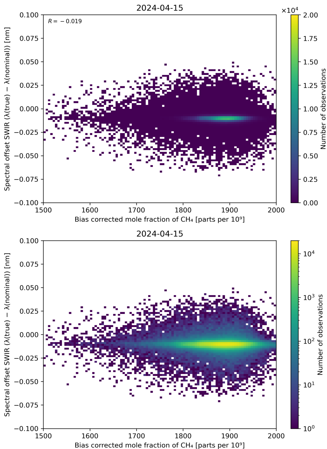
Figure 69: Scatter density plot of “Bias corrected mole fraction of \text{CH}_4 ” against “Spectral offset SWIR ( \lambda(\text{true}) - \lambda(\text{nominal}) )” for 2024-04-15 to 2024-04-16.
