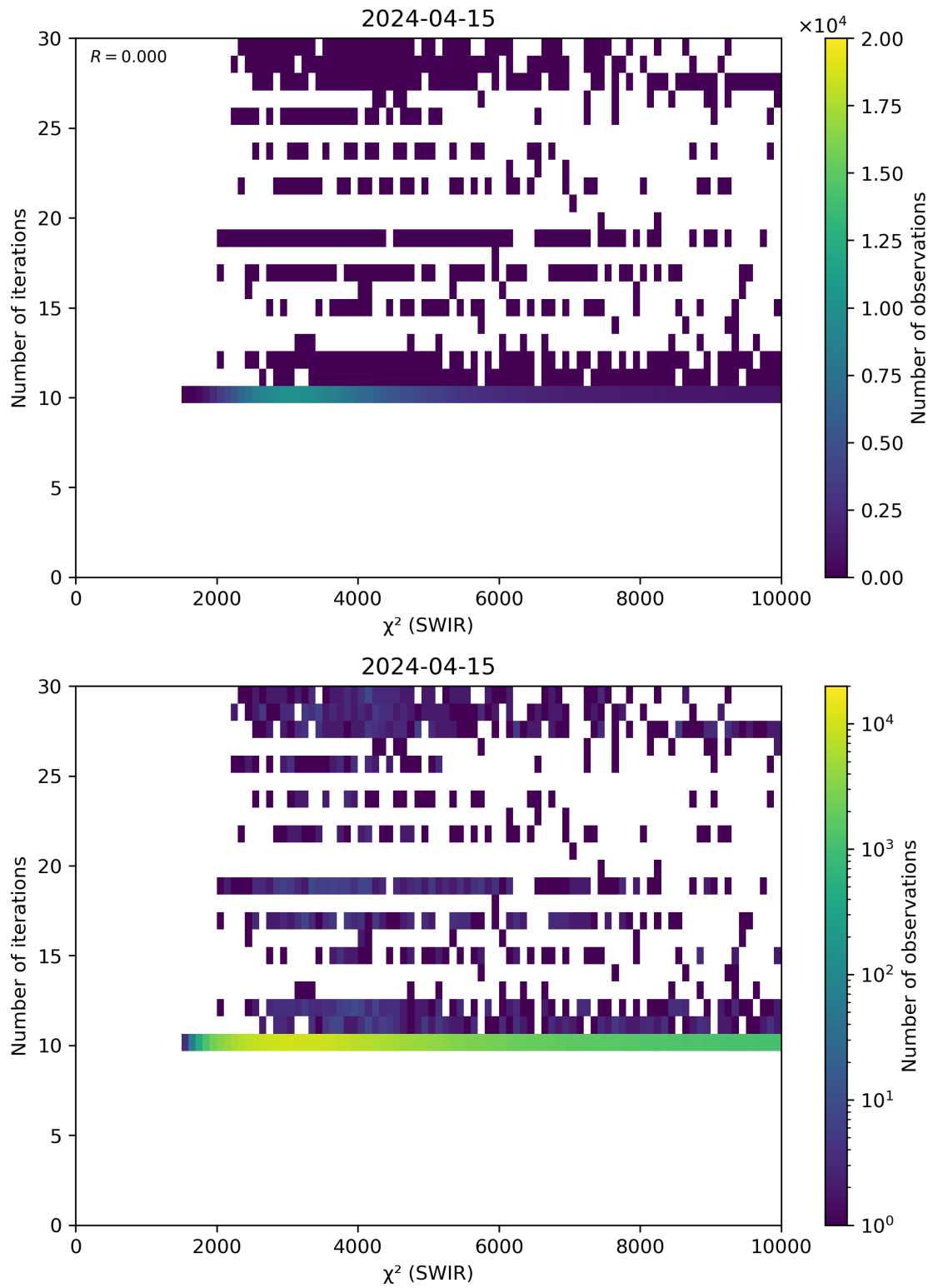
Figure 50: Scatter density plot of “ \chi^2 (SWIR)” against “Number of iterations” for 2024-04-15 to 2024-04-16.
