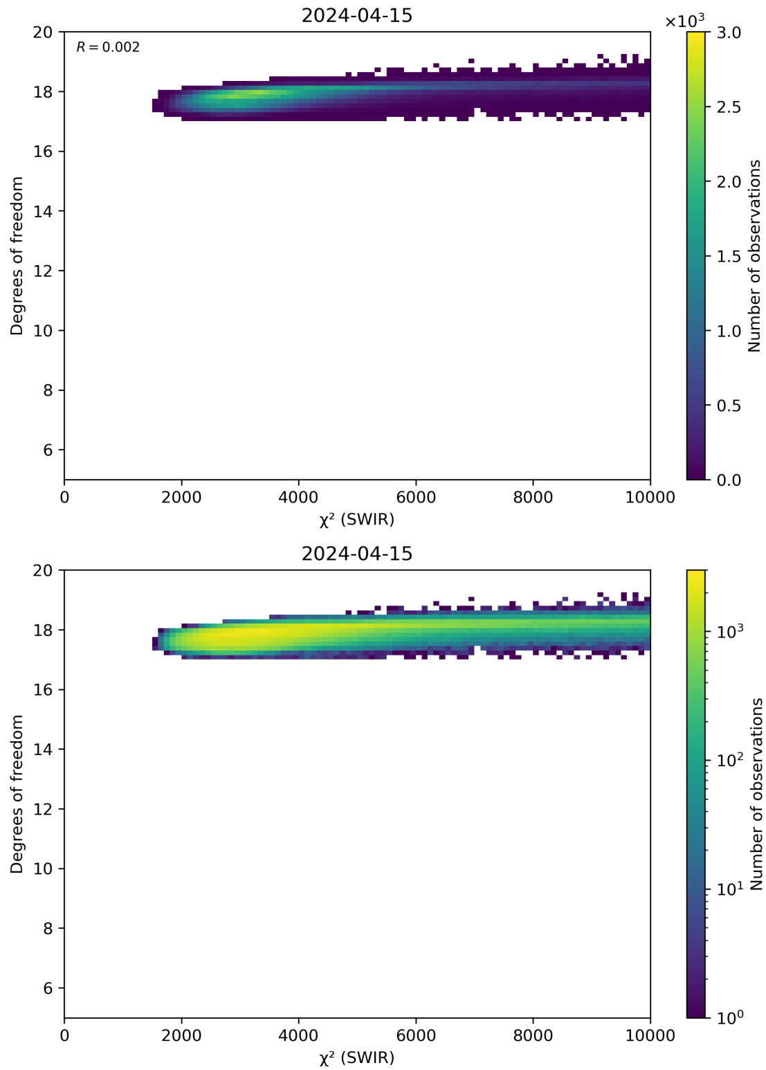
Figure 48: Scatter density plot of " \chi^2 (SWIR)" against "Degrees of freedom" for 2024-04-15 to 2024-04-16.
