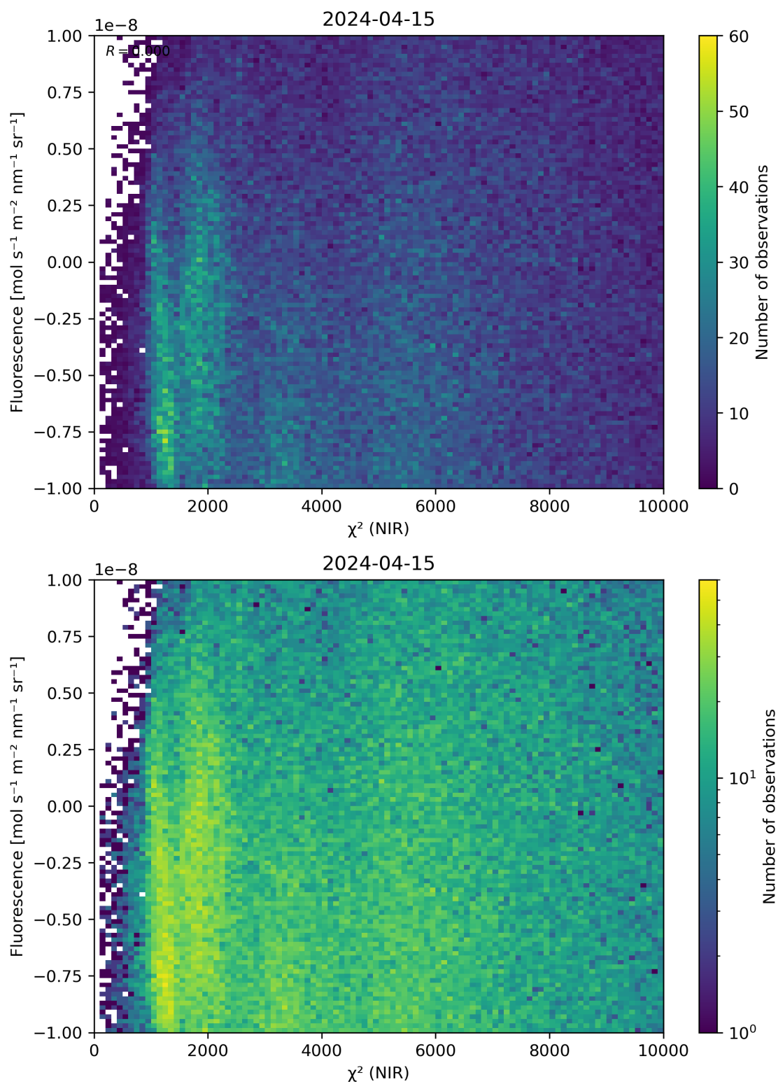
Figure 45: Scatter density plot of “ \chi^2 (NIR)” against “Fluorescence” for 2024-04-15 to 2024-04-16.
