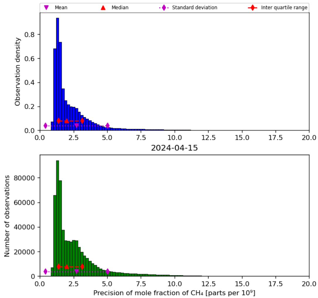
Figure 24: Histogram of “Precision of mole fraction of CH 4 ” for 2024-04-15 to 2024-04-16
