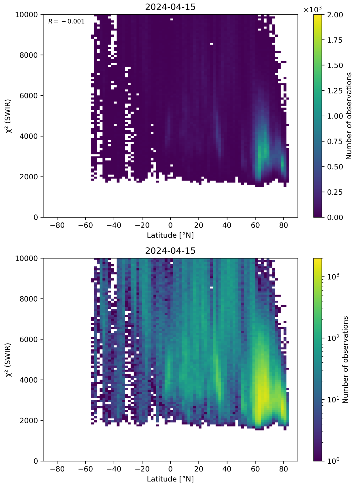
Figure 54: Scatter density plot of “Latitude” against “ \chi^2 (SWIR)” for 2024-04-15 to 2024-04-16.
