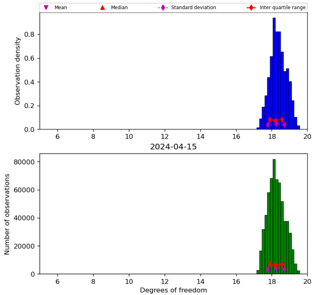
Figure 30: Histogram of “Degrees of freedom” for 2024-04-15 to 2024-04-16
