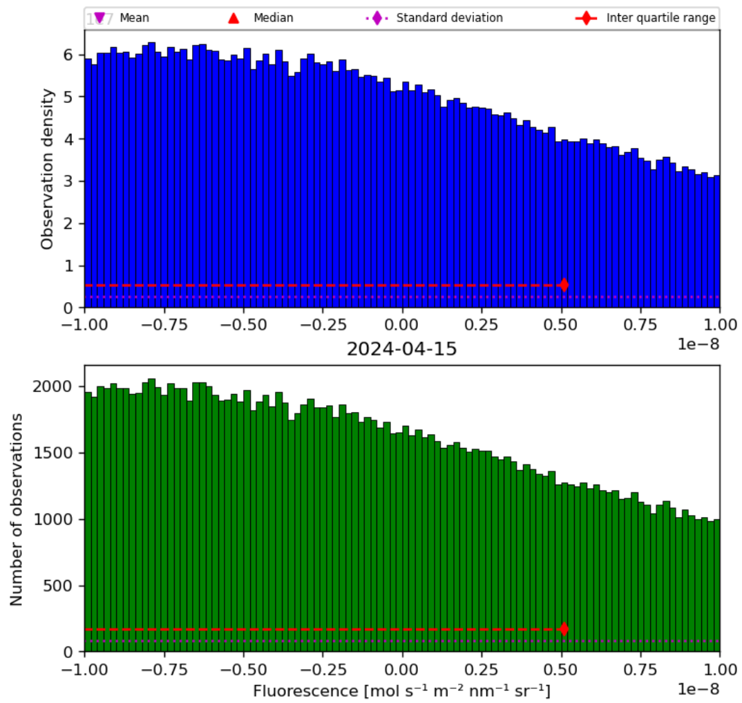
Figure 32: Histogram of “Fluorescence” for 2024-04-15 to 2024-04-16
