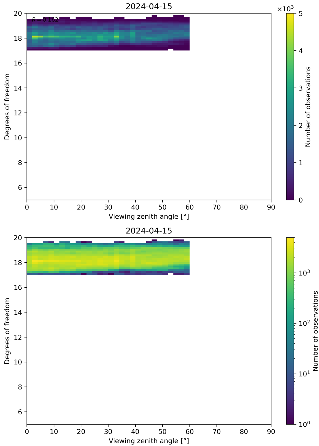
Figure 107: Scatter density plot of “Viewing zenith angle” against “Degrees of freedom” for 2024-04-15 to 2024-04-16.
