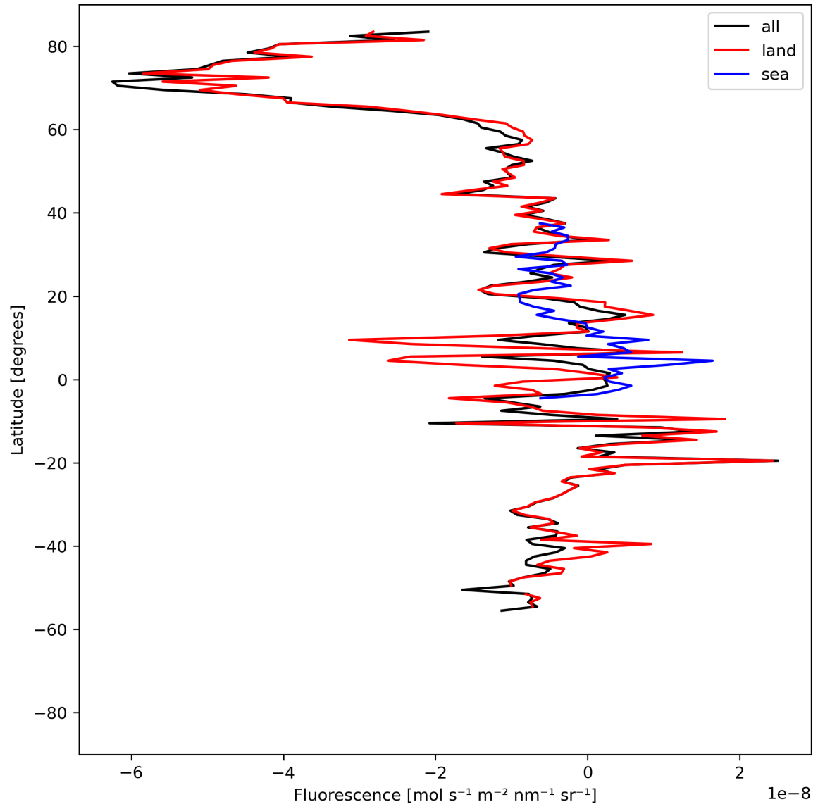
Figure 21: Zonal average of “Fluorescence” for 2024-04-15 to 2024-04-16.
