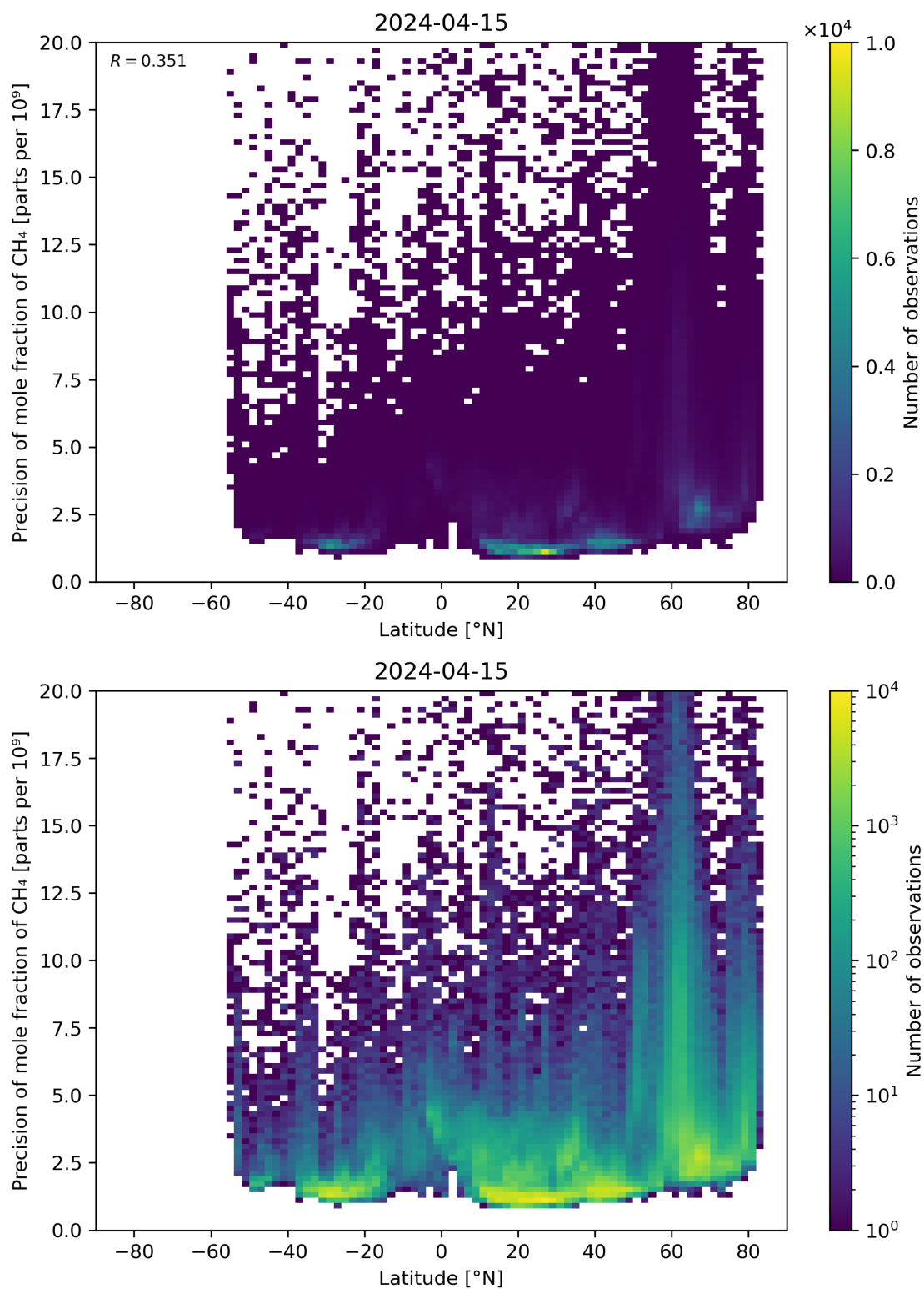
Figure 59: Scatter density plot of “Latitude” against “Precision of mole fraction of \text{CH}_4 ” for 2024-04-15 to 2024-04-16.
