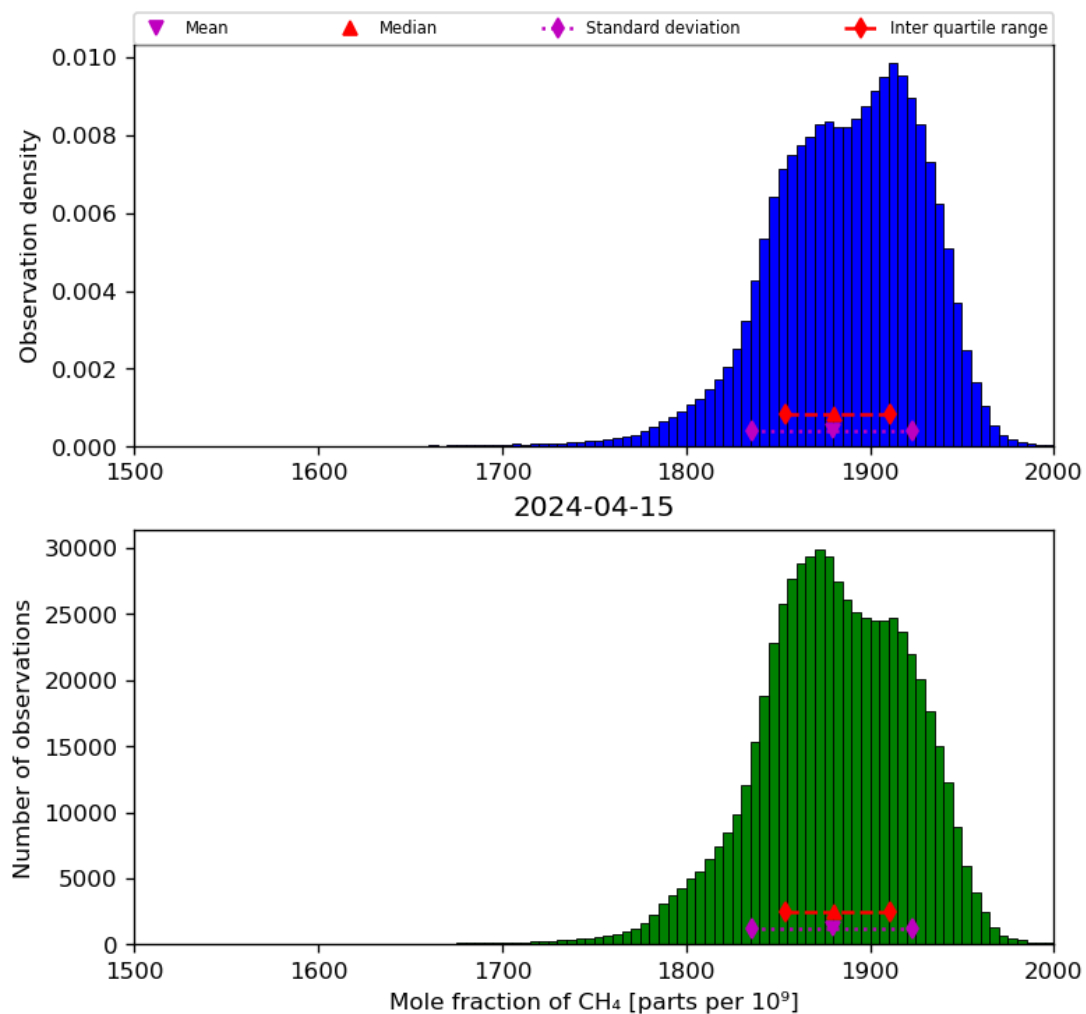
Figure 23: Histogram of “Mole fraction of CH 4 ” for 2024-04-15 to 2024-04-16
