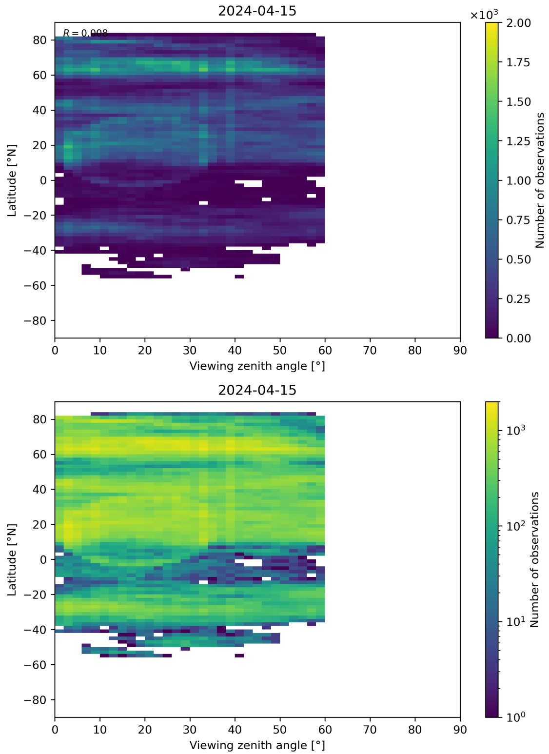
Figure 109: Scatter density plot of “Viewing zenith angle” against “Latitude” for 2024-04-15 to 2024-04-16.
