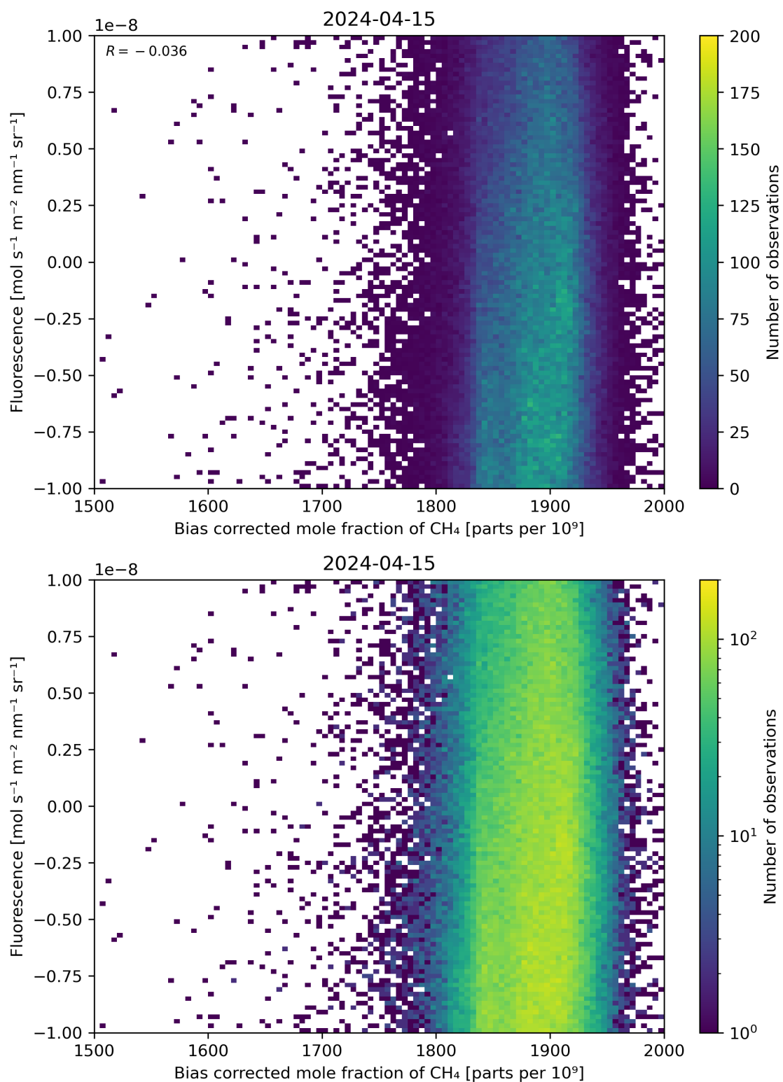
Figure 66: Scatter density plot of “Bias corrected mole fraction of \text{CH}_4 ” against “Fluorescence” for 2024-04-15 to 2024-04-16.
