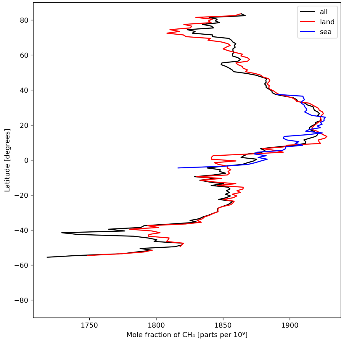
Figure 12: Zonal average of “Mole fraction of \text{CH}_4 ” for 2024-04-15 to 2024-04-16.
