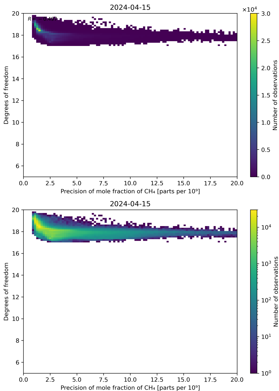
Figure 80: Scatter density plot of “Precision of mole fraction of CH 4 ” against “Degrees of freedom” for 2024-04-15 to 2024-04-16.
