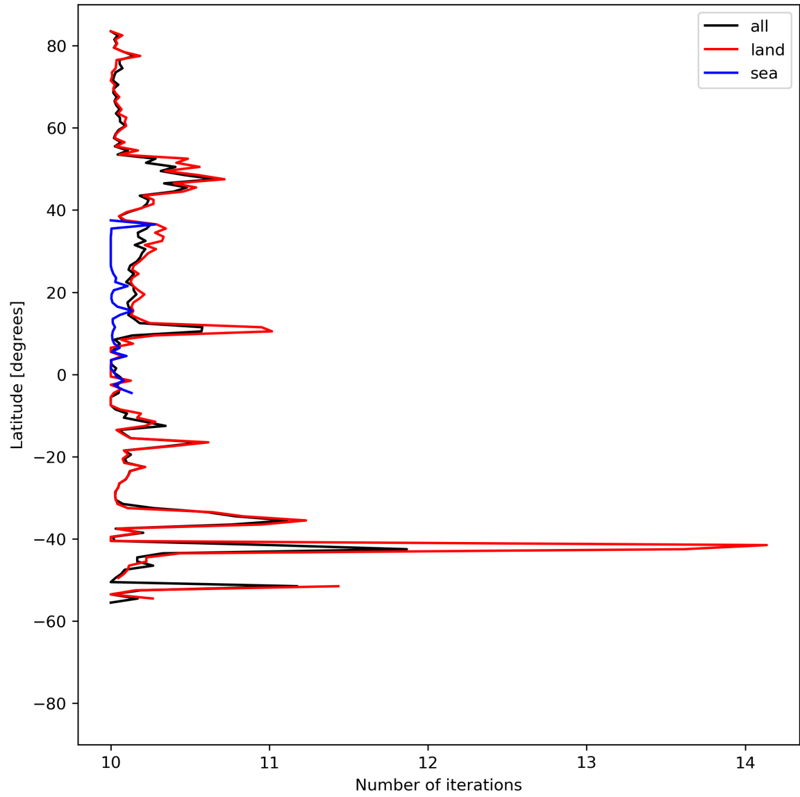
Figure 20: Zonal average of “Number of iterations” for 2024-04-15 to 2024-04-16.
