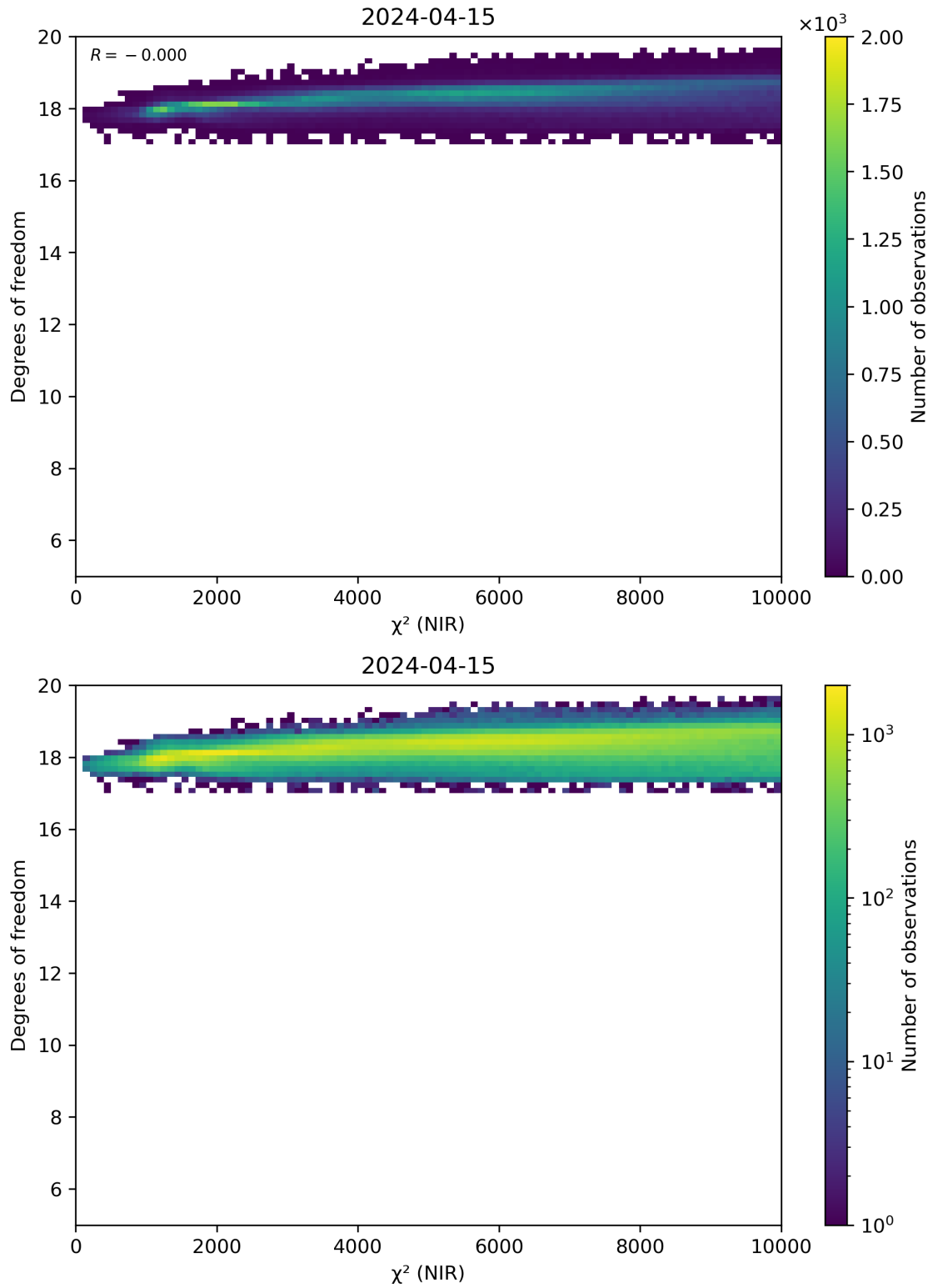
Figure 44: Scatter density plot of “ \chi^2 (NIR)” against “Degrees of freedom” for 2024-04-15 to 2024-04-16.
