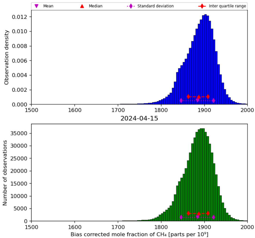
Figure 25: Histogram of “Bias corrected mole fraction of CH 4 ” for 2024-04-15 to 2024-04-16
