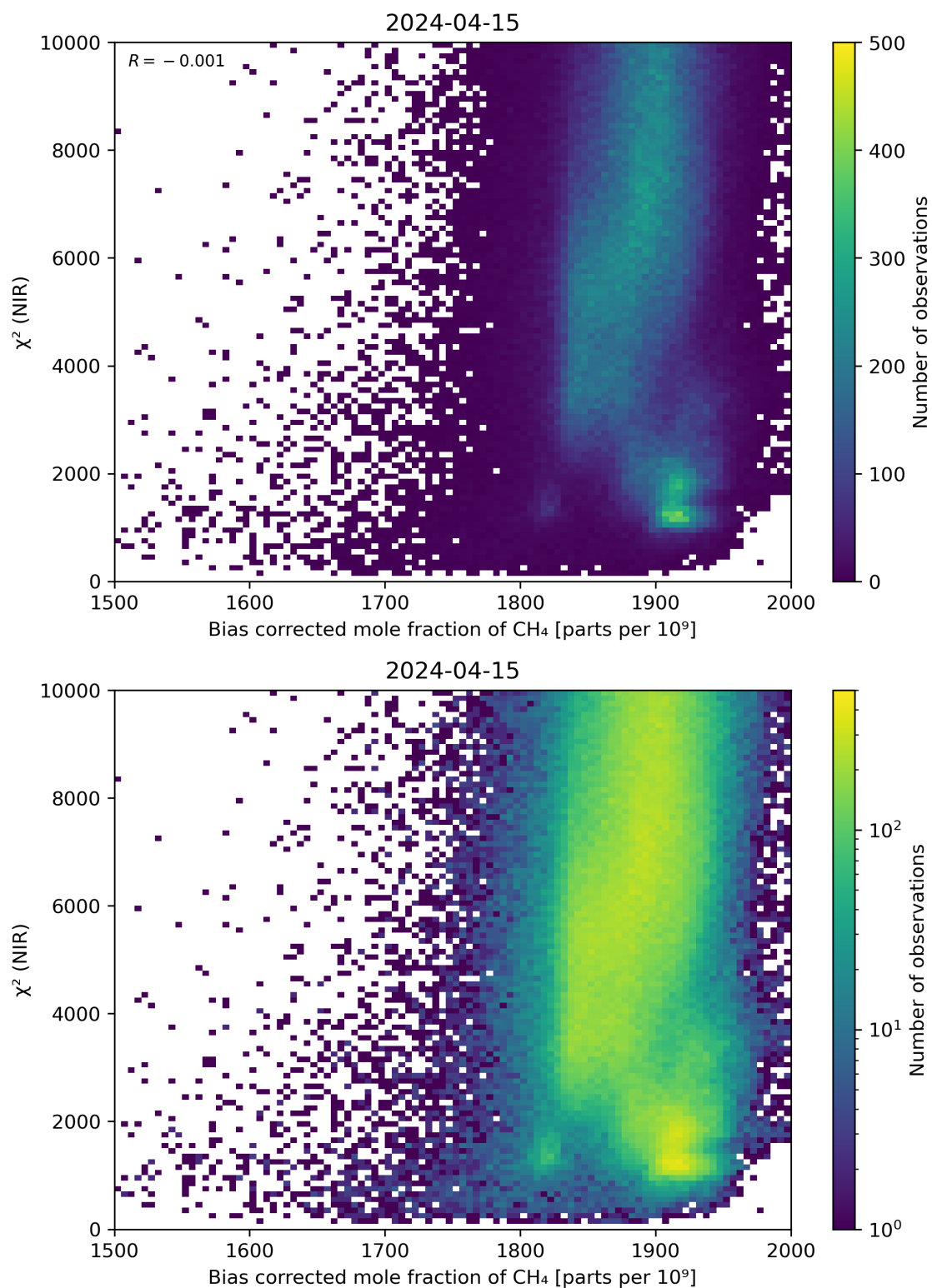
Figure 63: Scatter density plot of “Bias corrected mole fraction of \text{CH}_4 ” against “ \chi^2 (NIR)” for 2024-04-15 to 2024-04-16.
