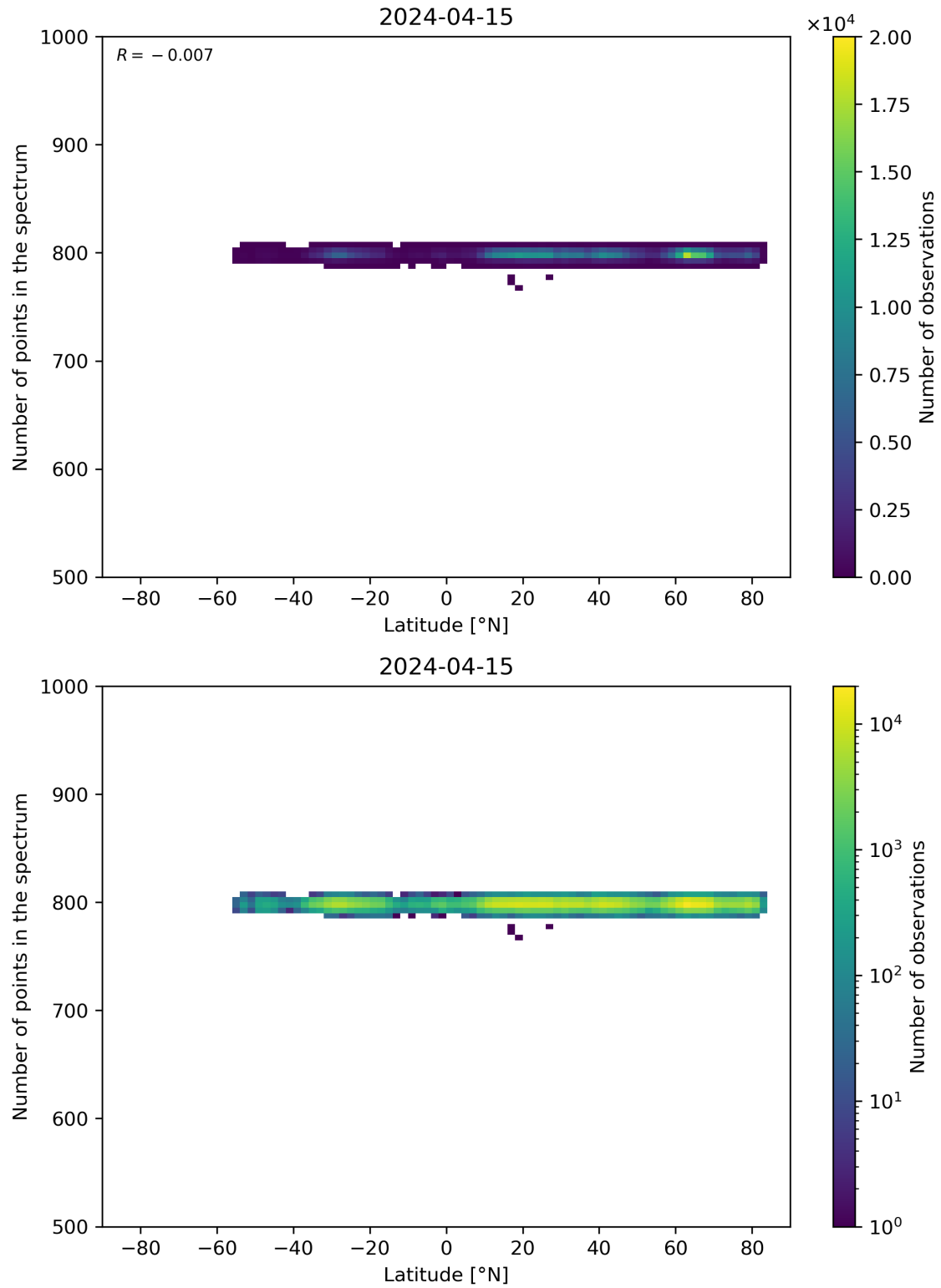
Figure 61: Scatter density plot of “Latitude” against “Number of points in the spectrum” for 2024-04-15 to 2024-04-16.
