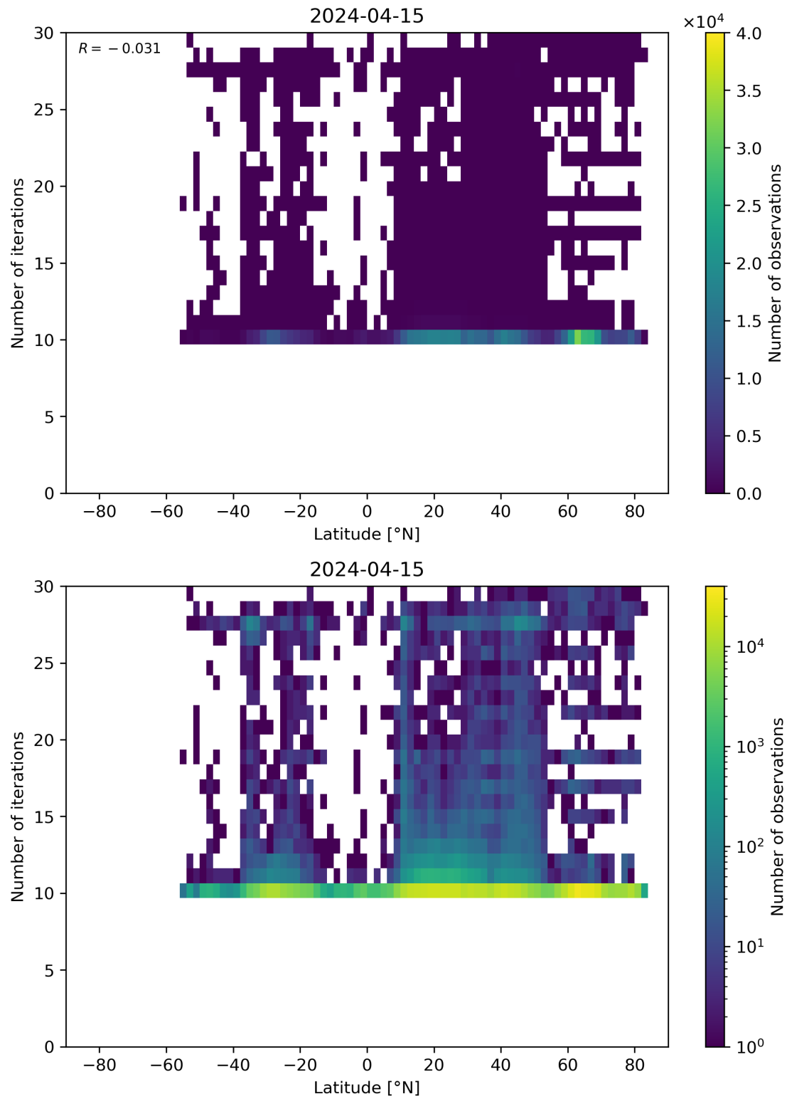
Figure 60: Scatter density plot of “Latitude” against “Number of iterations” for 2024-04-15 to 2024-04-16.
