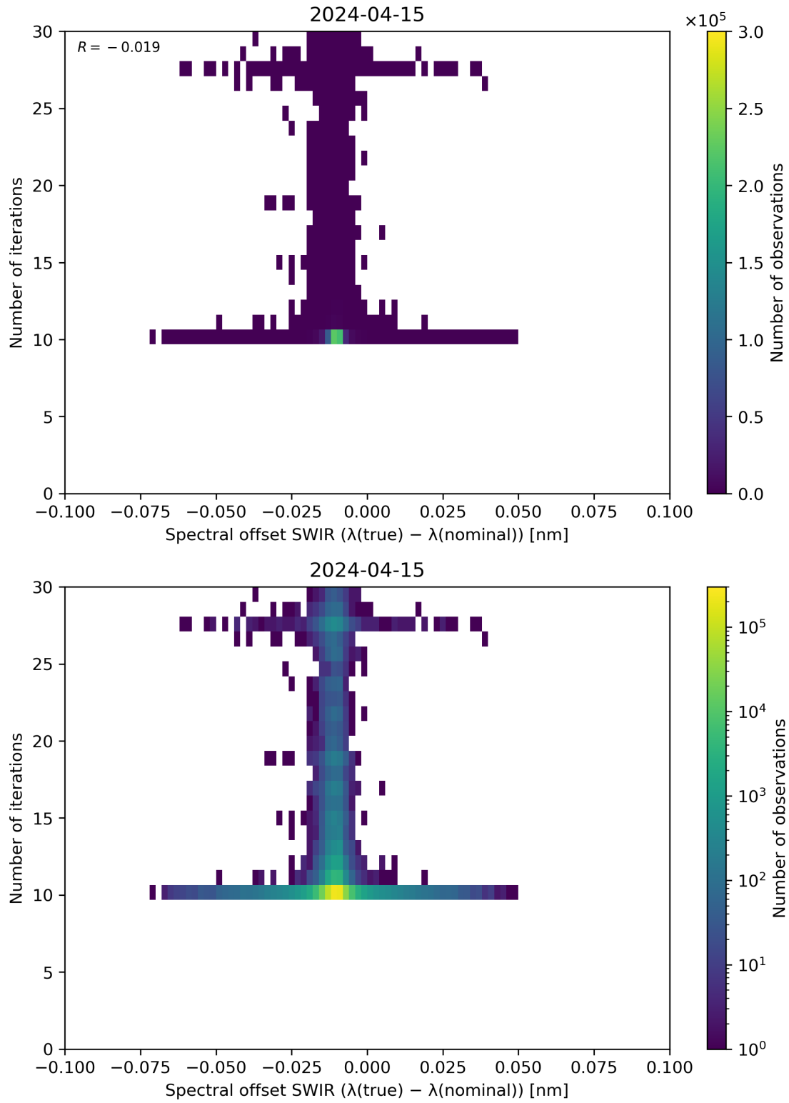
Figure 121: Scatter density plot of “Spectral offset SWIR ( \lambda(\text{true}) - \lambda(\text{nominal}) )” against “Number of iterations” for 2024-04-15 to 2024-04-16.
