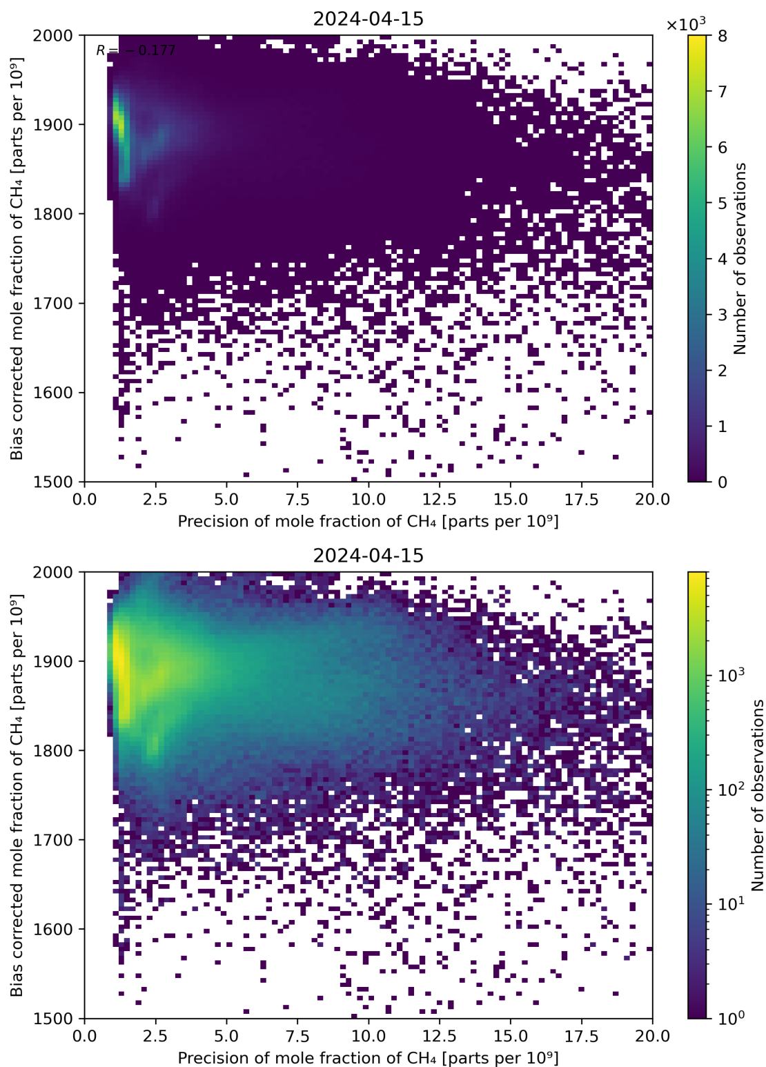
Figure 82: Scatter density plot of “Precision of mole fraction of \text{CH}_4 ” against “Bias corrected mole fraction of \text{CH}_4 ” for 2024-04-15 to 2024-04-16.
