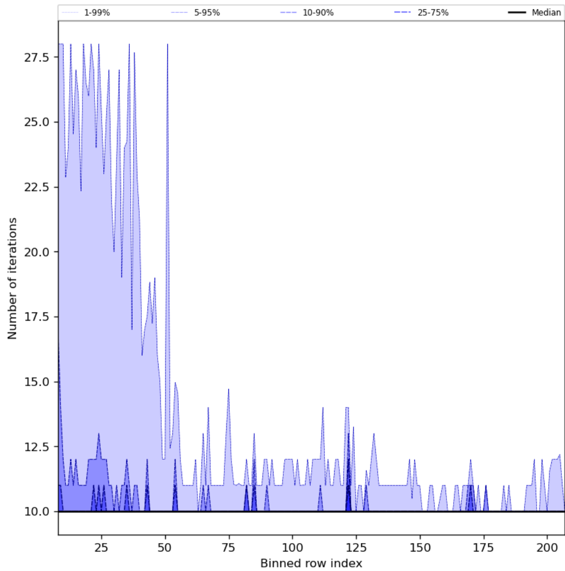
Figure 42: Along track statistics of “Number of iterations” for 2024-04-15 to 2024-04-16
