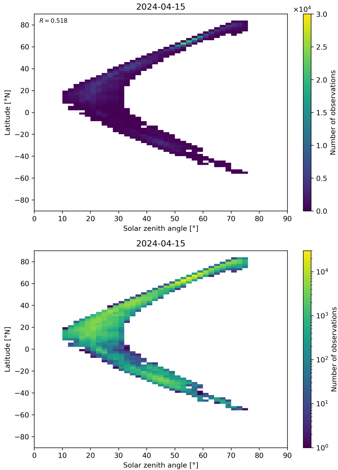
Figure 98: Scatter density plot of “Solar zenith angle” against “Latitude” for 2024-04-15 to 2024-04-16.
