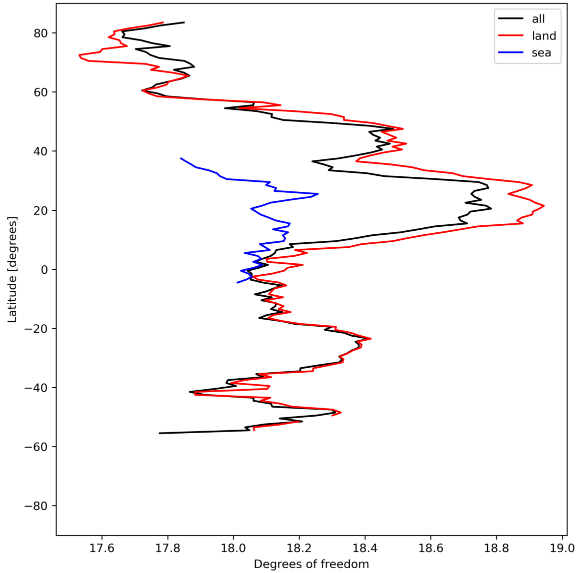
Figure 19: Zonal average of “Degrees of freedom” for 2024-04-15 to 2024-04-16.
