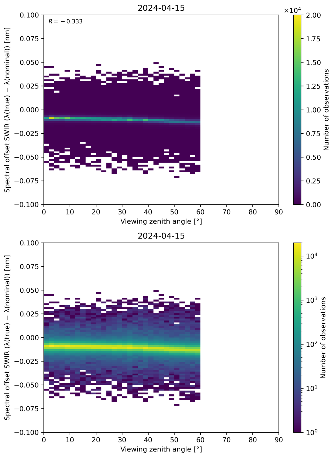
Figure 116: Scatter density plot of “Viewing zenith angle” against “Spectral offset SWIR ( \lambda(\text{true}) - \lambda(\text{nominal}) )” for 2024-04-15 to 2024-04-16.
