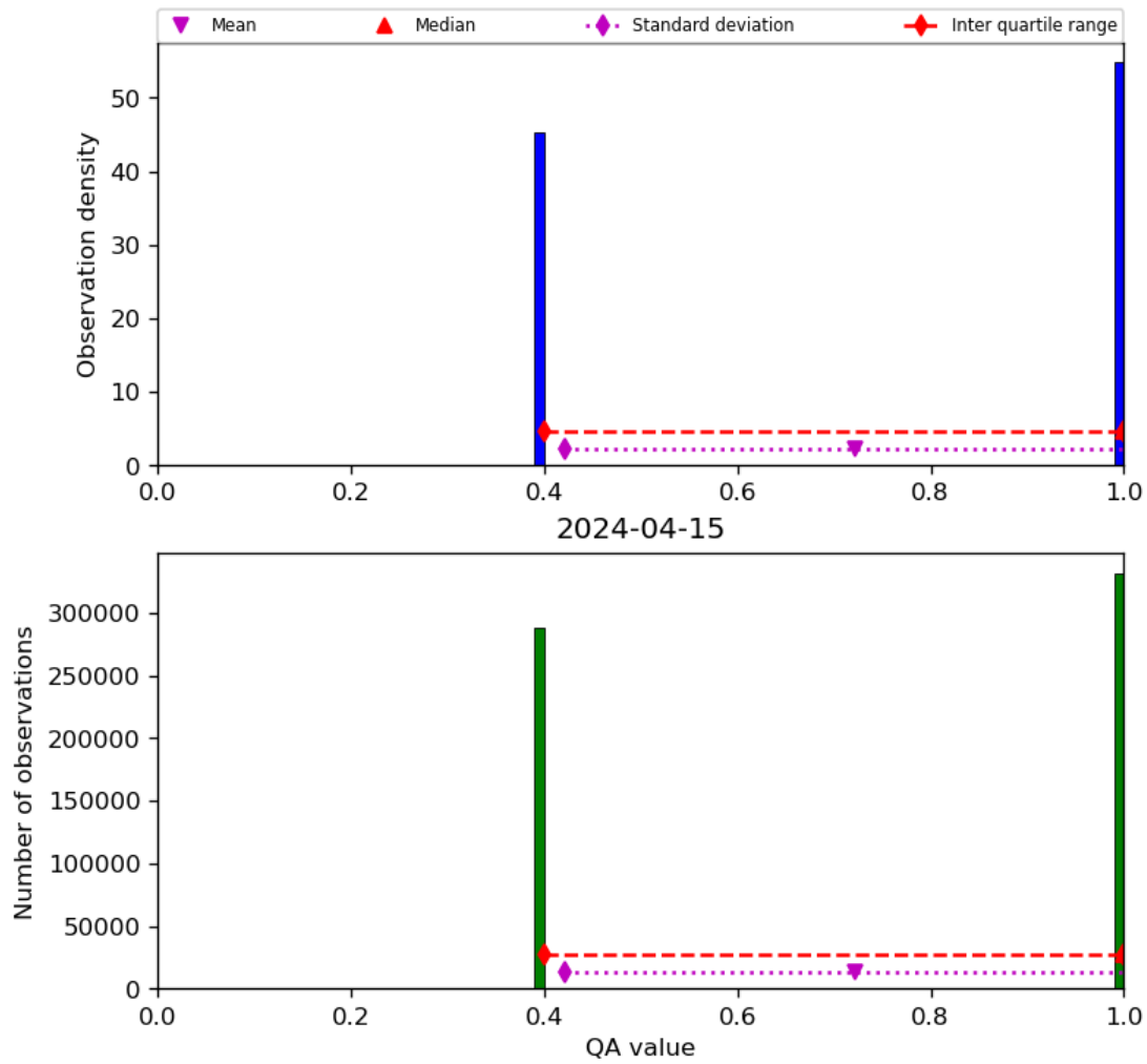
Figure 22: Histogram of “QA value” for 2024-04-15 to 2024-04-16
