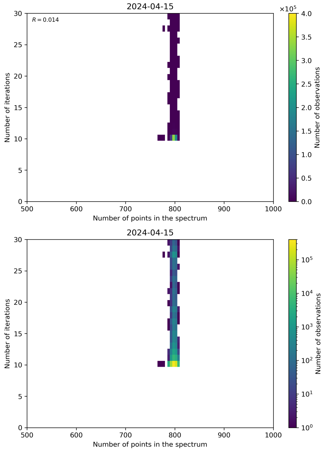
Figure 92: Scatter density plot of “Number of points in the spectrum” against “Number of iterations” for 2024-04-15 to 2024-04-16.
