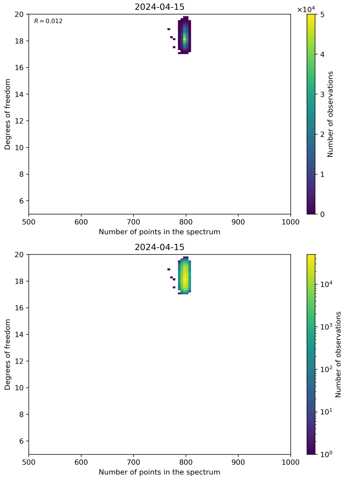
Figure 90: Scatter density plot of “Number of points in the spectrum” against “Degrees of freedom” for 2024-04-15 to 2024-04-16.
