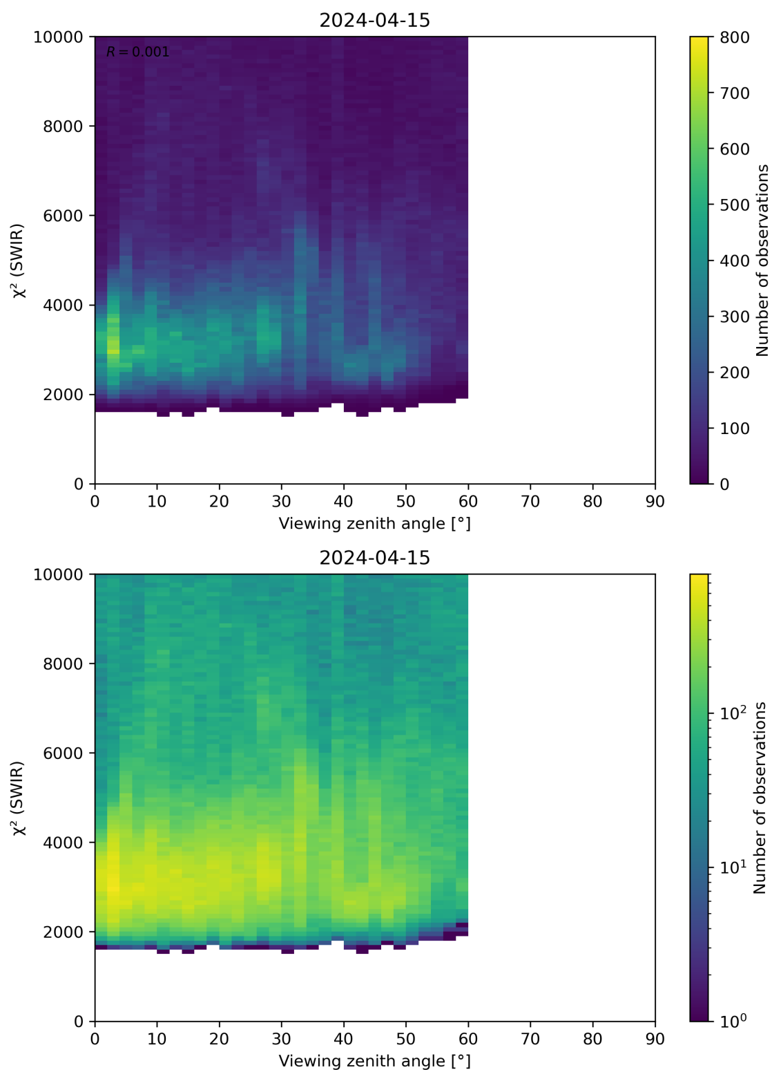
Figure 106: Scatter density plot of “Viewing zenith angle” against “ \chi^2 (SWIR)” for 2024-04-15 to 2024-04-16.
