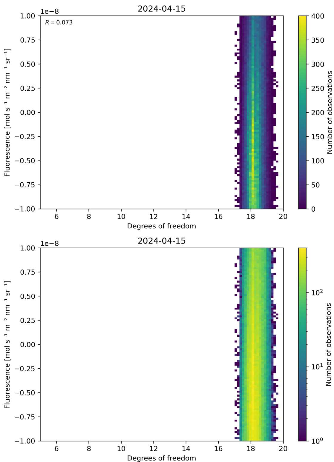
Figure 51: Scatter density plot of “Degrees of freedom” against “Fluorescence” for 2024-04-15 to 2024-04-16.
