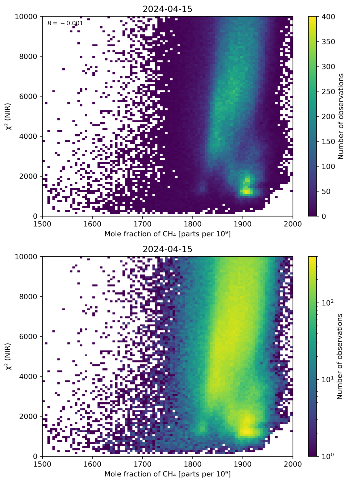
Figure 70: Scatter density plot of “Mole fraction of CH 4 ” against “ \chi^2 (NIR)” for 2024-04-15 to 2024-04-16.
