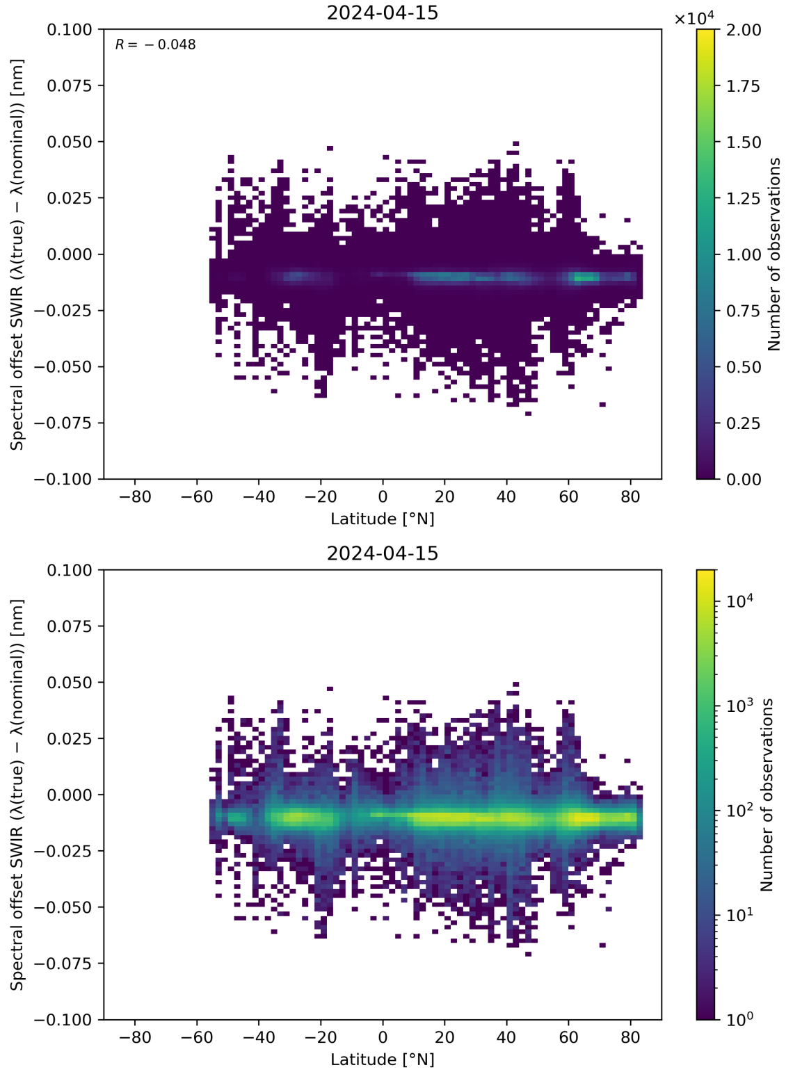
Figure 62: Scatter density plot of “Latitude” against “Spectral offset SWIR ( \lambda(\text{true}) - \lambda(\text{nominal}) )” for 2024-04-15 to 2024-04-16.
