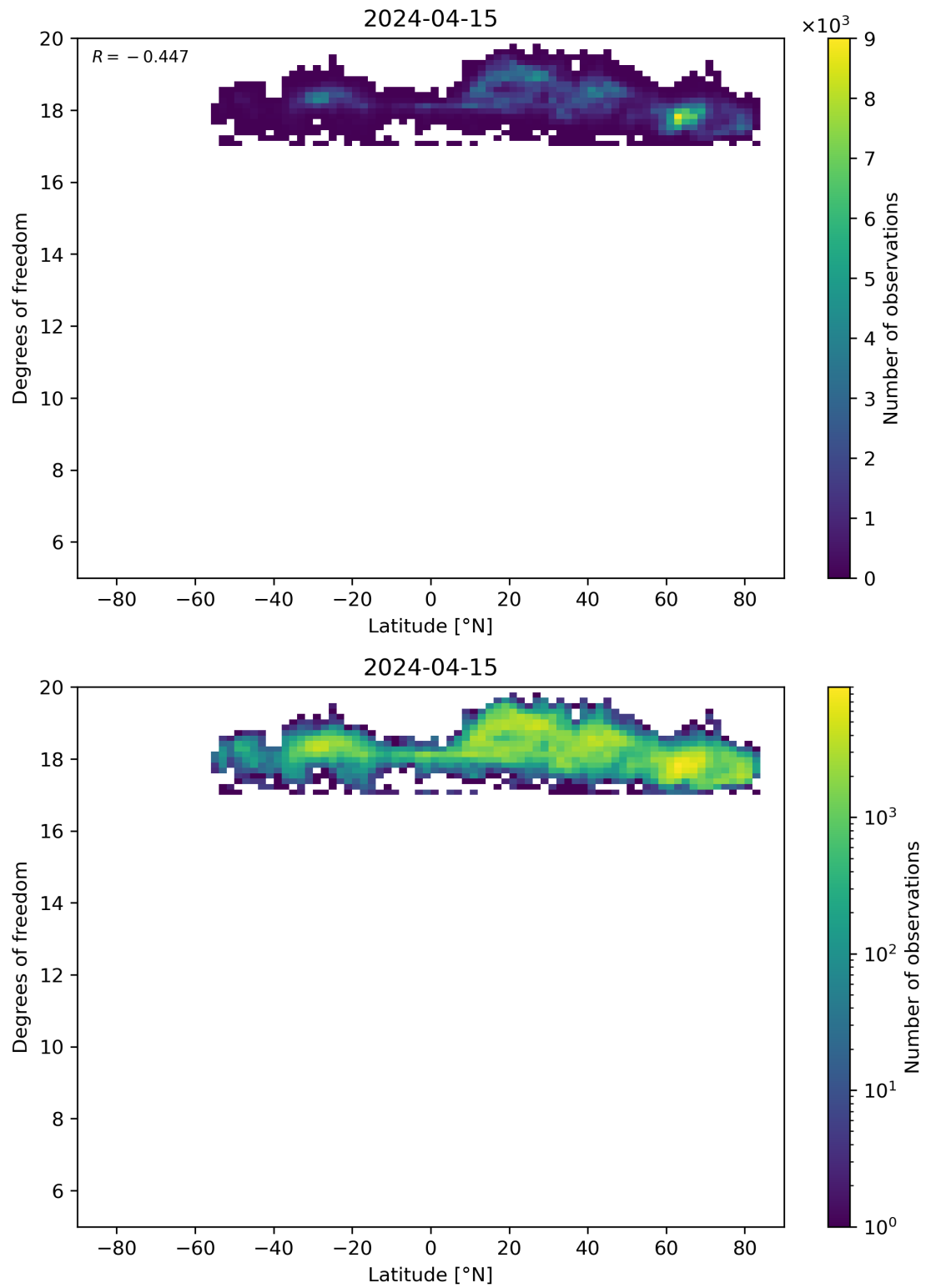
Figure 55: Scatter density plot of “Latitude” against “Degrees of freedom” for 2024-04-15 to 2024-04-16.
