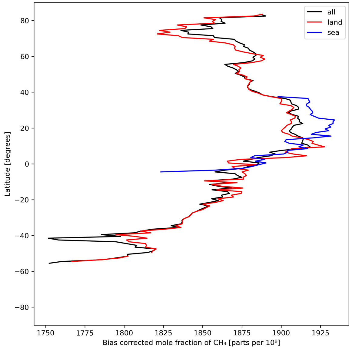
Figure 14: Zonal average of “Bias corrected mole fraction of \text{CH}_4 ” for 2024-04-15 to 2024-04-16.
