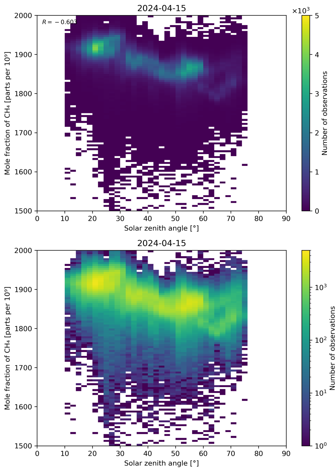
Figure 99: Scatter density plot of “Solar zenith angle” against “Mole fraction of CH 4 ” for 2024-04-15 to 2024-04-16.
