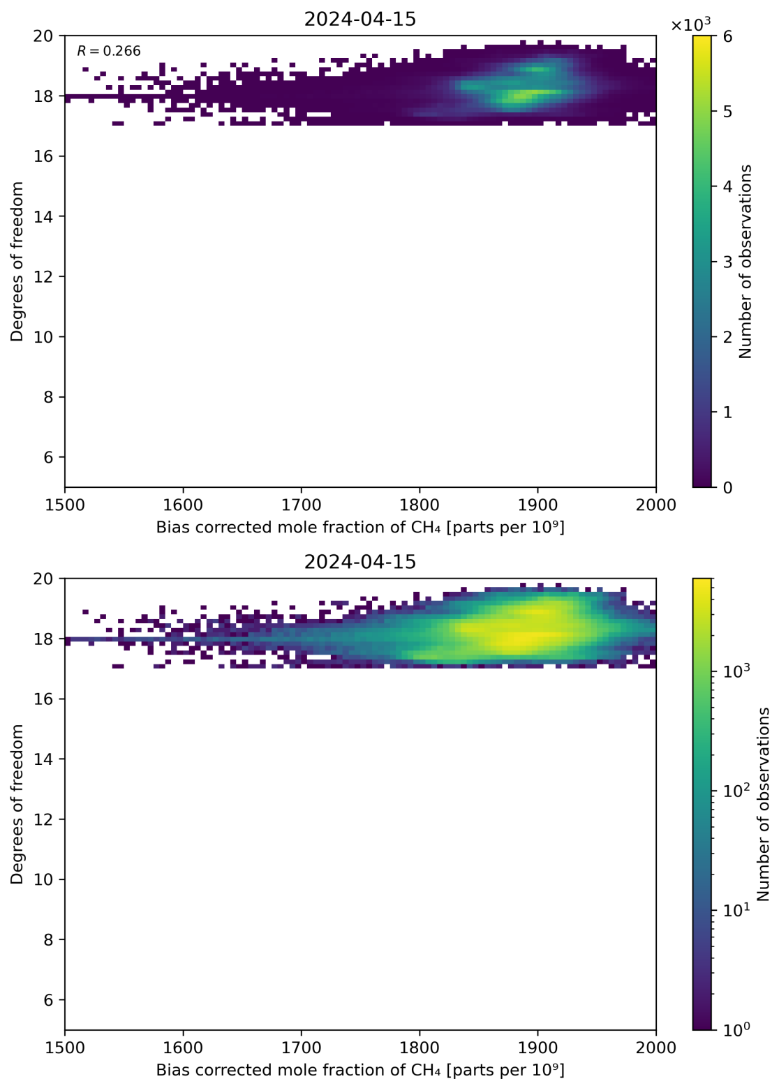
Figure 65: Scatter density plot of “Bias corrected mole fraction of CH 4 ” against “Degrees of freedom” for 2024-04-15 to 2024-04-16.
