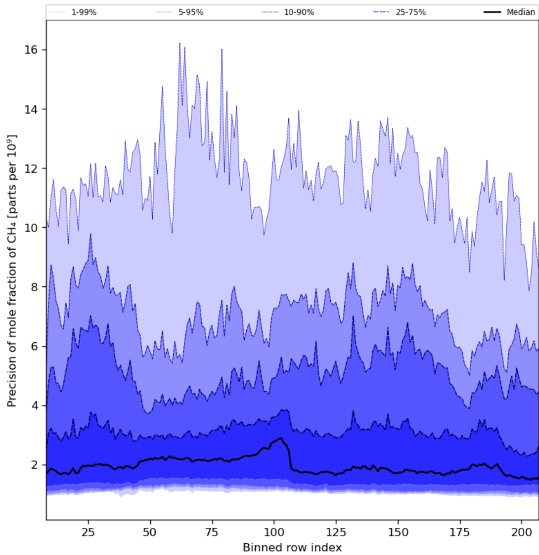
Figure 35: Along track statistics of “Precision of mole fraction of CH 4 ” for 2024-04-15 to 2024-04-16
