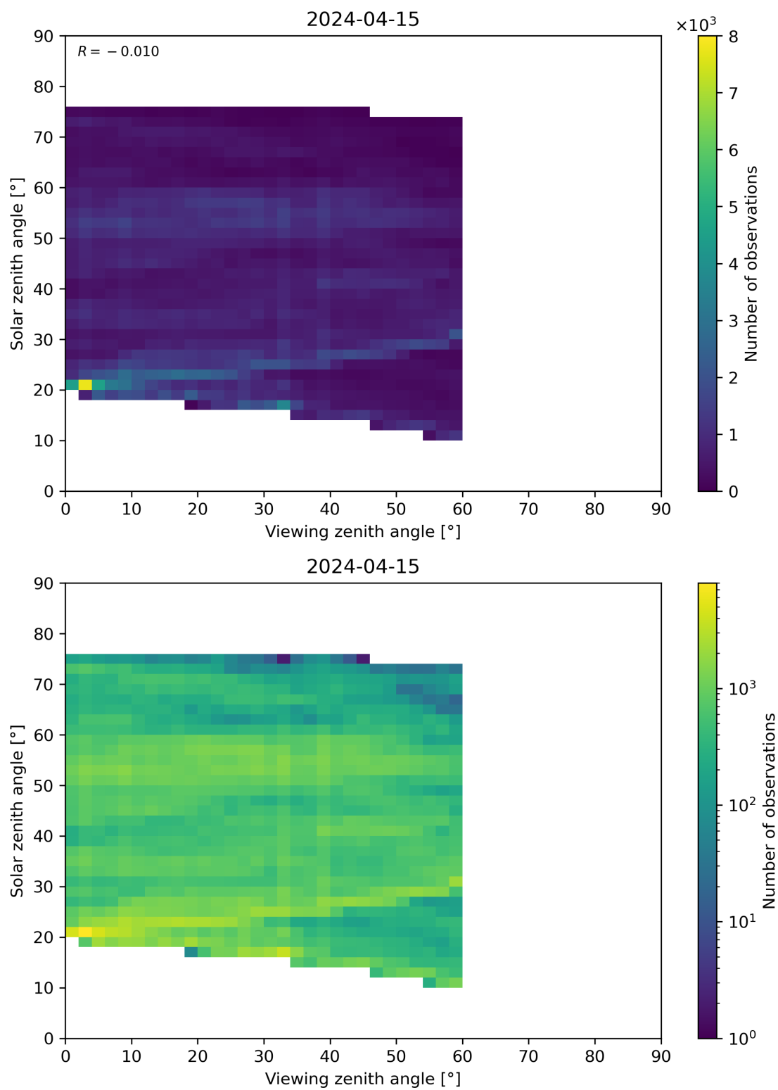
Figure 115: Scatter density plot of “Viewing zenith angle” against “Solar zenith angle” for 2024-04-15 to 2024-04-16.
