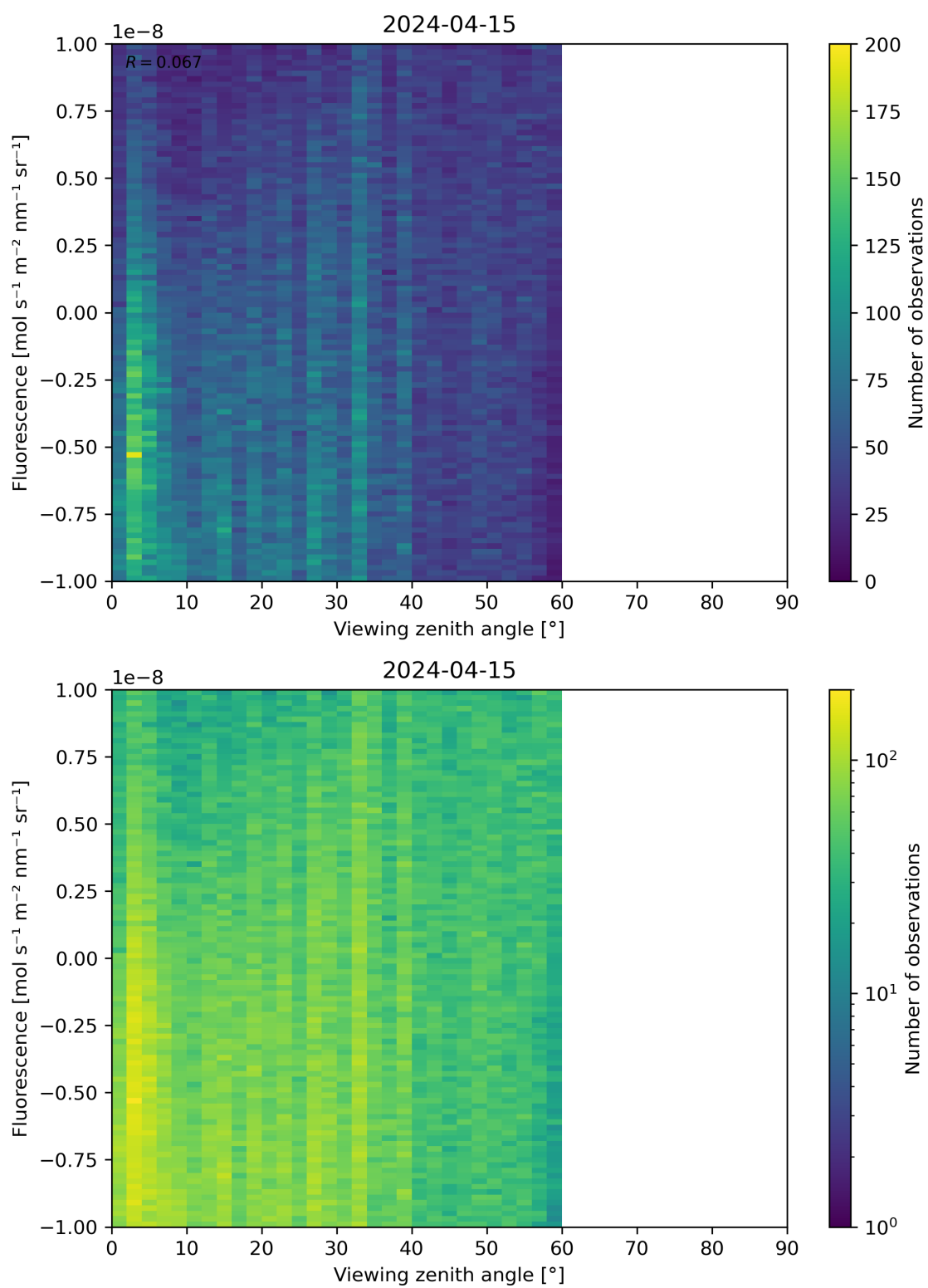
Figure 108: Scatter density plot of “Viewing zenith angle” against “Fluorescence” for 2024-04-15 to 2024-04-16.
