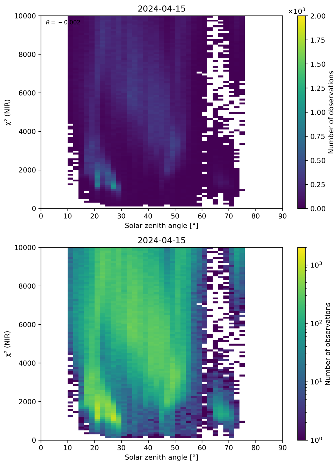
Figure 94: Scatter density plot of “Solar zenith angle” against “ \chi^2 (NIR)” for 2024-04-15 to 2024-04-16.
