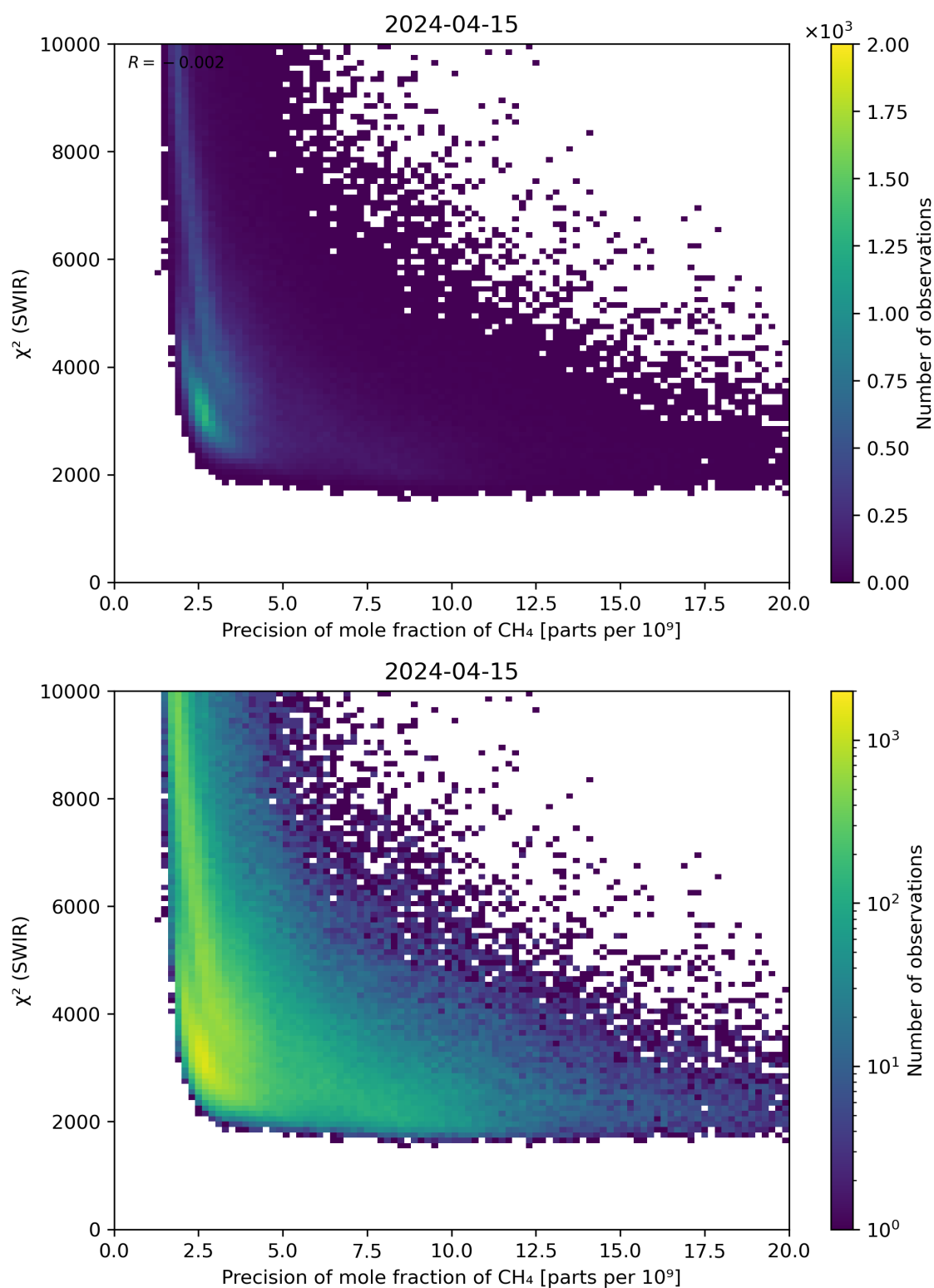
Figure 79: Scatter density plot of “Precision of mole fraction of \text{CH}_4 ” against “ \chi^2 (SWIR)” for 2024-04-15 to 2024-04-16.
