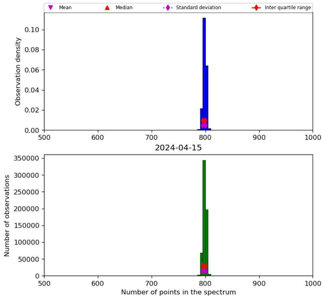
Figure 26: Histogram of “Number of points in the spectrum” for 2024-04-15 to 2024-04-16
