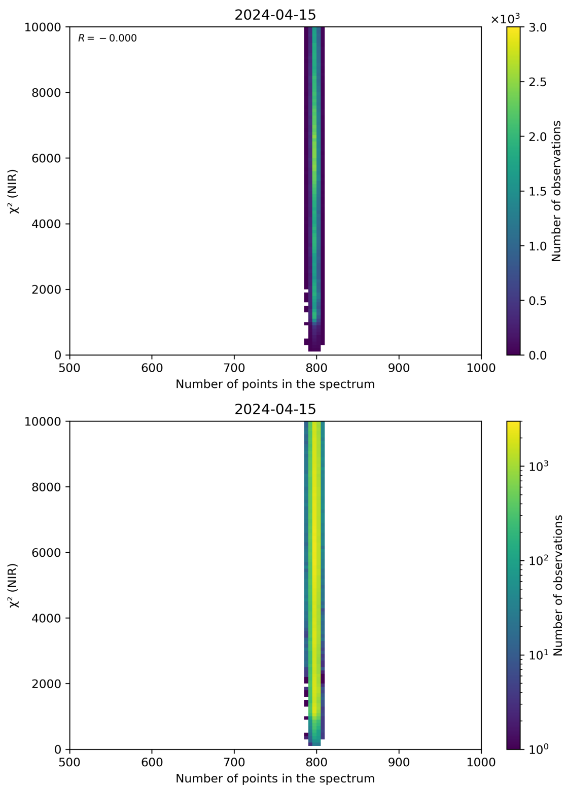
Figure 88: Scatter density plot of “Number of points in the spectrum” against “ \chi^2 (NIR)” for 2024-04-15 to 2024-04-16.
