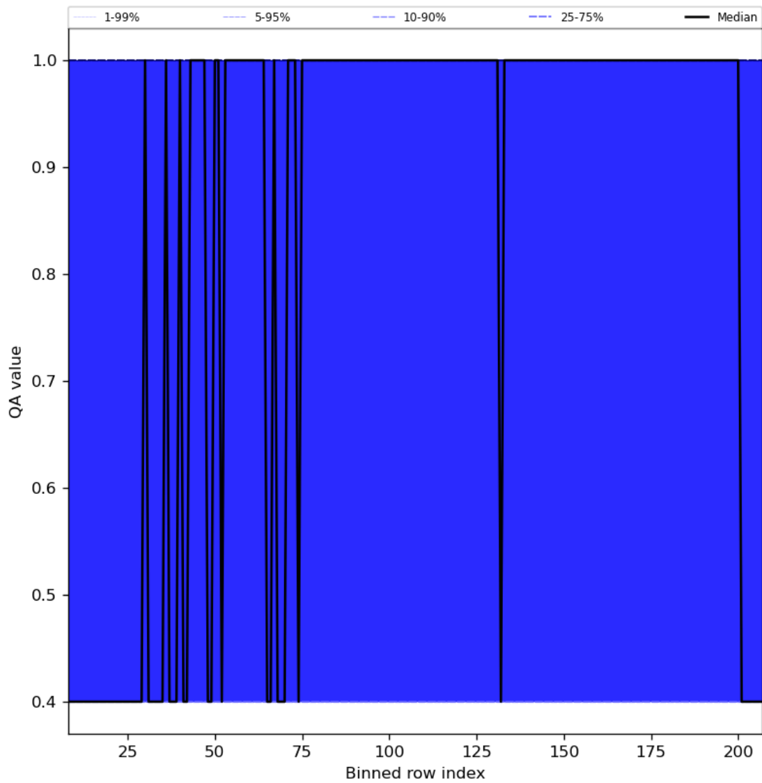
Figure 33: Along track statistics of “QA value” for 2024-04-15 to 2024-04-16
