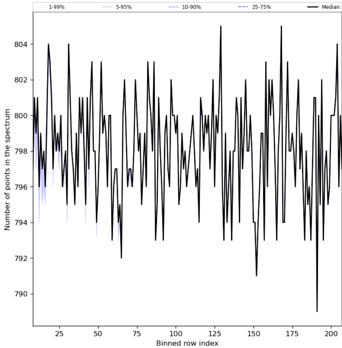
Figure 37: Along track statistics of “Number of points in the spectrum” for 2024-04-15 to 2024-04-16
