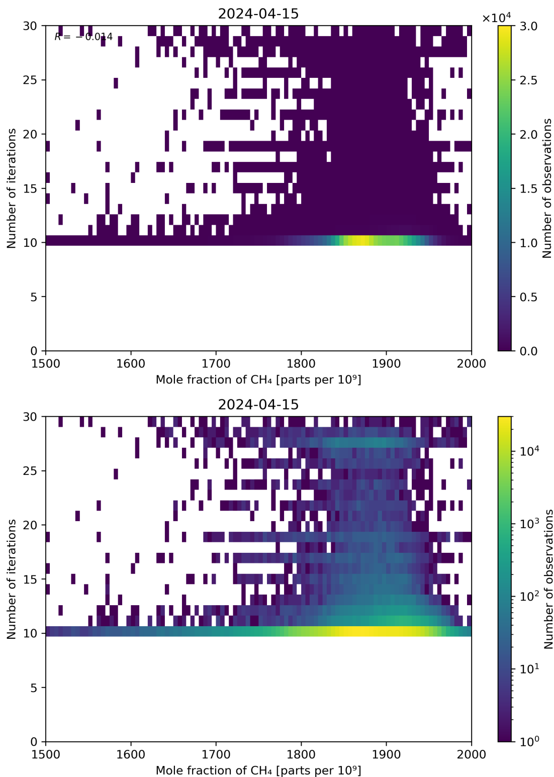
Figure 76: Scatter density plot of “Mole fraction of CH 4 ” against “Number of iterations” for 2024-04-15 to 2024-04-16.
