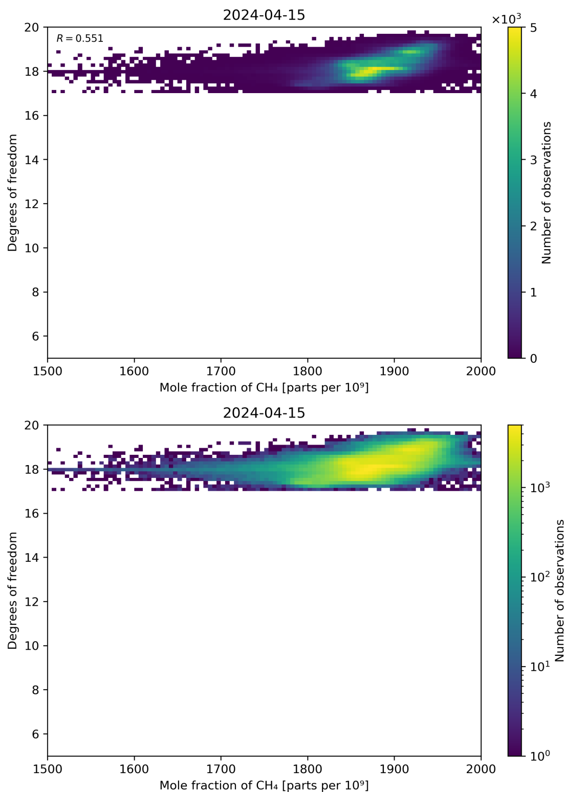
Figure 72: Scatter density plot of “Mole fraction of CH 4 ” against “Degrees of freedom” for 2024-04-15 to 2024-04-16.
