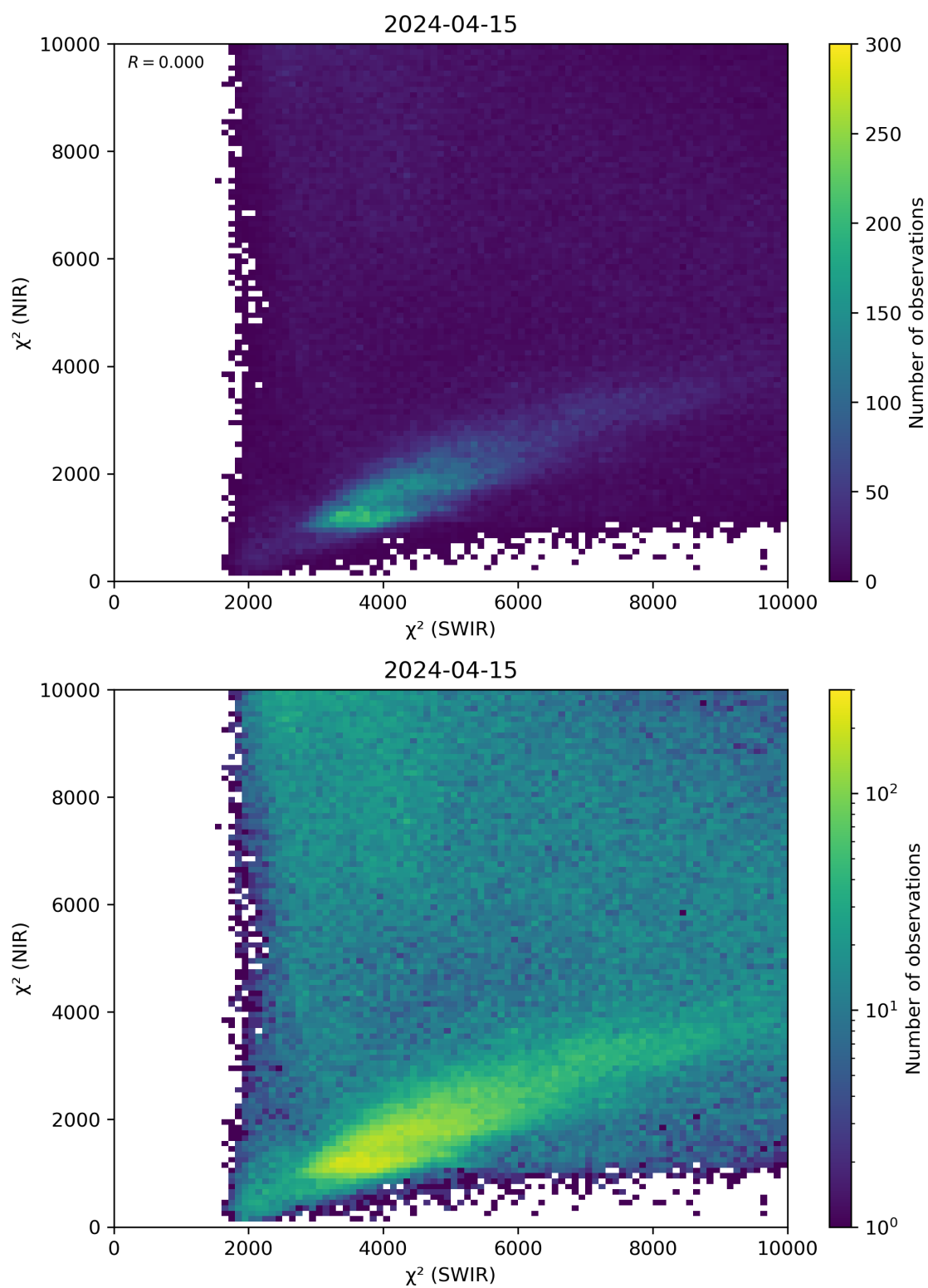
Figure 47: Scatter density plot of “ \chi^2 (SWIR)” against “ \chi^2 (NIR)” for 2024-04-15 to 2024-04-16.
