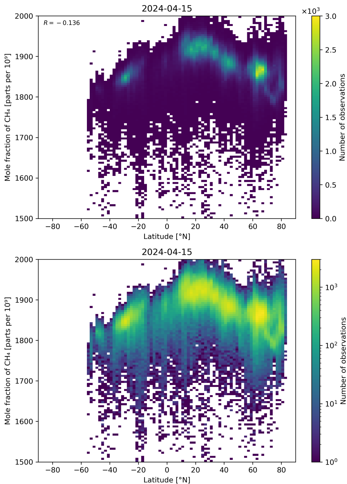
Figure 57: Scatter density plot of “Latitude” against “Mole fraction of \text{CH}_4 ” for 2024-04-15 to 2024-04-16.
