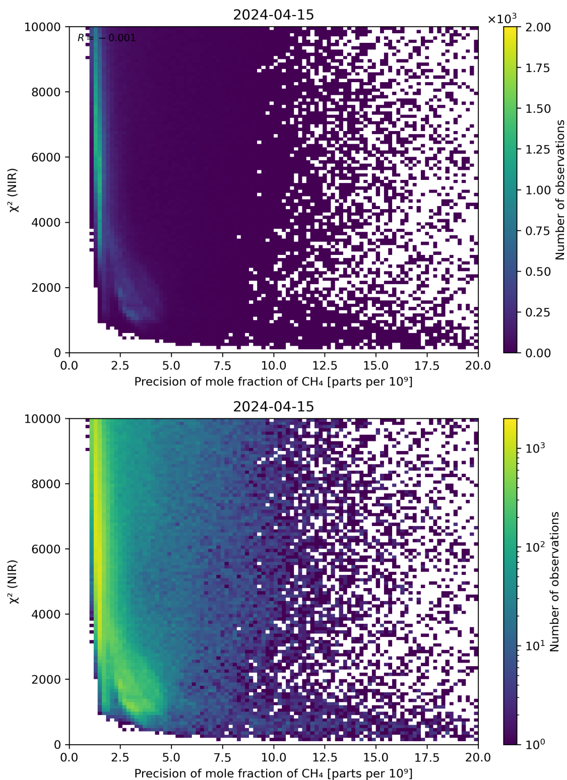
Figure 78: Scatter density plot of “Precision of mole fraction of CH 4 ” against “ \chi^2 (NIR)” for 2024-04-15 to 2024-04-16.
