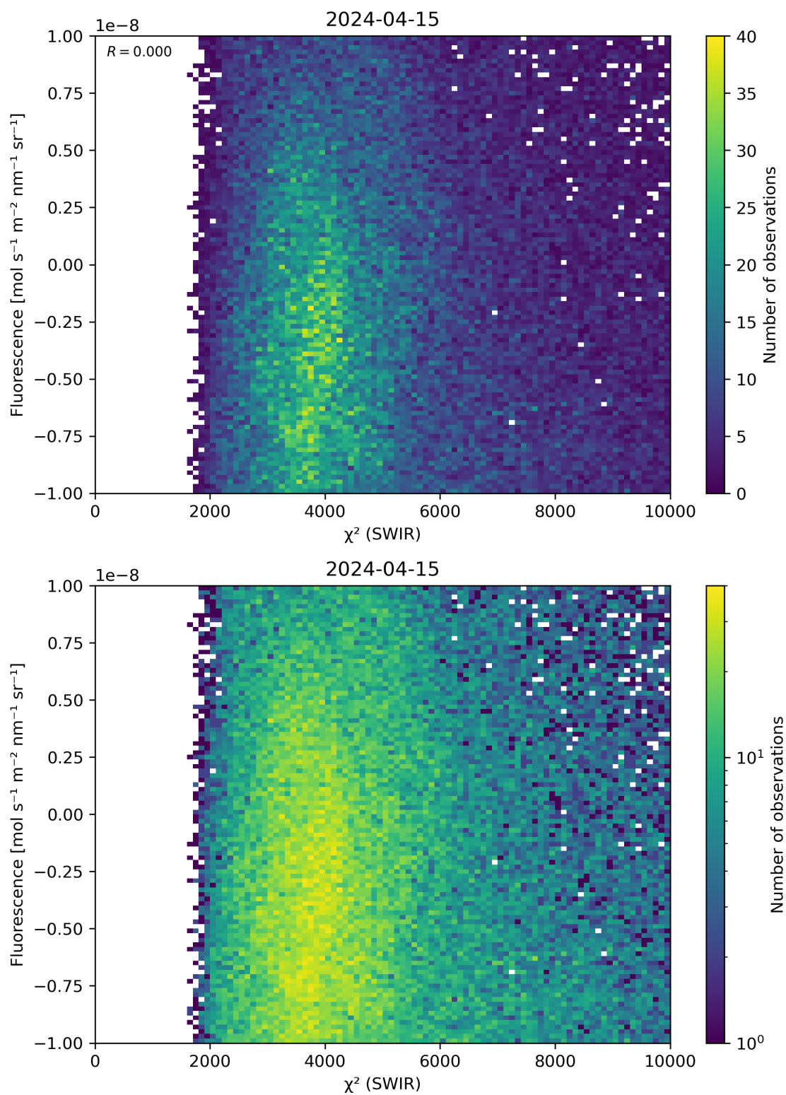
Figure 49: Scatter density plot of “ \chi^2 (SWIR)” against “Fluorescence” for 2024-04-15 to 2024-04-16.
