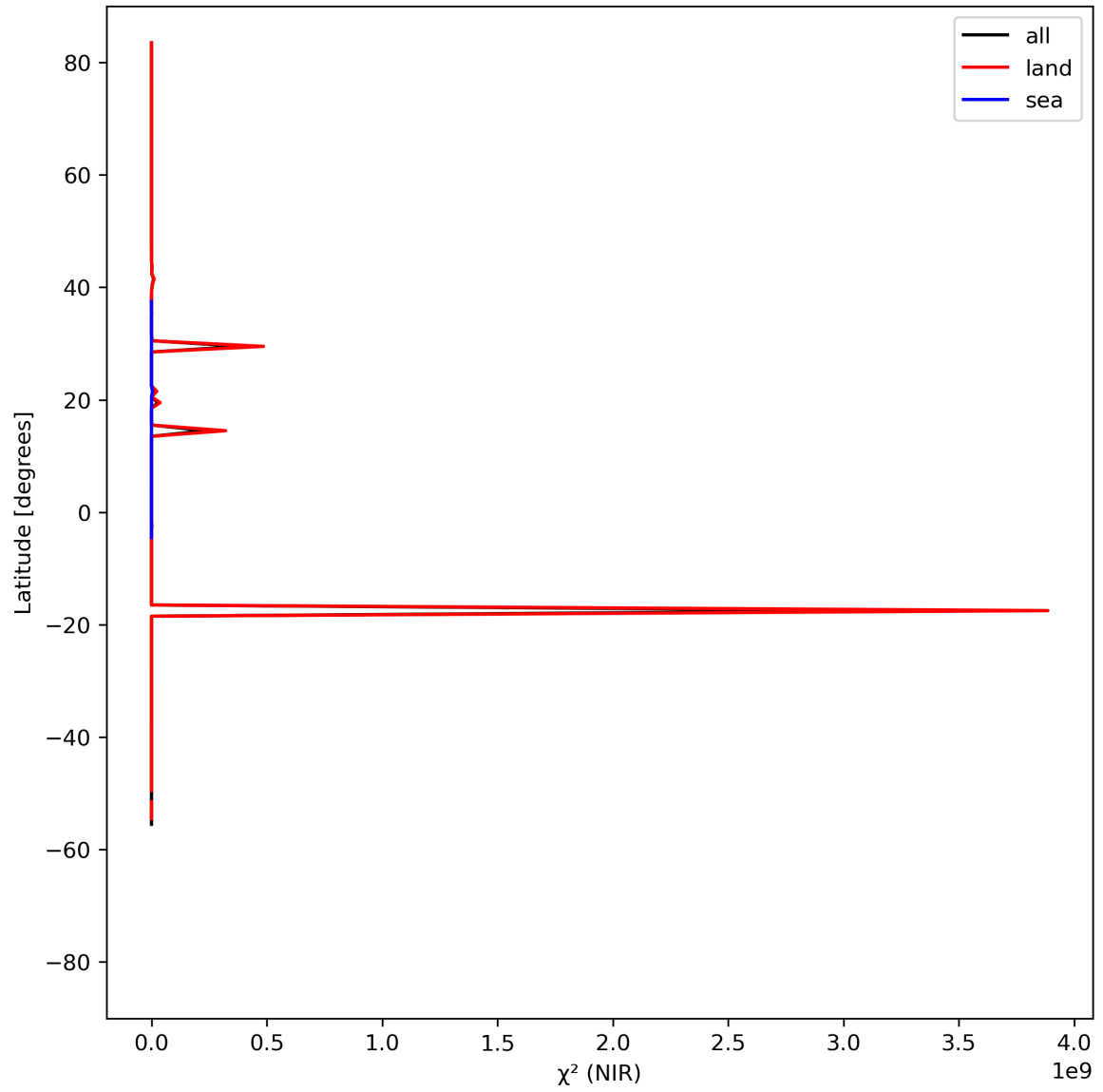
Figure 18: Zonal average of “ \chi^2 (NIR)” for 2024-04-15 to 2024-04-16.
