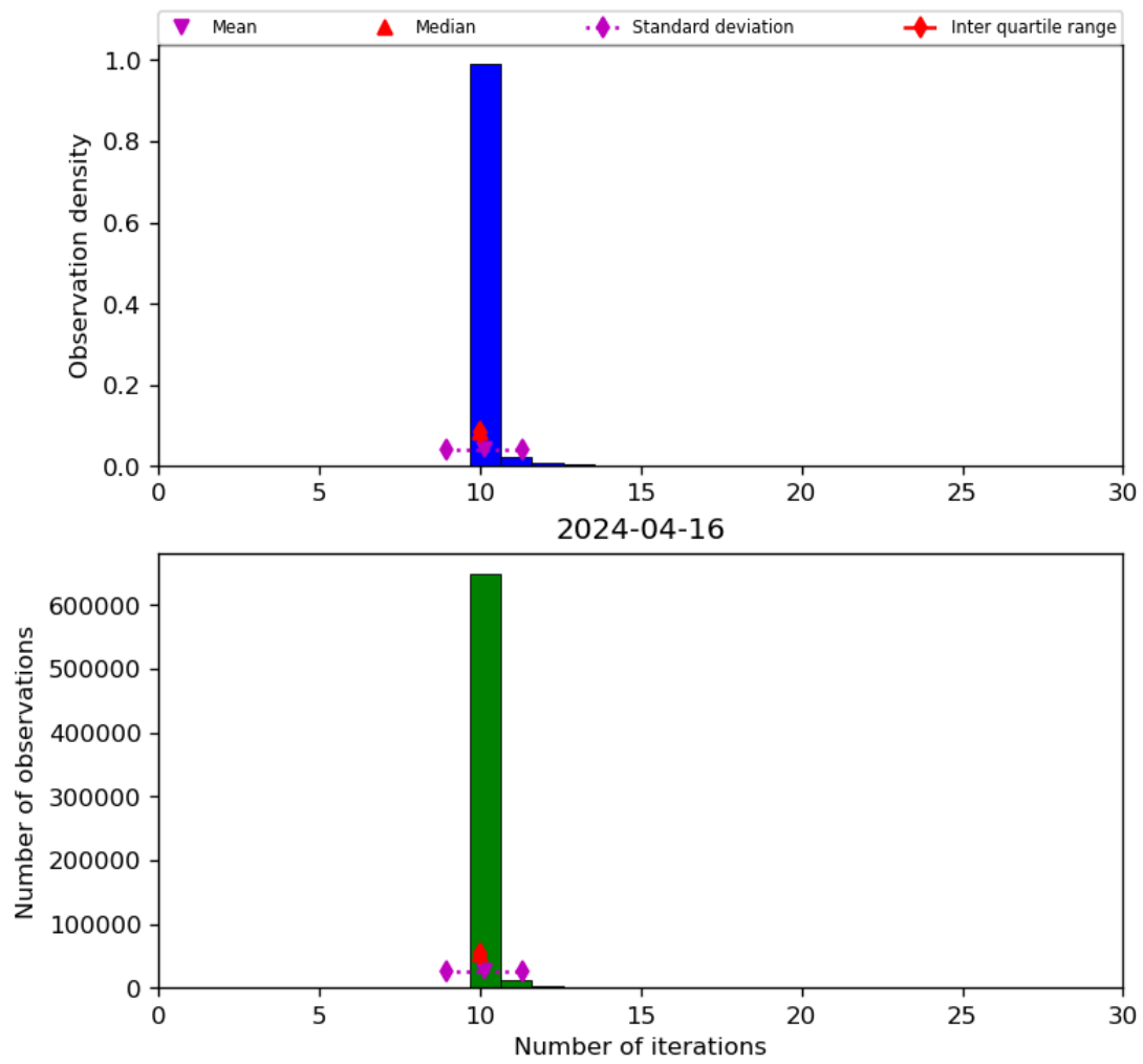
Figure 31: Histogram of “Number of iterations” for 2024-04-16 to 2024-04-17
