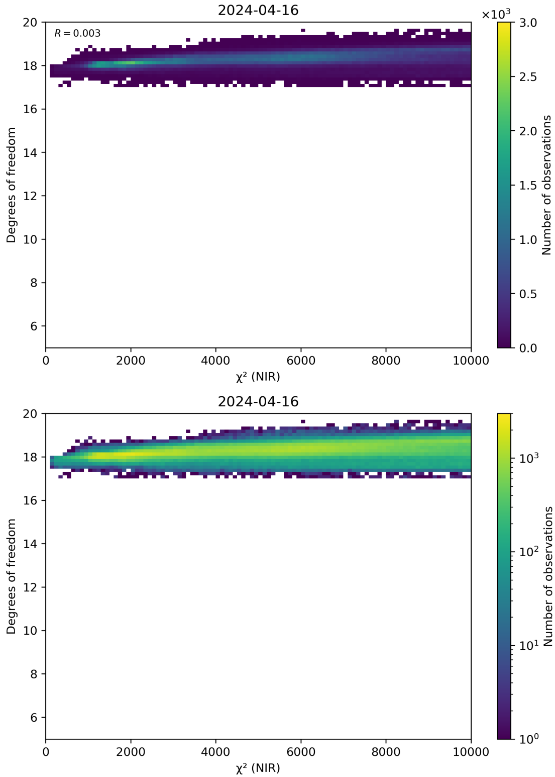
Figure 44: Scatter density plot of “ \chi^2 (NIR)” against “Degrees of freedom” for 2024-04-16 to 2024-04-17.
