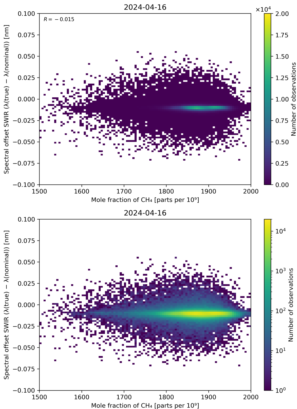
Figure 86: Scatter density plot of “Mole fraction of CH 4 ” against “Spectral offset SWIR ( \lambda(\text{true}) - \lambda(\text{nominal}) )” for 2024-04-16 to 2024-04-17.
