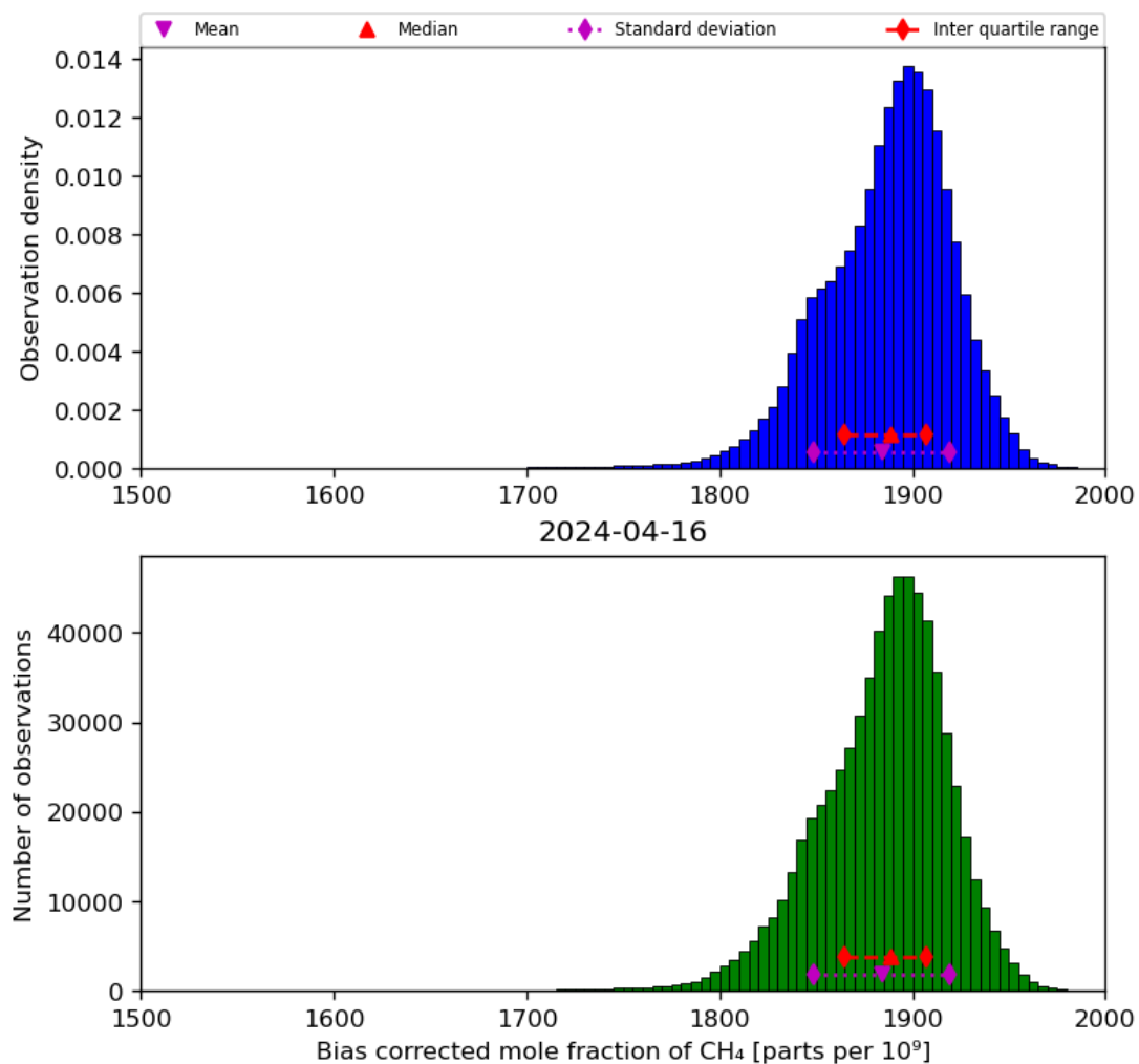
Figure 25: Histogram of “Bias corrected mole fraction of CH 4 ” for 2024-04-16 to 2024-04-17
