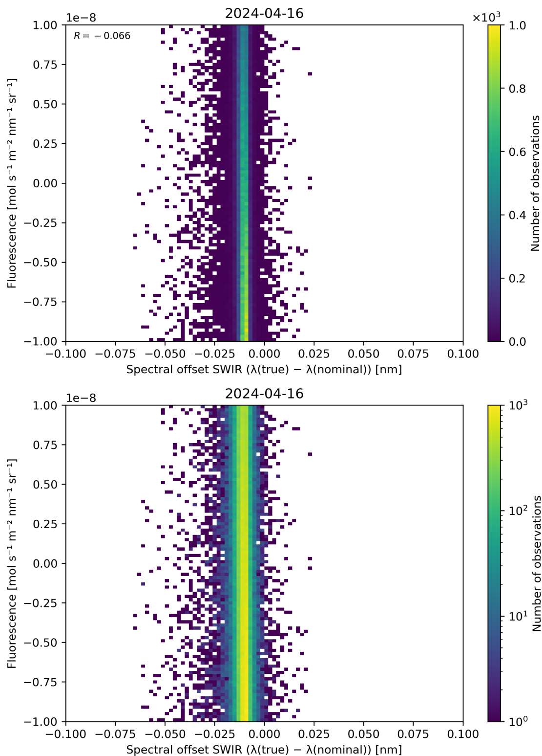
Figure 120: Scatter density plot of “Spectral offset SWIR ( \lambda(\text{true}) - \lambda(\text{nominal}) )” against “Fluorescence” for 2024-04-16 to 2024-04-17.
