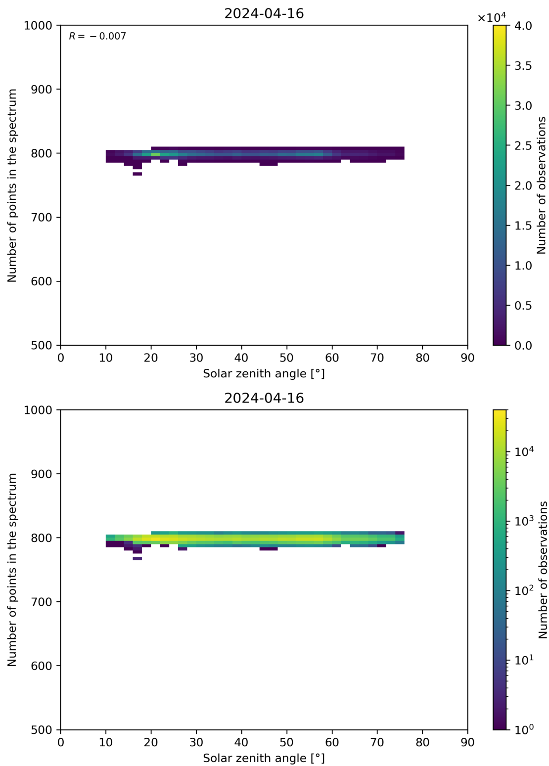
Figure 103: Scatter density plot of “Solar zenith angle” against “Number of points in the spectrum” for 2024-04-16 to 2024-04-17.
