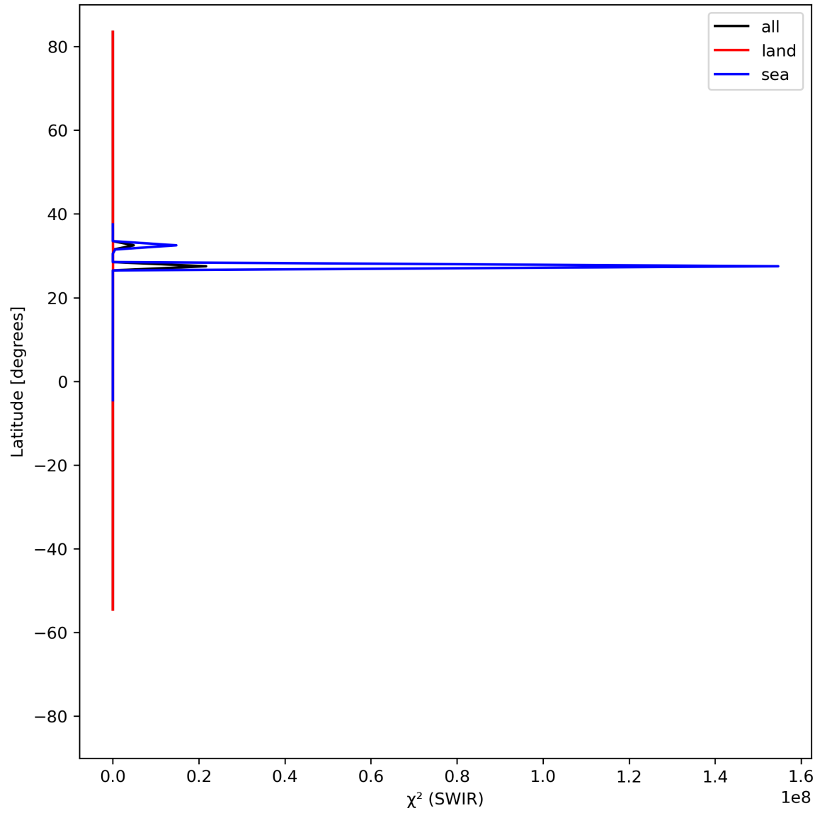
Figure 17: Zonal average of “ \chi^2 (SWIR)” for 2024-04-16 to 2024-04-17.
