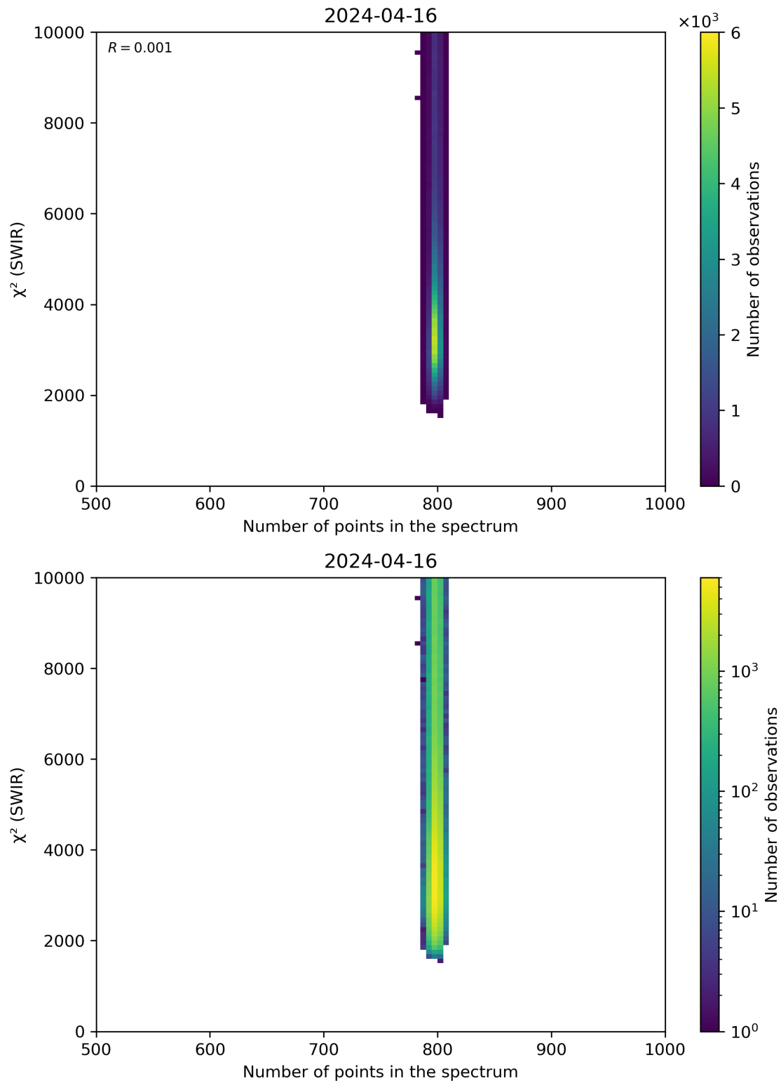
Figure 89: Scatter density plot of “Number of points in the spectrum” against “ \chi^2 (SWIR)” for 2024-04-16 to 2024-04-17.
