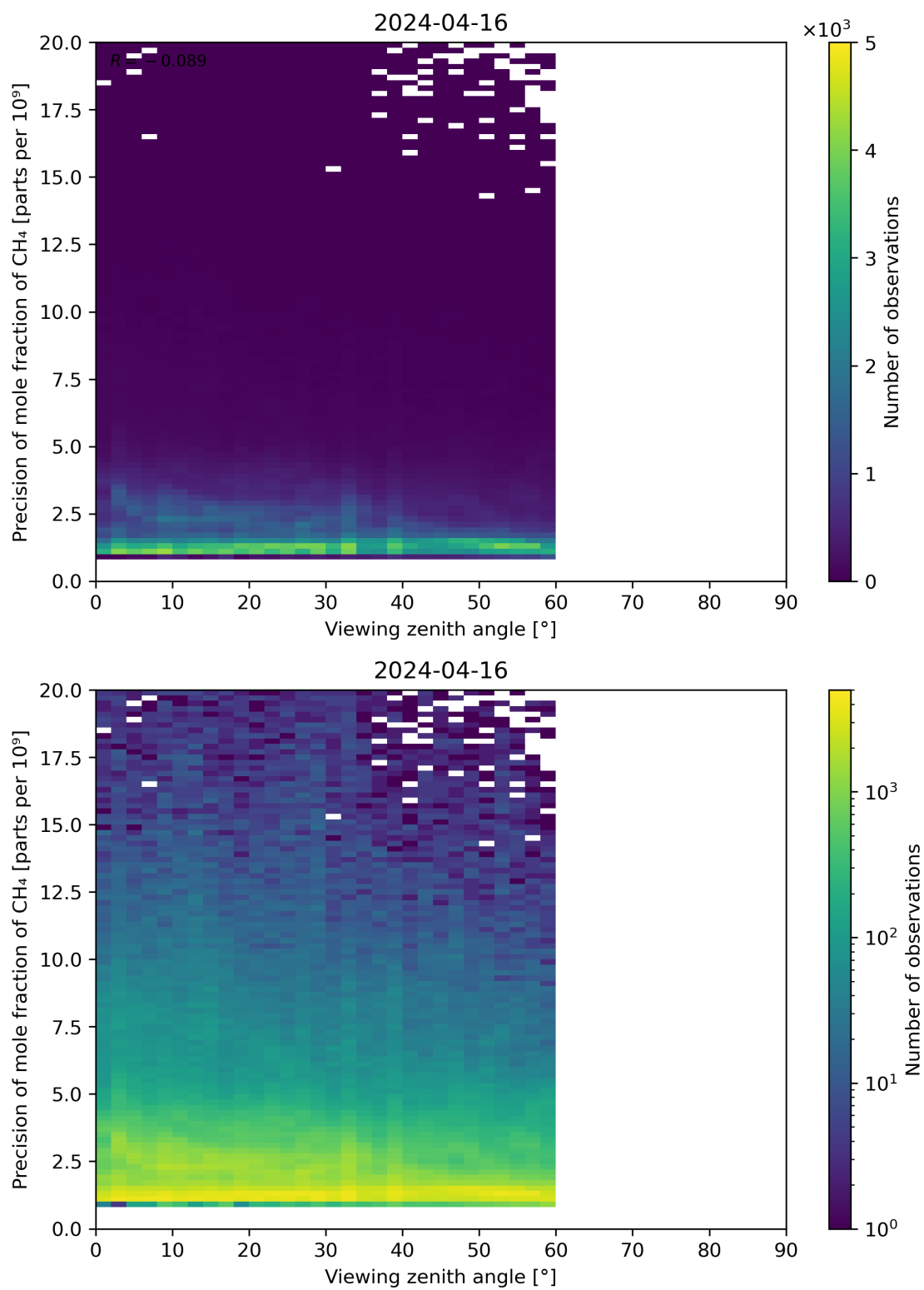
Figure 112: Scatter density plot of “Viewing zenith angle” against “Precision of mole fraction of CH 4 ” for 2024-04-16 to 2024-04-17.
