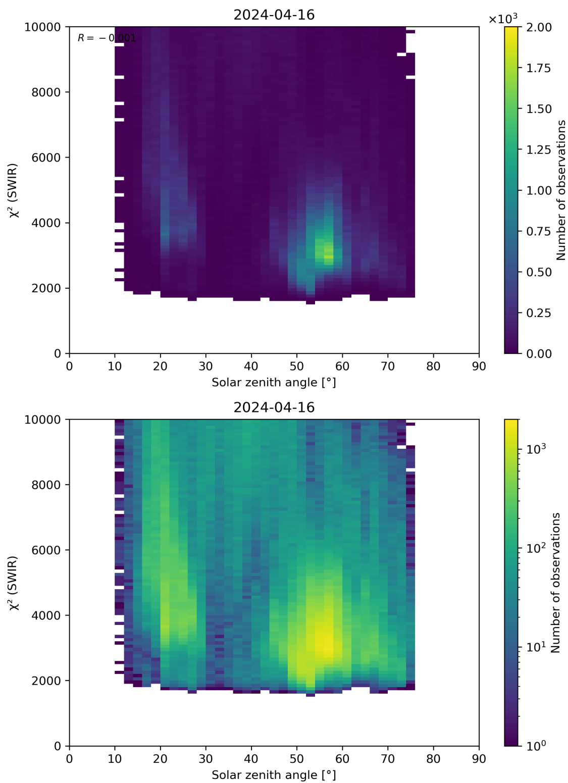
Figure 95: Scatter density plot of “Solar zenith angle” against “ \chi^2 (SWIR)” for 2024-04-16 to 2024-04-17.
