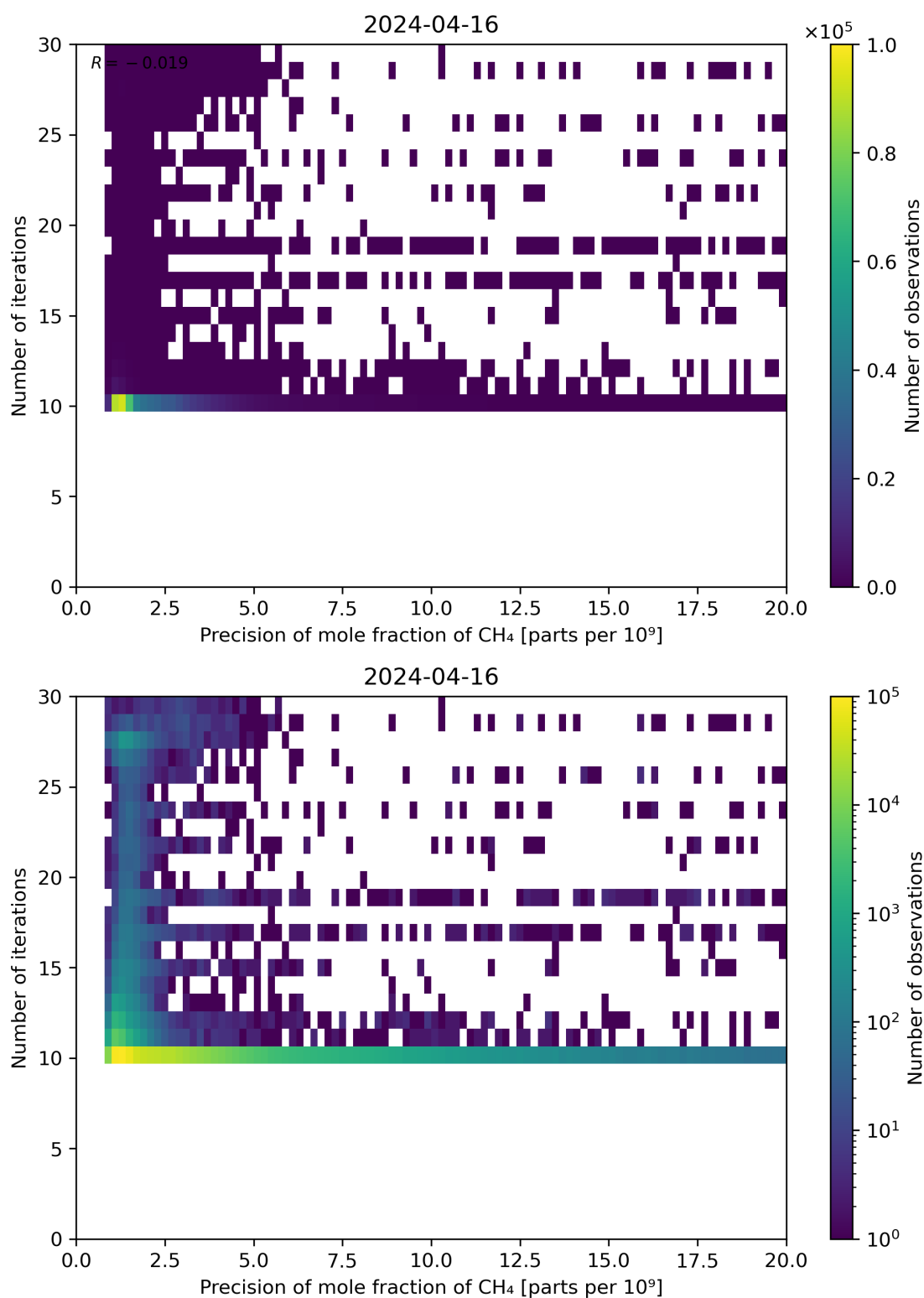
Figure 83: Scatter density plot of “Precision of mole fraction of CH 4 ” against “Number of iterations” for 2024-04-16 to 2024-04-17.
