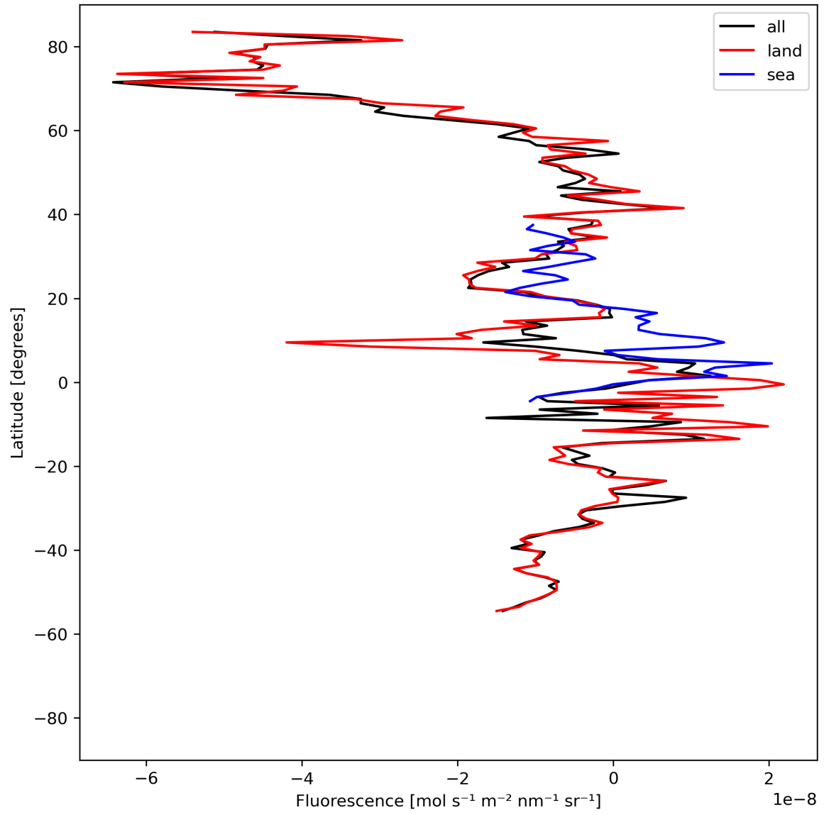
Figure 21: Zonal average of “Fluorescence” for 2024-04-16 to 2024-04-17.
