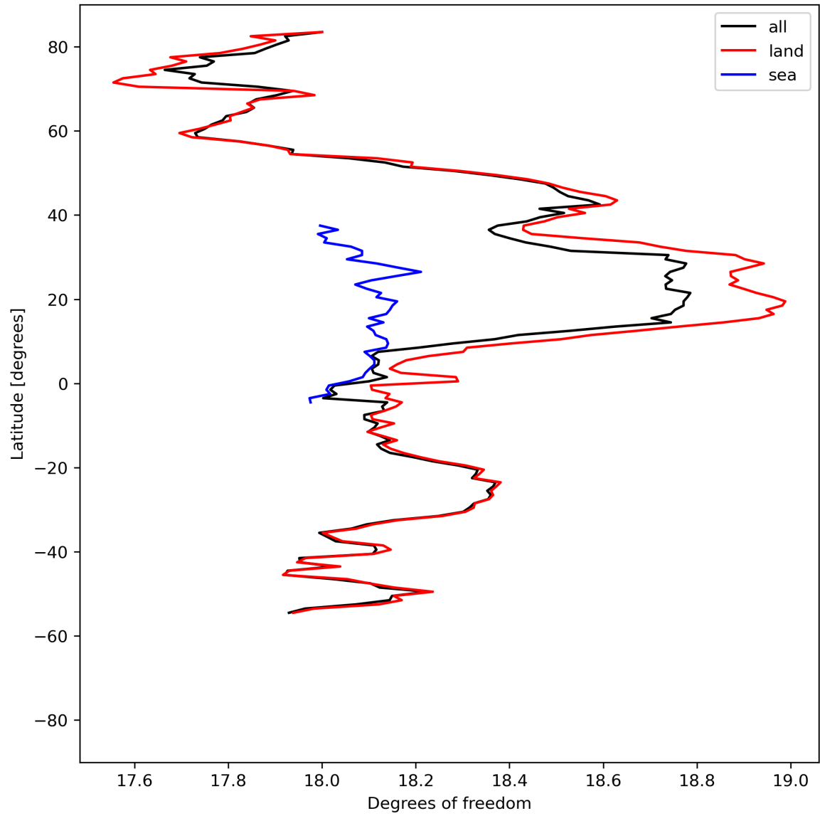
Figure 19: Zonal average of “Degrees of freedom” for 2024-04-16 to 2024-04-17.
