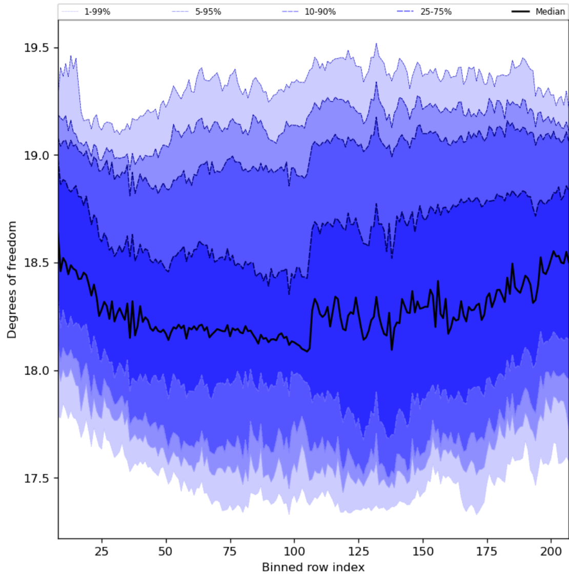
Figure 41: Along track statistics of “Degrees of freedom” for 2024-04-16 to 2024-04-17
