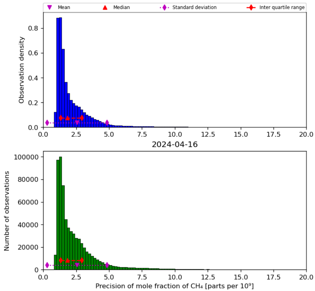
Figure 24: Histogram of “Precision of mole fraction of CH 4 ” for 2024-04-16 to 2024-04-17
