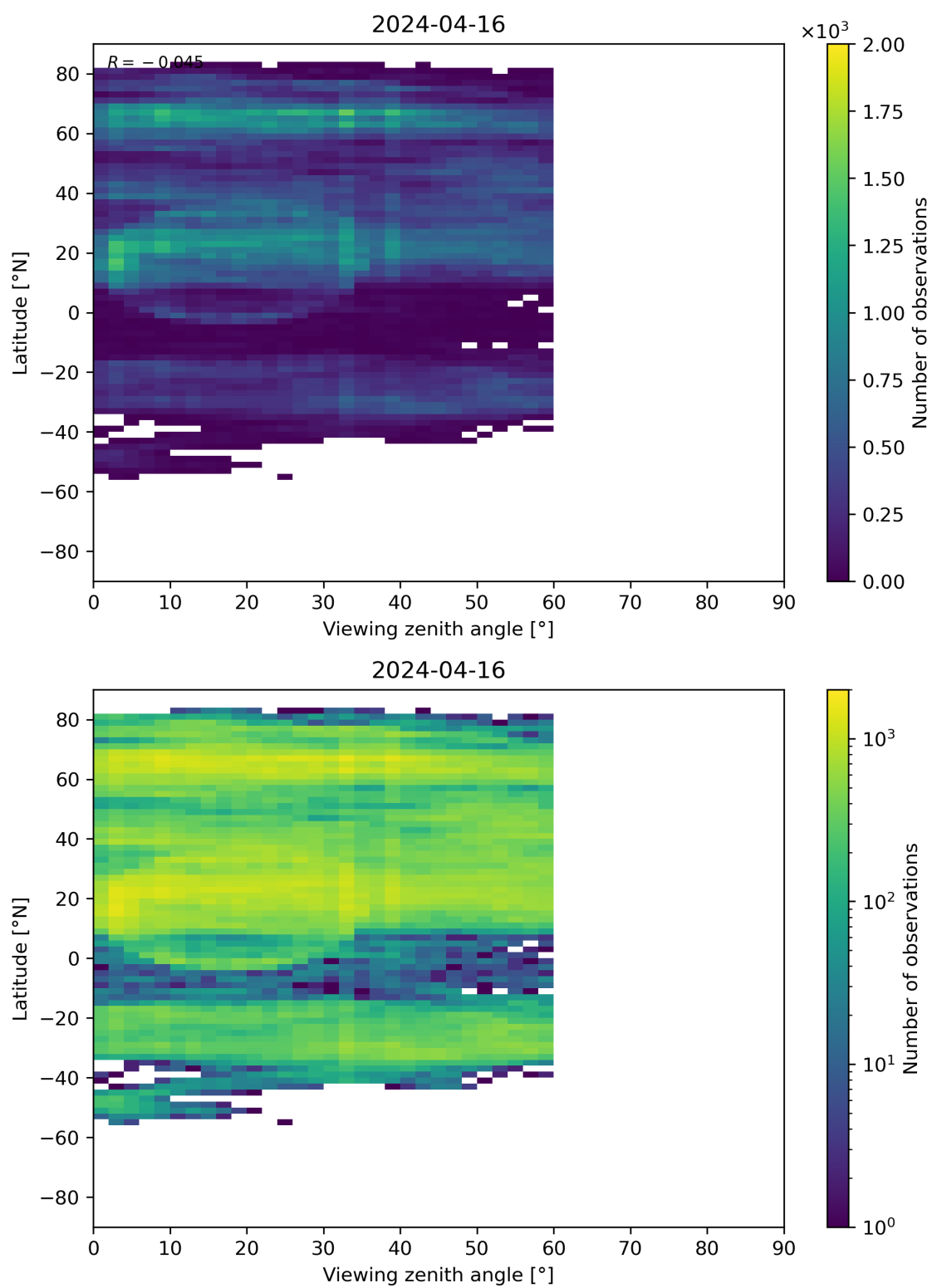
Figure 109: Scatter density plot of “Viewing zenith angle” against “Latitude” for 2024-04-16 to 2024-04-17.
