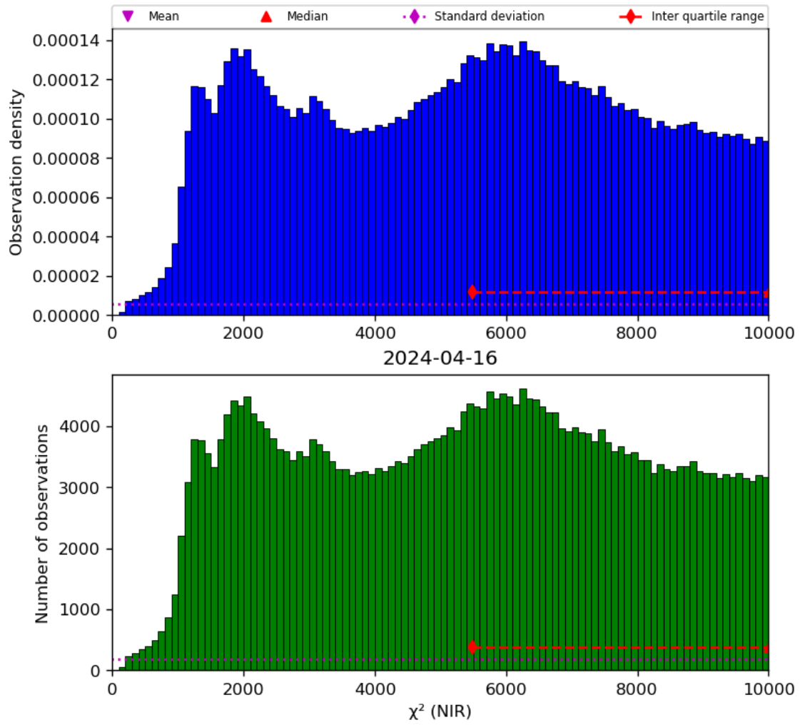
Figure 29: Histogram of " \chi^2 (NIR)" for 2024-04-16 to 2024-04-17
