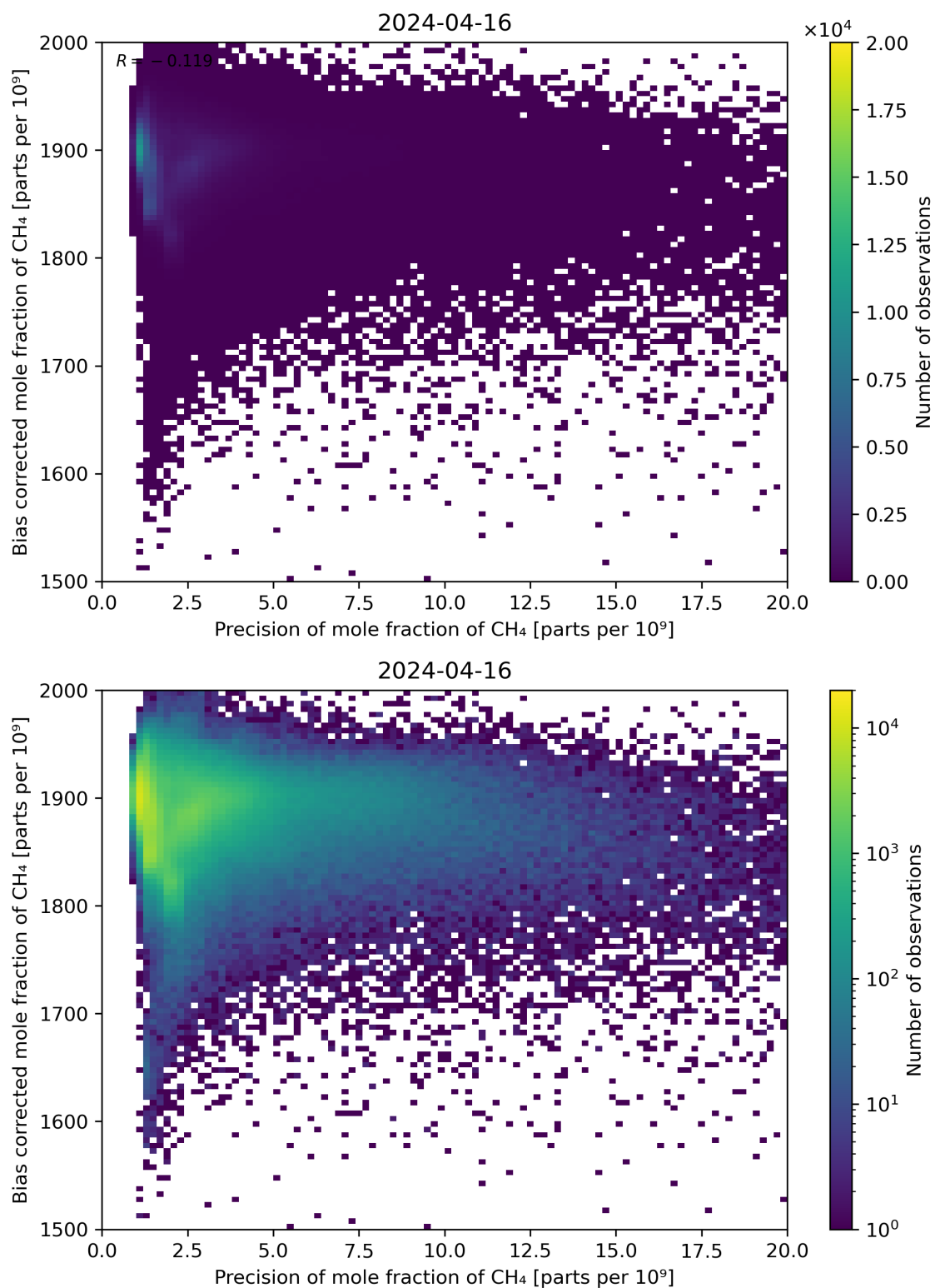
Figure 82: Scatter density plot of “Precision of mole fraction of CH 4 ” against “Bias corrected mole fraction of CH 4 ” for 2024-04-16 to 2024-04-17.
