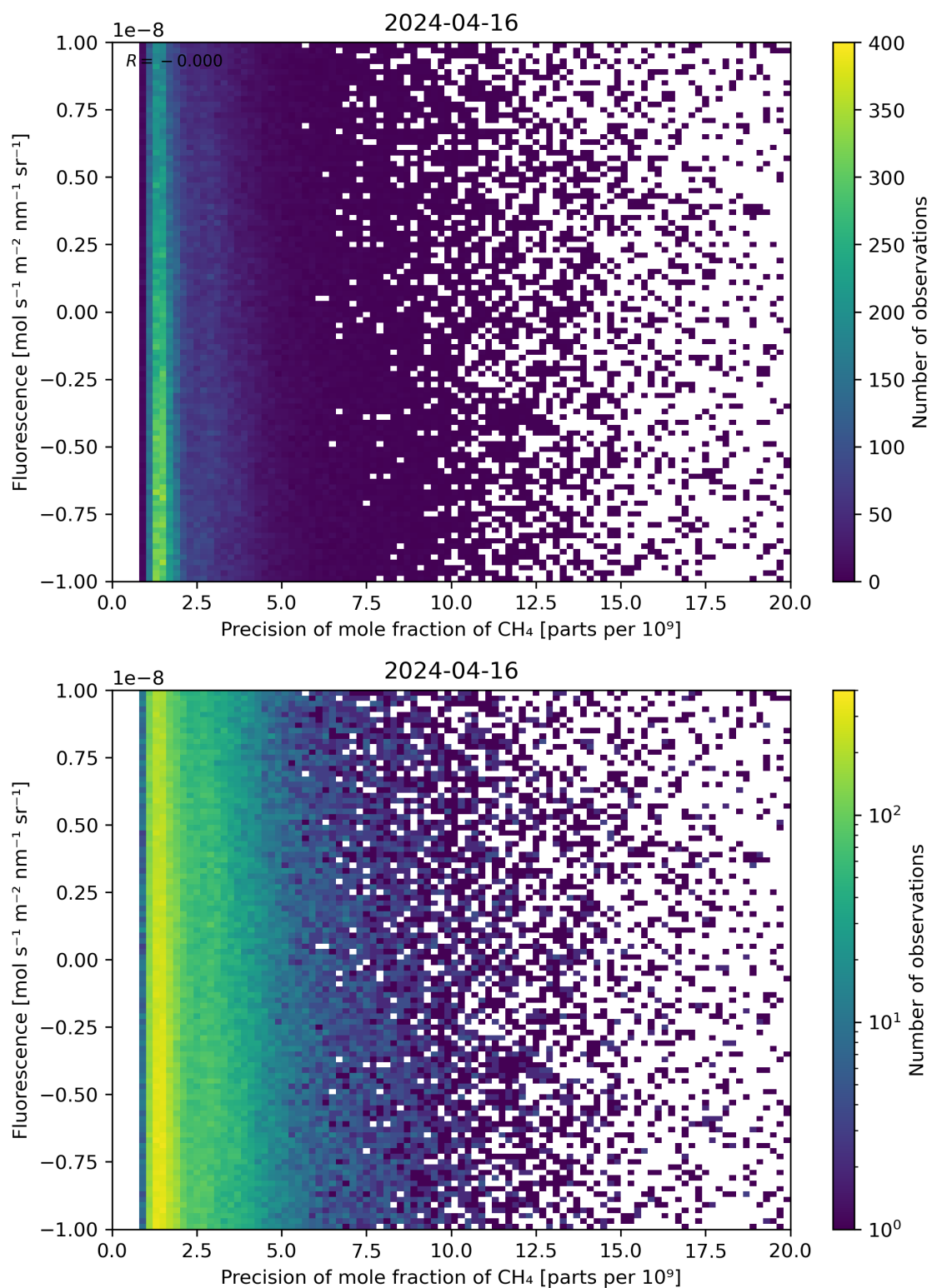
Figure 81: Scatter density plot of “Precision of mole fraction of CH 4 ” against “Fluorescence” for 2024-04-16 to 2024-04-17.
