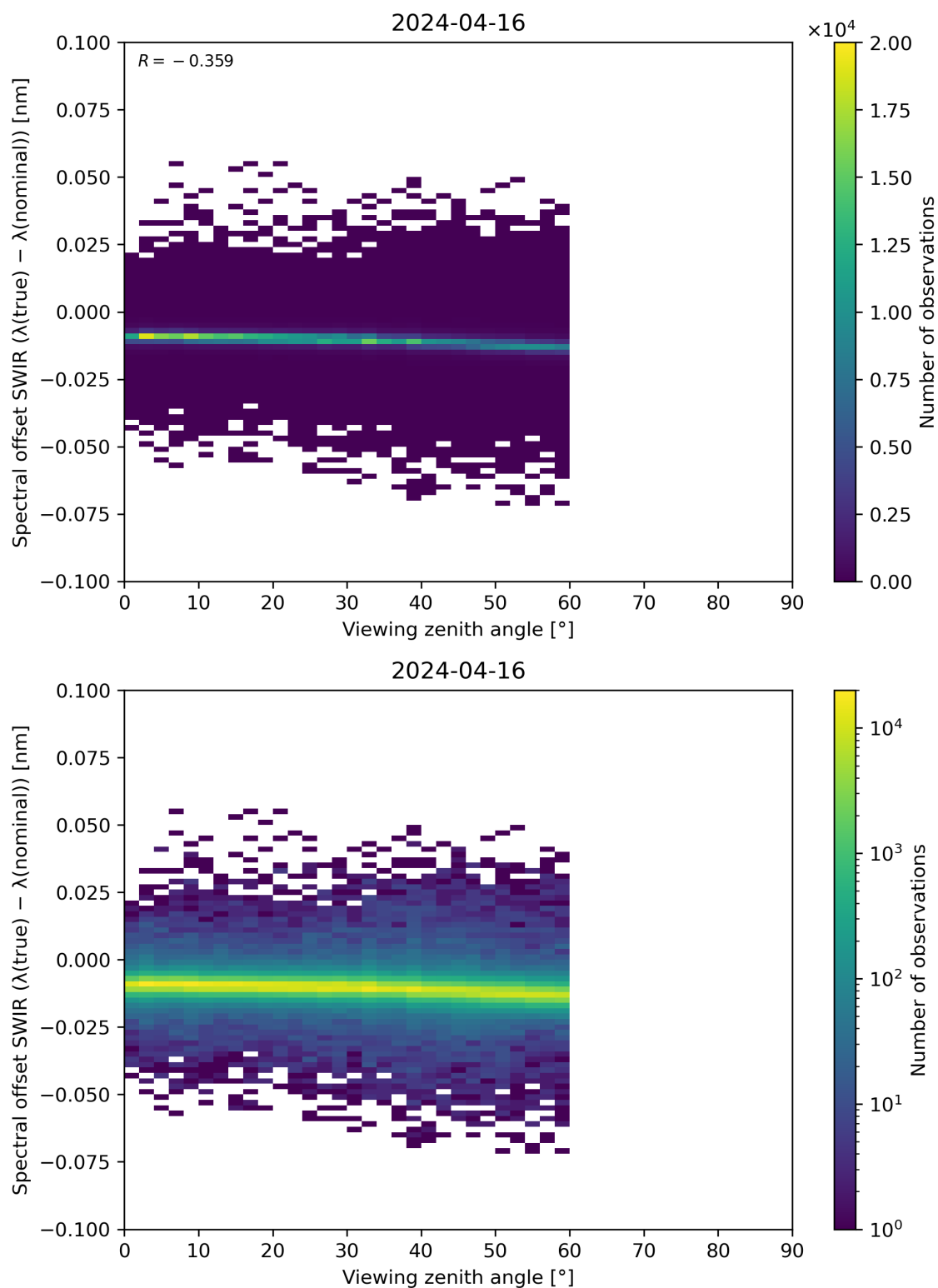
Figure 116: Scatter density plot of “Viewing zenith angle” against “Spectral offset SWIR ( \lambda(\text{true}) - \lambda(\text{nominal}) )” for 2024-04-16 to 2024-04-17.
