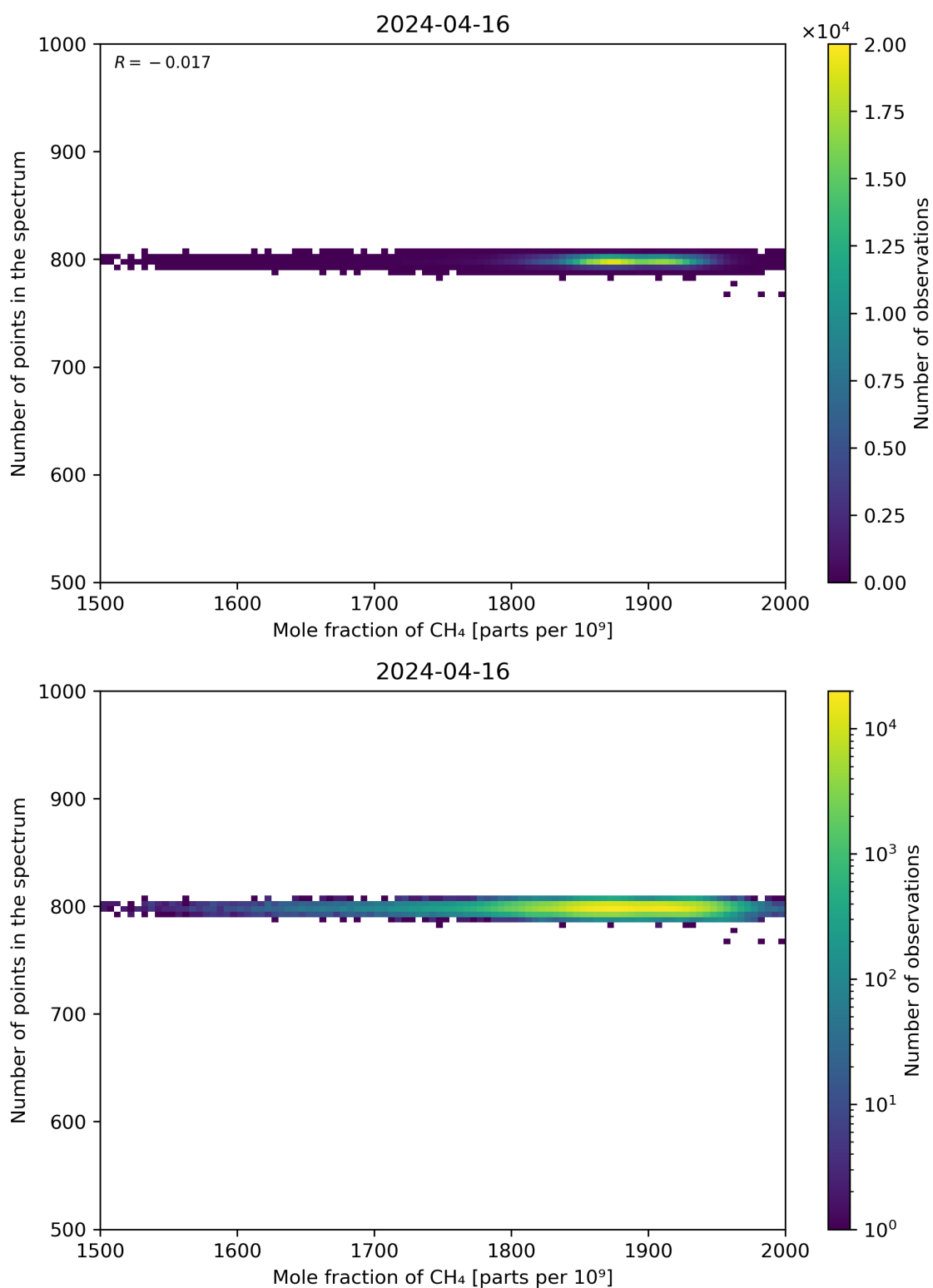
Figure 77: Scatter density plot of “Mole fraction of CH 4 ” against “Number of points in the spectrum” for 2024-04-16 to 2024-04-17.
