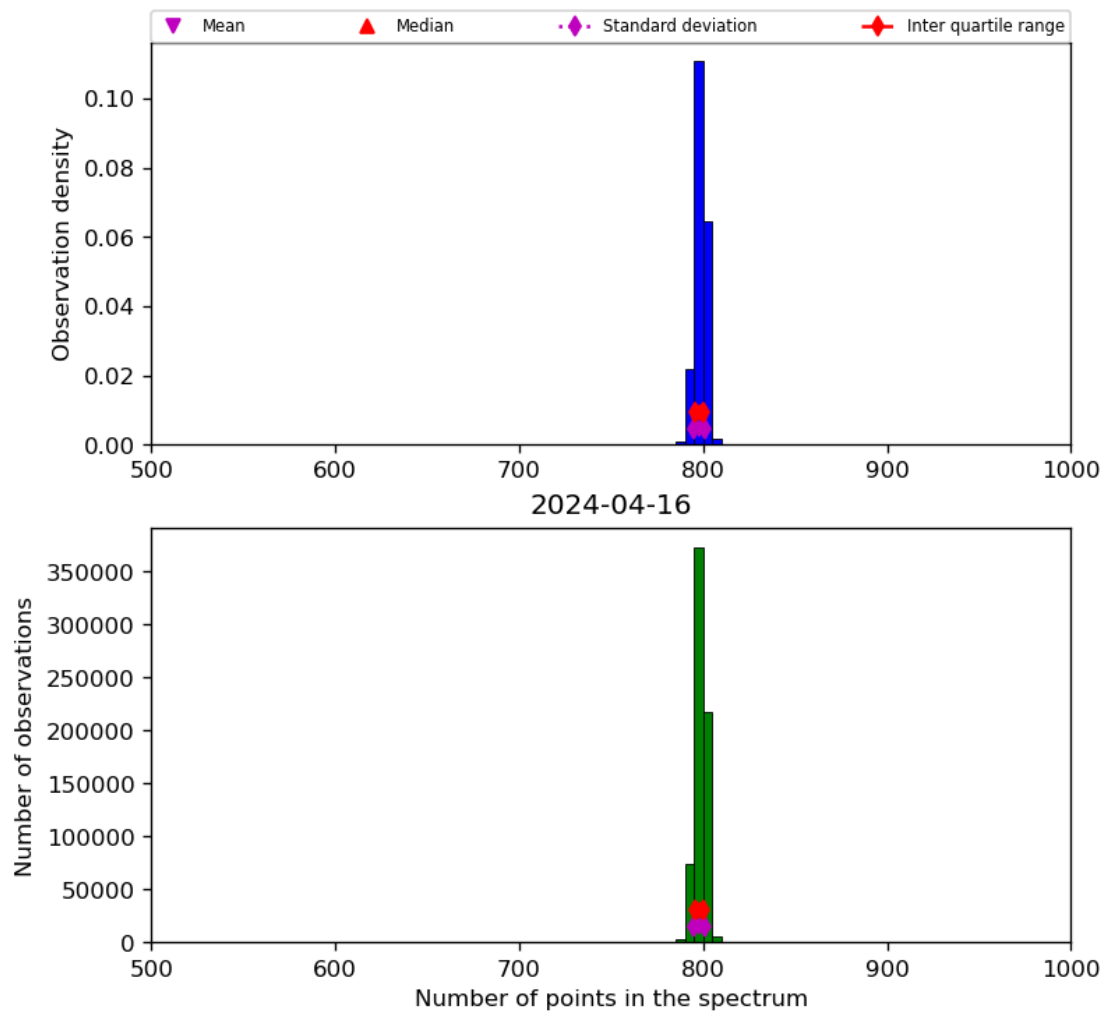
Figure 26: Histogram of “Number of points in the spectrum” for 2024-04-16 to 2024-04-17
