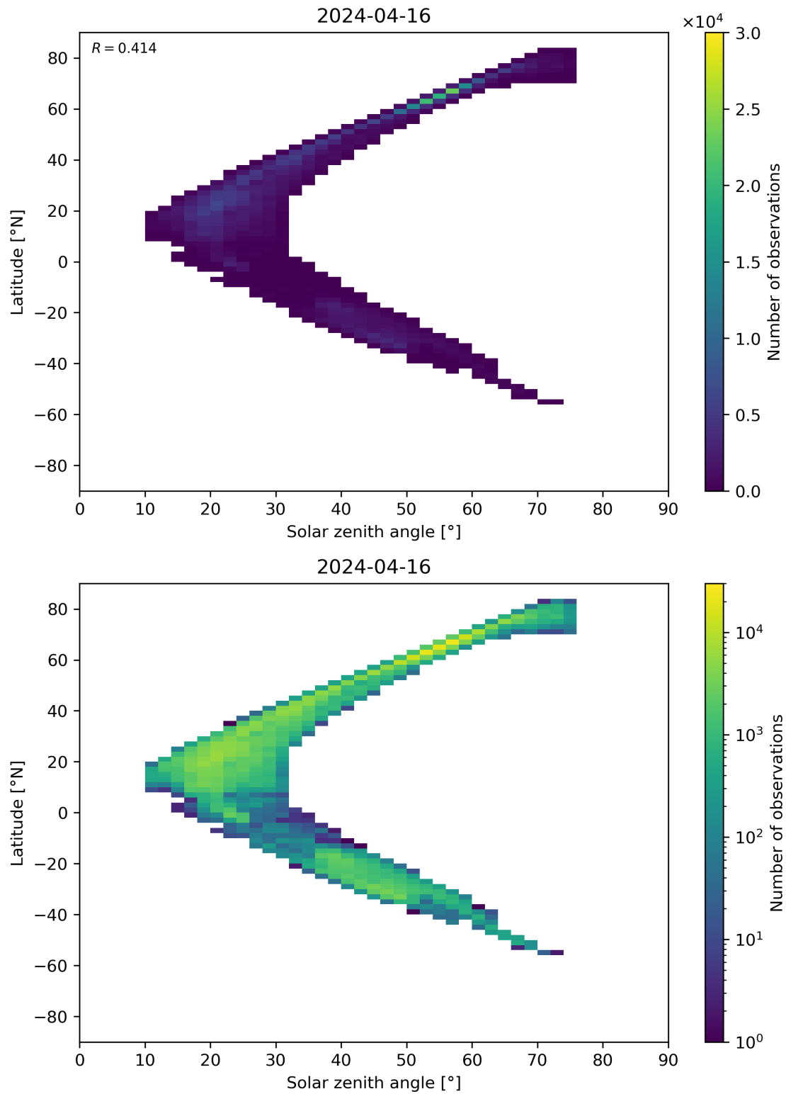
Figure 98: Scatter density plot of “Solar zenith angle” against “Latitude” for 2024-04-16 to 2024-04-17.
