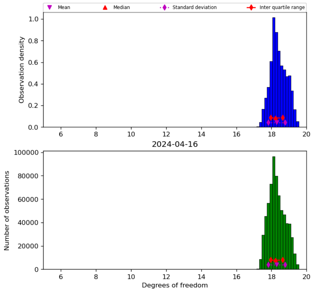
Figure 30: Histogram of “Degrees of freedom” for 2024-04-16 to 2024-04-17
