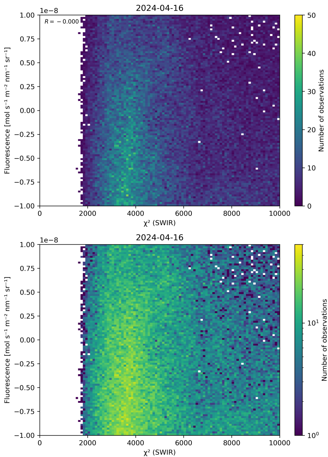
Figure 49: Scatter density plot of “ \chi^2 (SWIR)” against “Fluorescence” for 2024-04-16 to 2024-04-17.
