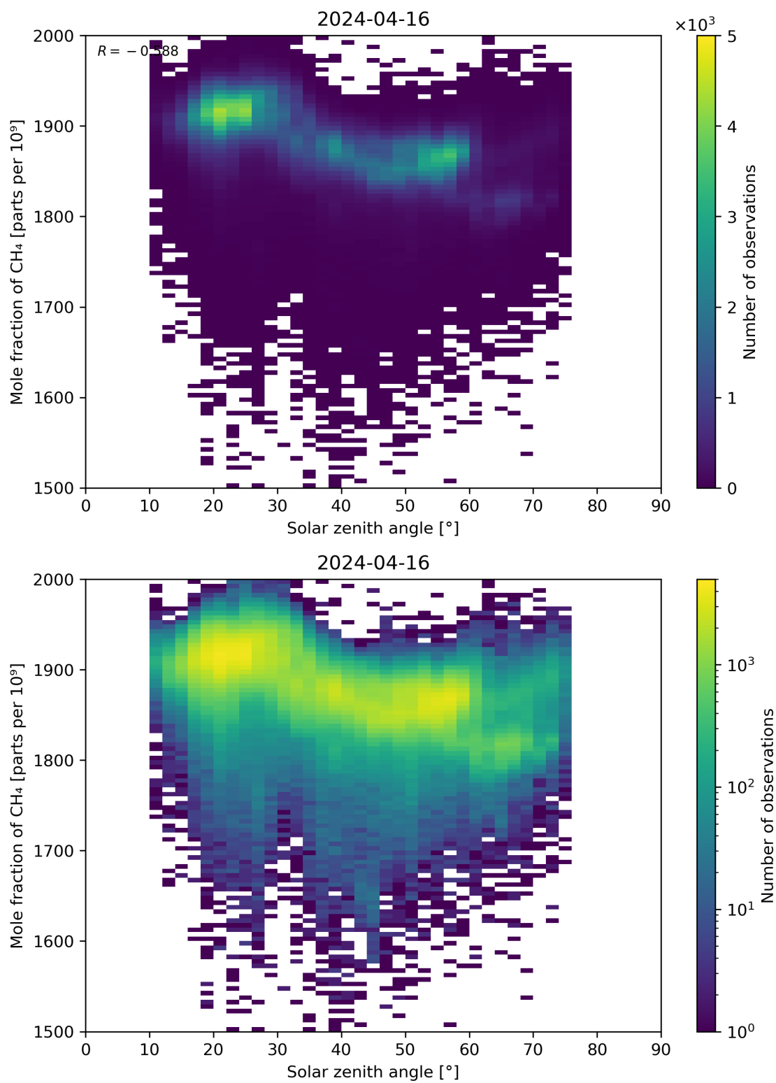
Figure 99: Scatter density plot of “Solar zenith angle” against “Mole fraction of CH 4 ” for 2024-04-16 to 2024-04-17.
