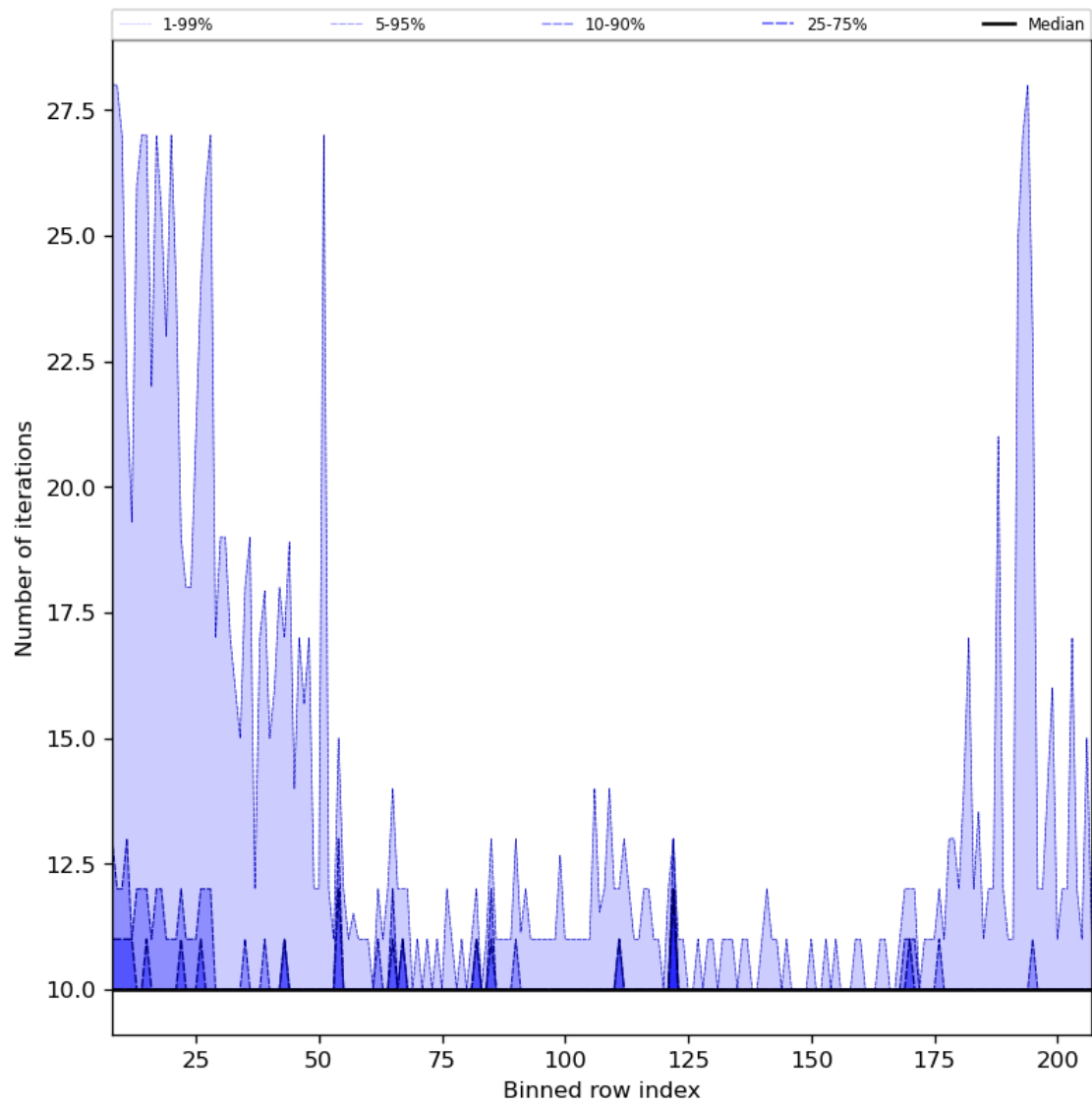
Figure 42: Along track statistics of “Number of iterations” for 2024-04-16 to 2024-04-17
