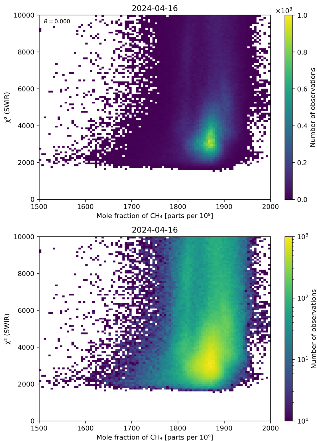
Figure 71: Scatter density plot of “Mole fraction of \text{CH}_4 ” against “ \chi^2 (SWIR)” for 2024-04-16 to 2024-04-17.
