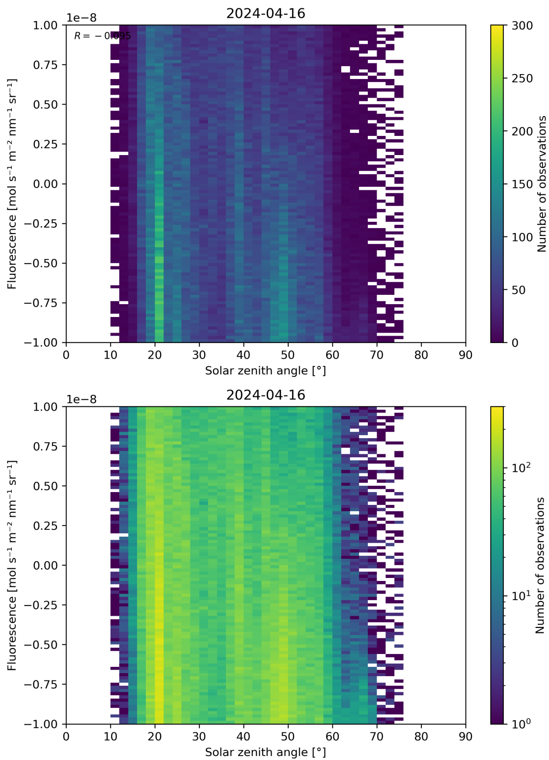
Figure 97: Scatter density plot of “Solar zenith angle” against “Fluorescence” for 2024-04-16 to 2024-04-17.
