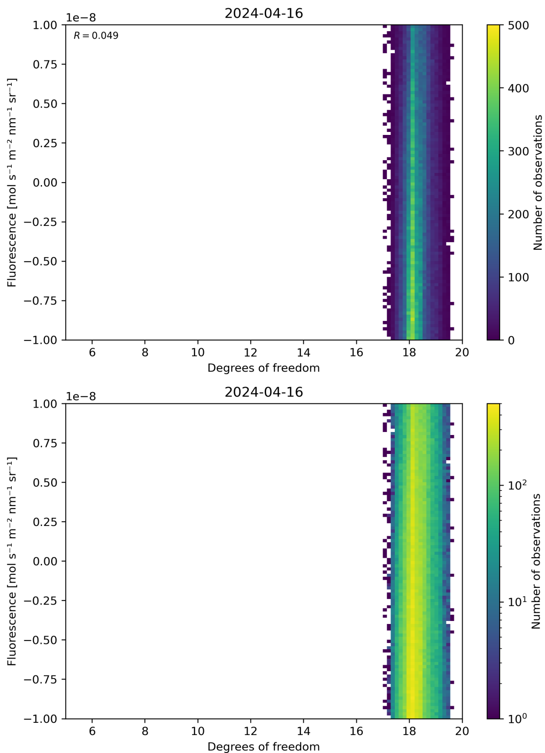
Figure 51: Scatter density plot of “Degrees of freedom” against “Fluorescence” for 2024-04-16 to 2024-04-17.
