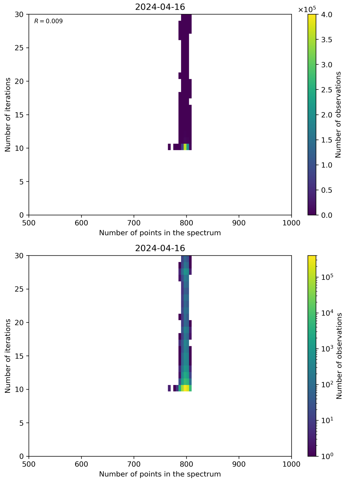
Figure 92: Scatter density plot of “Number of points in the spectrum” against “Number of iterations” for 2024-04-16 to 2024-04-17.
