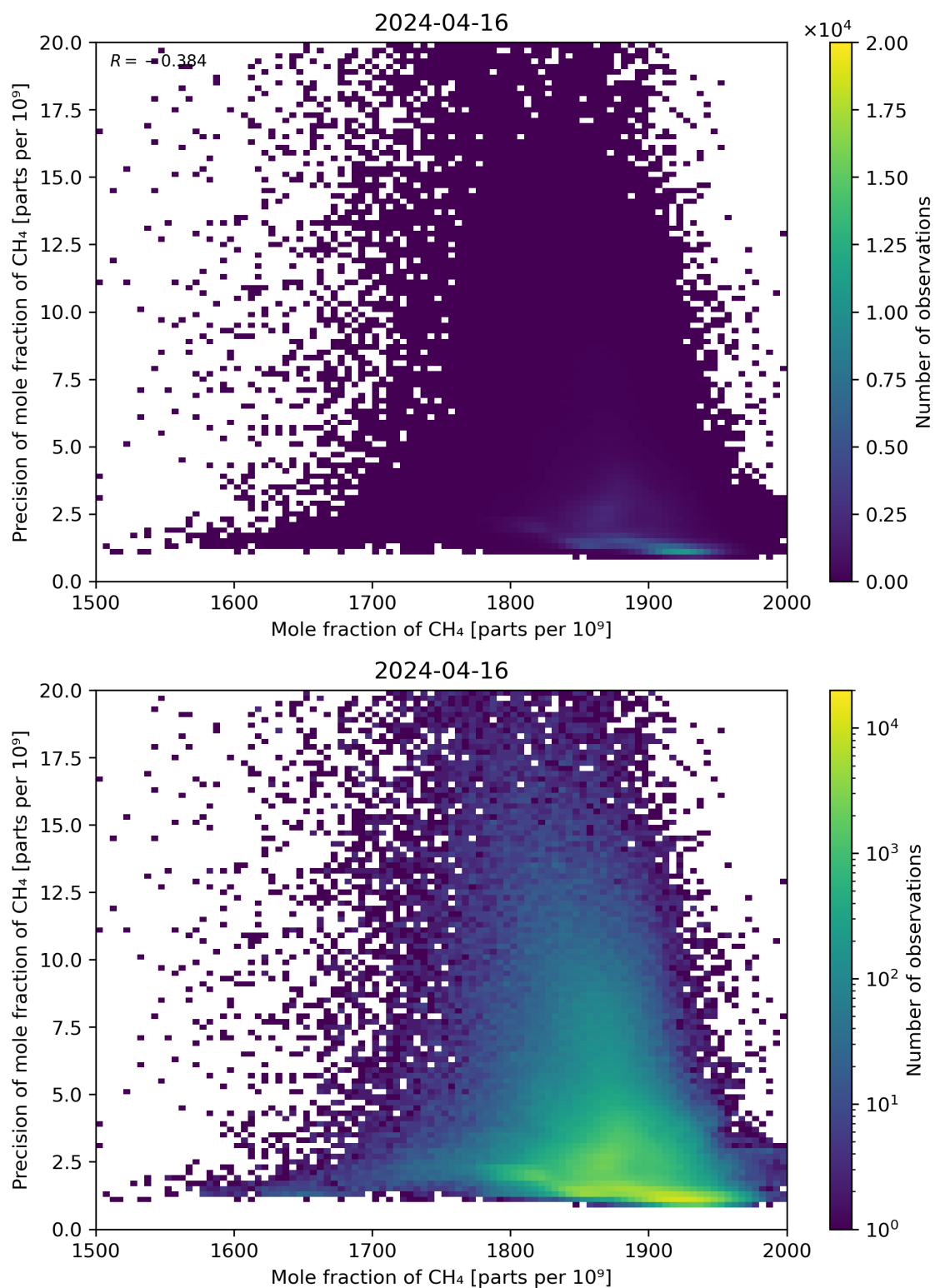
Figure 75: Scatter density plot of “Mole fraction of CH 4 ” against “Precision of mole fraction of CH 4 ” for 2024-04-16 to 2024-04-17.
