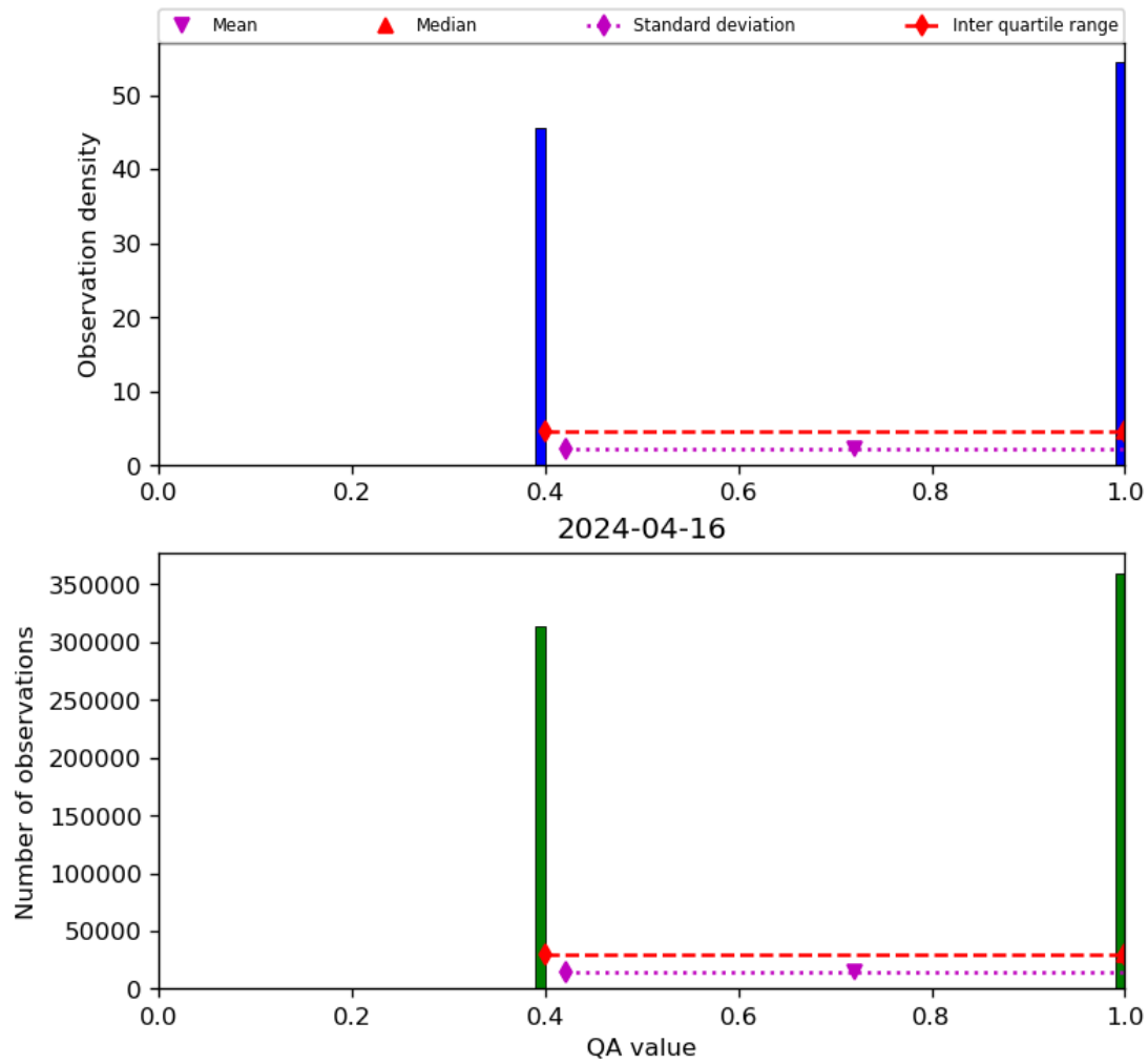
Figure 22: Histogram of “QA value” for 2024-04-16 to 2024-04-17
