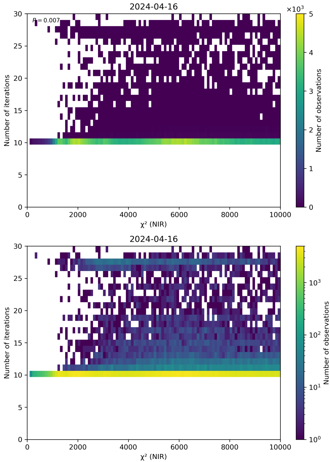
Figure 46: Scatter density plot of “ \chi^2 (NIR)” against “Number of iterations” for 2024-04-16 to 2024-04-17.
