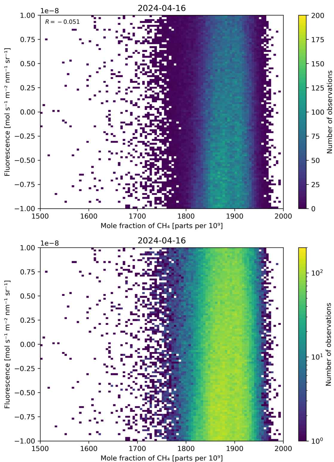
Figure 73: Scatter density plot of “Mole fraction of \text{CH}_4 ” against “Fluorescence” for 2024-04-16 to 2024-04-17.
