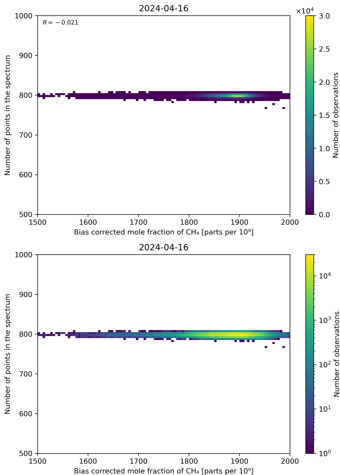
Figure 68: Scatter density plot of “Bias corrected mole fraction of CH 4 ” against “Number of points in the spectrum” for 2024-04-16 to 2024-04-17.
