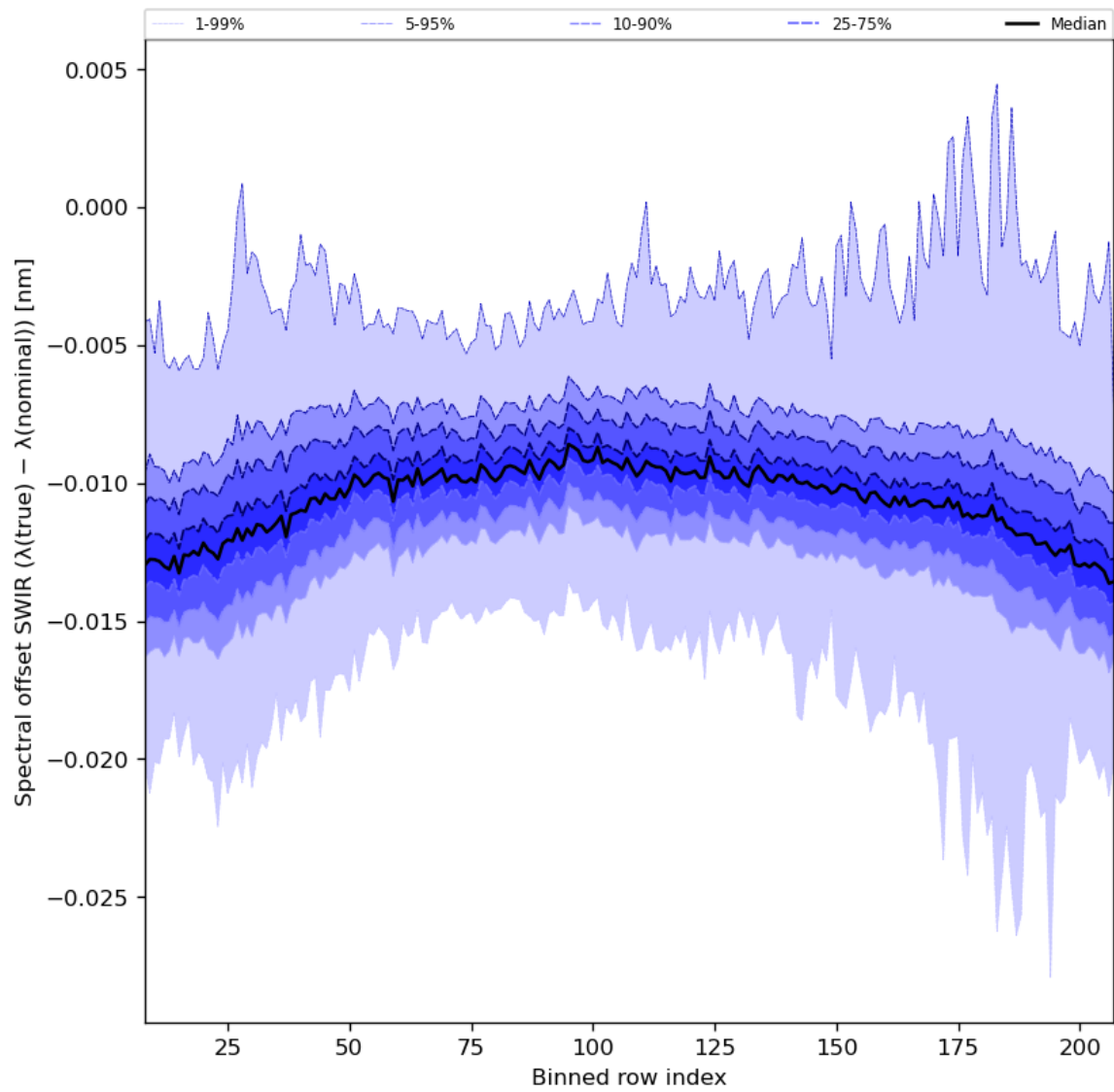
Figure 38: Along track statistics of “Spectral offset SWIR ( \lambda(\text{true}) - \lambda(\text{nominal}) )” for 2024-04-16 to 2024-04-17
