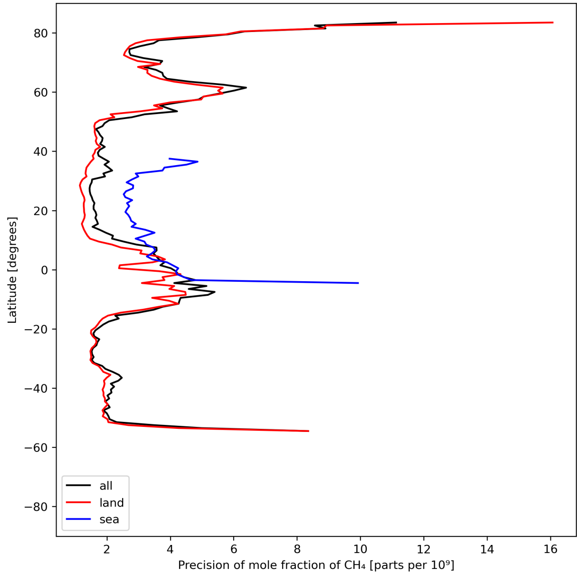
Figure 13: Zonal average of “Precision of mole fraction of CH 4 ” for 2024-04-16 to 2024-04-17.
