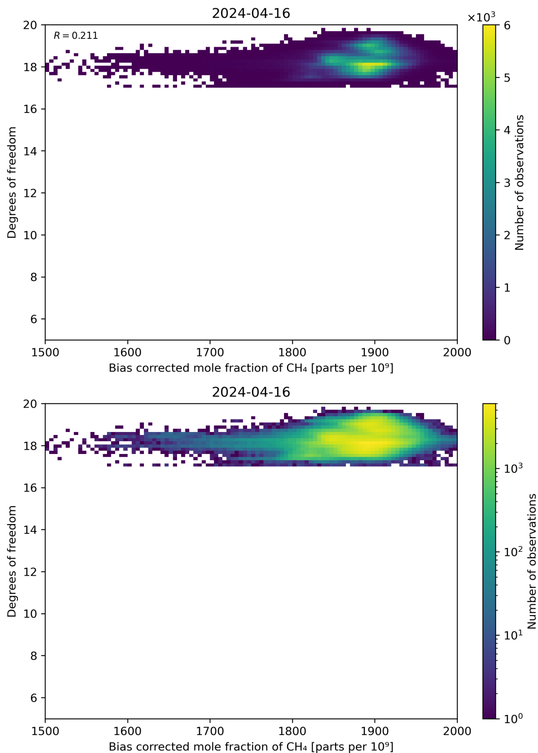
Figure 65: Scatter density plot of “Bias corrected mole fraction of CH 4 ” against “Degrees of freedom” for 2024-04-16 to 2024-04-17.
