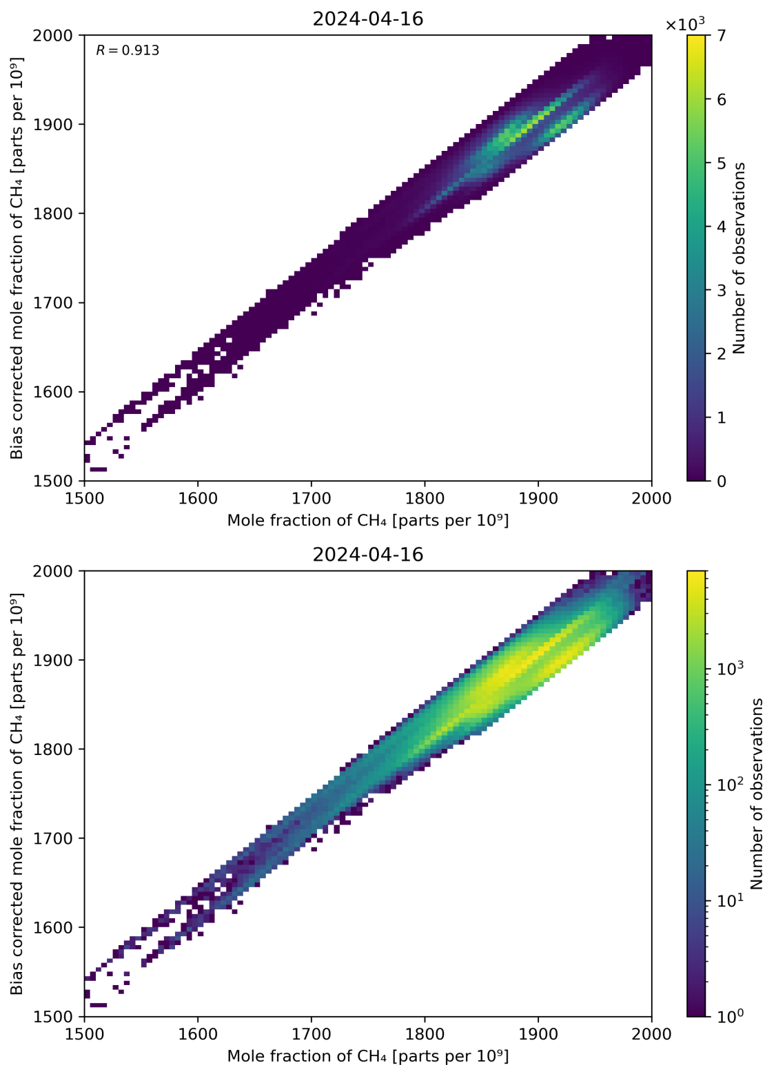
Figure 74: Scatter density plot of “Mole fraction of CH 4 ” against “Bias corrected mole fraction of CH 4 ” for 2024-04-16 to 2024-04-17.
