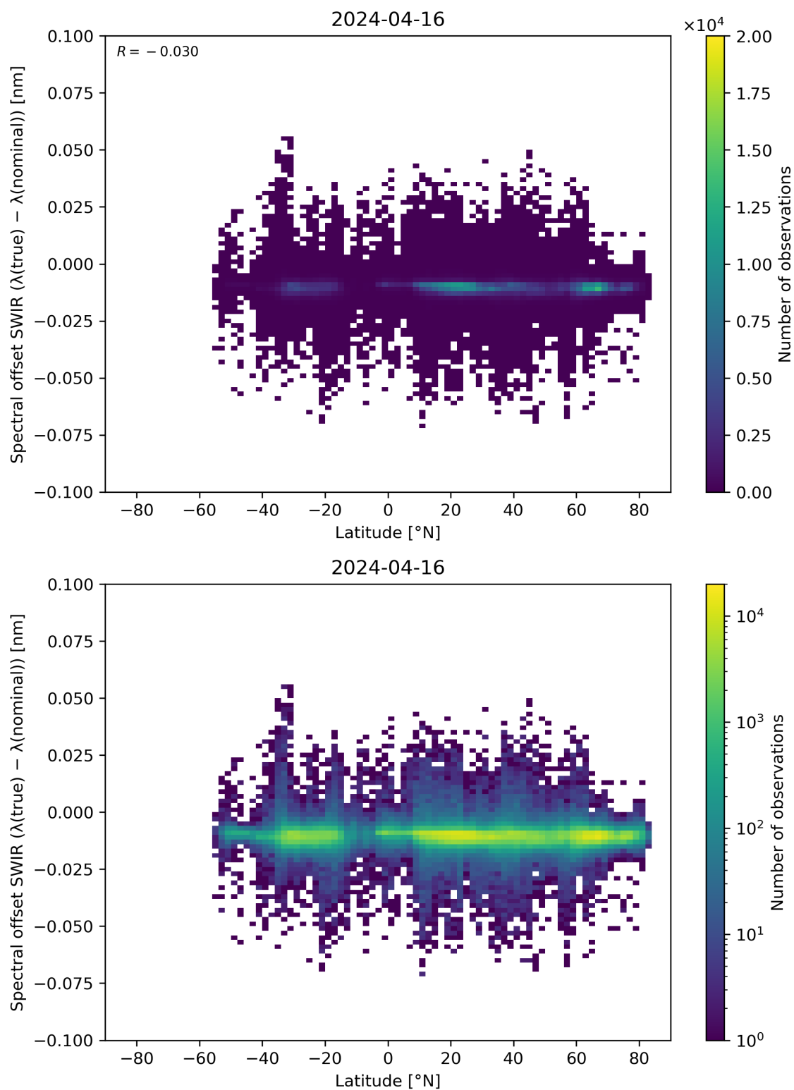
Figure 62: Scatter density plot of “Latitude” against “Spectral offset SWIR ( \lambda(\text{true}) - \lambda(\text{nominal}) )” for 2024-04-16 to 2024-04-17.
