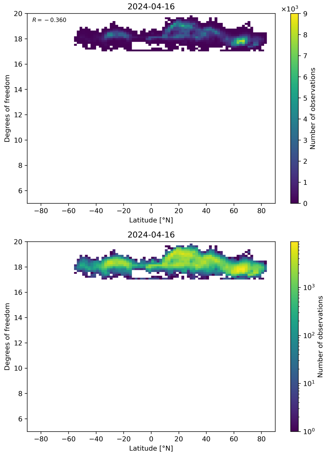
Figure 55: Scatter density plot of “Latitude” against “Degrees of freedom” for 2024-04-16 to 2024-04-17.
