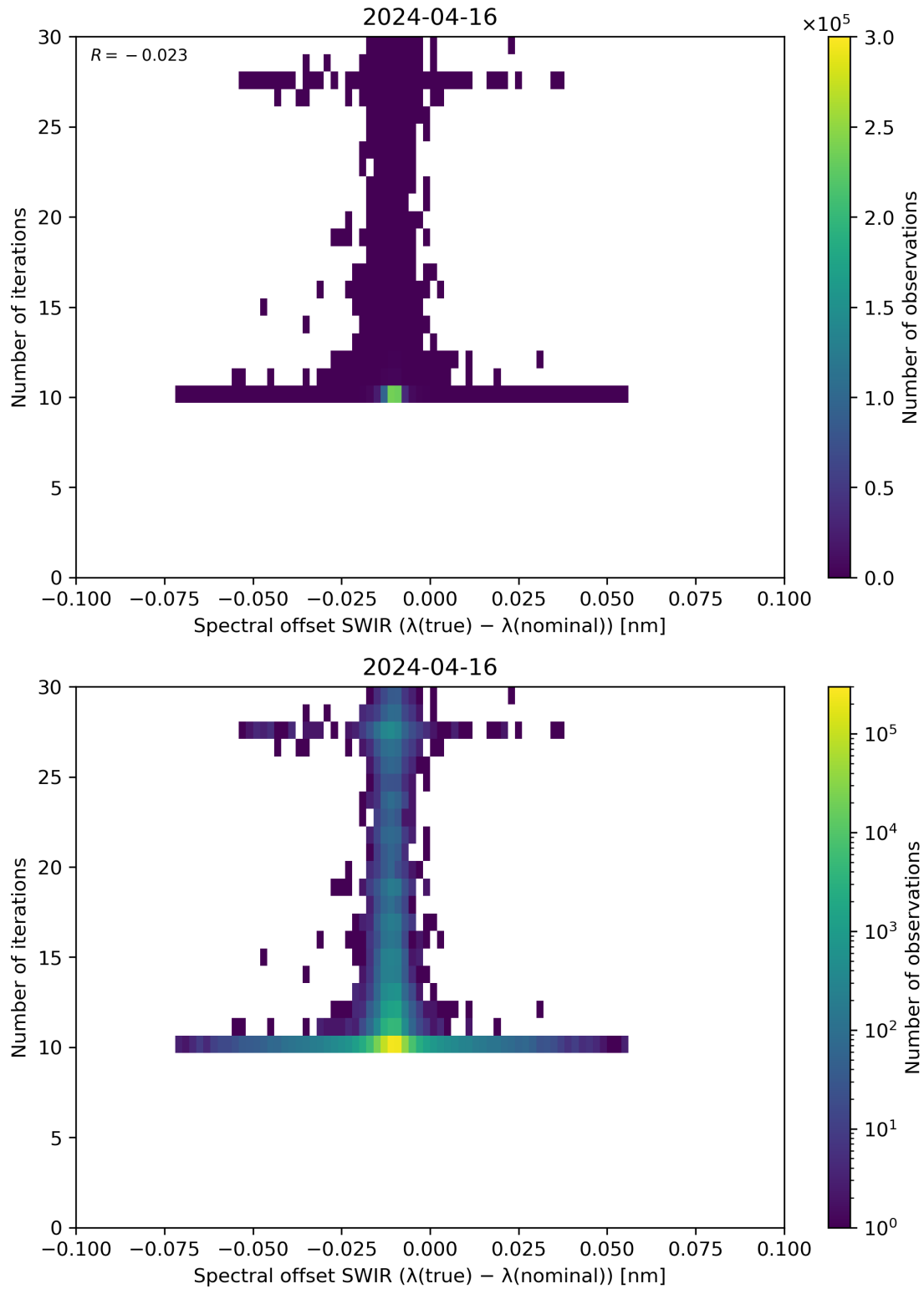
Figure 121: Scatter density plot of “Spectral offset SWIR ( \lambda(\text{true}) - \lambda(\text{nominal}) )” against “Number of iterations” for 2024-04-16 to 2024-04-17.
