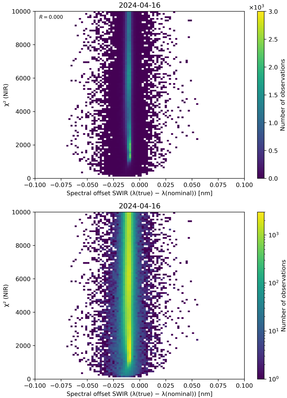
Figure 117: Scatter density plot of “Spectral offset SWIR ( \lambda(\text{true}) - \lambda(\text{nominal}) )” against “ \chi^2 (NIR)” for 2024-04-16 to 2024-04-17.
