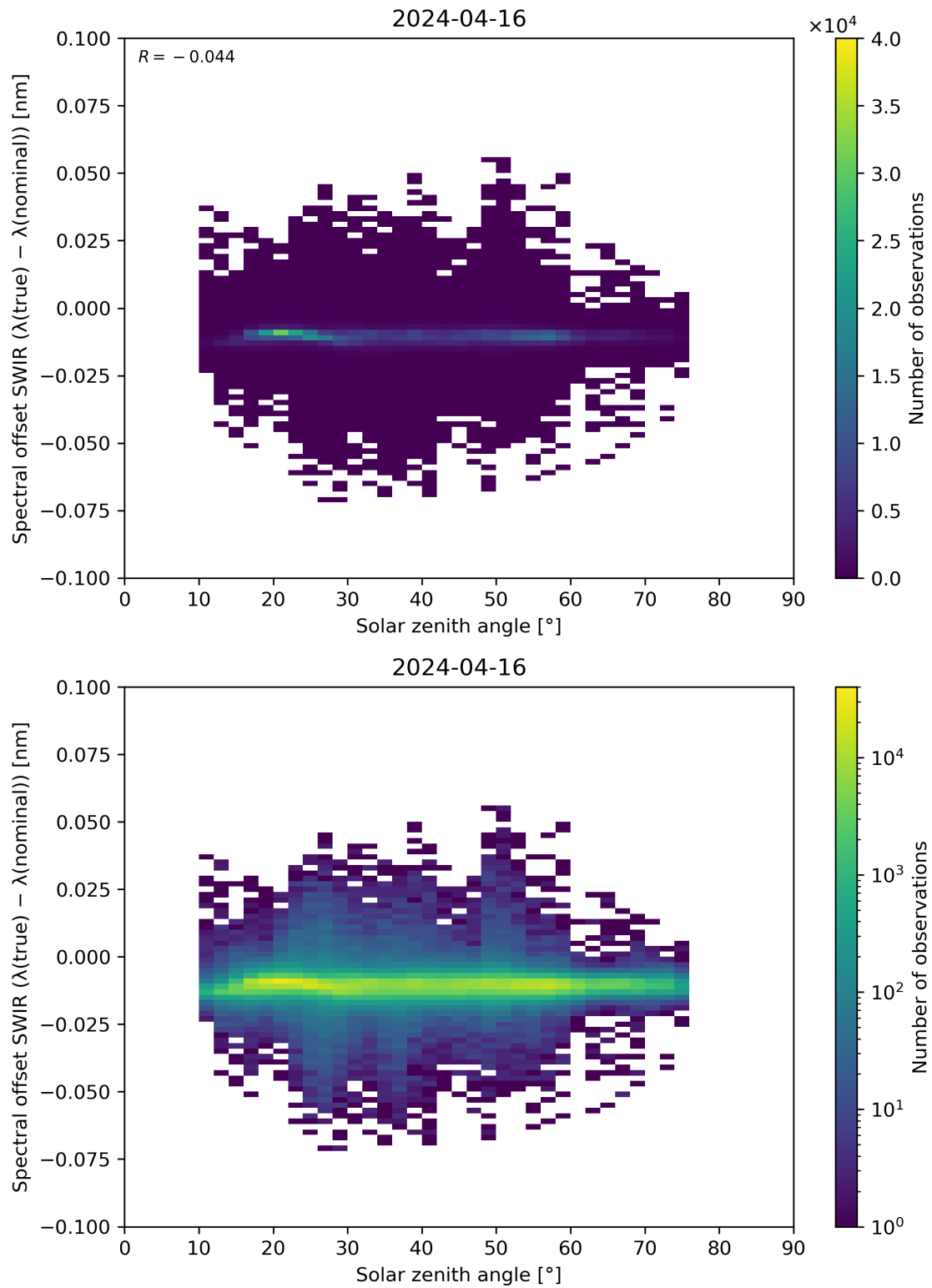
Figure 104: Scatter density plot of “Solar zenith angle” against “Spectral offset SWIR ( \lambda(\text{true}) - \lambda(\text{nominal}) )” for 2024-04-16 to 2024-04-17.
