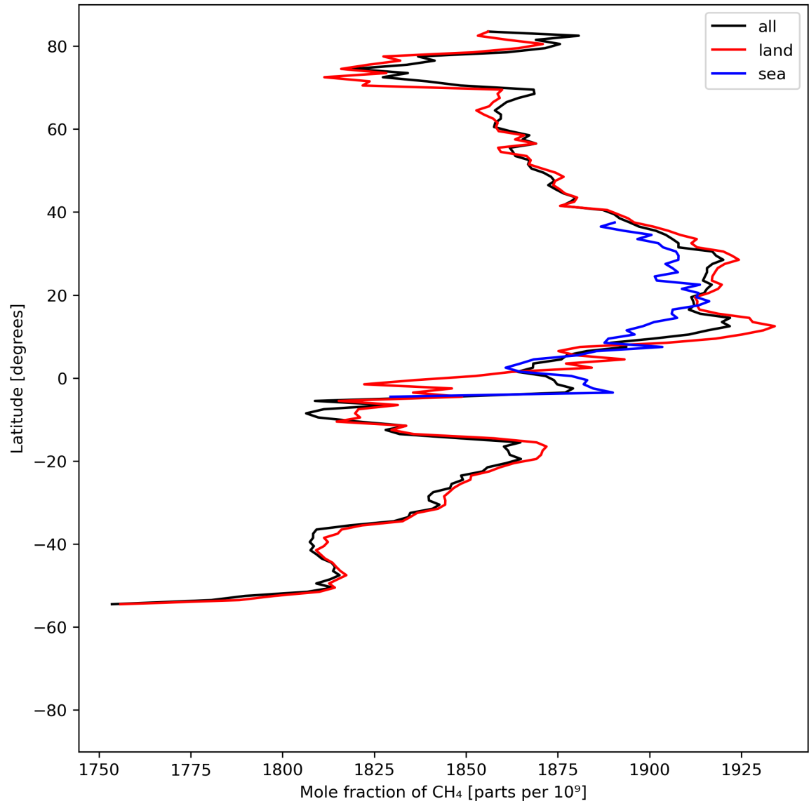
Figure 12: Zonal average of “Mole fraction of \text{CH}_4 ” for 2024-04-16 to 2024-04-17.
