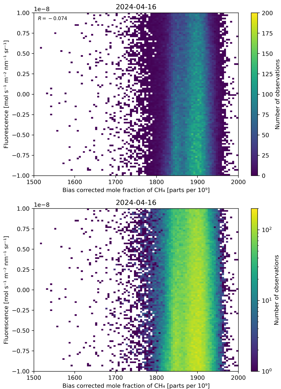
Figure 66: Scatter density plot of “Bias corrected mole fraction of \text{CH}_4 ” against “Fluorescence” for 2024-04-16 to 2024-04-17.
