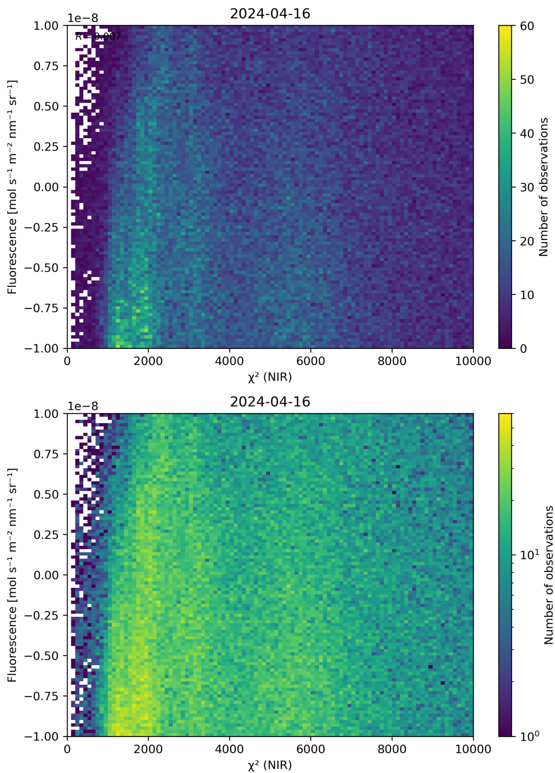
Figure 45: Scatter density plot of “ \chi^2 (NIR)” against “Fluorescence” for 2024-04-16 to 2024-04-17.
