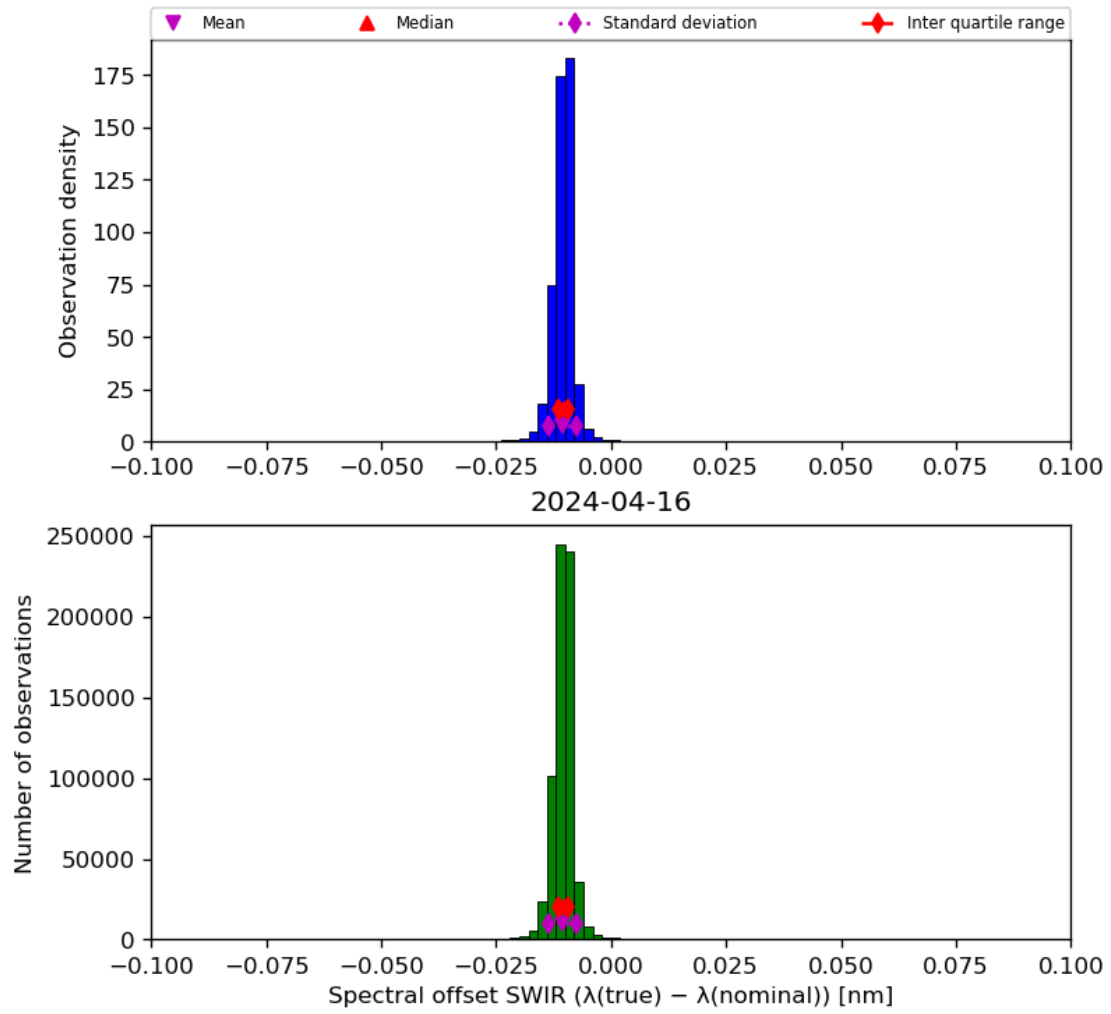
Figure 27: Histogram of “Spectral offset SWIR ( \lambda(\text{true}) - \lambda(\text{nominal}) )” for 2024-04-16 to 2024-04-17
