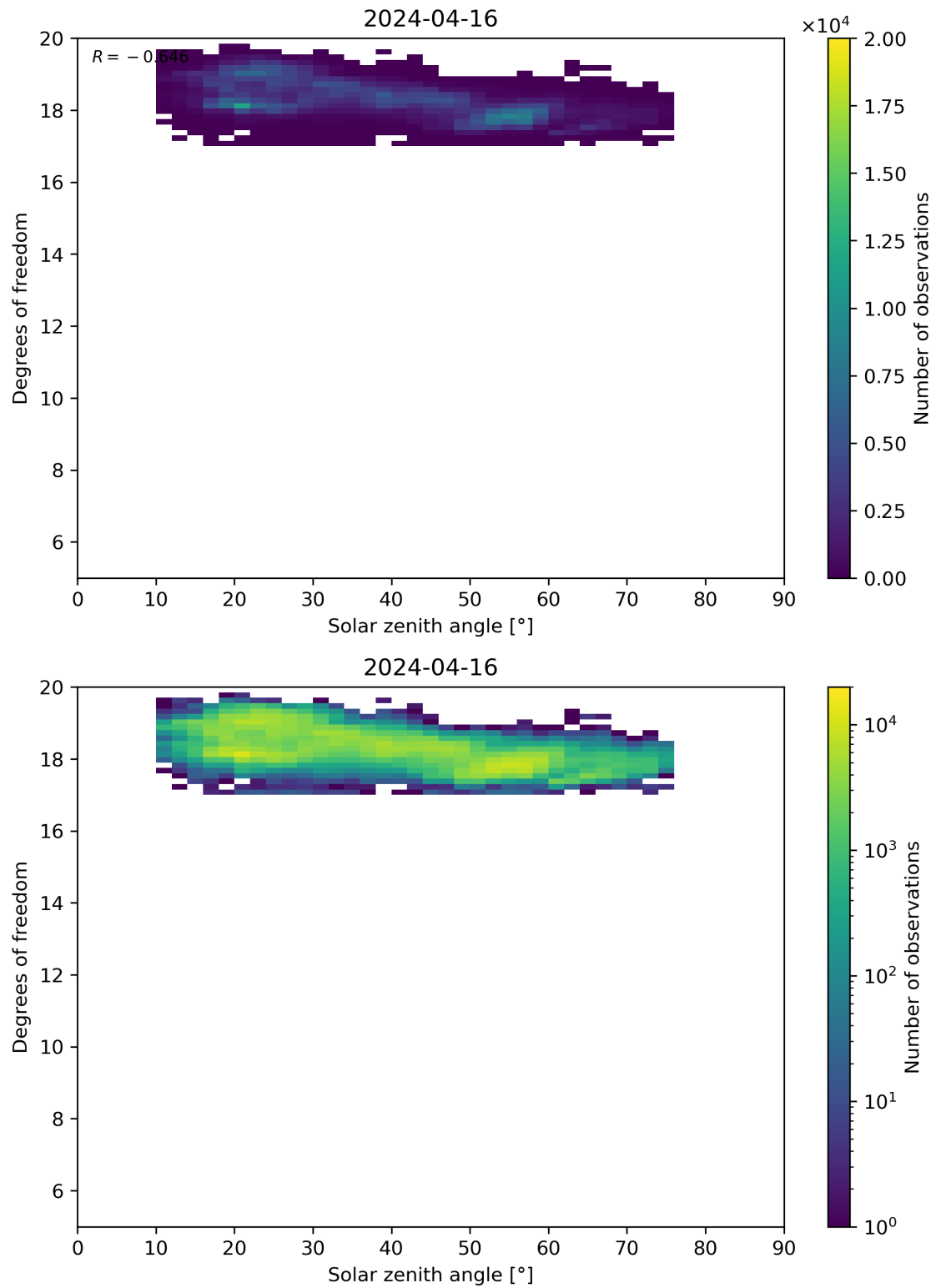
Figure 96: Scatter density plot of “Solar zenith angle” against “Degrees of freedom” for 2024-04-16 to 2024-04-17.
