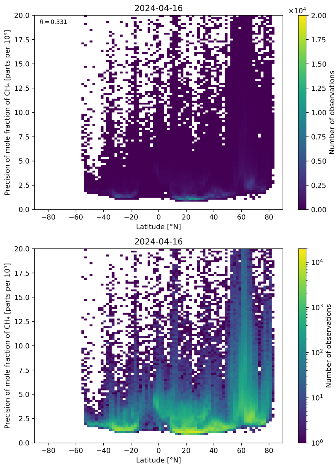
Figure 59: Scatter density plot of “Latitude” against “Precision of mole fraction of CH 4 ” for 2024-04-16 to 2024-04-17.
