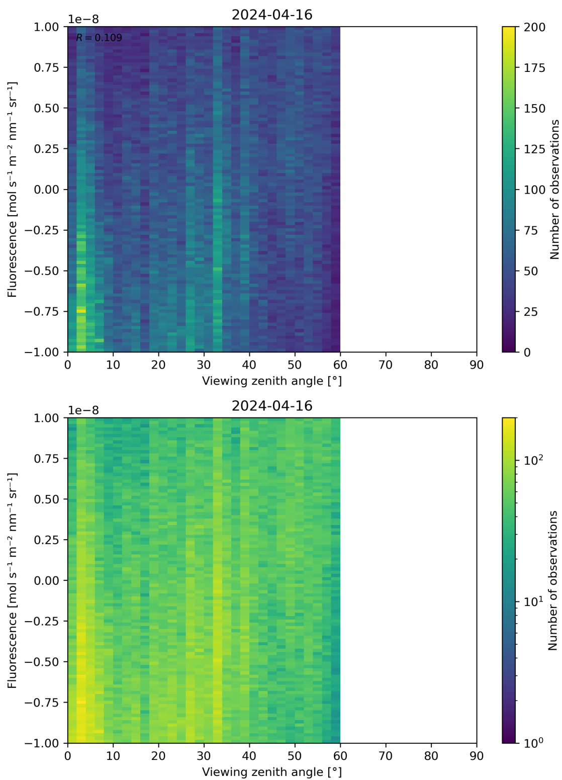
Figure 108: Scatter density plot of “Viewing zenith angle” against “Fluorescence” for 2024-04-16 to 2024-04-17.
