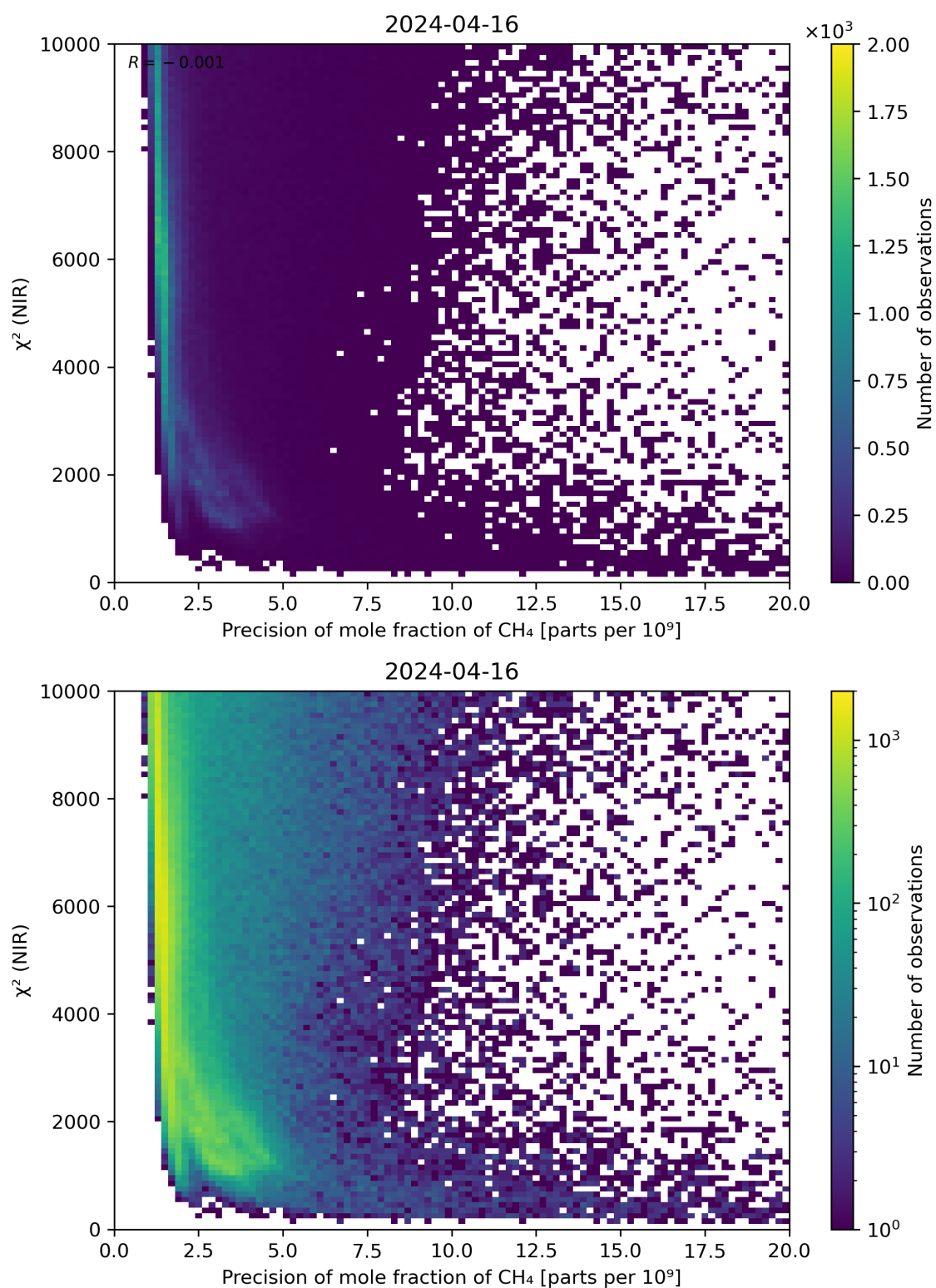
Figure 78: Scatter density plot of “Precision of mole fraction of CH 4 ” against “ \chi^2 (NIR)” for 2024-04-16 to 2024-04-17.
