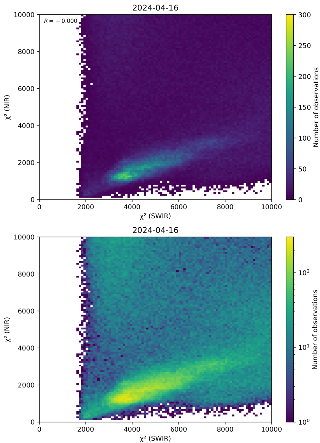
Figure 47: Scatter density plot of “ \chi^2 (SWIR)” against “ \chi^2 (NIR)” for 2024-04-16 to 2024-04-17.
