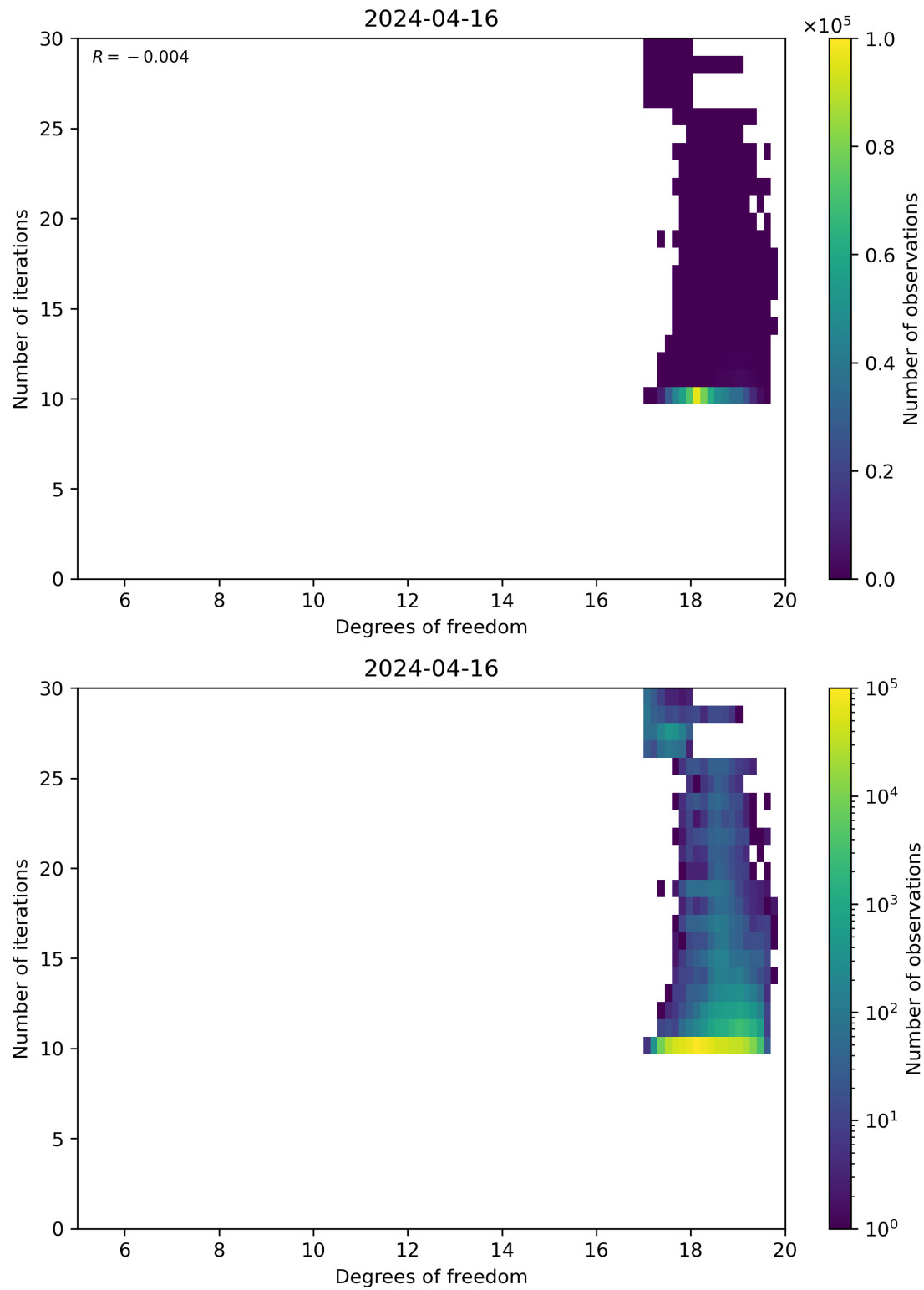
Figure 52: Scatter density plot of “Degrees of freedom” against “Number of iterations” for 2024-04-16 to 2024-04-17.
