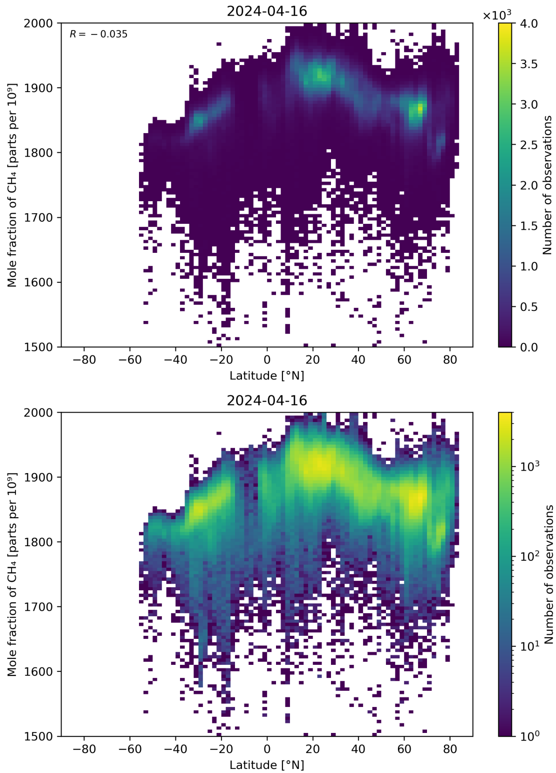
Figure 57: Scatter density plot of “Latitude” against “Mole fraction of CH 4 ” for 2024-04-16 to 2024-04-17.
