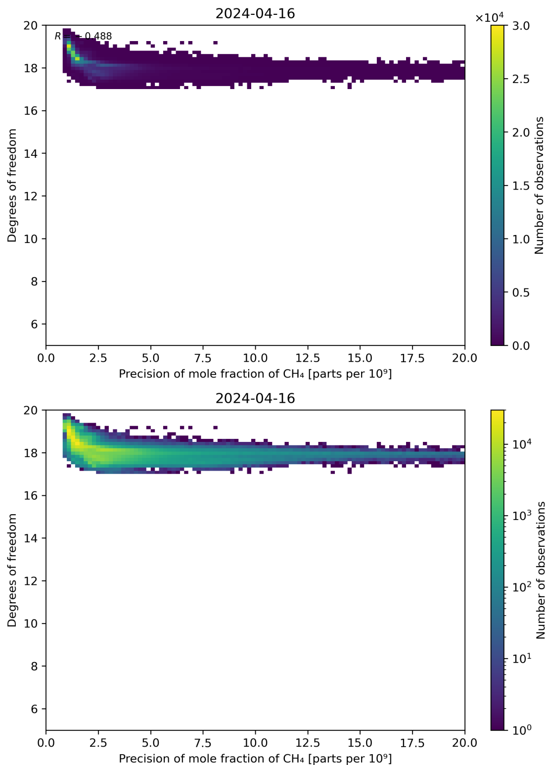
Figure 80: Scatter density plot of “Precision of mole fraction of CH 4 ” against “Degrees of freedom” for 2024-04-16 to 2024-04-17.
