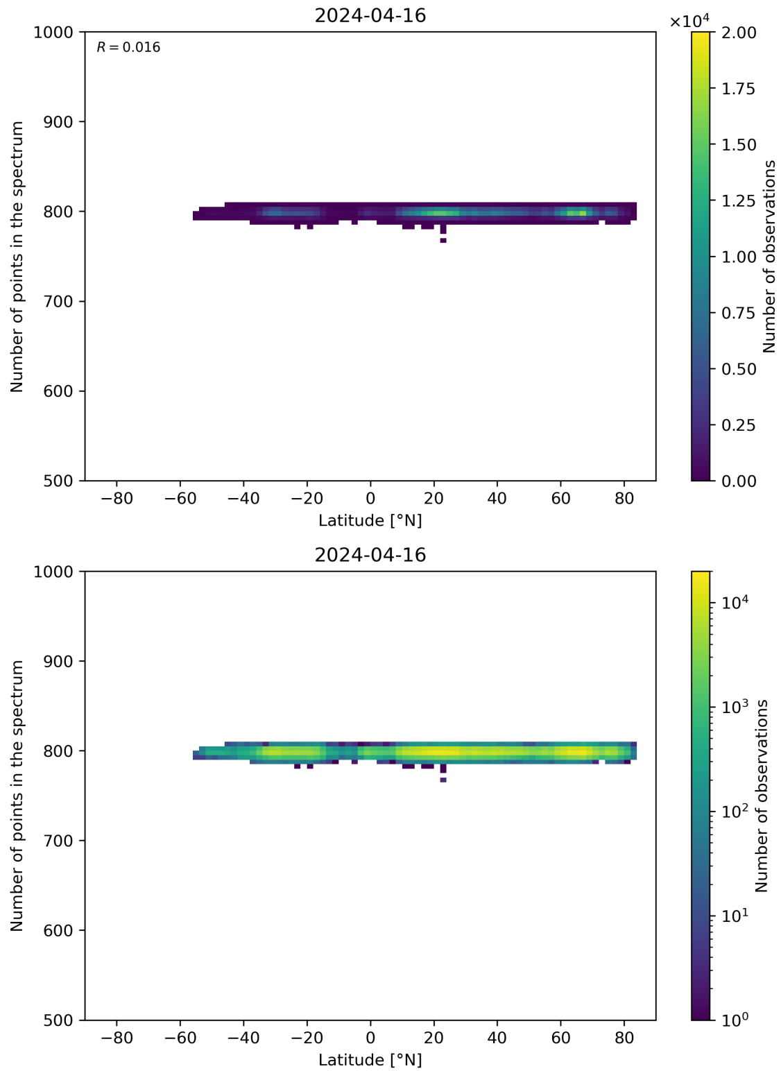
Figure 61: Scatter density plot of “Latitude” against “Number of points in the spectrum” for 2024-04-16 to 2024-04-17.
