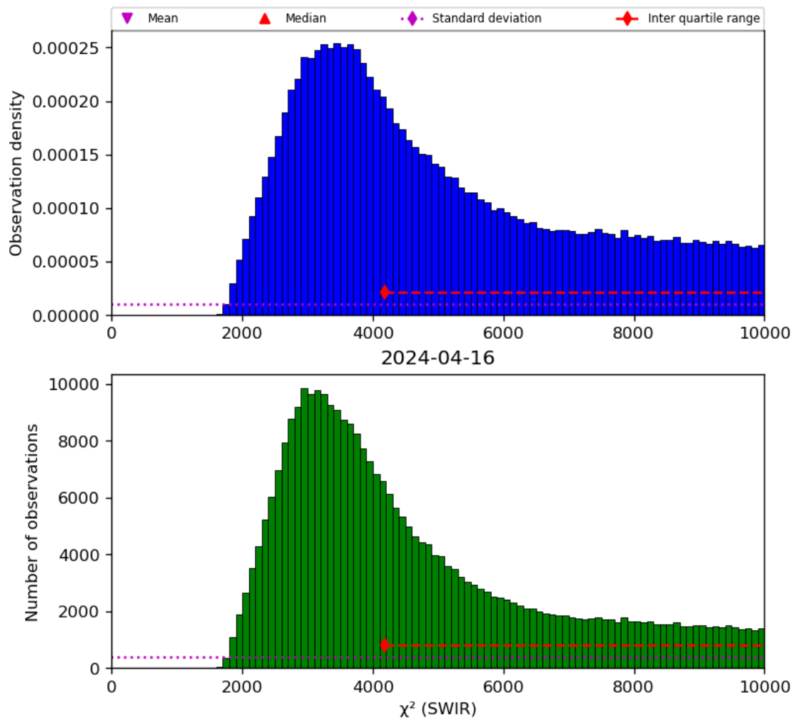
Figure 28: Histogram of “ \chi^2 (SWIR)” for 2024-04-16 to 2024-04-17
