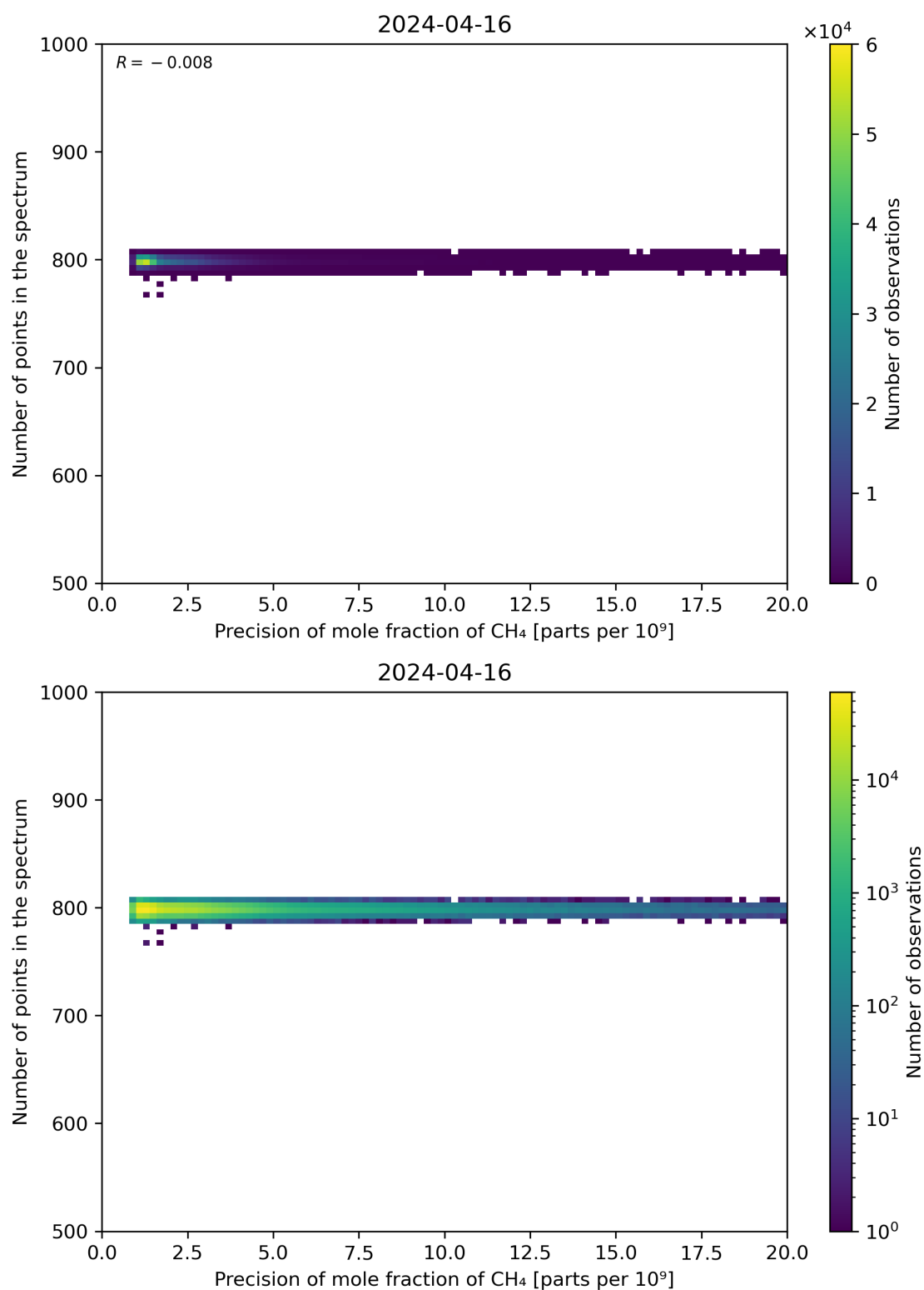
Figure 84: Scatter density plot of “Precision of mole fraction of CH 4 ” against “Number of points in the spectrum” for 2024-04-16 to 2024-04-17.
