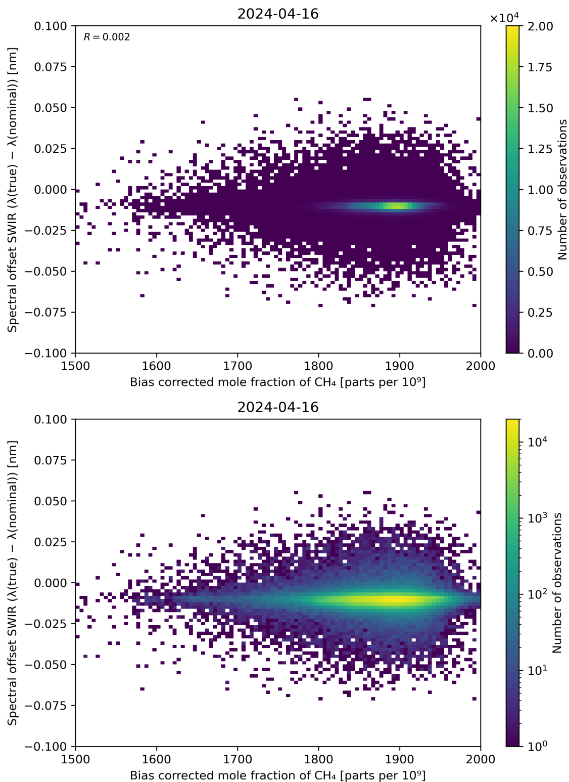
Figure 69: Scatter density plot of “Bias corrected mole fraction of \text{CH}_4 ” against “Spectral offset SWIR ( \lambda(\text{true}) - \lambda(\text{nominal}) )” for 2024-04-16 to 2024-04-17.
