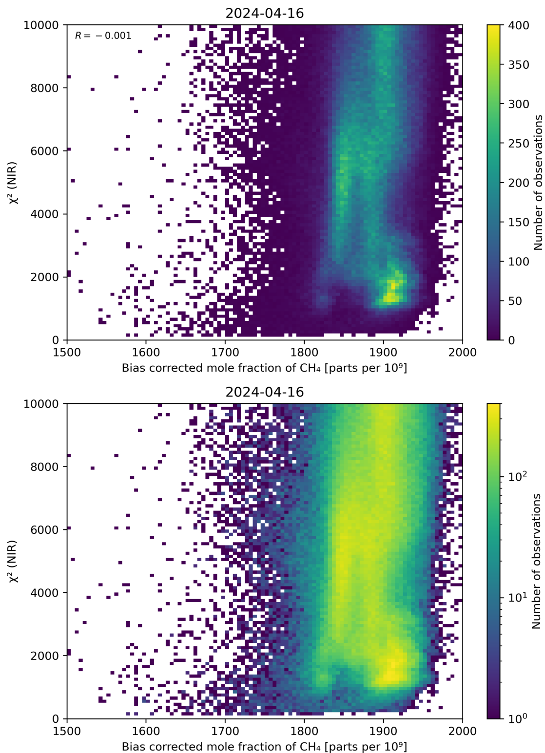
Figure 63: Scatter density plot of “Bias corrected mole fraction of CH 4 ” against “ \chi^2 (NIR)” for 2024-04-16 to 2024-04-17.
