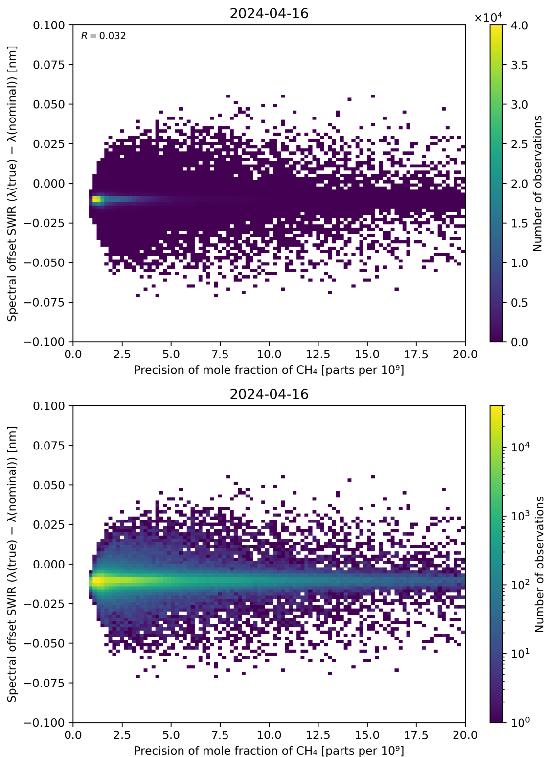
Figure 85: Scatter density plot of “Precision of mole fraction of \text{CH}_4 ” against “Spectral offset SWIR ( \lambda(\text{true}) - \lambda(\text{nominal}) )” for 2024-04-16 to 2024-04-17.
