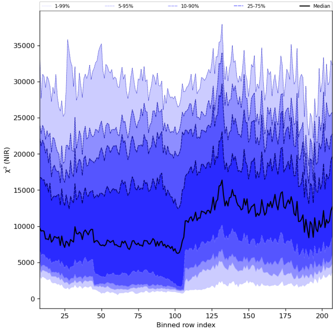
Figure 40: Along track statistics of “ \chi^2 (NIR)” for 2024-04-16 to 2024-04-17
