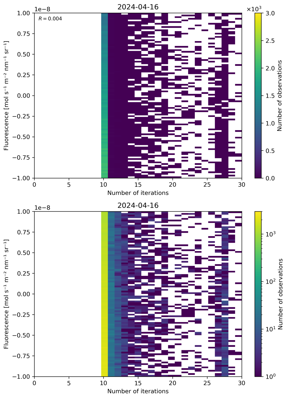
Figure 87: Scatter density plot of “Number of iterations” against “Fluorescence” for 2024-04-16 to 2024-04-17.
