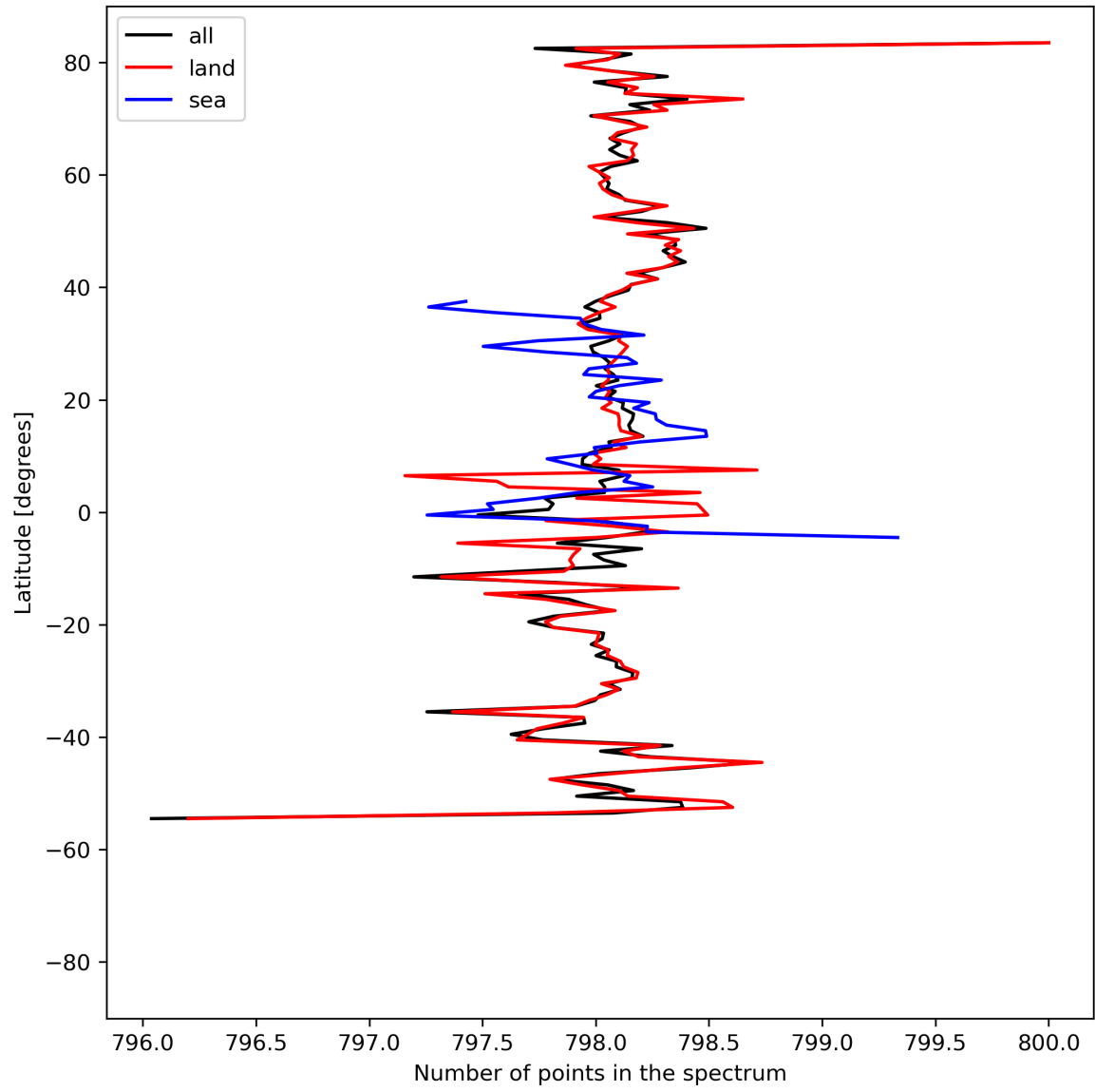
Figure 15: Zonal average of “Number of points in the spectrum” for 2024-04-16 to 2024-04-17.
