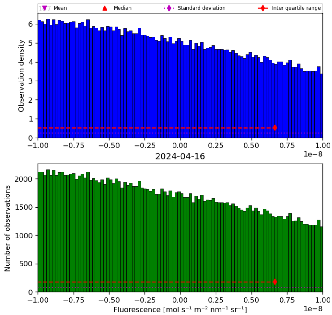
Figure 32: Histogram of “Fluorescence” for 2024-04-16 to 2024-04-17
