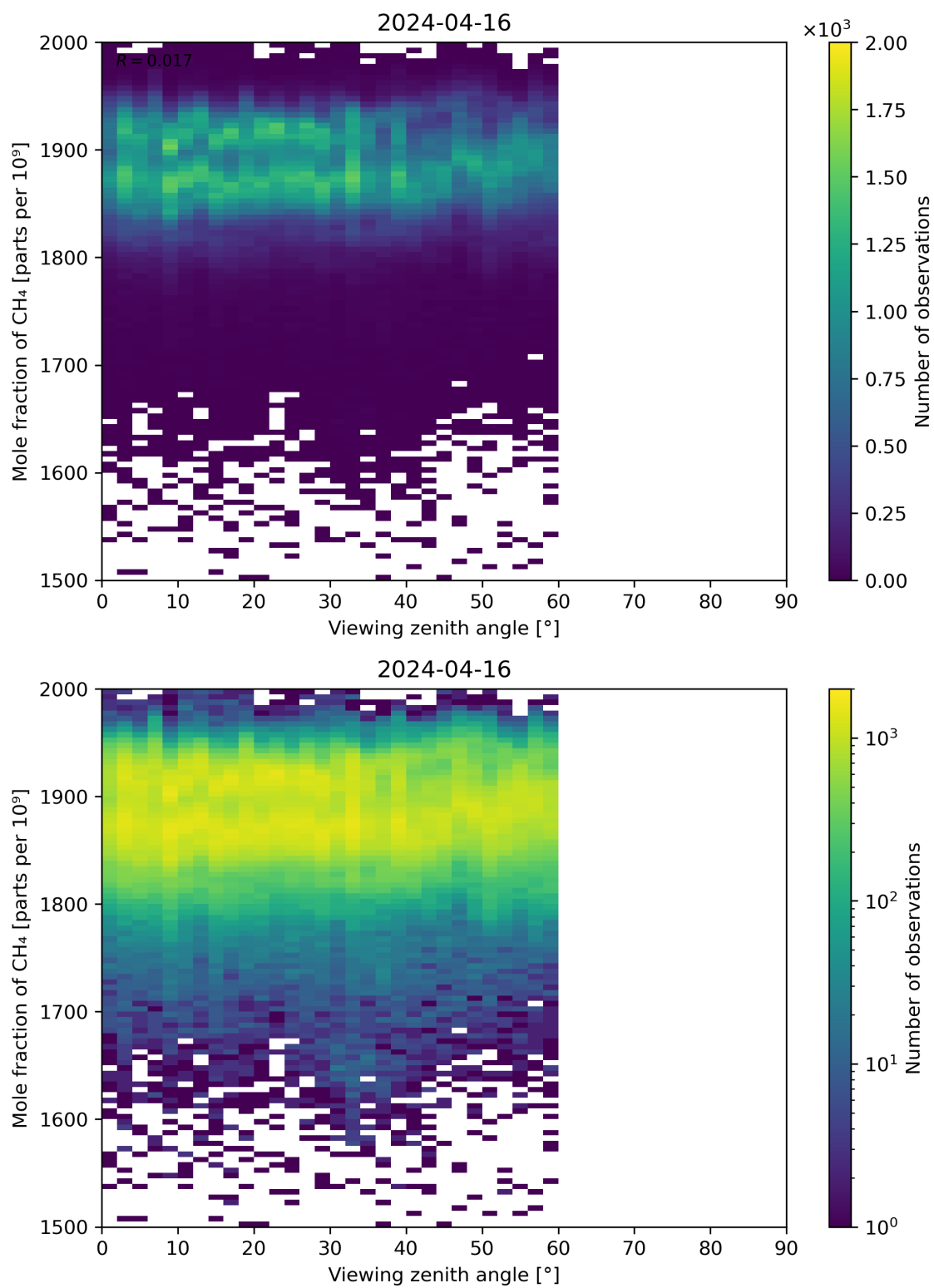
Figure 110: Scatter density plot of “Viewing zenith angle” against “Mole fraction of CH 4 ” for 2024-04-16 to 2024-04-17.
