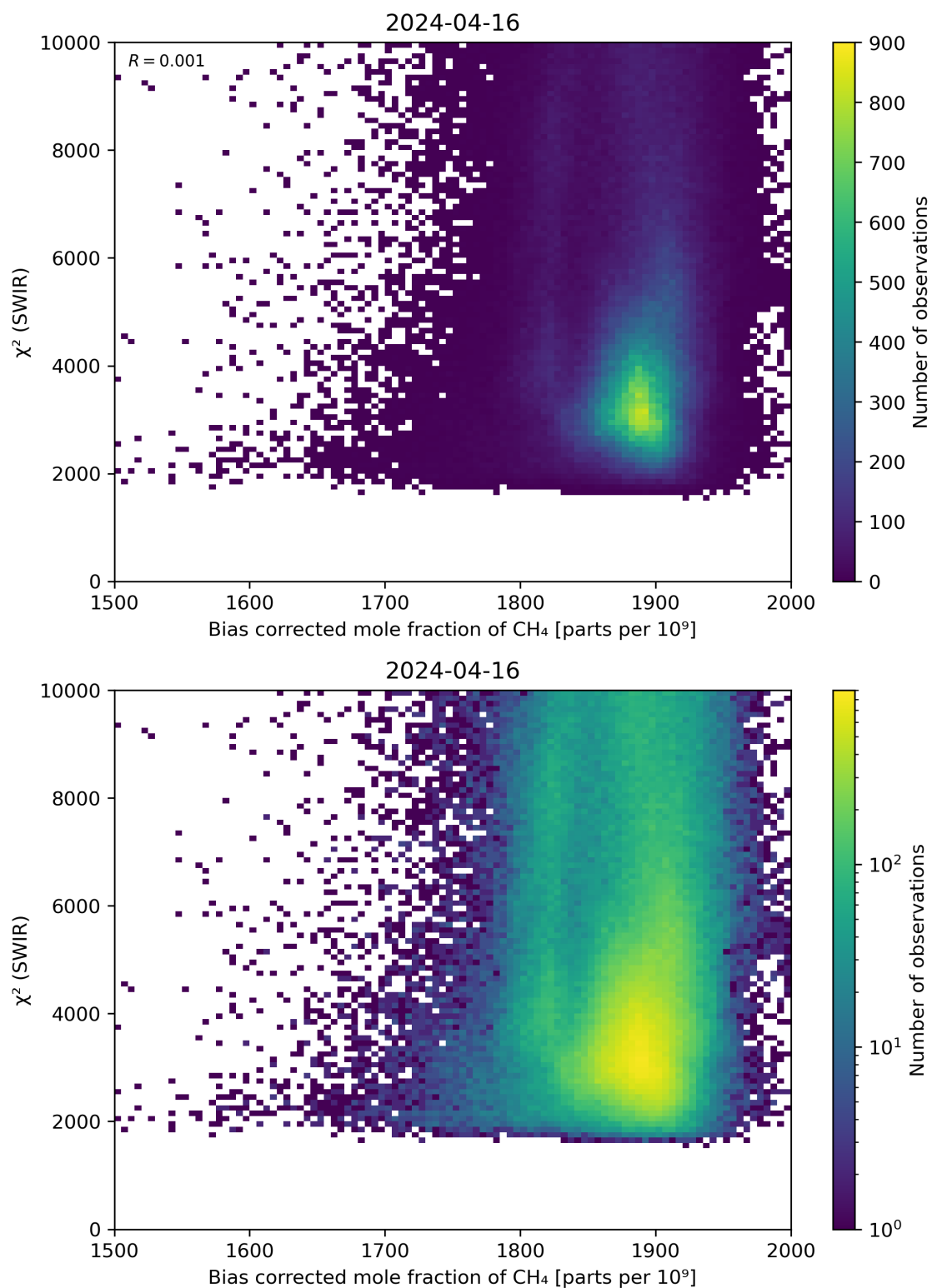
Figure 64: Scatter density plot of “Bias corrected mole fraction of CH 4 ” against “ \chi^2 (SWIR)” for 2024-04-16 to 2024-04-17.
