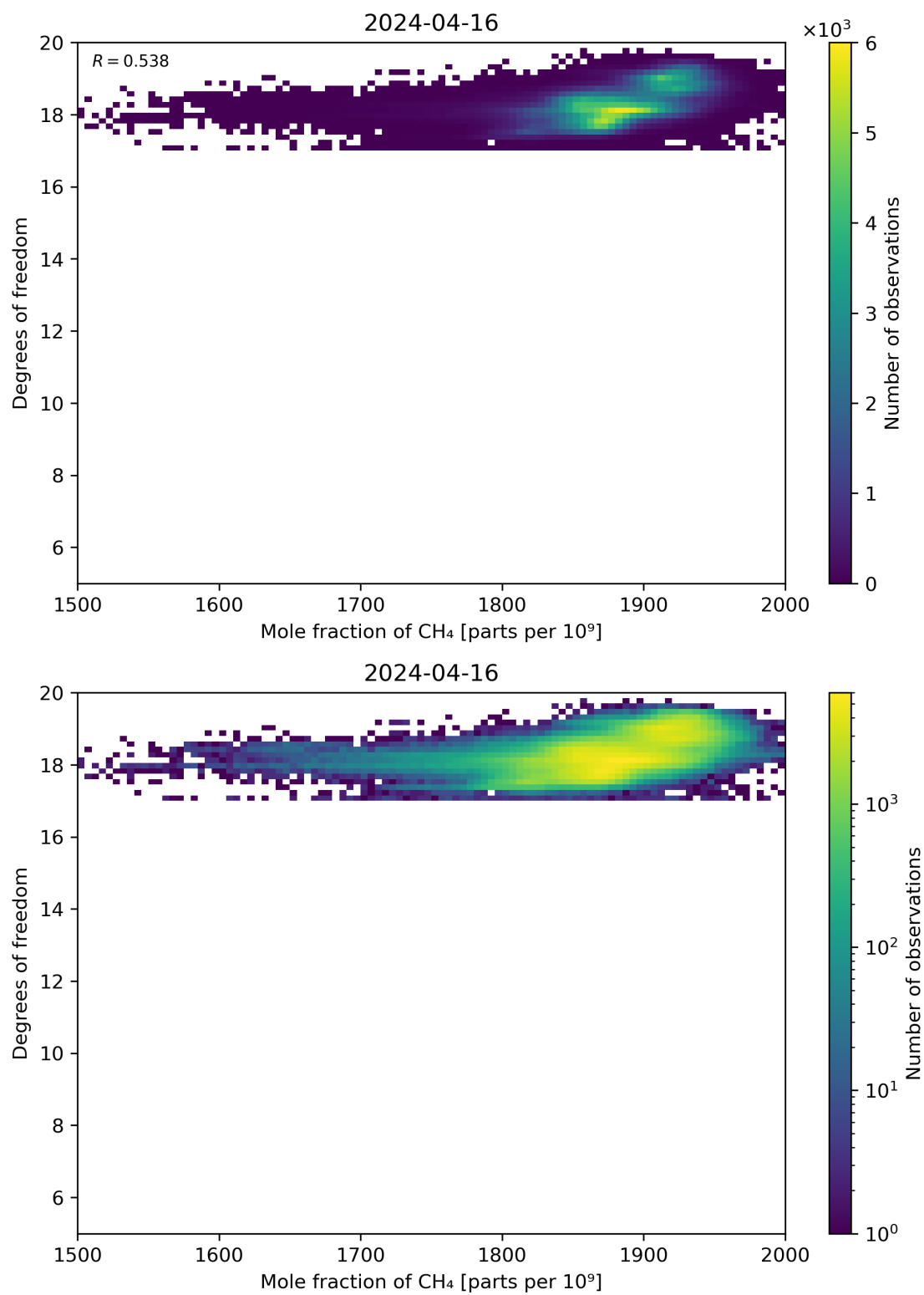
Figure 72: Scatter density plot of “Mole fraction of CH 4 ” against “Degrees of freedom” for 2024-04-16 to 2024-04-17.
