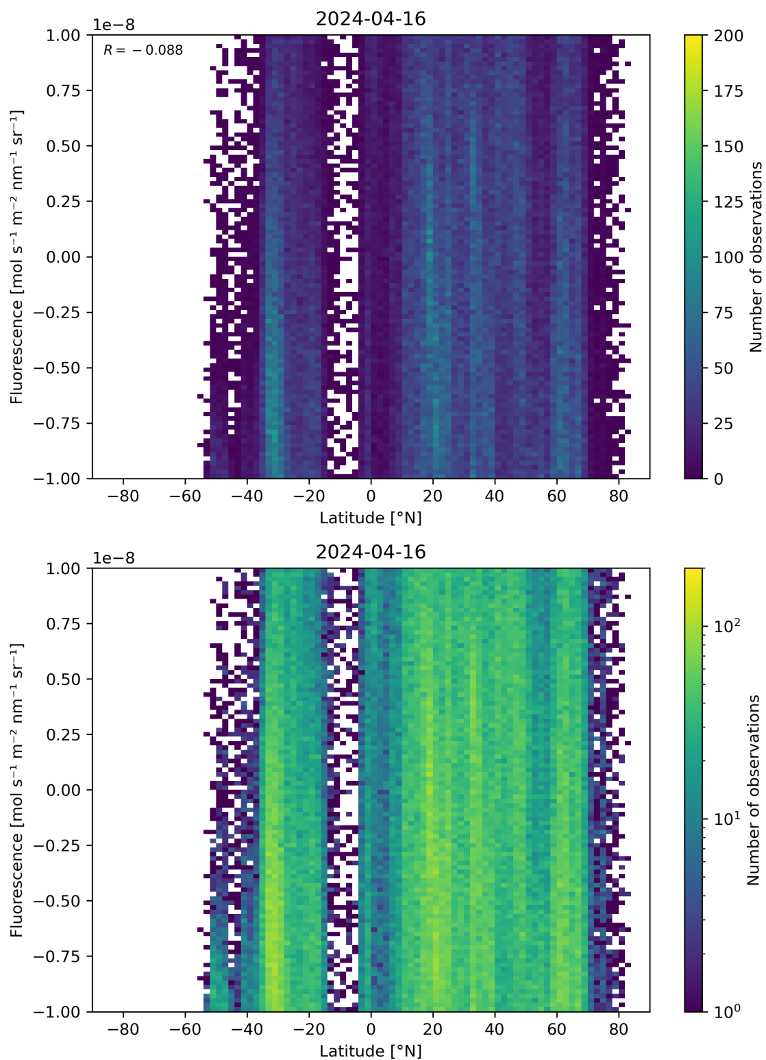
Figure 56: Scatter density plot of “Latitude” against “Fluorescence” for 2024-04-16 to 2024-04-17.
