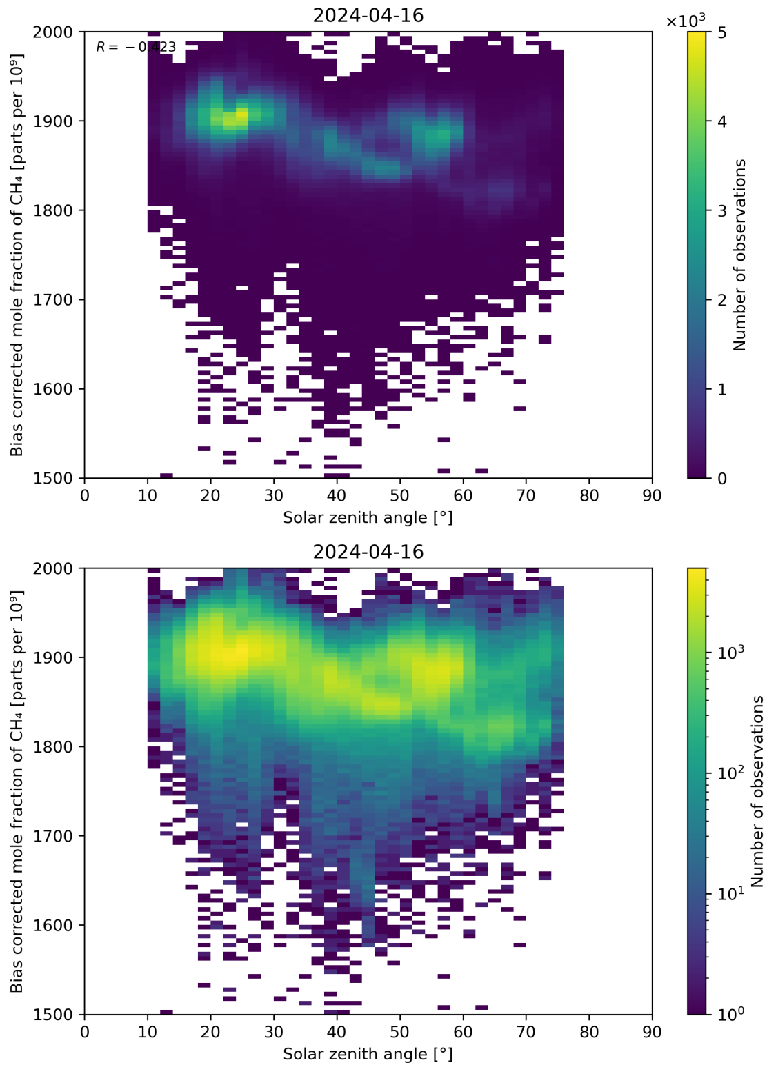
Figure 100: Scatter density plot of “Solar zenith angle” against “Bias corrected mole fraction of CH 4 ” for 2024-04-16 to 2024-04-17.
