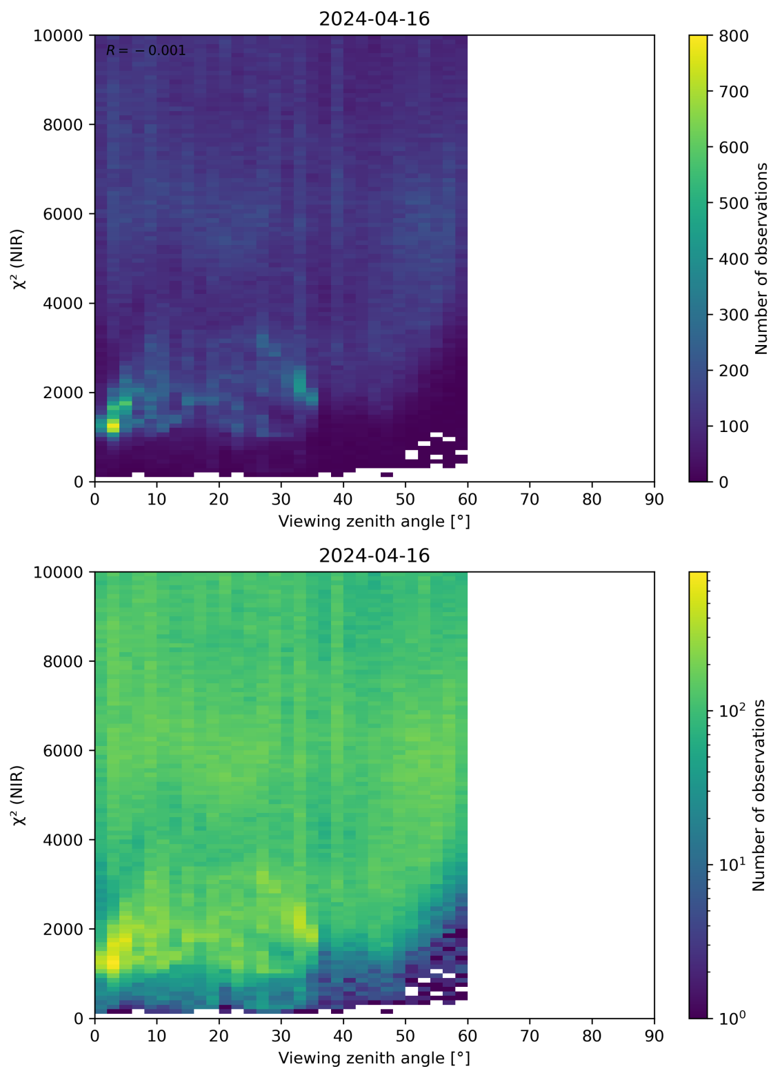
Figure 105: Scatter density plot of “Viewing zenith angle” against “ \chi^2 (NIR)” for 2024-04-16 to 2024-04-17.
