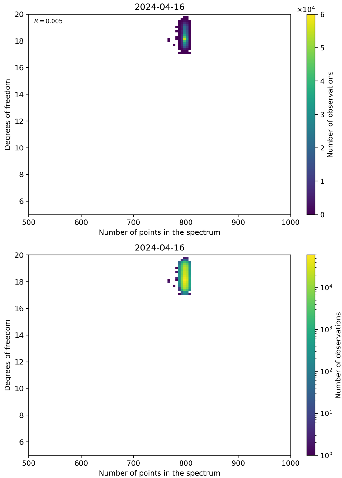
Figure 90: Scatter density plot of “Number of points in the spectrum” against “Degrees of freedom” for 2024-04-16 to 2024-04-17.
