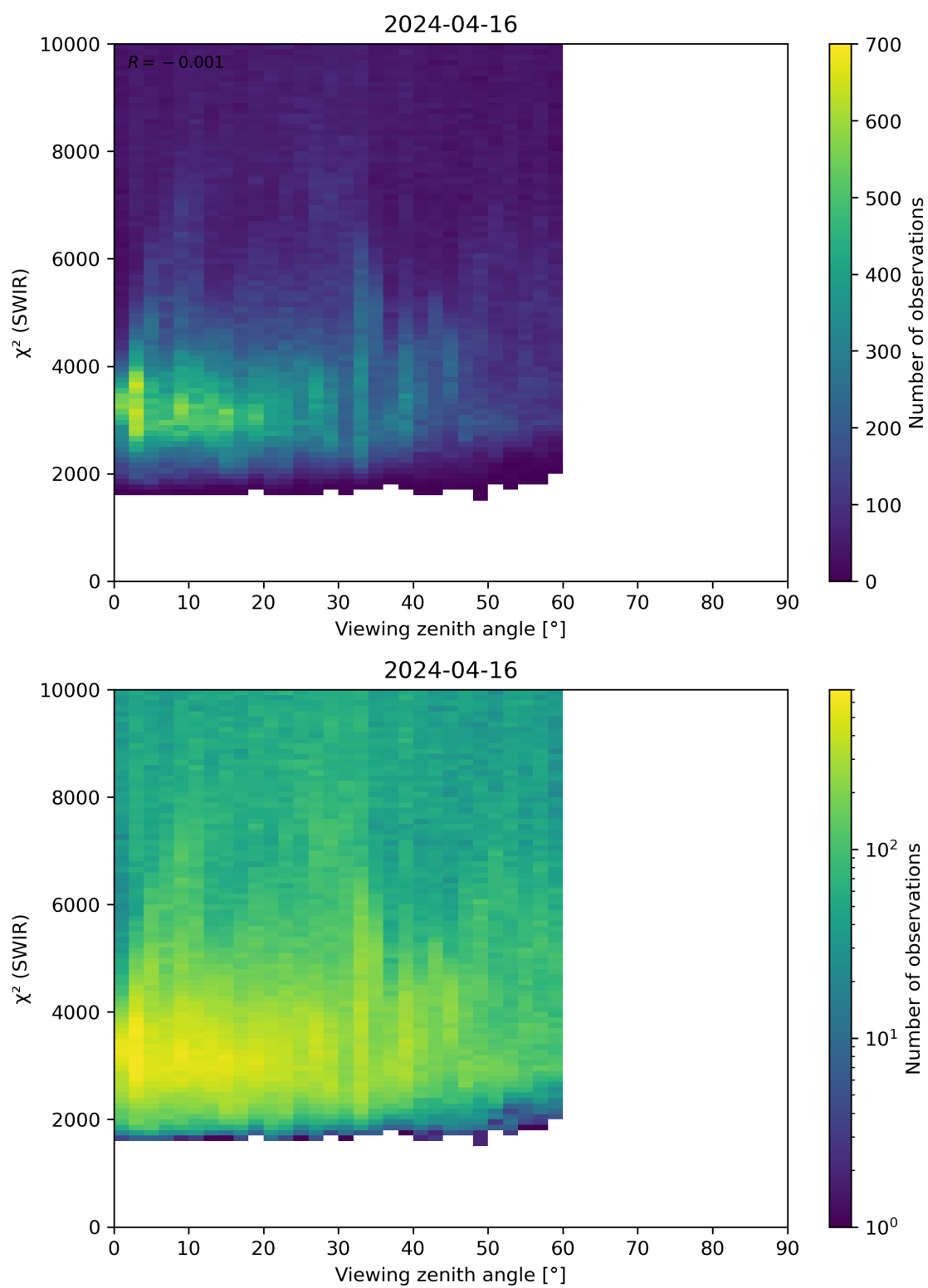
Figure 106: Scatter density plot of “Viewing zenith angle” against “ \chi^2 (SWIR)” for 2024-04-16 to 2024-04-17.
