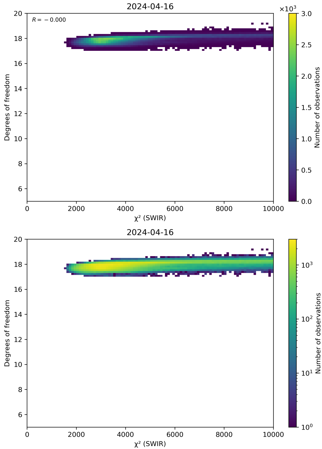
Figure 48: Scatter density plot of “ \chi^2 (SWIR)” against “Degrees of freedom” for 2024-04-16 to 2024-04-17.
