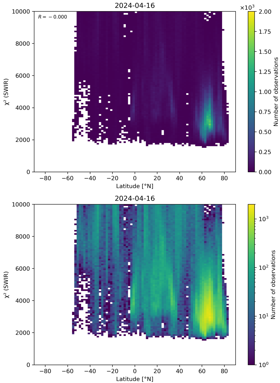
Figure 54: Scatter density plot of “Latitude” against “ \chi^2 (SWIR)” for 2024-04-16 to 2024-04-17.
