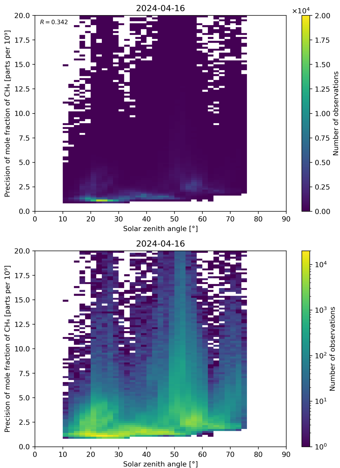
Figure 101: Scatter density plot of “Solar zenith angle” against “Precision of mole fraction of \text{CH}_4 ” for 2024-04-16 to 2024-04-17.
