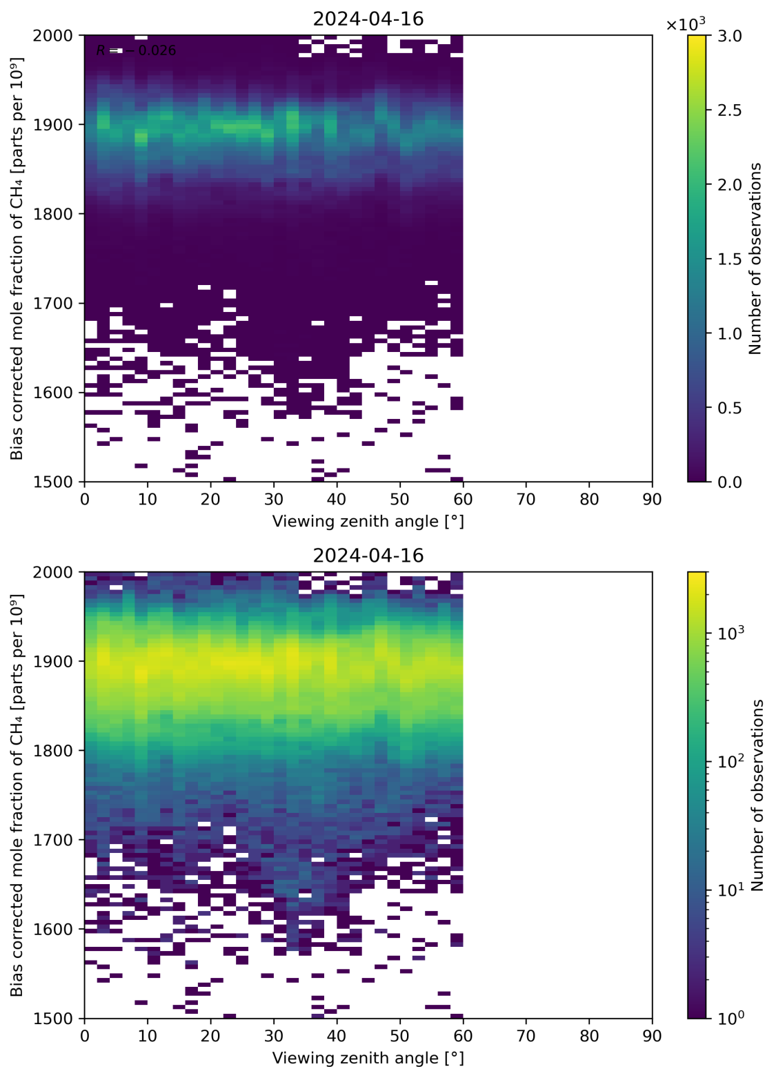
Figure 111: Scatter density plot of “Viewing zenith angle” against “Bias corrected mole fraction of CH 4 ” for 2024-04-16 to 2024-04-17.
