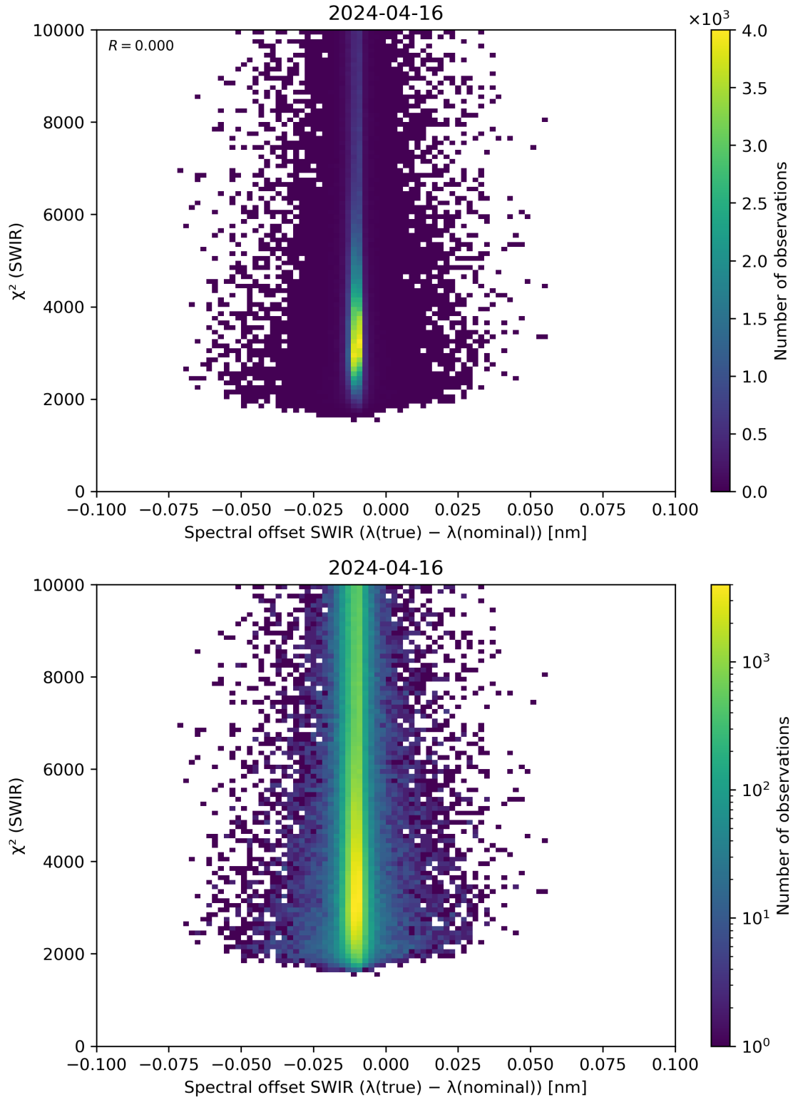
Figure 118: Scatter density plot of “Spectral offset SWIR ( \lambda(\text{true}) - \lambda(\text{nominal}) )” against “ \chi^2 (SWIR)” for 2024-04-16 to 2024-04-17.
