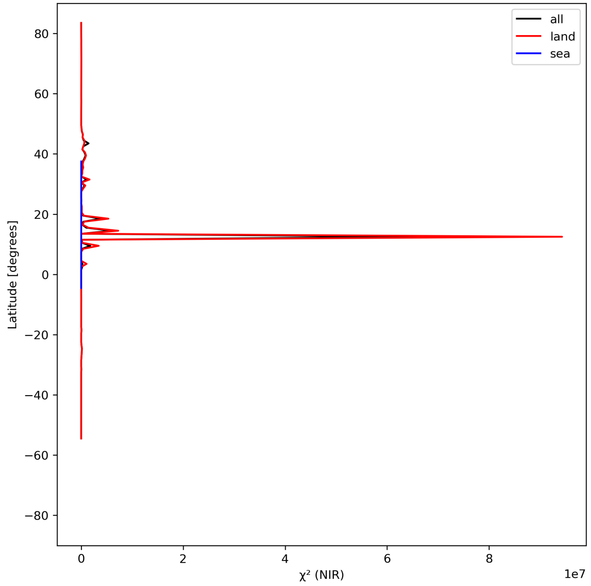
Figure 18: Zonal average of “ \chi^2 (NIR)” for 2024-04-16 to 2024-04-17.
