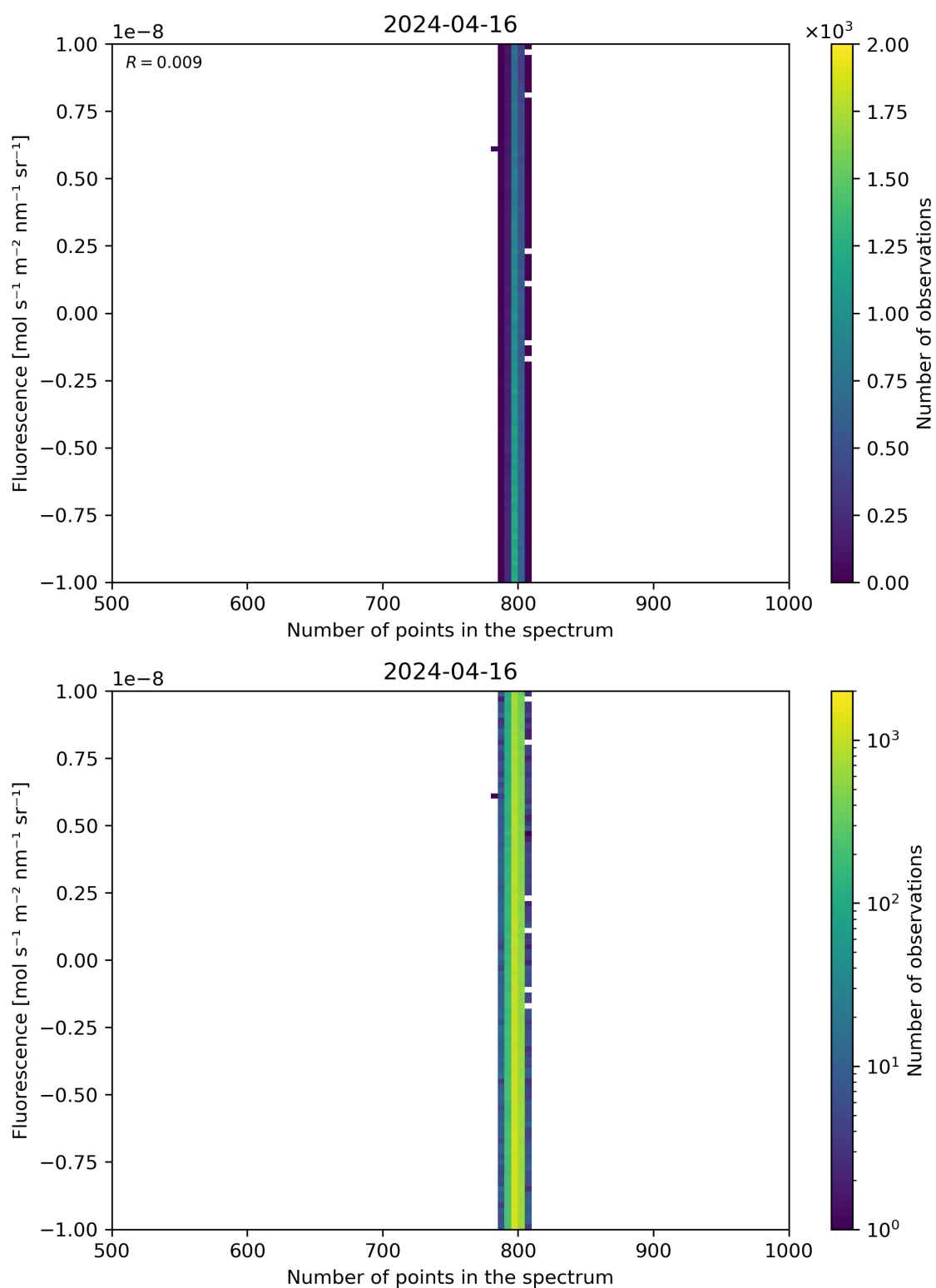
Figure 91: Scatter density plot of “Number of points in the spectrum” against “Fluorescence” for 2024-04-16 to 2024-04-17.
