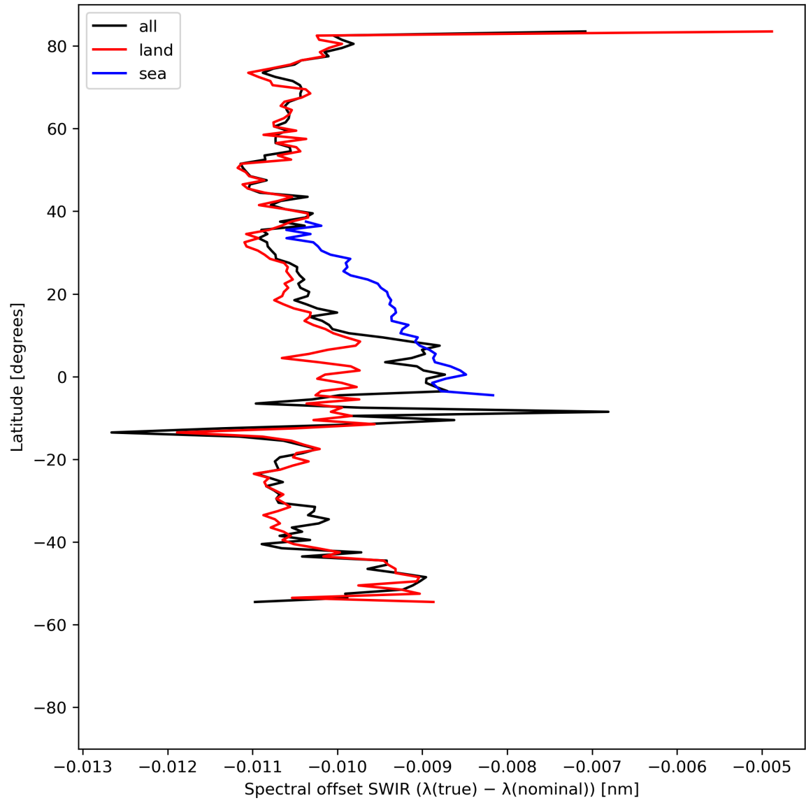
Figure 16: Zonal average of “Spectral offset SWIR ( \lambda(\text{true}) - \lambda(\text{nominal}) )” for 2024-04-16 to 2024-04-17.
