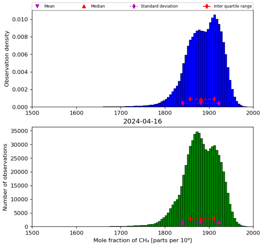
Figure 23: Histogram of “Mole fraction of CH 4 ” for 2024-04-16 to 2024-04-17
