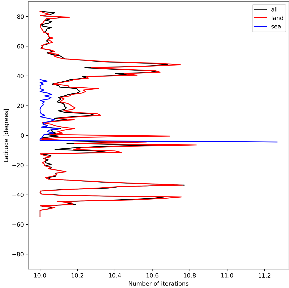
Figure 20: Zonal average of “Number of iterations” for 2024-04-16 to 2024-04-17.
