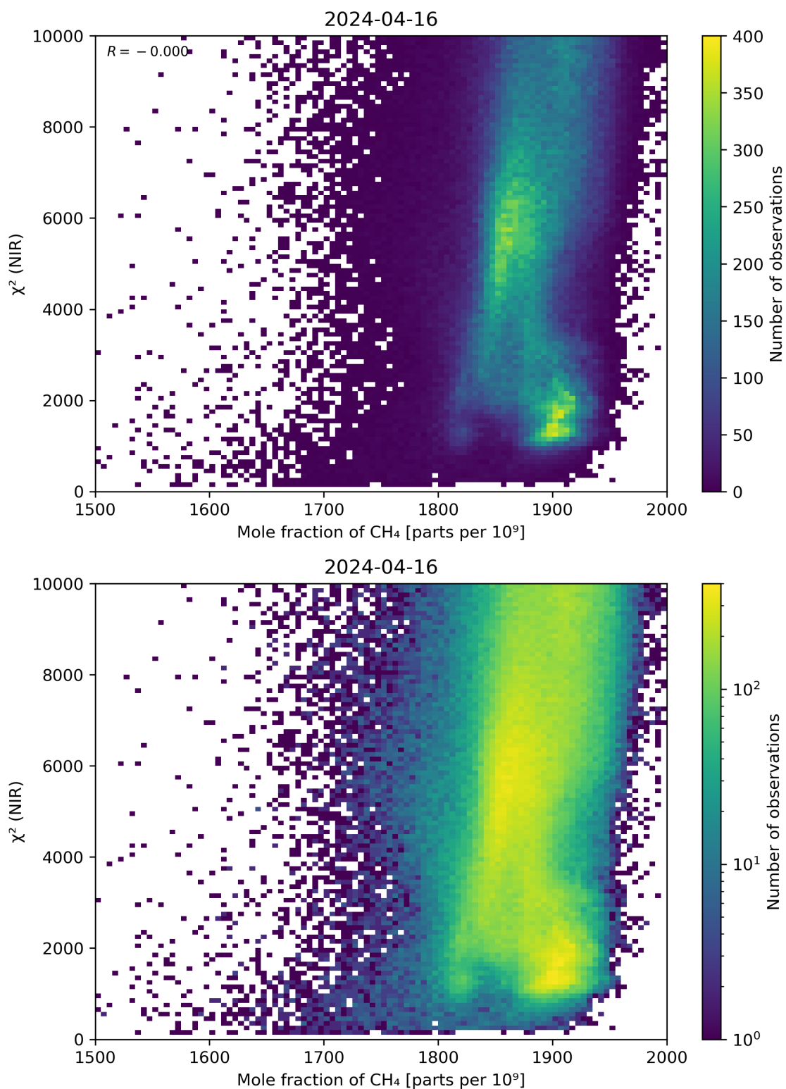
Figure 70: Scatter density plot of “Mole fraction of CH 4 ” against “ \chi^2 (NIR)” for 2024-04-16 to 2024-04-17.
