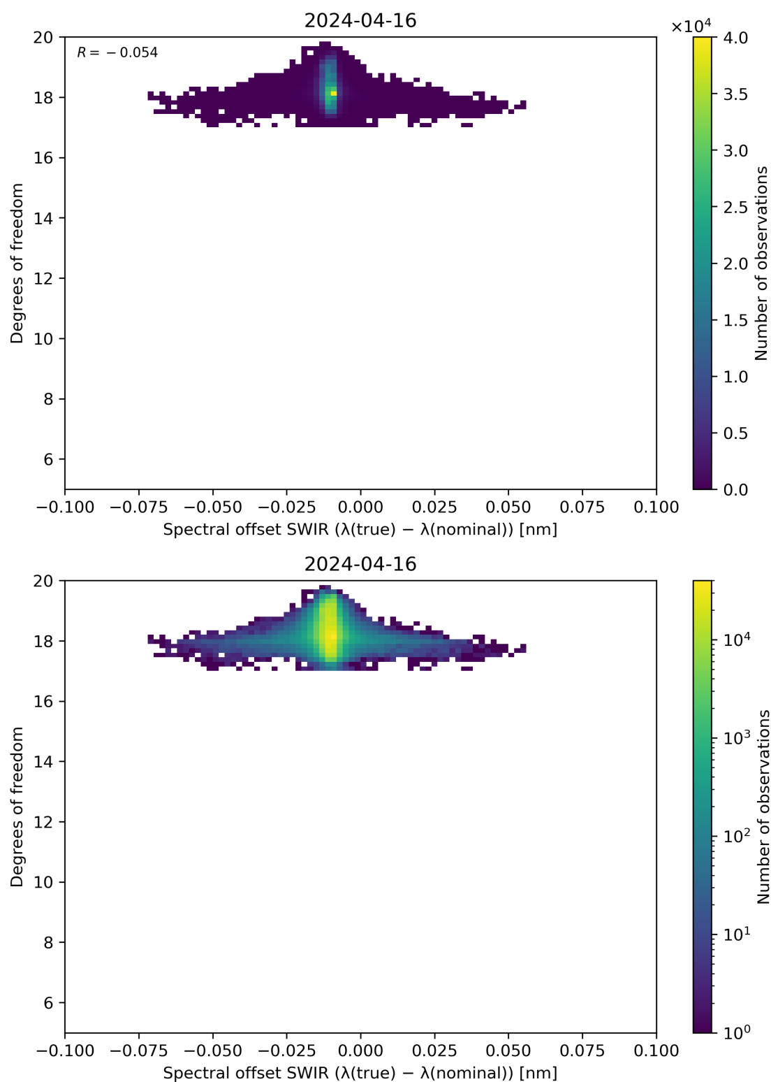
Figure 119: Scatter density plot of “Spectral offset SWIR ( \lambda(\text{true}) - \lambda(\text{nominal}) )” against “Degrees of freedom” for 2024-04-16 to 2024-04-17.
