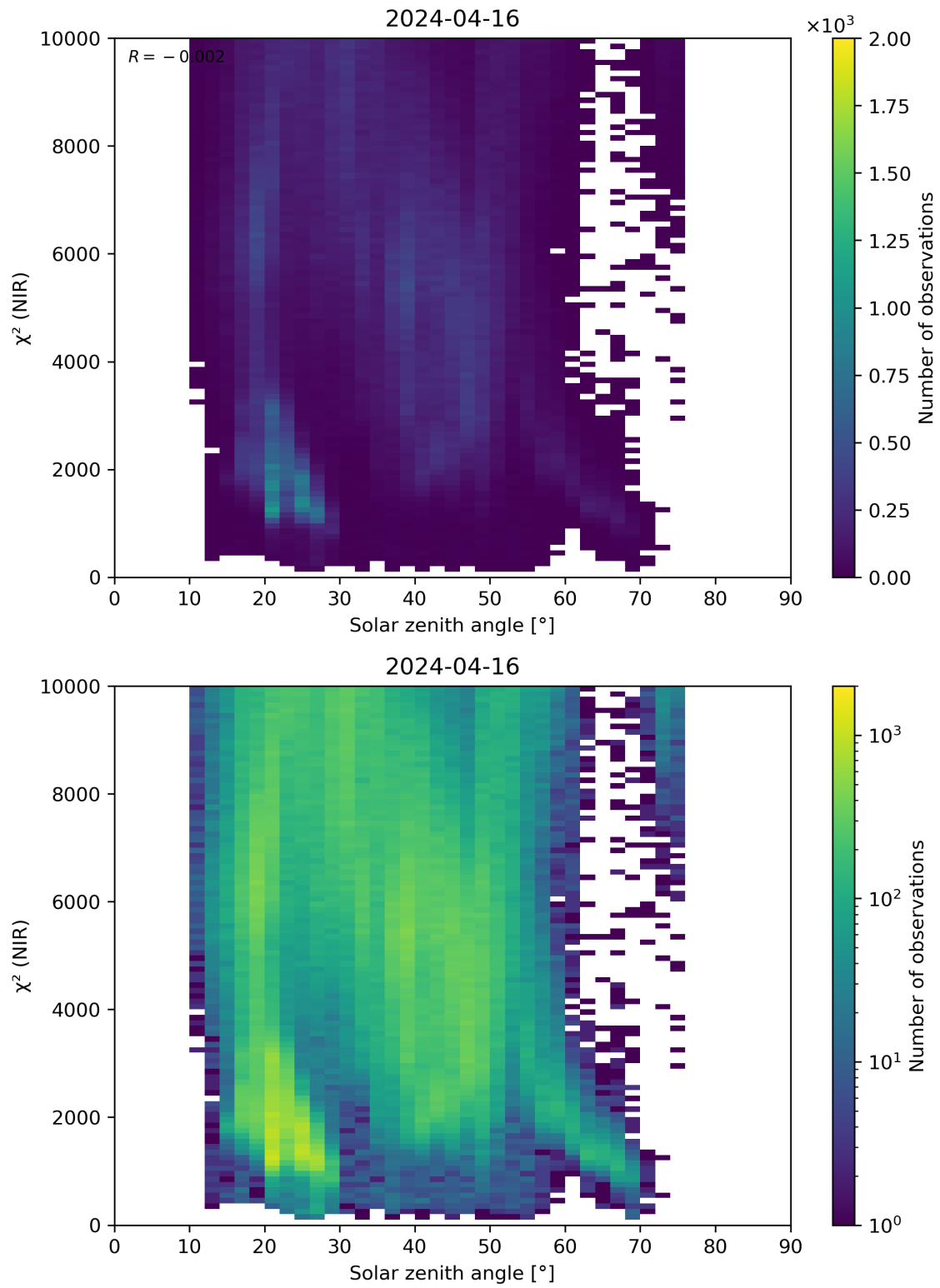
Figure 94: Scatter density plot of “Solar zenith angle” against “ \chi^2 (NIR)” for 2024-04-16 to 2024-04-17.
