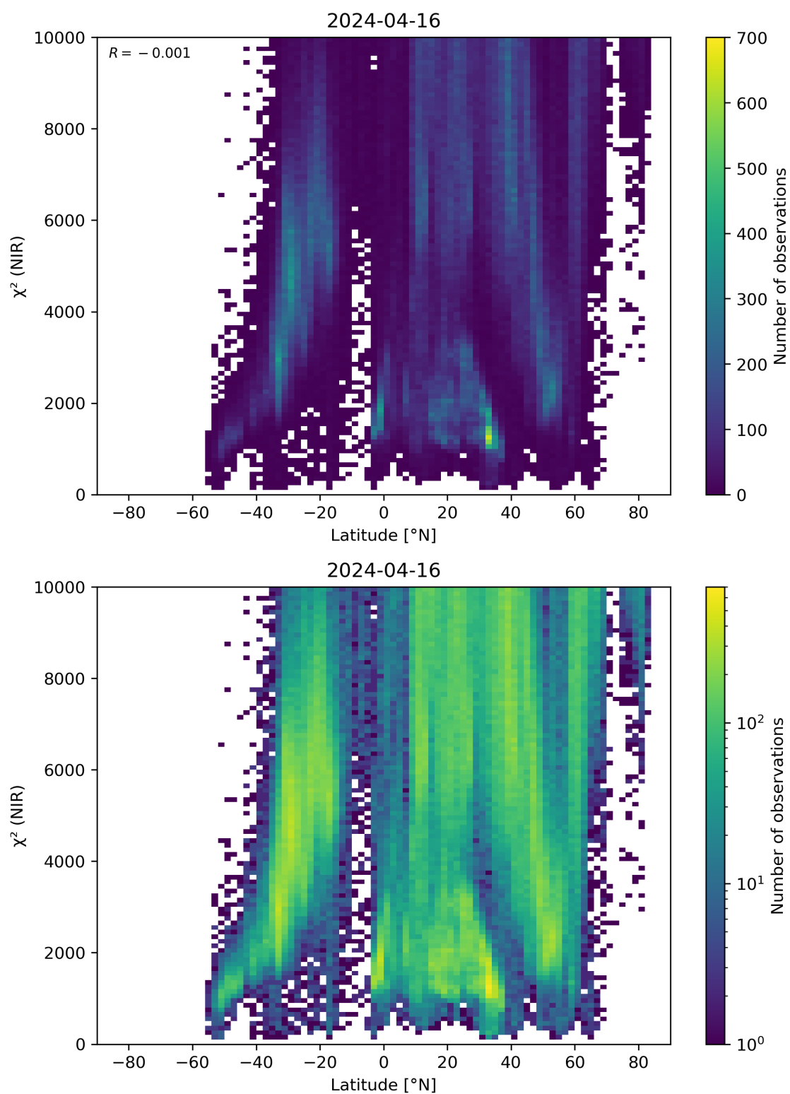
Figure 53: Scatter density plot of “Latitude” against “ \chi^2 (NIR)” for 2024-04-16 to 2024-04-17.
