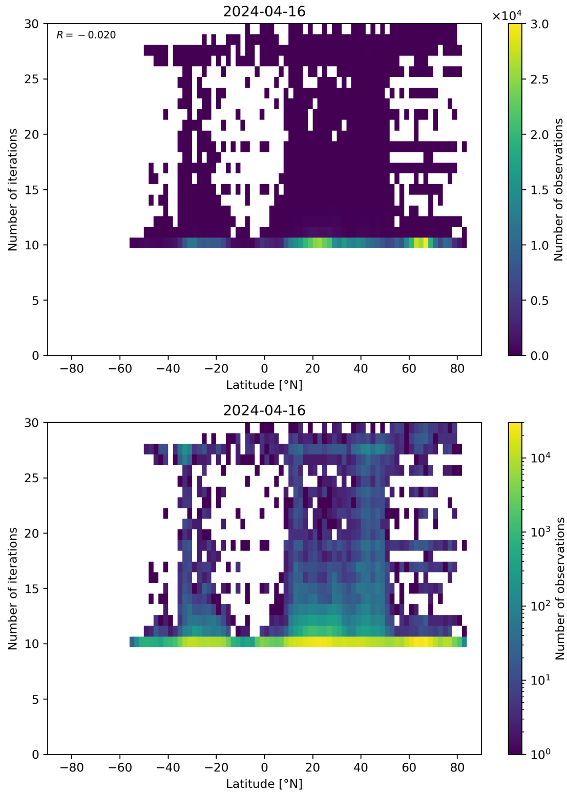
Figure 60: Scatter density plot of “Latitude” against “Number of iterations” for 2024-04-16 to 2024-04-17.
