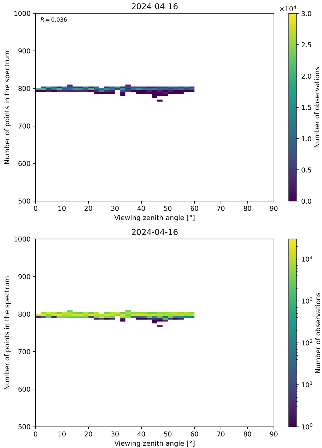
Figure 114: Scatter density plot of “Viewing zenith angle” against “Number of points in the spectrum” for 2024-04-16 to 2024-04-17.
