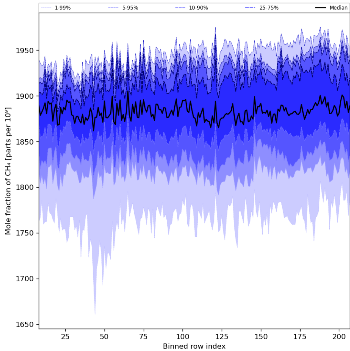
Figure 34: Along track statistics of “Mole fraction of CH 4 ” for 2024-04-16 to 2024-04-17
