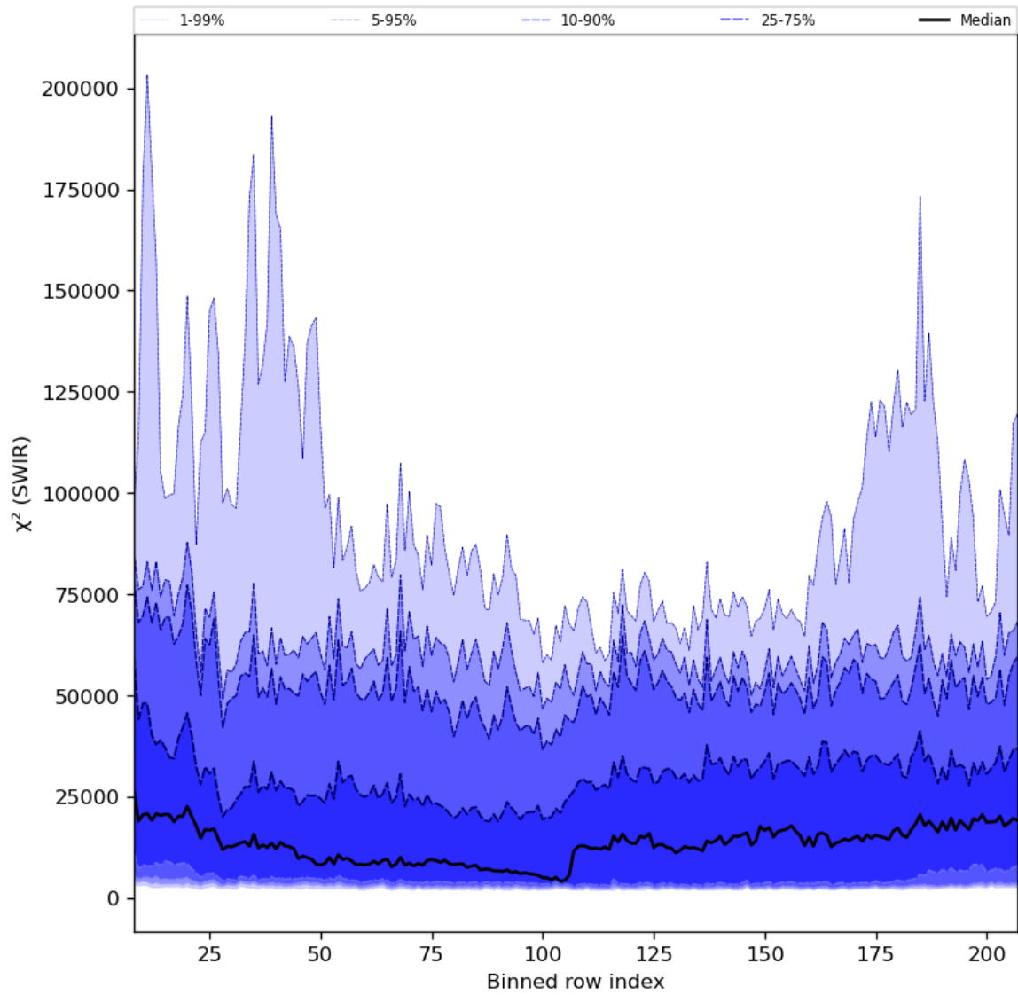
Figure 39: Along track statistics of “ \chi^2 (SWIR)” for 2024-04-16 to 2024-04-17
