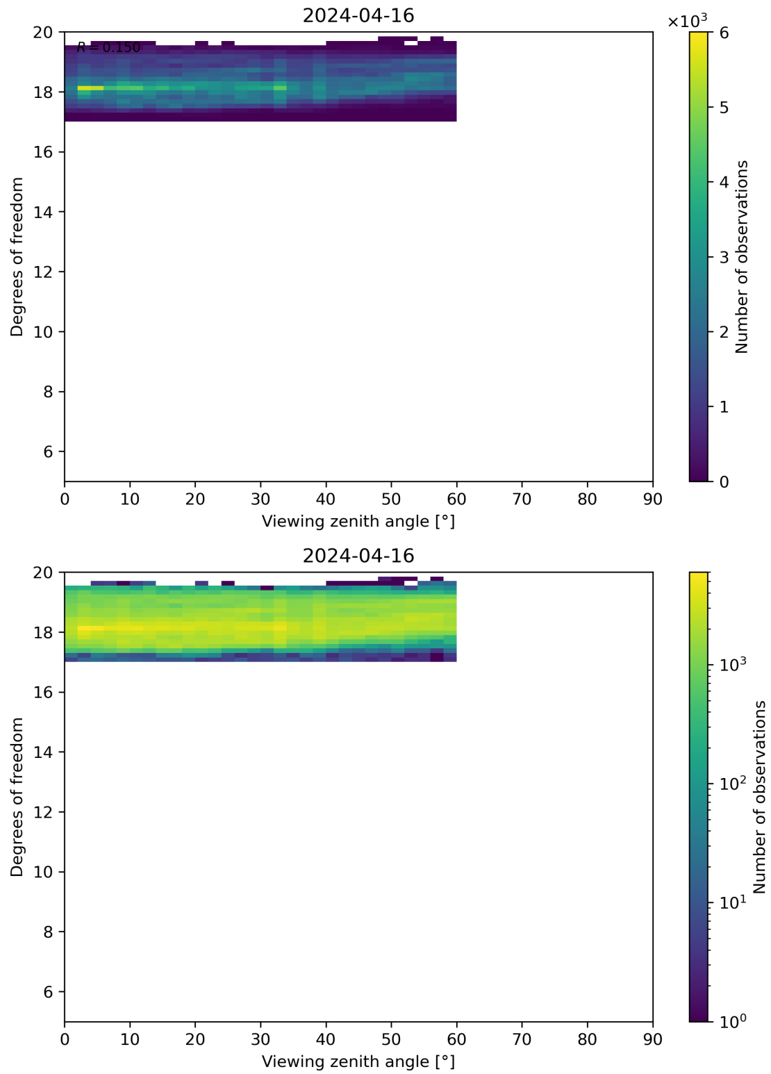
Figure 107: Scatter density plot of “Viewing zenith angle” against “Degrees of freedom” for 2024-04-16 to 2024-04-17.
