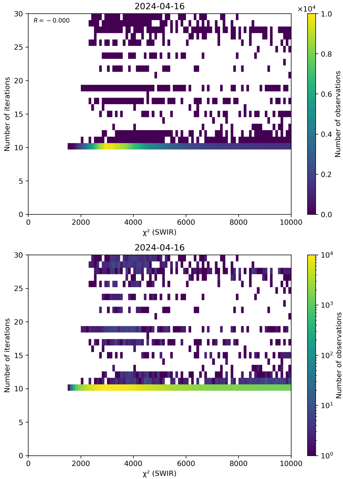
Figure 50: Scatter density plot of “ \chi^2 (SWIR)” against “Number of iterations” for 2024-04-16 to 2024-04-17.
