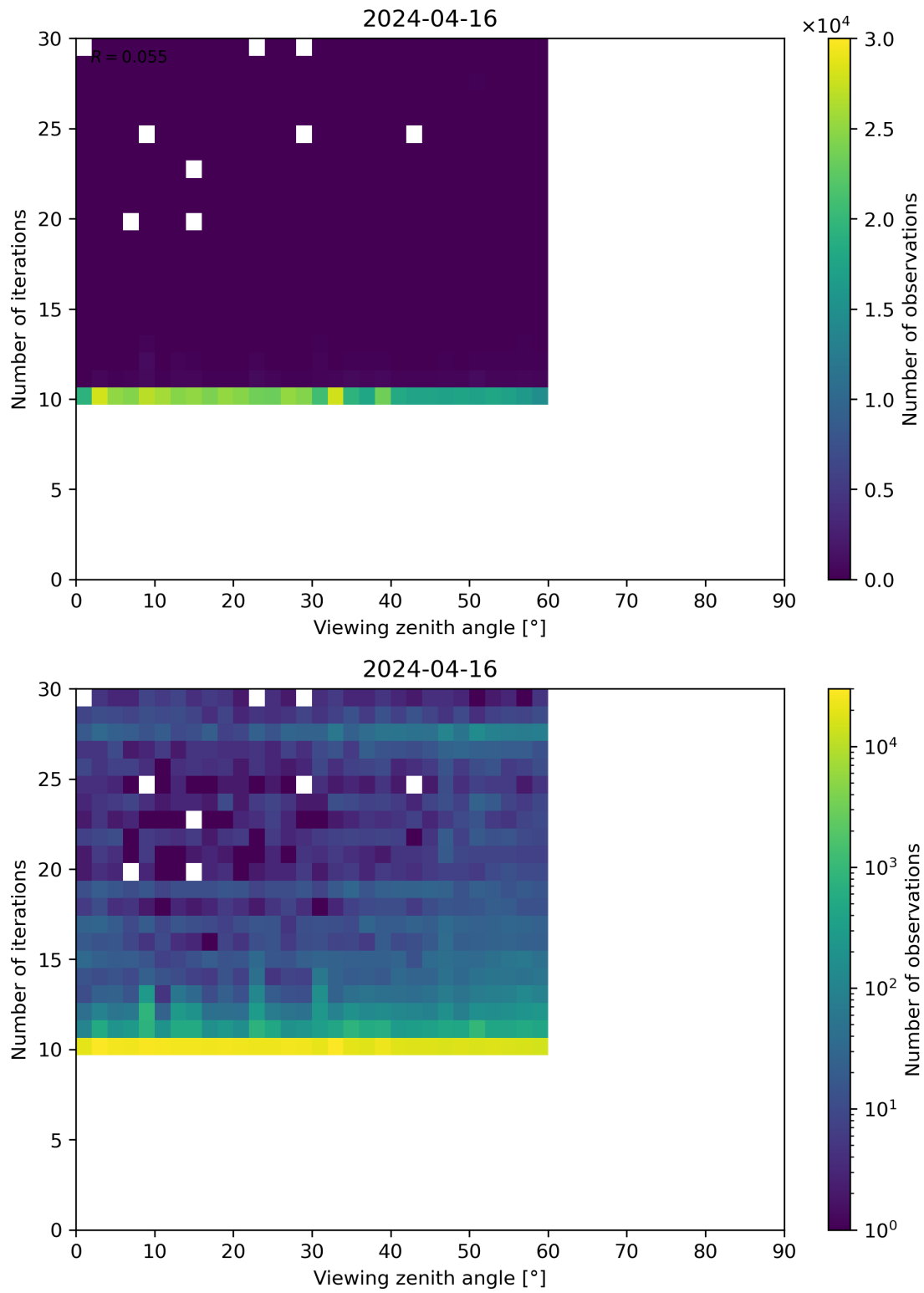
Figure 113: Scatter density plot of “Viewing zenith angle” against “Number of iterations” for 2024-04-16 to 2024-04-17.
