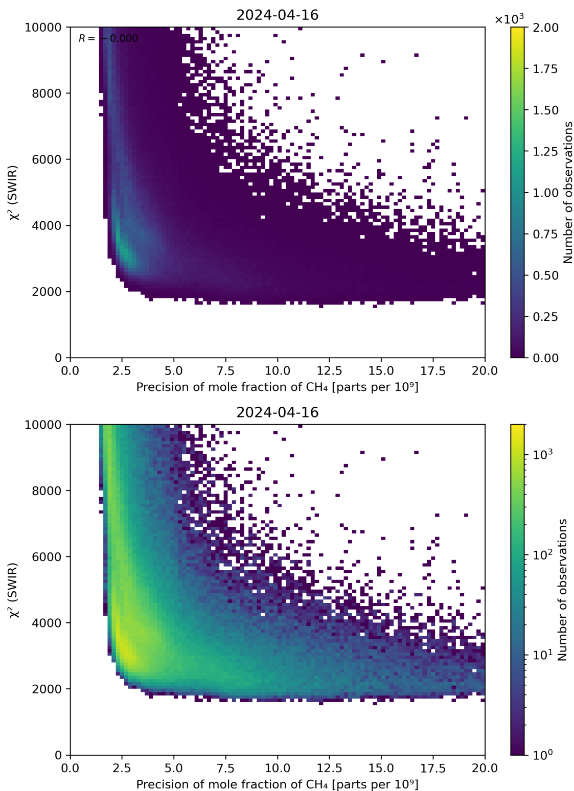
Figure 79: Scatter density plot of “Precision of mole fraction of CH 4 ” against “ \chi^2 (SWIR)” for 2024-04-16 to 2024-04-17.
