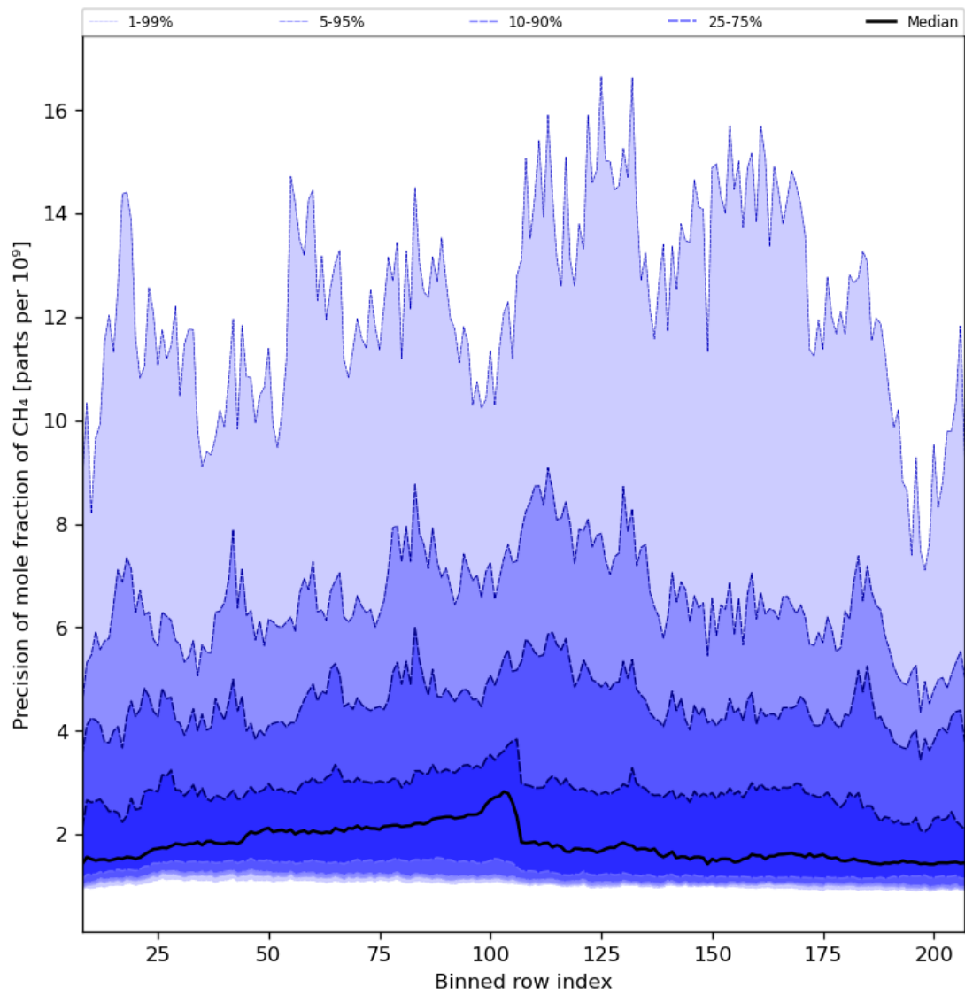
Figure 35: Along track statistics of “Precision of mole fraction of CH 4 ” for 2024-04-16 to 2024-04-17
