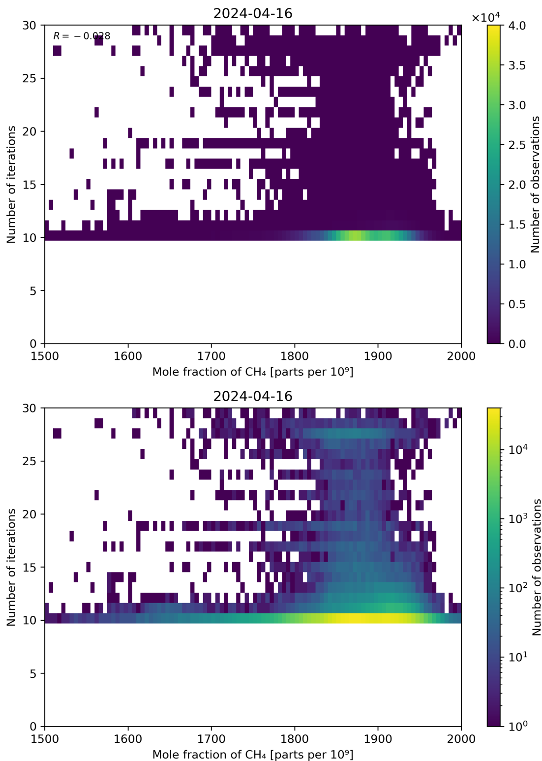
Figure 76: Scatter density plot of “Mole fraction of CH 4 ” against “Number of iterations” for 2024-04-16 to 2024-04-17.
