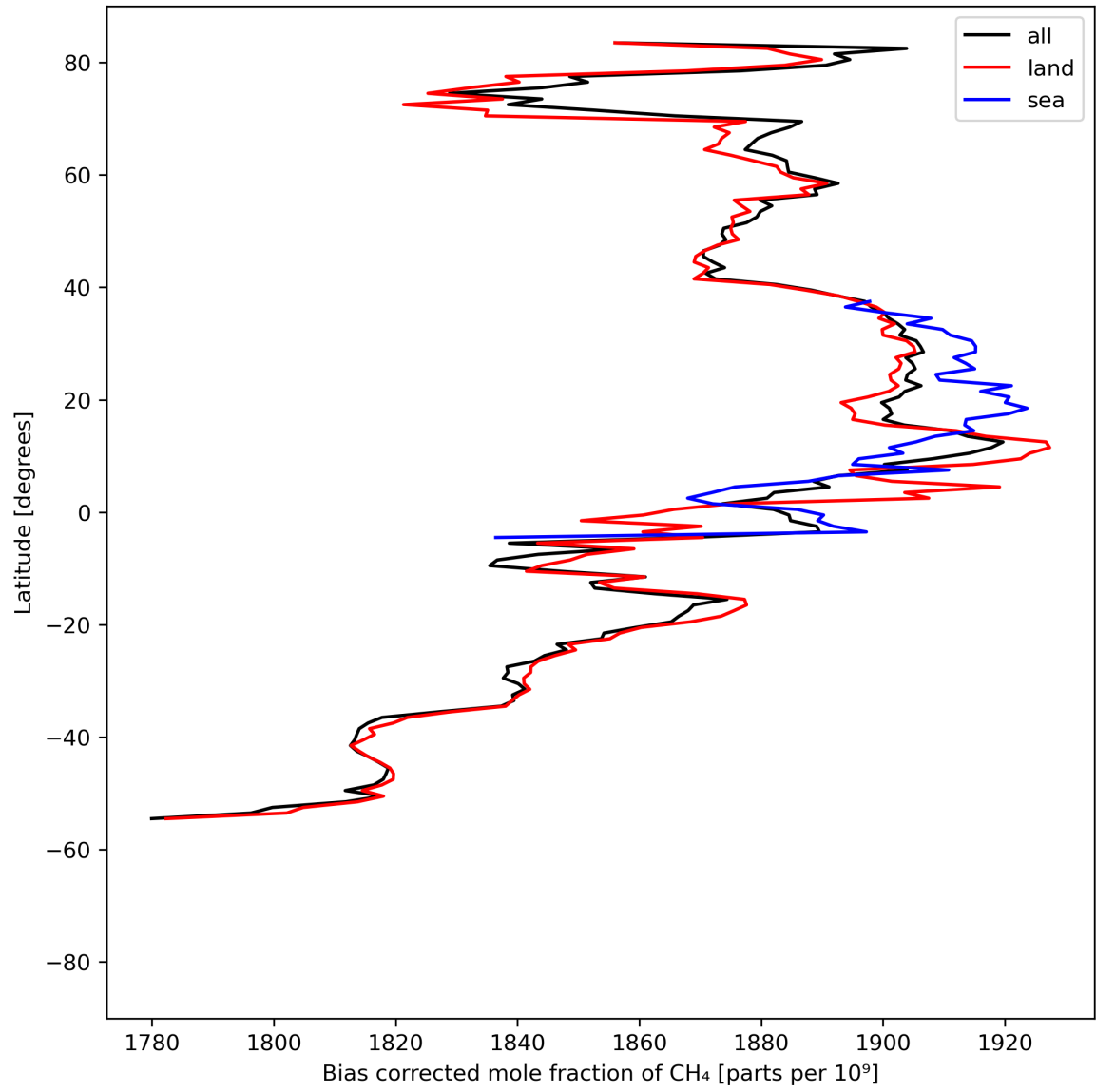
Figure 14: Zonal average of “Bias corrected mole fraction of \text{CH}_4 ” for 2024-04-16 to 2024-04-17.
