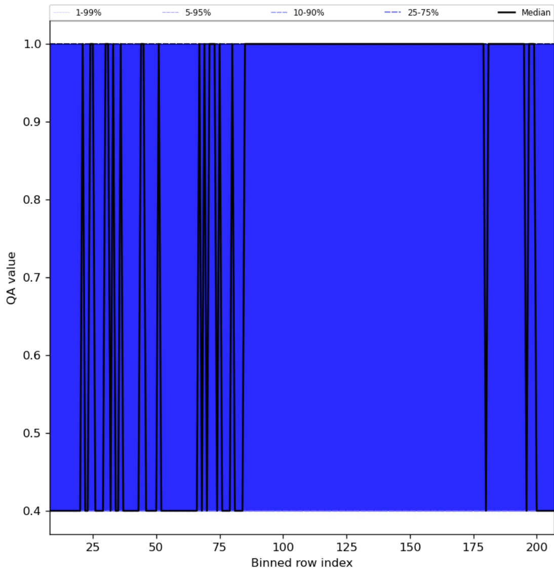
Figure 33: Along track statistics of “QA value” for 2024-04-16 to 2024-04-17
