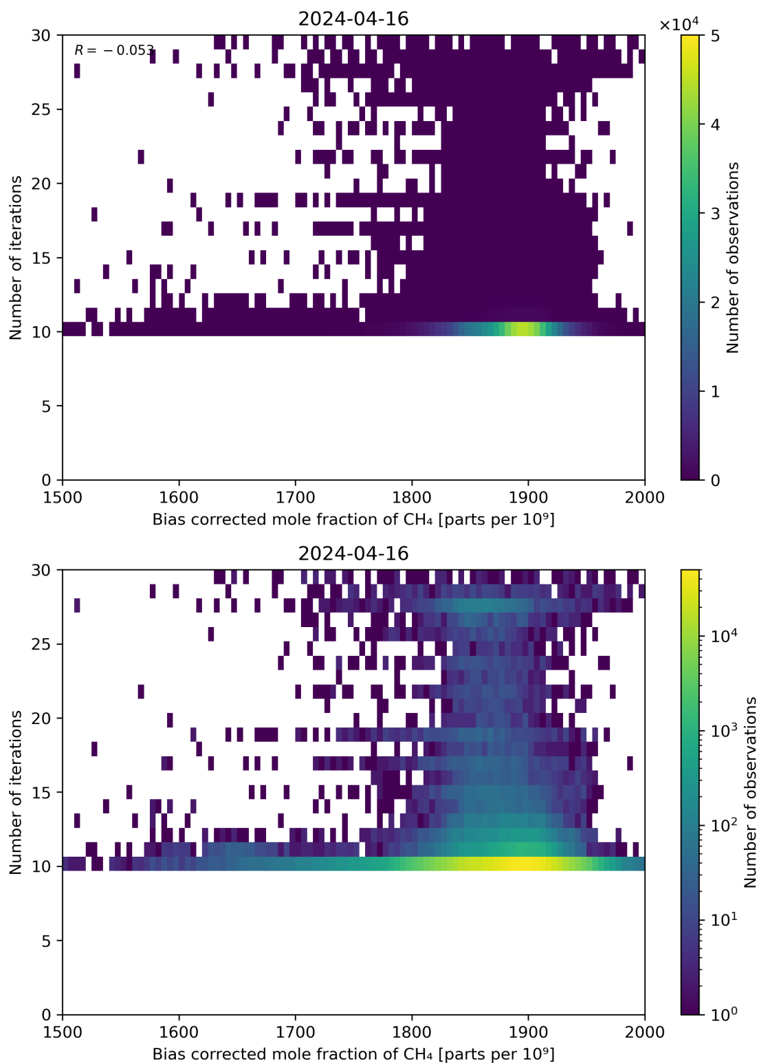
Figure 67: Scatter density plot of “Bias corrected mole fraction of \text{CH}_4 ” against “Number of iterations” for 2024-04-16 to 2024-04-17.
