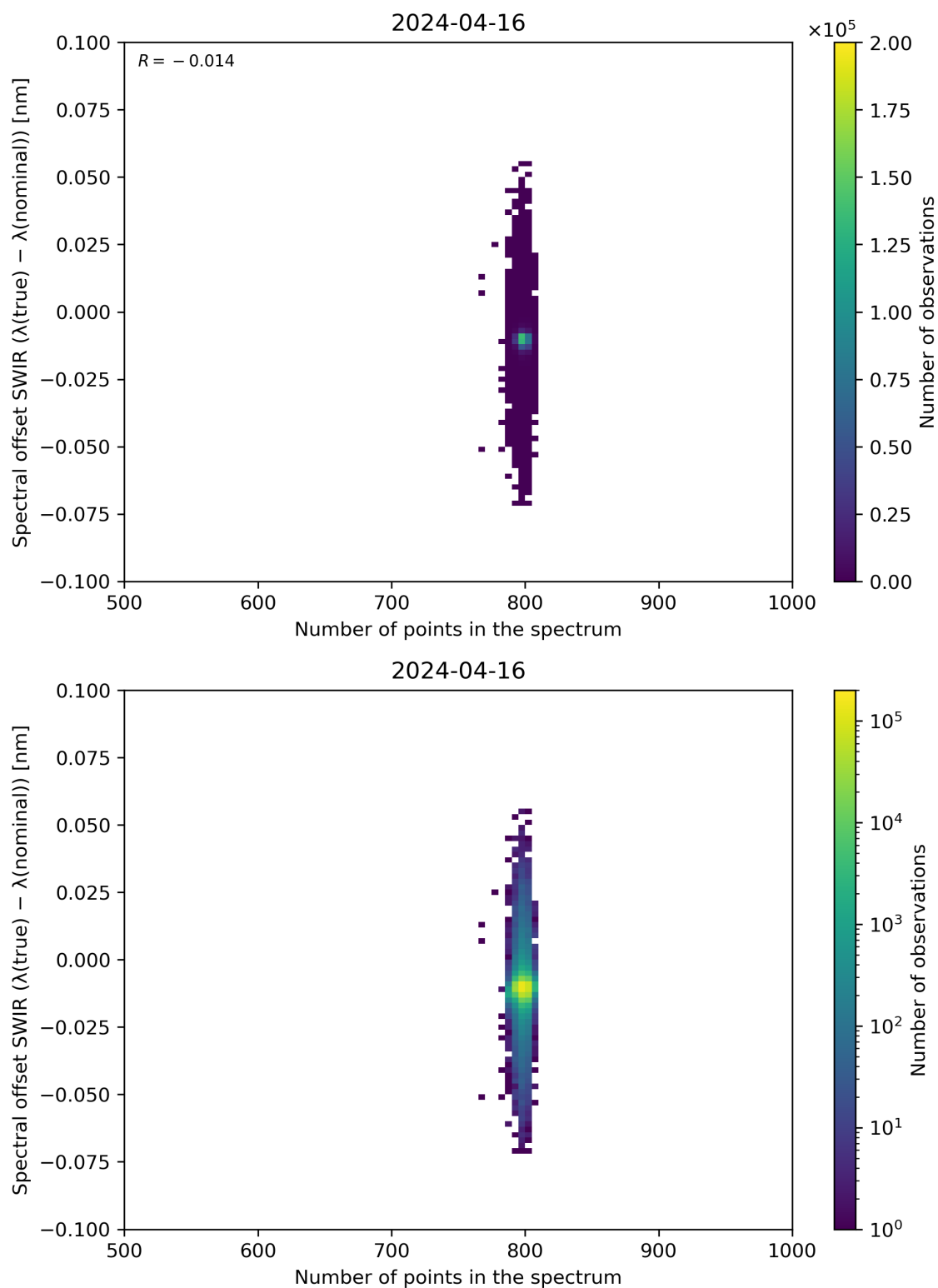
Figure 93: Scatter density plot of “Number of points in the spectrum” against “Spectral offset SWIR ( \lambda(\text{true}) - \lambda(\text{nominal}) )” for 2024-04-16 to 2024-04-17.
