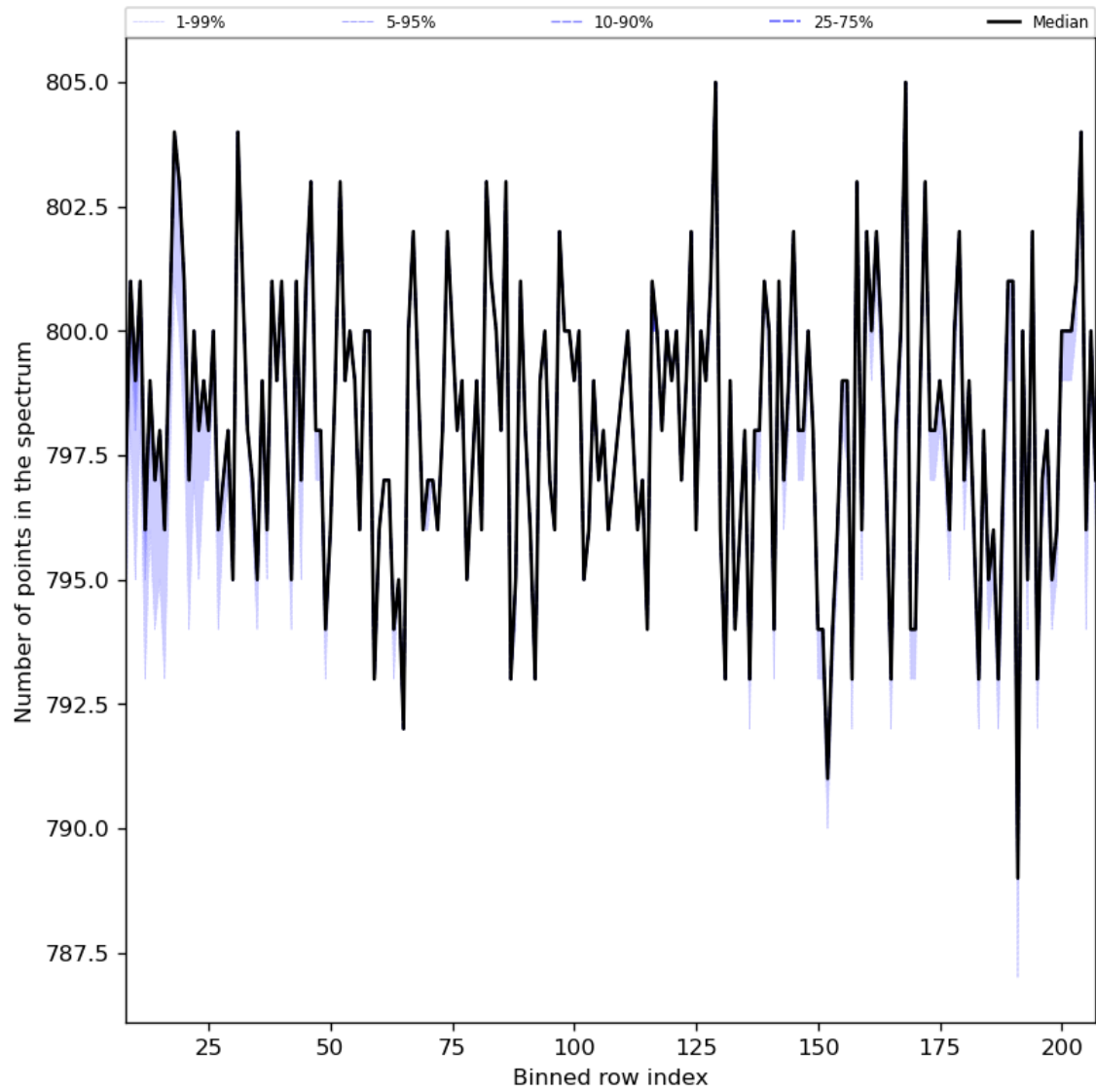
Figure 37: Along track statistics of “Number of points in the spectrum” for 2024-04-16 to 2024-04-17
