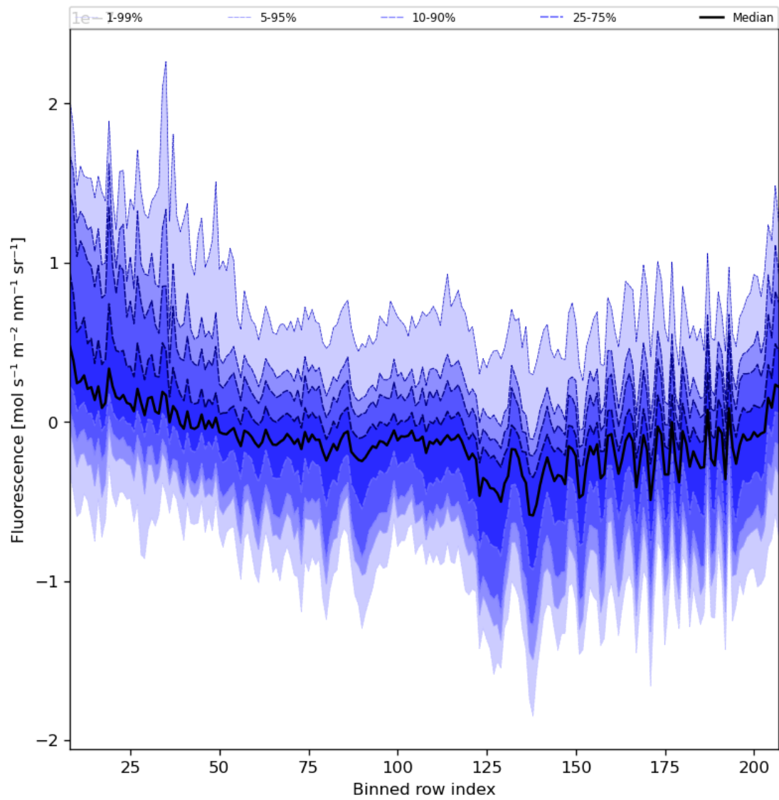
Figure 43: Along track statistics of “Fluorescence” for 2024-04-16 to 2024-04-17
