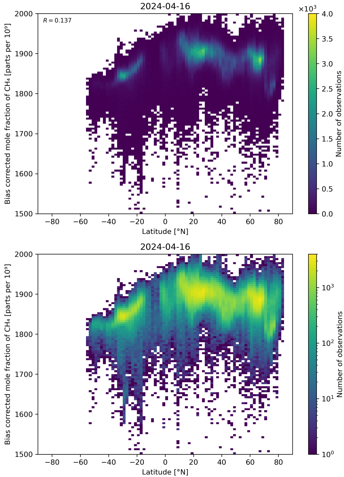
Figure 58: Scatter density plot of “Latitude” against “Bias corrected mole fraction of \text{CH}_4 ” for 2024-04-16 to 2024-04-17.
