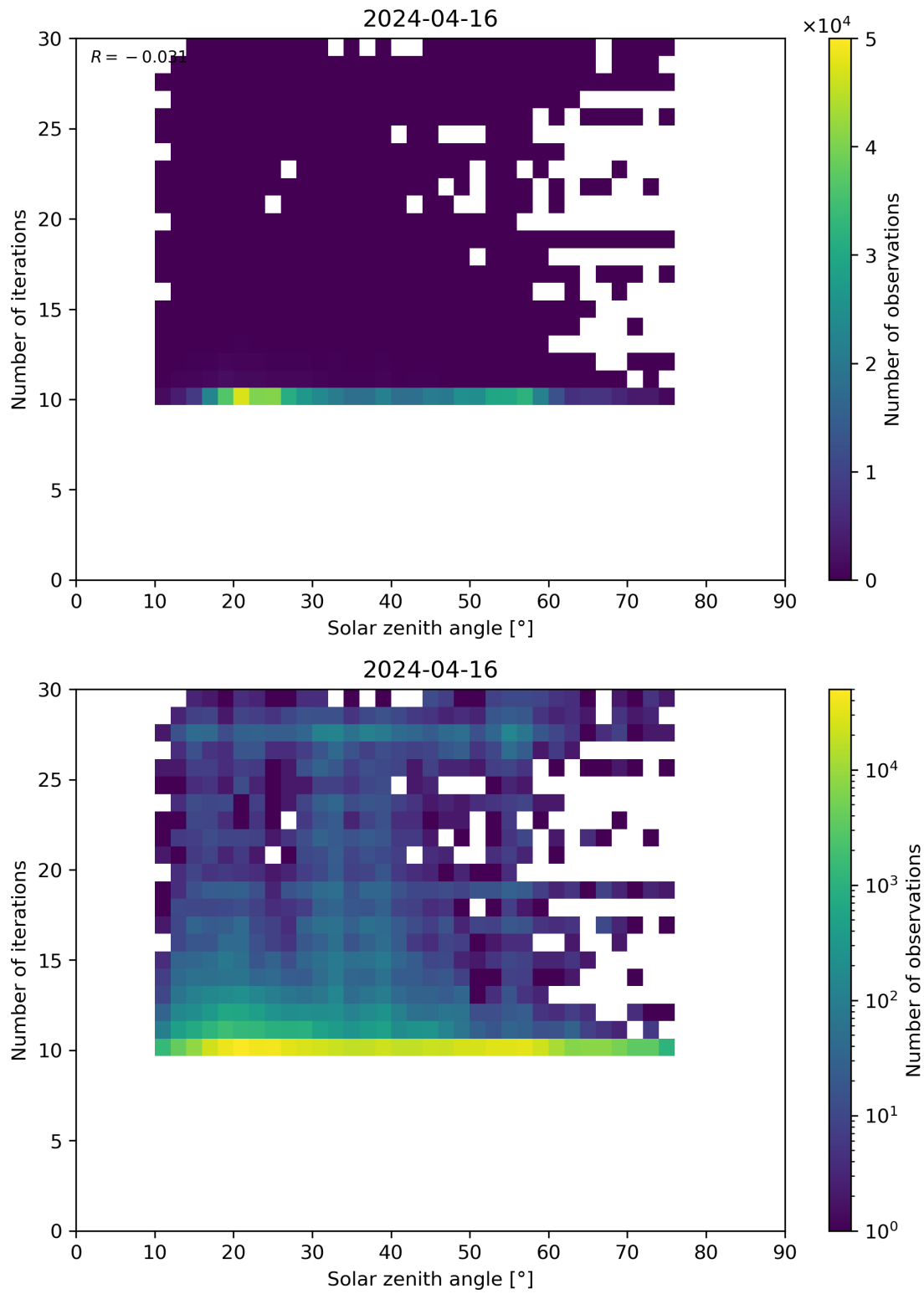
Figure 102: Scatter density plot of “Solar zenith angle” against “Number of iterations” for 2024-04-16 to 2024-04-17.
