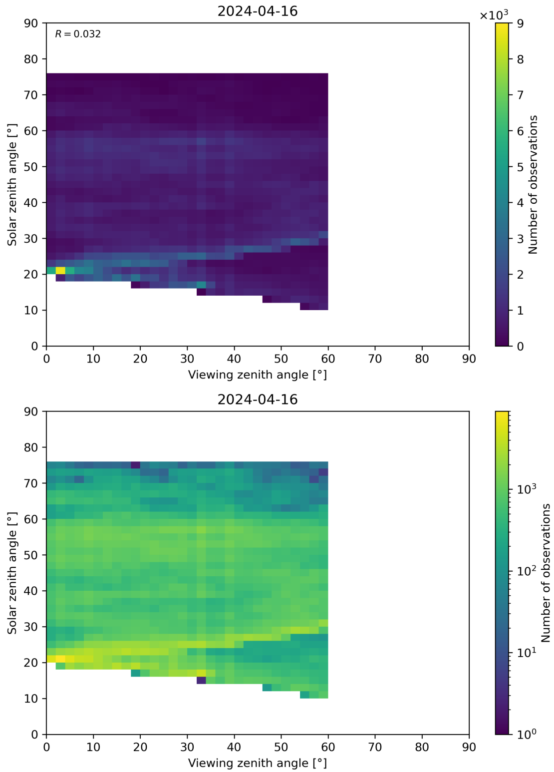
Figure 115: Scatter density plot of “Viewing zenith angle” against “Solar zenith angle” for 2024-04-16 to 2024-04-17.
