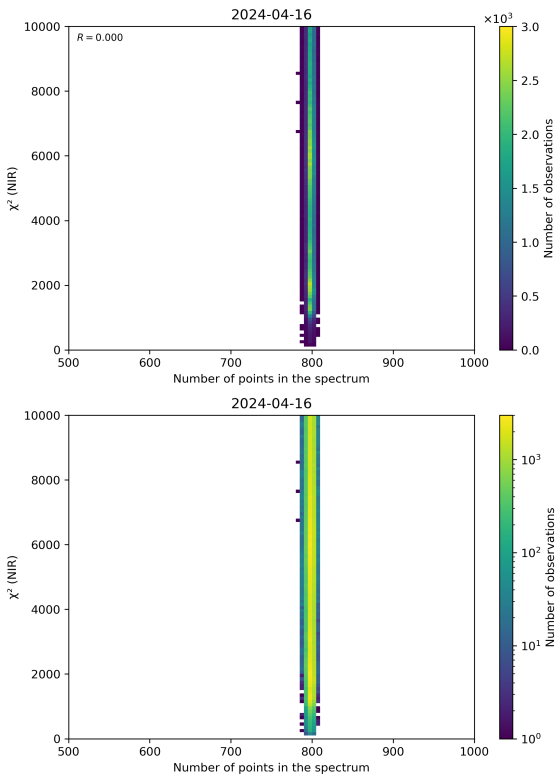
Figure 88: Scatter density plot of “Number of points in the spectrum” against “ \chi^2 (NIR)” for 2024-04-16 to 2024-04-17.
