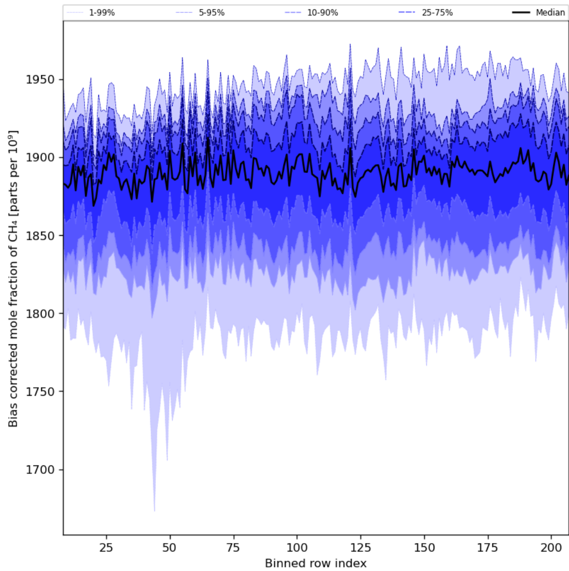
Figure 36: Along track statistics of “Bias corrected mole fraction of CH 4 ” for 2024-04-16 to 2024-04-17
