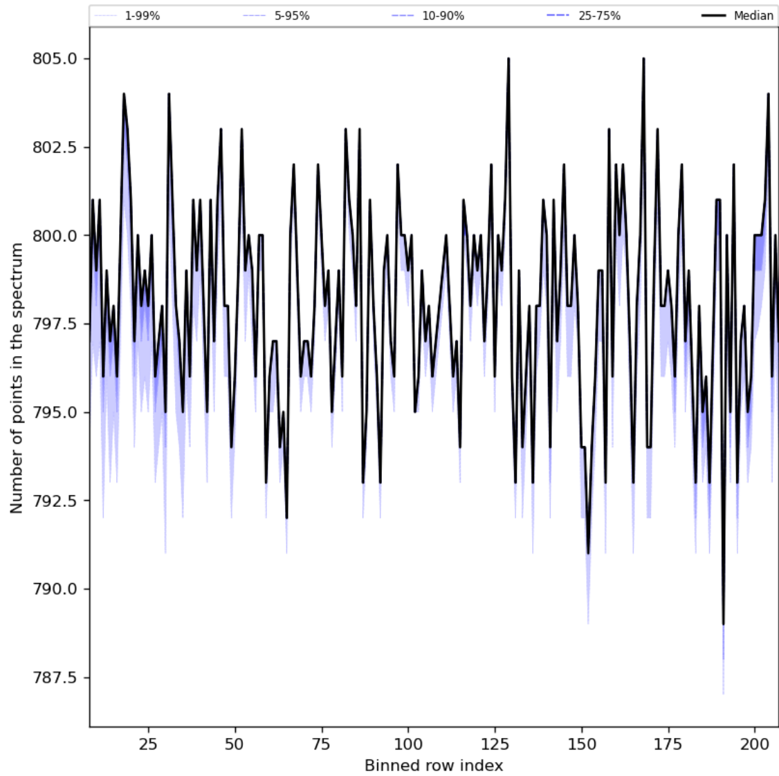
Figure 37: Along track statistics of “Number of points in the spectrum” for 2024-04-16 to 2024-04-18
