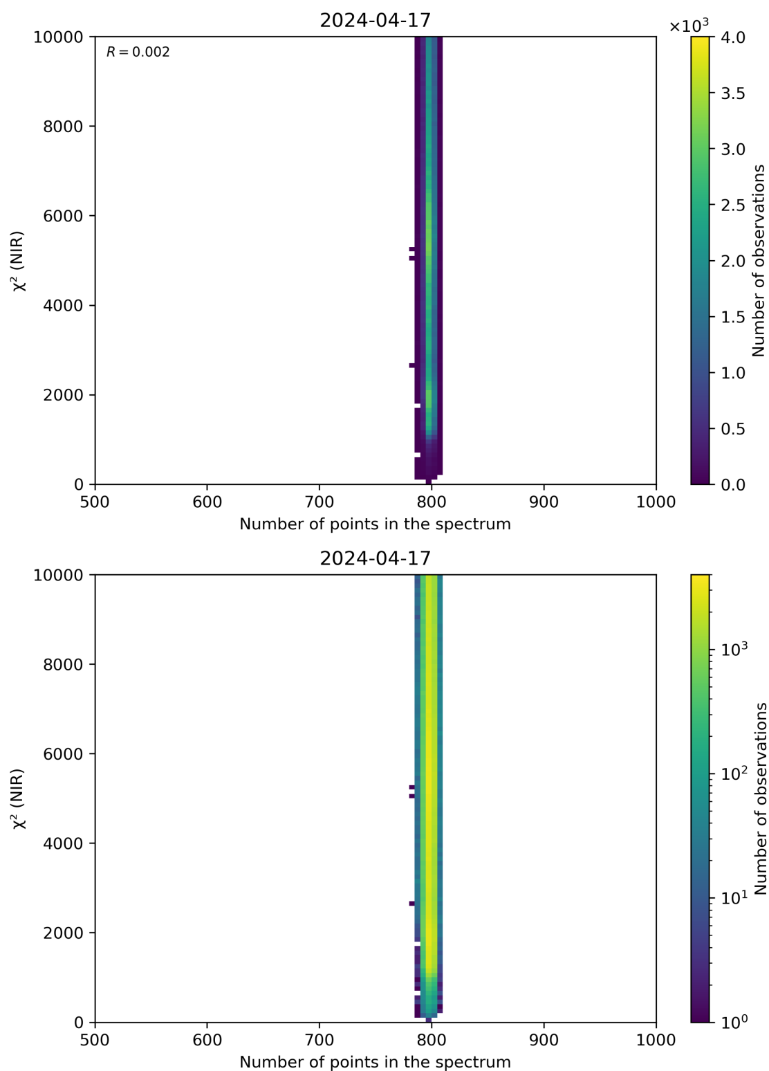
Figure 88: Scatter density plot of “Number of points in the spectrum” against “ \chi^2 (NIR)” for 2024-04-16 to 2024-04-18.
