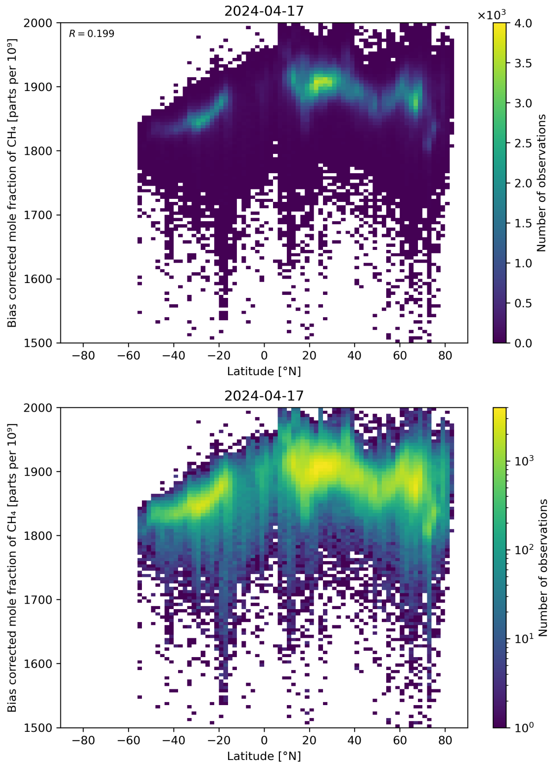
Figure 58: Scatter density plot of “Latitude” against “Bias corrected mole fraction of \text{CH}_4 ” for 2024-04-16 to 2024-04-18.
