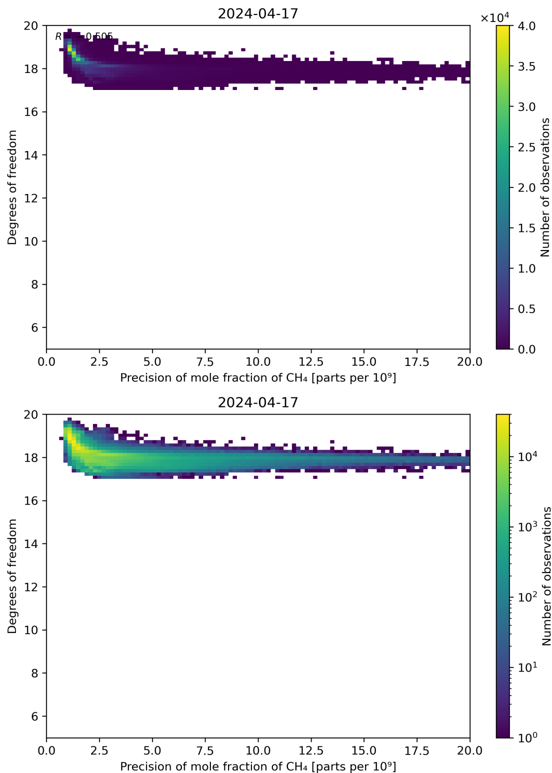
Figure 80: Scatter density plot of “Precision of mole fraction of CH 4 ” against “Degrees of freedom” for 2024-04-16 to 2024-04-18.
