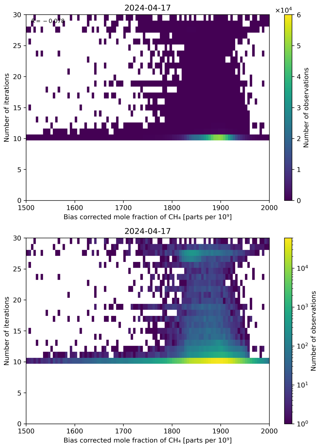
Figure 67: Scatter density plot of “Bias corrected mole fraction of CH 4 ” against “Number of iterations” for 2024-04-16 to 2024-04-18.
