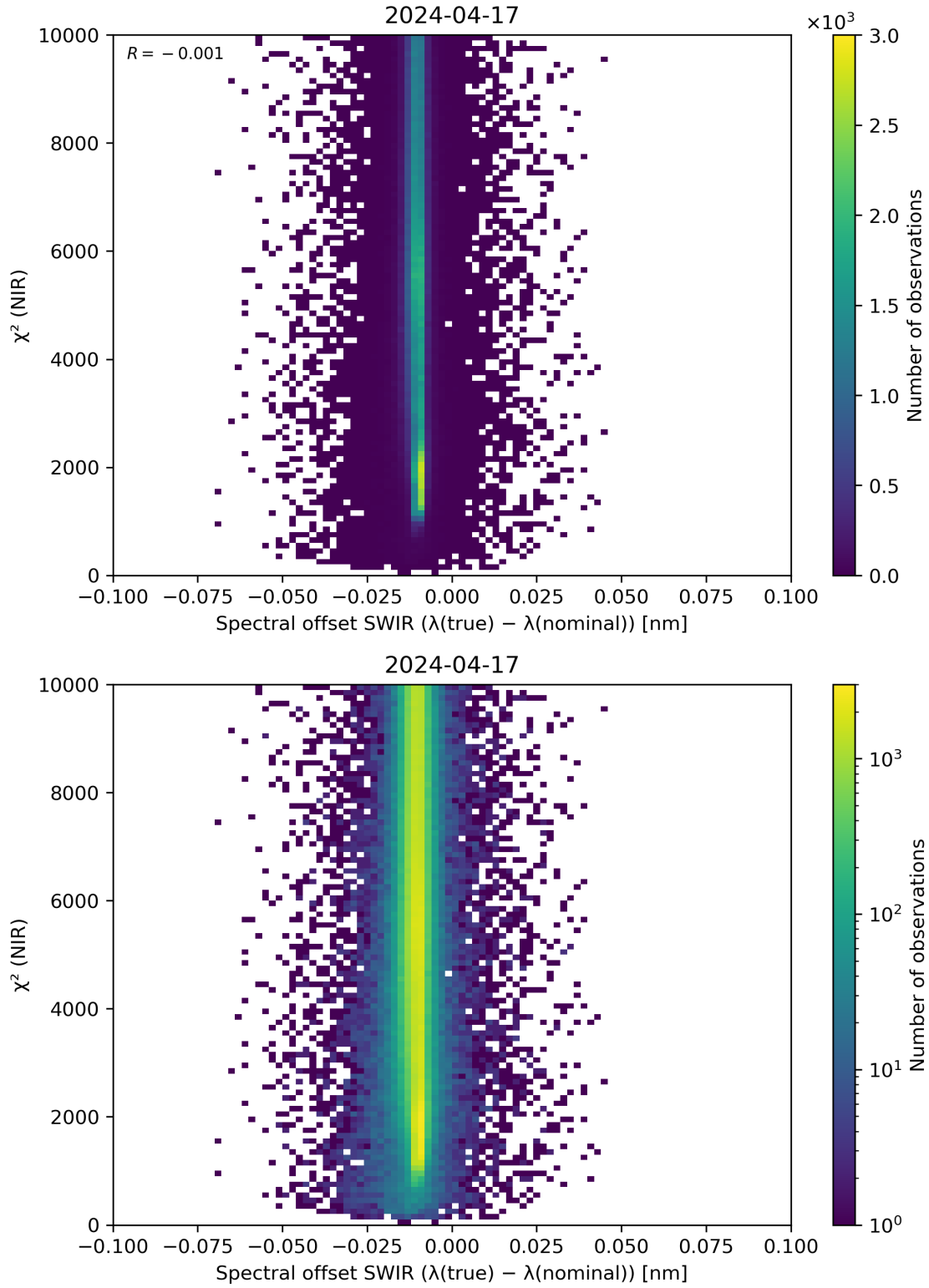
Figure 117: Scatter density plot of “Spectral offset SWIR ( \lambda(\text{true}) - \lambda(\text{nominal}) )” against “ \chi^2 (NIR)” for 2024-04-16 to 2024-04-18.
