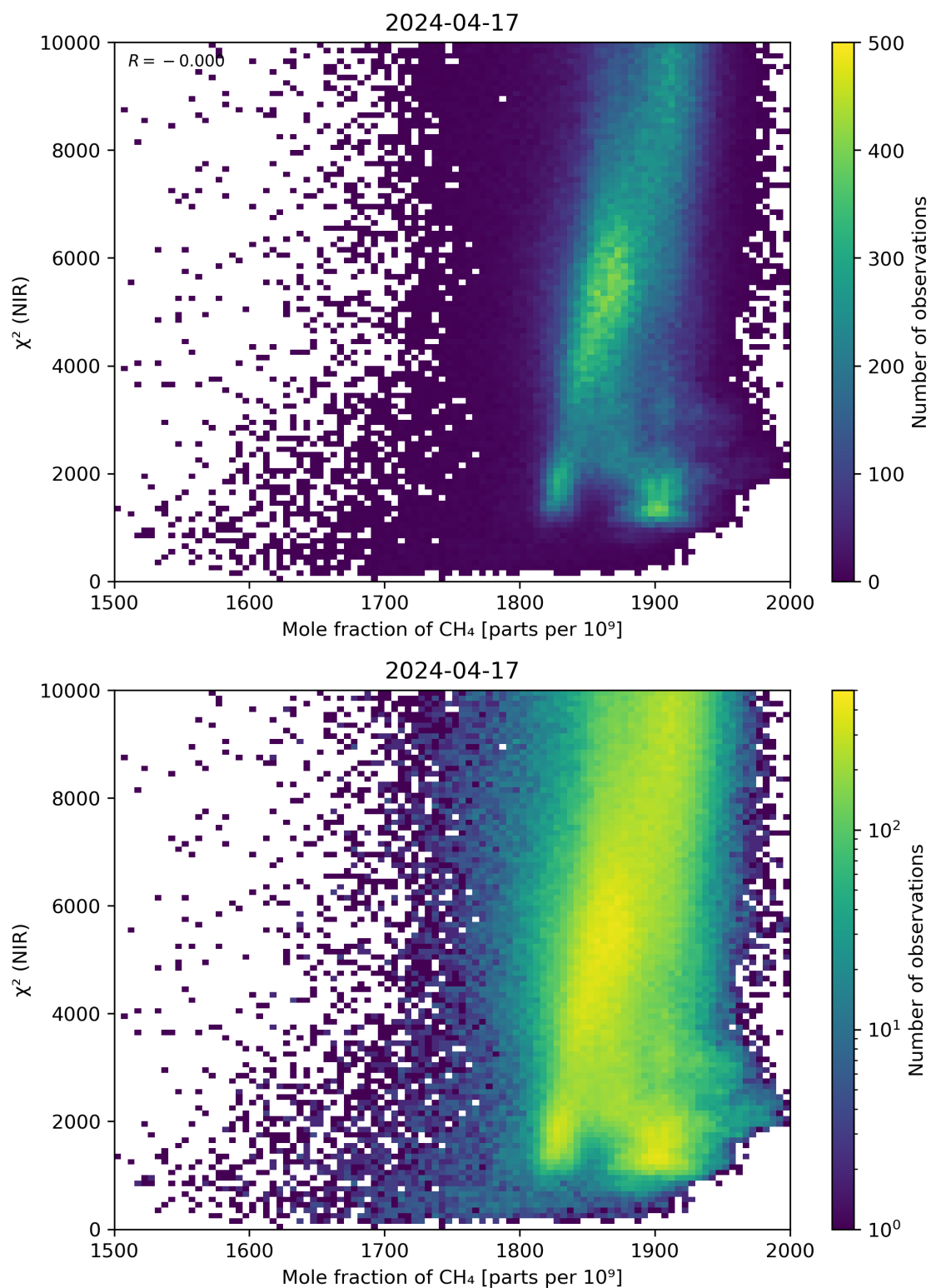
Figure 70: Scatter density plot of “Mole fraction of CH 4 ” against “ \chi^2 (NIR)” for 2024-04-16 to 2024-04-18.
