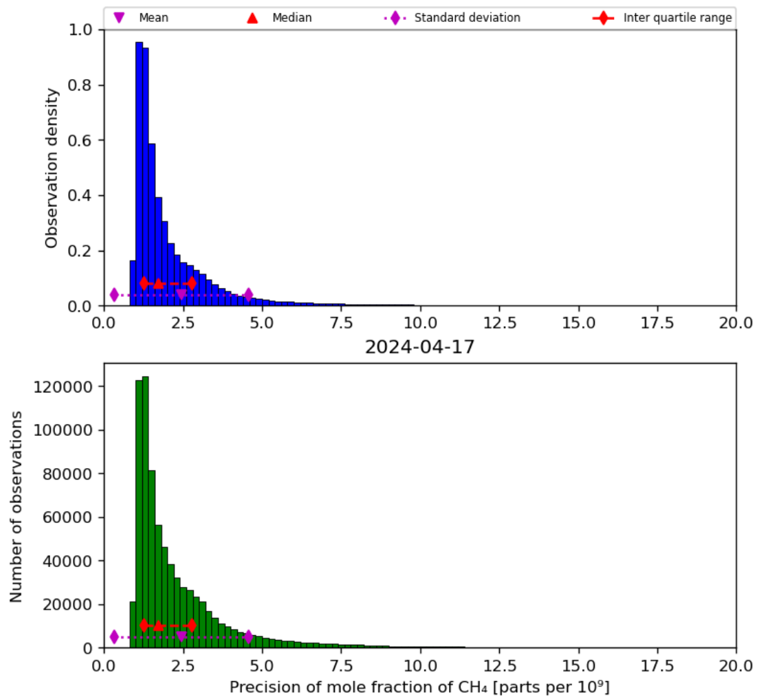
Figure 24: Histogram of “Precision of mole fraction of CH 4 ” for 2024-04-16 to 2024-04-18
