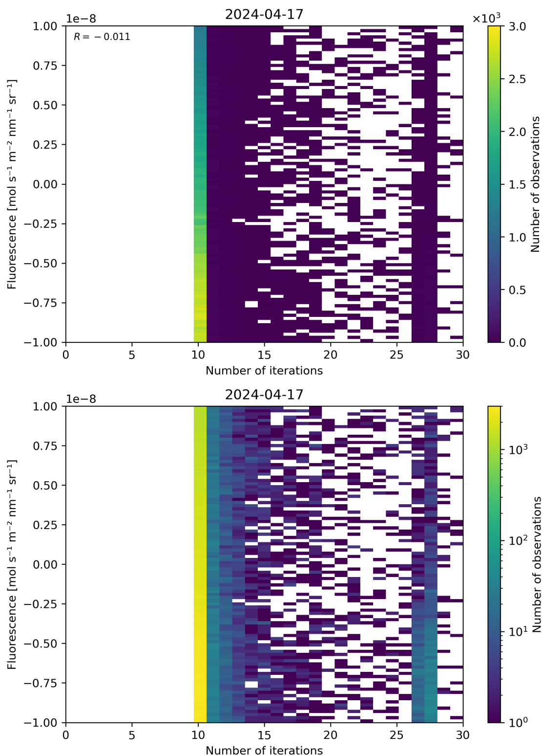
Figure 87: Scatter density plot of “Number of iterations” against “Fluorescence” for 2024-04-16 to 2024-04-18.
