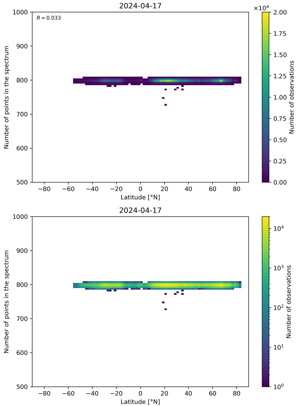
Figure 61: Scatter density plot of “Latitude” against “Number of points in the spectrum” for 2024-04-16 to 2024-04-18.
