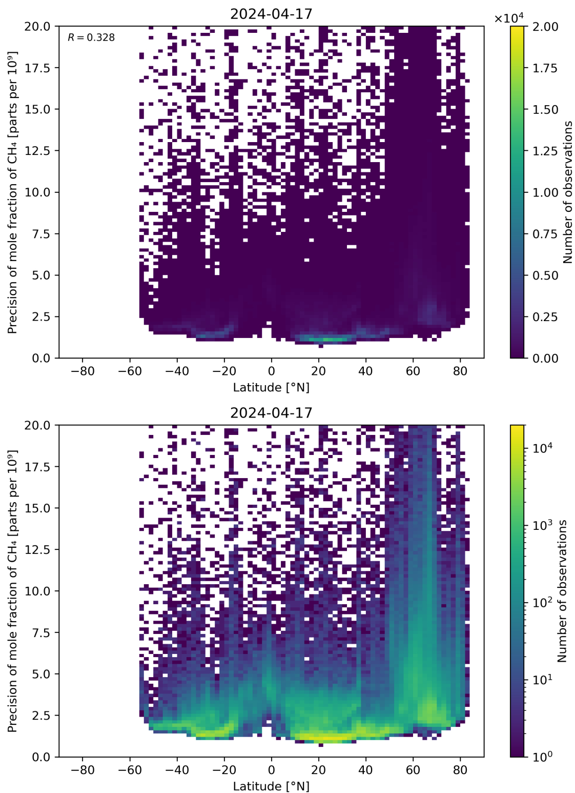
Figure 59: Scatter density plot of “Latitude” against “Precision of mole fraction of CH 4 ” for 2024-04-16 to 2024-04-18.
