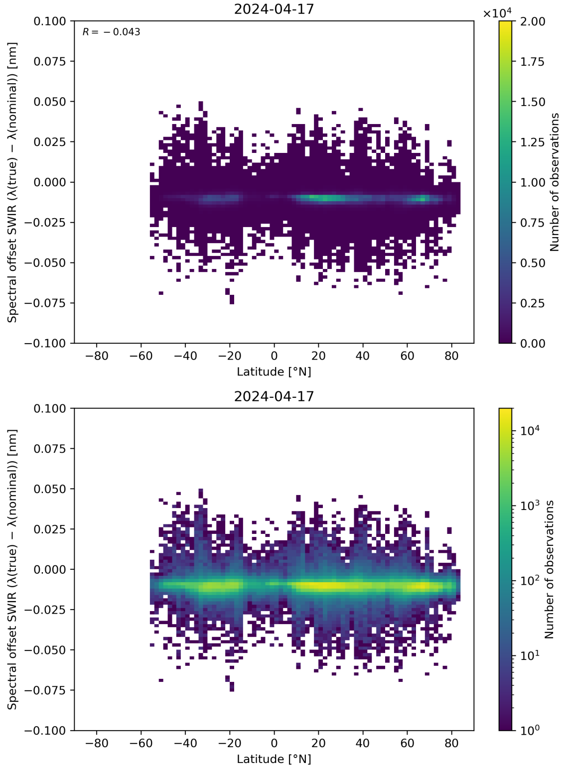
Figure 62: Scatter density plot of “Latitude” against “Spectral offset SWIR ( \lambda(\text{true}) - \lambda(\text{nominal}) )” for 2024-04-16 to 2024-04-18.
