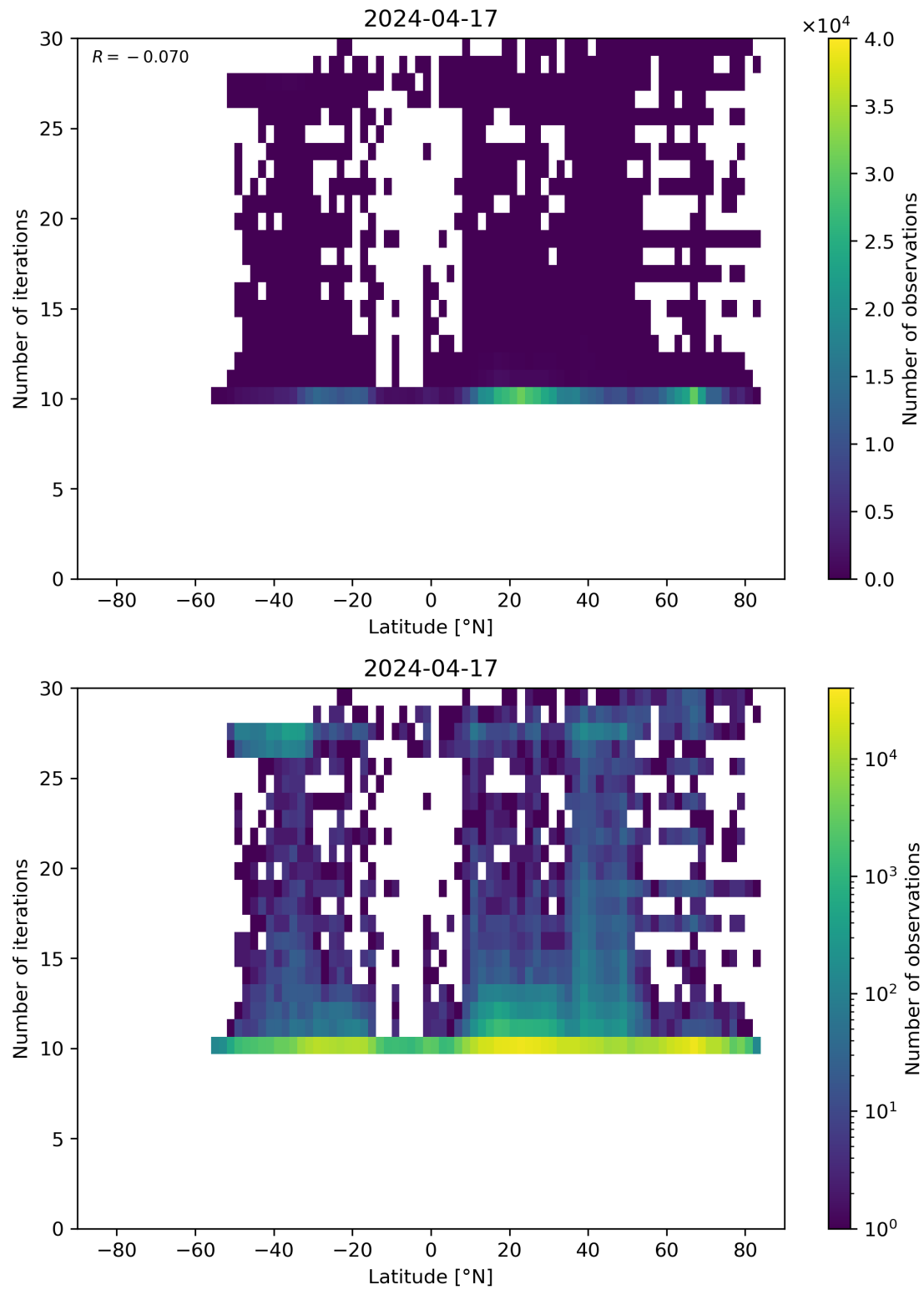
Figure 60: Scatter density plot of “Latitude” against “Number of iterations” for 2024-04-16 to 2024-04-18.
