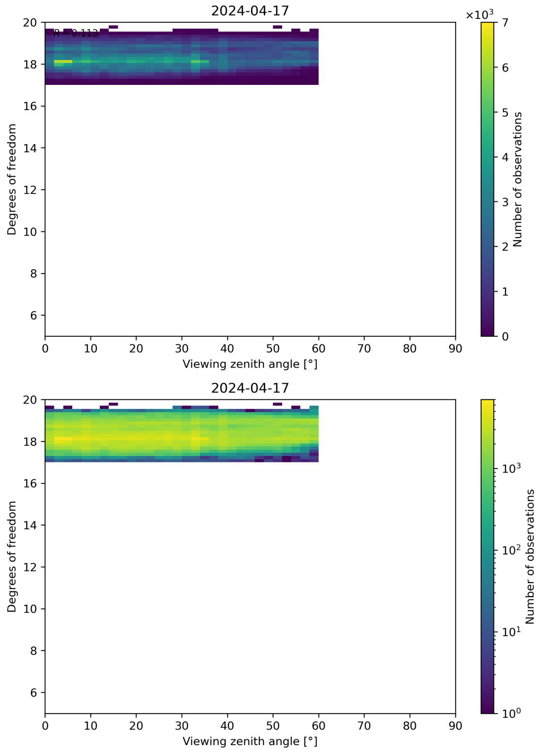
Figure 107: Scatter density plot of “Viewing zenith angle” against “Degrees of freedom” for 2024-04-16 to 2024-04-18.
