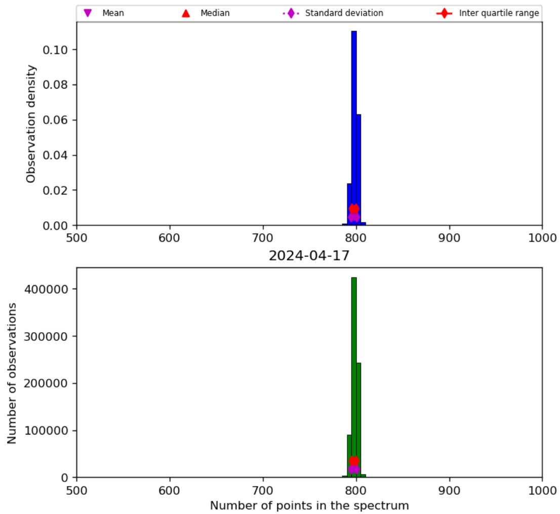
Figure 26: Histogram of “Number of points in the spectrum” for 2024-04-16 to 2024-04-18
