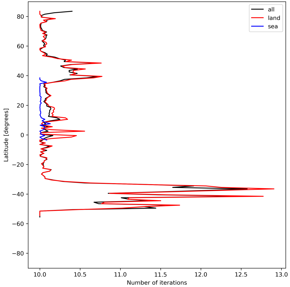
Figure 20: Zonal average of “Number of iterations” for 2024-04-16 to 2024-04-18.
