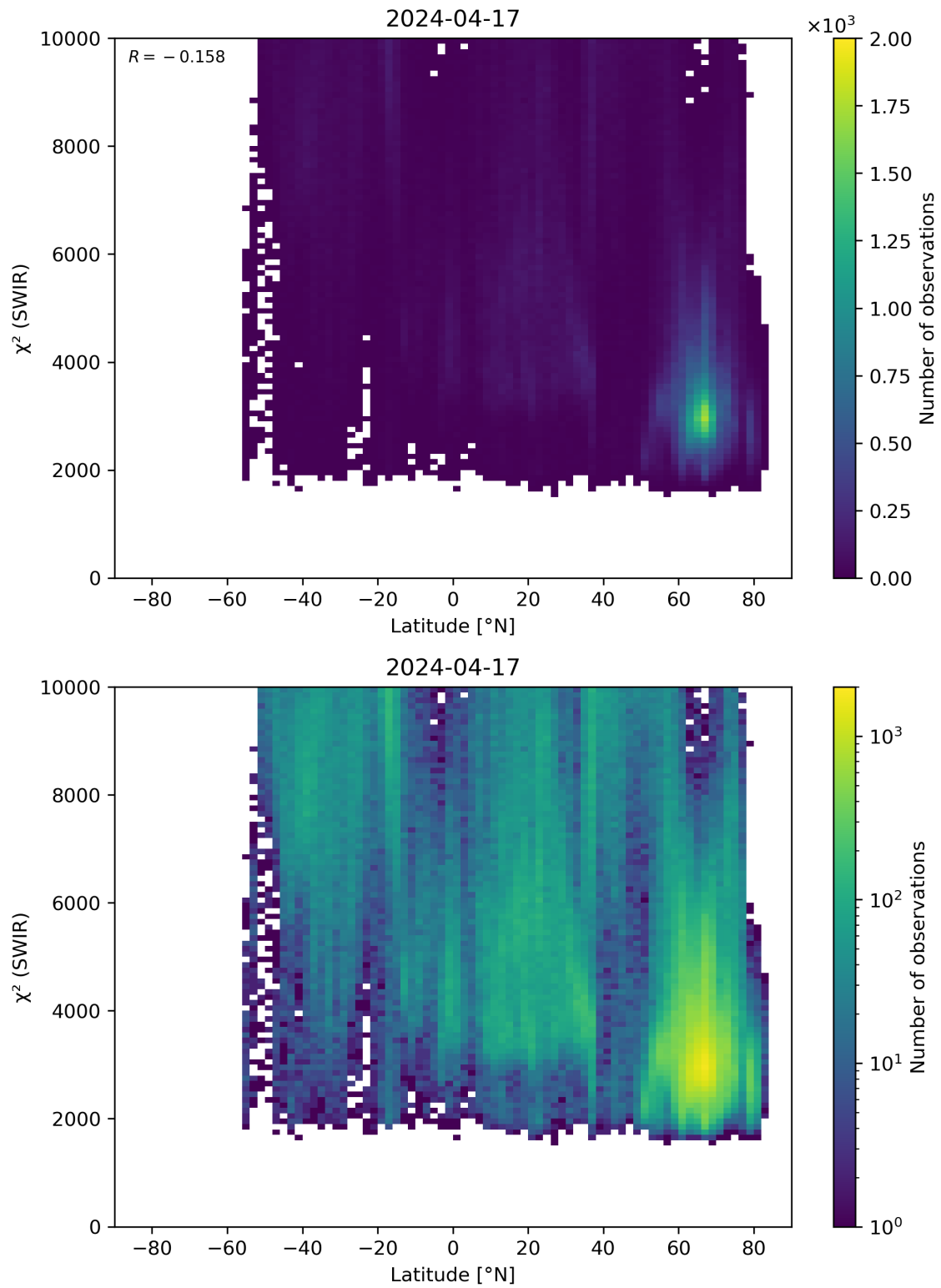
Figure 54: Scatter density plot of “Latitude” against “ \chi^2 (SWIR)” for 2024-04-16 to 2024-04-18.
