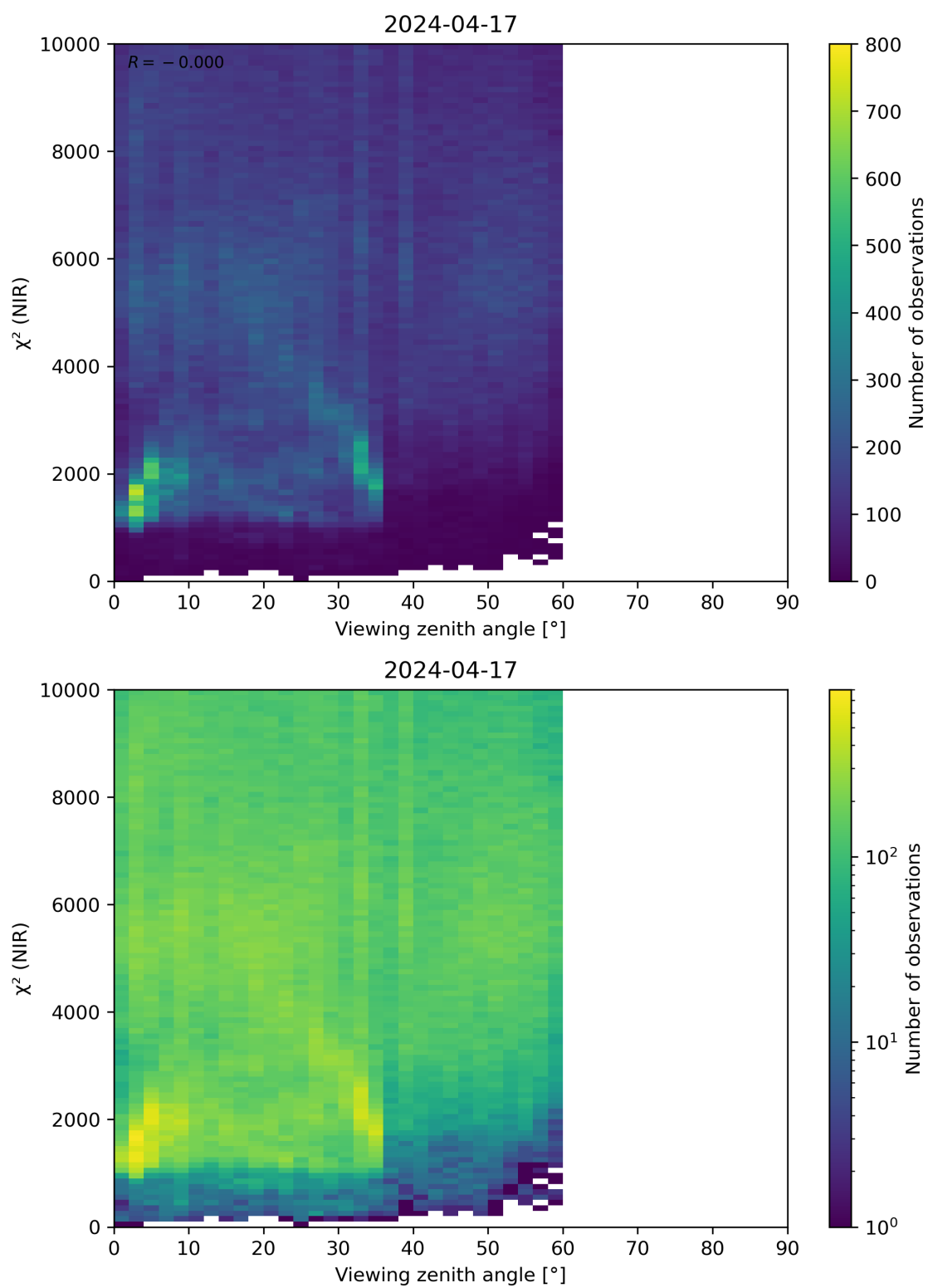
Figure 105: Scatter density plot of “Viewing zenith angle” against “ \chi^2 (NIR)” for 2024-04-16 to 2024-04-18.
