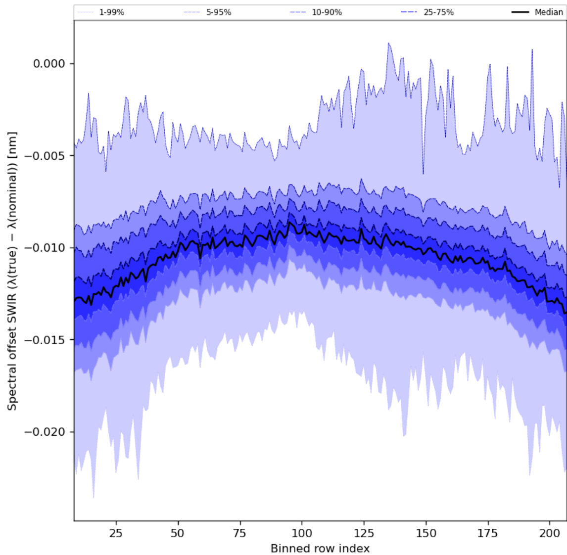
Figure 38: Along track statistics of “Spectral offset SWIR ( \lambda(\text{true}) - \lambda(\text{nominal}) )” for 2024-04-16 to 2024-04-18
