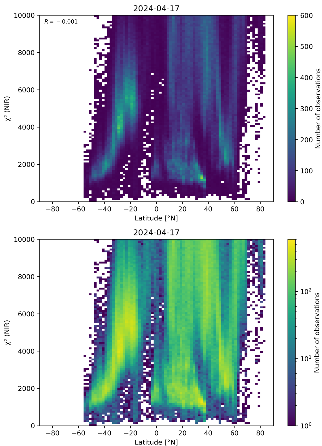
Figure 53: Scatter density plot of “Latitude” against “ \chi^2 (NIR)” for 2024-04-16 to 2024-04-18.
