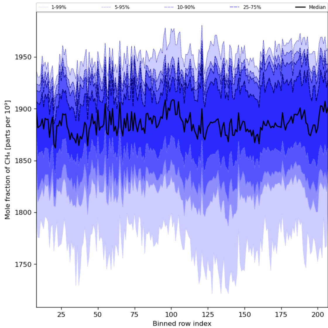
Figure 34: Along track statistics of “Mole fraction of CH 4 ” for 2024-04-16 to 2024-04-18
