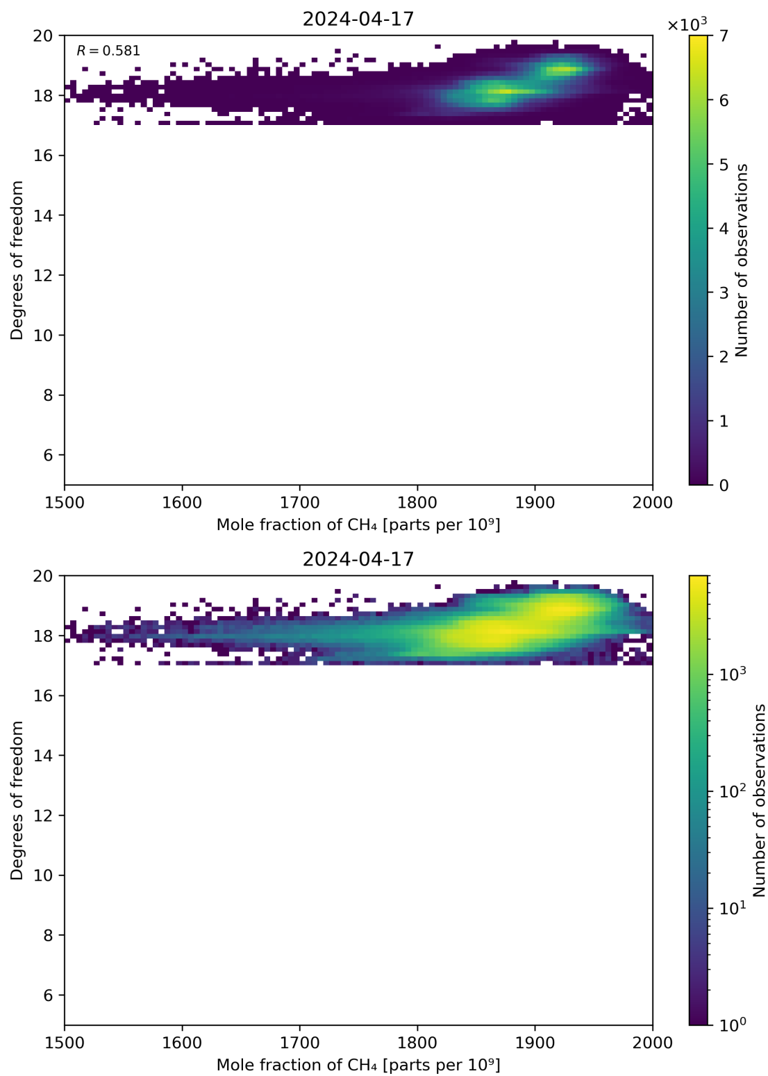
Figure 72: Scatter density plot of “Mole fraction of CH 4 ” against “Degrees of freedom” for 2024-04-16 to 2024-04-18.
