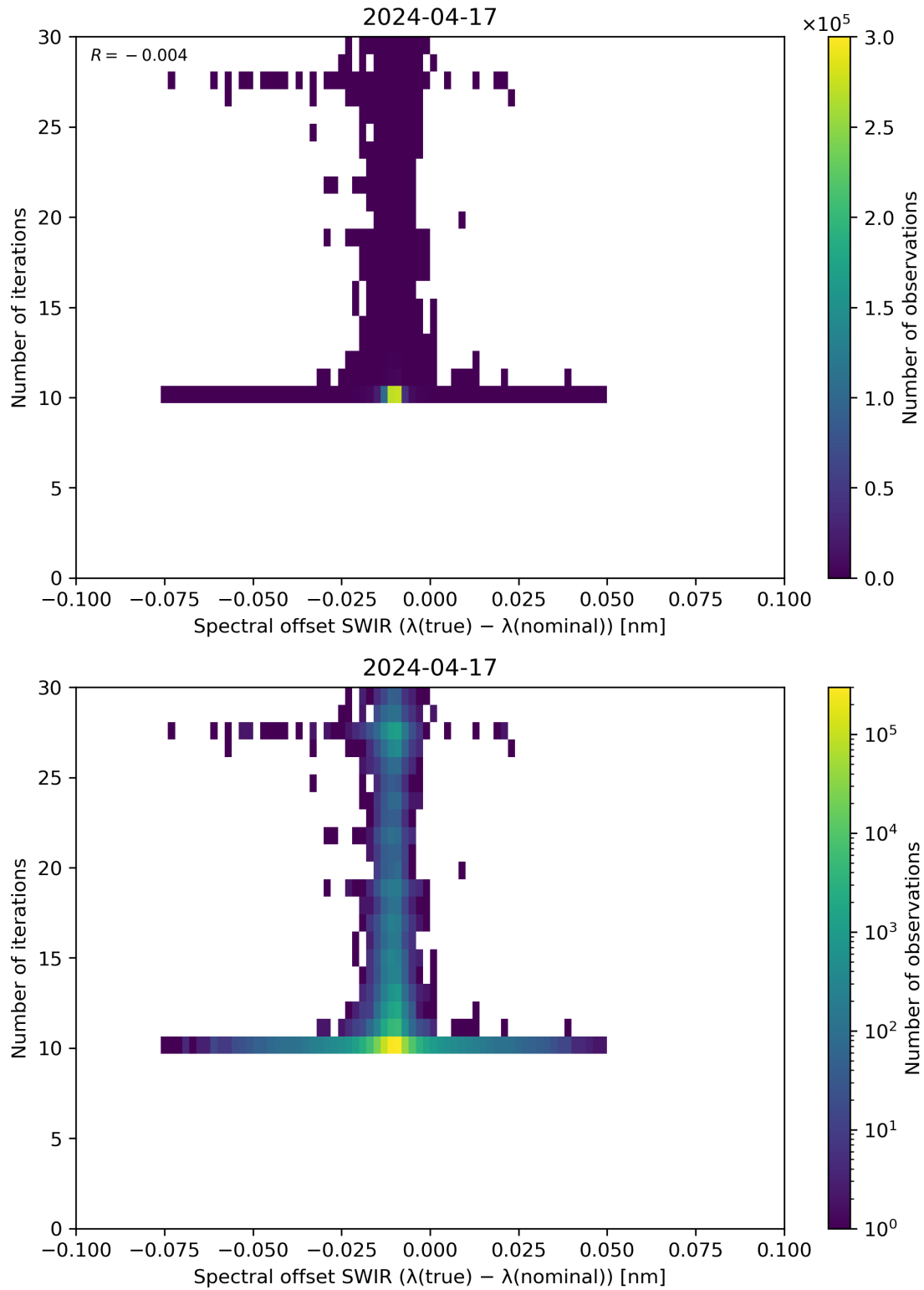
Figure 121: Scatter density plot of “Spectral offset SWIR ( \lambda(\text{true}) - \lambda(\text{nominal}) )” against “Number of iterations” for 2024-04-16 to 2024-04-18.
