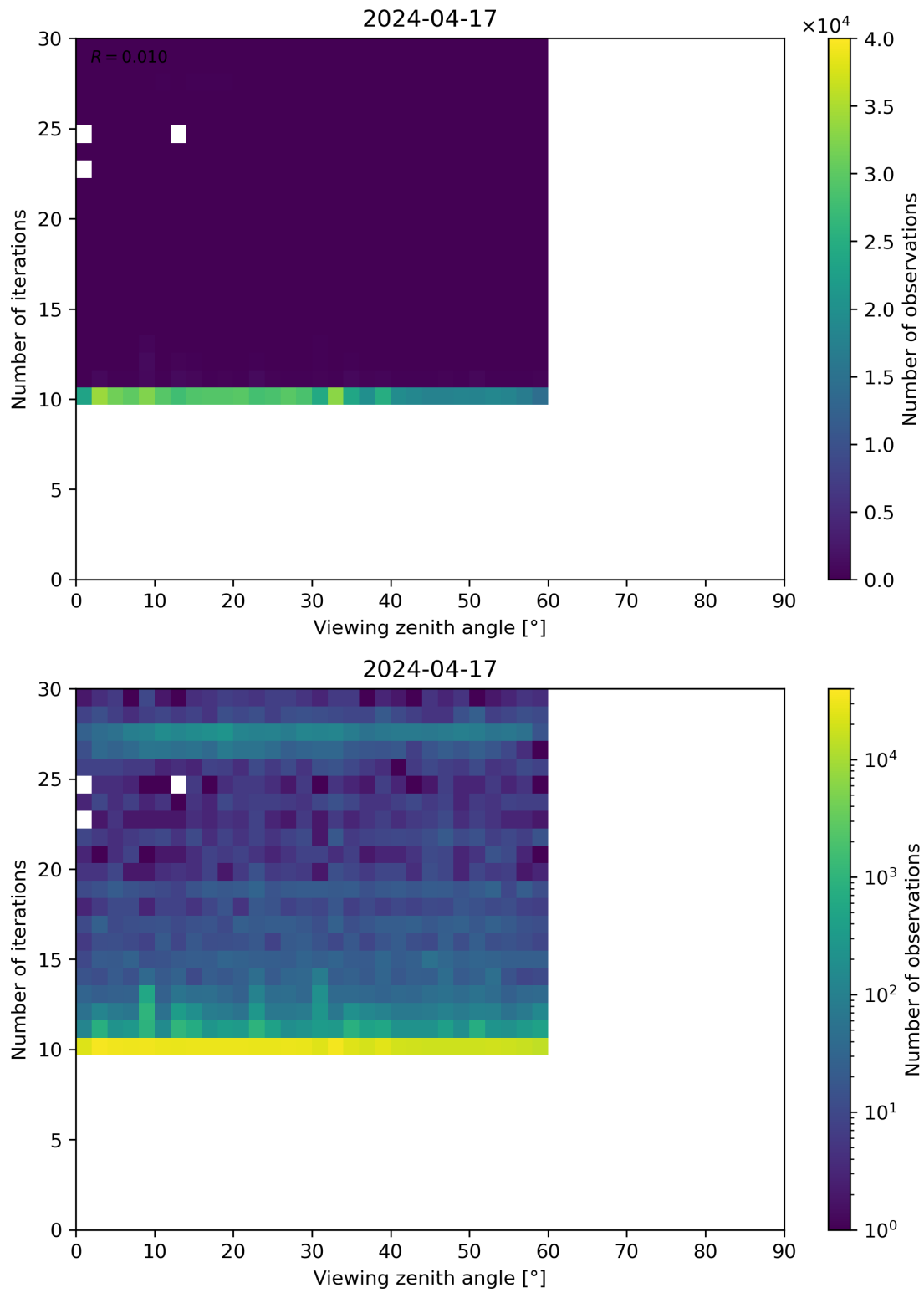
Figure 113: Scatter density plot of “Viewing zenith angle” against “Number of iterations” for 2024-04-16 to 2024-04-18.
