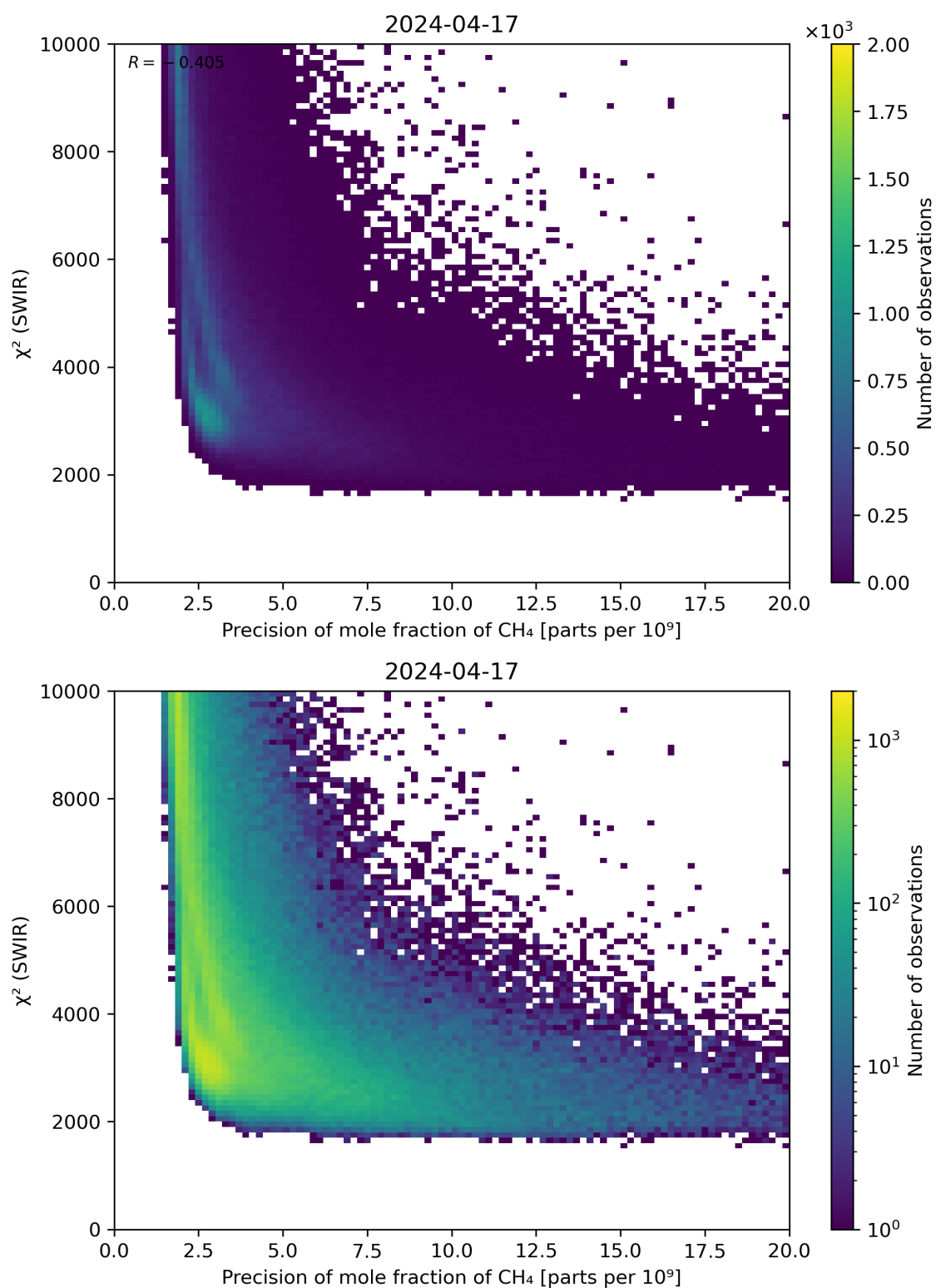
Figure 79: Scatter density plot of “Precision of mole fraction of \text{CH}_4 ” against “ \chi^2 (SWIR)” for 2024-04-16 to 2024-04-18.
