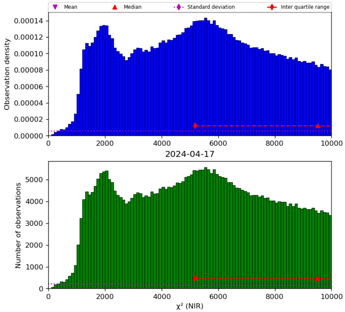
Figure 29: Histogram of “ \chi^2 (NIR)” for 2024-04-16 to 2024-04-18
