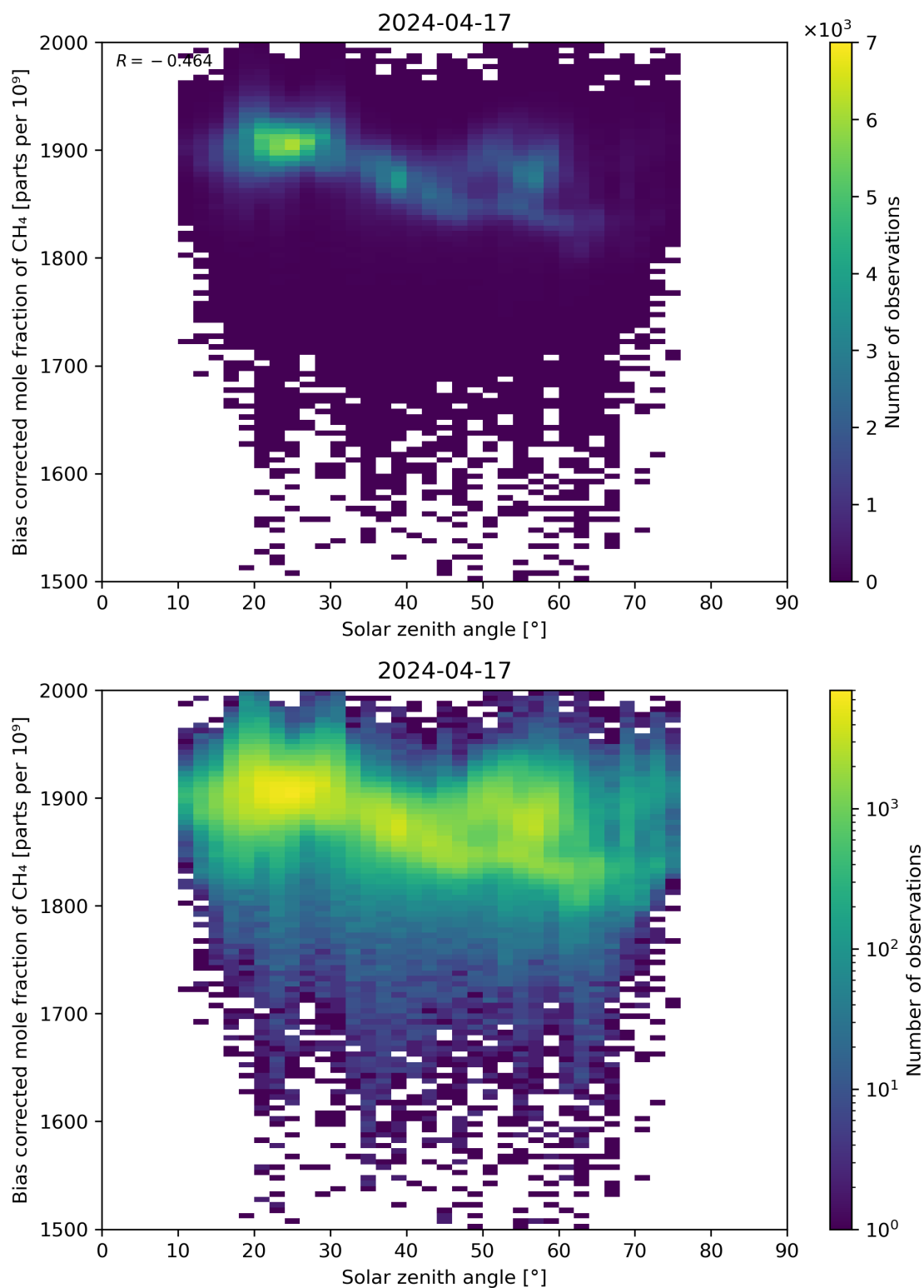
Figure 100: Scatter density plot of “Solar zenith angle” against “Bias corrected mole fraction of CH 4 ” for 2024-04-16 to 2024-04-18.
