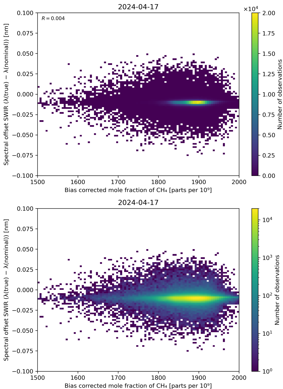
Figure 69: Scatter density plot of “Bias corrected mole fraction of \text{CH}_4 ” against “Spectral offset SWIR ( \lambda(\text{true}) - \lambda(\text{nominal}) )” for 2024-04-16 to 2024-04-18.
