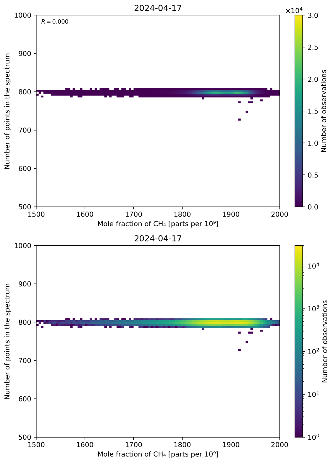
Figure 77: Scatter density plot of “Mole fraction of CH 4 ” against “Number of points in the spectrum” for 2024-04-16 to 2024-04-18.
