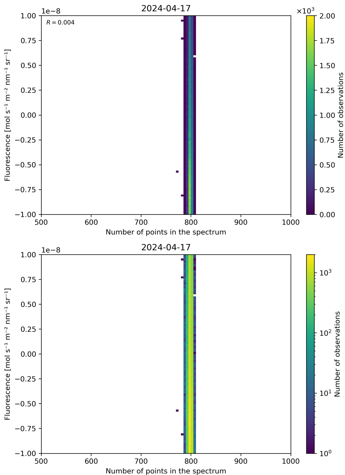
Figure 91: Scatter density plot of “Number of points in the spectrum” against “Fluorescence” for 2024-04-16 to 2024-04-18.
