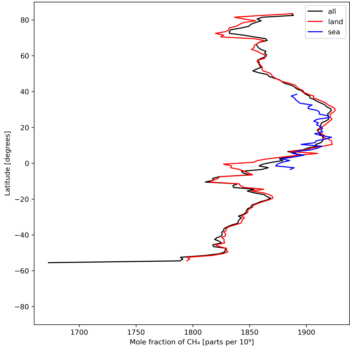
Figure 12: Zonal average of “Mole fraction of \text{CH}_4 ” for 2024-04-16 to 2024-04-18.
