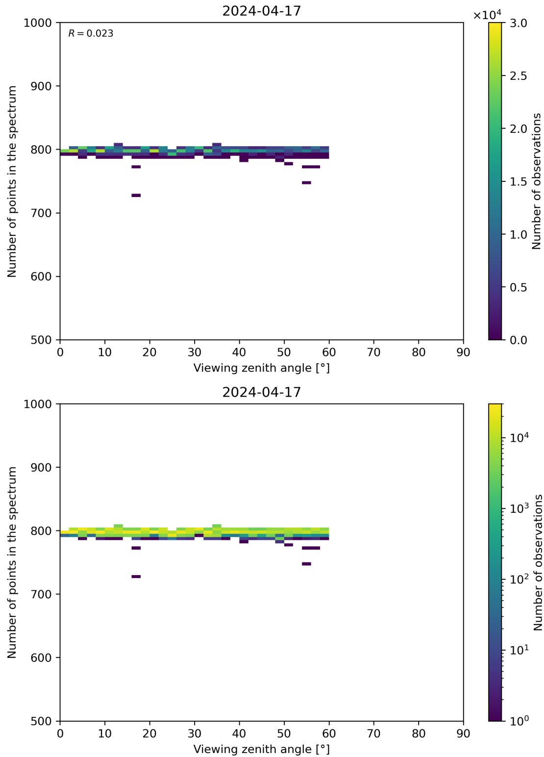
Figure 114: Scatter density plot of “Viewing zenith angle” against “Number of points in the spectrum” for 2024-04-16 to 2024-04-18.
