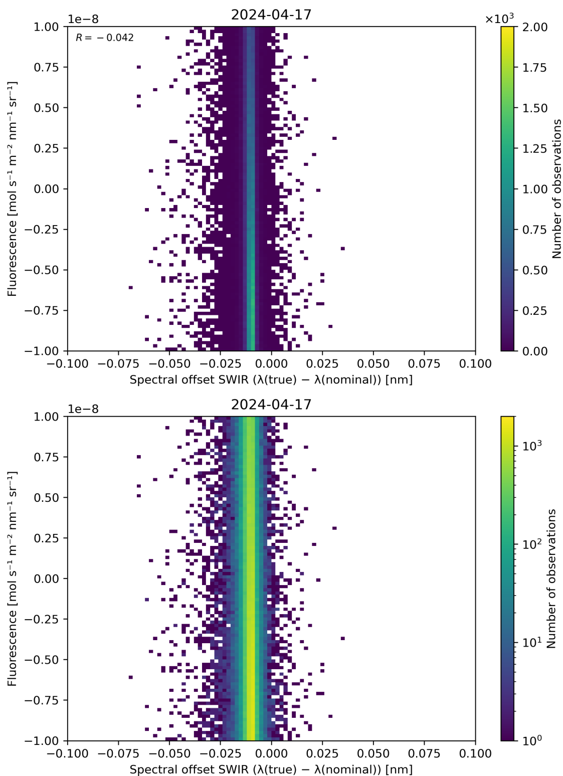
Figure 120: Scatter density plot of “Spectral offset SWIR ( \lambda(\text{true}) - \lambda(\text{nominal}) )” against “Fluorescence” for 2024-04-16 to 2024-04-18.
