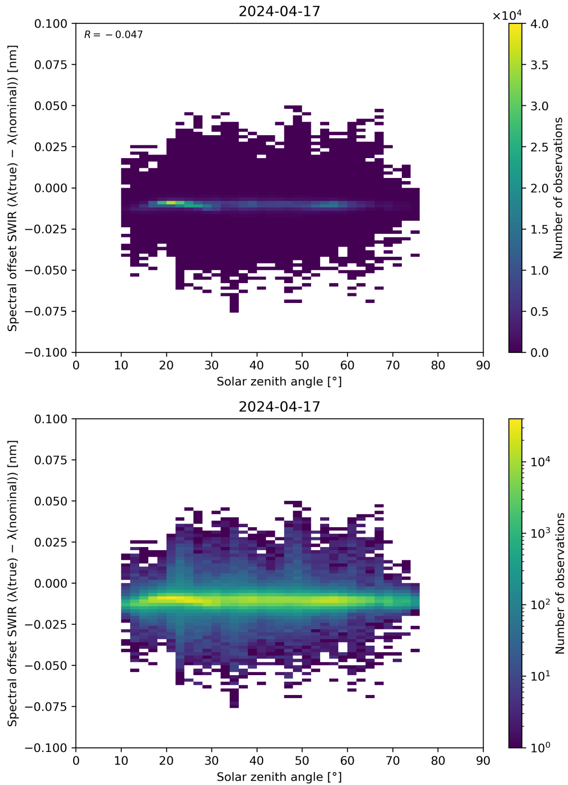
Figure 104: Scatter density plot of “Solar zenith angle” against “Spectral offset SWIR ( \lambda(\text{true}) - \lambda(\text{nominal}) )” for 2024-04-16 to 2024-04-18.
