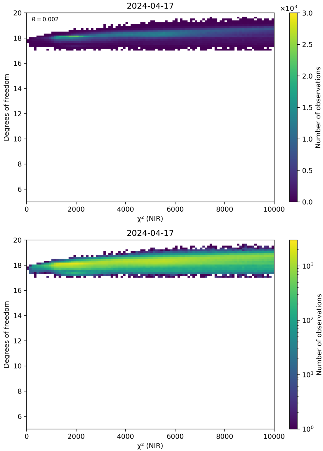
Figure 44: Scatter density plot of “ \chi^2 (NIR)” against “Degrees of freedom” for 2024-04-16 to 2024-04-18.
