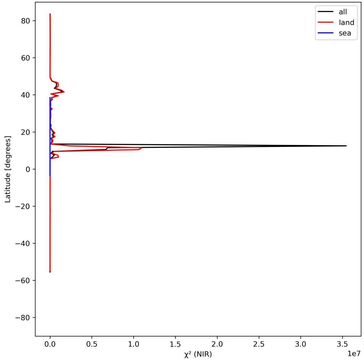
Figure 18: Zonal average of “ \chi^2 (NIR)” for 2024-04-16 to 2024-04-18.
