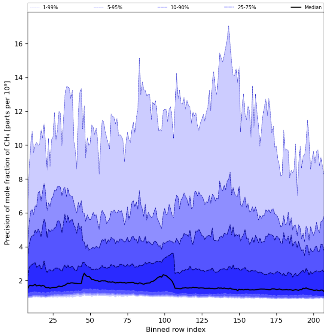
Figure 35: Along track statistics of “Precision of mole fraction of CH 4 ” for 2024-04-16 to 2024-04-18
