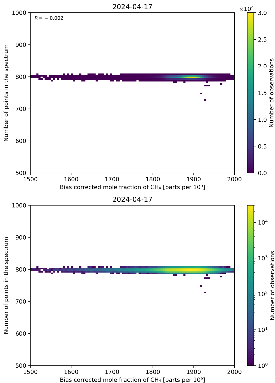
Figure 68: Scatter density plot of “Bias corrected mole fraction of CH 4 ” against “Number of points in the spectrum” for 2024-04-16 to 2024-04-18.
