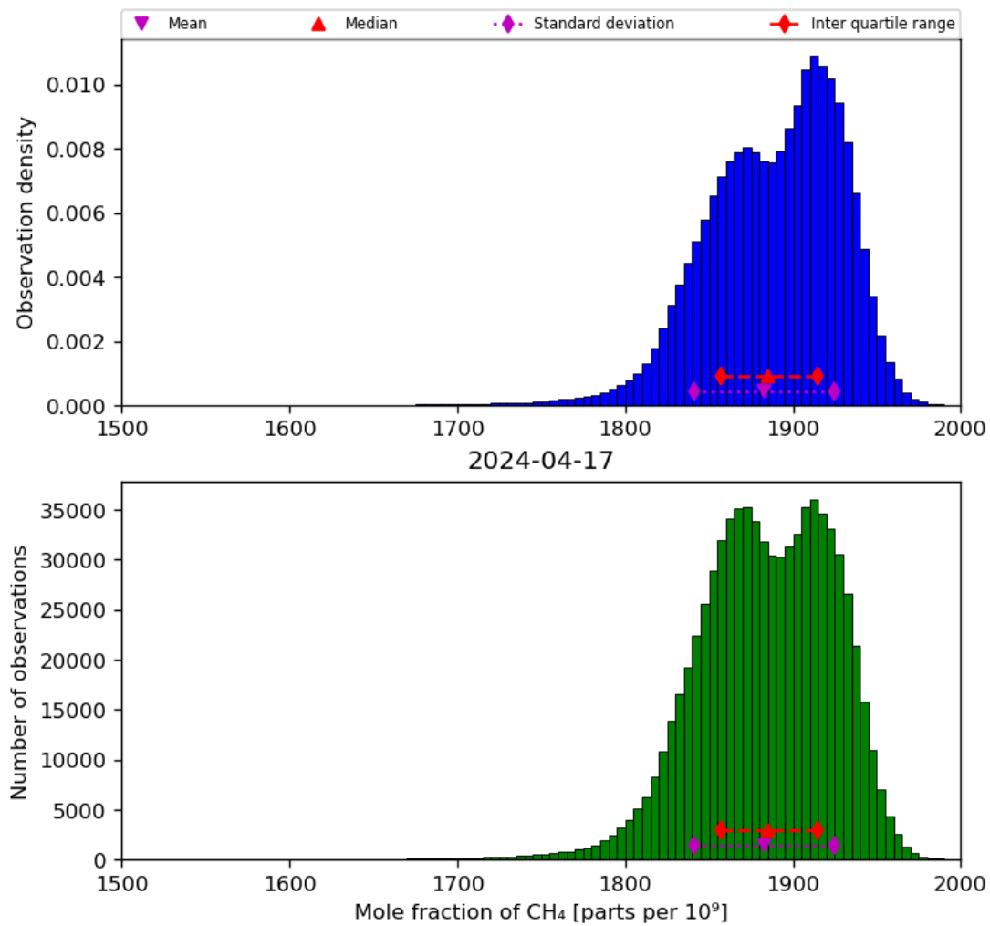
Figure 23: Histogram of “Mole fraction of CH 4 ” for 2024-04-16 to 2024-04-18
