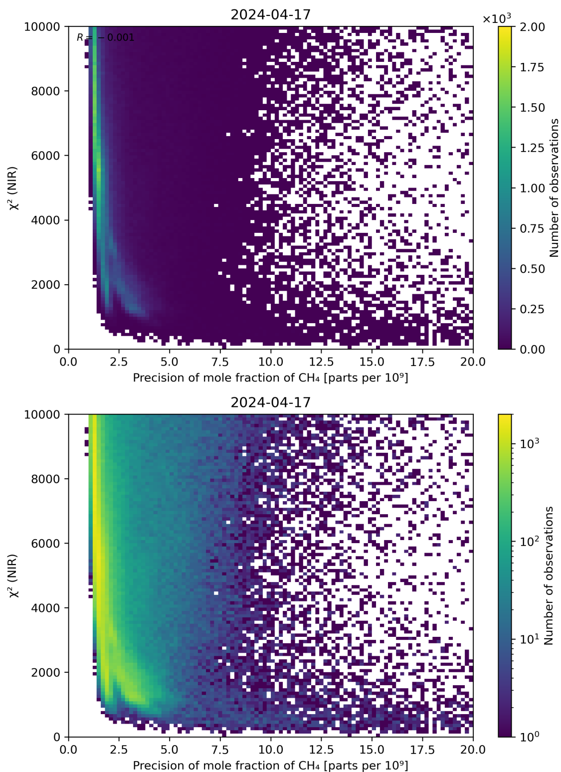
Figure 78: Scatter density plot of “Precision of mole fraction of CH 4 ” against “ \chi^2 (NIR)” for 2024-04-16 to 2024-04-18.
