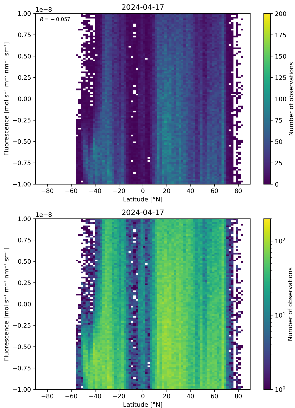
Figure 56: Scatter density plot of “Latitude” against “Fluorescence” for 2024-04-16 to 2024-04-18.
