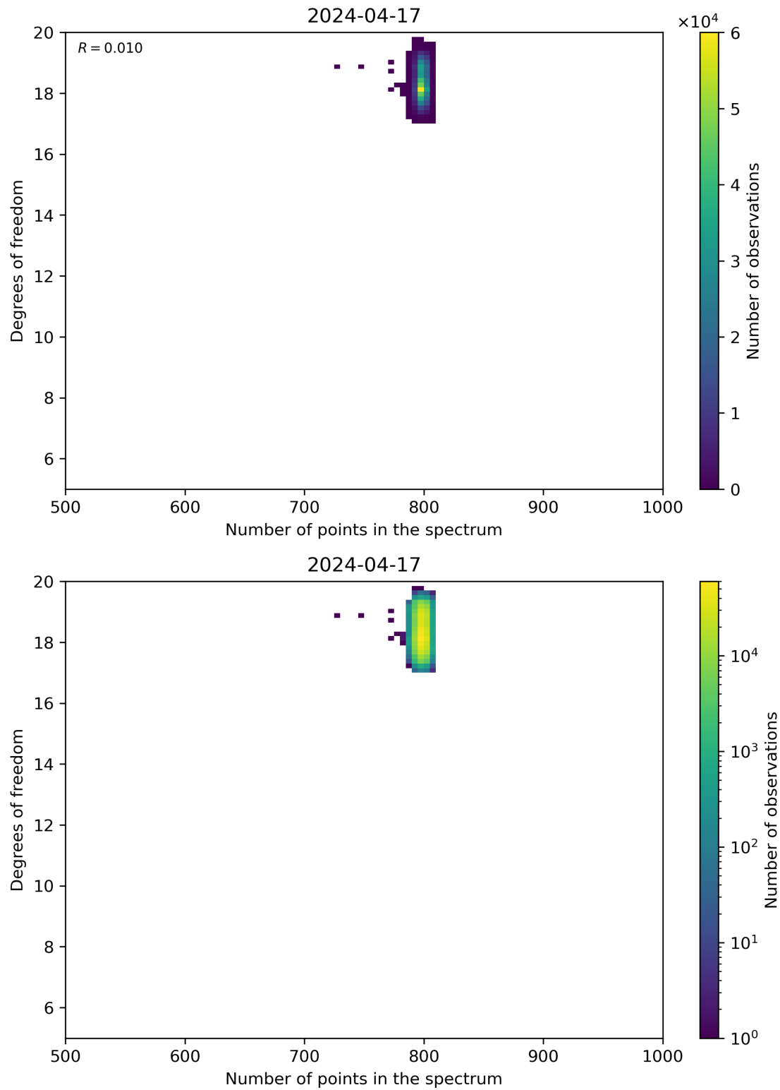
Figure 90: Scatter density plot of “Number of points in the spectrum” against “Degrees of freedom” for 2024-04-16 to 2024-04-18.
