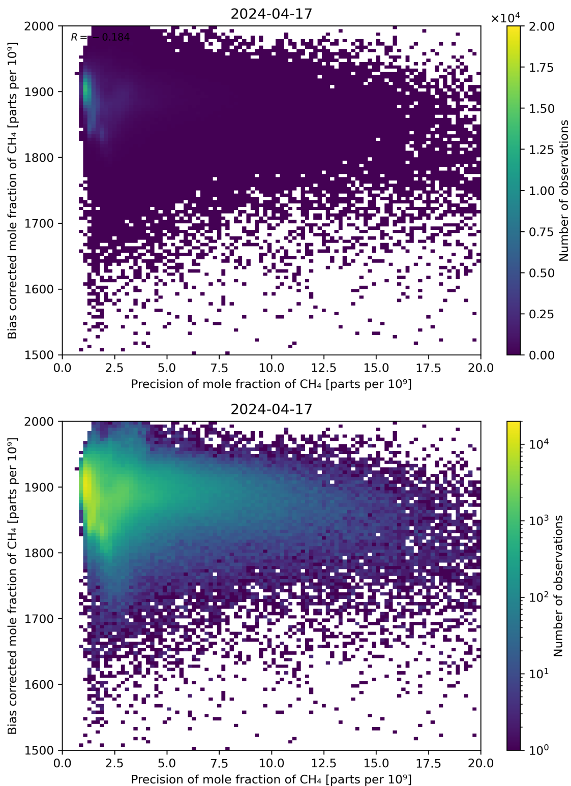
Figure 82: Scatter density plot of “Precision of mole fraction of CH 4 ” against “Bias corrected mole fraction of CH 4 ” for 2024-04-16 to 2024-04-18.
