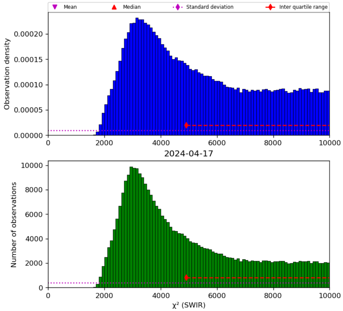
Figure 28: Histogram of “ \chi^2 (SWIR)” for 2024-04-16 to 2024-04-18
