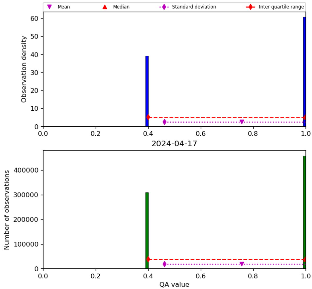
Figure 22: Histogram of “QA value” for 2024-04-16 to 2024-04-18
