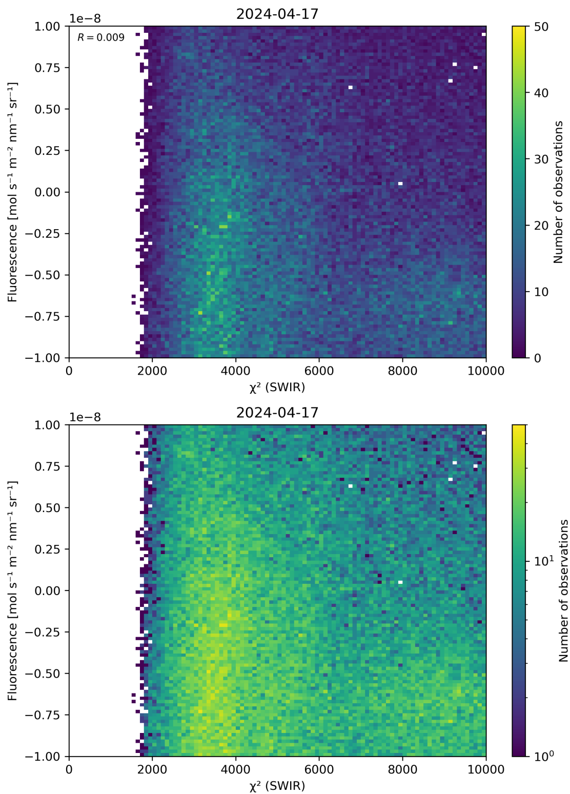
Figure 49: Scatter density plot of “ \chi^2 (SWIR)” against “Fluorescence” for 2024-04-16 to 2024-04-18.
