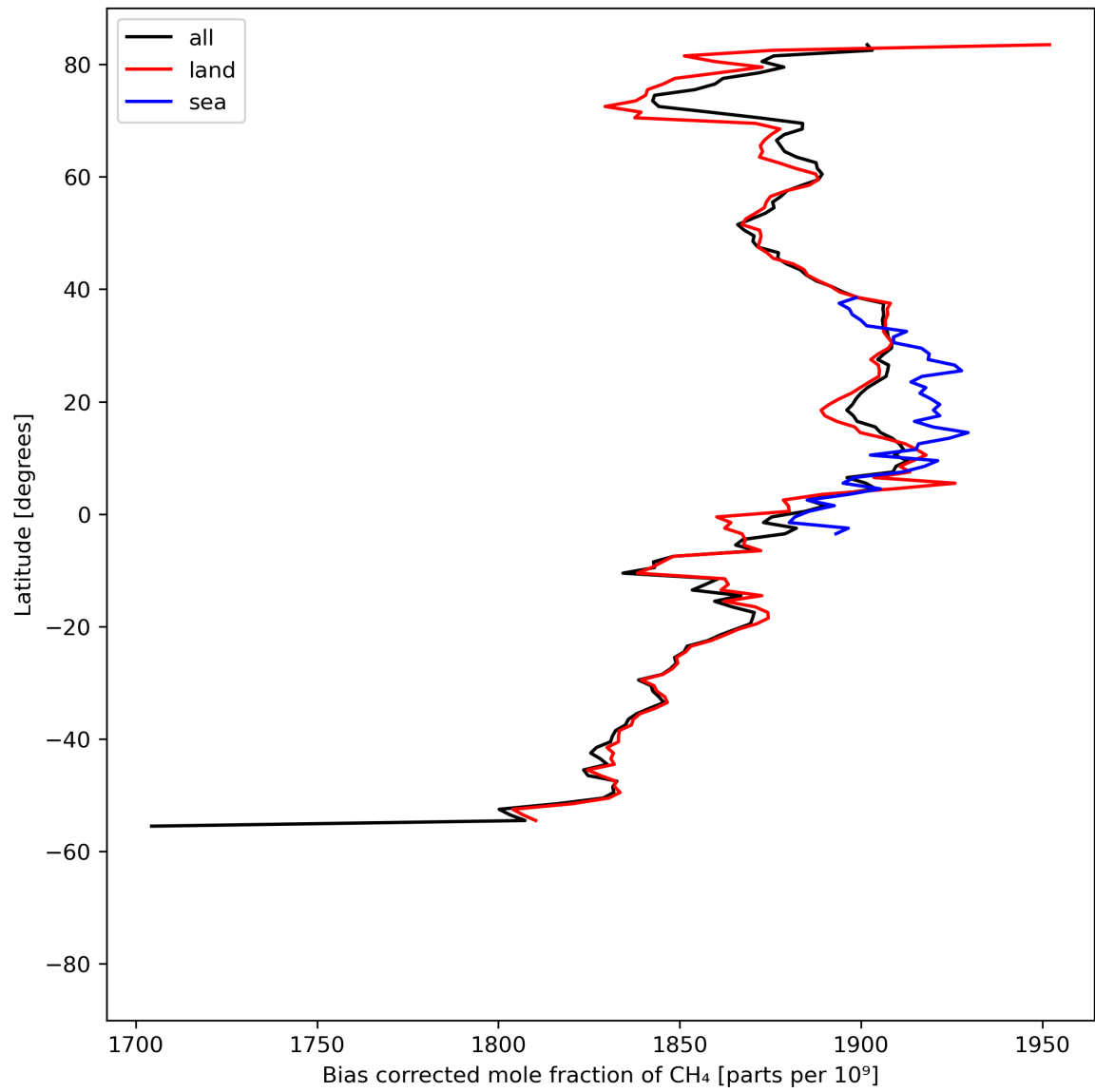
Figure 14: Zonal average of “Bias corrected mole fraction of CH 4 ” for 2024-04-16 to 2024-04-18.
