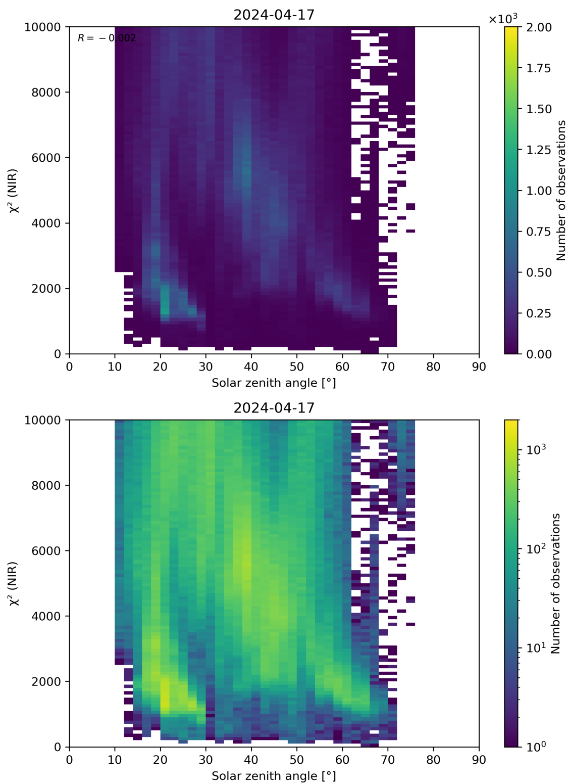
Figure 94: Scatter density plot of “Solar zenith angle” against “ \chi^2 (NIR)” for 2024-04-16 to 2024-04-18.
