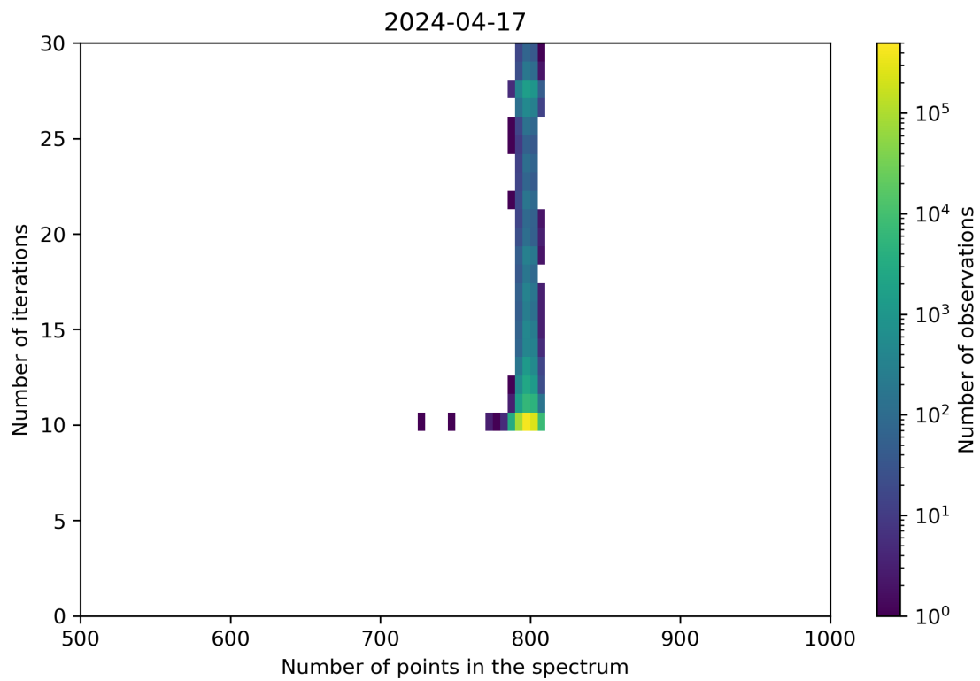
Figure 92: Scatter density plot of “Number of points in the spectrum” against “Number of iterations” for 2024-04-16 to 2024-04-18.
