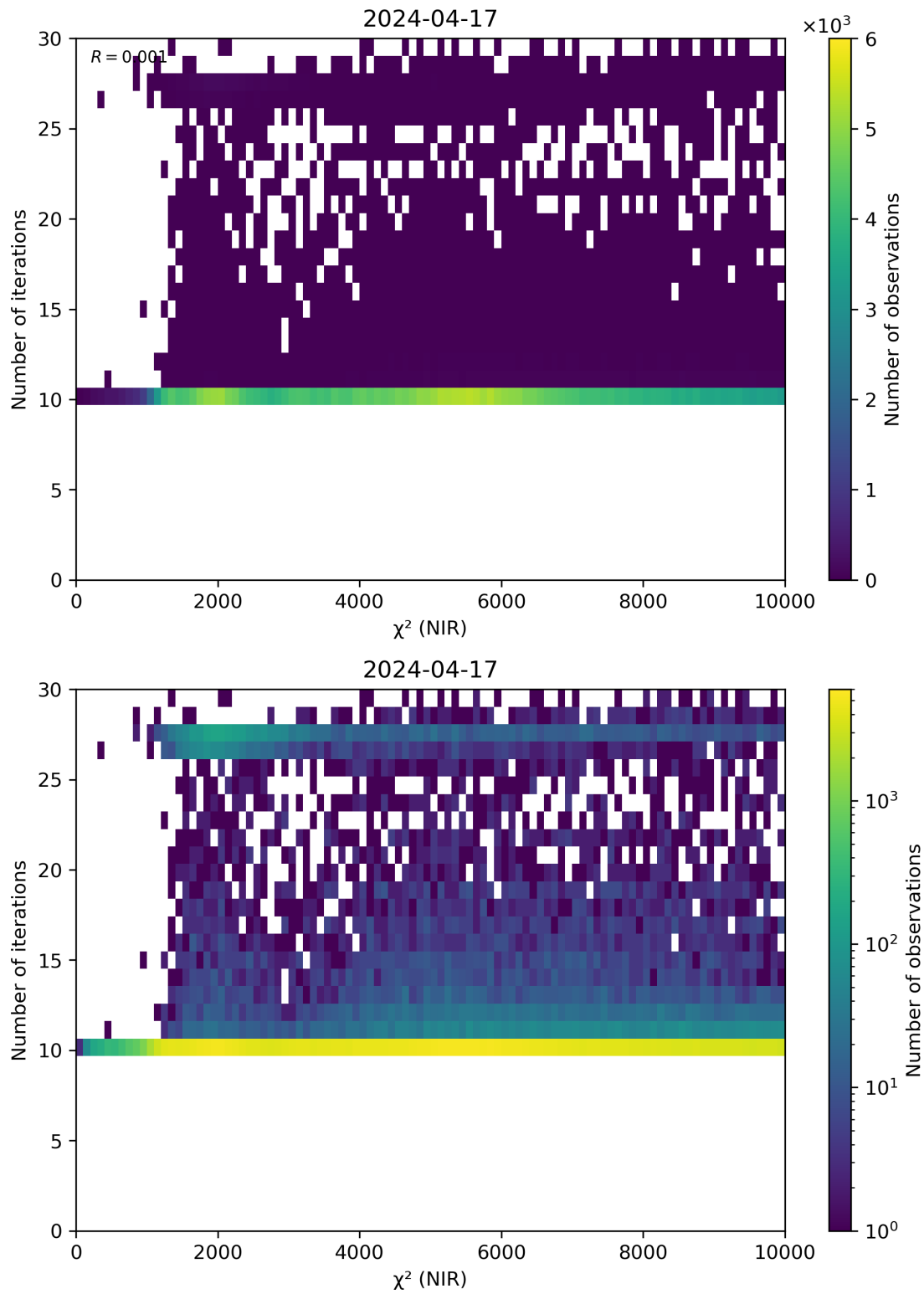
Figure 46: Scatter density plot of “ \chi^2 (NIR)” against “Number of iterations” for 2024-04-16 to 2024-04-18.
