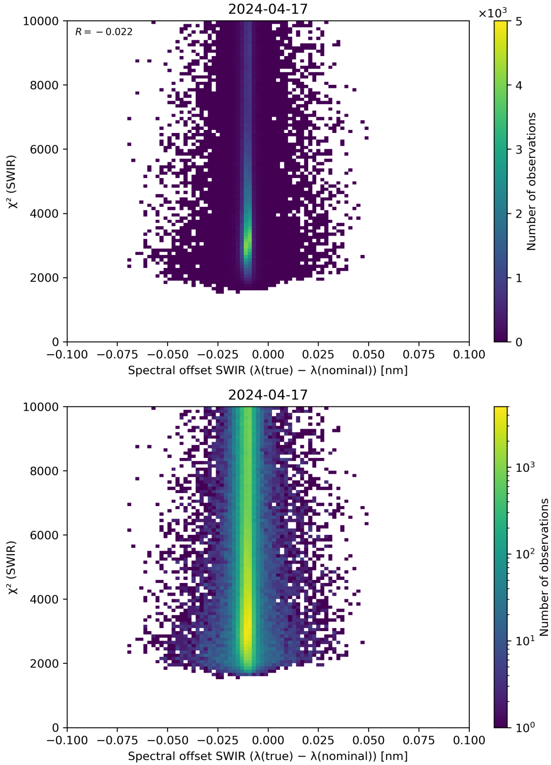
Figure 118: Scatter density plot of “Spectral offset SWIR ( \lambda(\text{true}) - \lambda(\text{nominal}) )” against “ \chi^2 (SWIR)” for 2024-04-16 to 2024-04-18.
