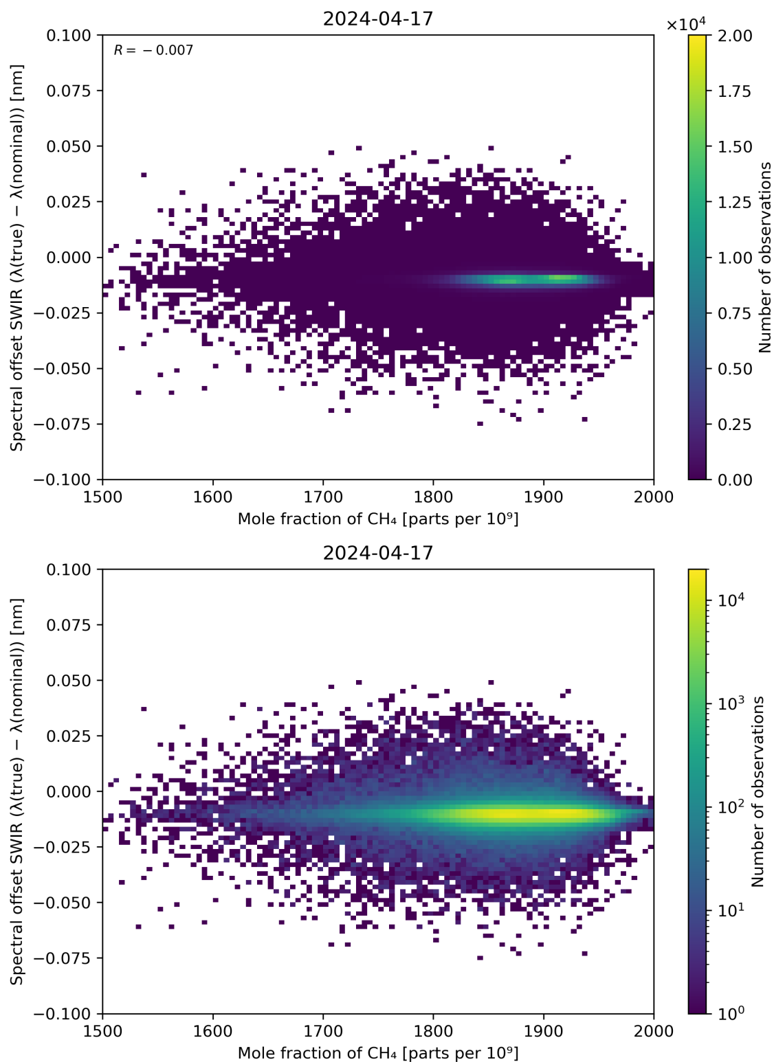
Figure 86: Scatter density plot of “Mole fraction of CH 4 ” against “Spectral offset SWIR ( \lambda(\text{true}) - \lambda(\text{nominal}) )” for 2024-04-16 to 2024-04-18.
