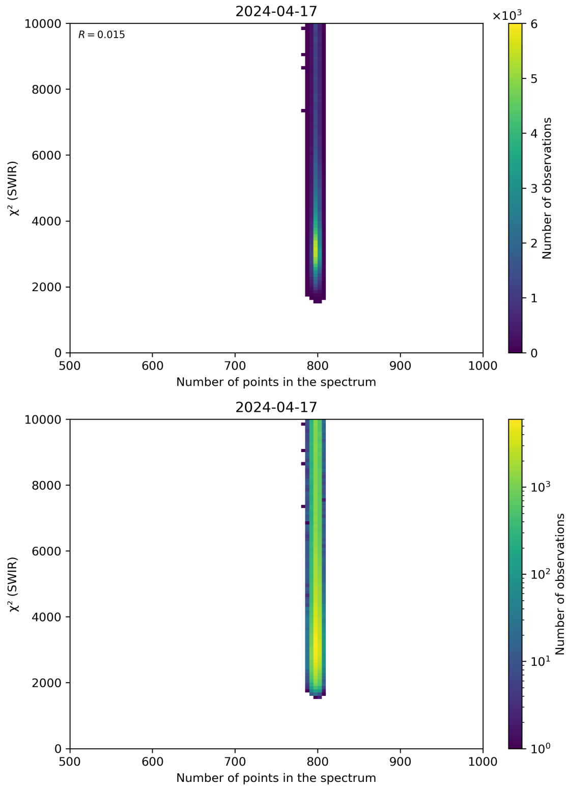
Figure 89: Scatter density plot of “Number of points in the spectrum” against “ \chi^2 (SWIR)” for 2024-04-16 to 2024-04-18.
