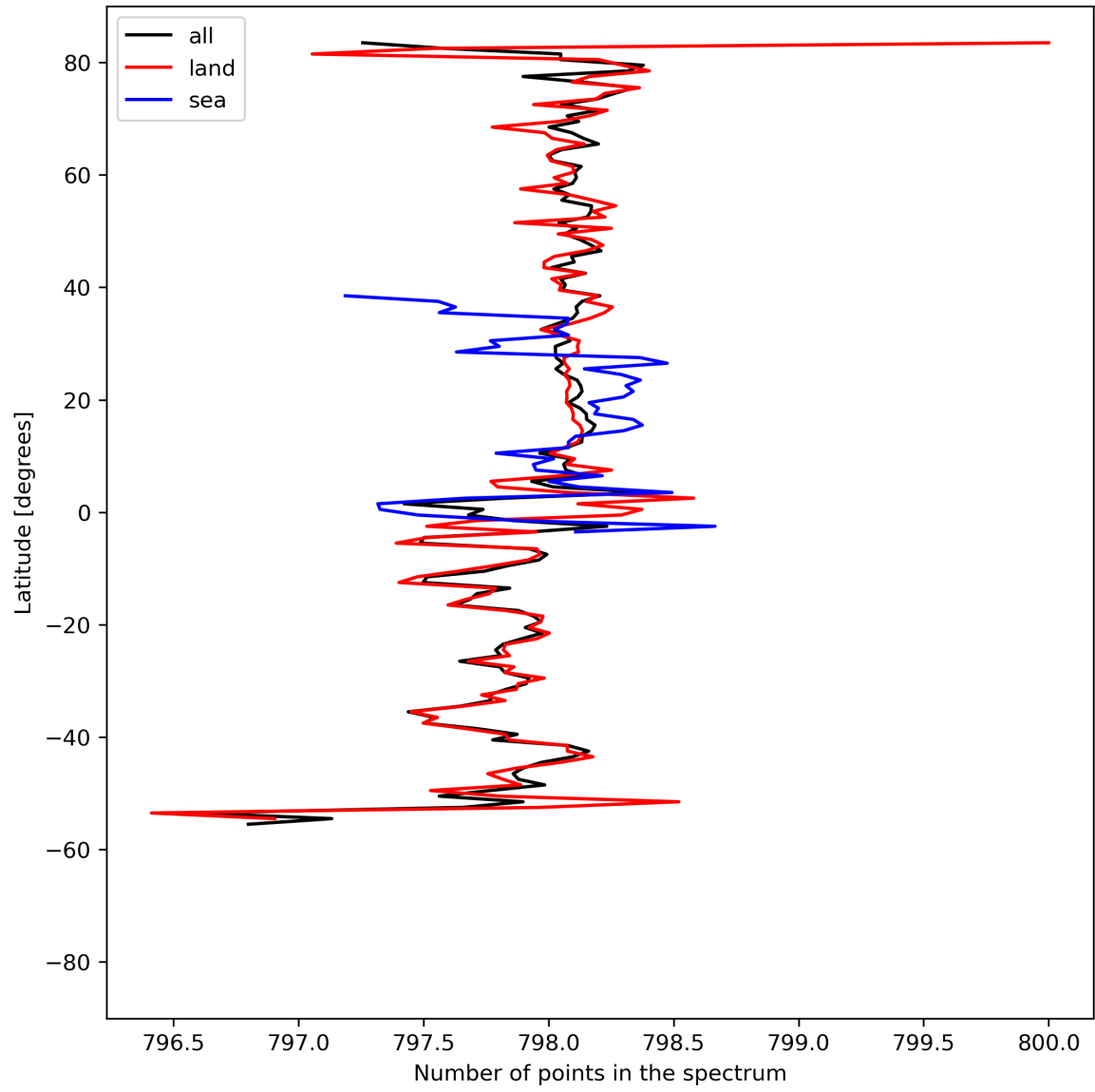
Figure 15: Zonal average of “Number of points in the spectrum” for 2024-04-16 to 2024-04-18.
