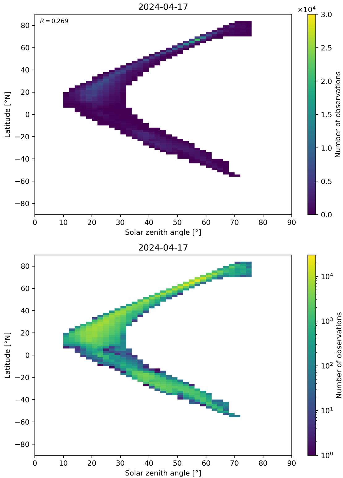
Figure 98: Scatter density plot of “Solar zenith angle” against “Latitude” for 2024-04-16 to 2024-04-18.
