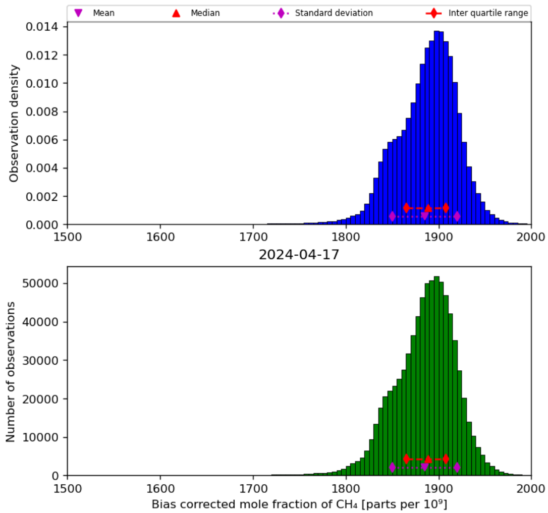
Figure 25: Histogram of “Bias corrected mole fraction of CH 4 ” for 2024-04-16 to 2024-04-18
