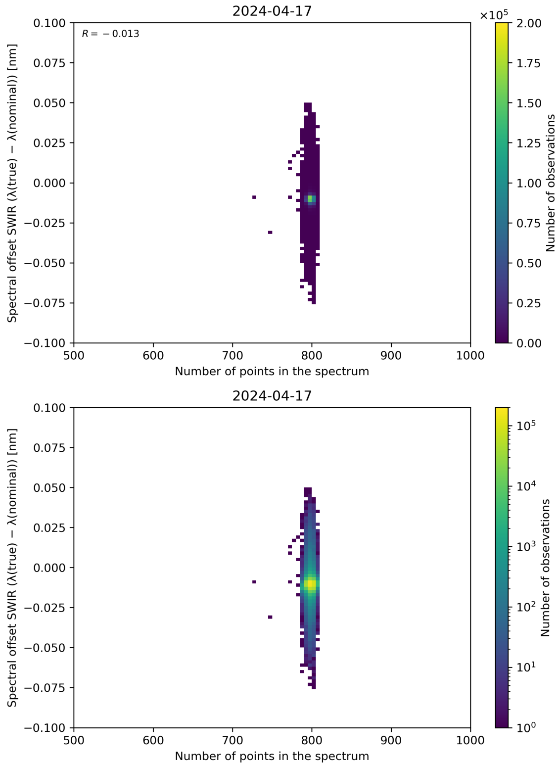
Figure 93: Scatter density plot of “Number of points in the spectrum” against “Spectral offset SWIR ( \lambda(\text{true}) - \lambda(\text{nominal}) )” for 2024-04-16 to 2024-04-18.
