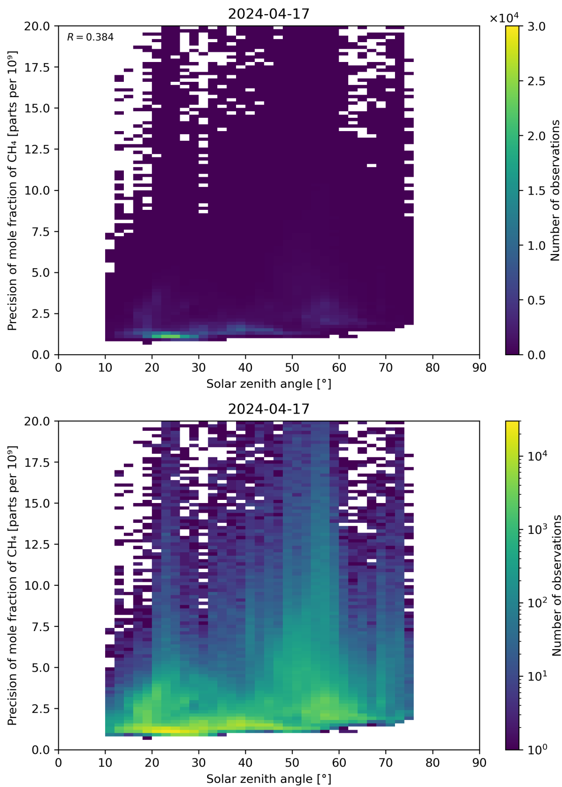
Figure 101: Scatter density plot of “Solar zenith angle” against “Precision of mole fraction of CH 4 ” for 2024-04-16 to 2024-04-18.
