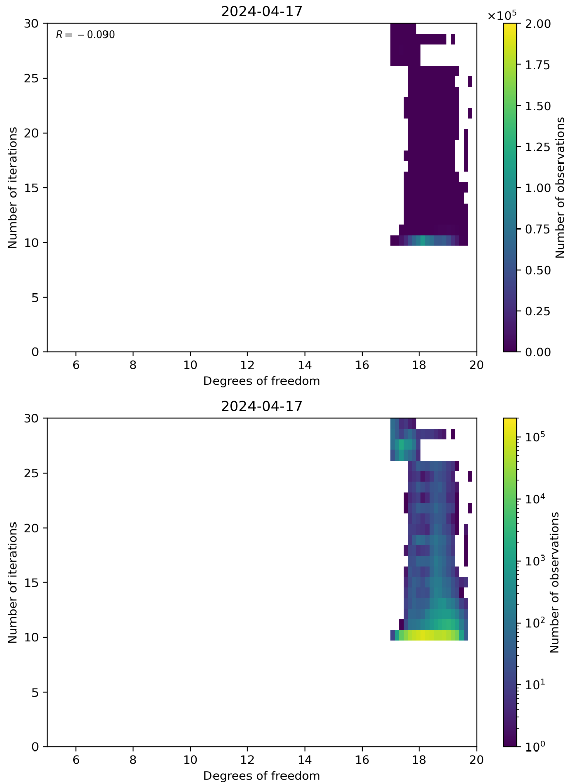
Figure 52: Scatter density plot of “Degrees of freedom” against “Number of iterations” for 2024-04-16 to 2024-04-18.
