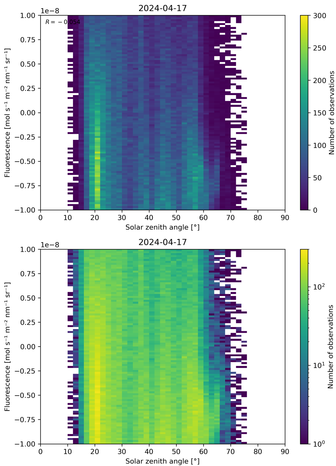
Figure 97: Scatter density plot of “Solar zenith angle” against “Fluorescence” for 2024-04-16 to 2024-04-18.
