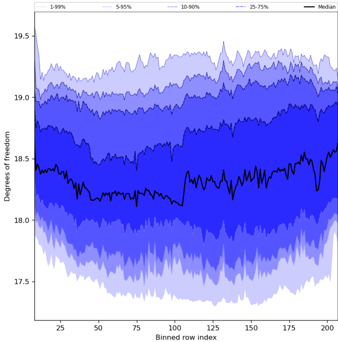
Figure 41: Along track statistics of “Degrees of freedom” for 2024-04-16 to 2024-04-18
