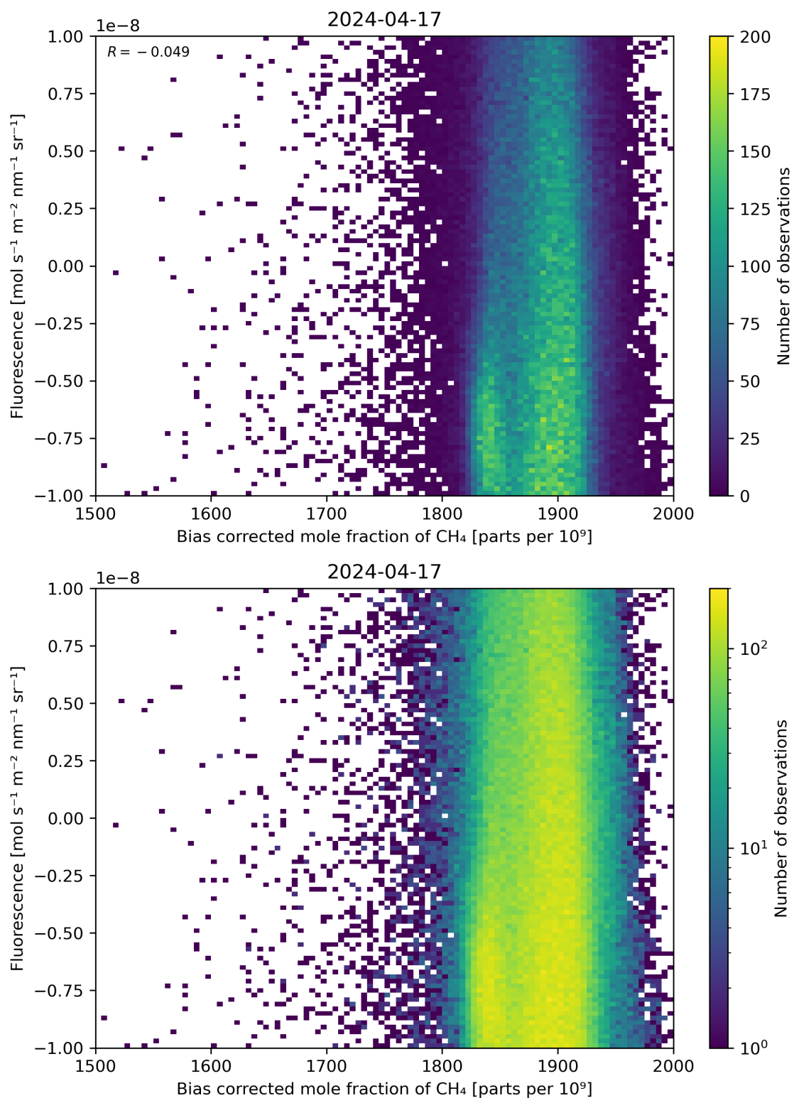
Figure 66: Scatter density plot of “Bias corrected mole fraction of \text{CH}_4 ” against “Fluorescence” for 2024-04-16 to 2024-04-18.
