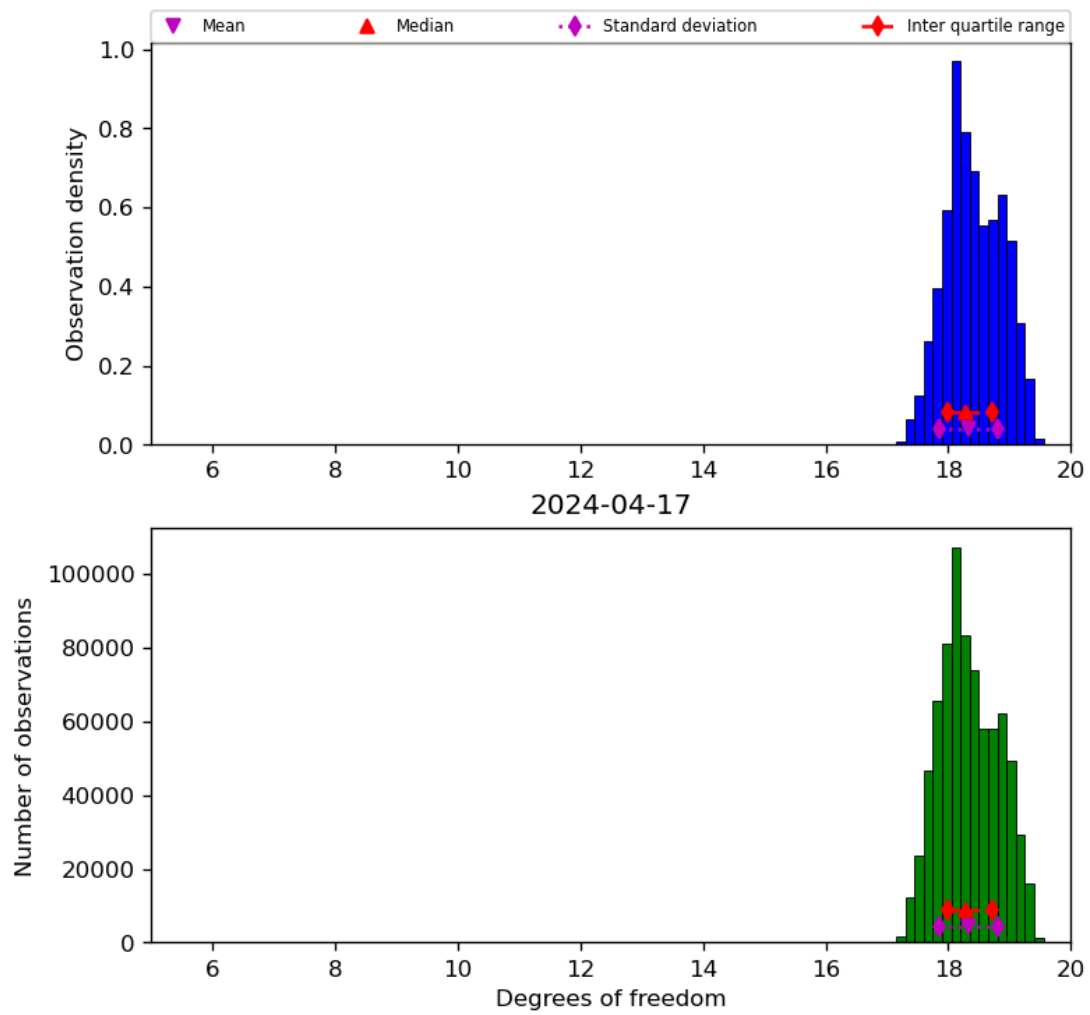
Figure 30: Histogram of “Degrees of freedom” for 2024-04-16 to 2024-04-18
