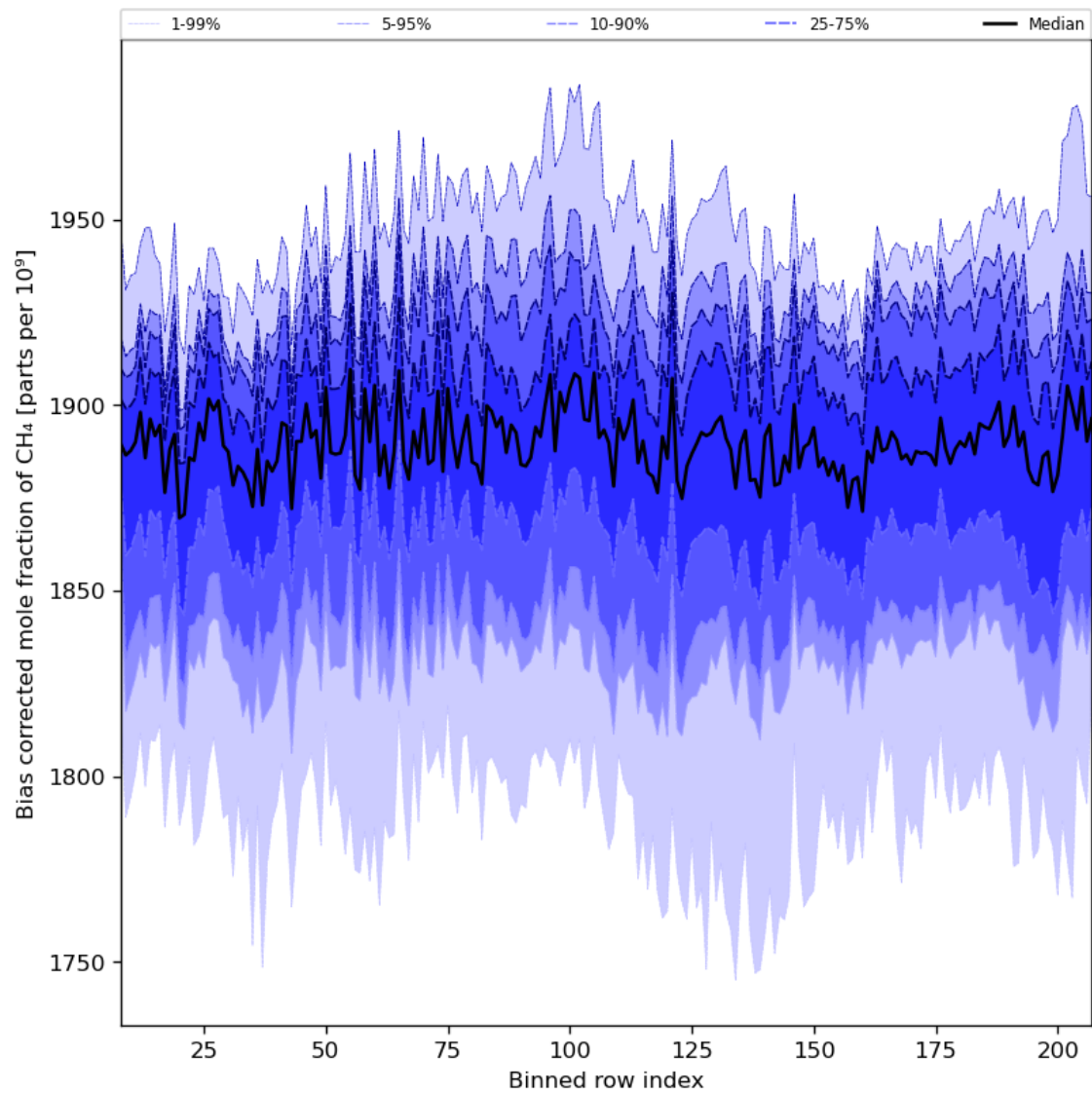
Figure 36: Along track statistics of “Bias corrected mole fraction of CH 4 ” for 2024-04-16 to 2024-04-18
