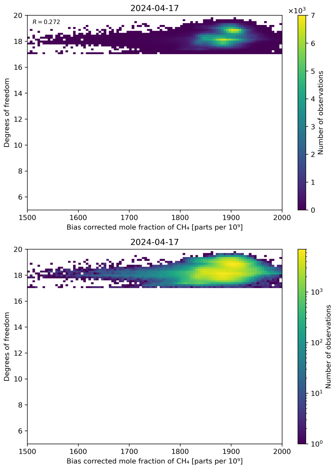
Figure 65: Scatter density plot of “Bias corrected mole fraction of CH 4 ” against “Degrees of freedom” for 2024-04-16 to 2024-04-18.
