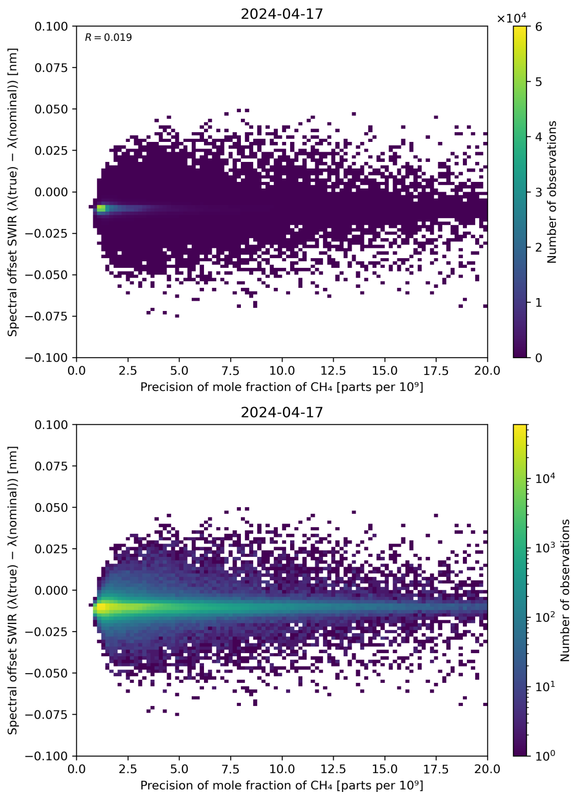
Figure 85: Scatter density plot of “Precision of mole fraction of \text{CH}_4 ” against “Spectral offset SWIR ( \lambda(\text{true}) - \lambda(\text{nominal}) )” for 2024-04-16 to 2024-04-18.
