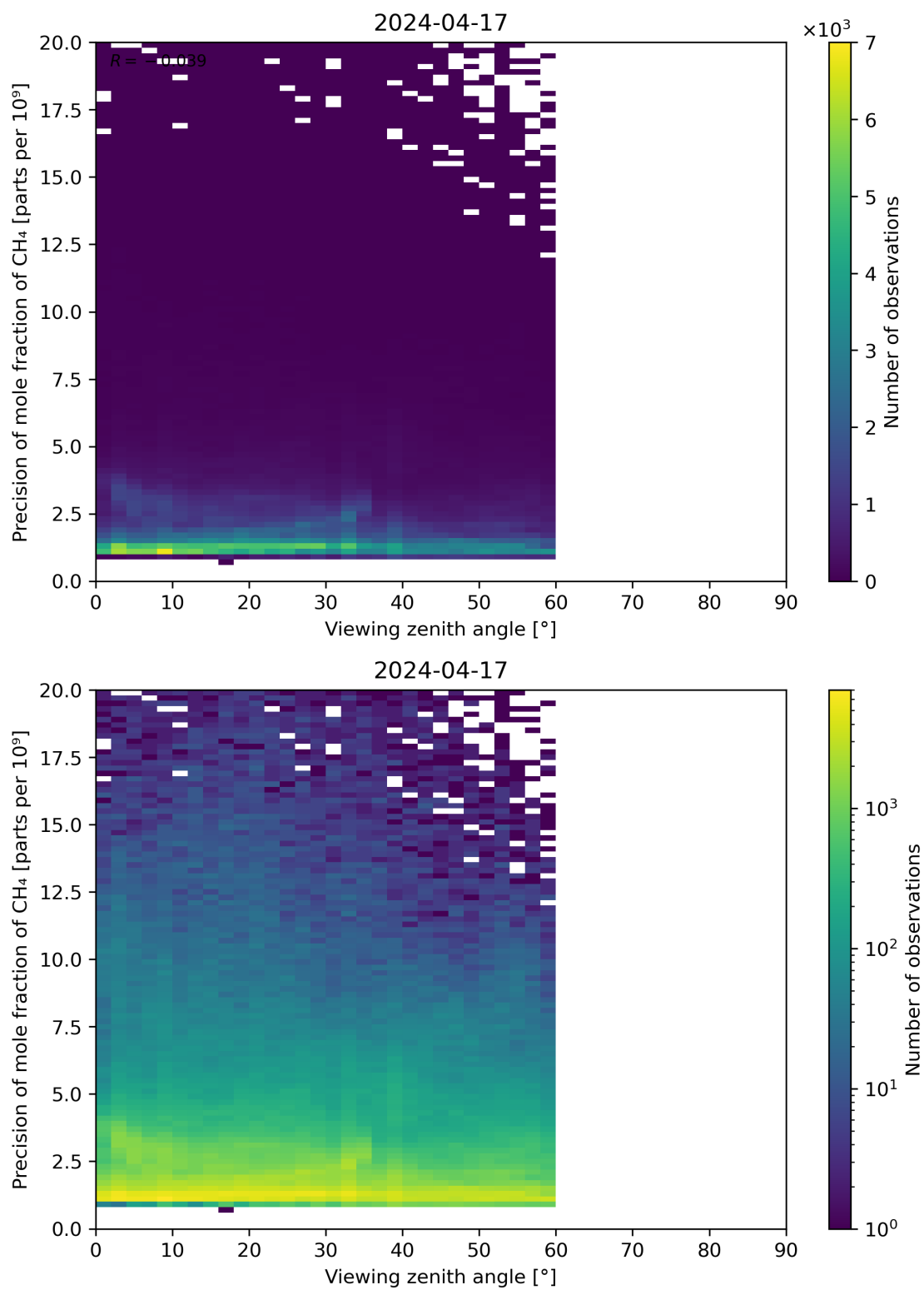
Figure 112: Scatter density plot of “Viewing zenith angle” against “Precision of mole fraction of CH 4 ” for 2024-04-16 to 2024-04-18.
