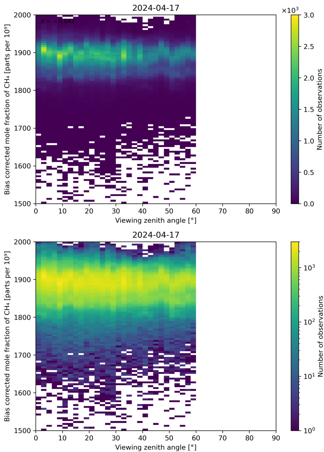
Figure 111: Scatter density plot of “Viewing zenith angle” against “Bias corrected mole fraction of \text{CH}_4 ” for 2024-04-16 to 2024-04-18.
