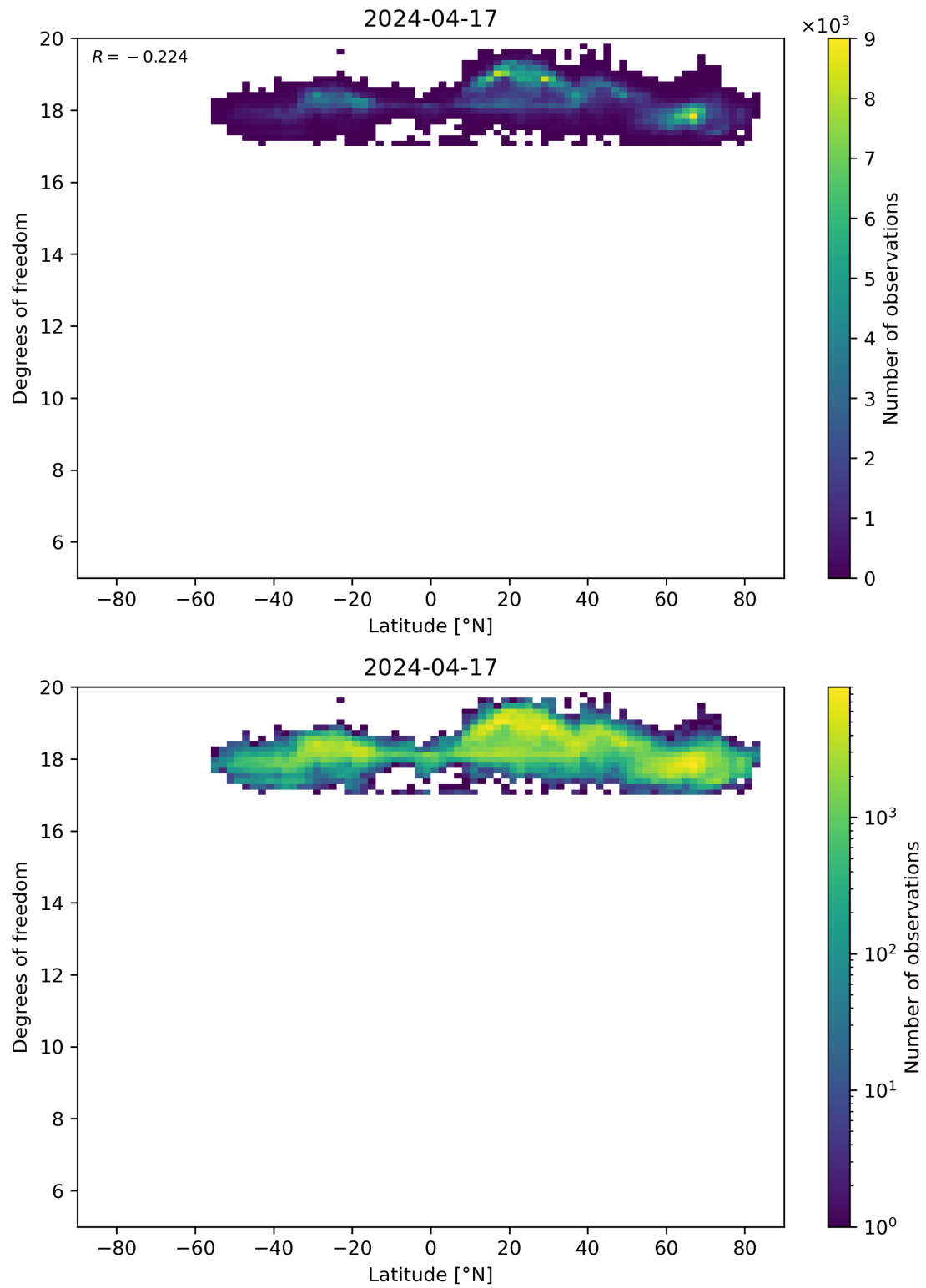
Figure 55: Scatter density plot of “Latitude” against “Degrees of freedom” for 2024-04-16 to 2024-04-18.
