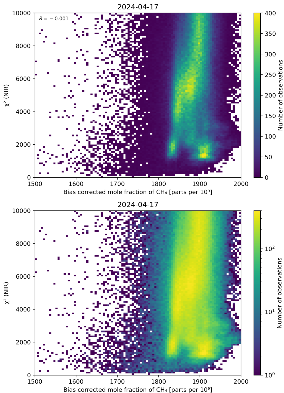
Figure 63: Scatter density plot of “Bias corrected mole fraction of CH 4 ” against “ \chi^2 (NIR)” for 2024-04-16 to 2024-04-18.
