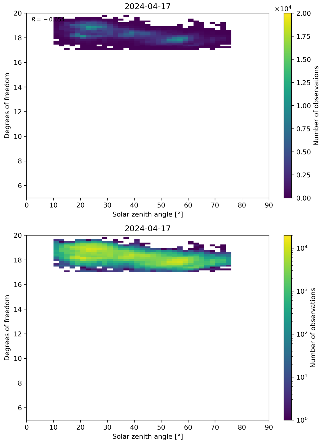
Figure 96: Scatter density plot of “Solar zenith angle” against “Degrees of freedom” for 2024-04-16 to 2024-04-18.
