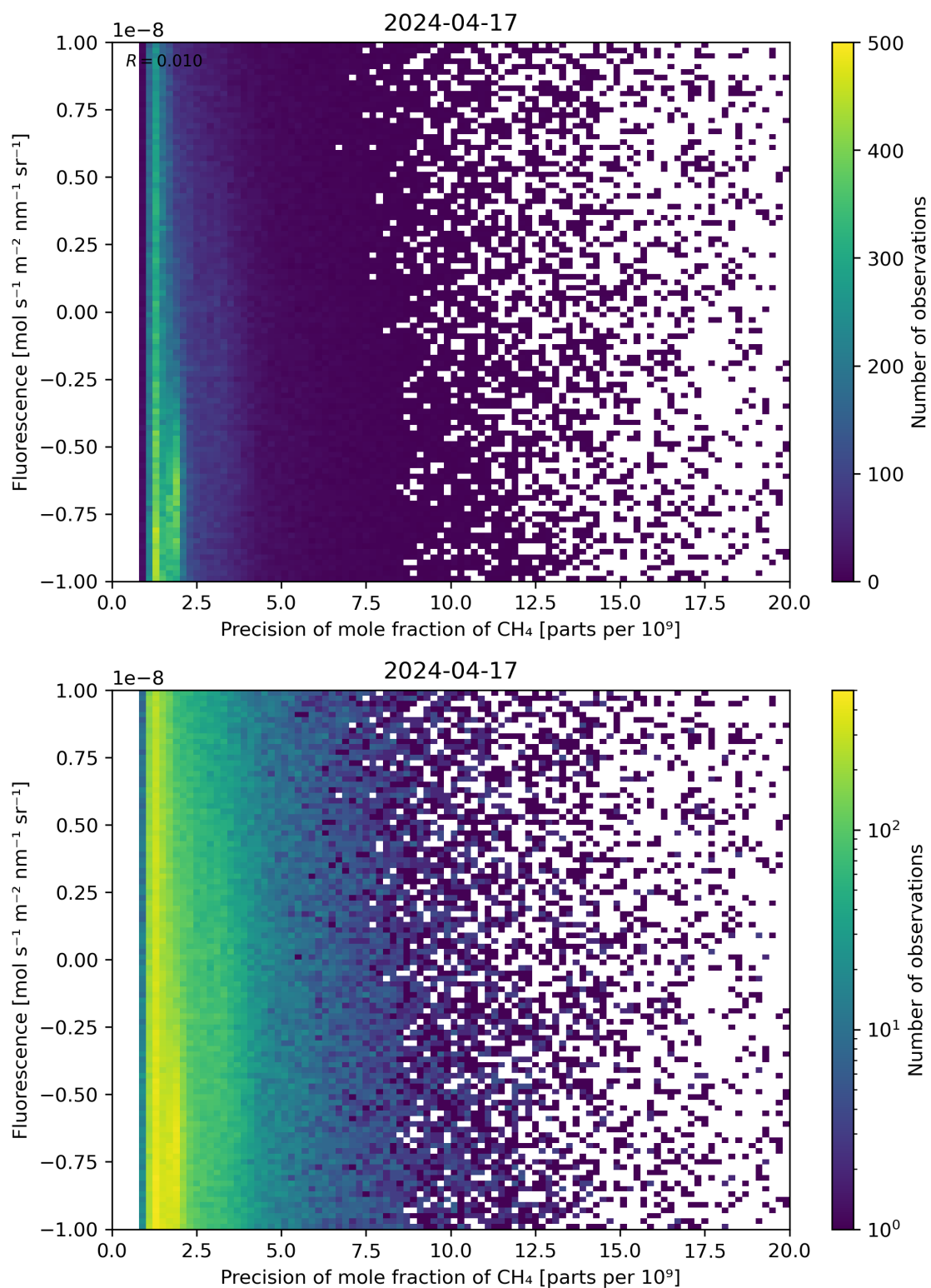
Figure 81: Scatter density plot of “Precision of mole fraction of \text{CH}_4 ” against “Fluorescence” for 2024-04-16 to 2024-04-18.
