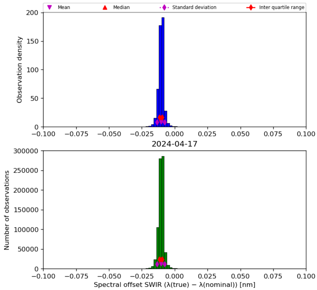
Figure 27: Histogram of “Spectral offset SWIR ( \lambda(\text{true}) - \lambda(\text{nominal}) )” for 2024-04-16 to 2024-04-18
