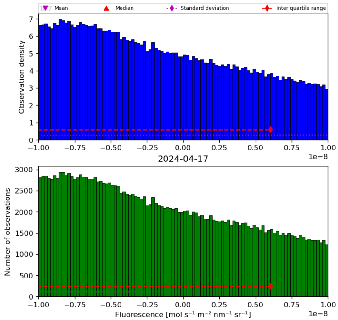
Figure 32: Histogram of “Fluorescence” for 2024-04-16 to 2024-04-18
