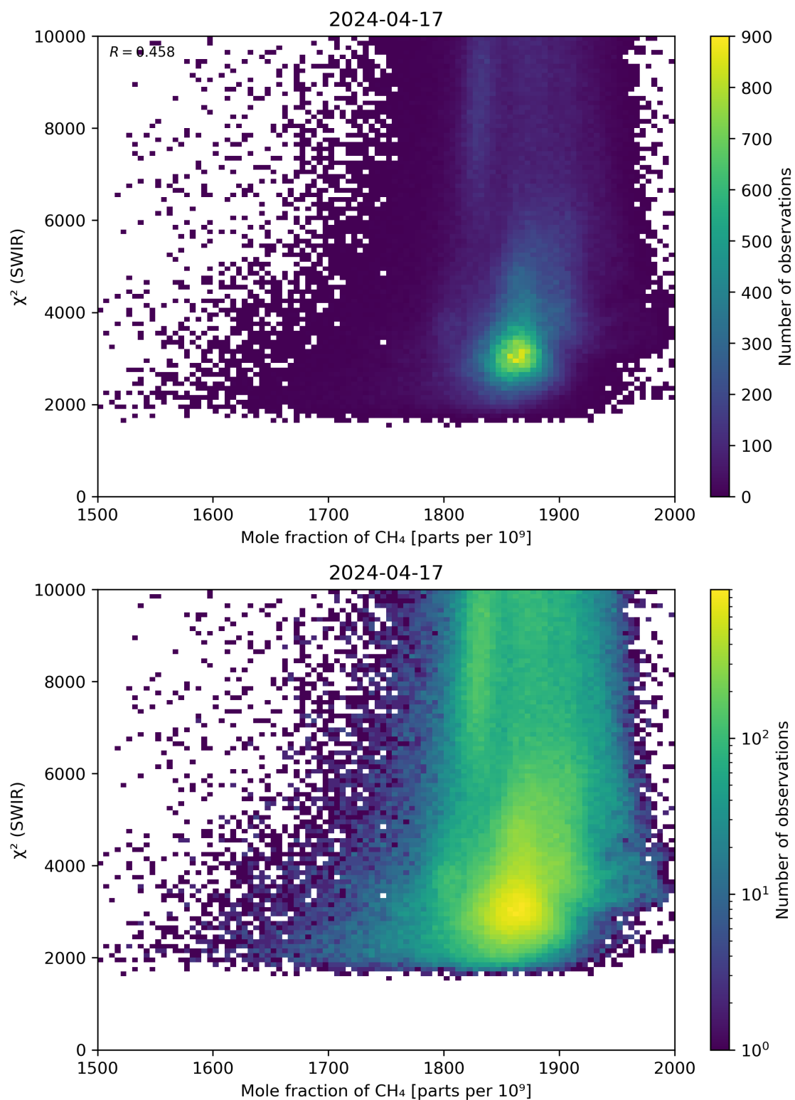
Figure 71: Scatter density plot of “Mole fraction of \text{CH}_4 ” against “ \chi^2 (SWIR)” for 2024-04-16 to 2024-04-18.
