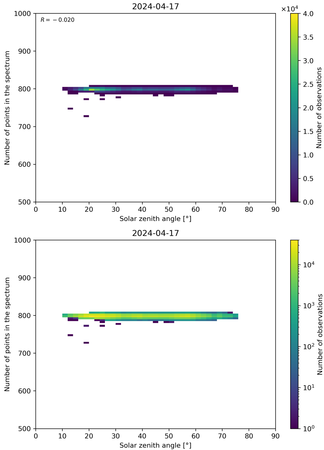
Figure 103: Scatter density plot of “Solar zenith angle” against “Number of points in the spectrum” for 2024-04-16 to 2024-04-18.
