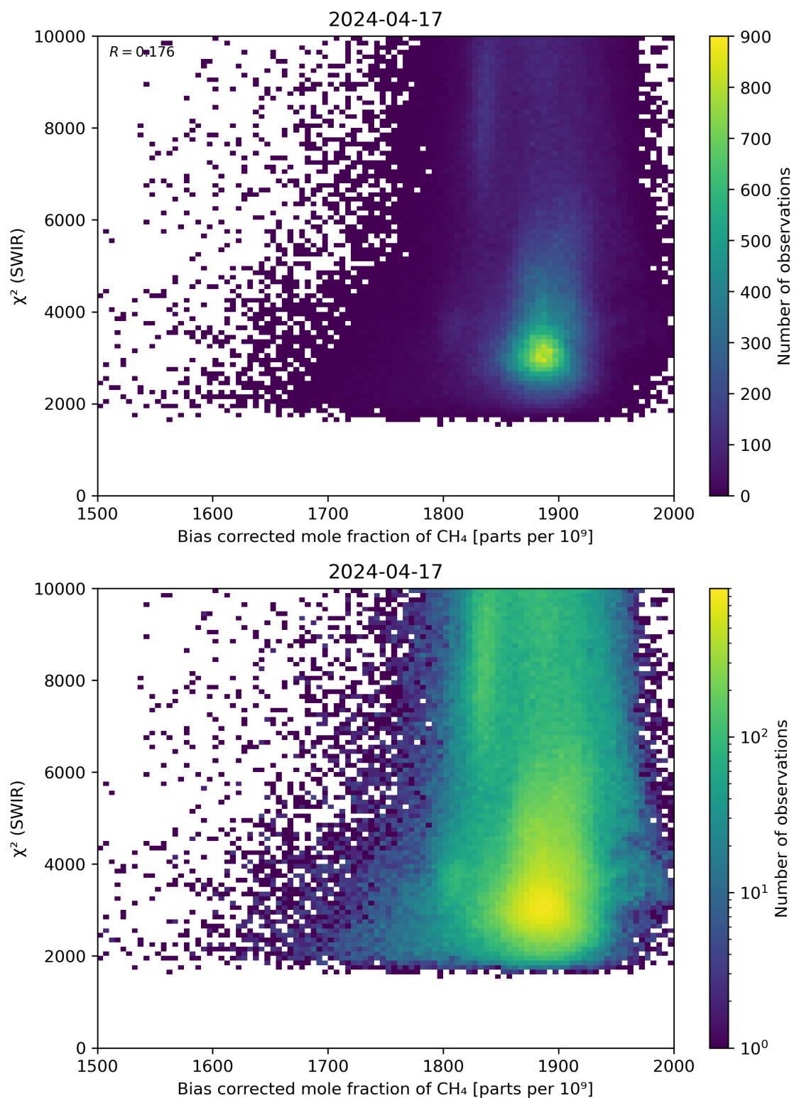
Figure 64: Scatter density plot of “Bias corrected mole fraction of \text{CH}_4 ” against “ \chi^2 (SWIR)” for 2024-04-16 to 2024-04-18.
