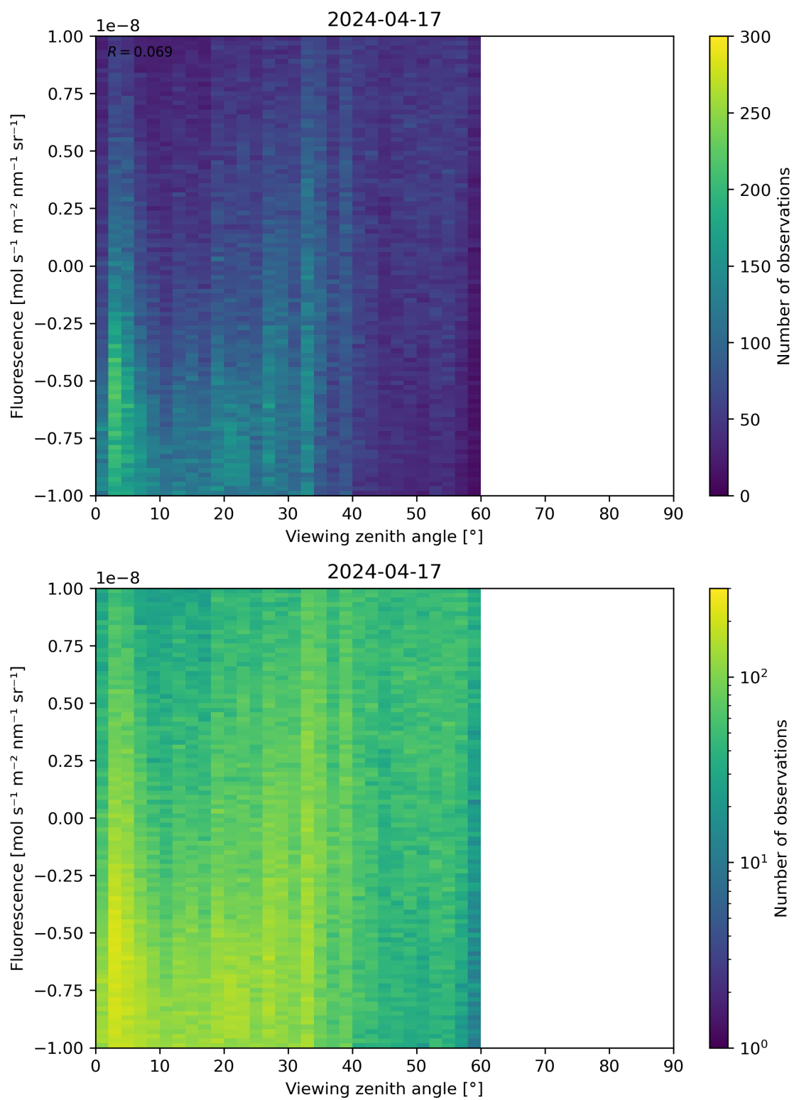
Figure 108: Scatter density plot of “Viewing zenith angle” against “Fluorescence” for 2024-04-16 to 2024-04-18.
