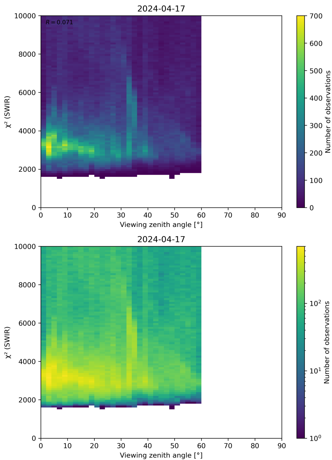
Figure 106: Scatter density plot of “Viewing zenith angle” against “ \chi^2 (SWIR)” for 2024-04-16 to 2024-04-18.
