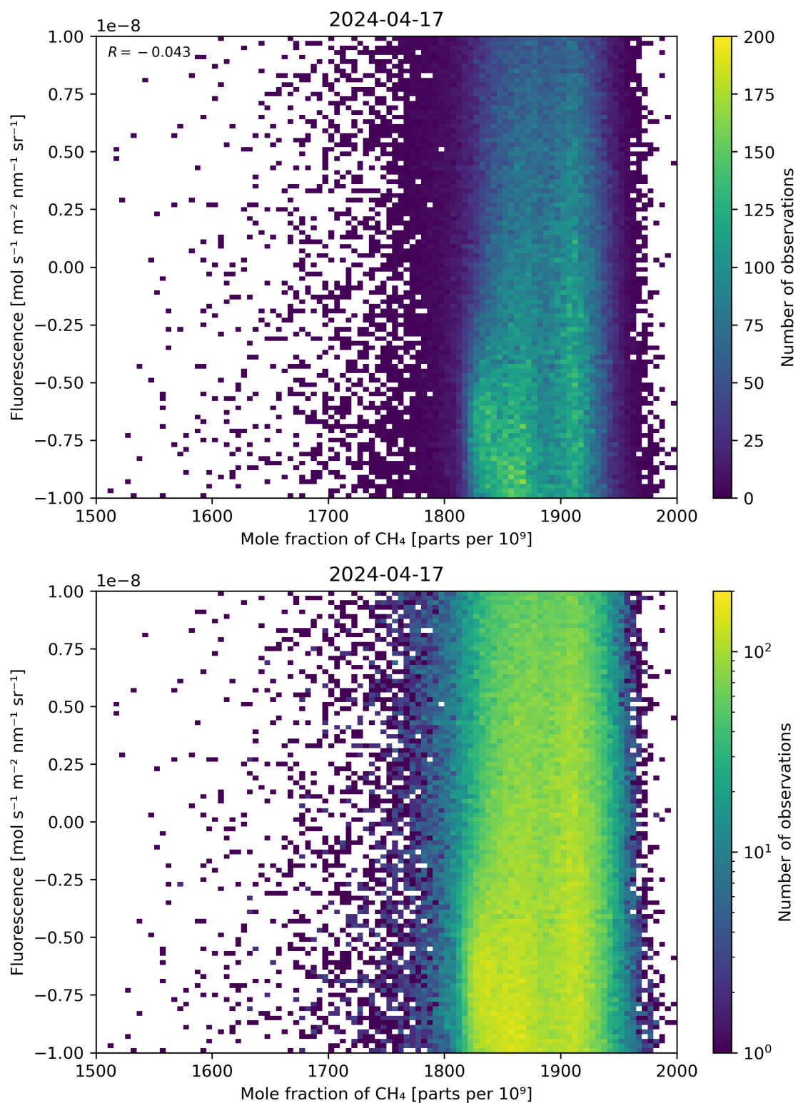
Figure 73: Scatter density plot of “Mole fraction of \text{CH}_4 ” against “Fluorescence” for 2024-04-16 to 2024-04-18.
