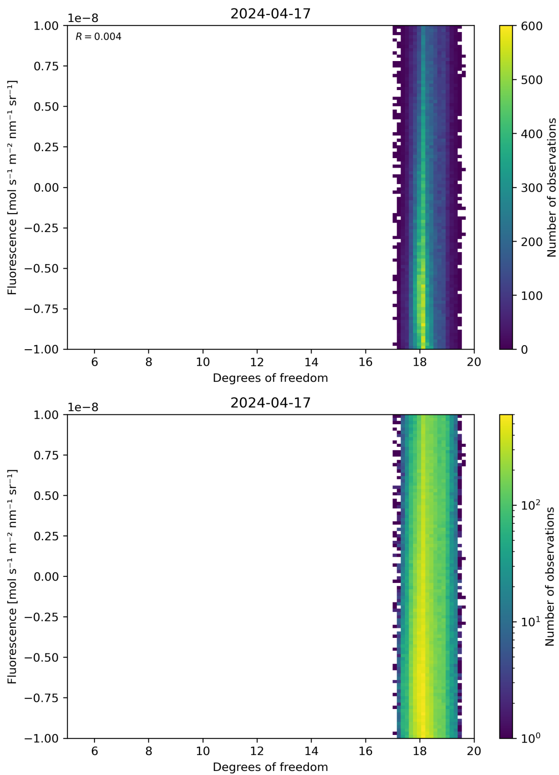
Figure 51: Scatter density plot of “Degrees of freedom” against “Fluorescence” for 2024-04-16 to 2024-04-18.
