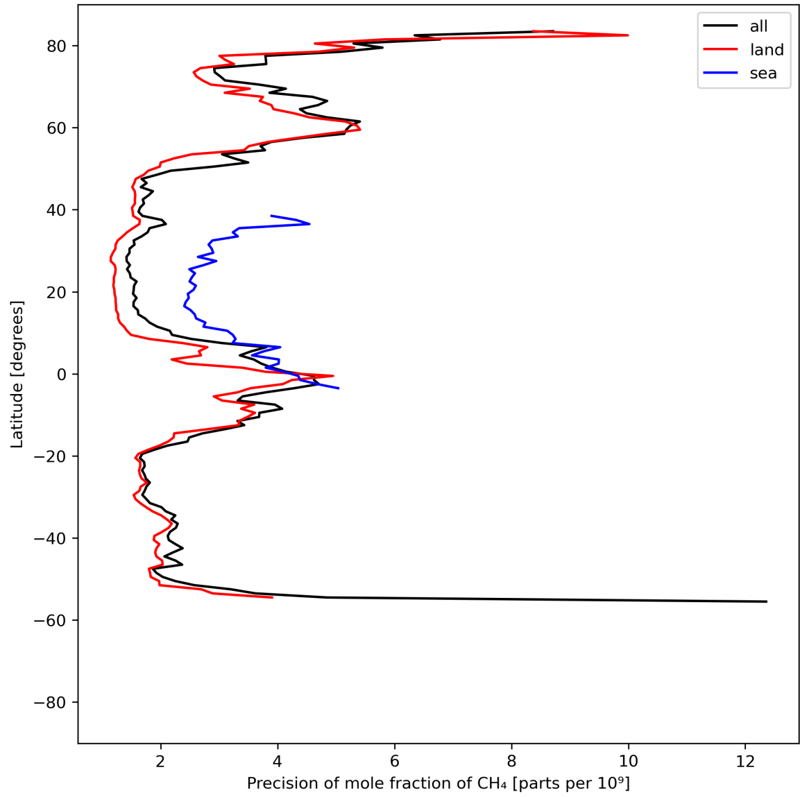
Figure 13: Zonal average of “Precision of mole fraction of CH 4 ” for 2024-04-16 to 2024-04-18.
