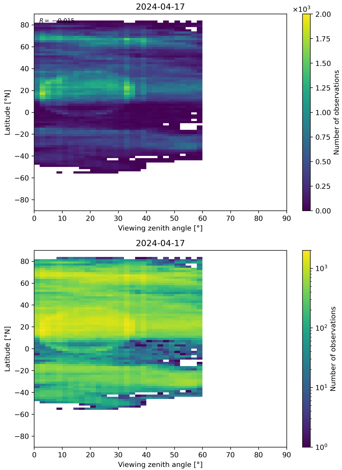
Figure 109: Scatter density plot of “Viewing zenith angle” against “Latitude” for 2024-04-16 to 2024-04-18.
