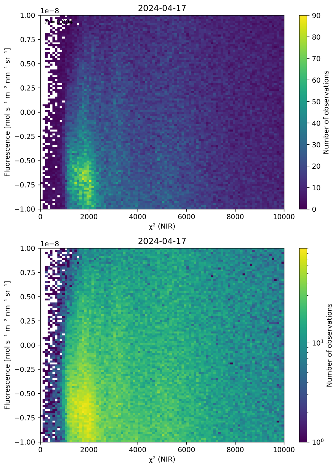
Figure 45: Scatter density plot of “ \chi^2 (NIR)” against “Fluorescence” for 2024-04-16 to 2024-04-18.
