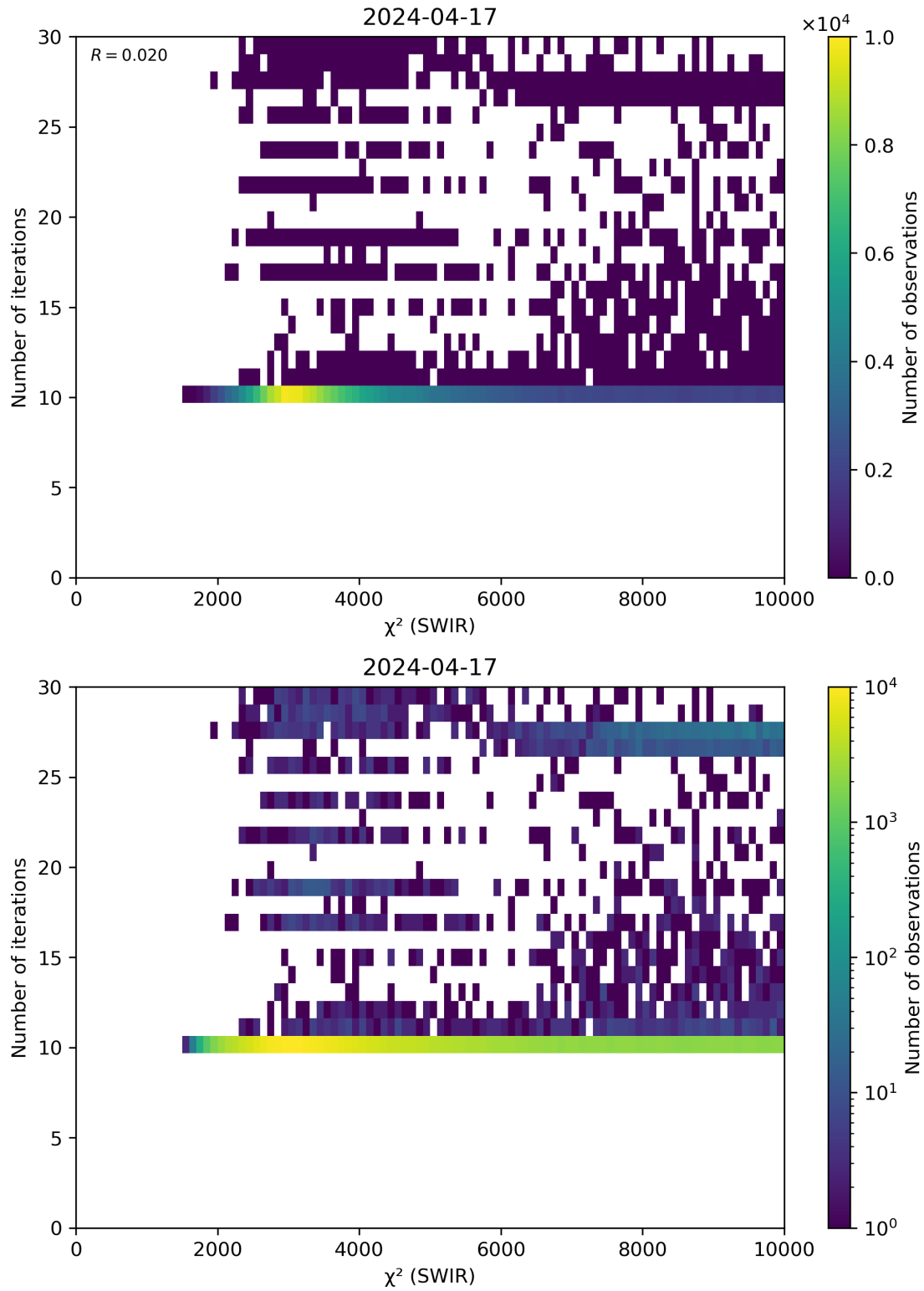
Figure 50: Scatter density plot of “ \chi^2 (SWIR)” against “Number of iterations” for 2024-04-16 to 2024-04-18.
