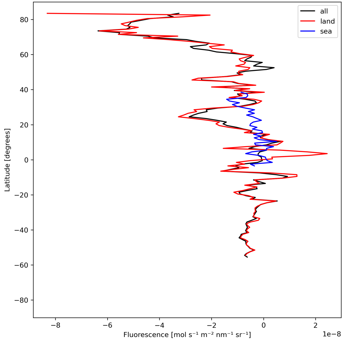
Figure 21: Zonal average of “Fluorescence” for 2024-04-16 to 2024-04-18.
