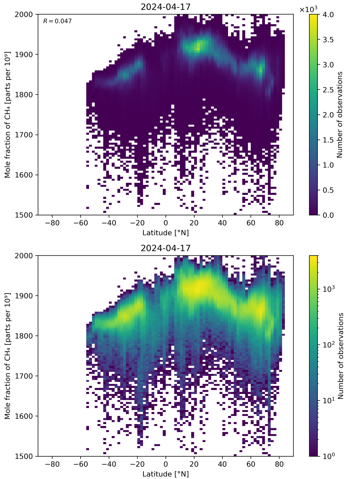
Figure 57: Scatter density plot of “Latitude” against “Mole fraction of \text{CH}_4 ” for 2024-04-16 to 2024-04-18.
