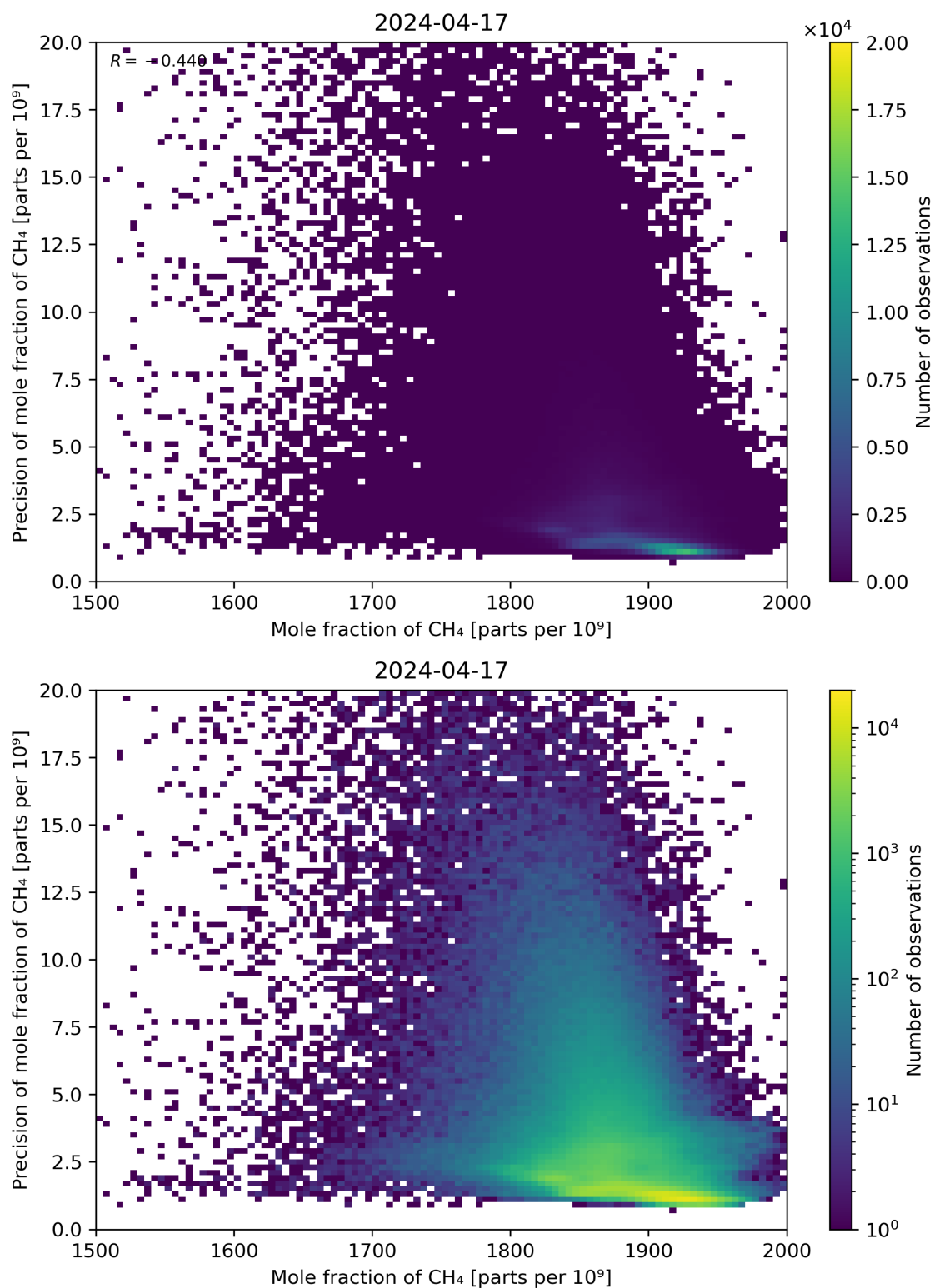
Figure 75: Scatter density plot of “Mole fraction of CH 4 ” against “Precision of mole fraction of CH 4 ” for 2024-04-16 to 2024-04-18.
