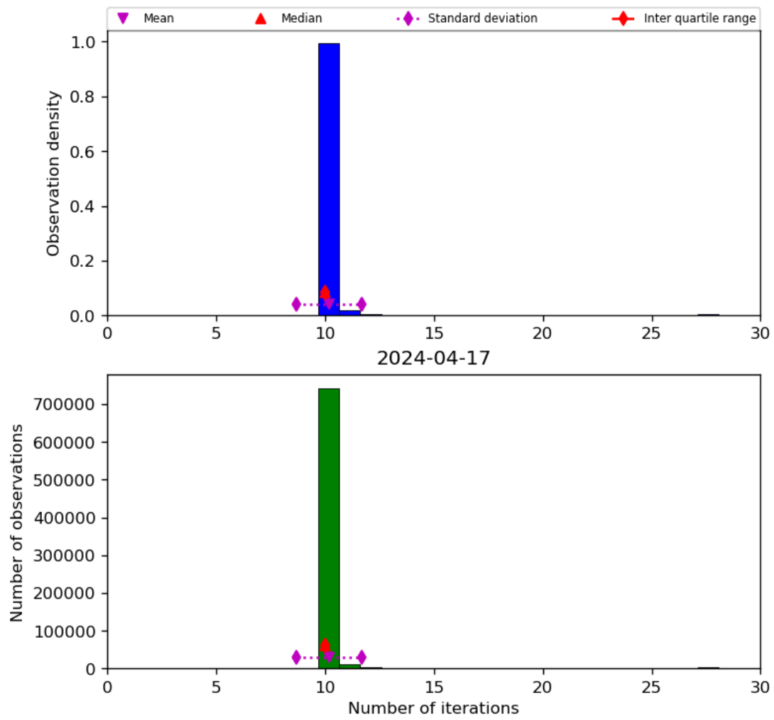
Figure 31: Histogram of “Number of iterations” for 2024-04-16 to 2024-04-18
