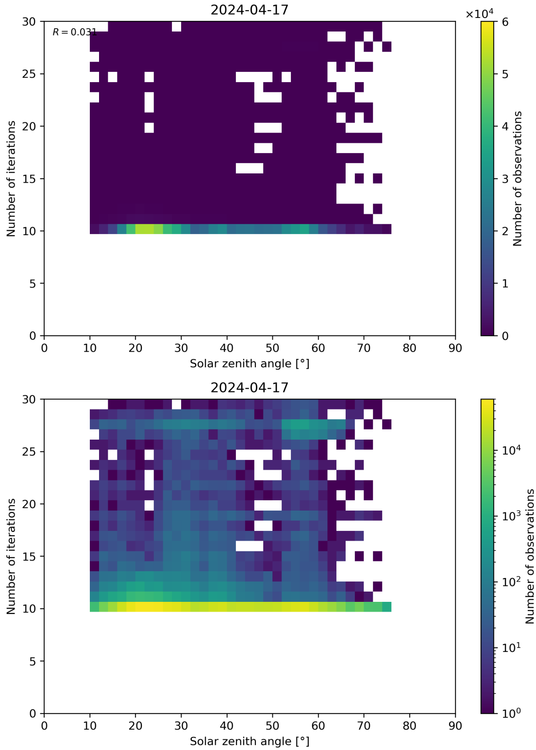
Figure 102: Scatter density plot of “Solar zenith angle” against “Number of iterations” for 2024-04-16 to 2024-04-18.
