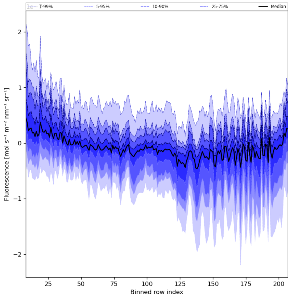
Figure 43: Along track statistics of “Fluorescence” for 2024-04-16 to 2024-04-18
