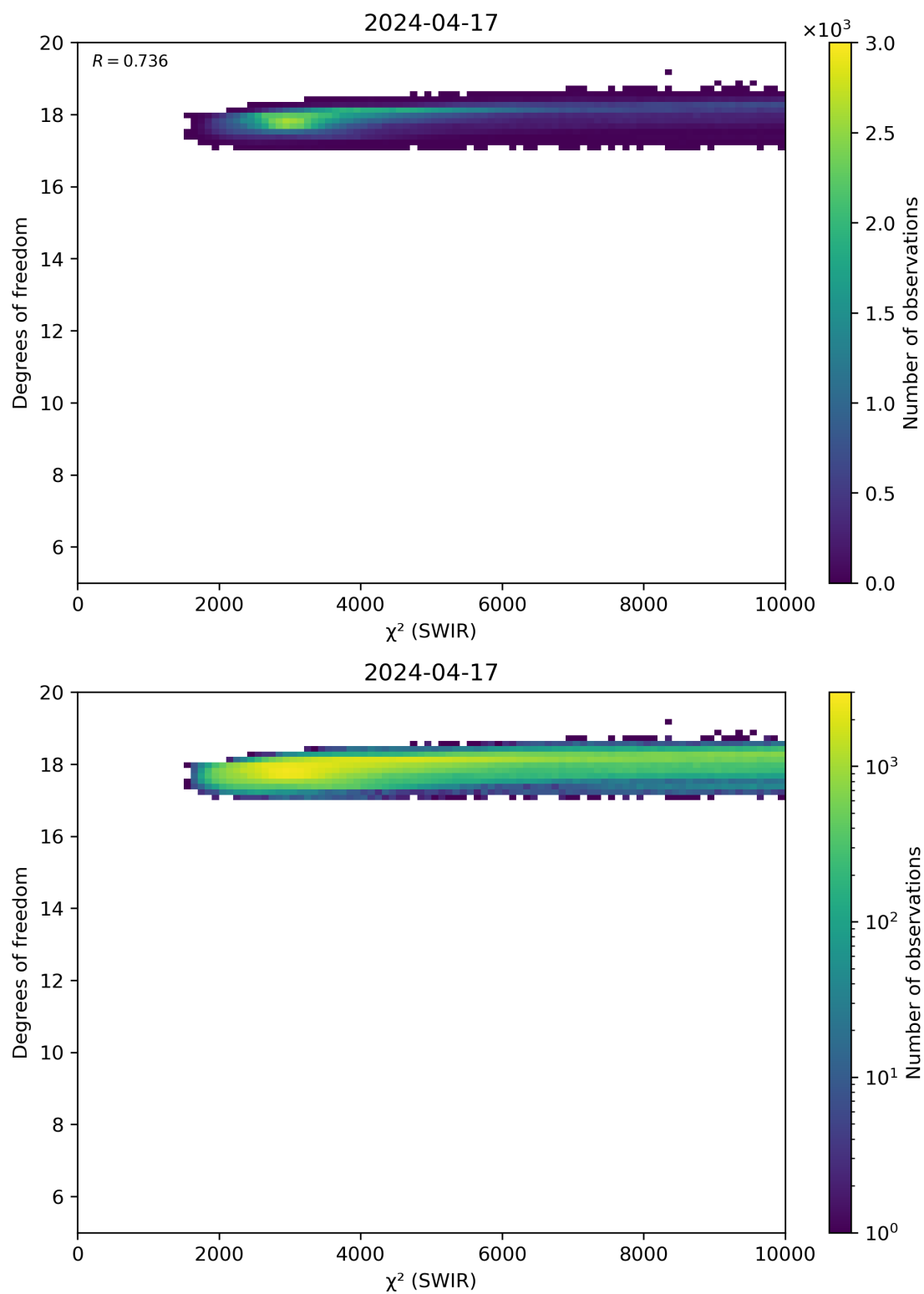
Figure 48: Scatter density plot of “ \chi^2 (SWIR)” against “Degrees of freedom” for 2024-04-16 to 2024-04-18.
