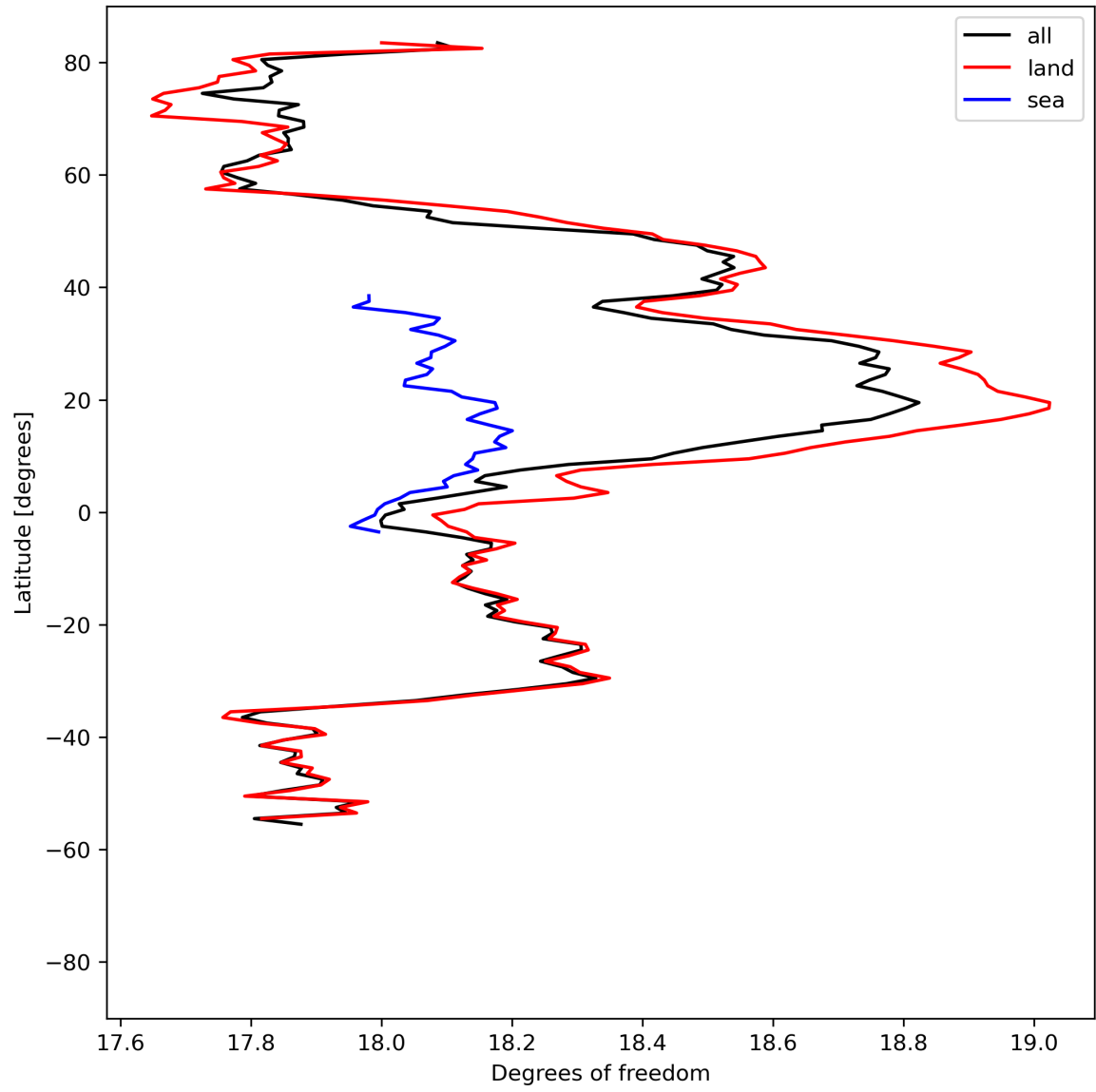
Figure 19: Zonal average of “Degrees of freedom” for 2024-04-16 to 2024-04-18.
