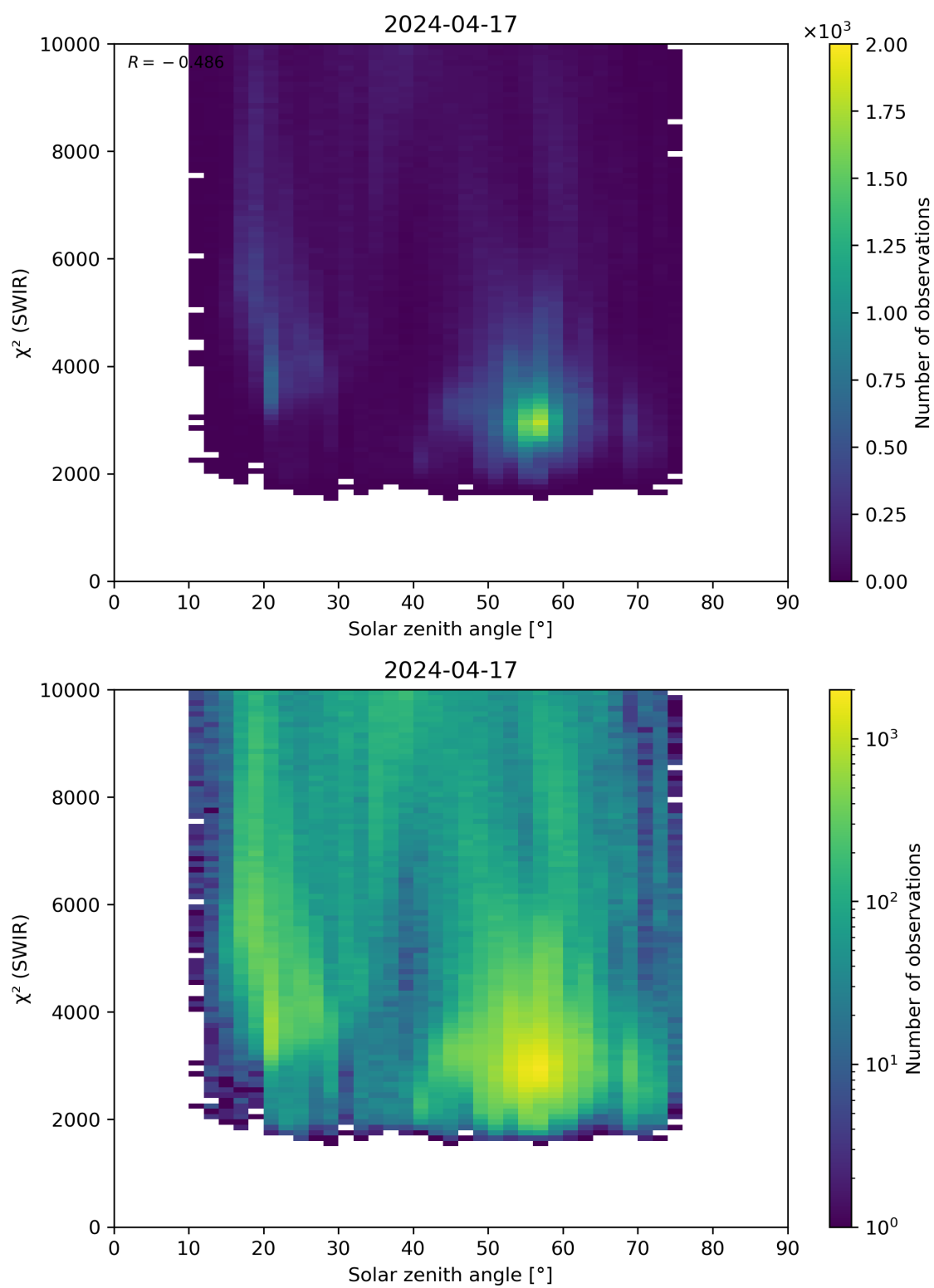
Figure 95: Scatter density plot of “Solar zenith angle” against “ \chi^2 (SWIR)” for 2024-04-16 to 2024-04-18.
