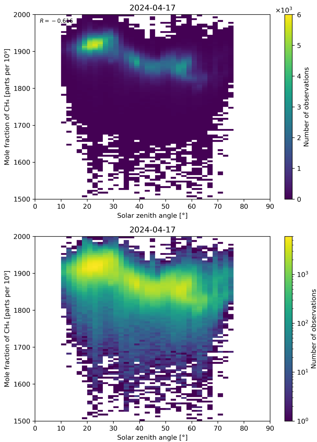
Figure 99: Scatter density plot of “Solar zenith angle” against “Mole fraction of CH 4 ” for 2024-04-16 to 2024-04-18.
