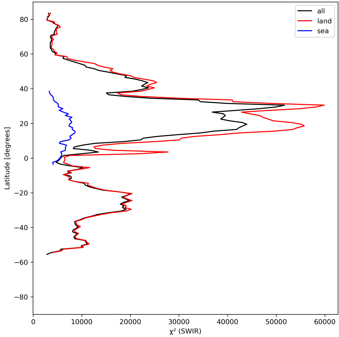
Figure 17: Zonal average of “ \chi^2 (SWIR)” for 2024-04-16 to 2024-04-18.
