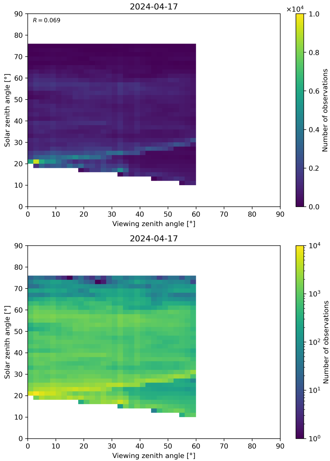
Figure 115: Scatter density plot of “Viewing zenith angle” against “Solar zenith angle” for 2024-04-16 to 2024-04-18.
