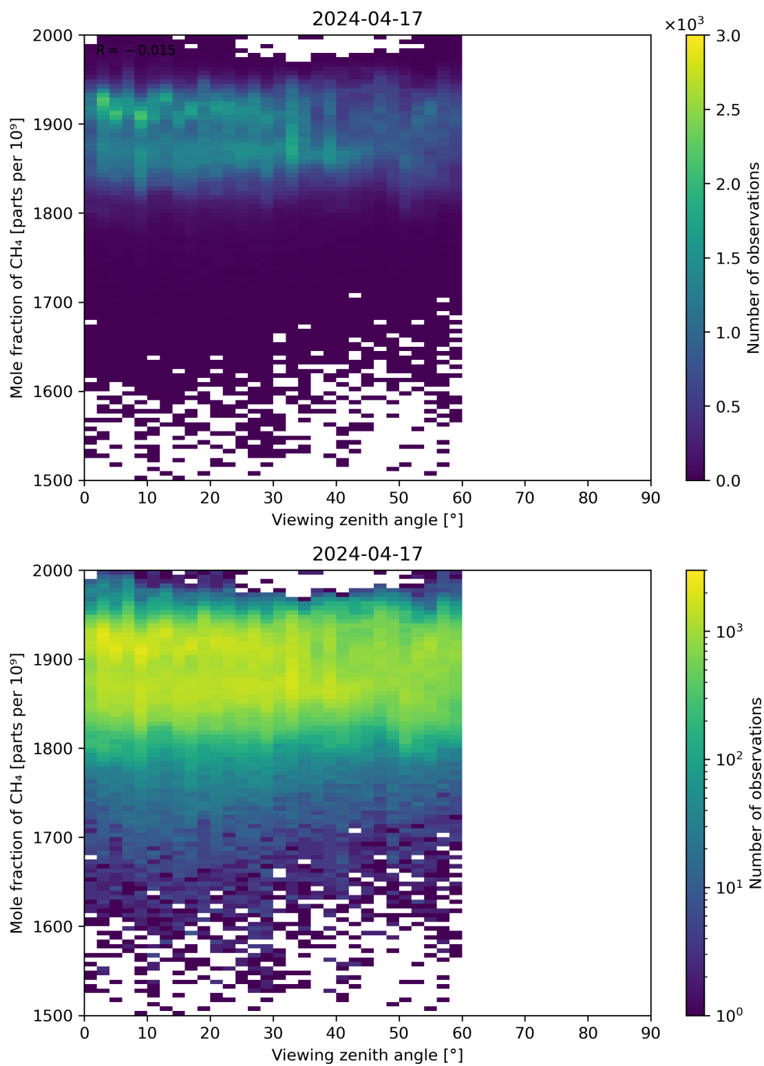
Figure 110: Scatter density plot of “Viewing zenith angle” against “Mole fraction of CH 4 ” for 2024-04-16 to 2024-04-18.
