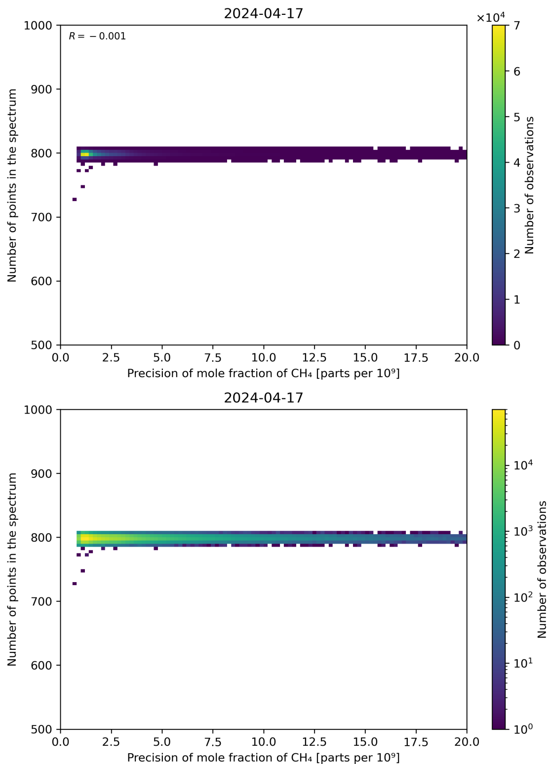
Figure 84: Scatter density plot of “Precision of mole fraction of CH 4 ” against “Number of points in the spectrum” for 2024-04-16 to 2024-04-18.
