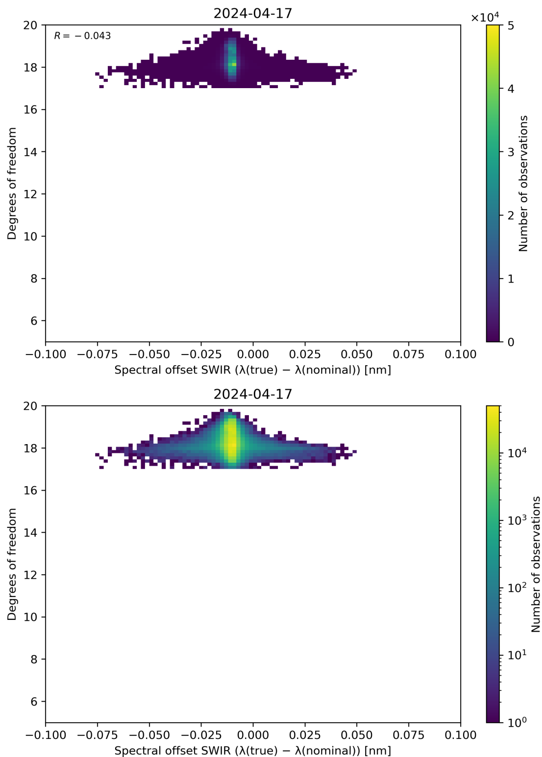
Figure 119: Scatter density plot of “Spectral offset SWIR ( \lambda(\text{true}) - \lambda(\text{nominal}) )” against “Degrees of freedom” for 2024-04-16 to 2024-04-18.
