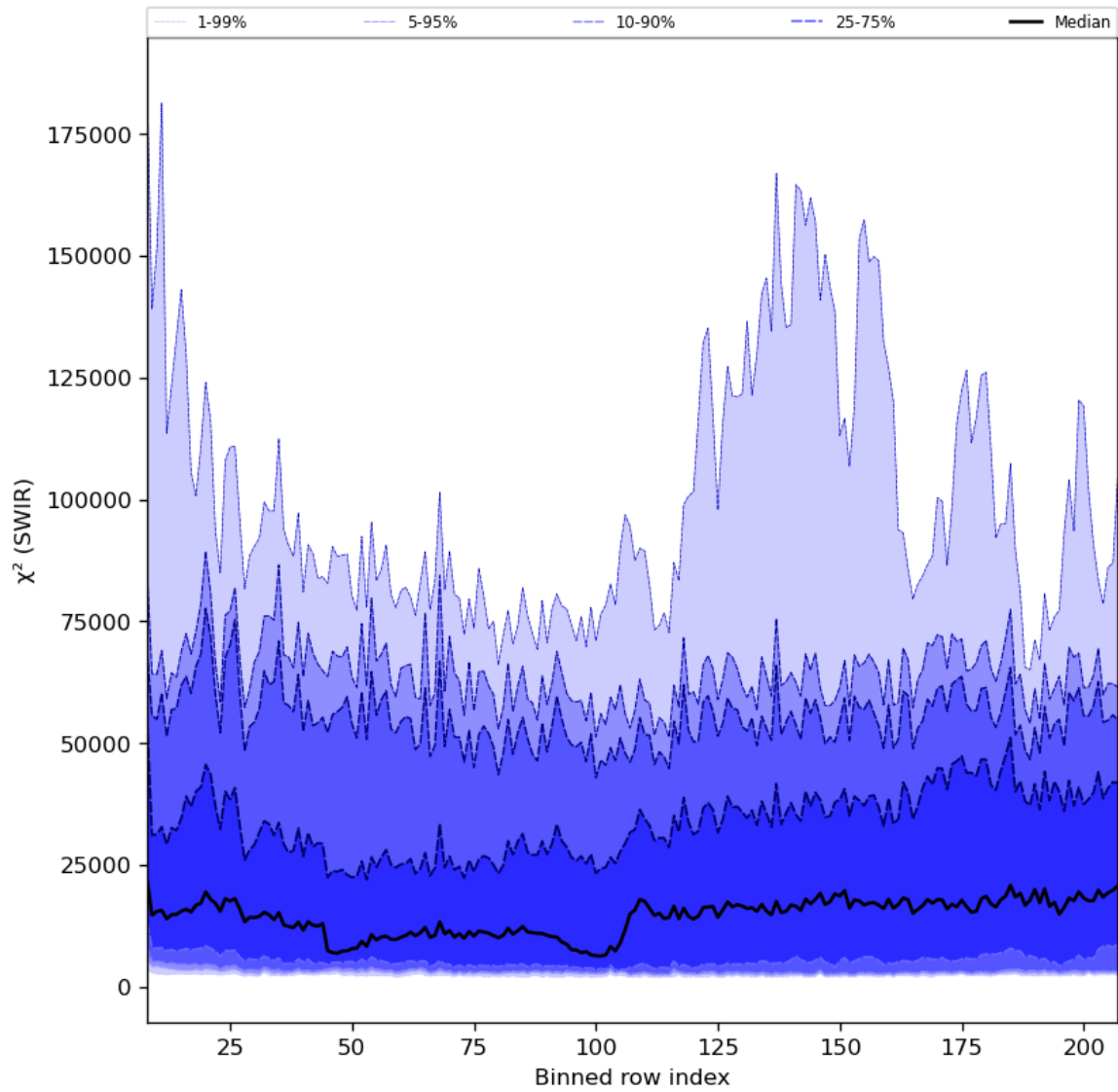
Figure 39: Along track statistics of “ \chi^2 (SWIR)” for 2024-04-16 to 2024-04-18
