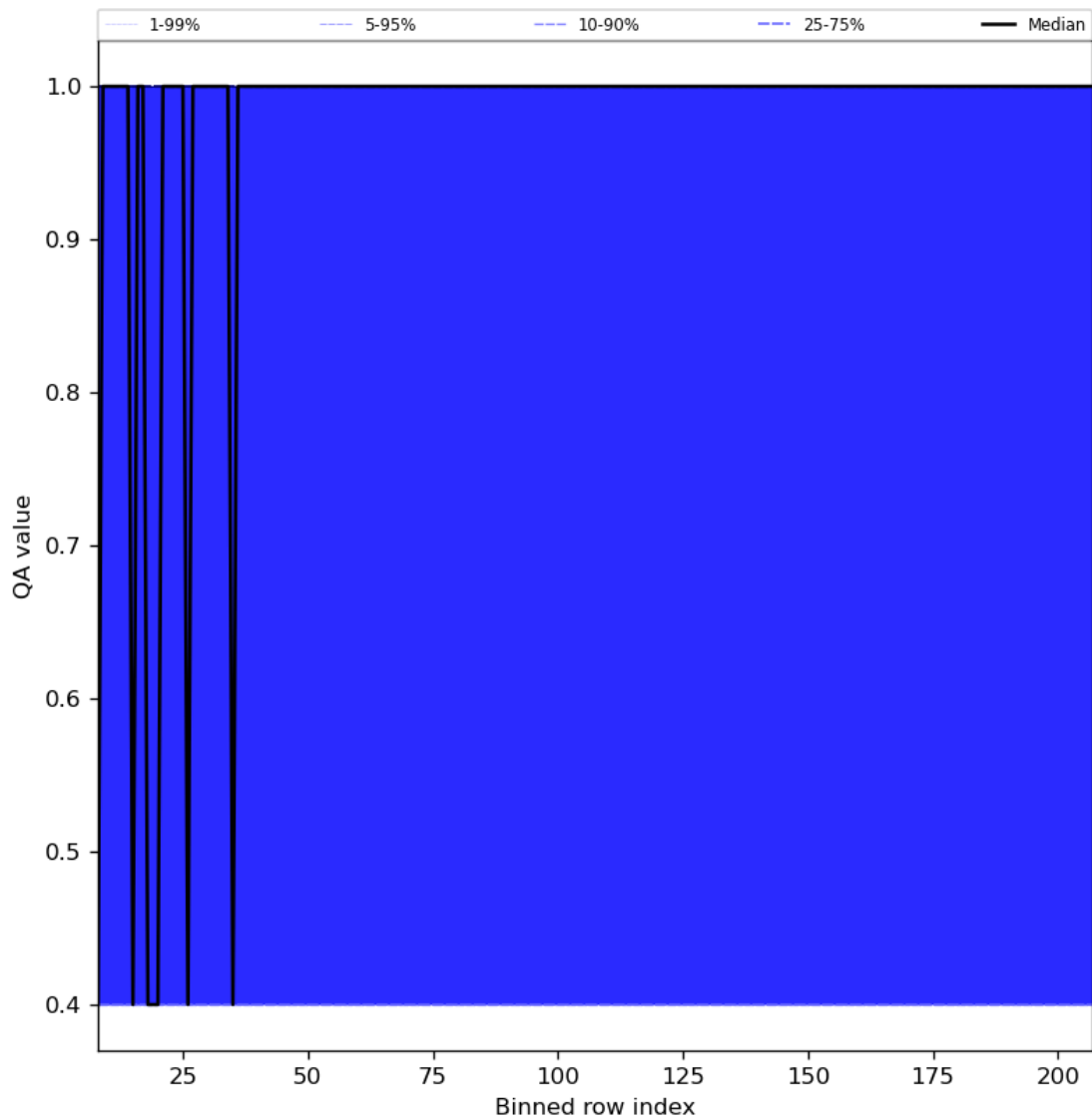
Figure 33: Along track statistics of “QA value” for 2024-04-16 to 2024-04-18
