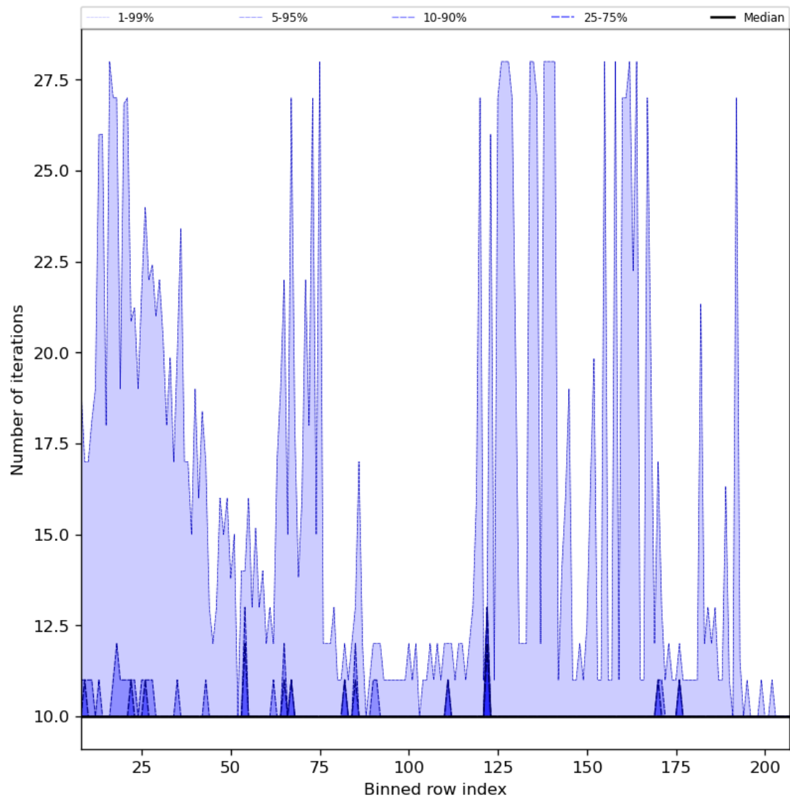
Figure 42: Along track statistics of “Number of iterations” for 2024-04-16 to 2024-04-18
