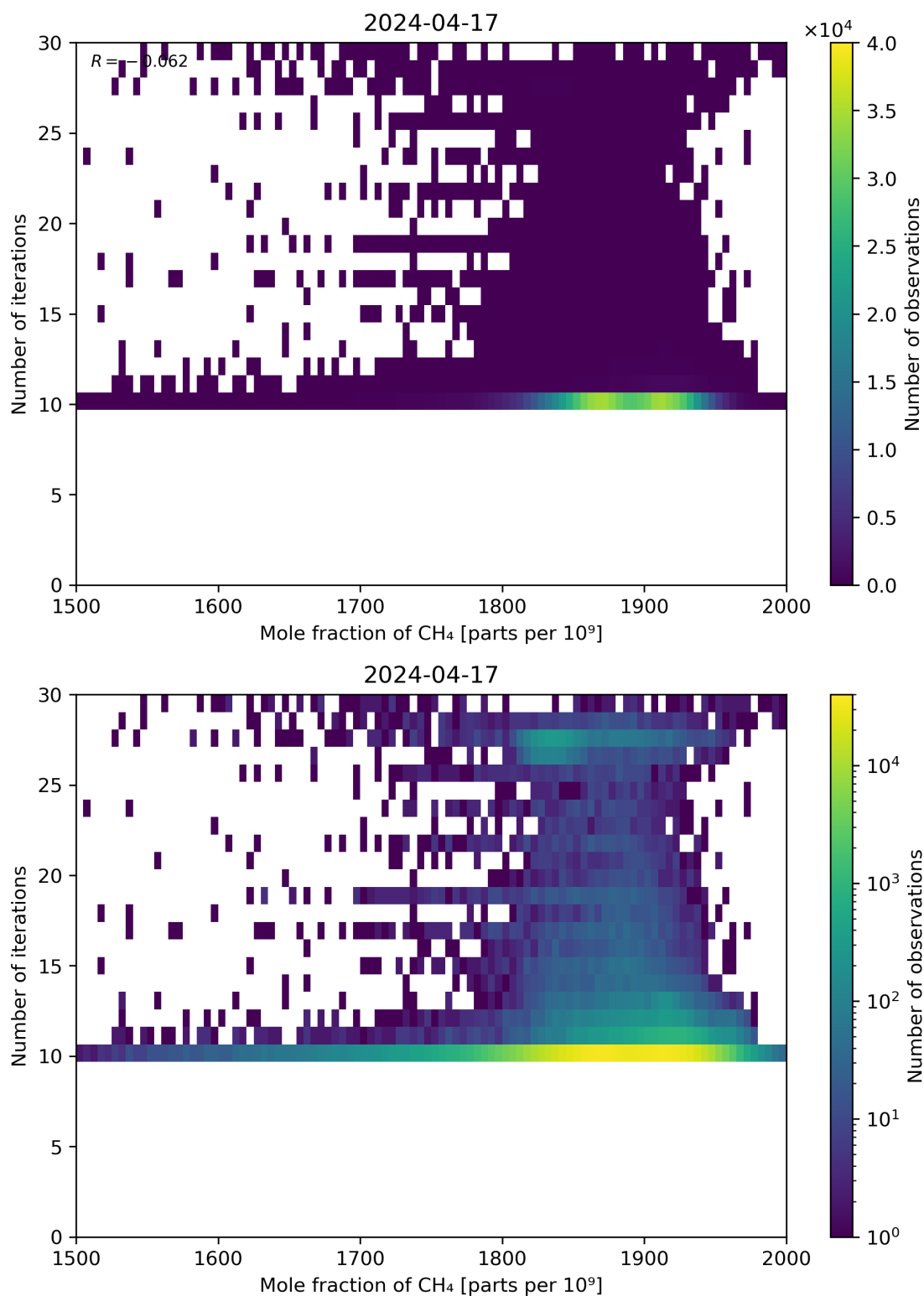
Figure 76: Scatter density plot of “Mole fraction of CH 4 ” against “Number of iterations” for 2024-04-16 to 2024-04-18.
