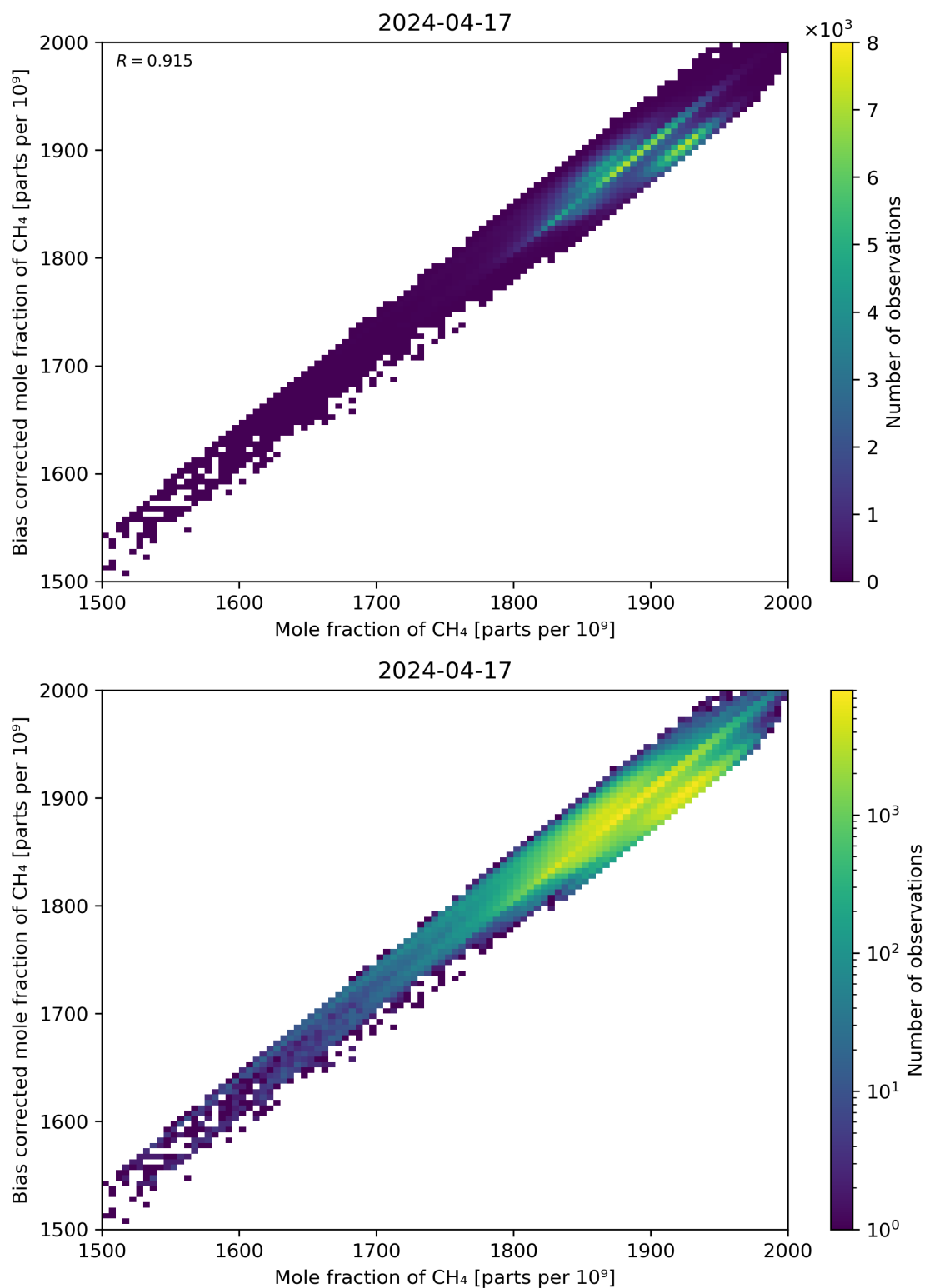
Figure 74: Scatter density plot of “Mole fraction of CH 4 ” against “Bias corrected mole fraction of CH 4 ” for 2024-04-16 to 2024-04-18.
