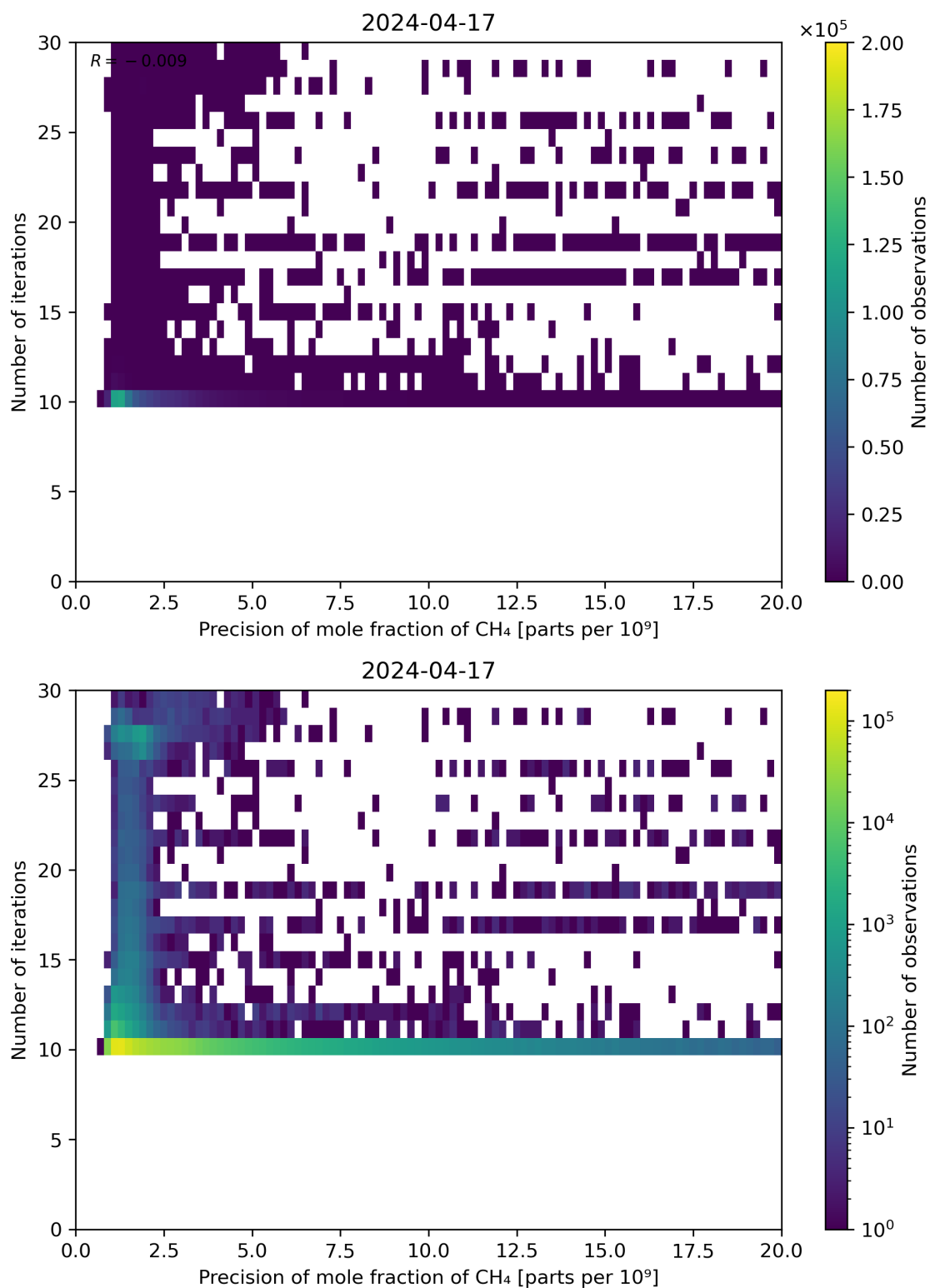
Figure 83: Scatter density plot of “Precision of mole fraction of CH 4 ” against “Number of iterations” for 2024-04-16 to 2024-04-18.
