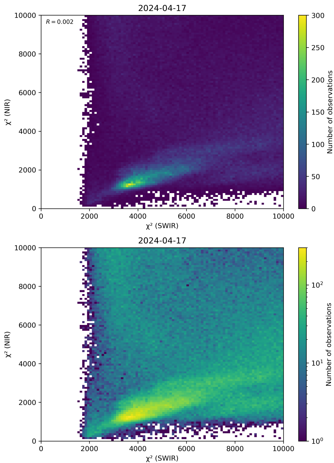
Figure 47: Scatter density plot of “ \chi^2 (SWIR)” against “ \chi^2 (NIR)” for 2024-04-16 to 2024-04-18.
