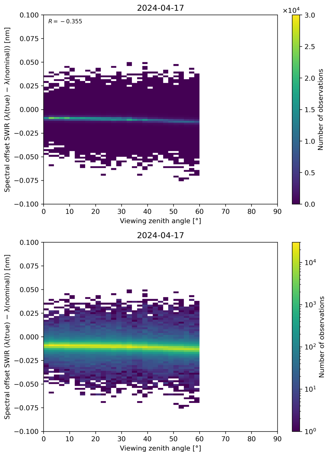
Figure 116: Scatter density plot of “Viewing zenith angle” against “Spectral offset SWIR ( \lambda(\text{true}) - \lambda(\text{nominal}) )” for 2024-04-16 to 2024-04-18.
