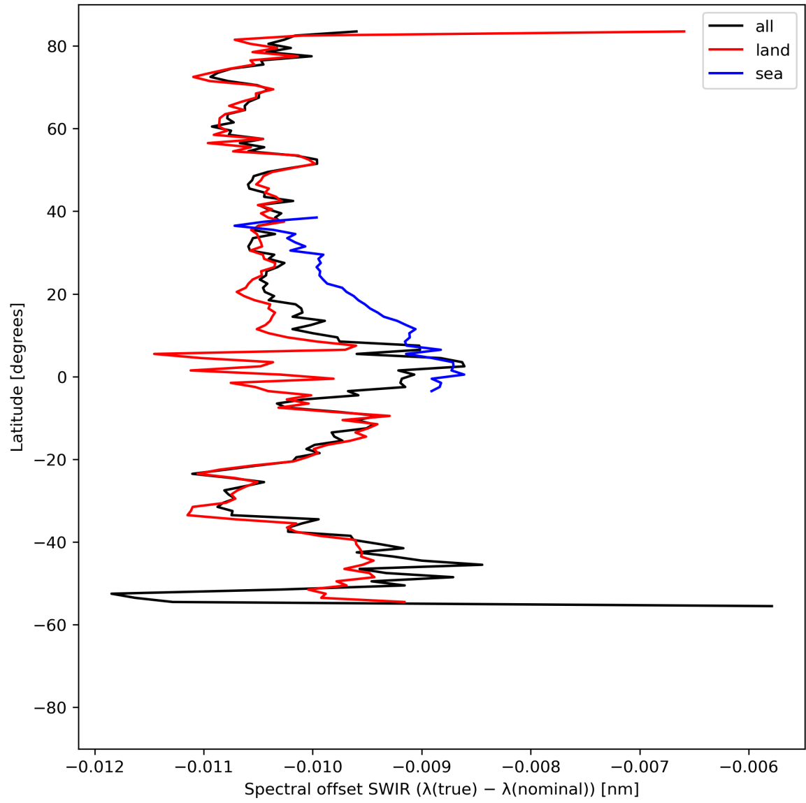
Figure 16: Zonal average of “Spectral offset SWIR ( \lambda(\text{true}) - \lambda(\text{nominal}) )” for 2024-04-16 to 2024-04-18.
