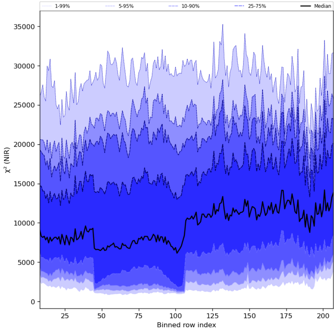
Figure 40: Along track statistics of “ \chi^2 (NIR)” for 2024-04-16 to 2024-04-18
