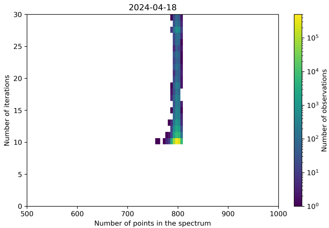
Figure 92: Scatter density plot of “Number of points in the spectrum” against “Number of iterations” for 2024-04-17 to 2024-04-19.
