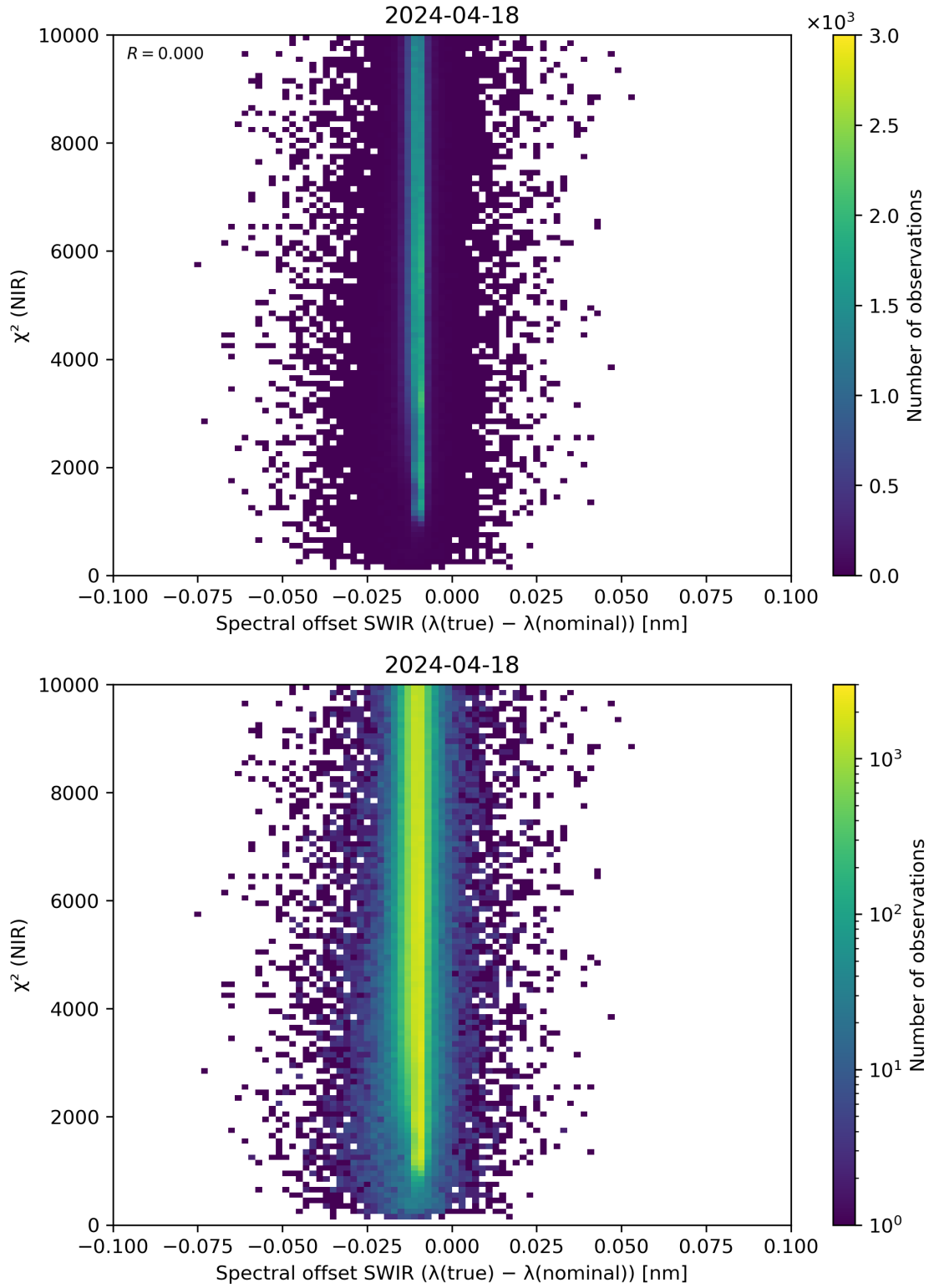
Figure 117: Scatter density plot of “Spectral offset SWIR ( \lambda(\text{true}) - \lambda(\text{nominal}) )” against “ \chi^2 (NIR)” for 2024-04-17 to 2024-04-19.
