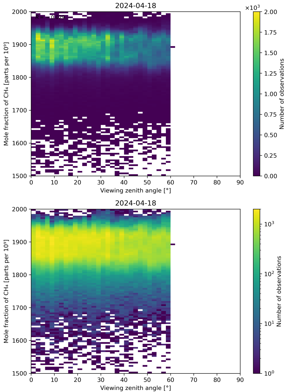
Figure 110: Scatter density plot of “Viewing zenith angle” against “Mole fraction of CH 4 ” for 2024-04-17 to 2024-04-19.
