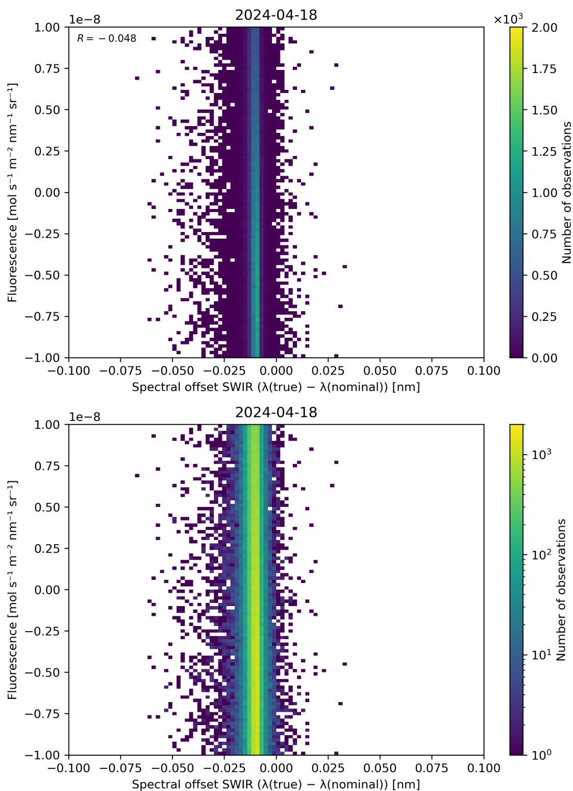
Figure 120: Scatter density plot of “Spectral offset SWIR ( \lambda(\text{true}) - \lambda(\text{nominal}) )” against “Fluorescence” for 2024-04-17 to 2024-04-19.
