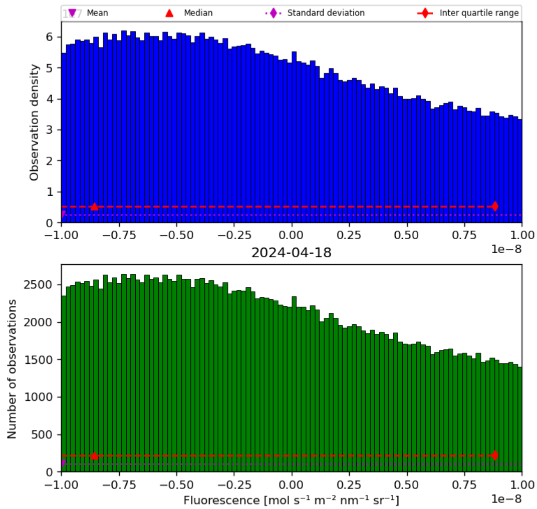
Figure 32: Histogram of “Fluorescence” for 2024-04-17 to 2024-04-19
