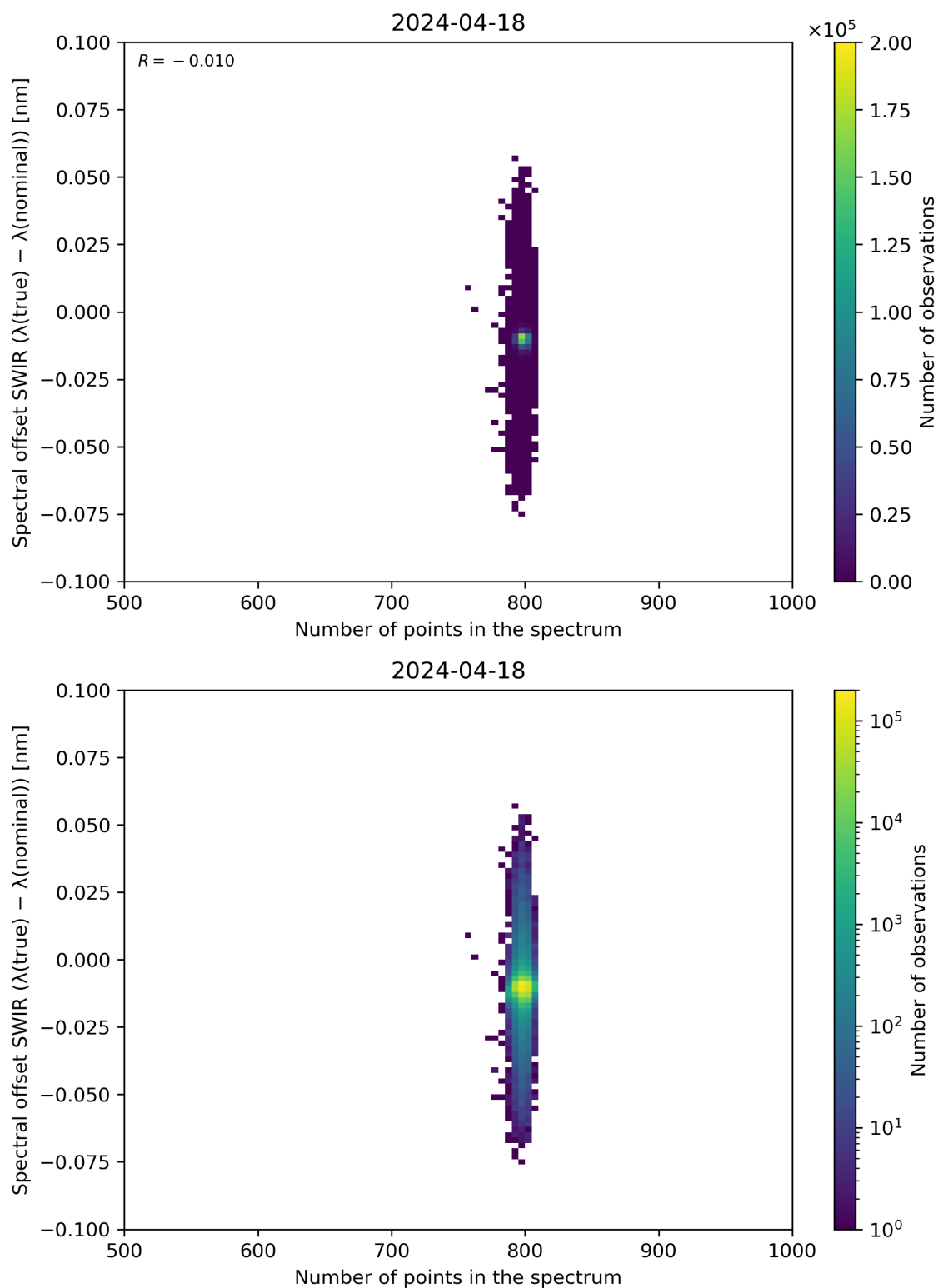
Figure 93: Scatter density plot of “Number of points in the spectrum” against “Spectral offset SWIR ( \lambda(\text{true}) - \lambda(\text{nominal}) )” for 2024-04-17 to 2024-04-19.
