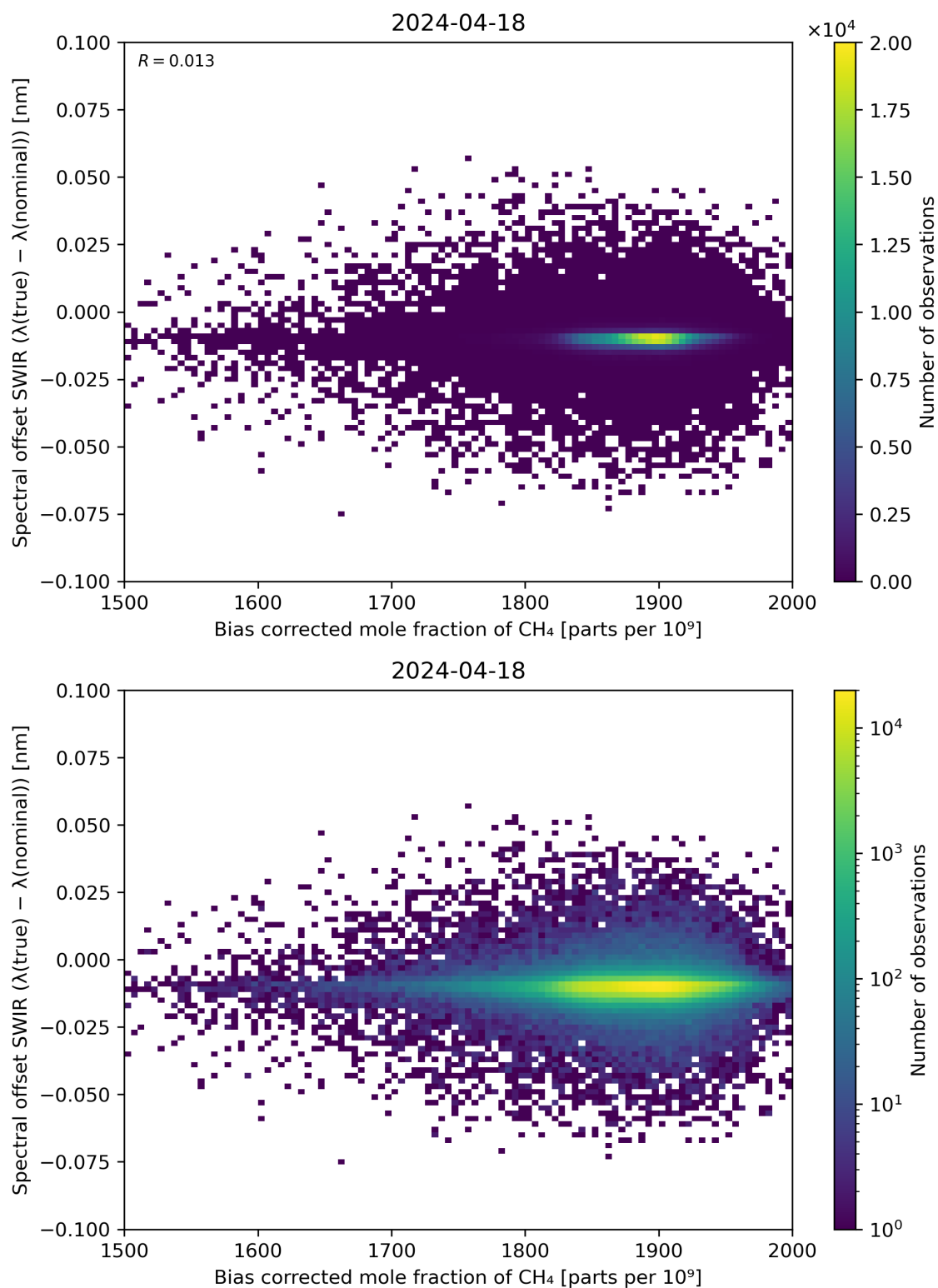
Figure 69: Scatter density plot of “Bias corrected mole fraction of \text{CH}_4 ” against “Spectral offset SWIR ( \lambda(\text{true}) - \lambda(\text{nominal}) )” for 2024-04-17 to 2024-04-19.
