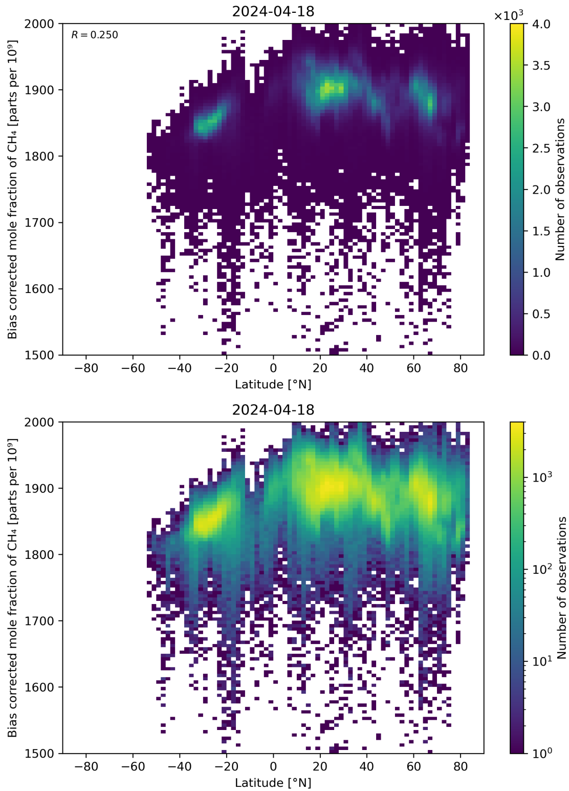
Figure 58: Scatter density plot of “Latitude” against “Bias corrected mole fraction of \text{CH}_4 ” for 2024-04-17 to 2024-04-19.
