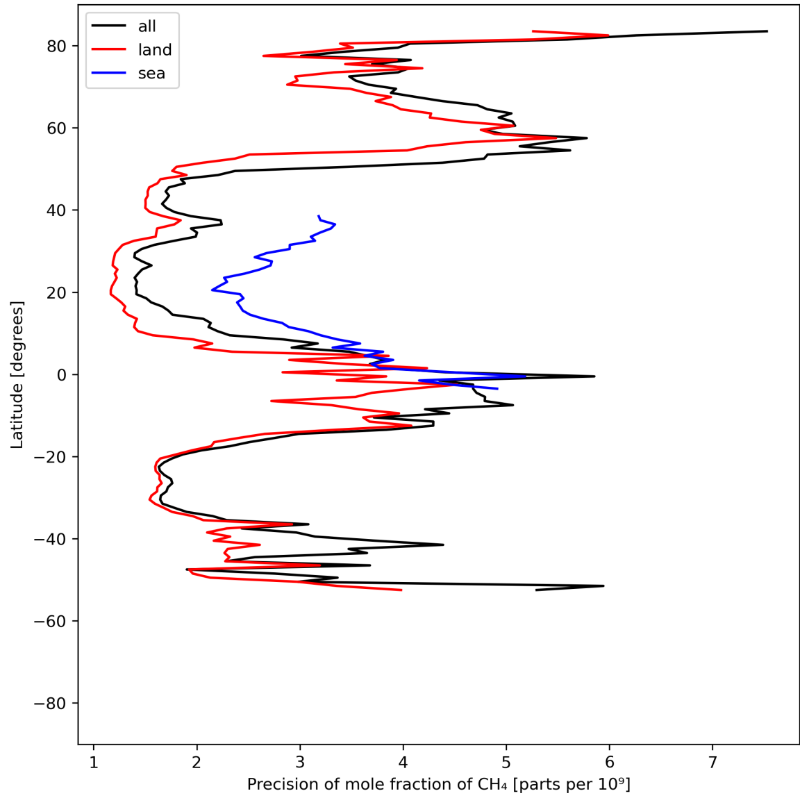
Figure 13: Zonal average of “Precision of mole fraction of CH 4 ” for 2024-04-17 to 2024-04-19.
