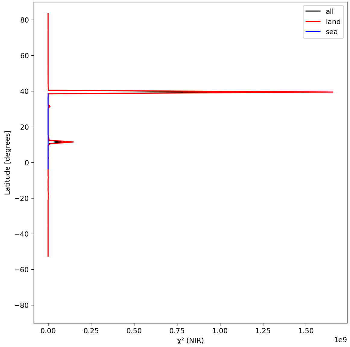
Figure 18: Zonal average of “ \chi^2 (NIR)” for 2024-04-17 to 2024-04-19.
