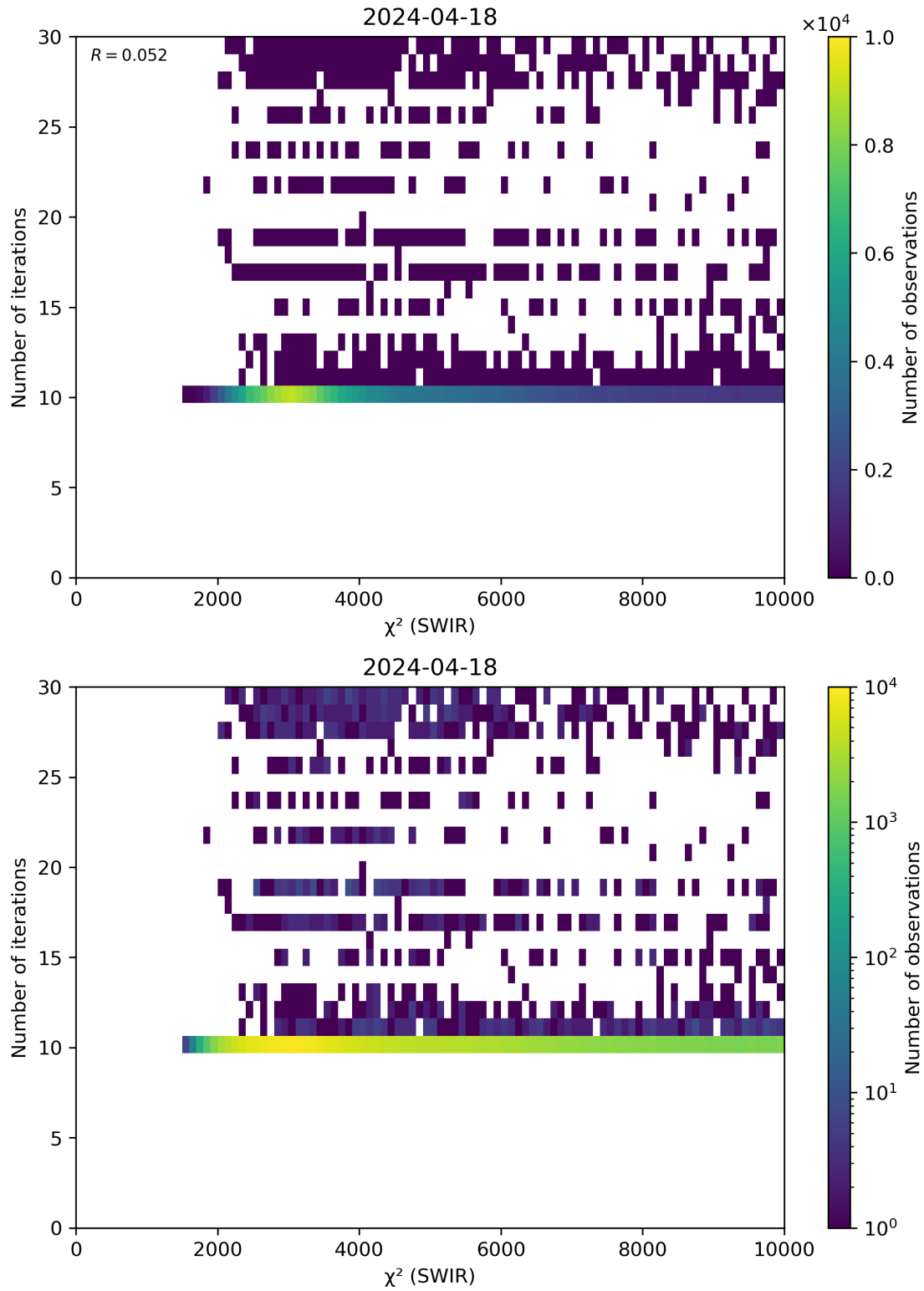
Figure 50: Scatter density plot of “ \chi^2 (SWIR)” against “Number of iterations” for 2024-04-17 to 2024-04-19.
