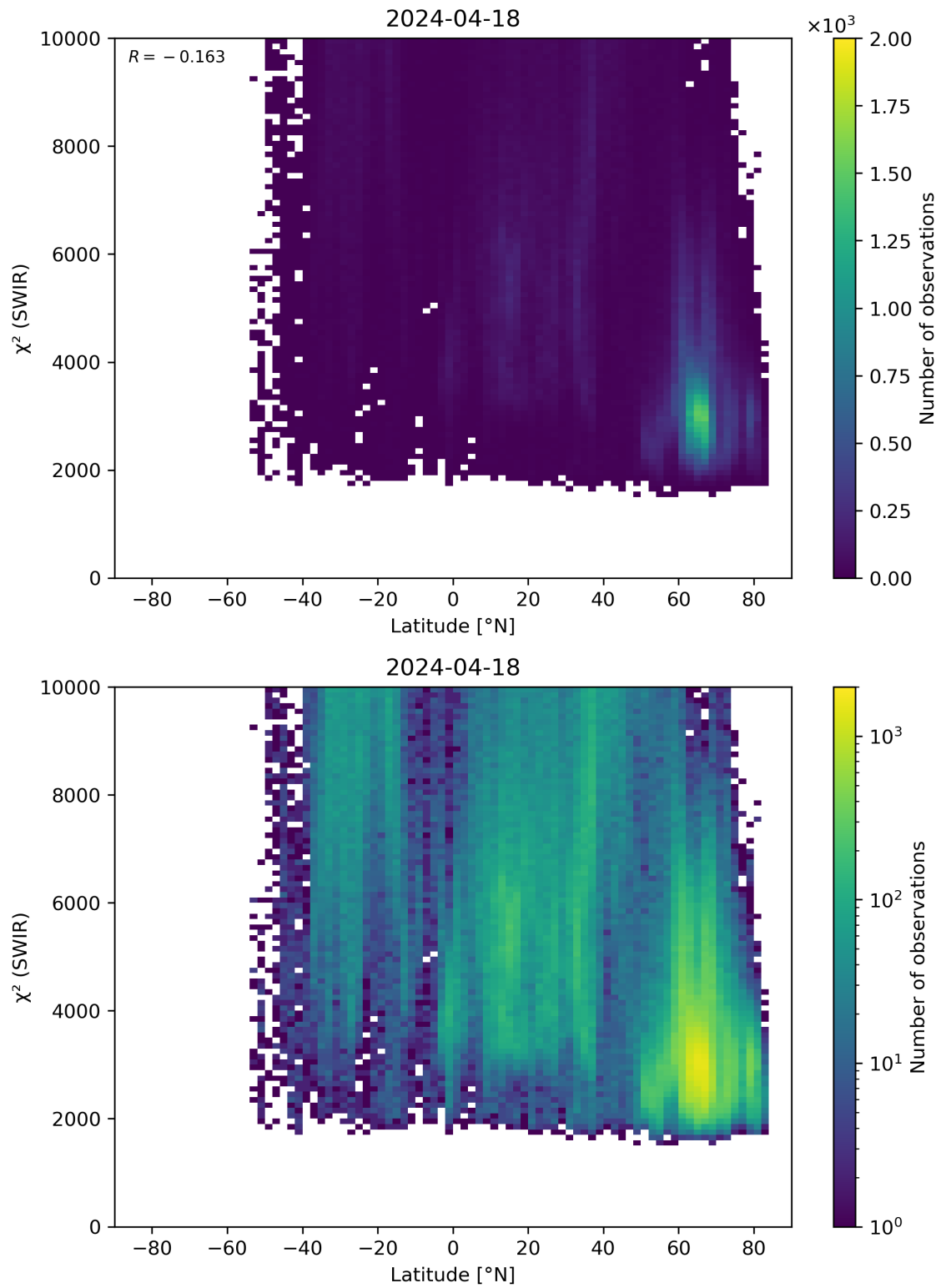
Figure 54: Scatter density plot of “Latitude” against “ \chi^2 (SWIR)” for 2024-04-17 to 2024-04-19.
