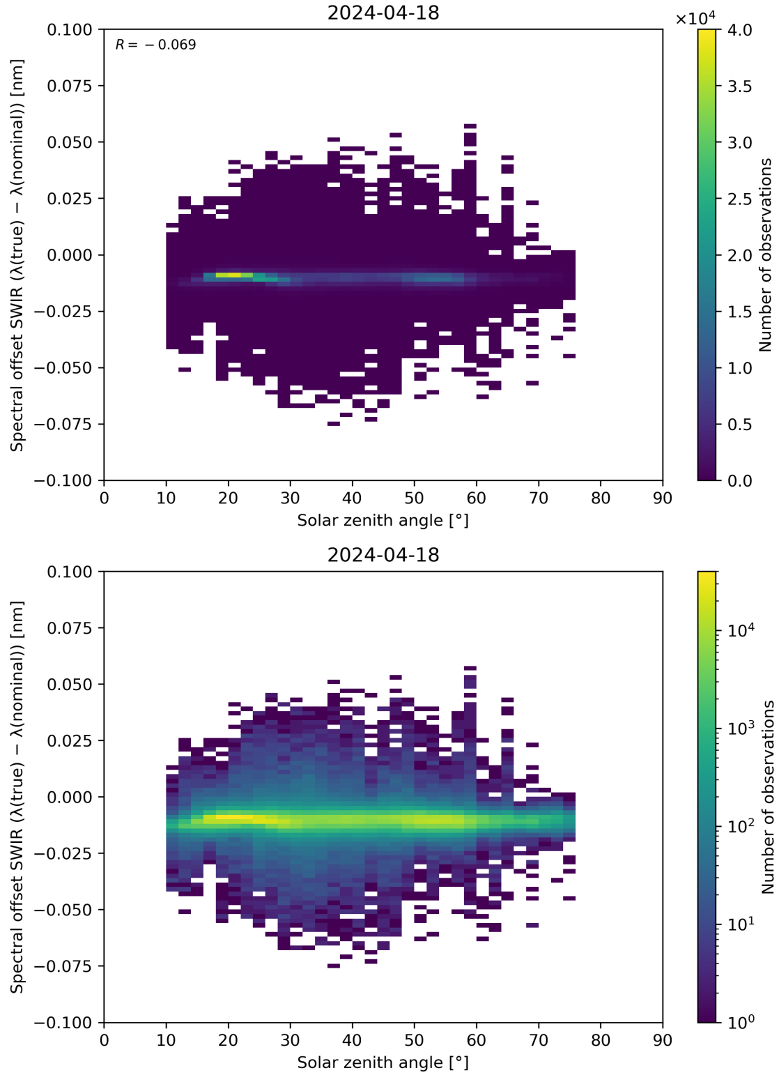
Figure 104: Scatter density plot of “Solar zenith angle” against “Spectral offset SWIR ( \lambda(\text{true}) - \lambda(\text{nominal}) )” for 2024-04-17 to 2024-04-19.
