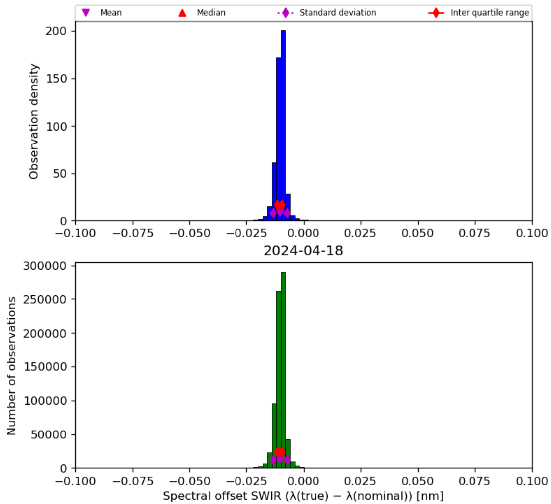
Figure 27: Histogram of “Spectral offset SWIR ( \lambda(\text{true}) - \lambda(\text{nominal}) )” for 2024-04-17 to 2024-04-19
