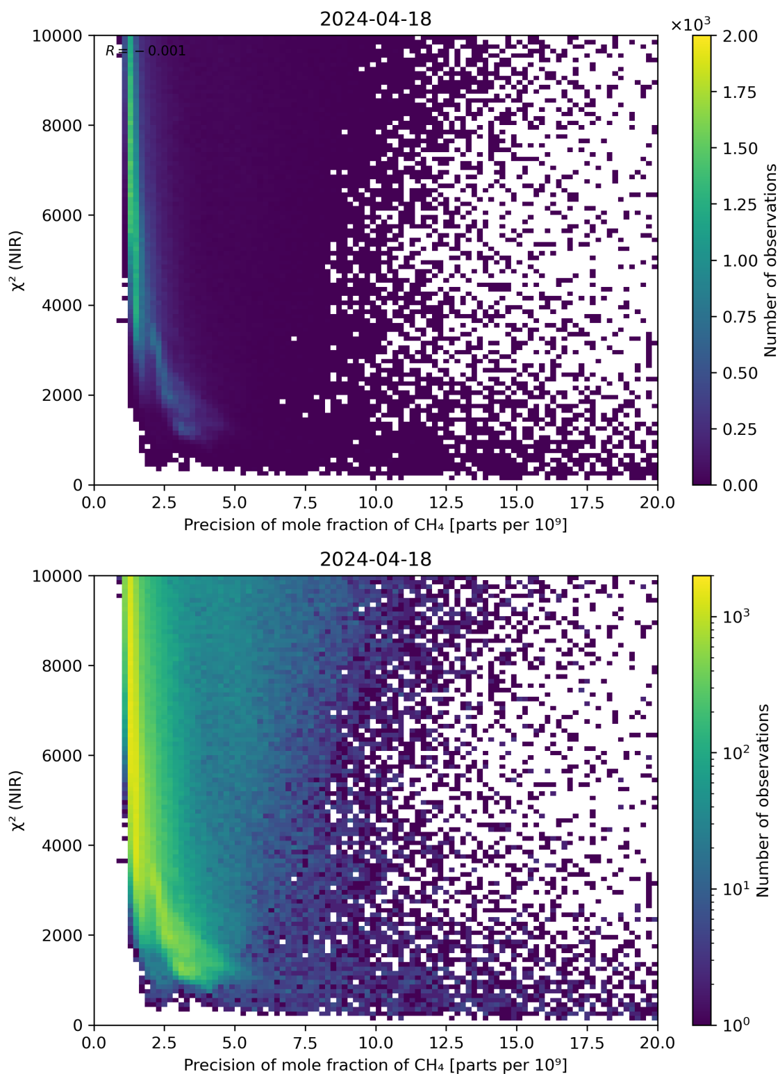
Figure 78: Scatter density plot of “Precision of mole fraction of CH 4 ” against “ \chi^2 (NIR)” for 2024-04-17 to 2024-04-19.
