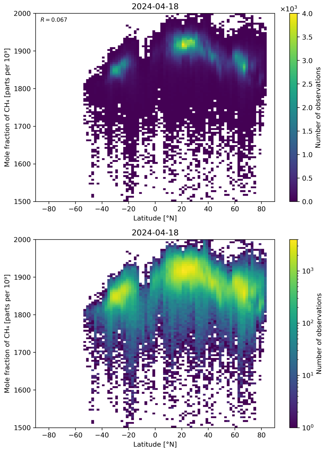
Figure 57: Scatter density plot of “Latitude” against “Mole fraction of \text{CH}_4 ” for 2024-04-17 to 2024-04-19.
