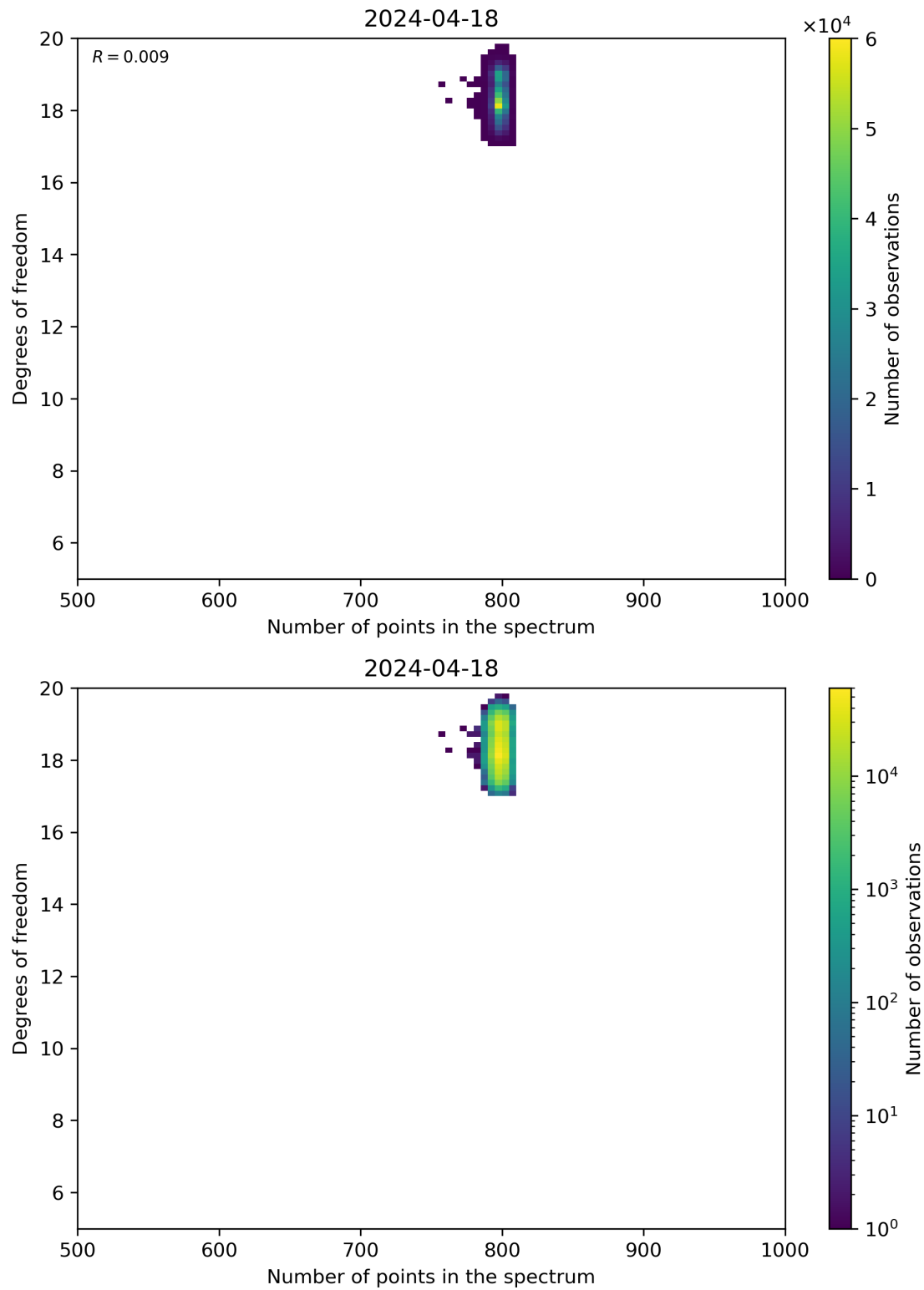
Figure 90: Scatter density plot of “Number of points in the spectrum” against “Degrees of freedom” for 2024-04-17 to 2024-04-19.
