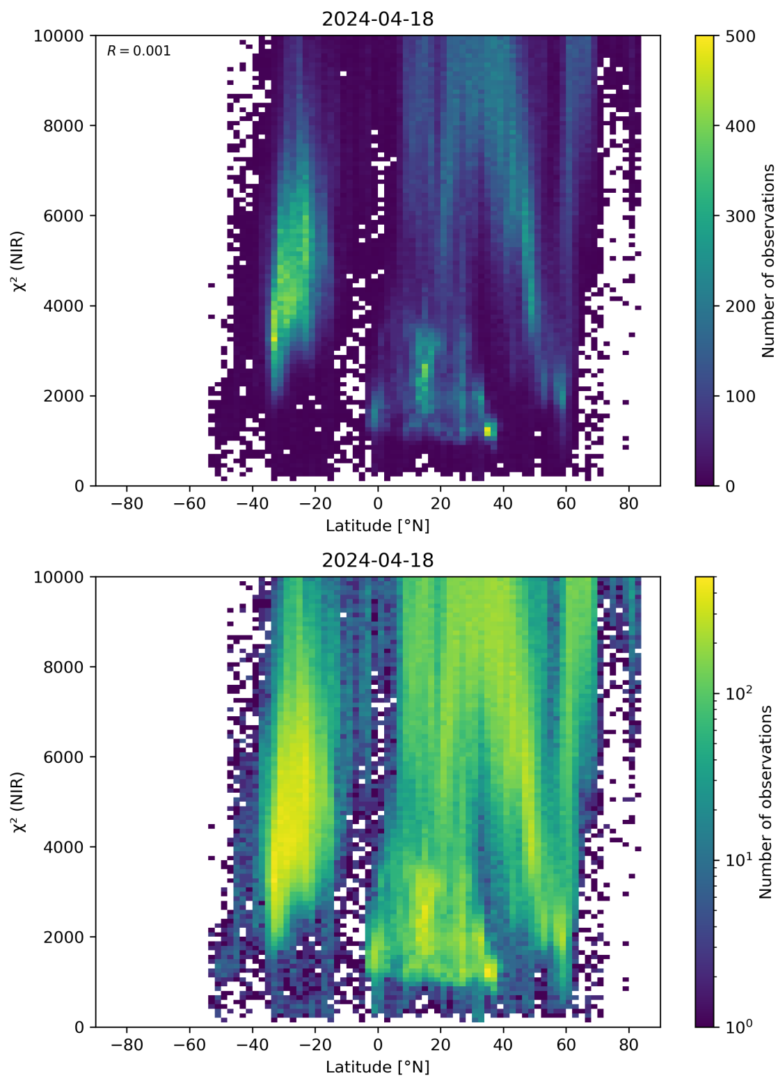
Figure 53: Scatter density plot of “Latitude” against “ \chi^2 (NIR)” for 2024-04-17 to 2024-04-19.
