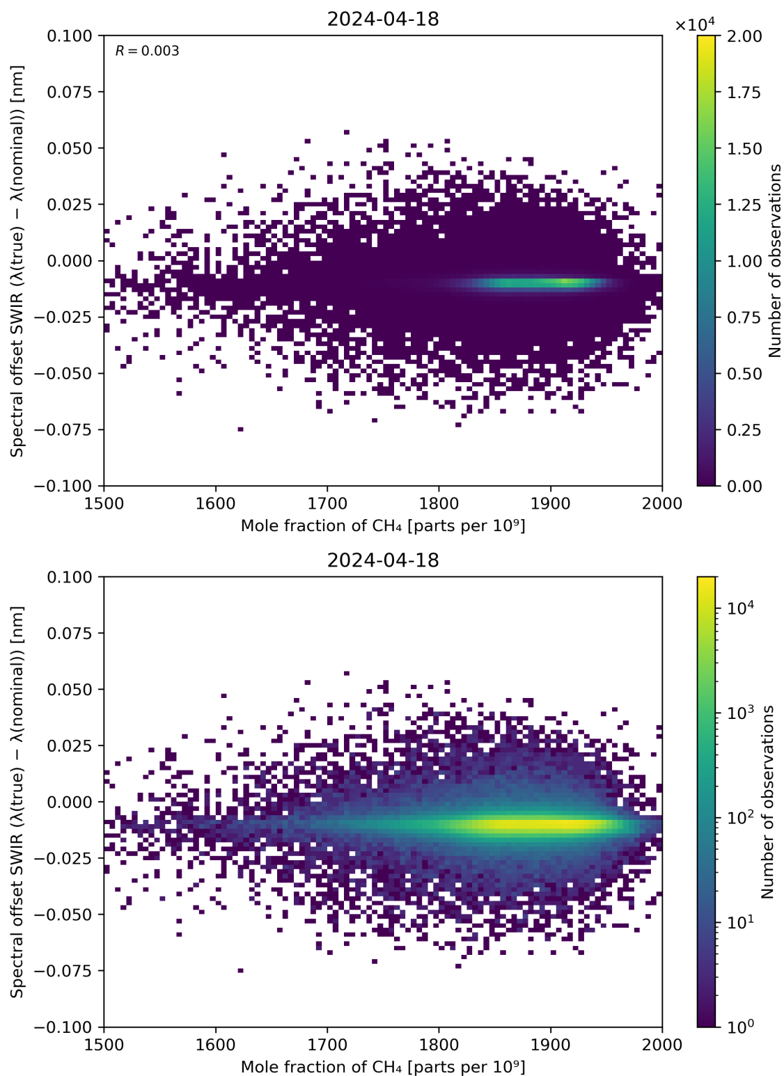
Figure 86: Scatter density plot of “Mole fraction of CH 4 ” against “Spectral offset SWIR ( \lambda(\text{true}) - \lambda(\text{nominal}) )” for 2024-04-17 to 2024-04-19.
