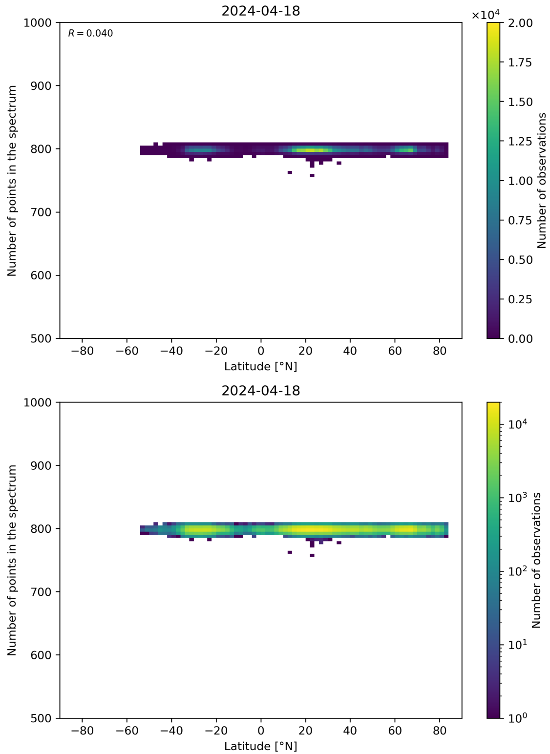
Figure 61: Scatter density plot of “Latitude” against “Number of points in the spectrum” for 2024-04-17 to 2024-04-19.
