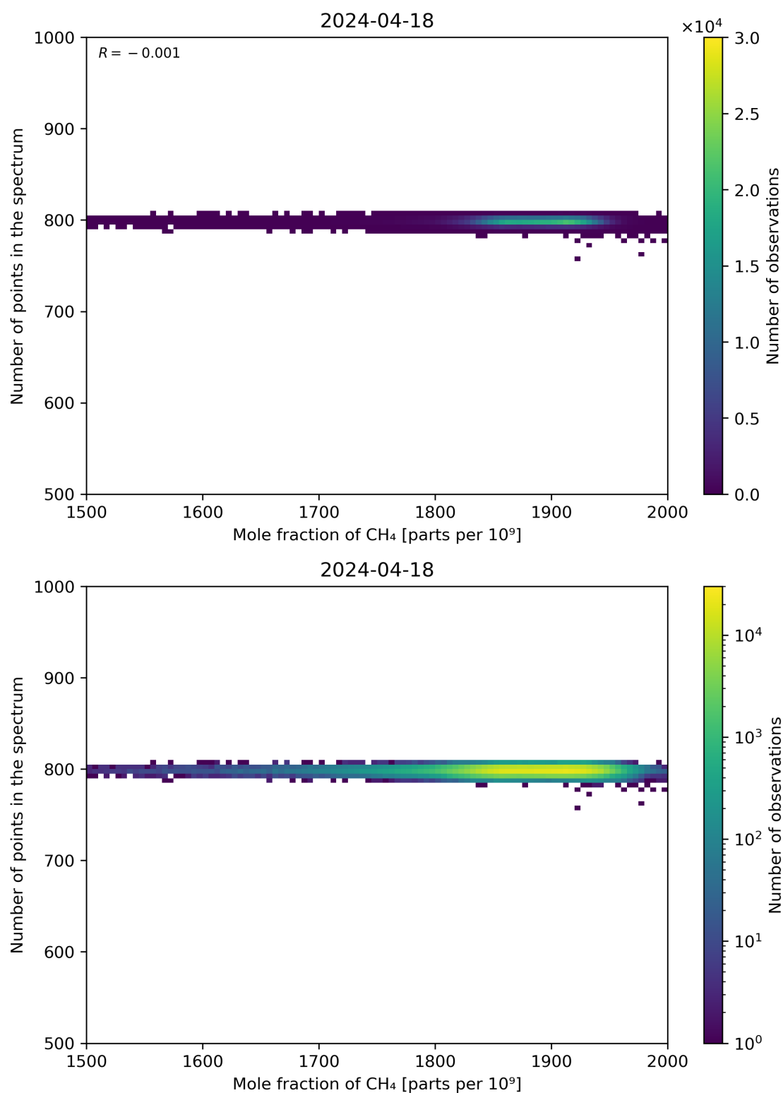
Figure 77: Scatter density plot of “Mole fraction of CH 4 ” against “Number of points in the spectrum” for 2024-04-17 to 2024-04-19.
