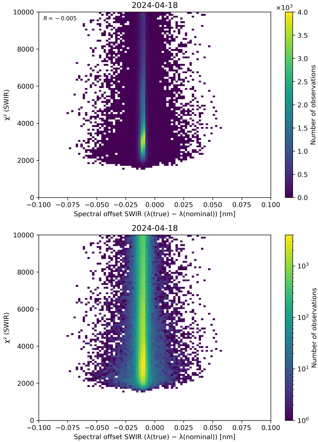
Figure 118: Scatter density plot of “Spectral offset SWIR ( \lambda(\text{true}) - \lambda(\text{nominal}) )” against “ \chi^2 (SWIR)” for 2024-04-17 to 2024-04-19.
