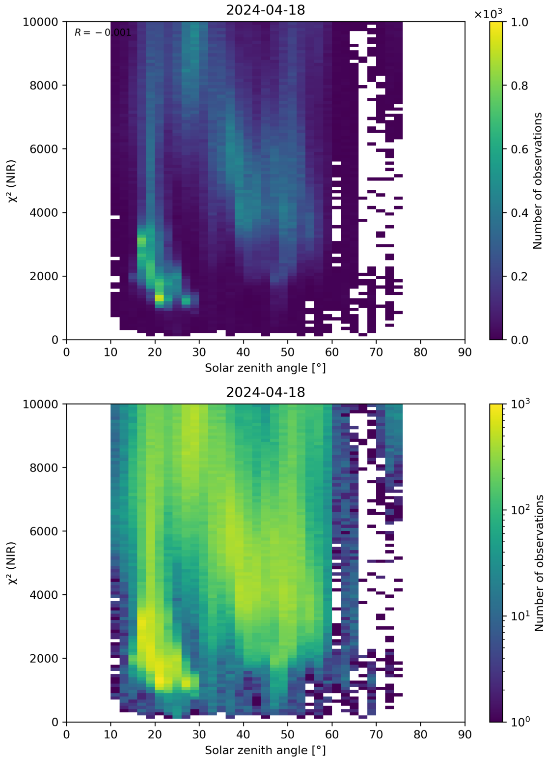
Figure 94: Scatter density plot of “Solar zenith angle” against “ \chi^2 (NIR)” for 2024-04-17 to 2024-04-19.
