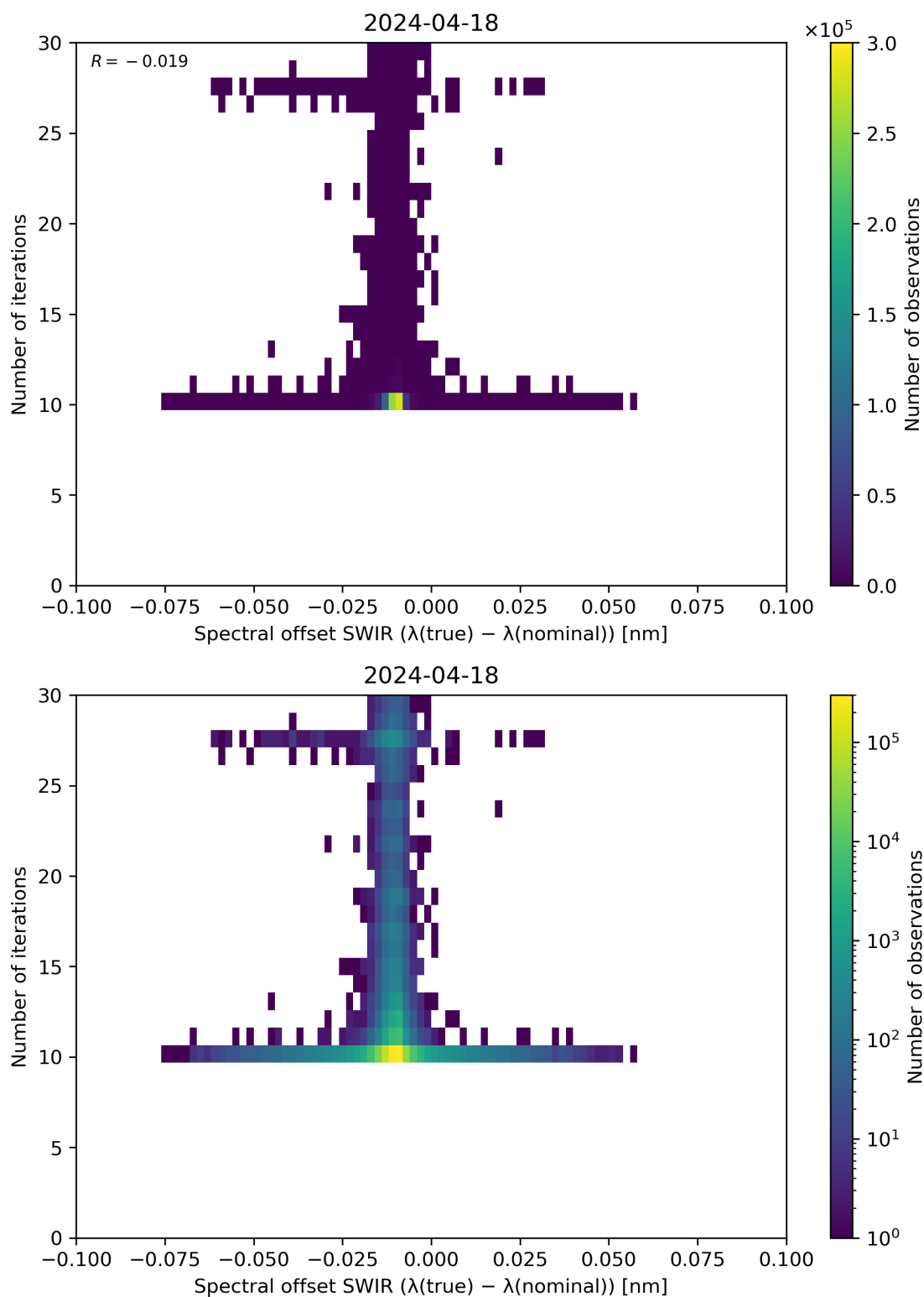
Figure 121: Scatter density plot of “Spectral offset SWIR ( \lambda(\text{true}) - \lambda(\text{nominal}) )” against “Number of iterations” for 2024-04-17 to 2024-04-19.
