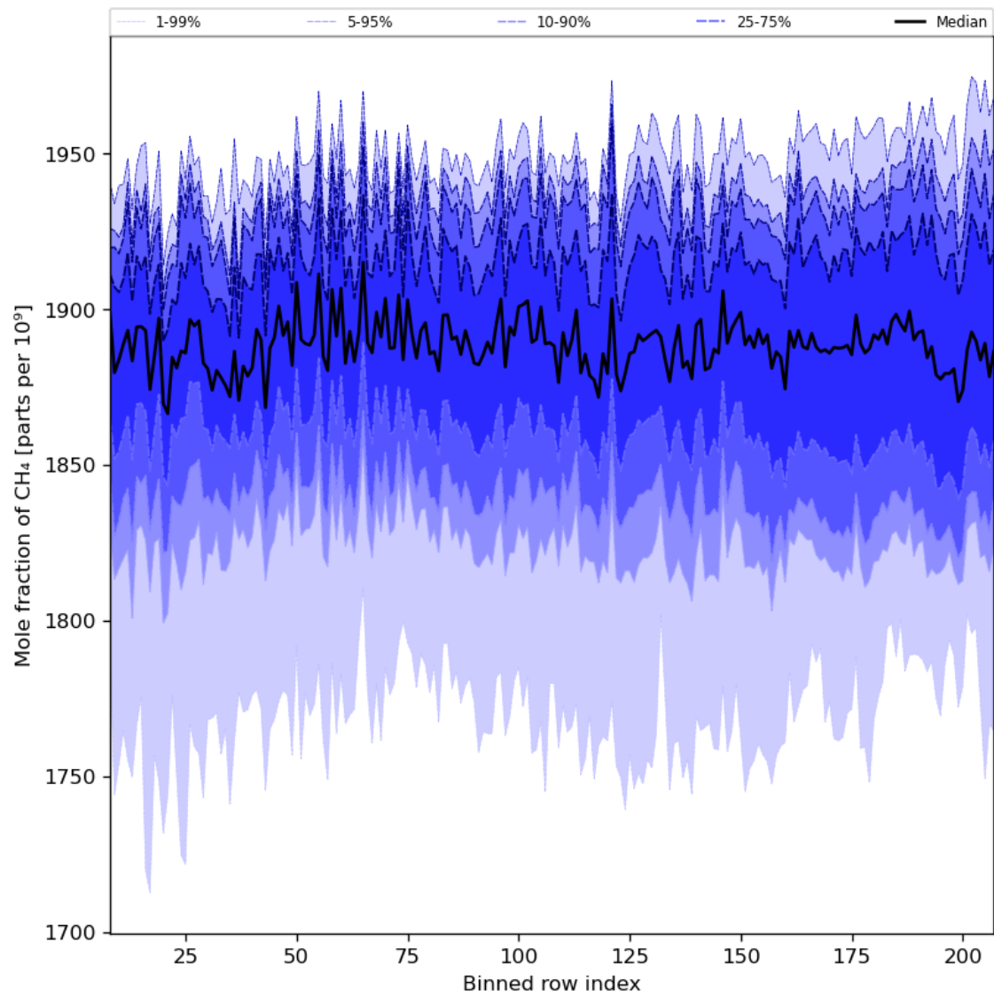
Figure 34: Along track statistics of “Mole fraction of CH 4 ” for 2024-04-17 to 2024-04-19
