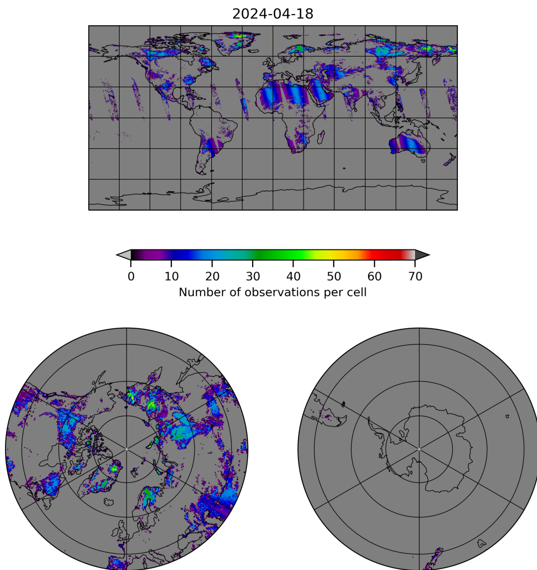
Figure 10: Map of the number of observations for 2024-04-17 to 2024-04-19
