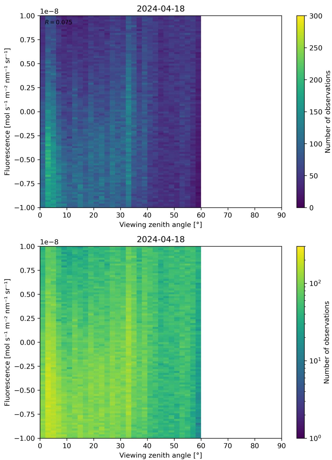
Figure 108: Scatter density plot of “Viewing zenith angle” against “Fluorescence” for 2024-04-17 to 2024-04-19.
