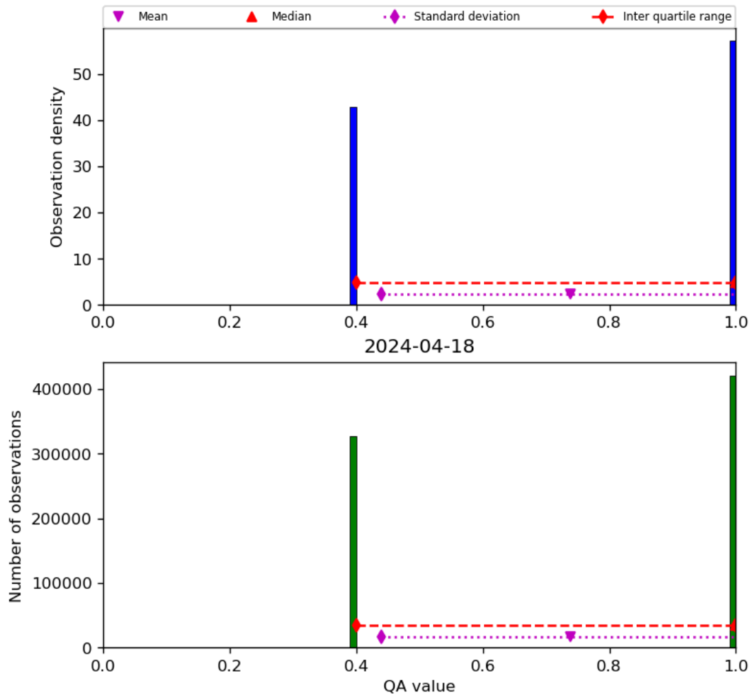
Figure 22: Histogram of “QA value” for 2024-04-17 to 2024-04-19
