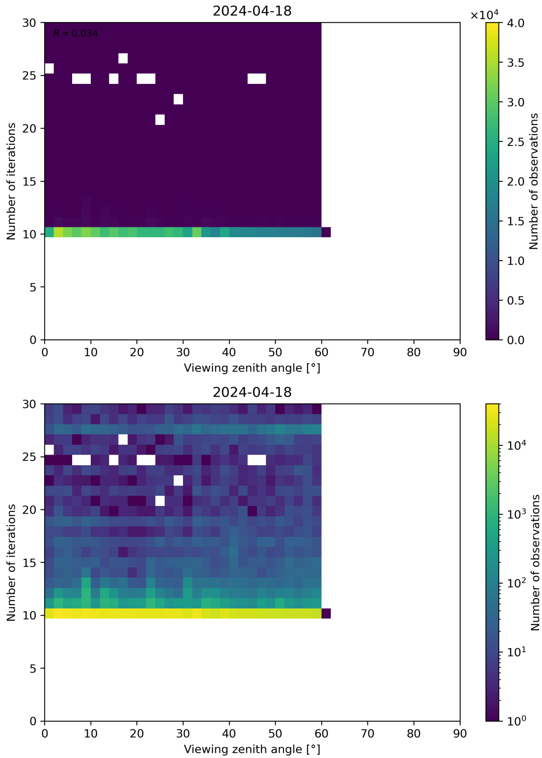
Figure 113: Scatter density plot of “Viewing zenith angle” against “Number of iterations” for 2024-04-17 to 2024-04-19.
