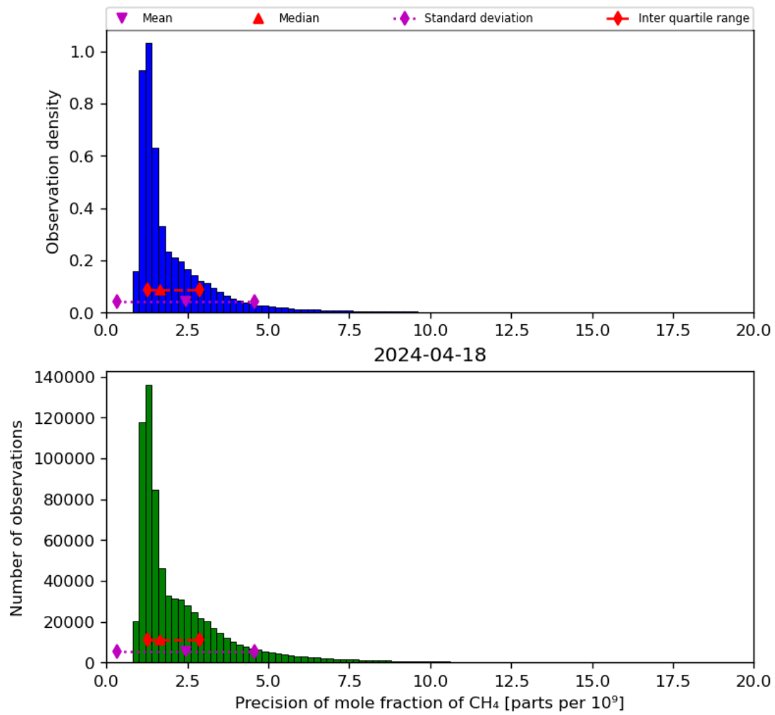
Figure 24: Histogram of “Precision of mole fraction of CH 4 ” for 2024-04-17 to 2024-04-19
