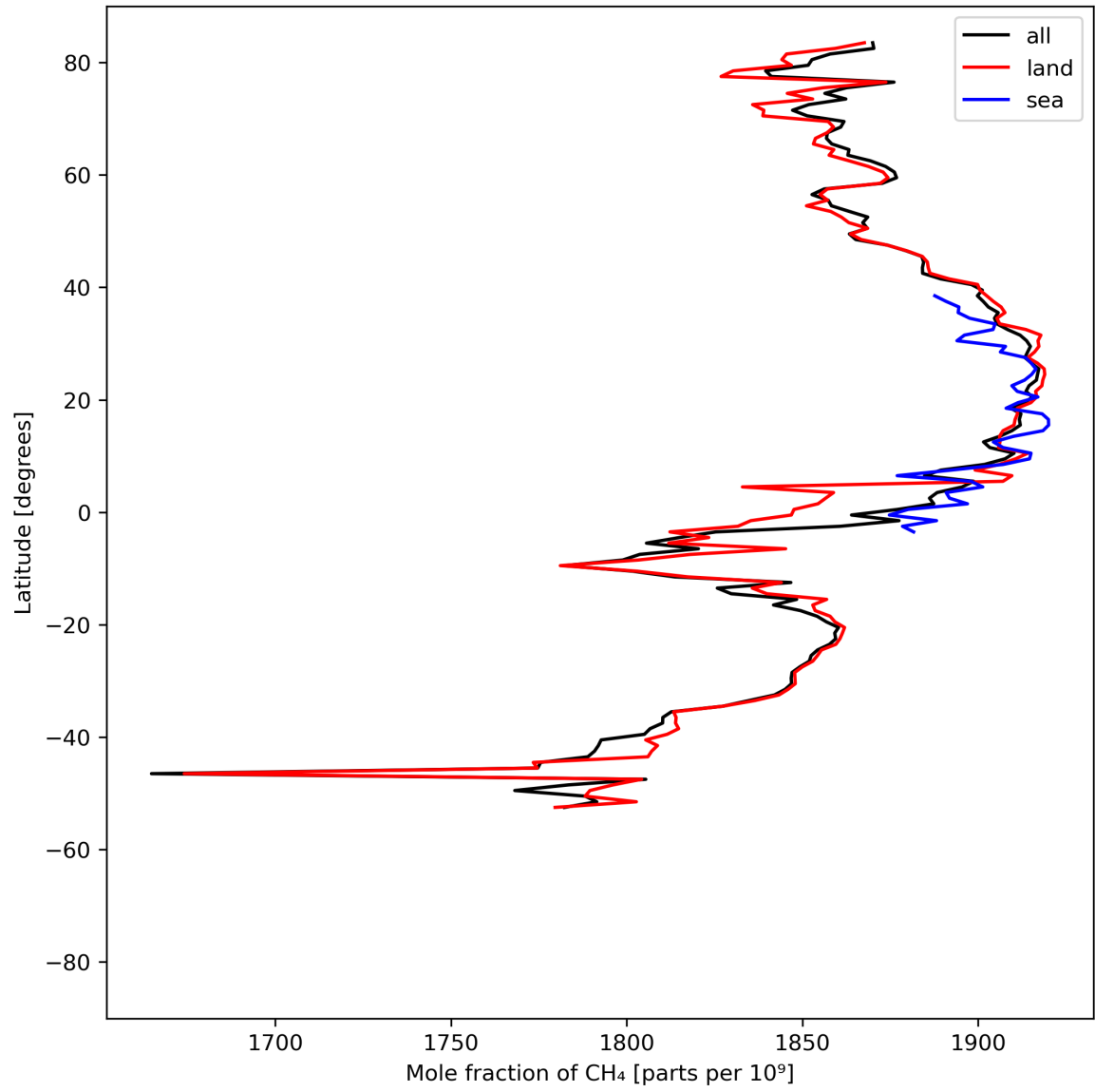
Figure 12: Zonal average of “Mole fraction of \text{CH}_4 ” for 2024-04-17 to 2024-04-19.
