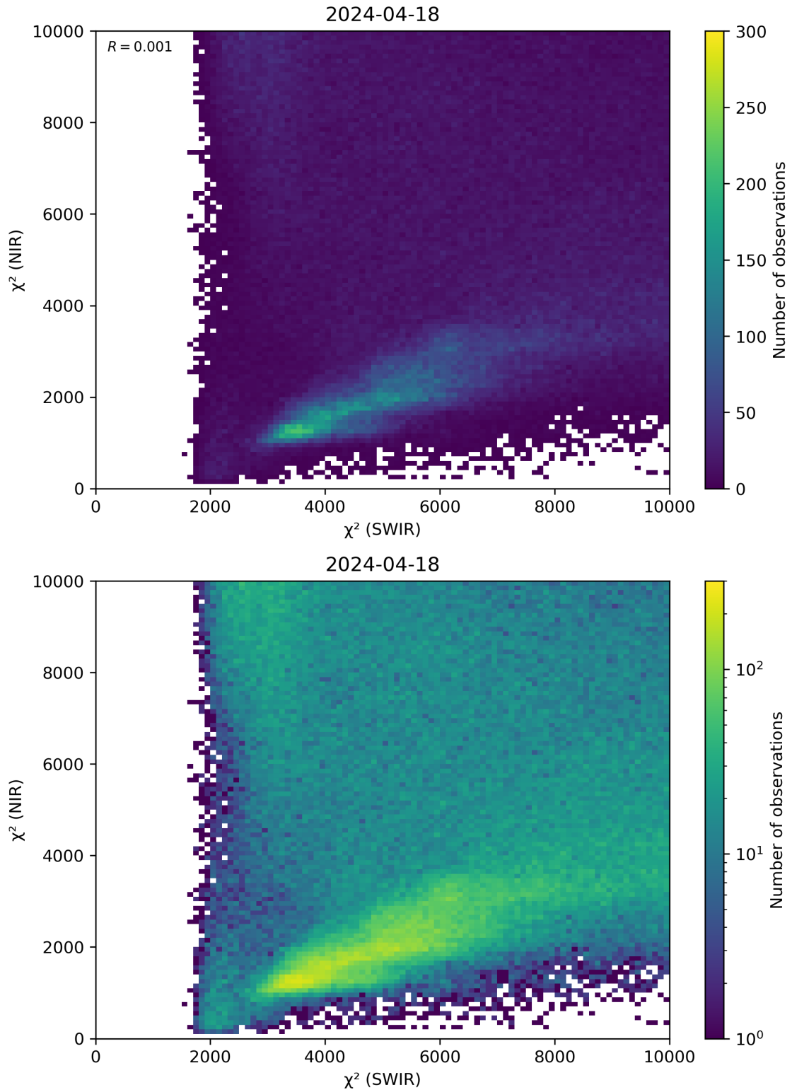
Figure 47: Scatter density plot of “ \chi^2 (SWIR)” against “ \chi^2 (NIR)” for 2024-04-17 to 2024-04-19.
