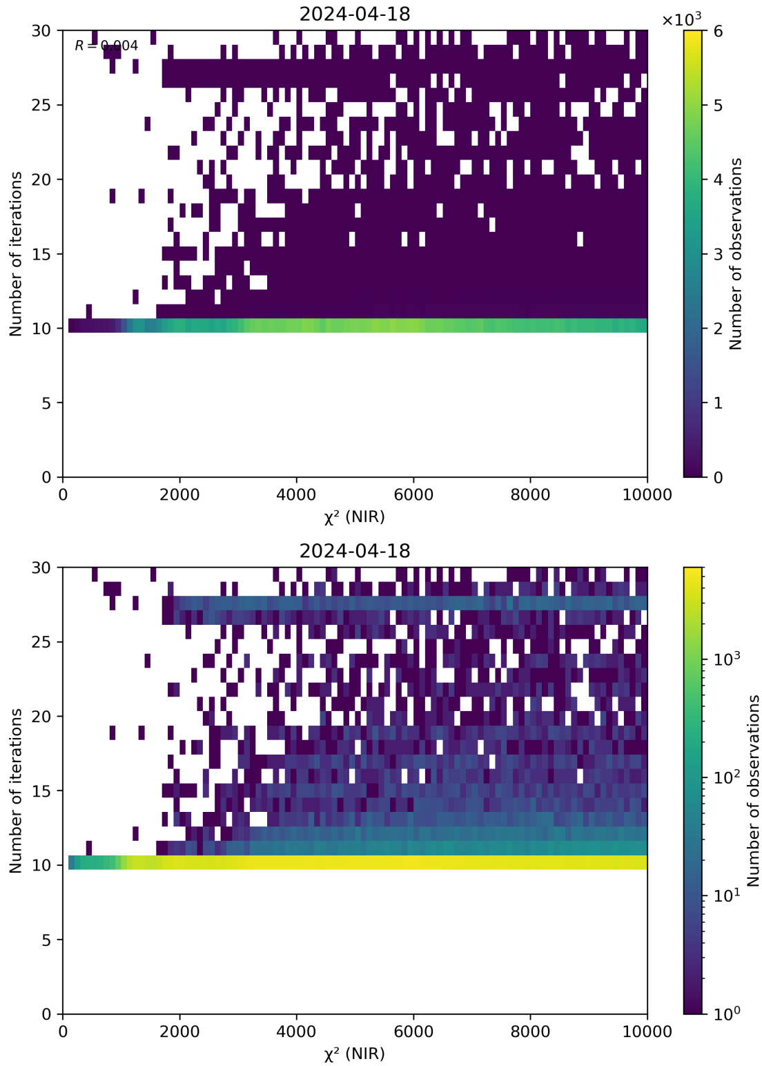
Figure 46: Scatter density plot of “ \chi^2 (NIR)” against “Number of iterations” for 2024-04-17 to 2024-04-19.
