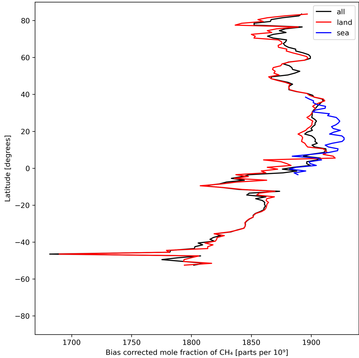
Figure 14: Zonal average of “Bias corrected mole fraction of CH 4 ” for 2024-04-17 to 2024-04-19.
