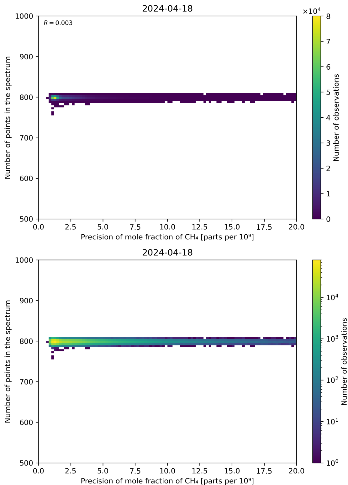
Figure 84: Scatter density plot of “Precision of mole fraction of CH 4 ” against “Number of points in the spectrum” for 2024-04-17 to 2024-04-19.
