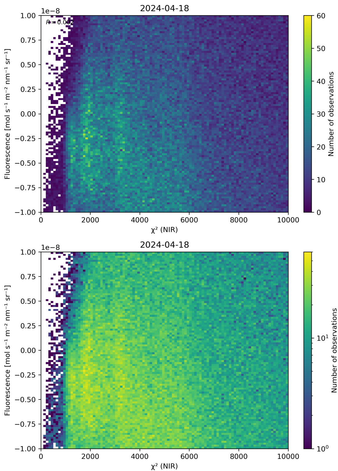
Figure 45: Scatter density plot of “ \chi^2 (NIR)” against “Fluorescence” for 2024-04-17 to 2024-04-19.
