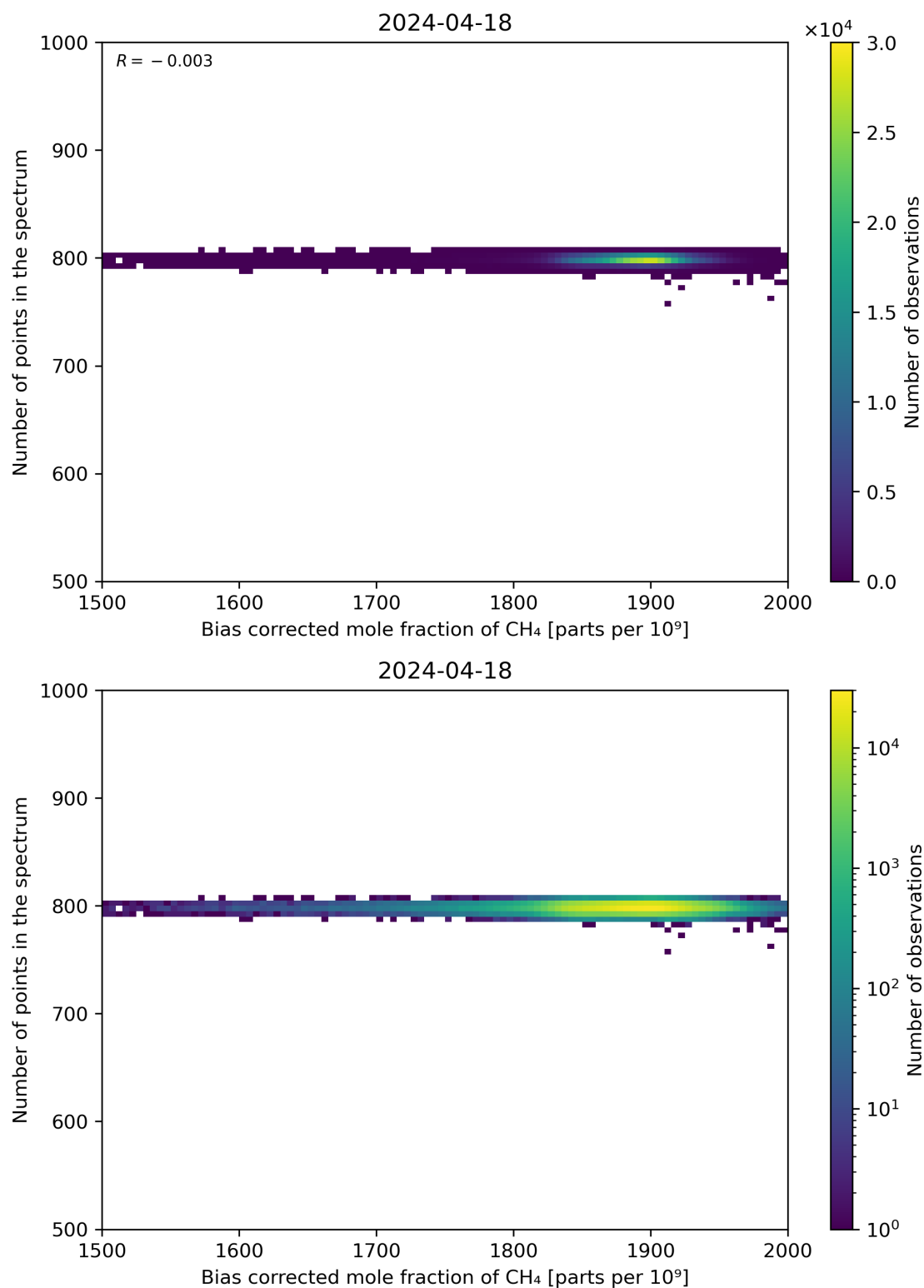
Figure 68: Scatter density plot of “Bias corrected mole fraction of CH 4 ” against “Number of points in the spectrum” for 2024-04-17 to 2024-04-19.
