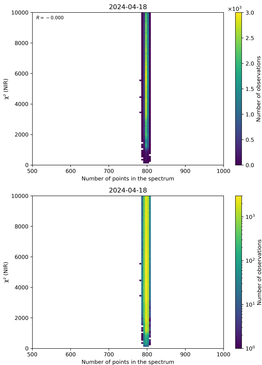
Figure 88: Scatter density plot of “Number of points in the spectrum” against “ \chi^2 (NIR)” for 2024-04-17 to 2024-04-19.
