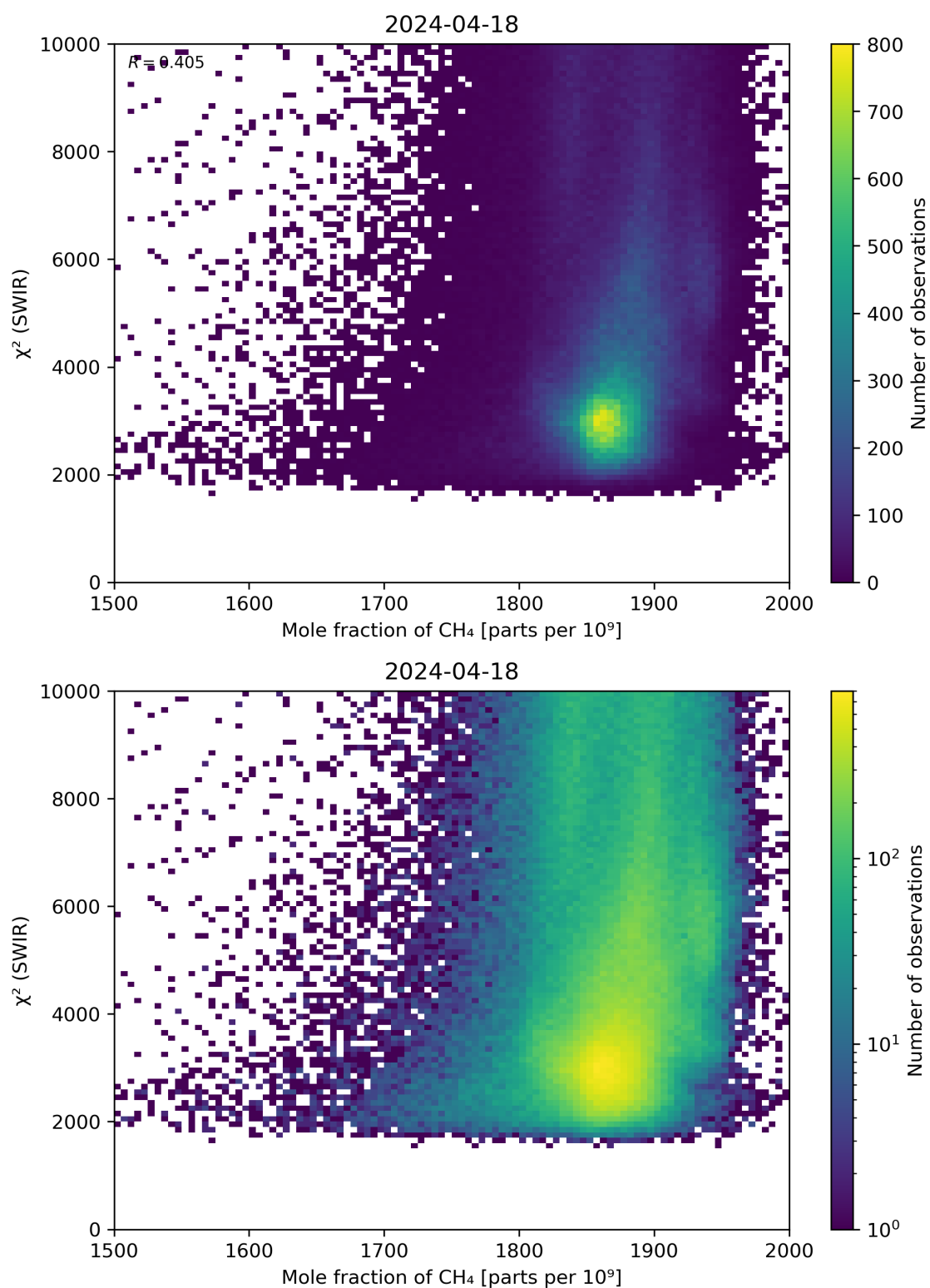
Figure 71: Scatter density plot of “Mole fraction of \text{CH}_4 ” against “ \chi^2 (SWIR)” for 2024-04-17 to 2024-04-19.
