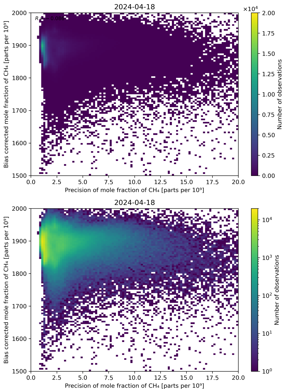
Figure 82: Scatter density plot of “Precision of mole fraction of CH 4 ” against “Bias corrected mole fraction of CH 4 ” for 2024-04-17 to 2024-04-19.
