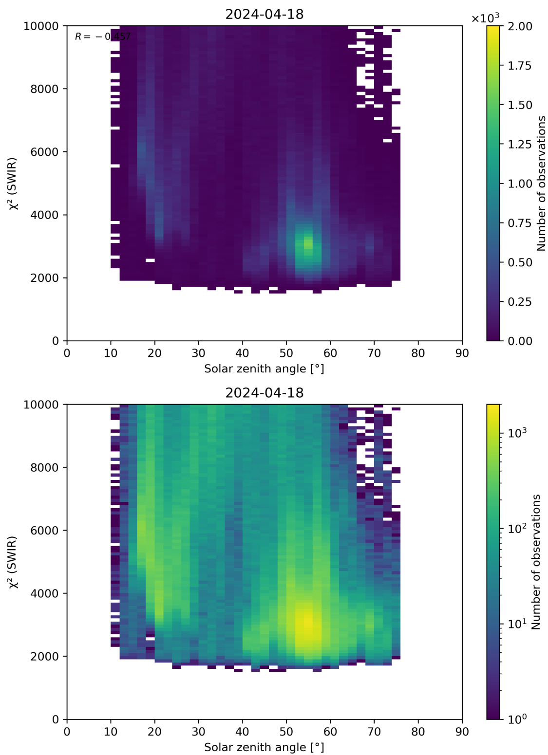
Figure 95: Scatter density plot of “Solar zenith angle” against “ \chi^2 (SWIR)” for 2024-04-17 to 2024-04-19.
