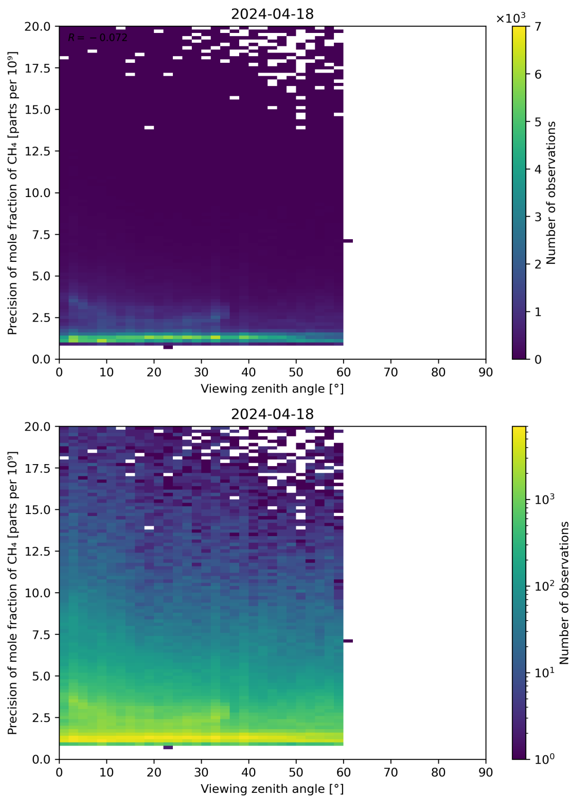
Figure 112: Scatter density plot of “Viewing zenith angle” against “Precision of mole fraction of CH 4 ” for 2024-04-17 to 2024-04-19.
