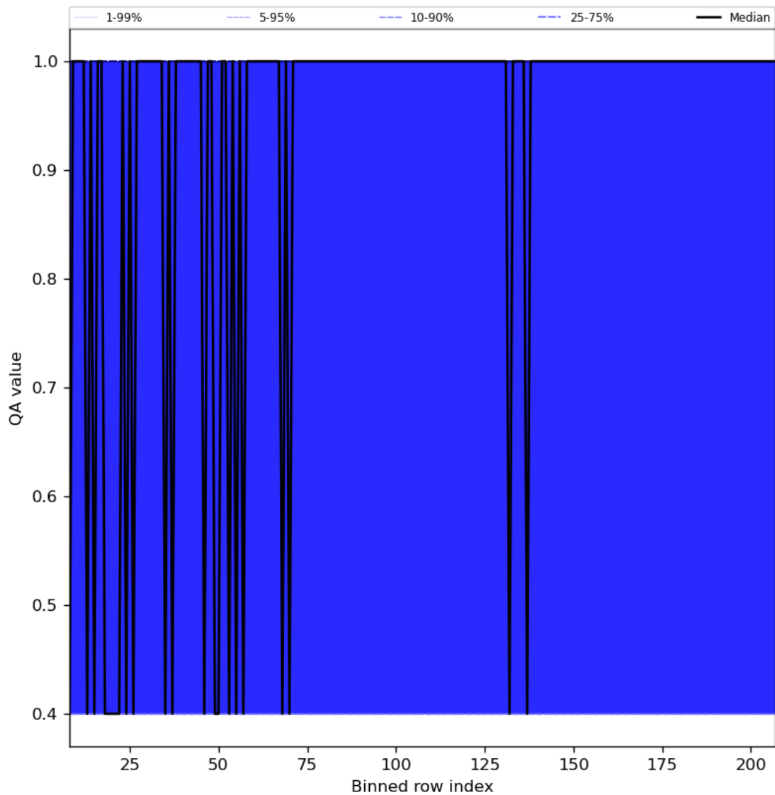
Figure 33: Along track statistics of “QA value” for 2024-04-17 to 2024-04-19
