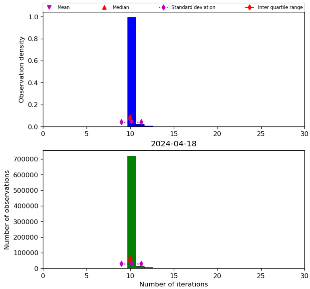
Figure 31: Histogram of "Number of iterations" for 2024-04-17 to 2024-04-19
