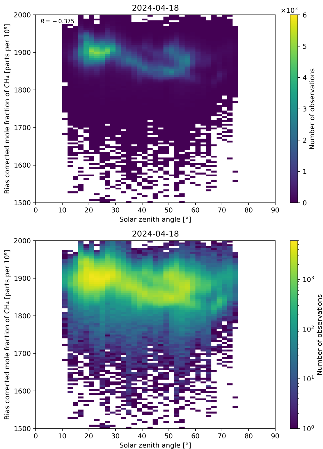
Figure 100: Scatter density plot of “Solar zenith angle” against “Bias corrected mole fraction of CH 4 ” for 2024-04-17 to 2024-04-19.
