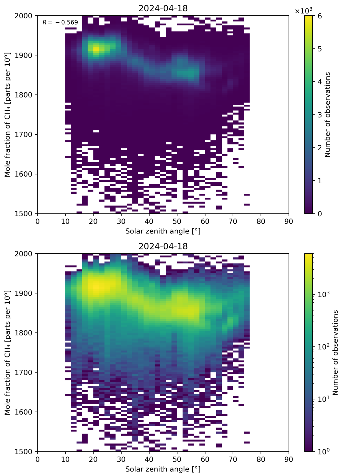
Figure 99: Scatter density plot of “Solar zenith angle” against “Mole fraction of CH 4 ” for 2024-04-17 to 2024-04-19.
