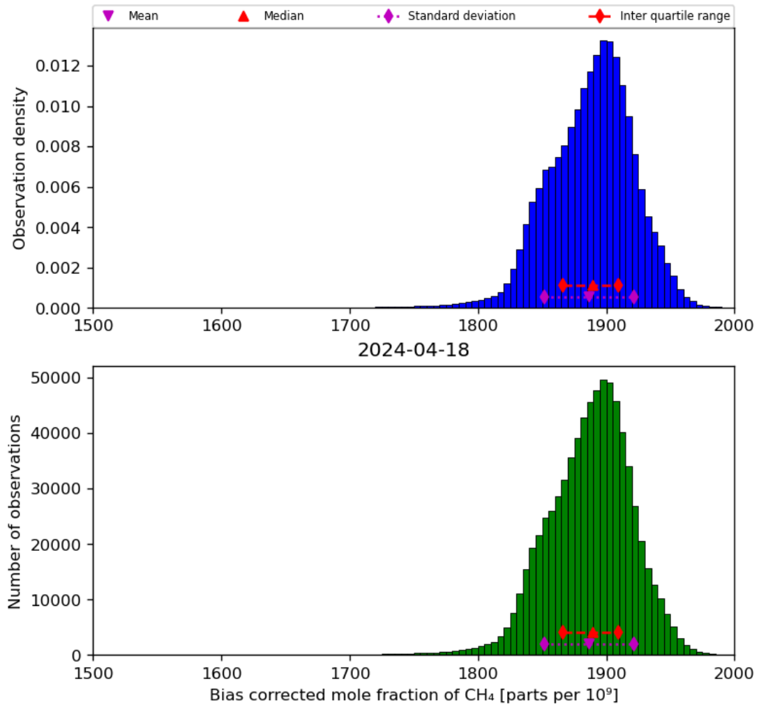
Figure 25: Histogram of “Bias corrected mole fraction of CH 4 ” for 2024-04-17 to 2024-04-19
