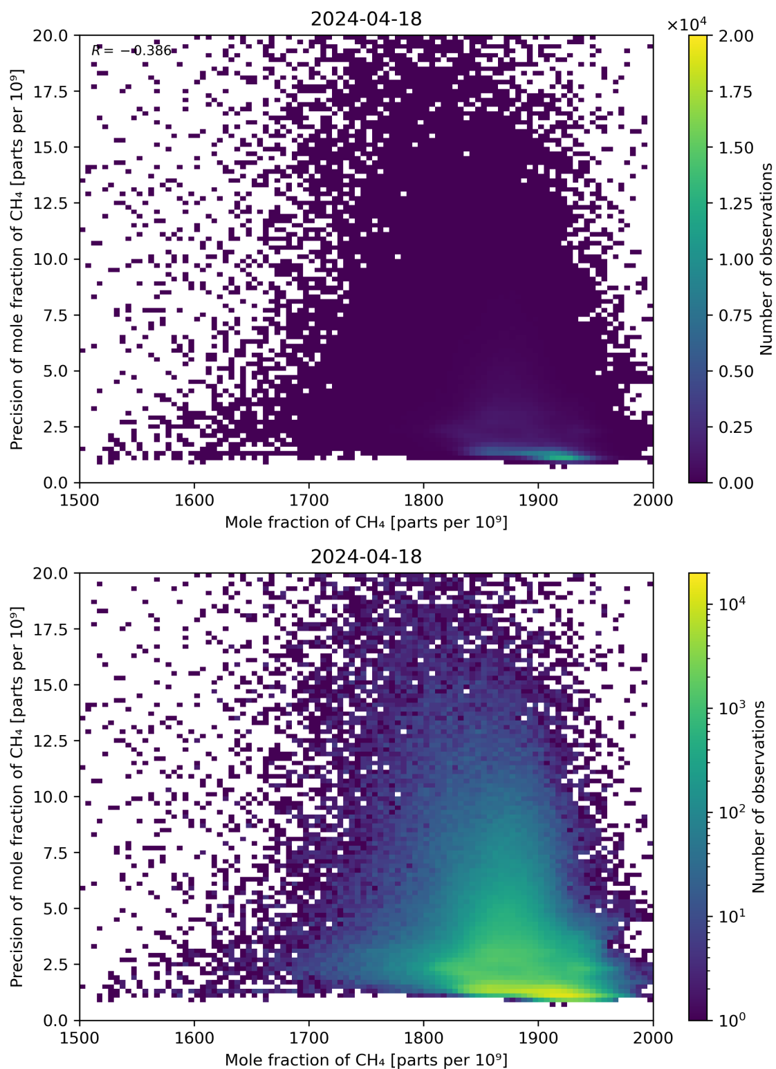
Figure 75: Scatter density plot of “Mole fraction of CH 4 ” against “Precision of mole fraction of CH 4 ” for 2024-04-17 to 2024-04-19.
