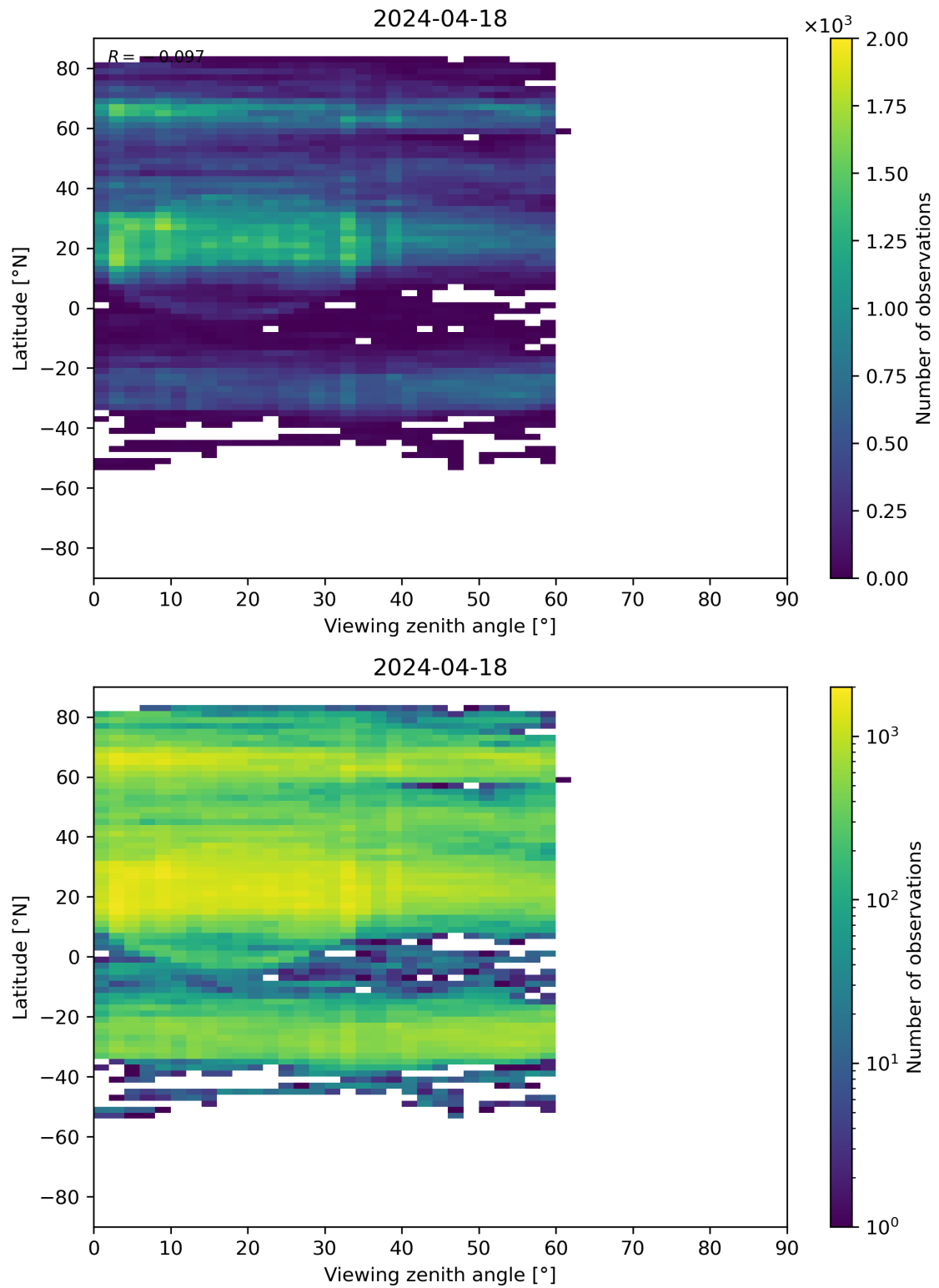
Figure 109: Scatter density plot of “Viewing zenith angle” against “Latitude” for 2024-04-17 to 2024-04-19.
