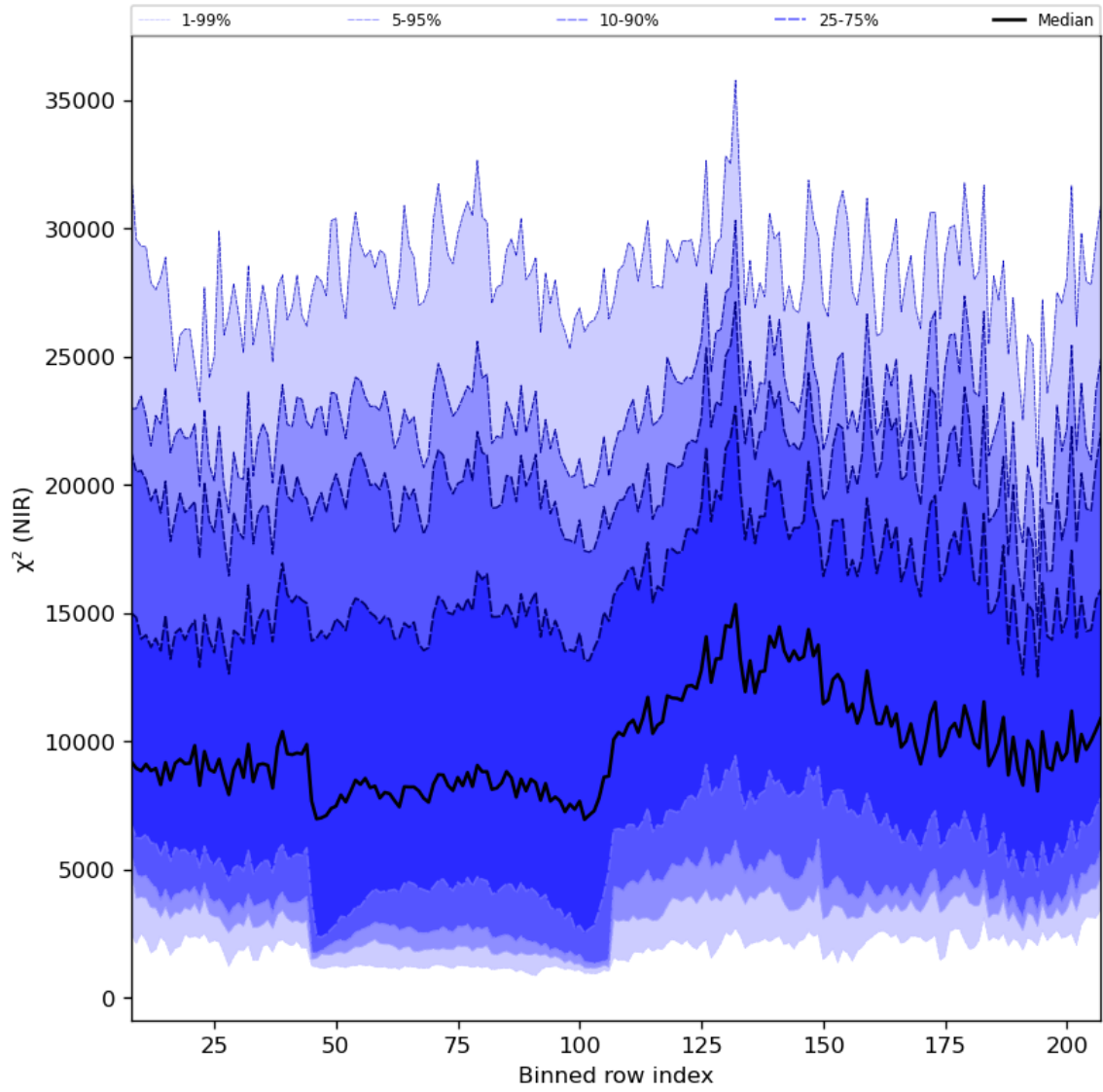
Figure 40: Along track statistics of “ \chi^2 (NIR)” for 2024-04-17 to 2024-04-19
