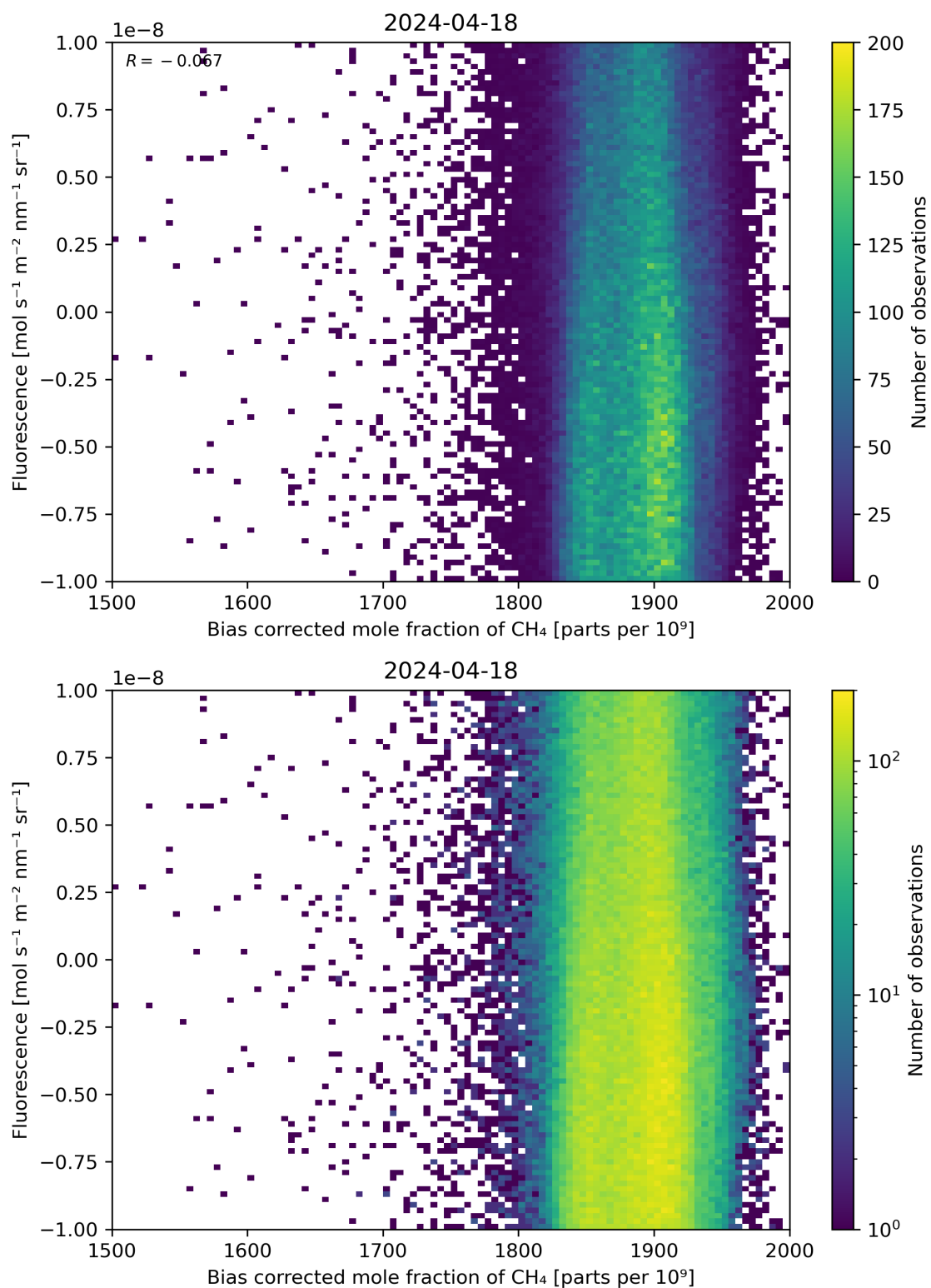
Figure 66: Scatter density plot of “Bias corrected mole fraction of \text{CH}_4 ” against “Fluorescence” for 2024-04-17 to 2024-04-19.
