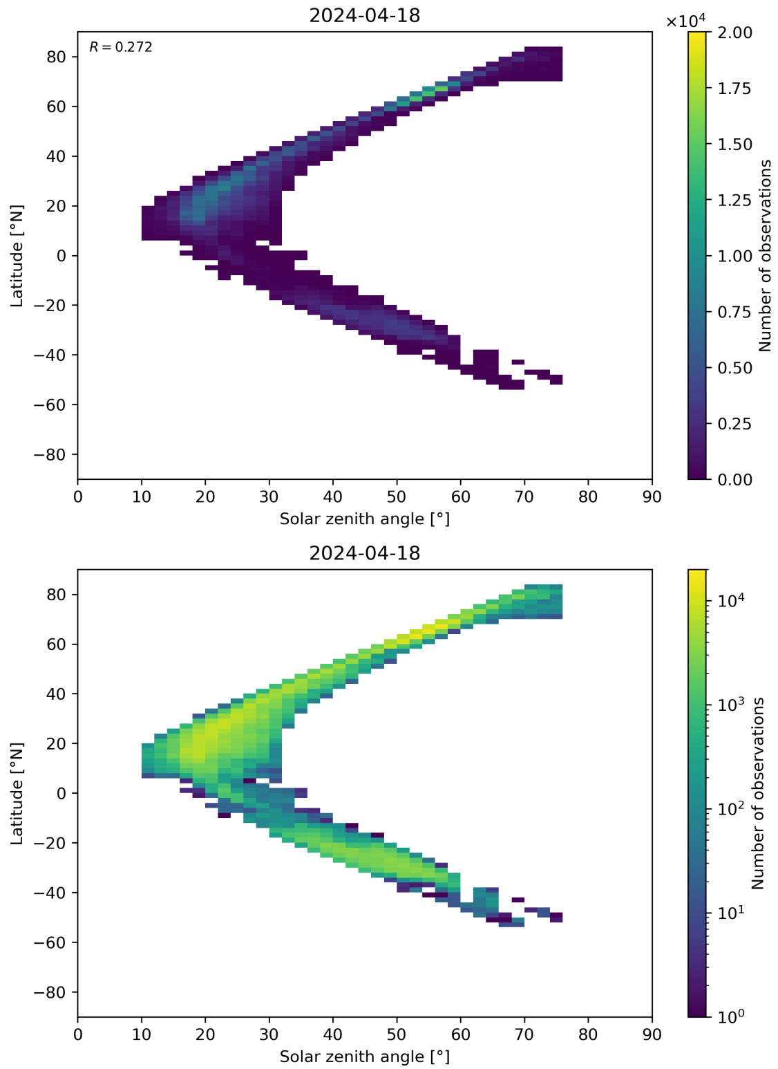
Figure 98: Scatter density plot of “Solar zenith angle” against “Latitude” for 2024-04-17 to 2024-04-19.
