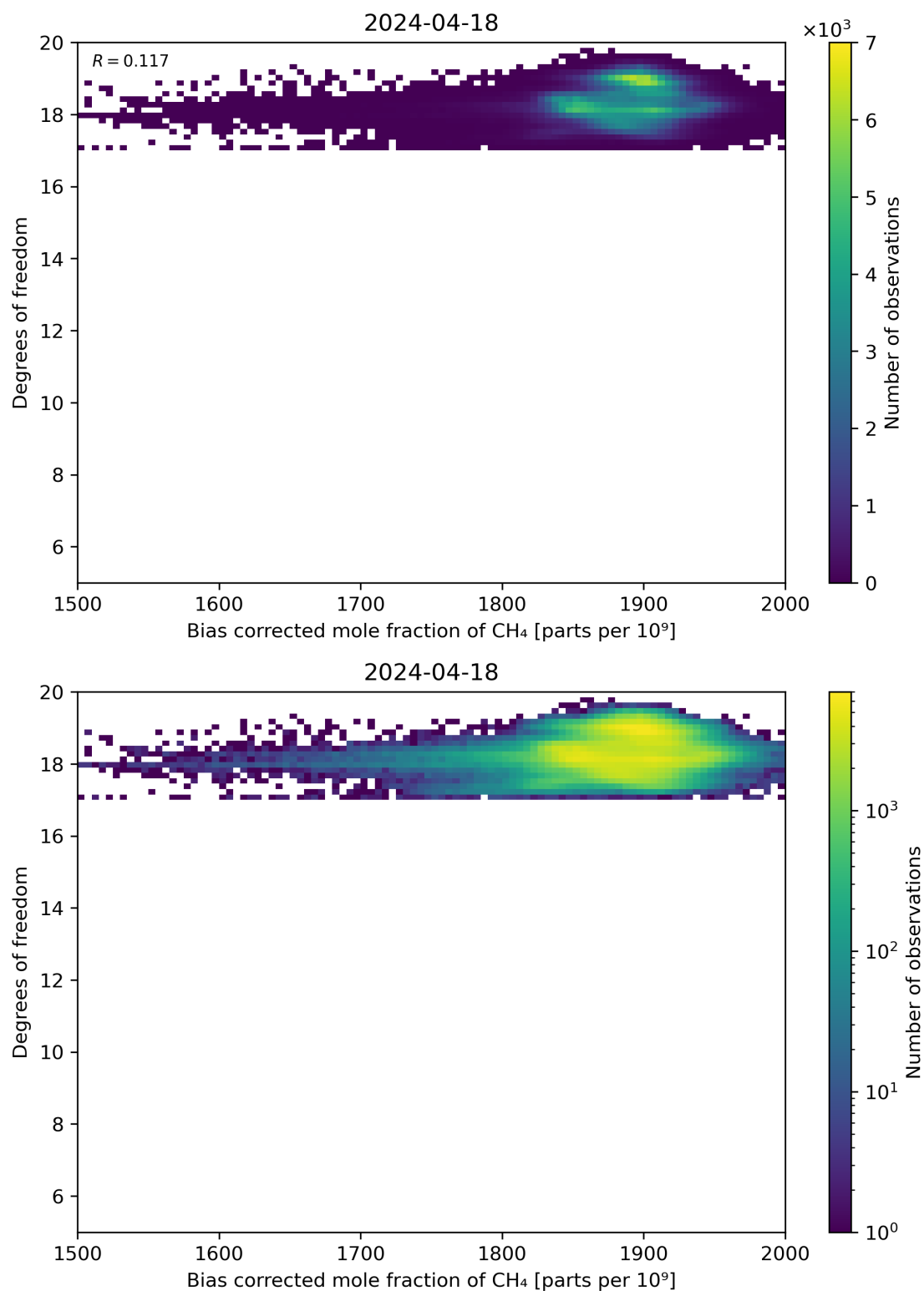
Figure 65: Scatter density plot of “Bias corrected mole fraction of CH 4 ” against “Degrees of freedom” for 2024-04-17 to 2024-04-19.
