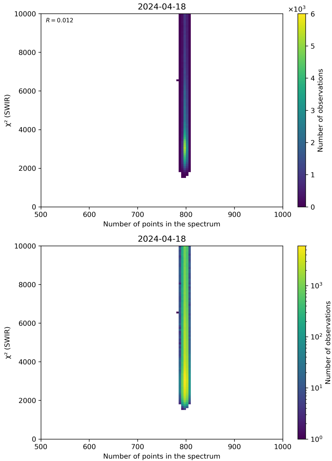
Figure 89: Scatter density plot of “Number of points in the spectrum” against “ \chi^2 (SWIR)” for 2024-04-17 to 2024-04-19.
