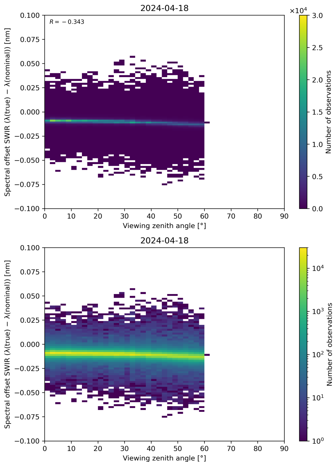
Figure 116: Scatter density plot of “Viewing zenith angle” against “Spectral offset SWIR ( \lambda(\text{true}) - \lambda(\text{nominal}) )” for 2024-04-17 to 2024-04-19.
