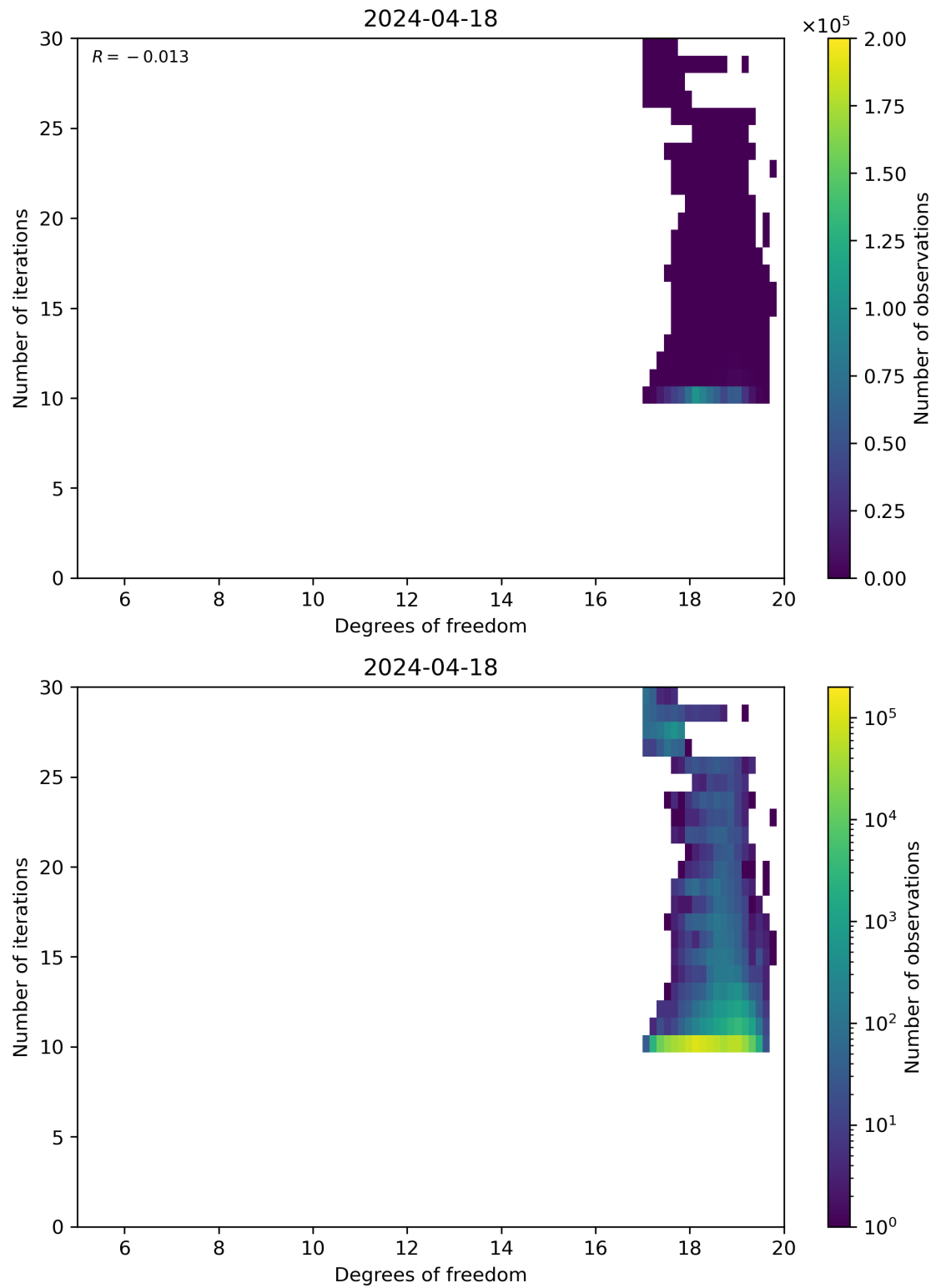
Figure 52: Scatter density plot of “Degrees of freedom” against “Number of iterations” for 2024-04-17 to 2024-04-19.
