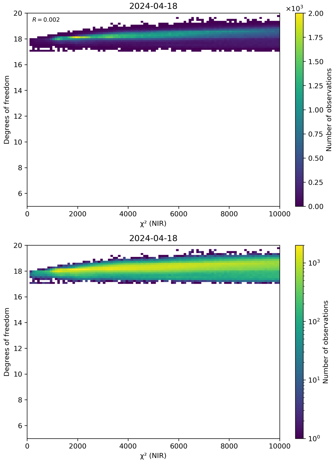
Figure 44: Scatter density plot of “ \chi^2 (NIR)” against “Degrees of freedom” for 2024-04-17 to 2024-04-19.
