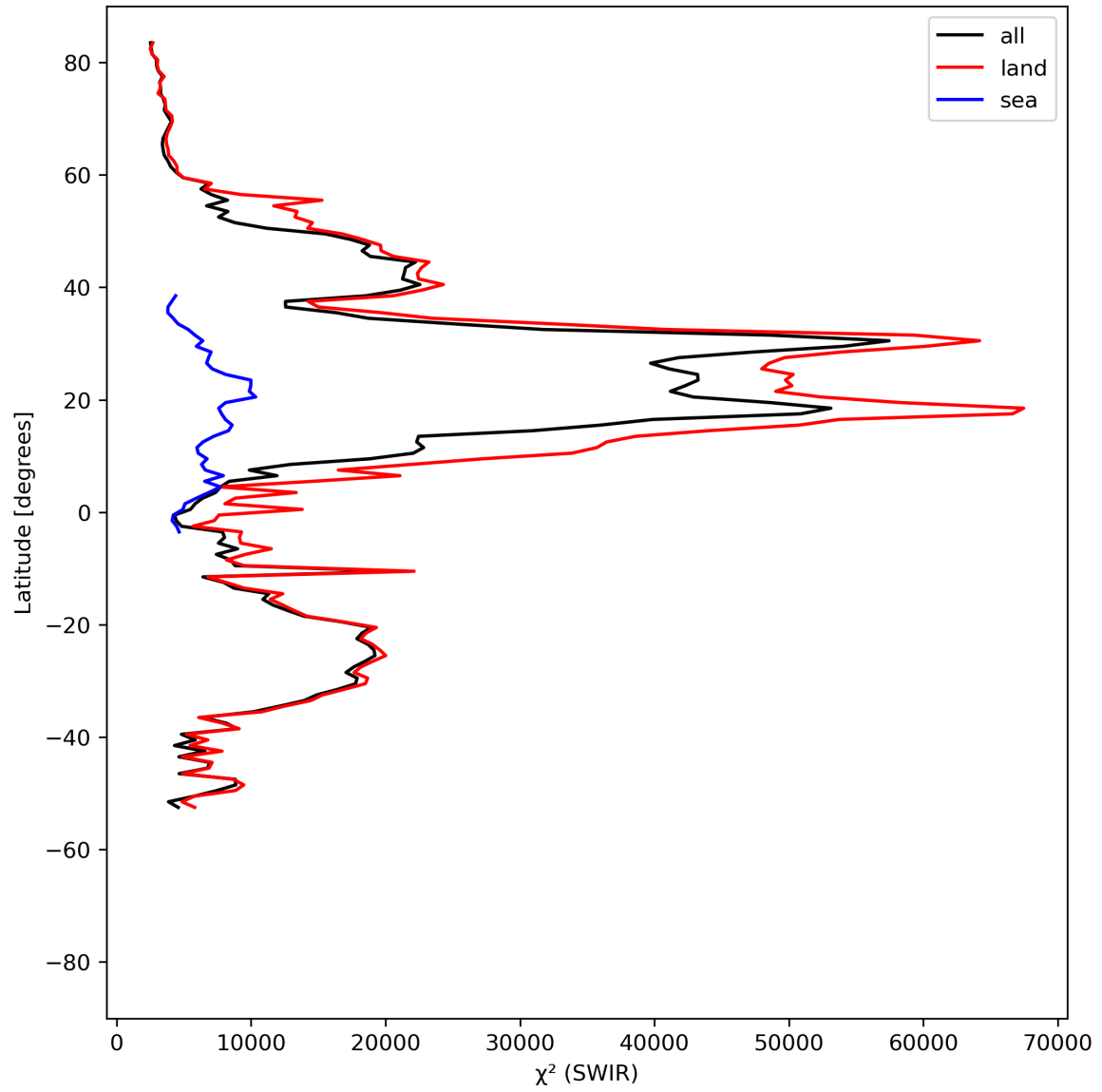
Figure 17: Zonal average of “ \chi^2 (SWIR)” for 2024-04-17 to 2024-04-19.
