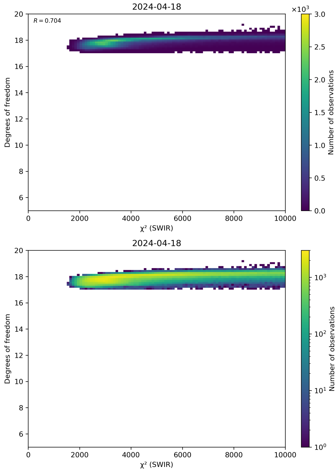
Figure 48: Scatter density plot of " \chi^2 (SWIR)" against "Degrees of freedom" for 2024-04-17 to 2024-04-19.
