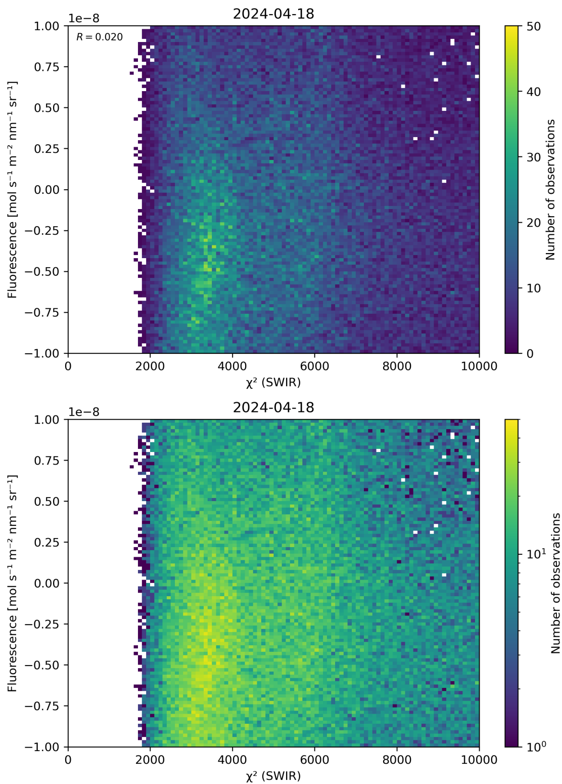
Figure 49: Scatter density plot of “ \chi^2 (SWIR)” against “Fluorescence” for 2024-04-17 to 2024-04-19.
