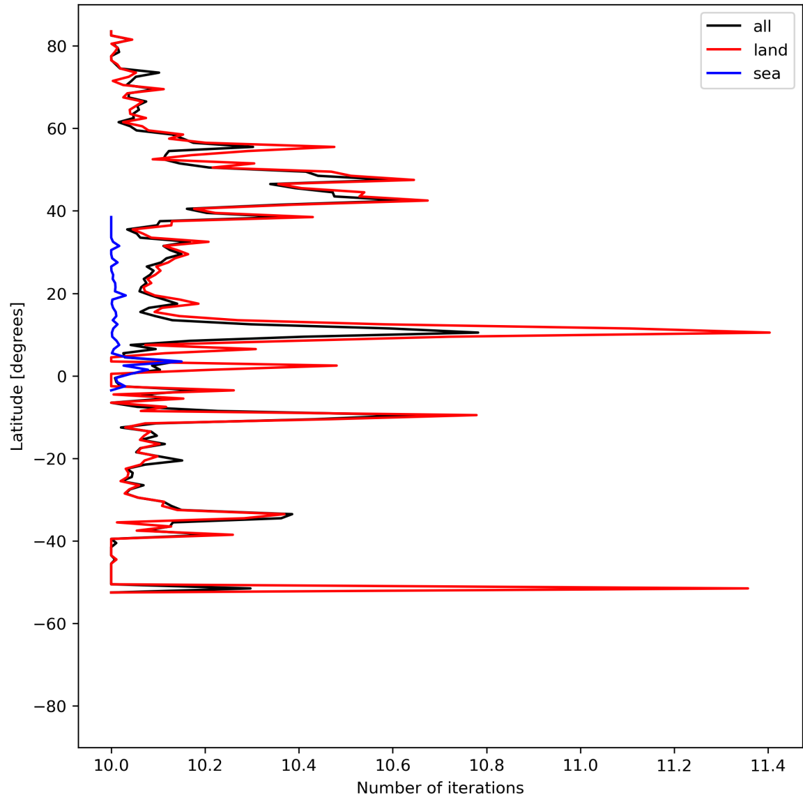
Figure 20: Zonal average of “Number of iterations” for 2024-04-17 to 2024-04-19.
