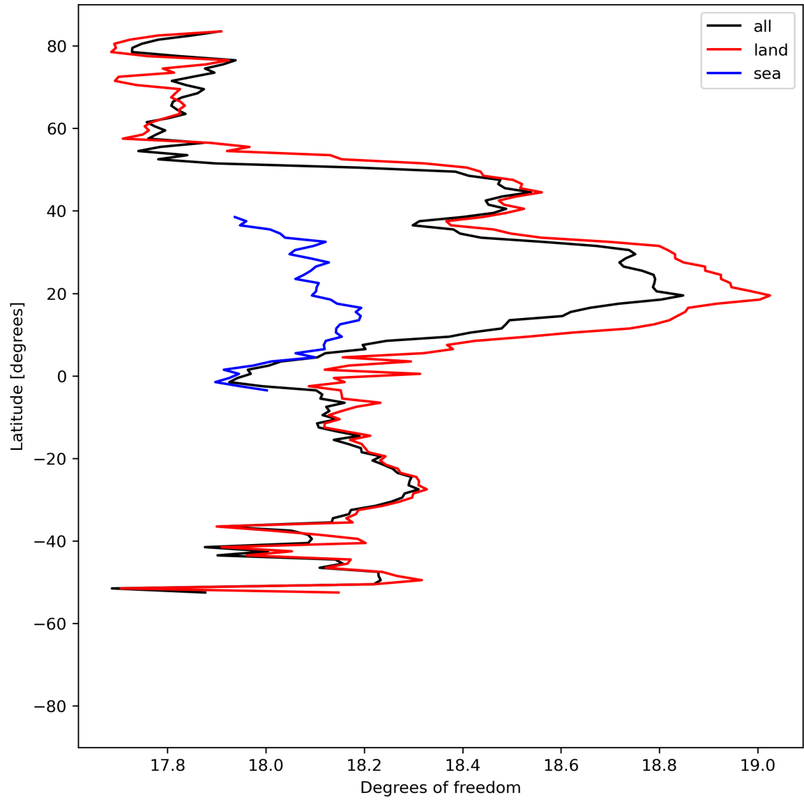
Figure 19: Zonal average of “Degrees of freedom” for 2024-04-17 to 2024-04-19.
