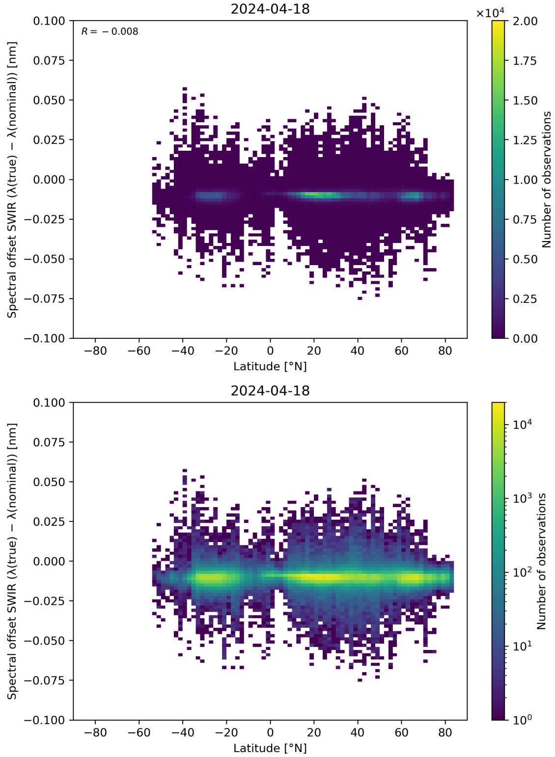
Figure 62: Scatter density plot of “Latitude” against “Spectral offset SWIR ( \lambda(\text{true}) - \lambda(\text{nominal}) )” for 2024-04-17 to 2024-04-19.
