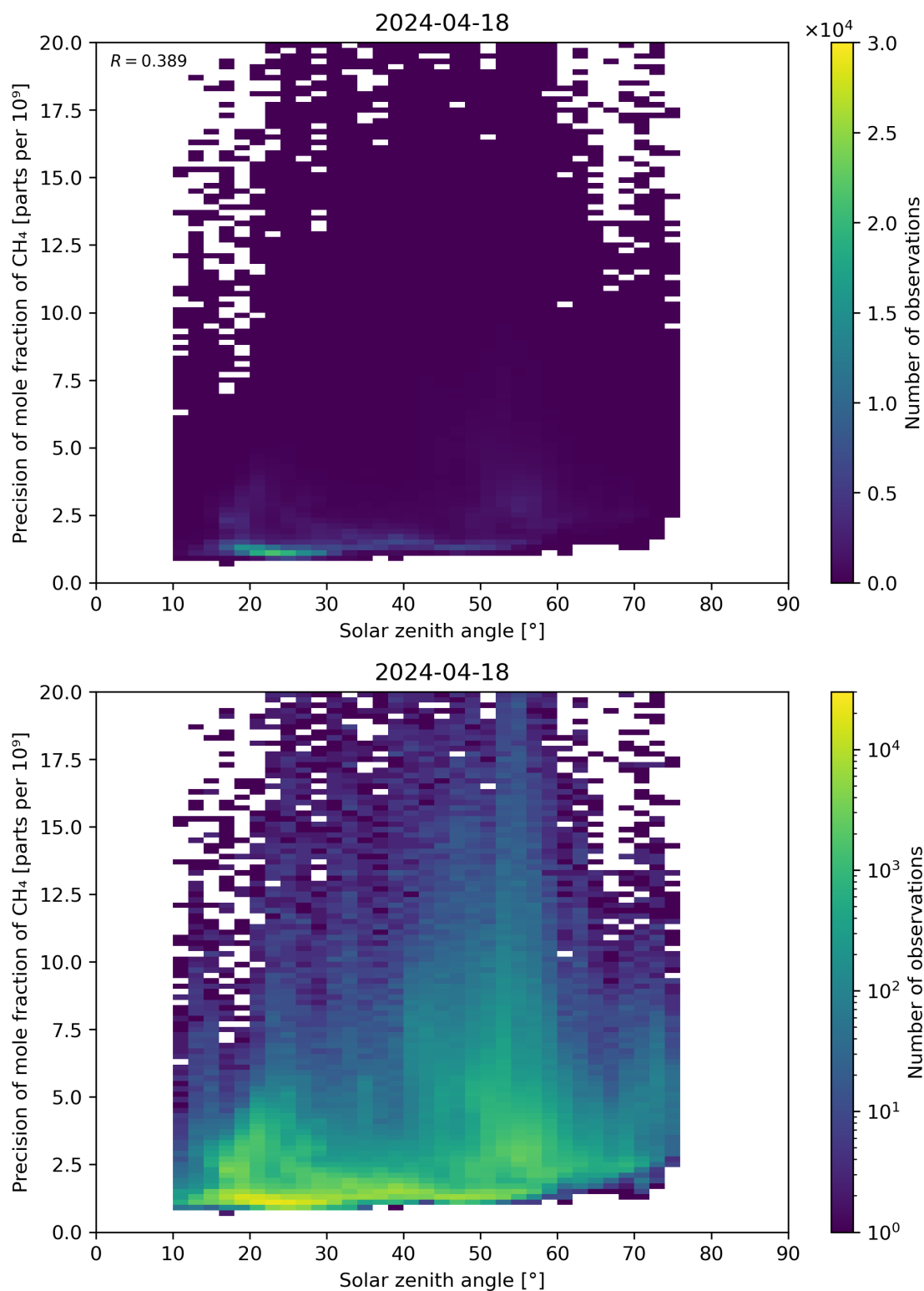
Figure 101: Scatter density plot of “Solar zenith angle” against “Precision of mole fraction of \text{CH}_4 ” for 2024-04-17 to 2024-04-19.
