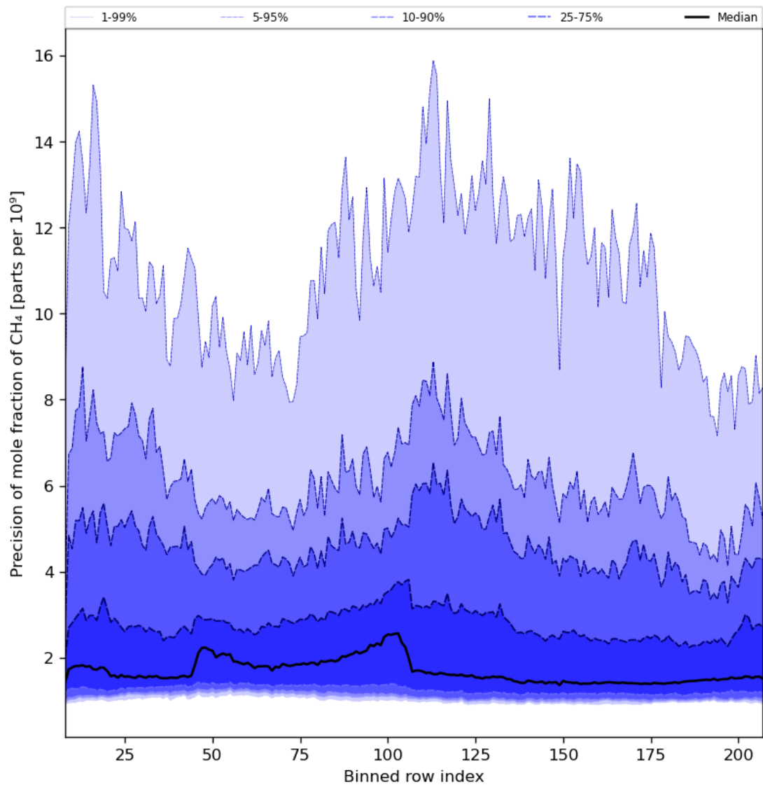
Figure 35: Along track statistics of “Precision of mole fraction of CH 4 ” for 2024-04-17 to 2024-04-19
