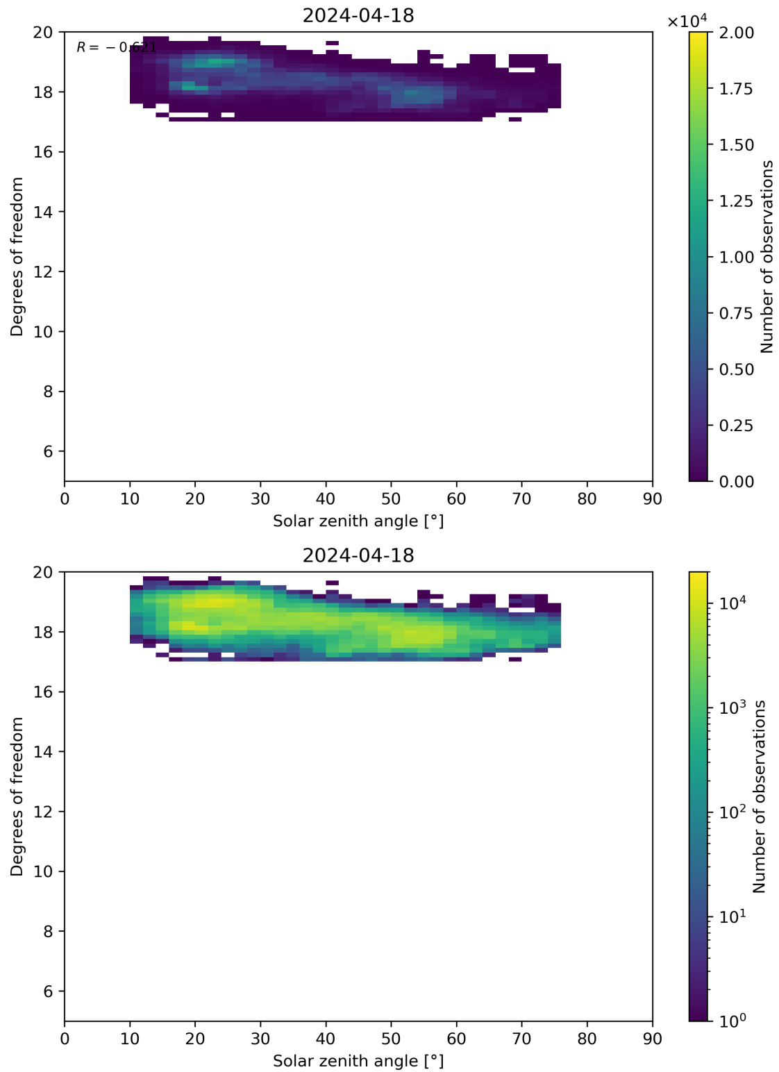
Figure 96: Scatter density plot of “Solar zenith angle” against “Degrees of freedom” for 2024-04-17 to 2024-04-19.
