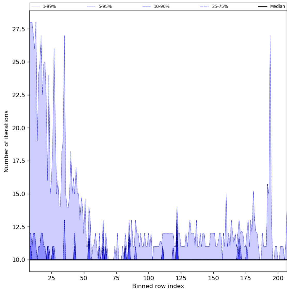
Figure 42: Along track statistics of “Number of iterations” for 2024-04-17 to 2024-04-19
