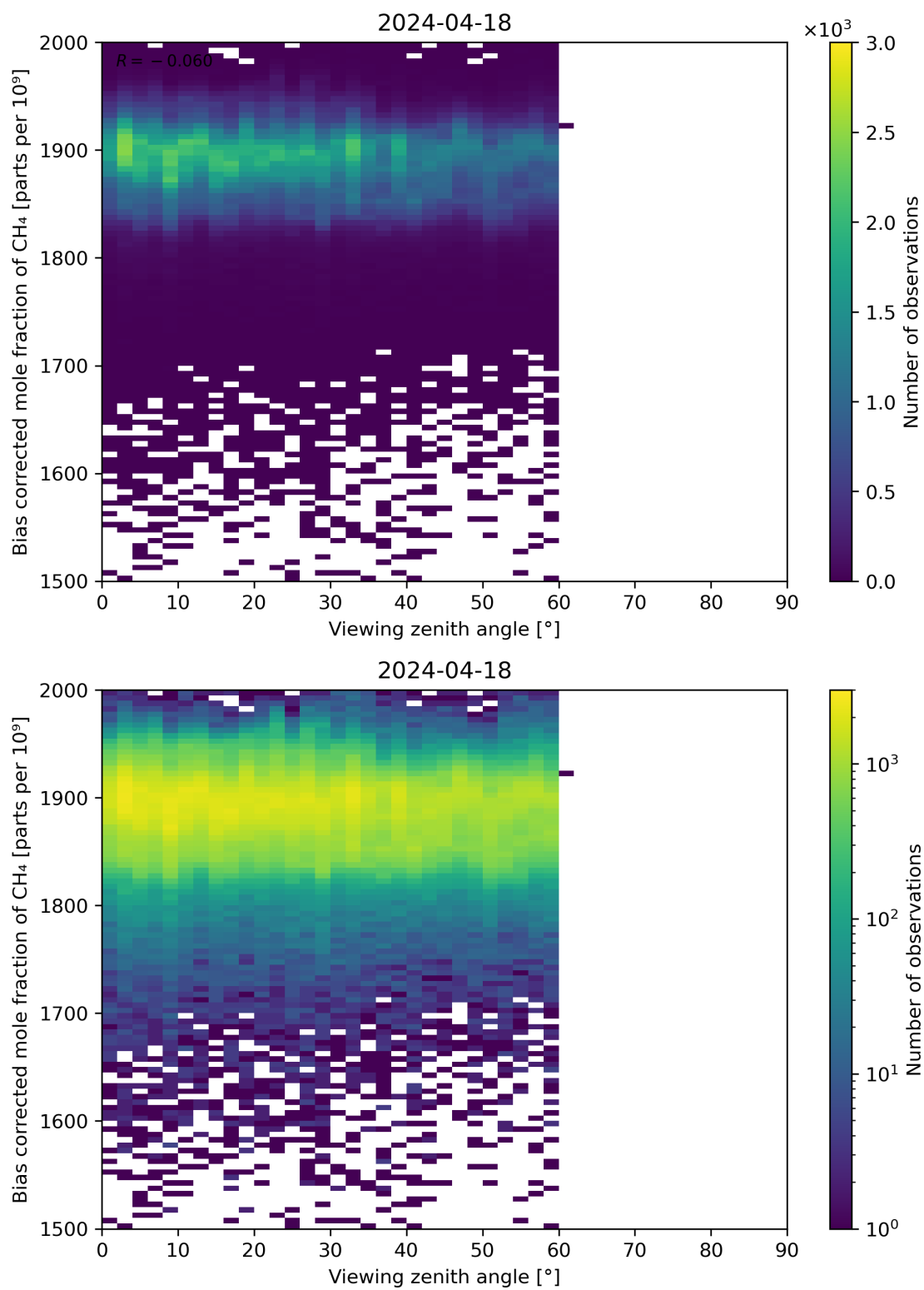
Figure 111: Scatter density plot of “Viewing zenith angle” against “Bias corrected mole fraction of CH 4 ” for 2024-04-17 to 2024-04-19.
