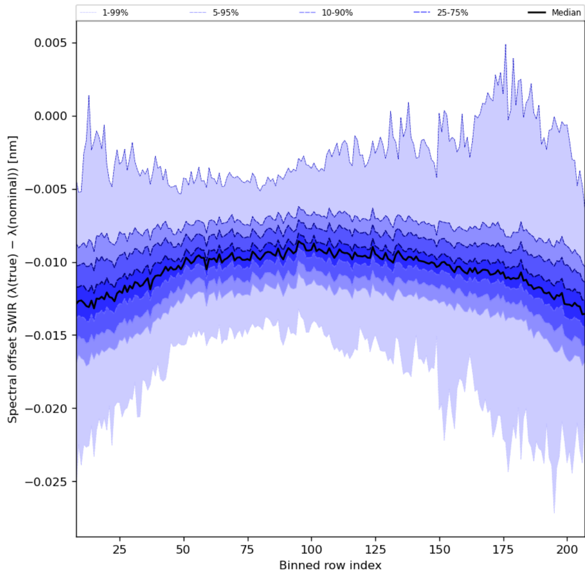
Figure 38: Along track statistics of “Spectral offset SWIR ( \lambda(\text{true}) - \lambda(\text{nominal}) )” for 2024-04-17 to 2024-04-19
