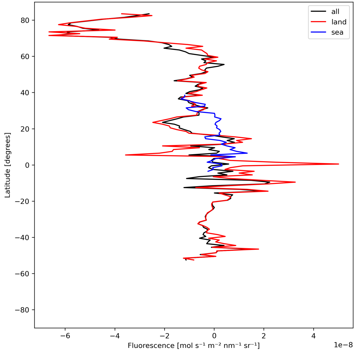
Figure 21: Zonal average of “Fluorescence” for 2024-04-17 to 2024-04-19.
