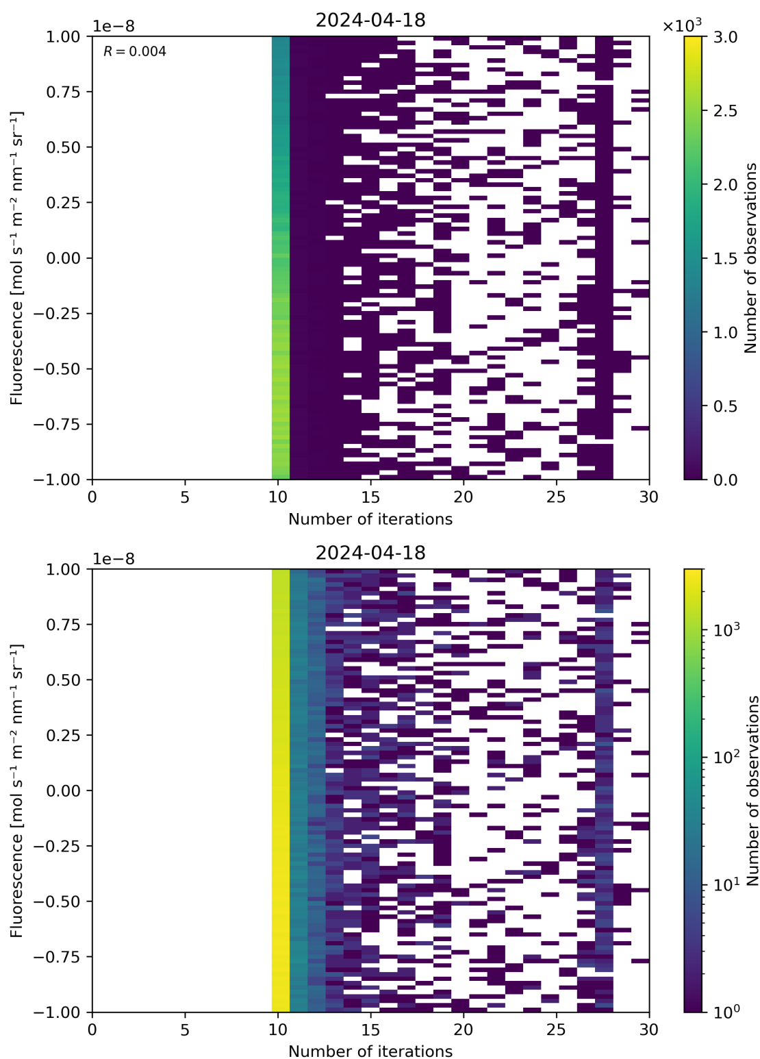
Figure 87: Scatter density plot of “Number of iterations” against “Fluorescence” for 2024-04-17 to 2024-04-19.
