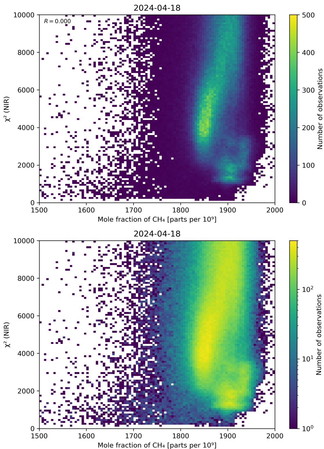
Figure 70: Scatter density plot of “Mole fraction of CH 4 ” against “ \chi^2 (NIR)” for 2024-04-17 to 2024-04-19.
