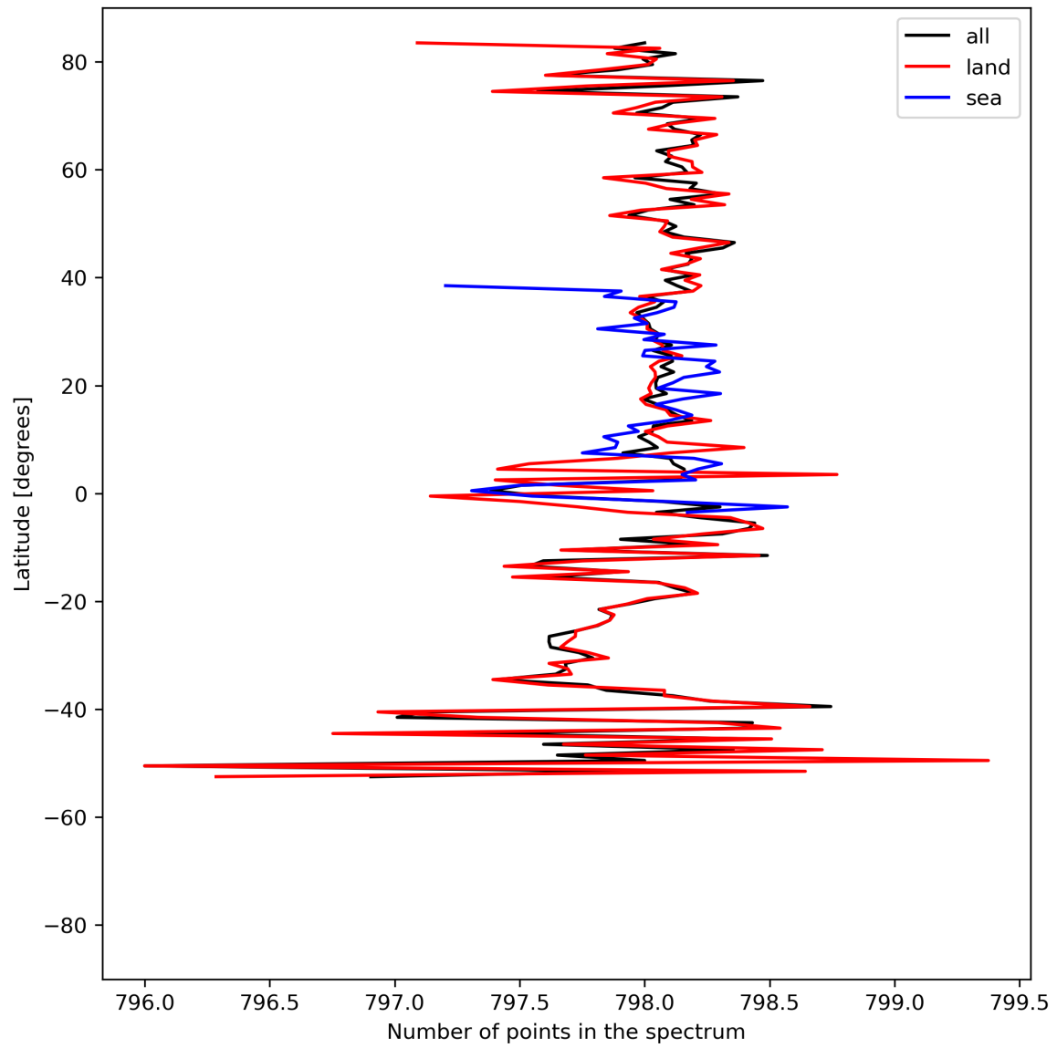
Figure 15: Zonal average of “Number of points in the spectrum” for 2024-04-17 to 2024-04-19.
