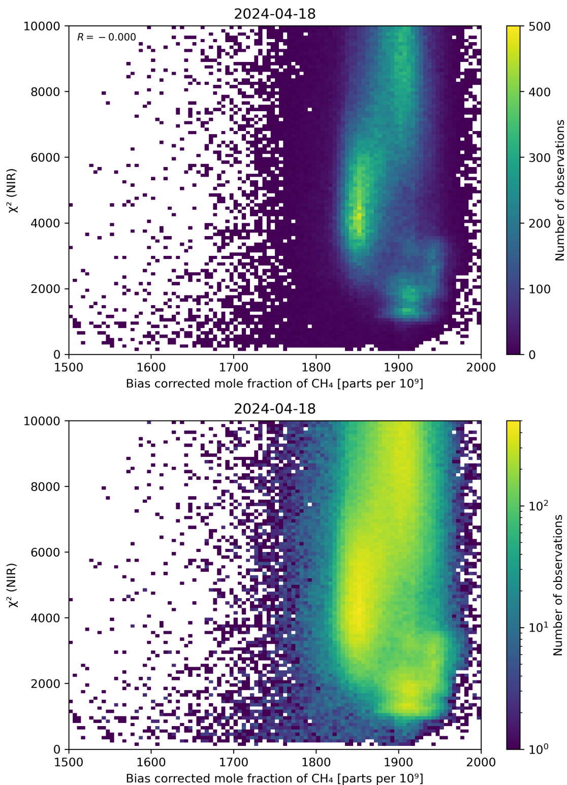
Figure 63: Scatter density plot of “Bias corrected mole fraction of CH 4 ” against “ \chi^2 (NIR)” for 2024-04-17 to 2024-04-19.
