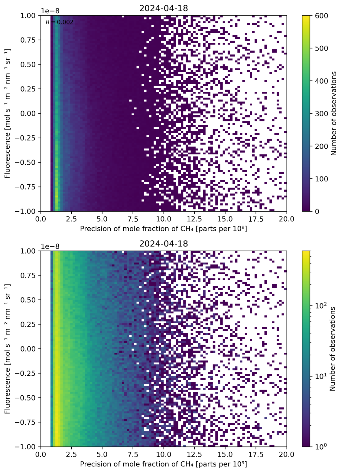
Figure 81: Scatter density plot of “Precision of mole fraction of \text{CH}_4 ” against “Fluorescence” for 2024-04-17 to 2024-04-19.
