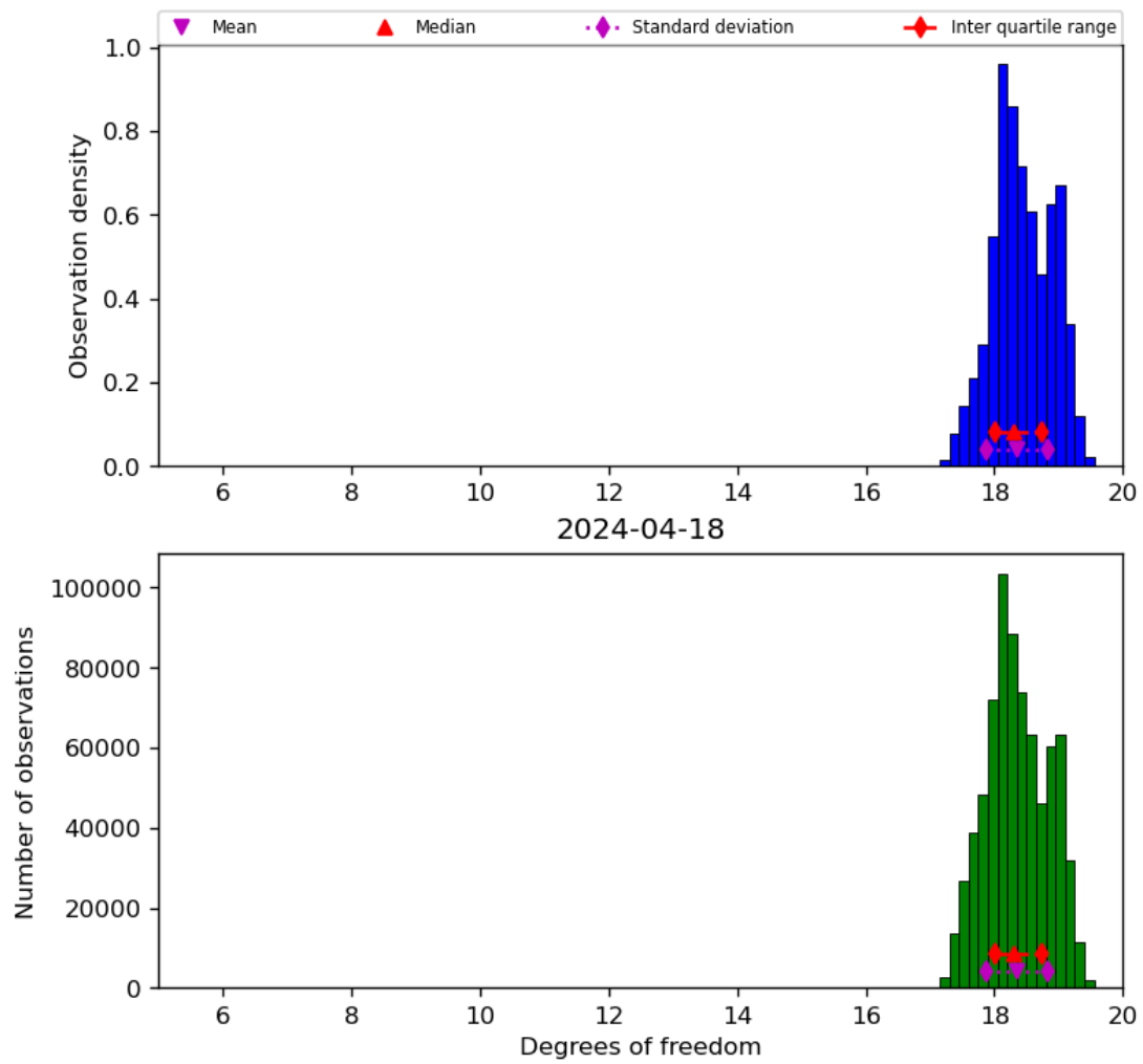
Figure 30: Histogram of “Degrees of freedom” for 2024-04-17 to 2024-04-19
