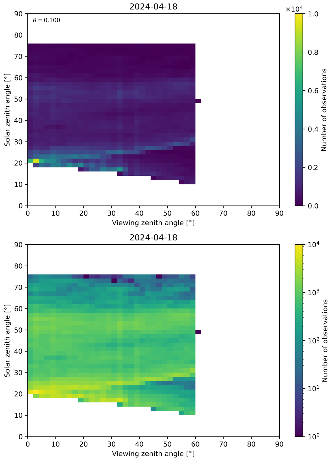
Figure 115: Scatter density plot of “Viewing zenith angle” against “Solar zenith angle” for 2024-04-17 to 2024-04-19.
