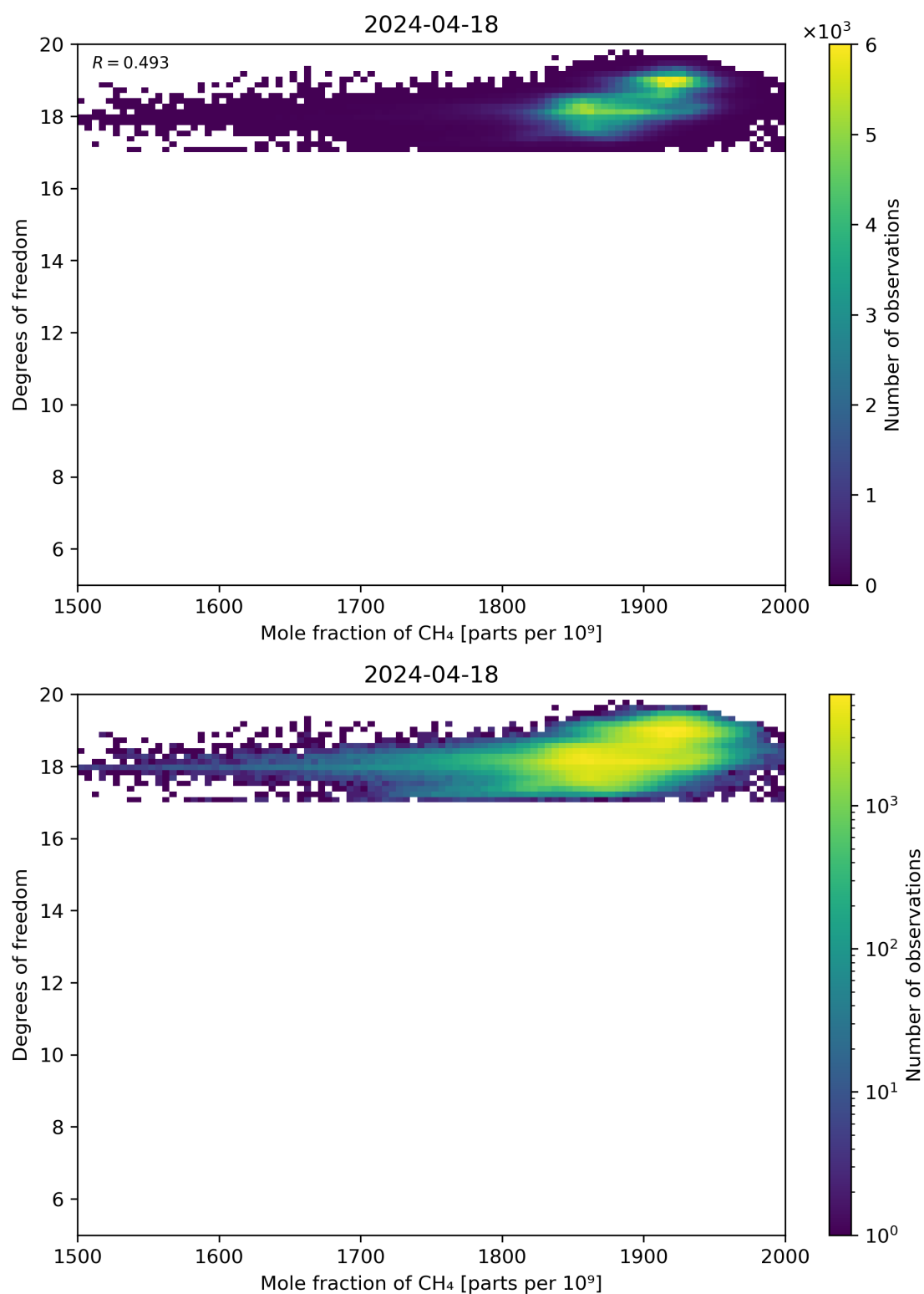
Figure 72: Scatter density plot of “Mole fraction of CH 4 ” against “Degrees of freedom” for 2024-04-17 to 2024-04-19.
