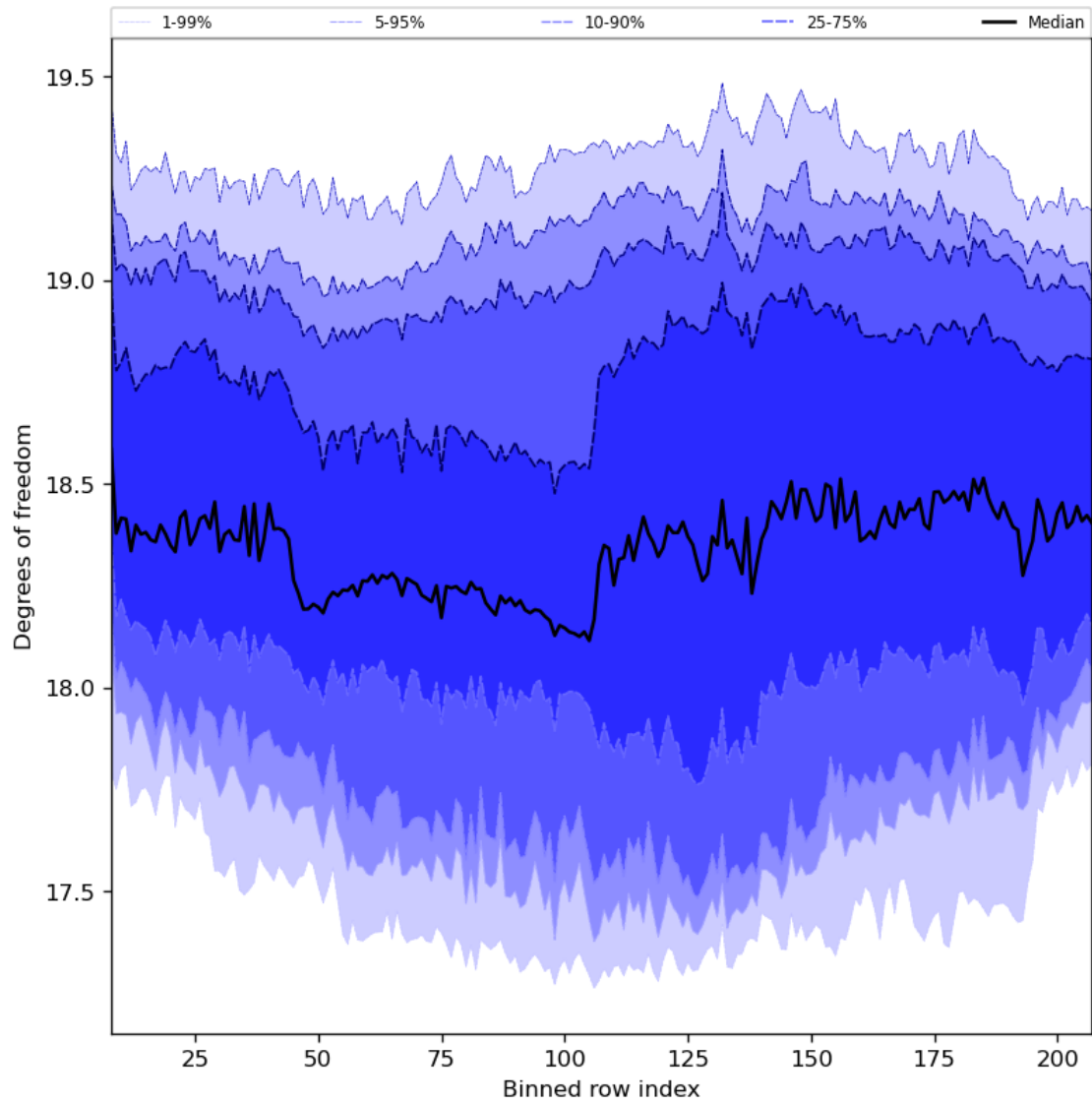
Figure 41: Along track statistics of “Degrees of freedom” for 2024-04-17 to 2024-04-19
