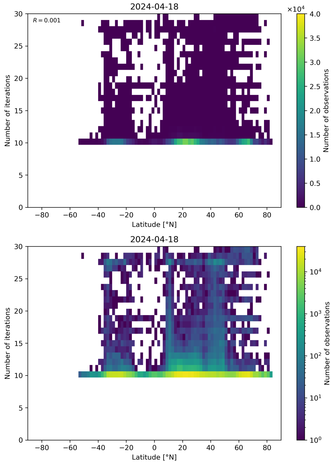
Figure 60: Scatter density plot of “Latitude” against “Number of iterations” for 2024-04-17 to 2024-04-19.
