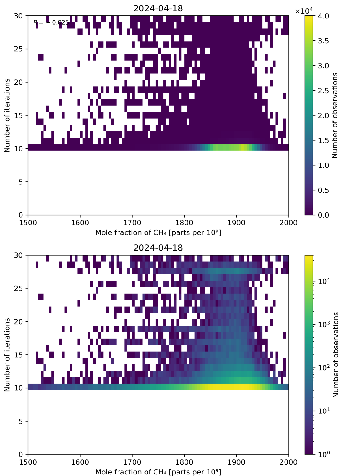
Figure 76: Scatter density plot of “Mole fraction of CH 4 ” against “Number of iterations” for 2024-04-17 to 2024-04-19.
