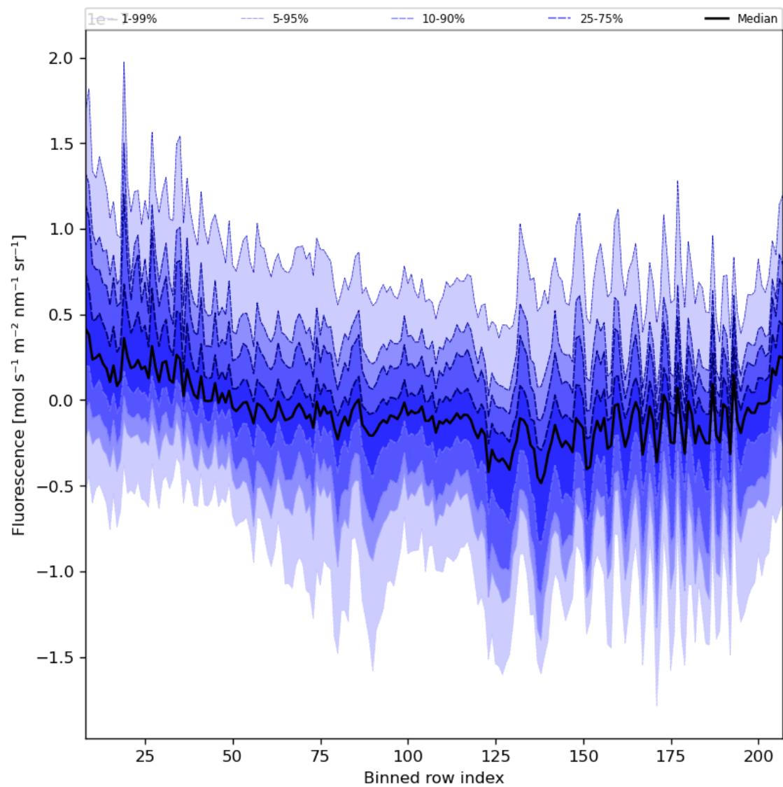
Figure 43: Along track statistics of “Fluorescence” for 2024-04-17 to 2024-04-19
