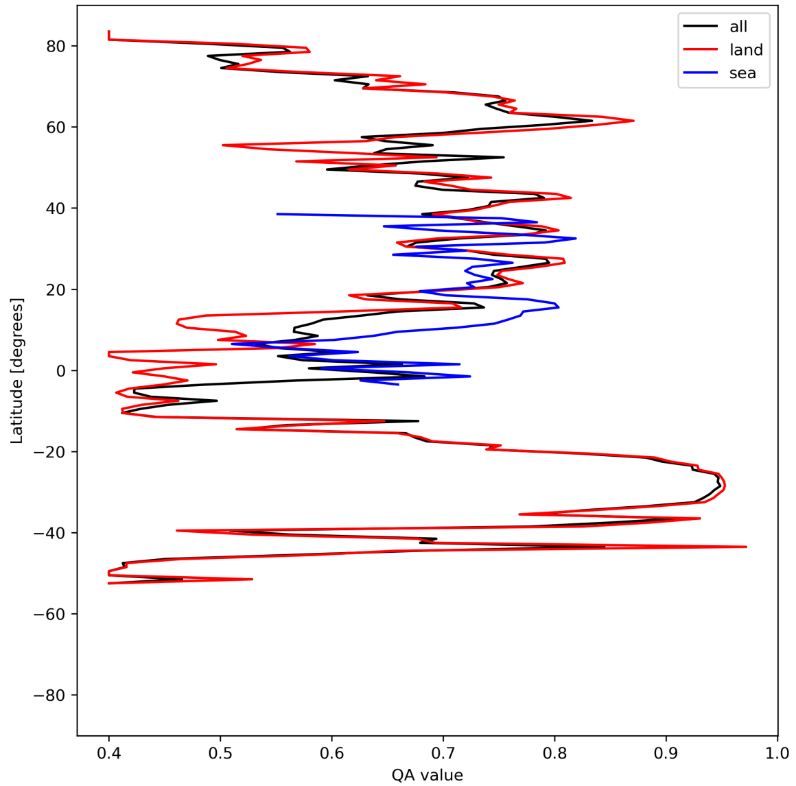
Figure 11: Zonal average of “QA value” for 2024-04-17 to 2024-04-19.
