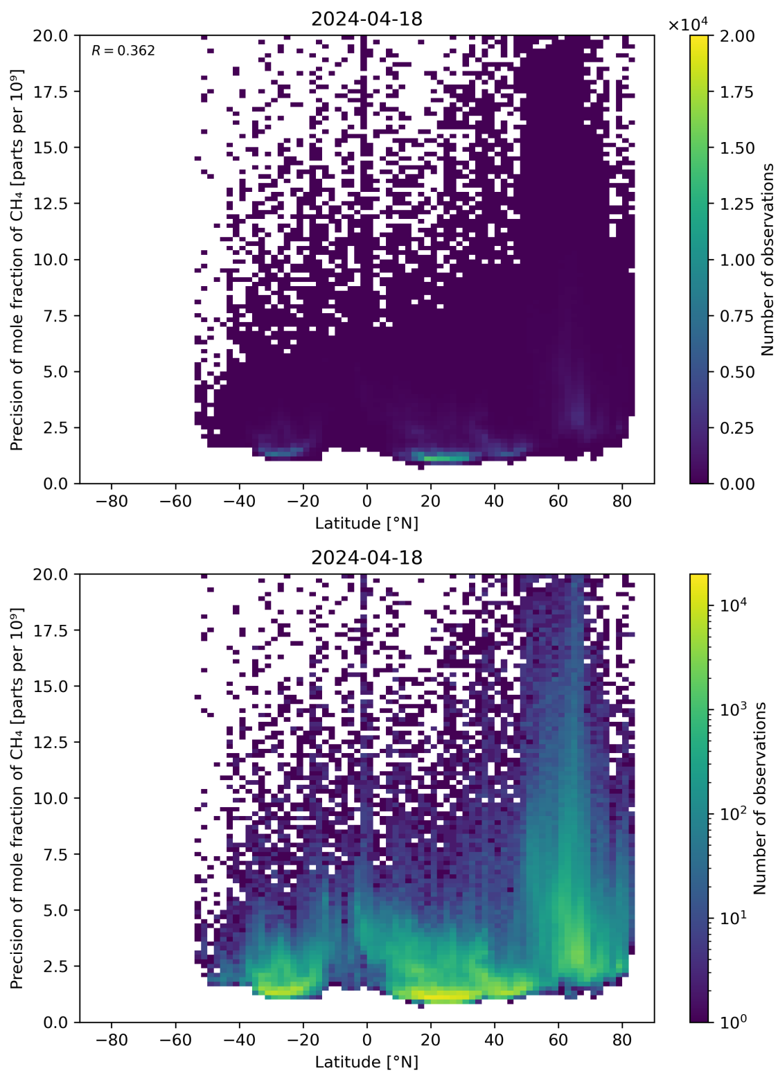
Figure 59: Scatter density plot of “Latitude” against “Precision of mole fraction of \text{CH}_4 ” for 2024-04-17 to 2024-04-19.
