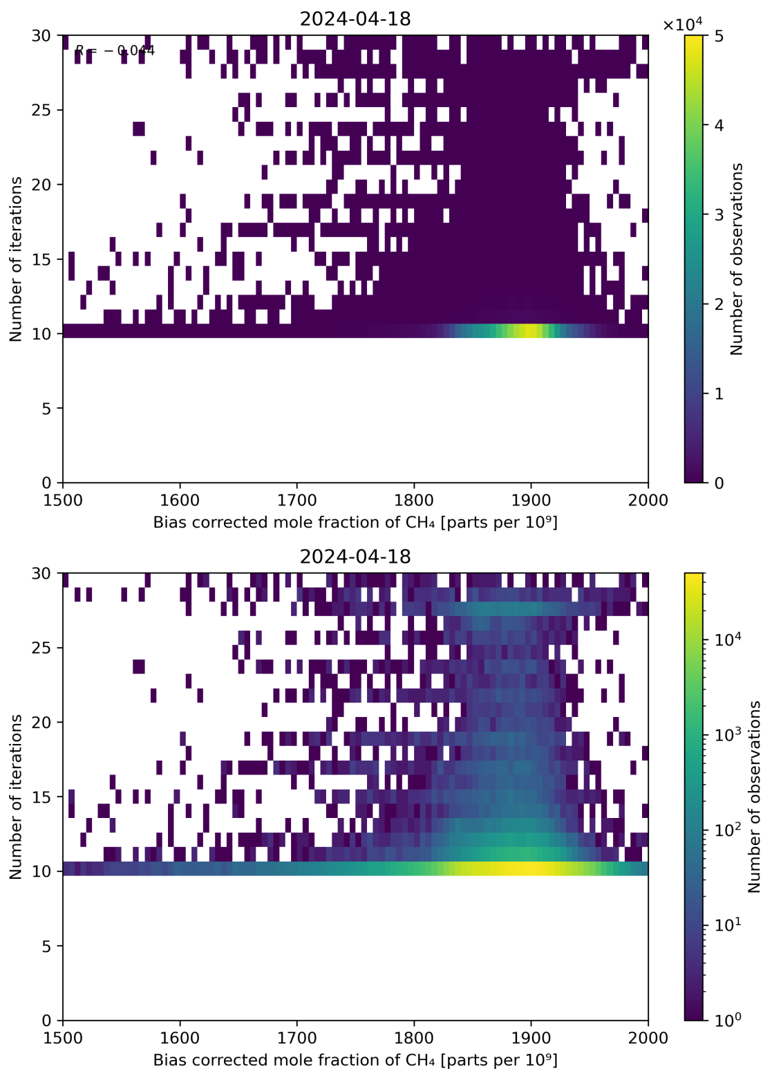
Figure 67: Scatter density plot of “Bias corrected mole fraction of \text{CH}_4 ” against “Number of iterations” for 2024-04-17 to 2024-04-19.
