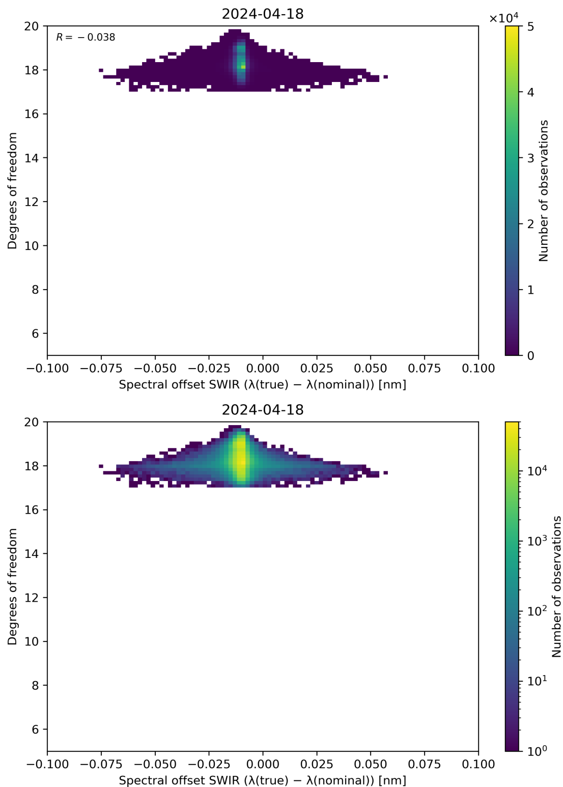
Figure 119: Scatter density plot of “Spectral offset SWIR ( \lambda(\text{true}) - \lambda(\text{nominal}) )” against “Degrees of freedom” for 2024-04-17 to 2024-04-19.
