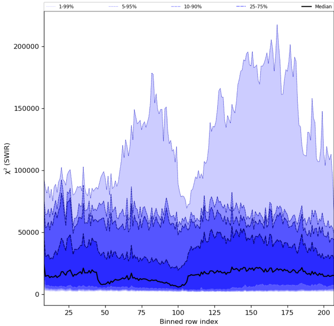
Figure 39: Along track statistics of “ \chi^2 (SWIR)” for 2024-04-17 to 2024-04-19
