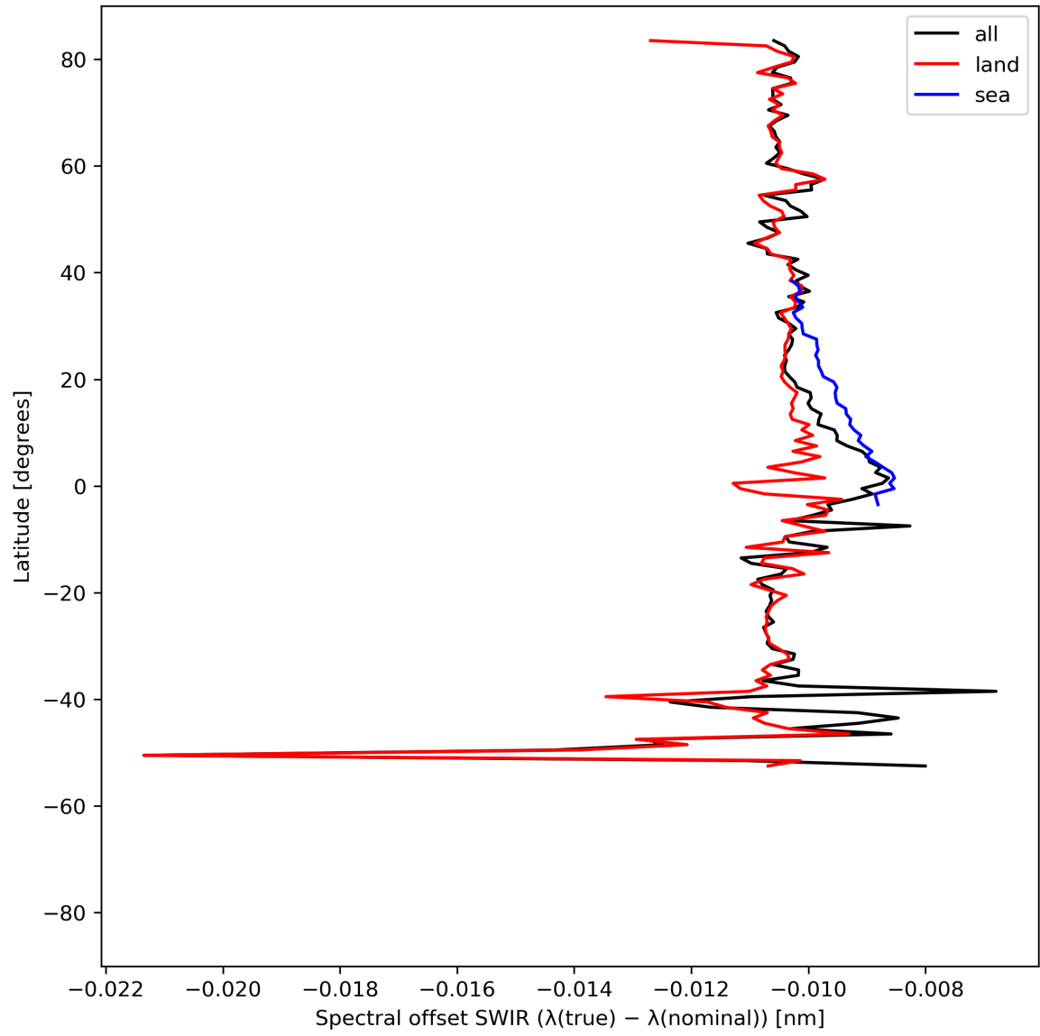
Figure 16: Zonal average of “Spectral offset SWIR ( \lambda(\text{true}) - \lambda(\text{nominal}) )” for 2024-04-17 to 2024-04-19.
