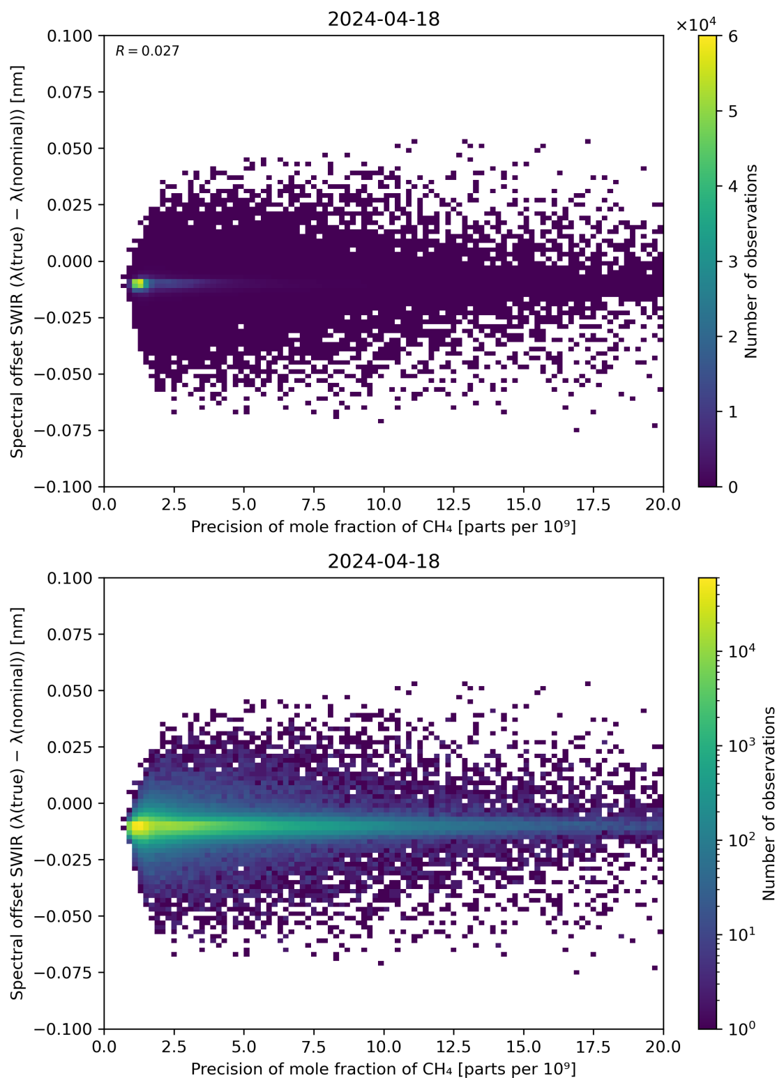
Figure 85: Scatter density plot of “Precision of mole fraction of CH 4 ” against “Spectral offset SWIR ( \lambda(\text{true}) - \lambda(\text{nominal}) )” for 2024-04-17 to 2024-04-19.
