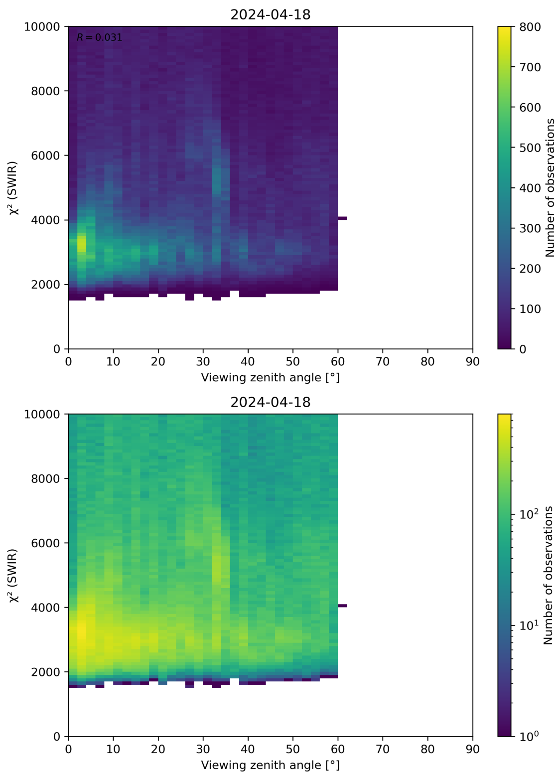
Figure 106: Scatter density plot of “Viewing zenith angle” against “ \chi^2 (SWIR)” for 2024-04-17 to 2024-04-19.
