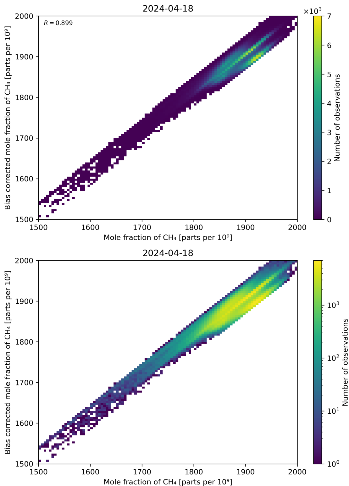
Figure 74: Scatter density plot of “Mole fraction of CH 4 ” against “Bias corrected mole fraction of CH 4 ” for 2024-04-17 to 2024-04-19.
