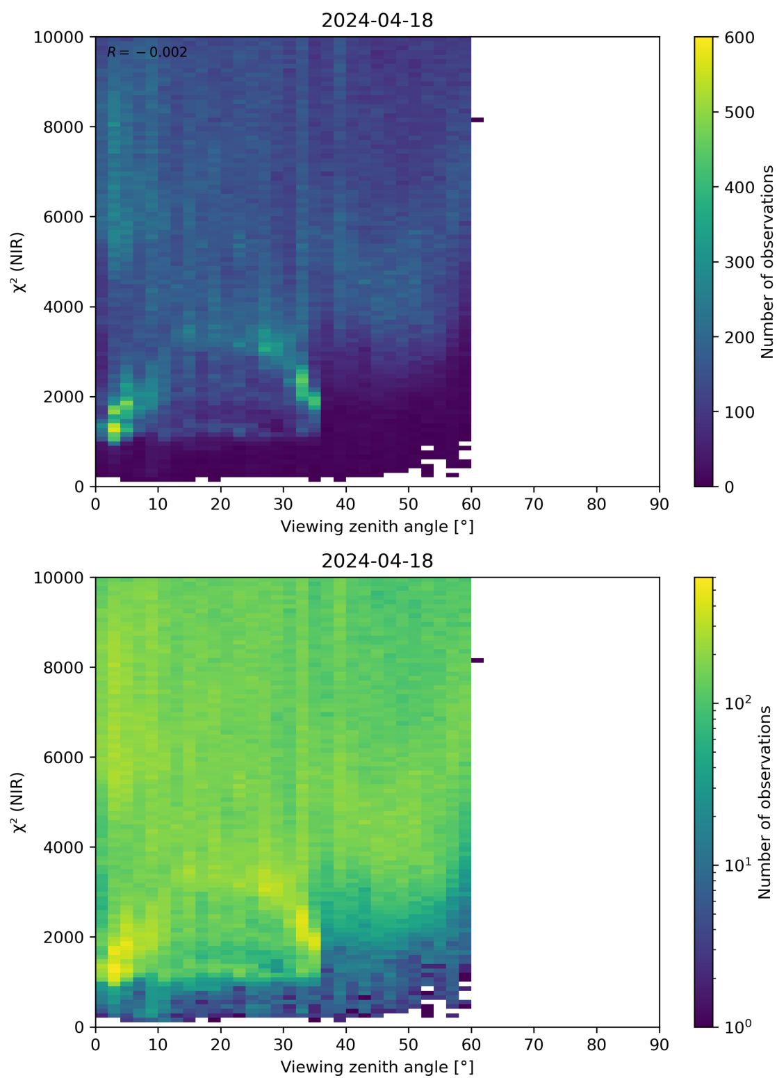
Figure 105: Scatter density plot of “Viewing zenith angle” against “ \chi^2 (NIR)” for 2024-04-17 to 2024-04-19.
