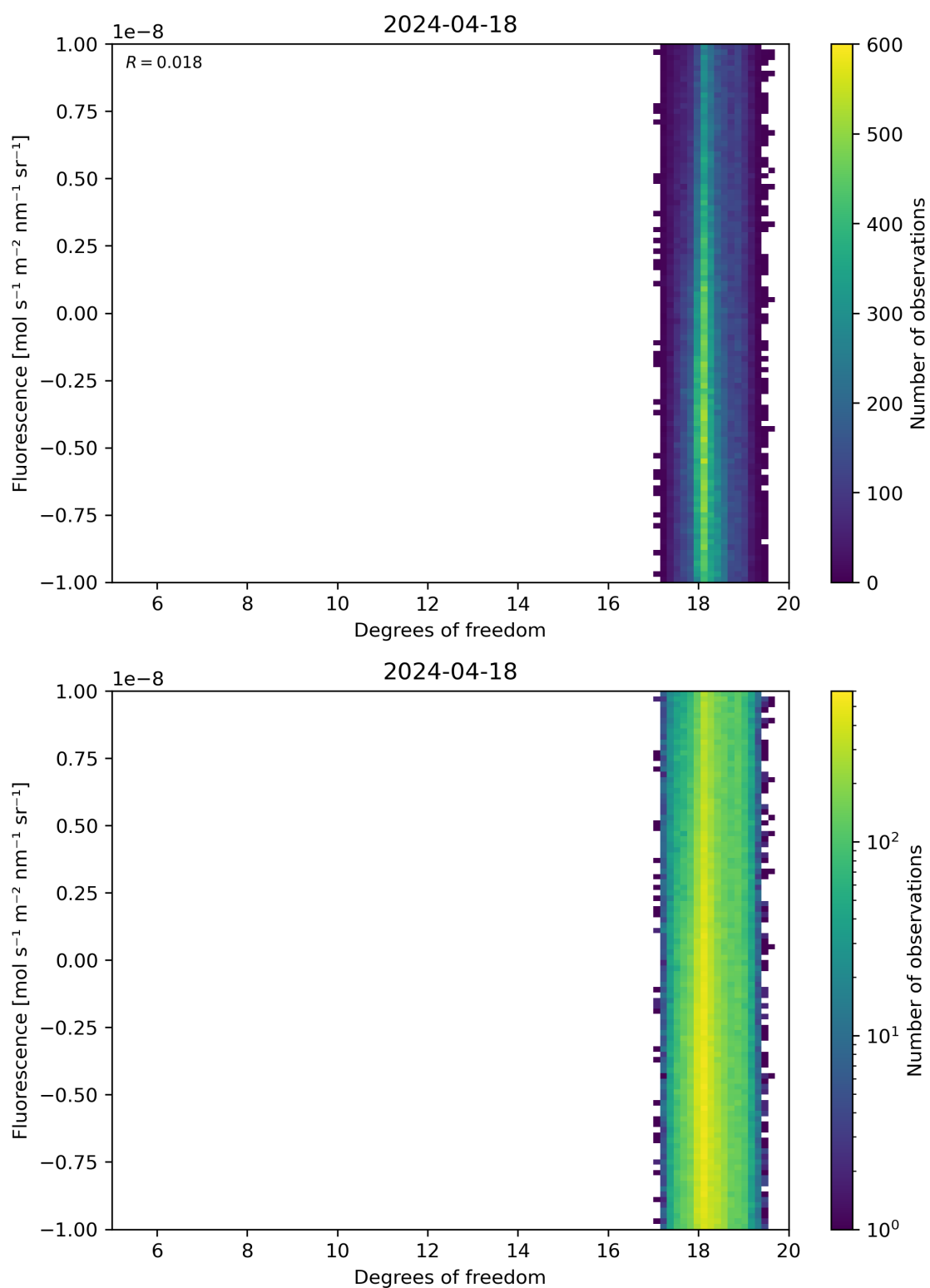
Figure 51: Scatter density plot of “Degrees of freedom” against “Fluorescence” for 2024-04-17 to 2024-04-19.
