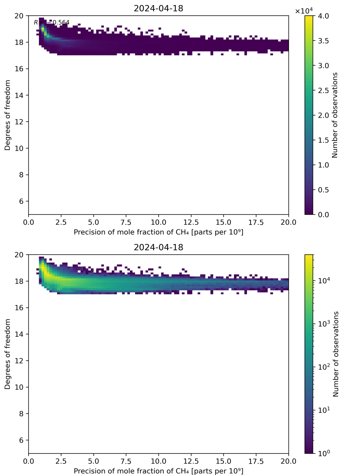
Figure 80: Scatter density plot of “Precision of mole fraction of CH 4 ” against “Degrees of freedom” for 2024-04-17 to 2024-04-19.
