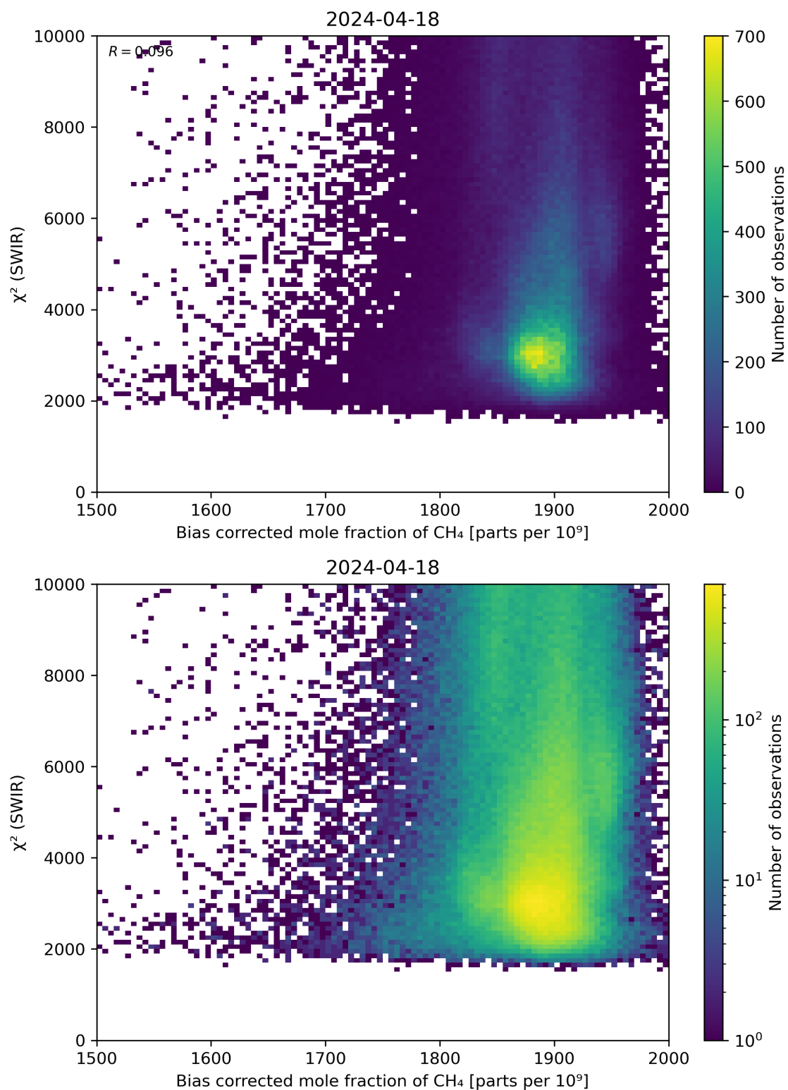
Figure 64: Scatter density plot of “Bias corrected mole fraction of \text{CH}_4 ” against “ \chi^2 (SWIR)” for 2024-04-17 to 2024-04-19.
