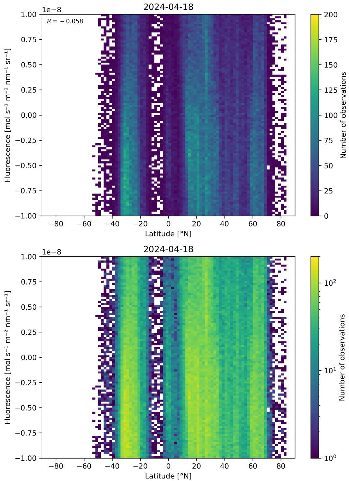
Figure 56: Scatter density plot of “Latitude” against “Fluorescence” for 2024-04-17 to 2024-04-19.
