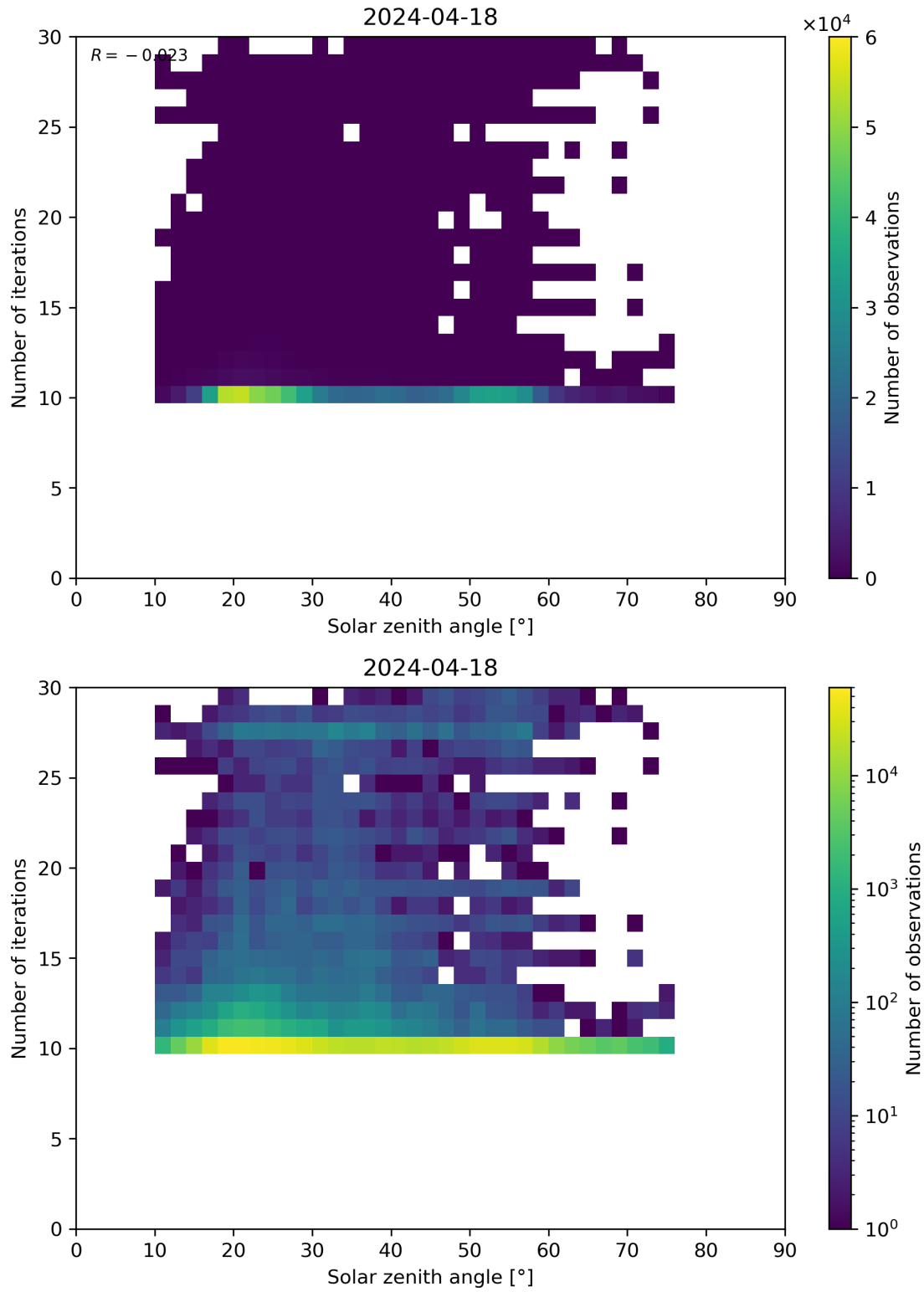
Figure 102: Scatter density plot of “Solar zenith angle” against “Number of iterations” for 2024-04-17 to 2024-04-19.
