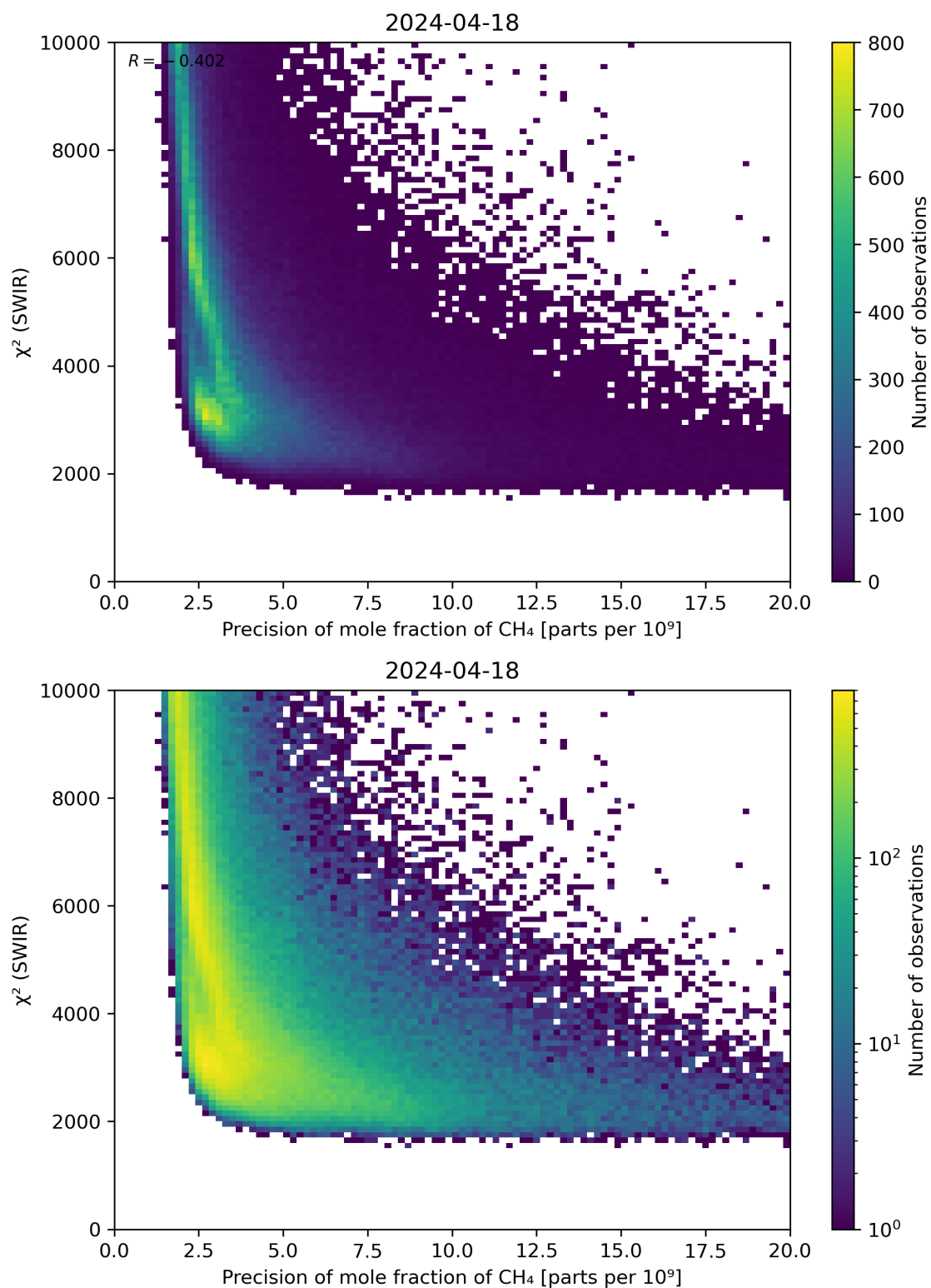
Figure 79: Scatter density plot of “Precision of mole fraction of \text{CH}_4 ” against “ \chi^2 (SWIR)” for 2024-04-17 to 2024-04-19.
