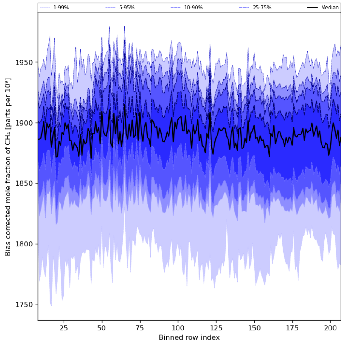
Figure 36: Along track statistics of “Bias corrected mole fraction of CH 4 ” for 2024-04-17 to 2024-04-19
