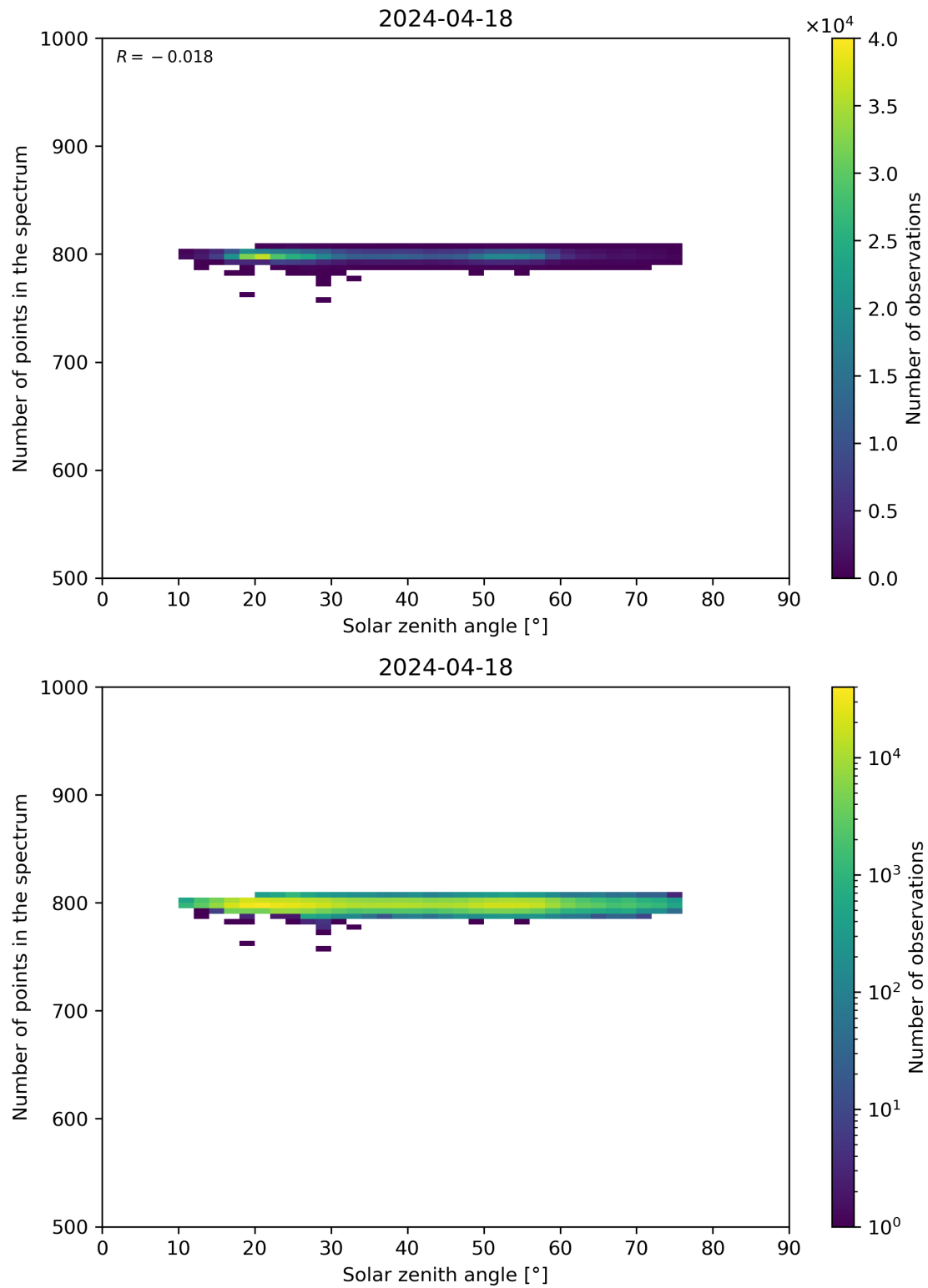
Figure 103: Scatter density plot of “Solar zenith angle” against “Number of points in the spectrum” for 2024-04-17 to 2024-04-19.
