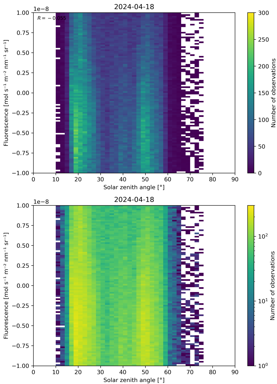
Figure 97: Scatter density plot of “Solar zenith angle” against “Fluorescence” for 2024-04-17 to 2024-04-19.
