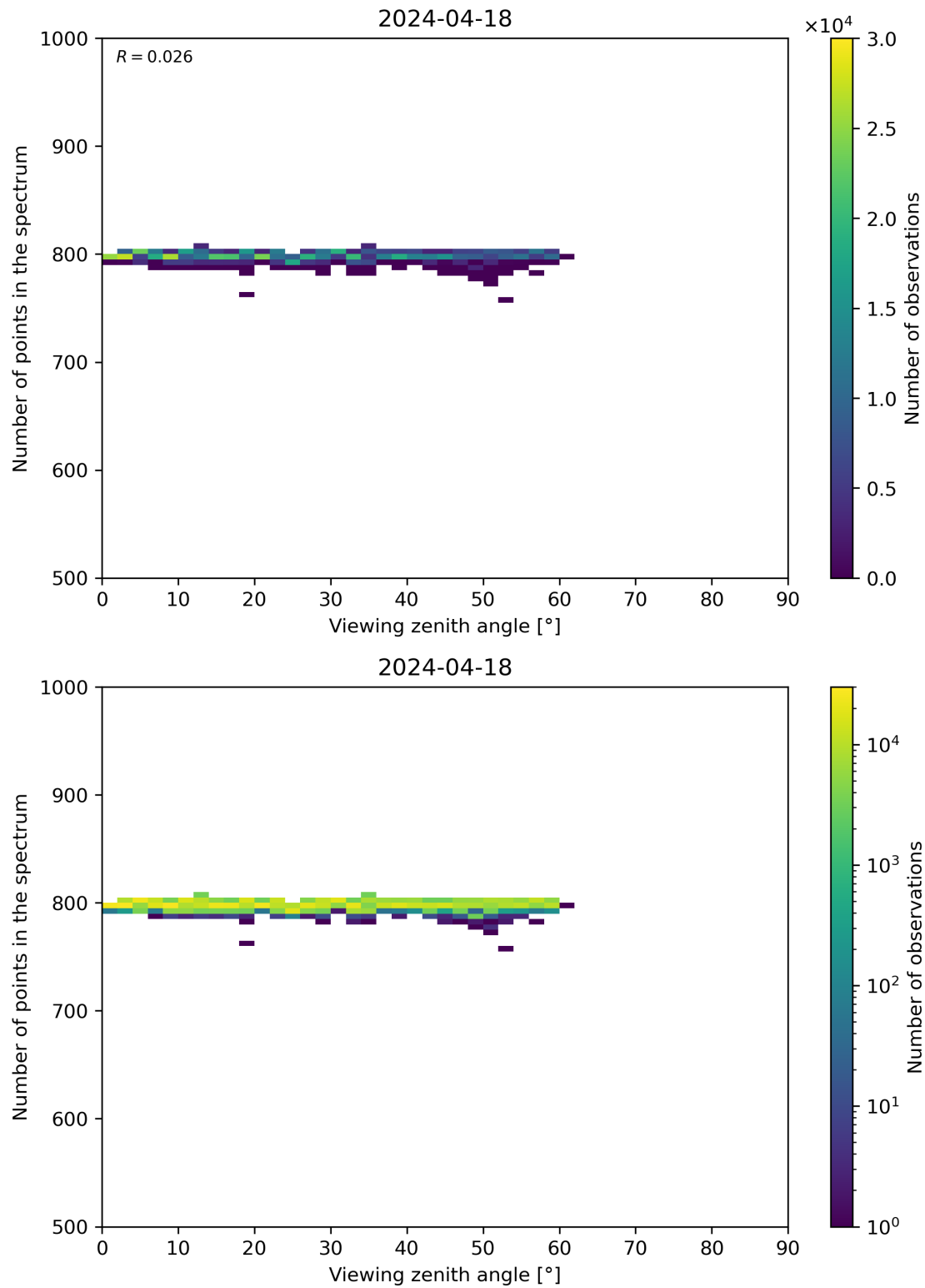
Figure 114: Scatter density plot of “Viewing zenith angle” against “Number of points in the spectrum” for 2024-04-17 to 2024-04-19.
