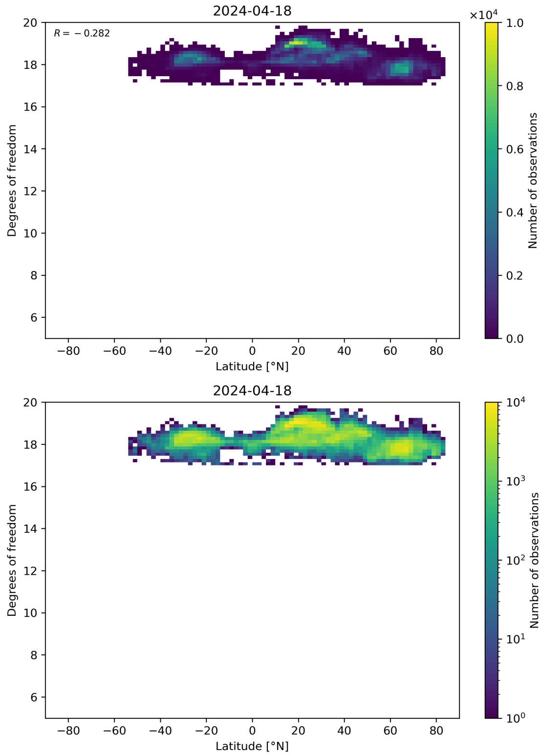
Figure 55: Scatter density plot of “Latitude” against “Degrees of freedom” for 2024-04-17 to 2024-04-19.
