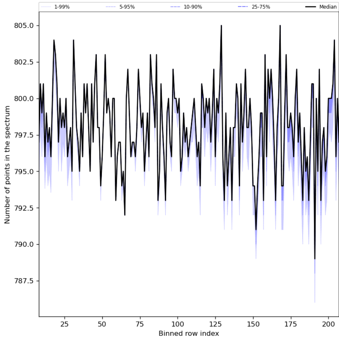
Figure 37: Along track statistics of “Number of points in the spectrum” for 2024-04-17 to 2024-04-19
