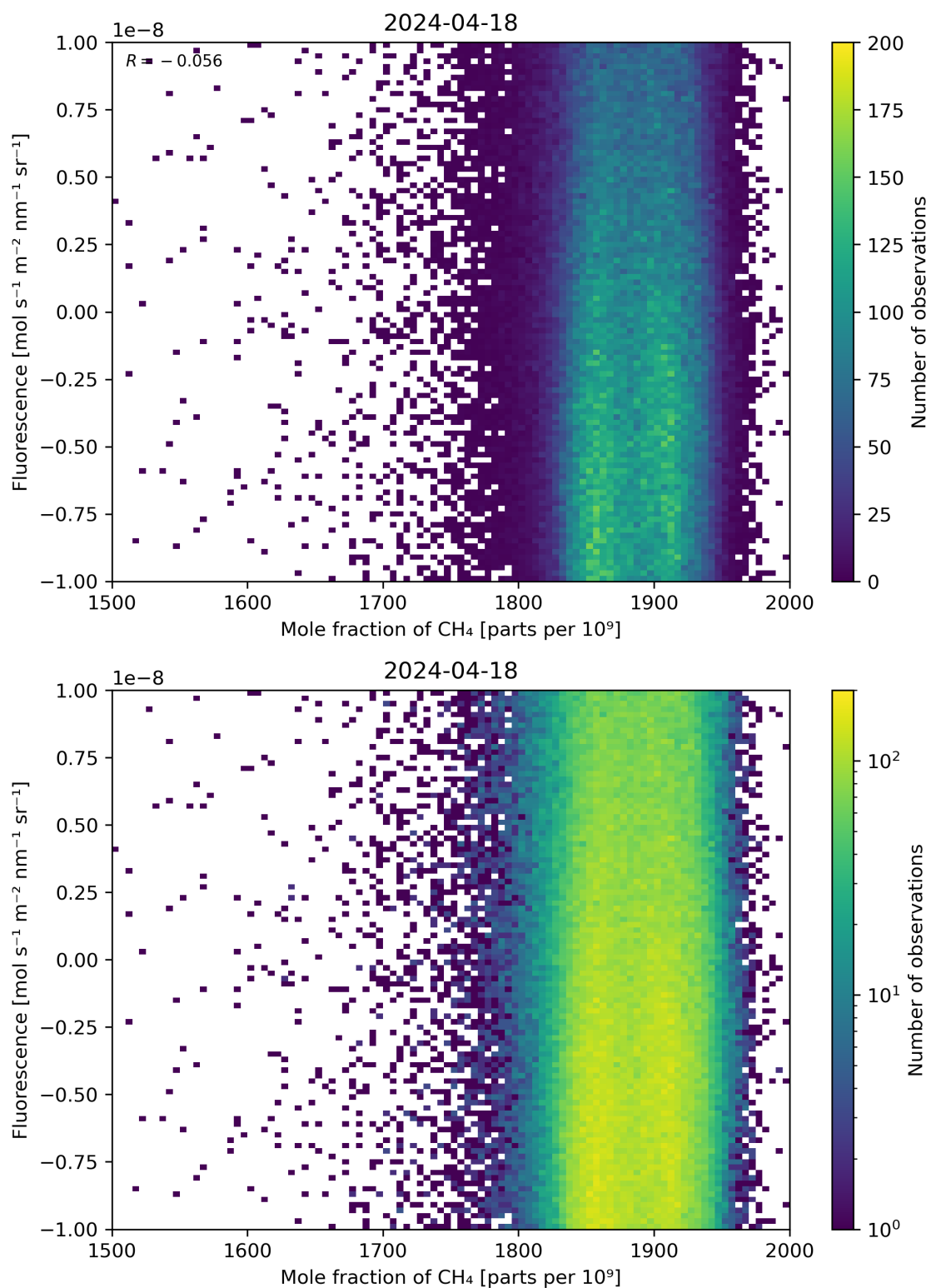
Figure 73: Scatter density plot of “Mole fraction of \text{CH}_4 ” against “Fluorescence” for 2024-04-17 to 2024-04-19.
