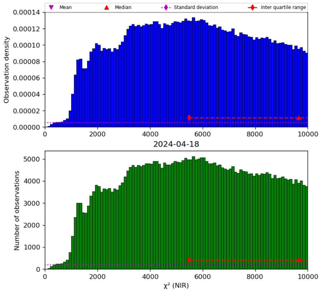
Figure 29: Histogram of “ \chi^2 (NIR)” for 2024-04-17 to 2024-04-19
