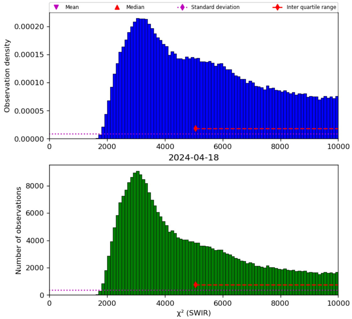
Figure 28: Histogram of “ \chi^2 (SWIR)” for 2024-04-17 to 2024-04-19
