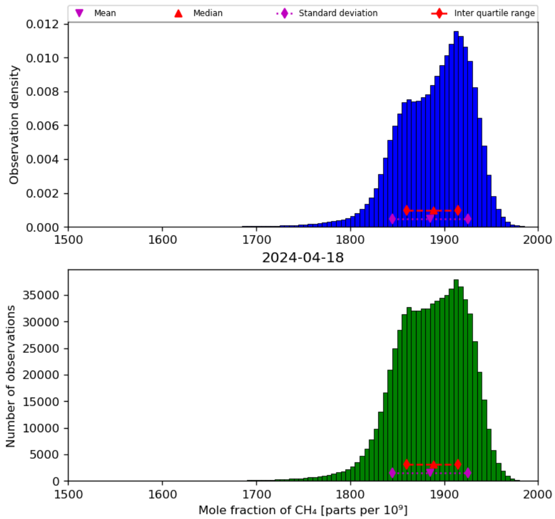
Figure 23: Histogram of “Mole fraction of CH 4 ” for 2024-04-17 to 2024-04-19
