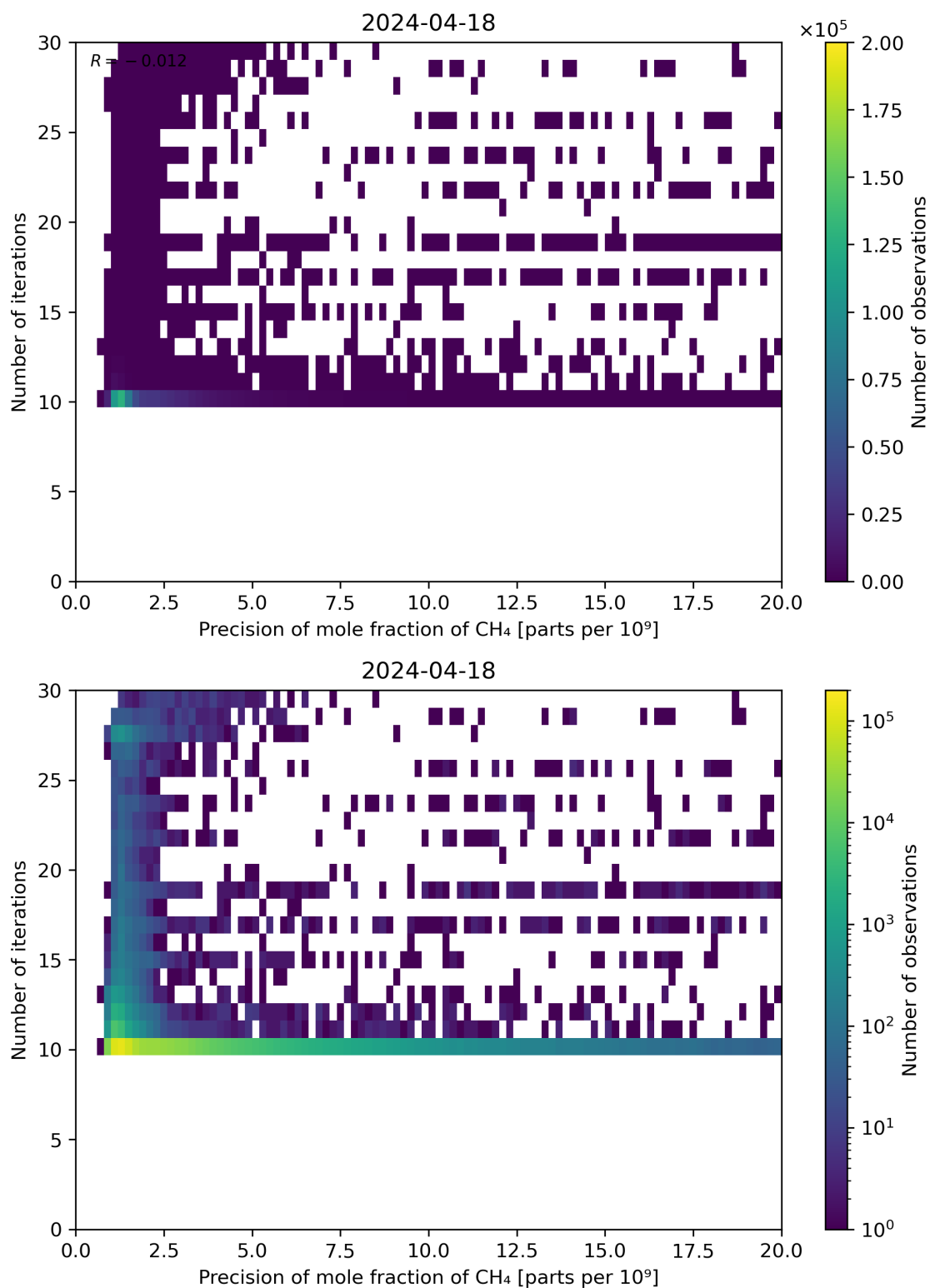
Figure 83: Scatter density plot of “Precision of mole fraction of CH 4 ” against “Number of iterations” for 2024-04-17 to 2024-04-19.
