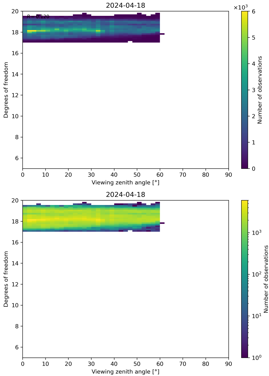
Figure 107: Scatter density plot of “Viewing zenith angle” against “Degrees of freedom” for 2024-04-17 to 2024-04-19.
