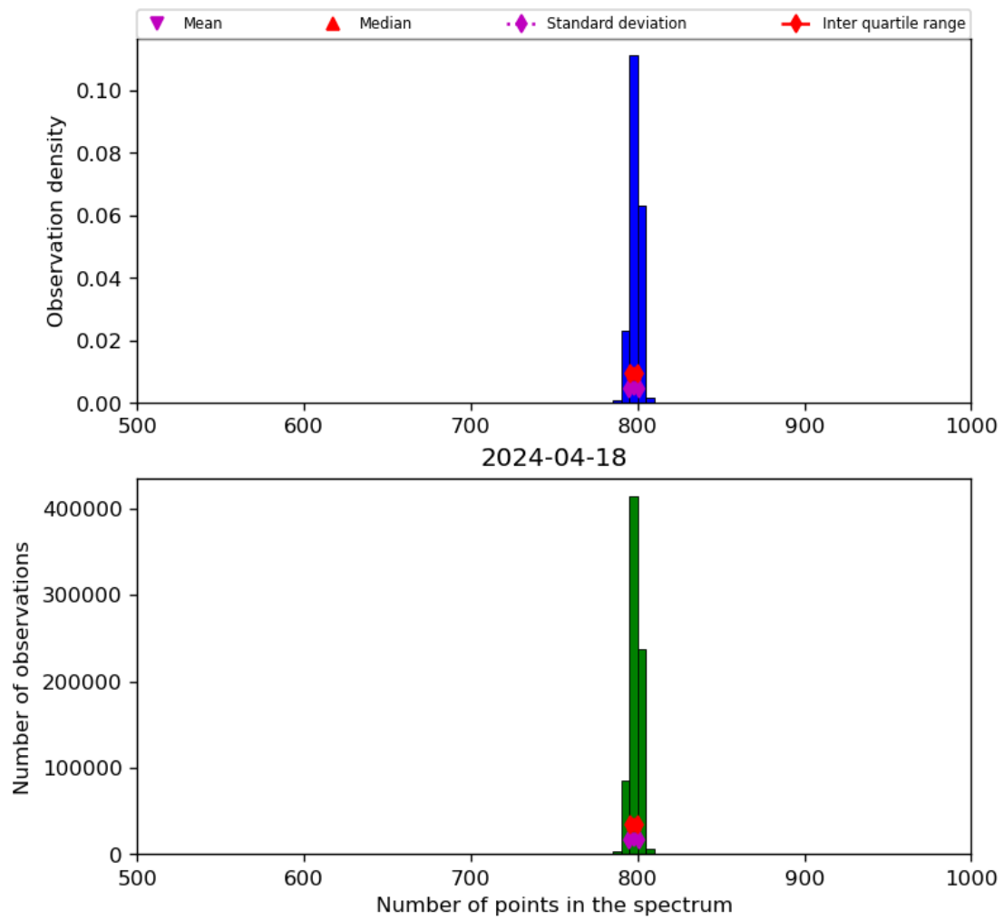
Figure 26: Histogram of “Number of points in the spectrum” for 2024-04-17 to 2024-04-19
