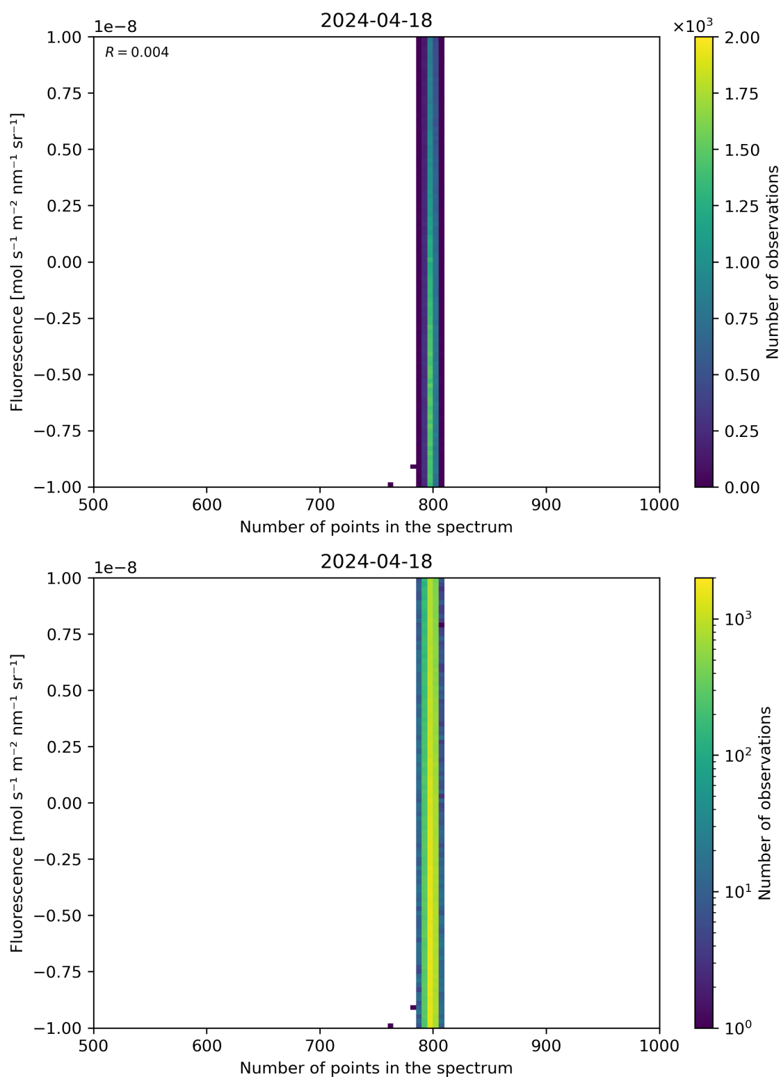
Figure 91: Scatter density plot of “Number of points in the spectrum” against “Fluorescence” for 2024-04-17 to 2024-04-19.
