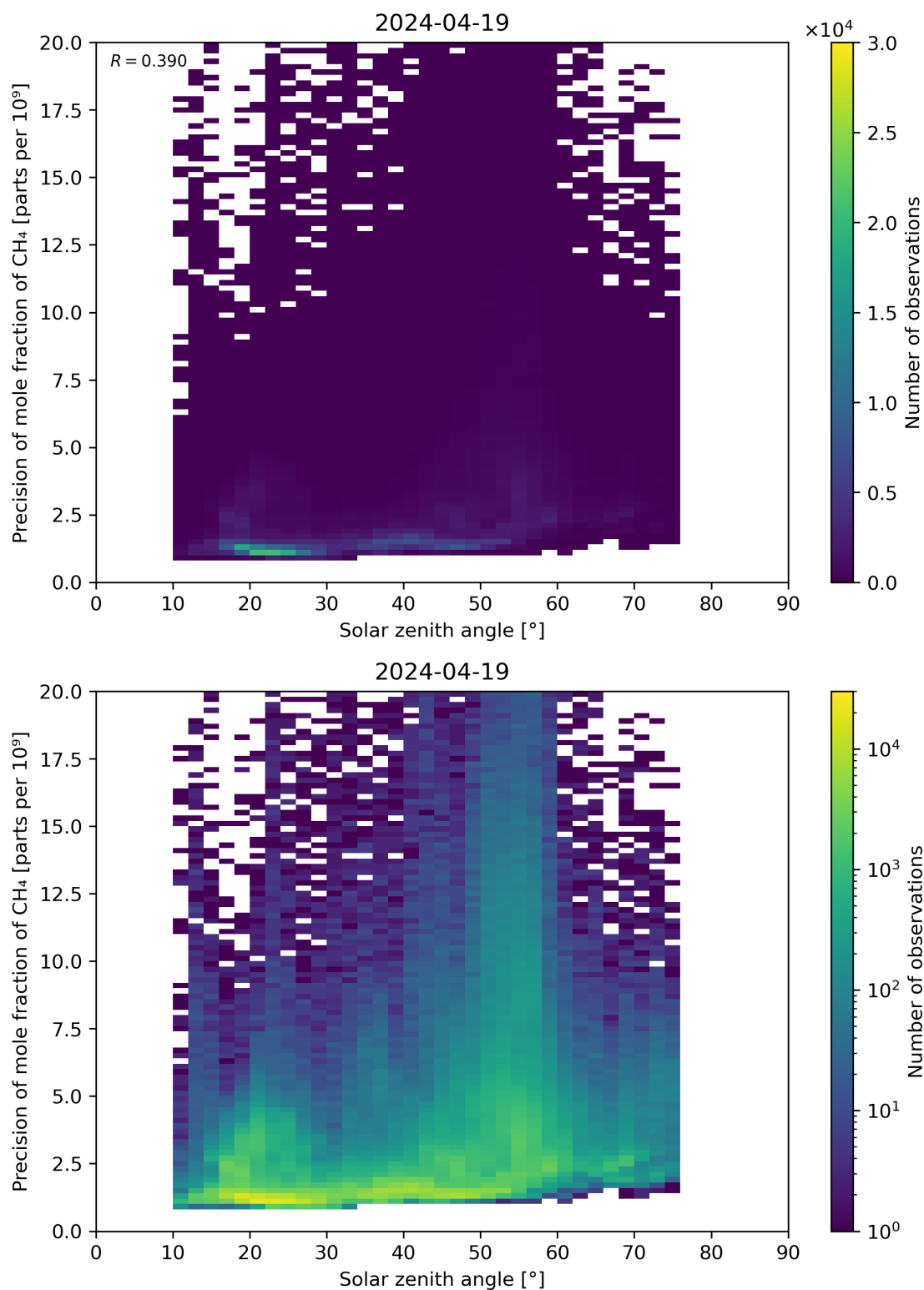
Figure 101: Scatter density plot of “Solar zenith angle” against “Precision of mole fraction of \text{CH}_4 ” for 2024-04-18 to 2024-04-20.
