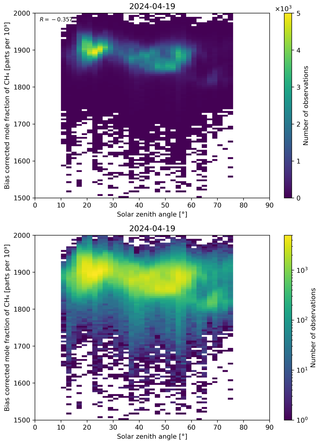
Figure 100: Scatter density plot of “Solar zenith angle” against “Bias corrected mole fraction of CH 4 ” for 2024-04-18 to 2024-04-20.
