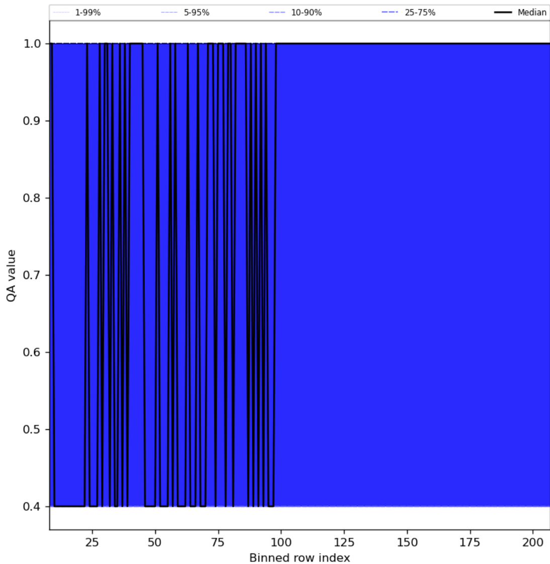
Figure 33: Along track statistics of “QA value” for 2024-04-18 to 2024-04-20
