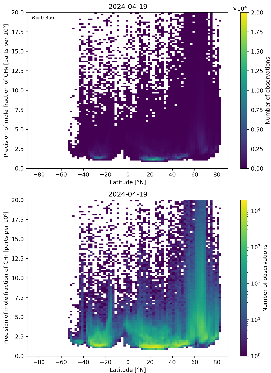
Figure 59: Scatter density plot of “Latitude” against “Precision of mole fraction of CH 4 ” for 2024-04-18 to 2024-04-20.
