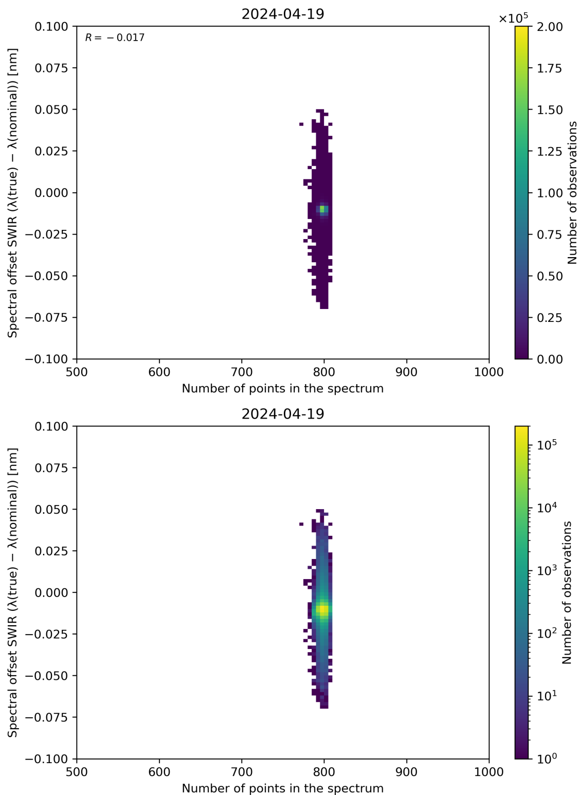
Figure 93: Scatter density plot of “Number of points in the spectrum” against “Spectral offset SWIR ( \lambda(\text{true}) - \lambda(\text{nominal}) )” for 2024-04-18 to 2024-04-20.
