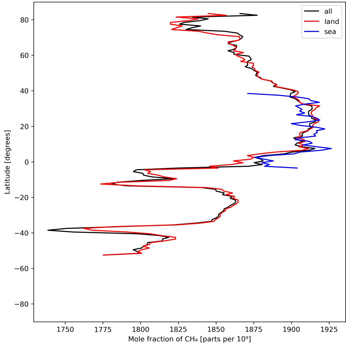
Figure 12: Zonal average of “Mole fraction of \text{CH}_4 ” for 2024-04-18 to 2024-04-20.
