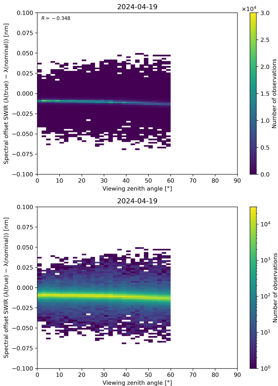
Figure 116: Scatter density plot of “Viewing zenith angle” against “Spectral offset SWIR ( \lambda(\text{true}) - \lambda(\text{nominal}) )” for 2024-04-18 to 2024-04-20.
