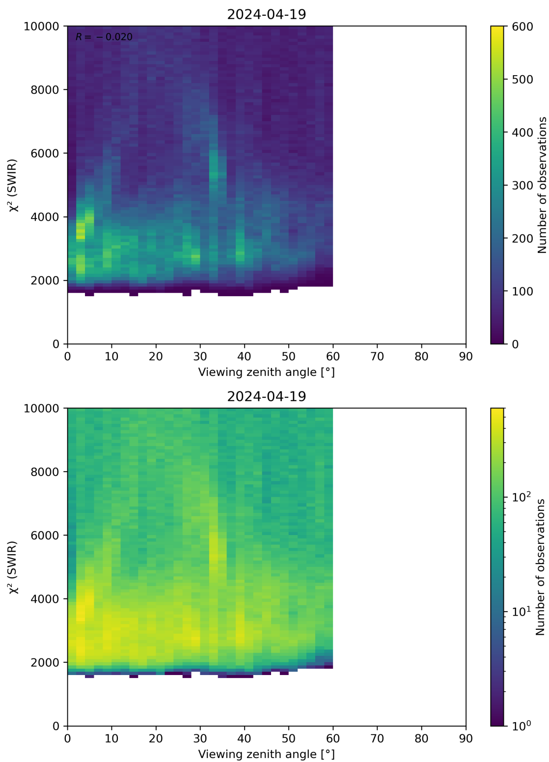
Figure 106: Scatter density plot of “Viewing zenith angle” against “ \chi^2 (SWIR)” for 2024-04-18 to 2024-04-20.
