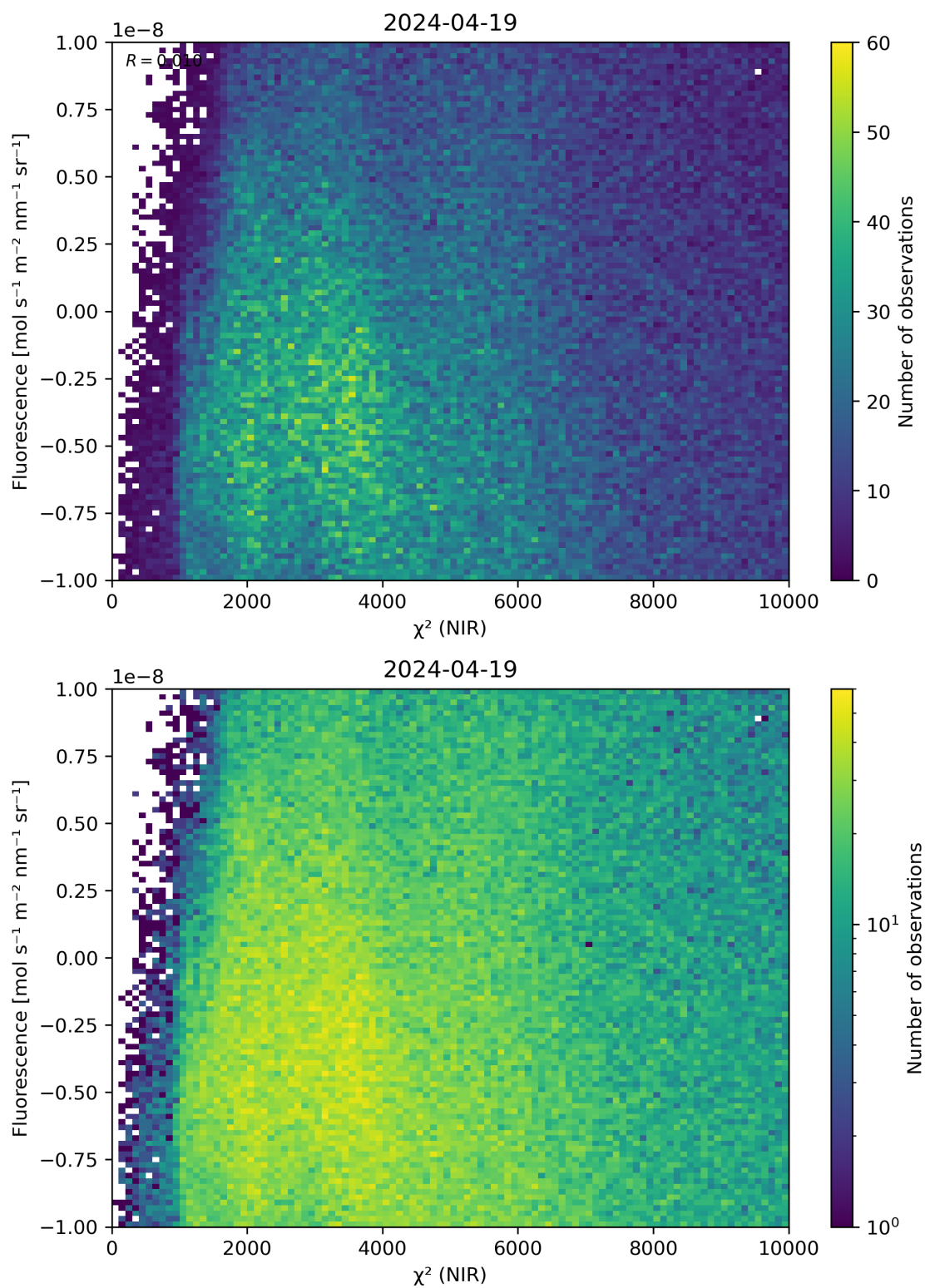
Figure 45: Scatter density plot of “ \chi^2 (NIR)” against “Fluorescence” for 2024-04-18 to 2024-04-20.
