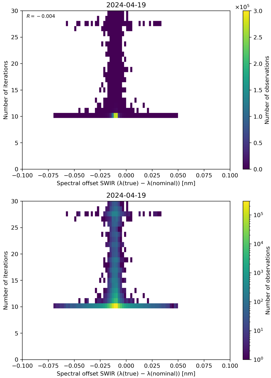
Figure 121: Scatter density plot of “Spectral offset SWIR ( \lambda(\text{true}) - \lambda(\text{nominal}) )” against “Number of iterations” for 2024-04-18 to 2024-04-20.
