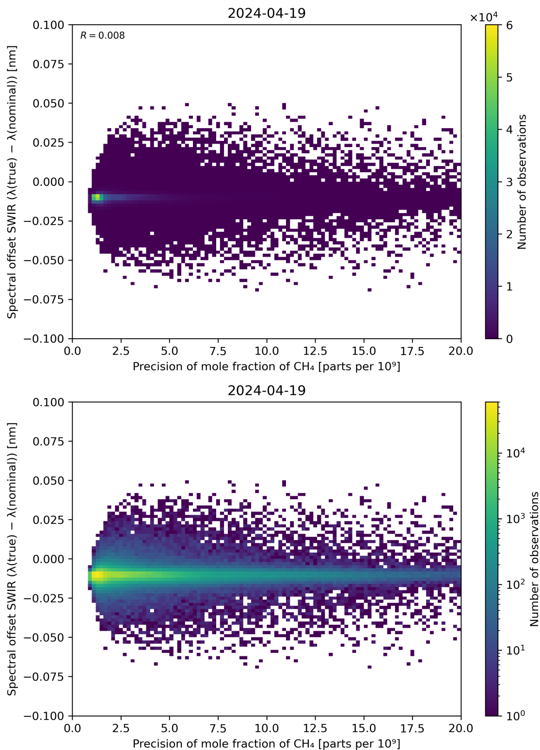
Figure 85: Scatter density plot of “Precision of mole fraction of \text{CH}_4 ” against “Spectral offset SWIR ( \lambda(\text{true}) - \lambda(\text{nominal}) )” for 2024-04-18 to 2024-04-20.
