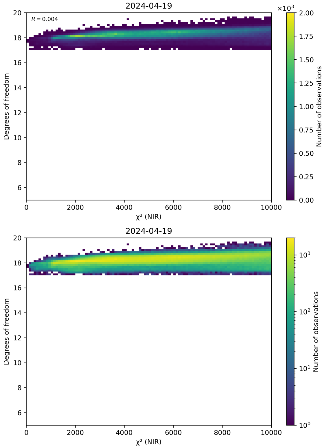
Figure 44: Scatter density plot of “ \chi^2 (NIR)” against “Degrees of freedom” for 2024-04-18 to 2024-04-20.
