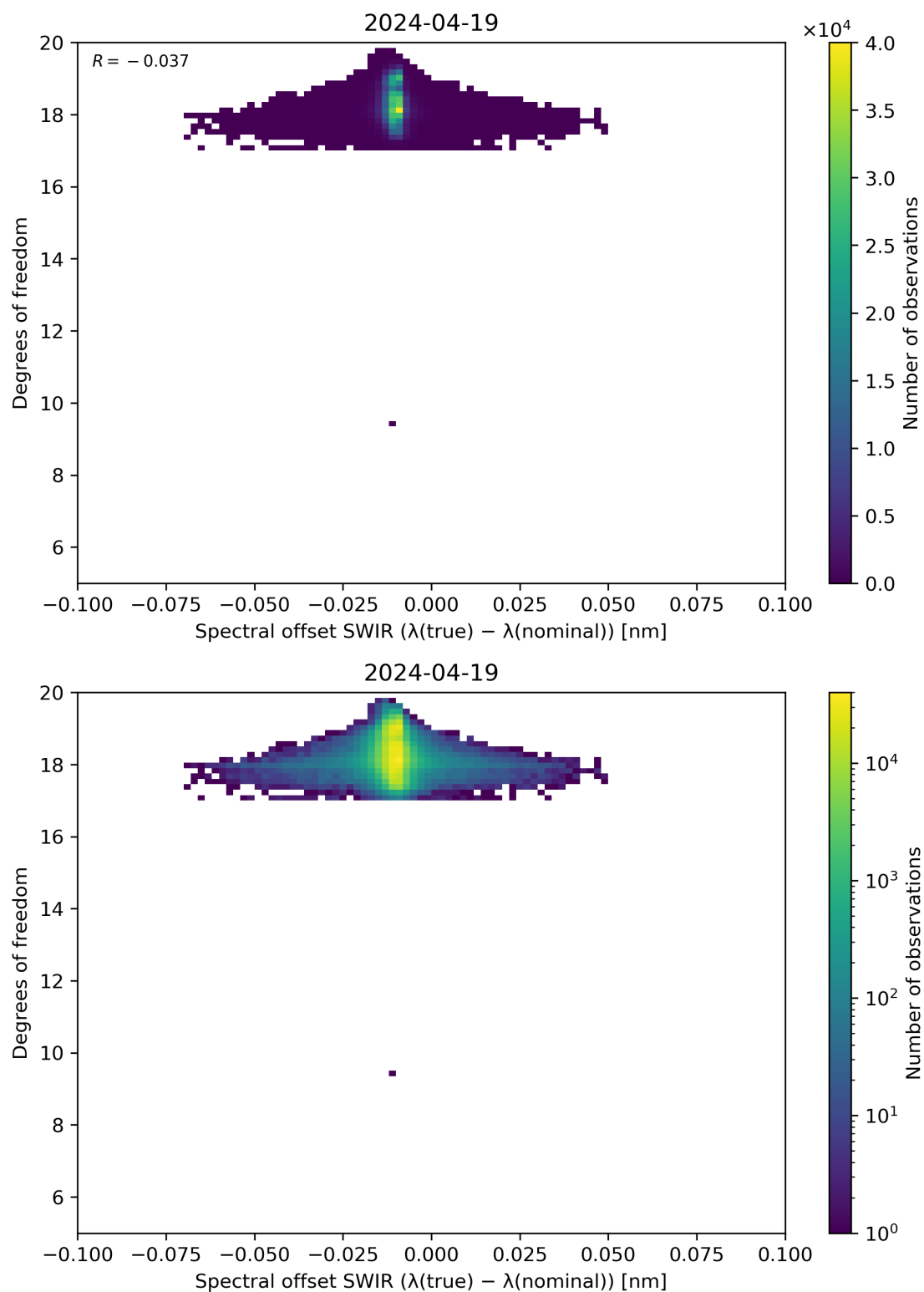
Figure 119: Scatter density plot of “Spectral offset SWIR ( \lambda(\text{true}) - \lambda(\text{nominal}) )” against “Degrees of freedom” for 2024-04-18 to 2024-04-20.
