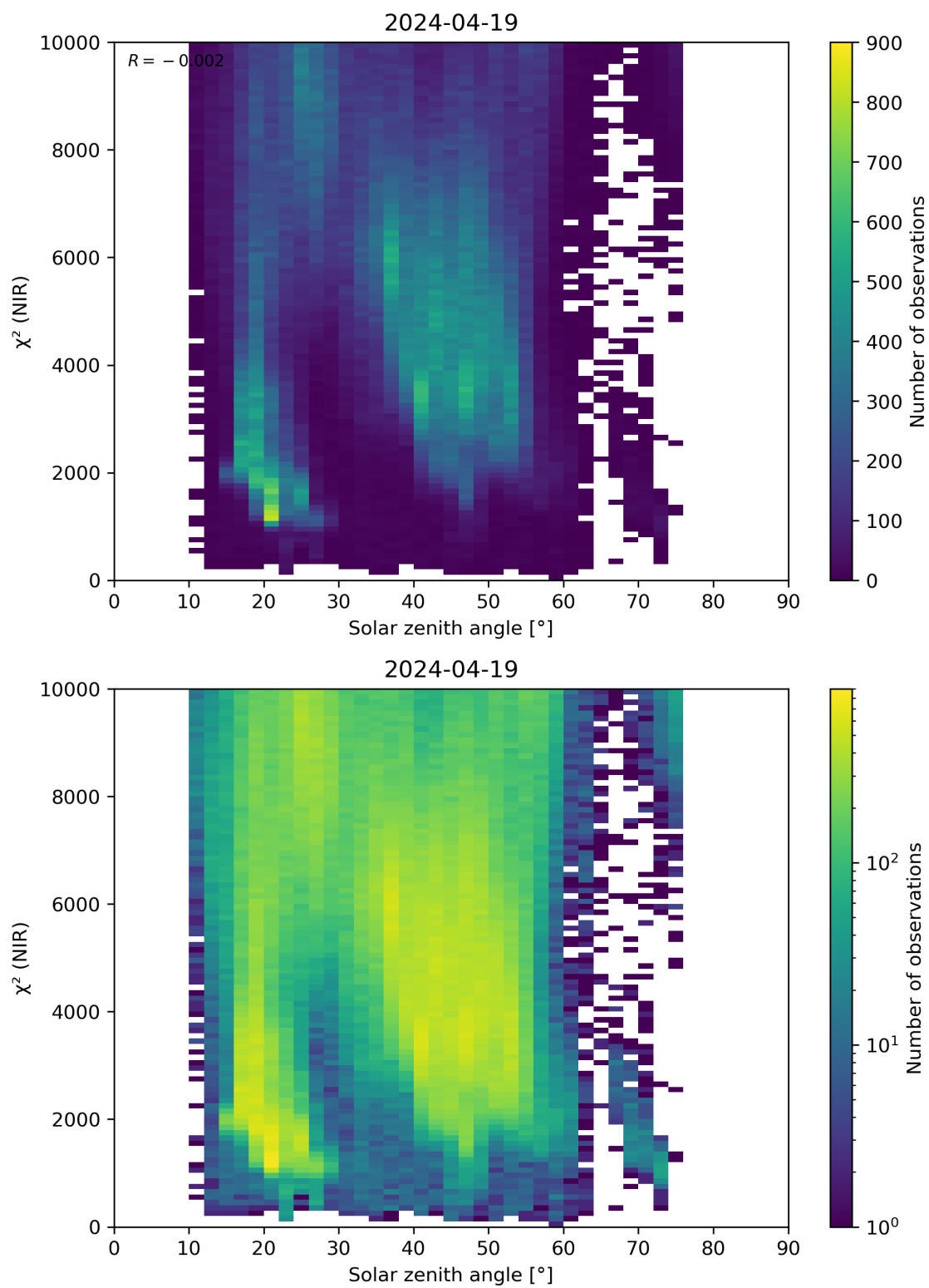
Figure 94: Scatter density plot of “Solar zenith angle” against “ \chi^2 (NIR)” for 2024-04-18 to 2024-04-20.
