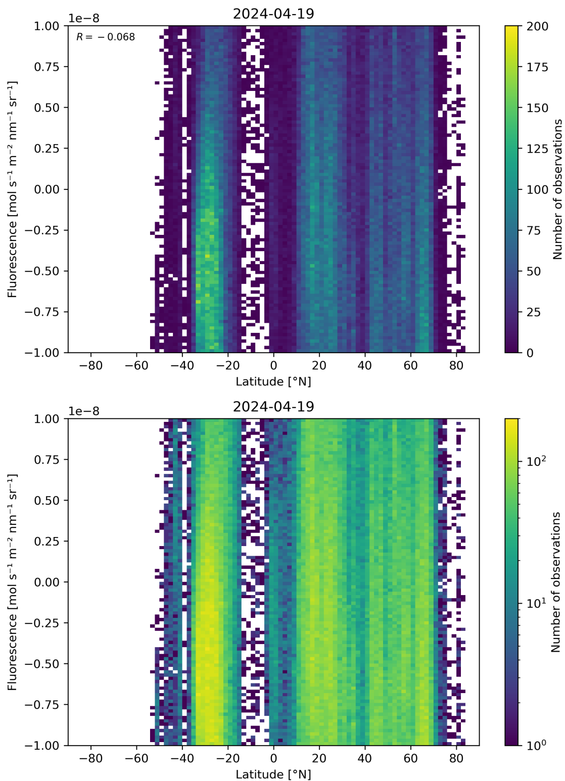
Figure 56: Scatter density plot of “Latitude” against “Fluorescence” for 2024-04-18 to 2024-04-20.
