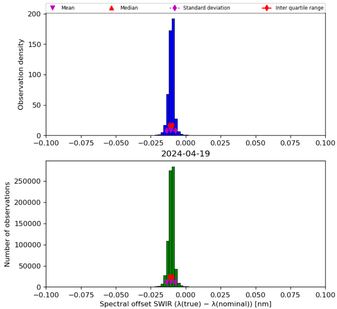
Figure 27: Histogram of “Spectral offset SWIR ( \lambda(\text{true}) - \lambda(\text{nominal}) )” for 2024-04-18 to 2024-04-20
