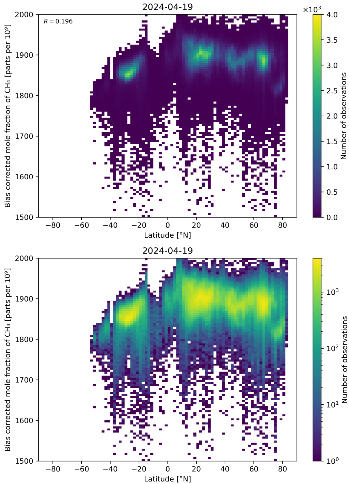
Figure 58: Scatter density plot of “Latitude” against “Bias corrected mole fraction of \text{CH}_4 ” for 2024-04-18 to 2024-04-20.
