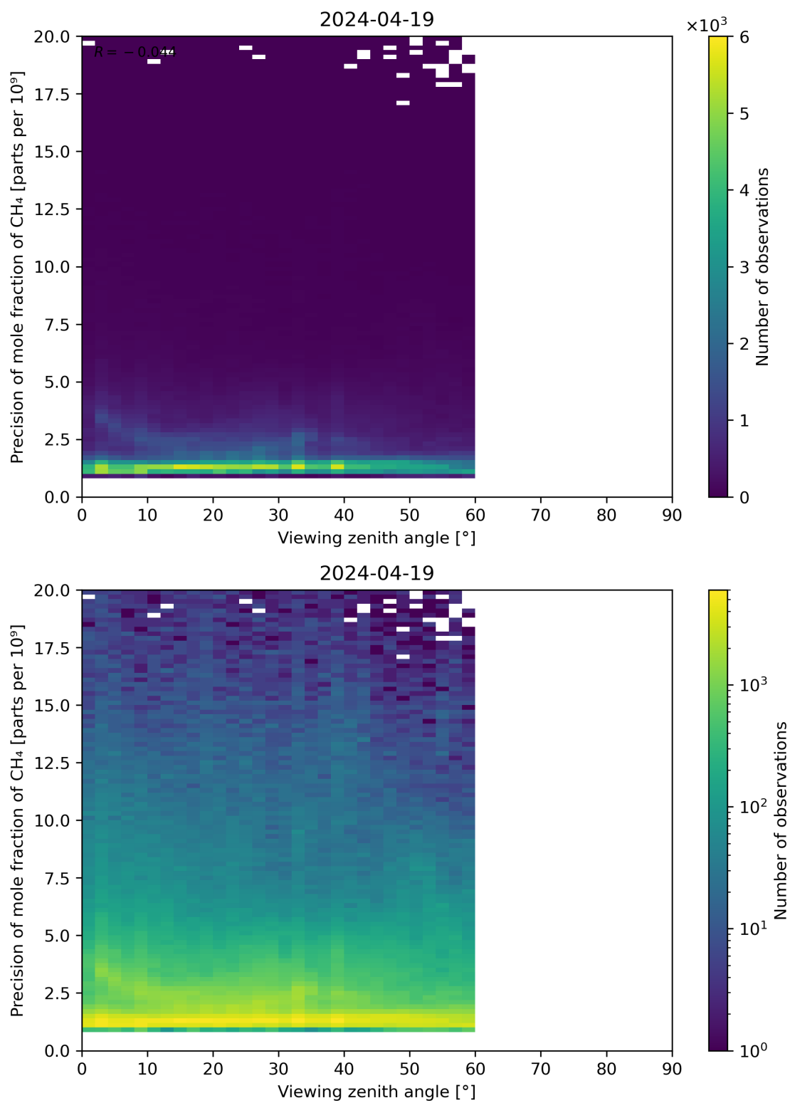
Figure 112: Scatter density plot of “Viewing zenith angle” against “Precision of mole fraction of CH 4 ” for 2024-04-18 to 2024-04-20.
