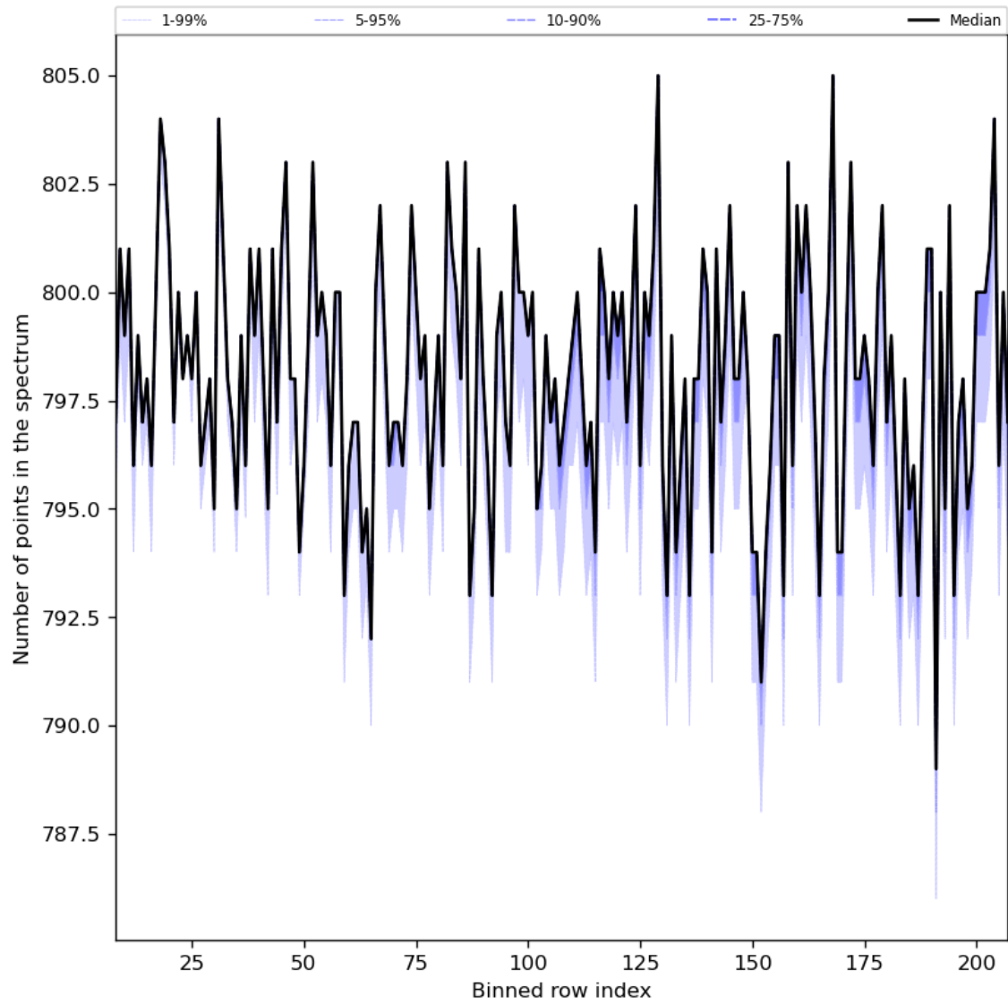
Figure 37: Along track statistics of “Number of points in the spectrum” for 2024-04-18 to 2024-04-20
