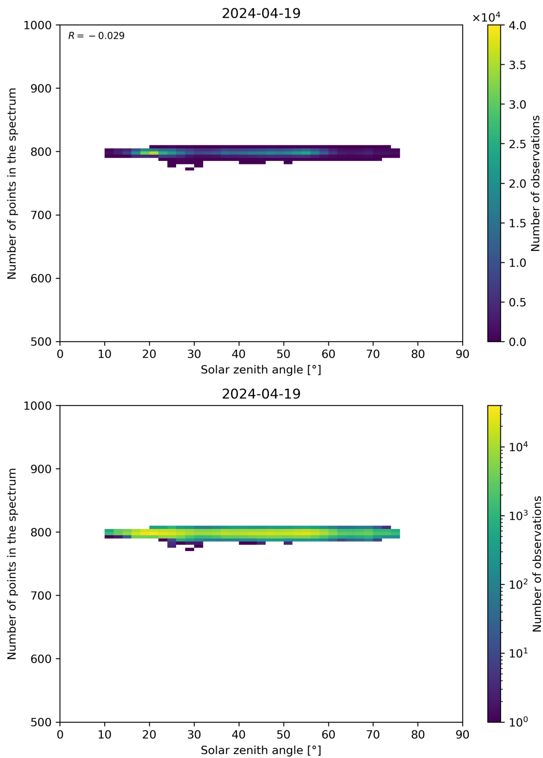
Figure 103: Scatter density plot of “Solar zenith angle” against “Number of points in the spectrum” for 2024-04-18 to 2024-04-20.
