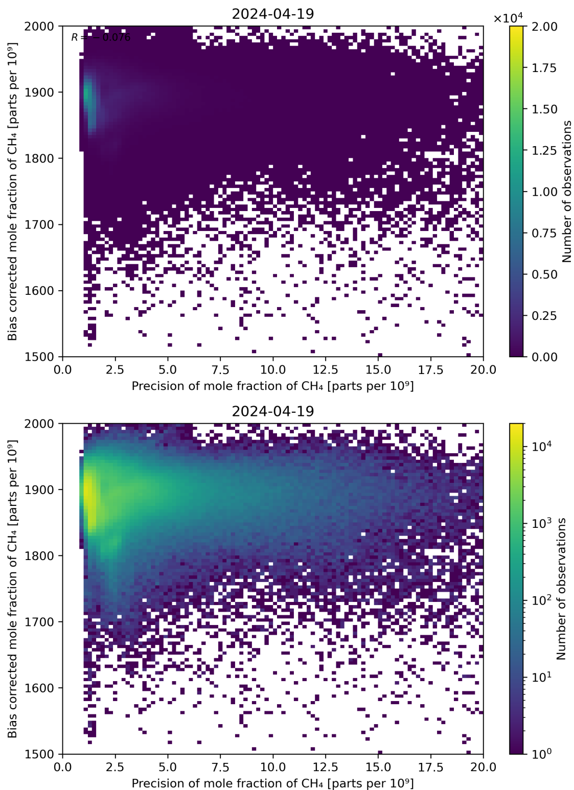
Figure 82: Scatter density plot of “Precision of mole fraction of CH 4 ” against “Bias corrected mole fraction of CH 4 ” for 2024-04-18 to 2024-04-20.
