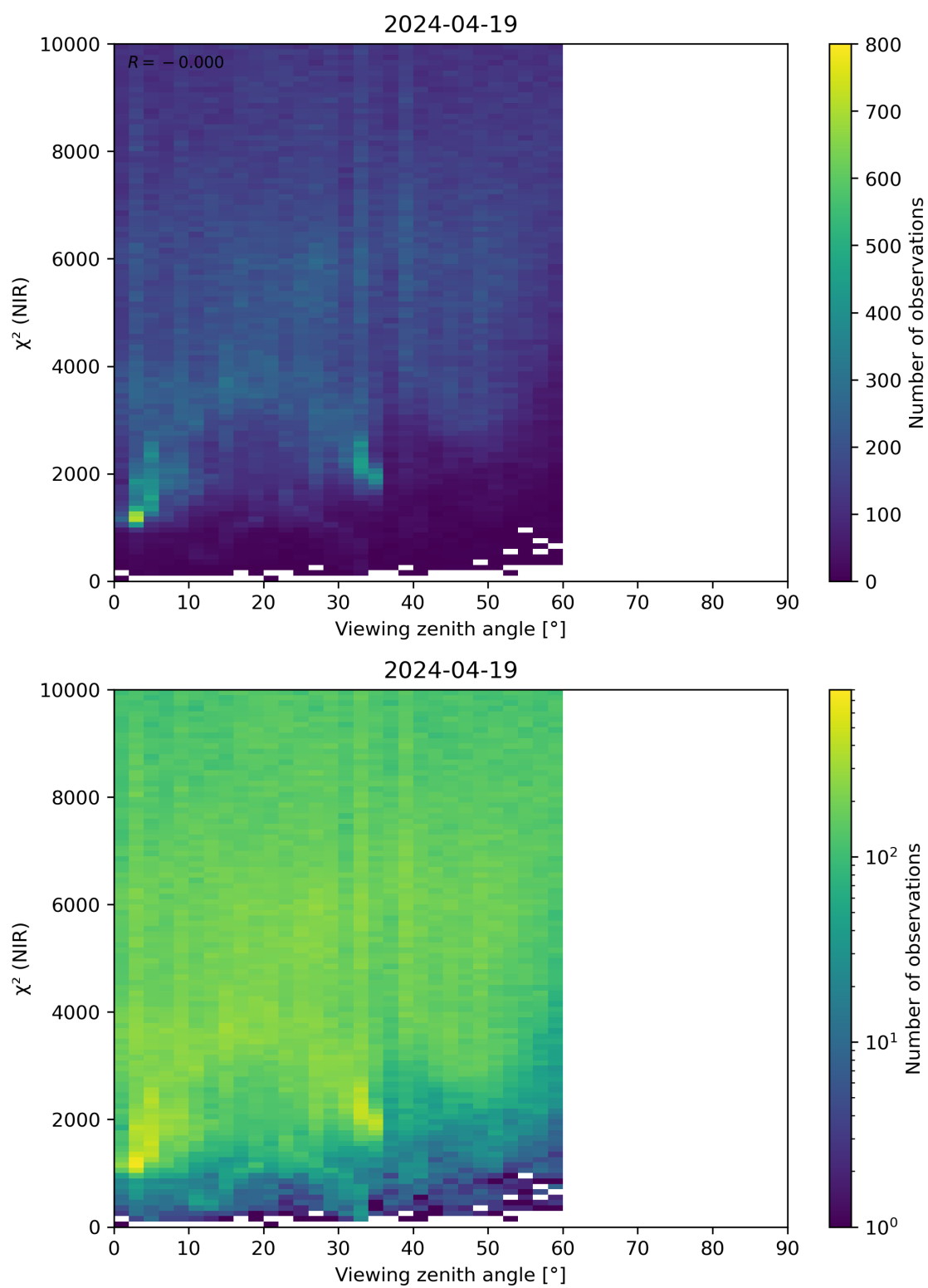
Figure 105: Scatter density plot of “Viewing zenith angle” against “ \chi^2 (NIR)” for 2024-04-18 to 2024-04-20.
