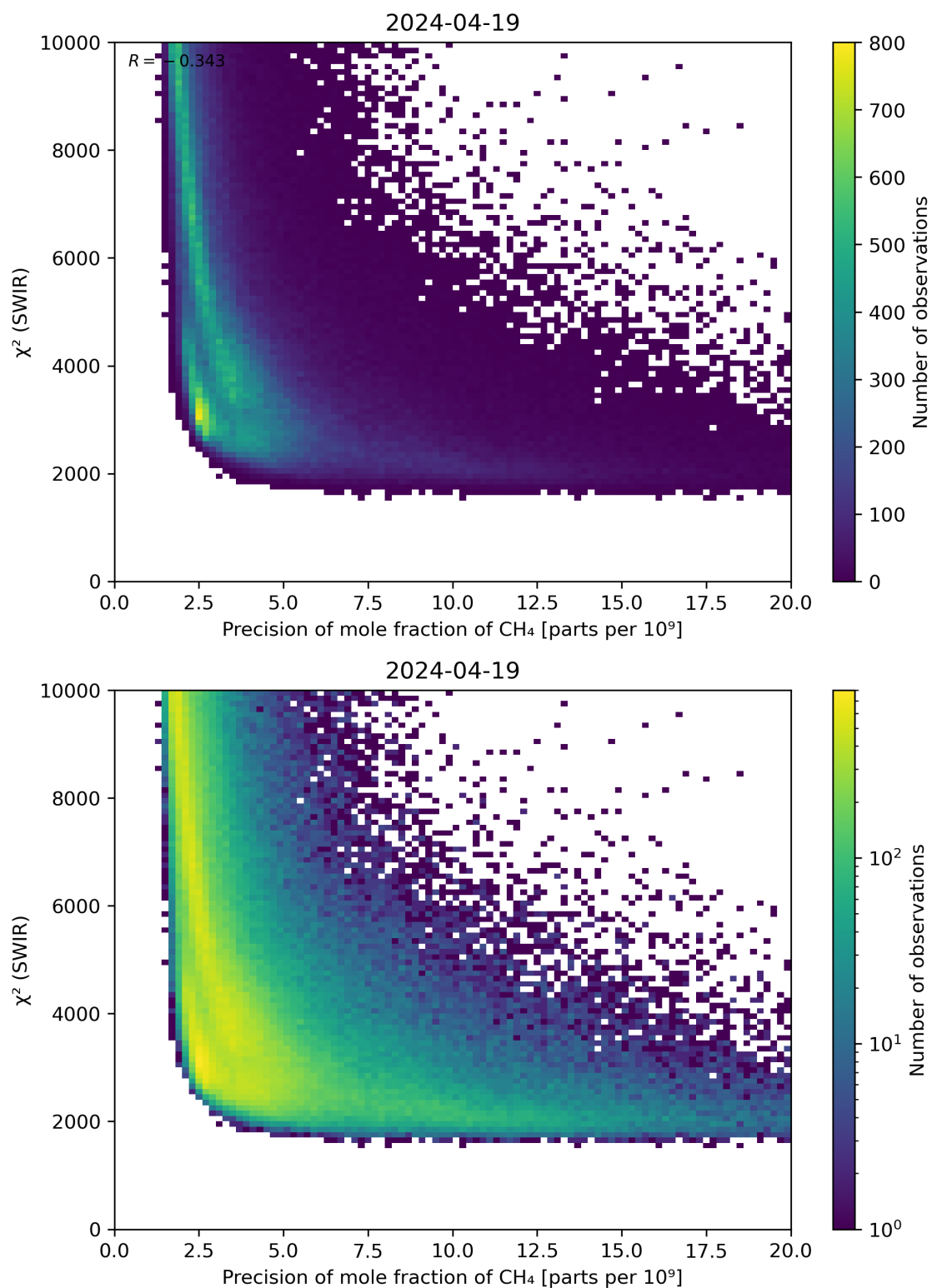
Figure 79: Scatter density plot of “Precision of mole fraction of \text{CH}_4 ” against “ \chi^2 (SWIR)” for 2024-04-18 to 2024-04-20.
