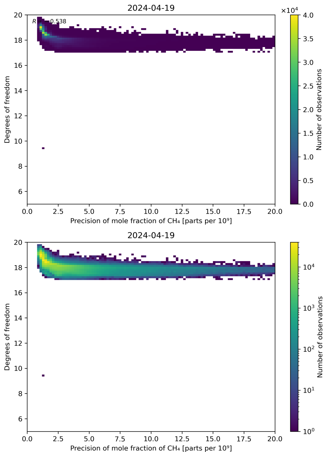
Figure 80: Scatter density plot of “Precision of mole fraction of CH 4 ” against “Degrees of freedom” for 2024-04-18 to 2024-04-20.
