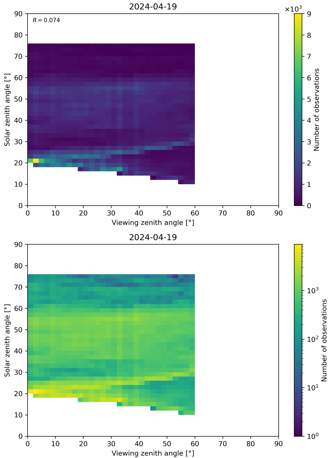
Figure 115: Scatter density plot of “Viewing zenith angle” against “Solar zenith angle” for 2024-04-18 to 2024-04-20.
