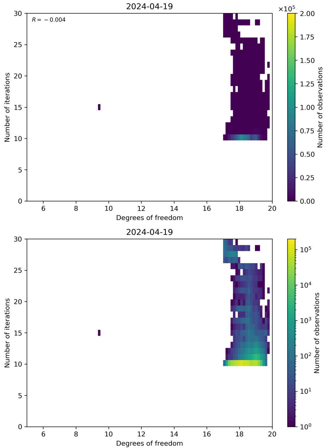
Figure 52: Scatter density plot of “Degrees of freedom” against “Number of iterations” for 2024-04-18 to 2024-04-20.
