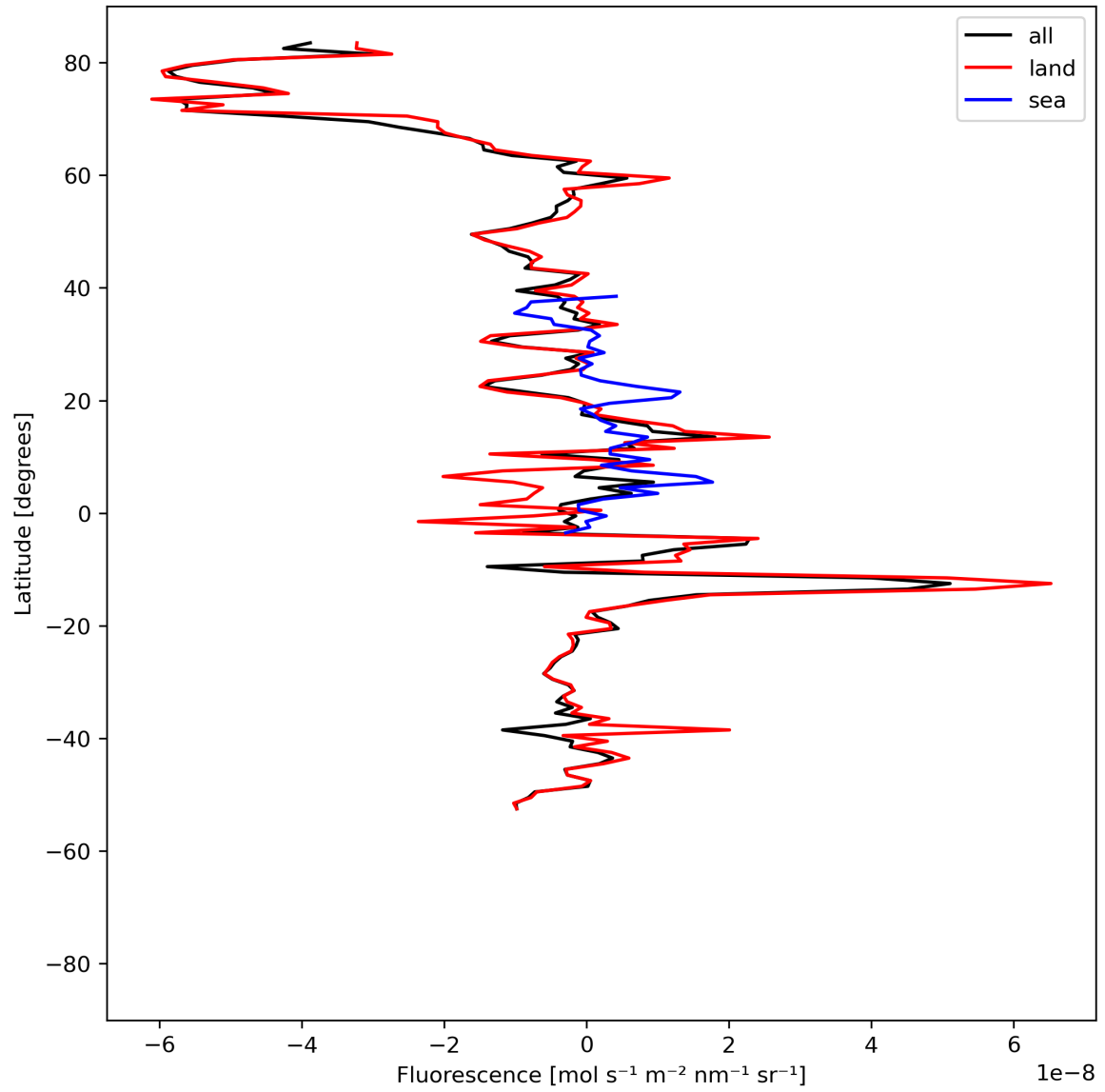
Figure 21: Zonal average of “Fluorescence” for 2024-04-18 to 2024-04-20.
