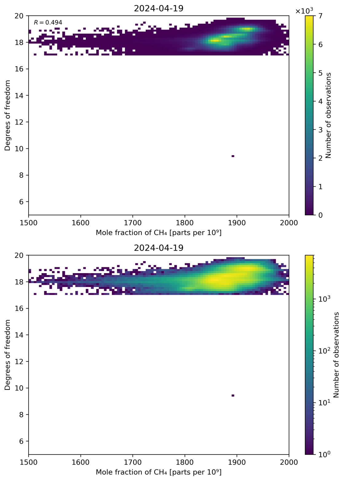
Figure 72: Scatter density plot of “Mole fraction of CH 4 ” against “Degrees of freedom” for 2024-04-18 to 2024-04-20.
