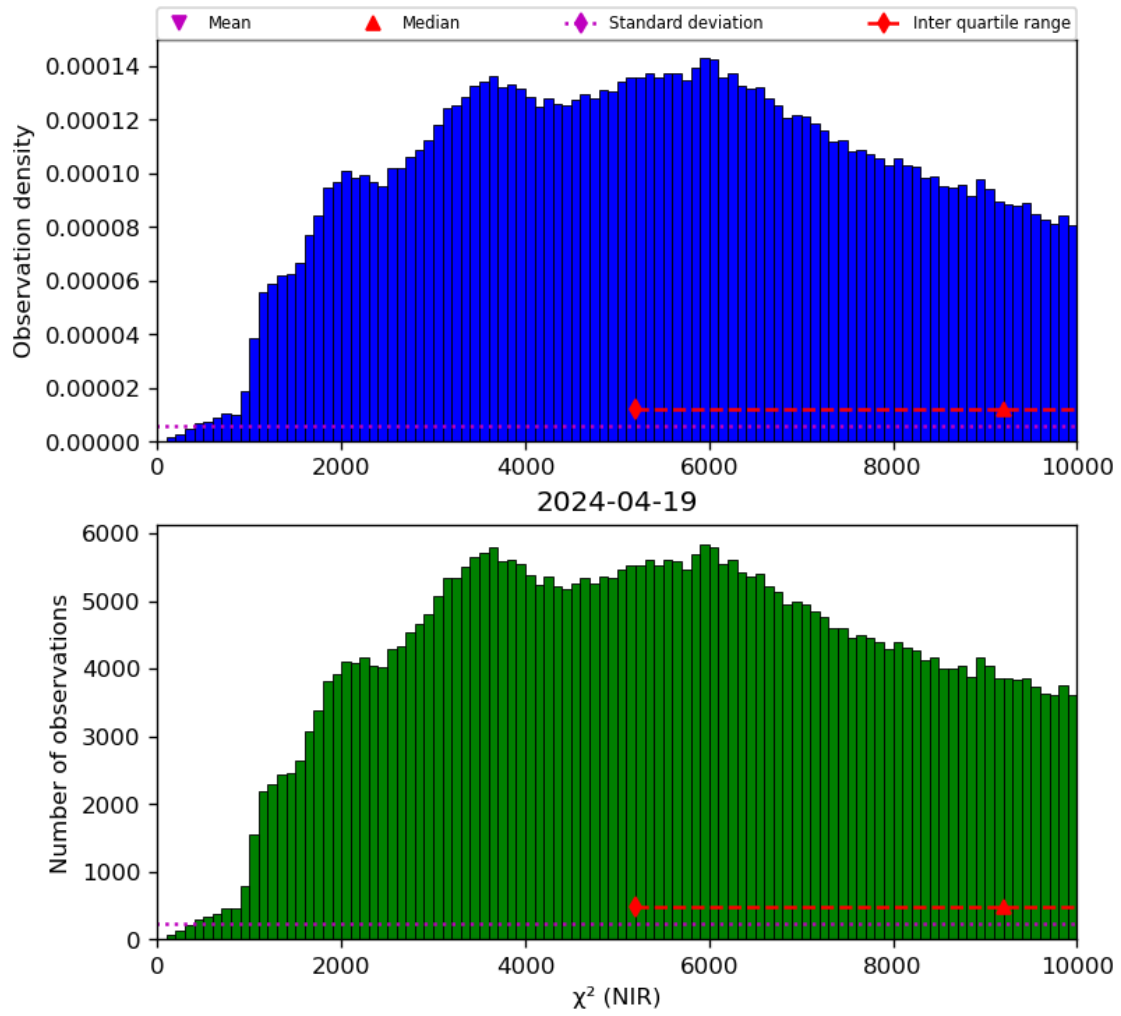
Figure 29: Histogram of “ \chi^2 (NIR)” for 2024-04-18 to 2024-04-20
