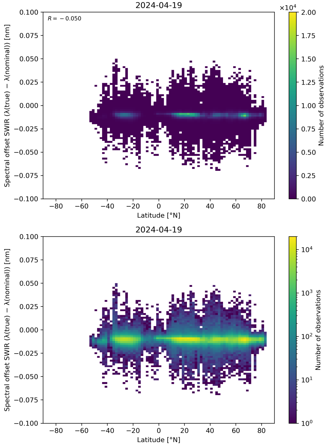
Figure 62: Scatter density plot of “Latitude” against “Spectral offset SWIR ( \lambda(\text{true}) - \lambda(\text{nominal}) )” for 2024-04-18 to 2024-04-20.
