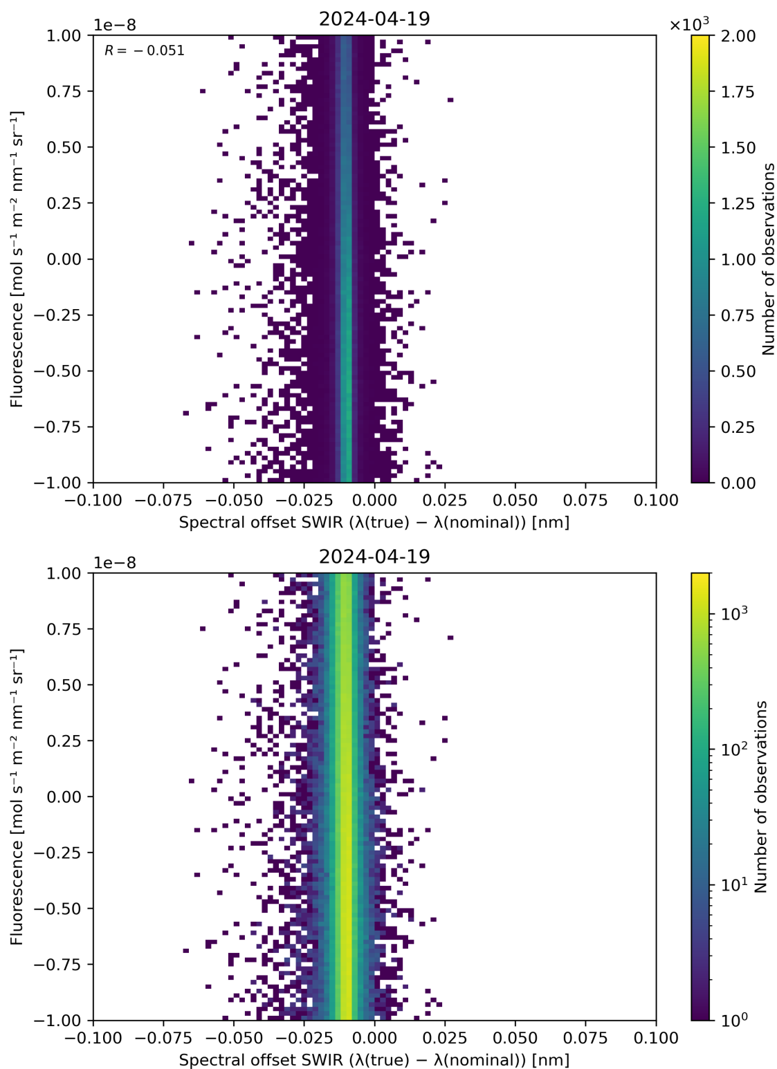
Figure 120: Scatter density plot of “Spectral offset SWIR ( \lambda(\text{true}) - \lambda(\text{nominal}) )” against “Fluorescence” for 2024-04-18 to 2024-04-20.
