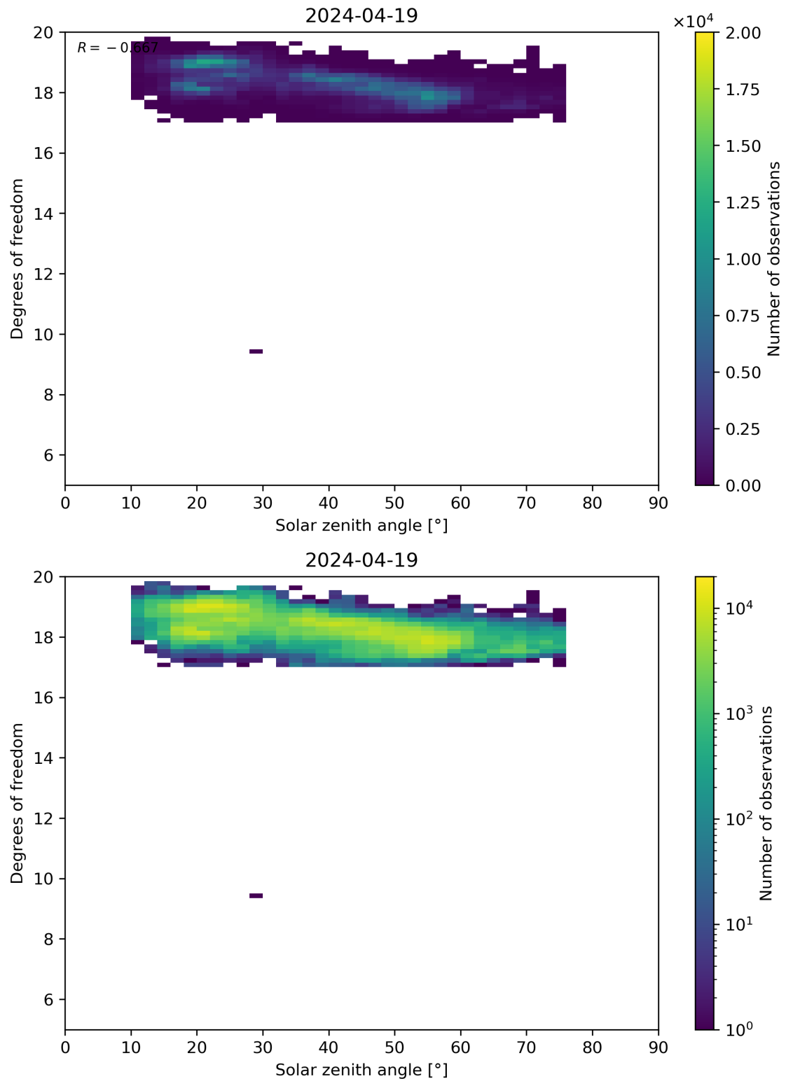
Figure 96: Scatter density plot of “Solar zenith angle” against “Degrees of freedom” for 2024-04-18 to 2024-04-20.
