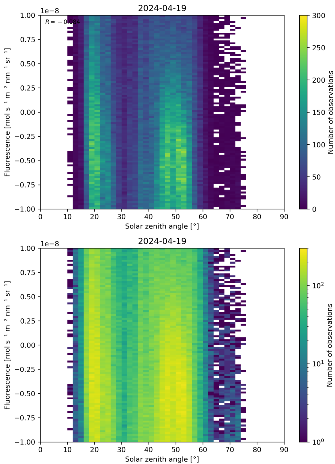
Figure 97: Scatter density plot of “Solar zenith angle” against “Fluorescence” for 2024-04-18 to 2024-04-20.
