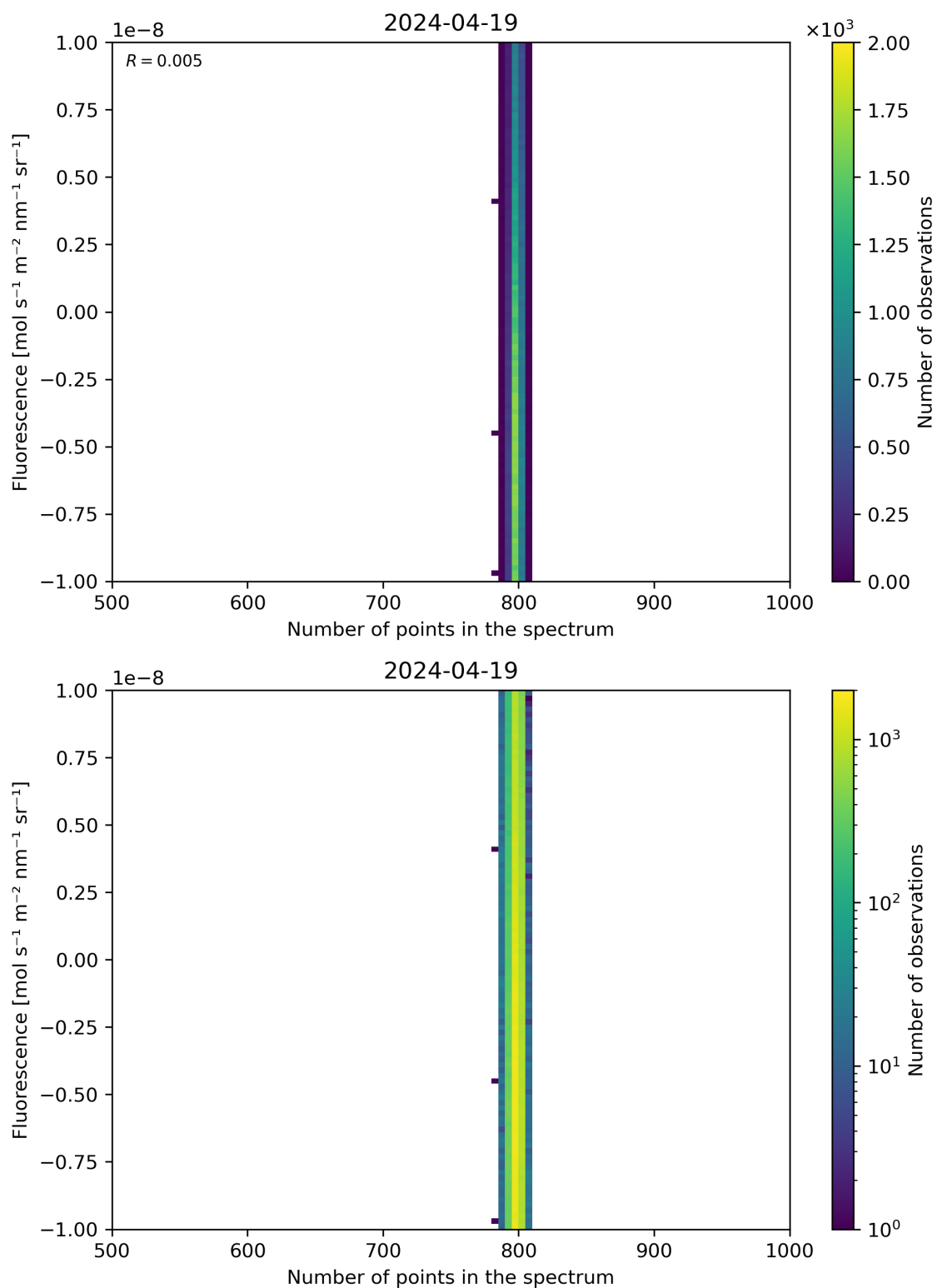
Figure 91: Scatter density plot of “Number of points in the spectrum” against “Fluorescence” for 2024-04-18 to 2024-04-20.
