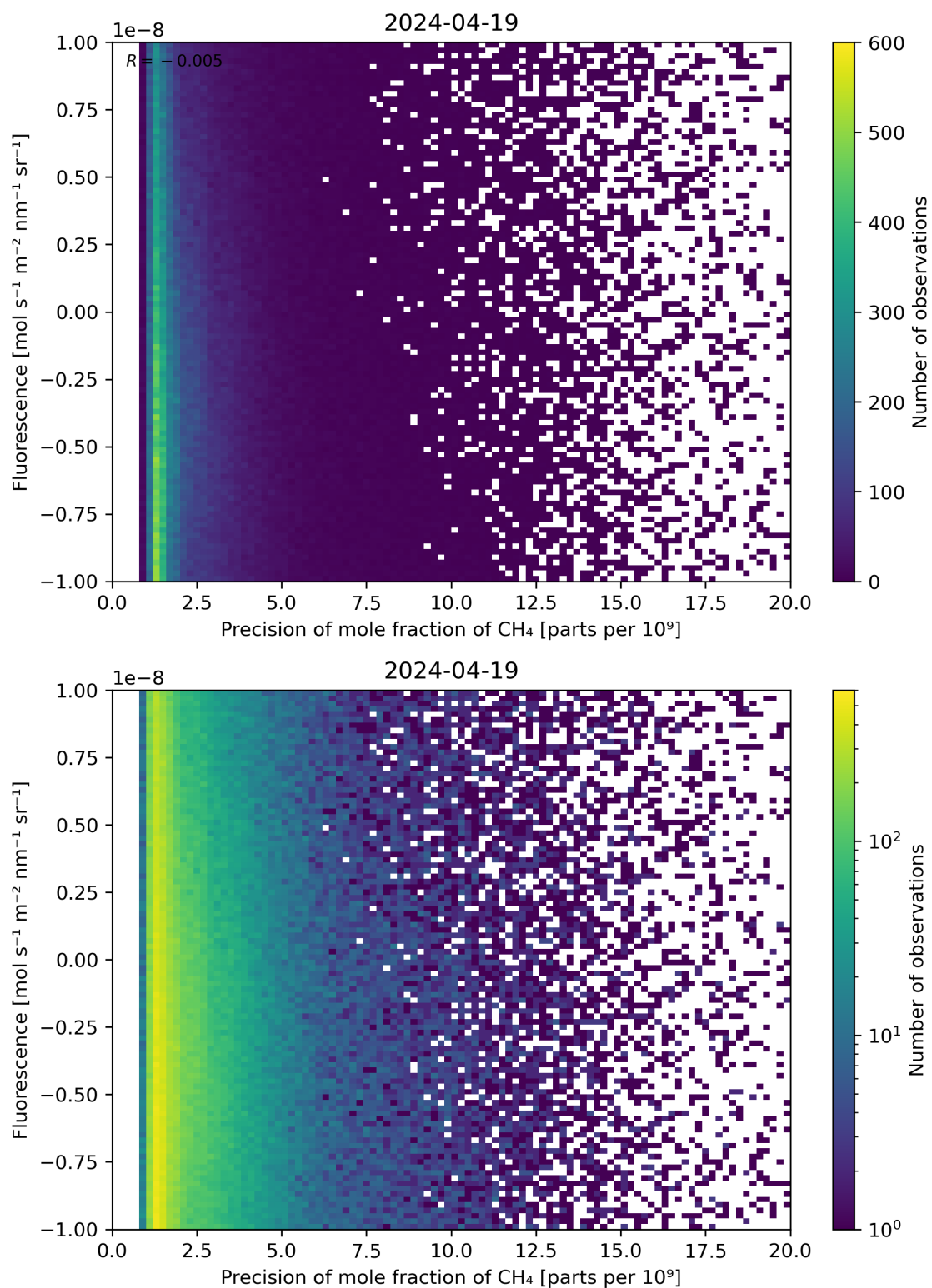
Figure 81: Scatter density plot of “Precision of mole fraction of CH 4 ” against “Fluorescence” for 2024-04-18 to 2024-04-20.
