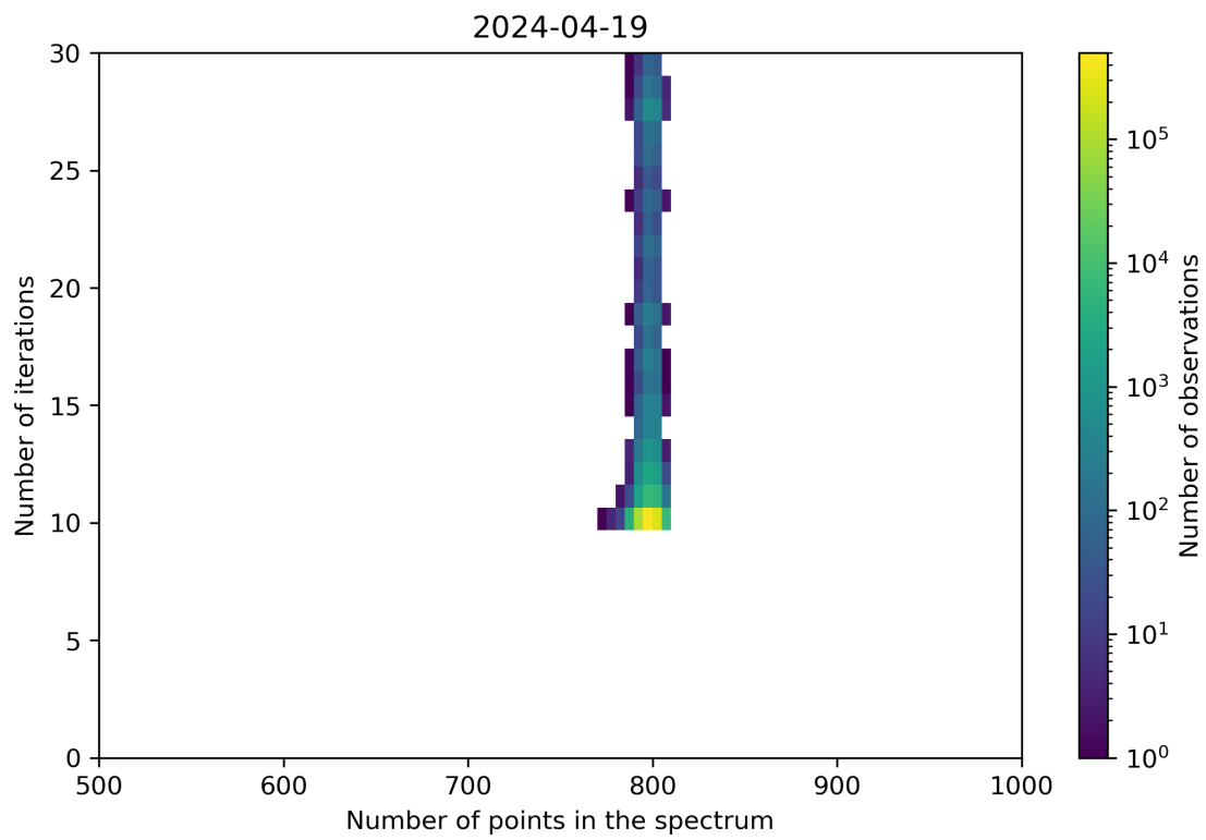
Figure 92: Scatter density plot of “Number of points in the spectrum” against “Number of iterations” for 2024-04-18 to 2024-04-20.
