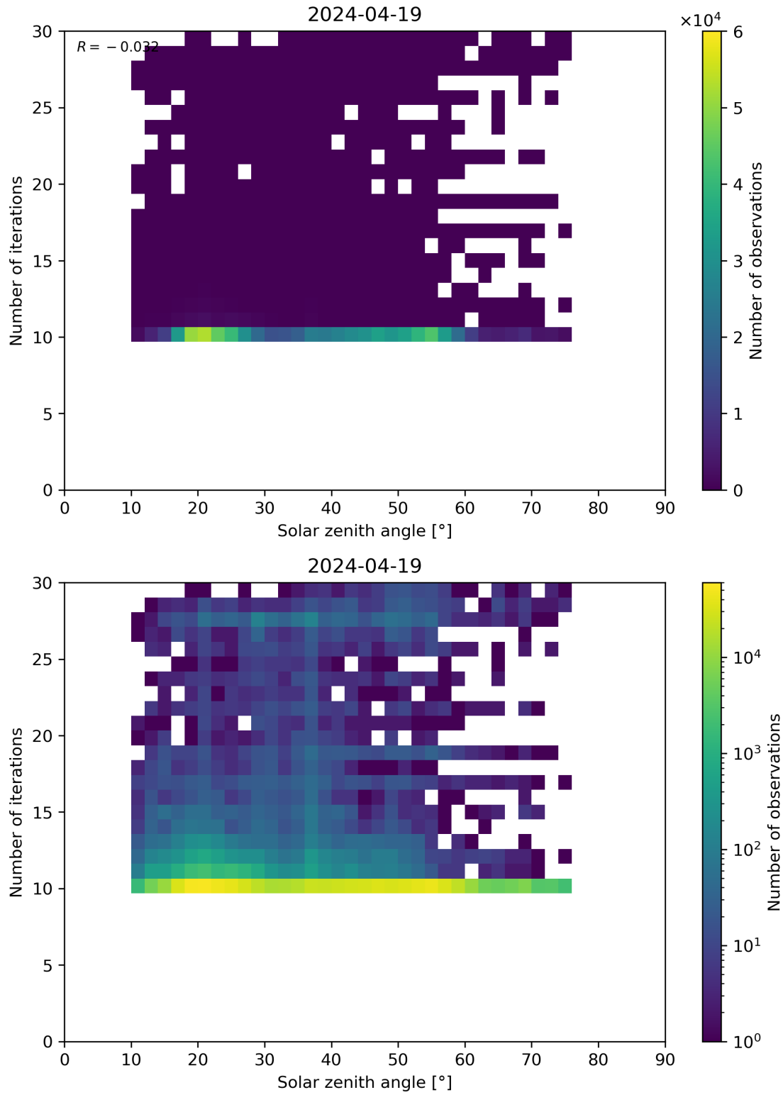
Figure 102: Scatter density plot of “Solar zenith angle” against “Number of iterations” for 2024-04-18 to 2024-04-20.
