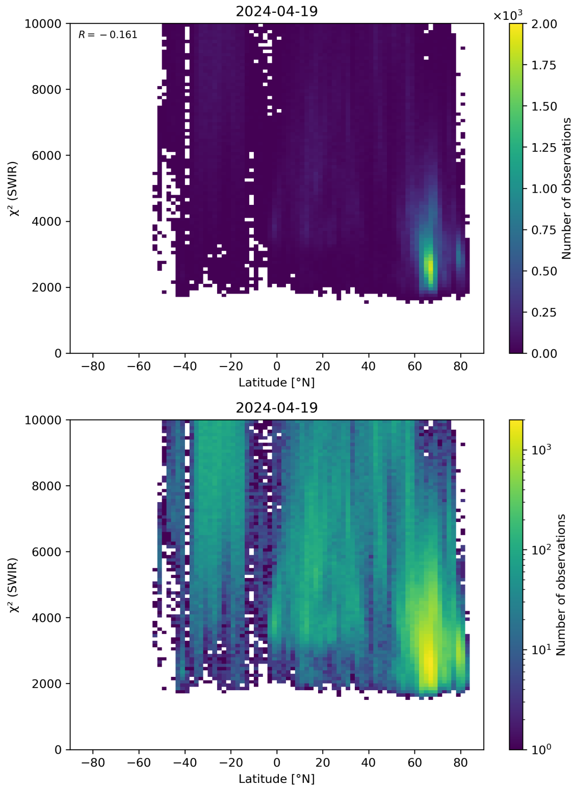
Figure 54: Scatter density plot of “Latitude” against “ \chi^2 (SWIR)” for 2024-04-18 to 2024-04-20.
