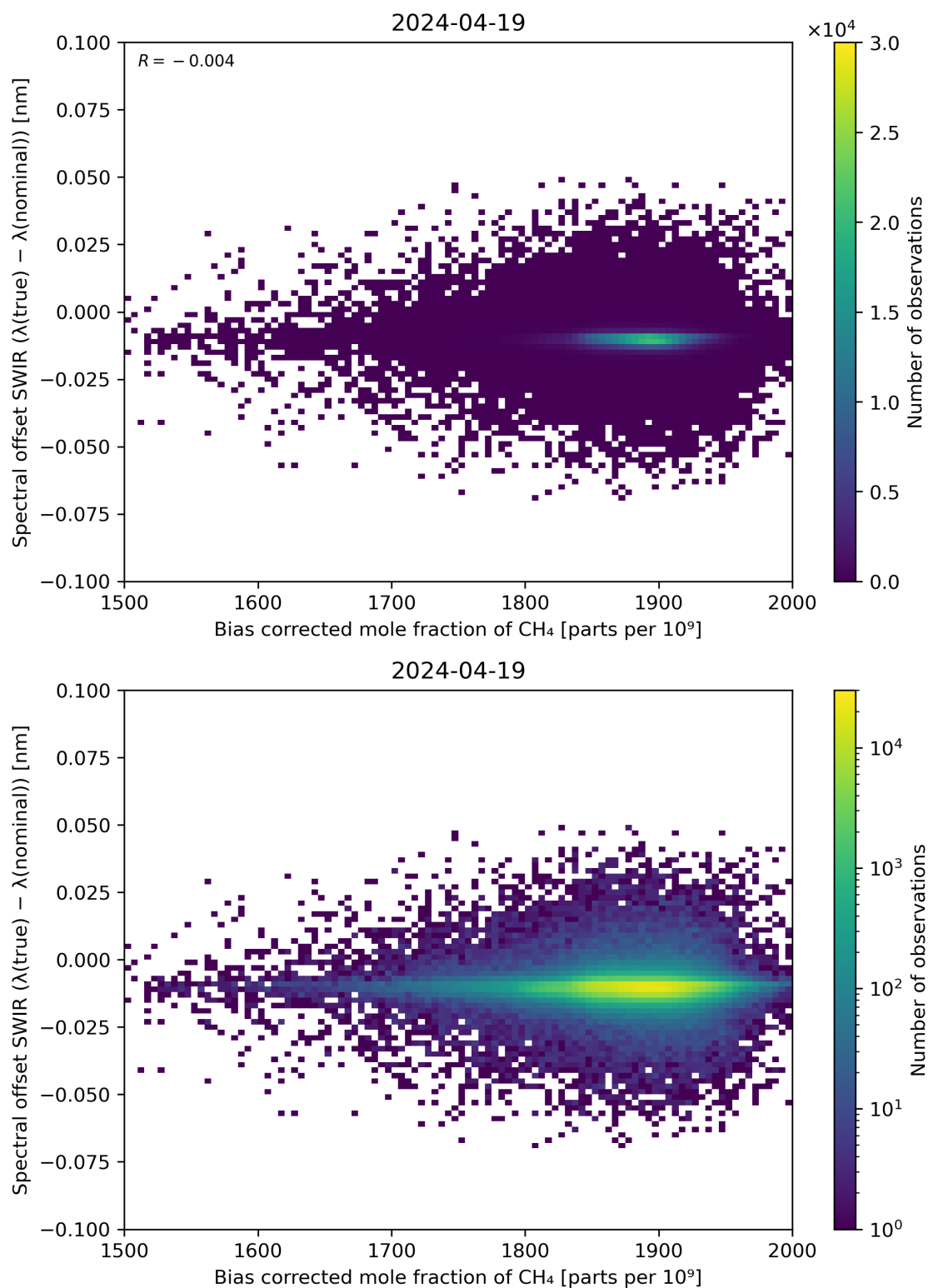
Figure 69: Scatter density plot of “Bias corrected mole fraction of \text{CH}_4 ” against “Spectral offset SWIR ( \lambda(\text{true}) - \lambda(\text{nominal}) )” for 2024-04-18 to 2024-04-20.
