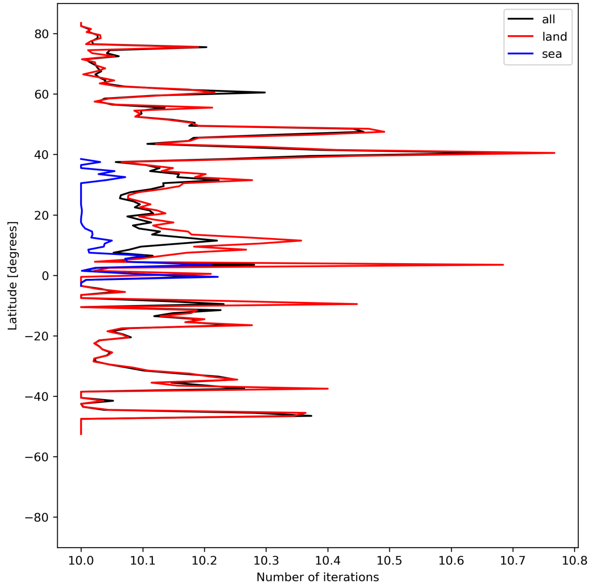
Figure 20: Zonal average of “Number of iterations” for 2024-04-18 to 2024-04-20.
