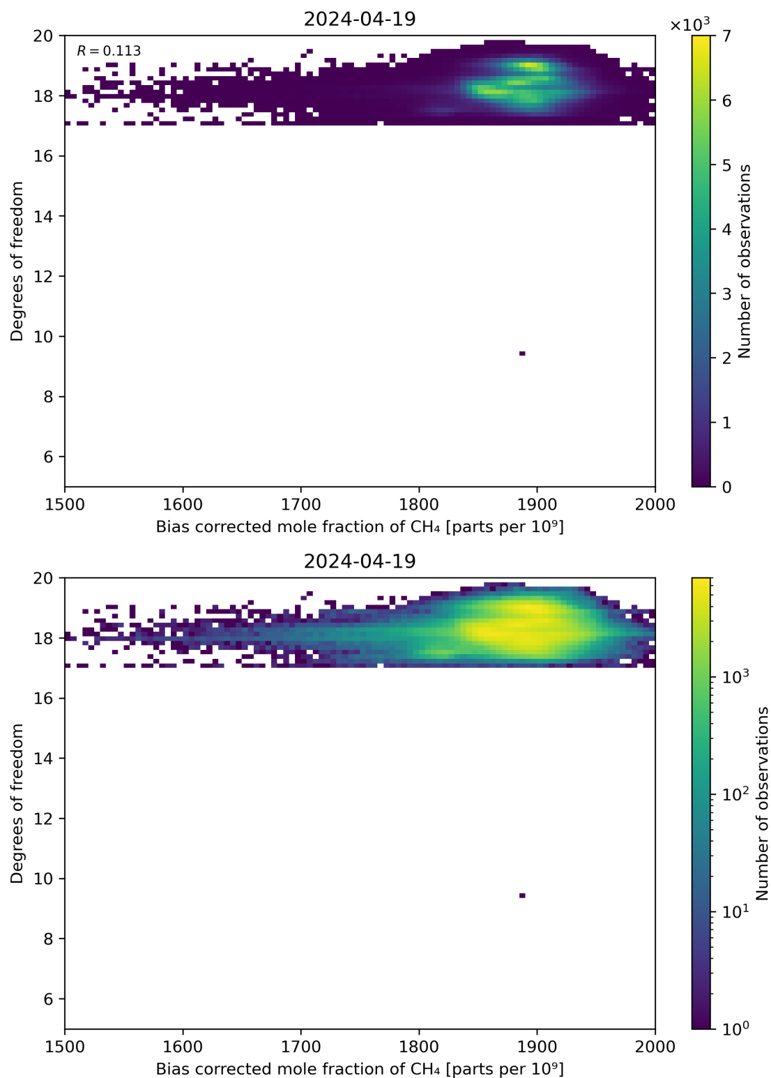
Figure 65: Scatter density plot of “Bias corrected mole fraction of CH 4 ” against “Degrees of freedom” for 2024-04-18 to 2024-04-20.
