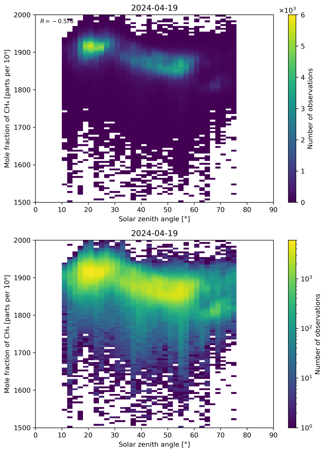
Figure 99: Scatter density plot of “Solar zenith angle” against “Mole fraction of CH 4 ” for 2024-04-18 to 2024-04-20.
