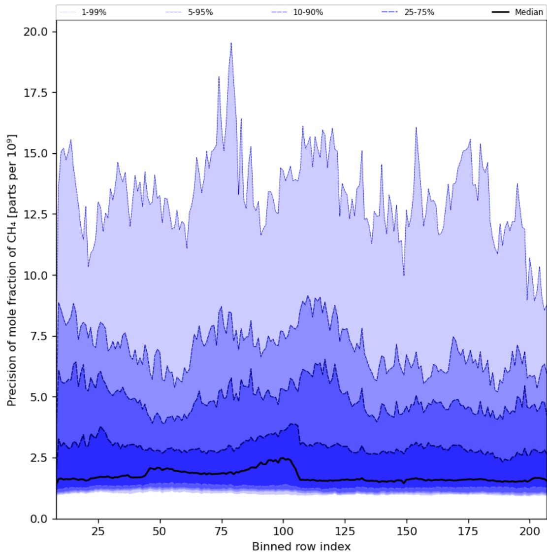
Figure 35: Along track statistics of “Precision of mole fraction of CH 4 ” for 2024-04-18 to 2024-04-20
