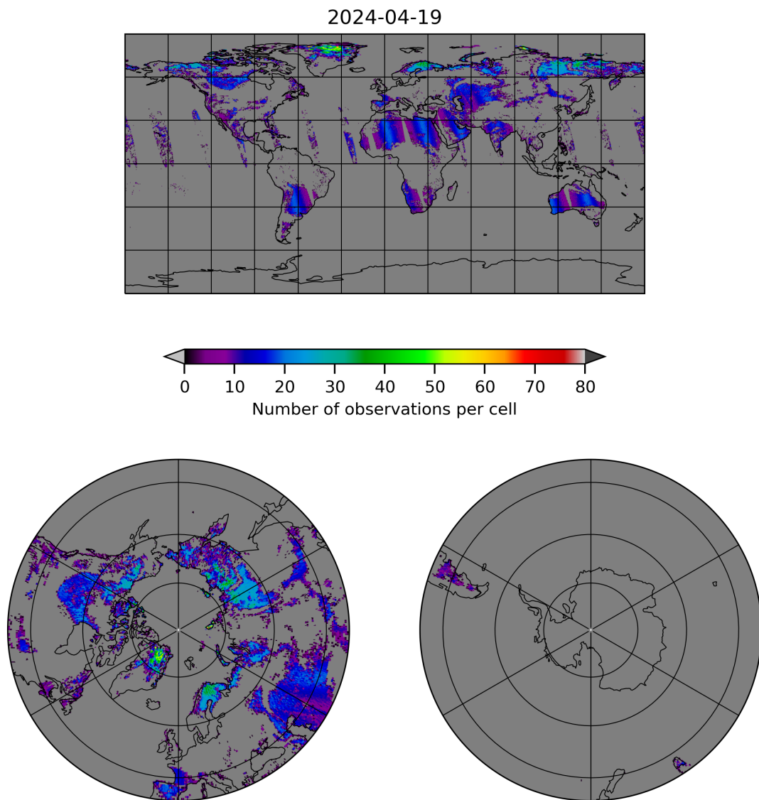
Figure 10: Map of the number of observations for 2024-04-18 to 2024-04-20
