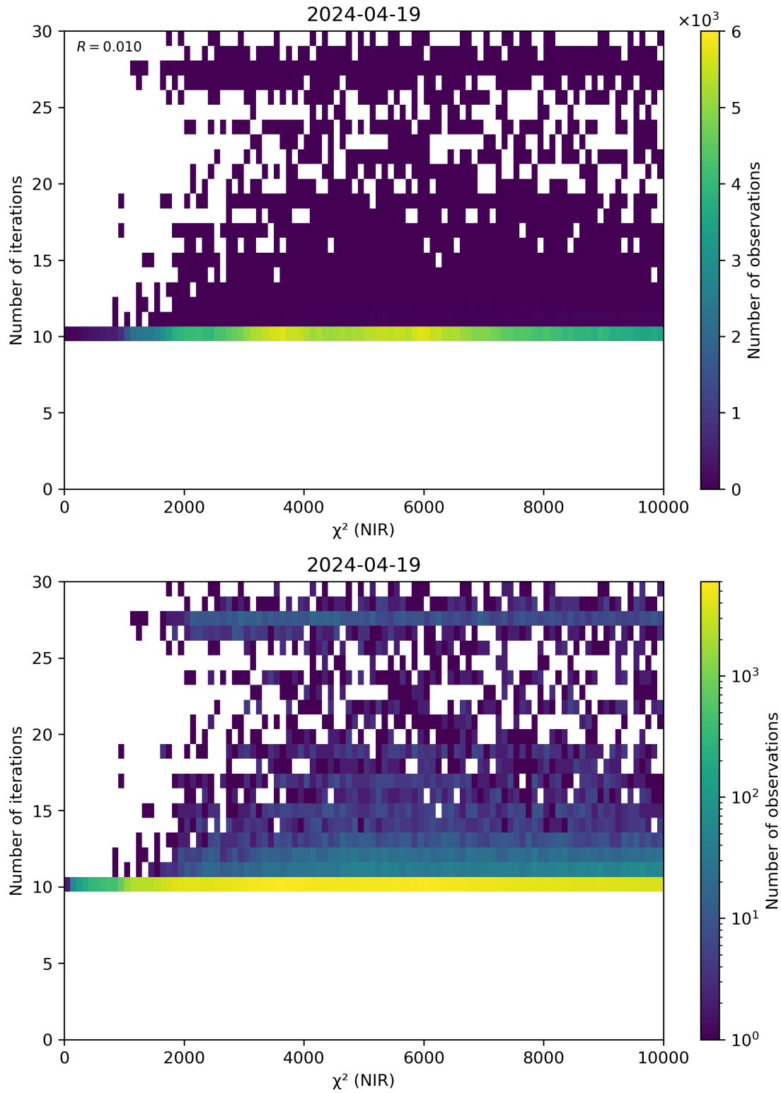
Figure 46: Scatter density plot of “ \chi^2 (NIR)” against “Number of iterations” for 2024-04-18 to 2024-04-20.
