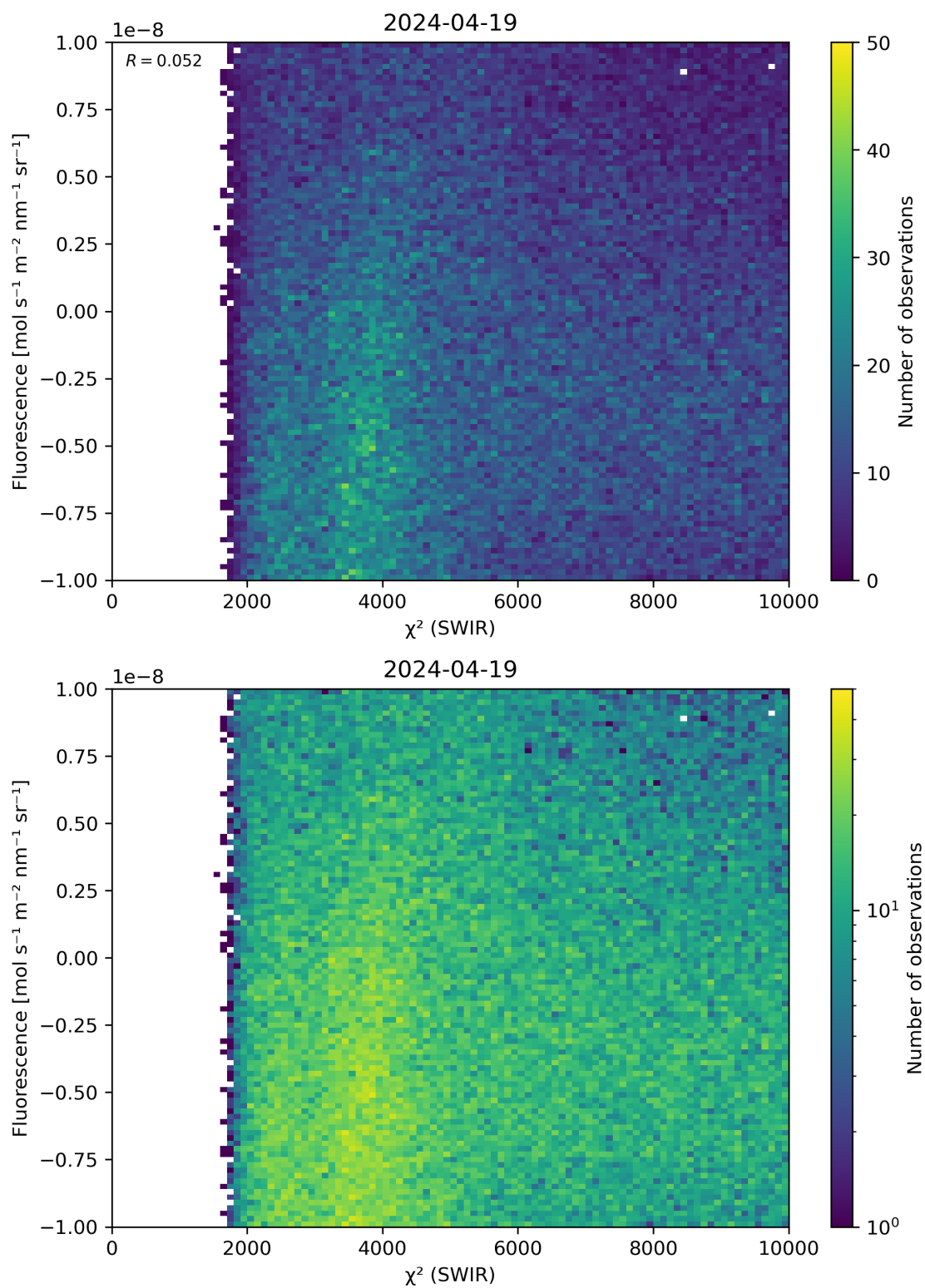
Figure 49: Scatter density plot of “ \chi^2 (SWIR)” against “Fluorescence” for 2024-04-18 to 2024-04-20.
