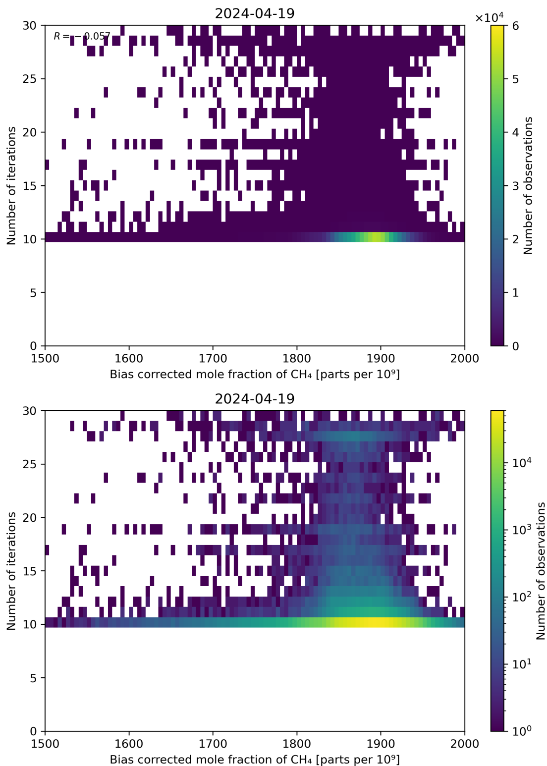
Figure 67: Scatter density plot of “Bias corrected mole fraction of \text{CH}_4 ” against “Number of iterations” for 2024-04-18 to 2024-04-20.
