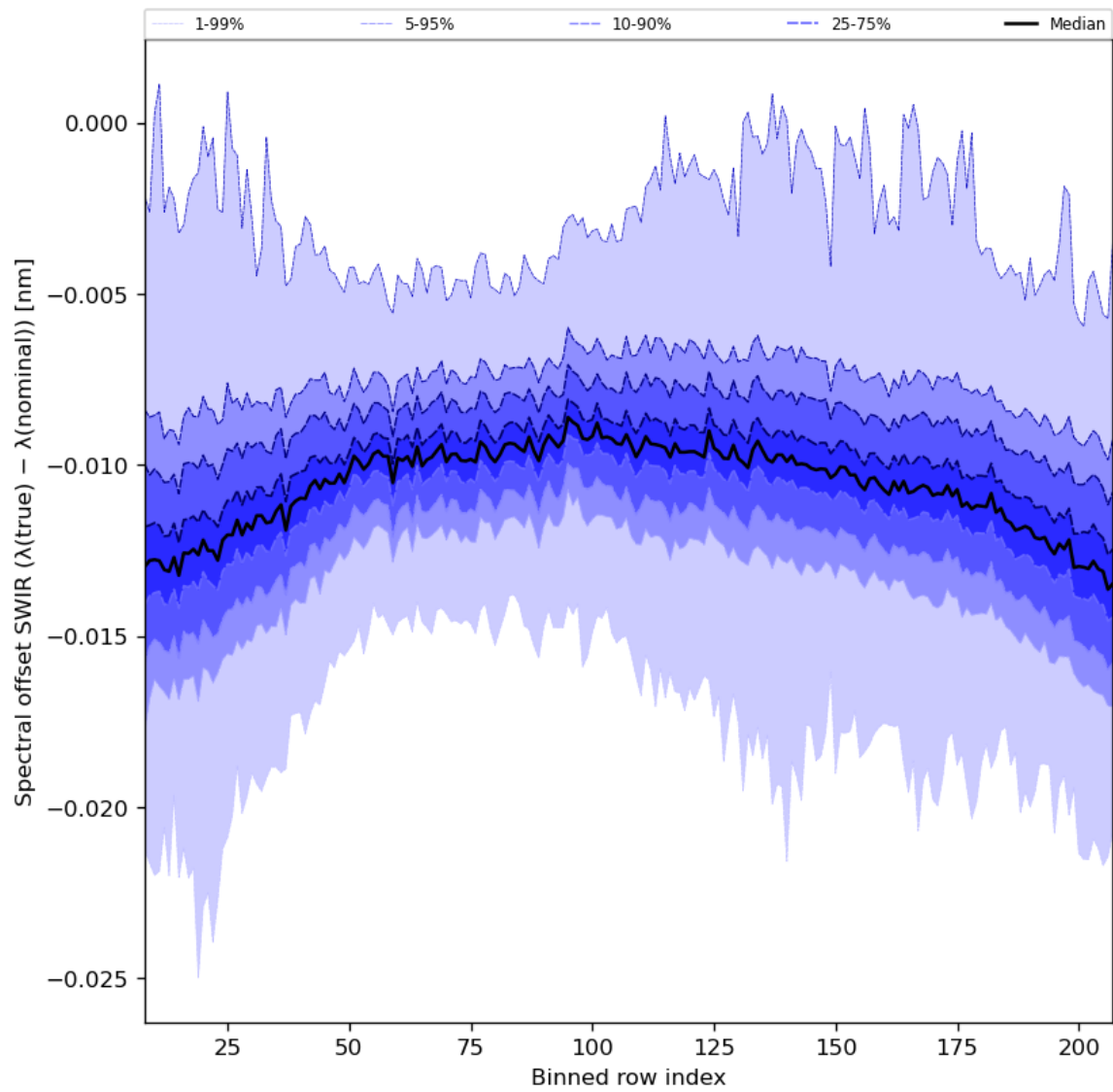
Figure 38: Along track statistics of "Spectral offset SWIR ( \lambda(\text{true}) - \lambda(\text{nominal}) )" for 2024-04-18 to 2024-04-20
