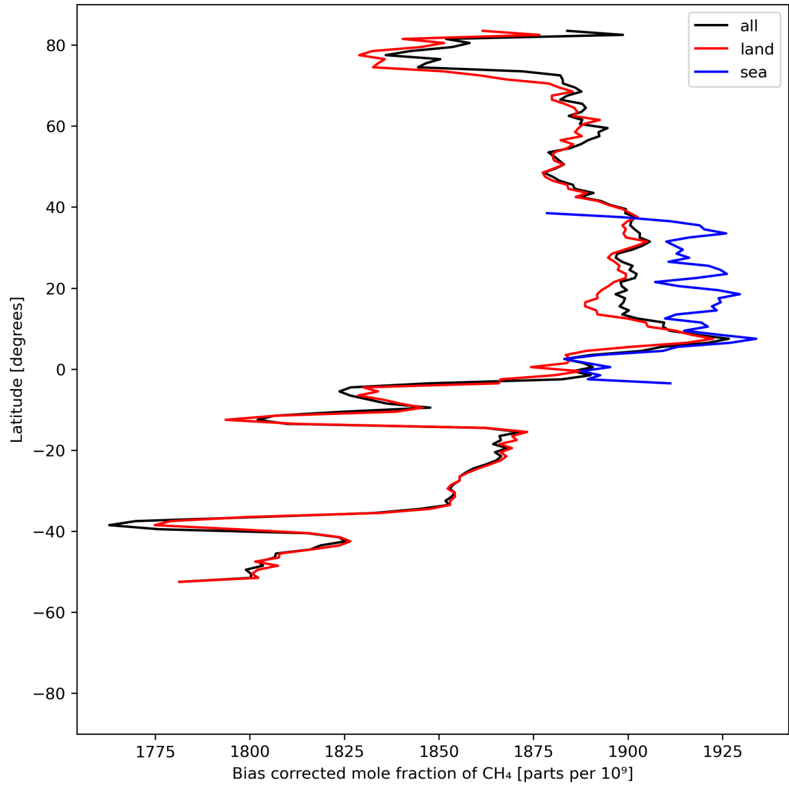
Figure 14: Zonal average of “Bias corrected mole fraction of \text{CH}_4 ” for 2024-04-18 to 2024-04-20.
