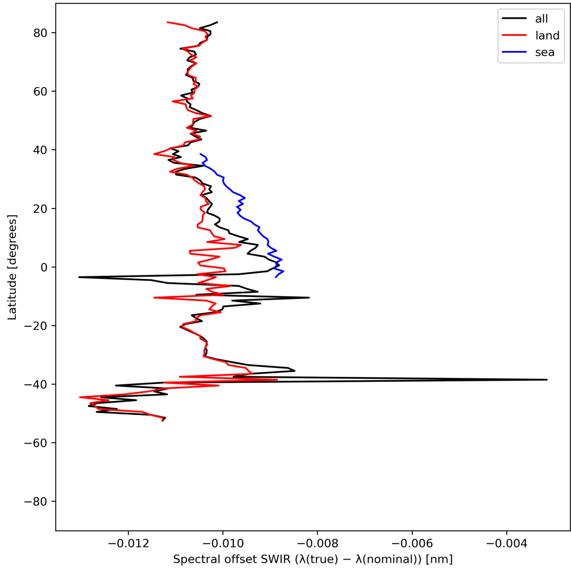
Figure 16: Zonal average of “Spectral offset SWIR ( \lambda(\text{true}) - \lambda(\text{nominal}) )” for 2024-04-18 to 2024-04-20.
