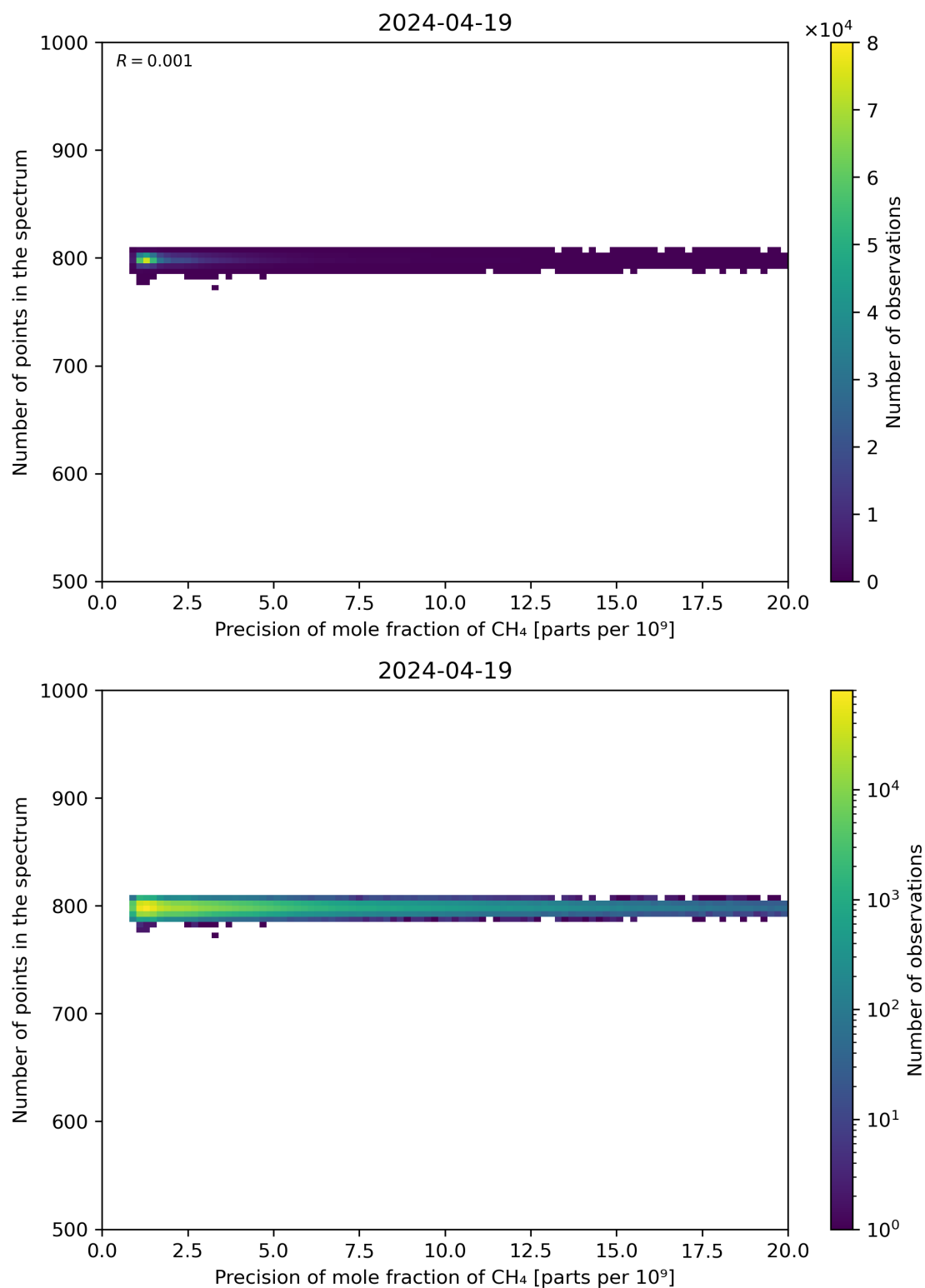
Figure 84: Scatter density plot of “Precision of mole fraction of \text{CH}_4 ” against “Number of points in the spectrum” for 2024-04-18 to 2024-04-20.
