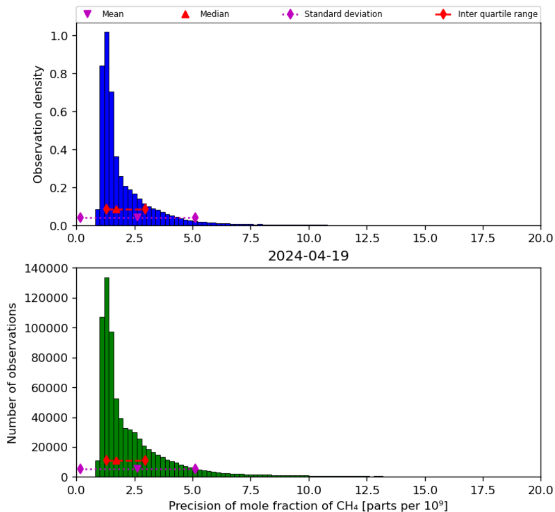
Figure 24: Histogram of “Precision of mole fraction of CH 4 ” for 2024-04-18 to 2024-04-20
