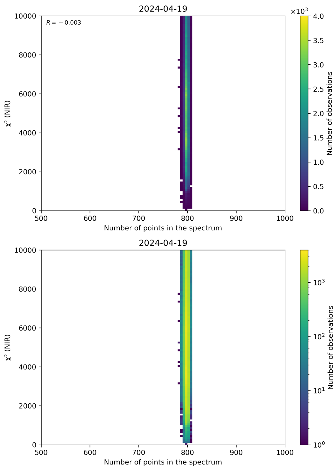
Figure 88: Scatter density plot of “Number of points in the spectrum” against “ \chi^2 (NIR)” for 2024-04-18 to 2024-04-20.
