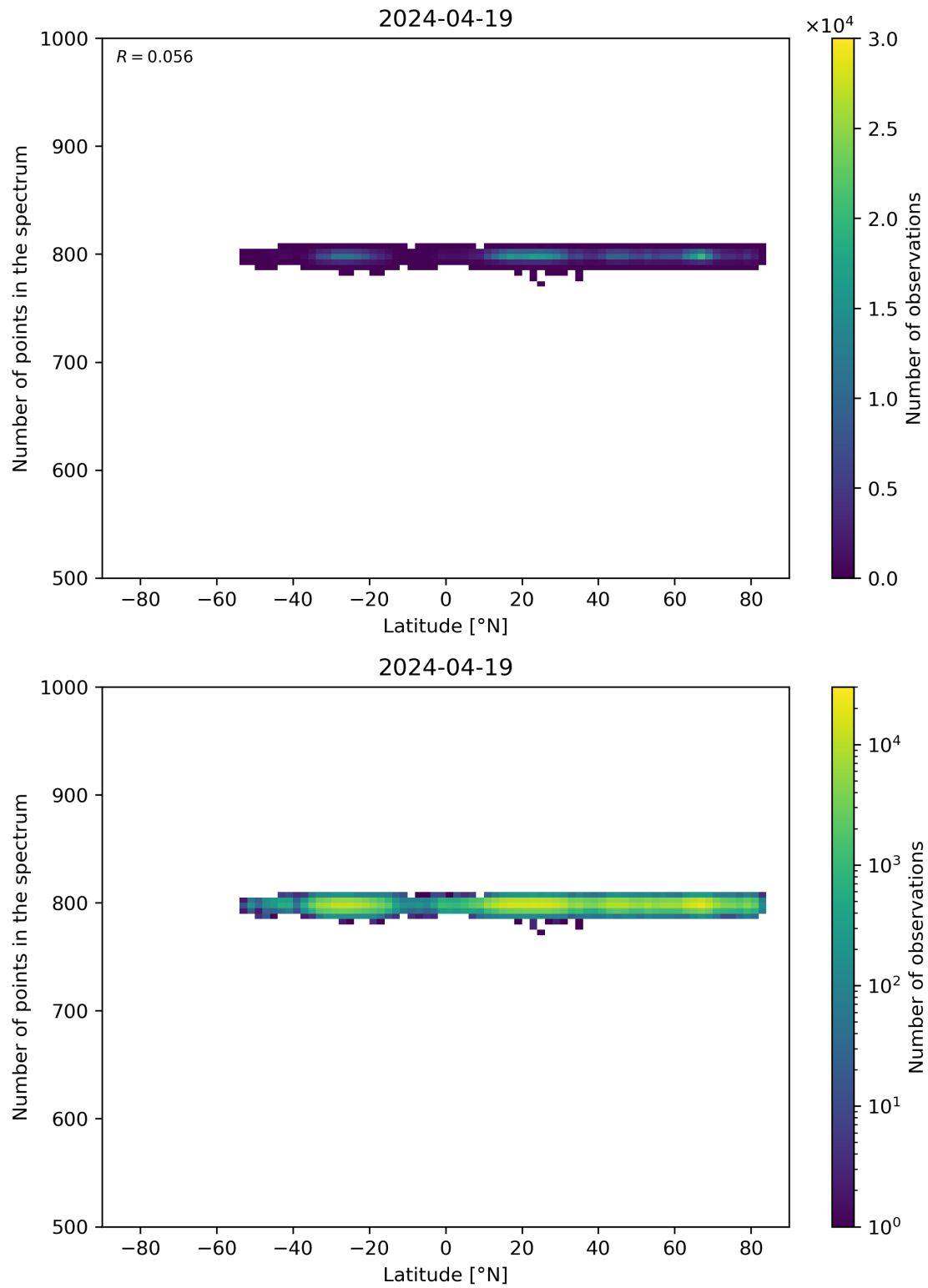
Figure 61: Scatter density plot of “Latitude” against “Number of points in the spectrum” for 2024-04-18 to 2024-04-20.
