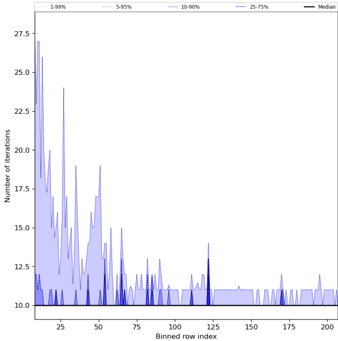
Figure 42: Along track statistics of “Number of iterations” for 2024-04-18 to 2024-04-20
