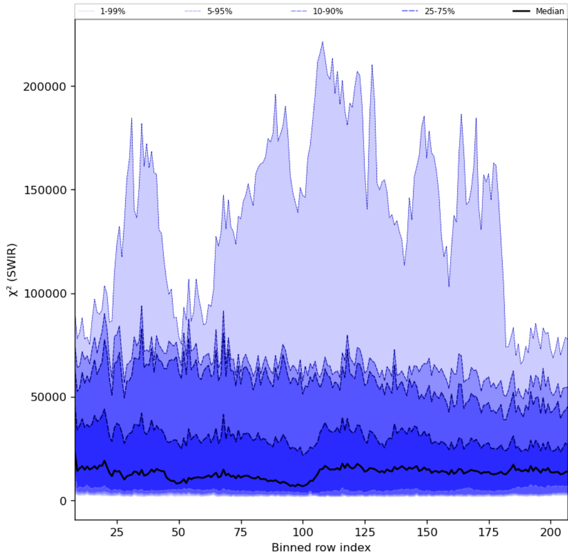
Figure 39: Along track statistics of “ \chi^2 (SWIR)” for 2024-04-18 to 2024-04-20
