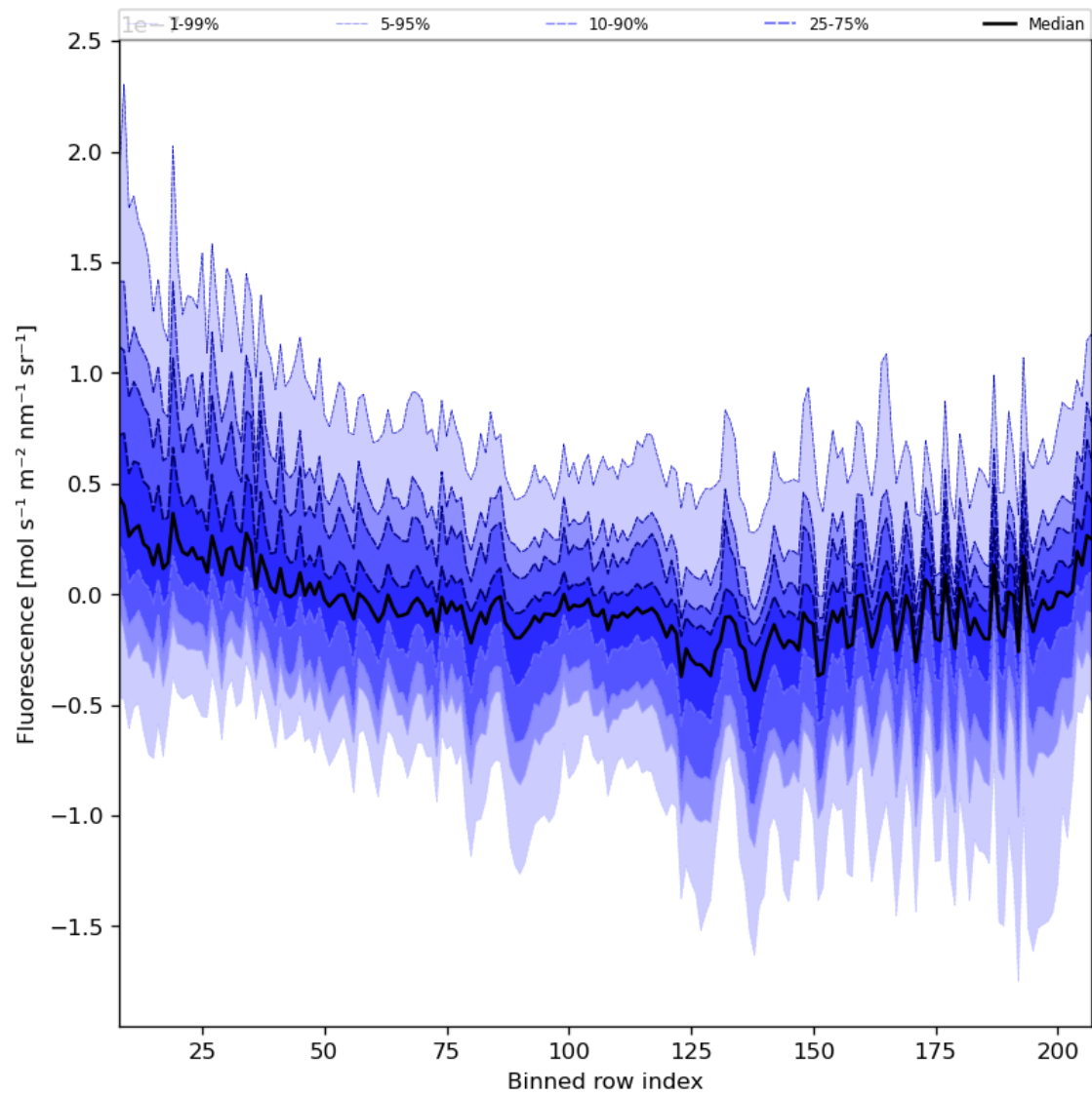
Figure 43: Along track statistics of “Fluorescence” for 2024-04-18 to 2024-04-20
