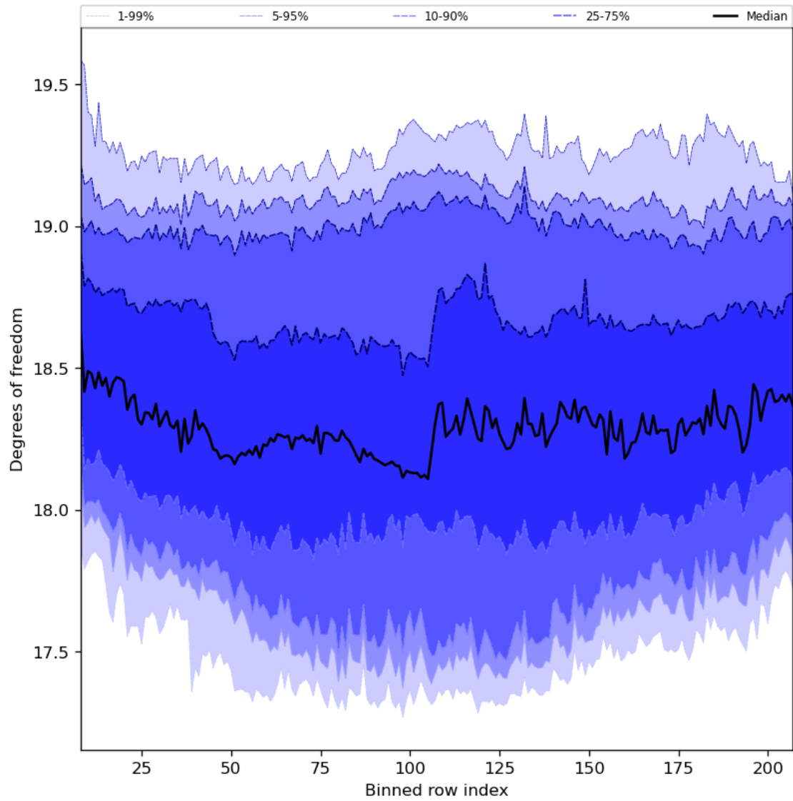
Figure 41: Along track statistics of “Degrees of freedom” for 2024-04-18 to 2024-04-20
