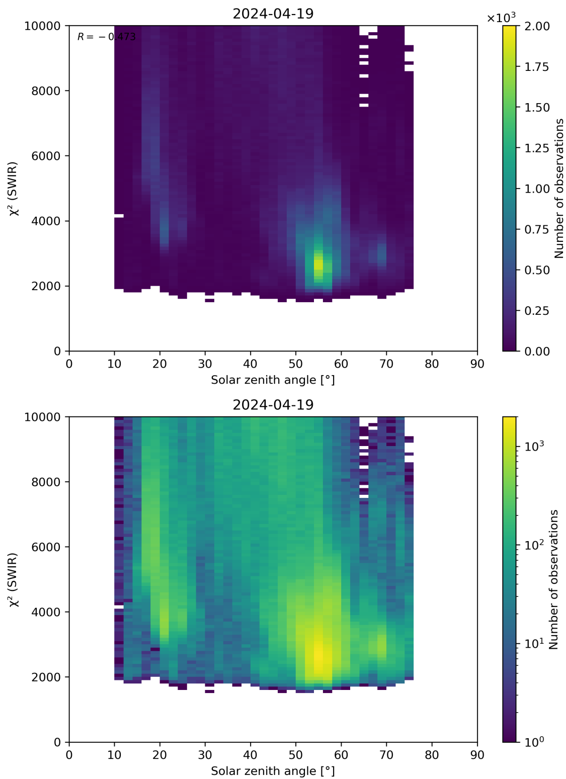
Figure 95: Scatter density plot of “Solar zenith angle” against “ \chi^2 (SWIR)” for 2024-04-18 to 2024-04-20.
