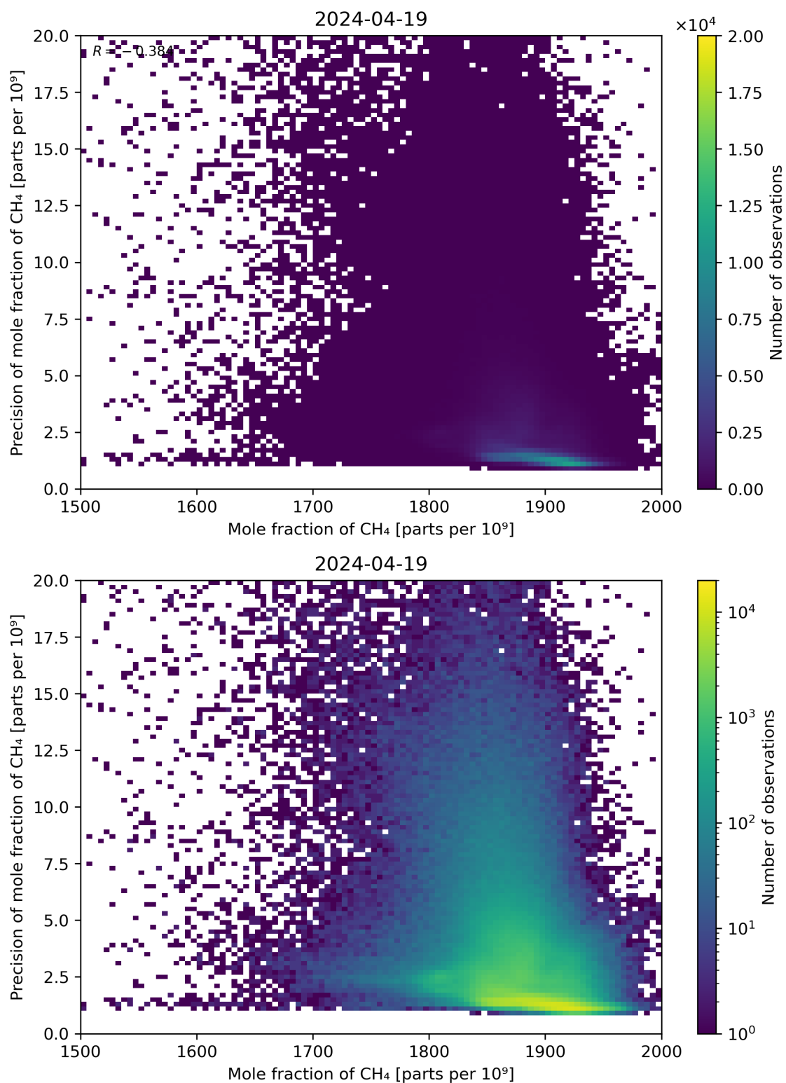
Figure 75: Scatter density plot of “Mole fraction of CH 4 ” against “Precision of mole fraction of CH 4 ” for 2024-04-18 to 2024-04-20.
