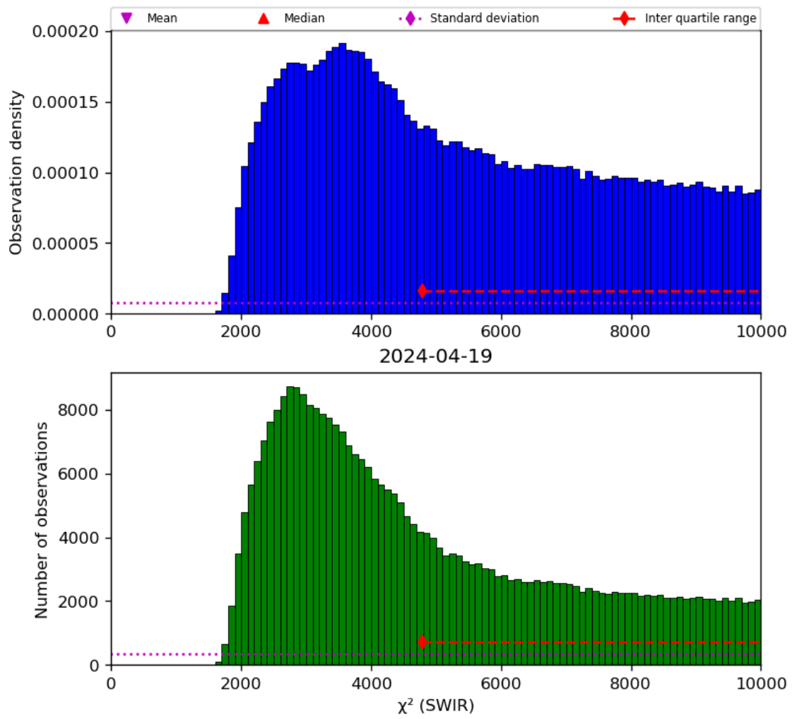
Figure 28: Histogram of " \chi^2 (SWIR)" for 2024-04-18 to 2024-04-20
