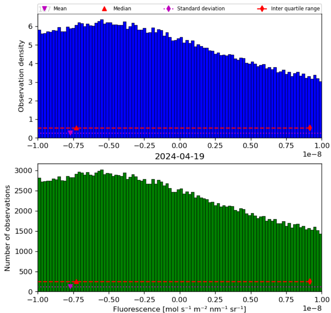
Figure 32: Histogram of “Fluorescence” for 2024-04-18 to 2024-04-20
