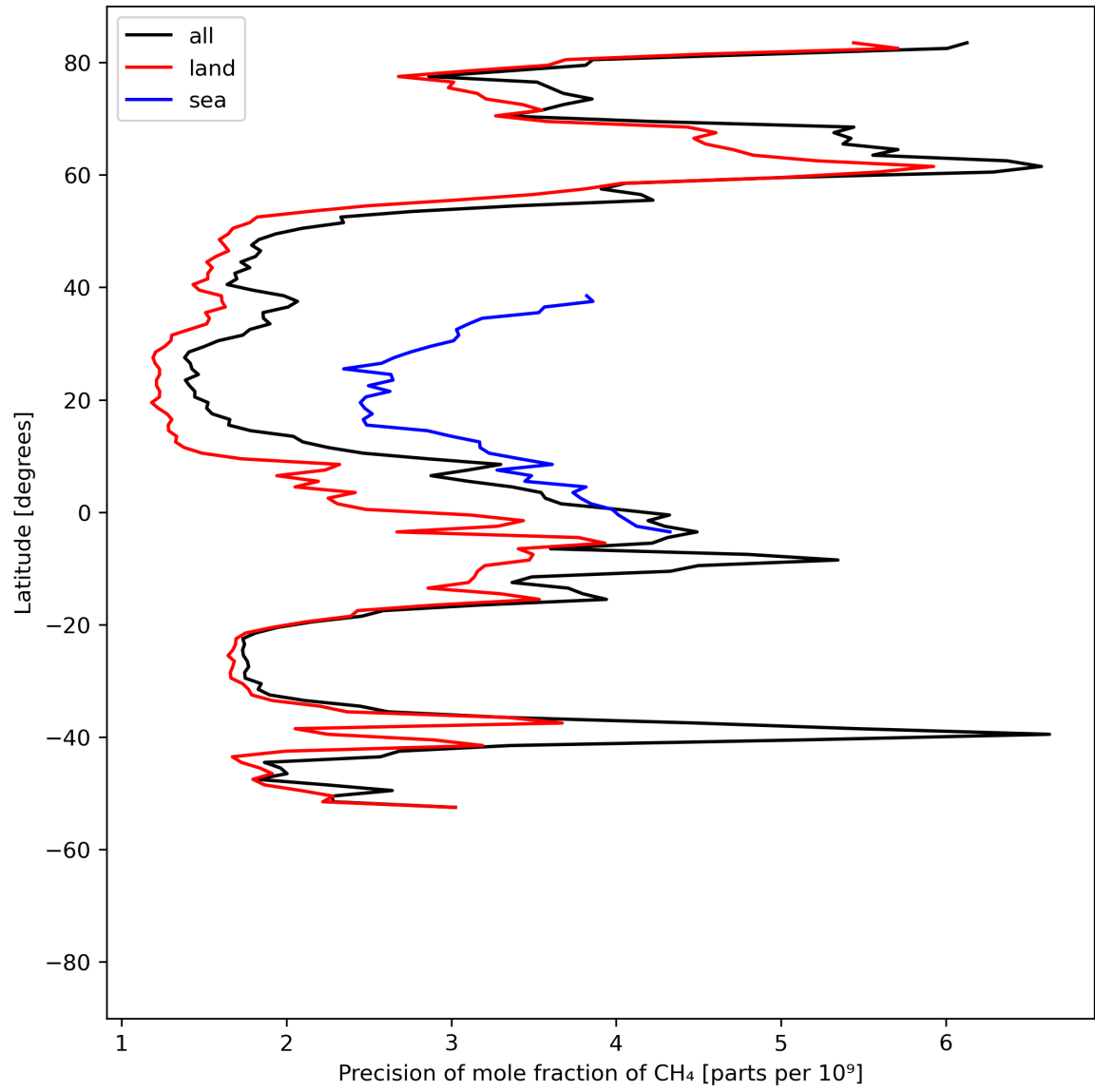
Figure 13: Zonal average of “Precision of mole fraction of CH 4 ” for 2024-04-18 to 2024-04-20.
