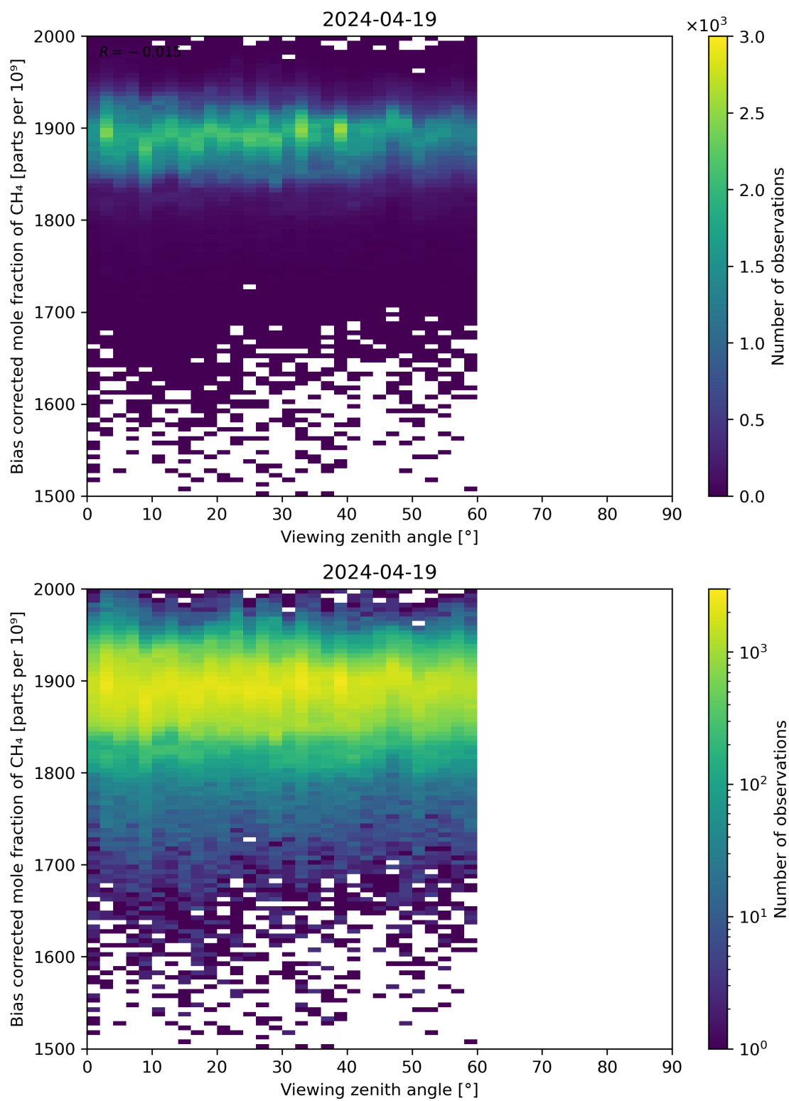
Figure 111: Scatter density plot of “Viewing zenith angle” against “Bias corrected mole fraction of CH 4 ” for 2024-04-18 to 2024-04-20.
