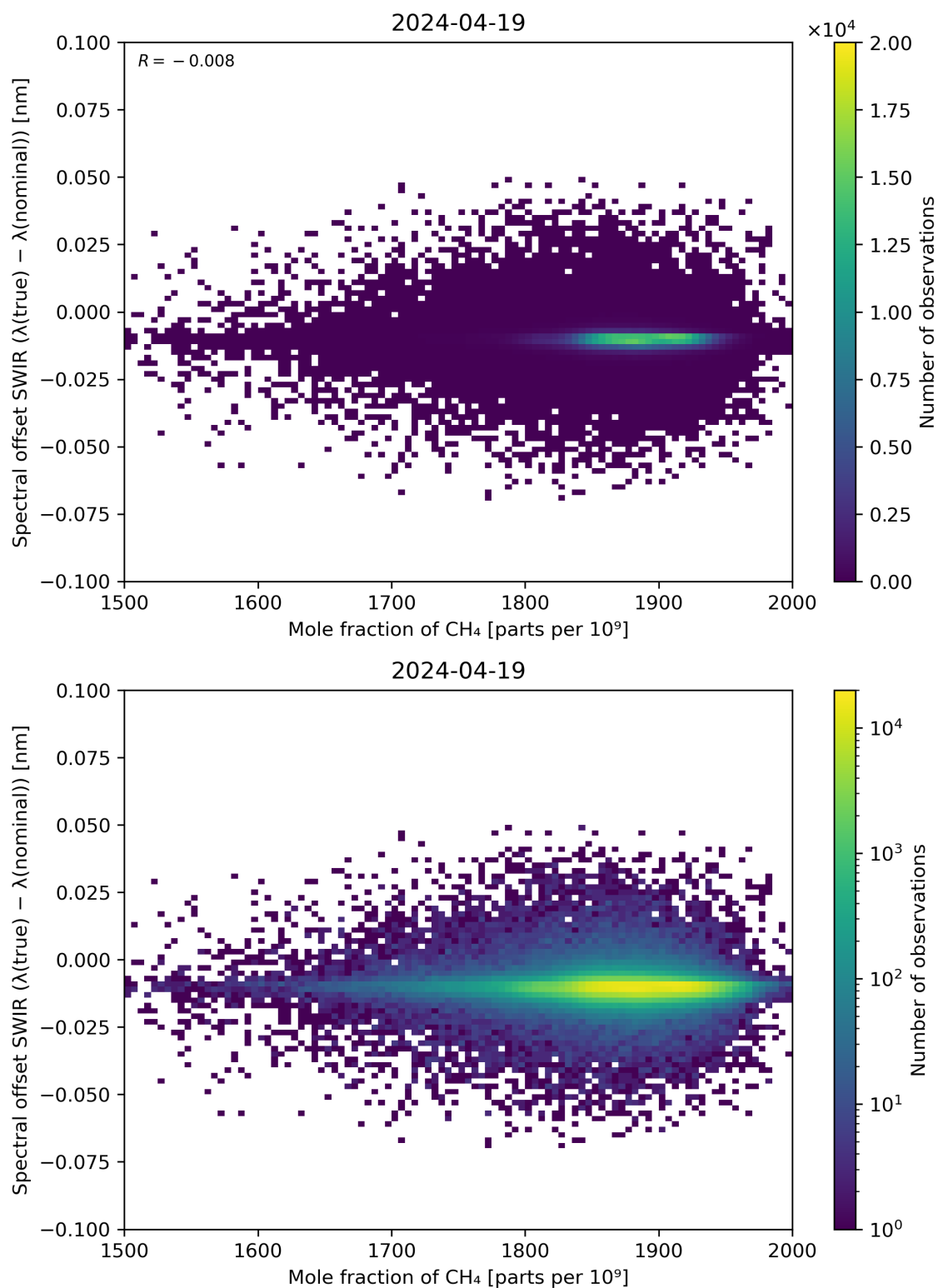
Figure 86: Scatter density plot of “Mole fraction of CH 4 ” against “Spectral offset SWIR ( \lambda(\text{true}) - \lambda(\text{nominal}) )” for 2024-04-18 to 2024-04-20.
