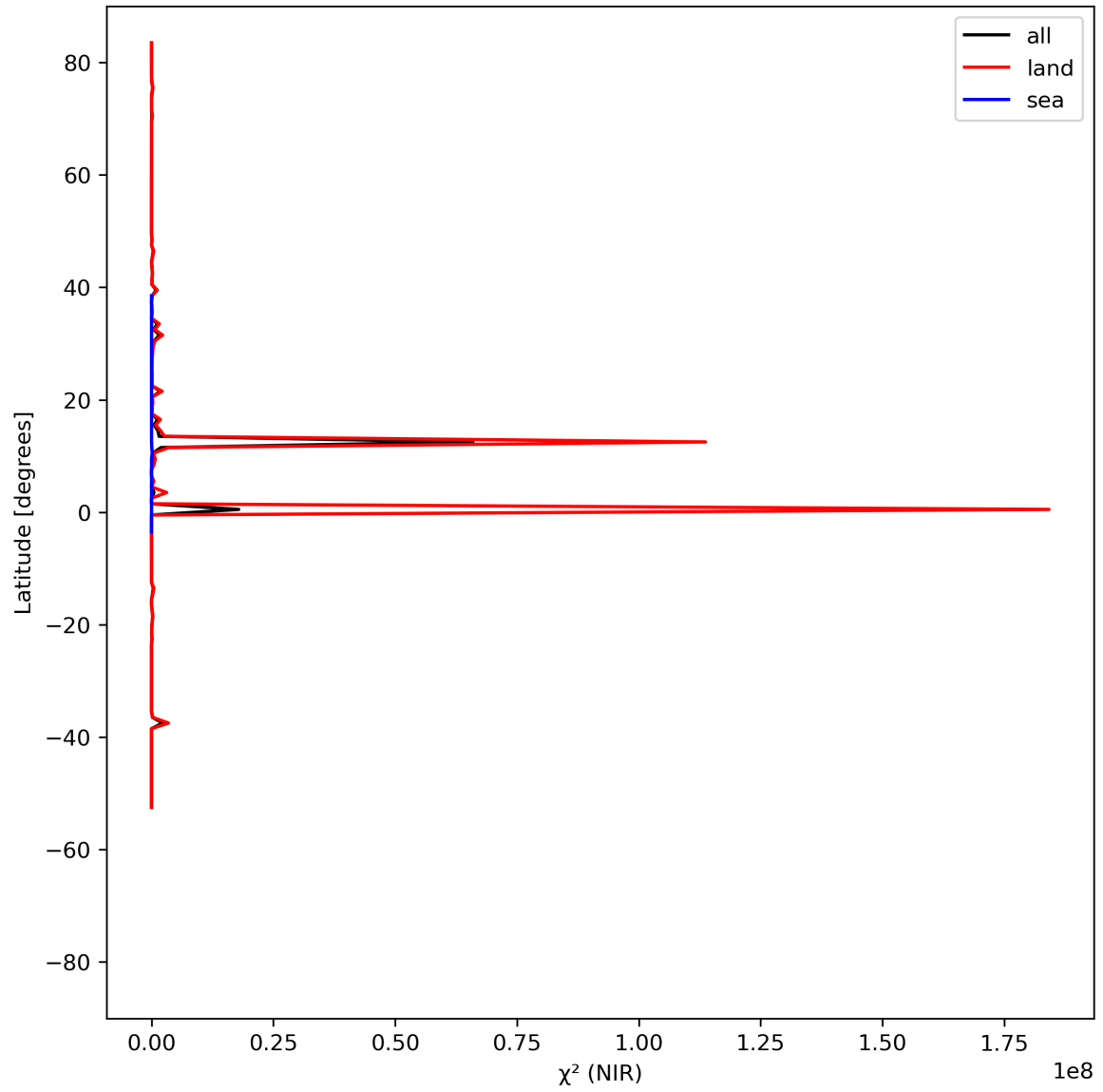
Figure 18: Zonal average of “ \chi^2 (NIR)” for 2024-04-18 to 2024-04-20.
