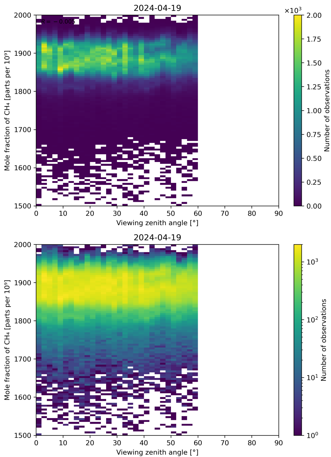
Figure 110: Scatter density plot of “Viewing zenith angle” against “Mole fraction of CH 4 ” for 2024-04-18 to 2024-04-20.
