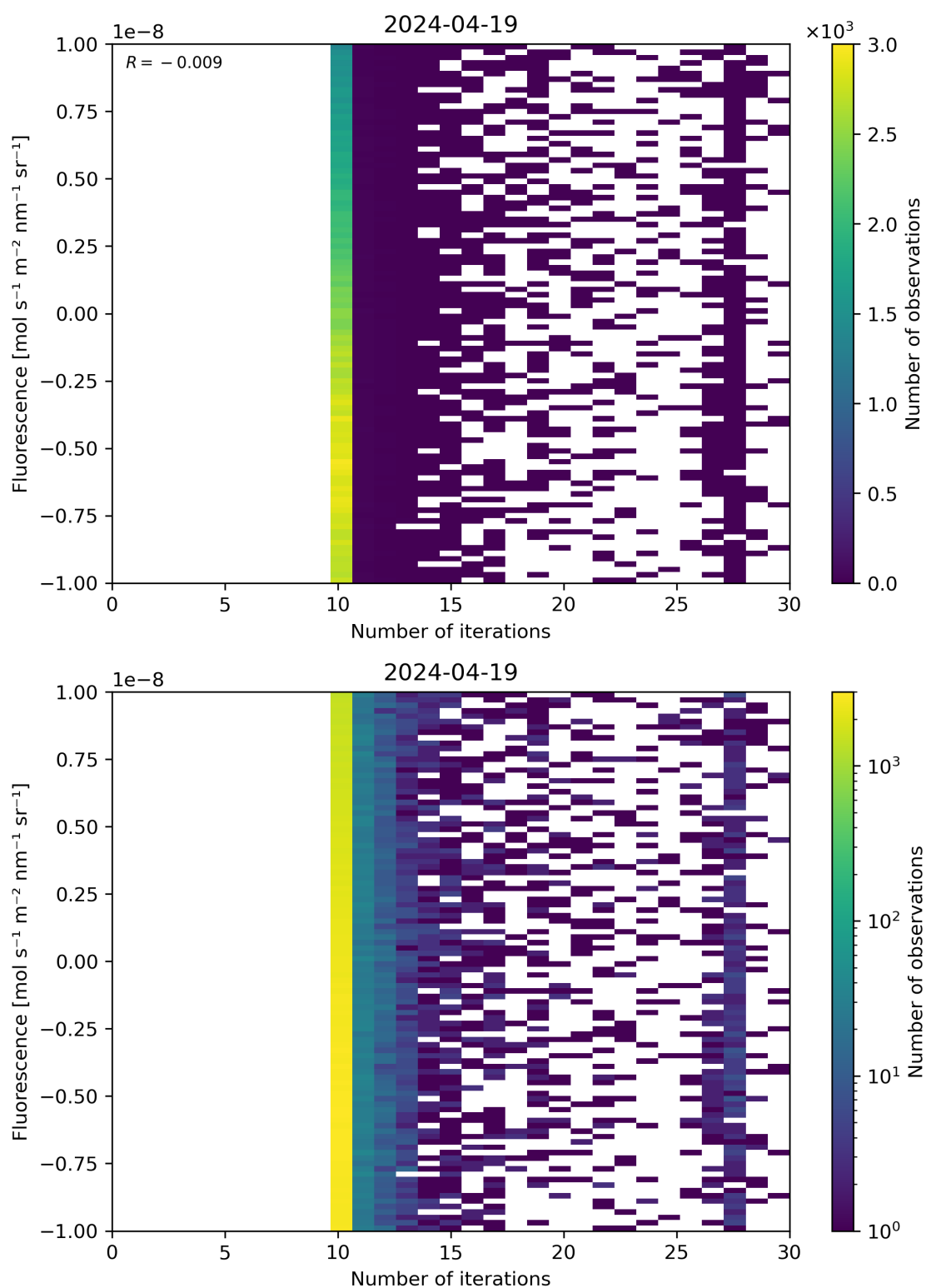
Figure 87: Scatter density plot of “Number of iterations” against “Fluorescence” for 2024-04-18 to 2024-04-20.
