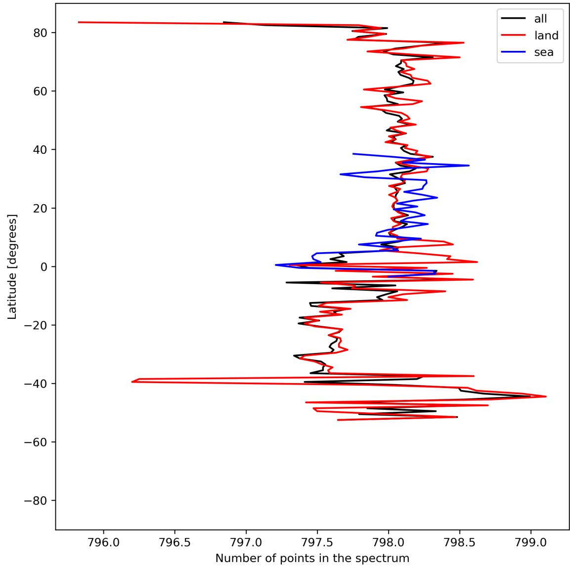
Figure 15: Zonal average of “Number of points in the spectrum” for 2024-04-18 to 2024-04-20.
