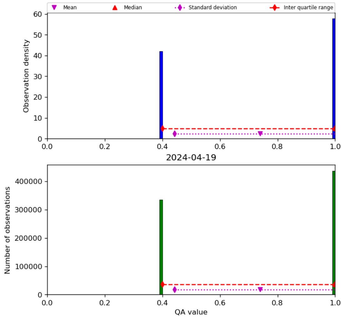
Figure 22: Histogram of “QA value” for 2024-04-18 to 2024-04-20
