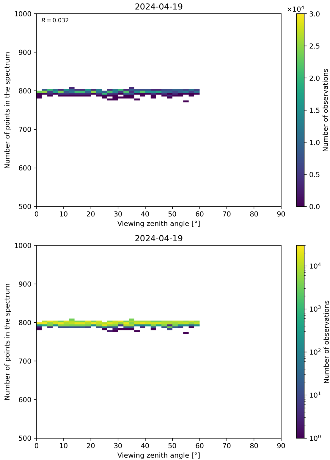
Figure 114: Scatter density plot of “Viewing zenith angle” against “Number of points in the spectrum” for 2024-04-18 to 2024-04-20.
