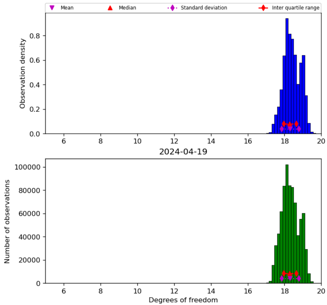
Figure 30: Histogram of “Degrees of freedom” for 2024-04-18 to 2024-04-20
