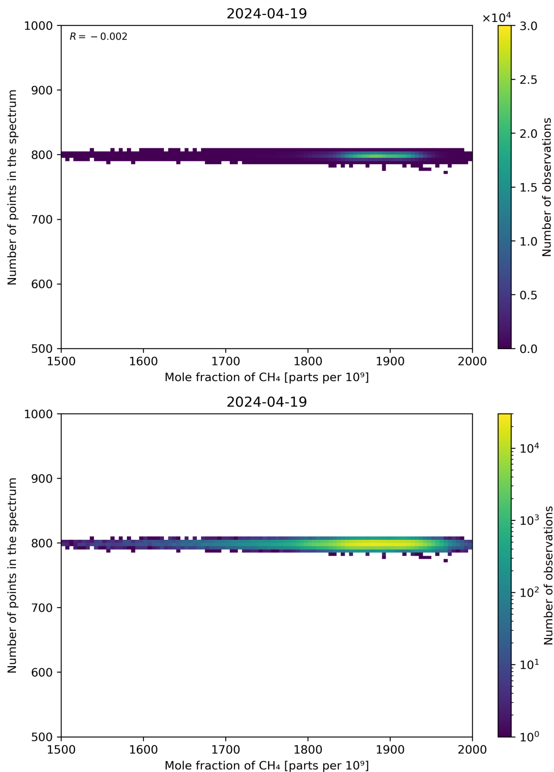
Figure 77: Scatter density plot of “Mole fraction of CH 4 ” against “Number of points in the spectrum” for 2024-04-18 to 2024-04-20.
