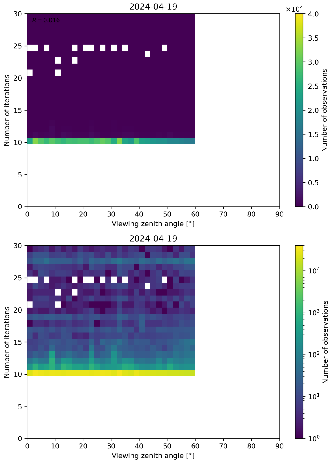
Figure 113: Scatter density plot of “Viewing zenith angle” against “Number of iterations” for 2024-04-18 to 2024-04-20.
