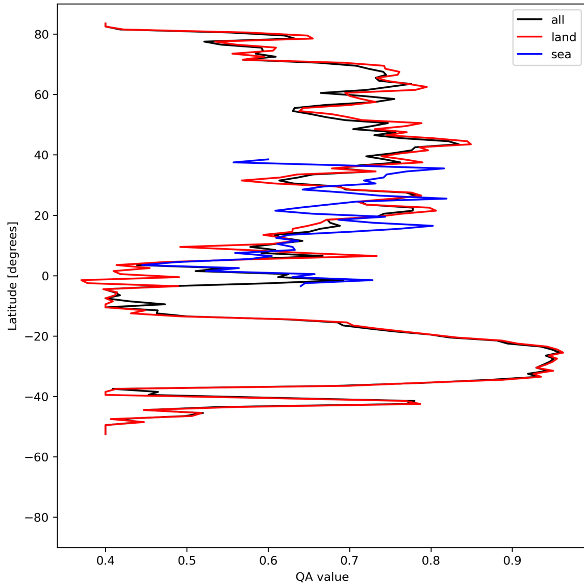
Figure 11: Zonal average of “QA value” for 2024-04-18 to 2024-04-20.
