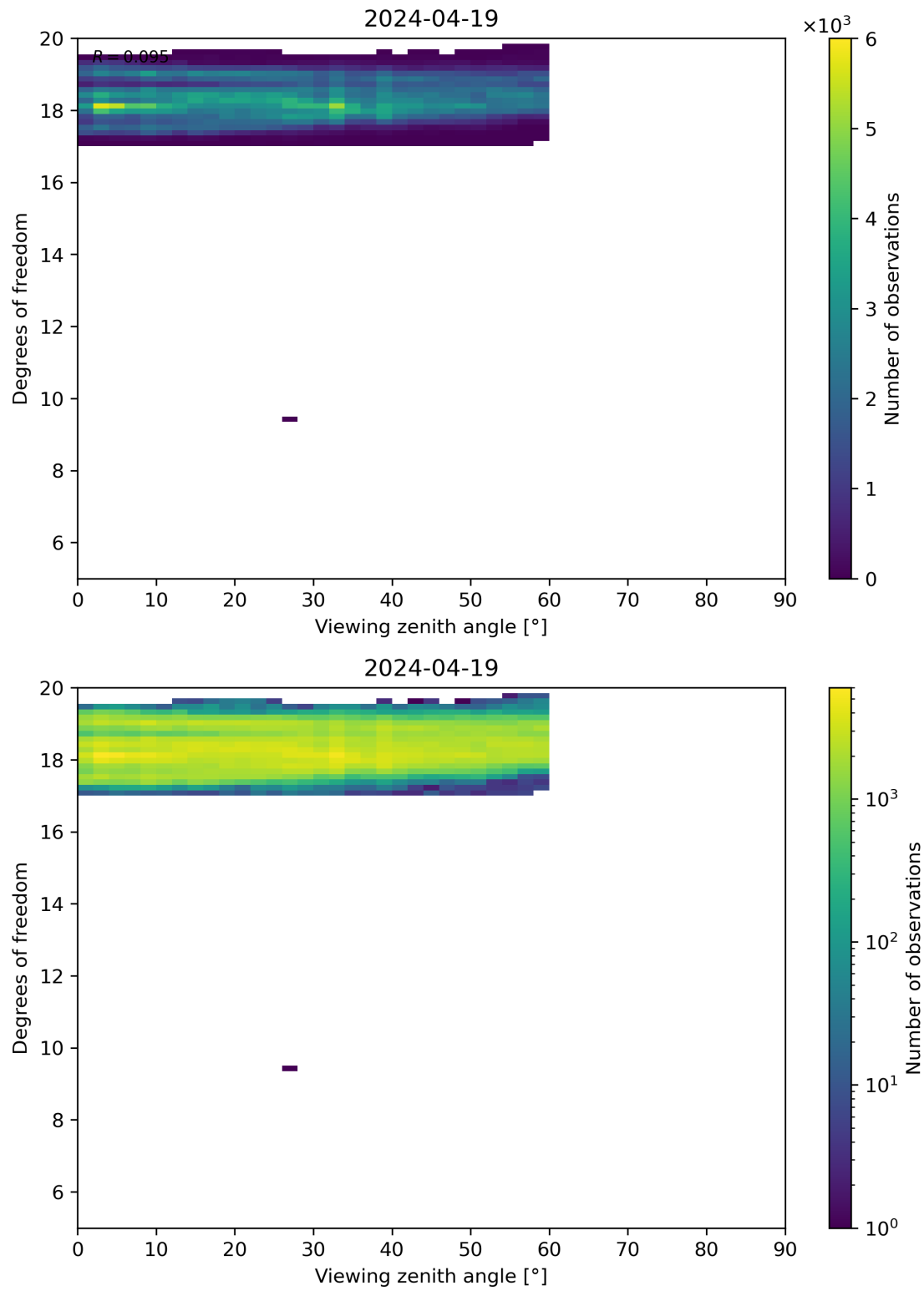
Figure 107: Scatter density plot of “Viewing zenith angle” against “Degrees of freedom” for 2024-04-18 to 2024-04-20.
