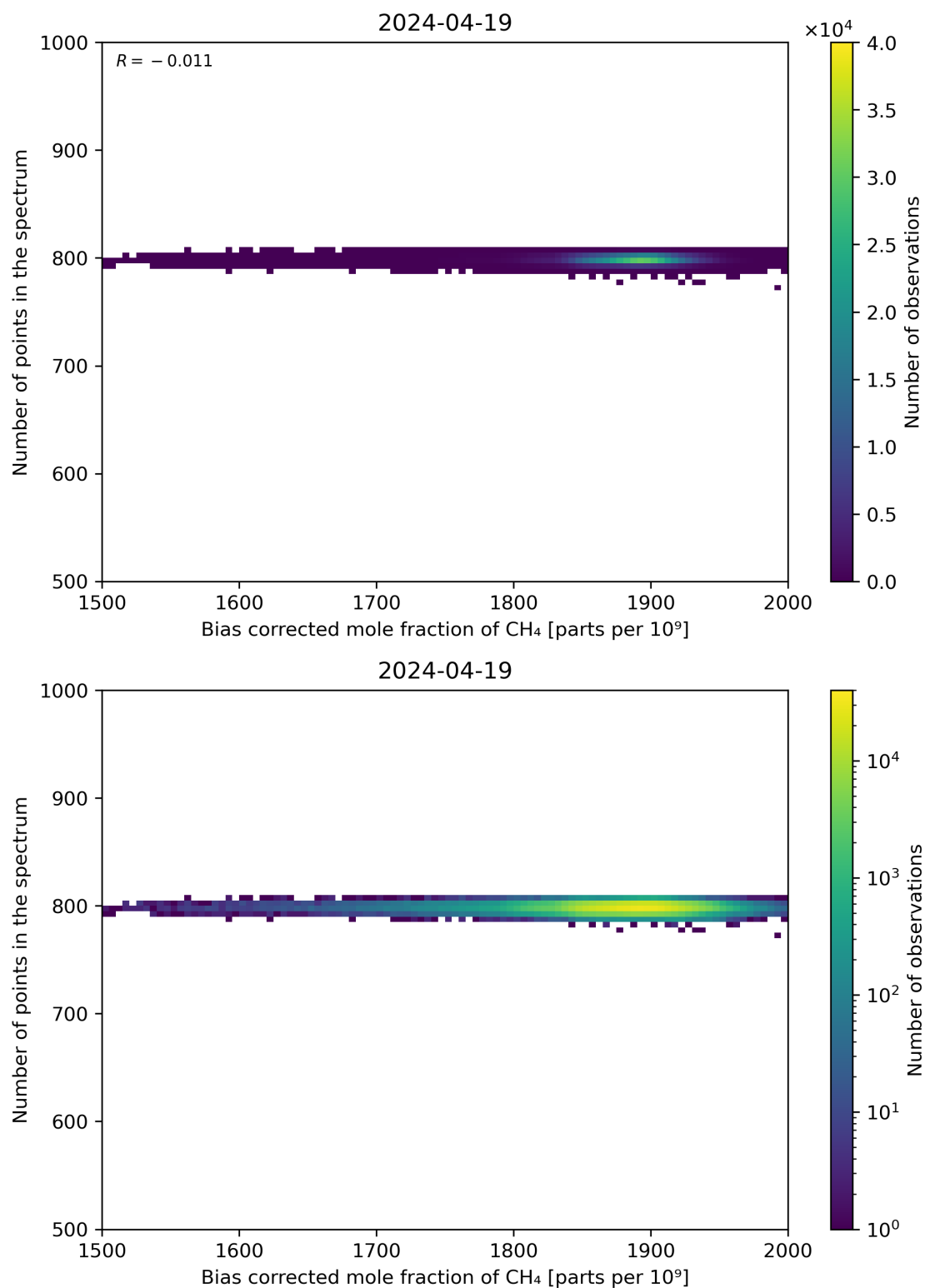
Figure 68: Scatter density plot of “Bias corrected mole fraction of CH 4 ” against “Number of points in the spectrum” for 2024-04-18 to 2024-04-20.
