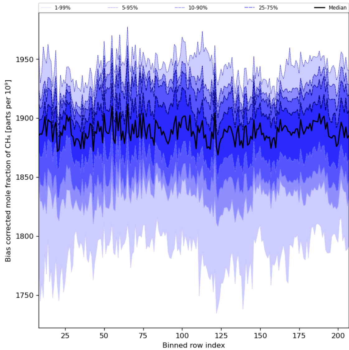
Figure 36: Along track statistics of “Bias corrected mole fraction of CH 4 ” for 2024-04-18 to 2024-04-20
