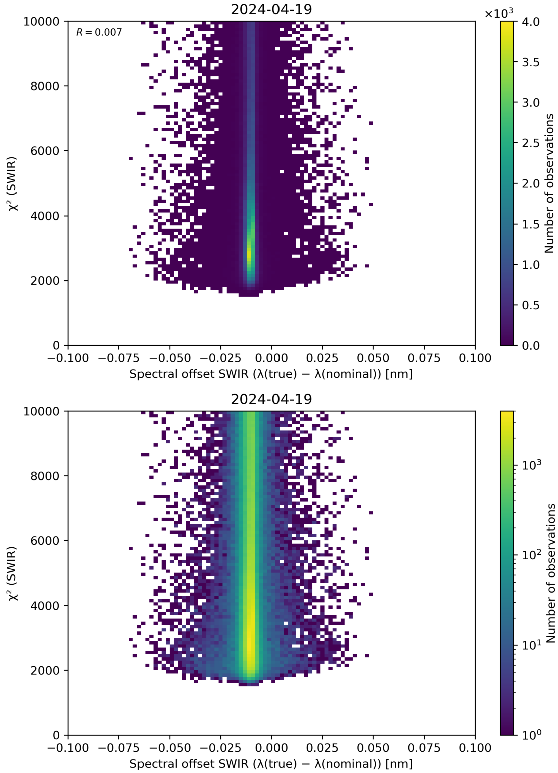
Figure 118: Scatter density plot of “Spectral offset SWIR ( \lambda(\text{true}) - \lambda(\text{nominal}) )” against “ \chi^2 (SWIR)” for 2024-04-18 to 2024-04-20.
