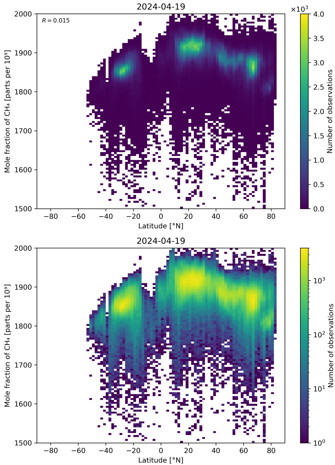
Figure 57: Scatter density plot of “Latitude” against “Mole fraction of CH 4 ” for 2024-04-18 to 2024-04-20.
