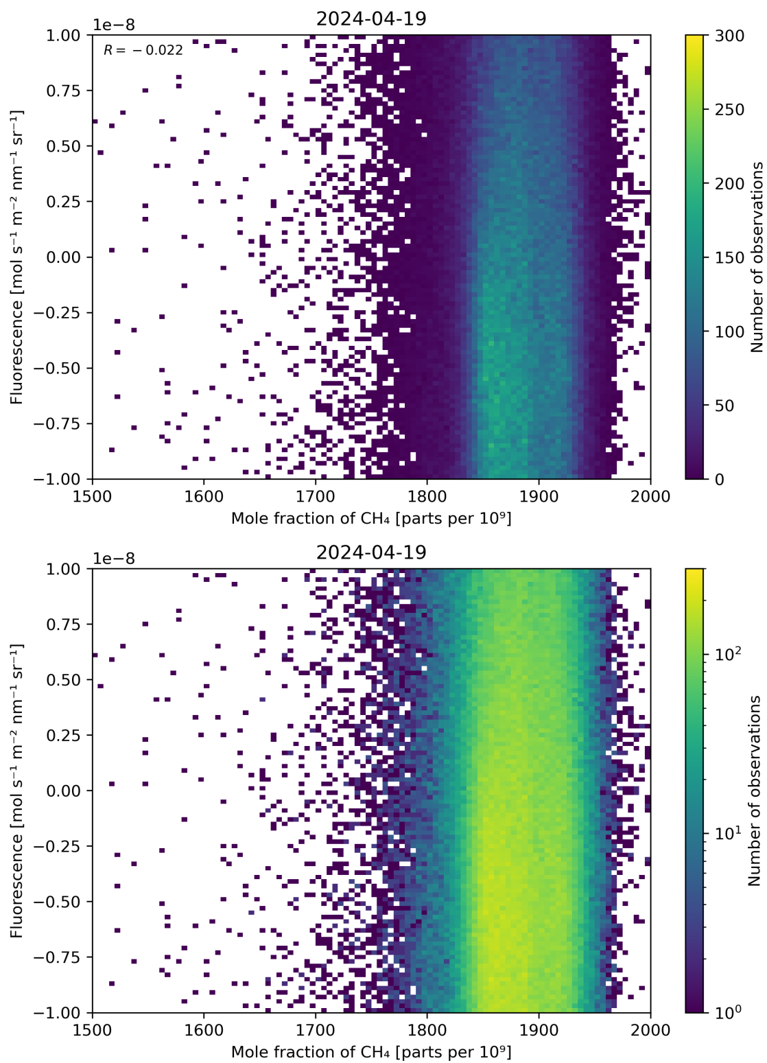
Figure 73: Scatter density plot of “Mole fraction of \text{CH}_4 ” against “Fluorescence” for 2024-04-18 to 2024-04-20.
