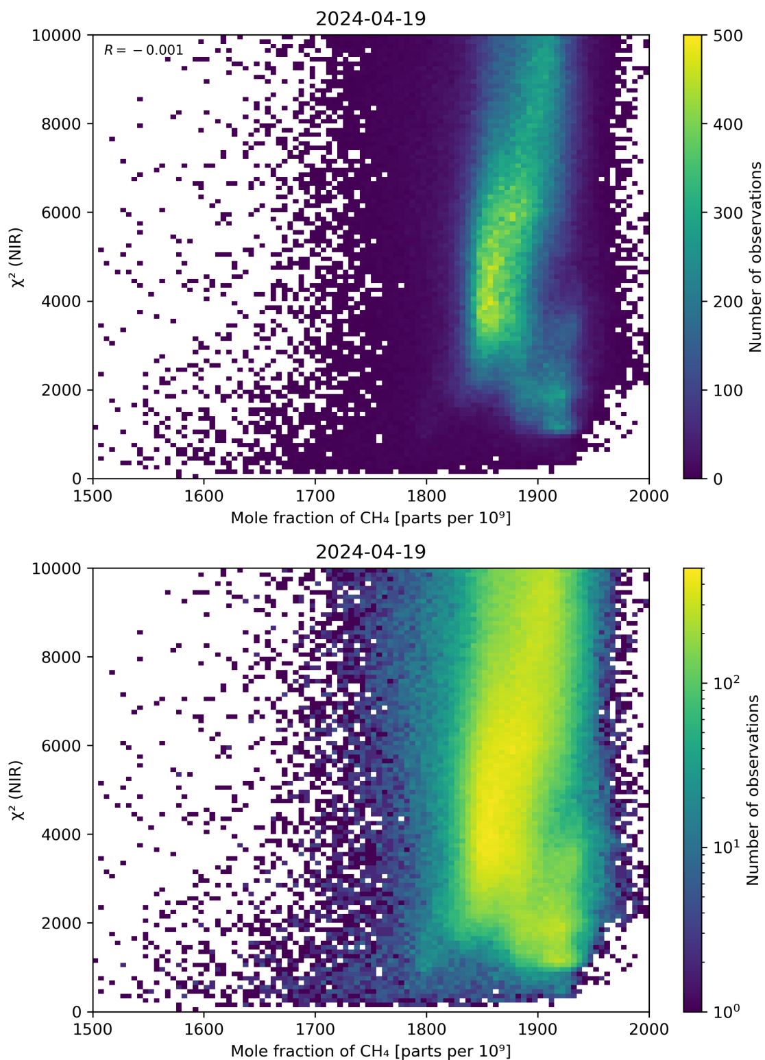
Figure 70: Scatter density plot of “Mole fraction of CH 4 ” against “ \chi^2 (NIR)” for 2024-04-18 to 2024-04-20.
