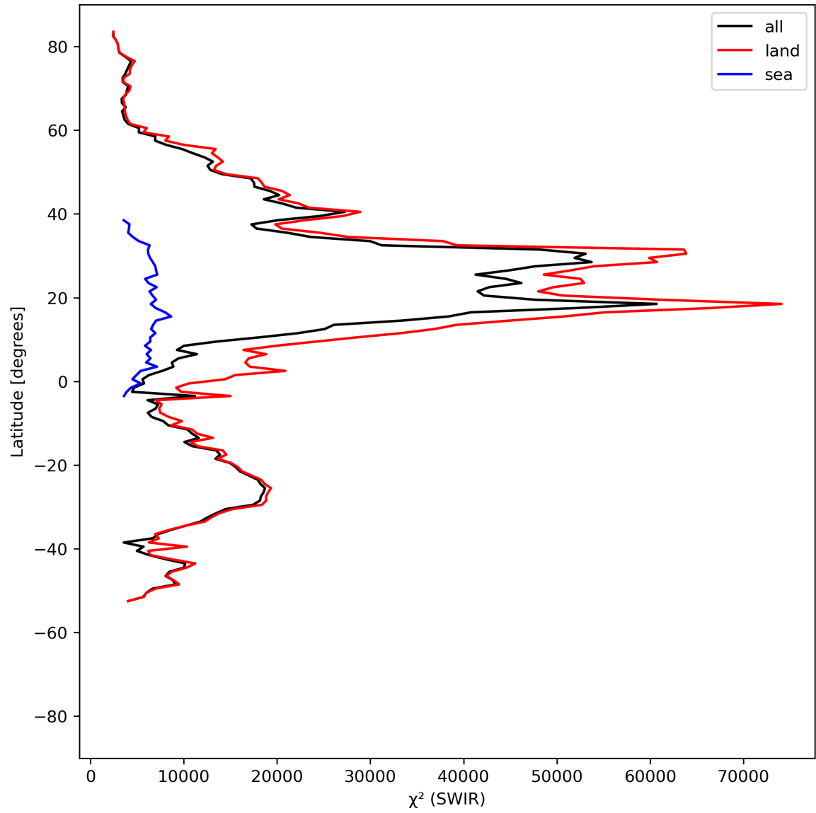
Figure 17: Zonal average of “ \chi^2 (SWIR)” for 2024-04-18 to 2024-04-20.
