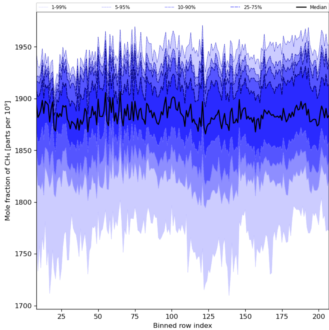
Figure 34: Along track statistics of “Mole fraction of CH 4 ” for 2024-04-18 to 2024-04-20
