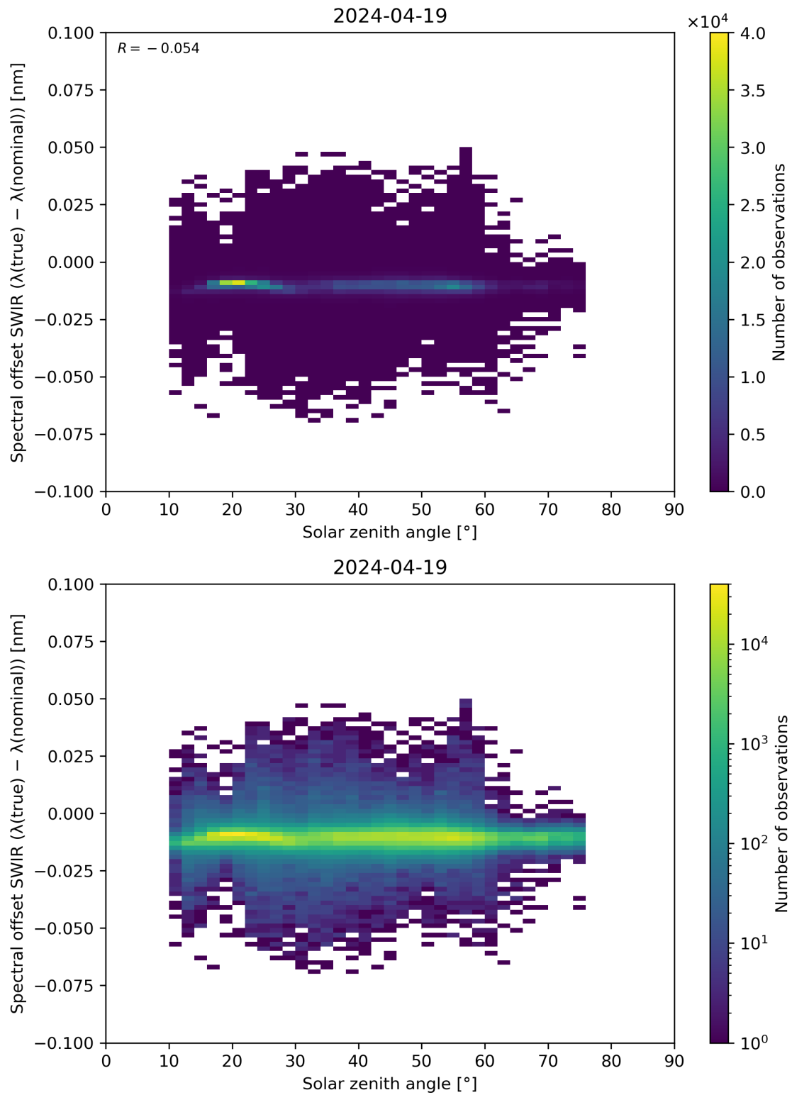
Figure 104: Scatter density plot of “Solar zenith angle” against “Spectral offset SWIR ( \lambda(\text{true}) - \lambda(\text{nominal}) )” for 2024-04-18 to 2024-04-20.
