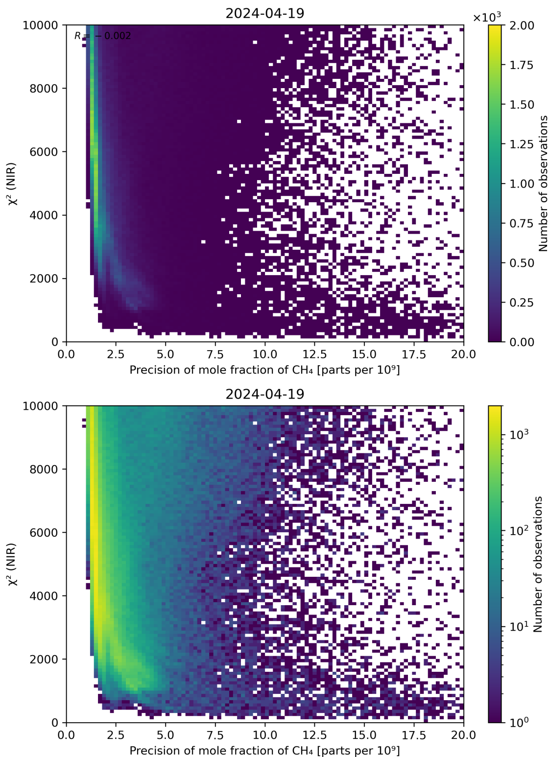
Figure 78: Scatter density plot of “Precision of mole fraction of CH 4 ” against “ \chi^2 (NIR)” for 2024-04-18 to 2024-04-20.
