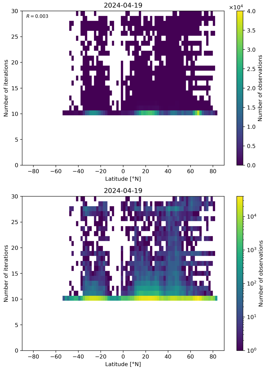
Figure 60: Scatter density plot of “Latitude” against “Number of iterations” for 2024-04-18 to 2024-04-20.
