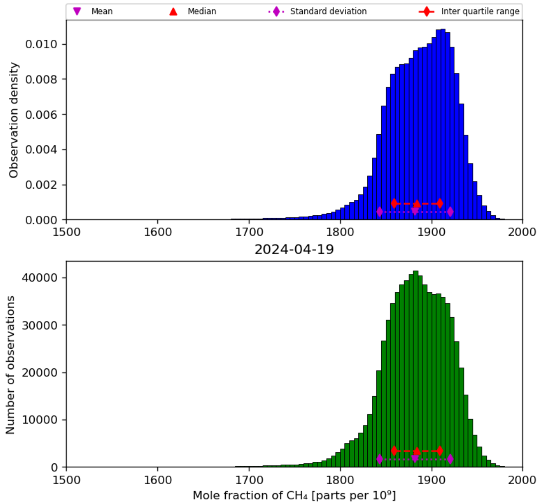
Figure 23: Histogram of "Mole fraction of CH 4 " for 2024-04-18 to 2024-04-20
