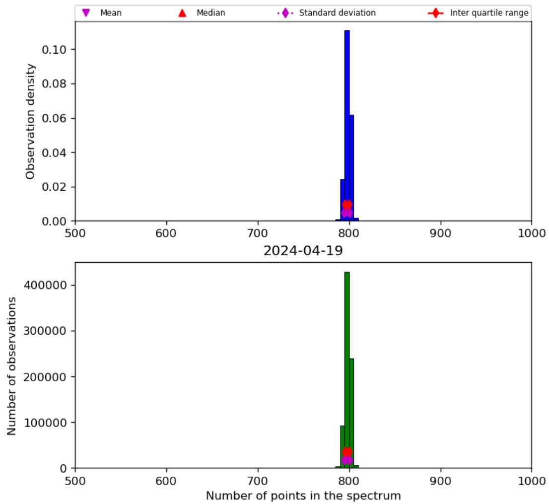
Figure 26: Histogram of “Number of points in the spectrum” for 2024-04-18 to 2024-04-20
