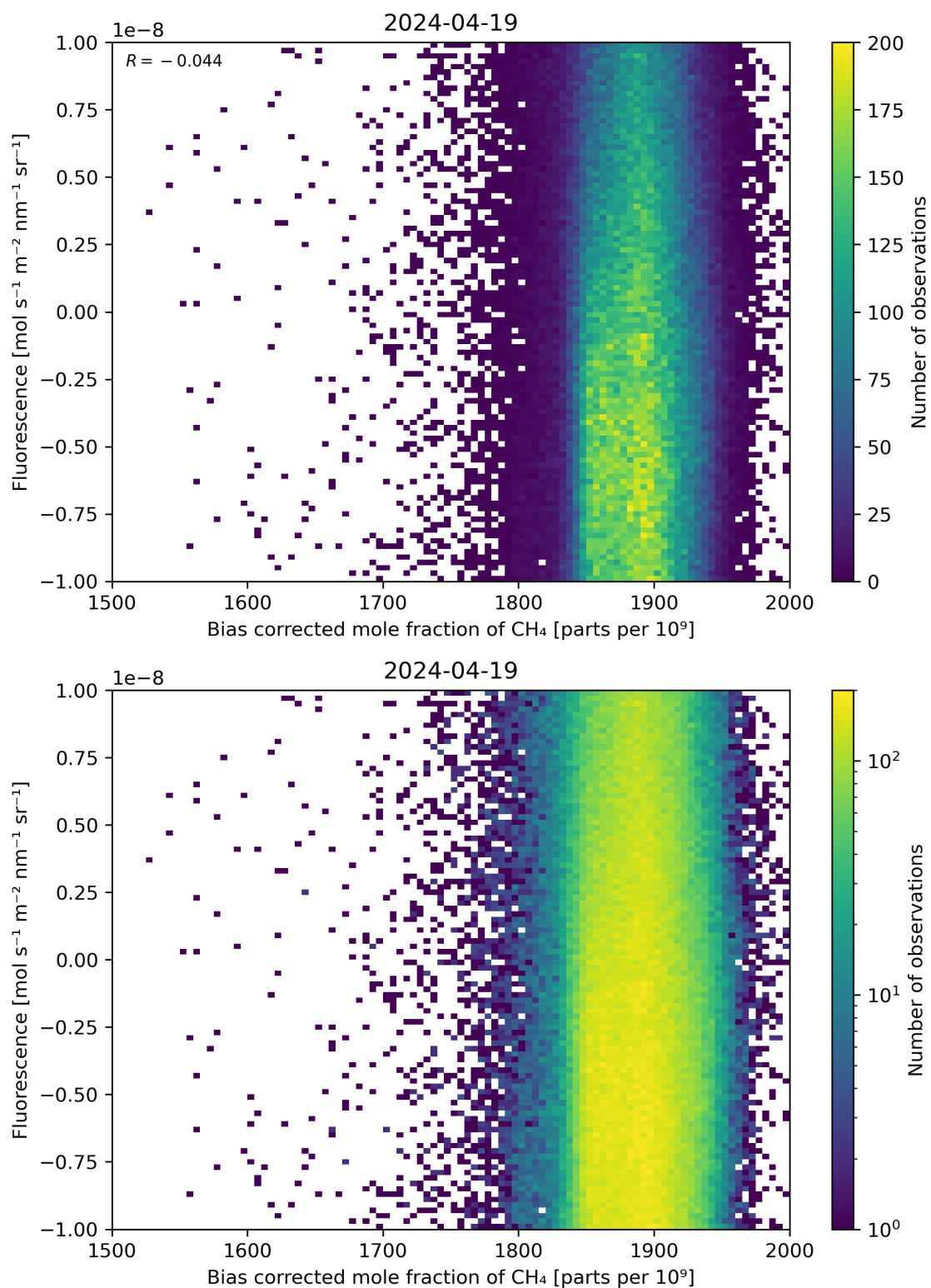
Figure 66: Scatter density plot of “Bias corrected mole fraction of \text{CH}_4 ” against “Fluorescence” for 2024-04-18 to 2024-04-20.
