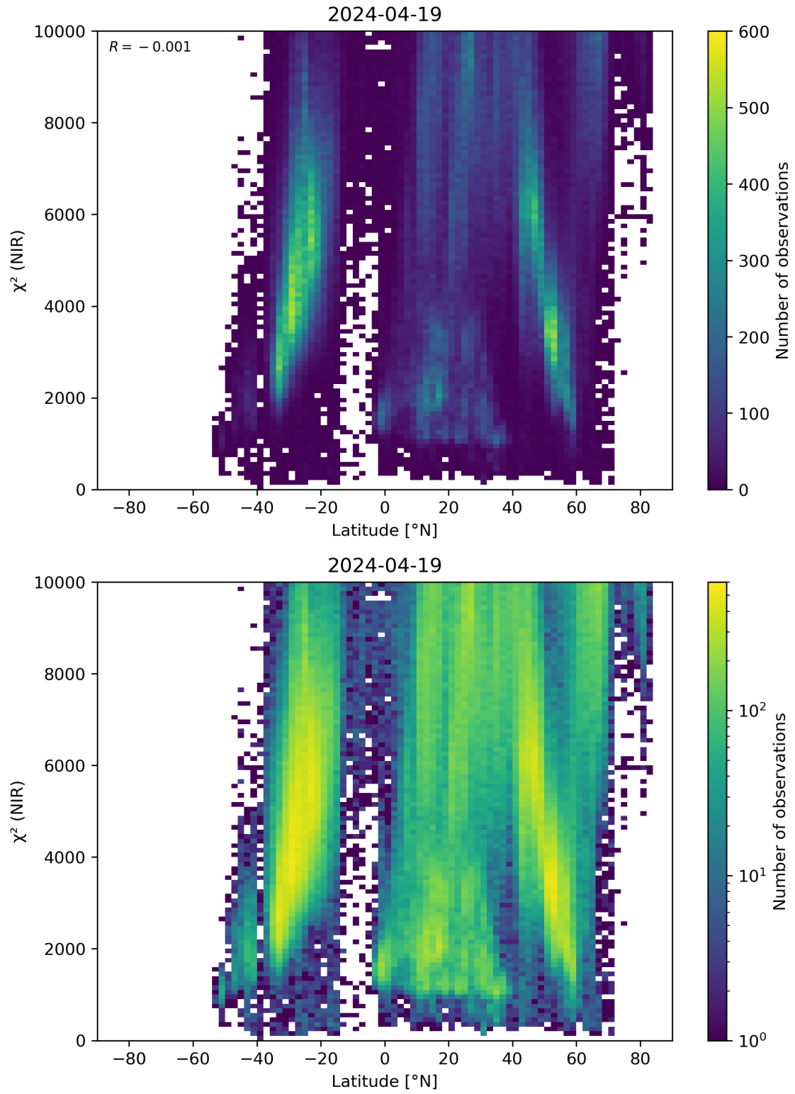
Figure 53: Scatter density plot of “Latitude” against “ \chi^2 (NIR)” for 2024-04-18 to 2024-04-20.
