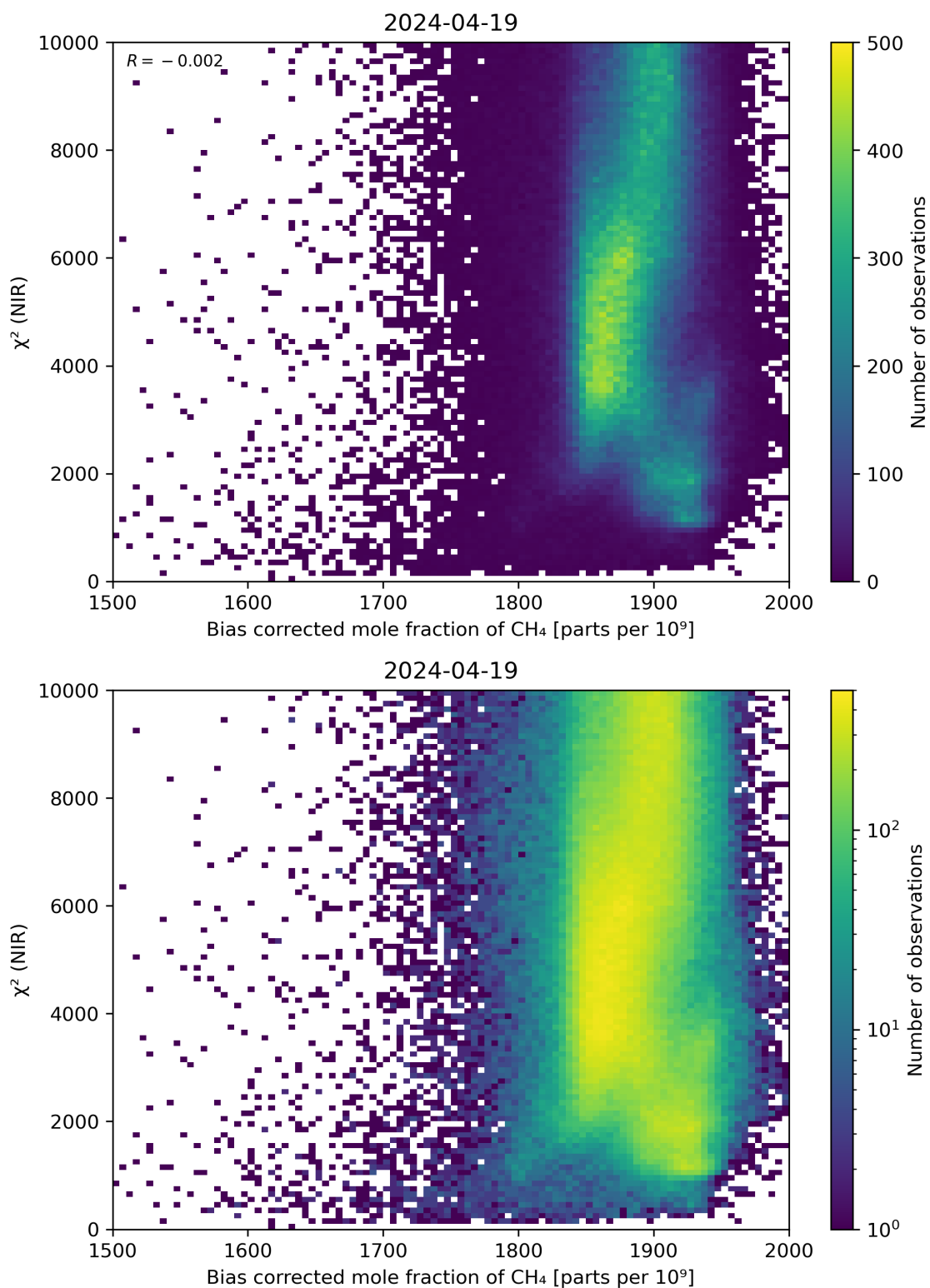
Figure 63: Scatter density plot of “Bias corrected mole fraction of CH 4 ” against “ \chi^2 (NIR)” for 2024-04-18 to 2024-04-20.
