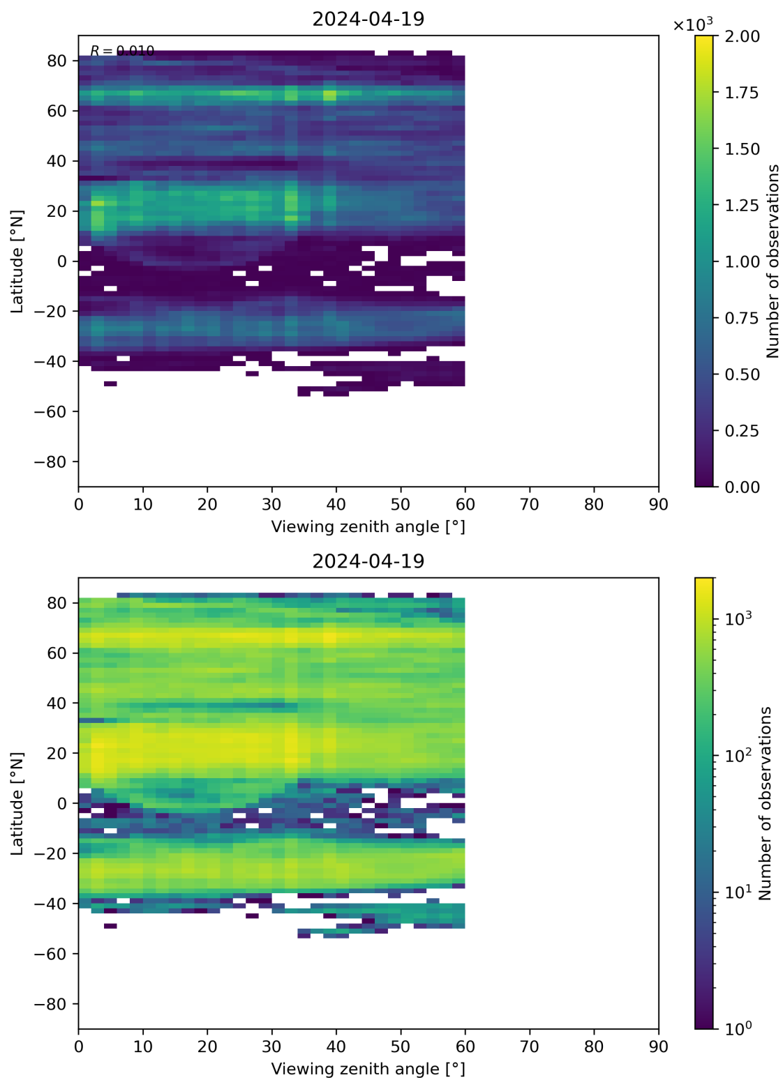
Figure 109: Scatter density plot of “Viewing zenith angle” against “Latitude” for 2024-04-18 to 2024-04-20.
