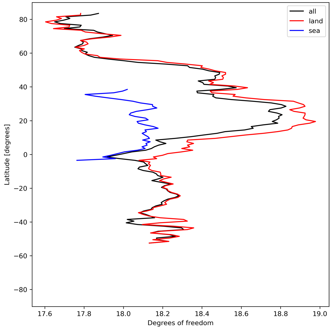
Figure 19: Zonal average of “Degrees of freedom” for 2024-04-18 to 2024-04-20.
