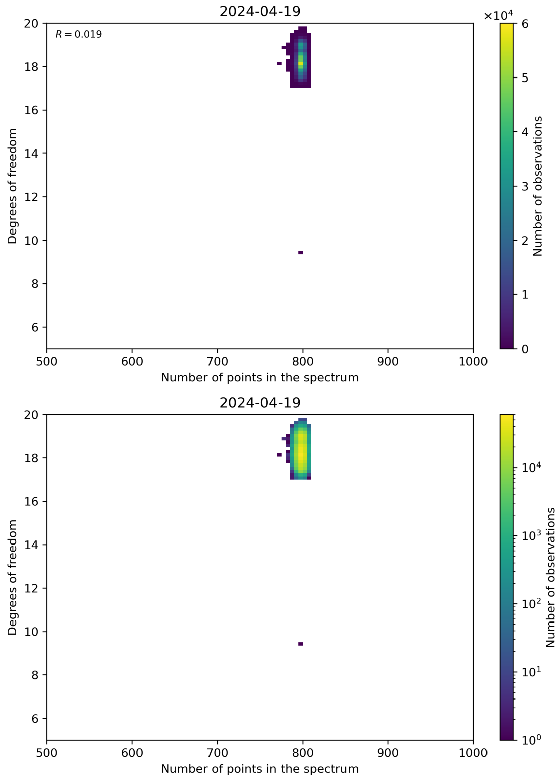
Figure 90: Scatter density plot of “Number of points in the spectrum” against “Degrees of freedom” for 2024-04-18 to 2024-04-20.
