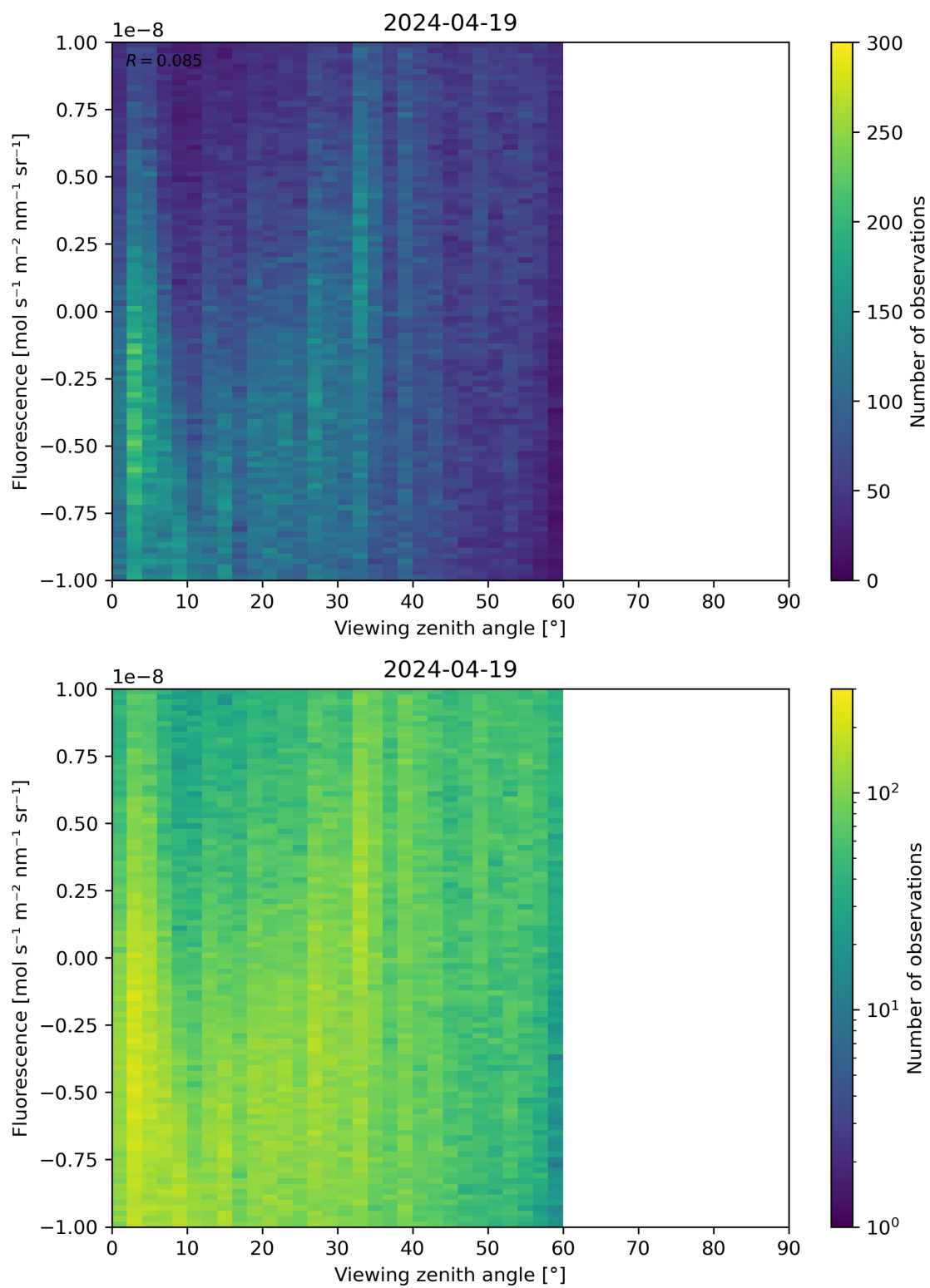
Figure 108: Scatter density plot of “Viewing zenith angle” against “Fluorescence” for 2024-04-18 to 2024-04-20.
