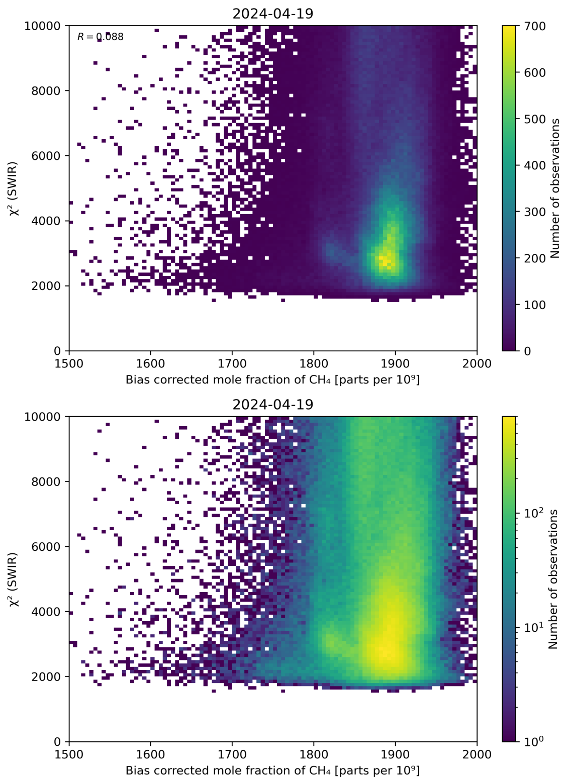
Figure 64: Scatter density plot of “Bias corrected mole fraction of \text{CH}_4 ” against “ \chi^2 (SWIR)” for 2024-04-18 to 2024-04-20.
