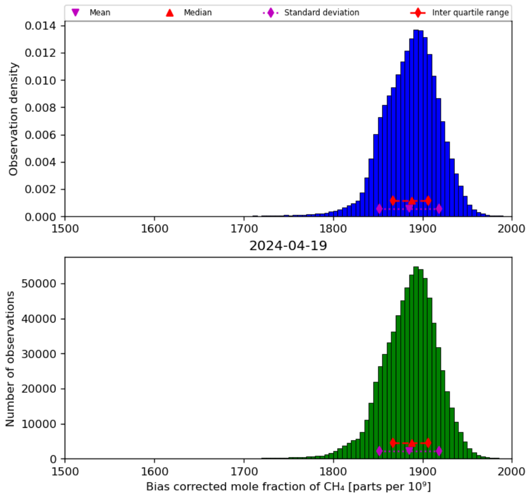
Figure 25: Histogram of “Bias corrected mole fraction of CH 4 ” for 2024-04-18 to 2024-04-20
