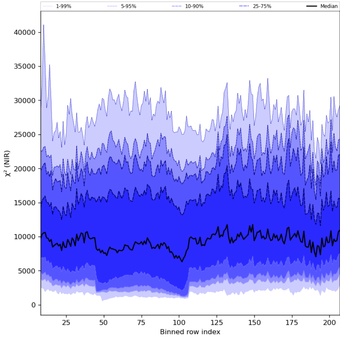
Figure 40: Along track statistics of “ \chi^2 (NIR)” for 2024-04-18 to 2024-04-20
