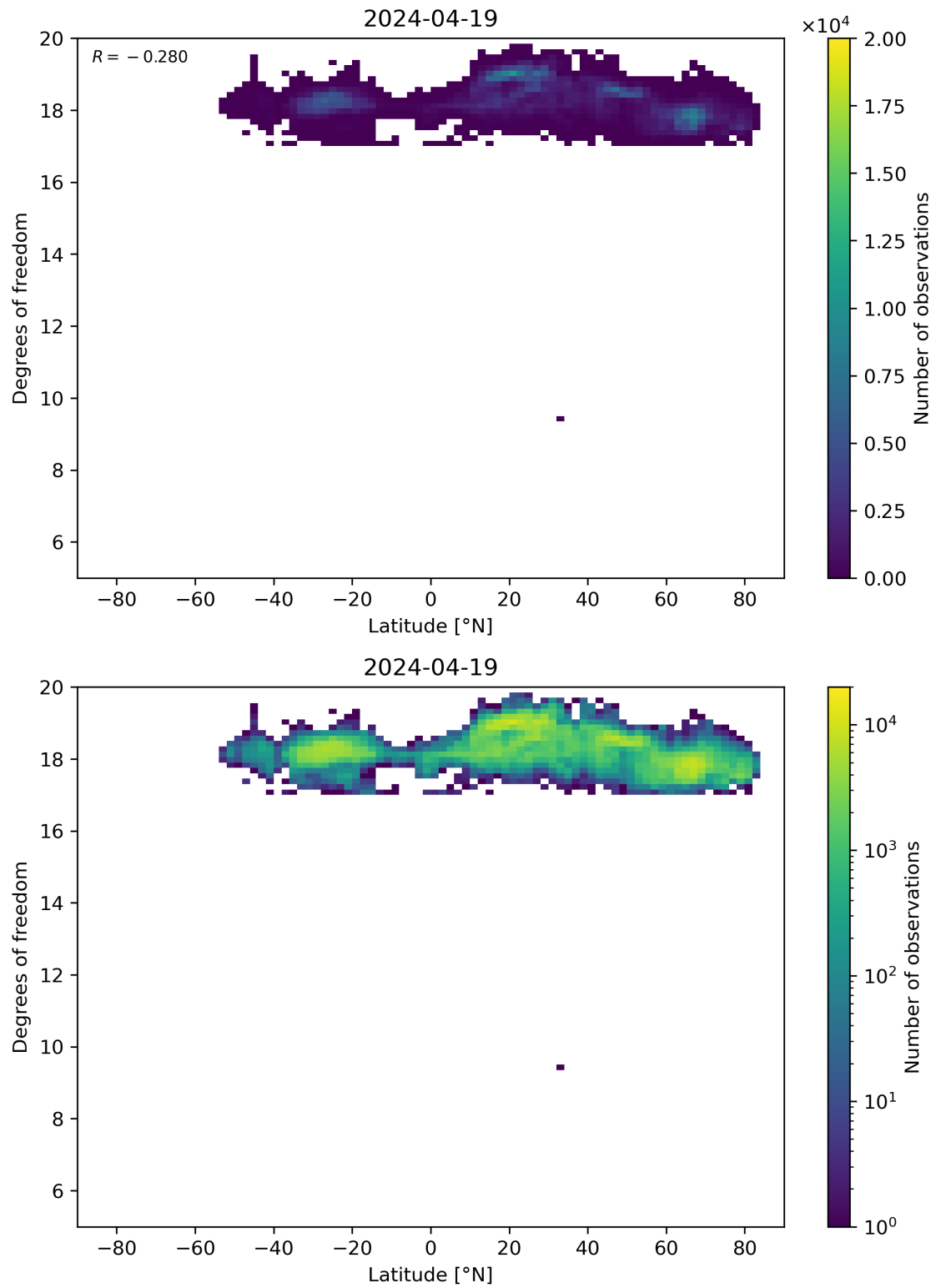
Figure 55: Scatter density plot of “Latitude” against “Degrees of freedom” for 2024-04-18 to 2024-04-20.
