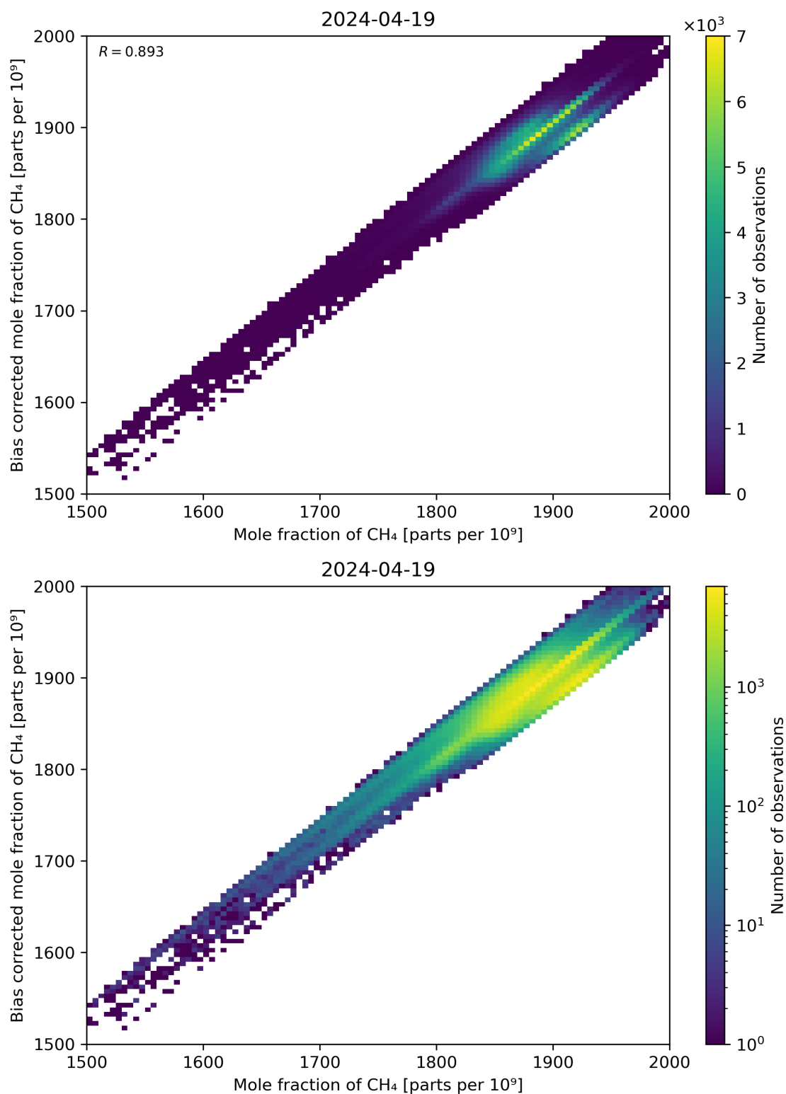
Figure 74: Scatter density plot of “Mole fraction of CH 4 ” against “Bias corrected mole fraction of CH 4 ” for 2024-04-18 to 2024-04-20.
