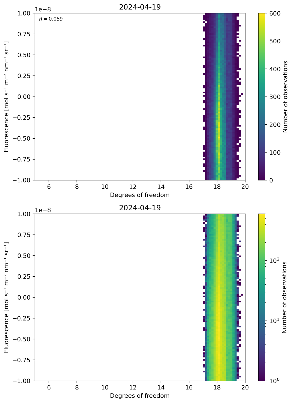
Figure 51: Scatter density plot of “Degrees of freedom” against “Fluorescence” for 2024-04-18 to 2024-04-20.
