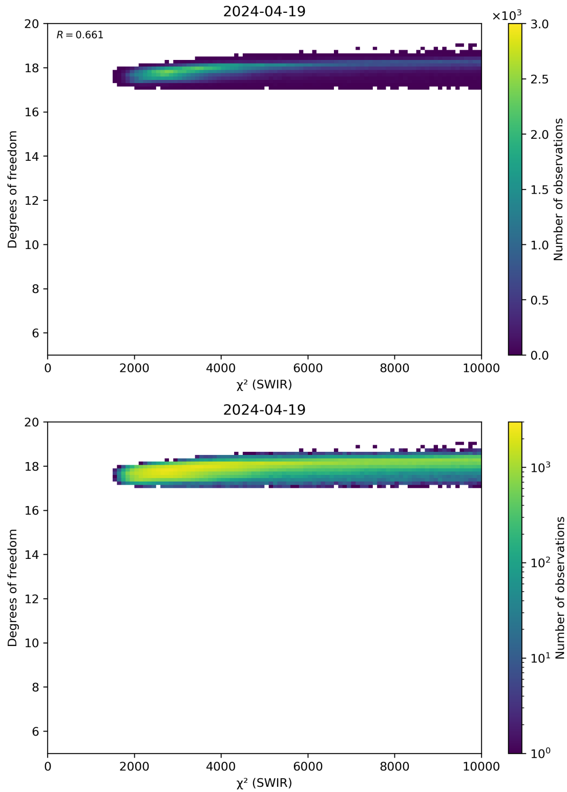
Figure 48: Scatter density plot of “ \chi^2 (SWIR)” against “Degrees of freedom” for 2024-04-18 to 2024-04-20.
