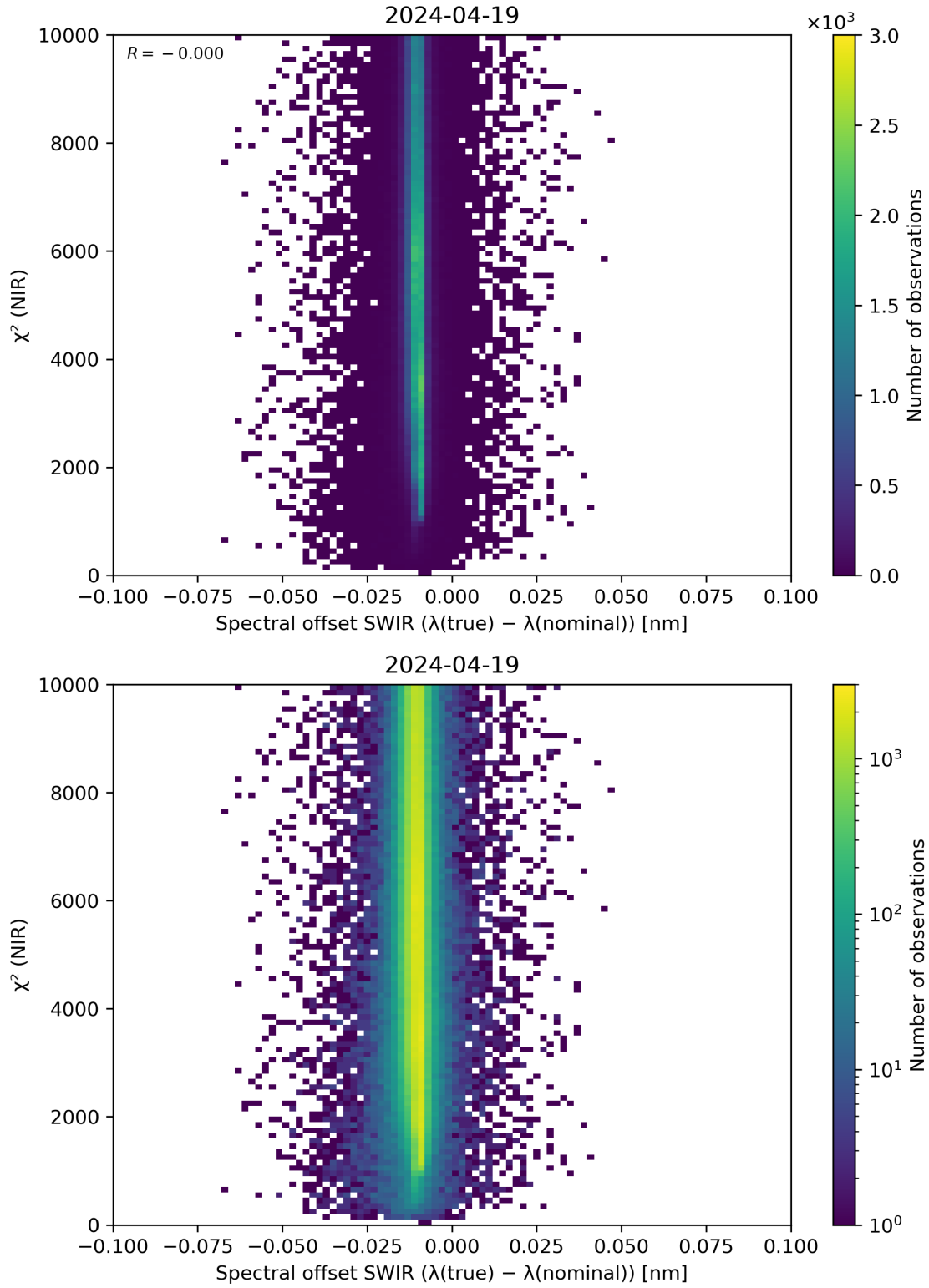
Figure 117: Scatter density plot of “Spectral offset SWIR ( \lambda(\text{true}) - \lambda(\text{nominal}) )” against “ \chi^2 (NIR)” for 2024-04-18 to 2024-04-20.
