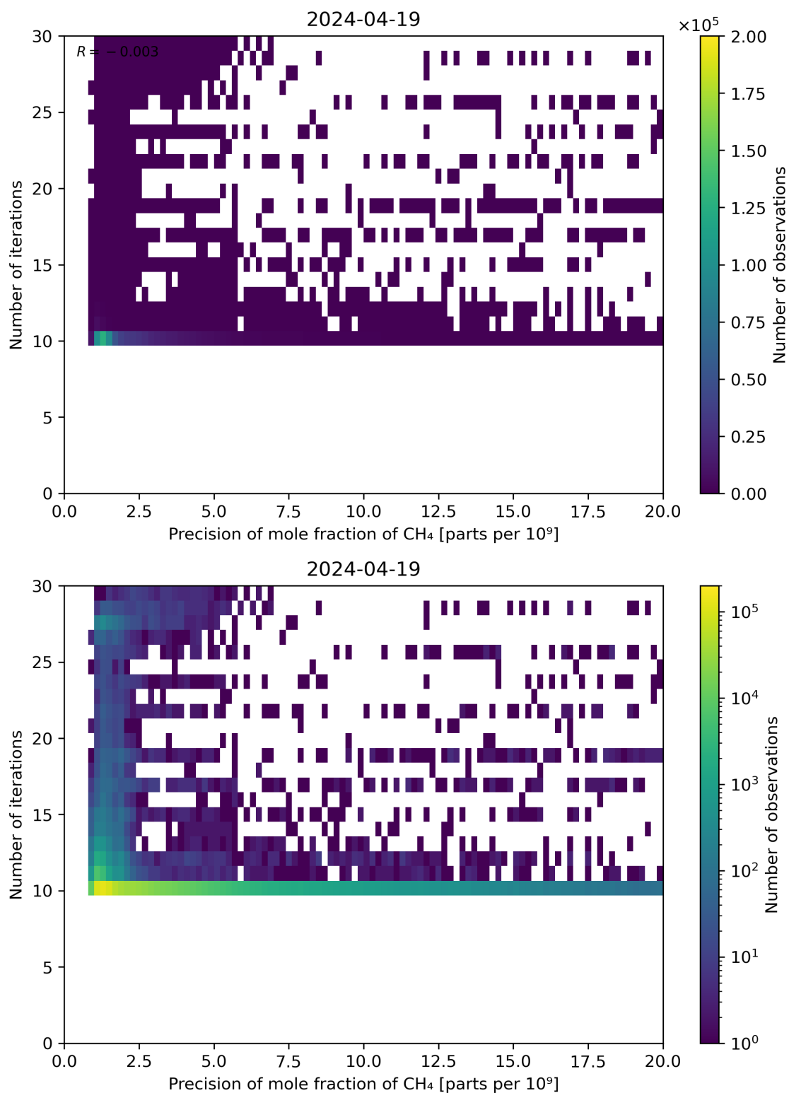
Figure 83: Scatter density plot of “Precision of mole fraction of CH 4 ” against “Number of iterations” for 2024-04-18 to 2024-04-20.
