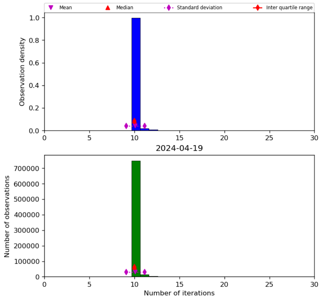
Figure 31: Histogram of “Number of iterations” for 2024-04-18 to 2024-04-20
