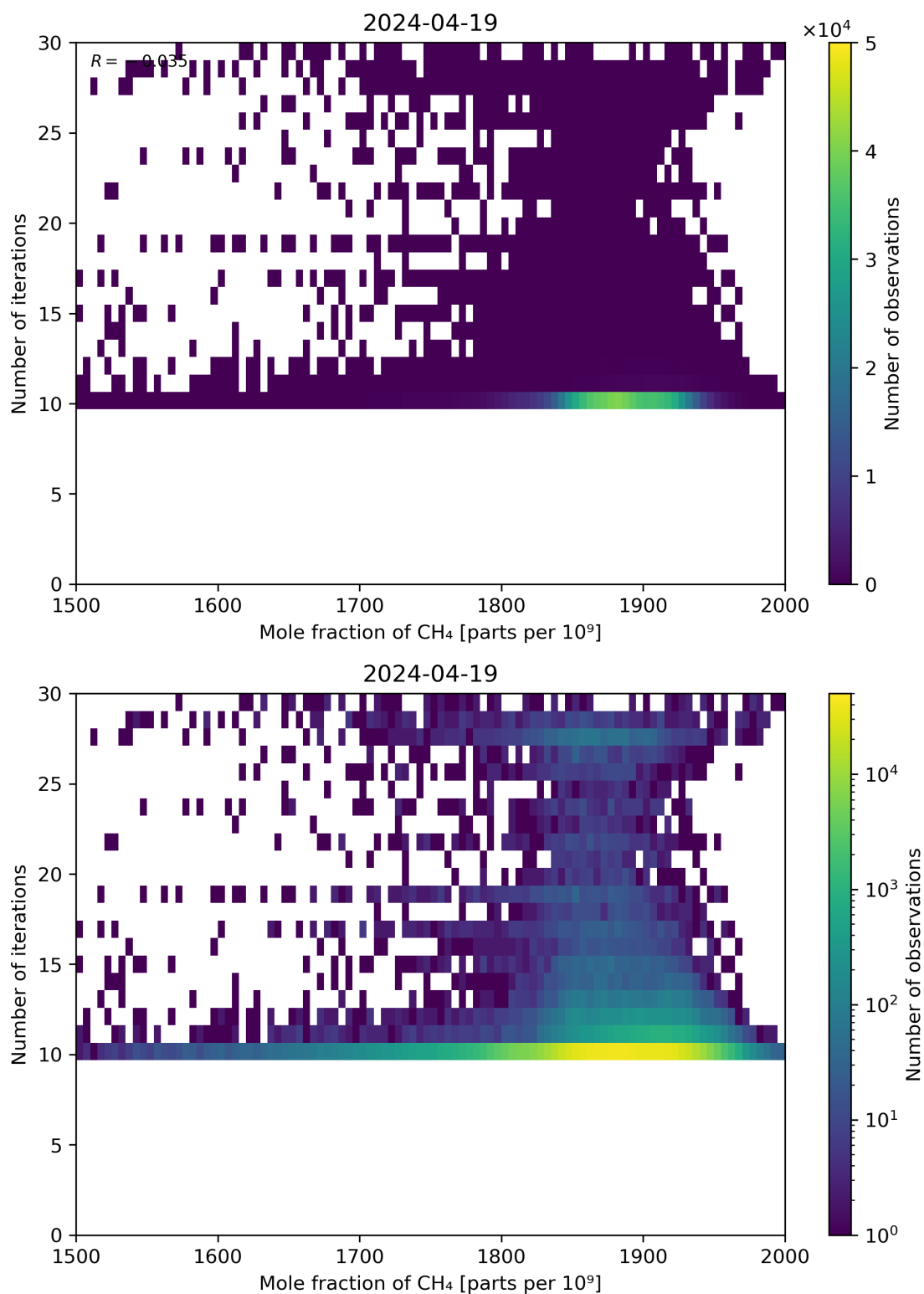
Figure 76: Scatter density plot of “Mole fraction of CH 4 ” against “Number of iterations” for 2024-04-18 to 2024-04-20.
