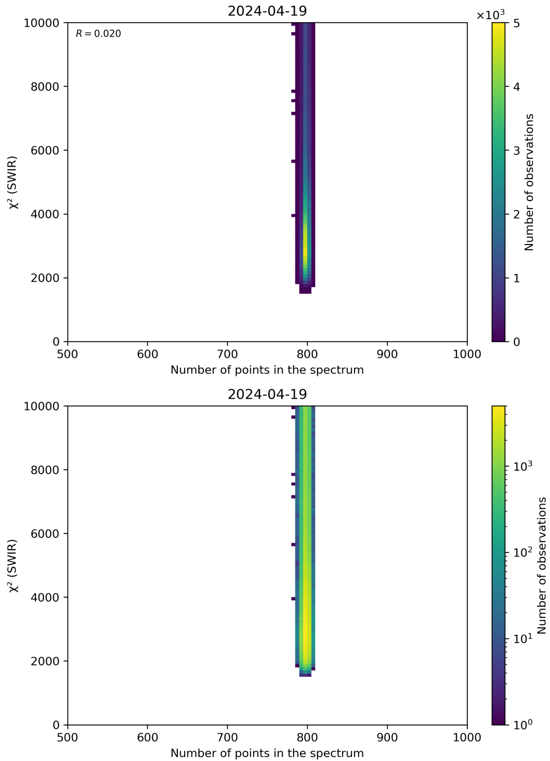
Figure 89: Scatter density plot of “Number of points in the spectrum” against “ \chi^2 (SWIR)” for 2024-04-18 to 2024-04-20.
