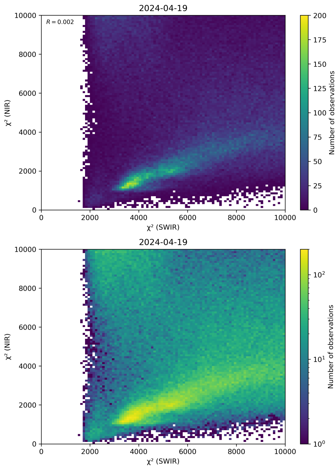
Figure 47: Scatter density plot of “ \chi^2 (SWIR)” against “ \chi^2 (NIR)” for 2024-04-18 to 2024-04-20.
