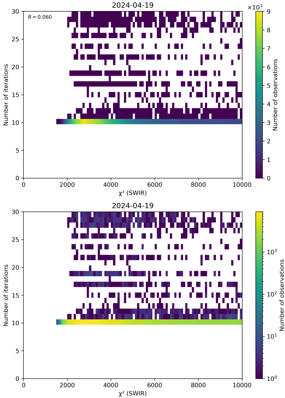
Figure 50: Scatter density plot of “ \chi^2 (SWIR)” against “Number of iterations” for 2024-04-18 to 2024-04-20.
