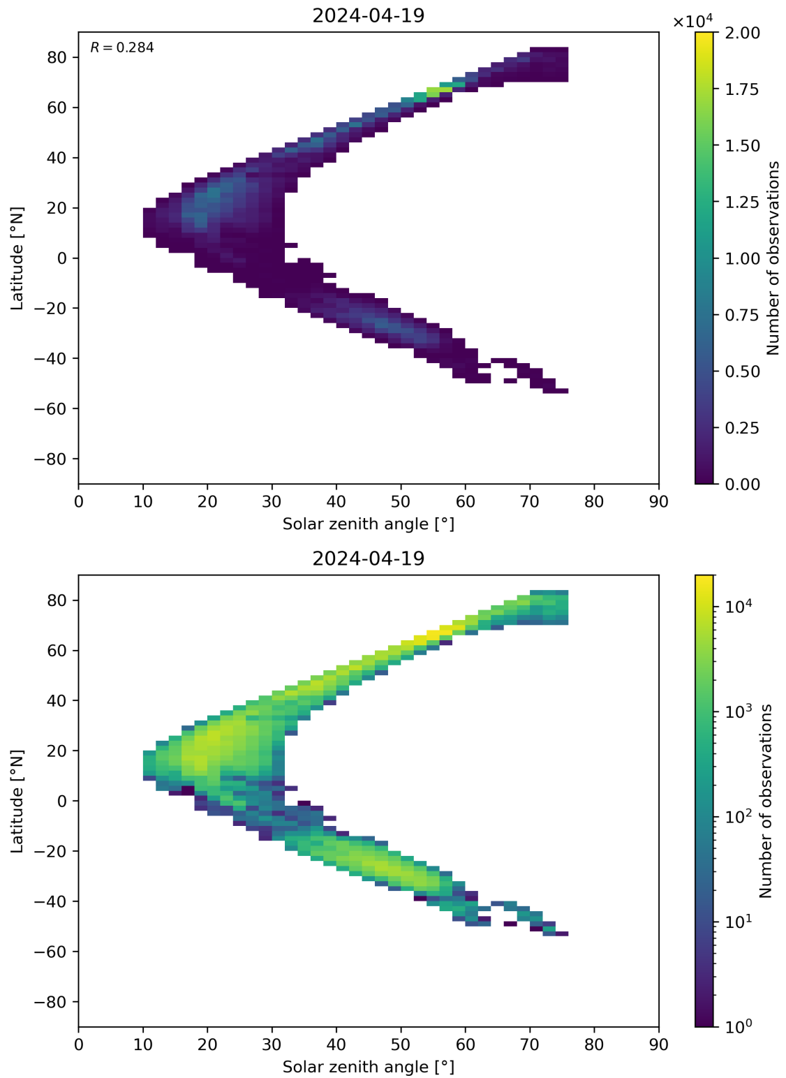
Figure 98: Scatter density plot of “Solar zenith angle” against “Latitude” for 2024-04-18 to 2024-04-20.
