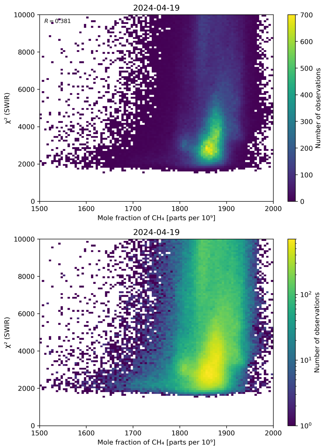
Figure 71: Scatter density plot of “Mole fraction of CH 4 ” against “ \chi^2 (SWIR)” for 2024-04-18 to 2024-04-20.
