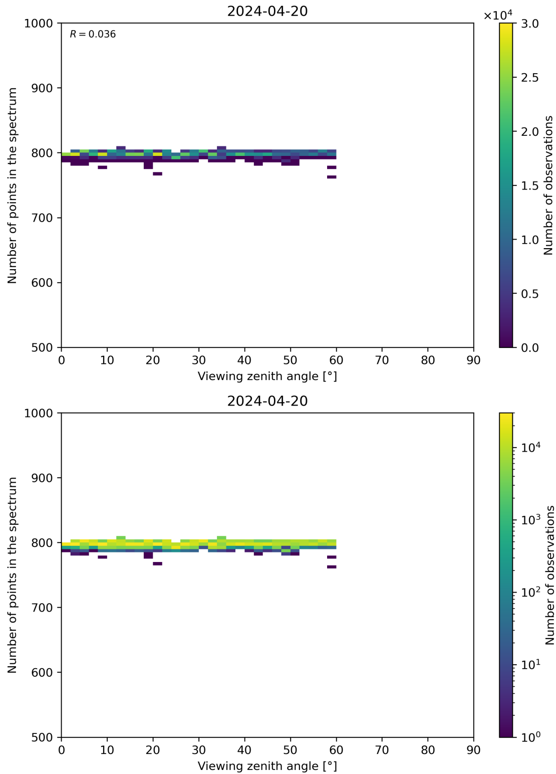
Figure 114: Scatter density plot of “Viewing zenith angle” against “Number of points in the spectrum” for 2024-04-19 to 2024-04-21.
