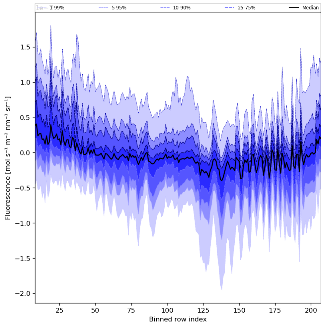
Figure 43: Along track statistics of “Fluorescence” for 2024-04-19 to 2024-04-21
