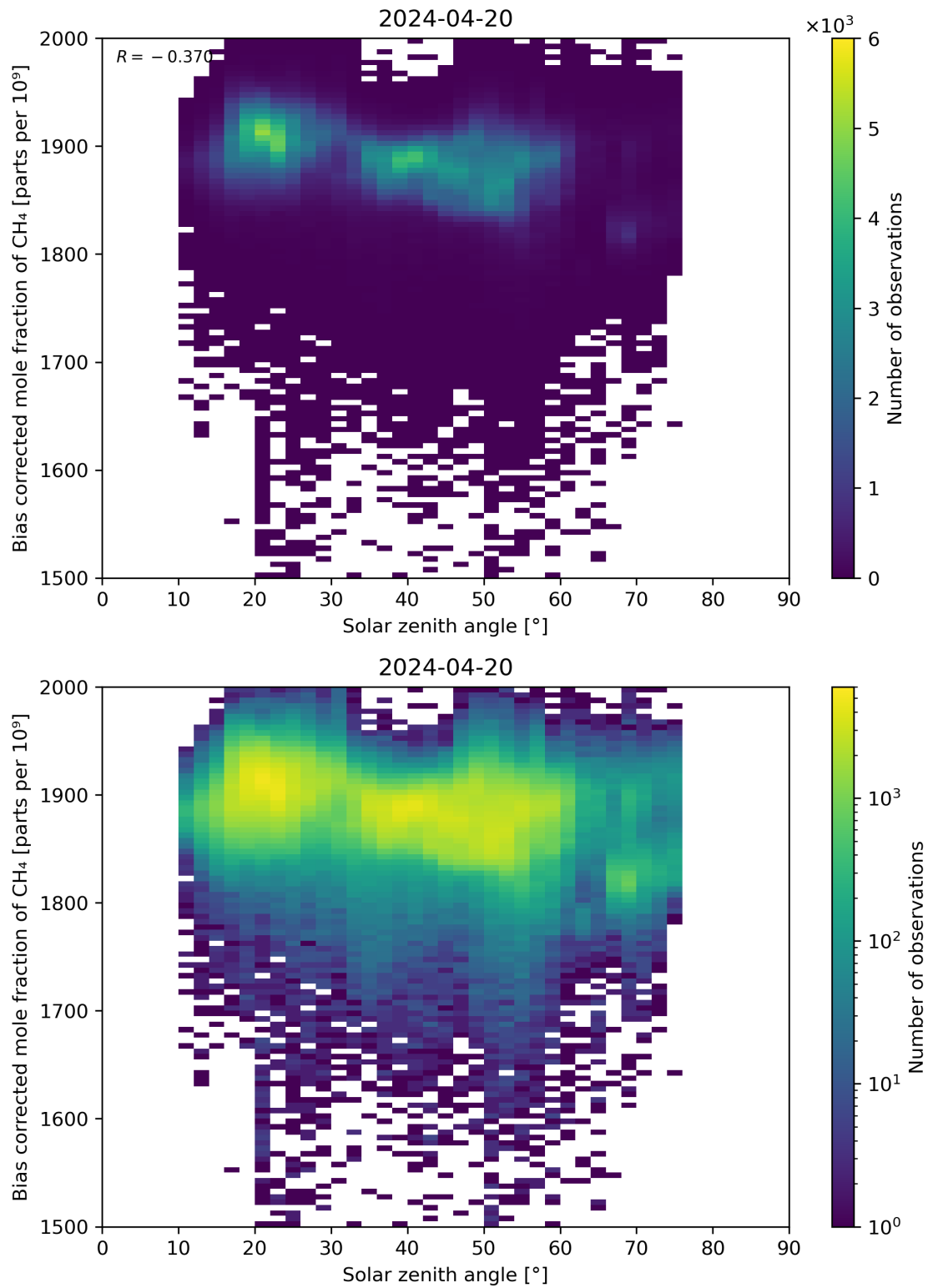
Figure 100: Scatter density plot of “Solar zenith angle” against “Bias corrected mole fraction of \text{CH}_4 ” for 2024-04-19 to 2024-04-21.
