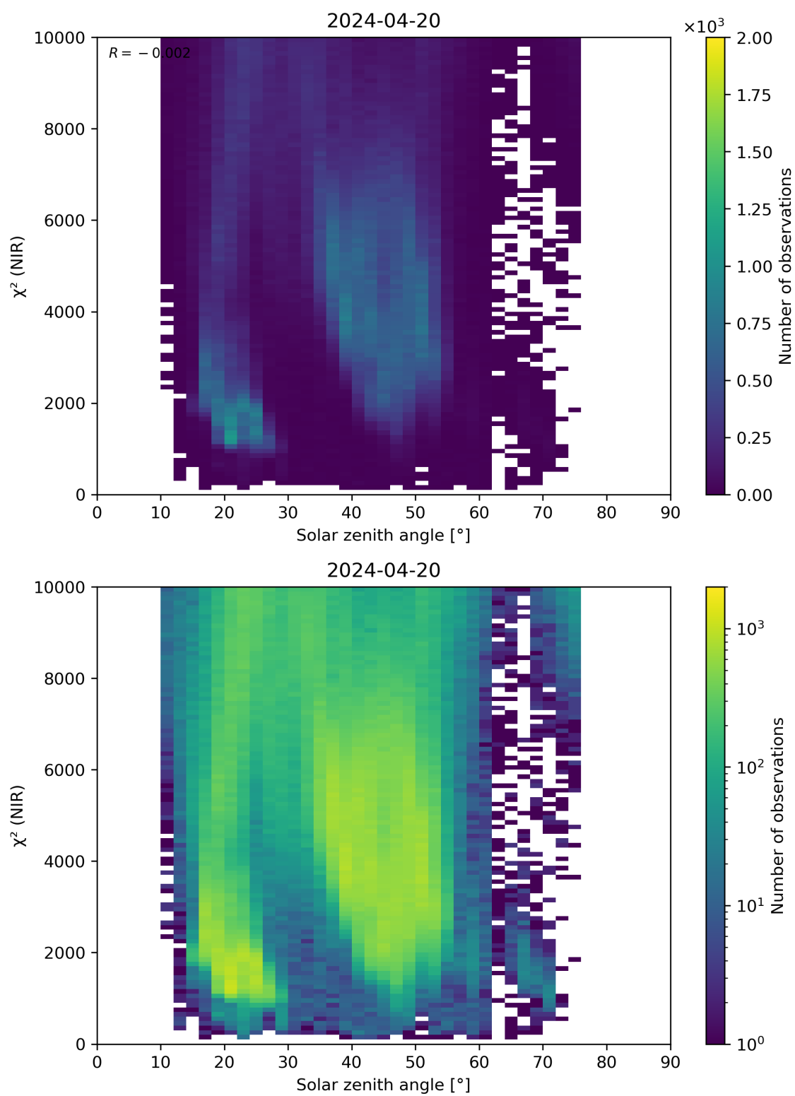
Figure 94: Scatter density plot of “Solar zenith angle” against “ \chi^2 (NIR)” for 2024-04-19 to 2024-04-21.
