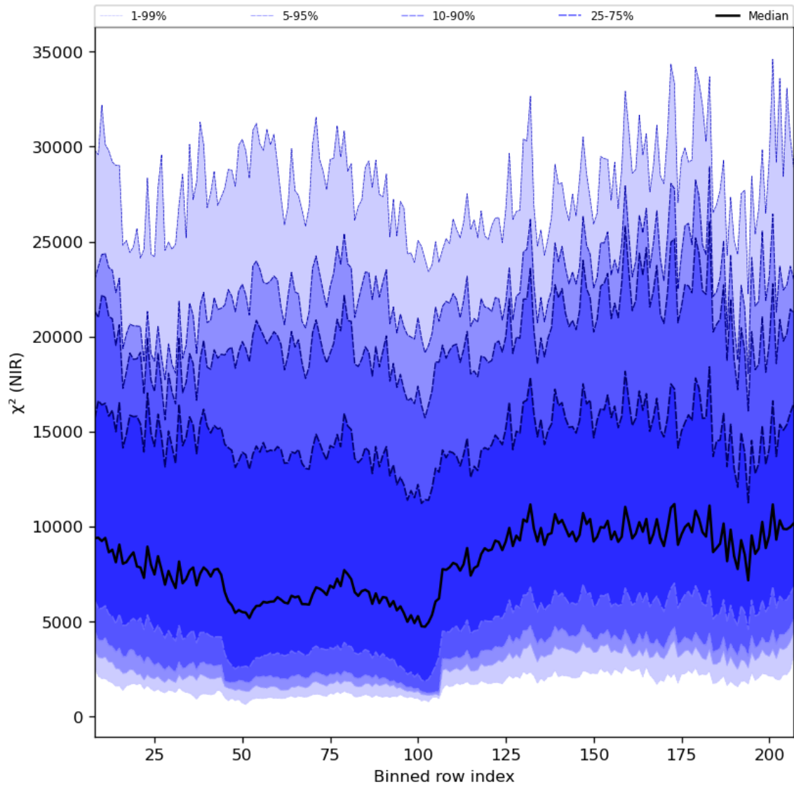
Figure 40: Along track statistics of “ \chi^2 (NIR)” for 2024-04-19 to 2024-04-21
