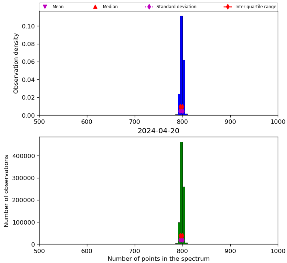
Figure 26: Histogram of “Number of points in the spectrum” for 2024-04-19 to 2024-04-21
