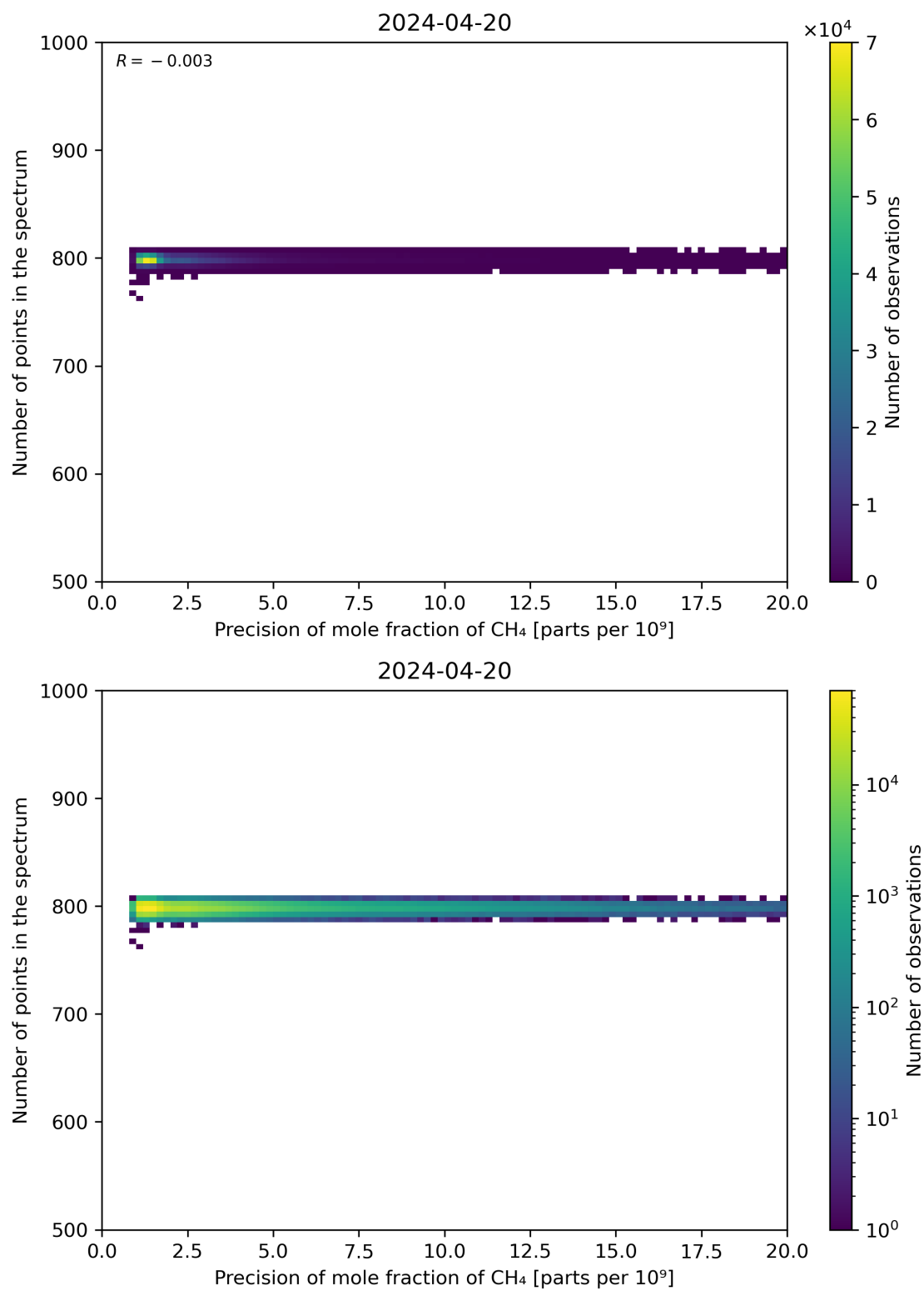
Figure 84: Scatter density plot of “Precision of mole fraction of CH 4 ” against “Number of points in the spectrum” for 2024-04-19 to 2024-04-21.
