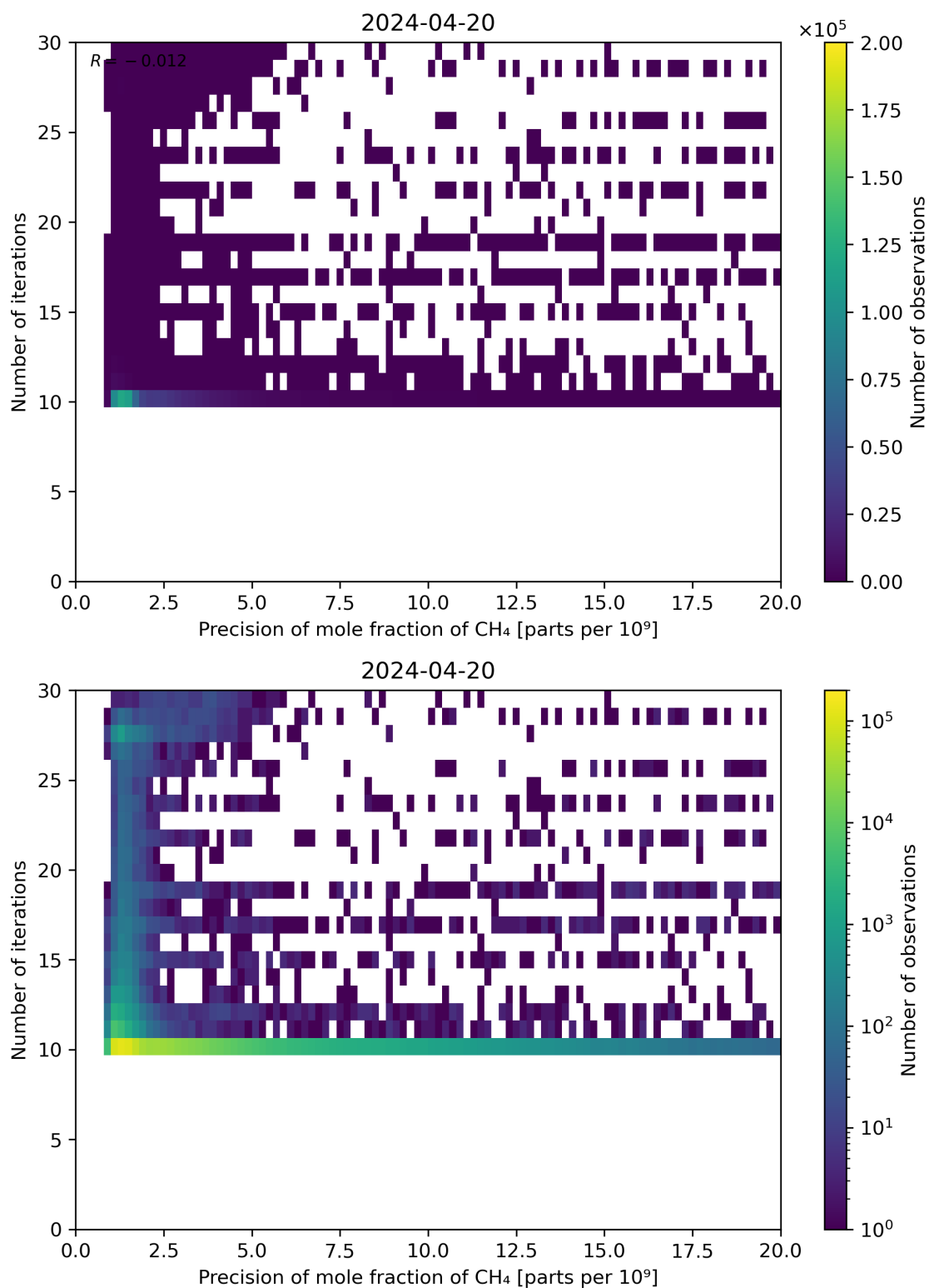
Figure 83: Scatter density plot of “Precision of mole fraction of CH 4 ” against “Number of iterations” for 2024-04-19 to 2024-04-21.
