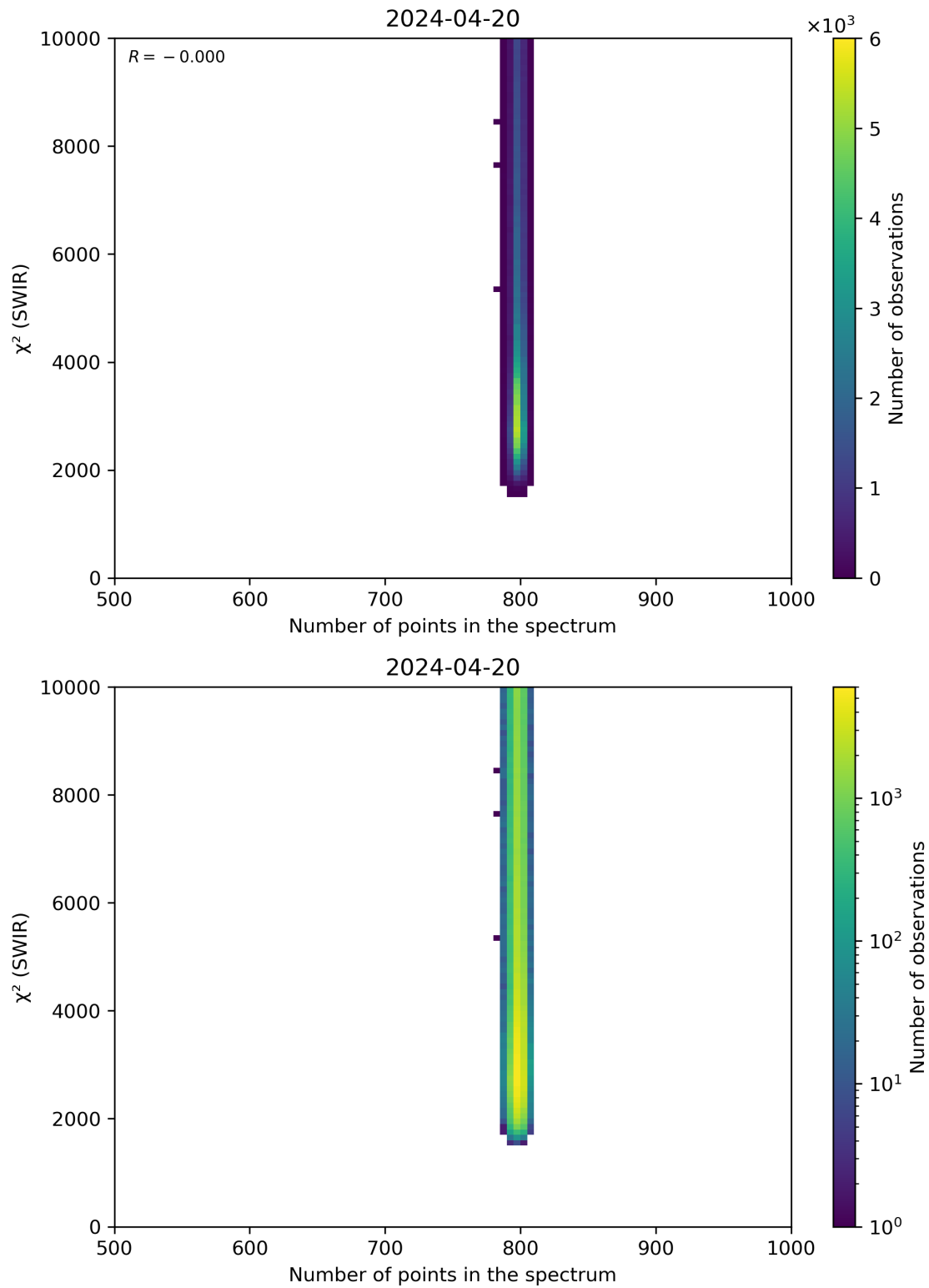
Figure 89: Scatter density plot of “Number of points in the spectrum” against “ \chi^2 (SWIR)” for 2024-04-19 to 2024-04-21.
