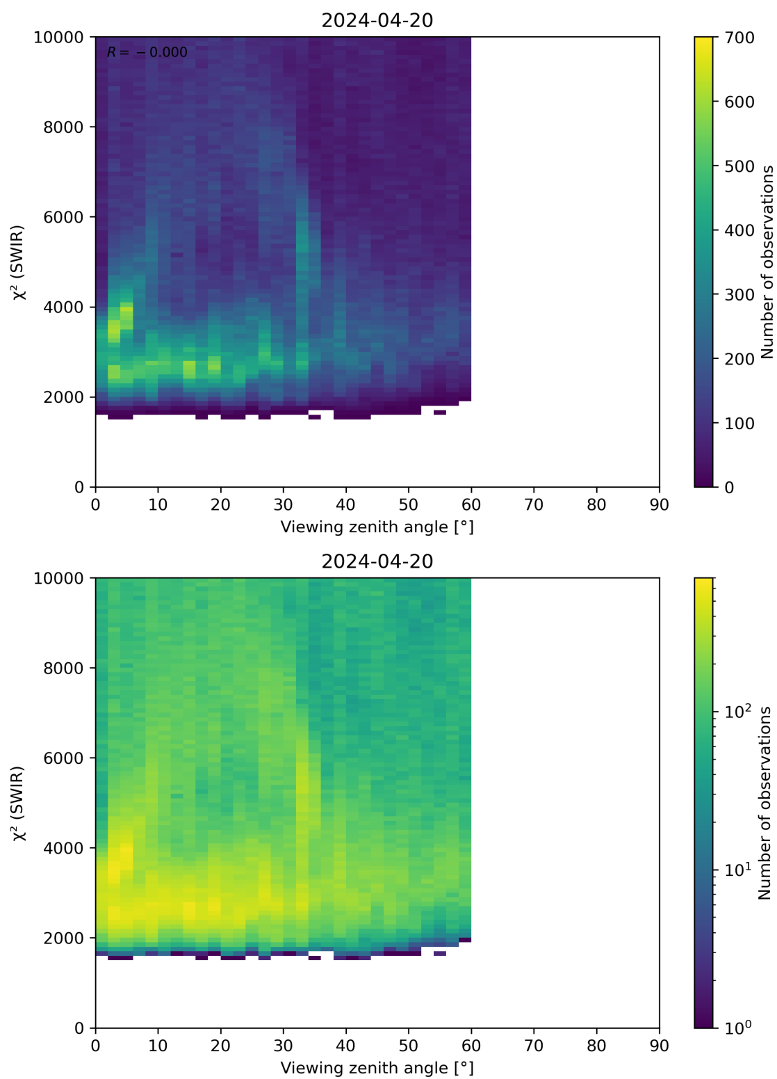
Figure 106: Scatter density plot of “Viewing zenith angle” against “ \chi^2 (SWIR)” for 2024-04-19 to 2024-04-21.
