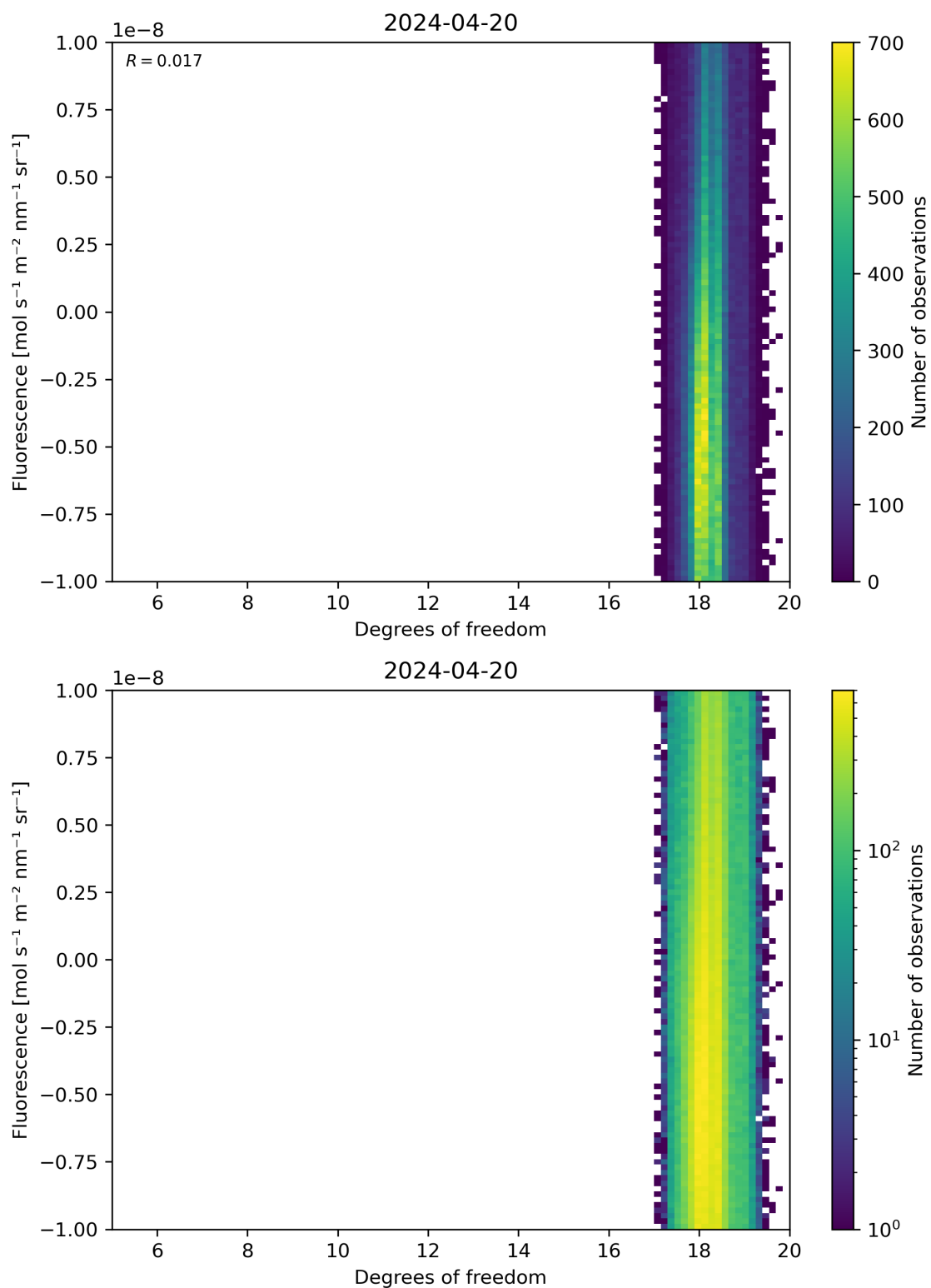
Figure 51: Scatter density plot of “Degrees of freedom” against “Fluorescence” for 2024-04-19 to 2024-04-21.
