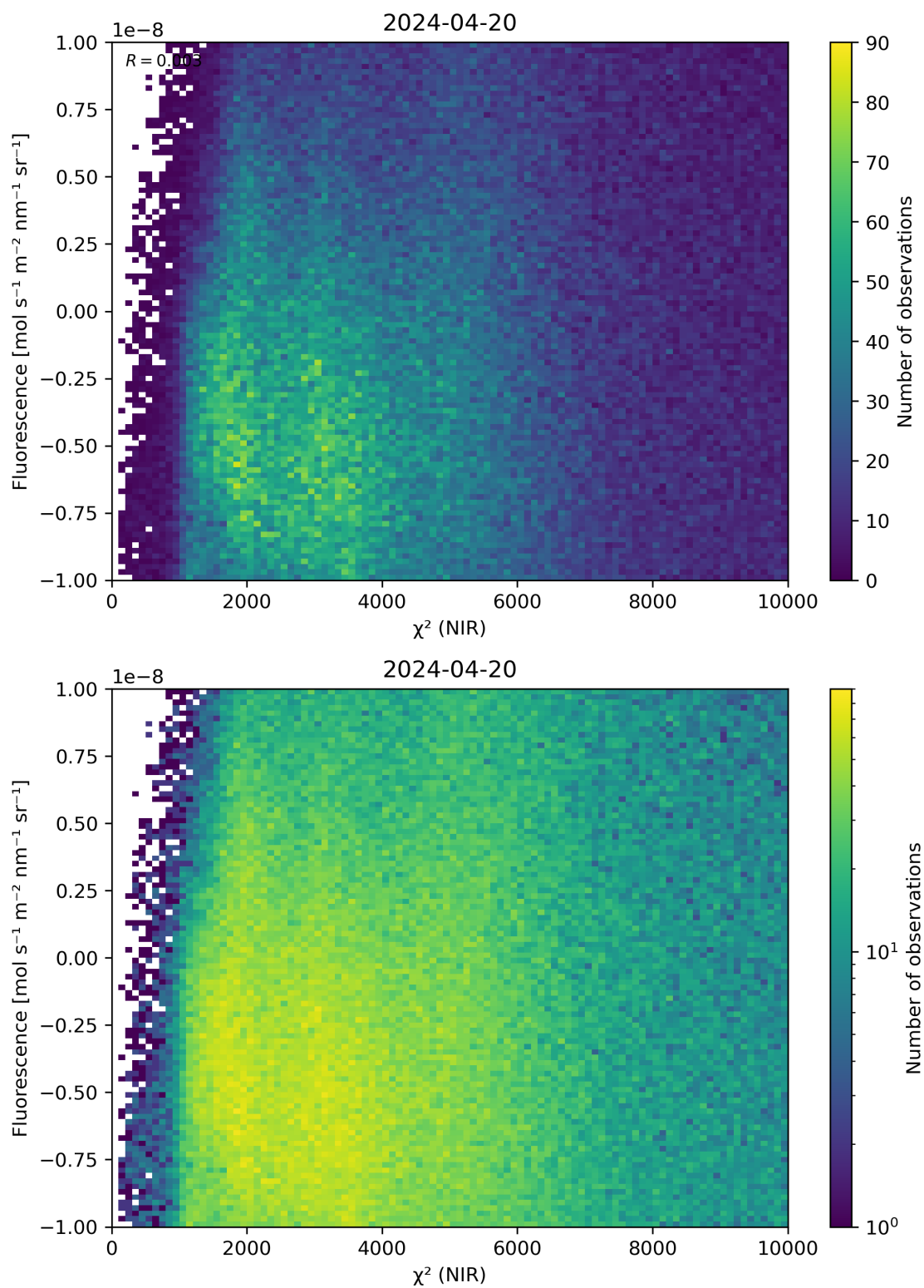
Figure 45: Scatter density plot of “ \chi^2 (NIR)” against “Fluorescence” for 2024-04-19 to 2024-04-21.
