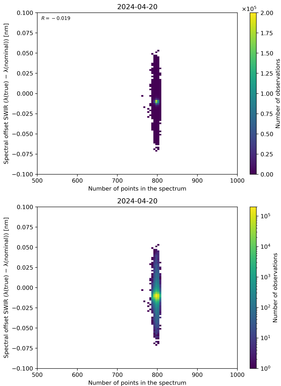
Figure 93: Scatter density plot of “Number of points in the spectrum” against “Spectral offset SWIR ( \lambda(\text{true}) - \lambda(\text{nominal}) )” for 2024-04-19 to 2024-04-21.
