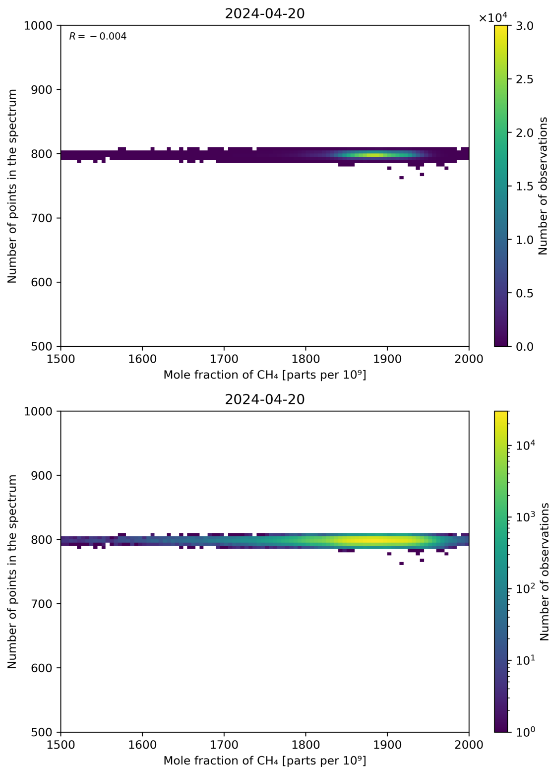
Figure 77: Scatter density plot of “Mole fraction of CH 4 ” against “Number of points in the spectrum” for 2024-04-19 to 2024-04-21.
