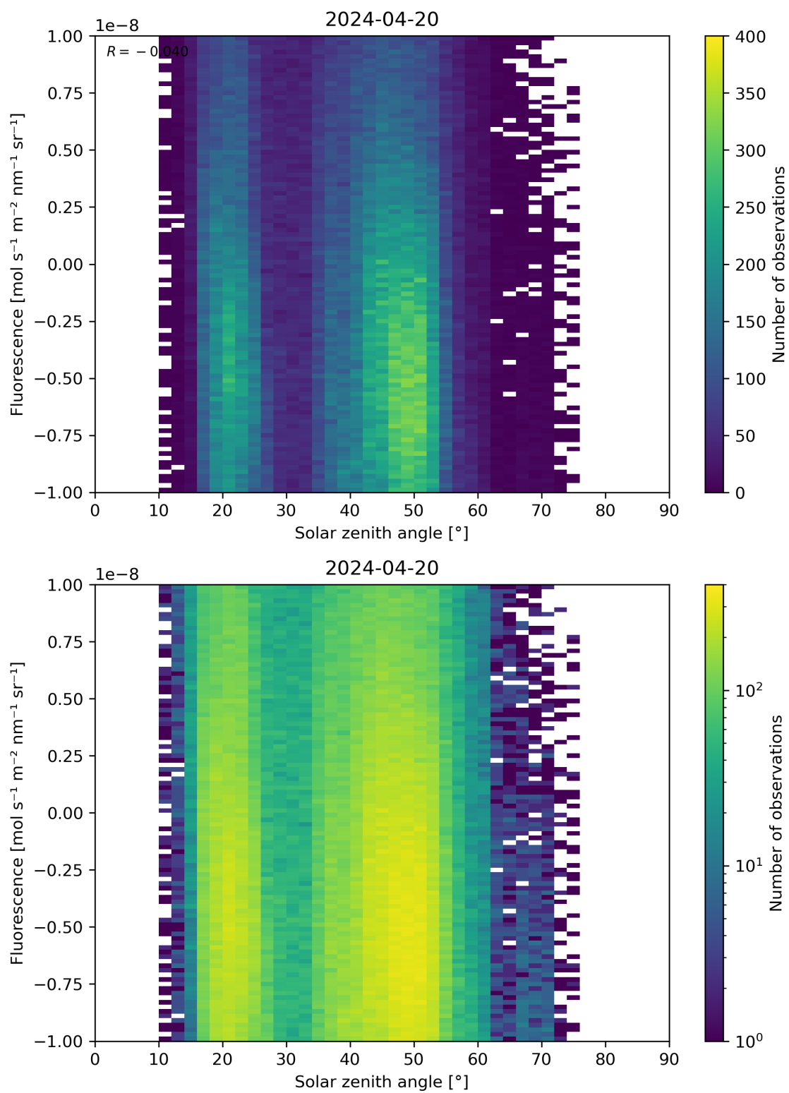
Figure 97: Scatter density plot of “Solar zenith angle” against “Fluorescence” for 2024-04-19 to 2024-04-21.
