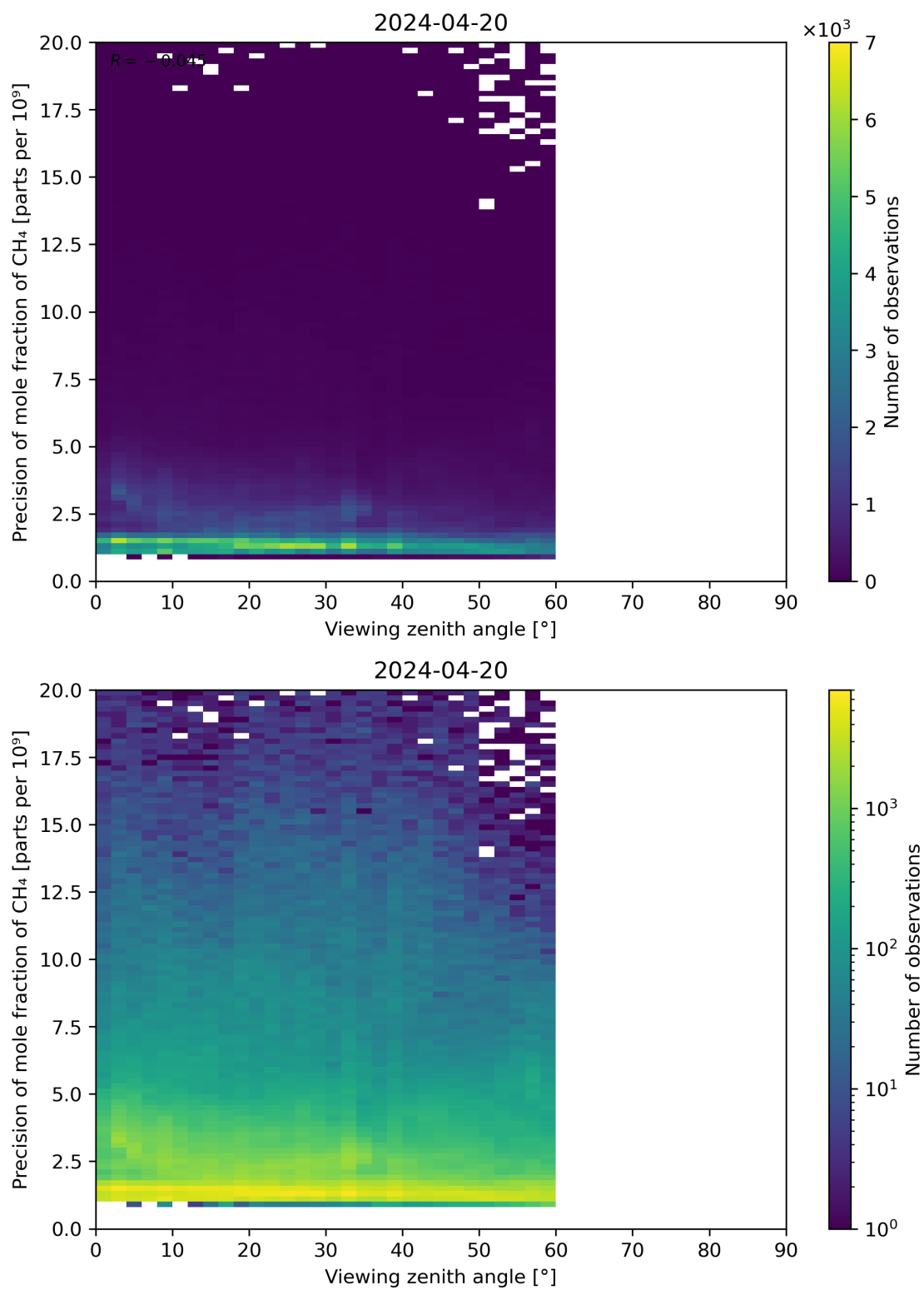
Figure 112: Scatter density plot of “Viewing zenith angle” against “Precision of mole fraction of CH 4 ” for 2024-04-19 to 2024-04-21.
