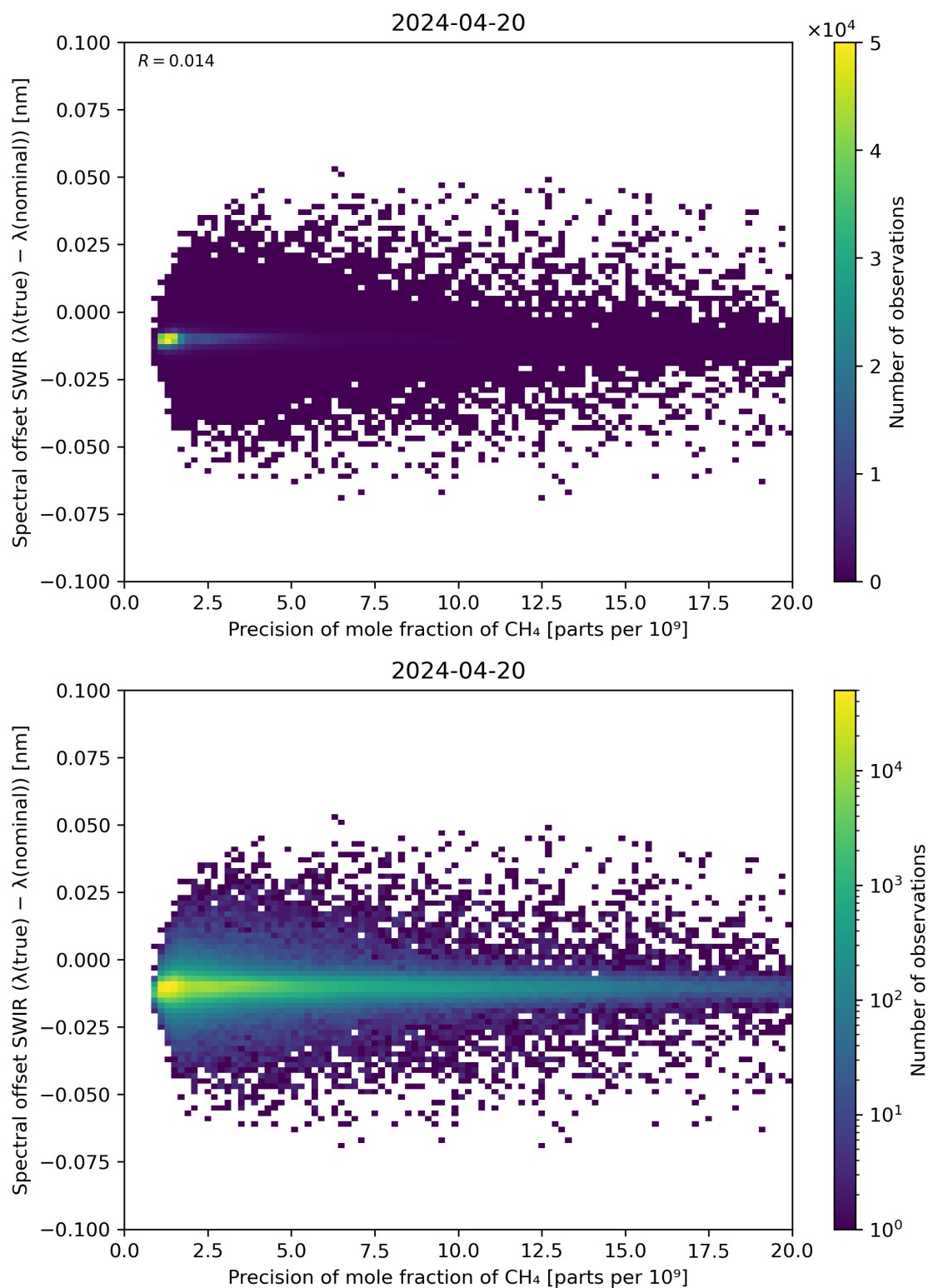
Figure 85: Scatter density plot of “Precision of mole fraction of CH 4 ” against “Spectral offset SWIR ( \lambda(\text{true}) - \lambda(\text{nominal}) )” for 2024-04-19 to 2024-04-21.
