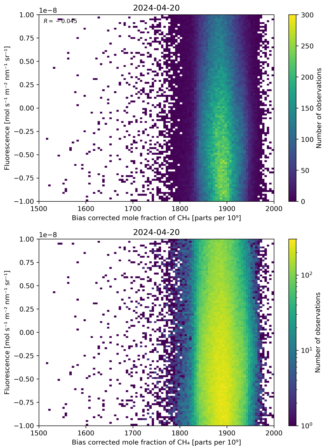
Figure 66: Scatter density plot of “Bias corrected mole fraction of CH 4 ” against “Fluorescence” for 2024-04-19 to 2024-04-21.
