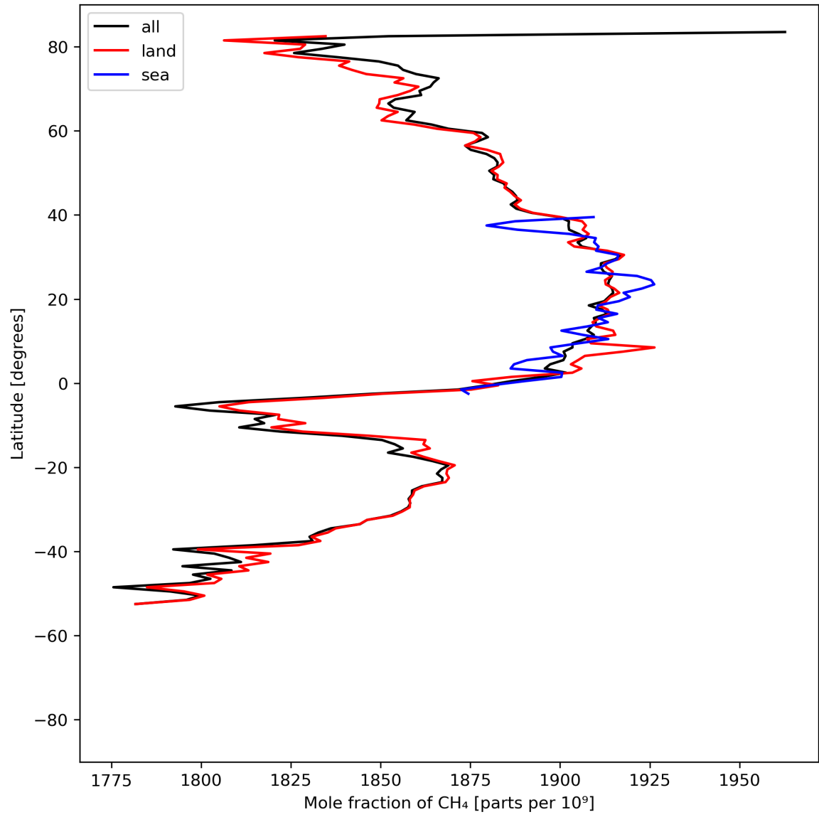
Figure 12: Zonal average of “Mole fraction of \text{CH}_4 ” for 2024-04-19 to 2024-04-21.
