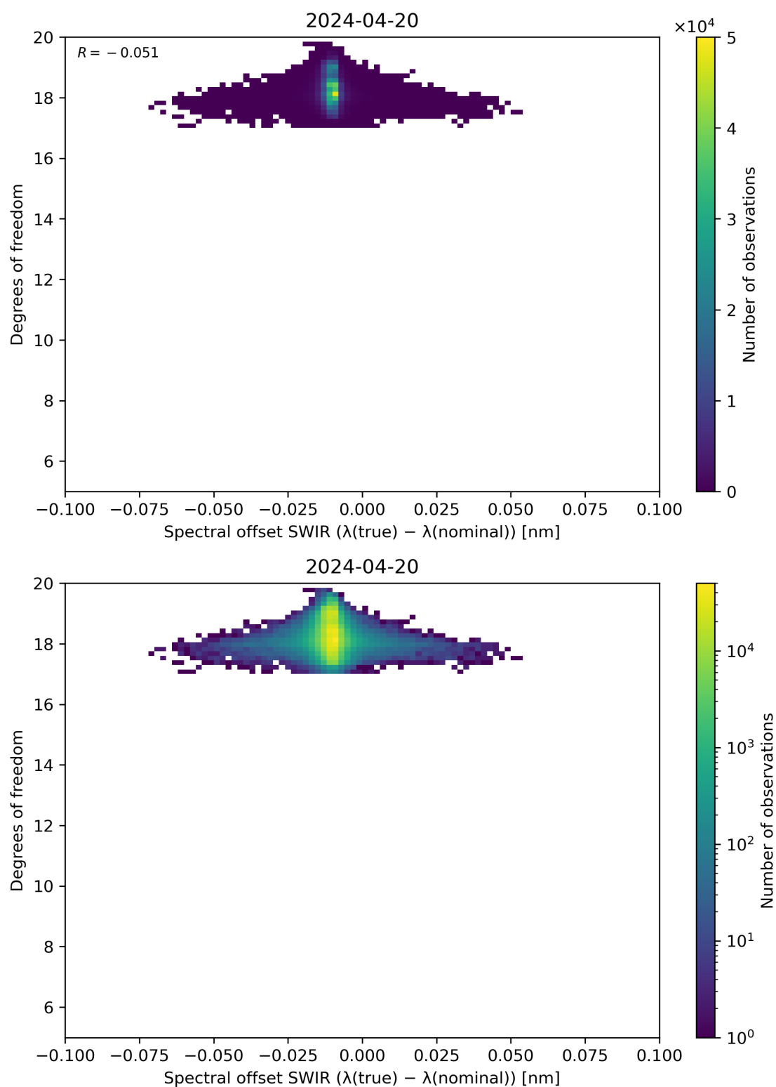
Figure 119: Scatter density plot of “Spectral offset SWIR ( \lambda(\text{true}) - \lambda(\text{nominal}) )” against “Degrees of freedom” for 2024-04-19 to 2024-04-21.
