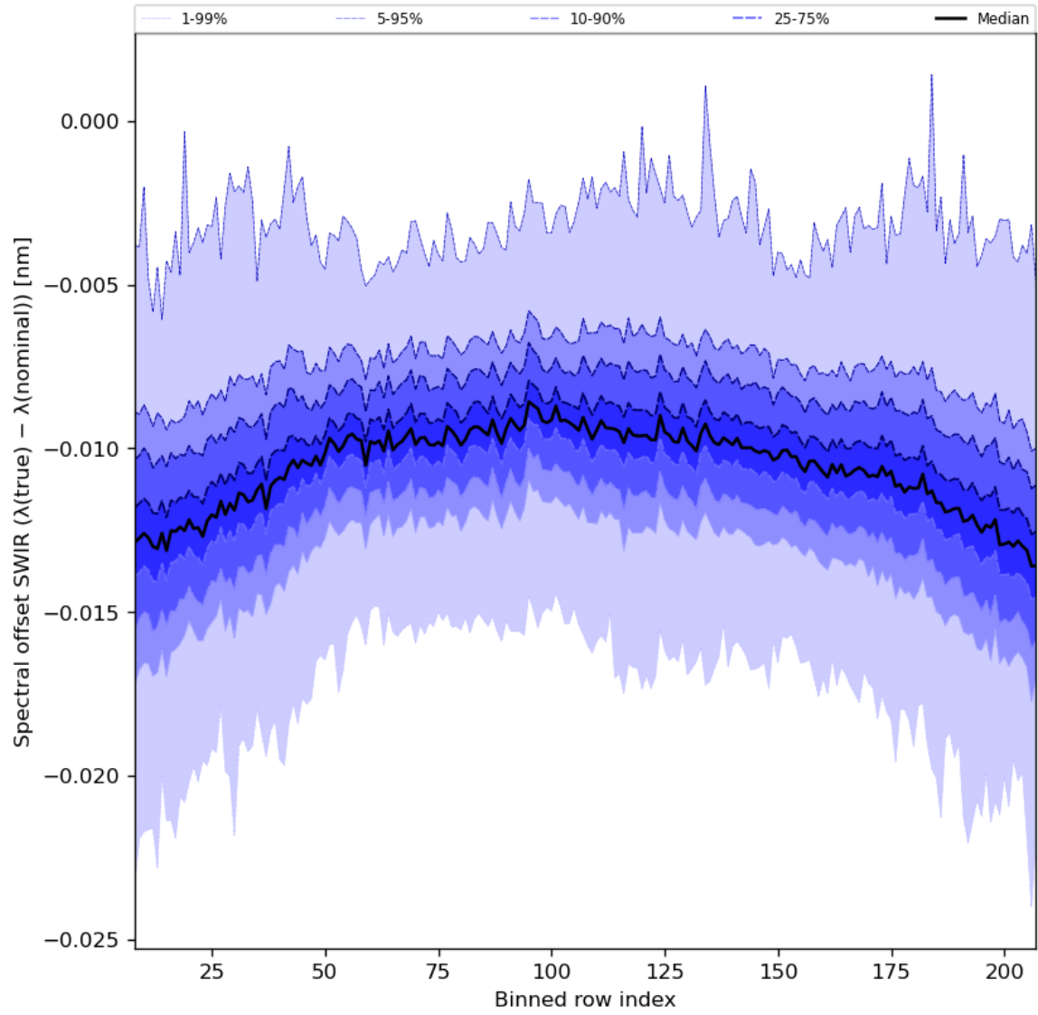
Figure 38: Along track statistics of “Spectral offset SWIR ( \lambda(\text{true}) - \lambda(\text{nominal}) )” for 2024-04-19 to 2024-04-21
