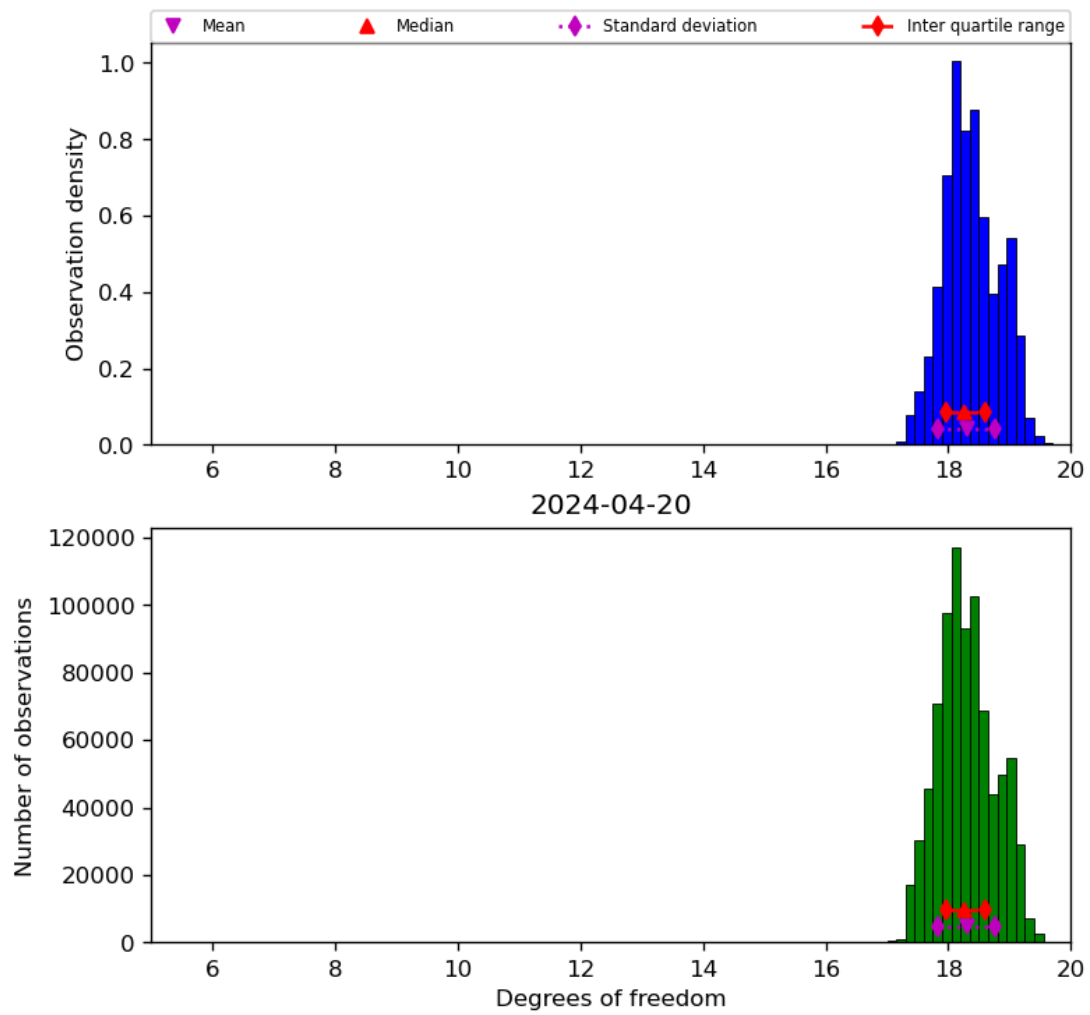
Figure 30: Histogram of “Degrees of freedom” for 2024-04-19 to 2024-04-21
