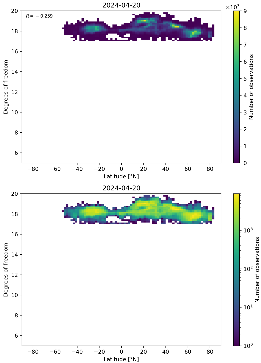
Figure 55: Scatter density plot of “Latitude” against “Degrees of freedom” for 2024-04-19 to 2024-04-21.
