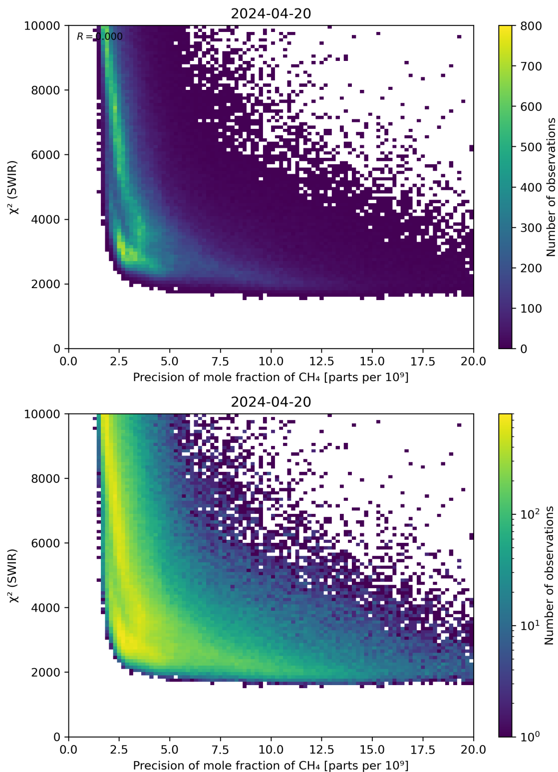
Figure 79: Scatter density plot of “Precision of mole fraction of CH 4 ” against “ \chi^2 (SWIR)” for 2024-04-19 to 2024-04-21.
