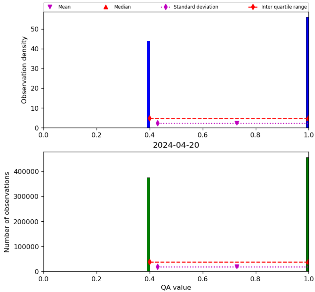
Figure 22: Histogram of “QA value” for 2024-04-19 to 2024-04-21
