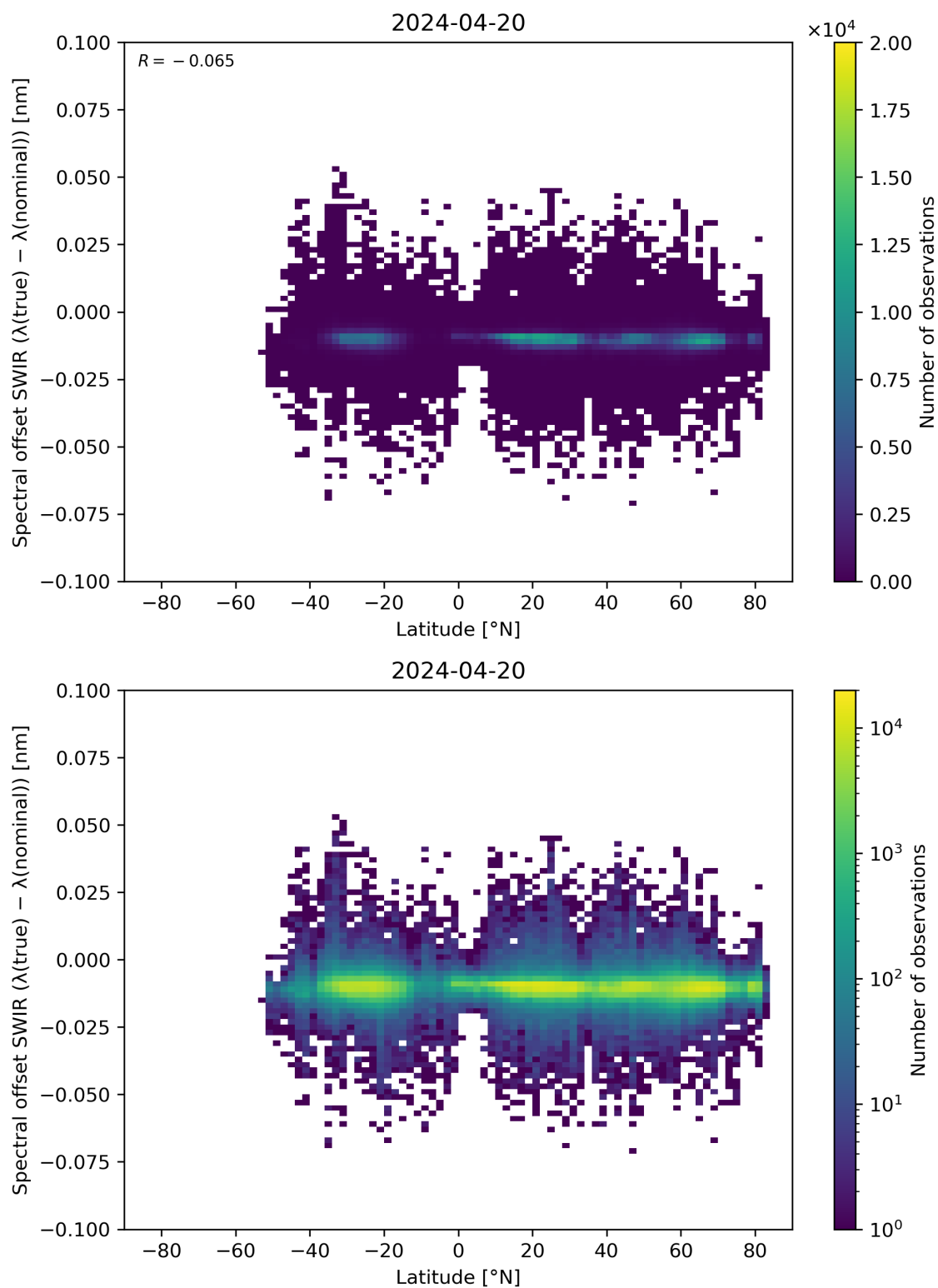
Figure 62: Scatter density plot of “Latitude” against “Spectral offset SWIR ( \lambda(\text{true}) - \lambda(\text{nominal}) )” for 2024-04-19 to 2024-04-21.
