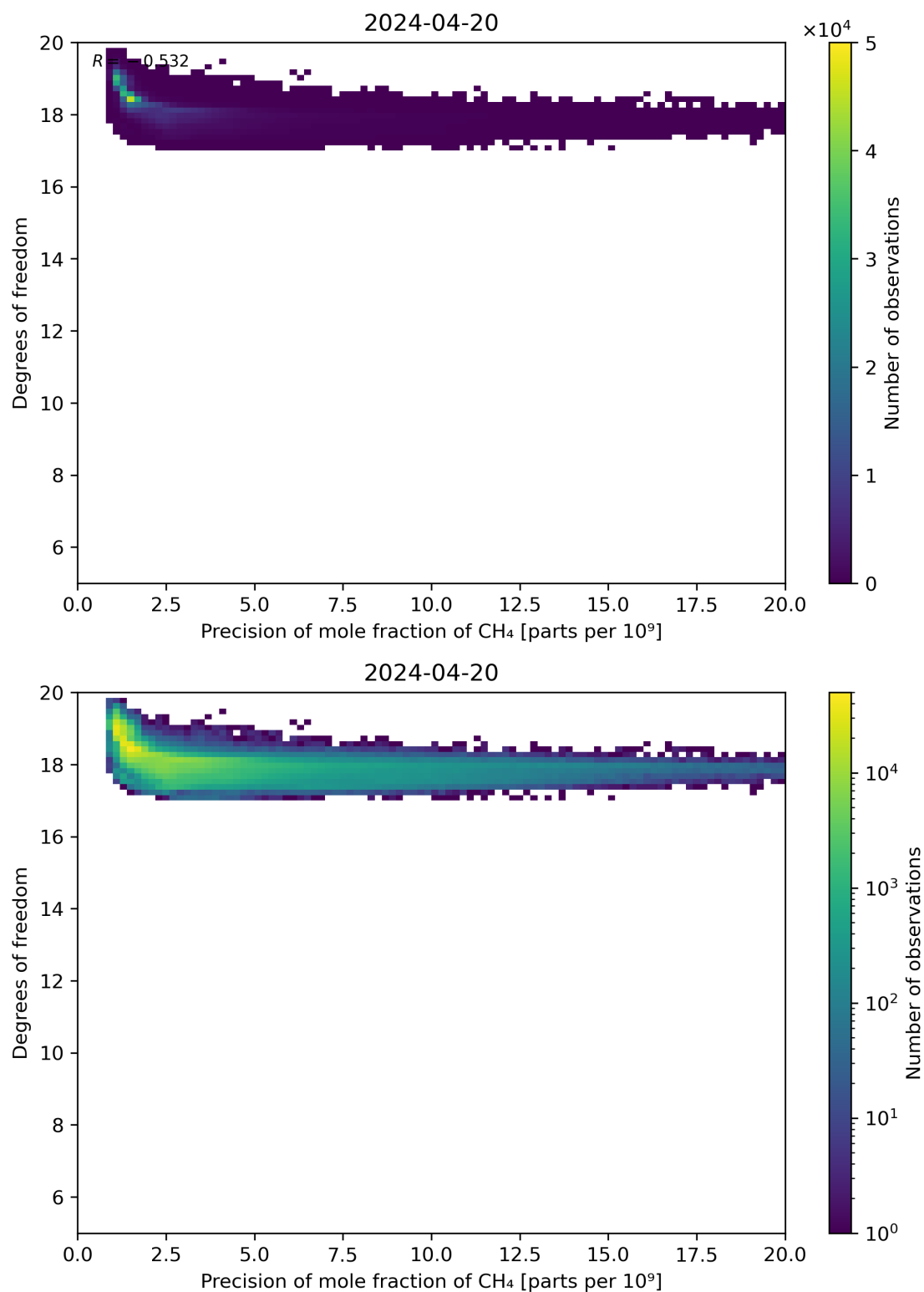
Figure 80: Scatter density plot of “Precision of mole fraction of CH 4 ” against “Degrees of freedom” for 2024-04-19 to 2024-04-21.
