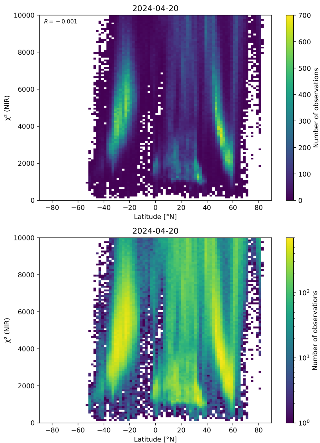
Figure 53: Scatter density plot of “Latitude” against “ \chi^2 (NIR)” for 2024-04-19 to 2024-04-21.
