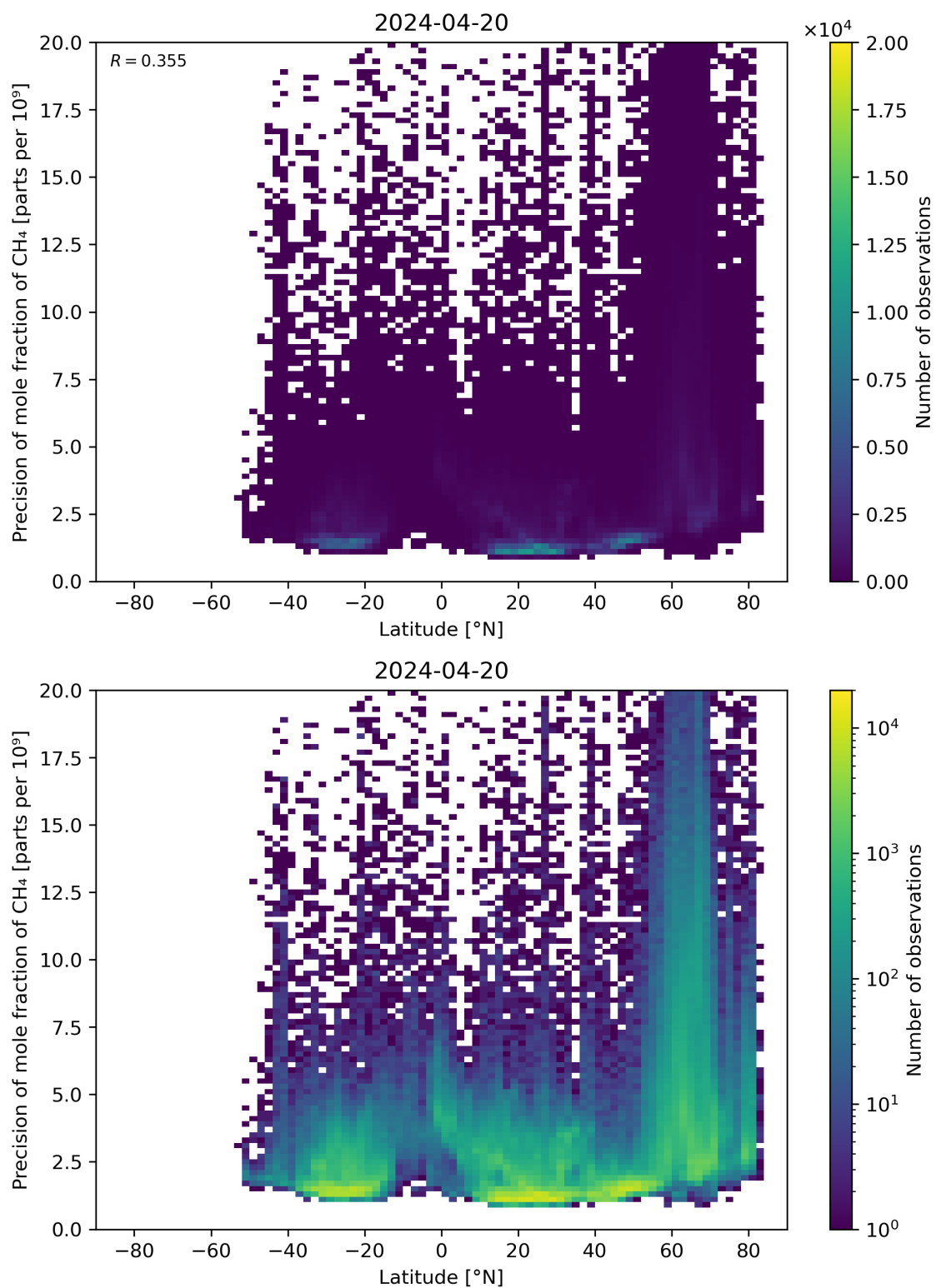
Figure 59: Scatter density plot of “Latitude” against “Precision of mole fraction of \text{CH}_4 ” for 2024-04-19 to 2024-04-21.
