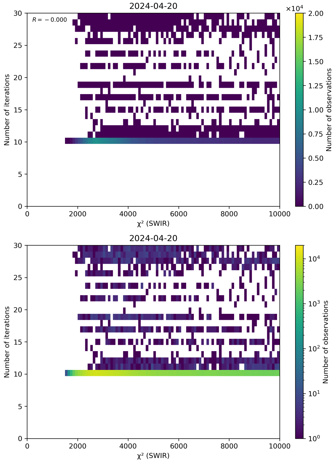
Figure 50: Scatter density plot of “ \chi^2 (SWIR)” against “Number of iterations” for 2024-04-19 to 2024-04-21.
