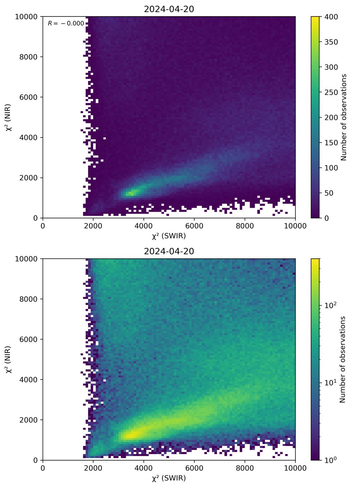
Figure 47: Scatter density plot of “ \chi^2 (SWIR)” against “ \chi^2 (NIR)” for 2024-04-19 to 2024-04-21.
