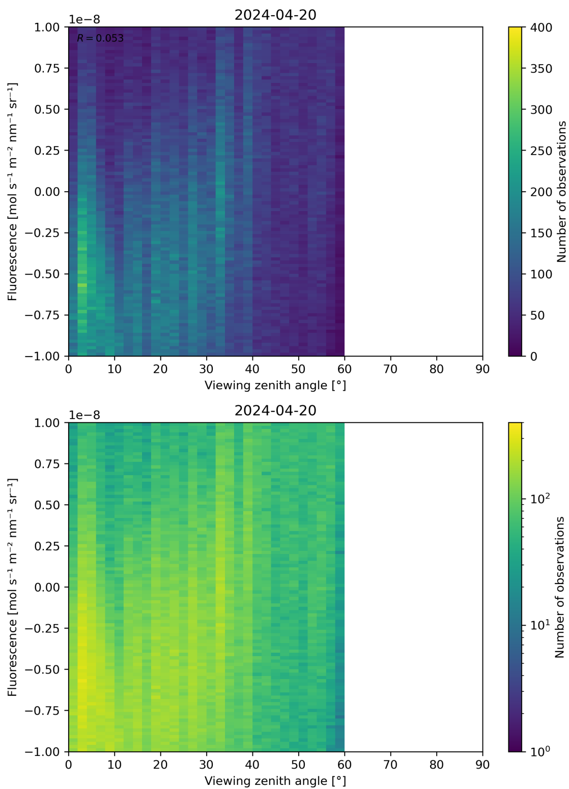
Figure 108: Scatter density plot of “Viewing zenith angle” against “Fluorescence” for 2024-04-19 to 2024-04-21.
