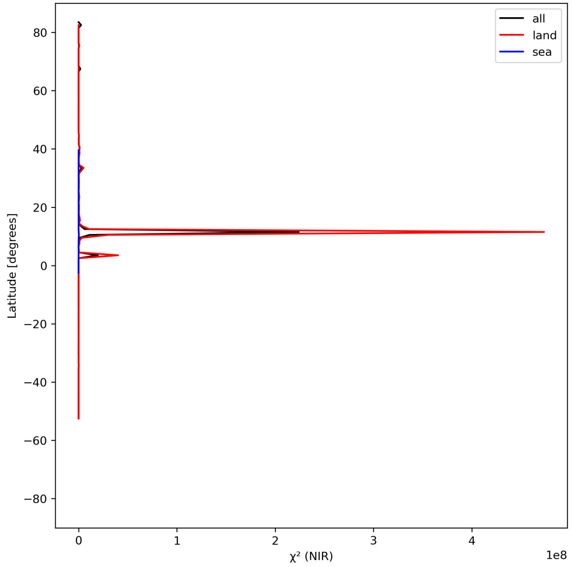
Figure 18: Zonal average of “ \chi^2 (NIR)” for 2024-04-19 to 2024-04-21.
