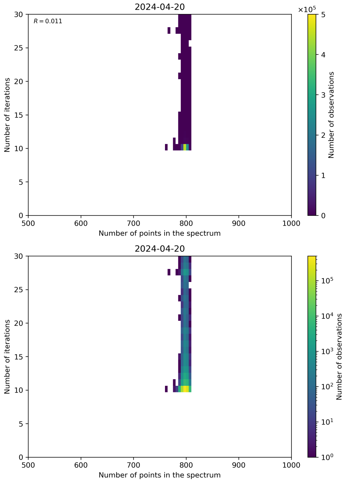
Figure 92: Scatter density plot of “Number of points in the spectrum” against “Number of iterations” for 2024-04-19 to 2024-04-21.
