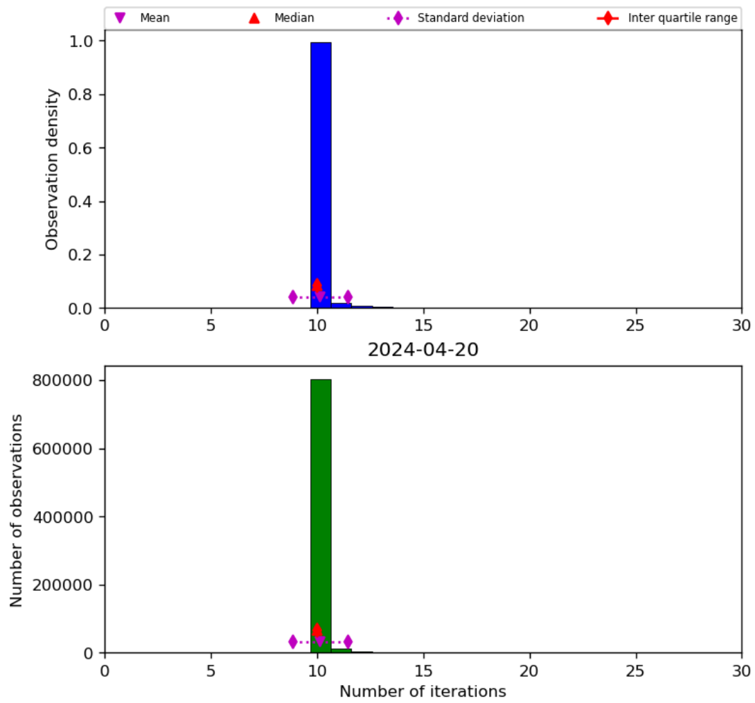
Figure 31: Histogram of “Number of iterations” for 2024-04-19 to 2024-04-21
