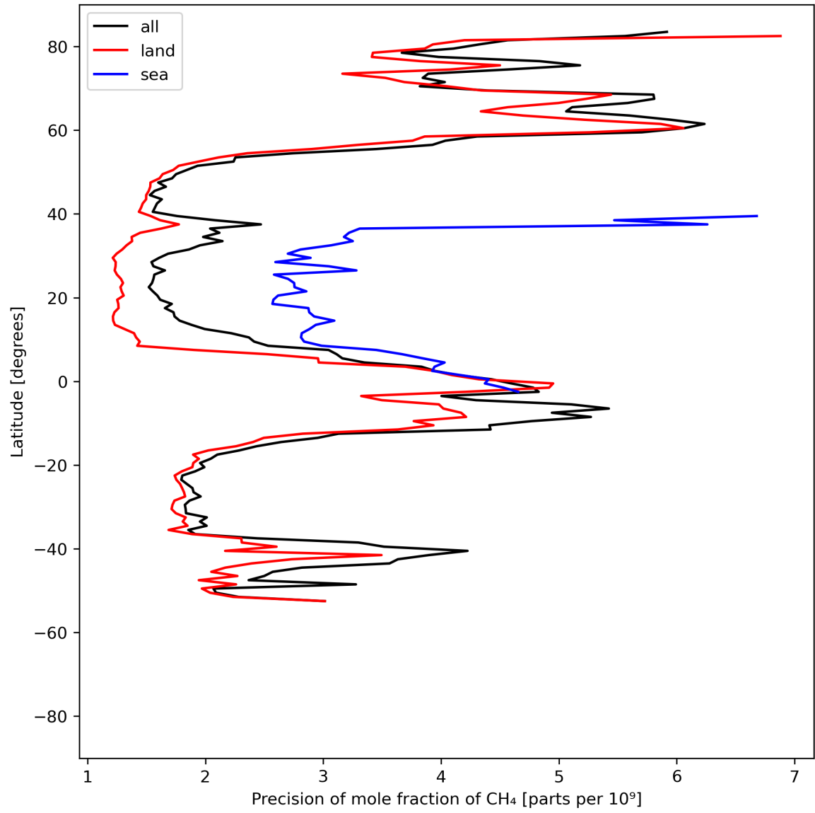
Figure 13: Zonal average of “Precision of mole fraction of \text{CH}_4 ” for 2024-04-19 to 2024-04-21.
