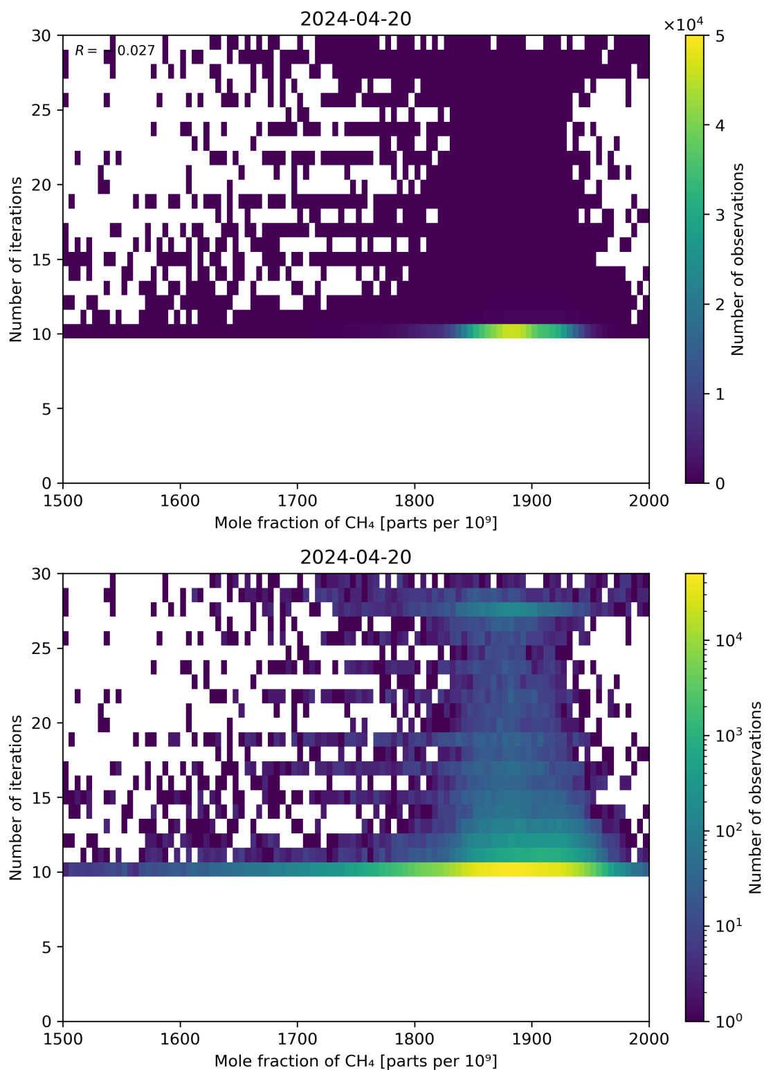
Figure 76: Scatter density plot of “Mole fraction of CH 4 ” against “Number of iterations” for 2024-04-19 to 2024-04-21.
