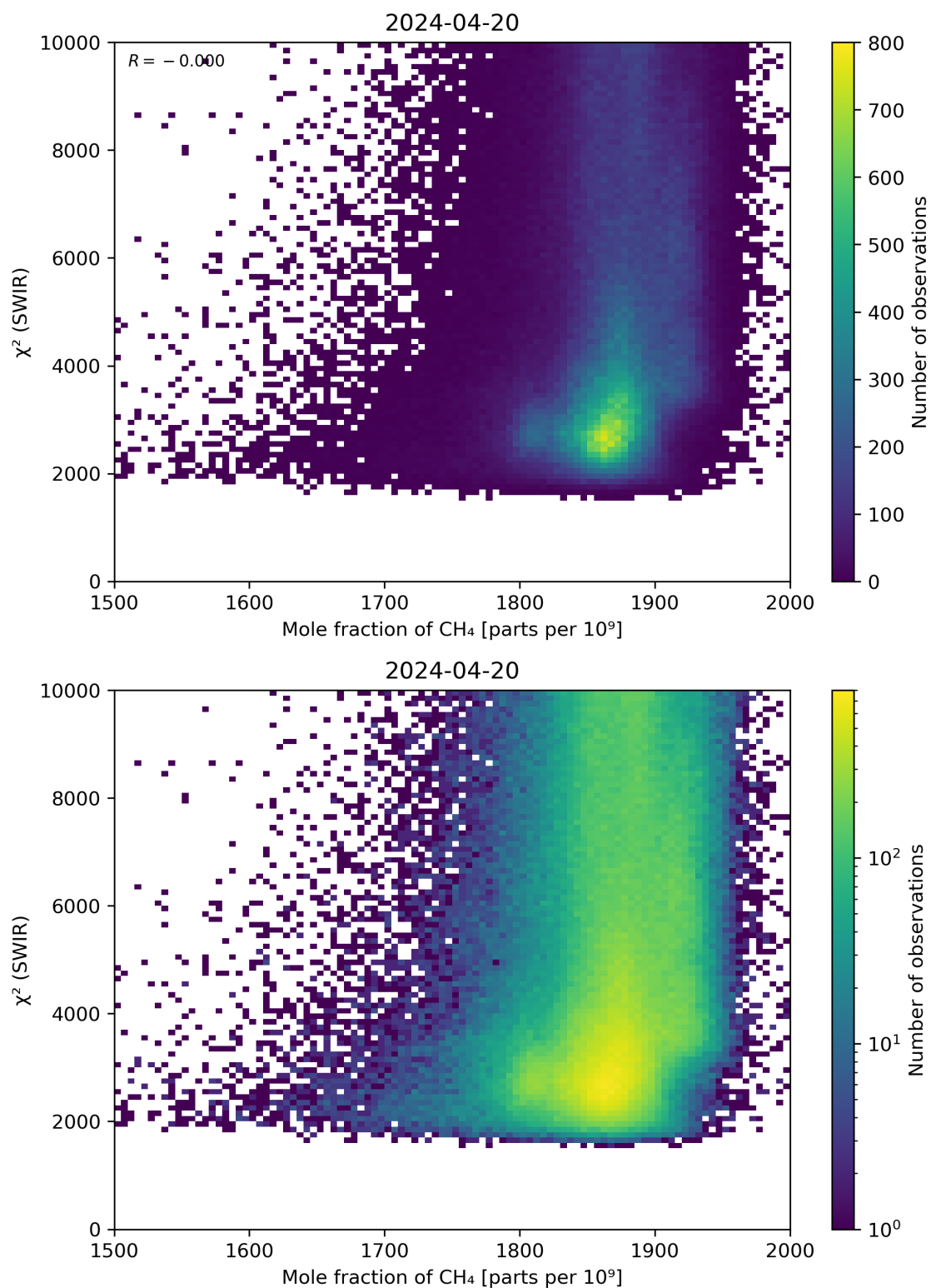
Figure 71: Scatter density plot of “Mole fraction of \text{CH}_4 ” against “ \chi^2 (SWIR)” for 2024-04-19 to 2024-04-21.
