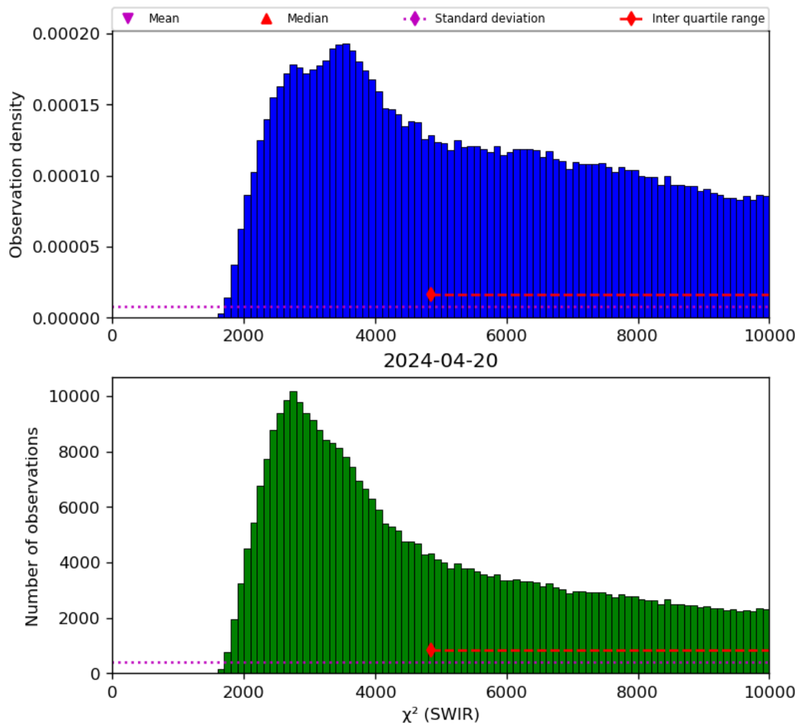
Figure 28: Histogram of " \chi^2 (SWIR)" for 2024-04-19 to 2024-04-21
