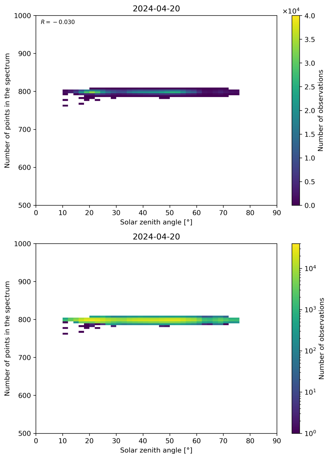
Figure 103: Scatter density plot of “Solar zenith angle” against “Number of points in the spectrum” for 2024-04-19 to 2024-04-21.
