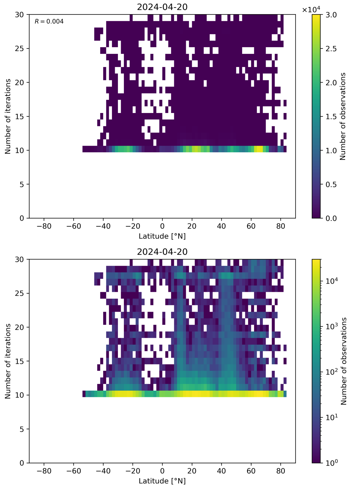
Figure 60: Scatter density plot of “Latitude” against “Number of iterations” for 2024-04-19 to 2024-04-21.
