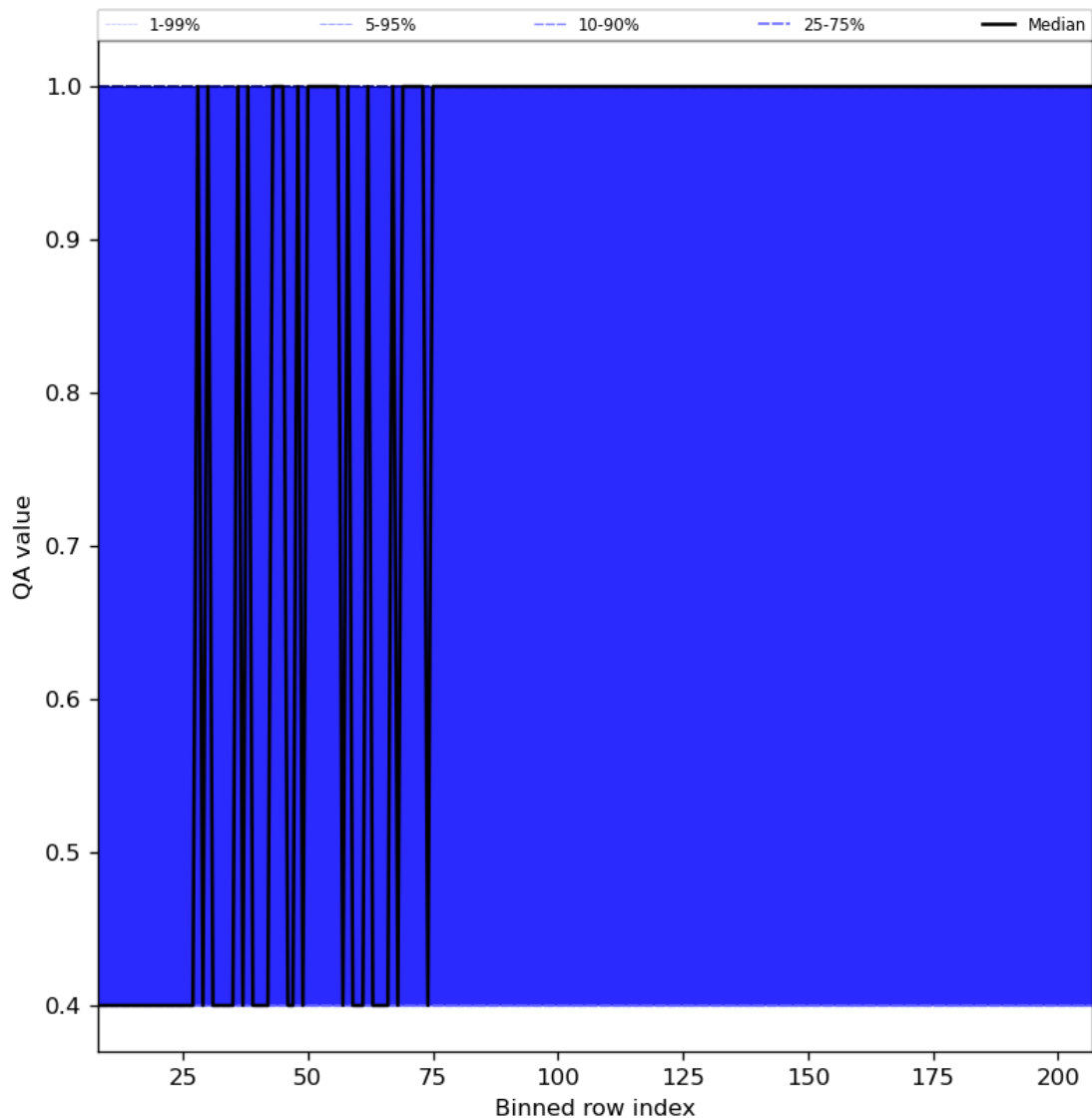
Figure 33: Along track statistics of “QA value” for 2024-04-19 to 2024-04-21
