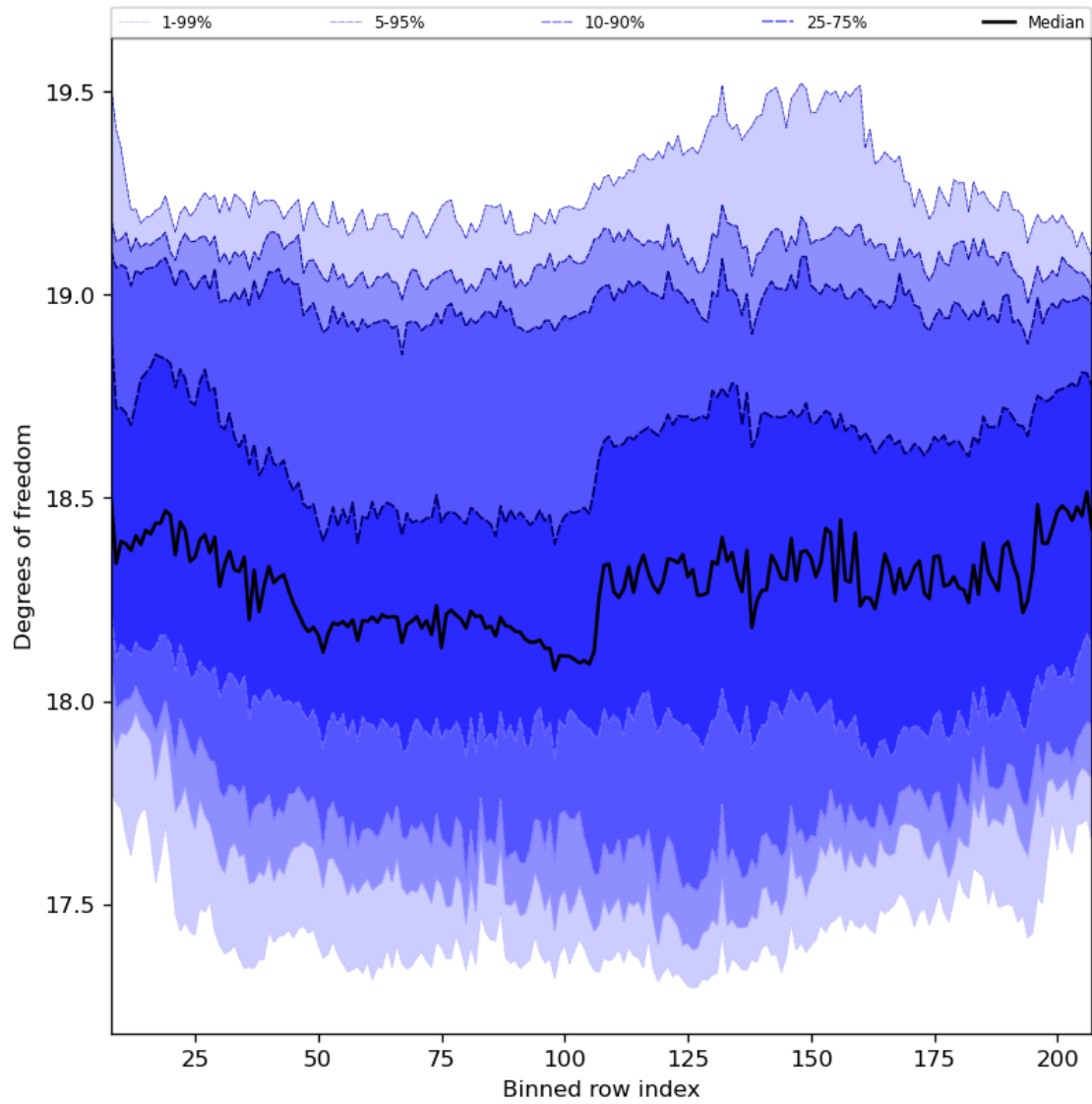
Figure 41: Along track statistics of “Degrees of freedom” for 2024-04-19 to 2024-04-21
