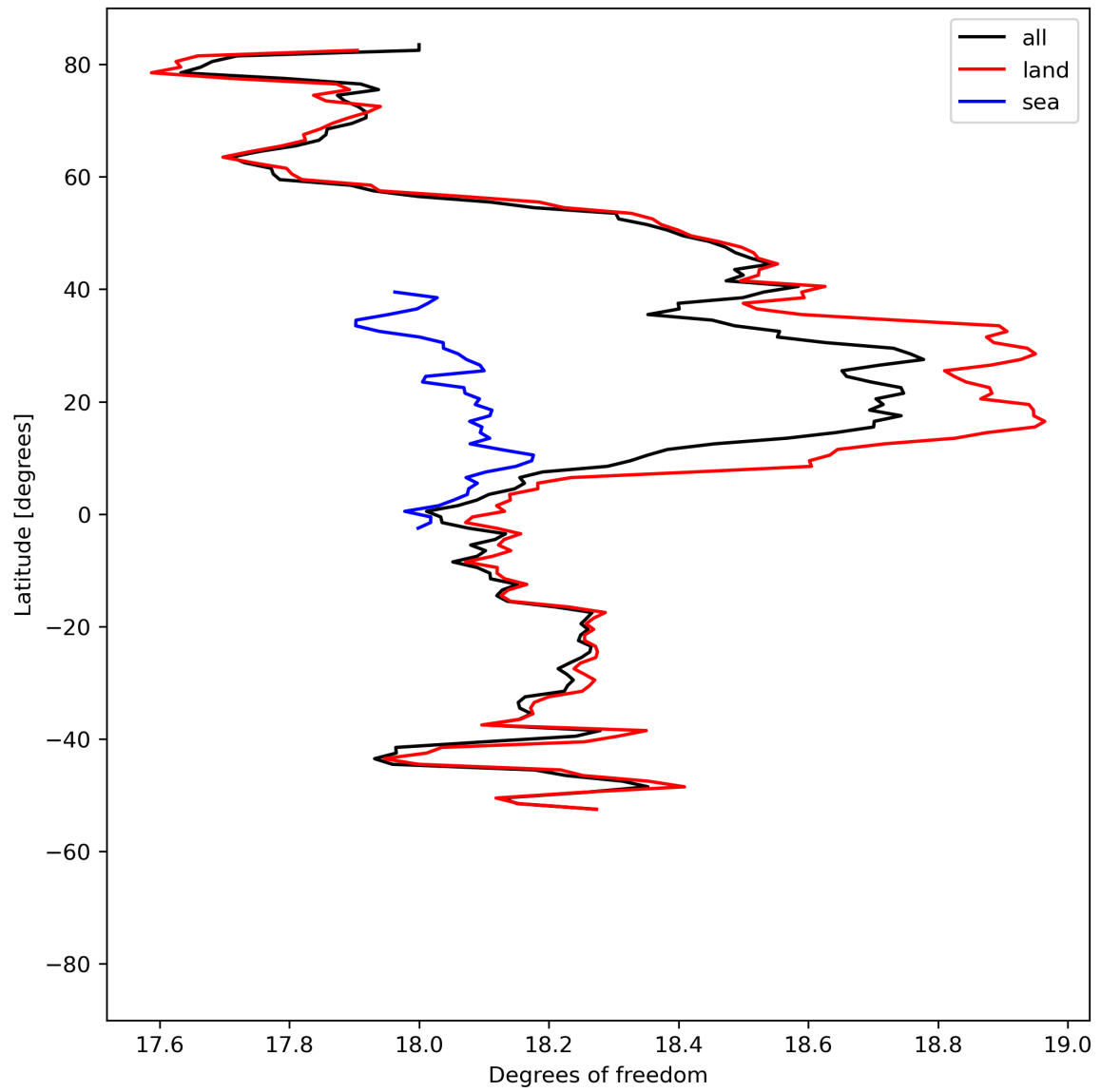
Figure 19: Zonal average of “Degrees of freedom” for 2024-04-19 to 2024-04-21.
