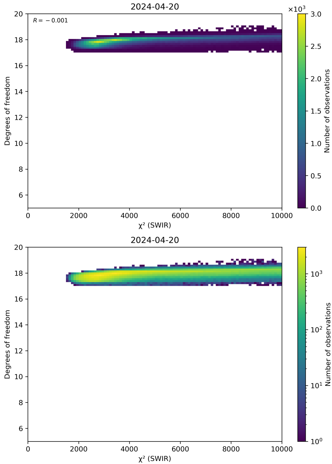
Figure 48: Scatter density plot of “ \chi^2 (SWIR)” against “Degrees of freedom” for 2024-04-19 to 2024-04-21.
