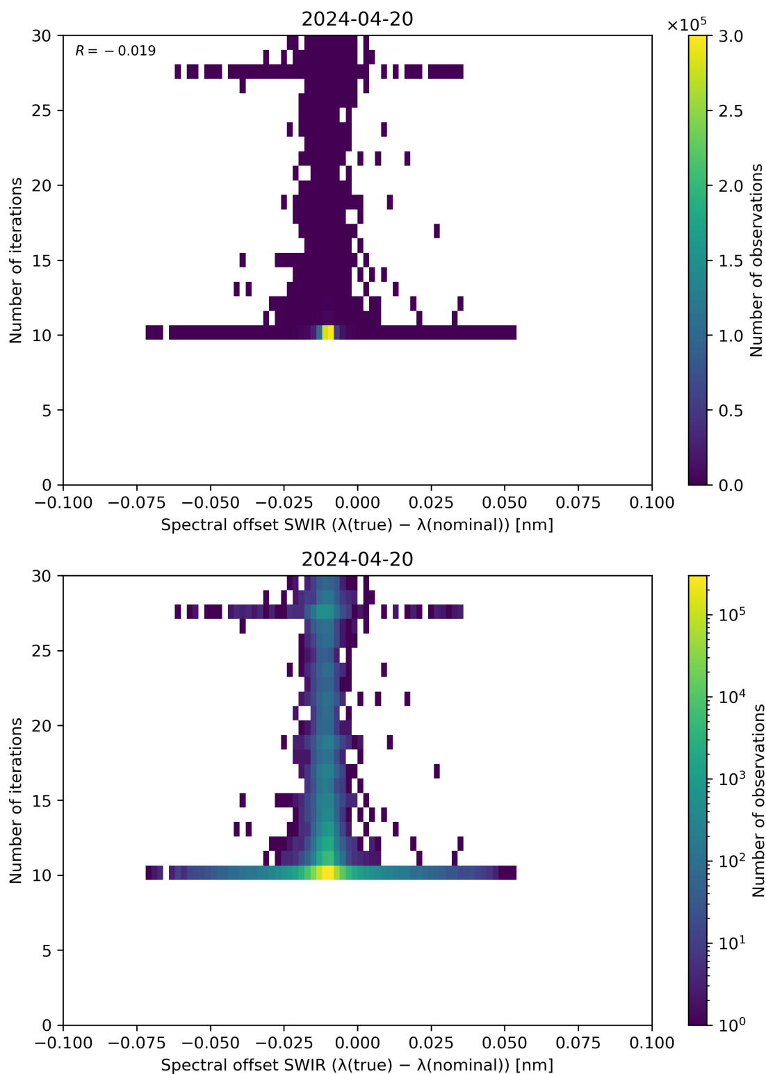
Figure 121: Scatter density plot of “Spectral offset SWIR ( \lambda(\text{true}) - \lambda(\text{nominal}) )” against “Number of iterations” for 2024-04-19 to 2024-04-21.
