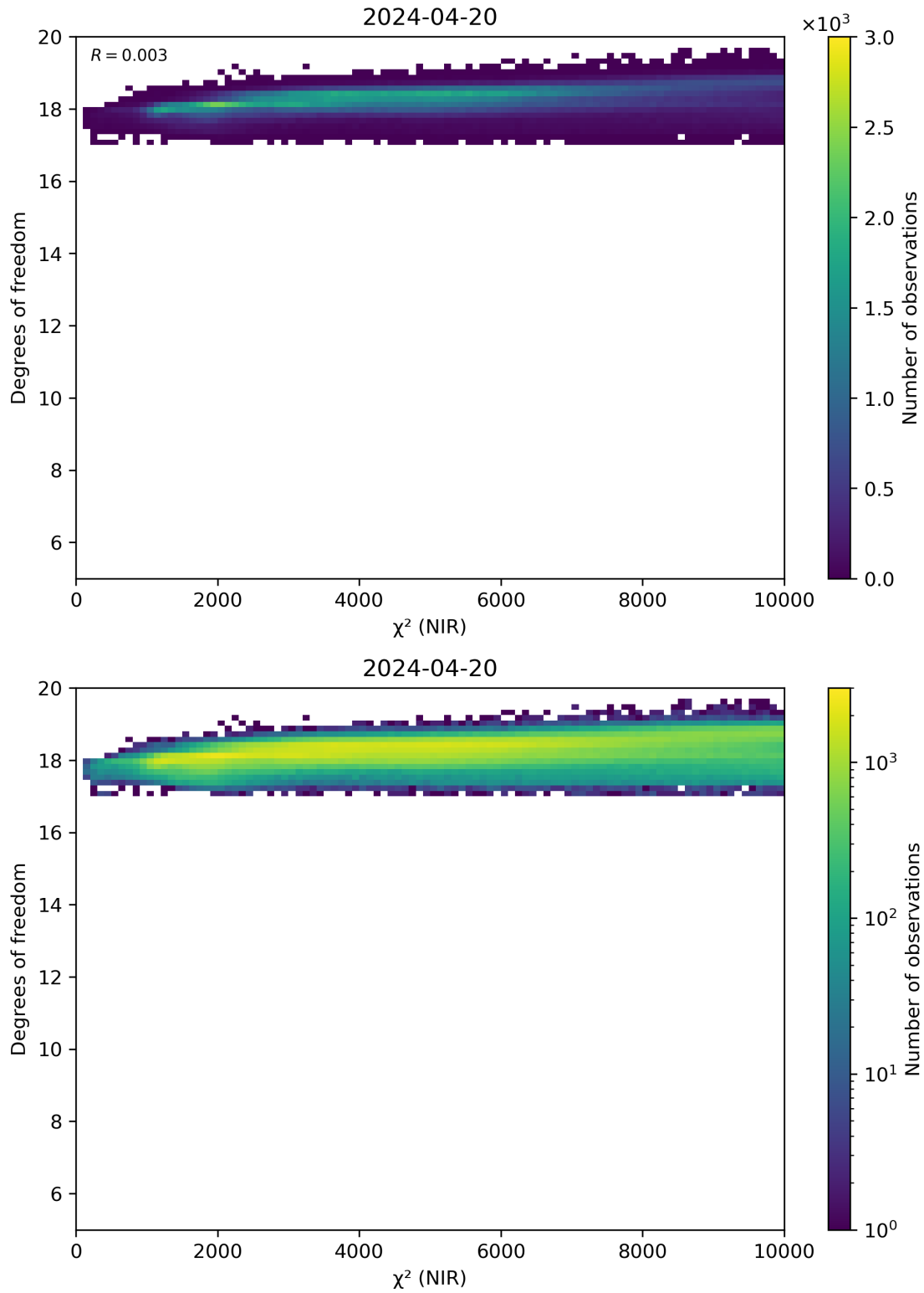
Figure 44: Scatter density plot of “ \chi^2 (NIR)” against “Degrees of freedom” for 2024-04-19 to 2024-04-21.
