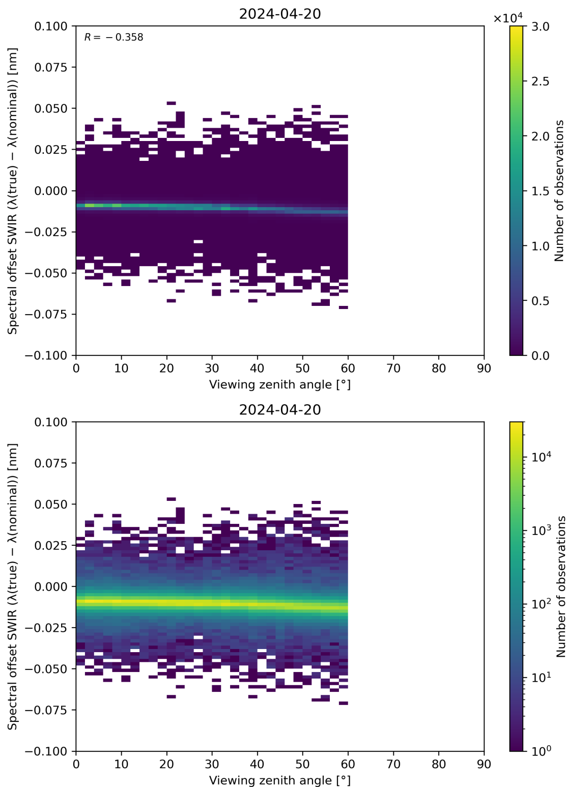
Figure 116: Scatter density plot of “Viewing zenith angle” against “Spectral offset SWIR ( \lambda(\text{true}) - \lambda(\text{nominal}) )” for 2024-04-19 to 2024-04-21.
