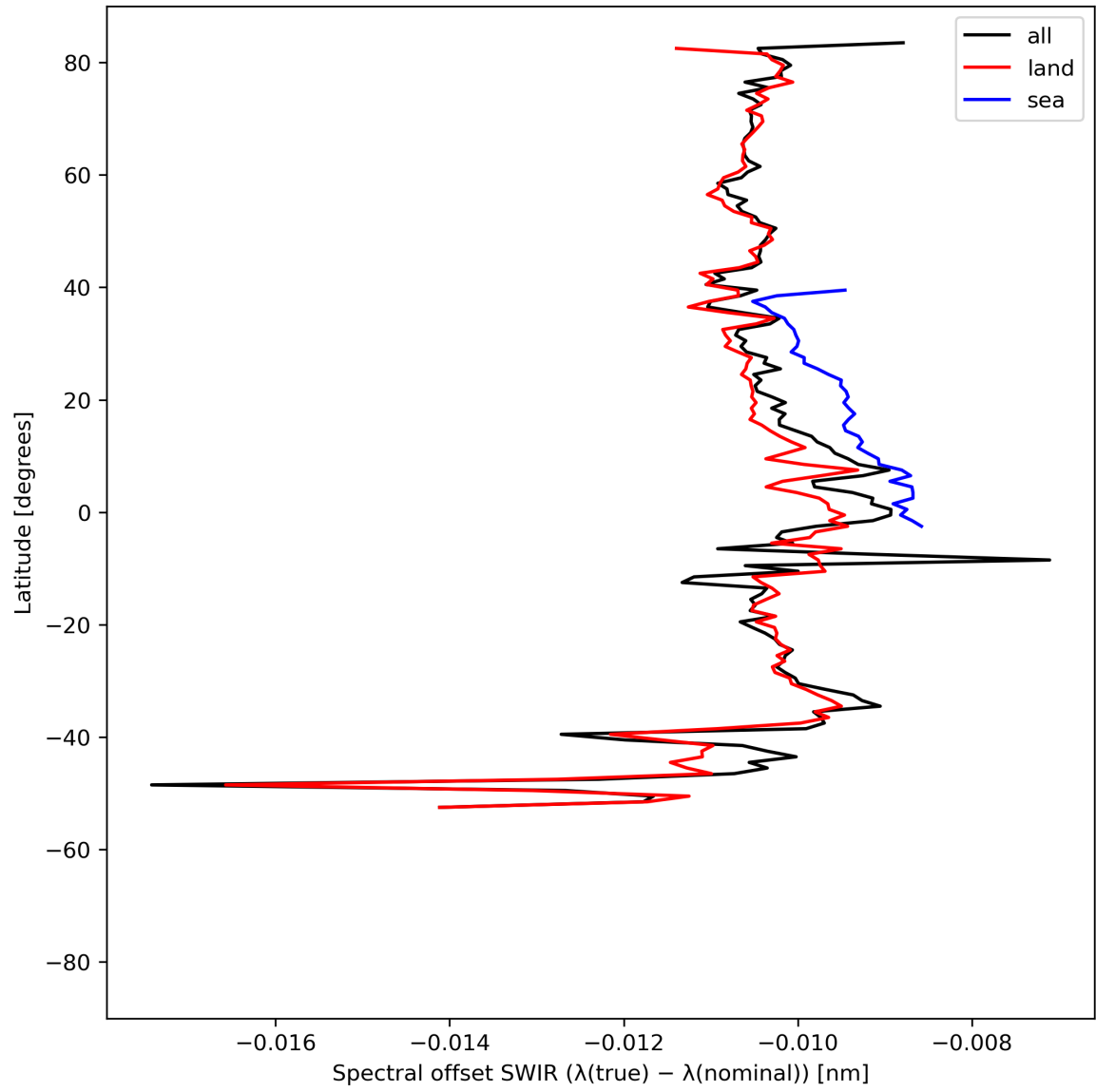
Figure 16: Zonal average of “Spectral offset SWIR ( \lambda(\text{true}) - \lambda(\text{nominal}) )” for 2024-04-19 to 2024-04-21.
