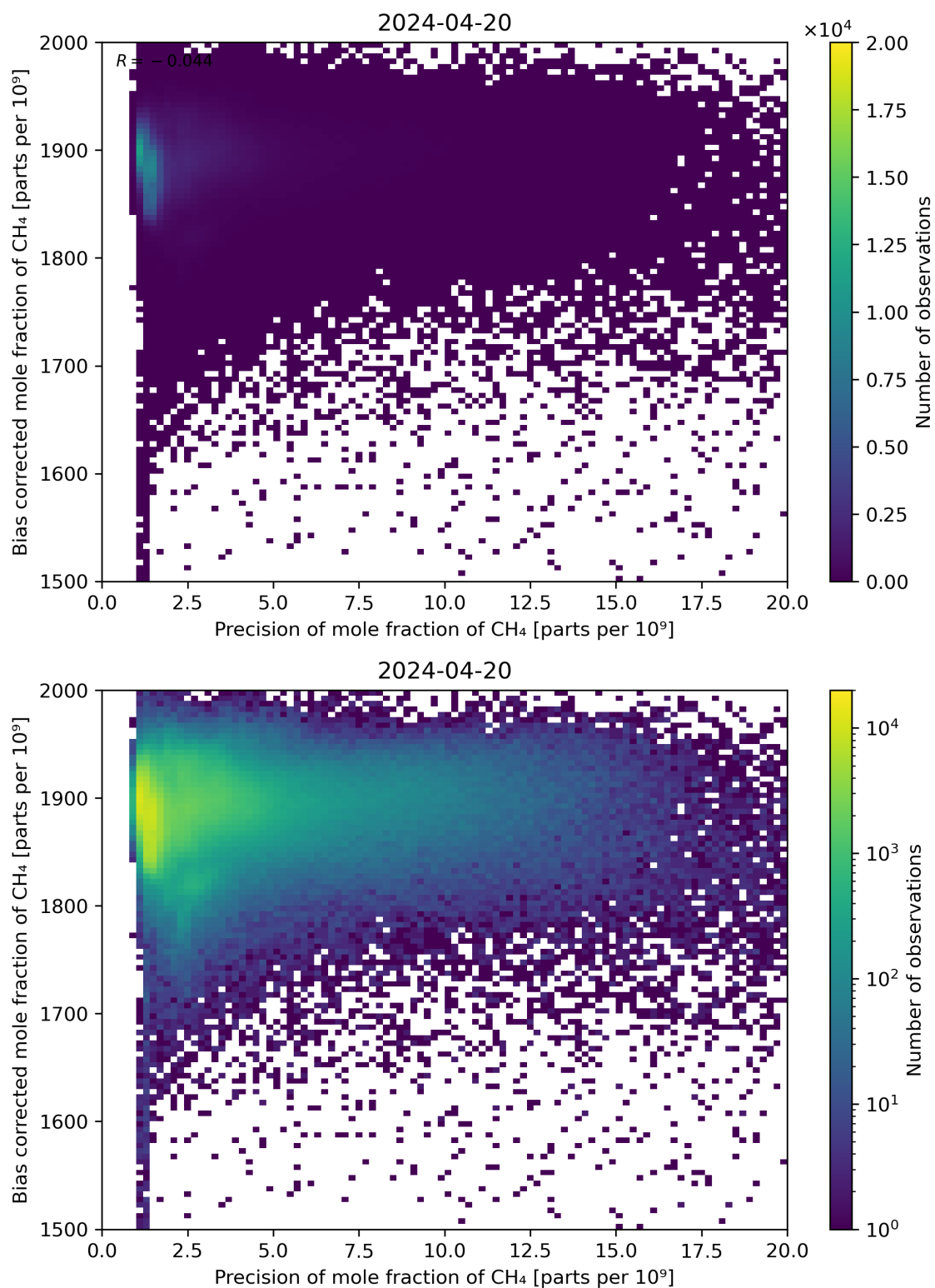
Figure 82: Scatter density plot of “Precision of mole fraction of CH 4 ” against “Bias corrected mole fraction of CH 4 ” for 2024-04-19 to 2024-04-21.
