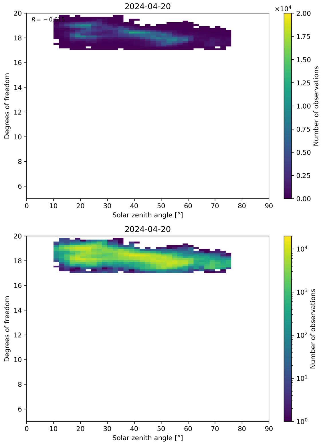
Figure 96: Scatter density plot of “Solar zenith angle” against “Degrees of freedom” for 2024-04-19 to 2024-04-21.
