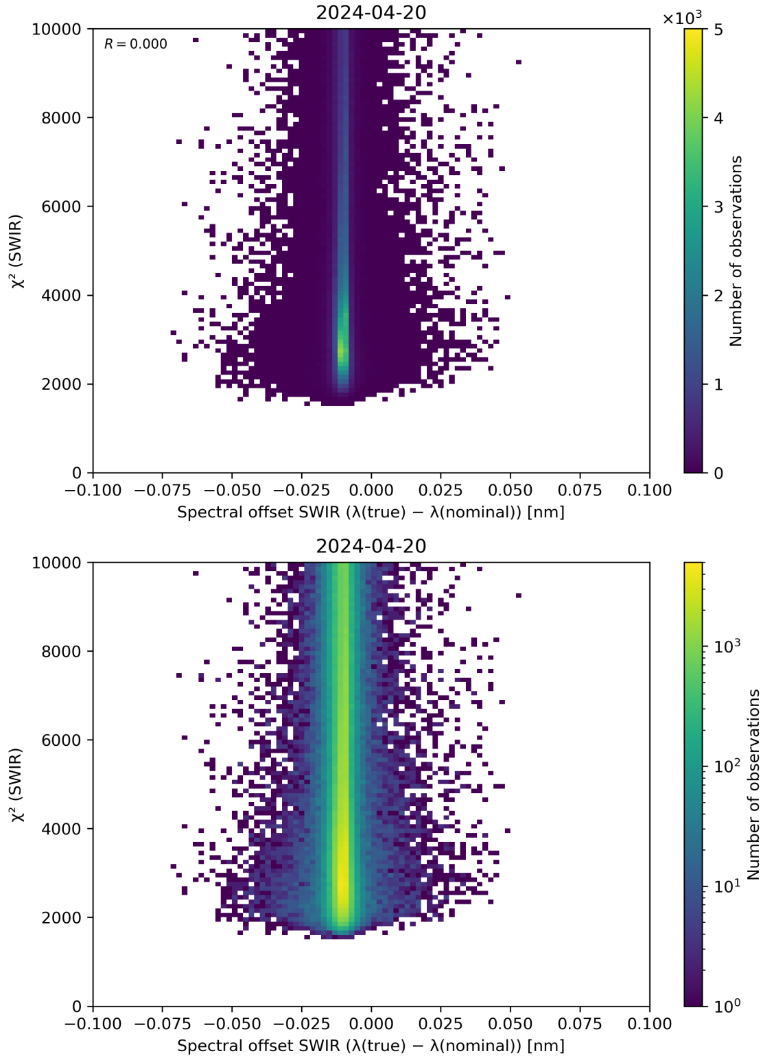
Figure 118: Scatter density plot of “Spectral offset SWIR ( \lambda(\text{true}) - \lambda(\text{nominal}) )” against “ \chi^2 (SWIR)” for 2024-04-19 to 2024-04-21.
