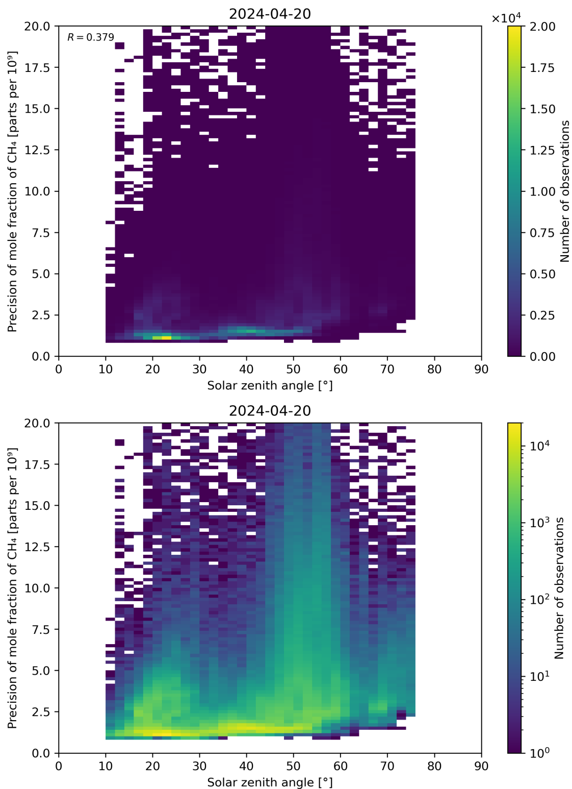
Figure 101: Scatter density plot of “Solar zenith angle” against “Precision of mole fraction of CH 4 ” for 2024-04-19 to 2024-04-21.
