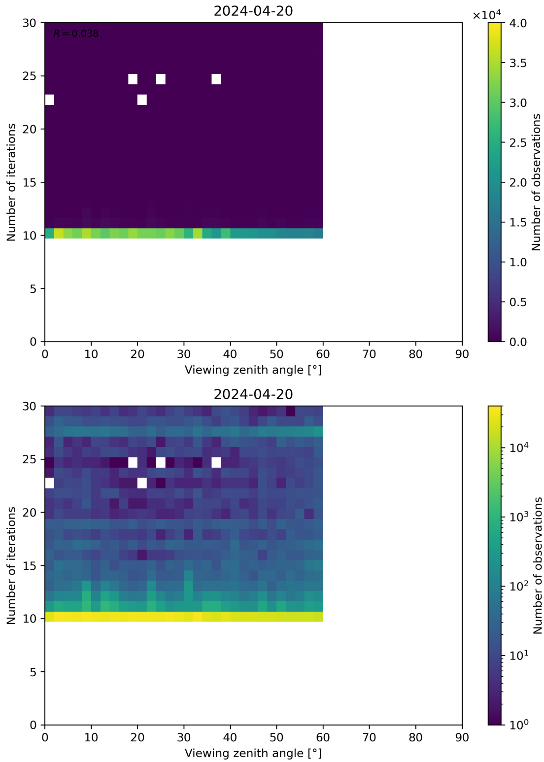
Figure 113: Scatter density plot of “Viewing zenith angle” against “Number of iterations” for 2024-04-19 to 2024-04-21.
