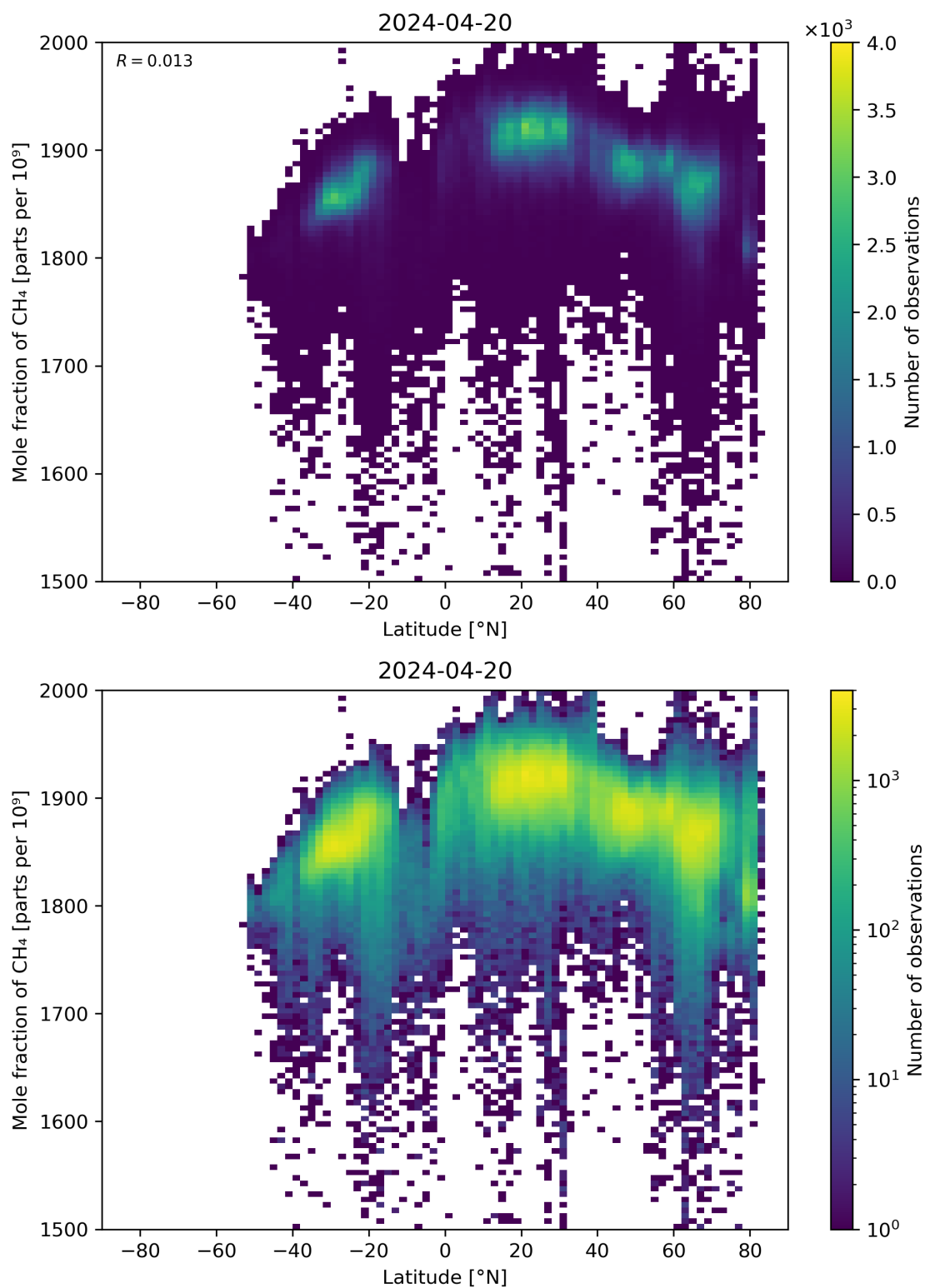
Figure 57: Scatter density plot of “Latitude” against “Mole fraction of \text{CH}_4 ” for 2024-04-19 to 2024-04-21.
