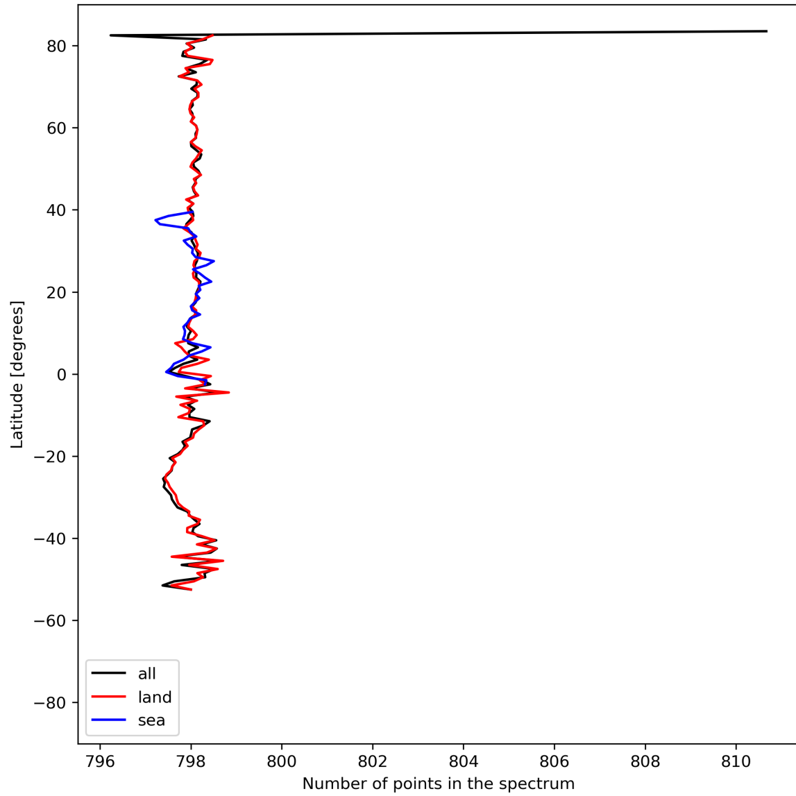
Figure 15: Zonal average of “Number of points in the spectrum” for 2024-04-19 to 2024-04-21.
