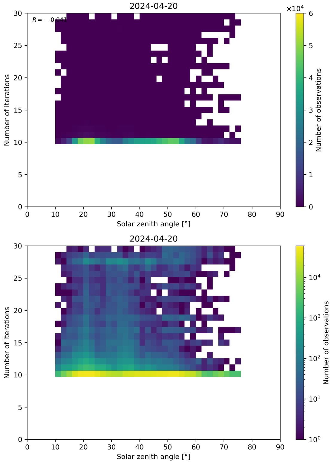
Figure 102: Scatter density plot of “Solar zenith angle” against “Number of iterations” for 2024-04-19 to 2024-04-21.
