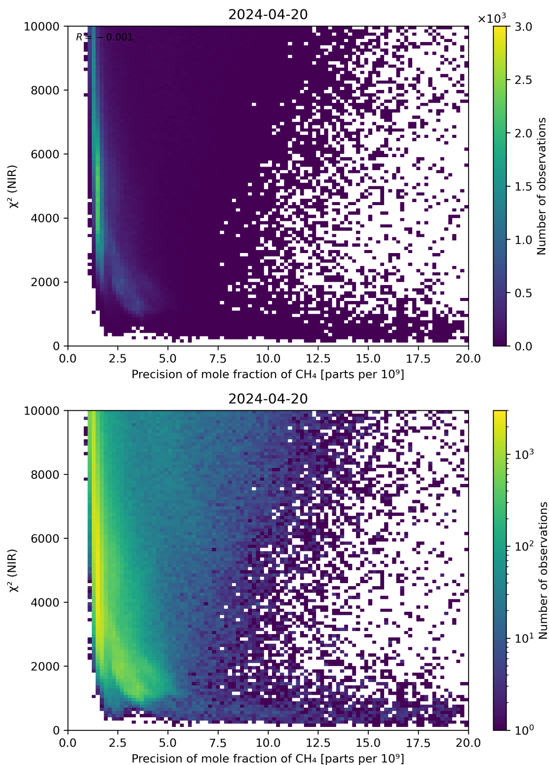
Figure 78: Scatter density plot of “Precision of mole fraction of \text{CH}_4 ” against “ \chi^2 (NIR)” for 2024-04-19 to 2024-04-21.
