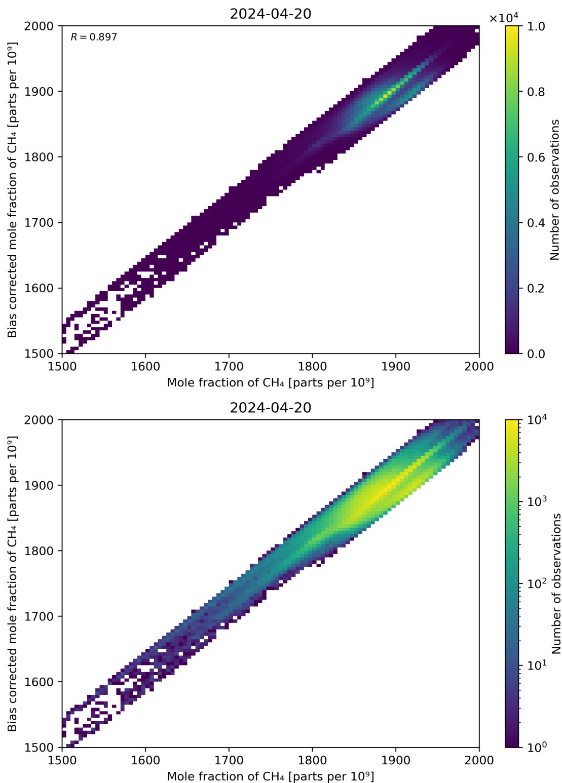
Figure 74: Scatter density plot of “Mole fraction of CH 4 ” against “Bias corrected mole fraction of CH 4 ” for 2024-04-19 to 2024-04-21.
