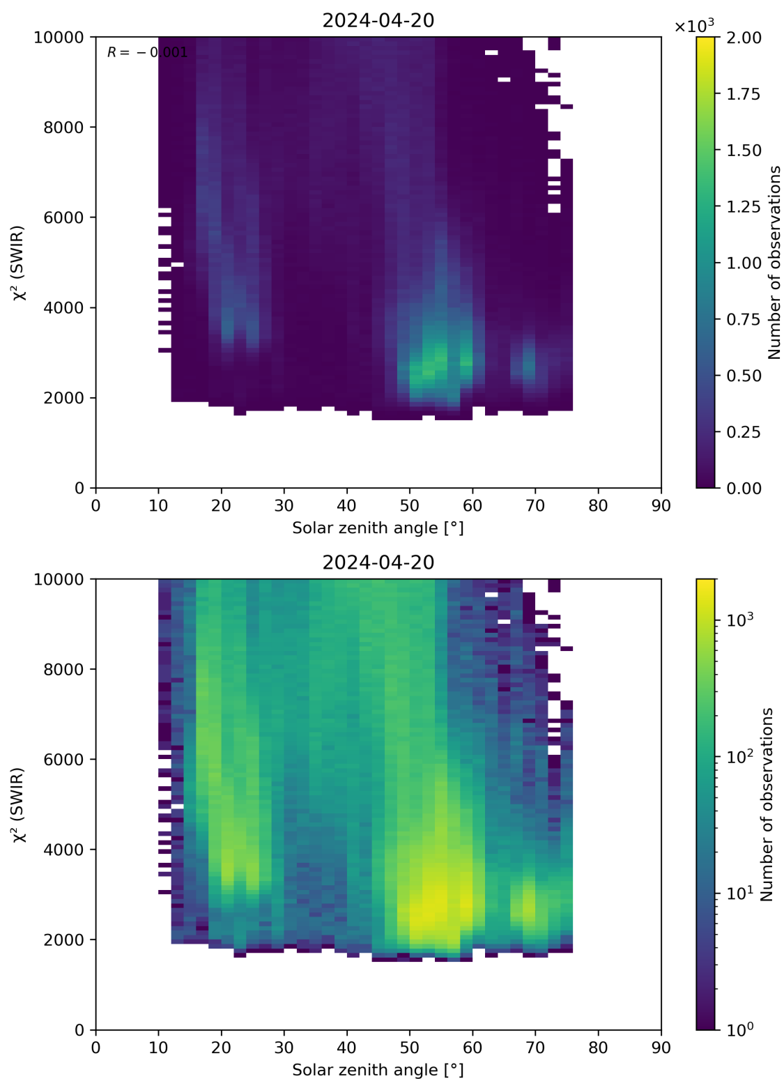
Figure 95: Scatter density plot of “Solar zenith angle” against “ \chi^2 (SWIR)” for 2024-04-19 to 2024-04-21.
