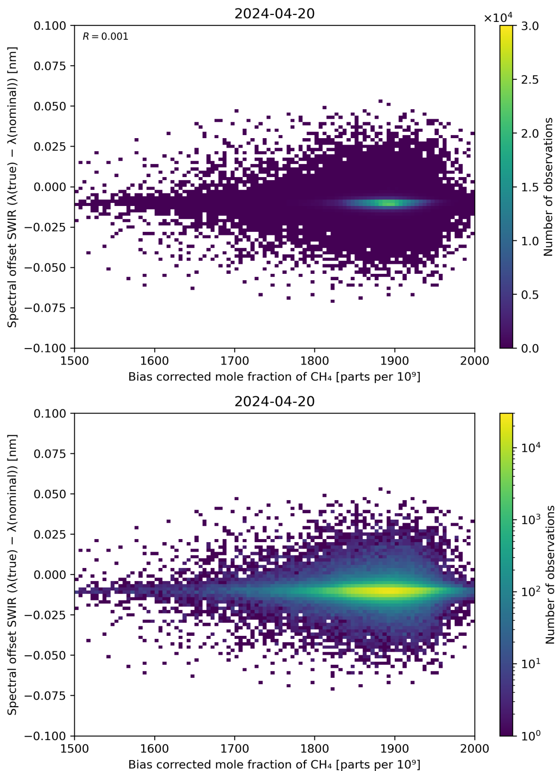
Figure 69: Scatter density plot of “Bias corrected mole fraction of \text{CH}_4 ” against “Spectral offset SWIR ( \lambda(\text{true}) - \lambda(\text{nominal}) )” for 2024-04-19 to 2024-04-21.
