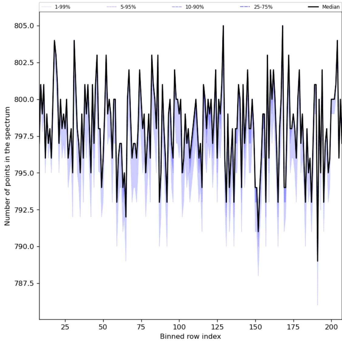
Figure 37: Along track statistics of “Number of points in the spectrum” for 2024-04-19 to 2024-04-21
