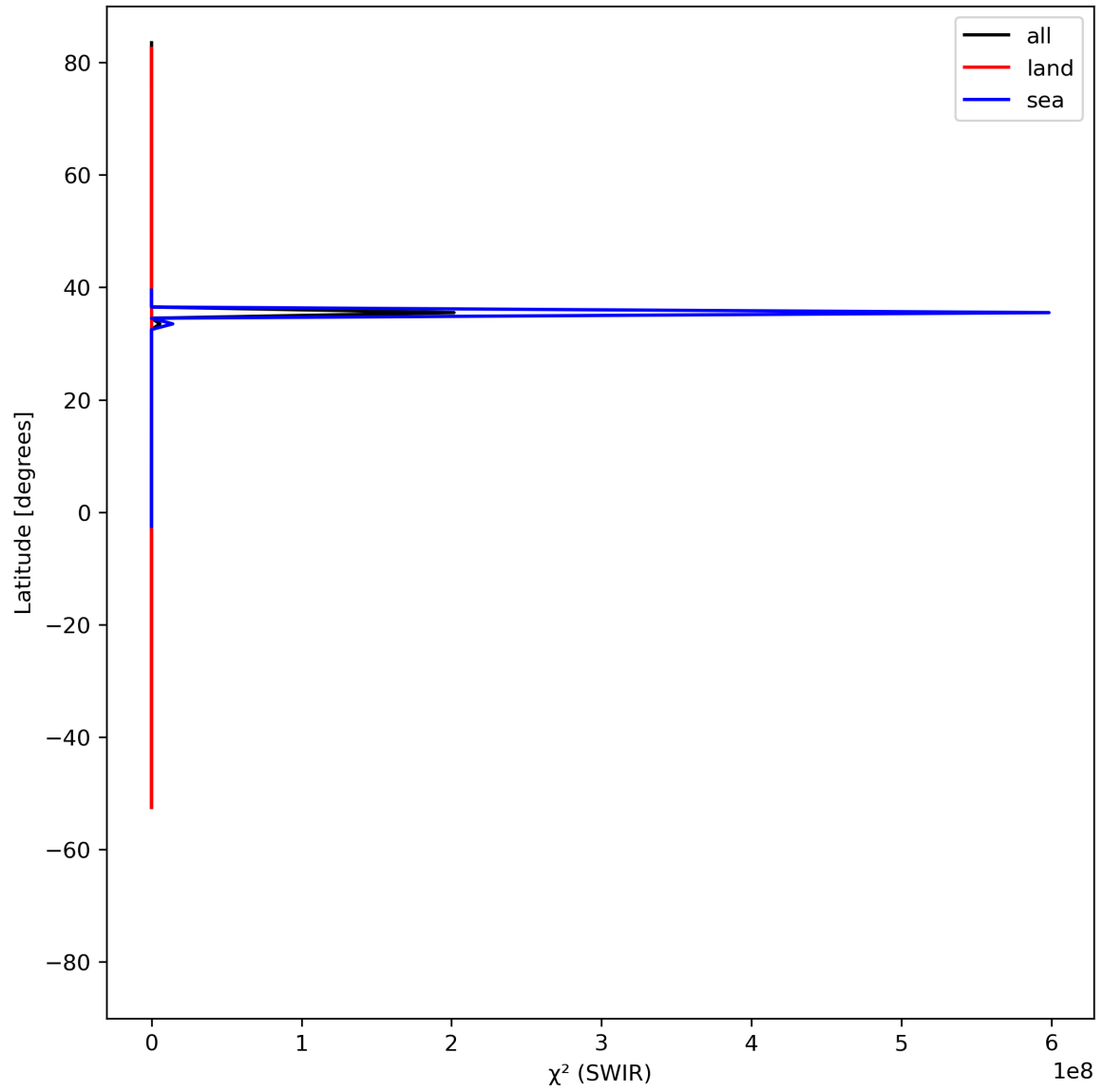
Figure 17: Zonal average of “ \chi^2 (SWIR)” for 2024-04-19 to 2024-04-21.
