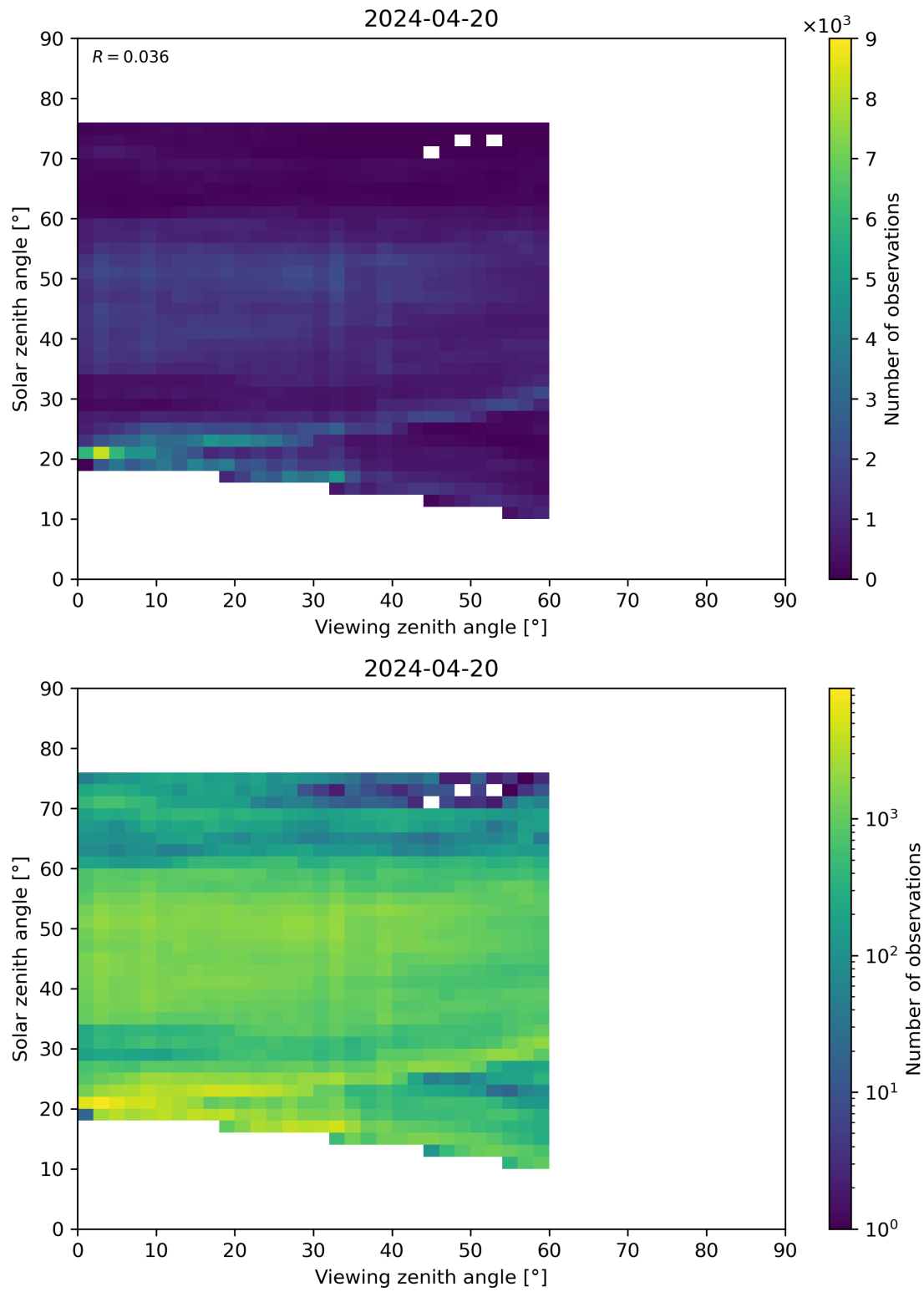
Figure 115: Scatter density plot of “Viewing zenith angle” against “Solar zenith angle” for 2024-04-19 to 2024-04-21.
