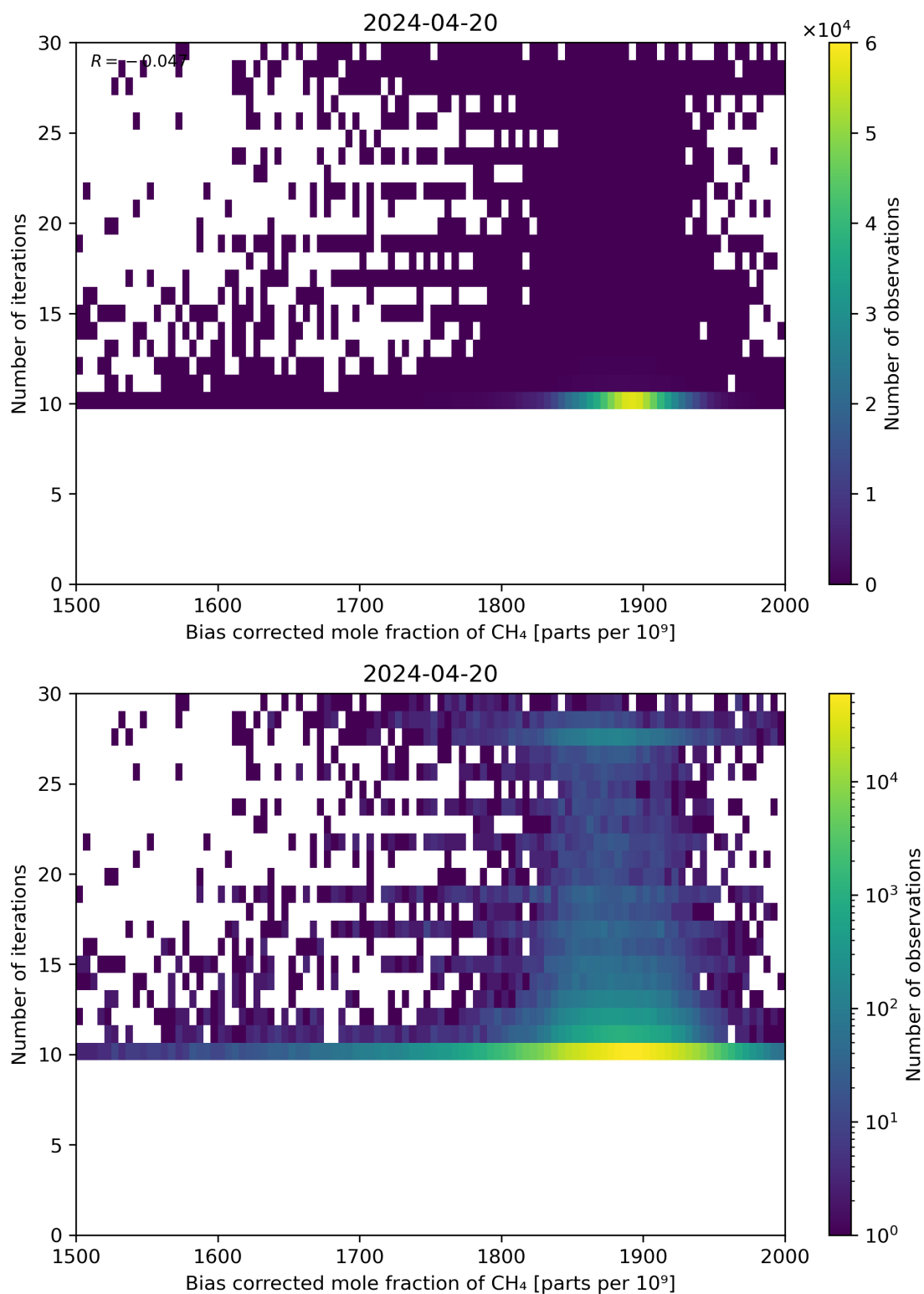
Figure 67: Scatter density plot of “Bias corrected mole fraction of CH 4 ” against “Number of iterations” for 2024-04-19 to 2024-04-21.
