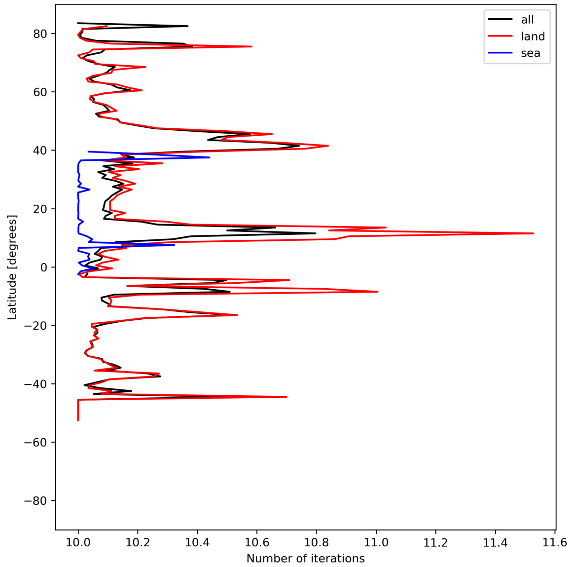
Figure 20: Zonal average of “Number of iterations” for 2024-04-19 to 2024-04-21.
