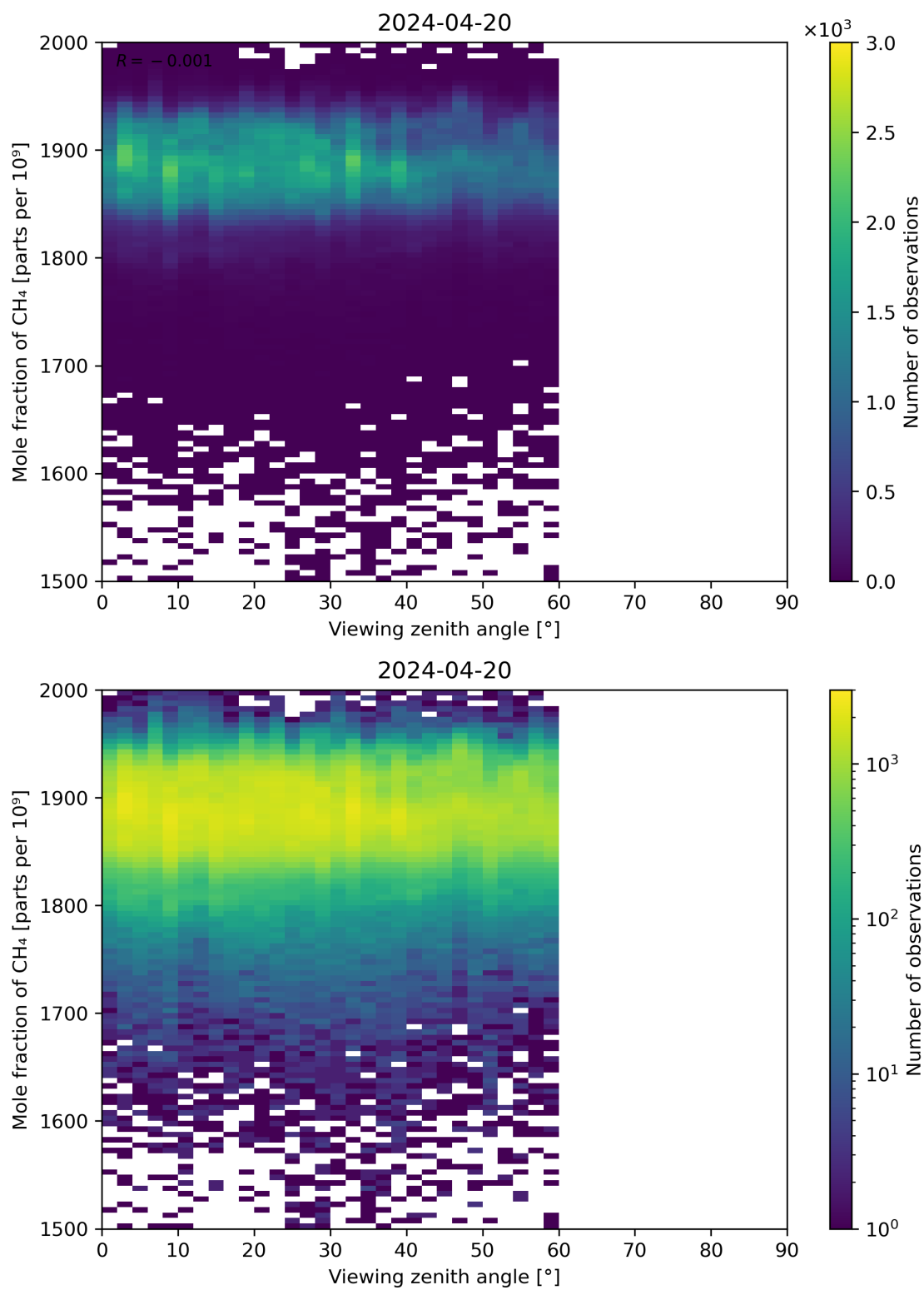
Figure 110: Scatter density plot of “Viewing zenith angle” against “Mole fraction of CH 4 ” for 2024-04-19 to 2024-04-21.
