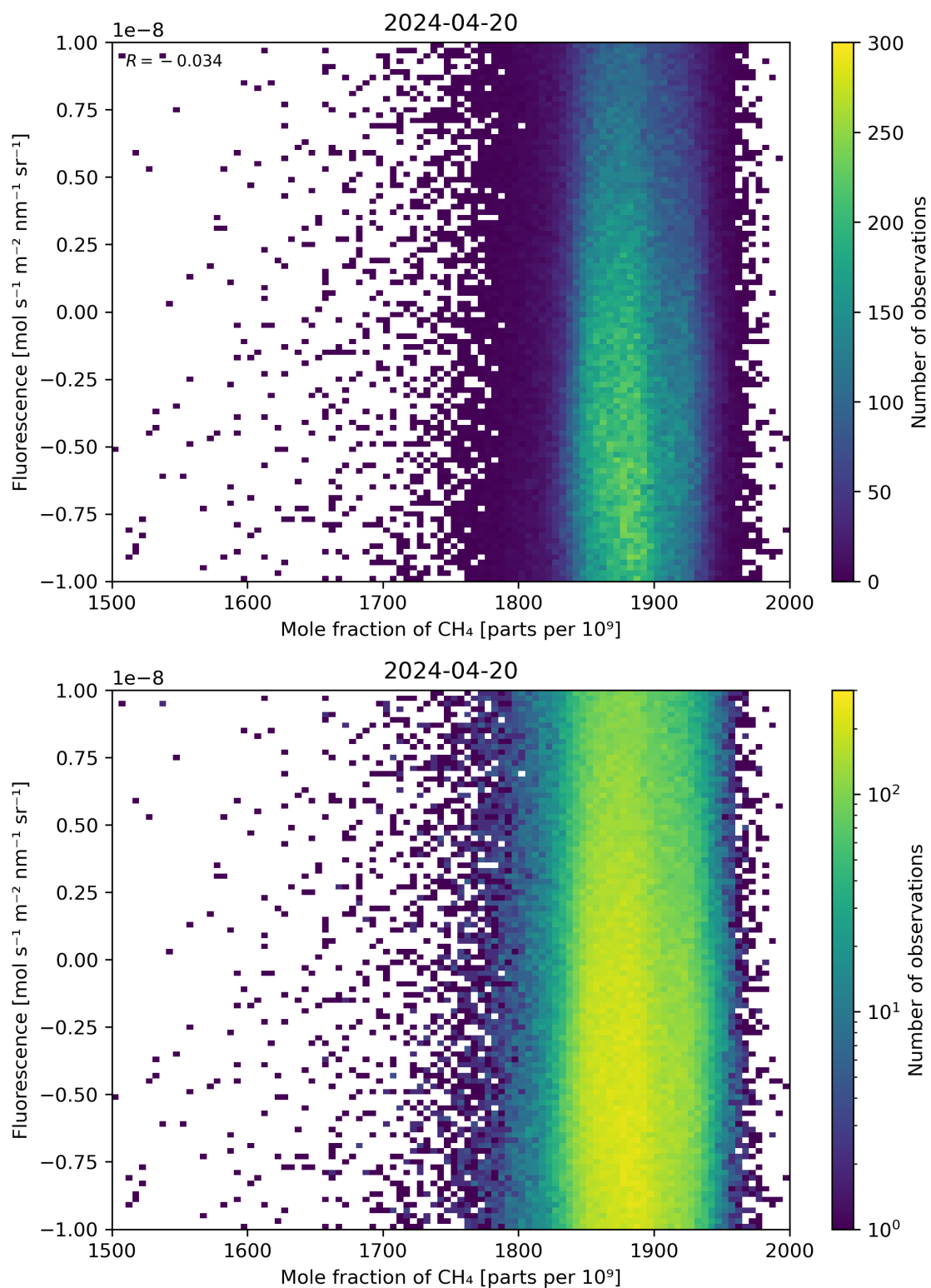
Figure 73: Scatter density plot of “Mole fraction of \text{CH}_4 ” against “Fluorescence” for 2024-04-19 to 2024-04-21.
