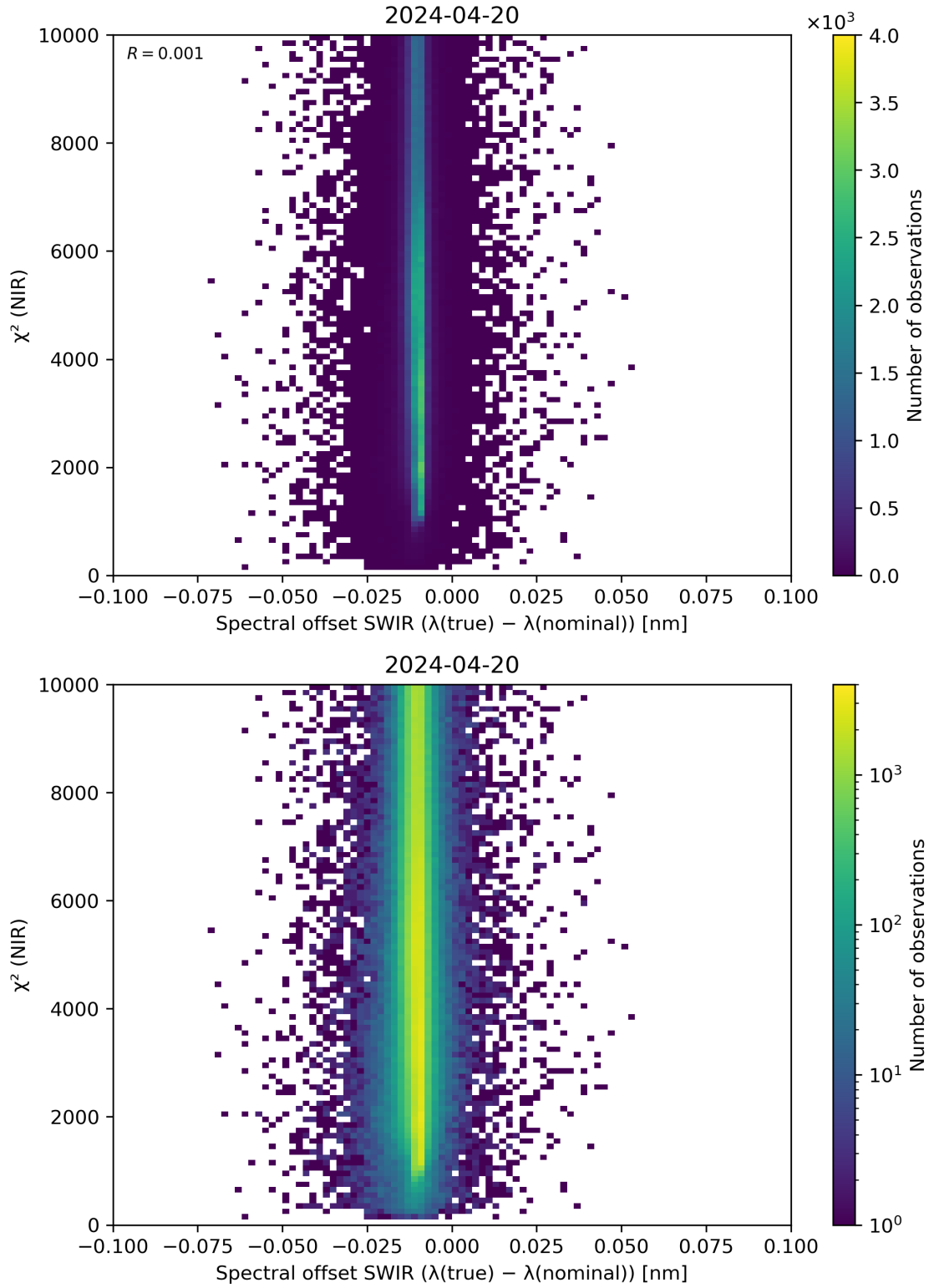
Figure 117: Scatter density plot of “Spectral offset SWIR ( \lambda(\text{true}) - \lambda(\text{nominal}) )” against “ \chi^2 (NIR)” for 2024-04-19 to 2024-04-21.
