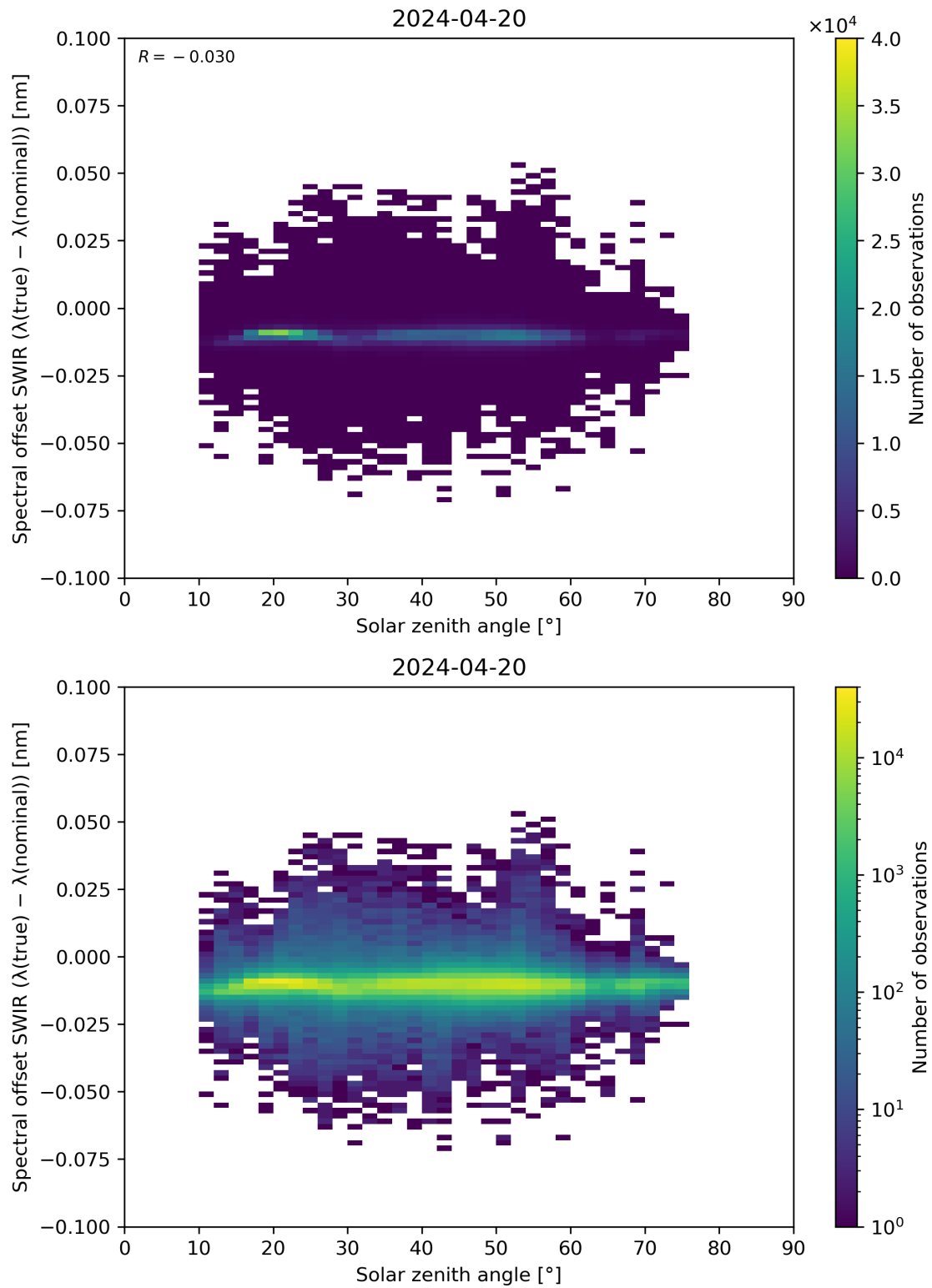
Figure 104: Scatter density plot of “Solar zenith angle” against “Spectral offset SWIR ( \lambda(\text{true}) - \lambda(\text{nominal}) )” for 2024-04-19 to 2024-04-21.
