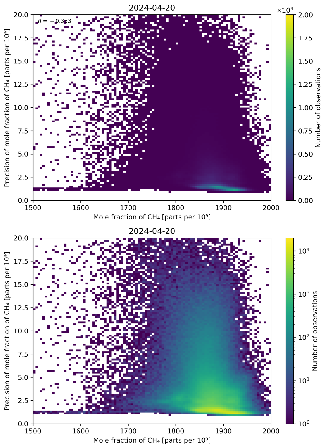
Figure 75: Scatter density plot of “Mole fraction of CH 4 ” against “Precision of mole fraction of CH 4 ” for 2024-04-19 to 2024-04-21.
