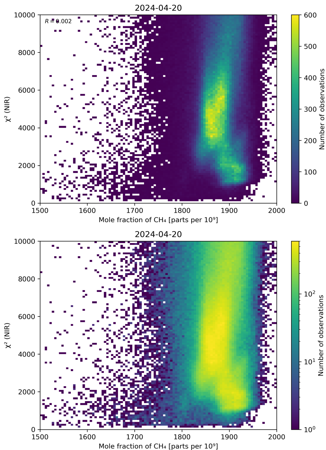
Figure 70: Scatter density plot of “Mole fraction of CH 4 ” against “ \chi^2 (NIR)” for 2024-04-19 to 2024-04-21.
