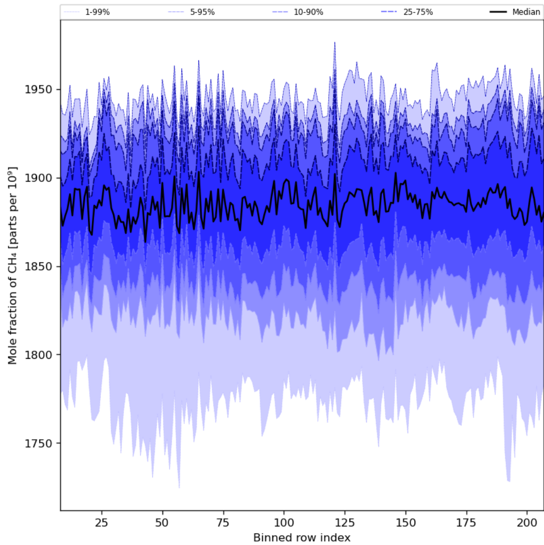
Figure 34: Along track statistics of “Mole fraction of CH 4 ” for 2024-04-19 to 2024-04-21
