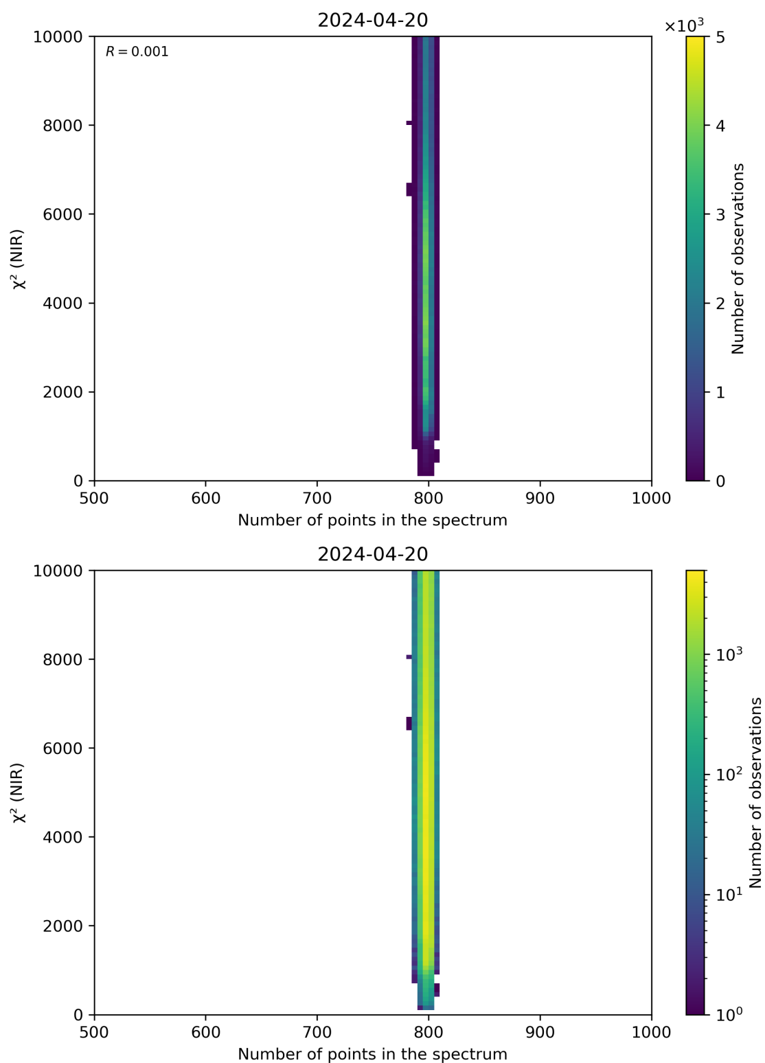
Figure 88: Scatter density plot of “Number of points in the spectrum” against “ \chi^2 (NIR)” for 2024-04-19 to 2024-04-21.
