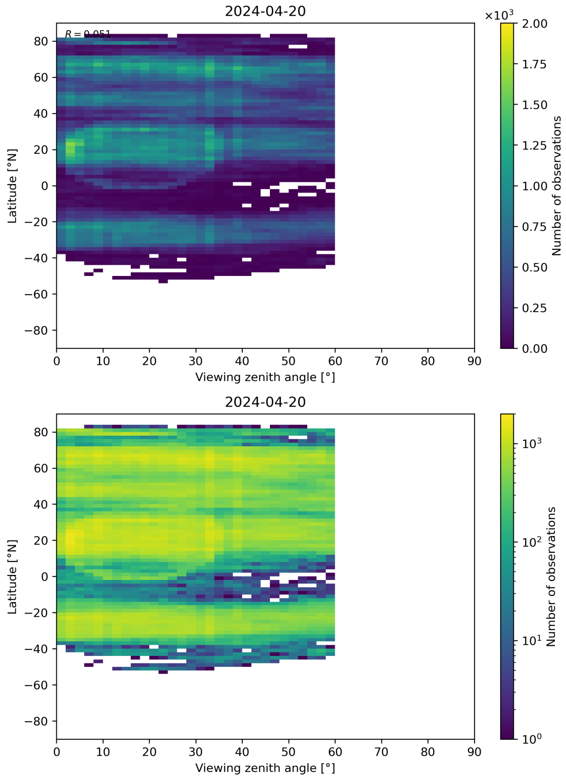
Figure 109: Scatter density plot of “Viewing zenith angle” against “Latitude” for 2024-04-19 to 2024-04-21.
