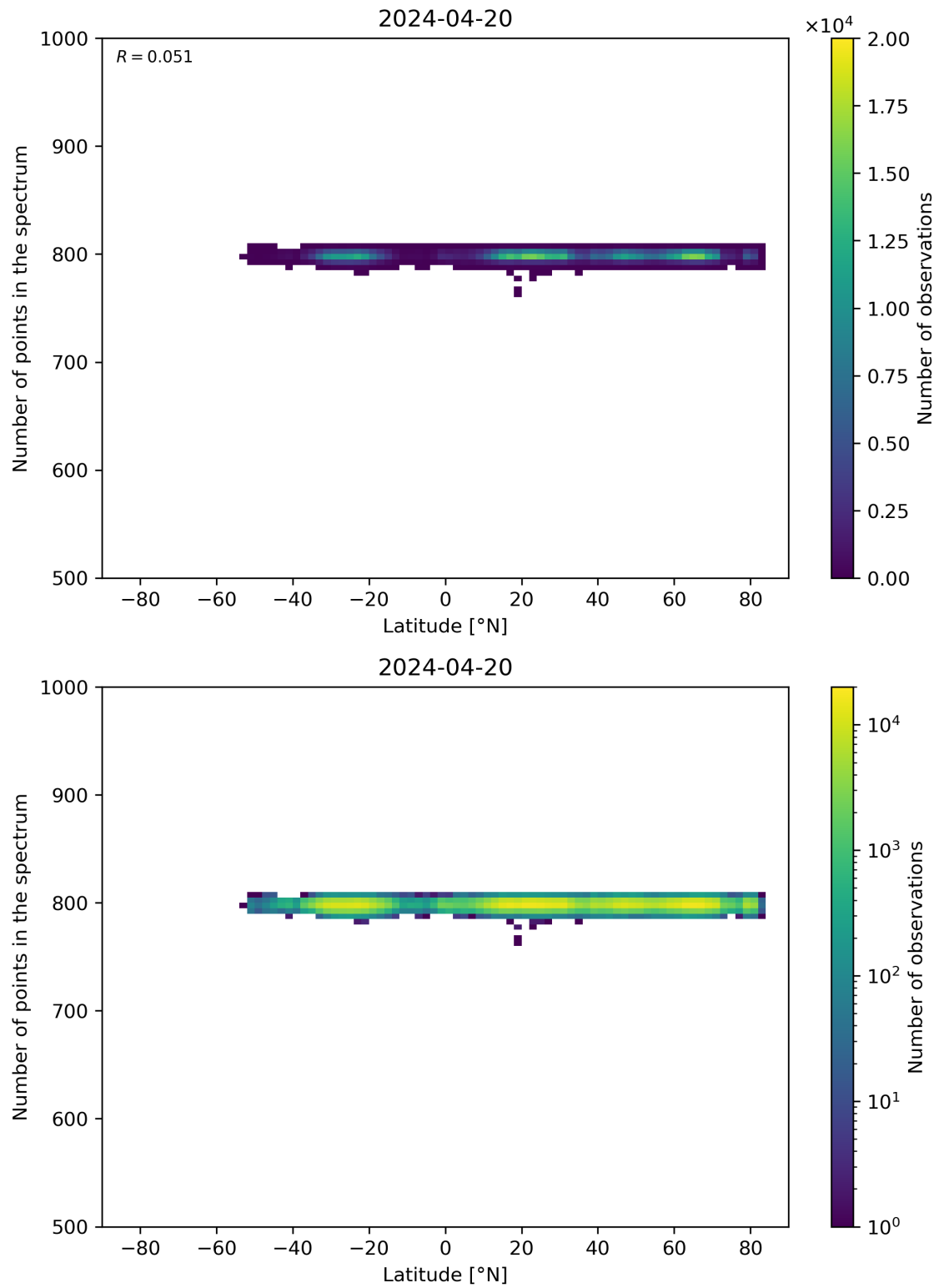
Figure 61: Scatter density plot of “Latitude” against “Number of points in the spectrum” for 2024-04-19 to 2024-04-21.
