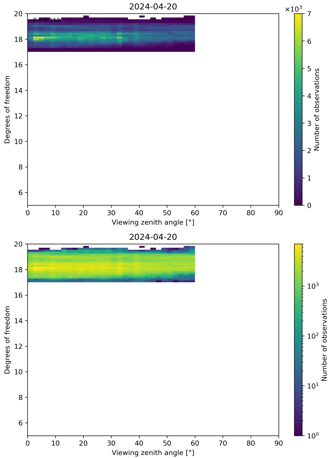
Figure 107: Scatter density plot of “Viewing zenith angle” against “Degrees of freedom” for 2024-04-19 to 2024-04-21.
