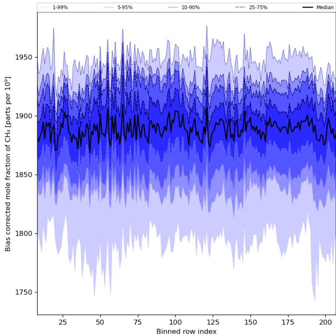
Figure 36: Along track statistics of “Bias corrected mole fraction of CH 4 ” for 2024-04-19 to 2024-04-21
