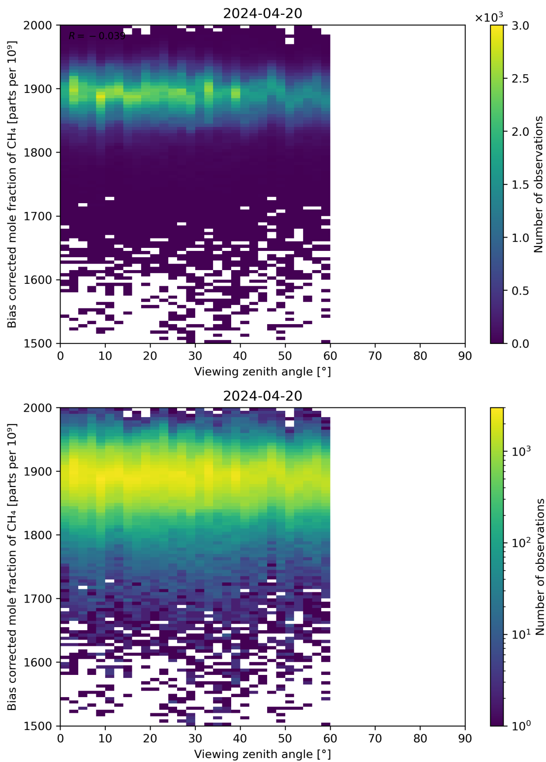
Figure 111: Scatter density plot of “Viewing zenith angle” against “Bias corrected mole fraction of CH 4 ” for 2024-04-19 to 2024-04-21.
