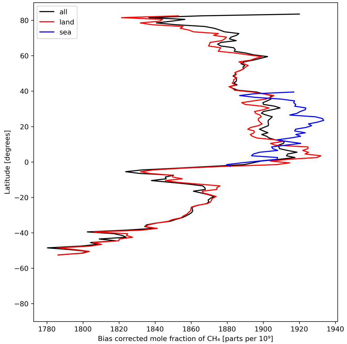
Figure 14: Zonal average of “Bias corrected mole fraction of \text{CH}_4 ” for 2024-04-19 to 2024-04-21.
