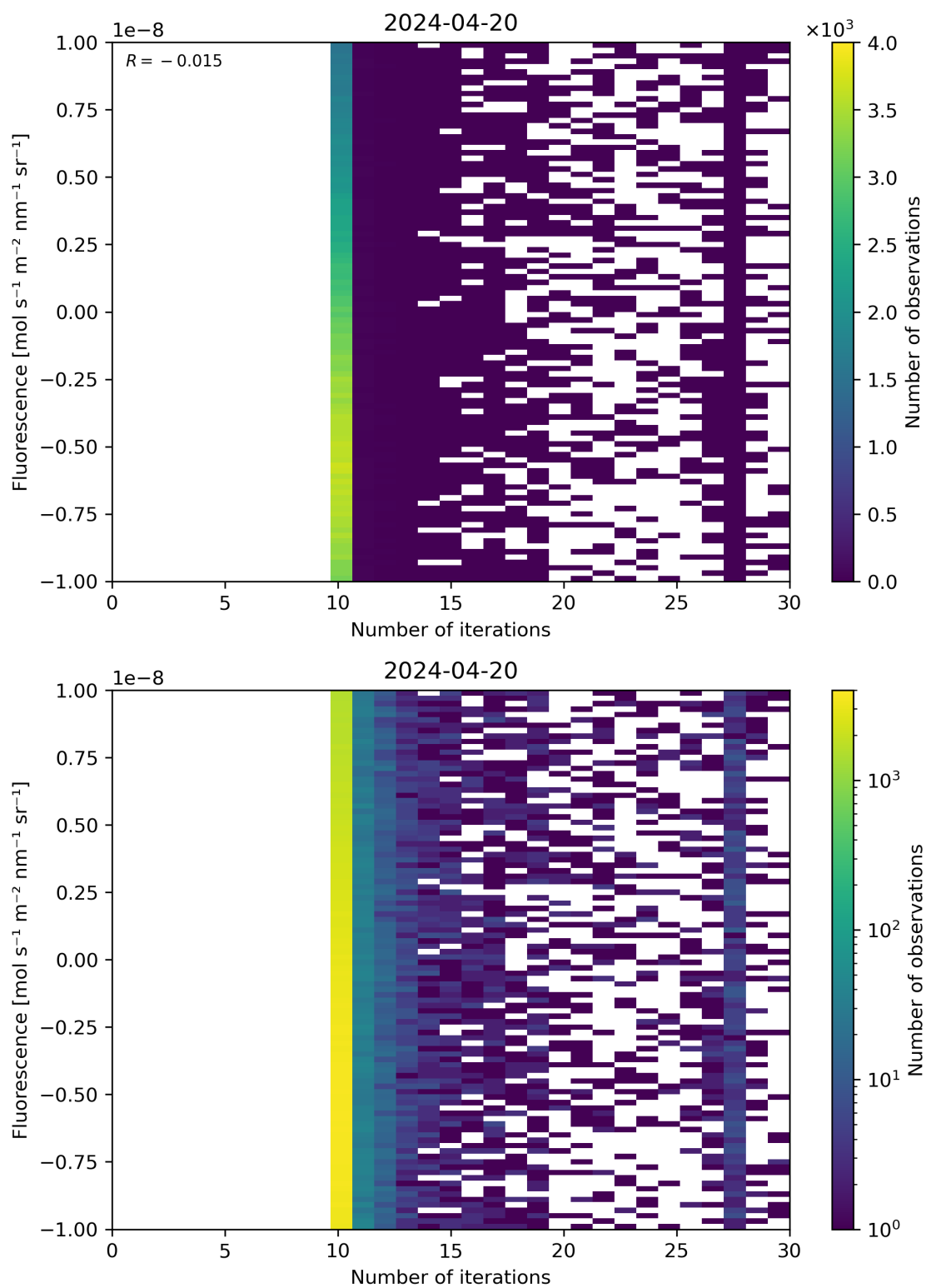
Figure 87: Scatter density plot of “Number of iterations” against “Fluorescence” for 2024-04-19 to 2024-04-21.
