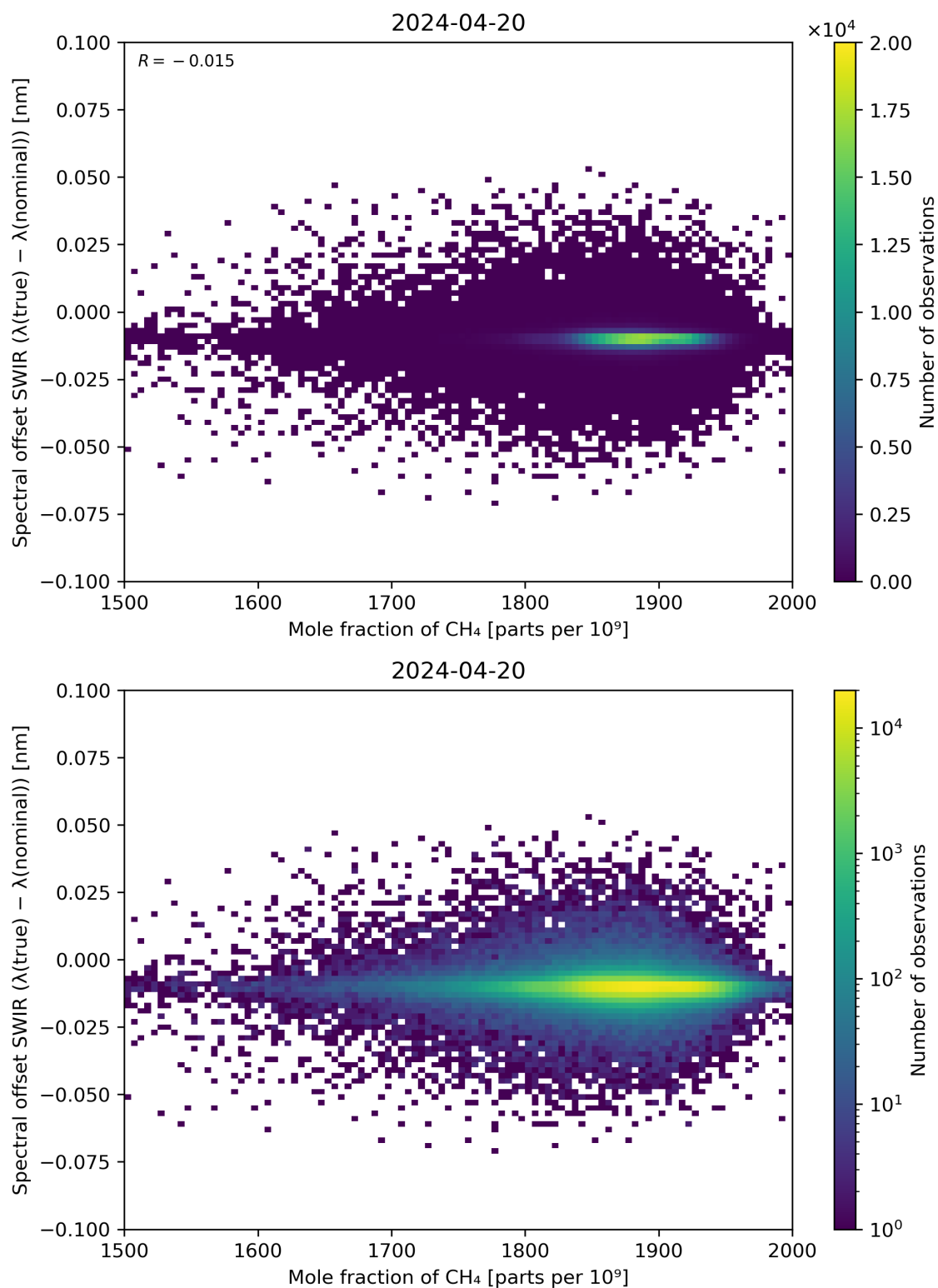
Figure 86: Scatter density plot of “Mole fraction of CH 4 ” against “Spectral offset SWIR ( \lambda(\text{true}) - \lambda(\text{nominal}) )” for 2024-04-19 to 2024-04-21.
