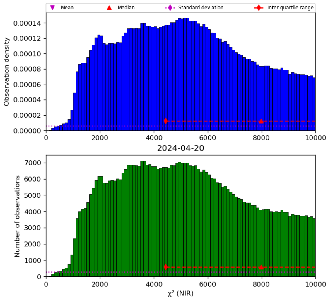
Figure 29: Histogram of “ \chi^2 (NIR)” for 2024-04-19 to 2024-04-21
