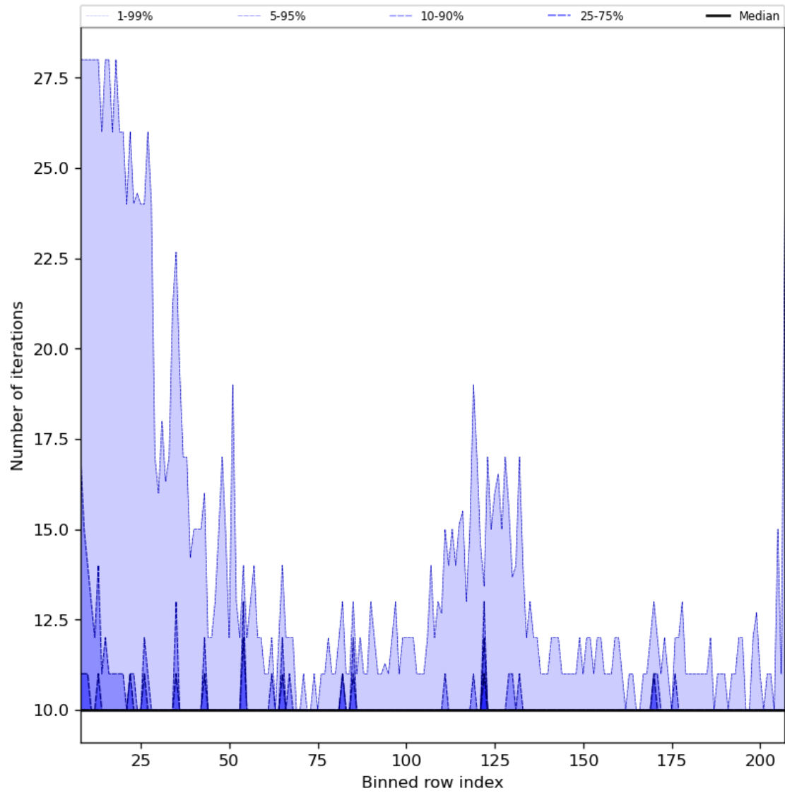
Figure 42: Along track statistics of “Number of iterations” for 2024-04-19 to 2024-04-21
