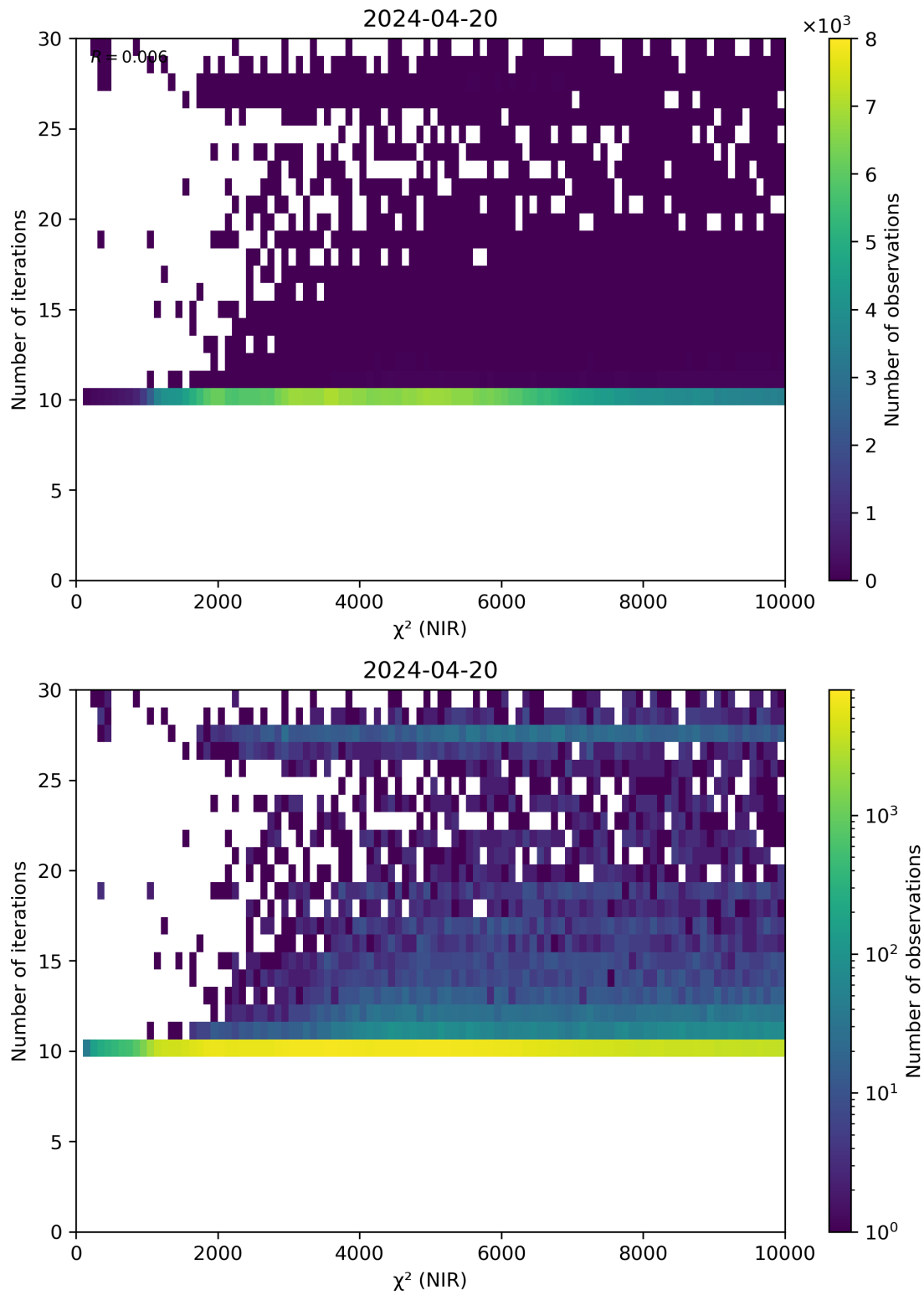
Figure 46: Scatter density plot of “ \chi^2 (NIR)” against “Number of iterations” for 2024-04-19 to 2024-04-21.
