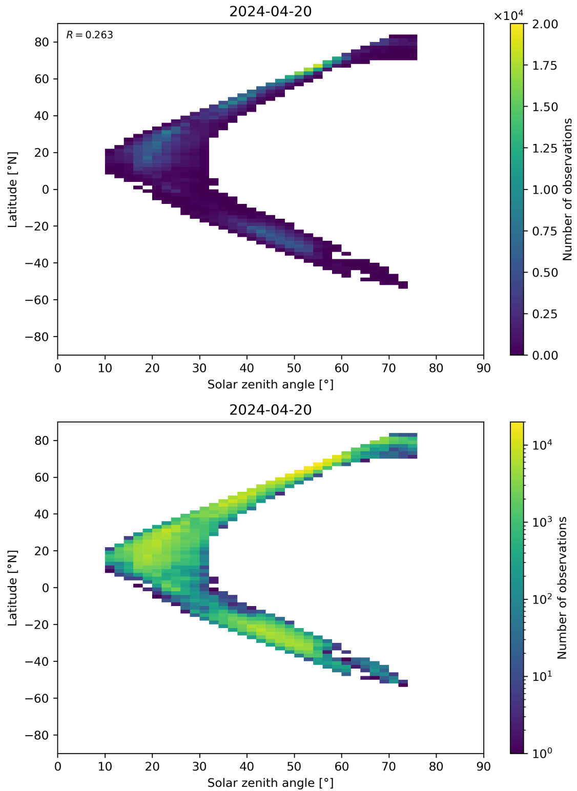
Figure 98: Scatter density plot of “Solar zenith angle” against “Latitude” for 2024-04-19 to 2024-04-21.
