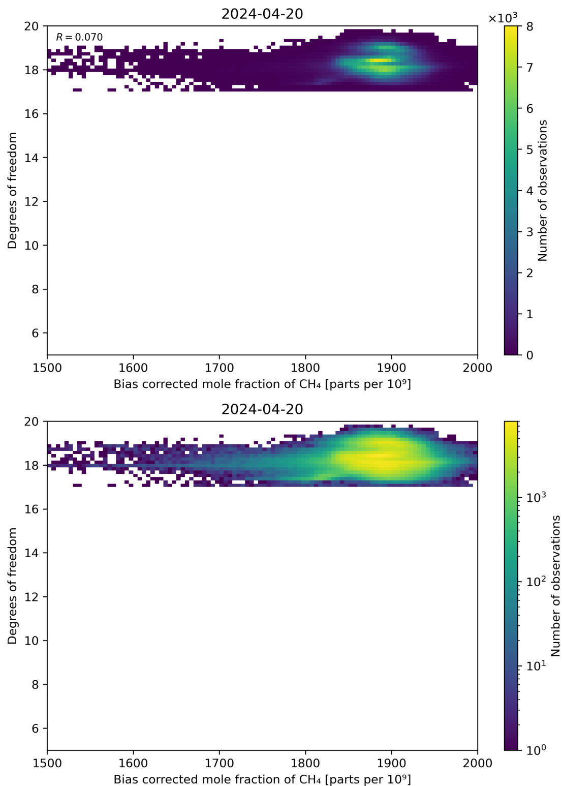
Figure 65: Scatter density plot of “Bias corrected mole fraction of CH 4 ” against “Degrees of freedom” for 2024-04-19 to 2024-04-21.
