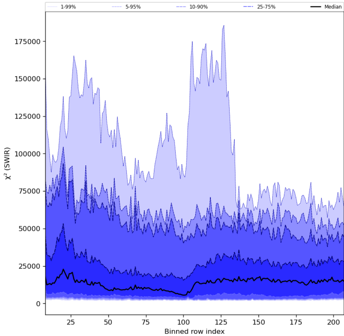
Figure 39: Along track statistics of “ \chi^2 (SWIR)” for 2024-04-19 to 2024-04-21
