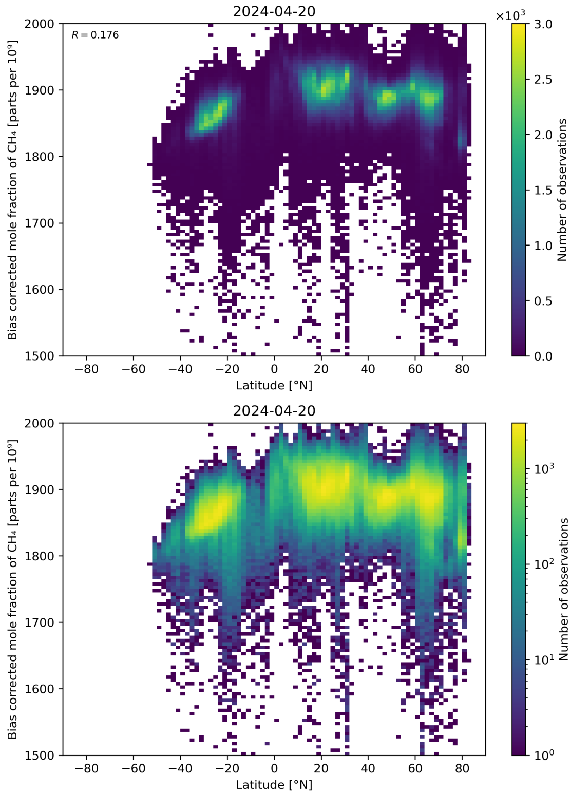
Figure 58: Scatter density plot of “Latitude” against “Bias corrected mole fraction of \text{CH}_4 ” for 2024-04-19 to 2024-04-21.
