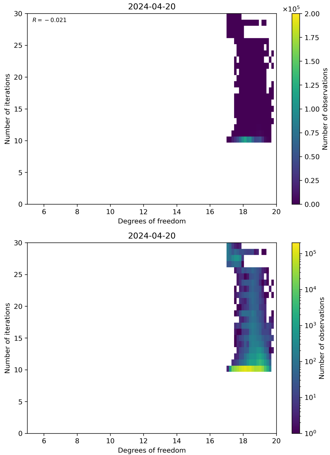
Figure 52: Scatter density plot of “Degrees of freedom” against “Number of iterations” for 2024-04-19 to 2024-04-21.
