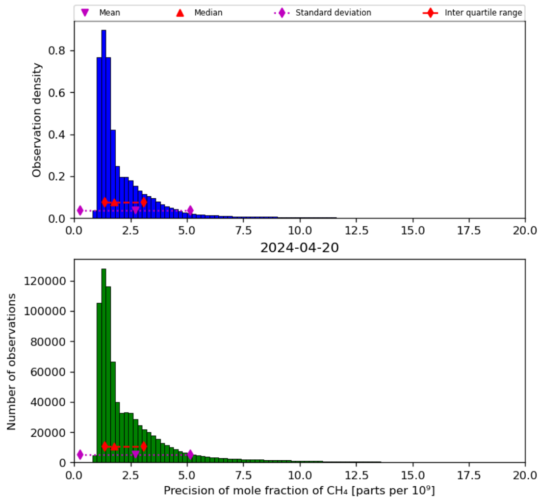
Figure 24: Histogram of “Precision of mole fraction of CH 4 ” for 2024-04-19 to 2024-04-21
