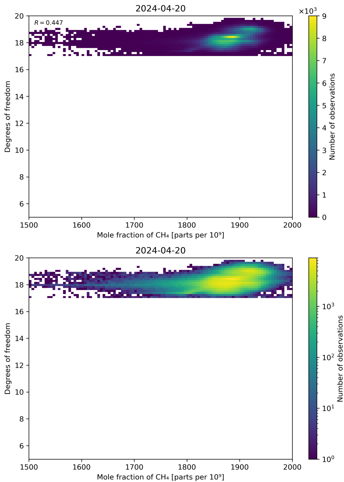
Figure 72: Scatter density plot of “Mole fraction of CH 4 ” against “Degrees of freedom” for 2024-04-19 to 2024-04-21.
