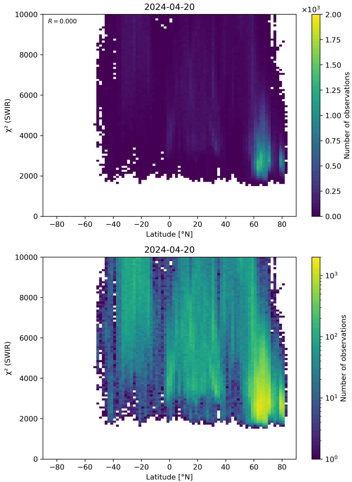
Figure 54: Scatter density plot of “Latitude” against “ \chi^2 (SWIR)” for 2024-04-19 to 2024-04-21.
