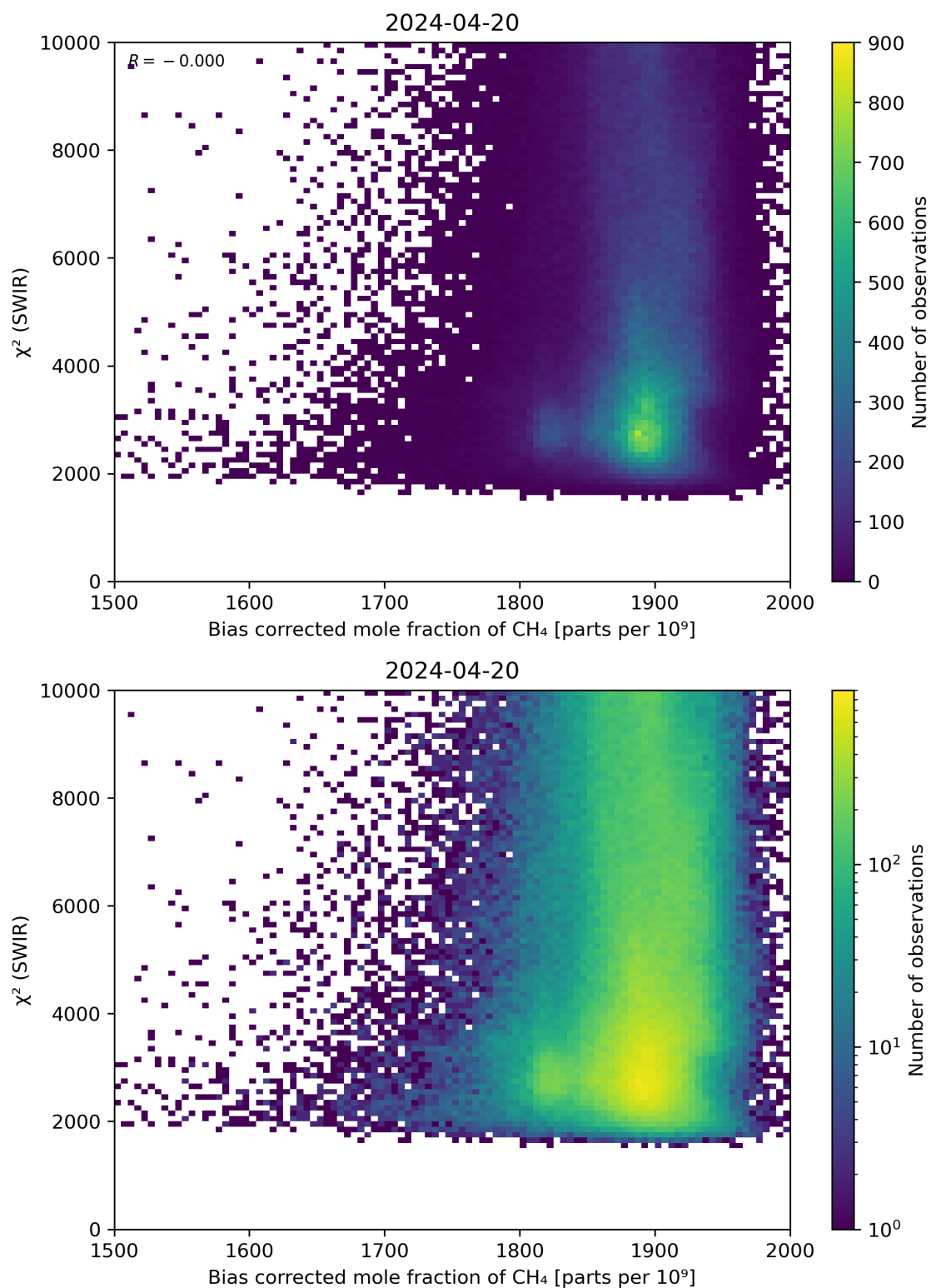
Figure 64: Scatter density plot of “Bias corrected mole fraction of CH 4 ” against “ \chi^2 (SWIR)” for 2024-04-19 to 2024-04-21.
