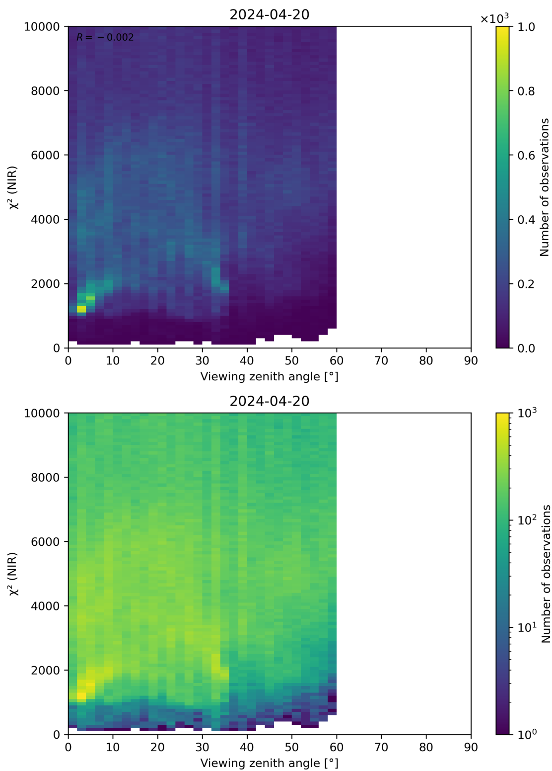
Figure 105: Scatter density plot of “Viewing zenith angle” against “ \chi^2 (NIR)” for 2024-04-19 to 2024-04-21.
