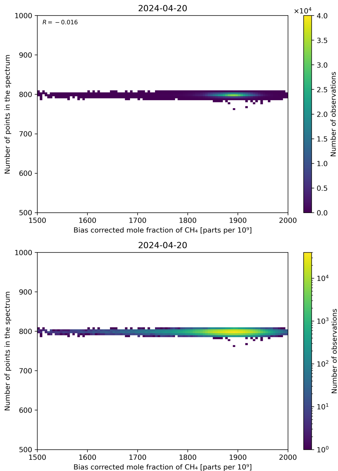
Figure 68: Scatter density plot of “Bias corrected mole fraction of CH 4 ” against “Number of points in the spectrum” for 2024-04-19 to 2024-04-21.
