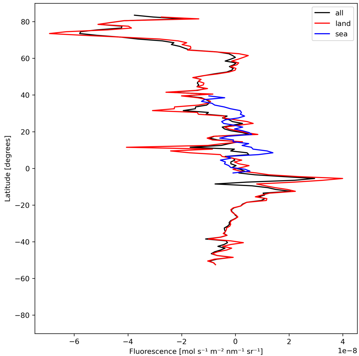
Figure 21: Zonal average of “Fluorescence” for 2024-04-19 to 2024-04-21.
