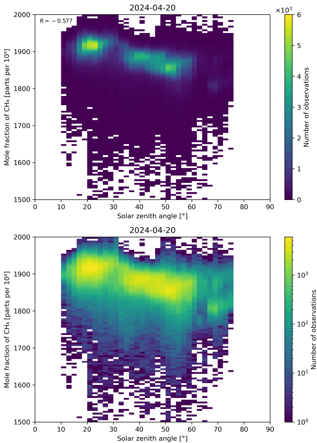
Figure 99: Scatter density plot of “Solar zenith angle” against “Mole fraction of CH 4 ” for 2024-04-19 to 2024-04-21.
