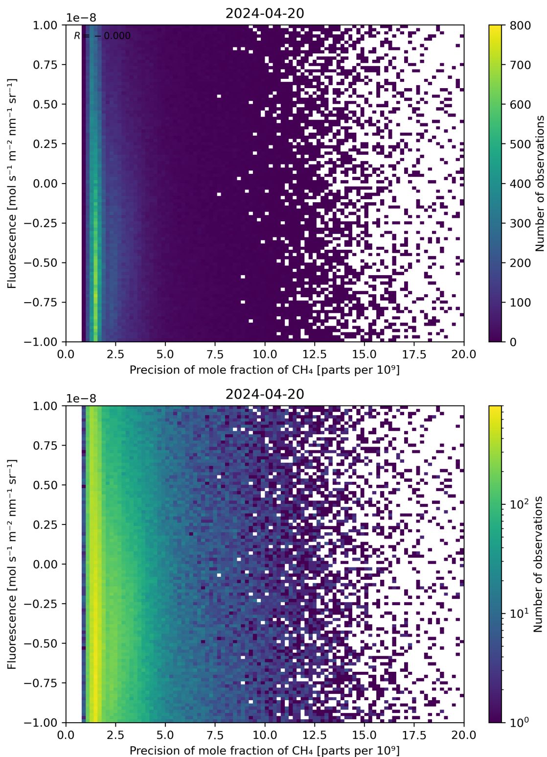
Figure 81: Scatter density plot of “Precision of mole fraction of \text{CH}_4 ” against “Fluorescence” for 2024-04-19 to 2024-04-21.
