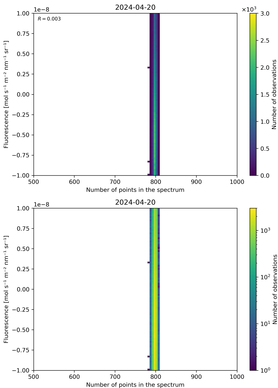
Figure 91: Scatter density plot of “Number of points in the spectrum” against “Fluorescence” for 2024-04-19 to 2024-04-21.
