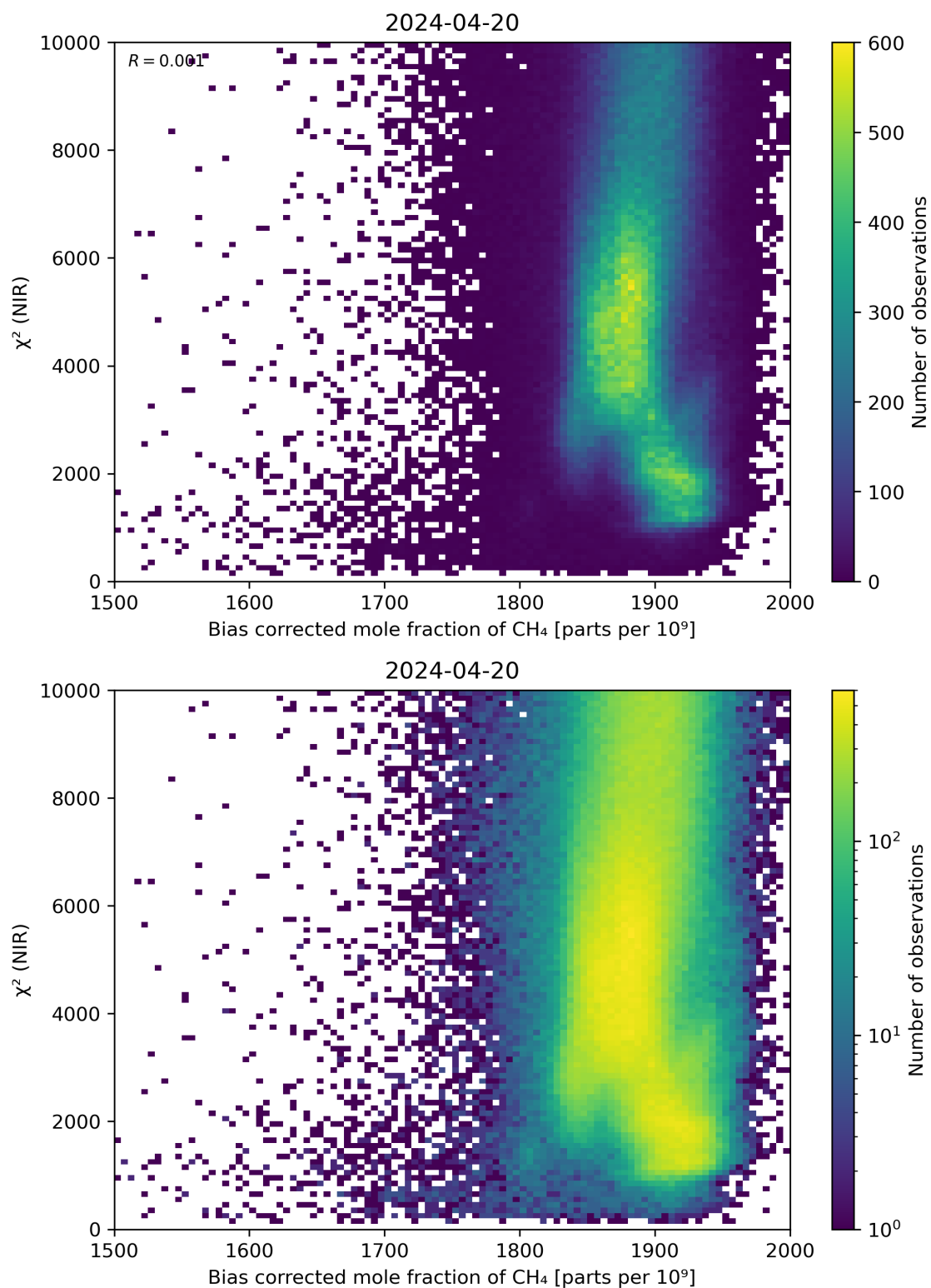
Figure 63: Scatter density plot of “Bias corrected mole fraction of CH 4 ” against “ \chi^2 (NIR)” for 2024-04-19 to 2024-04-21.
