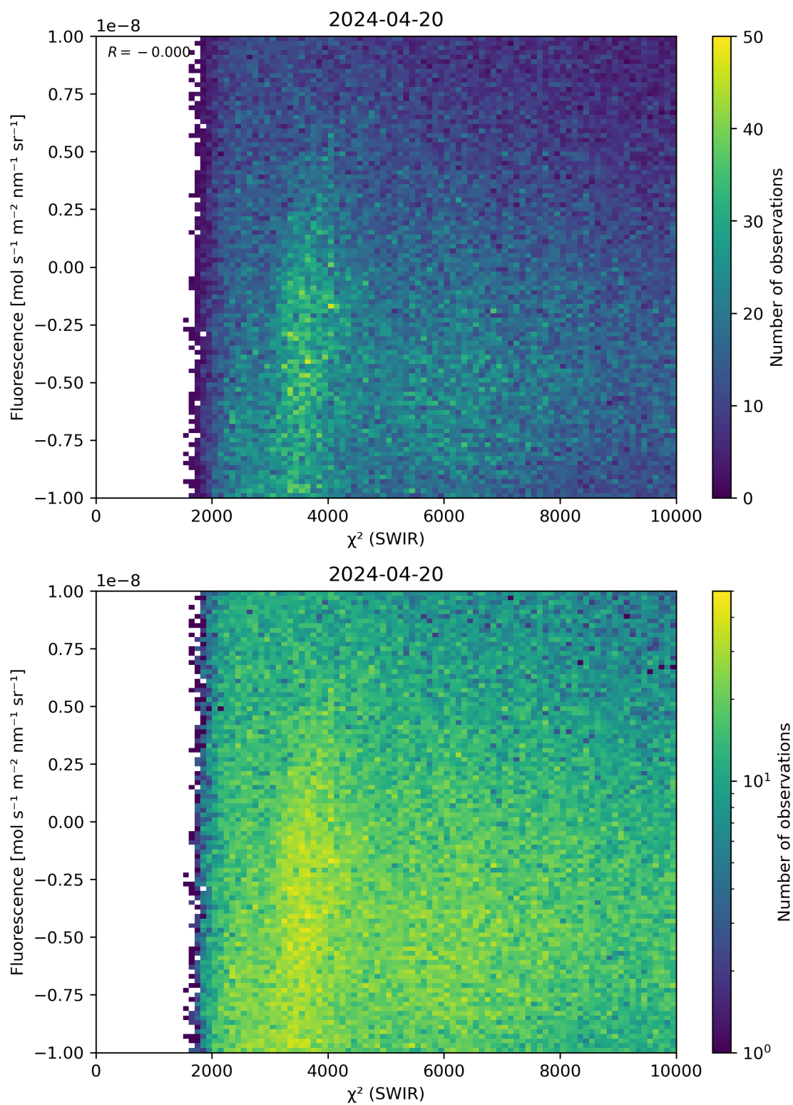
Figure 49: Scatter density plot of “ \chi^2 (SWIR)” against “Fluorescence” for 2024-04-19 to 2024-04-21.
