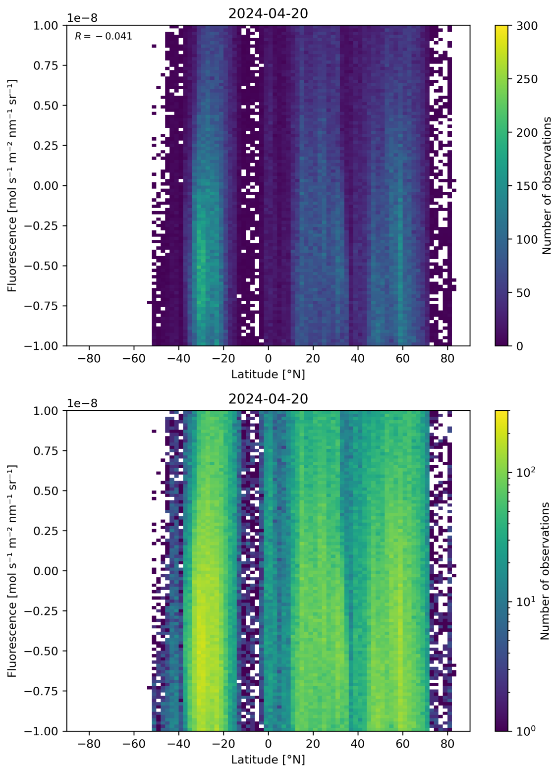
Figure 56: Scatter density plot of “Latitude” against “Fluorescence” for 2024-04-19 to 2024-04-21.
