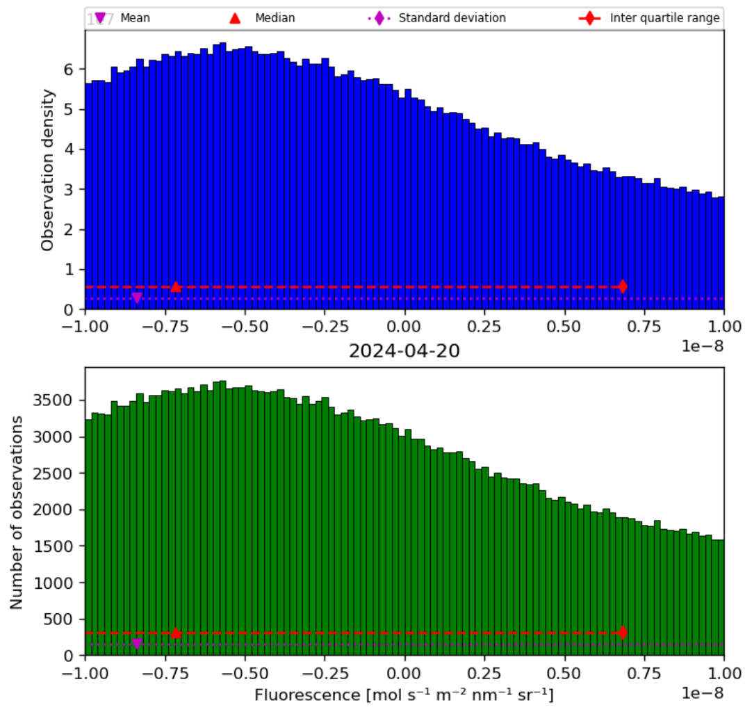
Figure 32: Histogram of “Fluorescence” for 2024-04-19 to 2024-04-21
