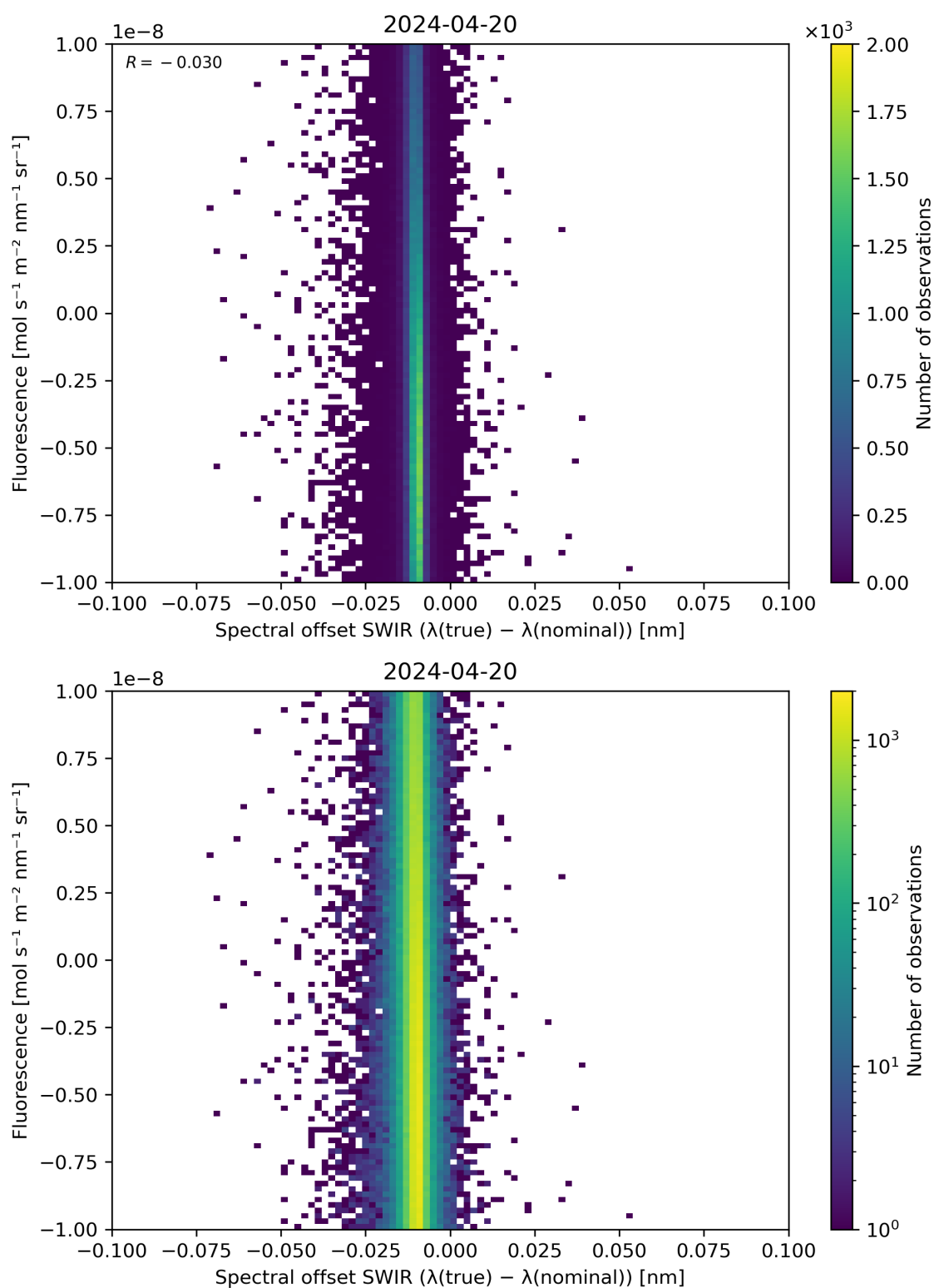
Figure 120: Scatter density plot of “Spectral offset SWIR ( \lambda(\text{true}) - \lambda(\text{nominal}) )” against “Fluorescence” for 2024-04-19 to 2024-04-21.
