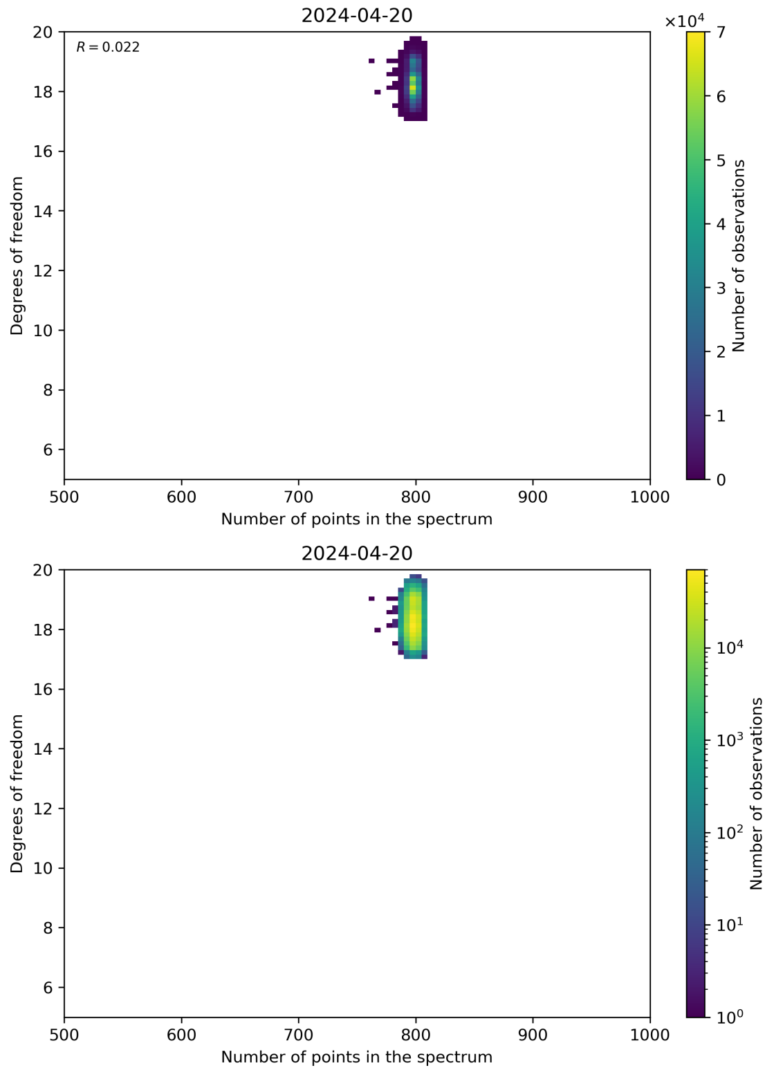
Figure 90: Scatter density plot of “Number of points in the spectrum” against “Degrees of freedom” for 2024-04-19 to 2024-04-21.
