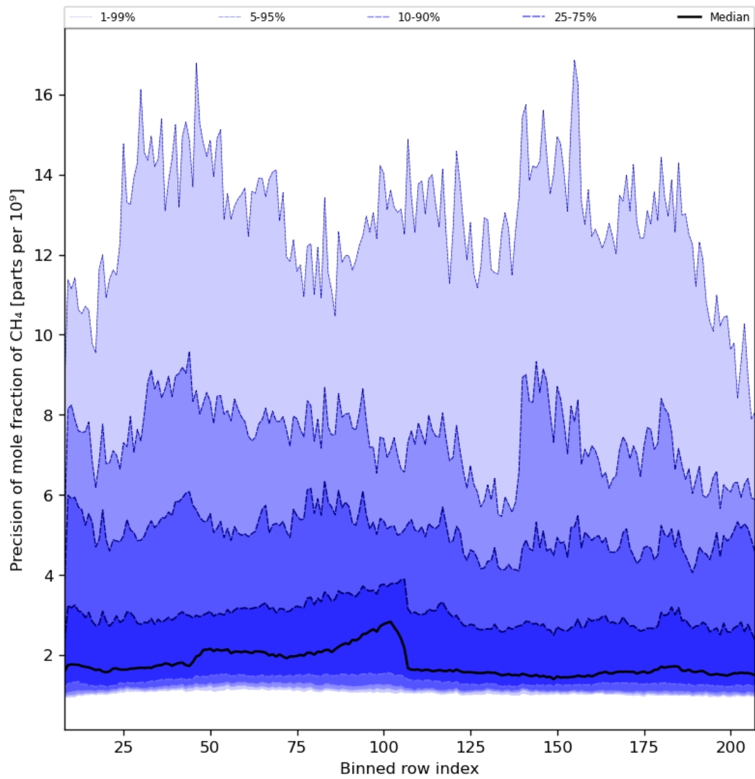
Figure 35: Along track statistics of “Precision of mole fraction of CH 4 ” for 2024-04-19 to 2024-04-21
