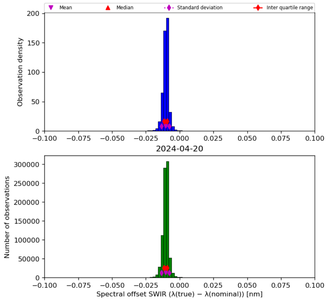
Figure 27: Histogram of “Spectral offset SWIR ( \lambda(\text{true}) - \lambda(\text{nominal}) )” for 2024-04-19 to 2024-04-21
