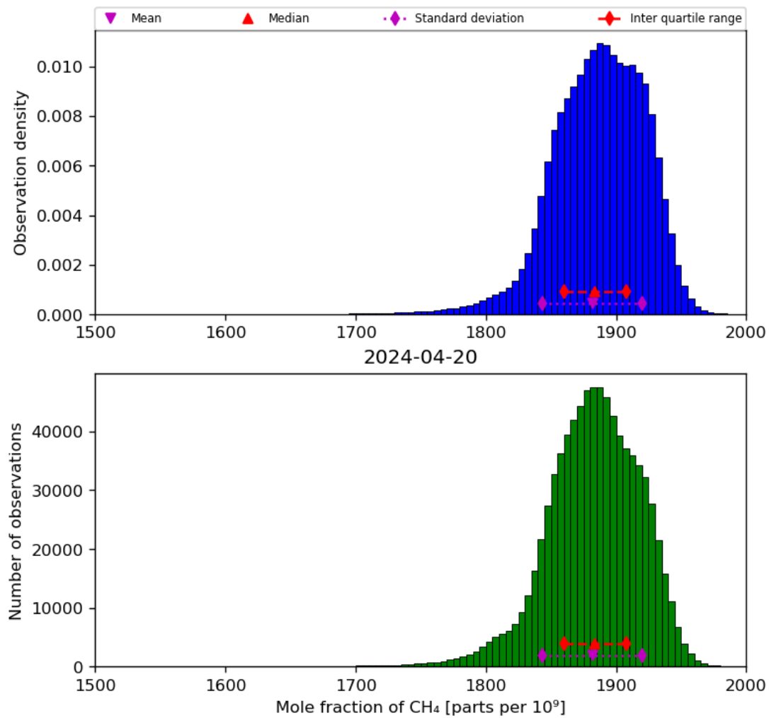
Figure 23: Histogram of “Mole fraction of CH 4 ” for 2024-04-19 to 2024-04-21
