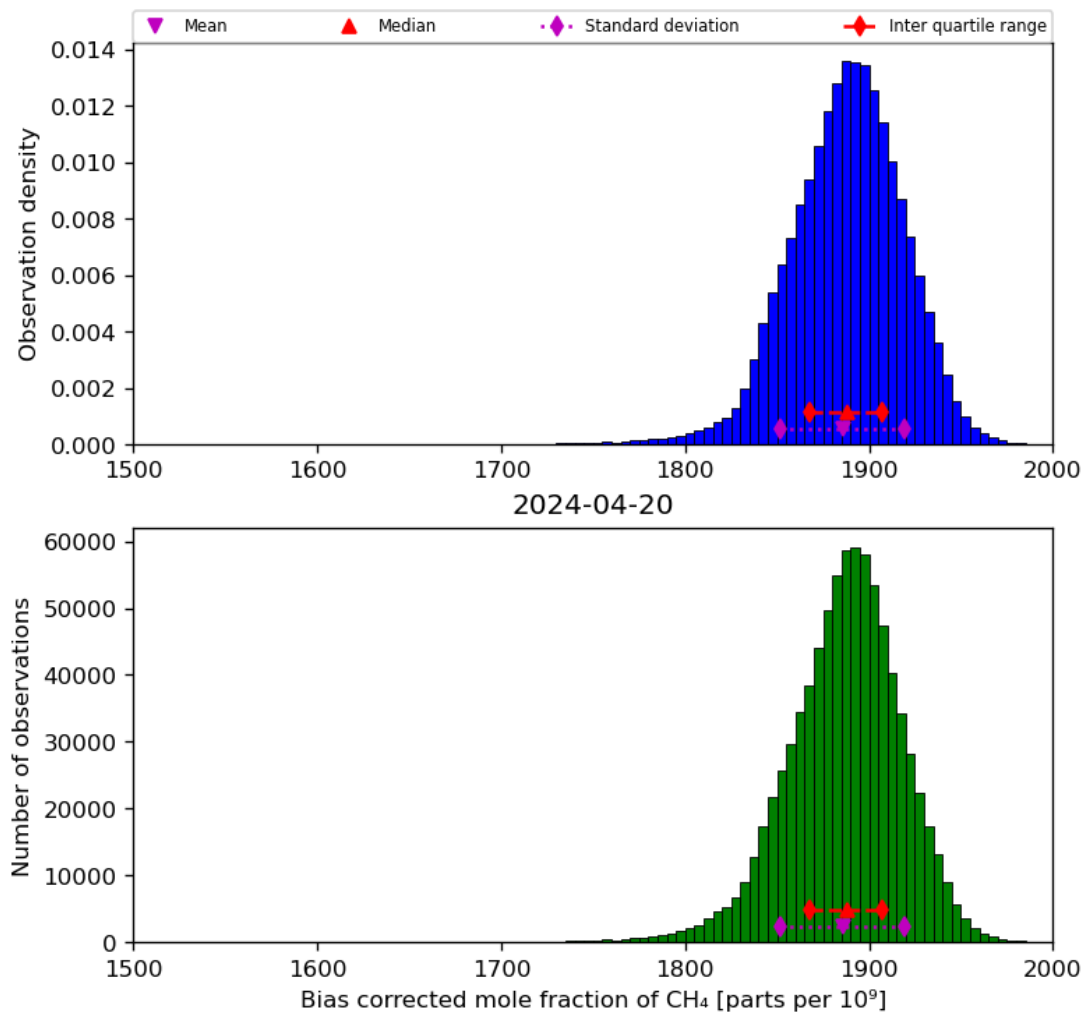
Figure 25: Histogram of “Bias corrected mole fraction of CH 4 ” for 2024-04-19 to 2024-04-21
