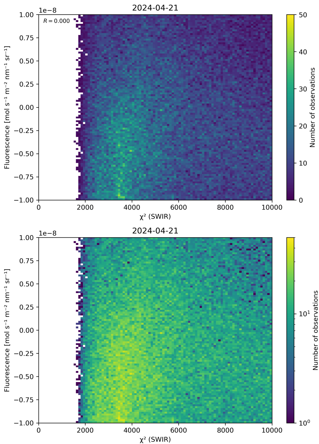
Figure 49: Scatter density plot of “ \chi^2 (SWIR)” against “Fluorescence” for 2024-04-21 to 2024-04-22.
