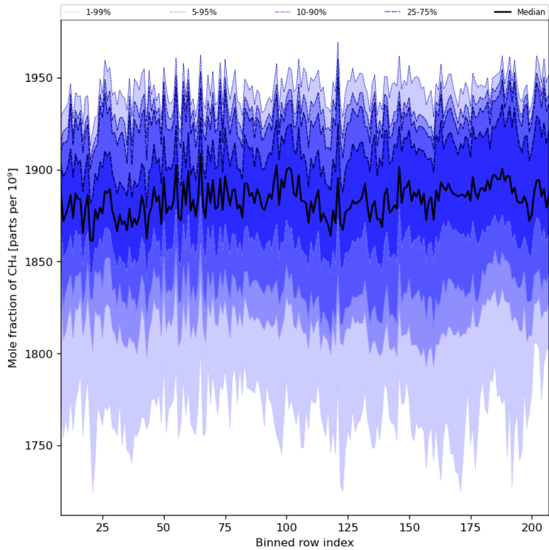
Figure 34: Along track statistics of “Mole fraction of CH 4 ” for 2024-04-21 to 2024-04-22
