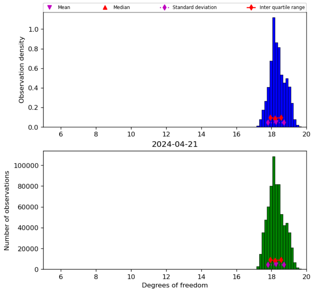
Figure 30: Histogram of “Degrees of freedom” for 2024-04-21 to 2024-04-22
