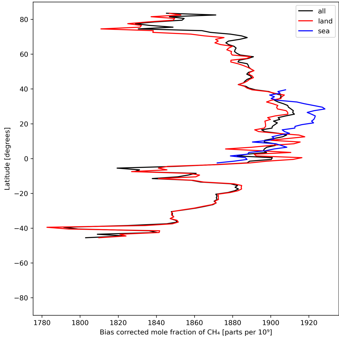
Figure 14: Zonal average of “Bias corrected mole fraction of CH 4 ” for 2024-04-21 to 2024-04-22.
