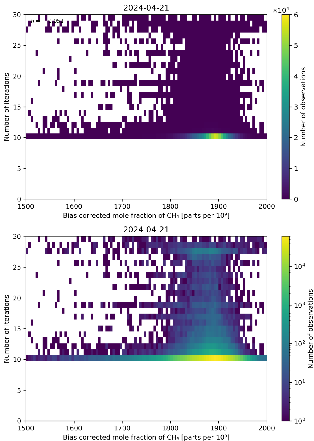
Figure 67: Scatter density plot of “Bias corrected mole fraction of CH 4 ” against “Number of iterations” for 2024-04-21 to 2024-04-22.
