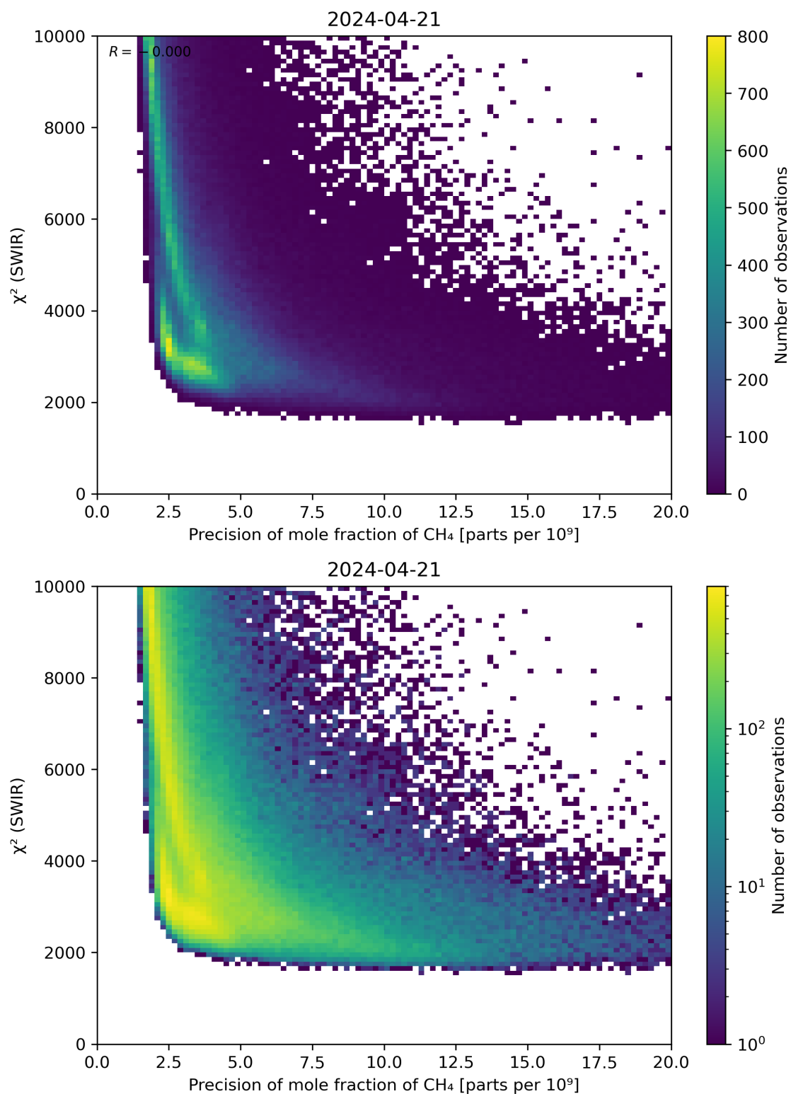
Figure 79: Scatter density plot of “Precision of mole fraction of \text{CH}_4 ” against “ \chi^2 (SWIR)” for 2024-04-21 to 2024-04-22.
