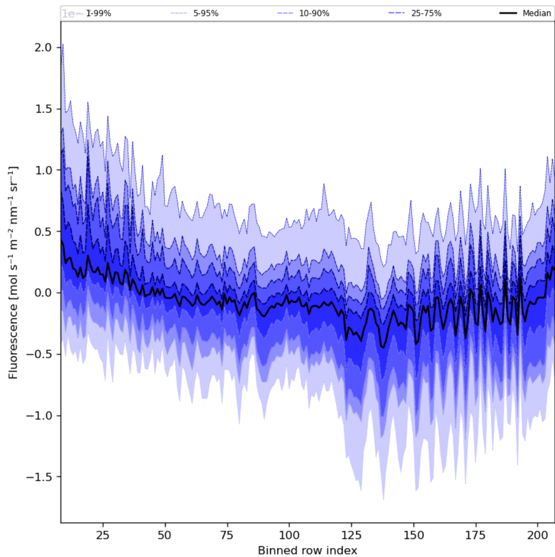
Figure 43: Along track statistics of “Fluorescence” for 2024-04-21 to 2024-04-22
