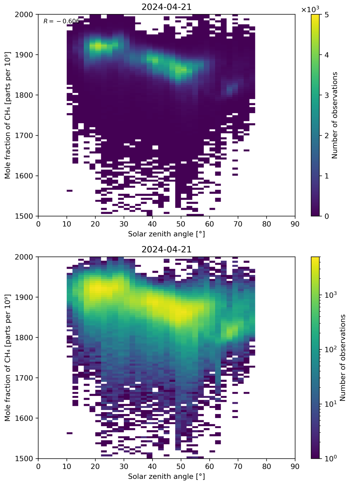
Figure 99: Scatter density plot of “Solar zenith angle” against “Mole fraction of CH 4 ” for 2024-04-21 to 2024-04-22.
