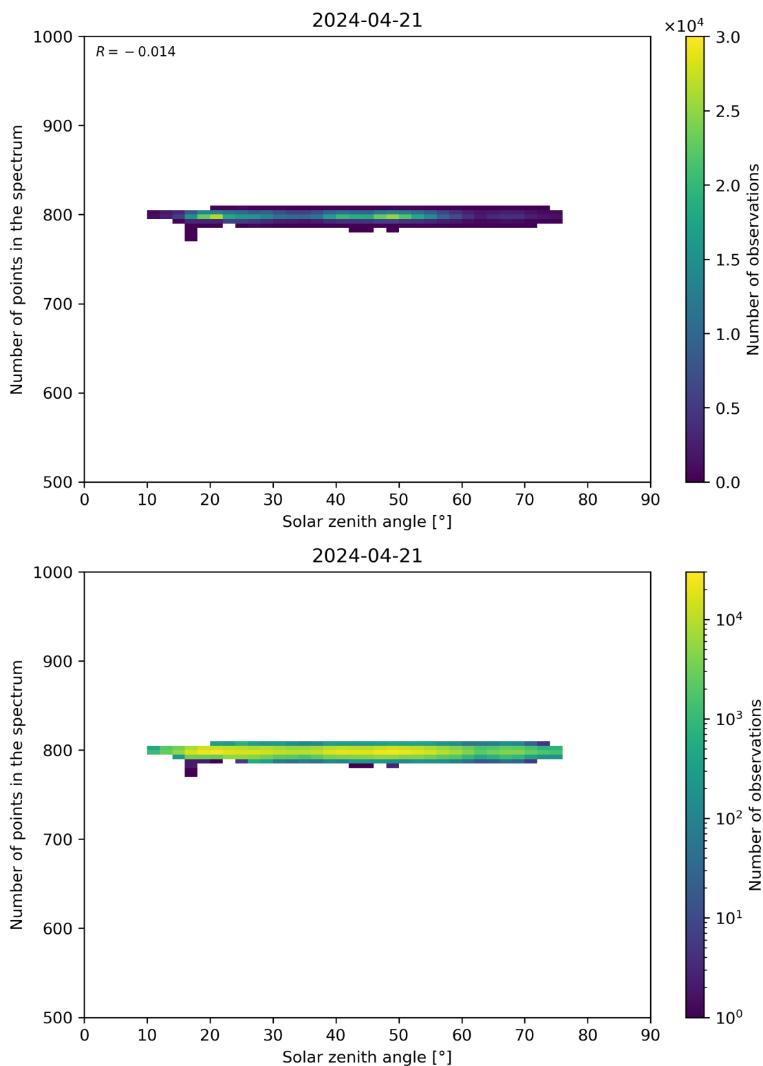
Figure 103: Scatter density plot of “Solar zenith angle” against “Number of points in the spectrum” for 2024-04-21 to 2024-04-22.
