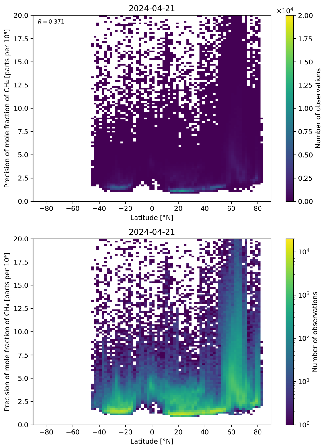
Figure 59: Scatter density plot of “Latitude” against “Precision of mole fraction of CH 4 ” for 2024-04-21 to 2024-04-22.
