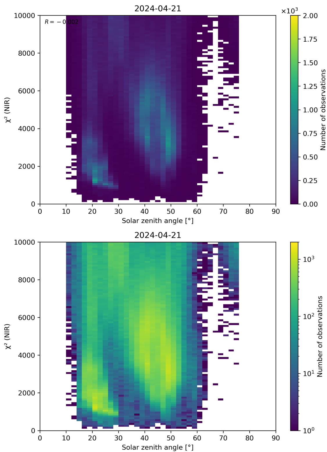
Figure 94: Scatter density plot of “Solar zenith angle” against “ \chi^2 (NIR)” for 2024-04-21 to 2024-04-22.
