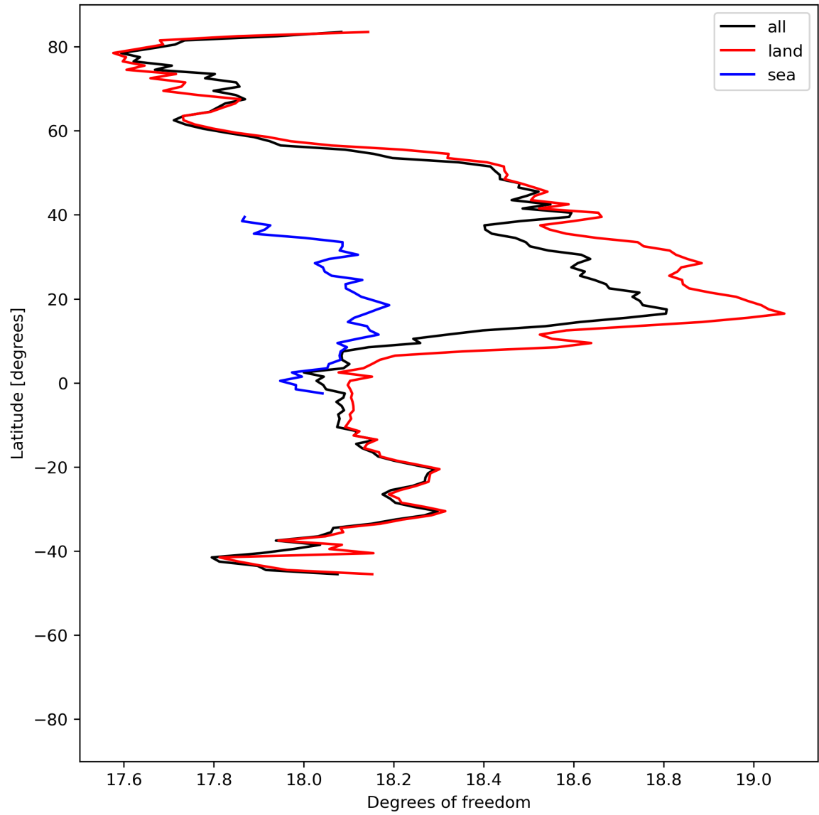
Figure 19: Zonal average of “Degrees of freedom” for 2024-04-21 to 2024-04-22.
