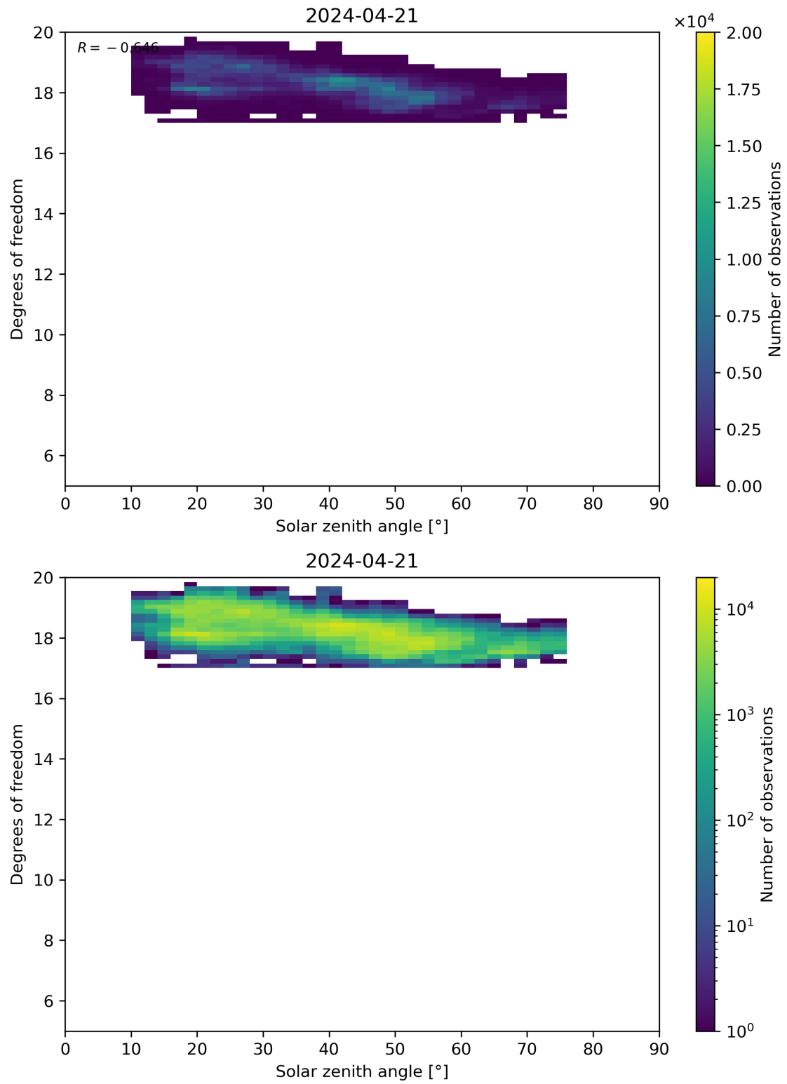
Figure 96: Scatter density plot of “Solar zenith angle” against “Degrees of freedom” for 2024-04-21 to 2024-04-22.
