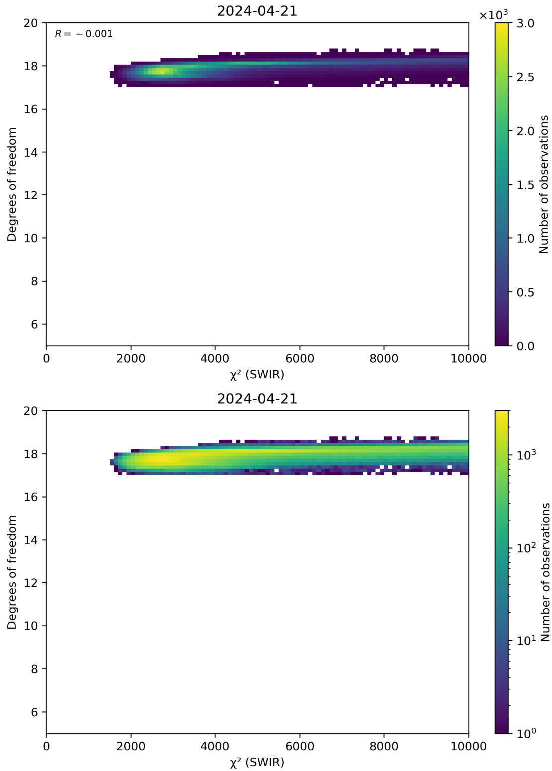
Figure 48: Scatter density plot of “ \chi^2 (SWIR)” against “Degrees of freedom” for 2024-04-21 to 2024-04-22.
