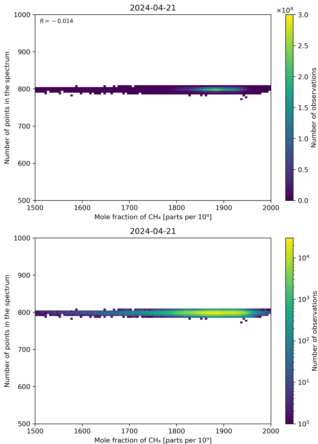
Figure 77: Scatter density plot of “Mole fraction of CH 4 ” against “Number of points in the spectrum” for 2024-04-21 to 2024-04-22.
