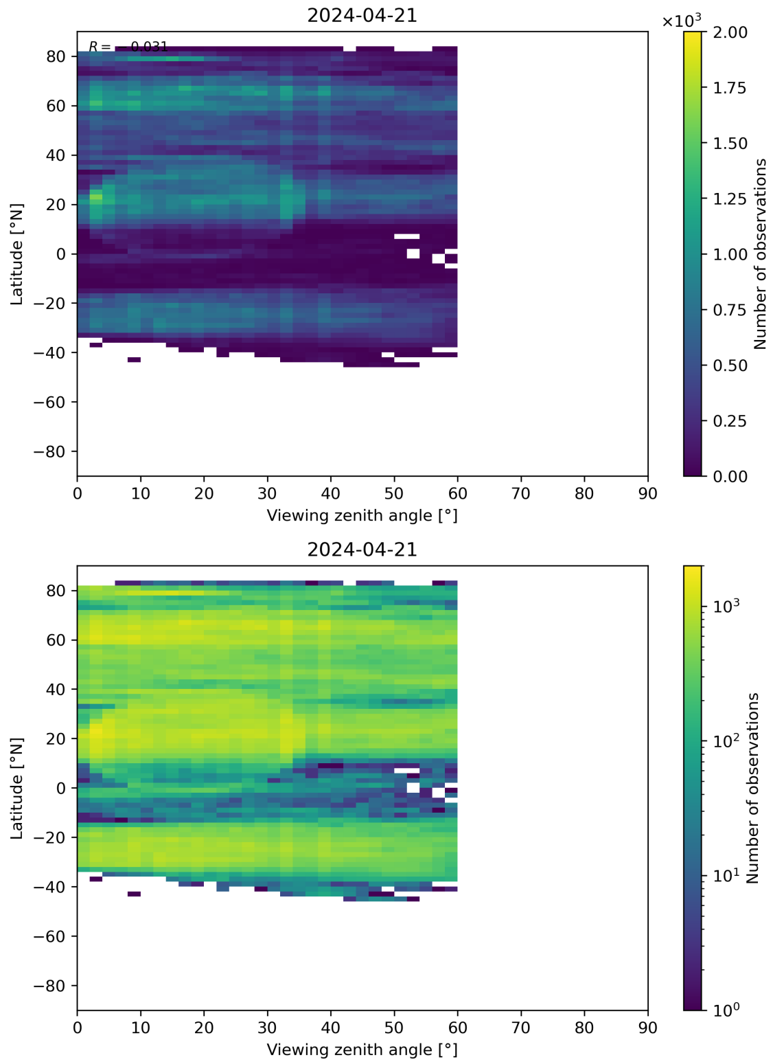
Figure 109: Scatter density plot of “Viewing zenith angle” against “Latitude” for 2024-04-21 to 2024-04-22.
