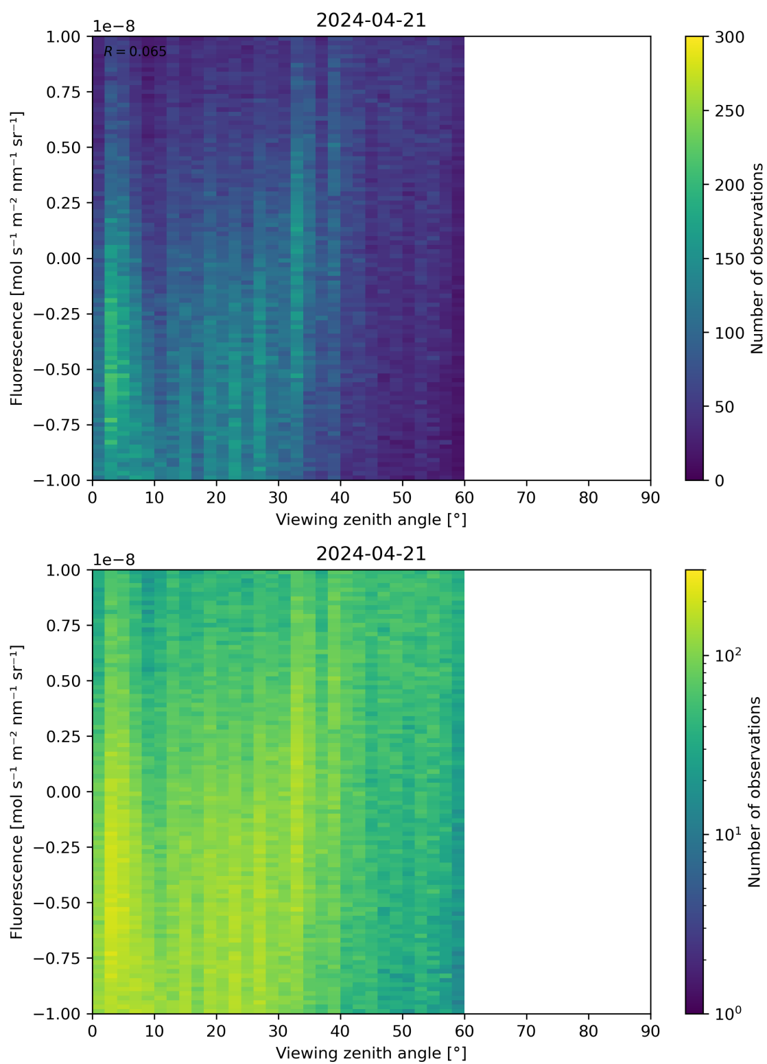
Figure 108: Scatter density plot of “Viewing zenith angle” against “Fluorescence” for 2024-04-21 to 2024-04-22.
