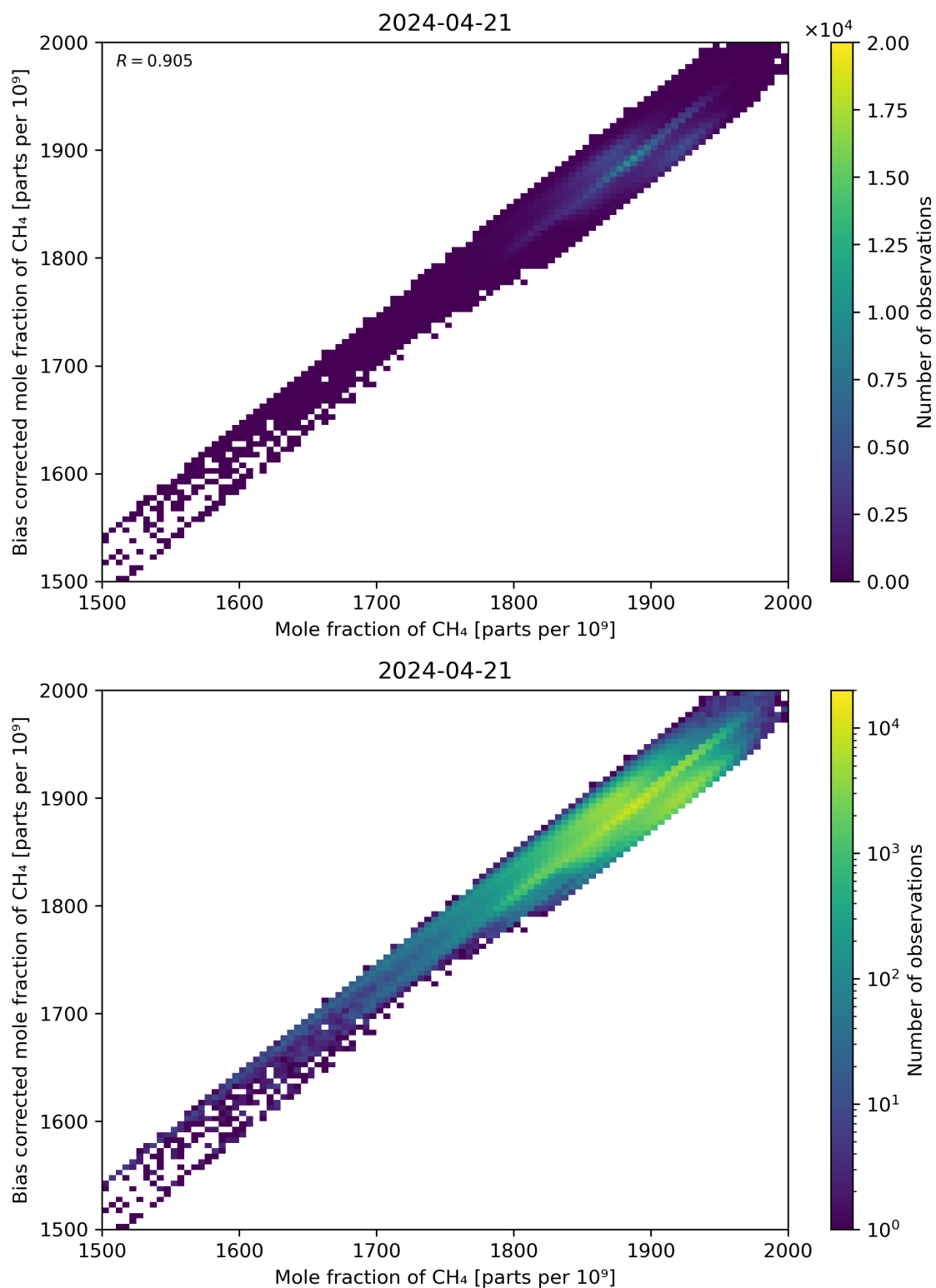
Figure 74: Scatter density plot of “Mole fraction of CH 4 ” against “Bias corrected mole fraction of CH 4 ” for 2024-04-21 to 2024-04-22.
