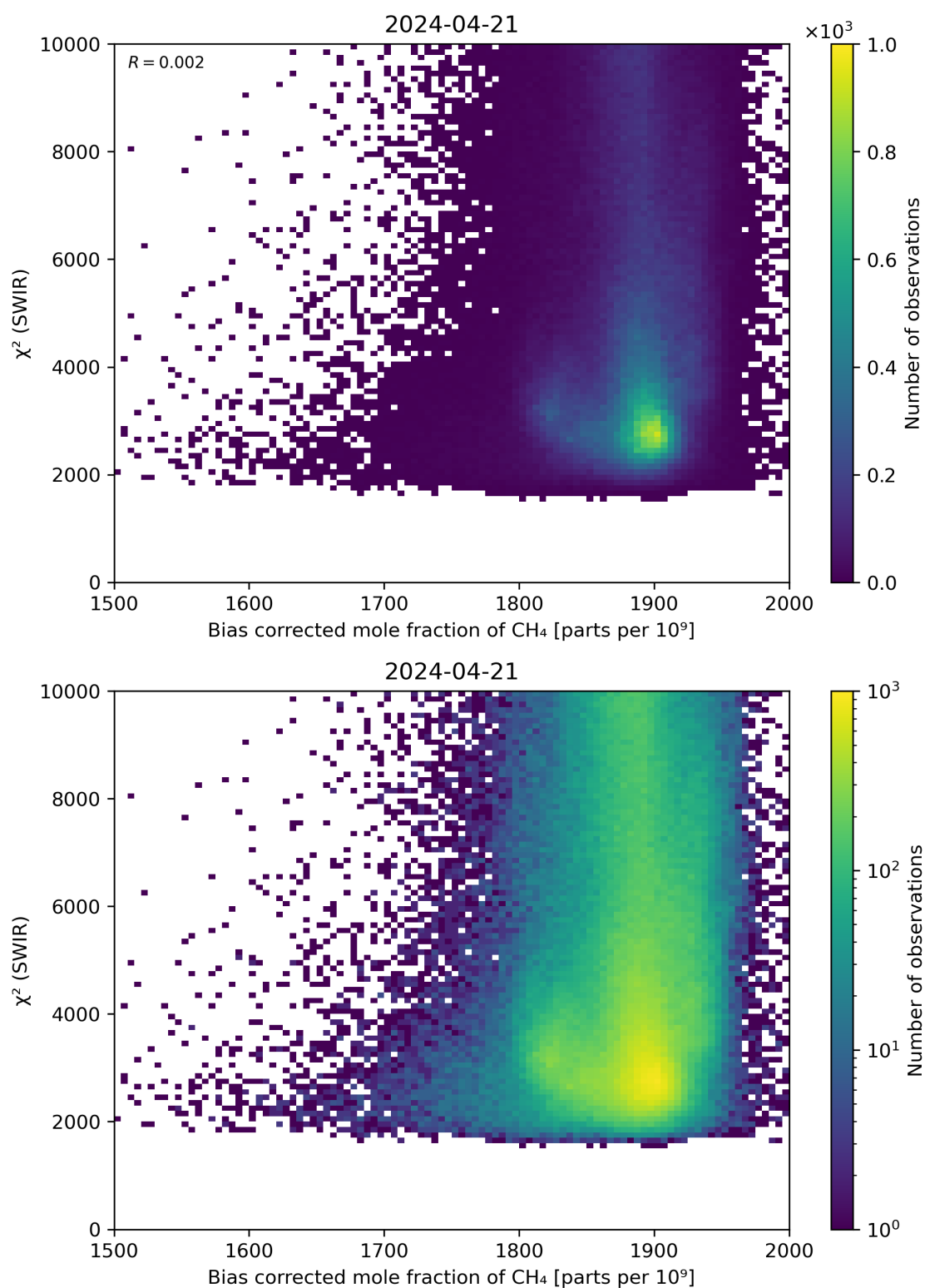
Figure 64: Scatter density plot of “Bias corrected mole fraction of CH 4 ” against “ \chi^2 (SWIR)” for 2024-04-21 to 2024-04-22.
