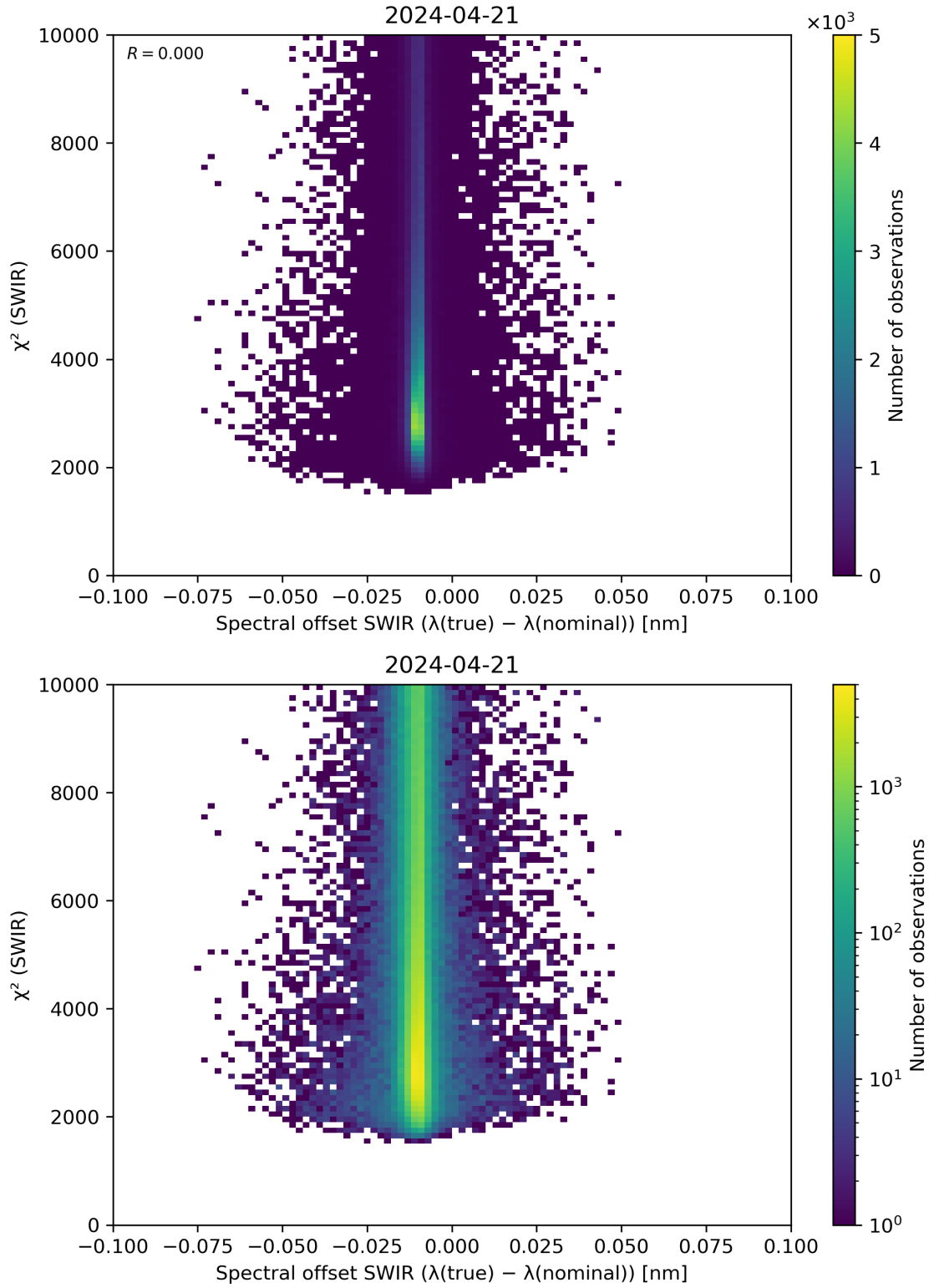
Figure 118: Scatter density plot of “Spectral offset SWIR ( \lambda(\text{true}) - \lambda(\text{nominal}) )” against “ \chi^2 (SWIR)” for 2024-04-21 to 2024-04-22.
