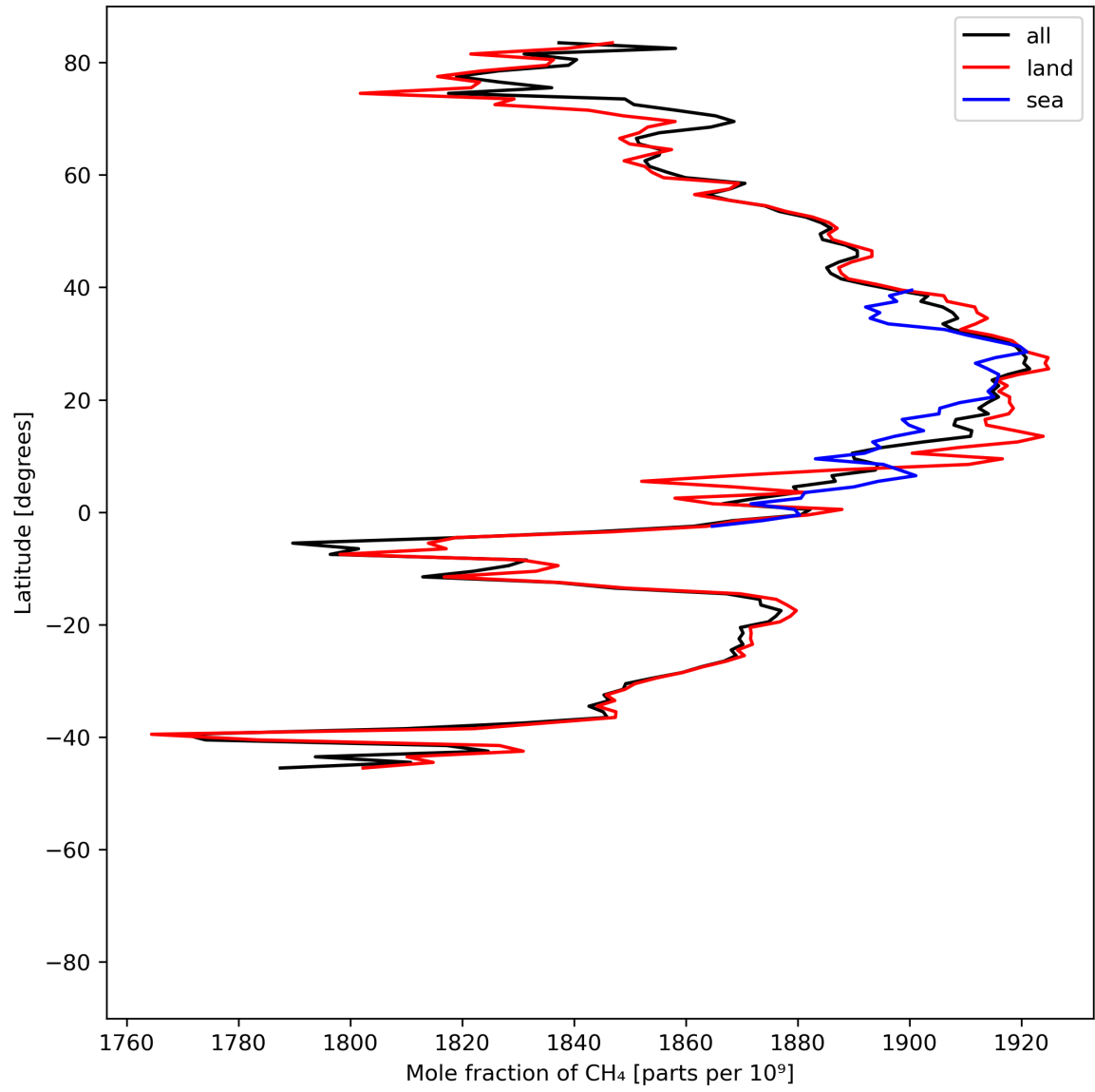
Figure 12: Zonal average of “Mole fraction of \text{CH}_4 ” for 2024-04-21 to 2024-04-22.
