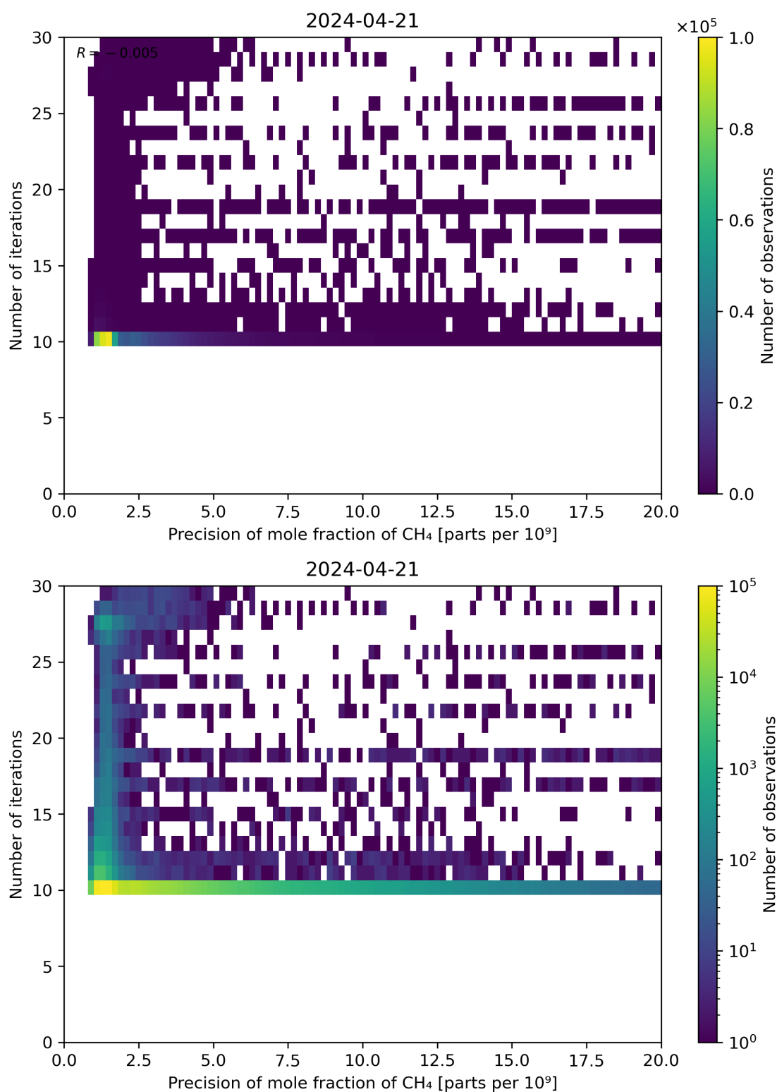
Figure 83: Scatter density plot of “Precision of mole fraction of CH 4 ” against “Number of iterations” for 2024-04-21 to 2024-04-22.
