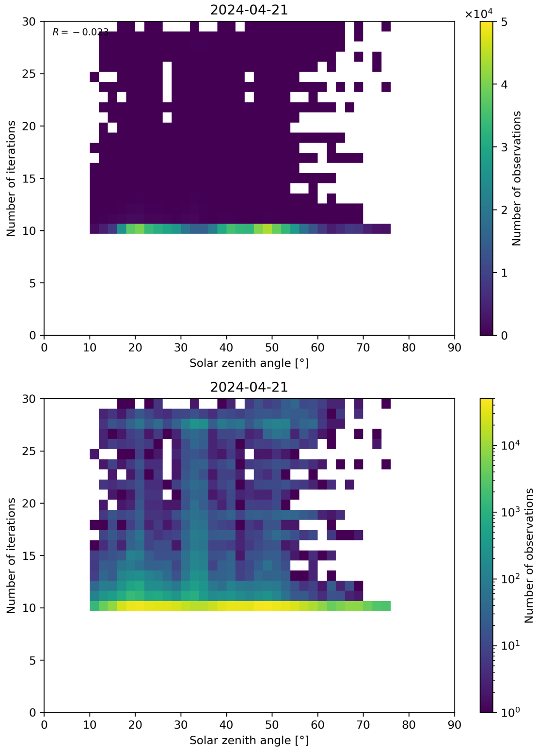
Figure 102: Scatter density plot of “Solar zenith angle” against “Number of iterations” for 2024-04-21 to 2024-04-22.
