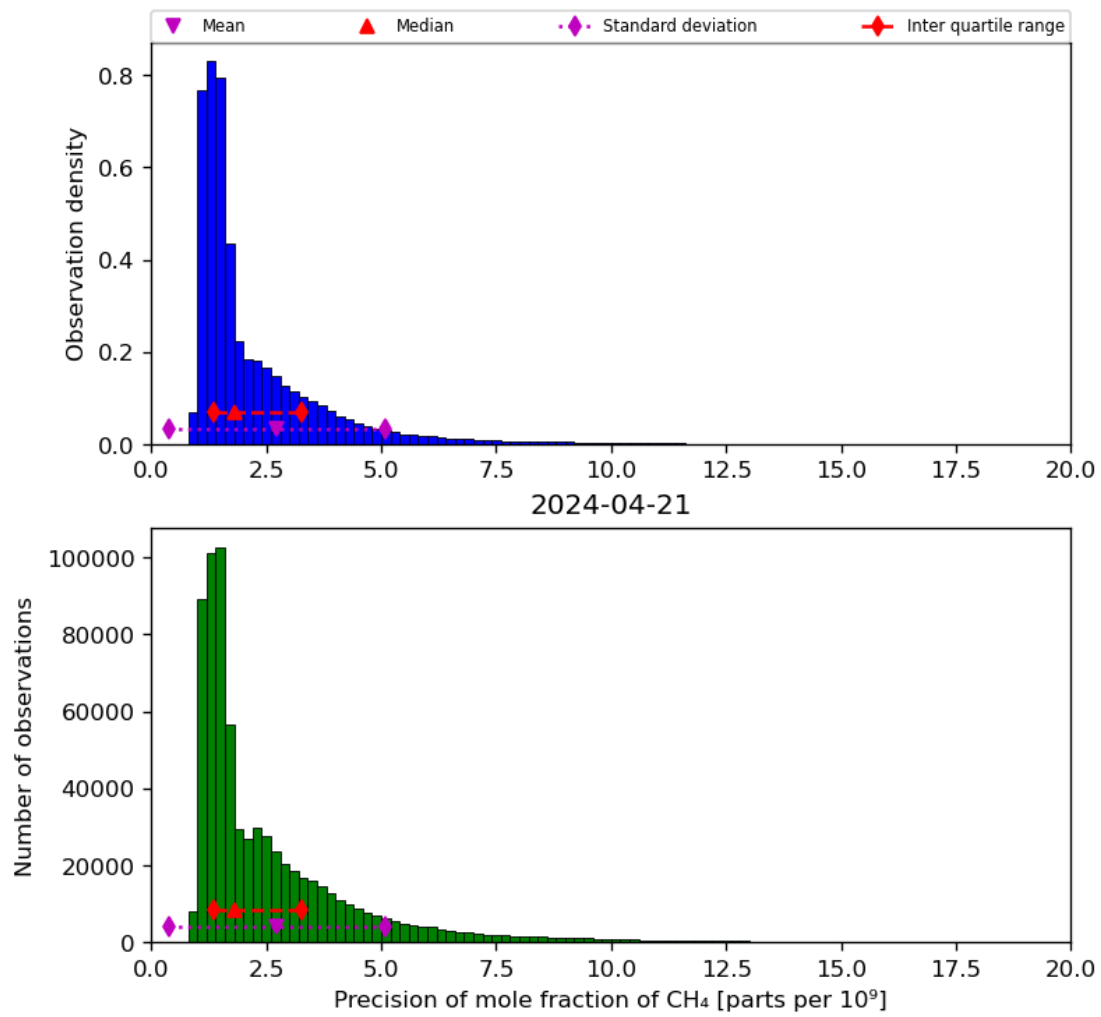
Figure 24: Histogram of “Precision of mole fraction of CH 4 ” for 2024-04-21 to 2024-04-22
