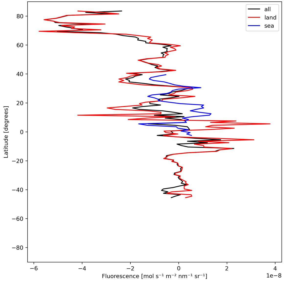
Figure 21: Zonal average of “Fluorescence” for 2024-04-21 to 2024-04-22.
