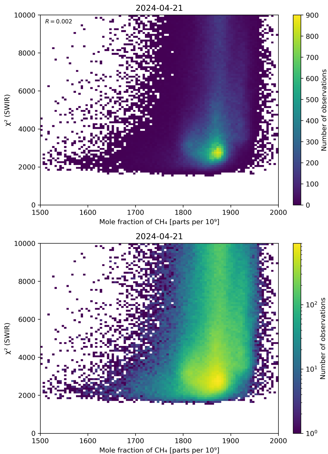
Figure 71: Scatter density plot of “Mole fraction of \text{CH}_4 ” against “ \chi^2 (SWIR)” for 2024-04-21 to 2024-04-22.
