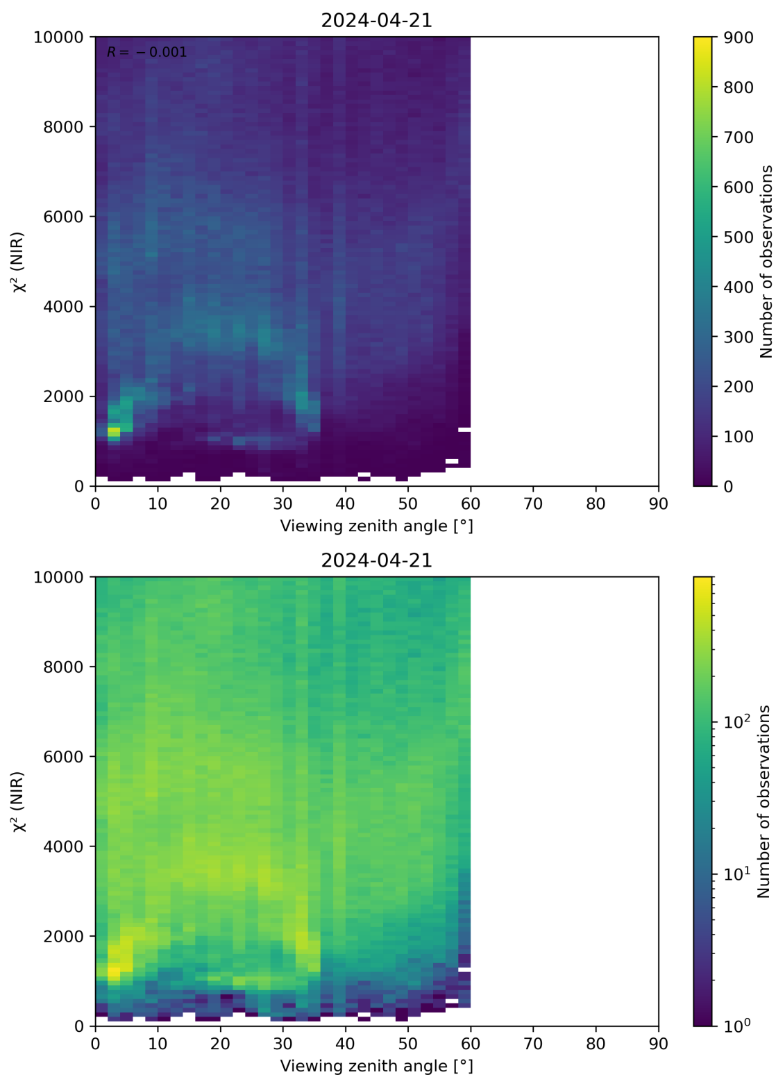
Figure 105: Scatter density plot of “Viewing zenith angle” against “ \chi^2 (NIR)” for 2024-04-21 to 2024-04-22.
