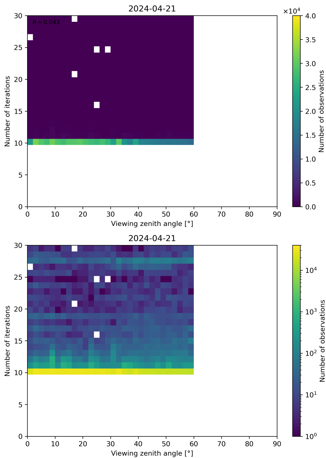
Figure 113: Scatter density plot of “Viewing zenith angle” against “Number of iterations” for 2024-04-21 to 2024-04-22.
