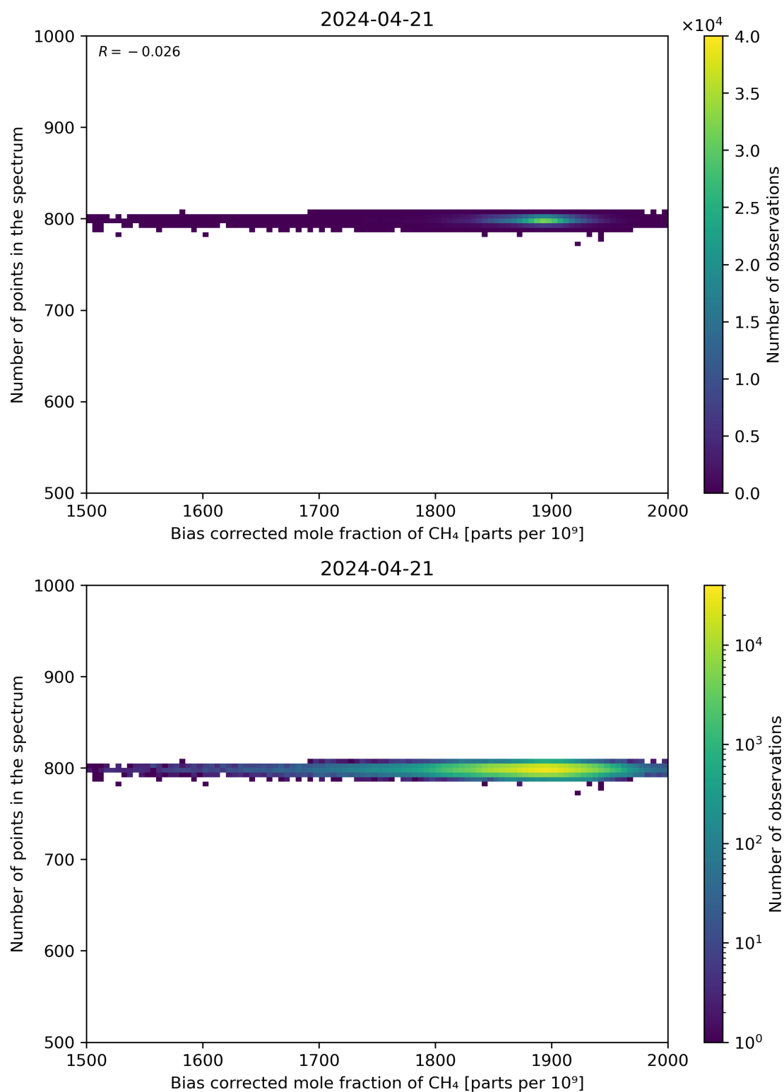
Figure 68: Scatter density plot of “Bias corrected mole fraction of CH 4 ” against “Number of points in the spectrum” for 2024-04-21 to 2024-04-22.
