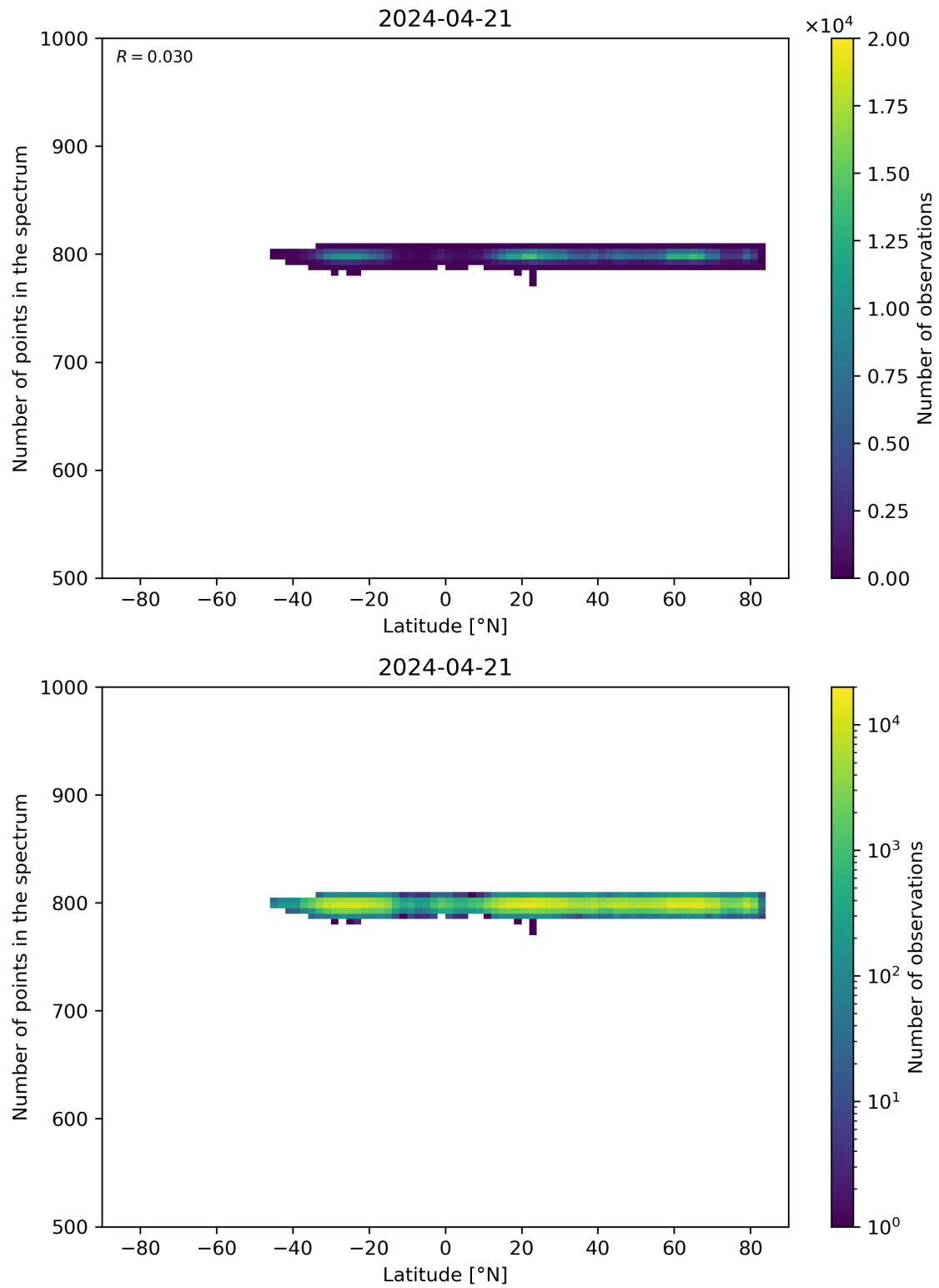
Figure 61: Scatter density plot of “Latitude” against “Number of points in the spectrum” for 2024-04-21 to 2024-04-22.
