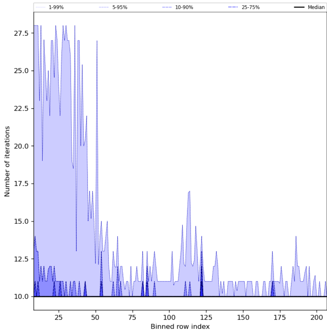
Figure 42: Along track statistics of “Number of iterations” for 2024-04-21 to 2024-04-22
