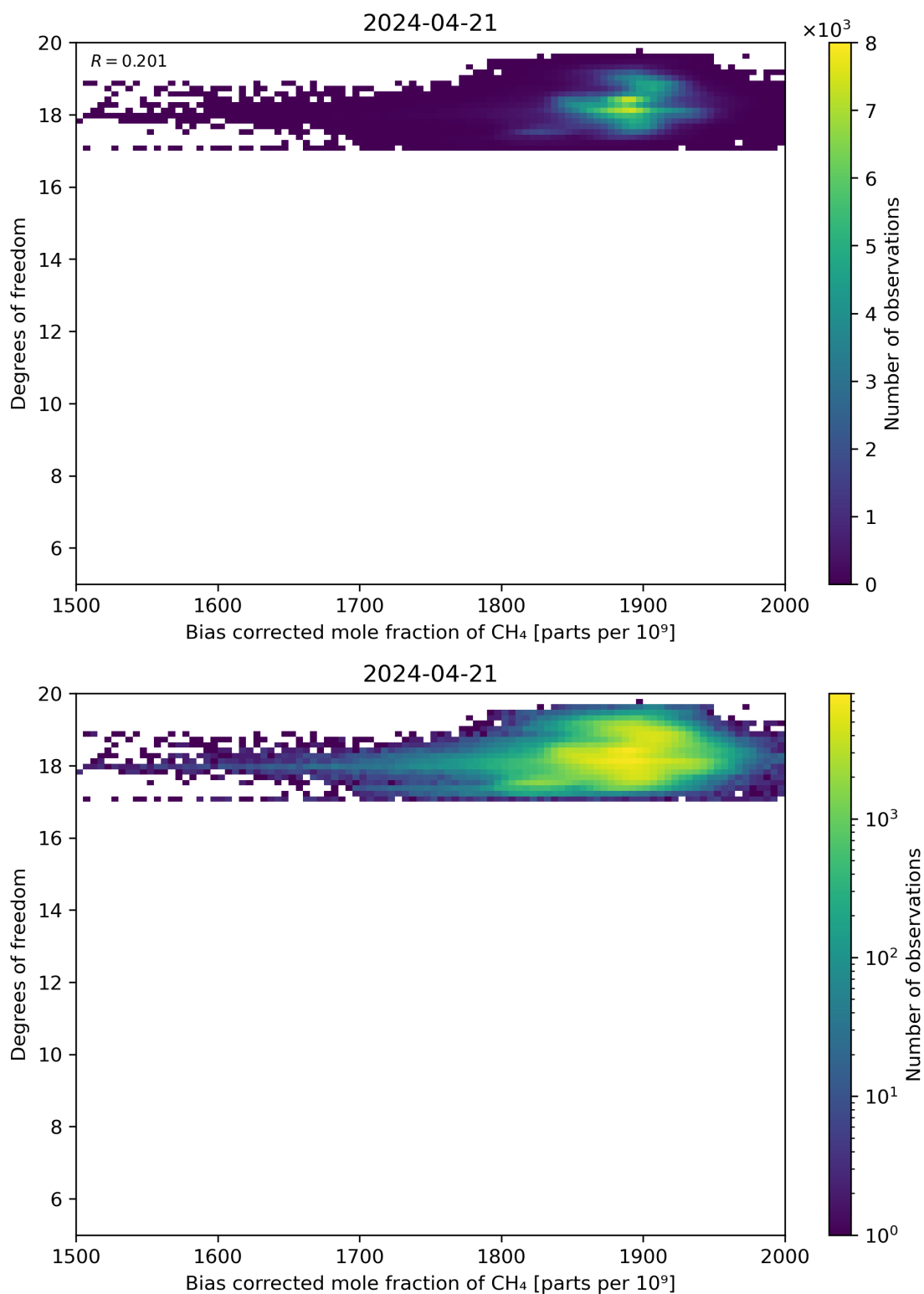
Figure 65: Scatter density plot of “Bias corrected mole fraction of CH 4 ” against “Degrees of freedom” for 2024-04-21 to 2024-04-22.
