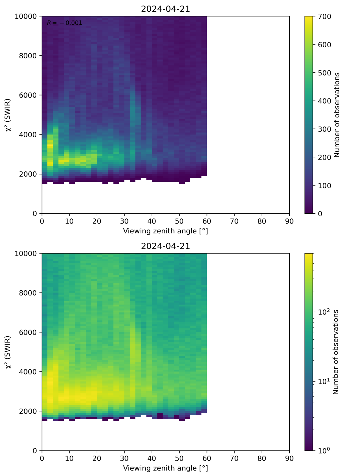
Figure 106: Scatter density plot of “Viewing zenith angle” against “ \chi^2 (SWIR)” for 2024-04-21 to 2024-04-22.
