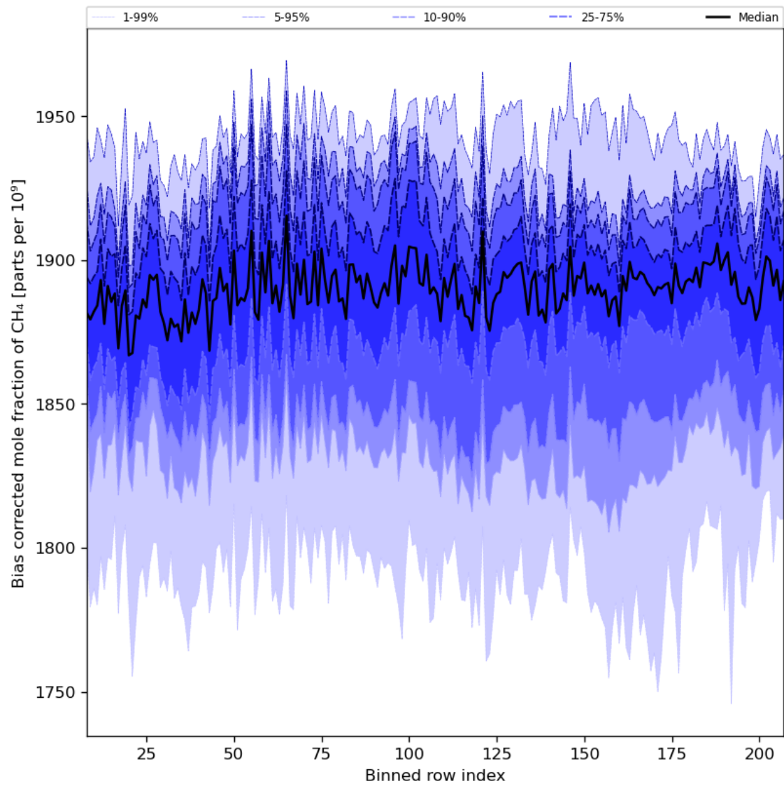
Figure 36: Along track statistics of “Bias corrected mole fraction of CH 4 ” for 2024-04-21 to 2024-04-22
