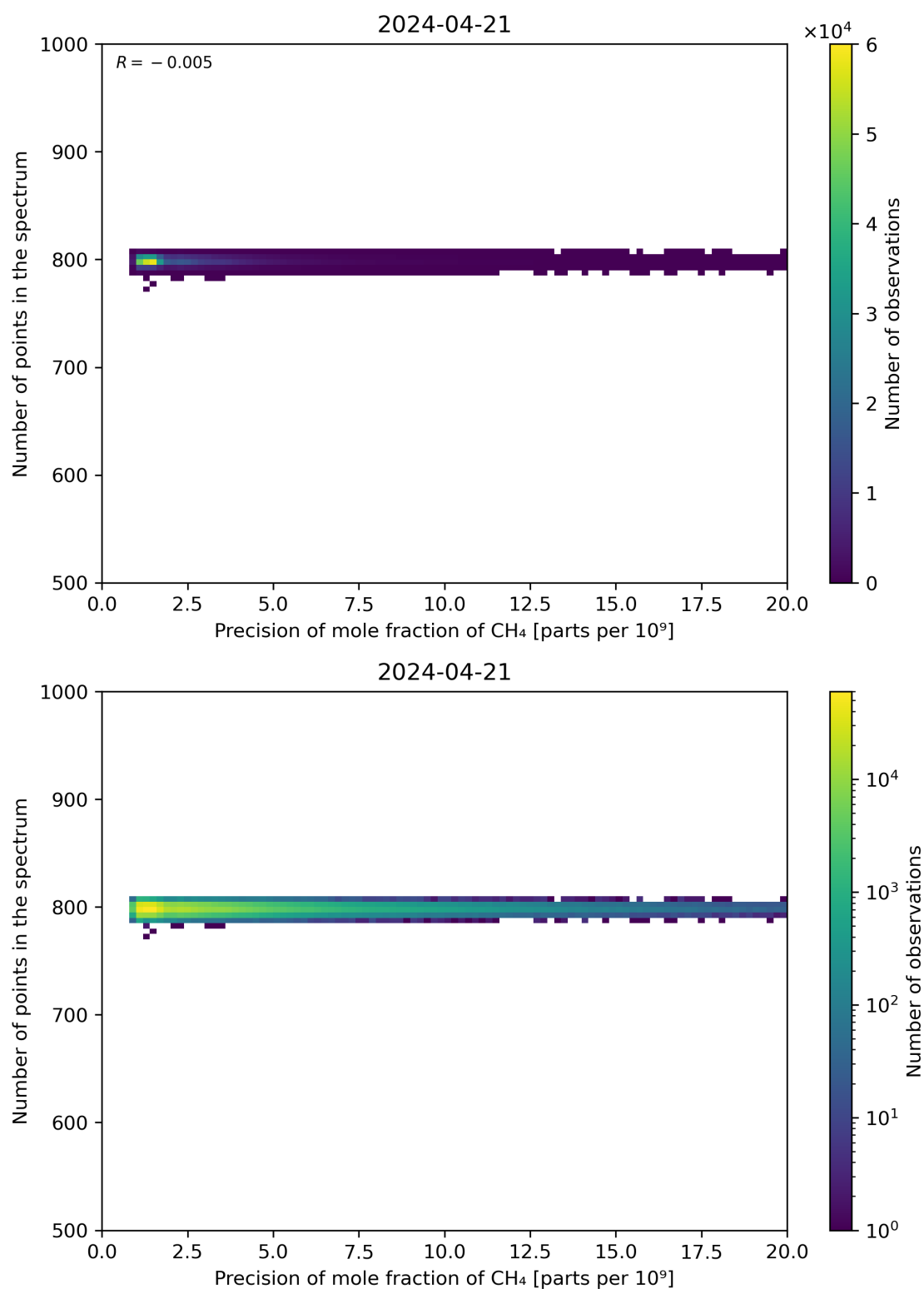
Figure 84: Scatter density plot of “Precision of mole fraction of CH 4 ” against “Number of points in the spectrum” for 2024-04-21 to 2024-04-22.
