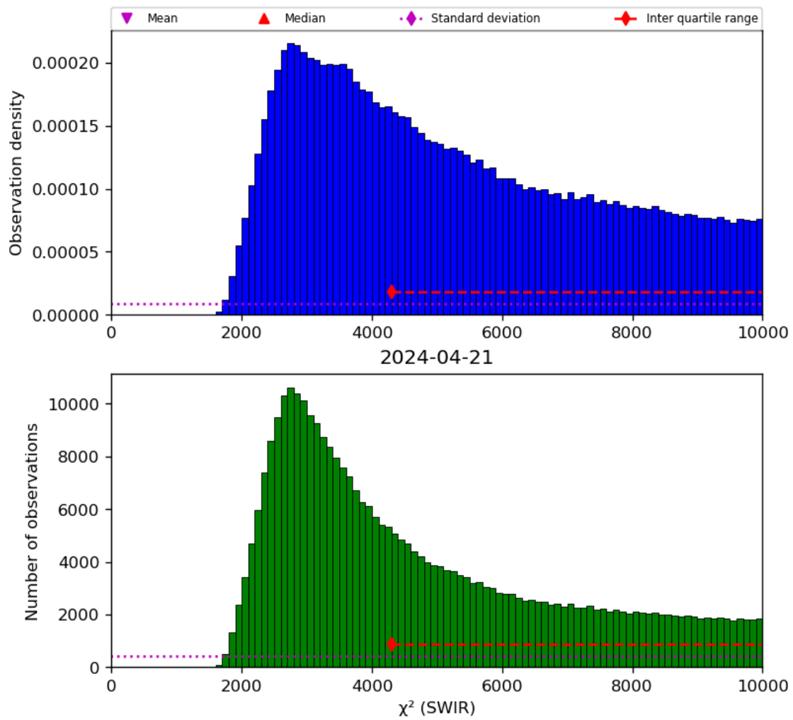
Figure 28: Histogram of “ \chi^2 (SWIR)” for 2024-04-21 to 2024-04-22
