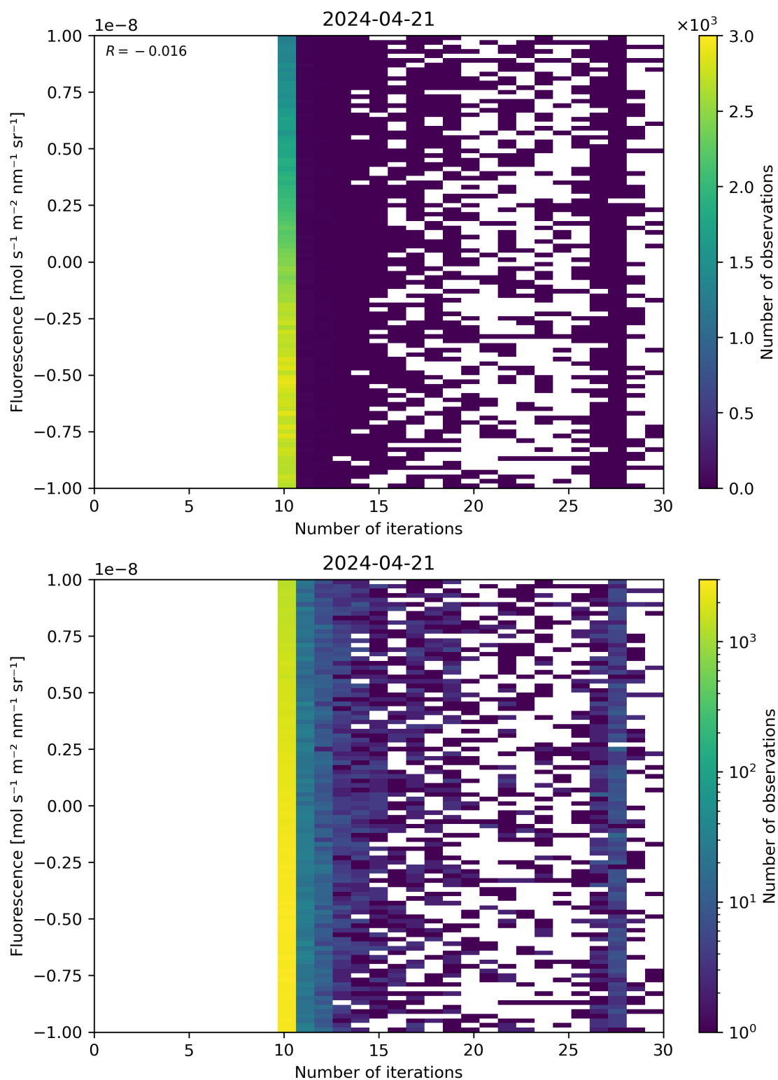
Figure 87: Scatter density plot of “Number of iterations” against “Fluorescence” for 2024-04-21 to 2024-04-22.
