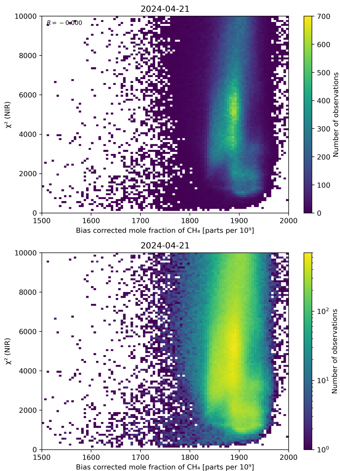
Figure 63: Scatter density plot of “Bias corrected mole fraction of CH 4 ” against “ \chi^2 (NIR)” for 2024-04-21 to 2024-04-22.
