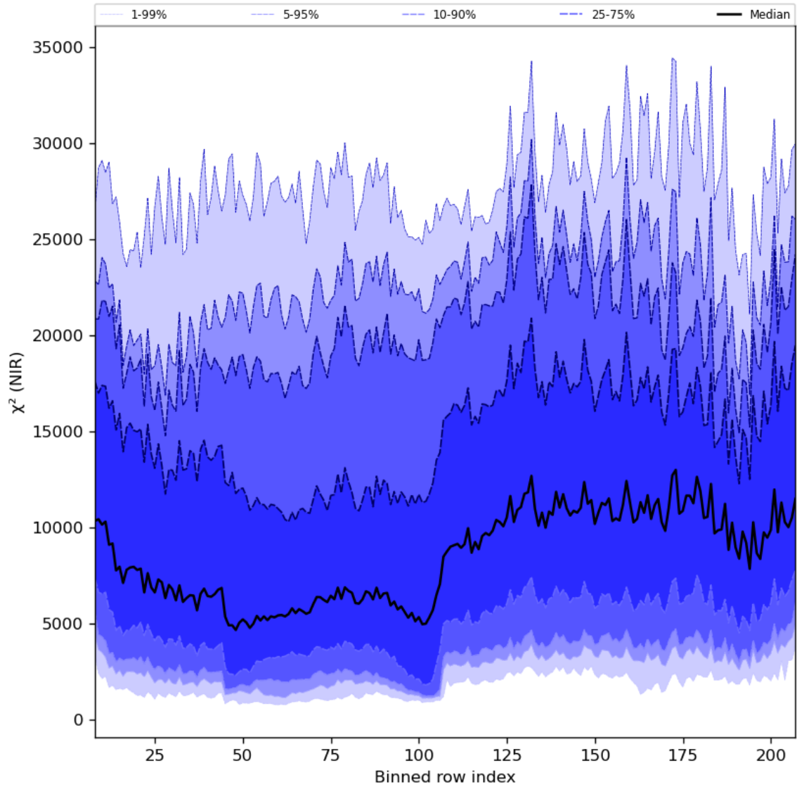
Figure 40: Along track statistics of “ \chi^2 (NIR)” for 2024-04-21 to 2024-04-22
