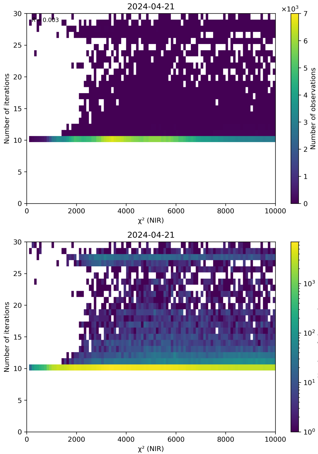
Figure 46: Scatter density plot of “ \chi^2 (NIR)” against “Number of iterations” for 2024-04-21 to 2024-04-22.
