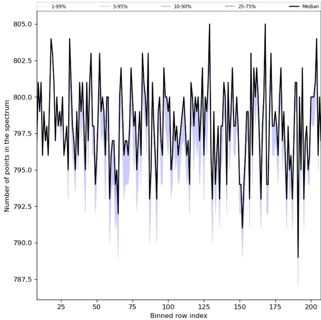
Figure 37: Along track statistics of “Number of points in the spectrum” for 2024-04-21 to 2024-04-22
