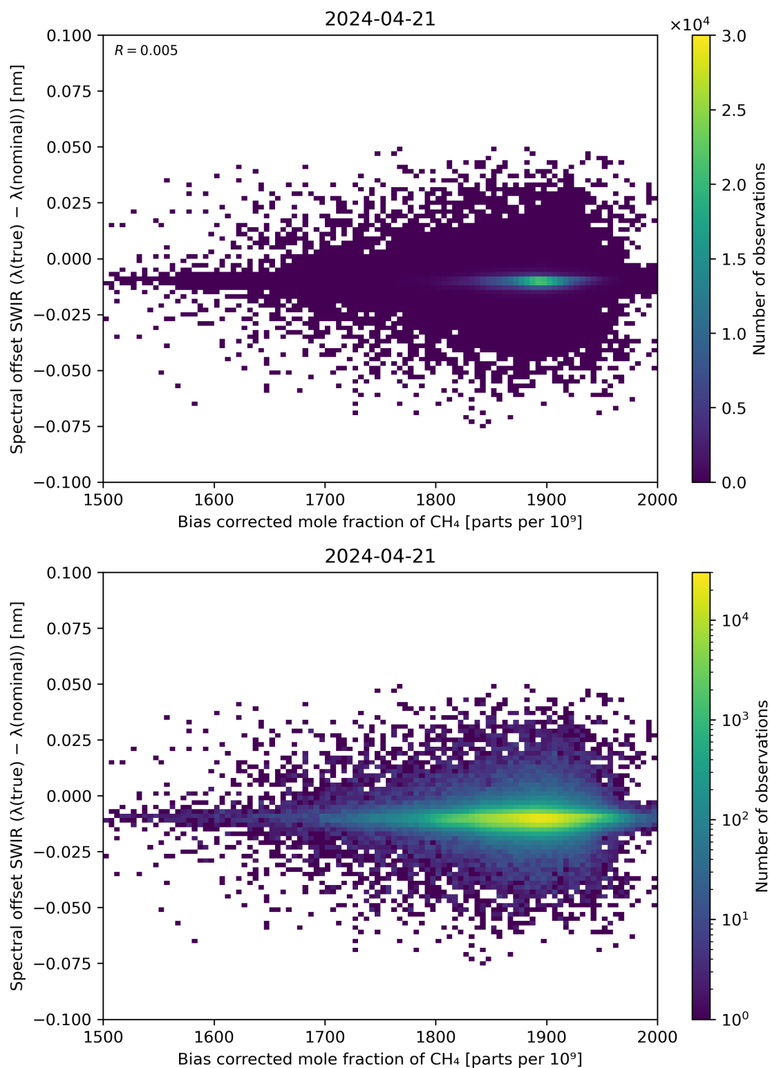
Figure 69: Scatter density plot of “Bias corrected mole fraction of \text{CH}_4 ” against “Spectral offset SWIR ( \lambda(\text{true}) - \lambda(\text{nominal}) )” for 2024-04-21 to 2024-04-22.
