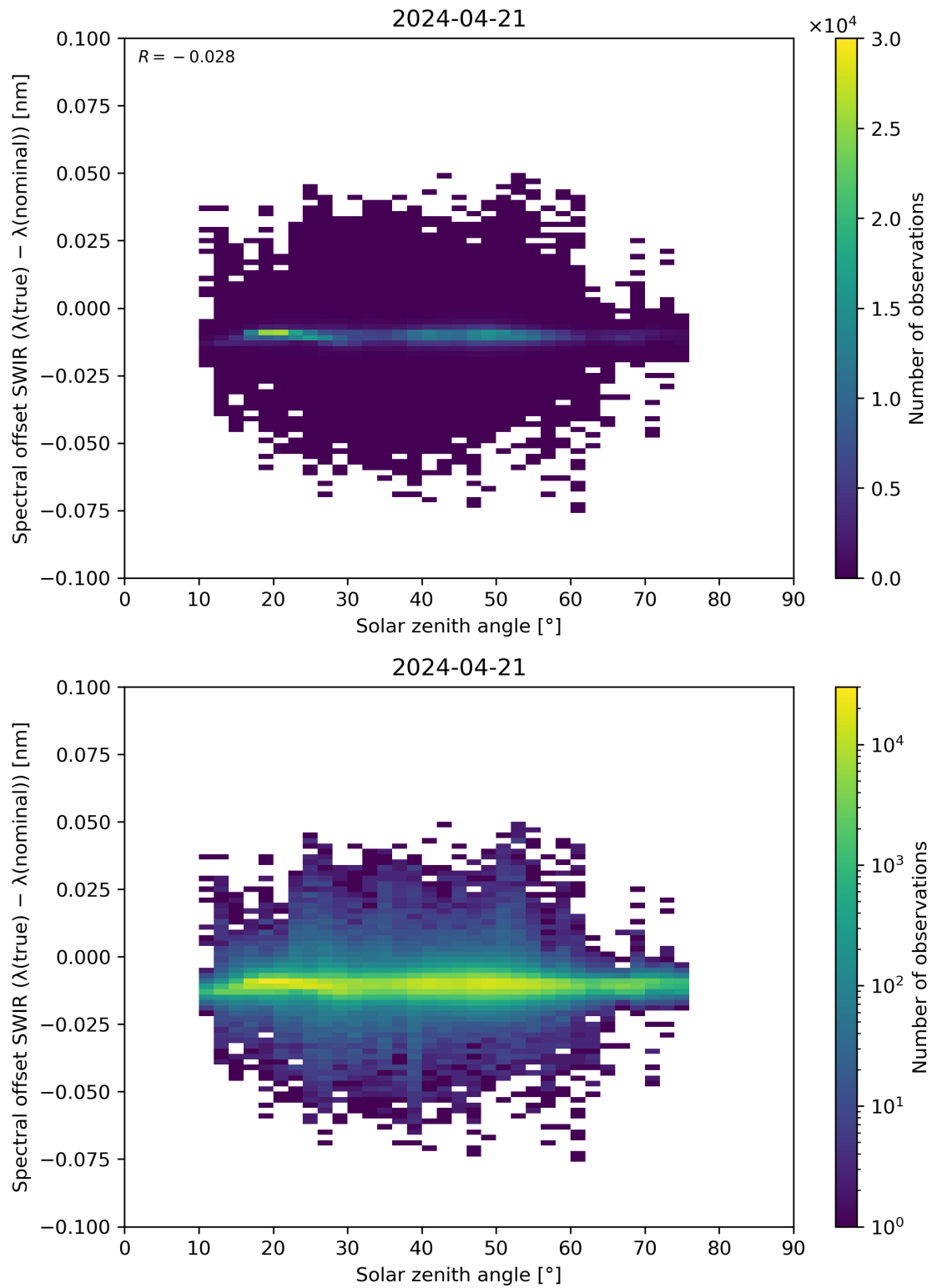
Figure 104: Scatter density plot of “Solar zenith angle” against “Spectral offset SWIR ( \lambda(\text{true}) - \lambda(\text{nominal}) )” for 2024-04-21 to 2024-04-22.
