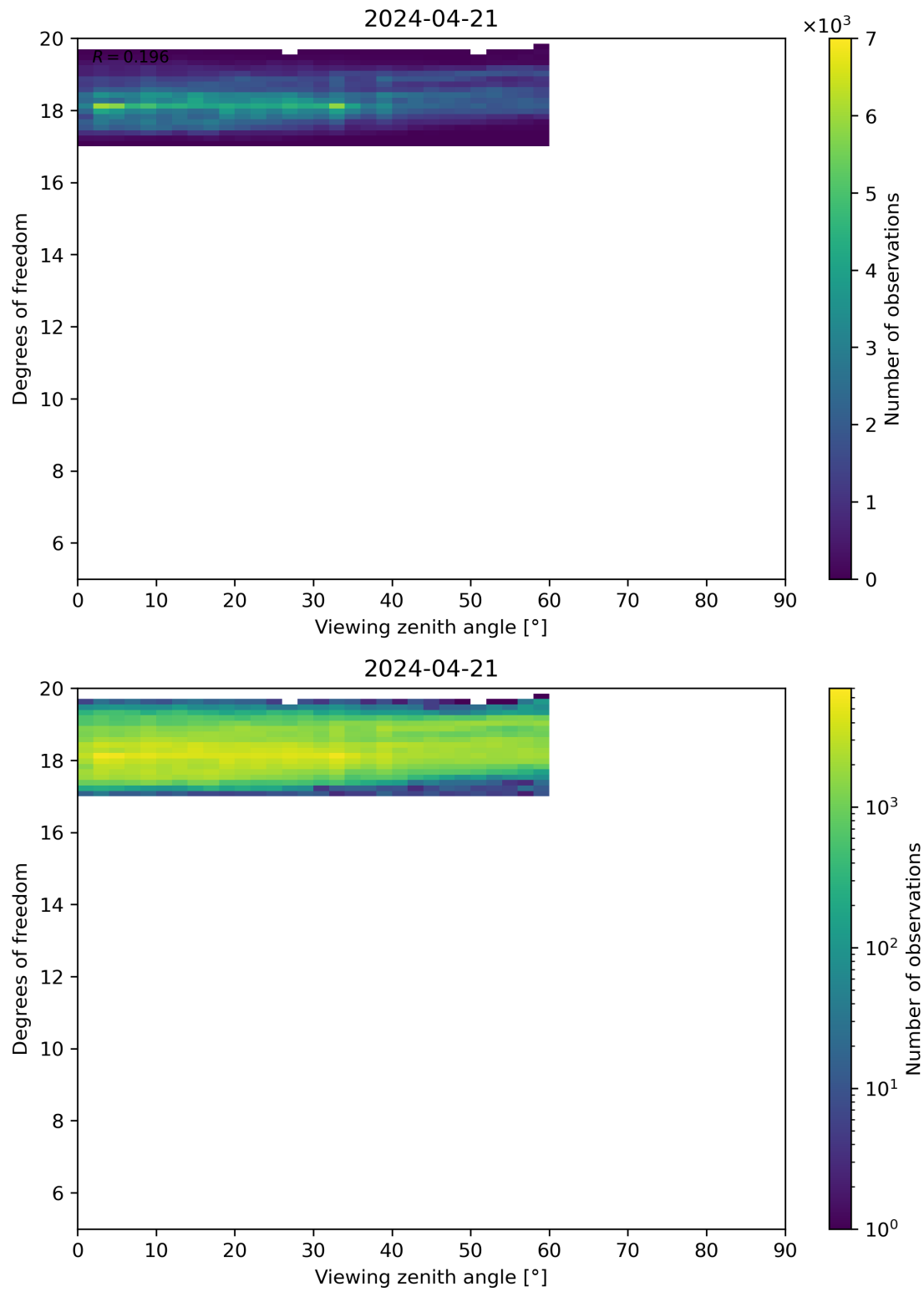
Figure 107: Scatter density plot of “Viewing zenith angle” against “Degrees of freedom” for 2024-04-21 to 2024-04-22.
