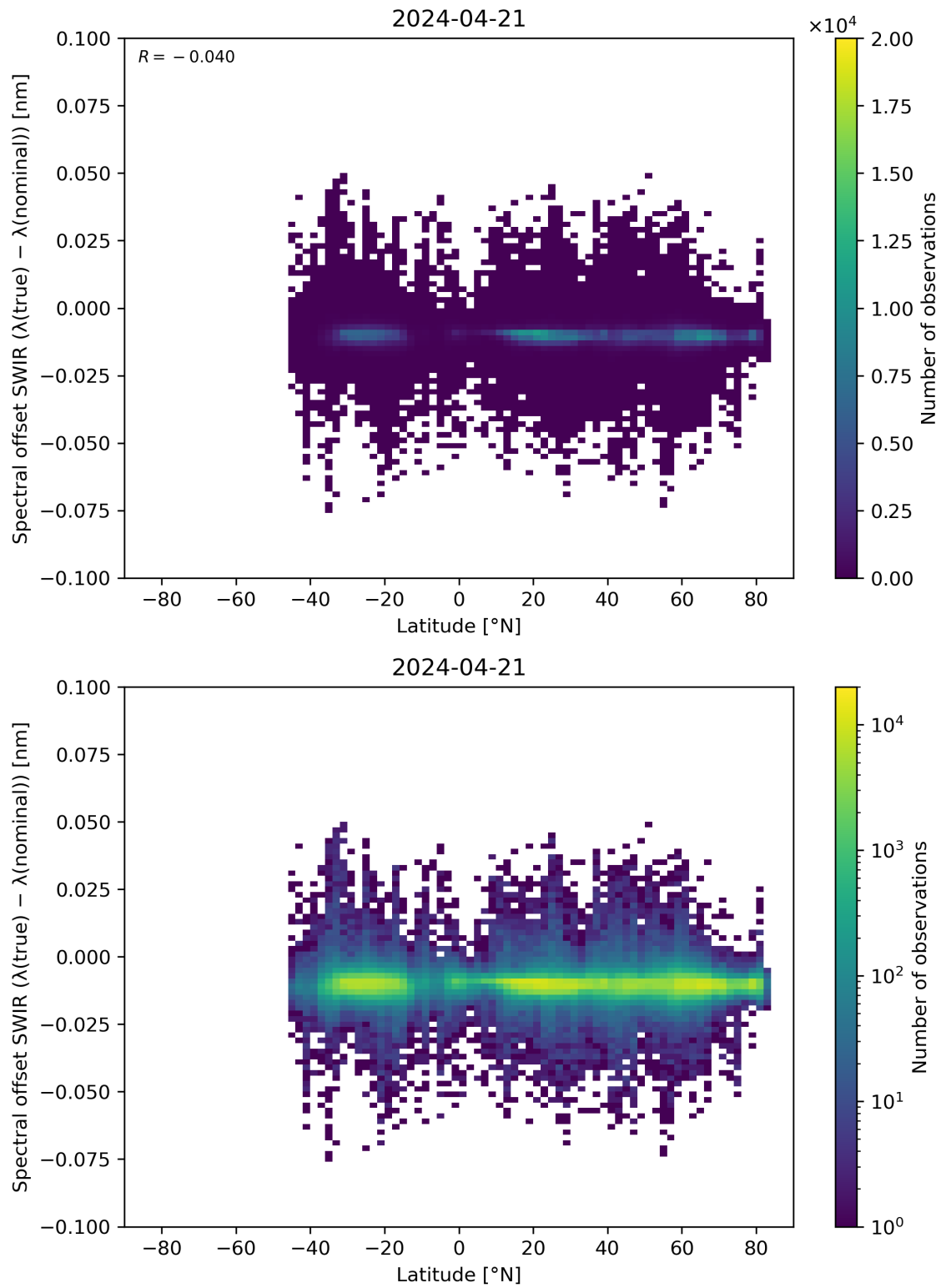
Figure 62: Scatter density plot of “Latitude” against “Spectral offset SWIR ( \lambda(\text{true}) - \lambda(\text{nominal}) )” for 2024-04-21 to 2024-04-22.
