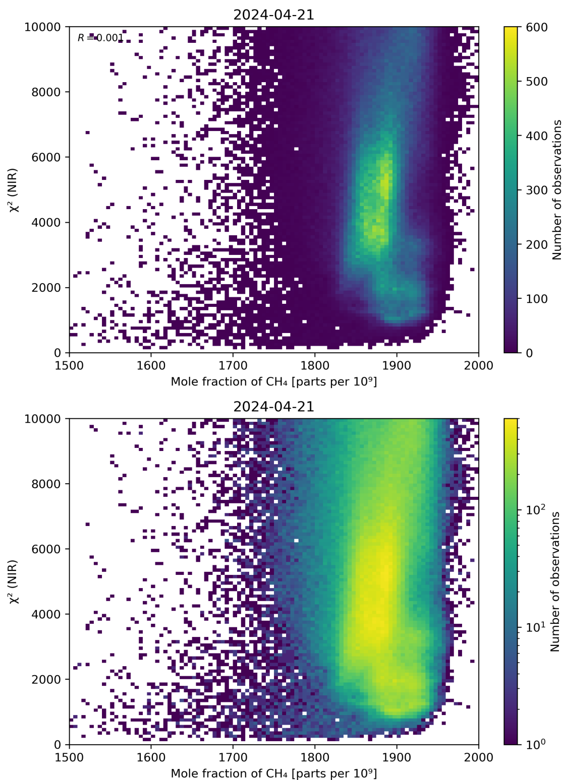
Figure 70: Scatter density plot of “Mole fraction of \text{CH}_4 ” against “ \chi^2 (NIR)” for 2024-04-21 to 2024-04-22.
