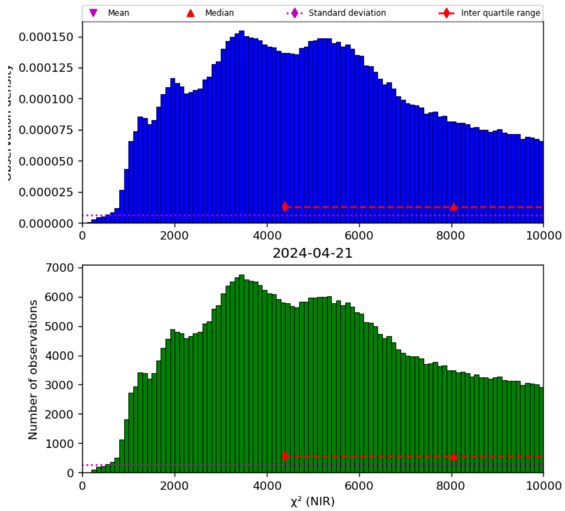
Figure 29: Histogram of “ \chi^2 (NIR)” for 2024-04-21 to 2024-04-22
