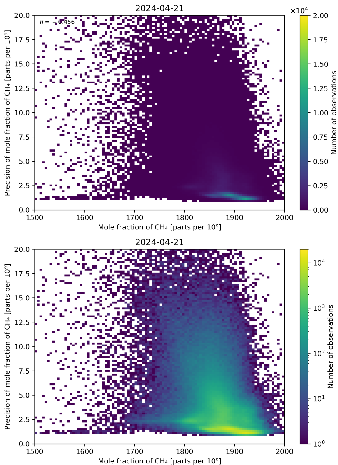
Figure 75: Scatter density plot of “Mole fraction of CH 4 ” against “Precision of mole fraction of CH 4 ” for 2024-04-21 to 2024-04-22.
