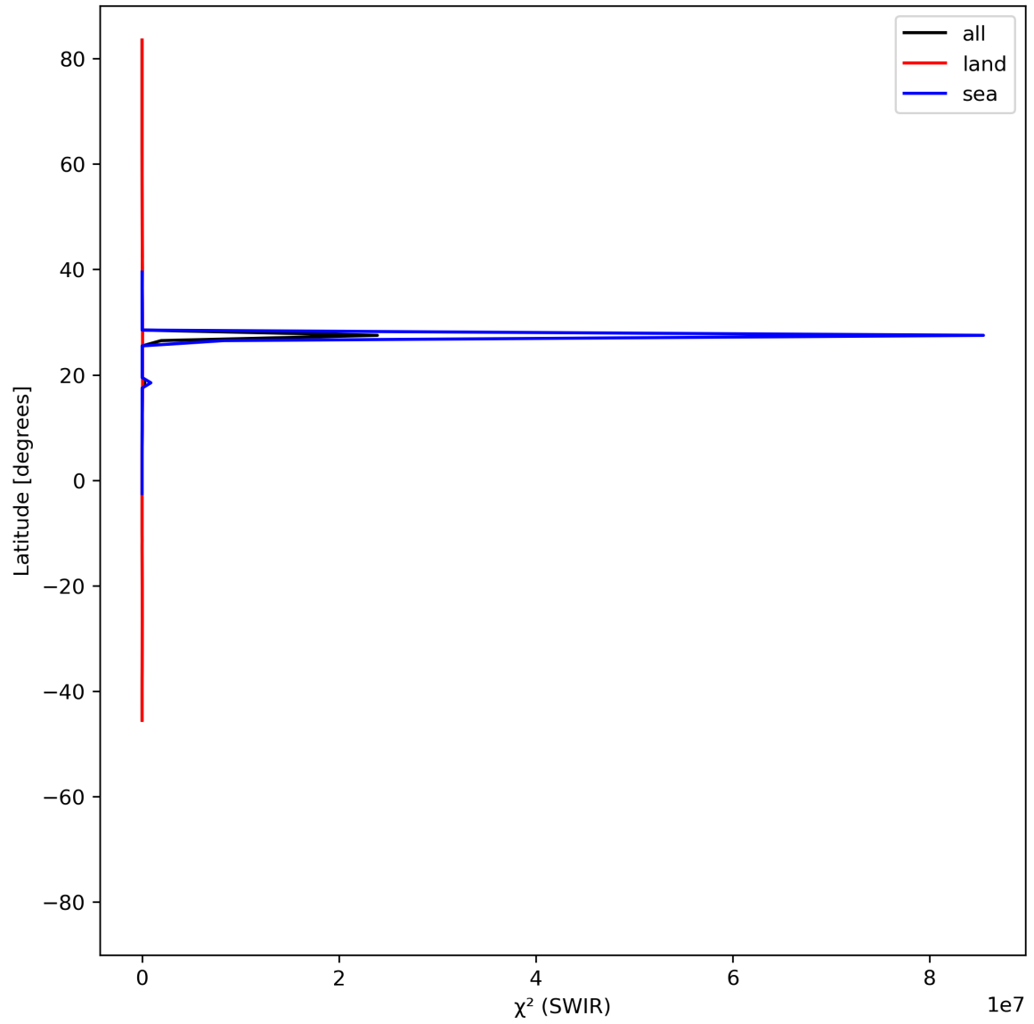
Figure 17: Zonal average of “ \chi^2 (SWIR)” for 2024-04-21 to 2024-04-22.
