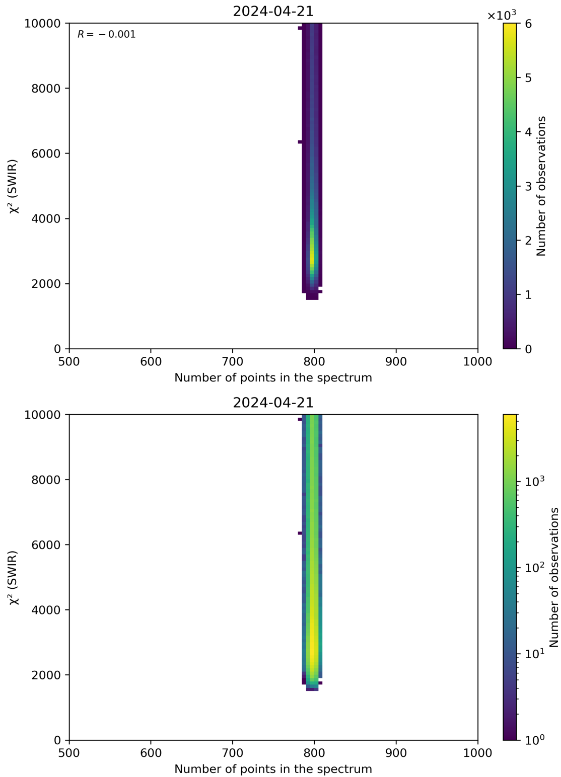
Figure 89: Scatter density plot of “Number of points in the spectrum” against “ \chi^2 (SWIR)” for 2024-04-21 to 2024-04-22.
