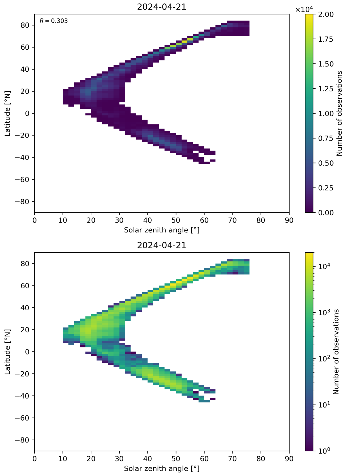
Figure 98: Scatter density plot of “Solar zenith angle” against “Latitude” for 2024-04-21 to 2024-04-22.
