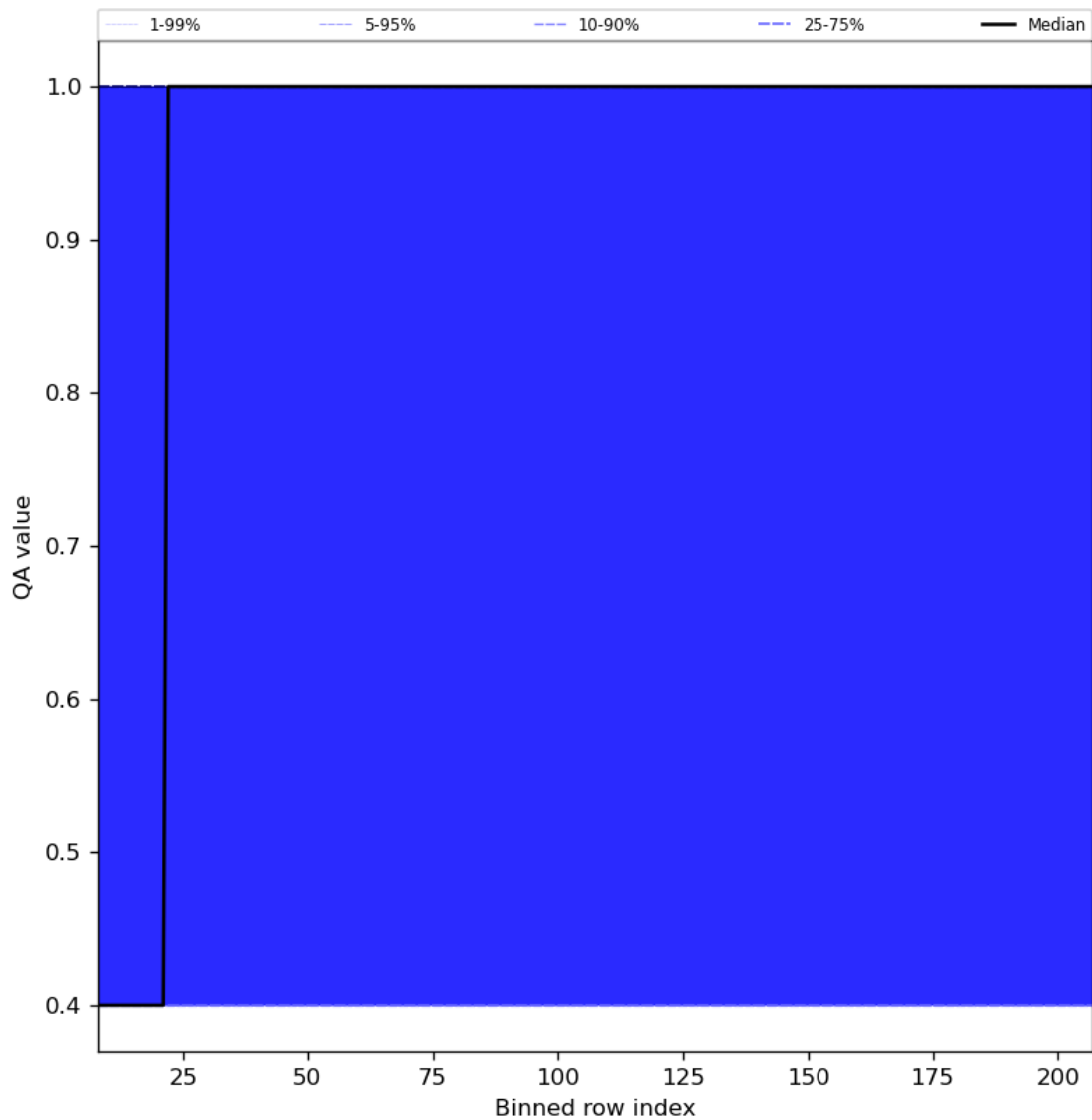
Figure 33: Along track statistics of “QA value” for 2024-04-21 to 2024-04-22
