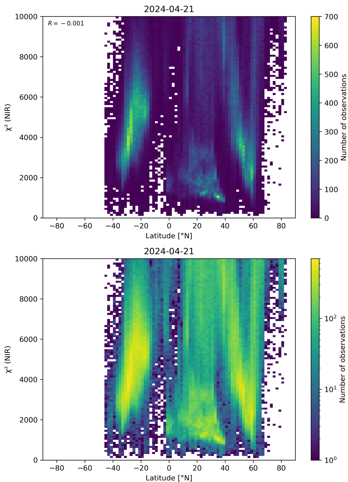
Figure 53: Scatter density plot of “Latitude” against “ \chi^2 (NIR)” for 2024-04-21 to 2024-04-22.
