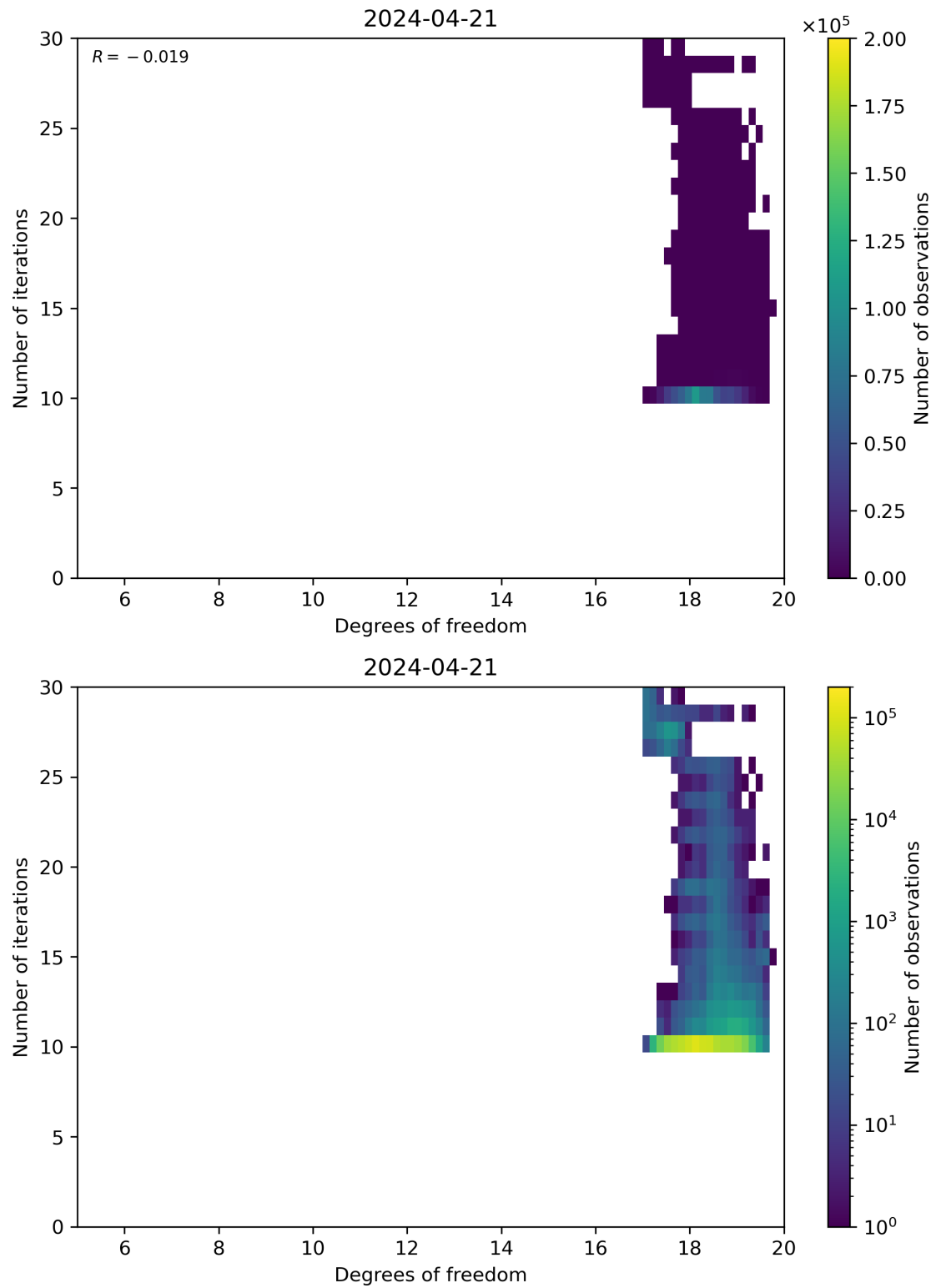
Figure 52: Scatter density plot of “Degrees of freedom” against “Number of iterations” for 2024-04-21 to 2024-04-22.
