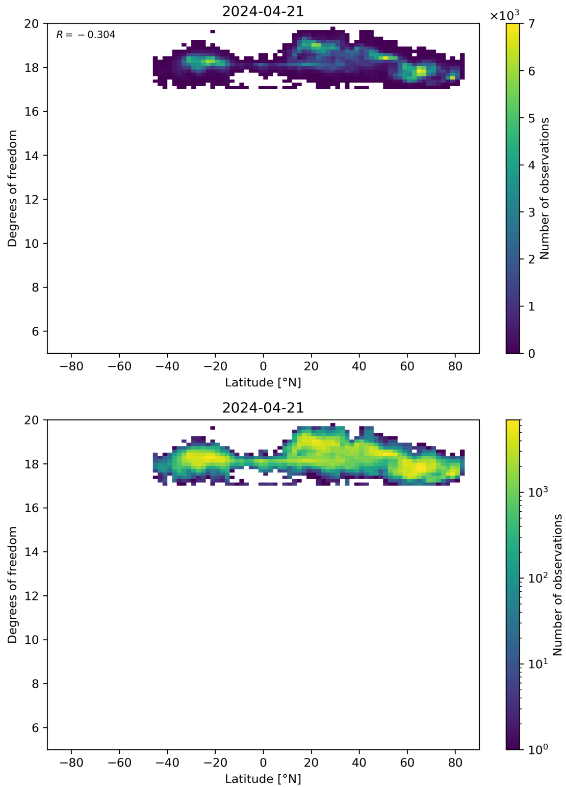
Figure 55: Scatter density plot of “Latitude” against “Degrees of freedom” for 2024-04-21 to 2024-04-22.
