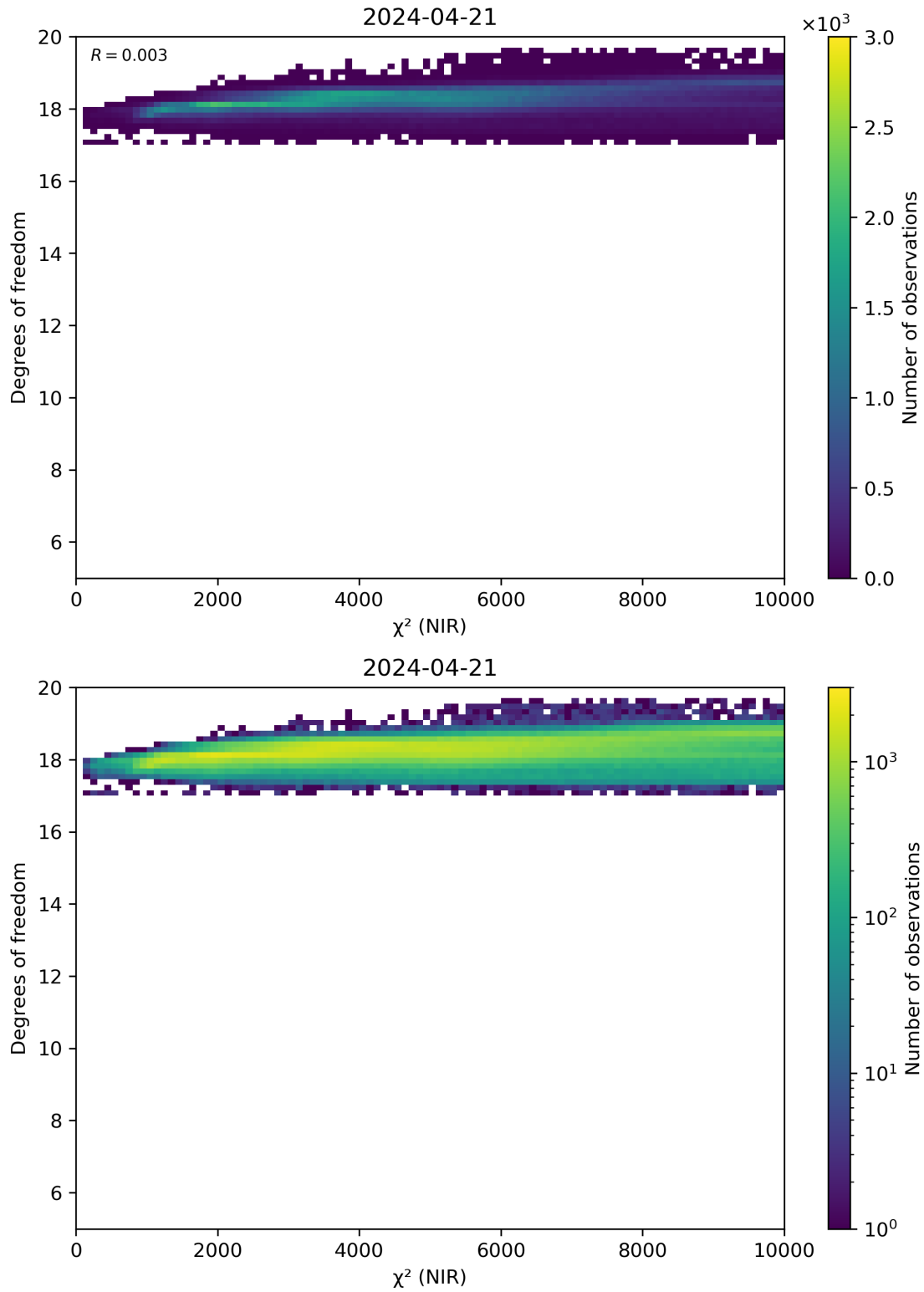
Figure 44: Scatter density plot of “ \chi^2 (NIR)” against “Degrees of freedom” for 2024-04-21 to 2024-04-22.
