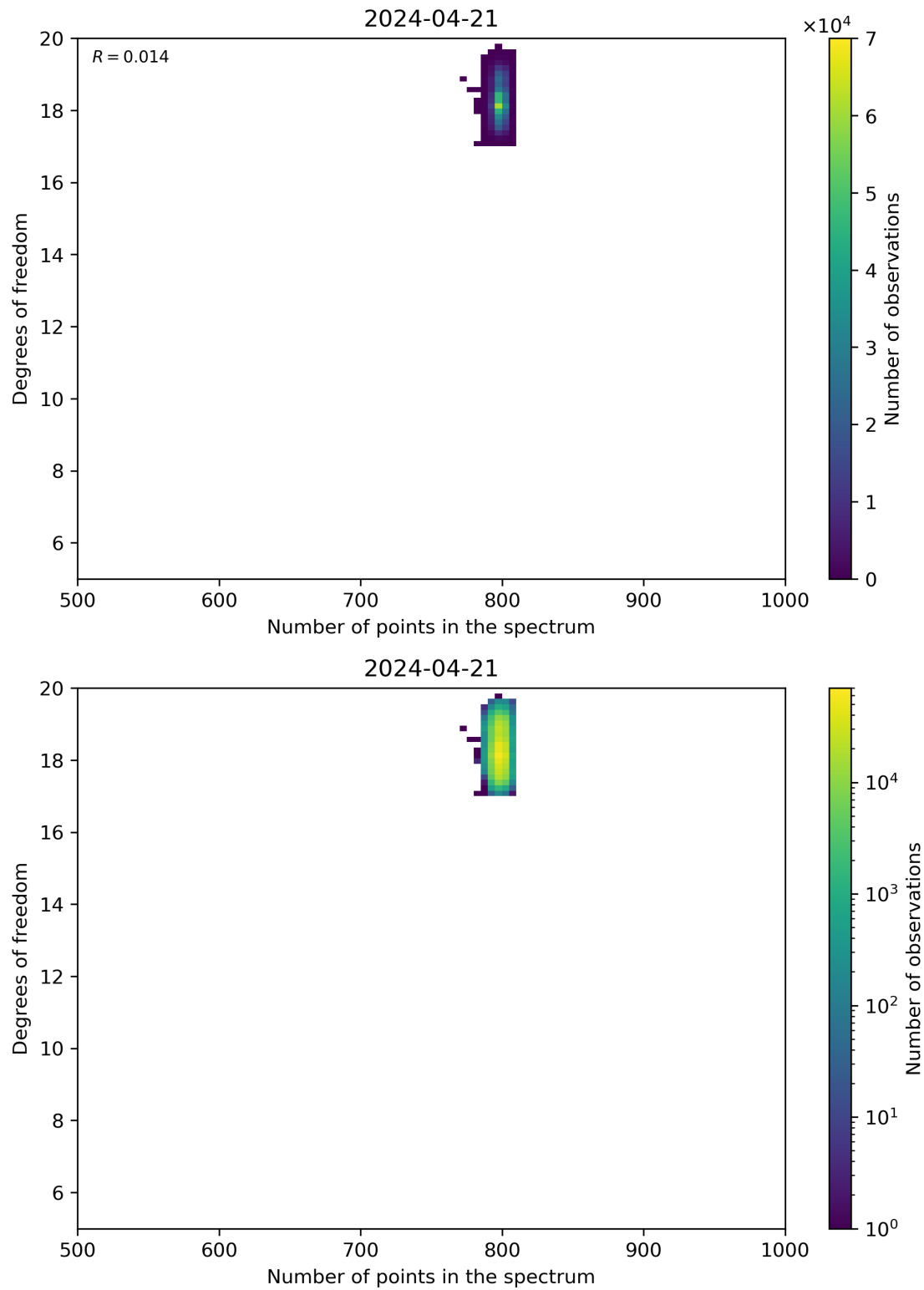
Figure 90: Scatter density plot of “Number of points in the spectrum” against “Degrees of freedom” for 2024-04-21 to 2024-04-22.
