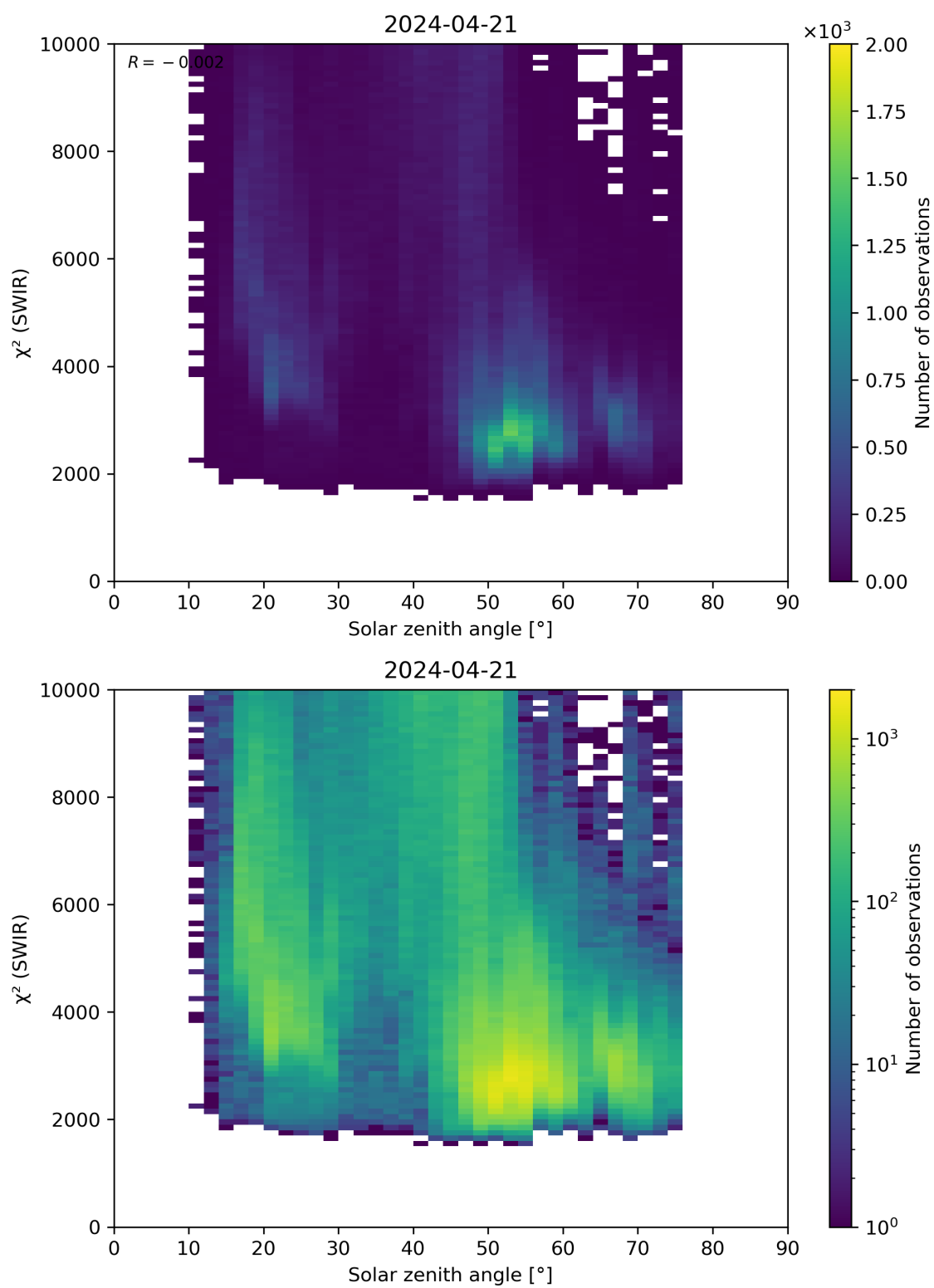
Figure 95: Scatter density plot of “Solar zenith angle” against “ \chi^2 (SWIR)” for 2024-04-21 to 2024-04-22.
