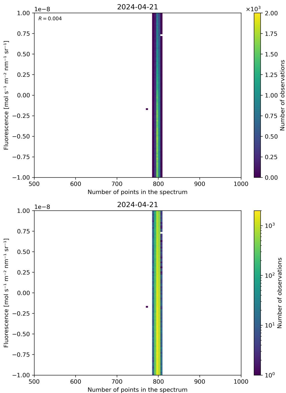
Figure 91: Scatter density plot of “Number of points in the spectrum” against “Fluorescence” for 2024-04-21 to 2024-04-22.
