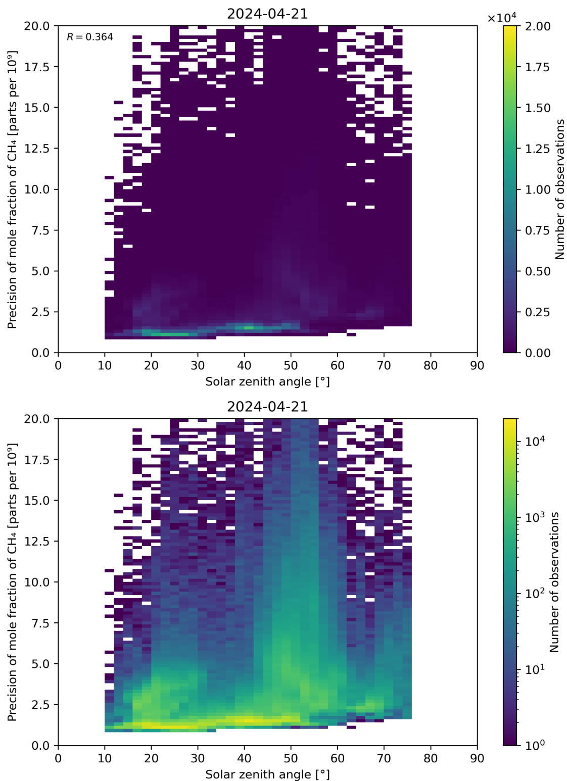
Figure 101: Scatter density plot of “Solar zenith angle” against “Precision of mole fraction of \text{CH}_4 ” for 2024-04-21 to 2024-04-22.
