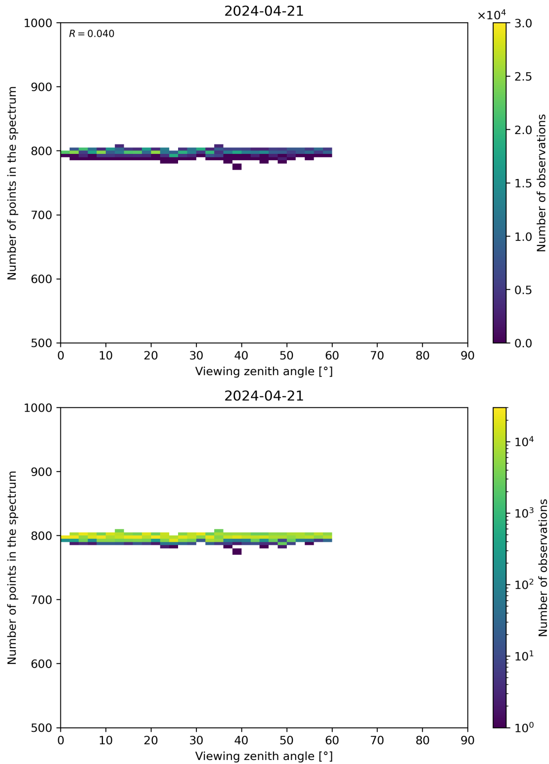
Figure 114: Scatter density plot of “Viewing zenith angle” against “Number of points in the spectrum” for 2024-04-21 to 2024-04-22.
