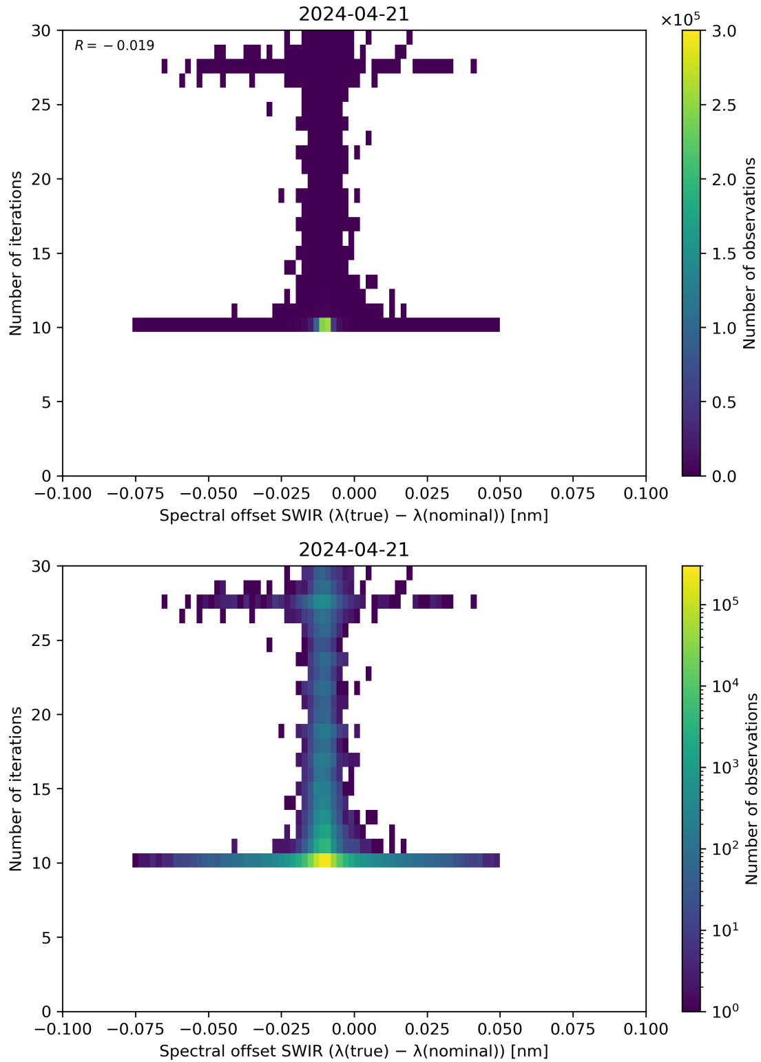
Figure 121: Scatter density plot of “Spectral offset SWIR ( \lambda(\text{true}) - \lambda(\text{nominal}) )” against “Number of iterations” for 2024-04-21 to 2024-04-22.
