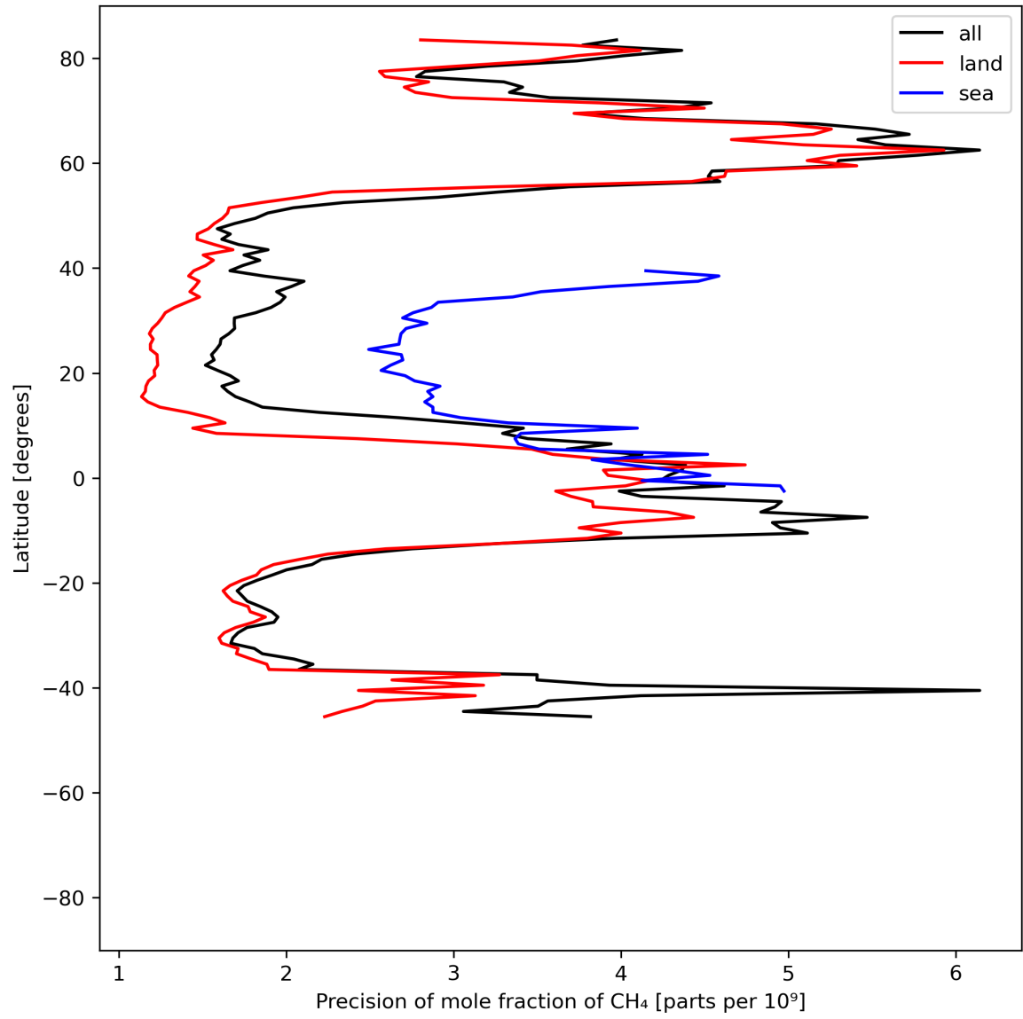
Figure 13: Zonal average of “Precision of mole fraction of CH 4 ” for 2024-04-21 to 2024-04-22.
