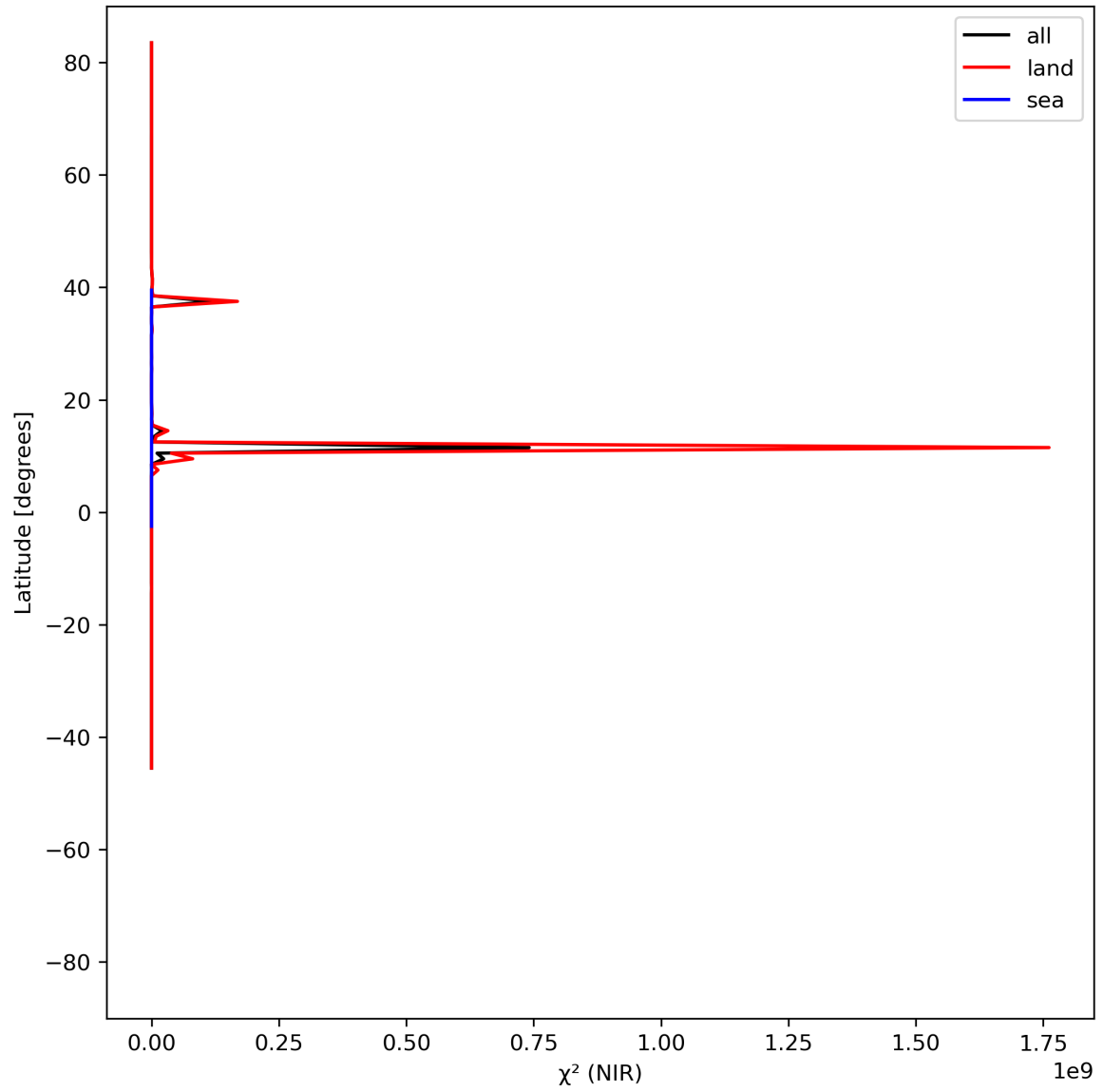
Figure 18: Zonal average of “ \chi^2 (NIR)” for 2024-04-21 to 2024-04-22.
