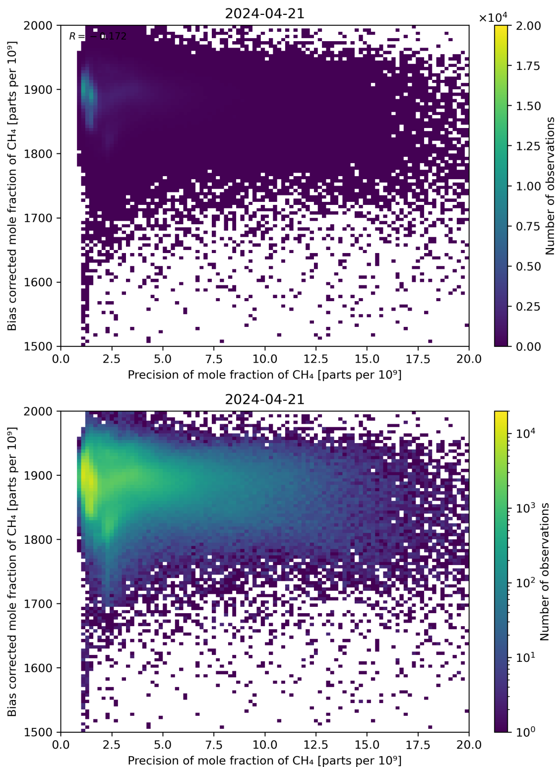
Figure 82: Scatter density plot of “Precision of mole fraction of CH 4 ” against “Bias corrected mole fraction of CH 4 ” for 2024-04-21 to 2024-04-22.
