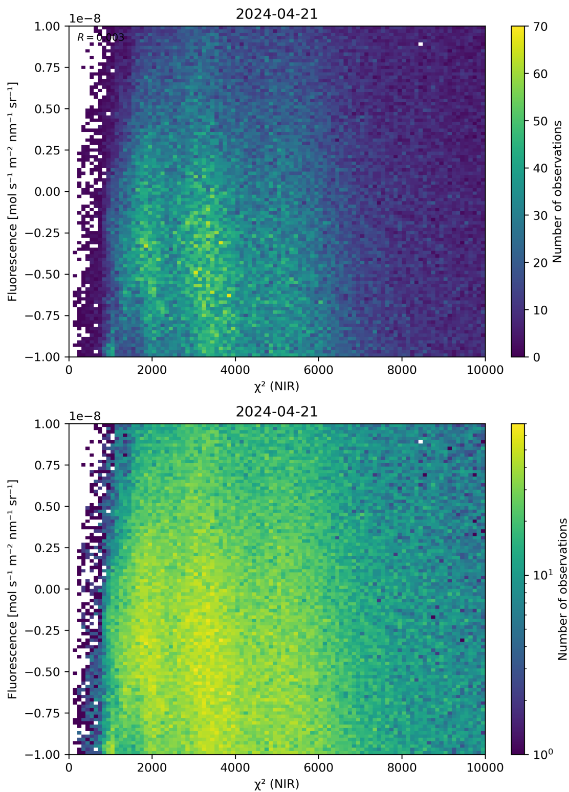
Figure 45: Scatter density plot of “ \chi^2 (NIR)” against “Fluorescence” for 2024-04-21 to 2024-04-22.
