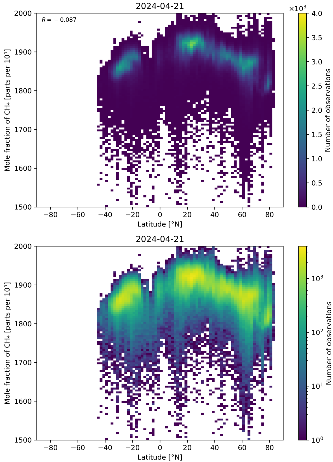
Figure 57: Scatter density plot of “Latitude” against “Mole fraction of \text{CH}_4 ” for 2024-04-21 to 2024-04-22.
