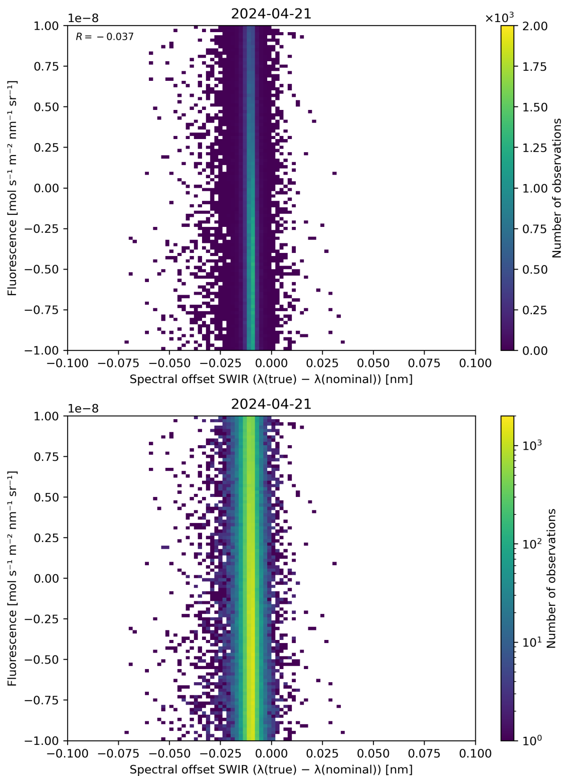
Figure 120: Scatter density plot of “Spectral offset SWIR ( \lambda(\text{true}) - \lambda(\text{nominal}) )” against “Fluorescence” for 2024-04-21 to 2024-04-22.
