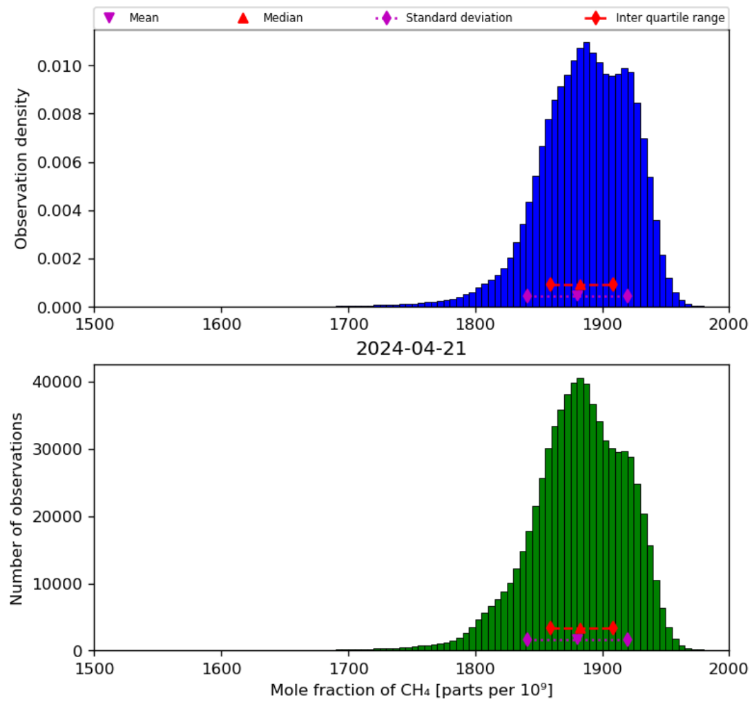
Figure 23: Histogram of “Mole fraction of CH 4 ” for 2024-04-21 to 2024-04-22
