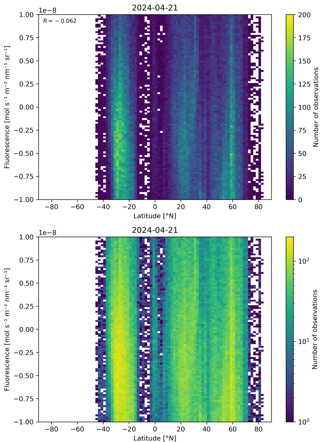
Figure 56: Scatter density plot of “Latitude” against “Fluorescence” for 2024-04-21 to 2024-04-22.
