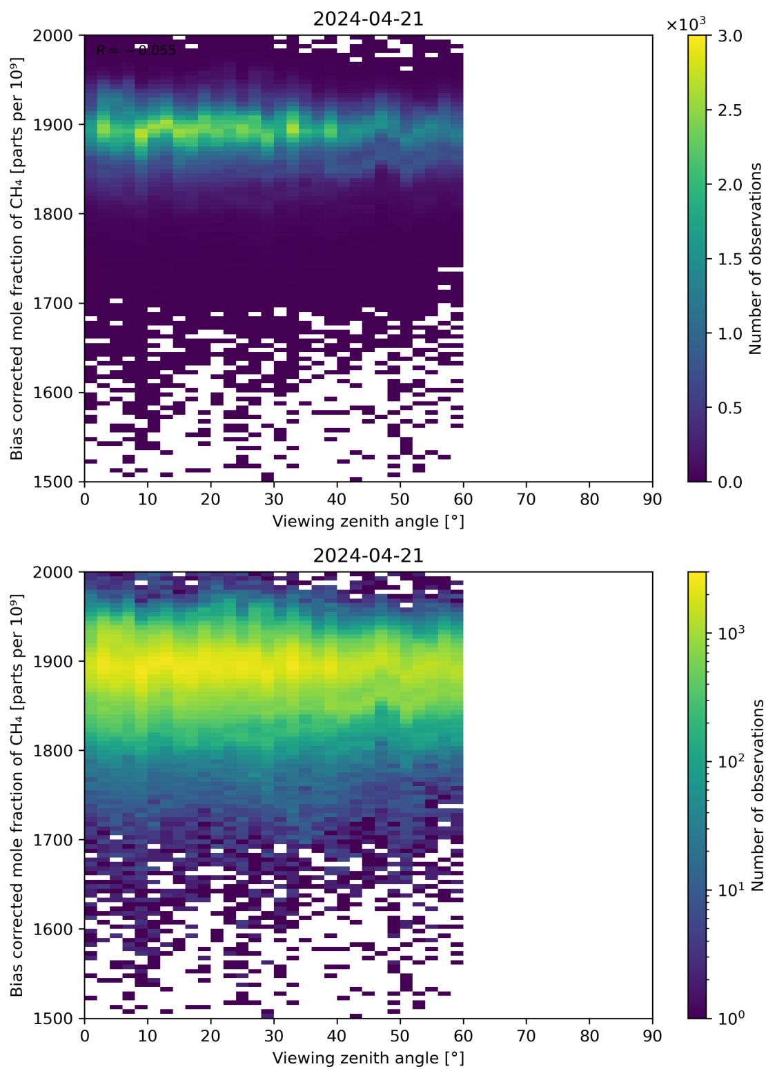
Figure 111: Scatter density plot of “Viewing zenith angle” against “Bias corrected mole fraction of CH 4 ” for 2024-04-21 to 2024-04-22.
