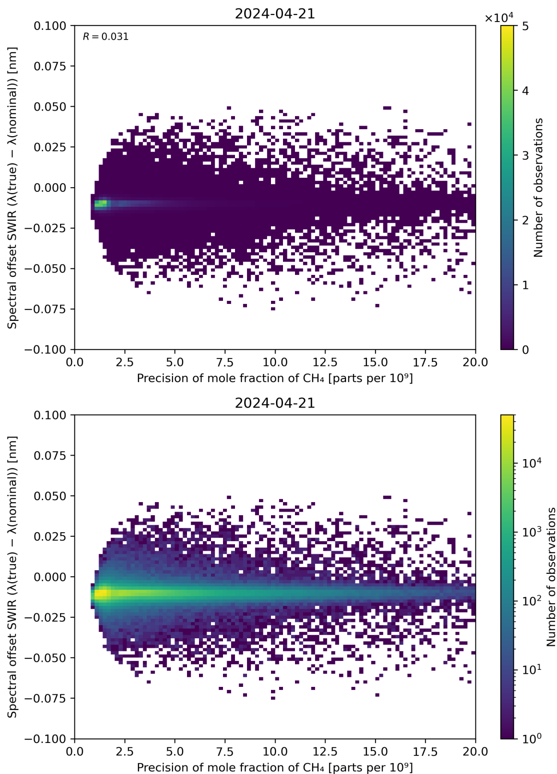
Figure 85: Scatter density plot of “Precision of mole fraction of CH 4 ” against “Spectral offset SWIR ( \lambda(\text{true}) - \lambda(\text{nominal}) )” for 2024-04-21 to 2024-04-22.
