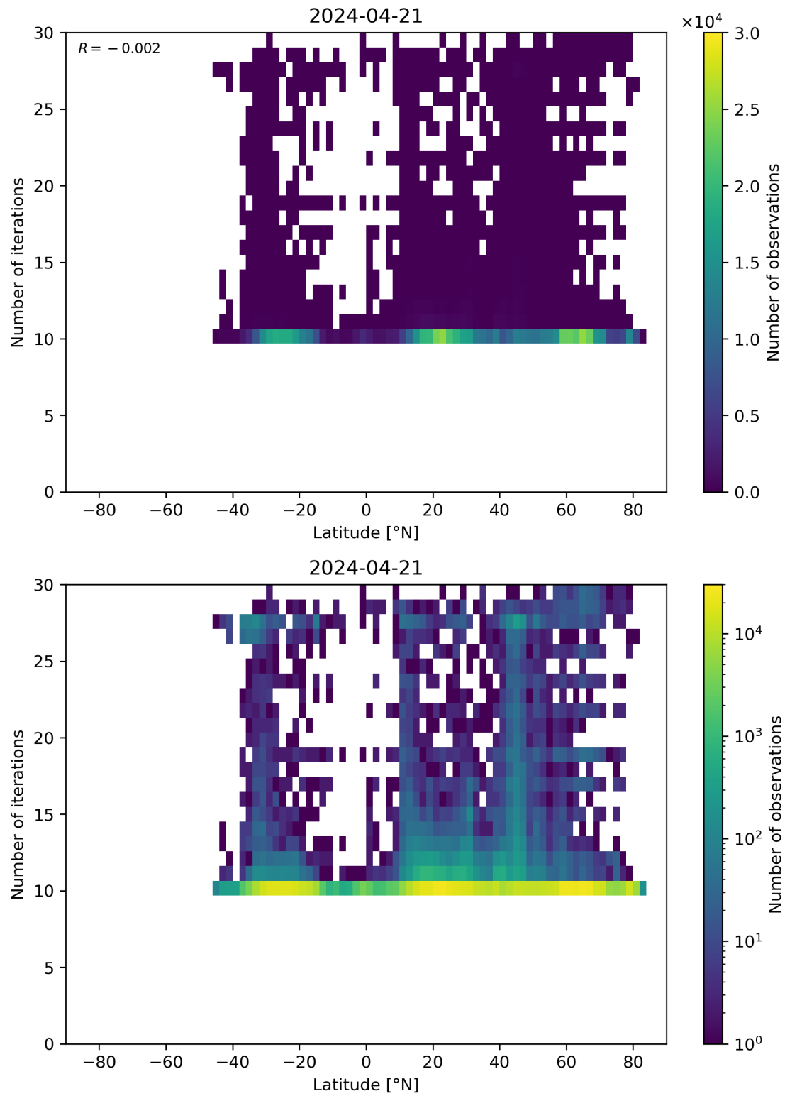
Figure 60: Scatter density plot of “Latitude” against “Number of iterations” for 2024-04-21 to 2024-04-22.
