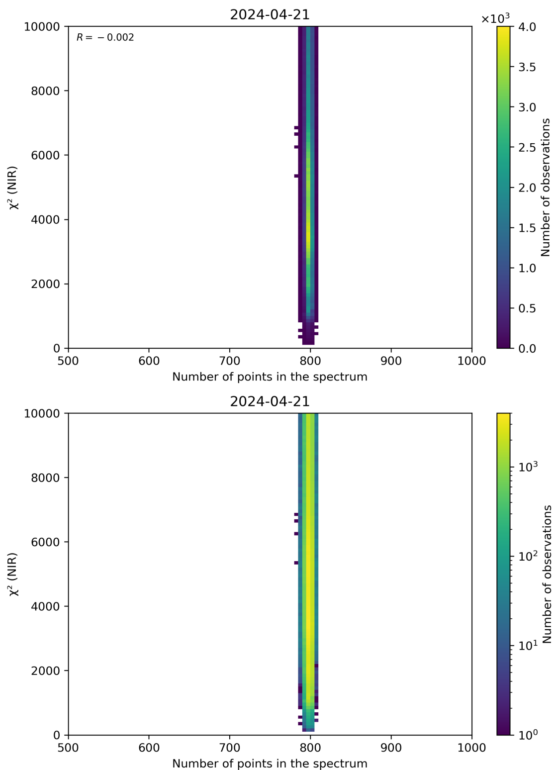
Figure 88: Scatter density plot of “Number of points in the spectrum” against “ \chi^2 (NIR)” for 2024-04-21 to 2024-04-22.
