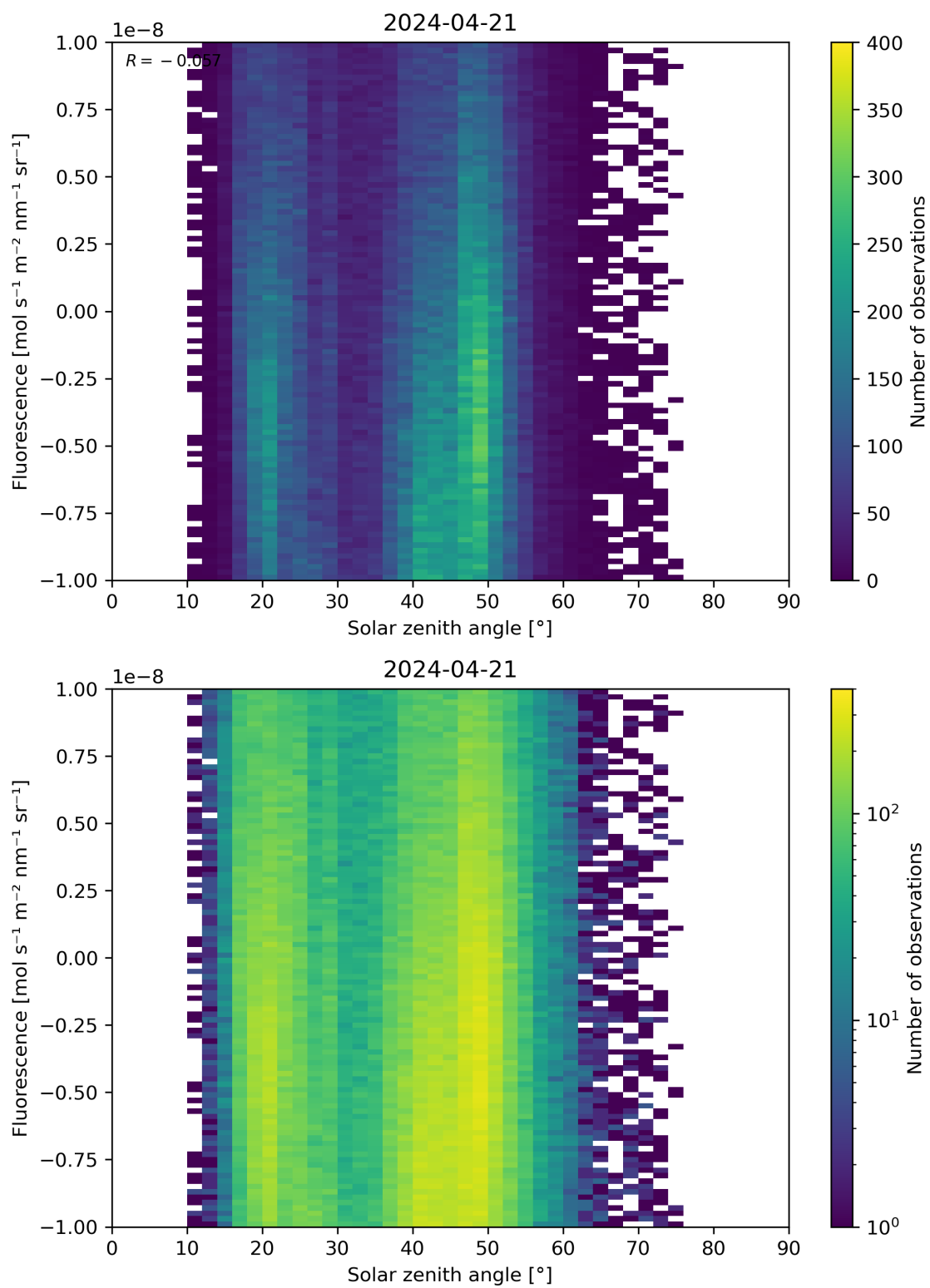
Figure 97: Scatter density plot of “Solar zenith angle” against “Fluorescence” for 2024-04-21 to 2024-04-22.
