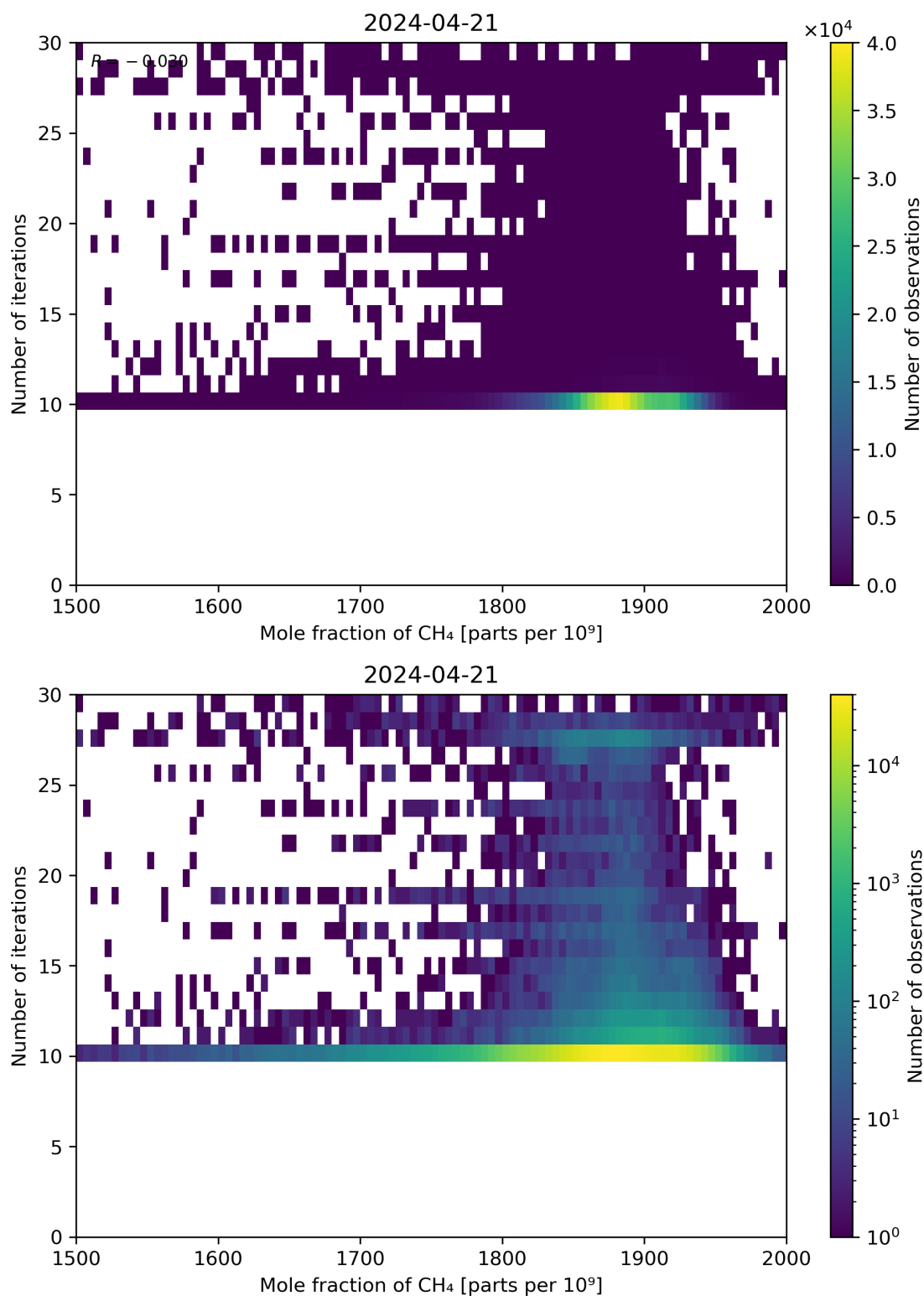
Figure 76: Scatter density plot of “Mole fraction of CH 4 ” against “Number of iterations” for 2024-04-21 to 2024-04-22.
