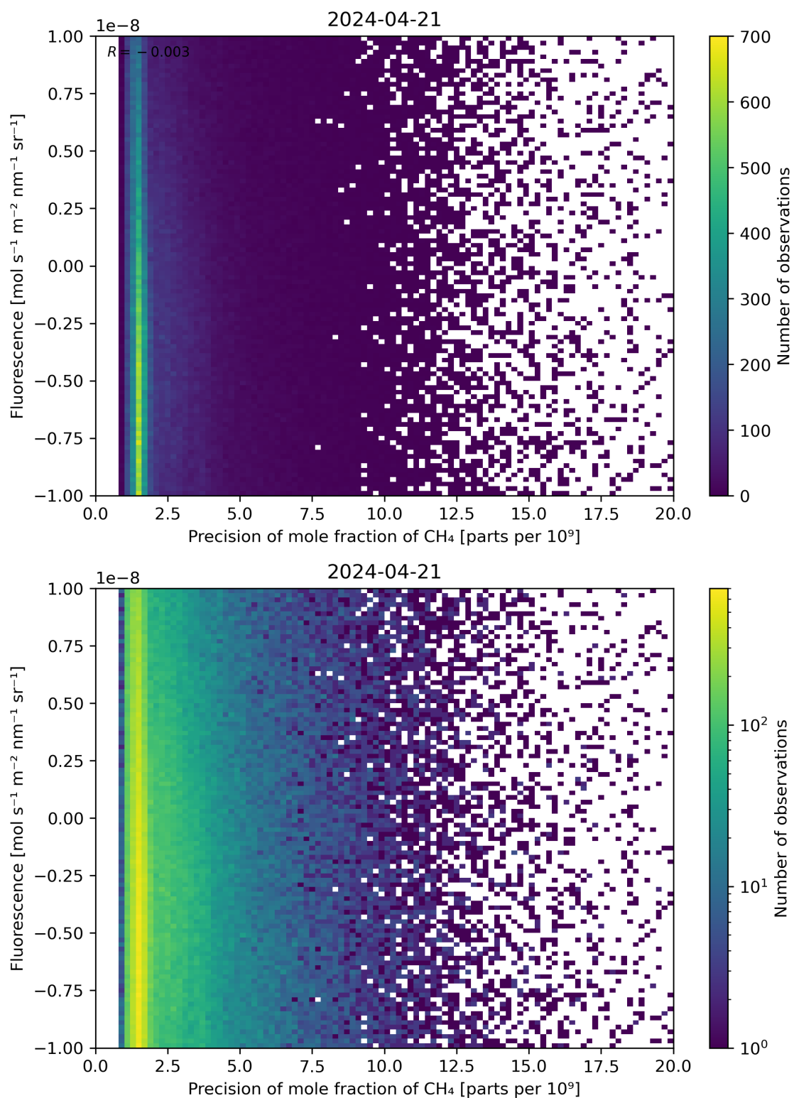
Figure 81: Scatter density plot of “Precision of mole fraction of CH 4 ” against “Fluorescence” for 2024-04-21 to 2024-04-22.
