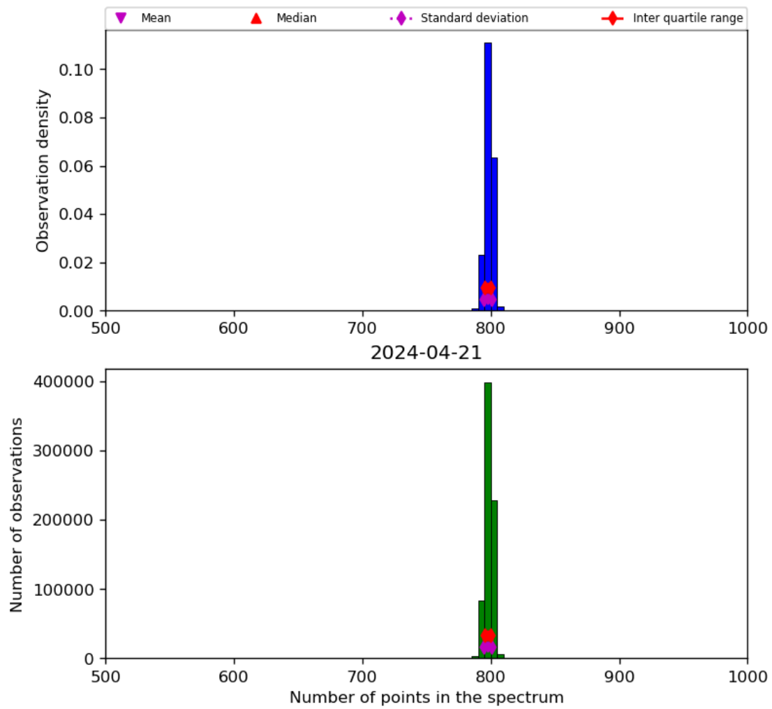
Figure 26: Histogram of “Number of points in the spectrum” for 2024-04-21 to 2024-04-22
