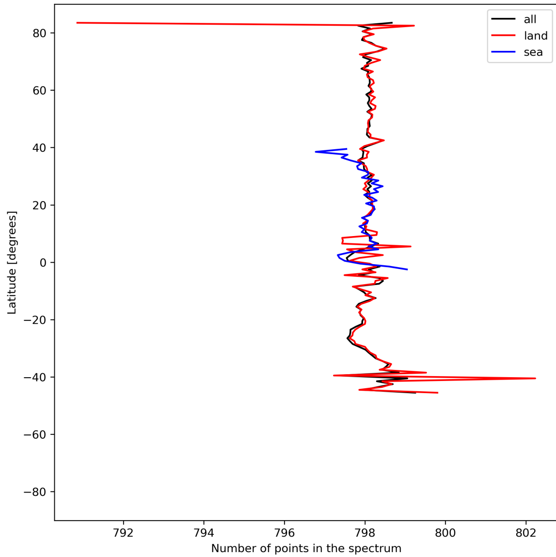
Figure 15: Zonal average of “Number of points in the spectrum” for 2024-04-21 to 2024-04-22.
