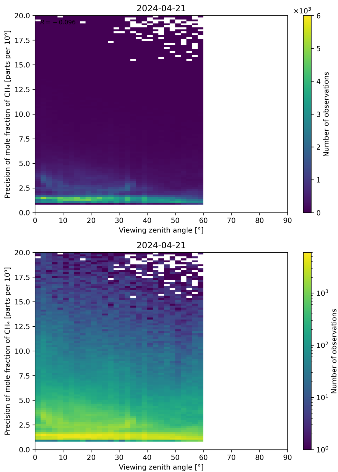
Figure 112: Scatter density plot of “Viewing zenith angle” against “Precision of mole fraction of CH 4 ” for 2024-04-21 to 2024-04-22.
