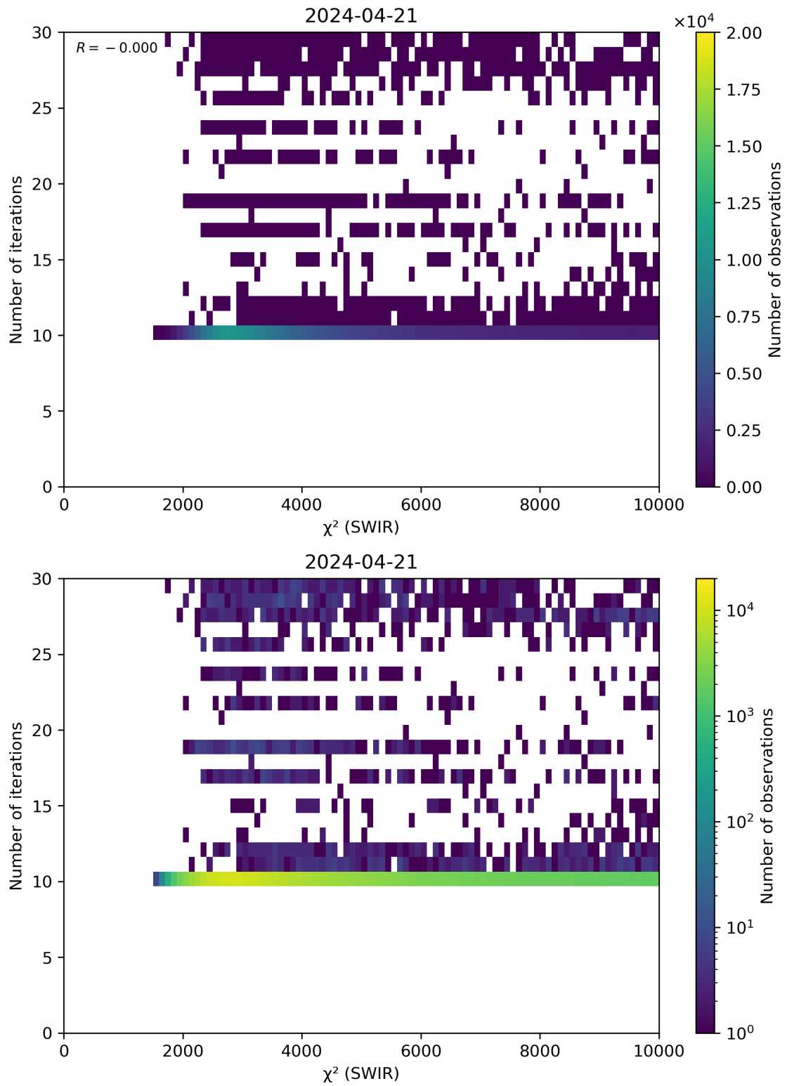
Figure 50: Scatter density plot of “ \chi^2 (SWIR)” against “Number of iterations” for 2024-04-21 to 2024-04-22.
