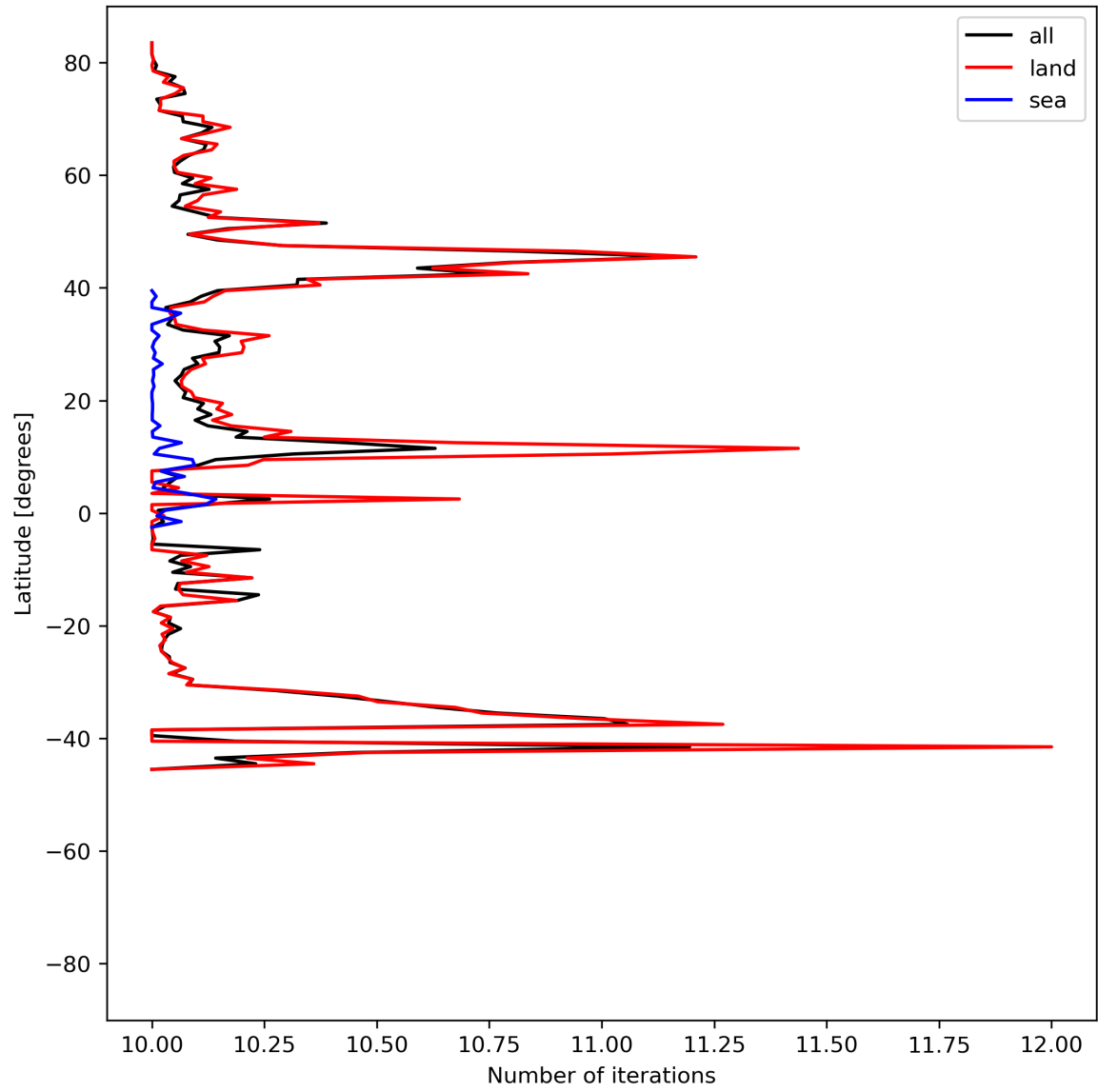
Figure 20: Zonal average of “Number of iterations” for 2024-04-21 to 2024-04-22.
