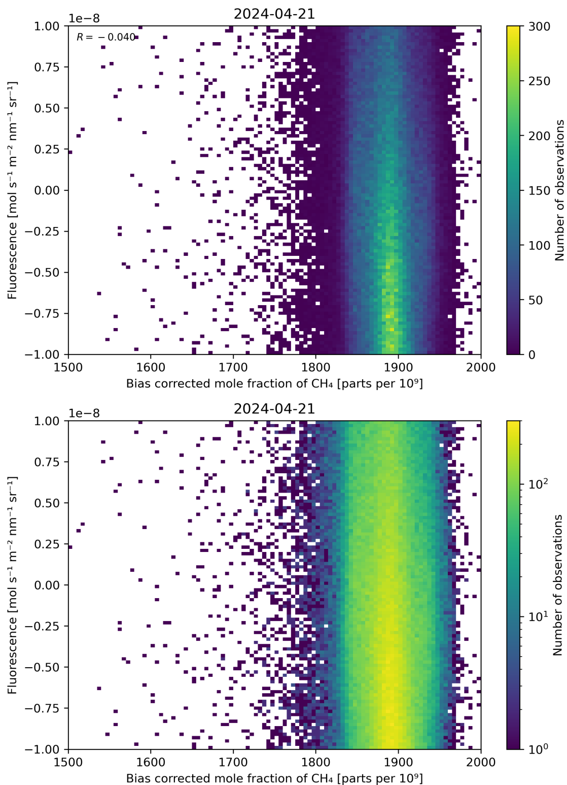
Figure 66: Scatter density plot of “Bias corrected mole fraction of \text{CH}_4 ” against “Fluorescence” for 2024-04-21 to 2024-04-22.
