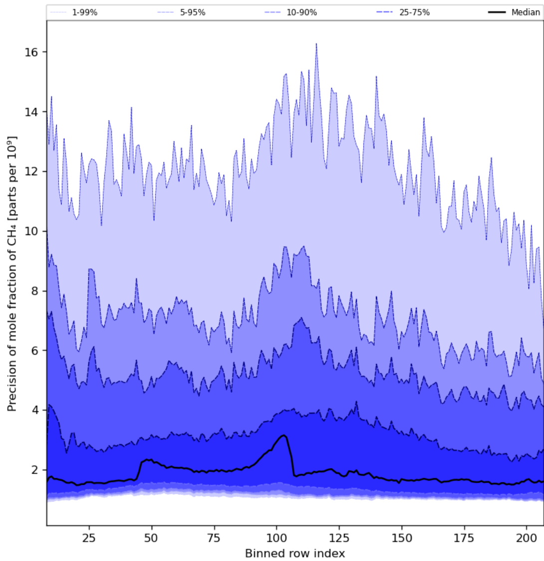
Figure 35: Along track statistics of “Precision of mole fraction of CH 4 ” for 2024-04-21 to 2024-04-22
