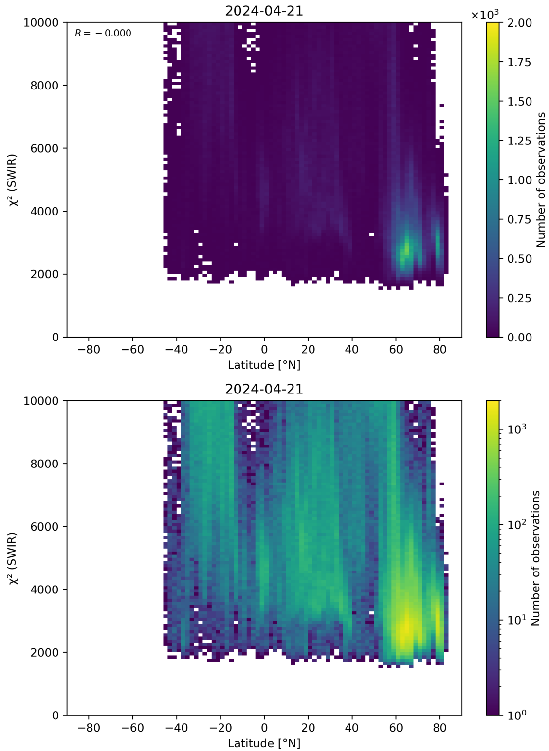
Figure 54: Scatter density plot of “Latitude” against “ \chi^2 (SWIR)” for 2024-04-21 to 2024-04-22.
