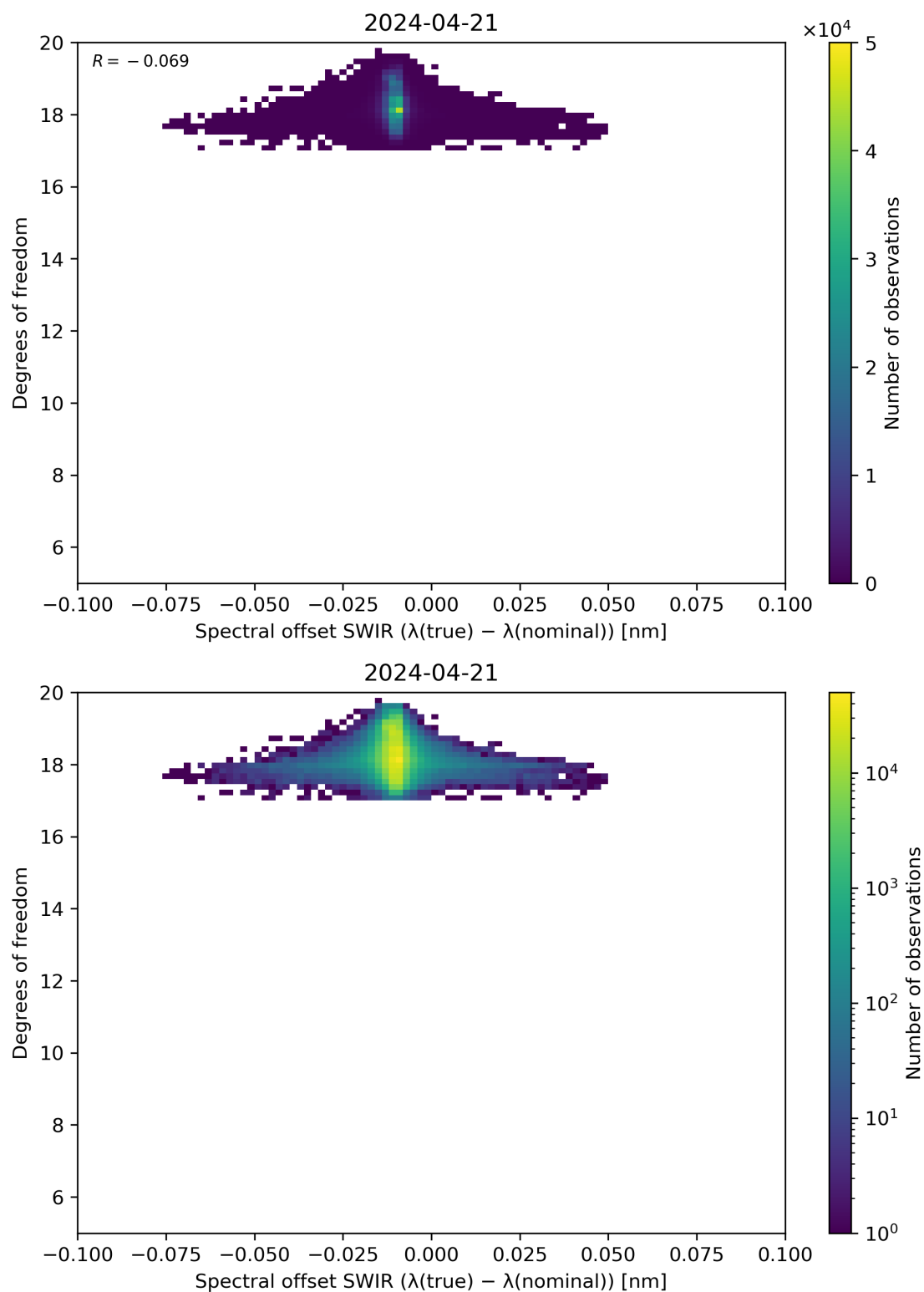
Figure 119: Scatter density plot of “Spectral offset SWIR ( \lambda(\text{true}) - \lambda(\text{nominal}) )” against “Degrees of freedom” for 2024-04-21 to 2024-04-22.
