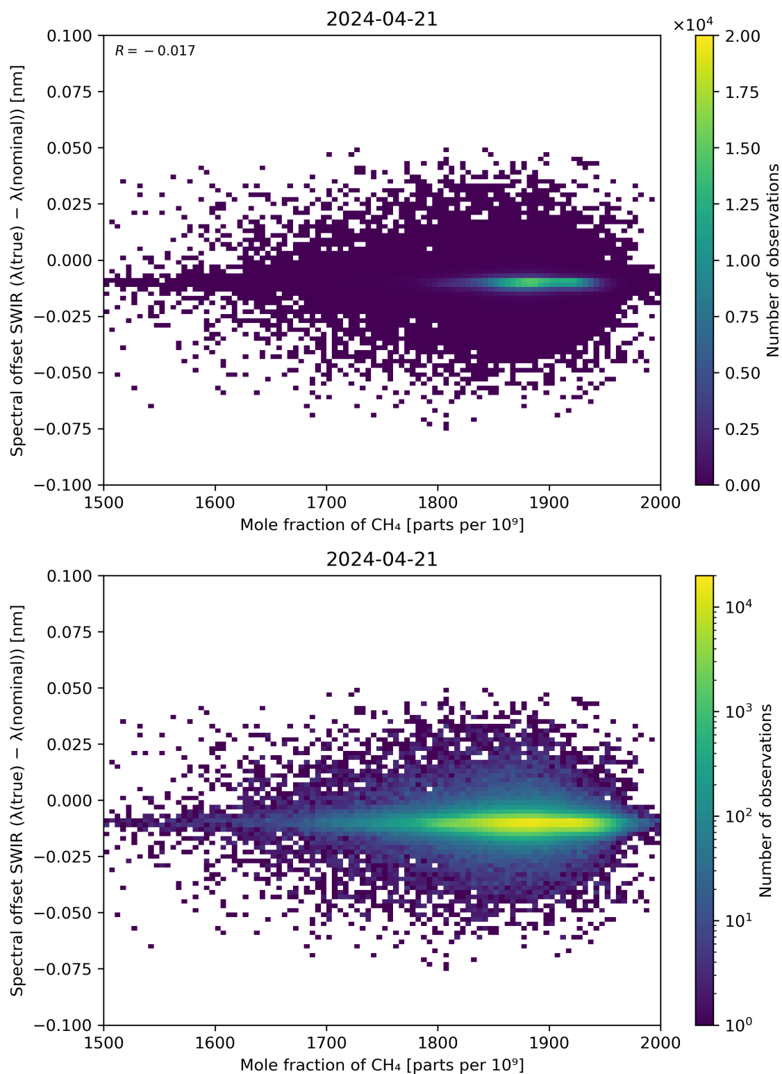
Figure 86: Scatter density plot of “Mole fraction of CH 4 ” against “Spectral offset SWIR ( \lambda(\text{true}) - \lambda(\text{nominal}) )” for 2024-04-21 to 2024-04-22.
