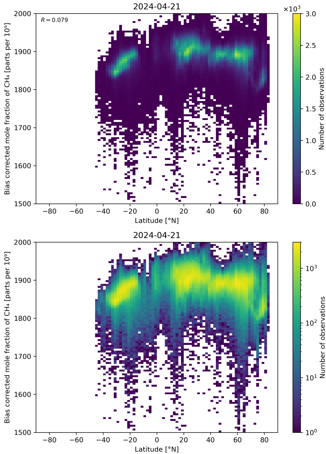
Figure 58: Scatter density plot of “Latitude” against “Bias corrected mole fraction of CH 4 ” for 2024-04-21 to 2024-04-22.
