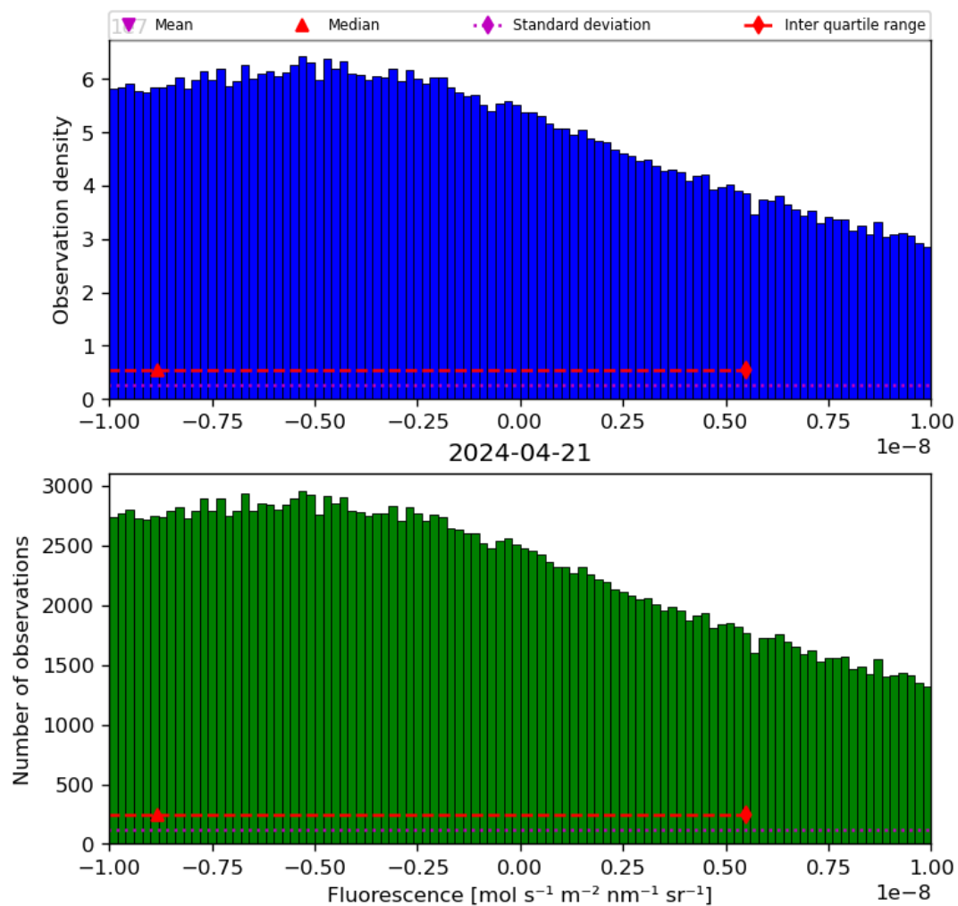
Figure 32: Histogram of “Fluorescence” for 2024-04-21 to 2024-04-22
