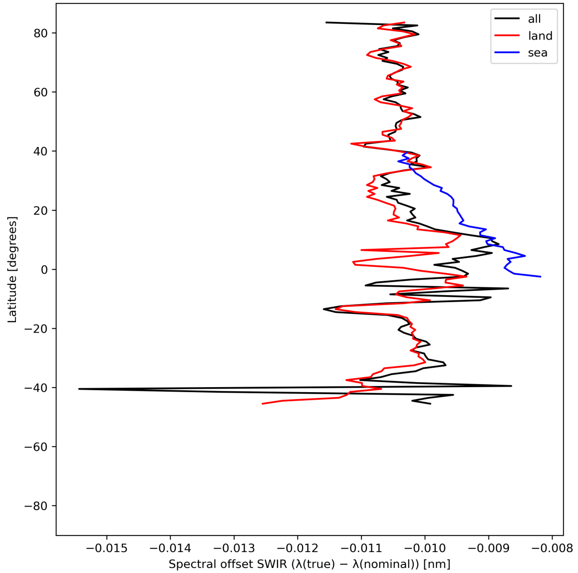
Figure 16: Zonal average of “Spectral offset SWIR ( \lambda(\text{true}) - \lambda(\text{nominal}) )” for 2024-04-21 to 2024-04-22.
