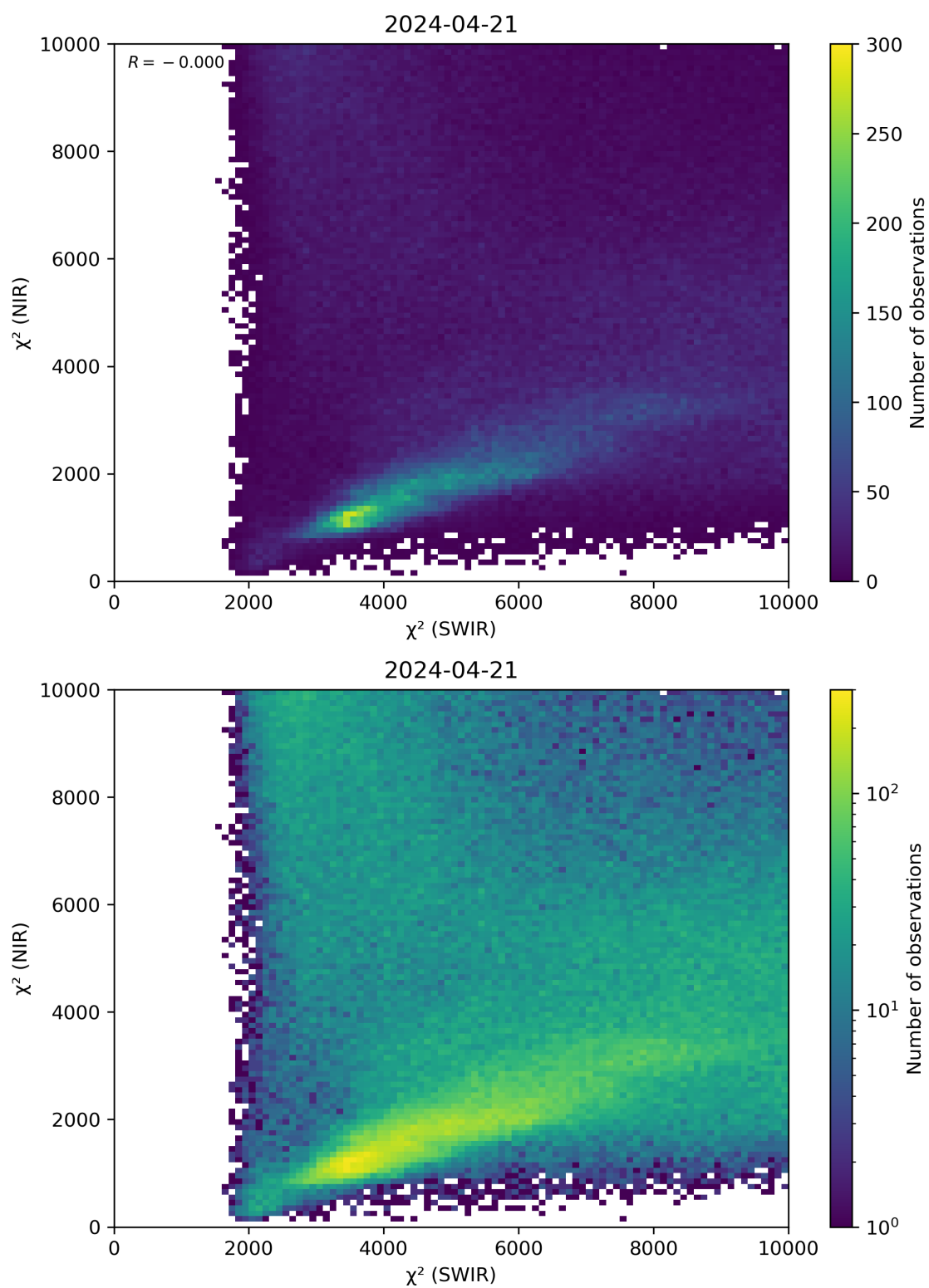
Figure 47: Scatter density plot of “ \chi^2 (SWIR)” against “ \chi^2 (NIR)” for 2024-04-21 to 2024-04-22.
