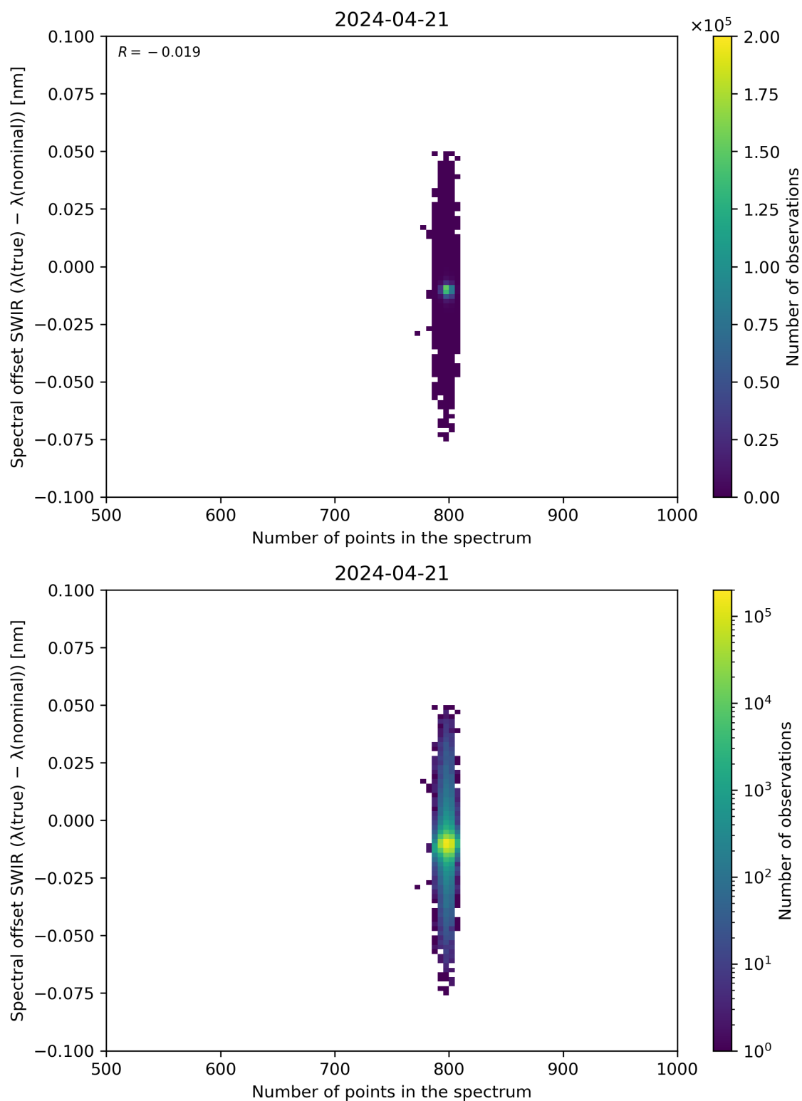
Figure 93: Scatter density plot of “Number of points in the spectrum” against “Spectral offset SWIR ( \lambda(\text{true}) - \lambda(\text{nominal}) )” for 2024-04-21 to 2024-04-22.
