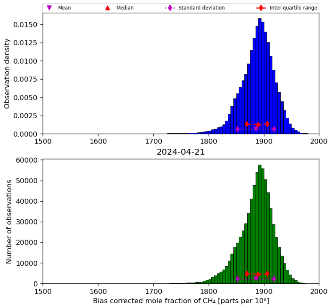
Figure 25: Histogram of “Bias corrected mole fraction of CH 4 ” for 2024-04-21 to 2024-04-22
