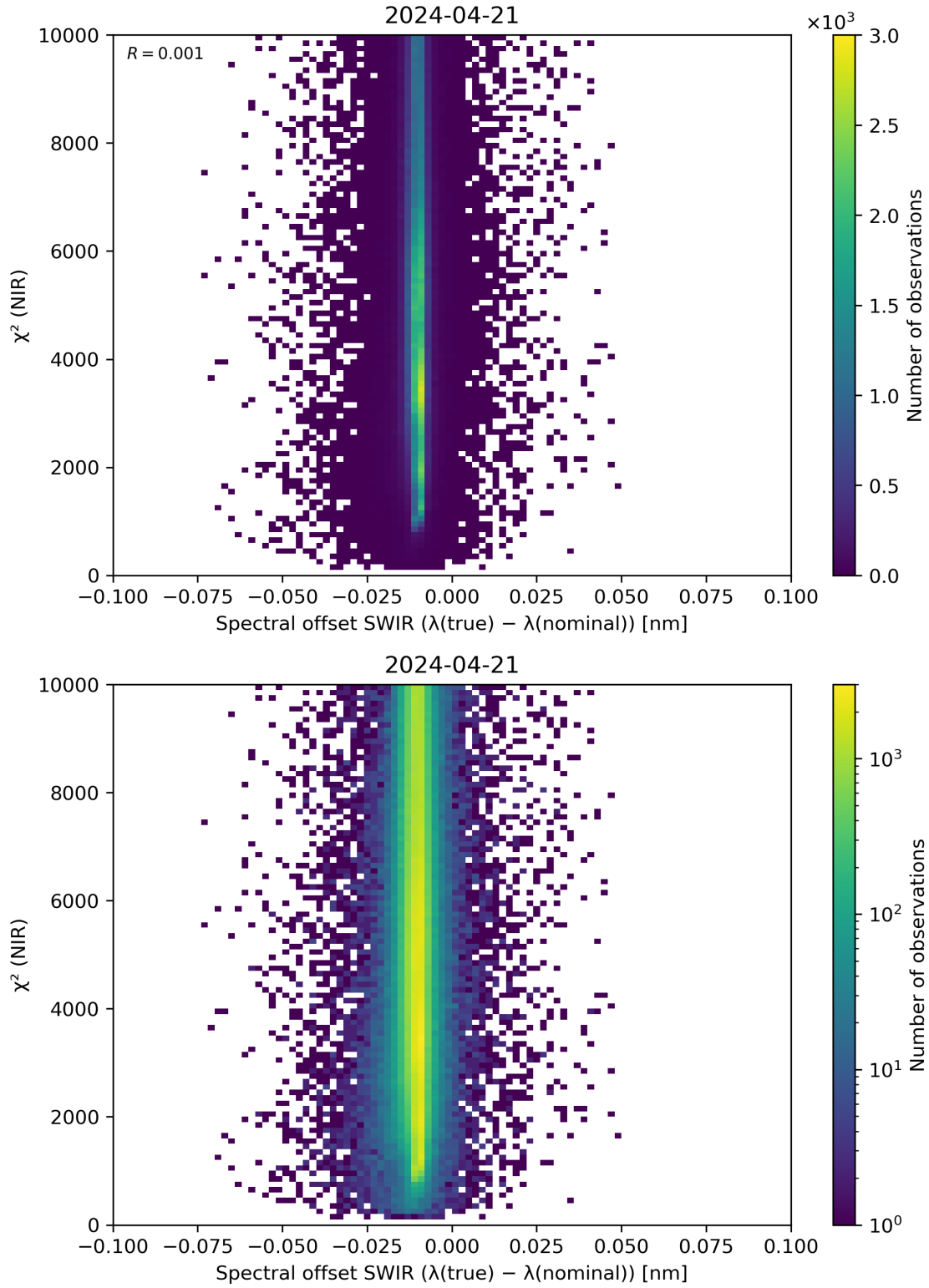
Figure 117: Scatter density plot of “Spectral offset SWIR ( \lambda(\text{true}) - \lambda(\text{nominal}) )” against “ \chi^2 (NIR)” for 2024-04-21 to 2024-04-22.
