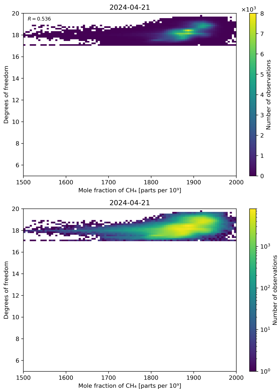
Figure 72: Scatter density plot of “Mole fraction of CH 4 ” against “Degrees of freedom” for 2024-04-21 to 2024-04-22.
