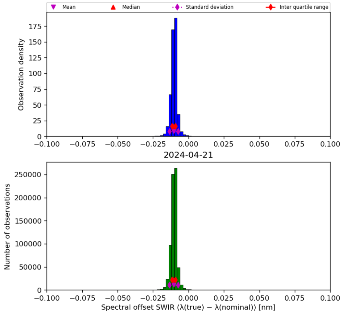
Figure 27: Histogram of “Spectral offset SWIR ( \lambda(\text{true}) - \lambda(\text{nominal}) )” for 2024-04-21 to 2024-04-22
