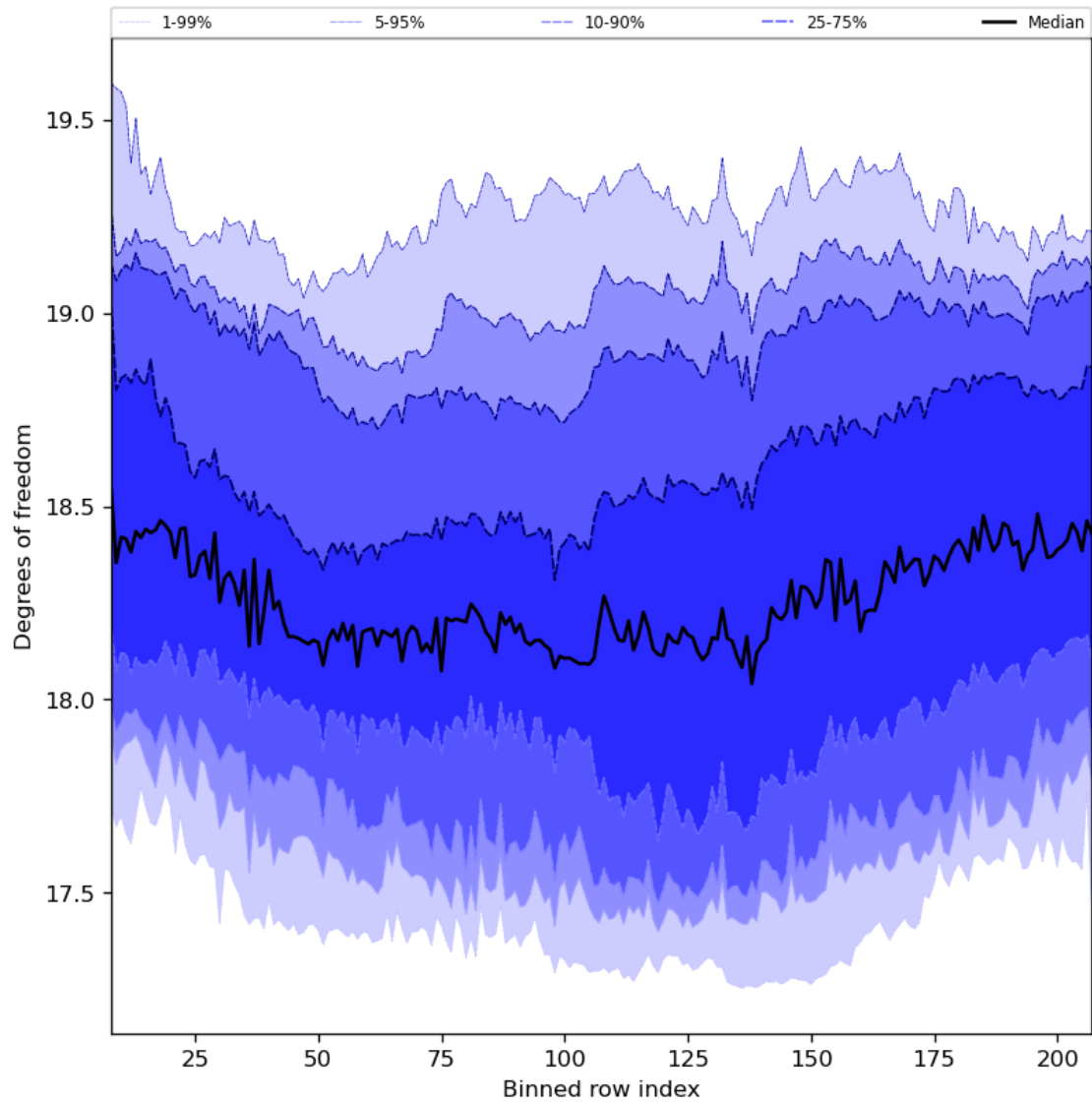
Figure 41: Along track statistics of “Degrees of freedom” for 2024-04-21 to 2024-04-22
