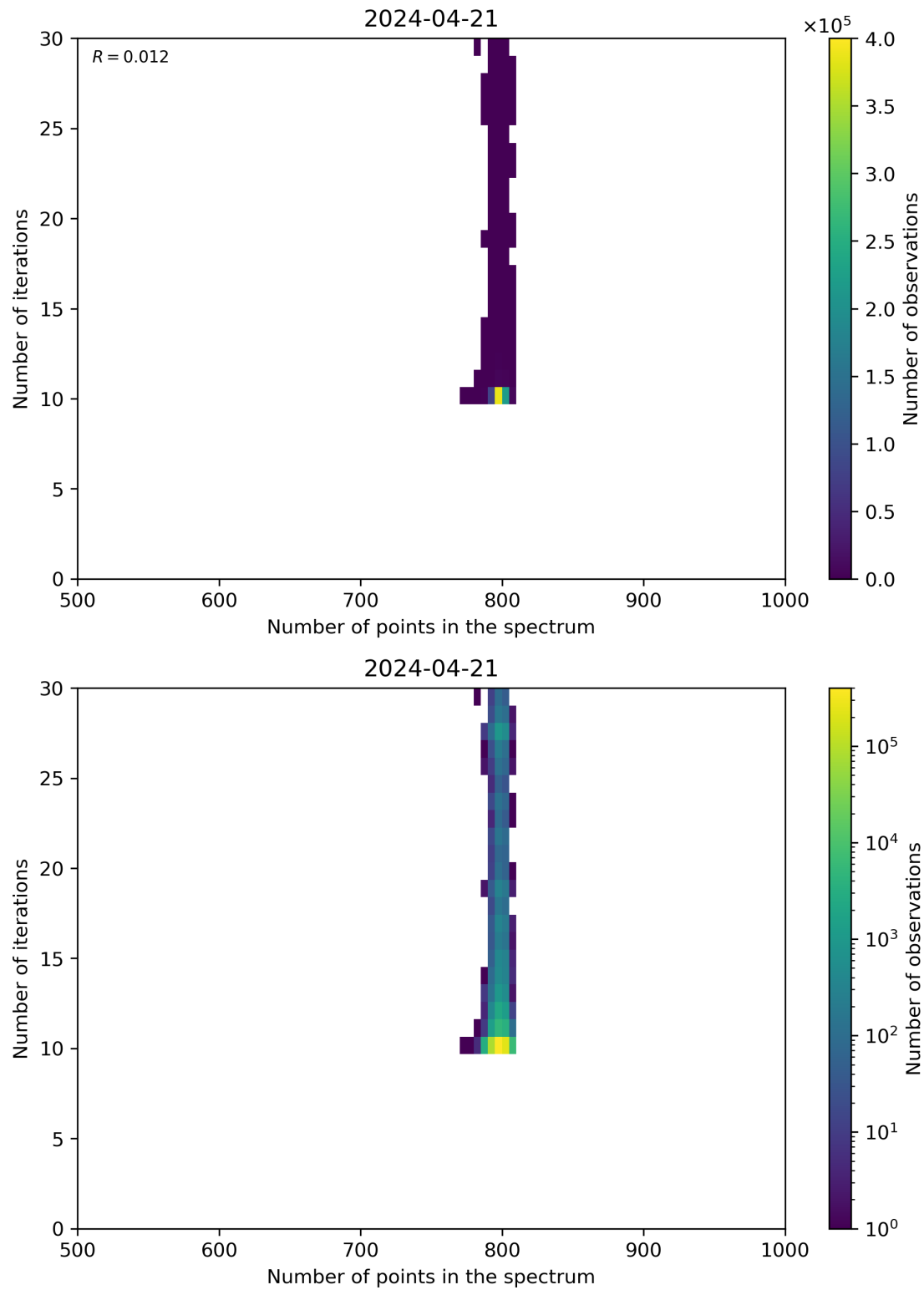
Figure 92: Scatter density plot of “Number of points in the spectrum” against “Number of iterations” for 2024-04-21 to 2024-04-22.
