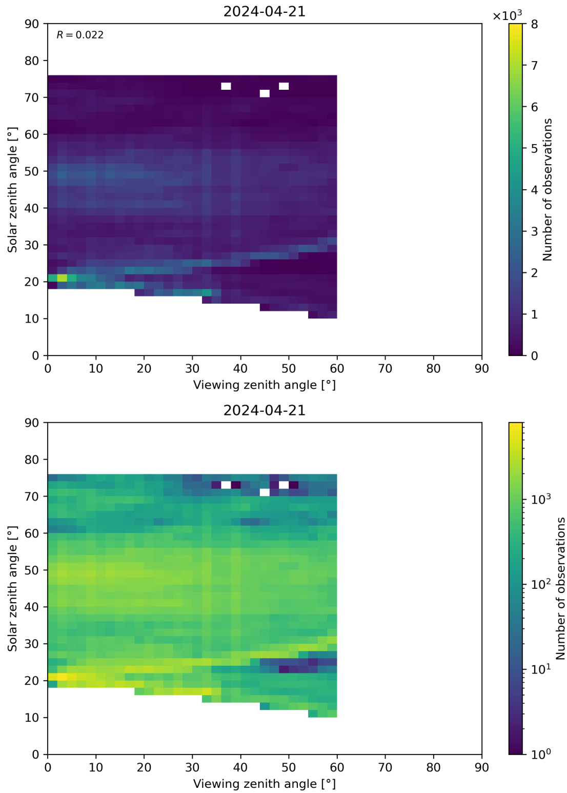
Figure 115: Scatter density plot of “Viewing zenith angle” against “Solar zenith angle” for 2024-04-21 to 2024-04-22.
