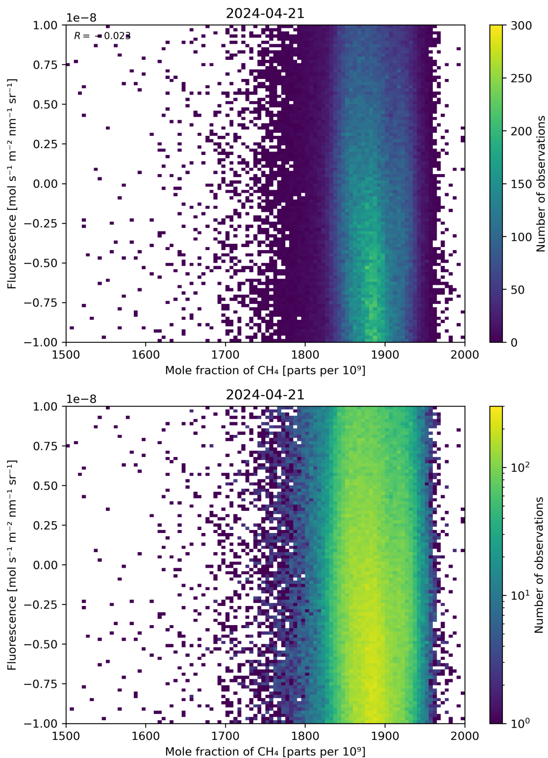
Figure 73: Scatter density plot of “Mole fraction of \text{CH}_4 ” against “Fluorescence” for 2024-04-21 to 2024-04-22.
