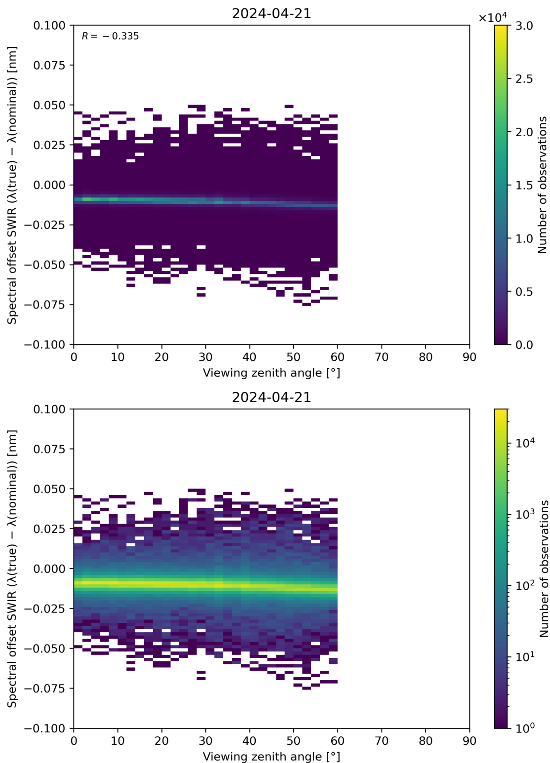
Figure 116: Scatter density plot of “Viewing zenith angle” against “Spectral offset SWIR ( \lambda(\text{true}) - \lambda(\text{nominal}) )” for 2024-04-21 to 2024-04-22.
