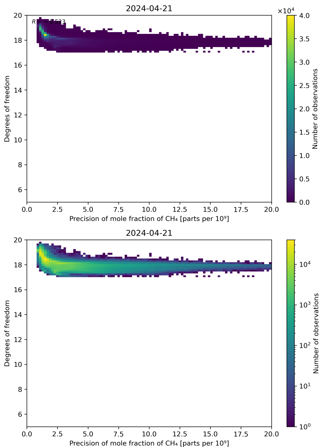
Figure 80: Scatter density plot of “Precision of mole fraction of CH 4 ” against “Degrees of freedom” for 2024-04-21 to 2024-04-22.
