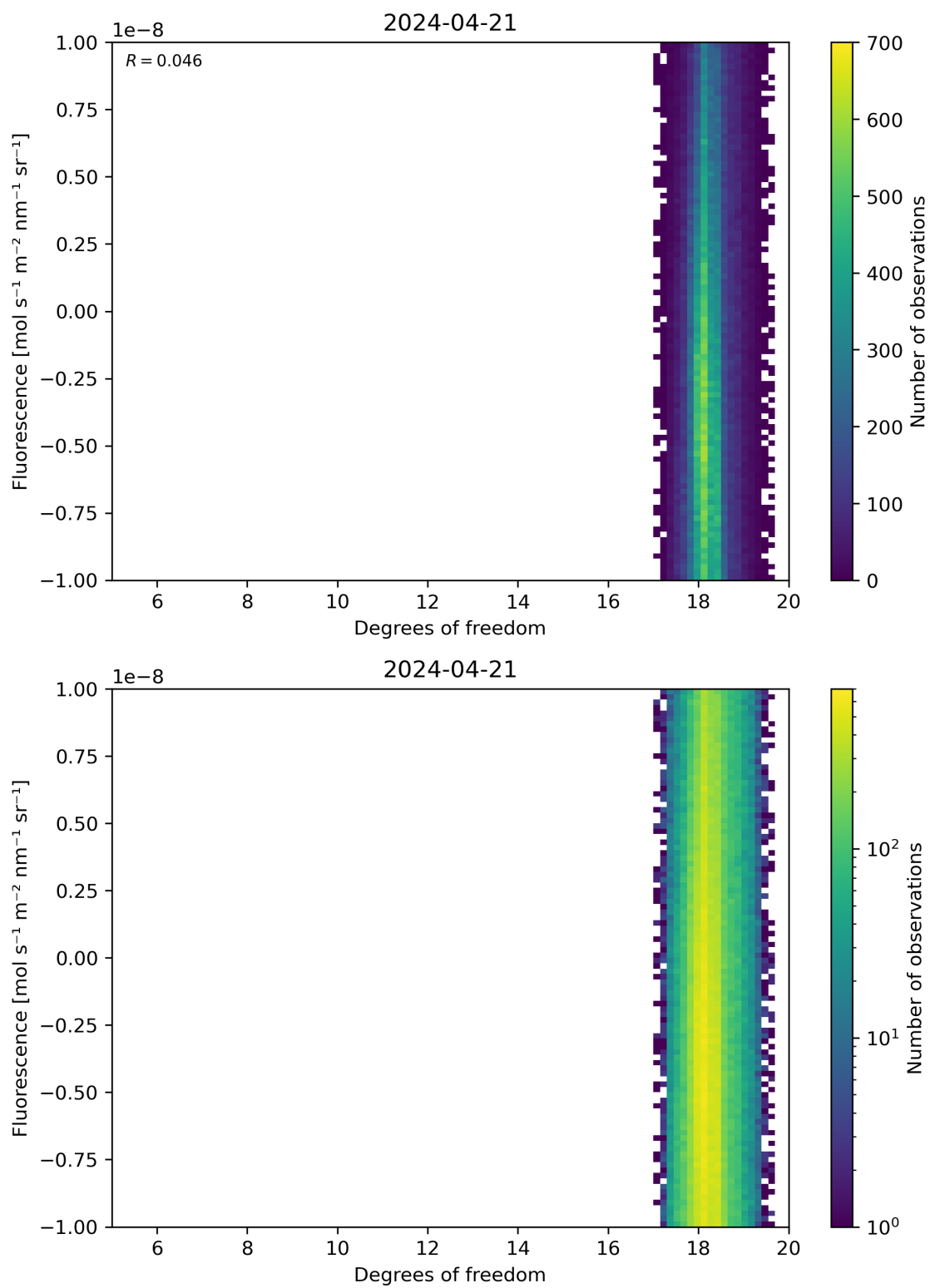
Figure 51: Scatter density plot of “Degrees of freedom” against “Fluorescence” for 2024-04-21 to 2024-04-22.
