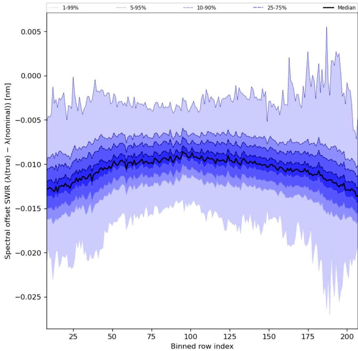
Figure 38: Along track statistics of “Spectral offset SWIR ( \lambda(\text{true}) - \lambda(\text{nominal}) )” for 2024-04-21 to 2024-04-22
