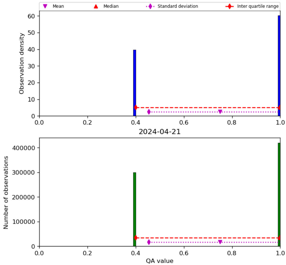
Figure 22: Histogram of “QA value” for 2024-04-21 to 2024-04-22
