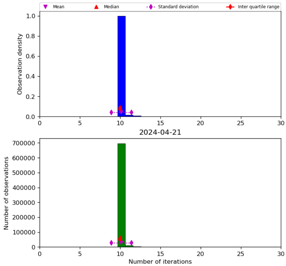
Figure 31: Histogram of “Number of iterations” for 2024-04-21 to 2024-04-22
