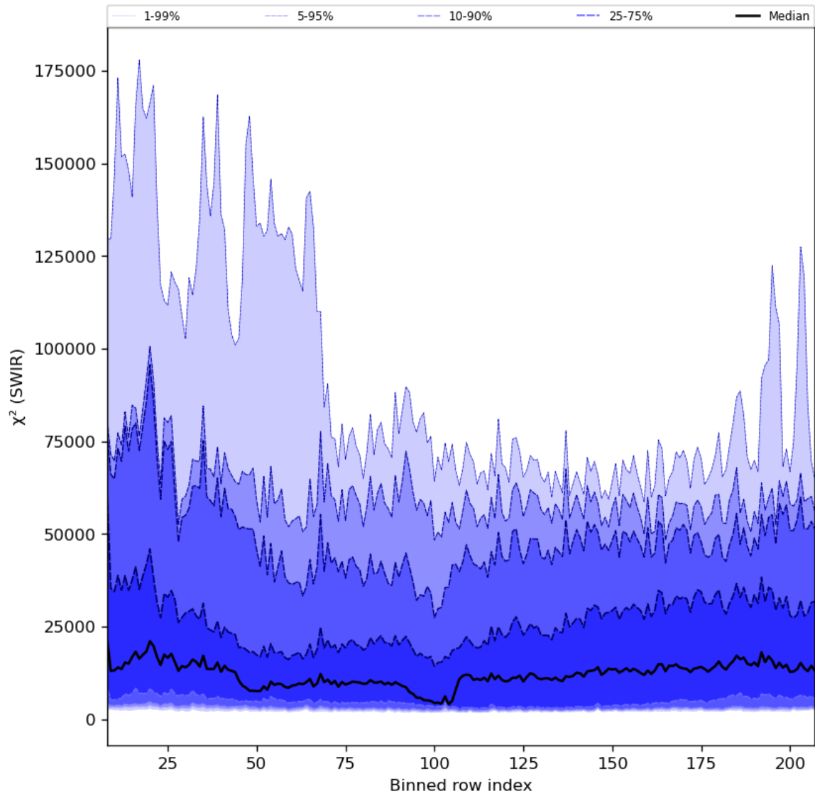
Figure 39: Along track statistics of “ \chi^2 (SWIR)” for 2024-04-21 to 2024-04-22
