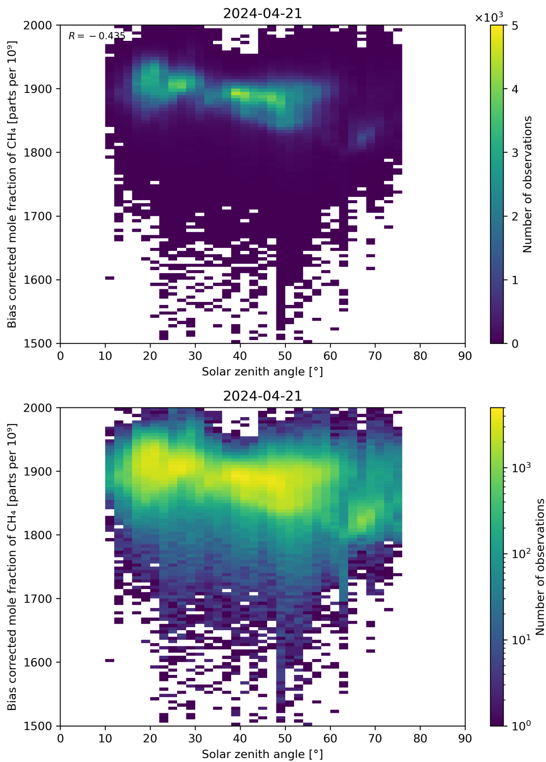
Figure 100: Scatter density plot of “Solar zenith angle” against “Bias corrected mole fraction of CH 4 ” for 2024-04-21 to 2024-04-22.
