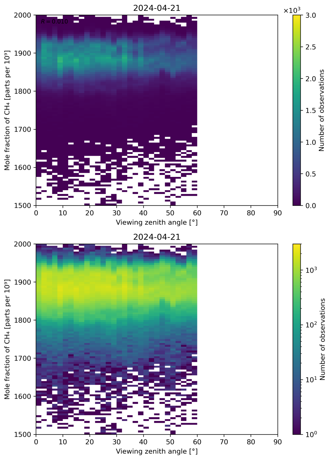
Figure 110: Scatter density plot of “Viewing zenith angle” against “Mole fraction of CH 4 ” for 2024-04-21 to 2024-04-22.
