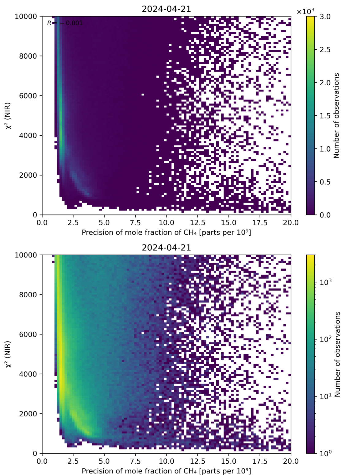
Figure 78: Scatter density plot of “Precision of mole fraction of CH 4 ” against “ \chi^2 (NIR)” for 2024-04-21 to 2024-04-22.
