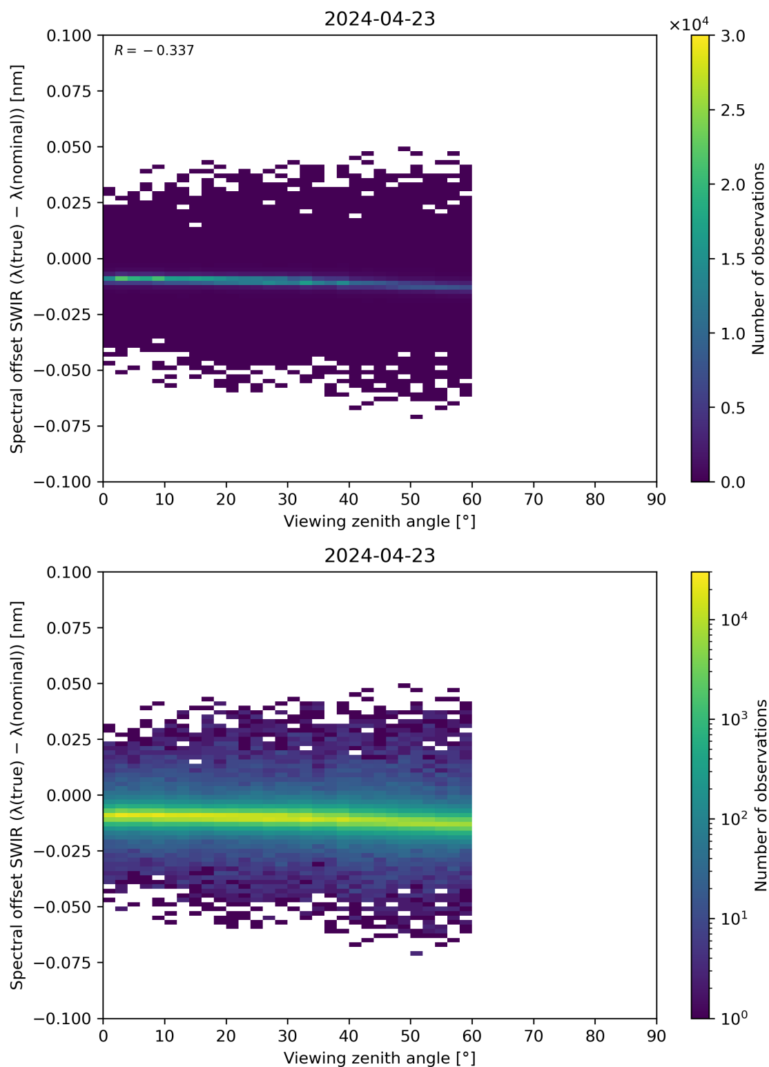
Figure 116: Scatter density plot of “Viewing zenith angle” against “Spectral offset SWIR ( \lambda(\text{true}) - \lambda(\text{nominal}) )” for 2024-04-22 to 2024-04-24.
