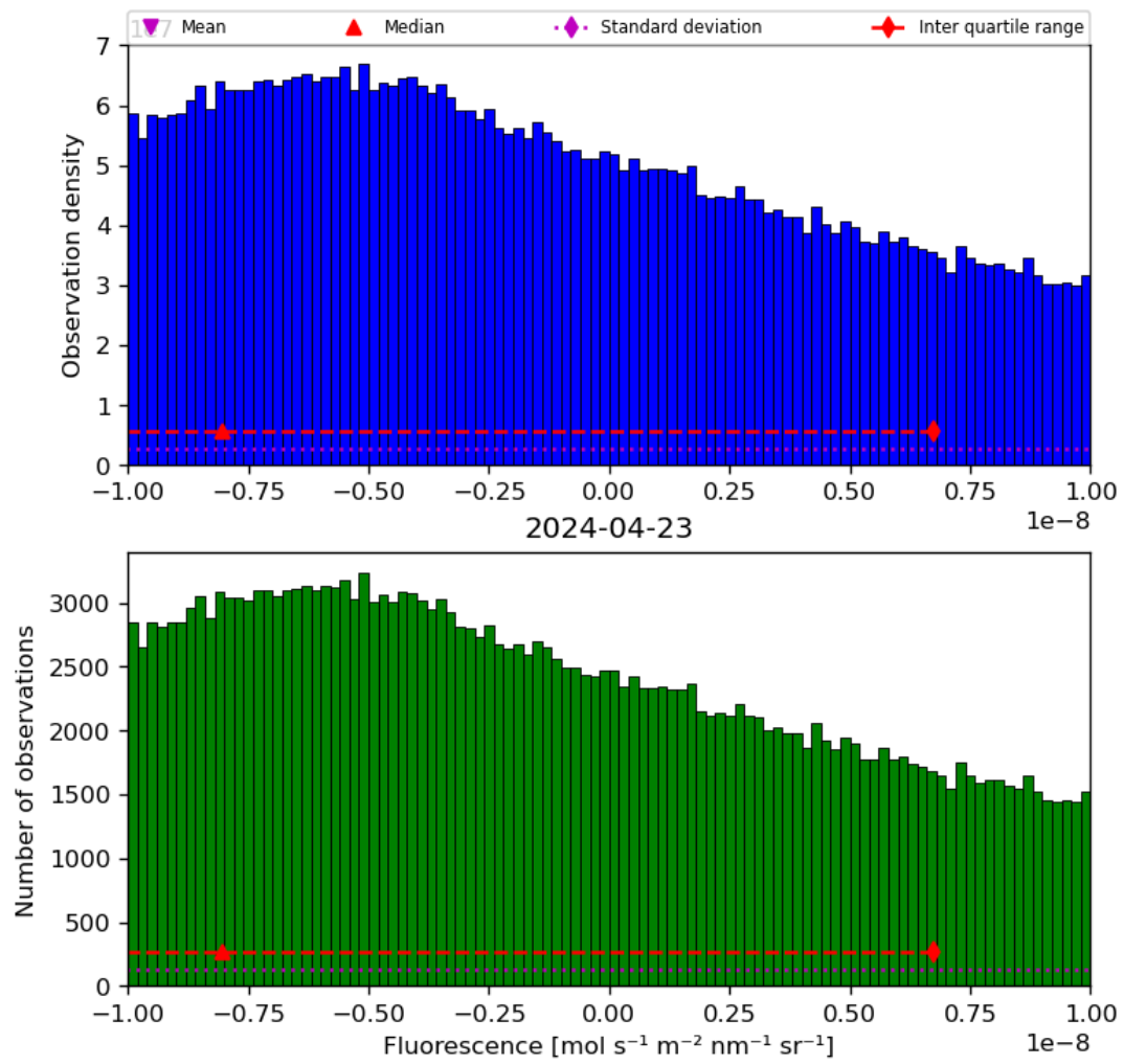
Figure 32: Histogram of “Fluorescence” for 2024-04-22 to 2024-04-24
