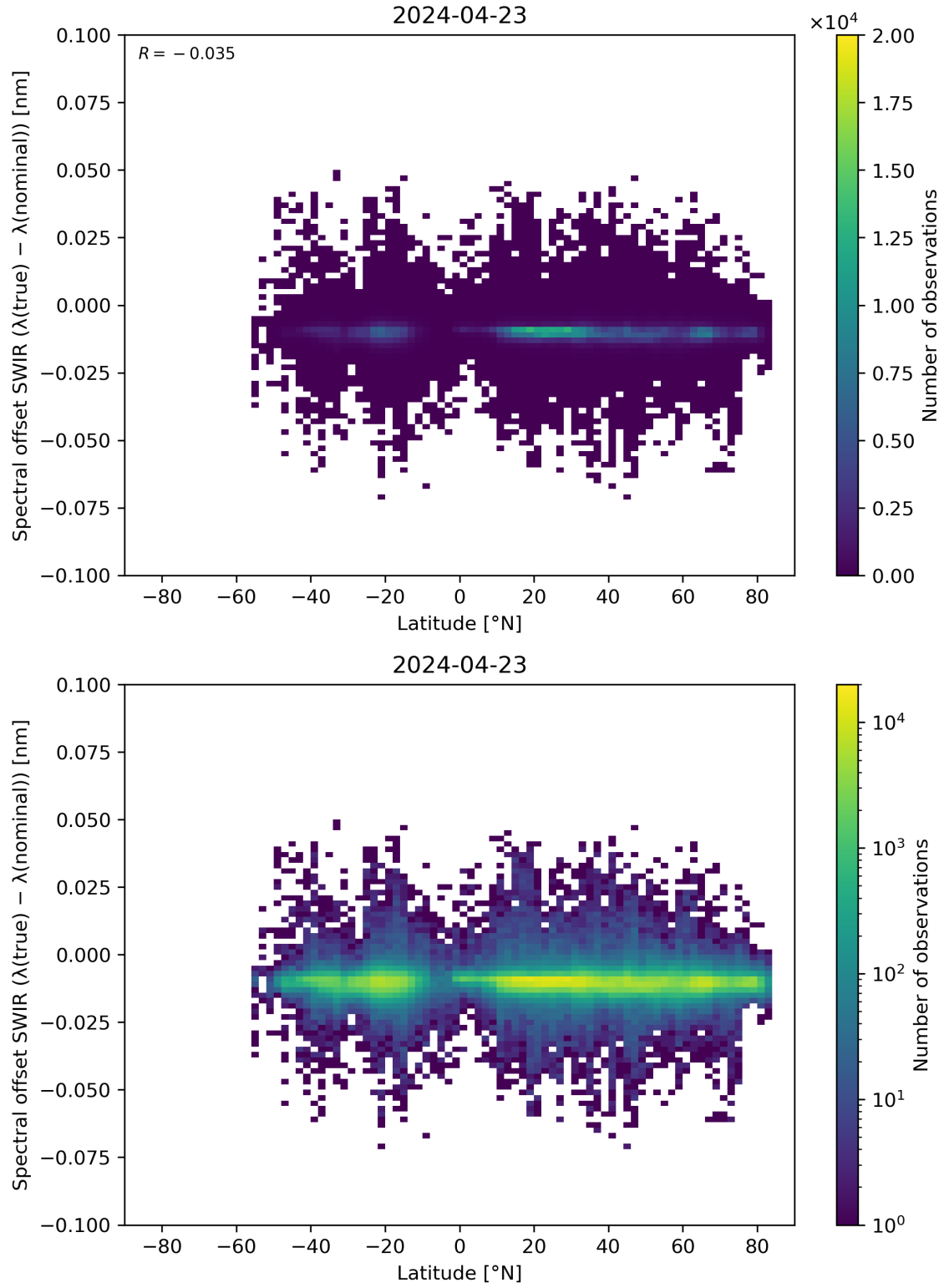
Figure 62: Scatter density plot of “Latitude” against “Spectral offset SWIR ( \lambda(\text{true}) - \lambda(\text{nominal}) )” for 2024-04-22 to 2024-04-24.
