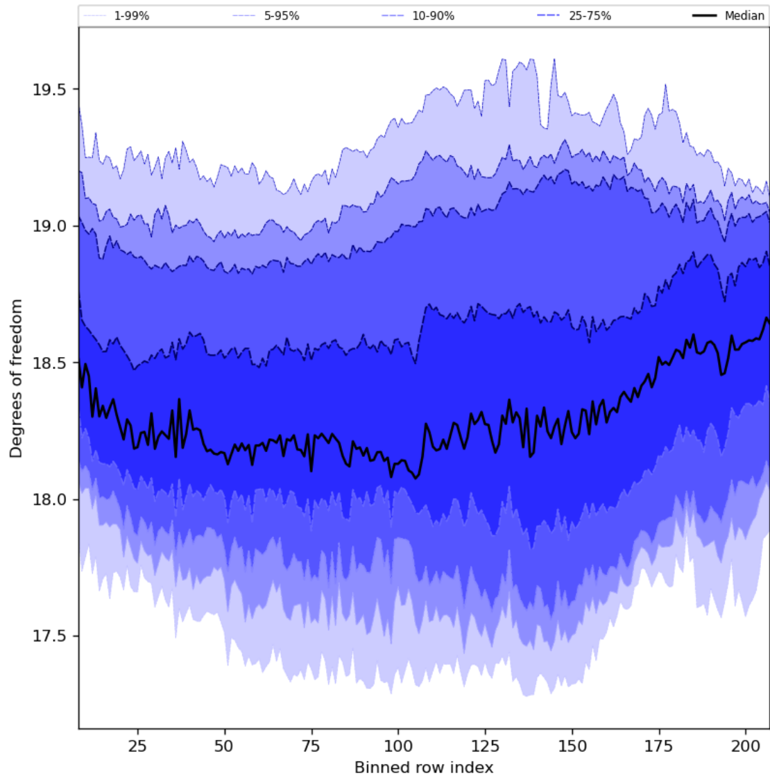
Figure 41: Along track statistics of “Degrees of freedom” for 2024-04-22 to 2024-04-24
