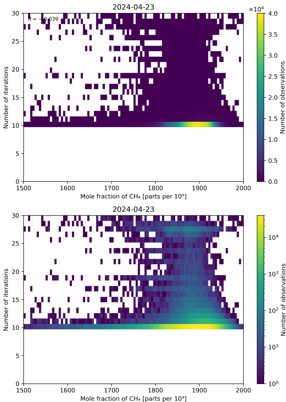
Figure 76: Scatter density plot of “Mole fraction of CH 4 ” against “Number of iterations” for 2024-04-22 to 2024-04-24.
