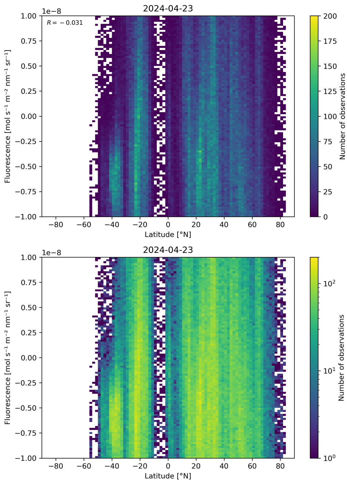
Figure 56: Scatter density plot of “Latitude” against “Fluorescence” for 2024-04-22 to 2024-04-24.
