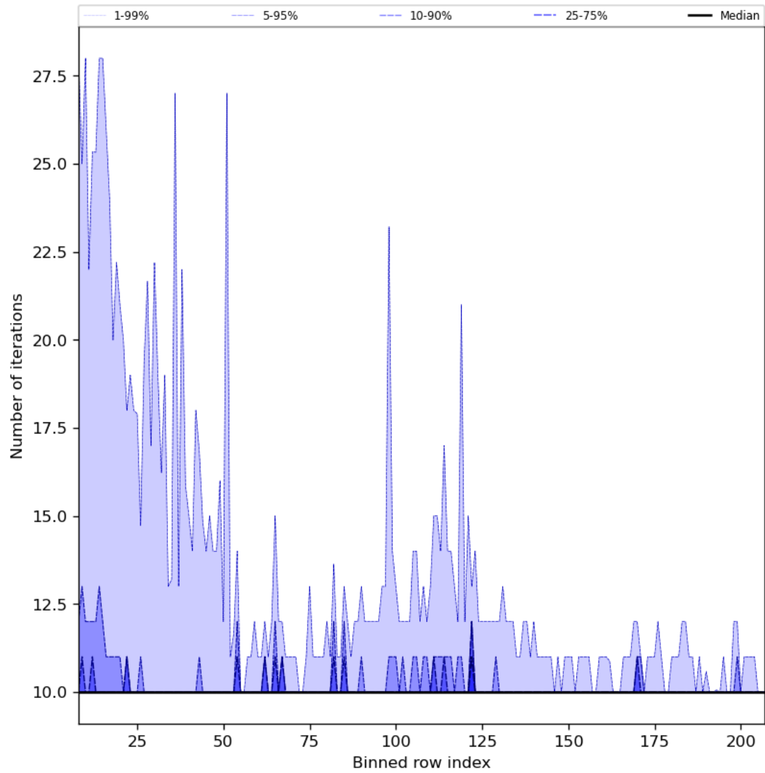
Figure 42: Along track statistics of “Number of iterations” for 2024-04-22 to 2024-04-24
