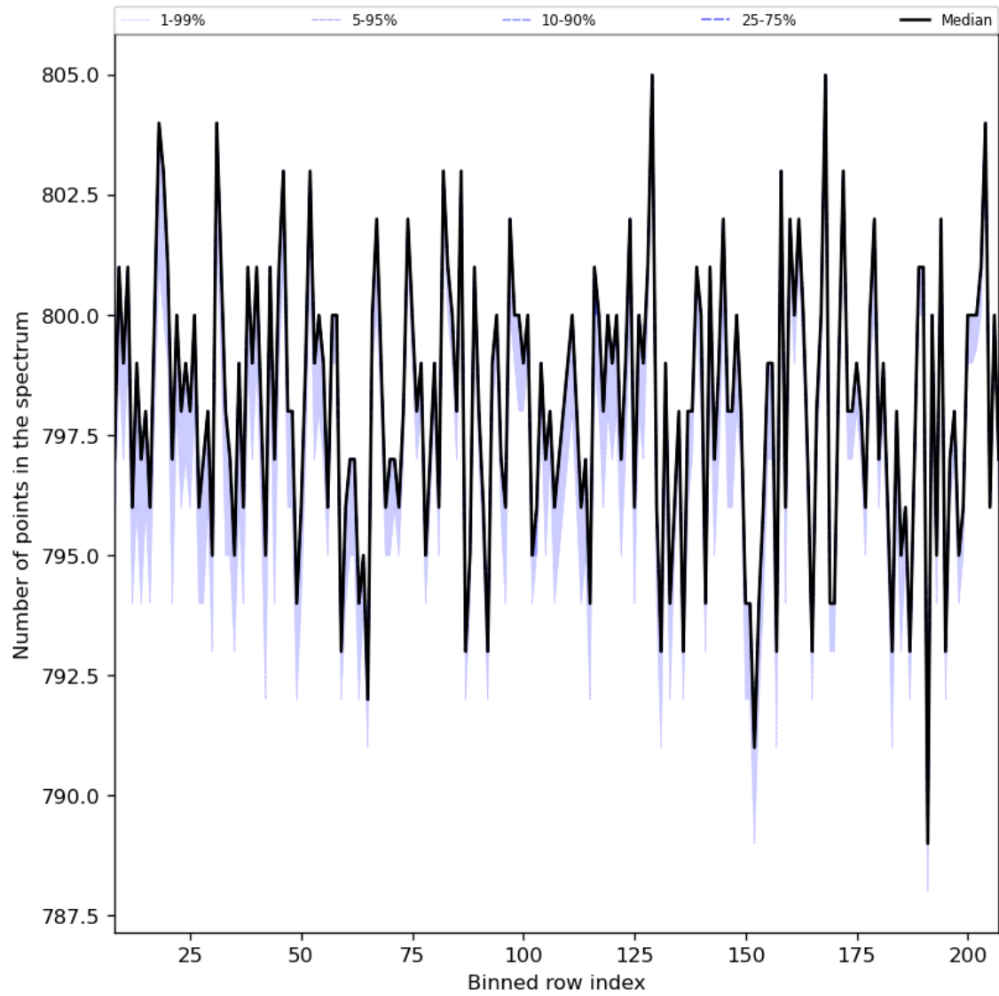
Figure 37: Along track statistics of “Number of points in the spectrum” for 2024-04-22 to 2024-04-24
