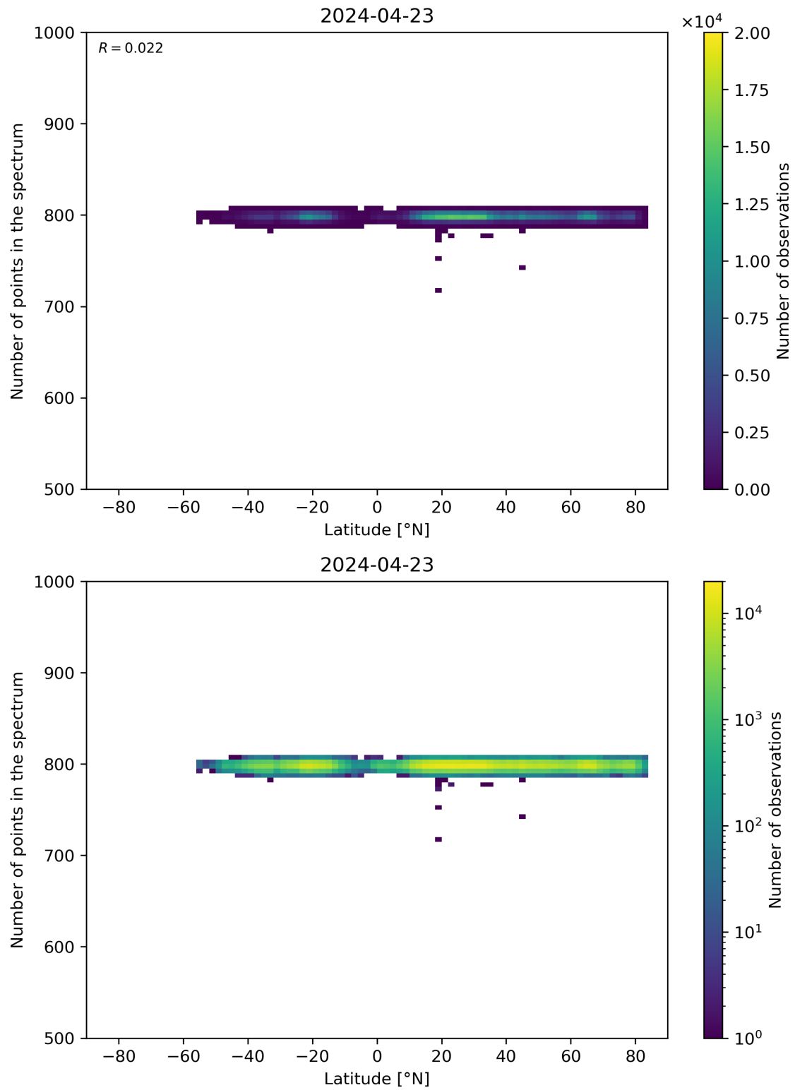
Figure 61: Scatter density plot of “Latitude” against “Number of points in the spectrum” for 2024-04-22 to 2024-04-24.
