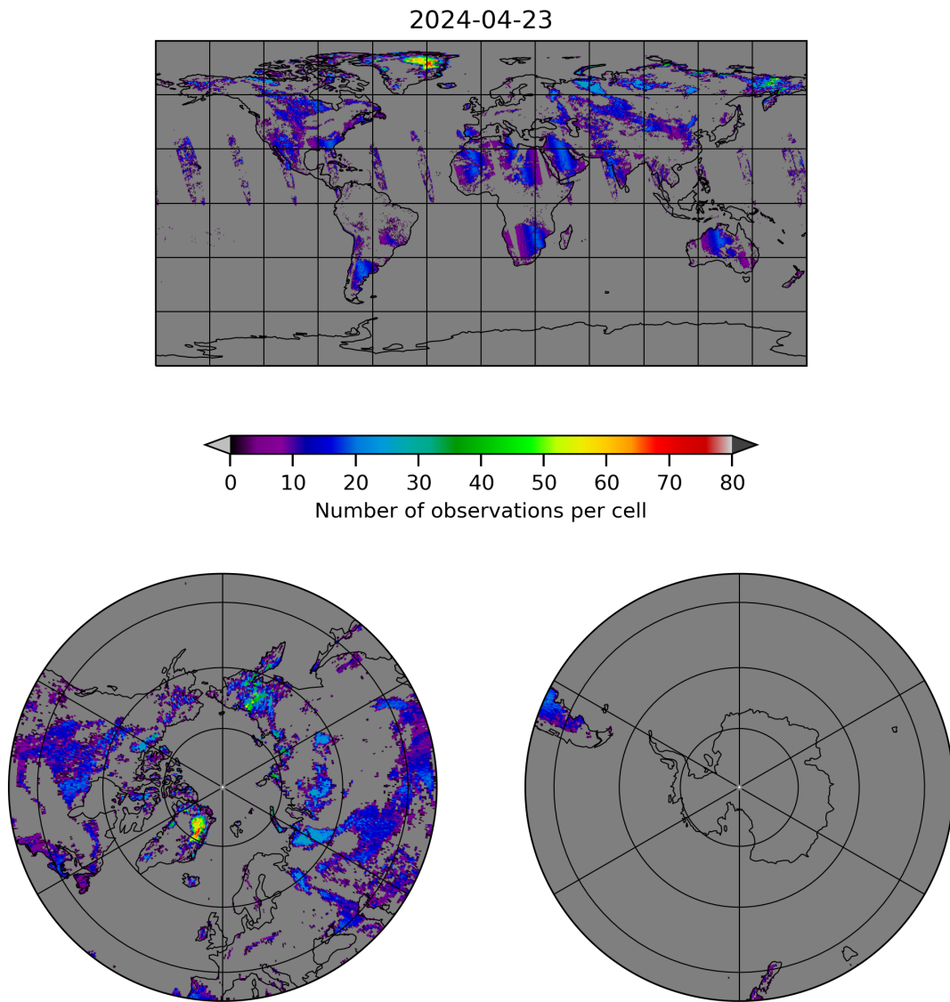
Figure 10: Map of the number of observations for 2024-04-22 to 2024-04-24
