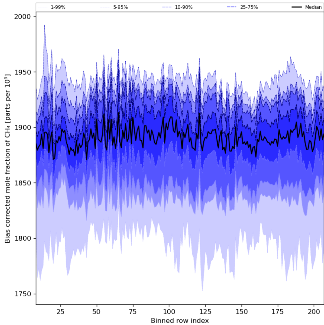
Figure 36: Along track statistics of “Bias corrected mole fraction of CH 4 ” for 2024-04-22 to 2024-04-24
