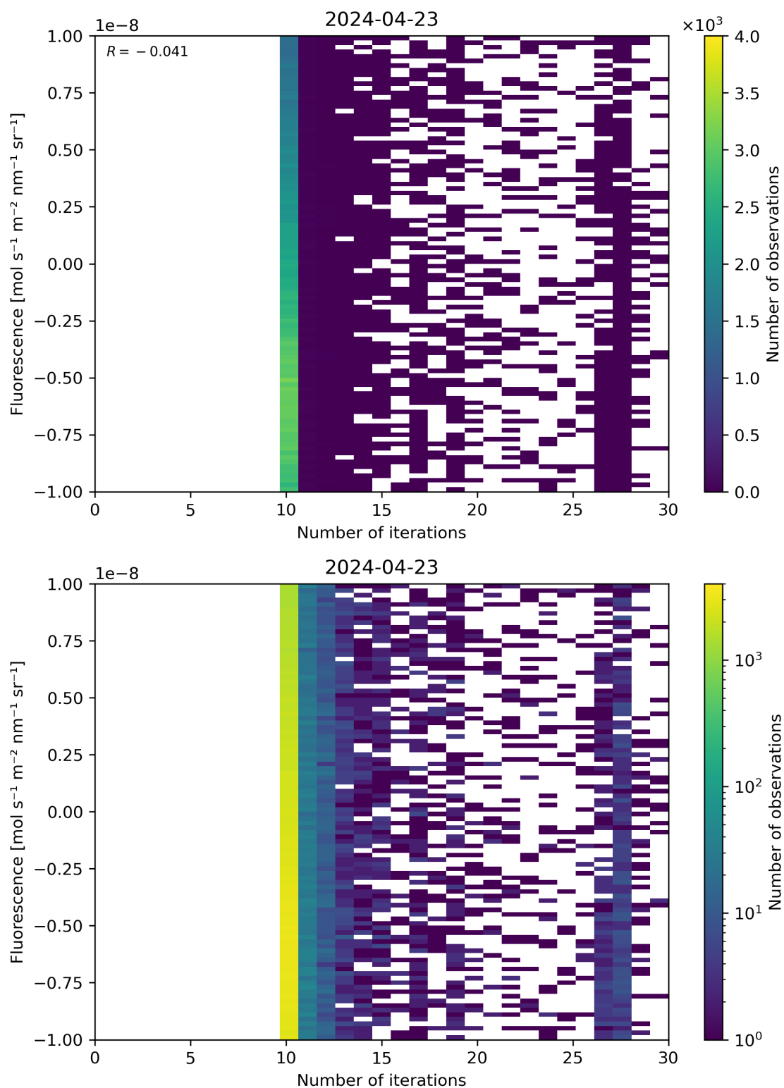
Figure 87: Scatter density plot of “Number of iterations” against “Fluorescence” for 2024-04-22 to 2024-04-24.
