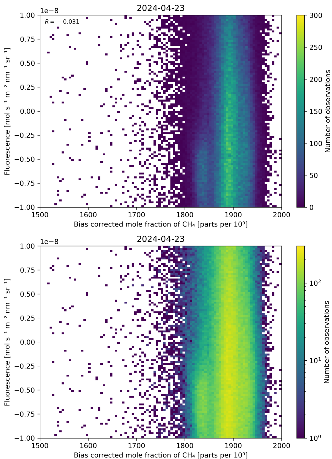
Figure 66: Scatter density plot of “Bias corrected mole fraction of \text{CH}_4 ” against “Fluorescence” for 2024-04-22 to 2024-04-24.
