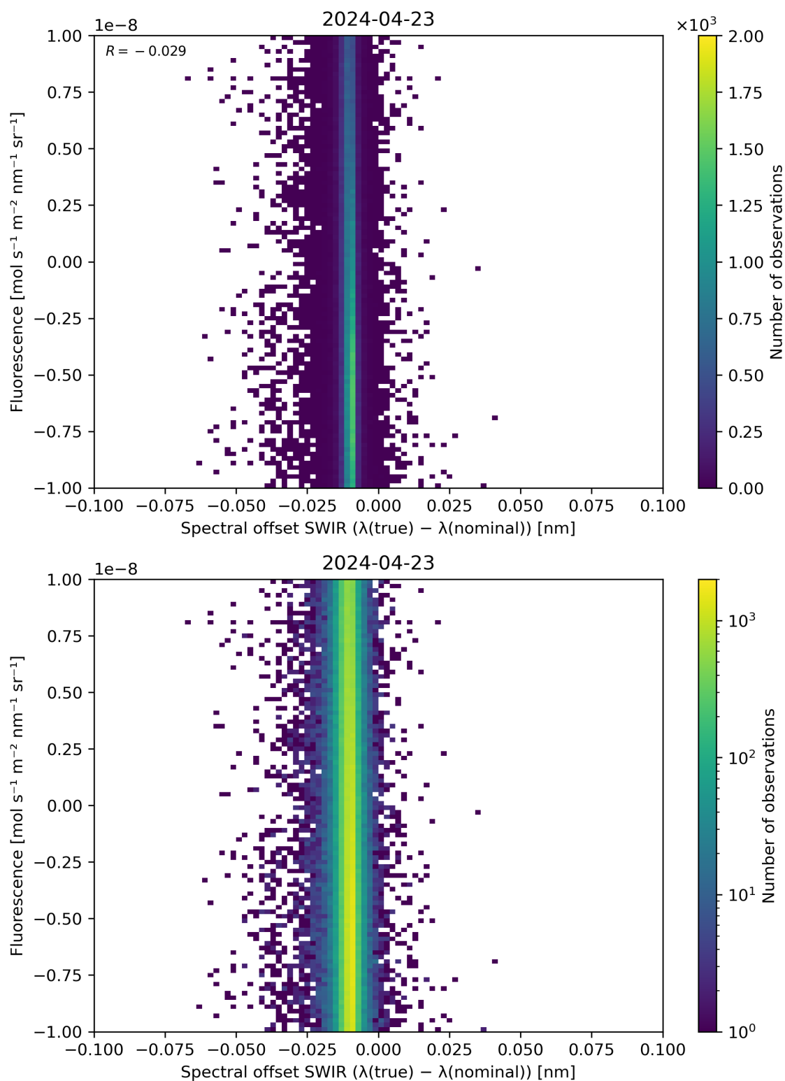
Figure 120: Scatter density plot of “Spectral offset SWIR ( \lambda(\text{true}) - \lambda(\text{nominal}) )” against “Fluorescence” for 2024-04-22 to 2024-04-24.
