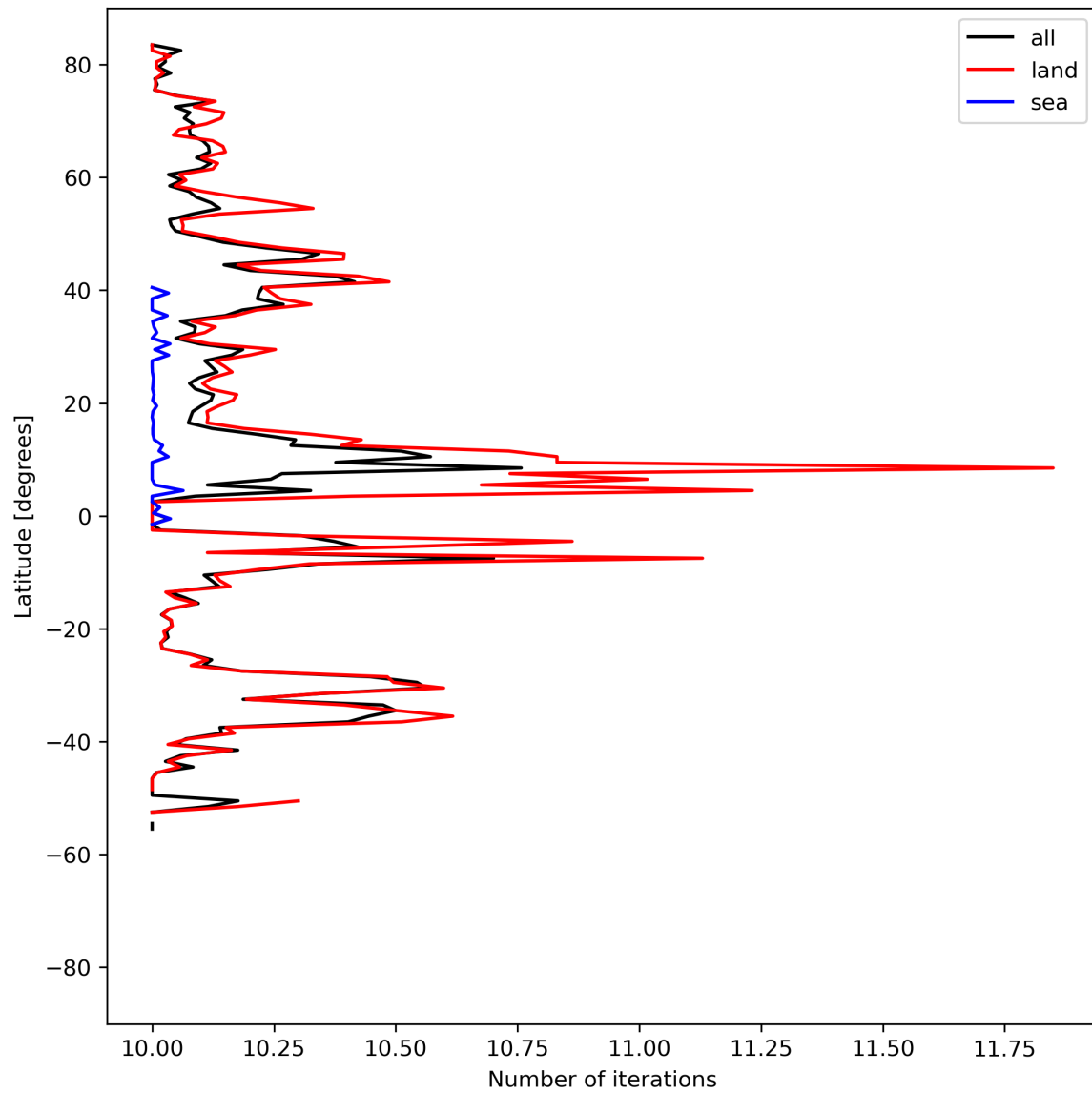
Figure 20: Zonal average of “Number of iterations” for 2024-04-22 to 2024-04-24.
