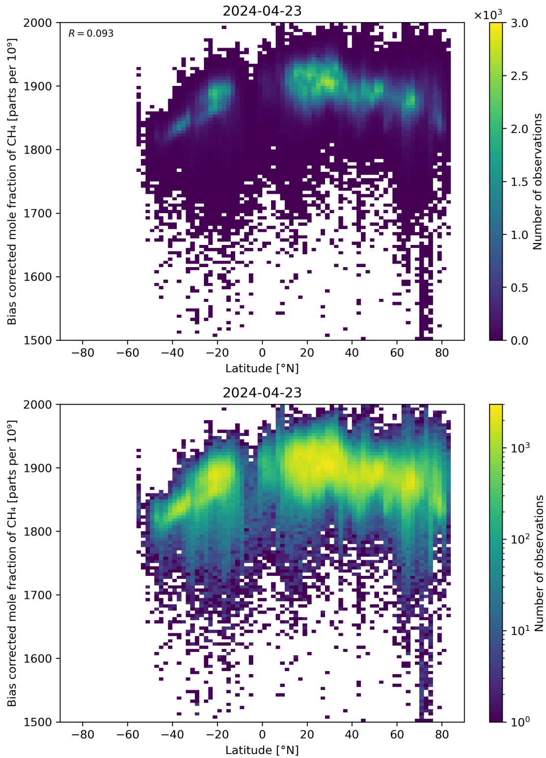
Figure 58: Scatter density plot of “Latitude” against “Bias corrected mole fraction of \text{CH}_4 ” for 2024-04-22 to 2024-04-24.
