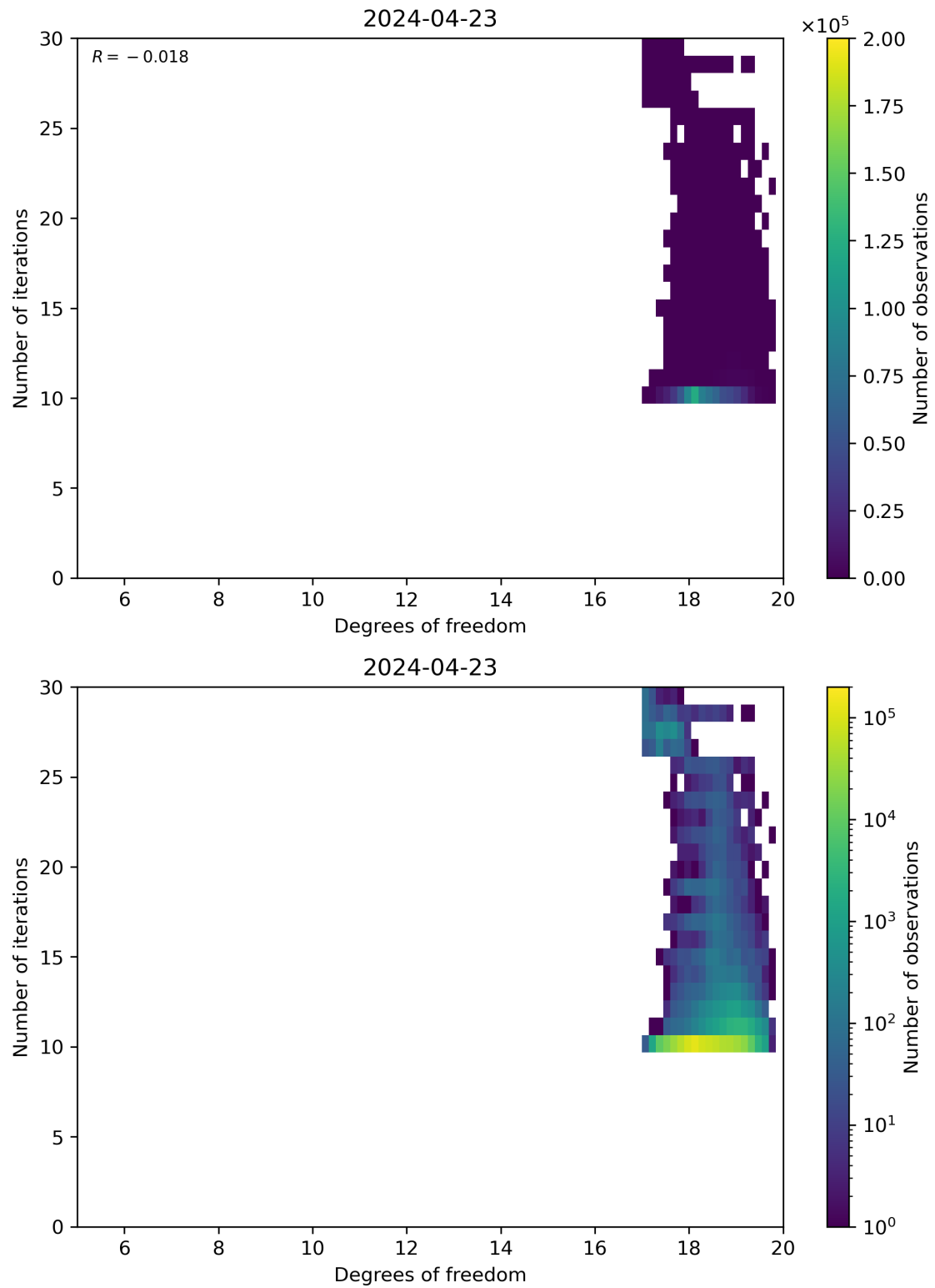
Figure 52: Scatter density plot of “Degrees of freedom” against “Number of iterations” for 2024-04-22 to 2024-04-24.
