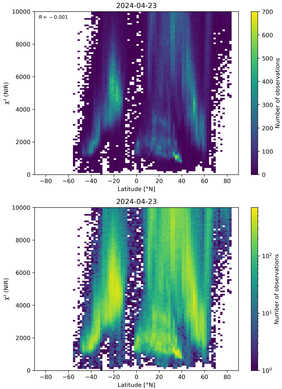
Figure 53: Scatter density plot of “Latitude” against “ \chi^2 (NIR)” for 2024-04-22 to 2024-04-24.
