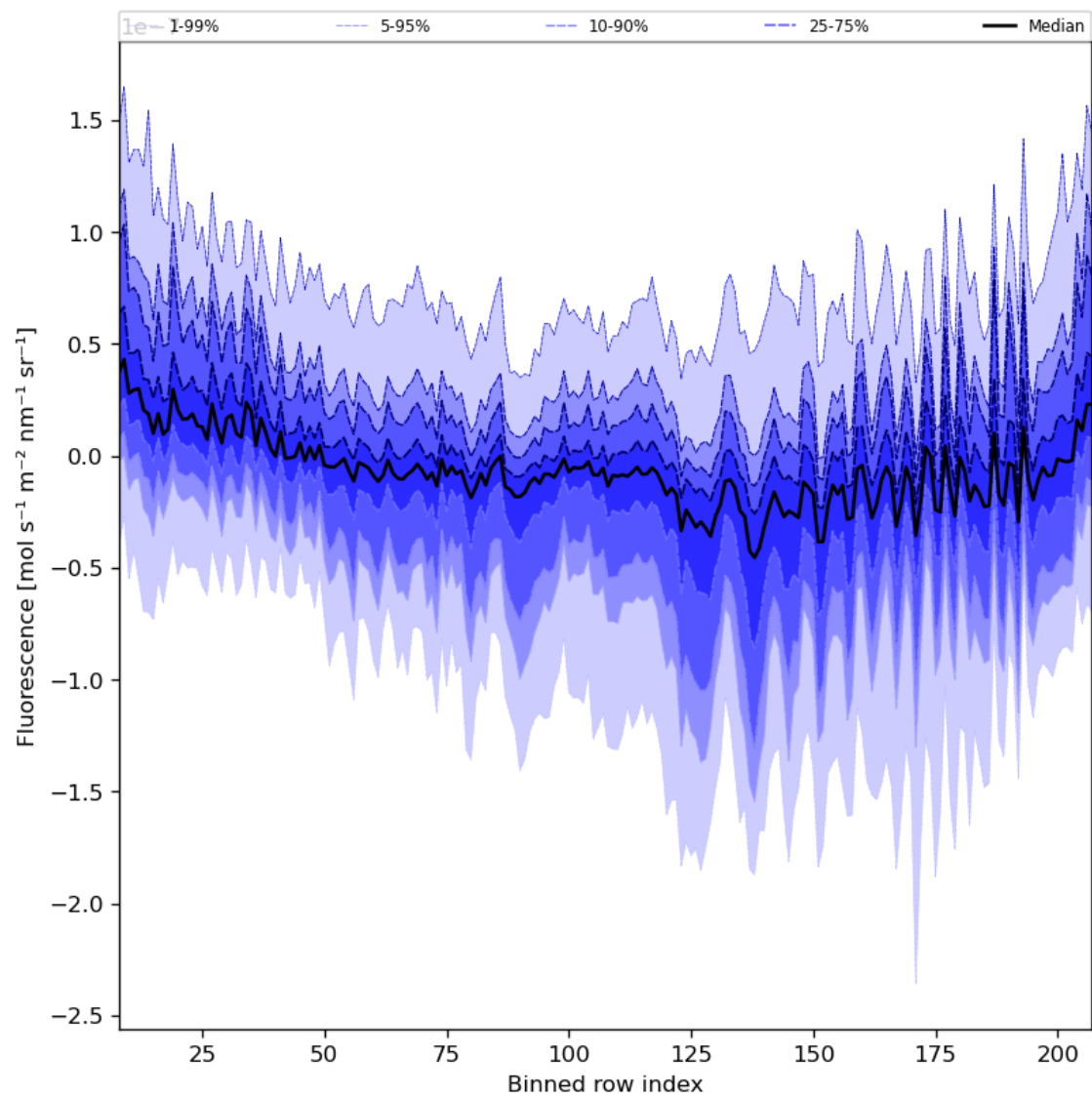
Figure 43: Along track statistics of “Fluorescence” for 2024-04-22 to 2024-04-24
