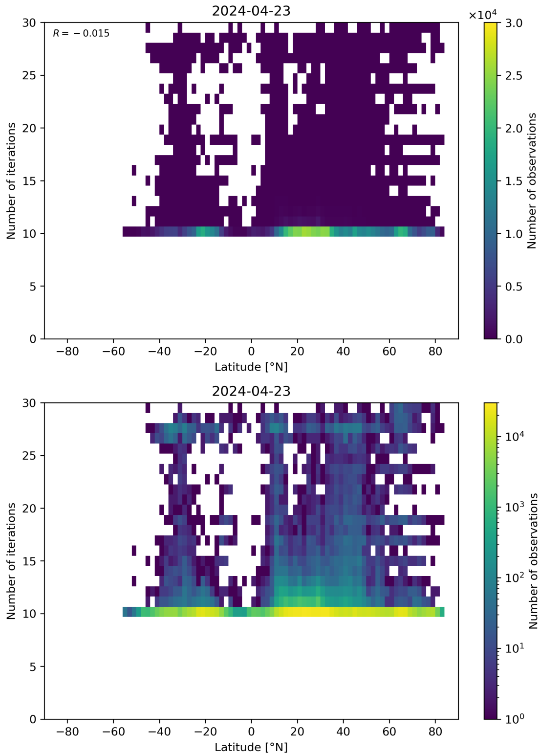
Figure 60: Scatter density plot of “Latitude” against “Number of iterations” for 2024-04-22 to 2024-04-24.
