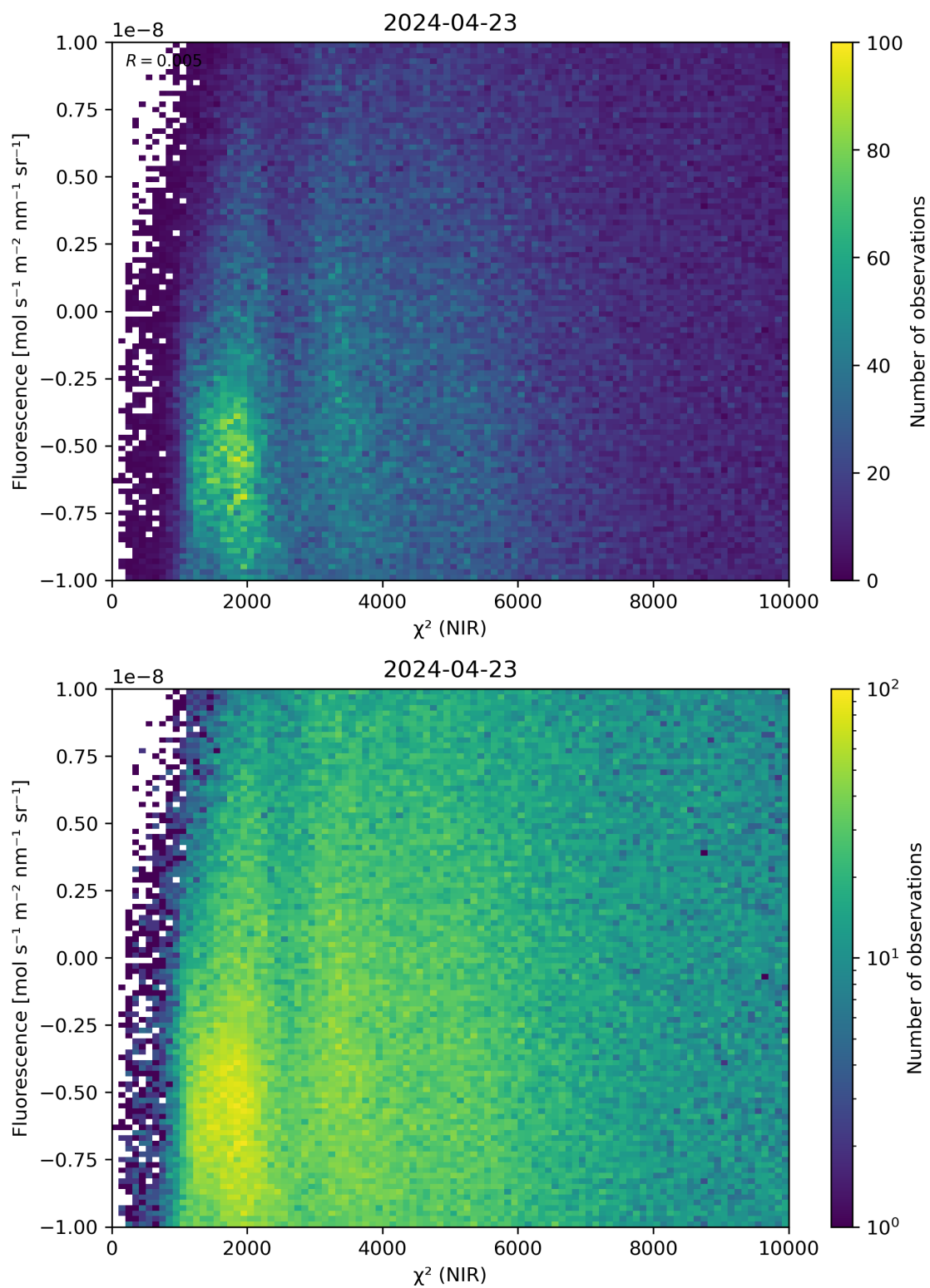
Figure 45: Scatter density plot of “ \chi^2 (NIR)” against “Fluorescence” for 2024-04-22 to 2024-04-24.
