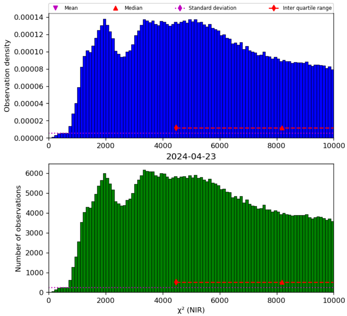
Figure 29: Histogram of “ \chi^2 (NIR)” for 2024-04-22 to 2024-04-24
