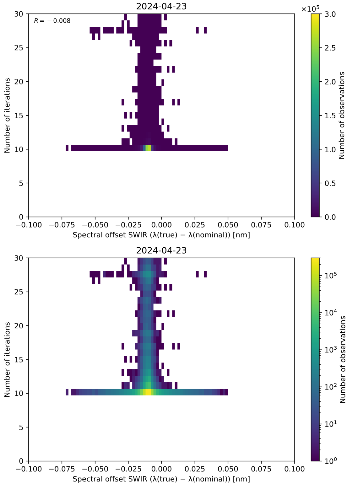
Figure 121: Scatter density plot of “Spectral offset SWIR ( \lambda(\text{true}) - \lambda(\text{nominal}) )” against “Number of iterations” for 2024-04-22 to 2024-04-24.
