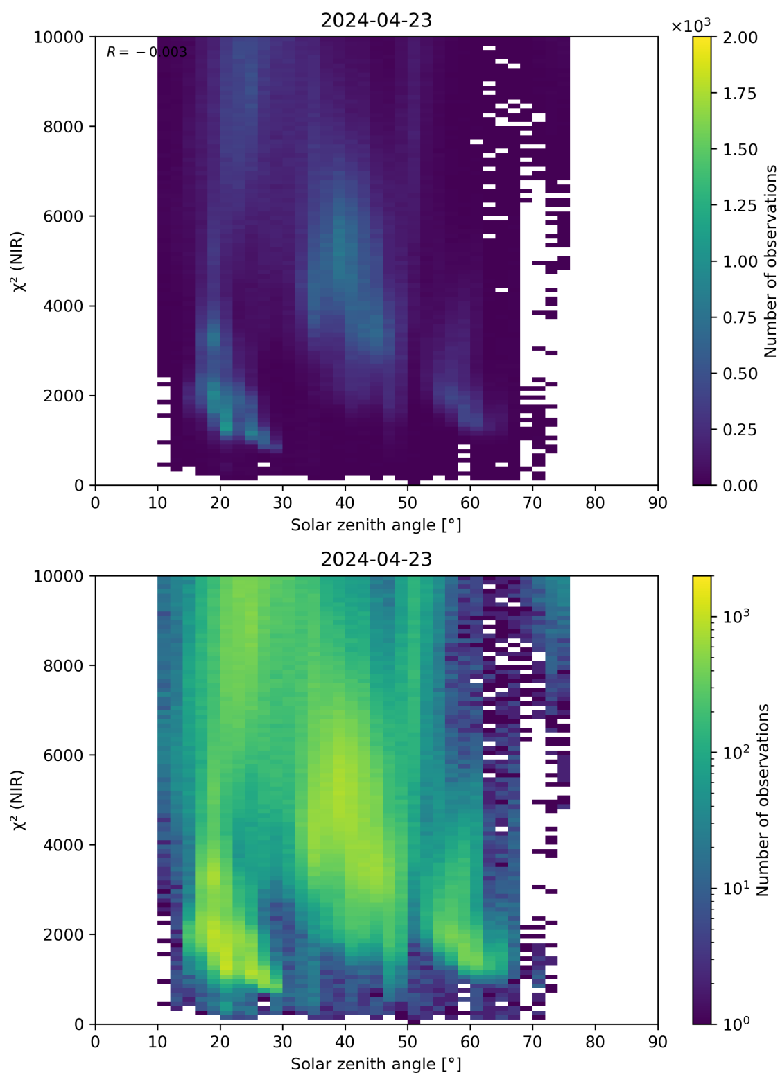
Figure 94: Scatter density plot of “Solar zenith angle” against “ \chi^2 (NIR)” for 2024-04-22 to 2024-04-24.
