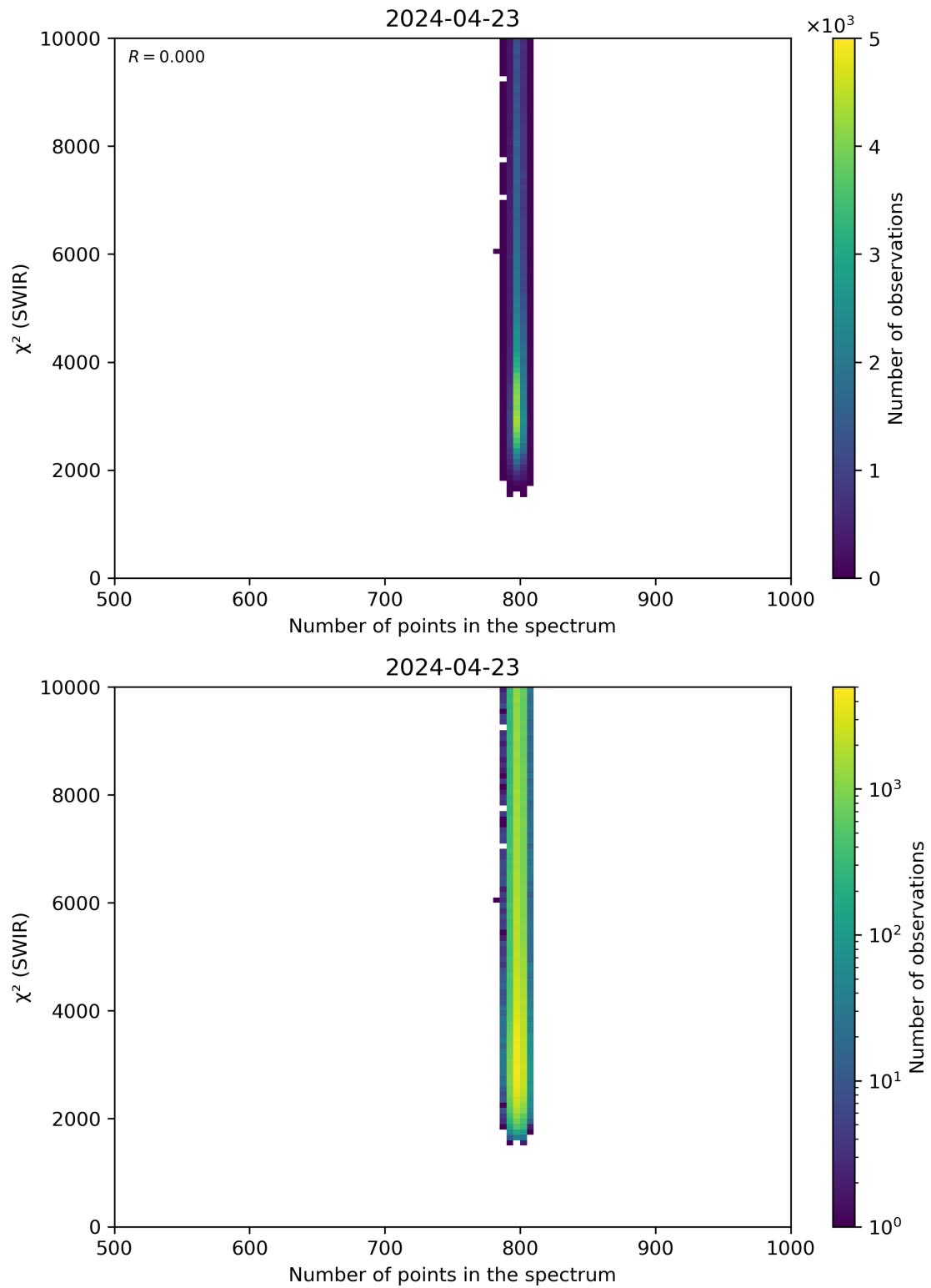
Figure 89: Scatter density plot of “Number of points in the spectrum” against “ \chi^2 (SWIR)” for 2024-04-22 to 2024-04-24.
