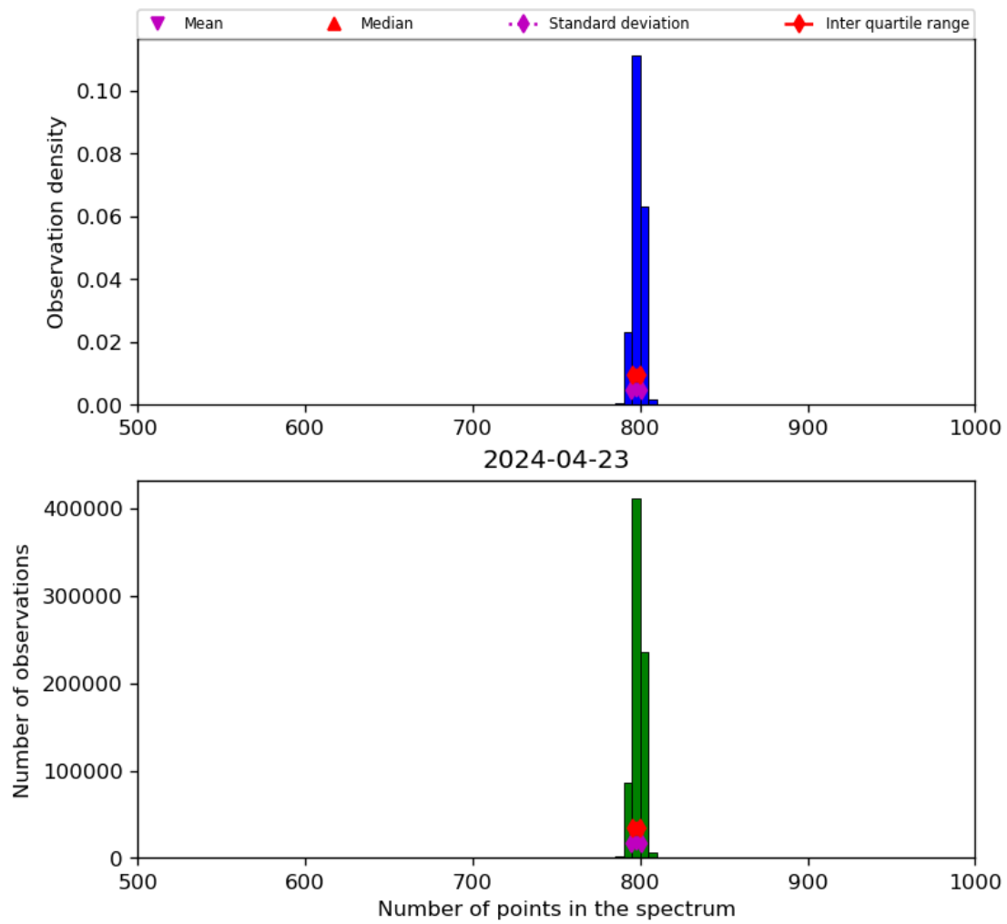
Figure 26: Histogram of “Number of points in the spectrum” for 2024-04-22 to 2024-04-24
