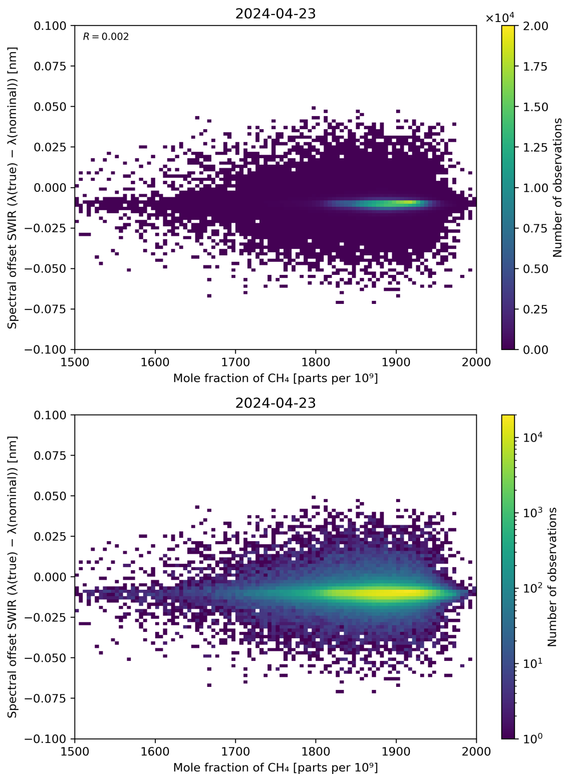
Figure 86: Scatter density plot of “Mole fraction of CH 4 ” against “Spectral offset SWIR ( \lambda(\text{true}) - \lambda(\text{nominal}) )” for 2024-04-22 to 2024-04-24.
