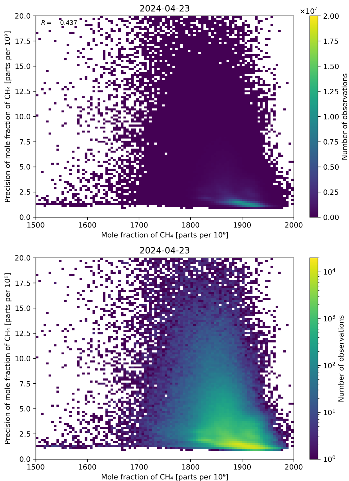
Figure 75: Scatter density plot of “Mole fraction of CH 4 ” against “Precision of mole fraction of CH 4 ” for 2024-04-22 to 2024-04-24.
