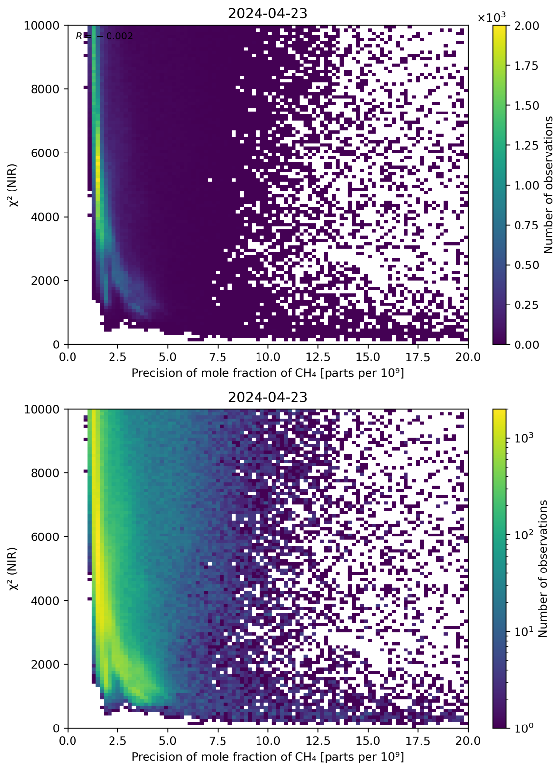
Figure 78: Scatter density plot of “Precision of mole fraction of CH 4 ” against “ \chi^2 (NIR)” for 2024-04-22 to 2024-04-24.
