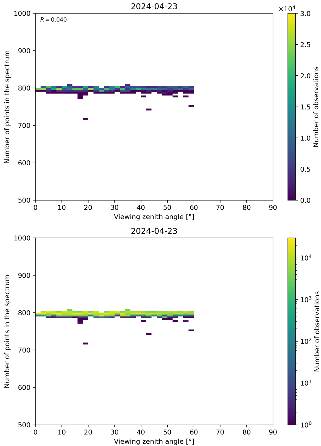
Figure 114: Scatter density plot of “Viewing zenith angle” against “Number of points in the spectrum” for 2024-04-22 to 2024-04-24.
