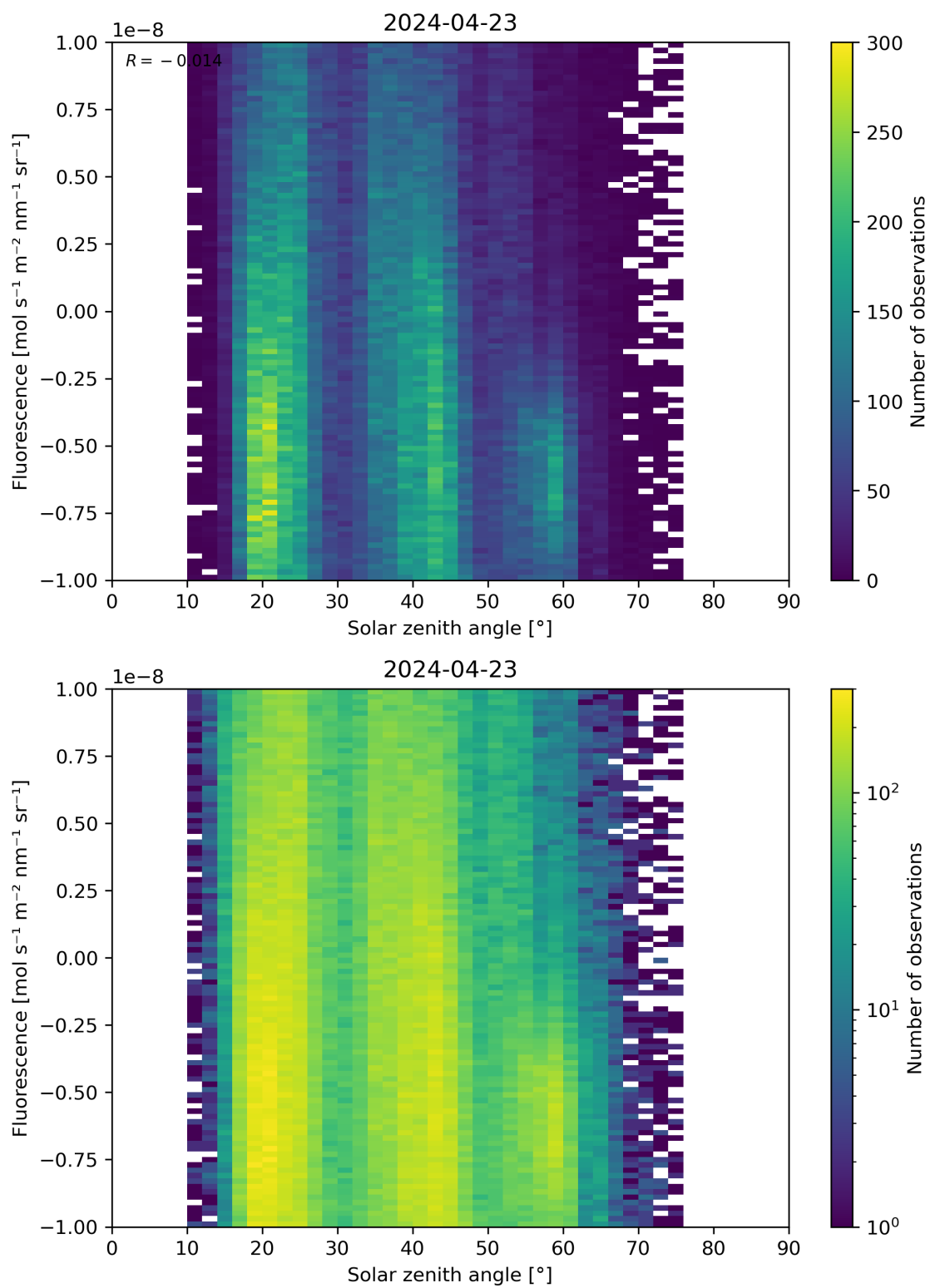
Figure 97: Scatter density plot of “Solar zenith angle” against “Fluorescence” for 2024-04-22 to 2024-04-24.
