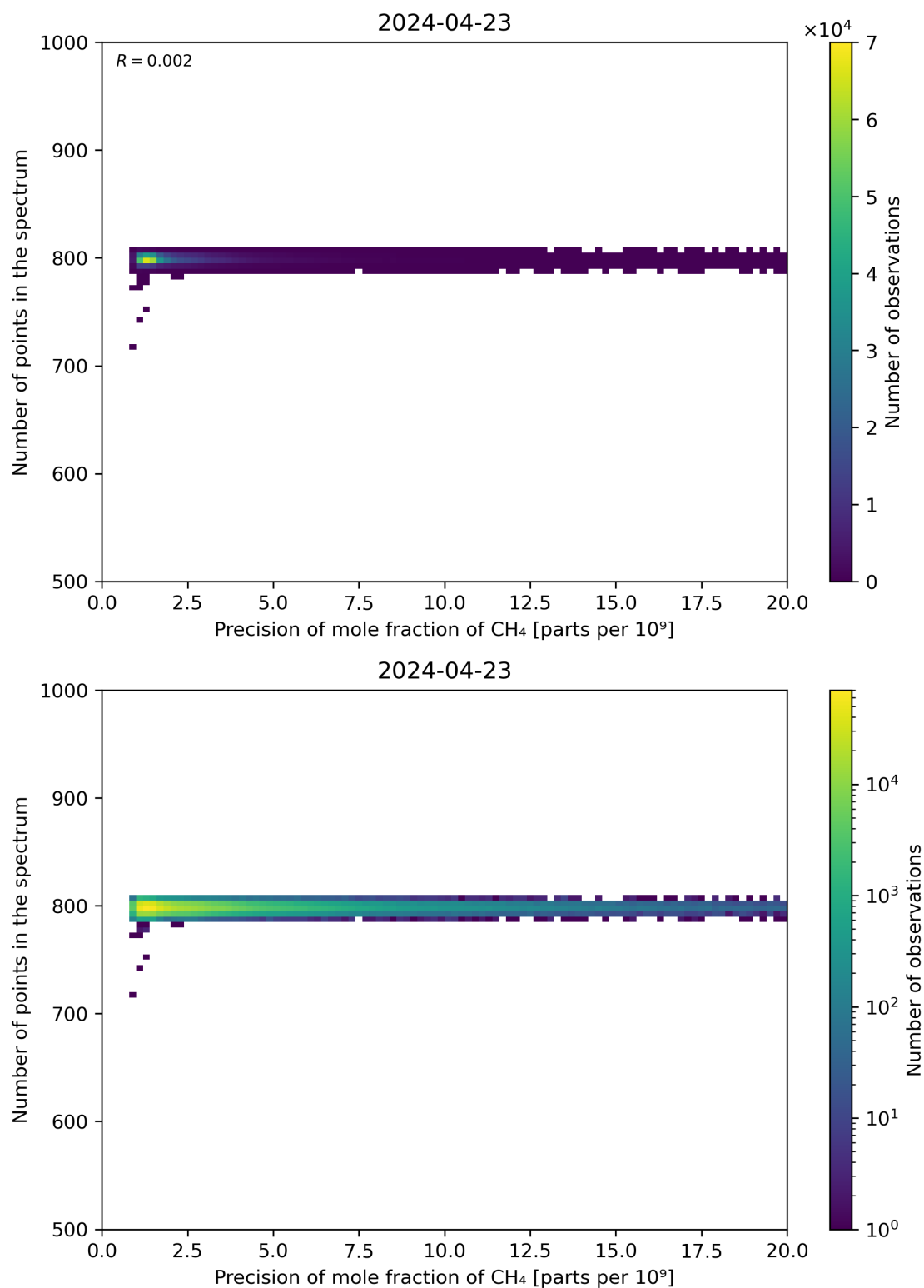
Figure 84: Scatter density plot of “Precision of mole fraction of CH 4 ” against “Number of points in the spectrum” for 2024-04-22 to 2024-04-24.
