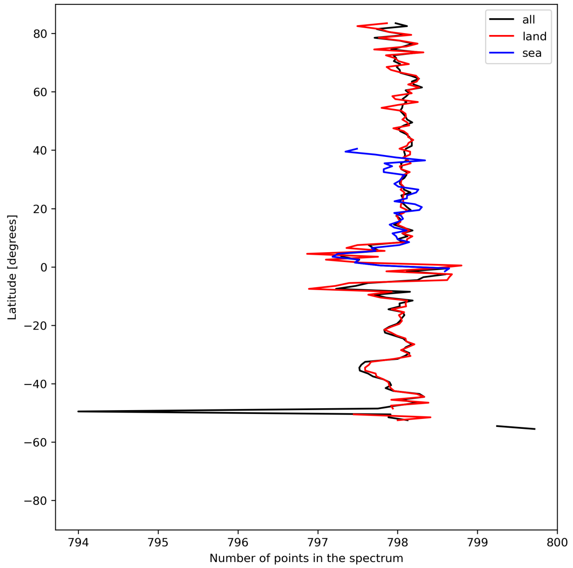
Figure 15: Zonal average of “Number of points in the spectrum” for 2024-04-22 to 2024-04-24.
