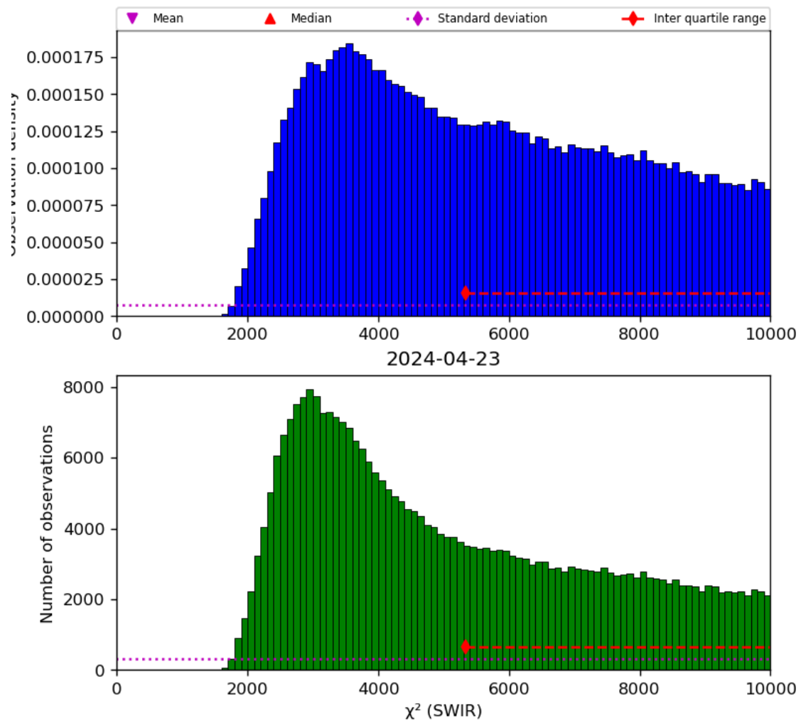
Figure 28: Histogram of “ \chi^2 (SWIR)” for 2024-04-22 to 2024-04-24
