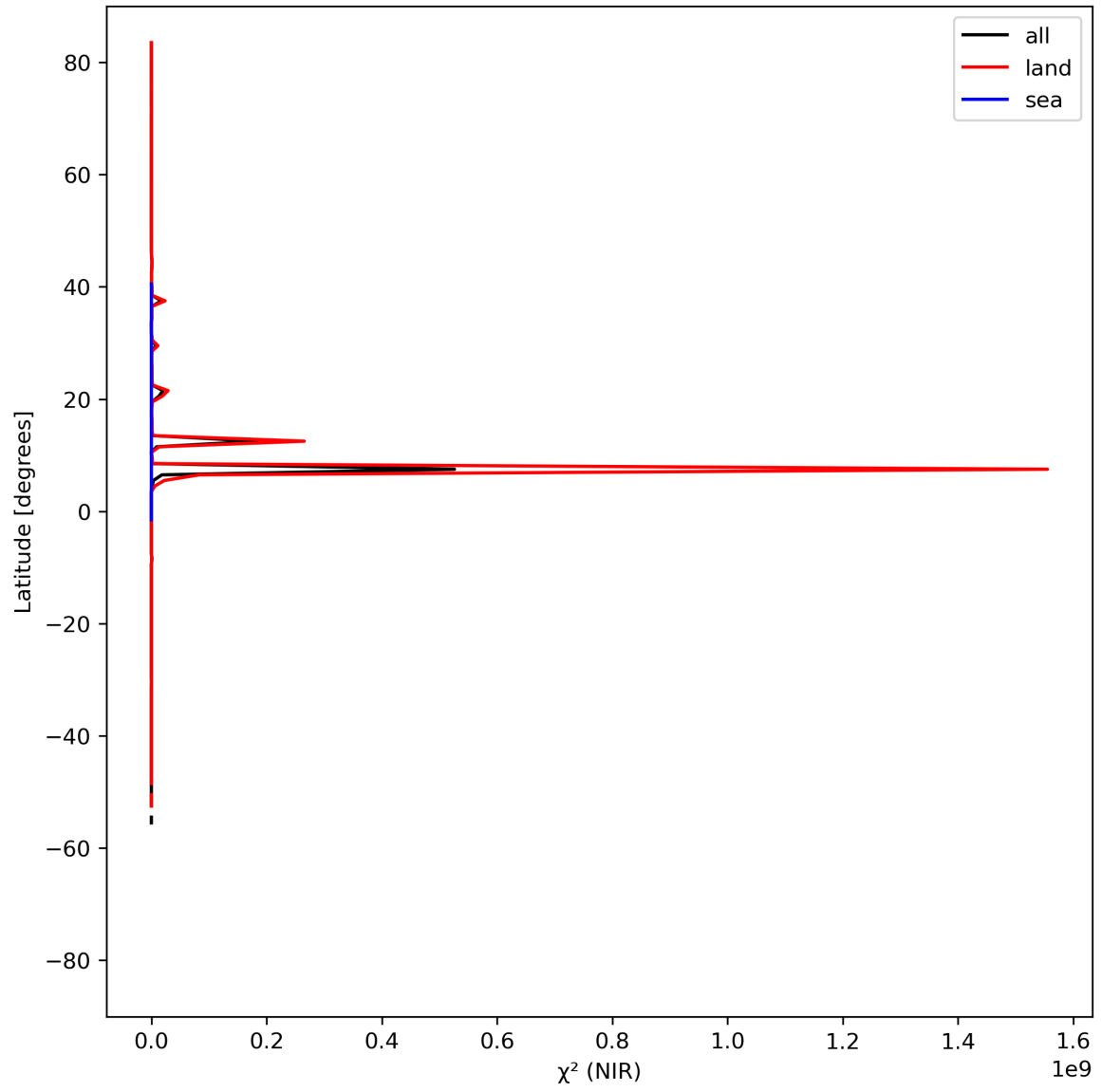
Figure 18: Zonal average of “ \chi^2 (NIR)” for 2024-04-22 to 2024-04-24.
