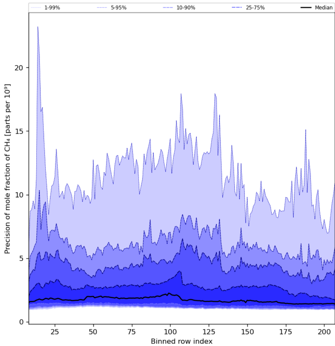
Figure 35: Along track statistics of “Precision of mole fraction of CH 4 ” for 2024-04-22 to 2024-04-24
