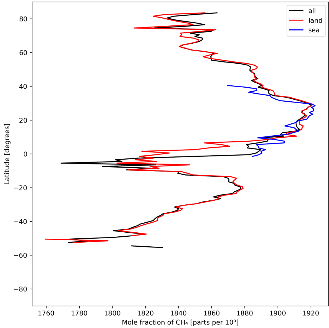
Figure 12: Zonal average of “Mole fraction of \text{CH}_4 ” for 2024-04-22 to 2024-04-24.
