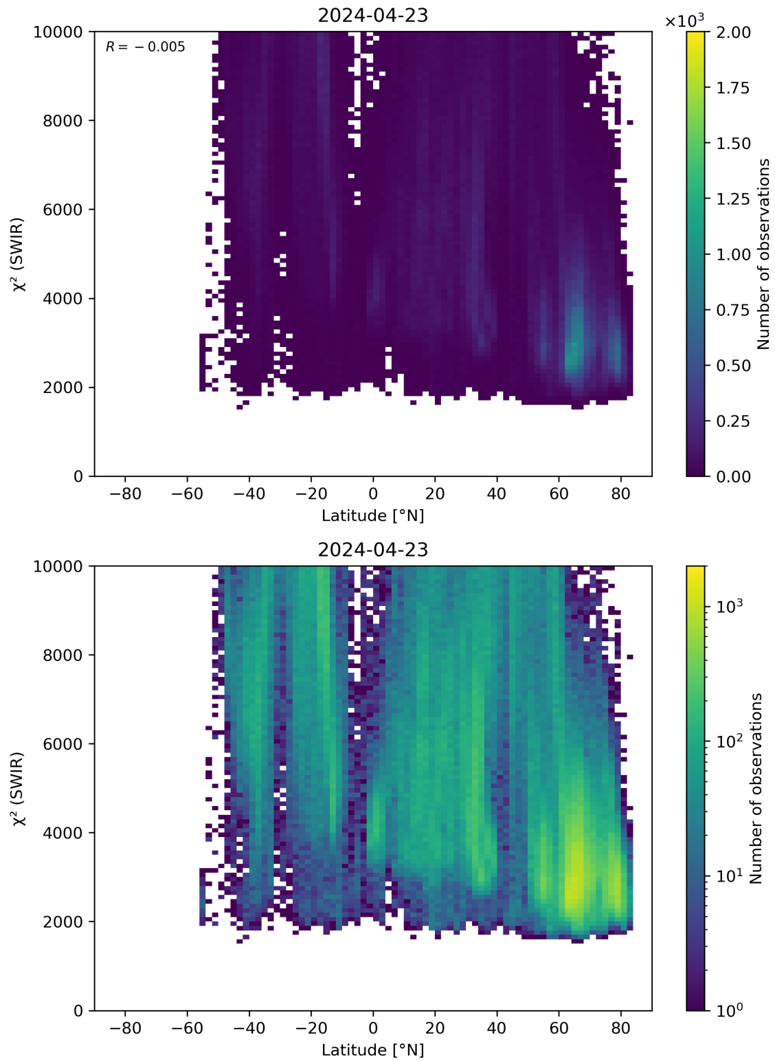
Figure 54: Scatter density plot of “Latitude” against “ \chi^2 (SWIR)” for 2024-04-22 to 2024-04-24.
