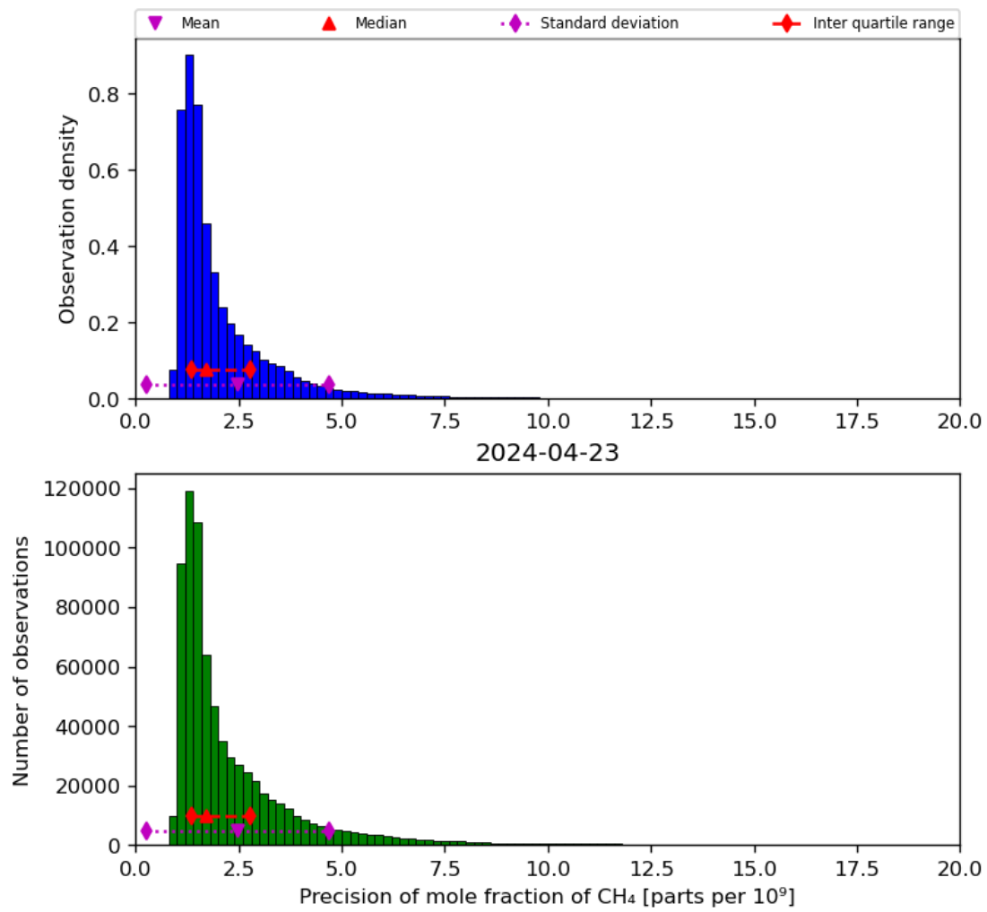
Figure 24: Histogram of “Precision of mole fraction of CH 4 ” for 2024-04-22 to 2024-04-24
