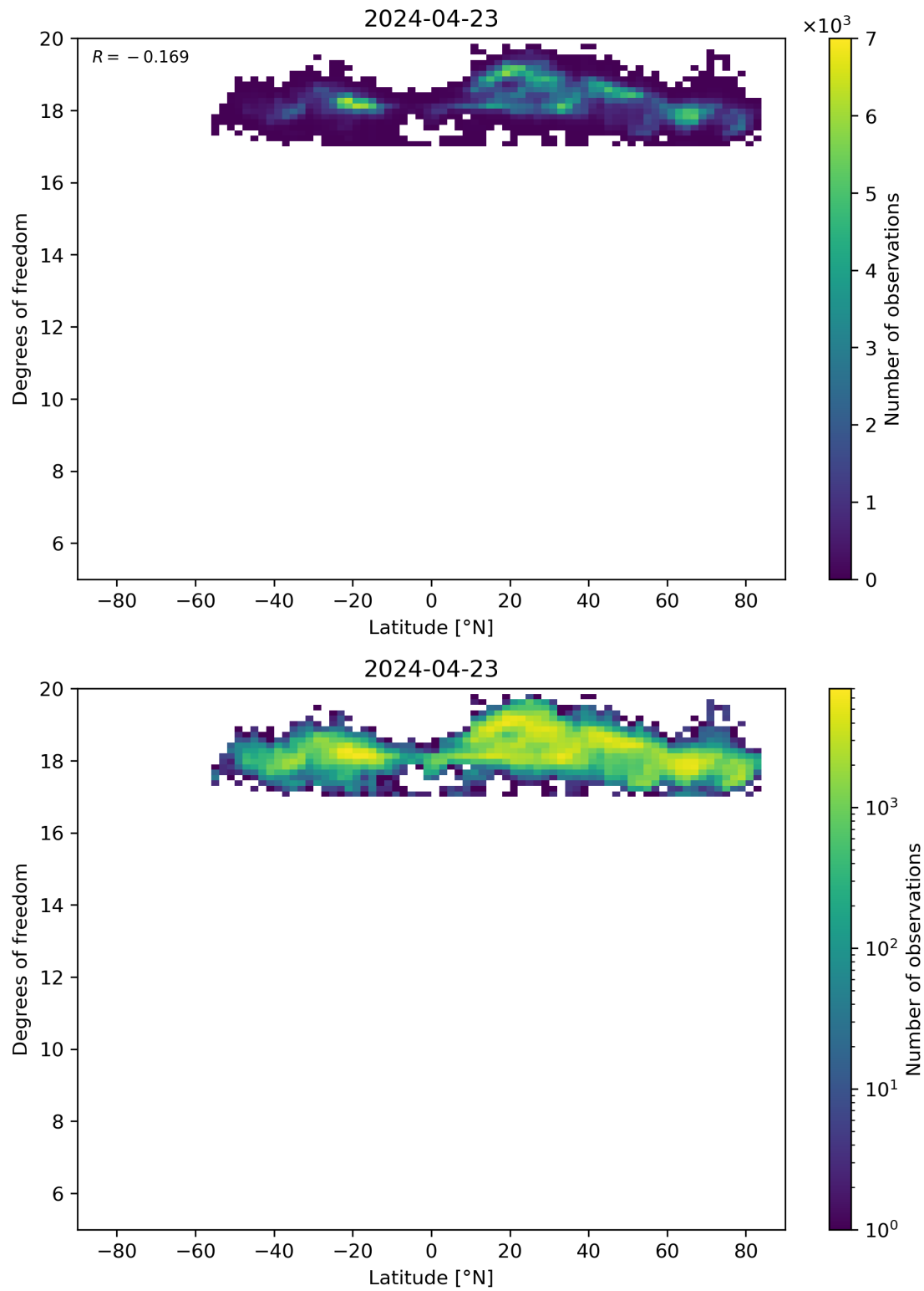
Figure 55: Scatter density plot of “Latitude” against “Degrees of freedom” for 2024-04-22 to 2024-04-24.
