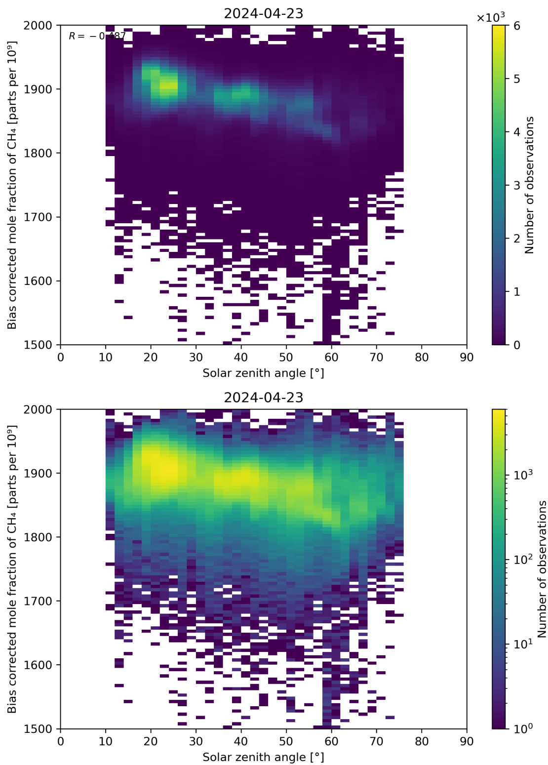
Figure 100: Scatter density plot of “Solar zenith angle” against “Bias corrected mole fraction of CH 4 ” for 2024-04-22 to 2024-04-24.
