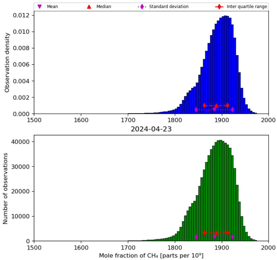
Figure 23: Histogram of “Mole fraction of CH 4 ” for 2024-04-22 to 2024-04-24
