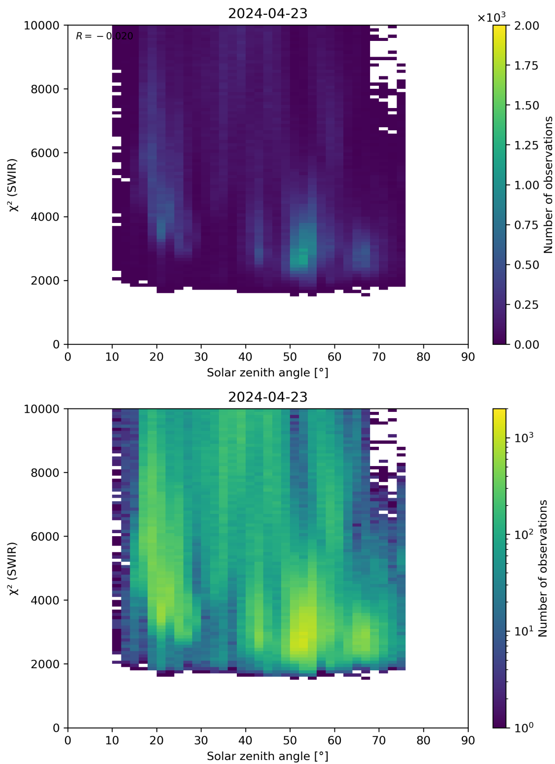
Figure 95: Scatter density plot of “Solar zenith angle” against “ \chi^2 (SWIR)” for 2024-04-22 to 2024-04-24.
