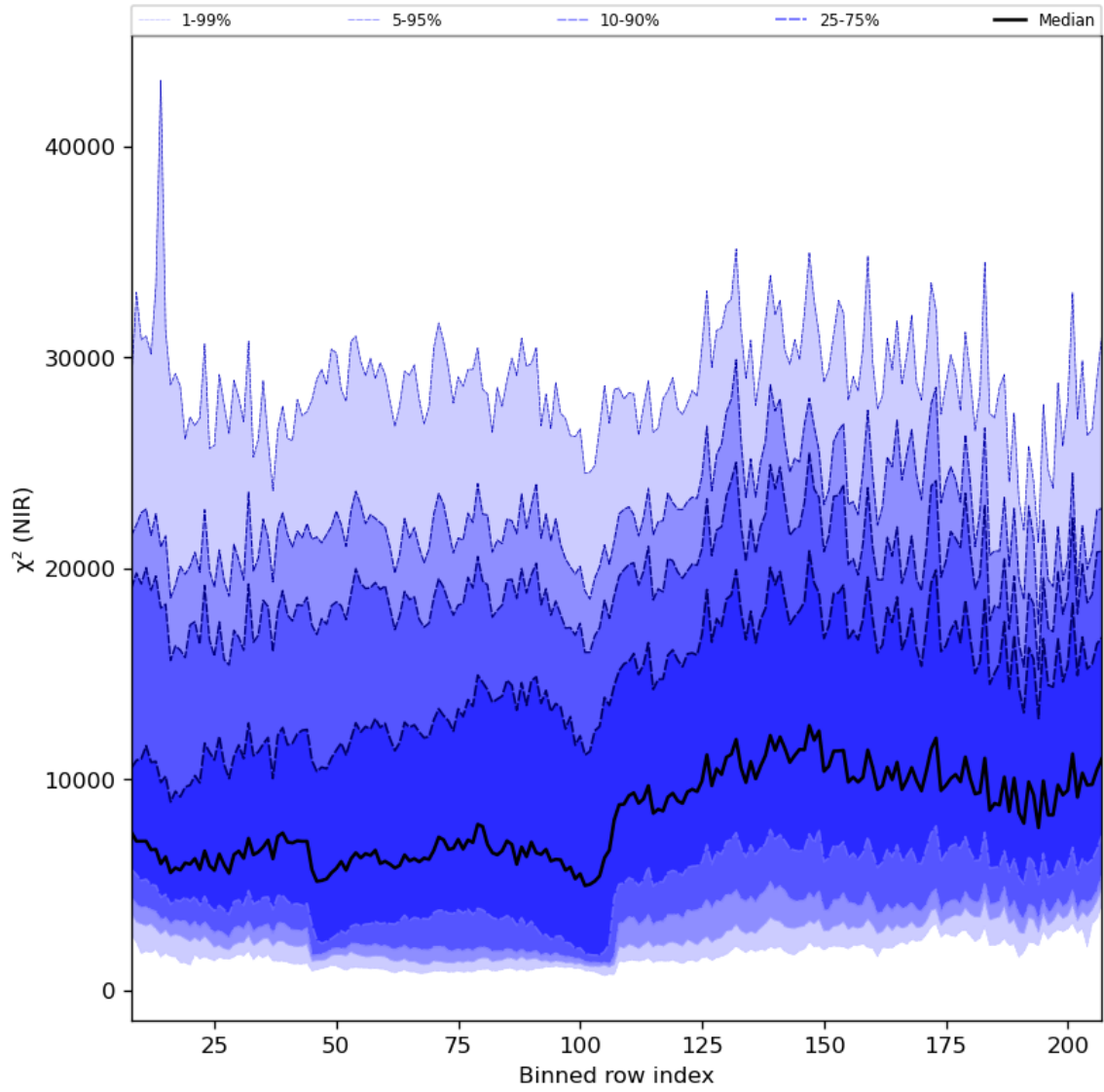
Figure 40: Along track statistics of “ \chi^2 (NIR)” for 2024-04-22 to 2024-04-24
