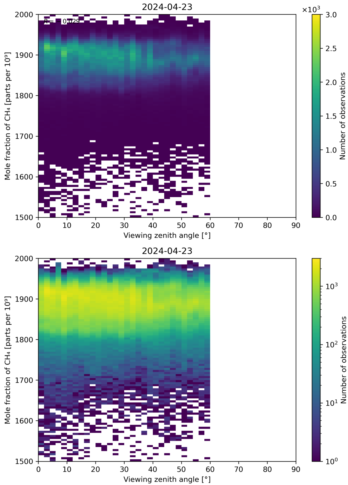
Figure 110: Scatter density plot of “Viewing zenith angle” against “Mole fraction of CH 4 ” for 2024-04-22 to 2024-04-24.
