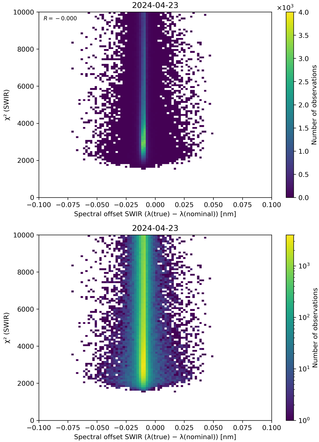
Figure 118: Scatter density plot of “Spectral offset SWIR ( \lambda(\text{true}) - \lambda(\text{nominal}) )” against “ \chi^2 (SWIR)” for 2024-04-22 to 2024-04-24.
