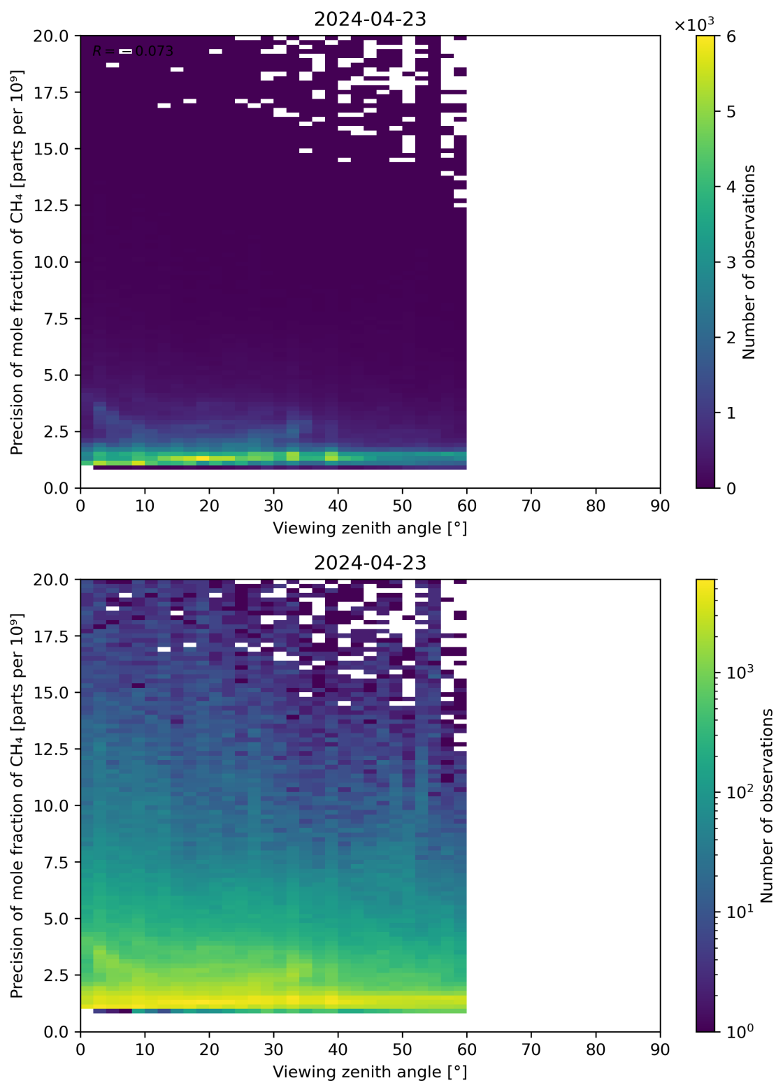
Figure 112: Scatter density plot of “Viewing zenith angle” against “Precision of mole fraction of CH 4 ” for 2024-04-22 to 2024-04-24.
