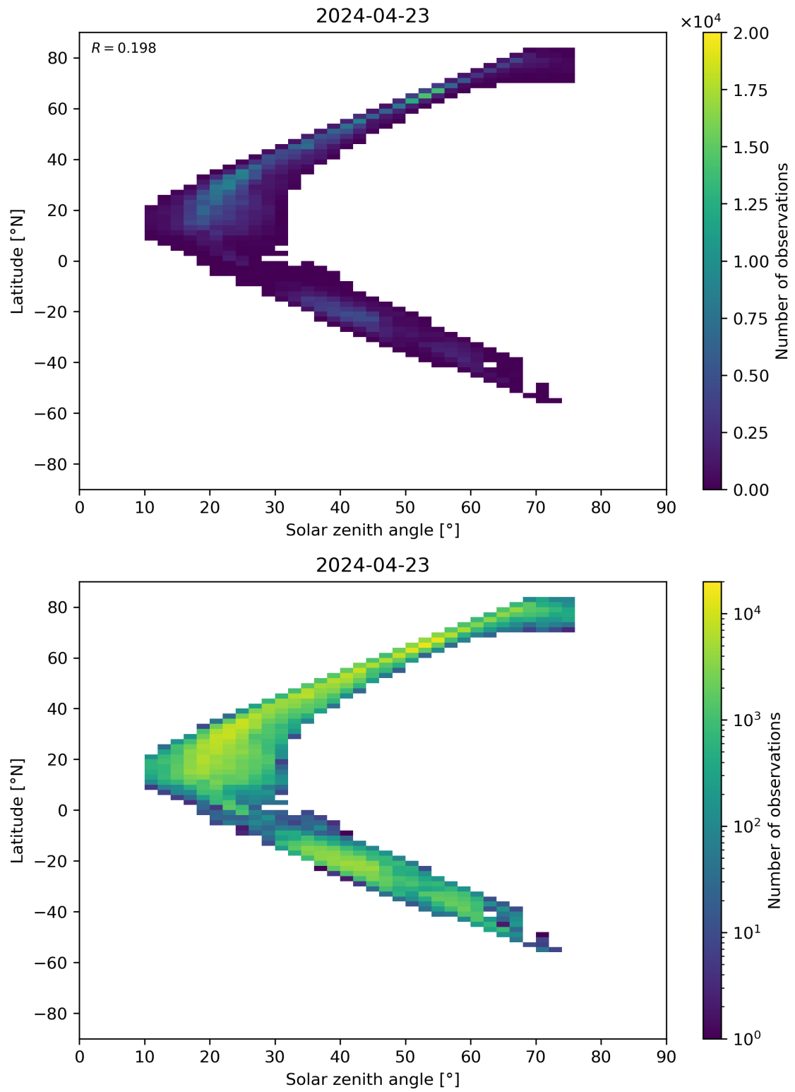
Figure 98: Scatter density plot of “Solar zenith angle” against “Latitude” for 2024-04-22 to 2024-04-24.
