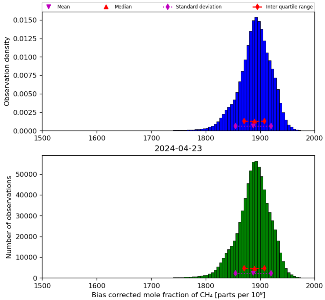
Figure 25: Histogram of “Bias corrected mole fraction of CH 4 ” for 2024-04-22 to 2024-04-24
