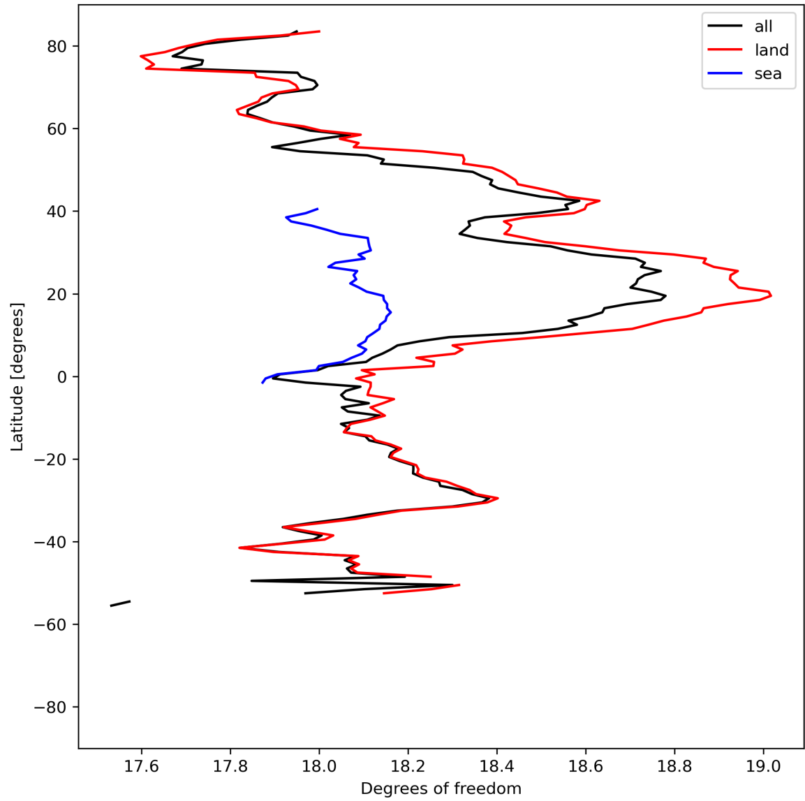
Figure 19: Zonal average of “Degrees of freedom” for 2024-04-22 to 2024-04-24.
