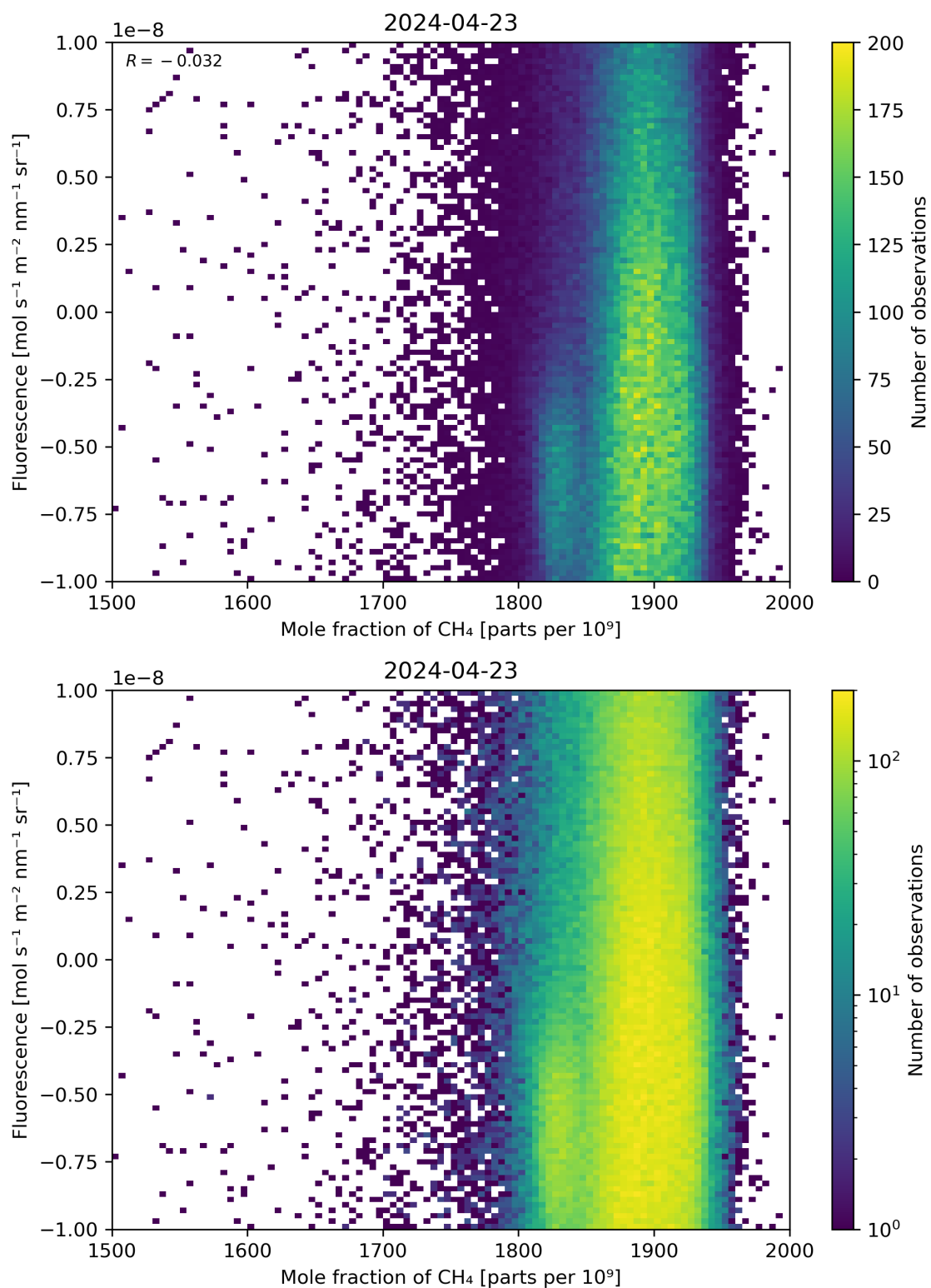
Figure 73: Scatter density plot of “Mole fraction of \text{CH}_4 ” against “Fluorescence” for 2024-04-22 to 2024-04-24.
