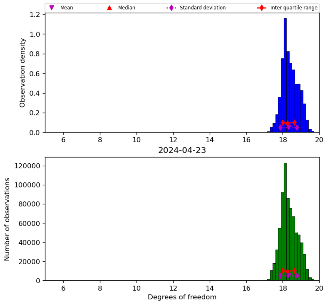
Figure 30: Histogram of “Degrees of freedom” for 2024-04-22 to 2024-04-24
