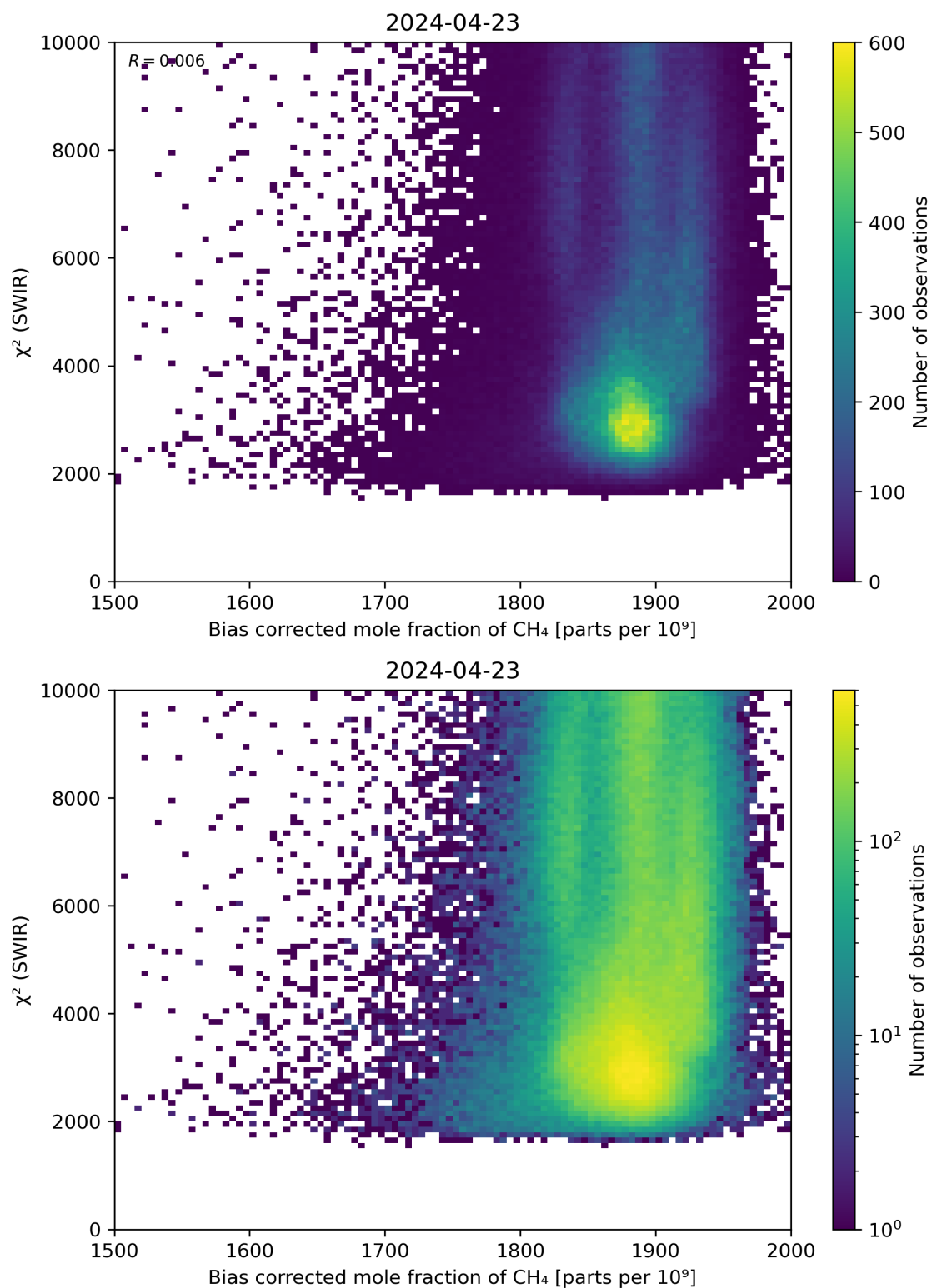
Figure 64: Scatter density plot of “Bias corrected mole fraction of CH 4 ” against “ \chi^2 (SWIR)” for 2024-04-22 to 2024-04-24.
