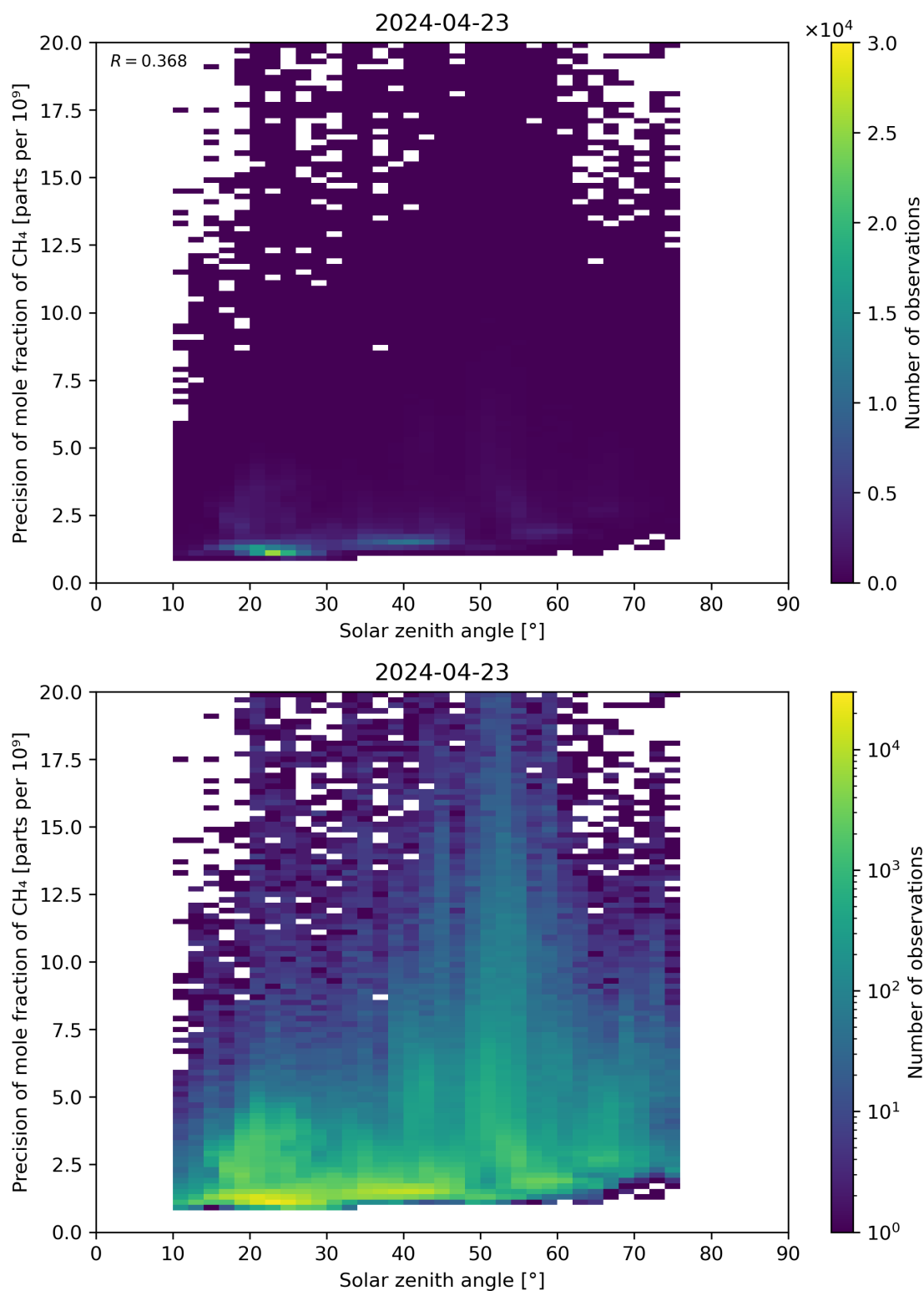
Figure 101: Scatter density plot of “Solar zenith angle” against “Precision of mole fraction of CH 4 ” for 2024-04-22 to 2024-04-24.
