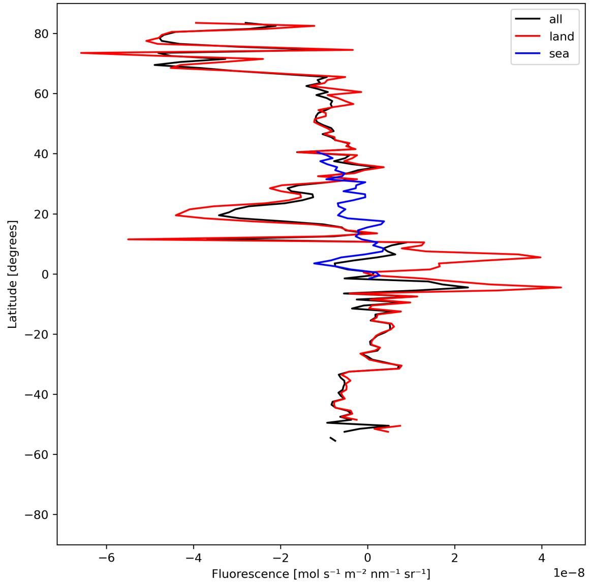
Figure 21: Zonal average of “Fluorescence” for 2024-04-22 to 2024-04-24.
