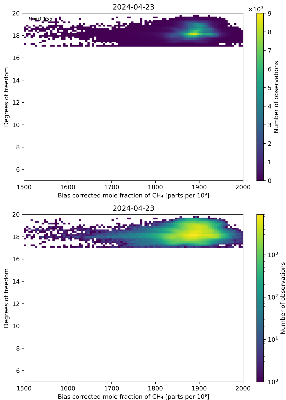
Figure 65: Scatter density plot of “Bias corrected mole fraction of CH 4 ” against “Degrees of freedom” for 2024-04-22 to 2024-04-24.
