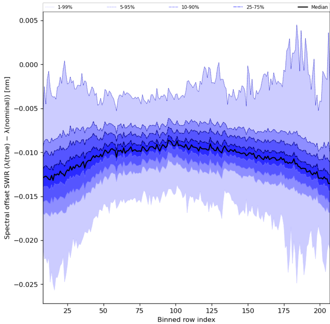
Figure 38: Along track statistics of “Spectral offset SWIR ( \lambda(\text{true}) - \lambda(\text{nominal}) )” for 2024-04-22 to 2024-04-24
