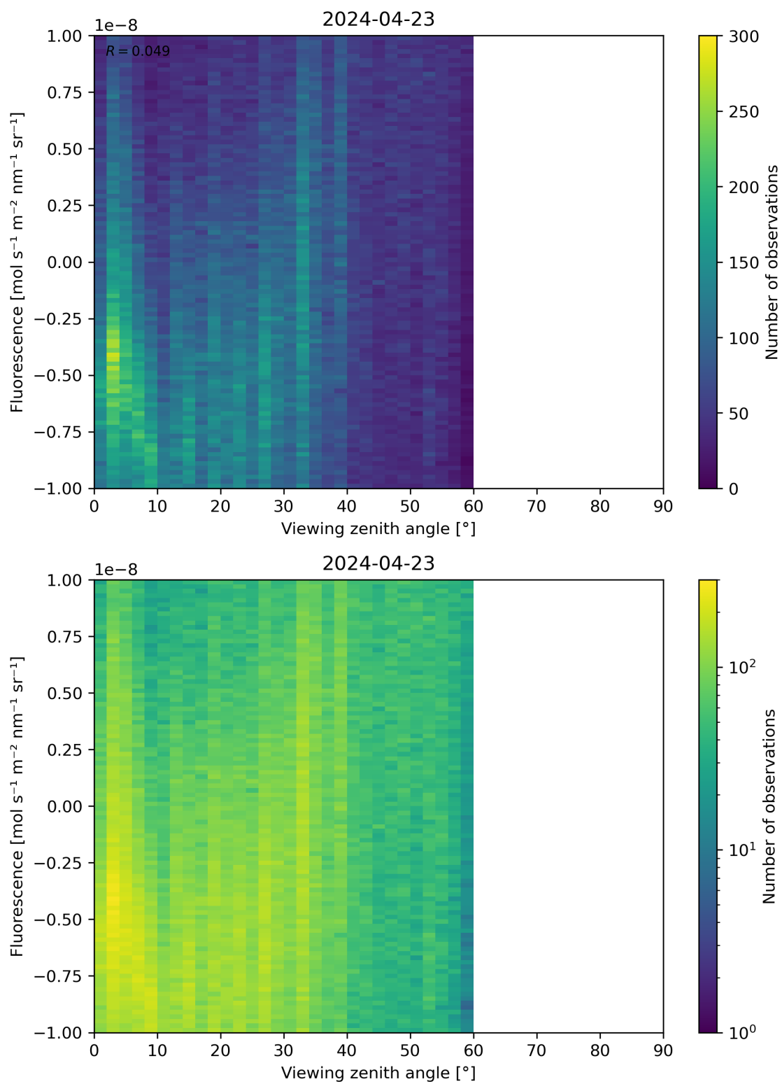
Figure 108: Scatter density plot of “Viewing zenith angle” against “Fluorescence” for 2024-04-22 to 2024-04-24.
