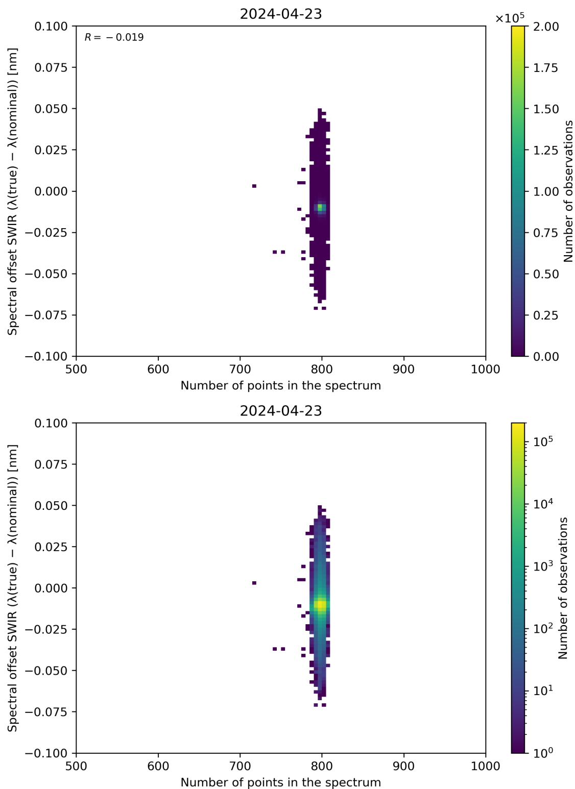
Figure 93: Scatter density plot of “Number of points in the spectrum” against “Spectral offset SWIR ( \lambda(\text{true}) - \lambda(\text{nominal}) )” for 2024-04-22 to 2024-04-24.
