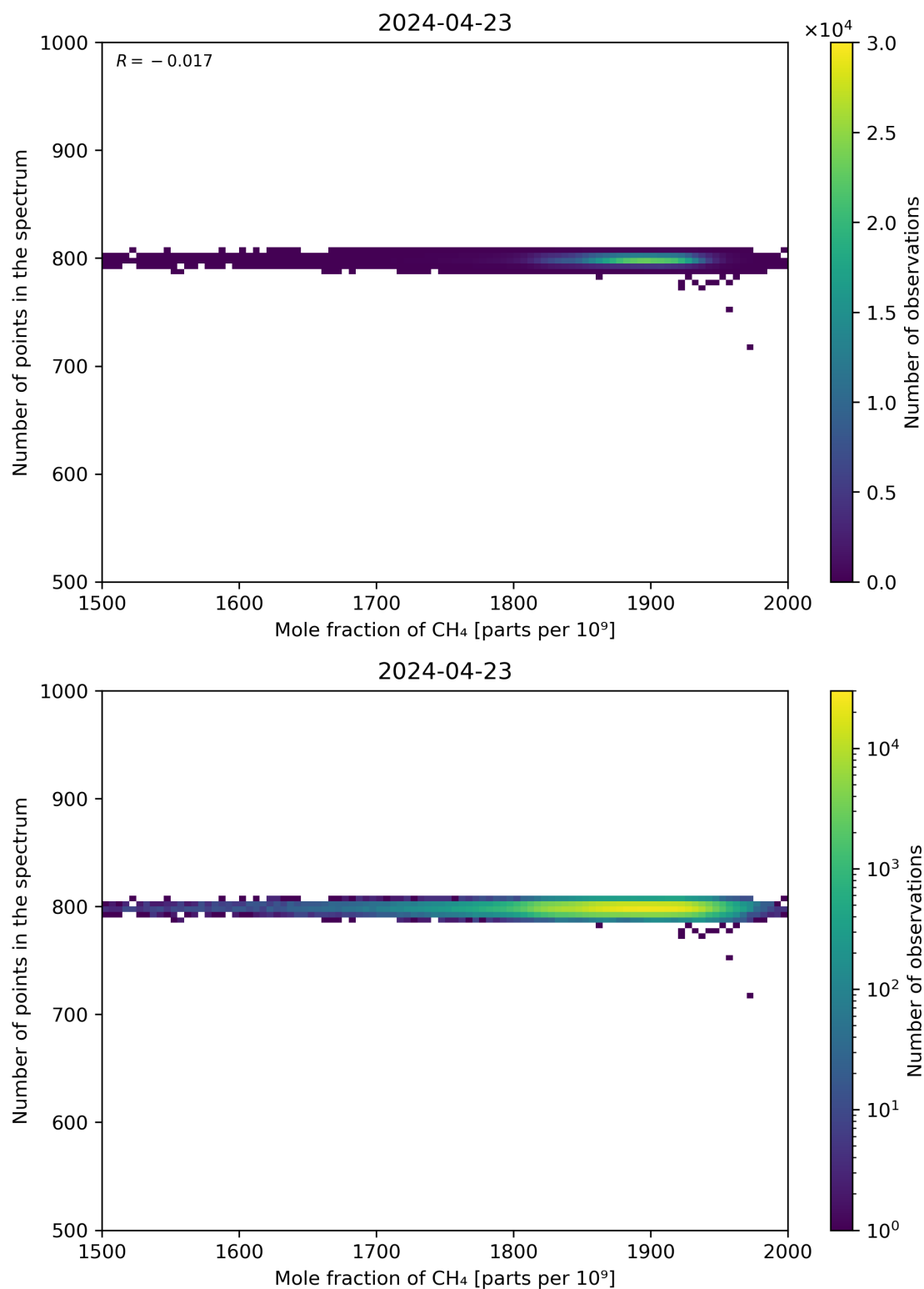
Figure 77: Scatter density plot of “Mole fraction of CH 4 ” against “Number of points in the spectrum” for 2024-04-22 to 2024-04-24.
