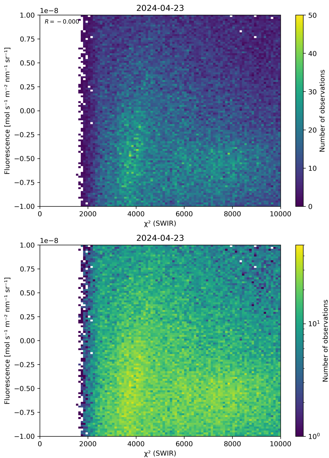
Figure 49: Scatter density plot of “ \chi^2 (SWIR)” against “Fluorescence” for 2024-04-22 to 2024-04-24.
