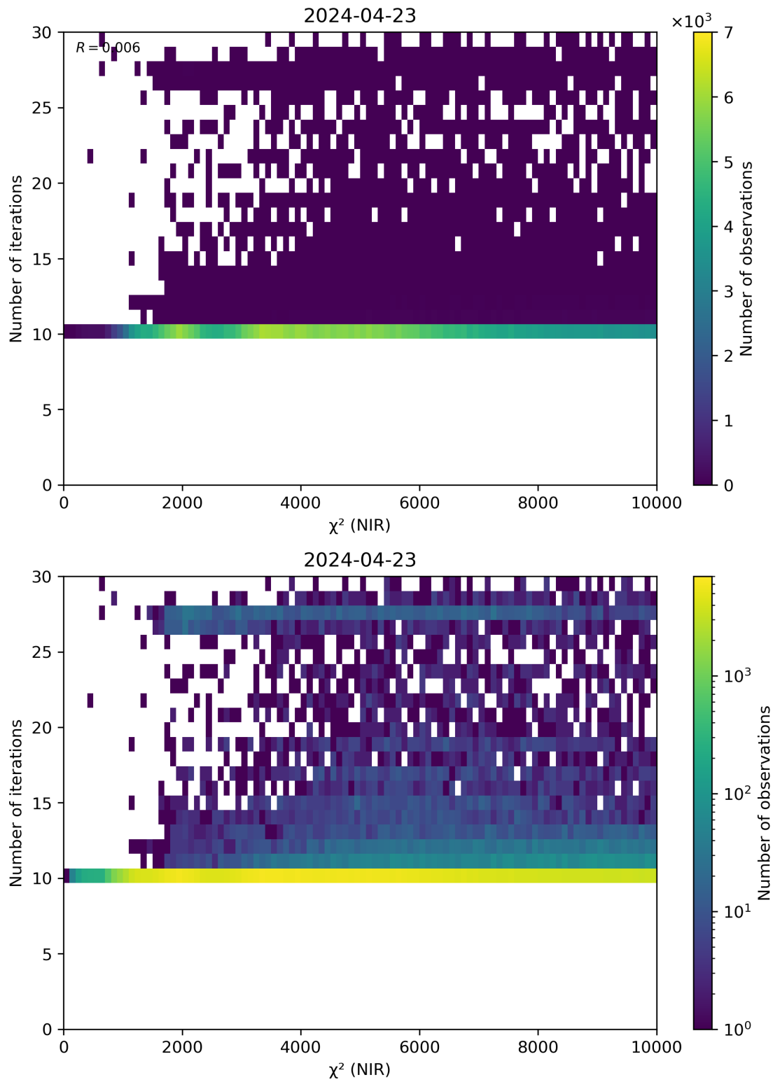
Figure 46: Scatter density plot of “ \chi^2 (NIR)” against “Number of iterations” for 2024-04-22 to 2024-04-24.
