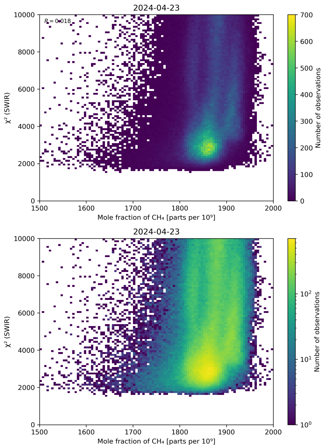
Figure 71: Scatter density plot of “Mole fraction of CH 4 ” against “ \chi^2 (SWIR)” for 2024-04-22 to 2024-04-24.
