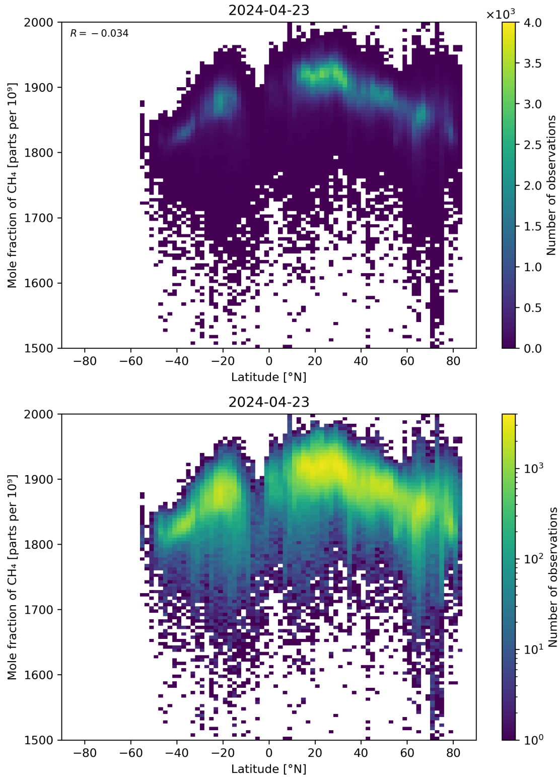
Figure 57: Scatter density plot of “Latitude” against “Mole fraction of CH 4 ” for 2024-04-22 to 2024-04-24.
