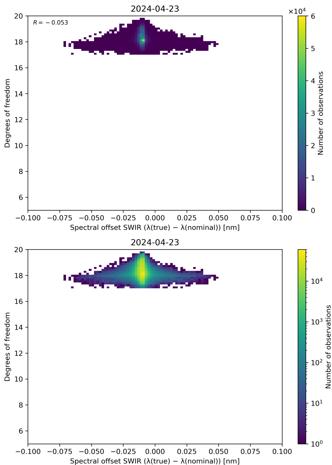
Figure 119: Scatter density plot of “Spectral offset SWIR ( \lambda(\text{true}) - \lambda(\text{nominal}) )” against “Degrees of freedom” for 2024-04-22 to 2024-04-24.
