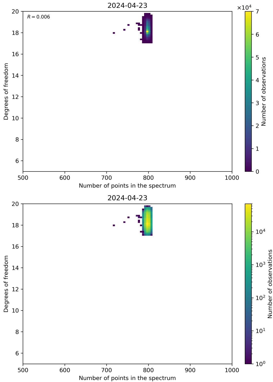
Figure 90: Scatter density plot of “Number of points in the spectrum” against “Degrees of freedom” for 2024-04-22 to 2024-04-24.
