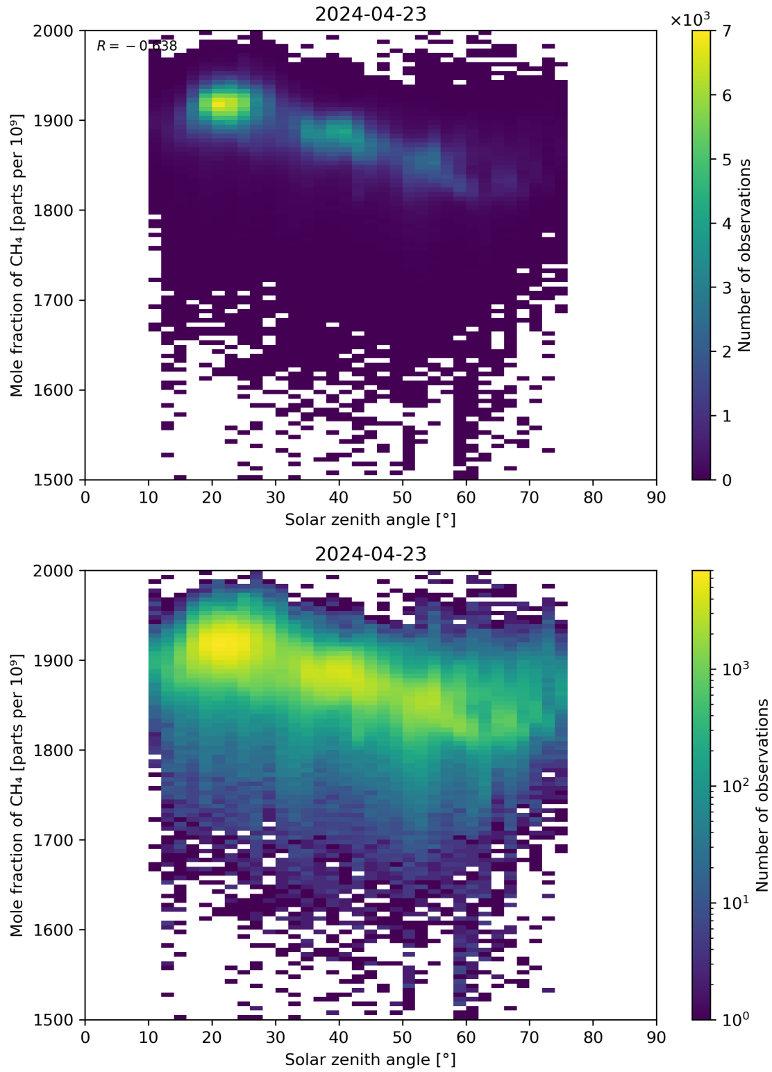
Figure 99: Scatter density plot of “Solar zenith angle” against “Mole fraction of \text{CH}_4 ” for 2024-04-22 to 2024-04-24.
