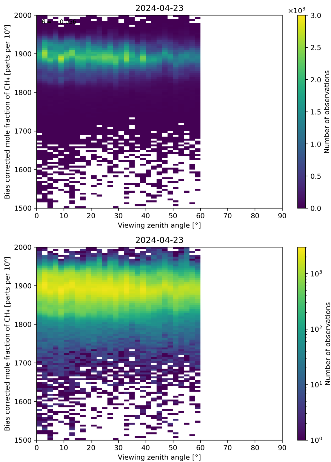
Figure 111: Scatter density plot of “Viewing zenith angle” against “Bias corrected mole fraction of CH 4 ” for 2024-04-22 to 2024-04-24.
