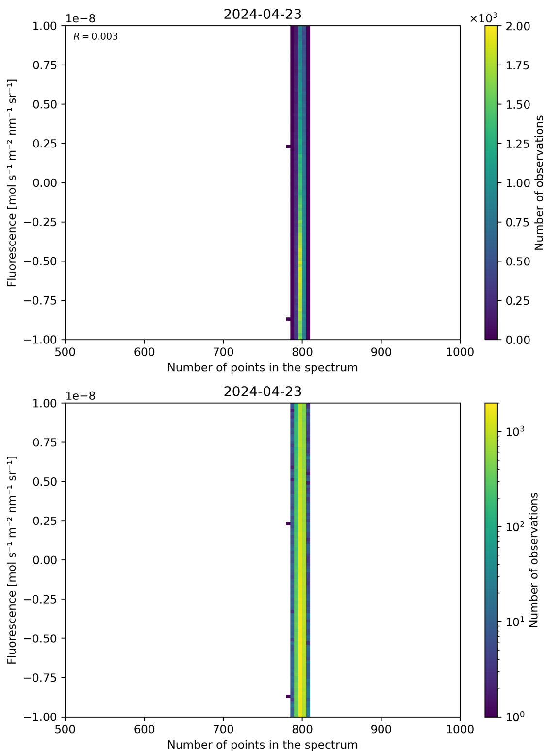
Figure 91: Scatter density plot of “Number of points in the spectrum” against “Fluorescence” for 2024-04-22 to 2024-04-24.
