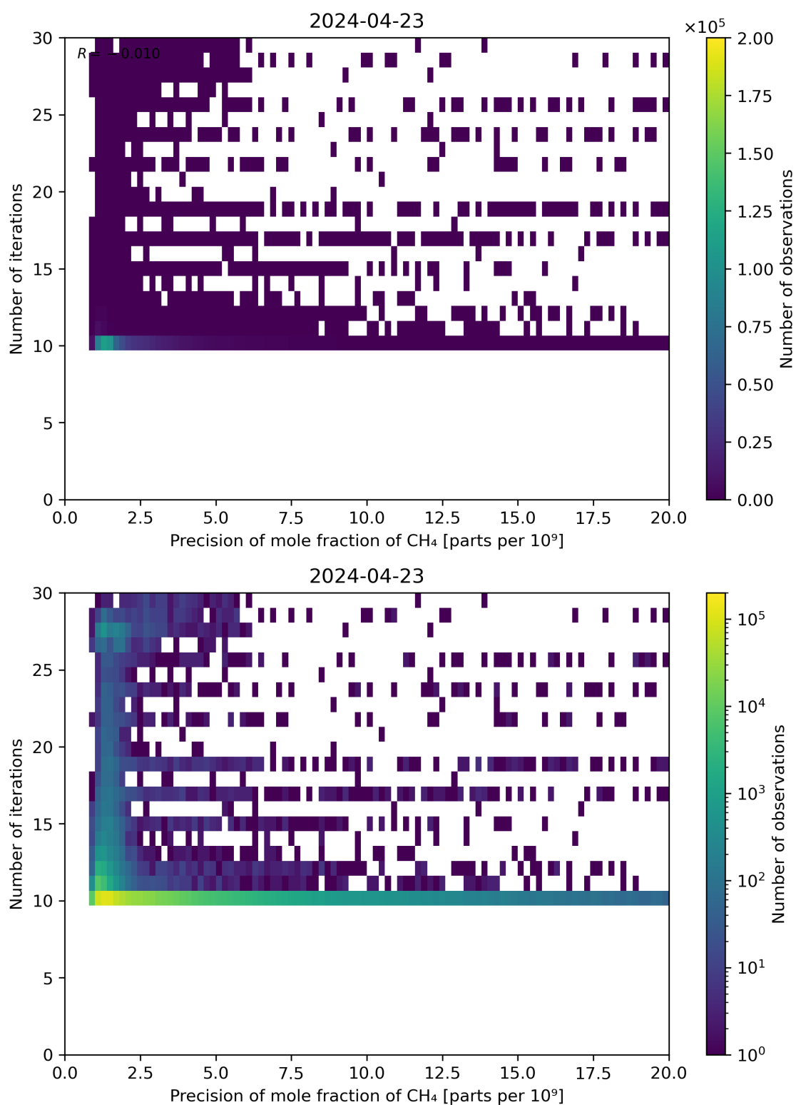
Figure 83: Scatter density plot of “Precision of mole fraction of CH 4 ” against “Number of iterations” for 2024-04-22 to 2024-04-24.
