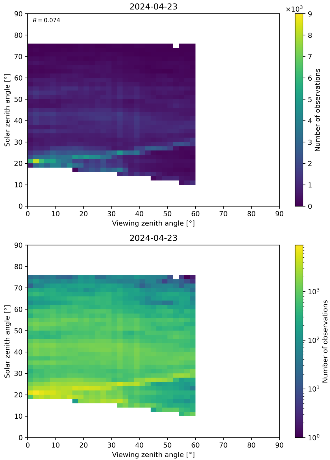
Figure 115: Scatter density plot of “Viewing zenith angle” against “Solar zenith angle” for 2024-04-22 to 2024-04-24.
