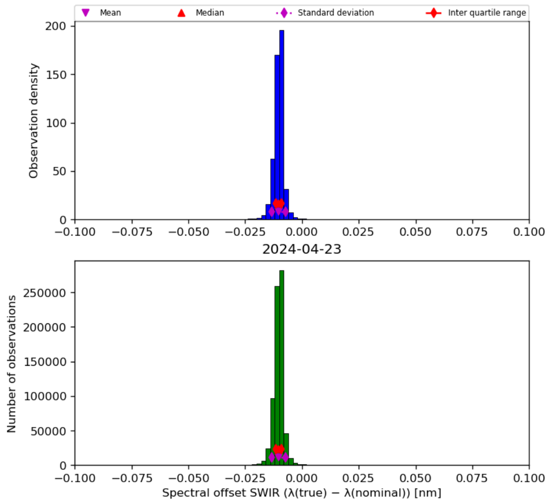
Figure 27: Histogram of “Spectral offset SWIR ( \lambda(\text{true}) - \lambda(\text{nominal}) )” for 2024-04-22 to 2024-04-24
