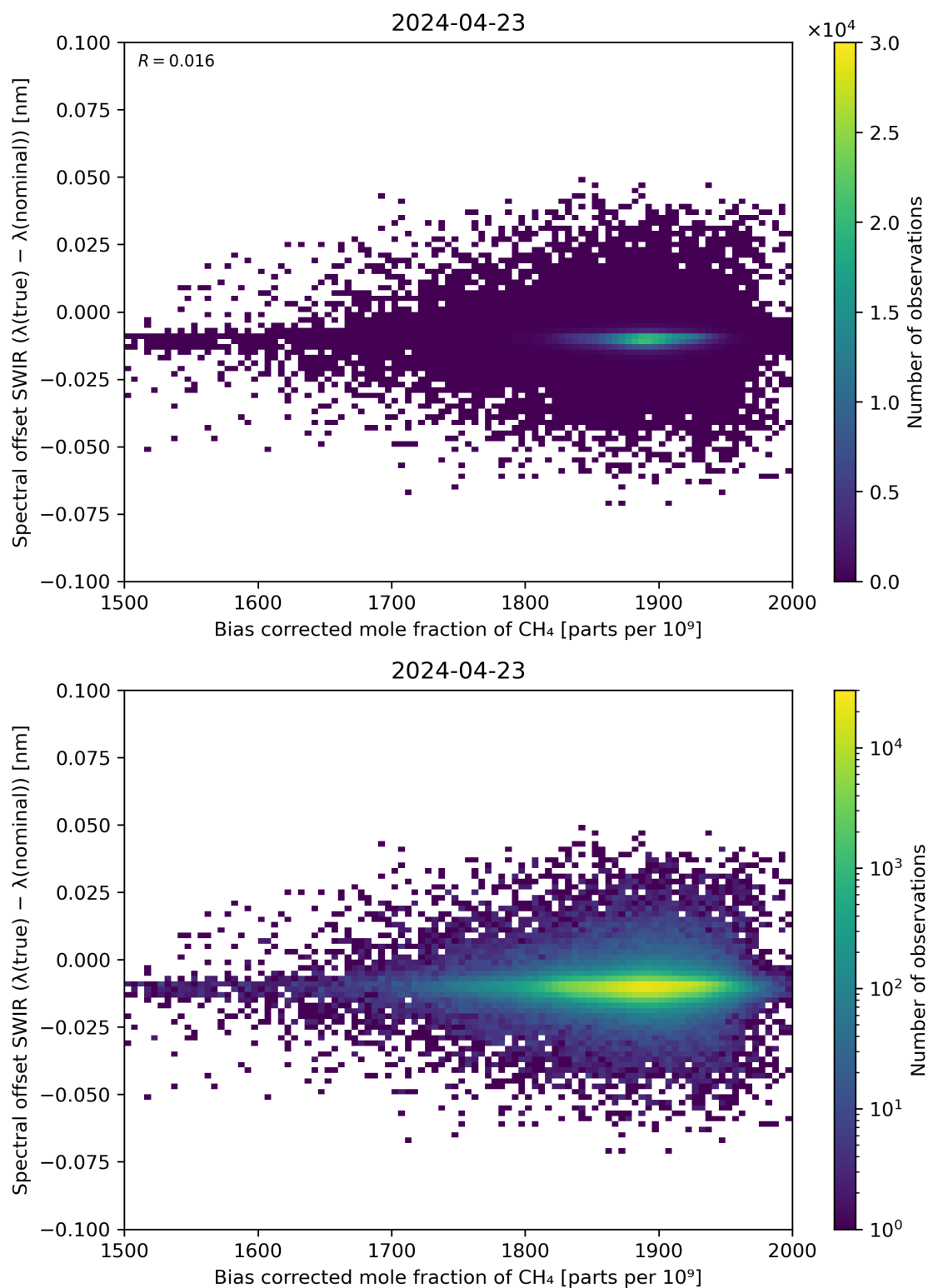
Figure 69: Scatter density plot of “Bias corrected mole fraction of \text{CH}_4 ” against “Spectral offset SWIR ( \lambda(\text{true}) - \lambda(\text{nominal}) )” for 2024-04-22 to 2024-04-24.
