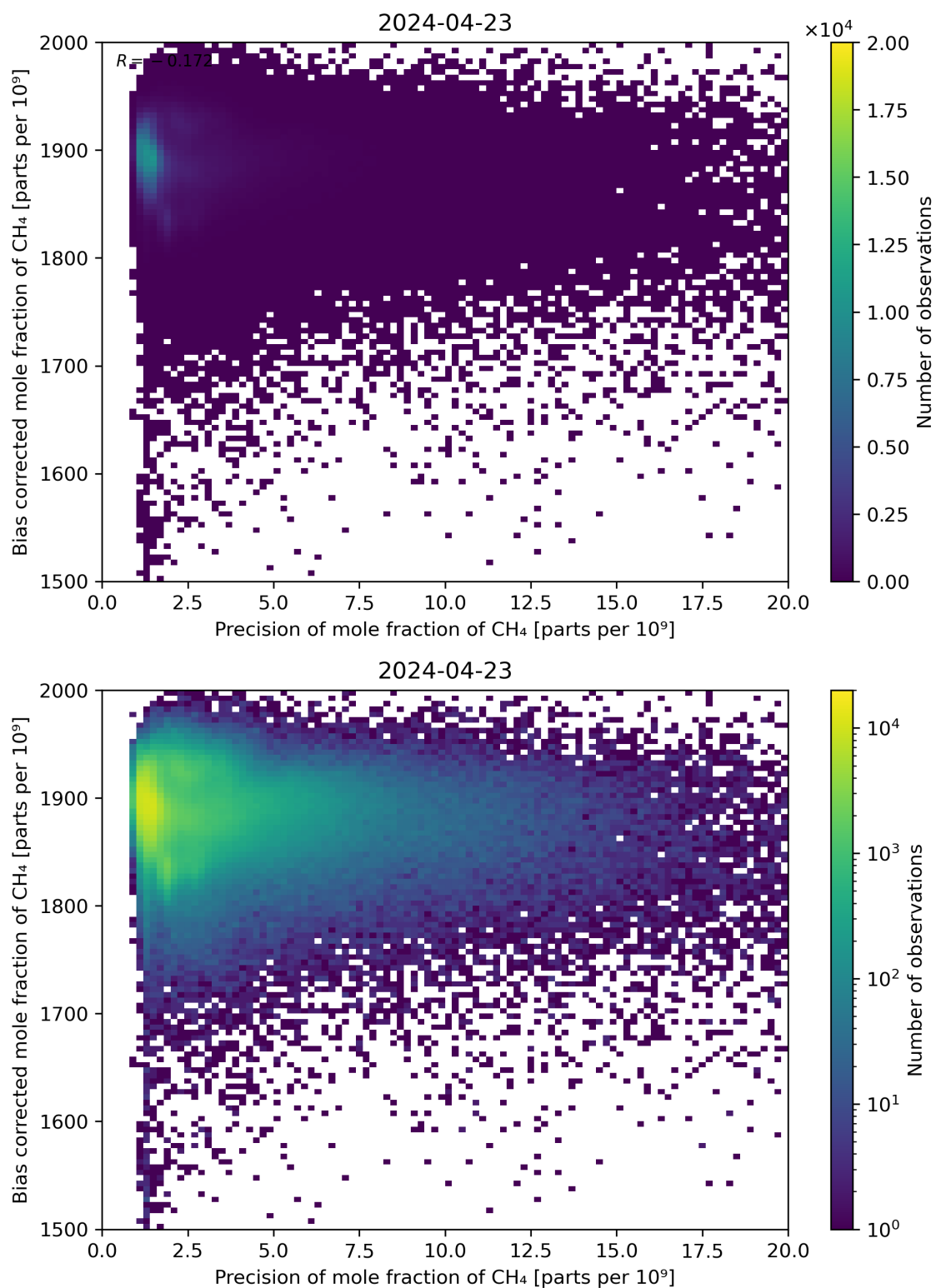
Figure 82: Scatter density plot of “Precision of mole fraction of CH 4 ” against “Bias corrected mole fraction of CH 4 ” for 2024-04-22 to 2024-04-24.
