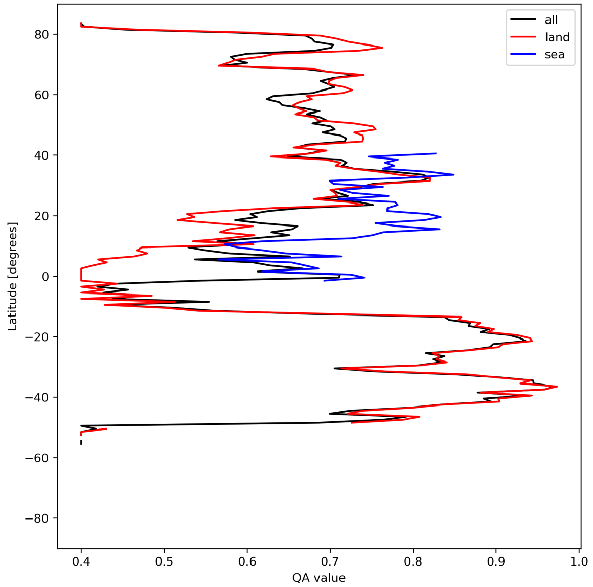
Figure 11: Zonal average of “QA value” for 2024-04-22 to 2024-04-24.
