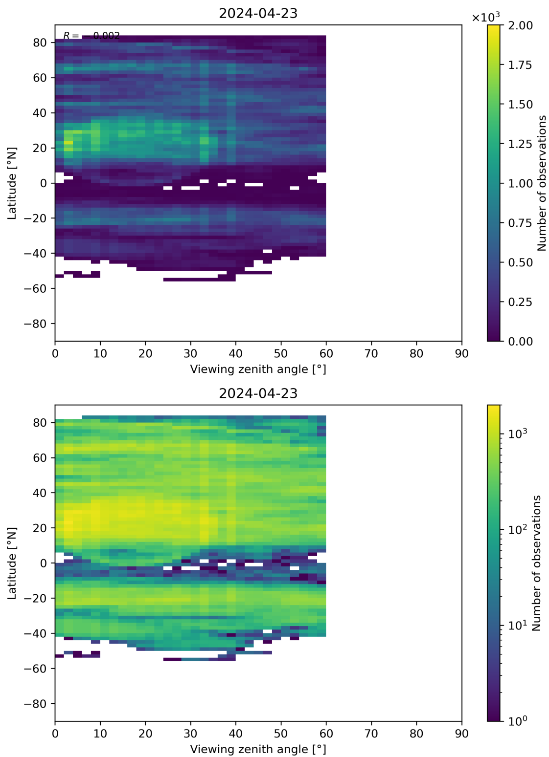
Figure 109: Scatter density plot of “Viewing zenith angle” against “Latitude” for 2024-04-22 to 2024-04-24.
