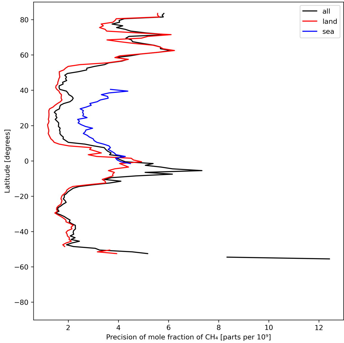
Figure 13: Zonal average of “Precision of mole fraction of CH 4 ” for 2024-04-22 to 2024-04-24.
