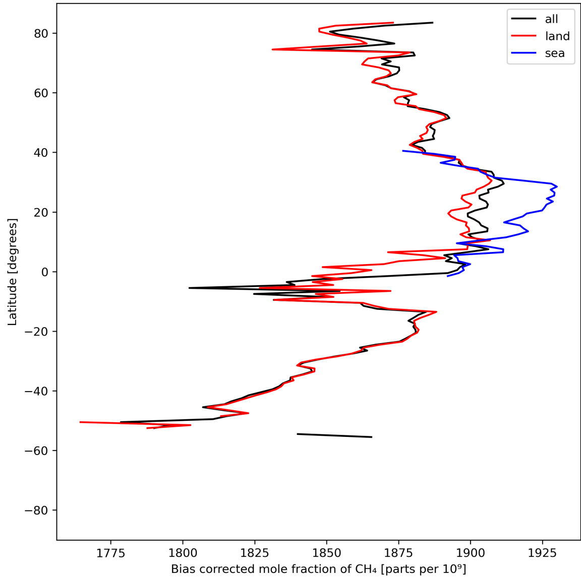
Figure 14: Zonal average of “Bias corrected mole fraction of CH 4 ” for 2024-04-22 to 2024-04-24.
