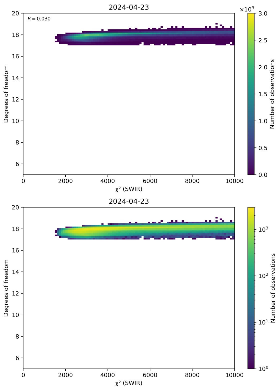
Figure 48: Scatter density plot of “ \chi^2 (SWIR)” against “Degrees of freedom” for 2024-04-22 to 2024-04-24.
