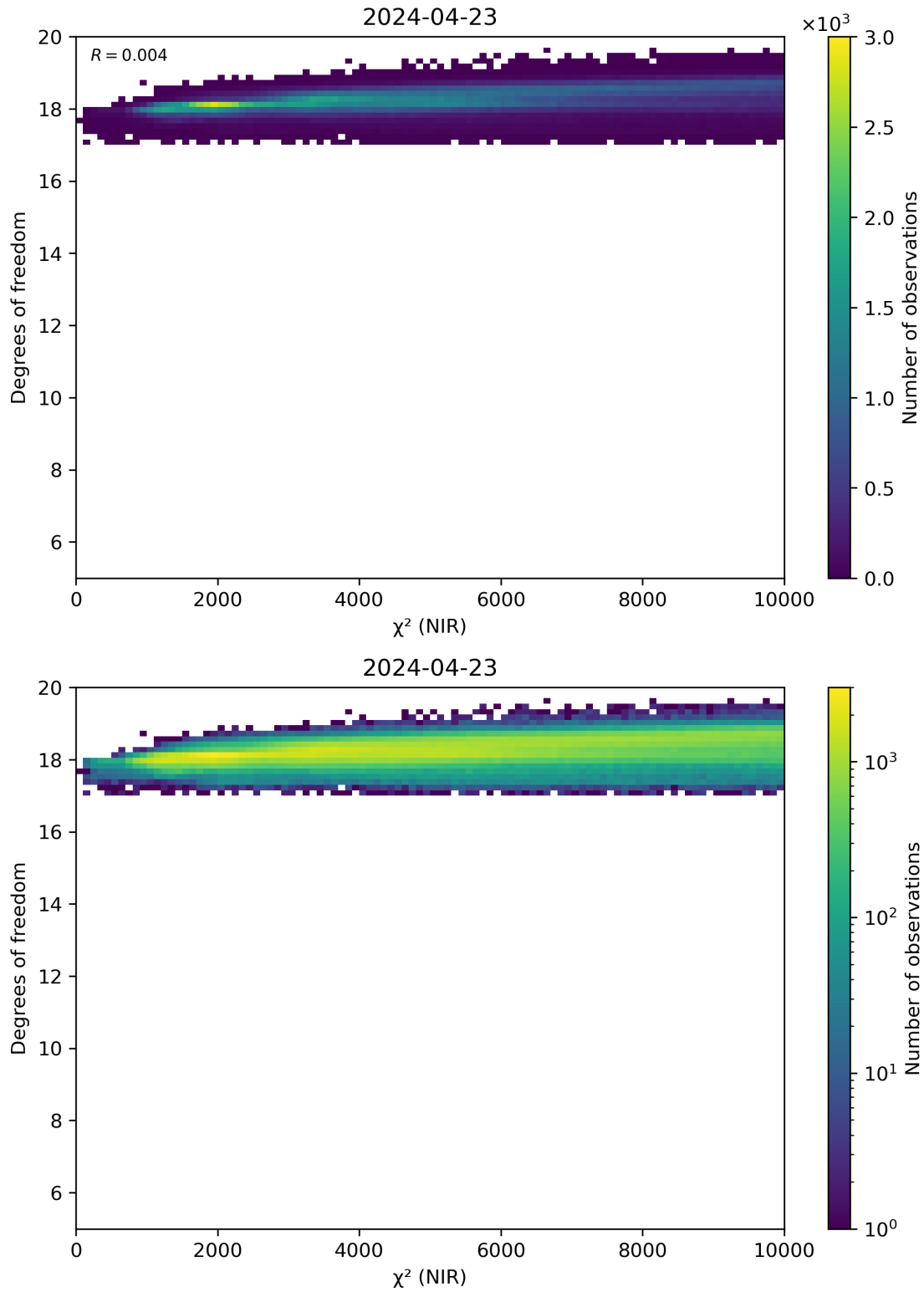
Figure 44: Scatter density plot of “ \chi^2 (NIR)” against “Degrees of freedom” for 2024-04-22 to 2024-04-24.
