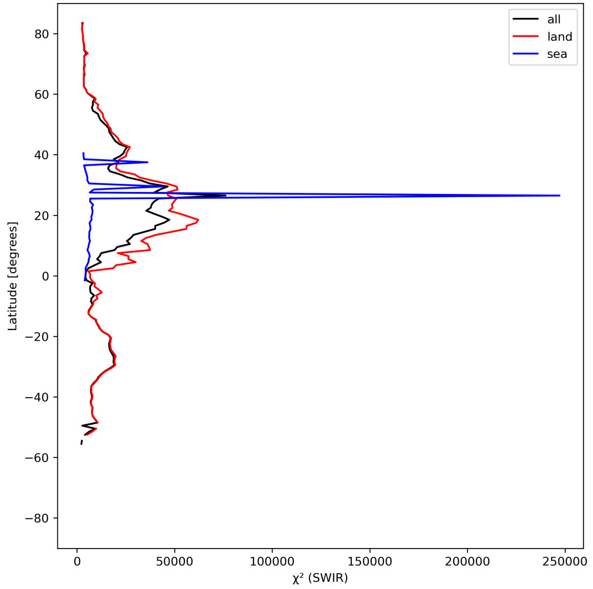
Figure 17: Zonal average of “ \chi^2 (SWIR)” for 2024-04-22 to 2024-04-24.
