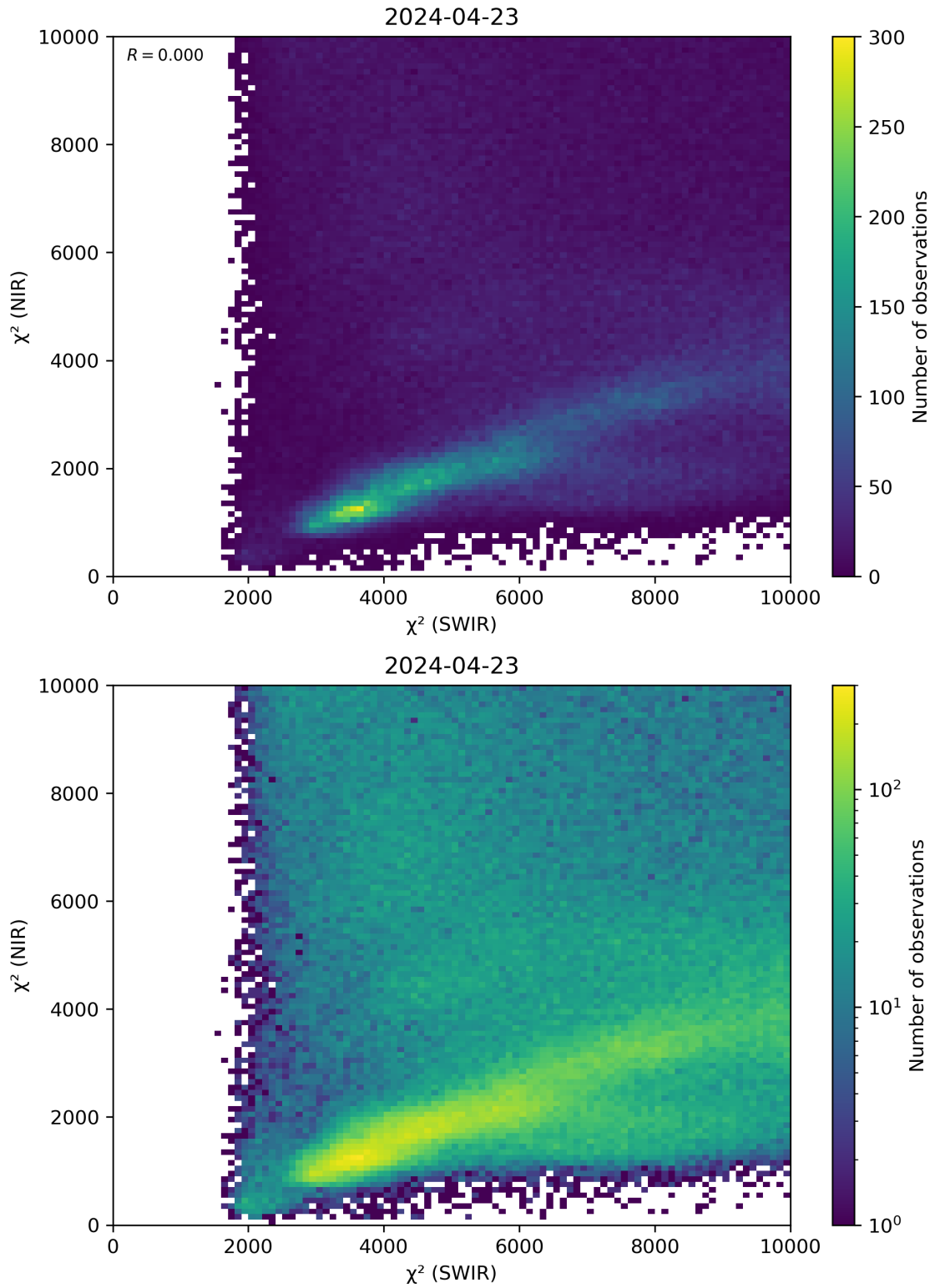
Figure 47: Scatter density plot of “ \chi^2 (SWIR)” against “ \chi^2 (NIR)” for 2024-04-22 to 2024-04-24.
