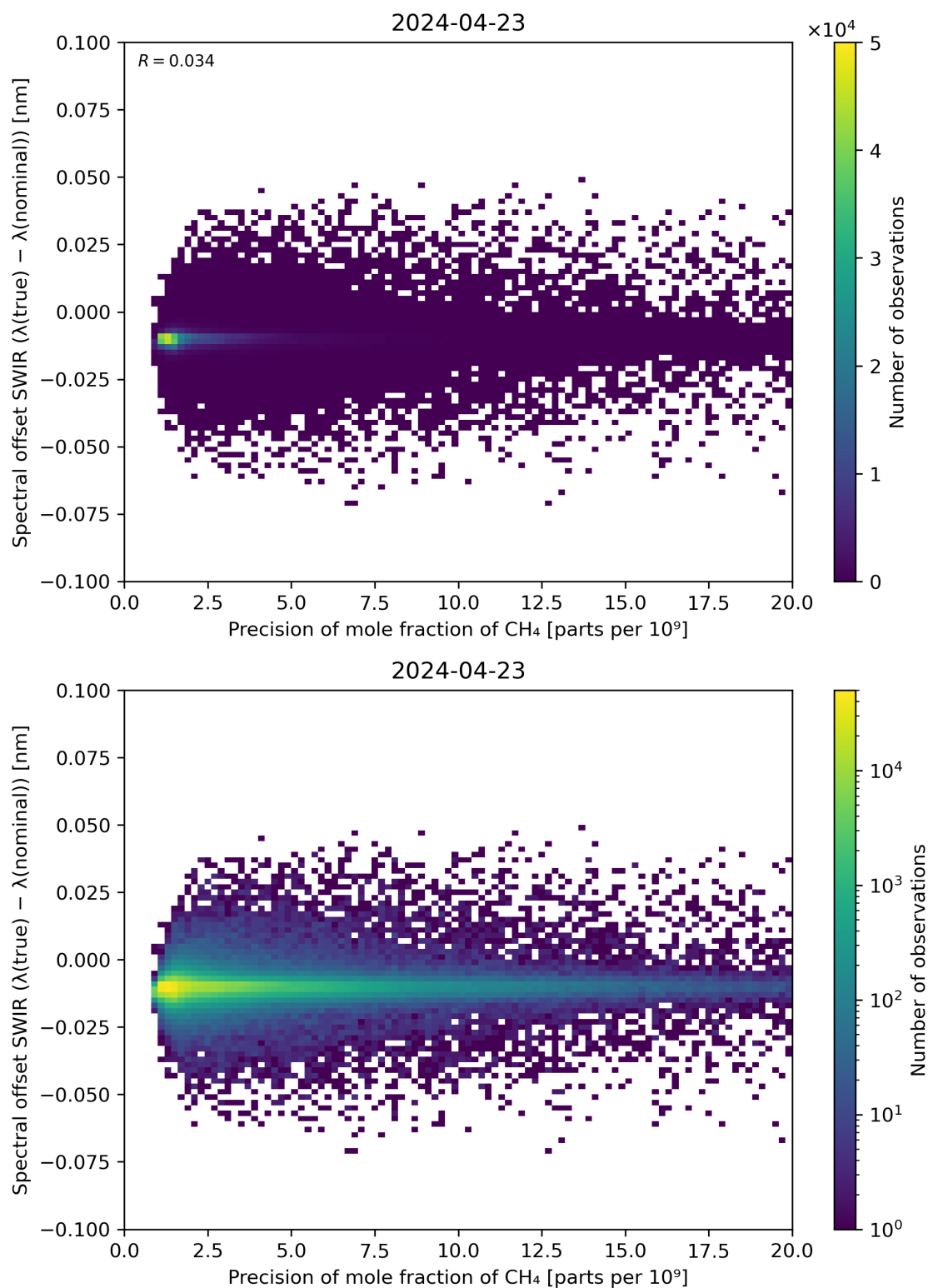
Figure 85: Scatter density plot of “Precision of mole fraction of CH 4 ” against “Spectral offset SWIR ( \lambda(\text{true}) - \lambda(\text{nominal}) )” for 2024-04-22 to 2024-04-24.
