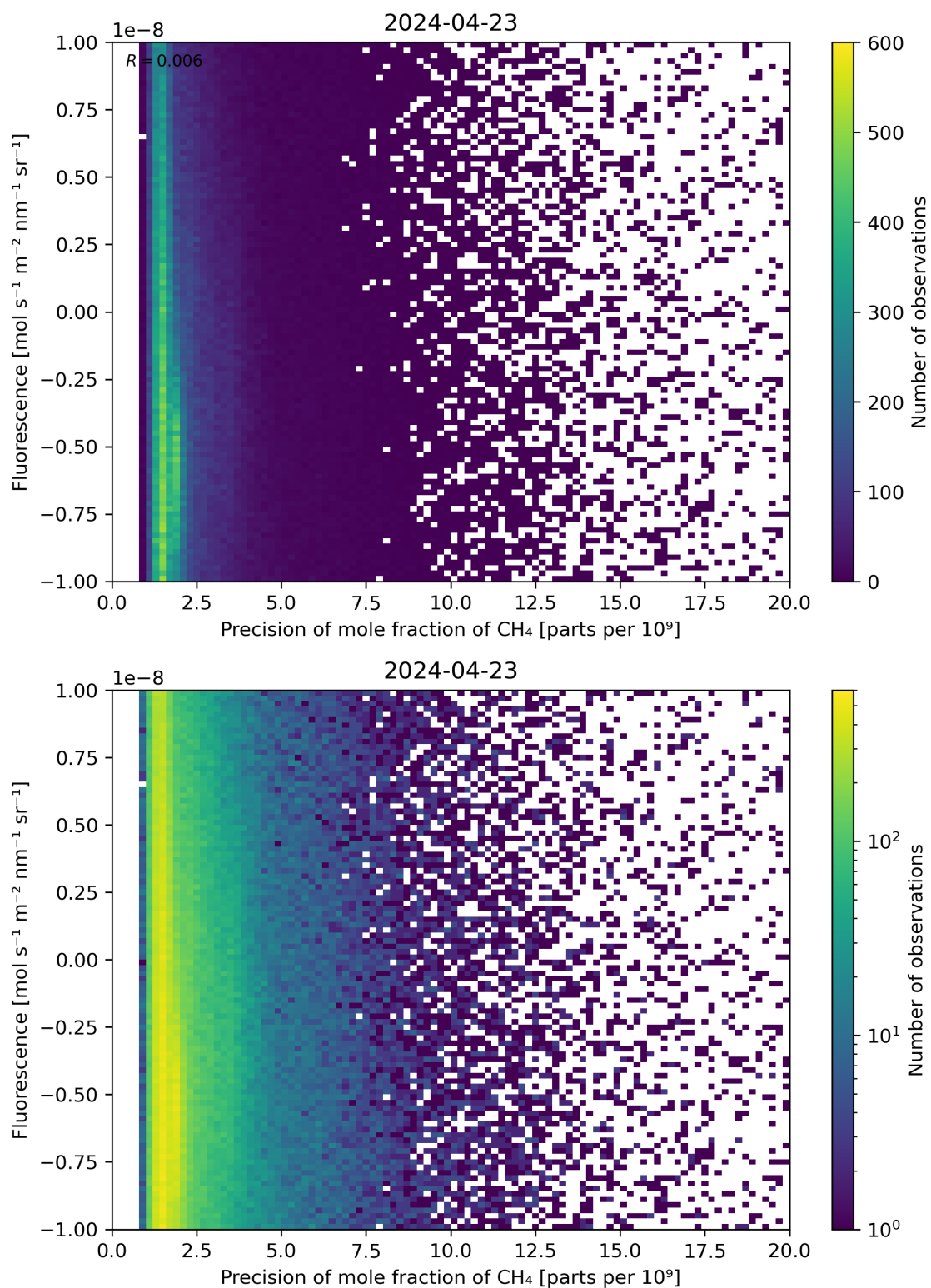
Figure 81: Scatter density plot of “Precision of mole fraction of \text{CH}_4 ” against “Fluorescence” for 2024-04-22 to 2024-04-24.
