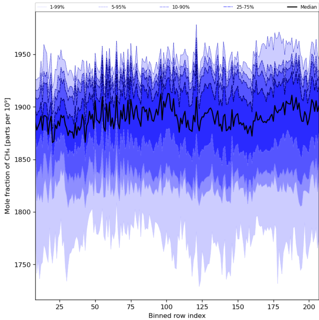
Figure 34: Along track statistics of “Mole fraction of CH 4 ” for 2024-04-22 to 2024-04-24
