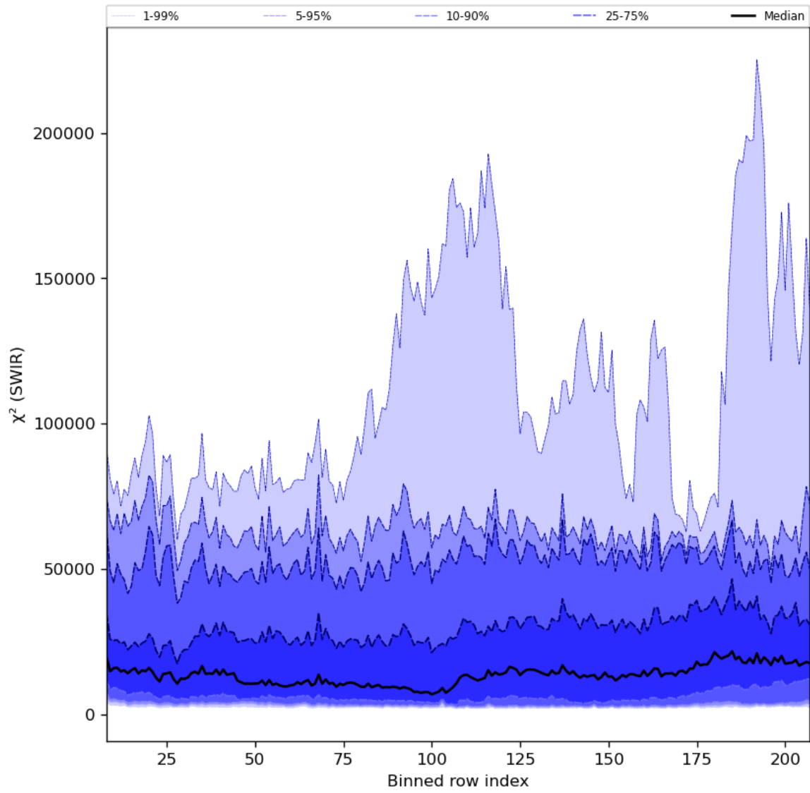
Figure 39: Along track statistics of “ \chi^2 (SWIR)” for 2024-04-22 to 2024-04-24
