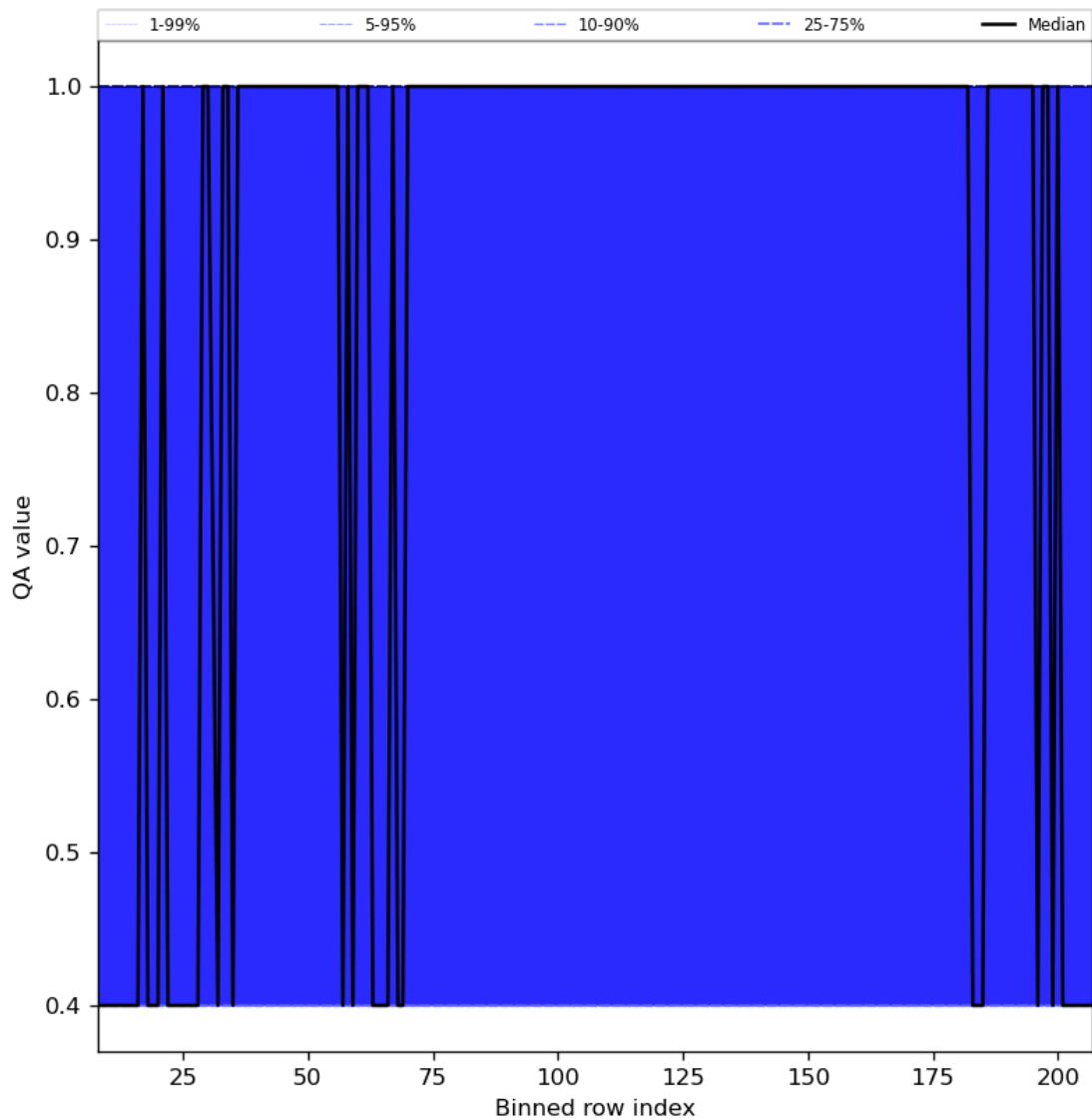
Figure 33: Along track statistics of “QA value” for 2024-04-22 to 2024-04-24
