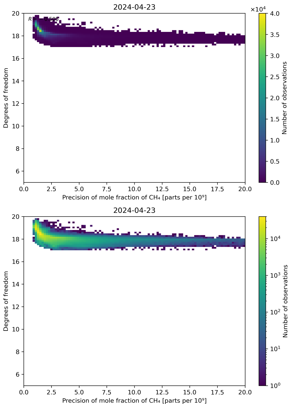
Figure 80: Scatter density plot of “Precision of mole fraction of CH 4 ” against “Degrees of freedom” for 2024-04-22 to 2024-04-24.
