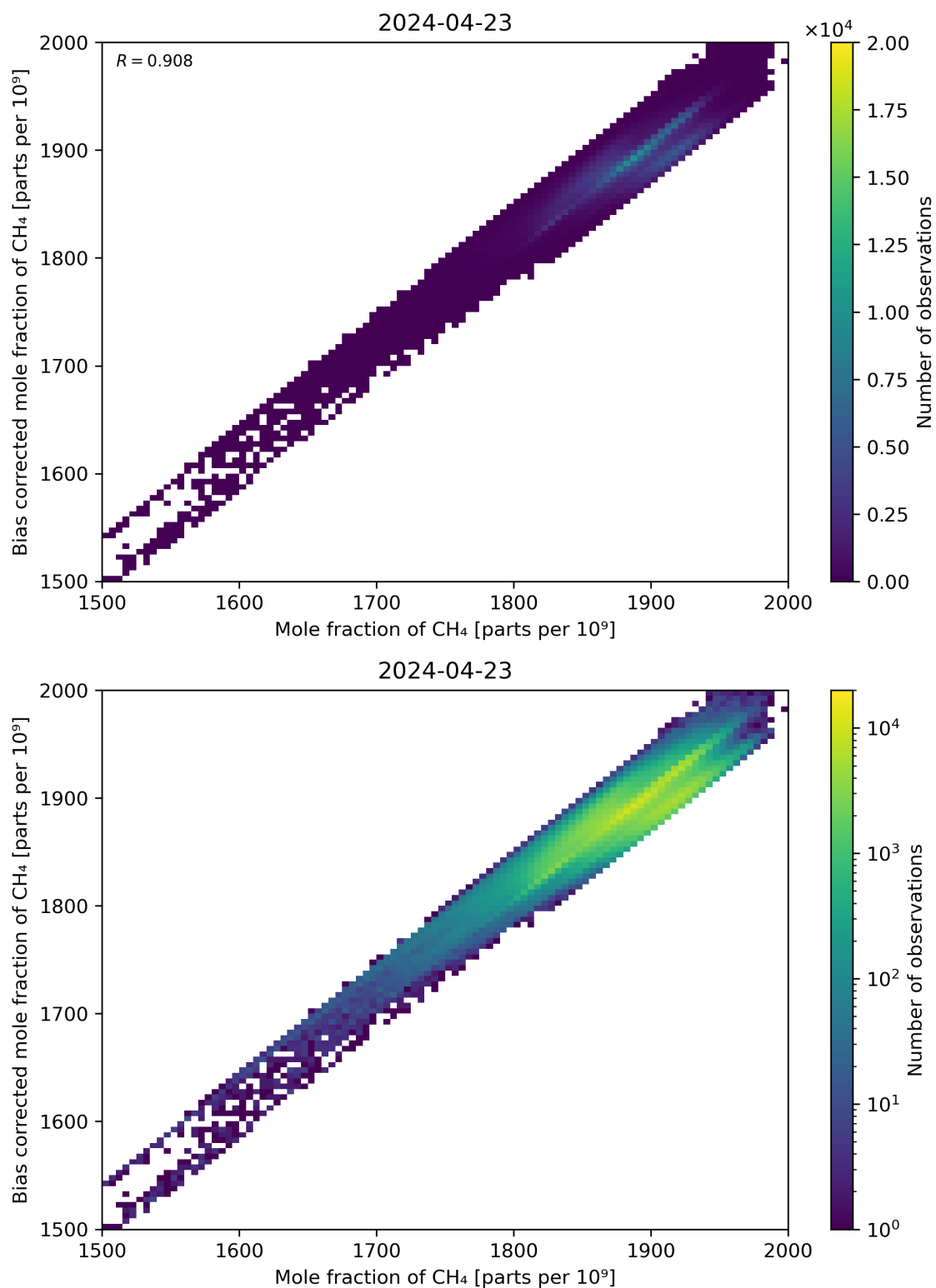
Figure 74: Scatter density plot of “Mole fraction of CH 4 ” against “Bias corrected mole fraction of CH 4 ” for 2024-04-22 to 2024-04-24.
