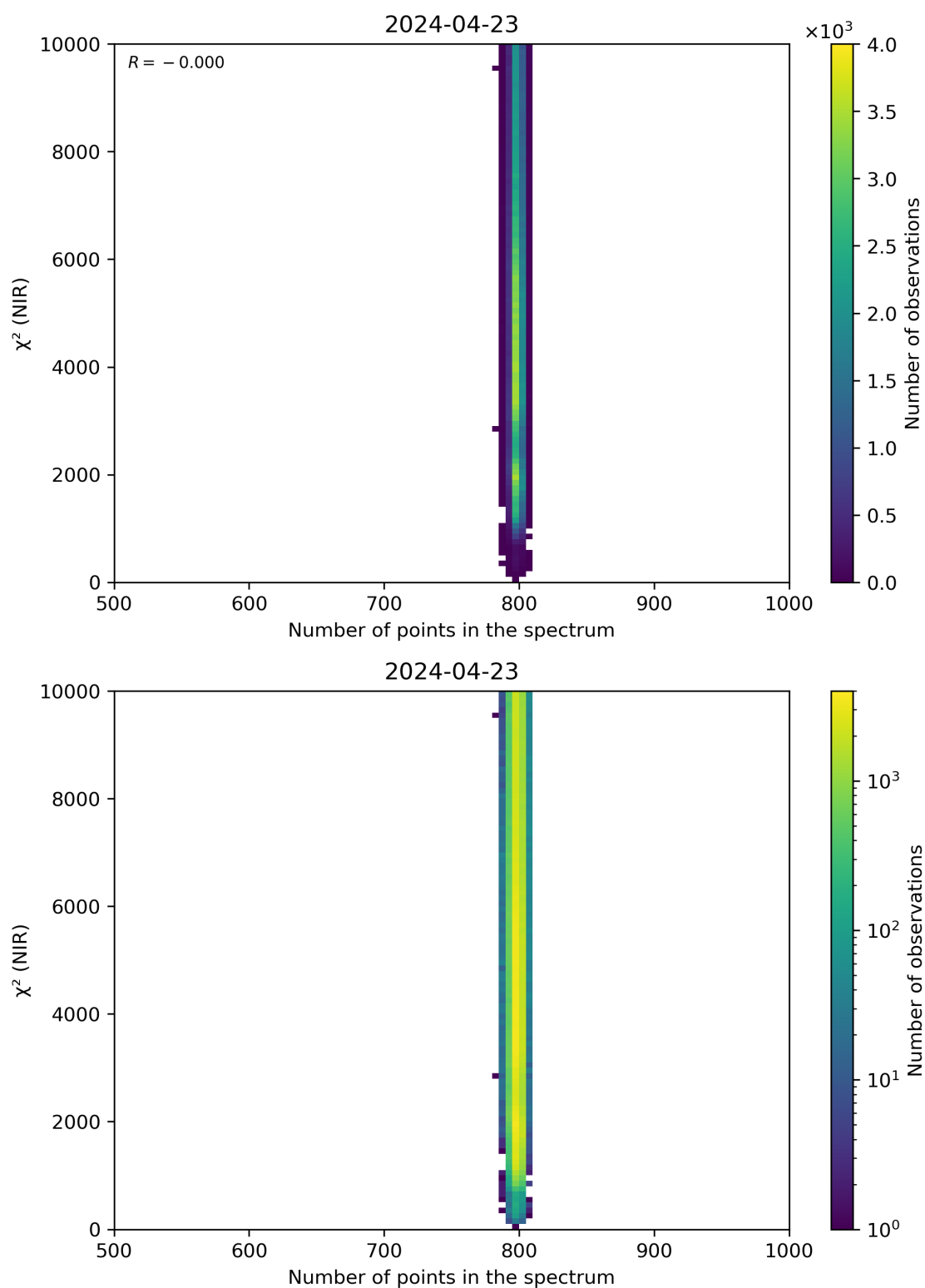
Figure 88: Scatter density plot of “Number of points in the spectrum” against “ \chi^2 (NIR)” for 2024-04-22 to 2024-04-24.
