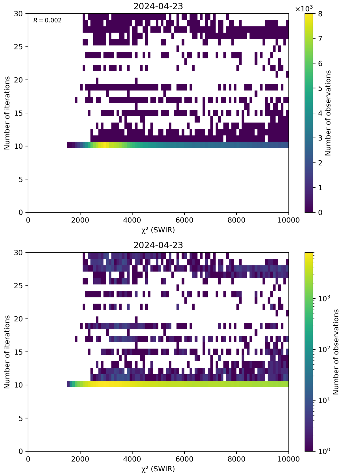
Figure 50: Scatter density plot of “ \chi^2 (SWIR)” against “Number of iterations” for 2024-04-22 to 2024-04-24.
