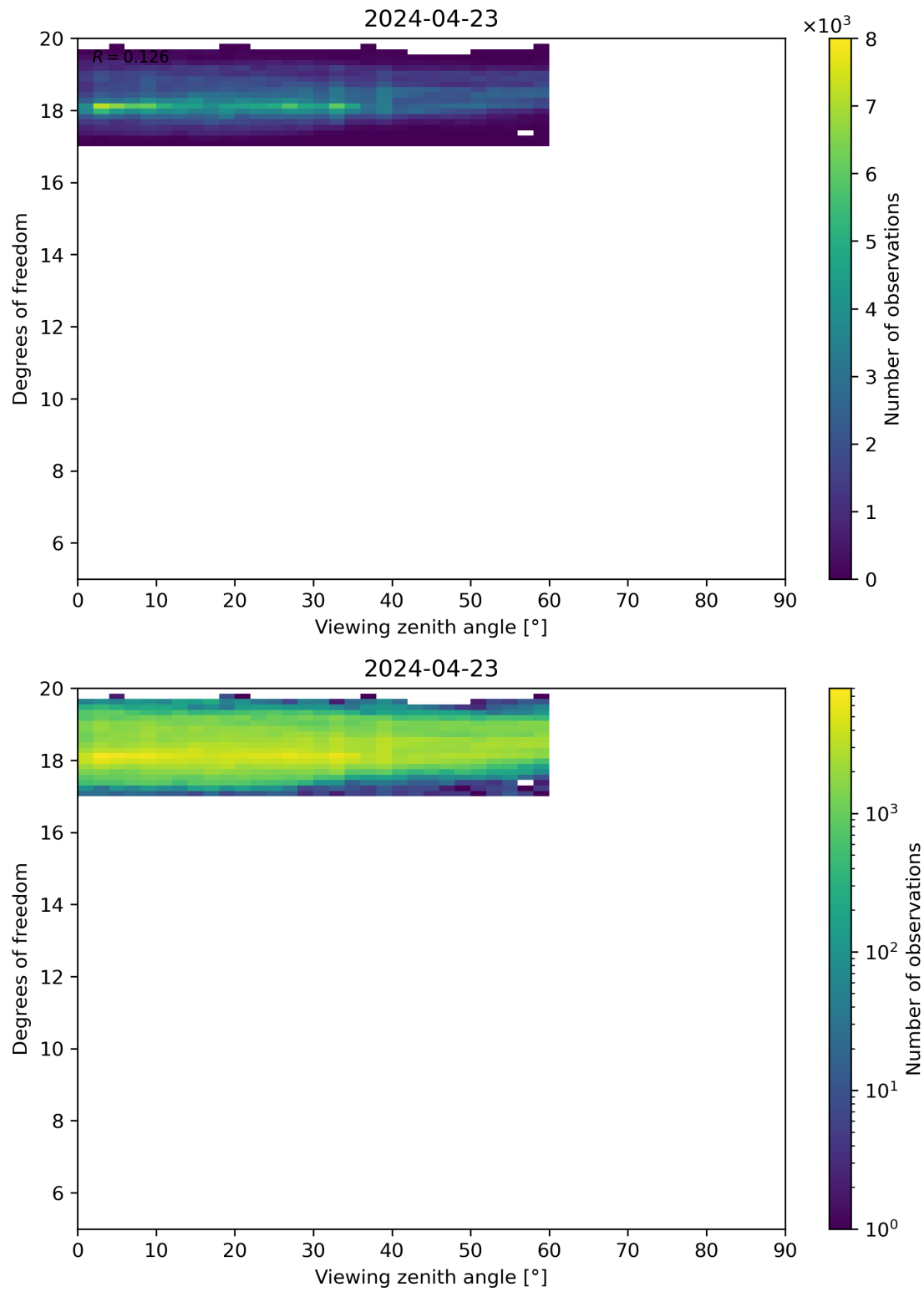
Figure 107: Scatter density plot of “Viewing zenith angle” against “Degrees of freedom” for 2024-04-22 to 2024-04-24.
