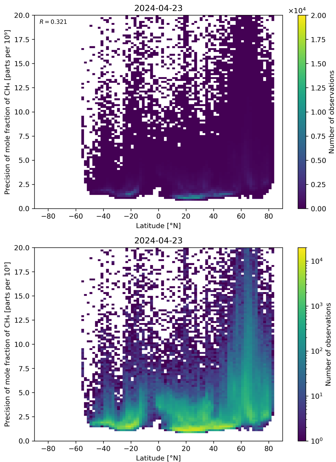
Figure 59: Scatter density plot of “Latitude” against “Precision of mole fraction of \text{CH}_4 ” for 2024-04-22 to 2024-04-24.
