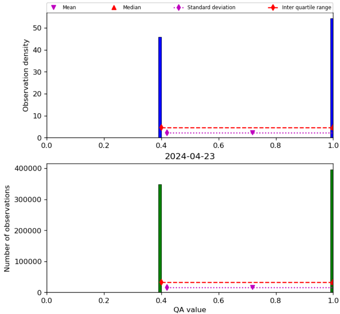
Figure 22: Histogram of "QA value" for 2024-04-22 to 2024-04-24
