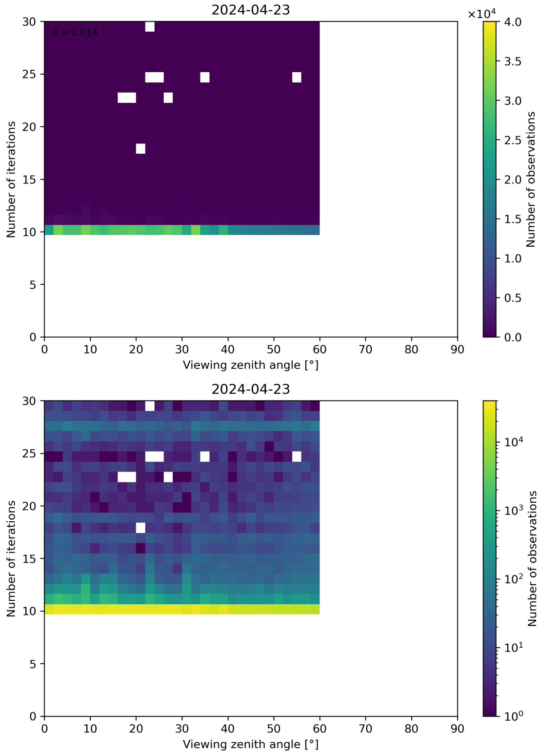
Figure 113: Scatter density plot of “Viewing zenith angle” against “Number of iterations” for 2024-04-22 to 2024-04-24.
