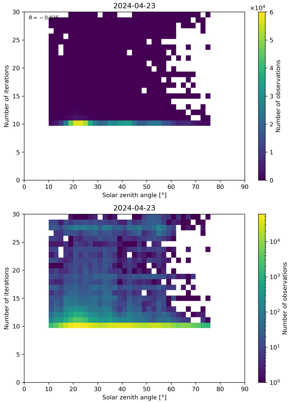
Figure 102: Scatter density plot of “Solar zenith angle” against “Number of iterations” for 2024-04-22 to 2024-04-24.
