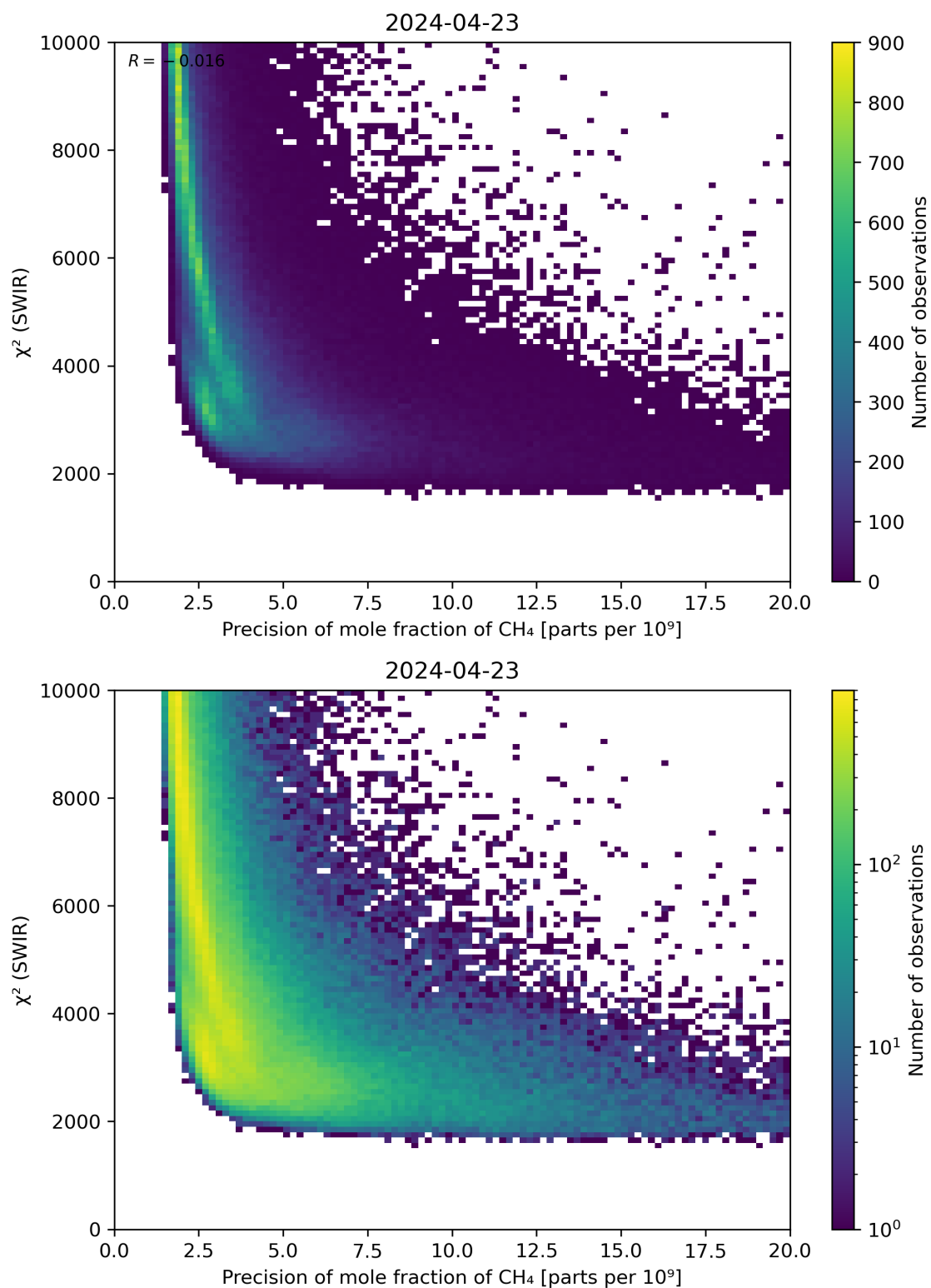
Figure 79: Scatter density plot of “Precision of mole fraction of \text{CH}_4 ” against “ \chi^2 (SWIR)” for 2024-04-22 to 2024-04-24.
