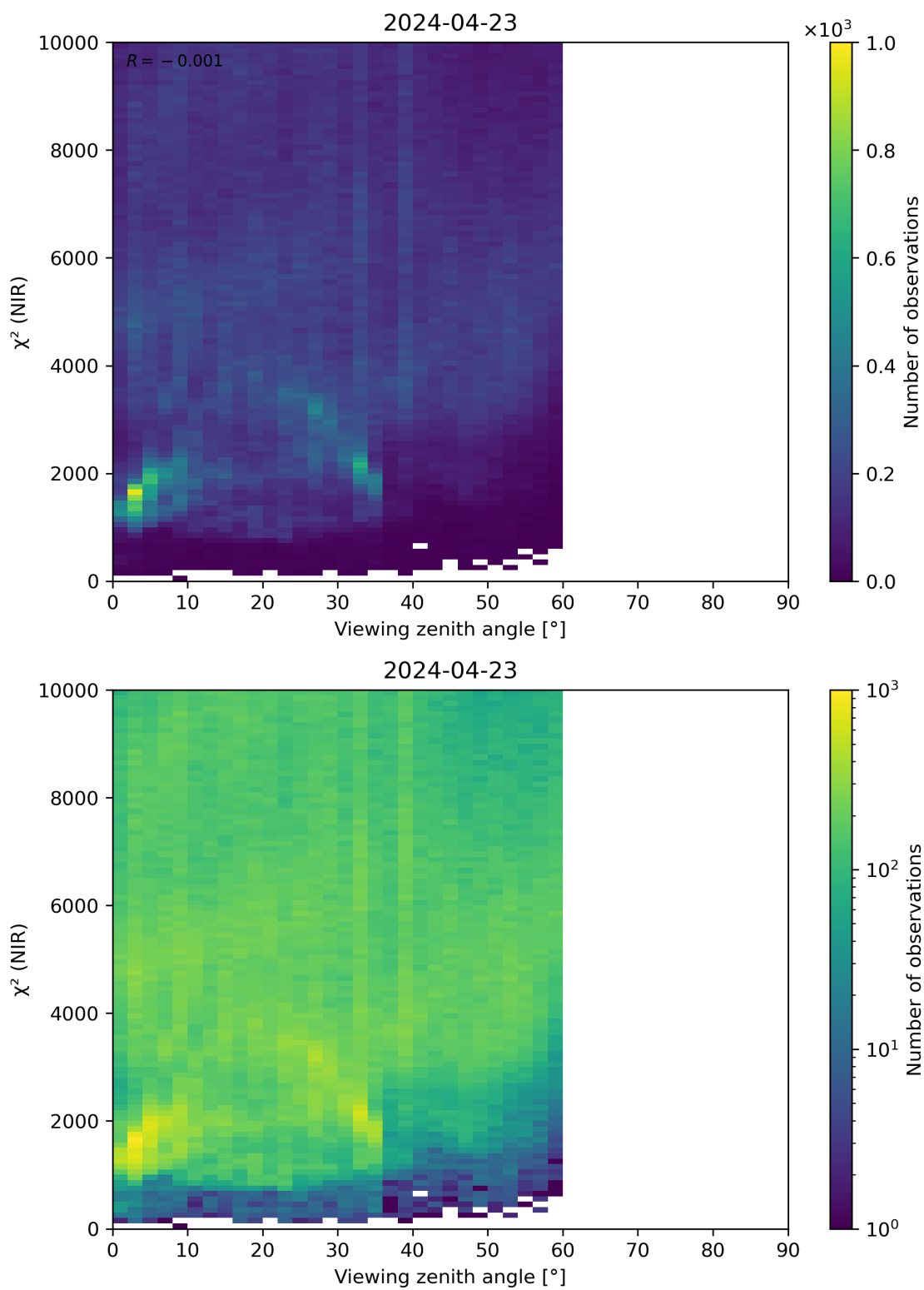
Figure 105: Scatter density plot of “Viewing zenith angle” against “ \chi^2 (NIR)” for 2024-04-22 to 2024-04-24.
