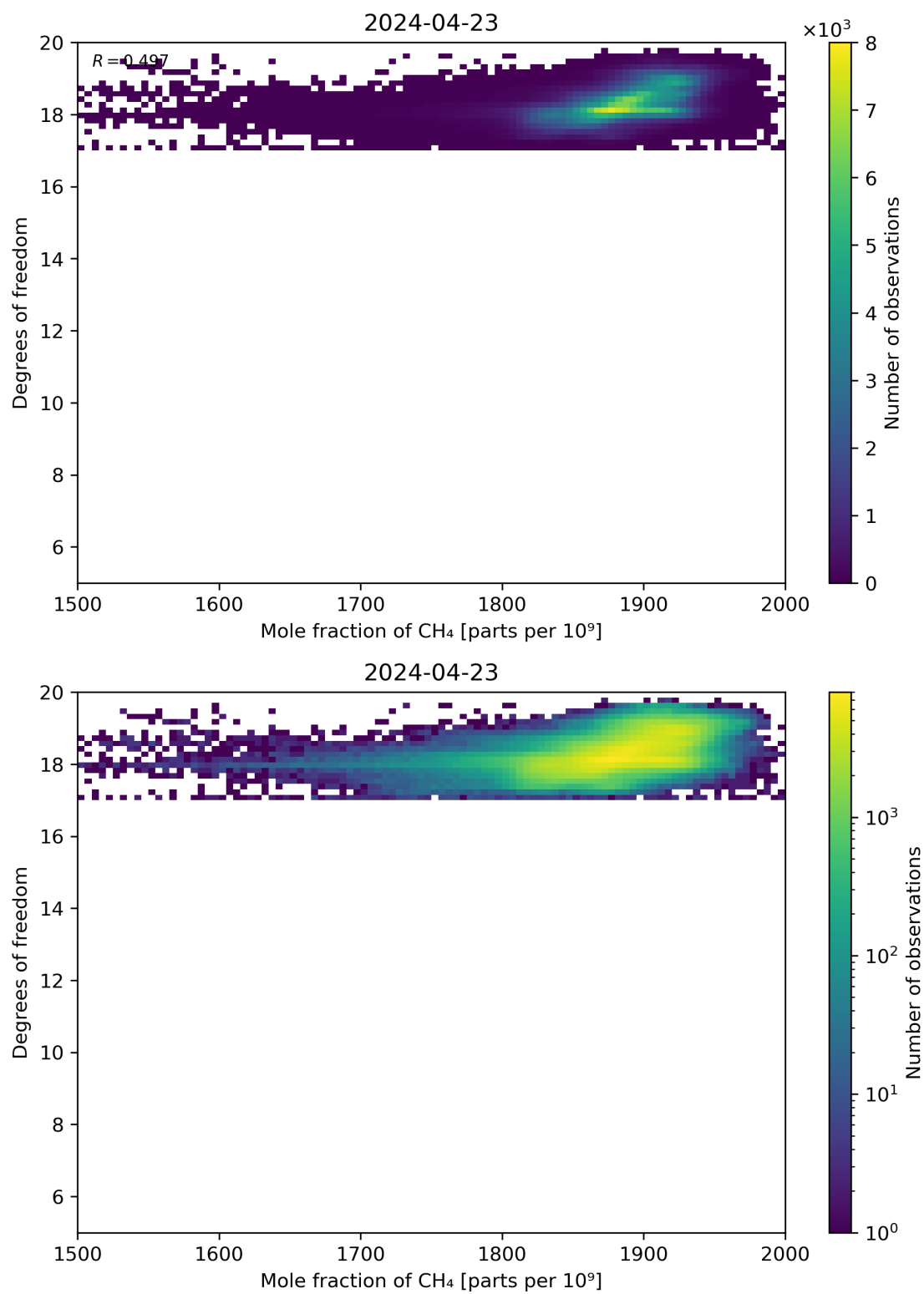
Figure 72: Scatter density plot of “Mole fraction of CH 4 ” against “Degrees of freedom” for 2024-04-22 to 2024-04-24.
