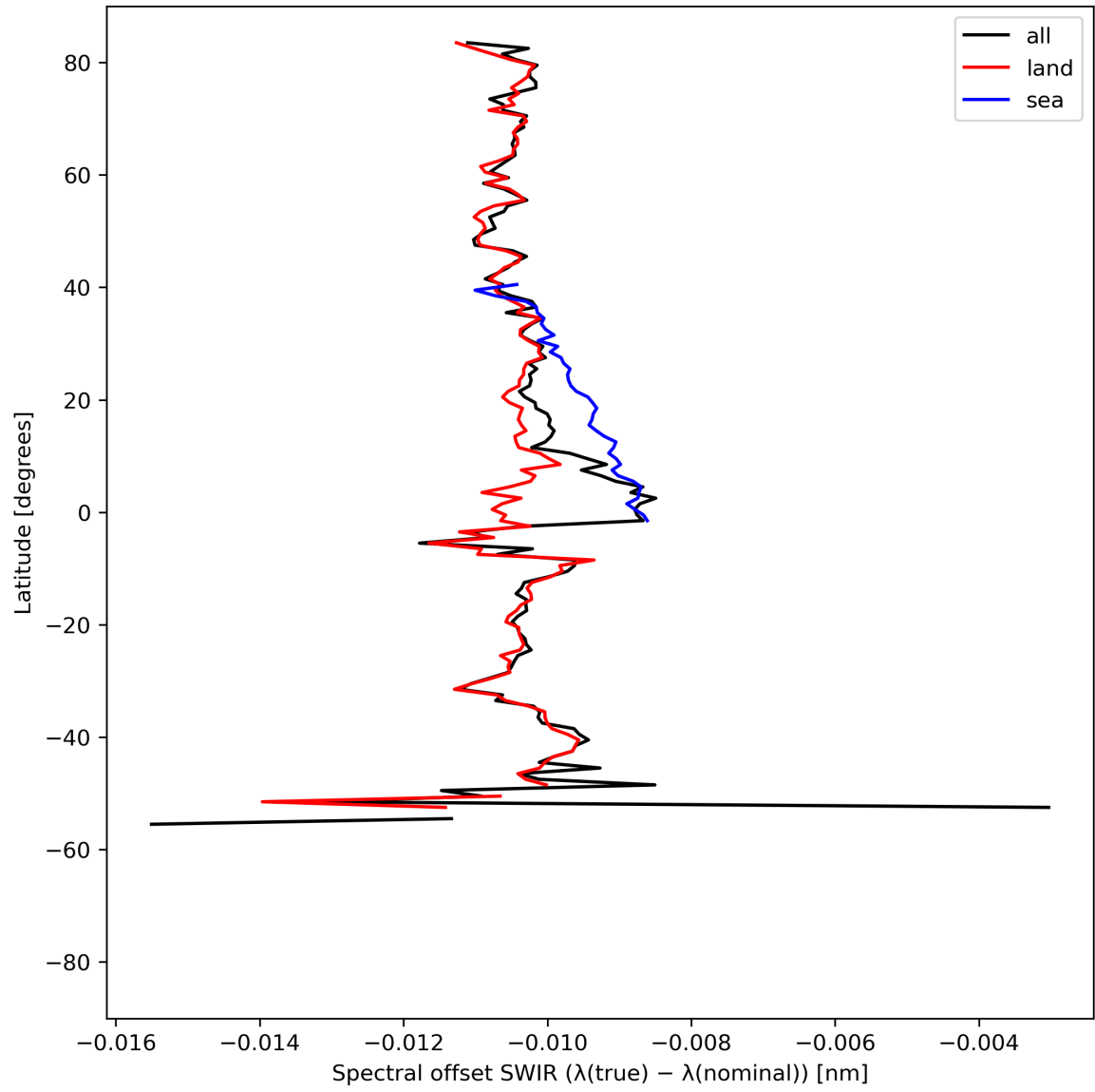
Figure 16: Zonal average of “Spectral offset SWIR ( \lambda(\text{true}) - \lambda(\text{nominal}) )” for 2024-04-22 to 2024-04-24.
