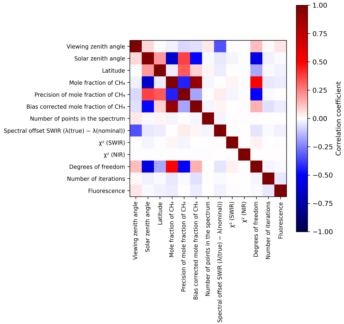
Figure 2: Map of correlation matrix for 2024-04-22 to 2024-04-24.
