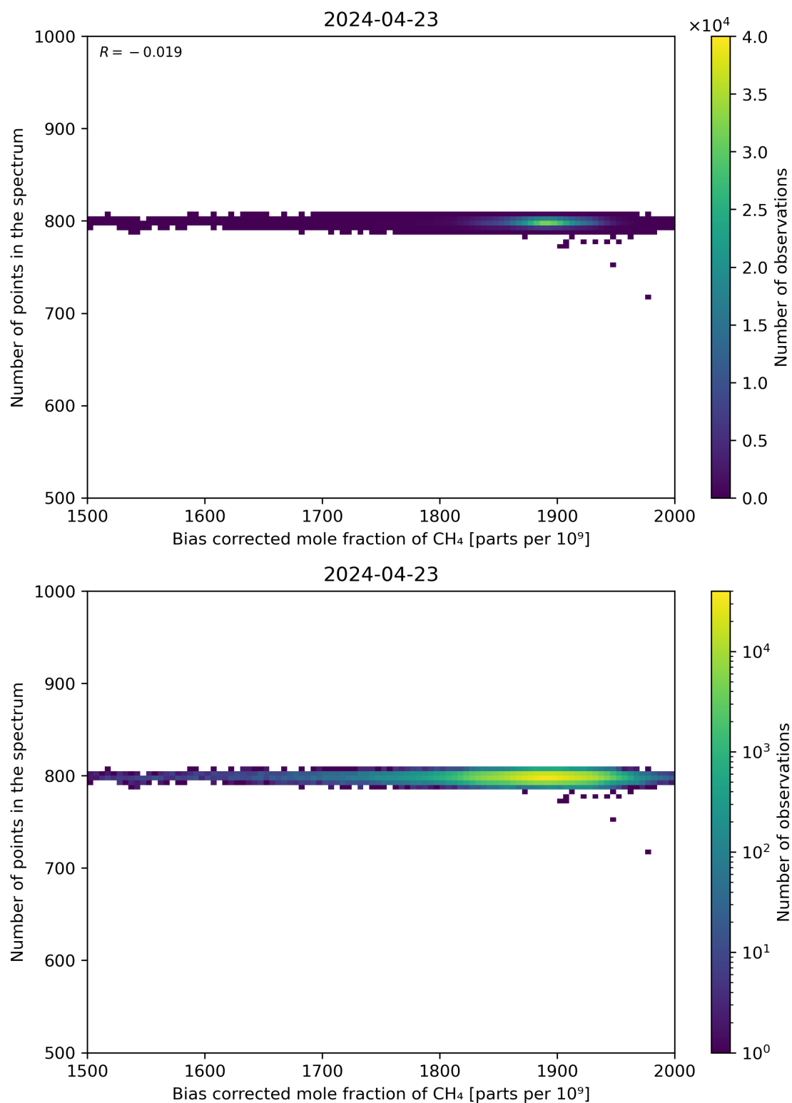
Figure 68: Scatter density plot of “Bias corrected mole fraction of CH 4 ” against “Number of points in the spectrum” for 2024-04-22 to 2024-04-24.
