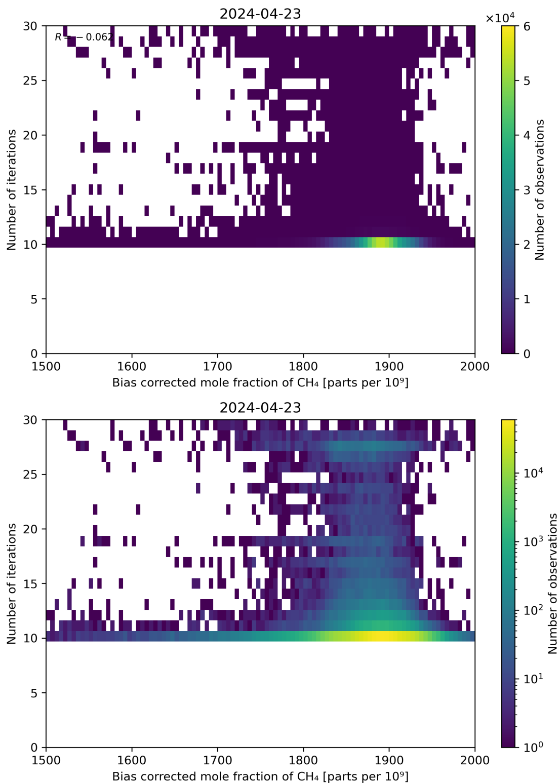
Figure 67: Scatter density plot of “Bias corrected mole fraction of CH 4 ” against “Number of iterations” for 2024-04-22 to 2024-04-24.
