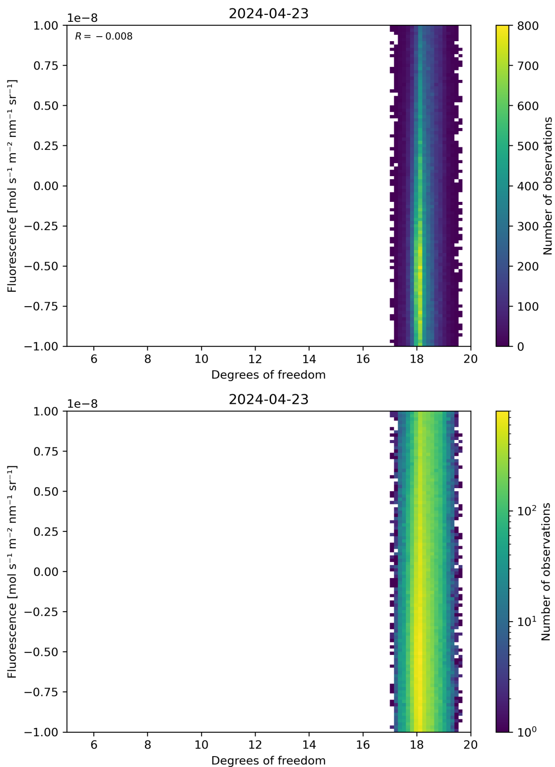
Figure 51: Scatter density plot of “Degrees of freedom” against “Fluorescence” for 2024-04-22 to 2024-04-24.
