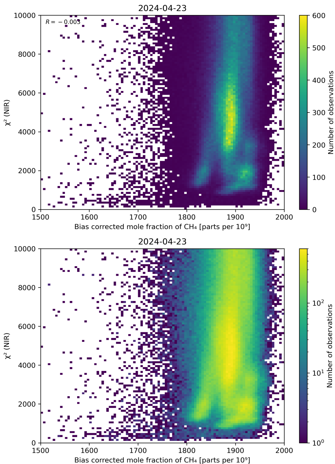
Figure 63: Scatter density plot of “Bias corrected mole fraction of CH 4 ” against “ \chi^2 (NIR)” for 2024-04-22 to 2024-04-24.
