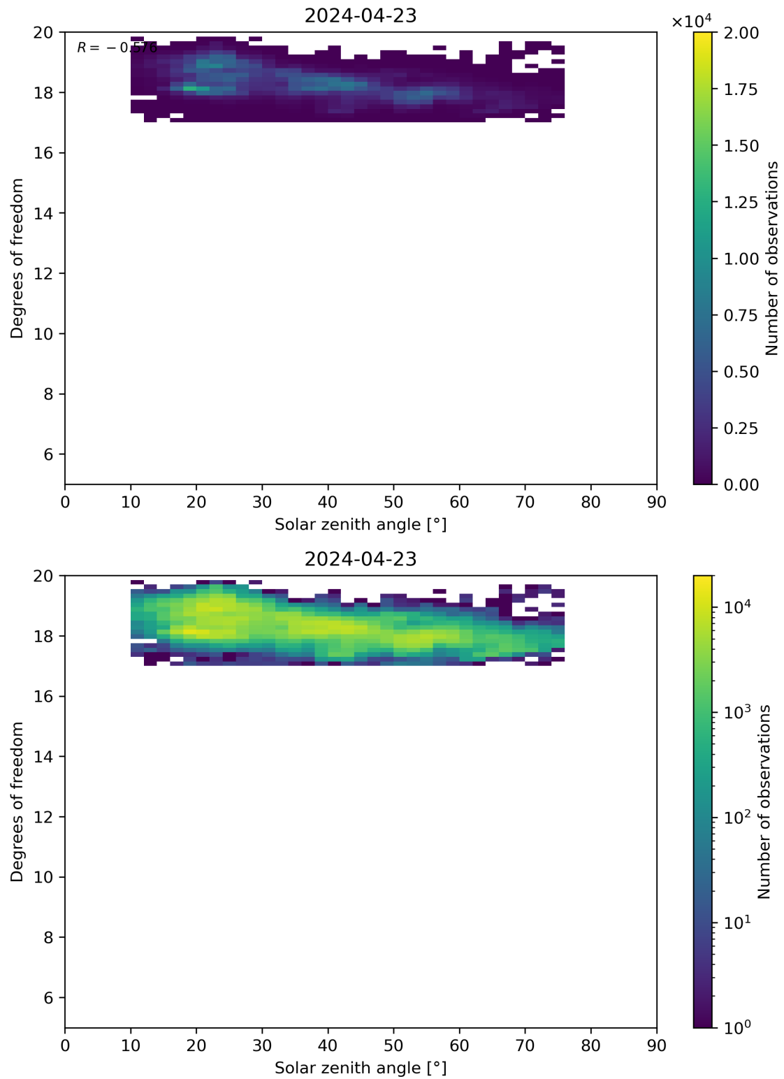
Figure 96: Scatter density plot of “Solar zenith angle” against “Degrees of freedom” for 2024-04-22 to 2024-04-24.
