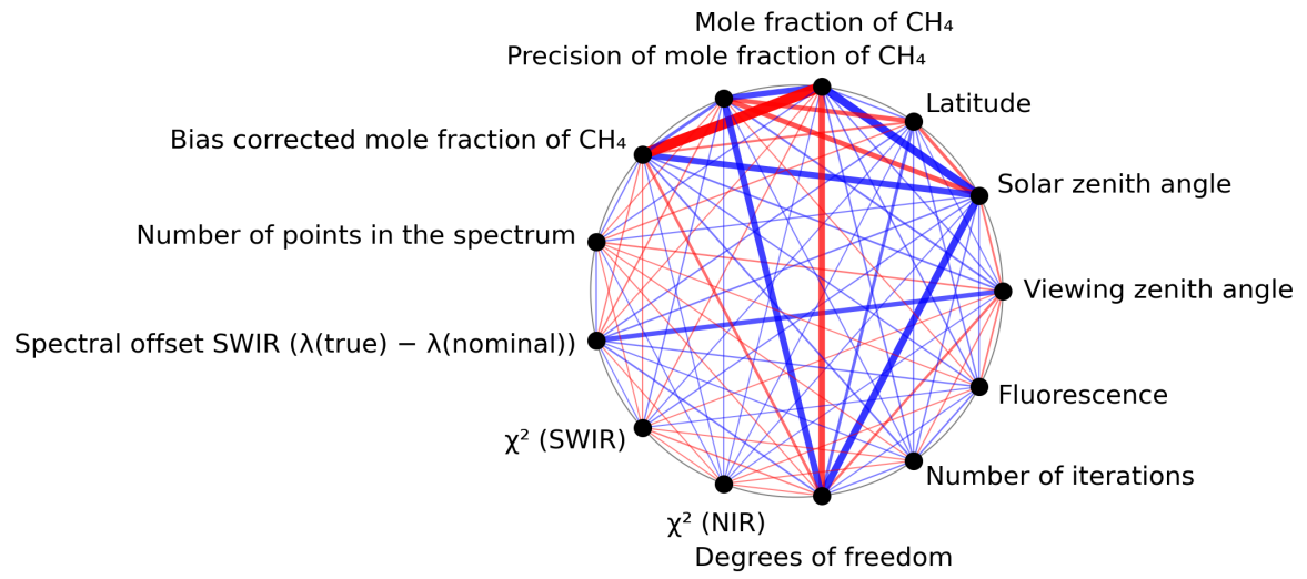
Figure 1: Map of correlation graph for 2024-04-22 to 2024-04-24.
