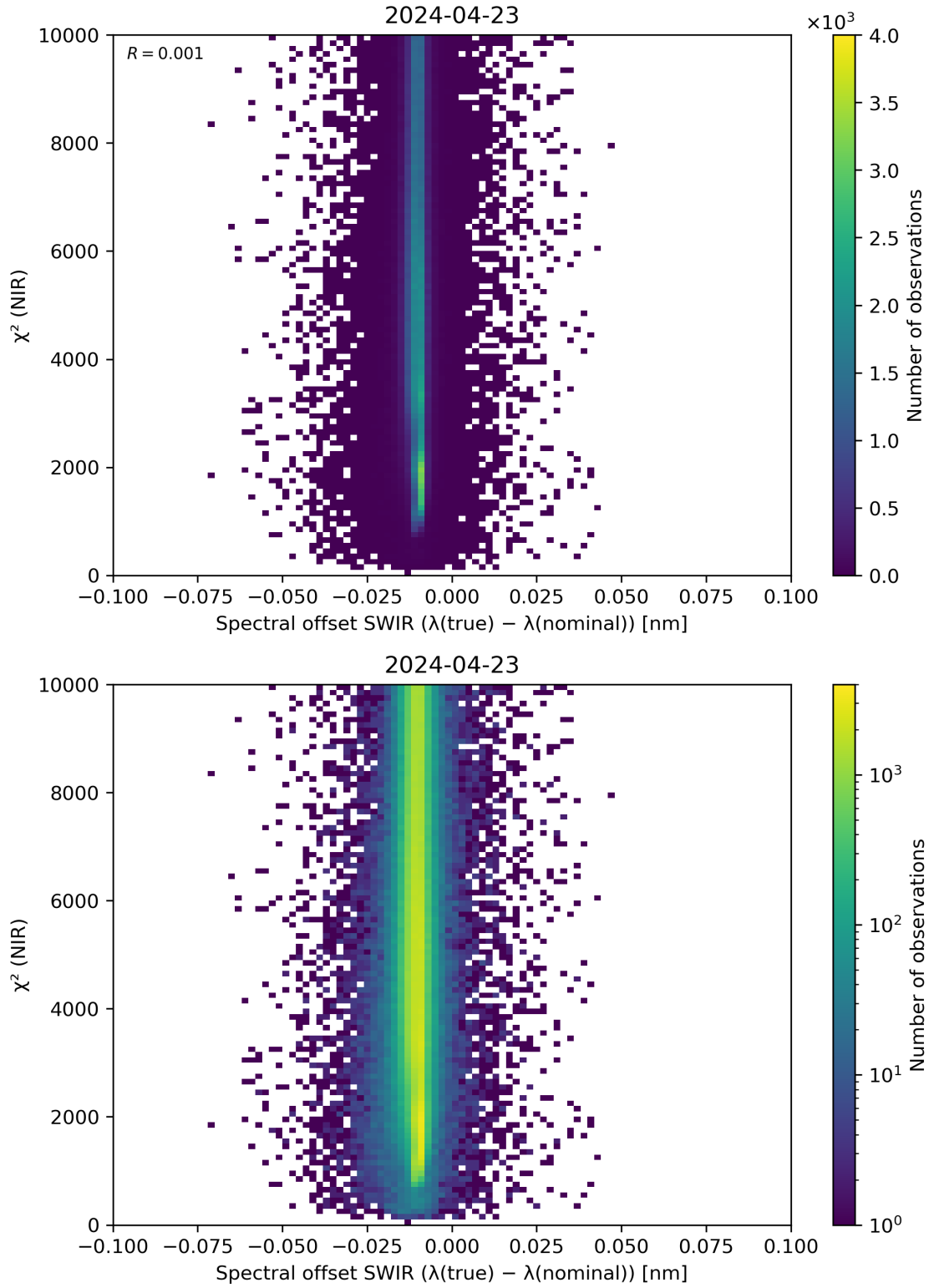
Figure 117: Scatter density plot of “Spectral offset SWIR ( \lambda(\text{true}) - \lambda(\text{nominal}) )” against “ \chi^2 (NIR)” for 2024-04-22 to 2024-04-24.
