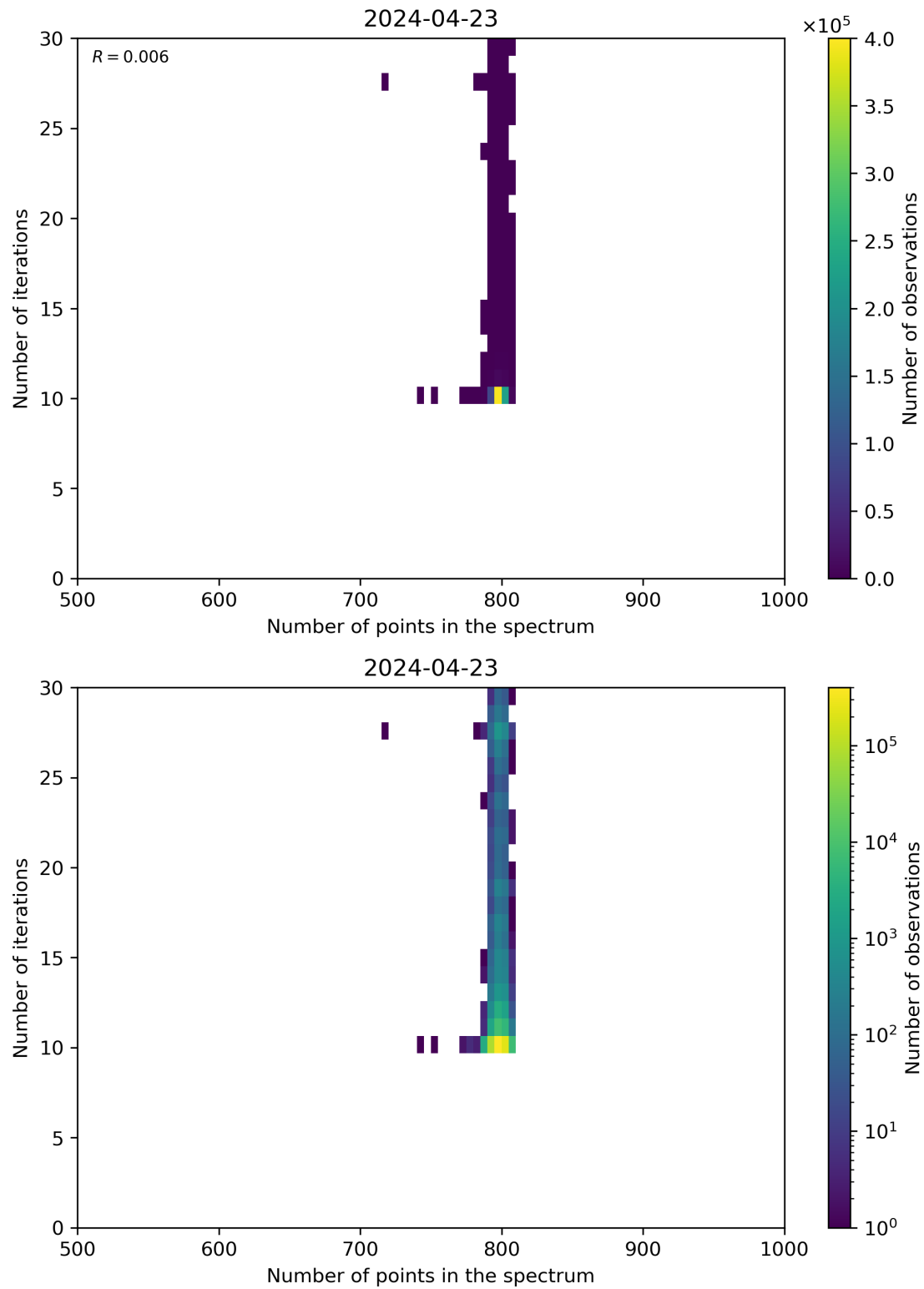
Figure 92: Scatter density plot of “Number of points in the spectrum” against “Number of iterations” for 2024-04-22 to 2024-04-24.
