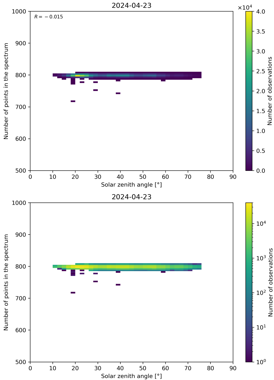
Figure 103: Scatter density plot of “Solar zenith angle” against “Number of points in the spectrum” for 2024-04-22 to 2024-04-24.
