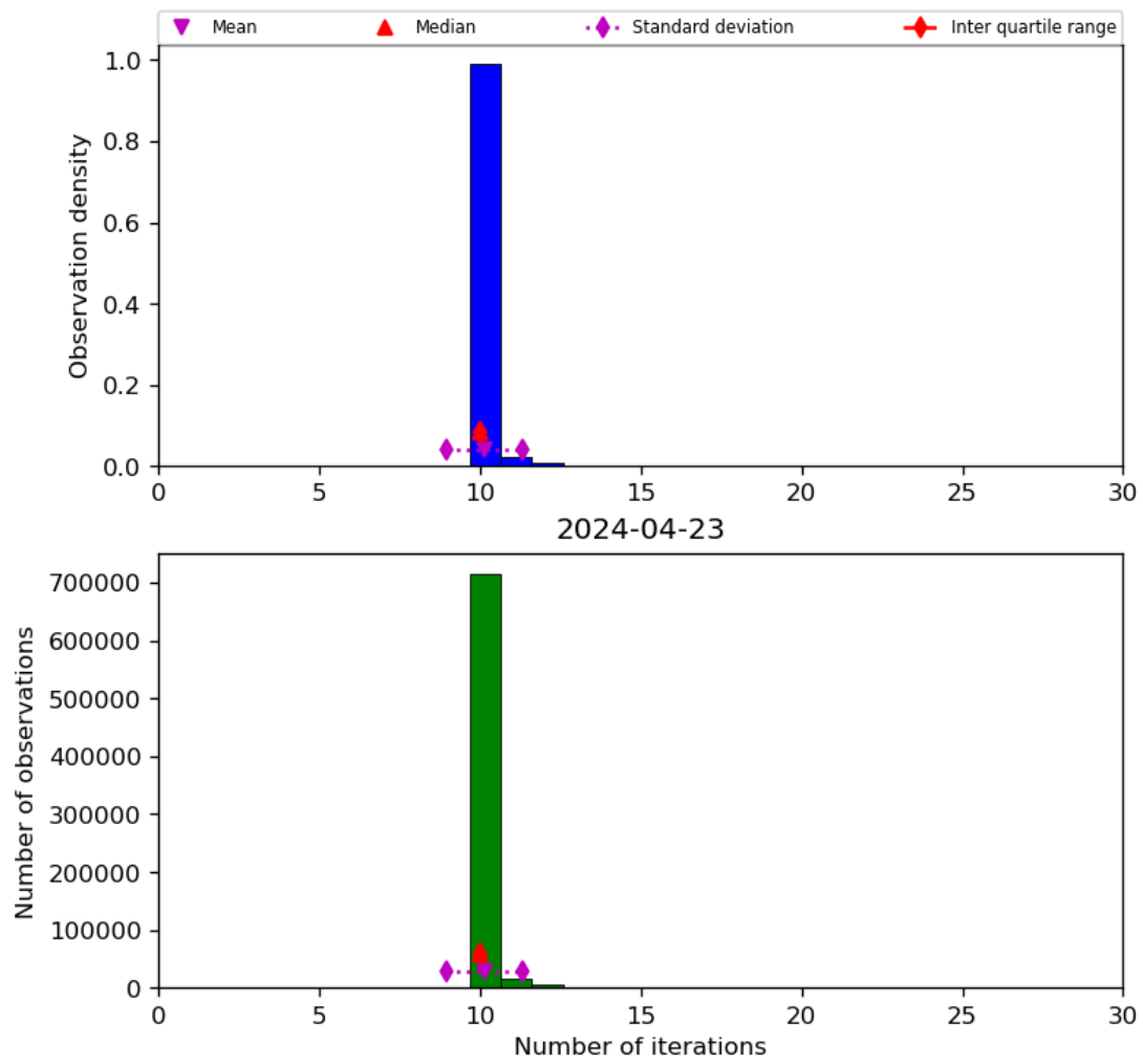
Figure 31: Histogram of “Number of iterations” for 2024-04-22 to 2024-04-24
