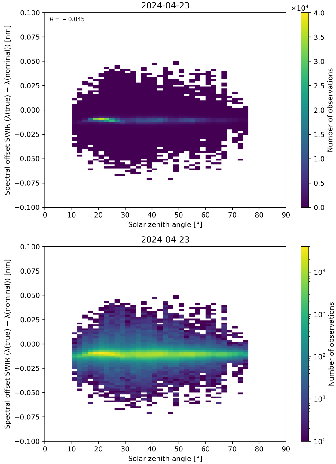
Figure 104: Scatter density plot of “Solar zenith angle” against “Spectral offset SWIR ( \lambda(\text{true}) - \lambda(\text{nominal}) )” for 2024-04-22 to 2024-04-24.
