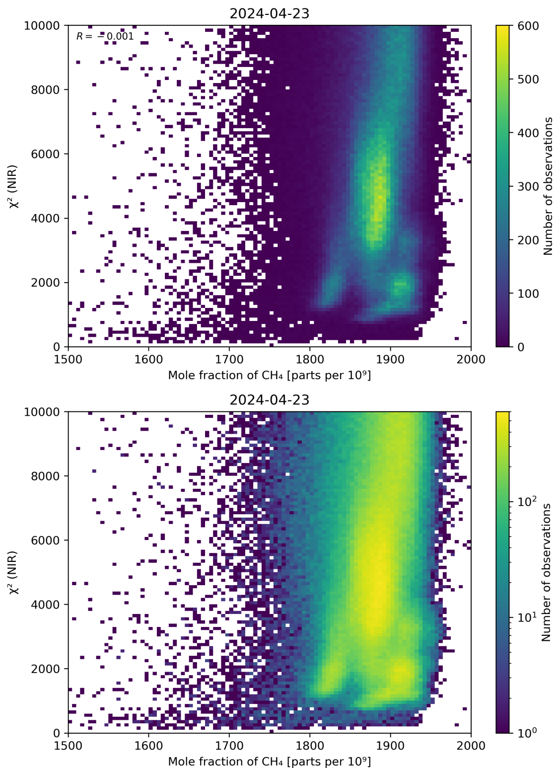
Figure 70: Scatter density plot of “Mole fraction of \text{CH}_4 ” against “ \chi^2 (NIR)” for 2024-04-22 to 2024-04-24.
