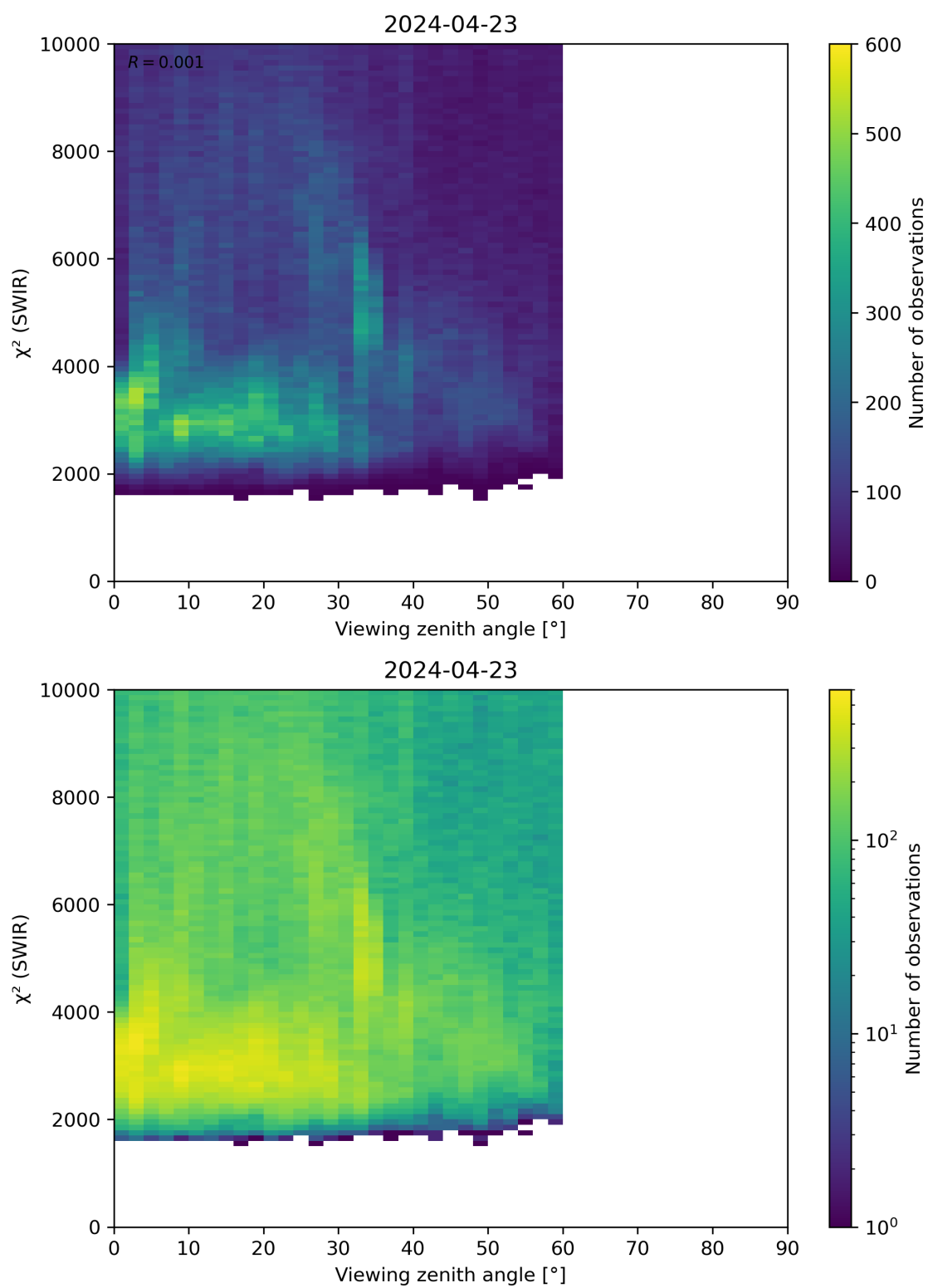
Figure 106: Scatter density plot of “Viewing zenith angle” against “ \chi^2 (SWIR)” for 2024-04-22 to 2024-04-24.
