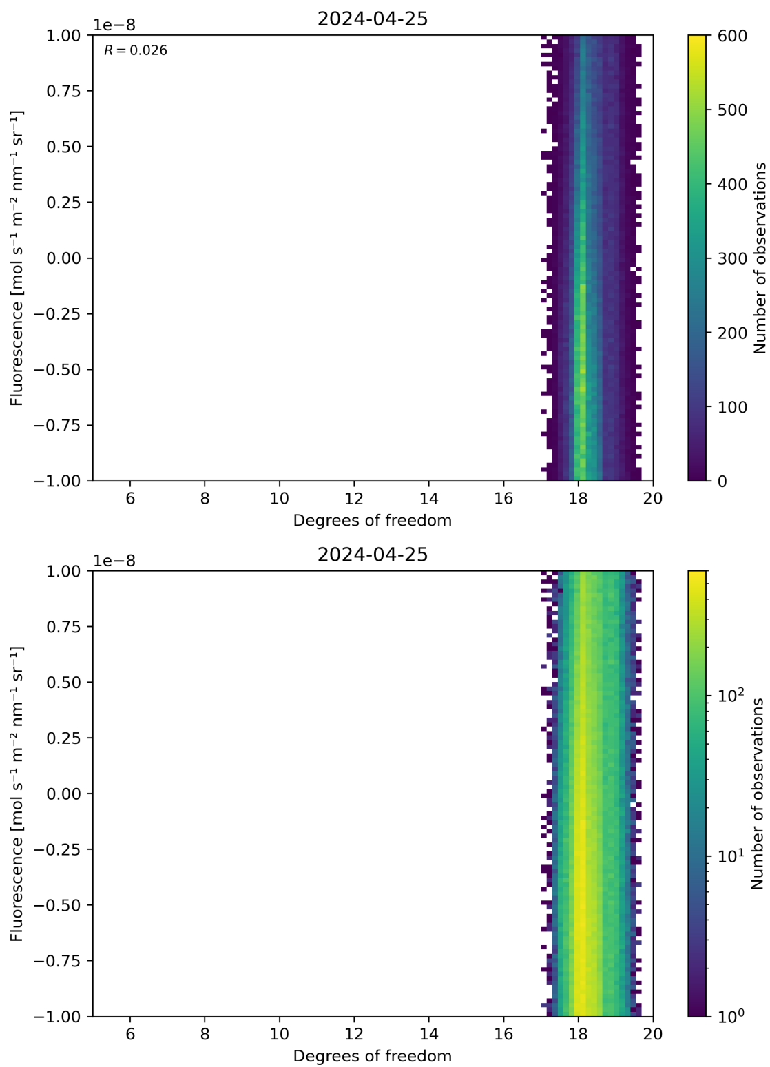
Figure 51: Scatter density plot of “Degrees of freedom” against “Fluorescence” for 2024-04-24 to 2024-04-26.
