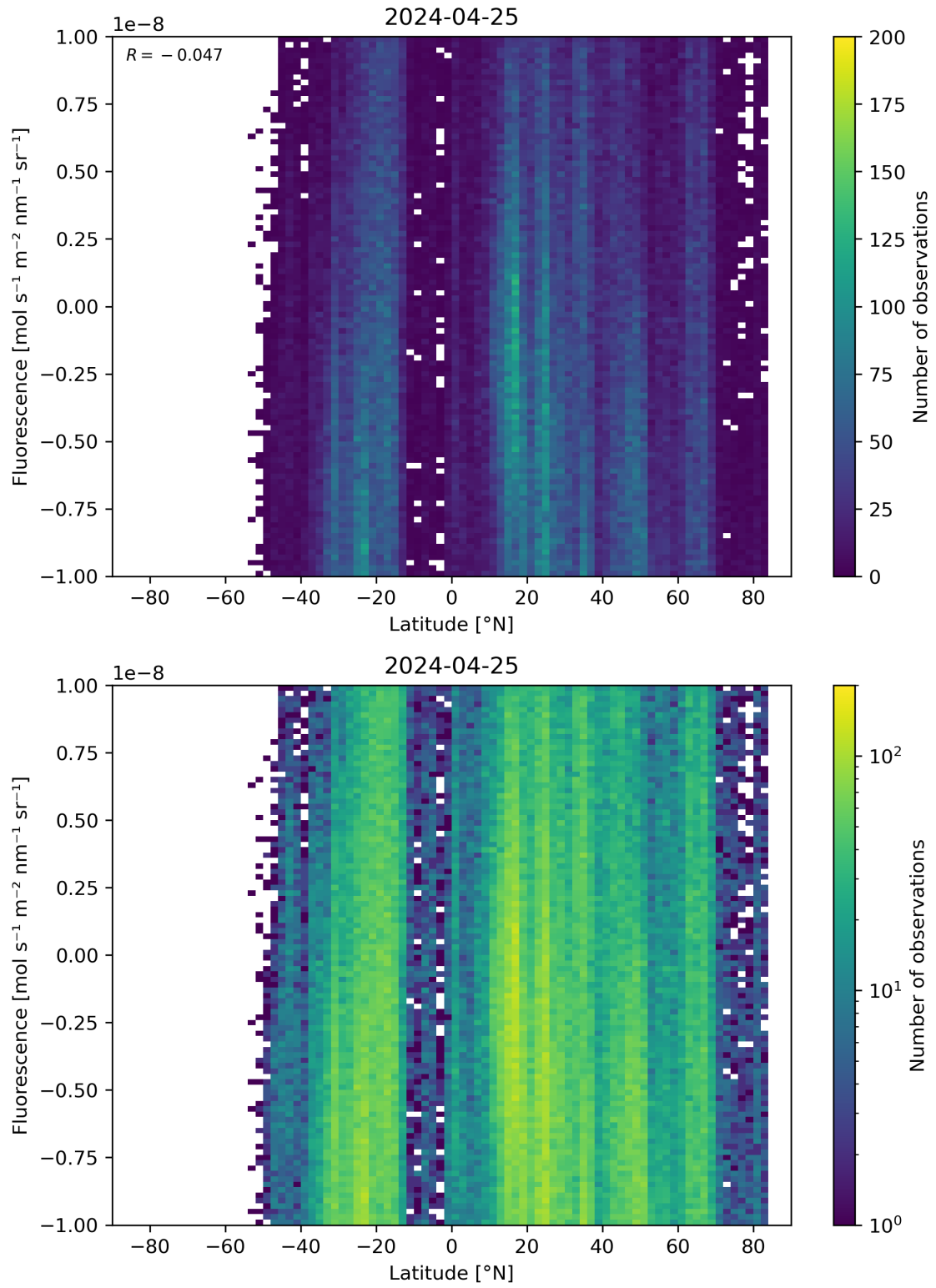
Figure 56: Scatter density plot of “Latitude” against “Fluorescence” for 2024-04-24 to 2024-04-26.
