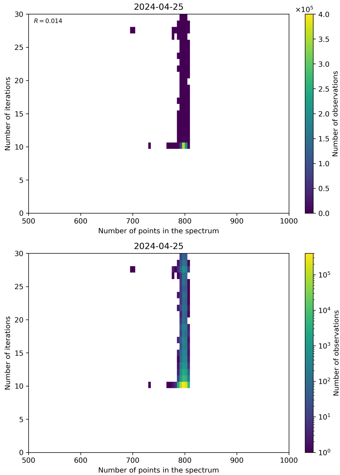
Figure 92: Scatter density plot of “Number of points in the spectrum” against “Number of iterations” for 2024-04-24 to 2024-04-26.
