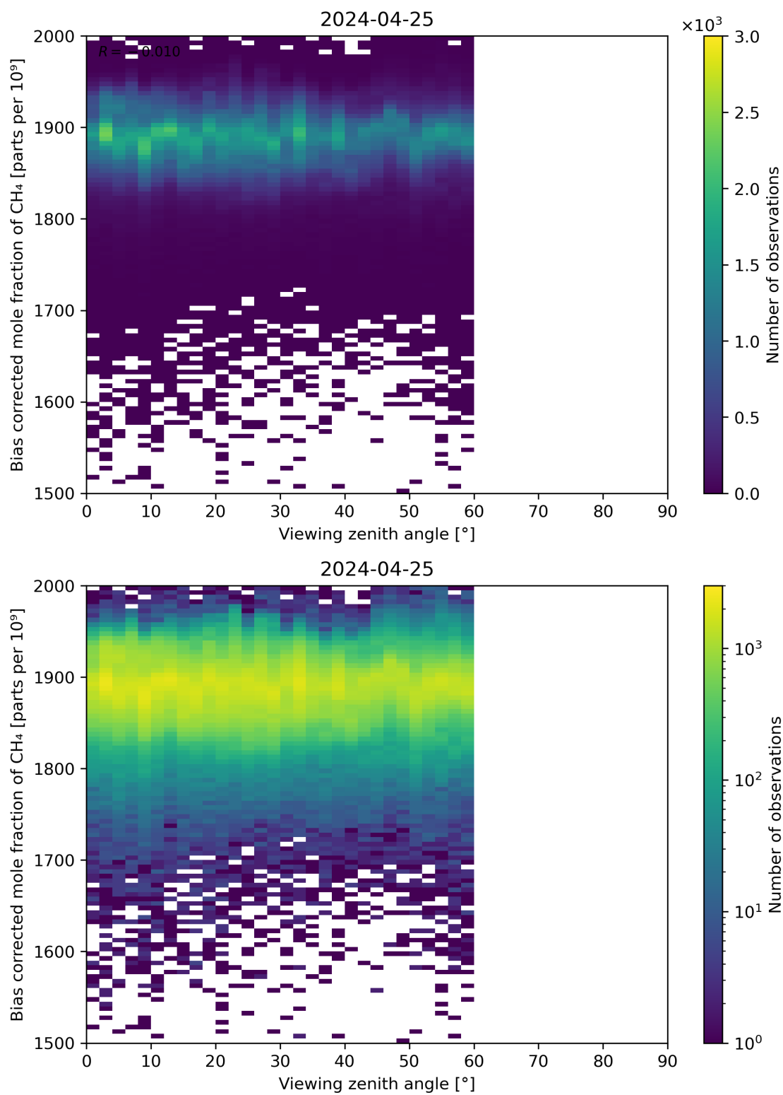
Figure 111: Scatter density plot of “Viewing zenith angle” against “Bias corrected mole fraction of CH 4 ” for 2024-04-24 to 2024-04-26.
