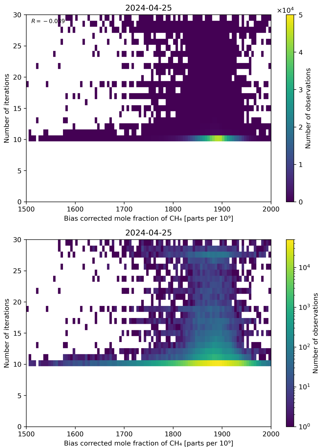
Figure 67: Scatter density plot of “Bias corrected mole fraction of \text{CH}_4 ” against “Number of iterations” for 2024-04-24 to 2024-04-26.
