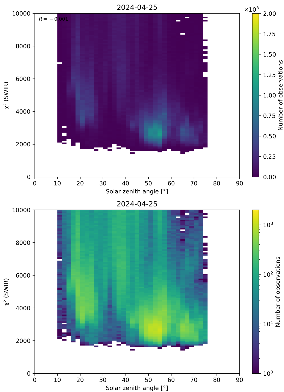
Figure 95: Scatter density plot of “Solar zenith angle” against “ \chi^2 (SWIR)” for 2024-04-24 to 2024-04-26.
