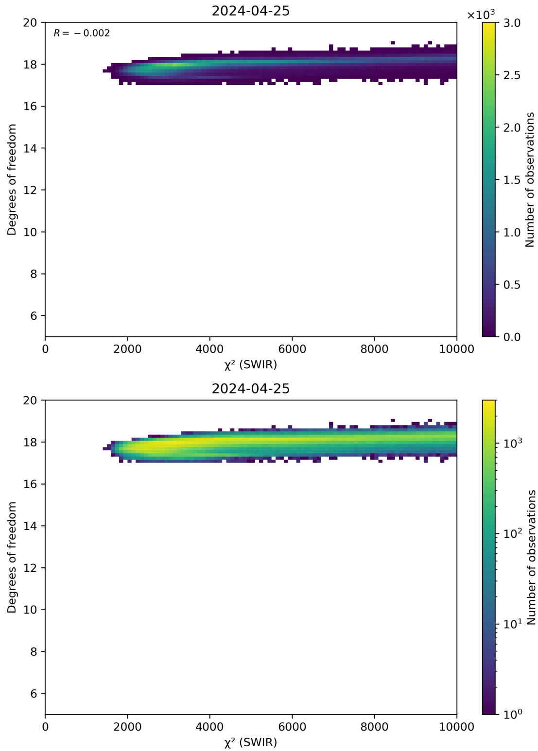
Figure 48: Scatter density plot of “ \chi^2 (SWIR)” against “Degrees of freedom” for 2024-04-24 to 2024-04-26.
