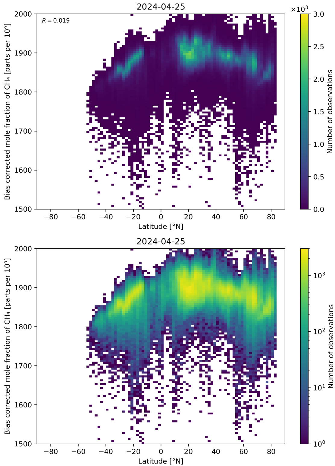
Figure 58: Scatter density plot of “Latitude” against “Bias corrected mole fraction of \text{CH}_4 ” for 2024-04-24 to 2024-04-26.
