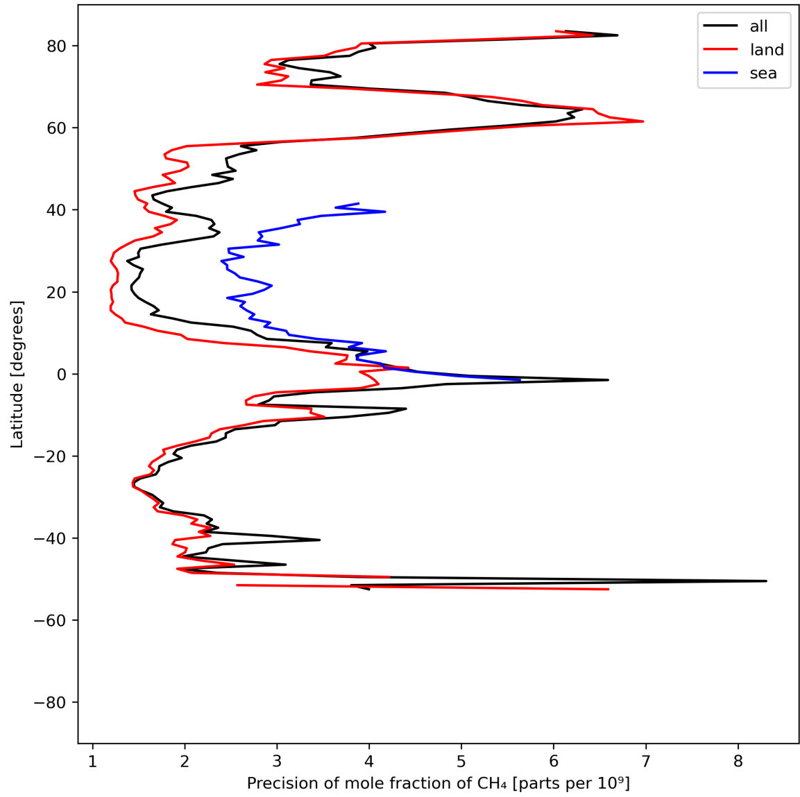
Figure 13: Zonal average of “Precision of mole fraction of CH 4 ” for 2024-04-24 to 2024-04-26.
