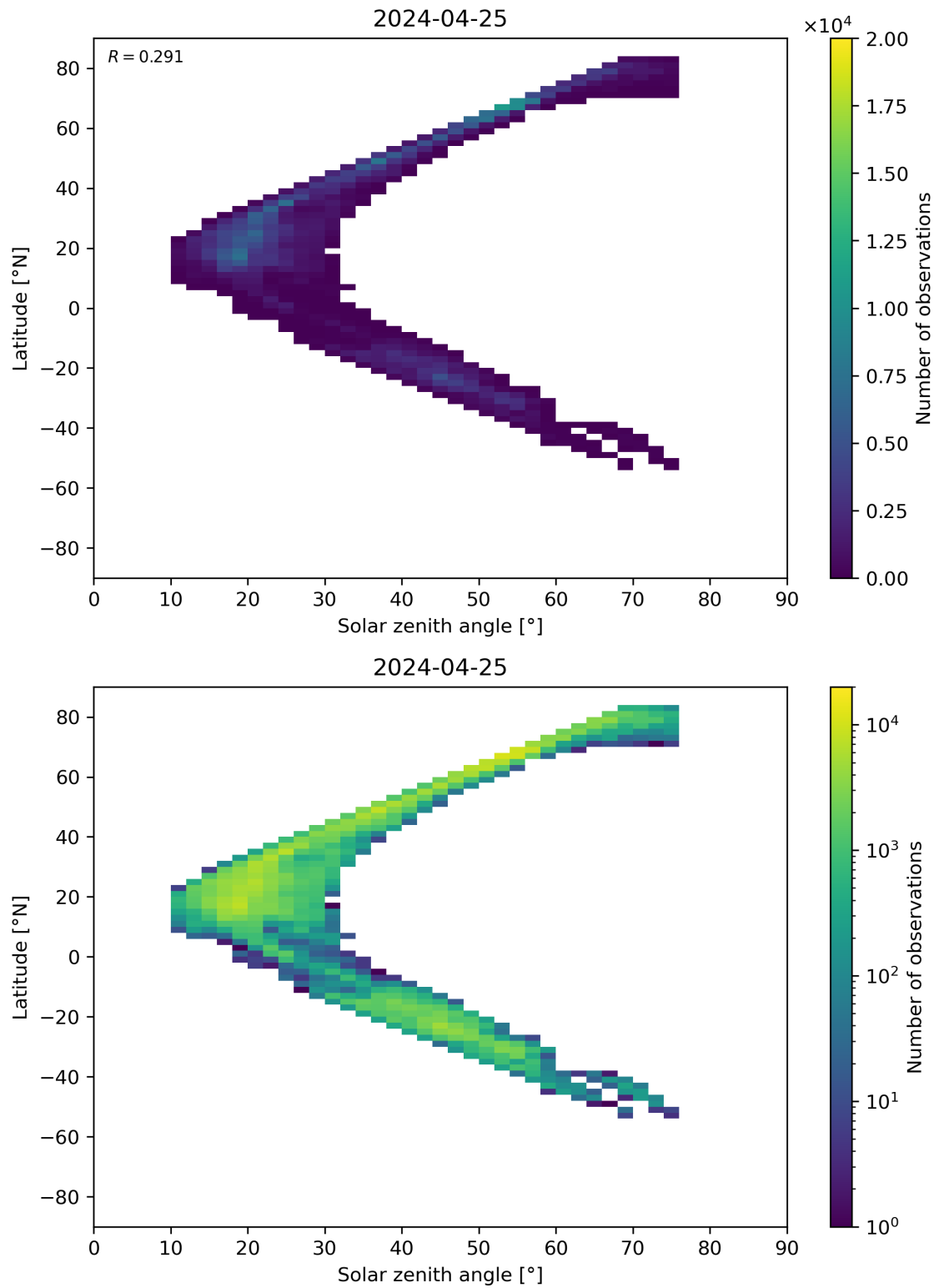
Figure 98: Scatter density plot of “Solar zenith angle” against “Latitude” for 2024-04-24 to 2024-04-26.
