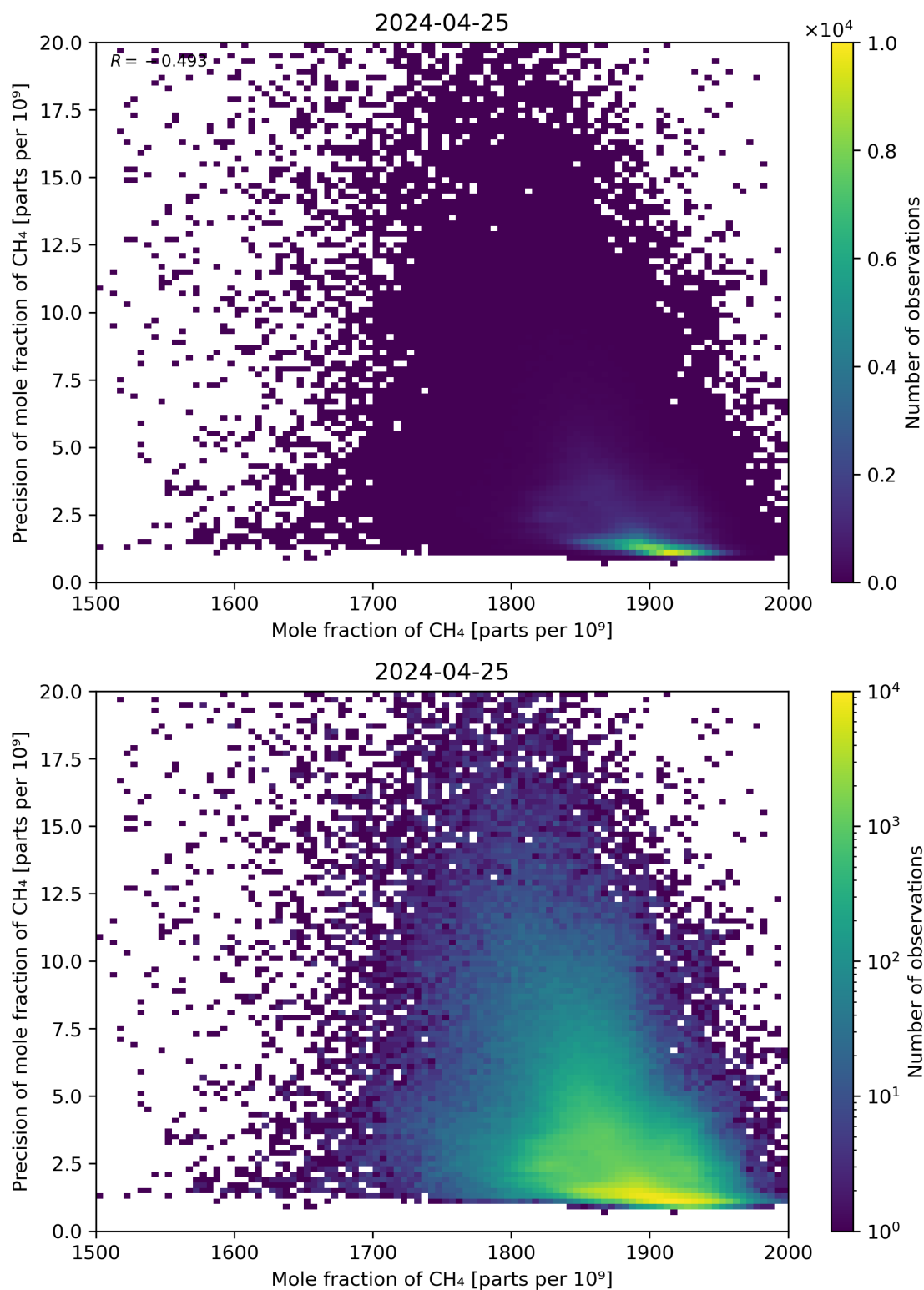
Figure 75: Scatter density plot of “Mole fraction of CH 4 ” against “Precision of mole fraction of CH 4 ” for 2024-04-24 to 2024-04-26.
