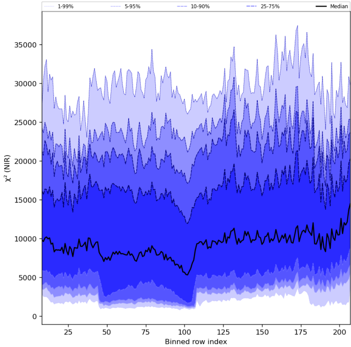
Figure 40: Along track statistics of " \chi^2 (NIR)" for 2024-04-24 to 2024-04-26
