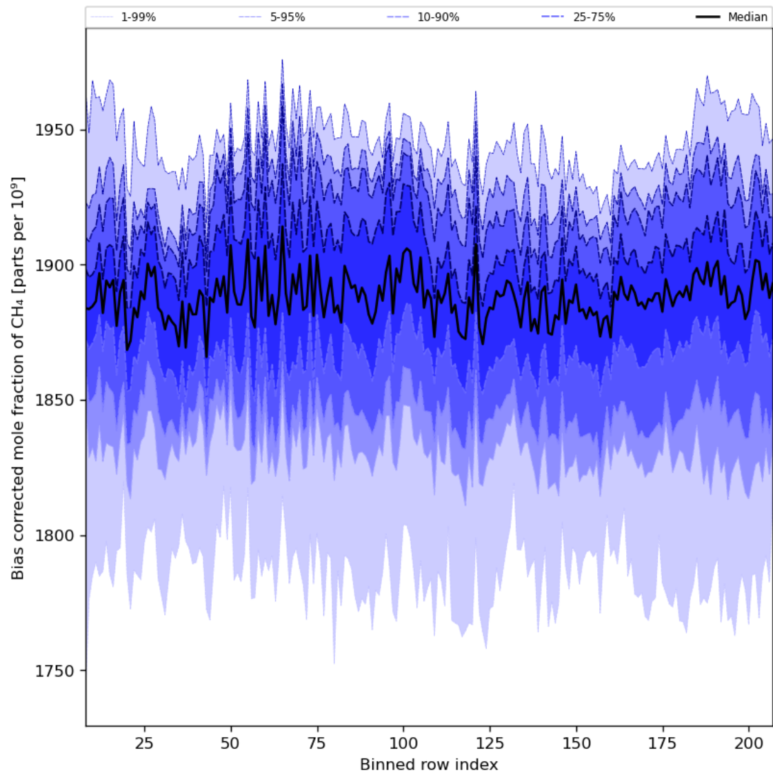
Figure 36: Along track statistics of “Bias corrected mole fraction of CH 4 ” for 2024-04-24 to 2024-04-26
