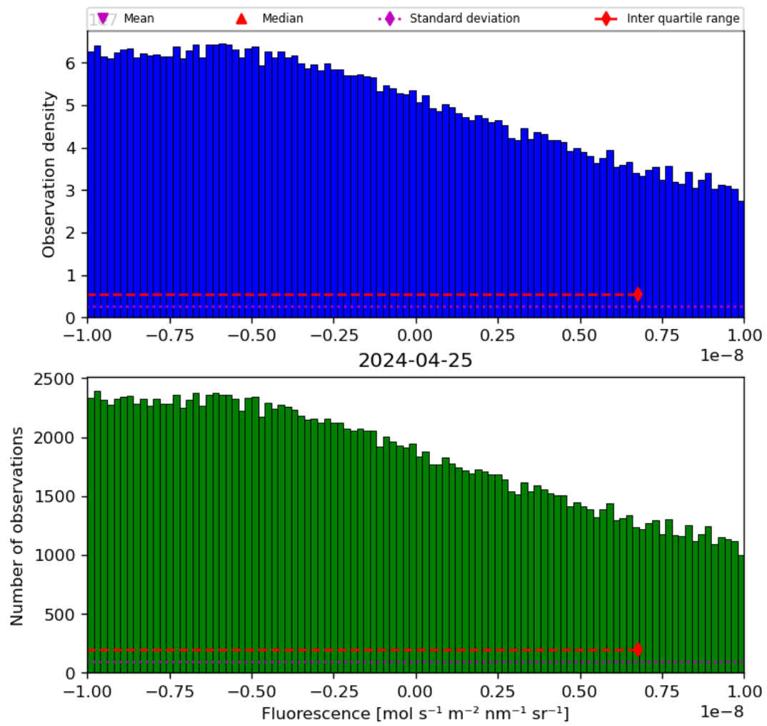
Figure 32: Histogram of “Fluorescence” for 2024-04-24 to 2024-04-26
