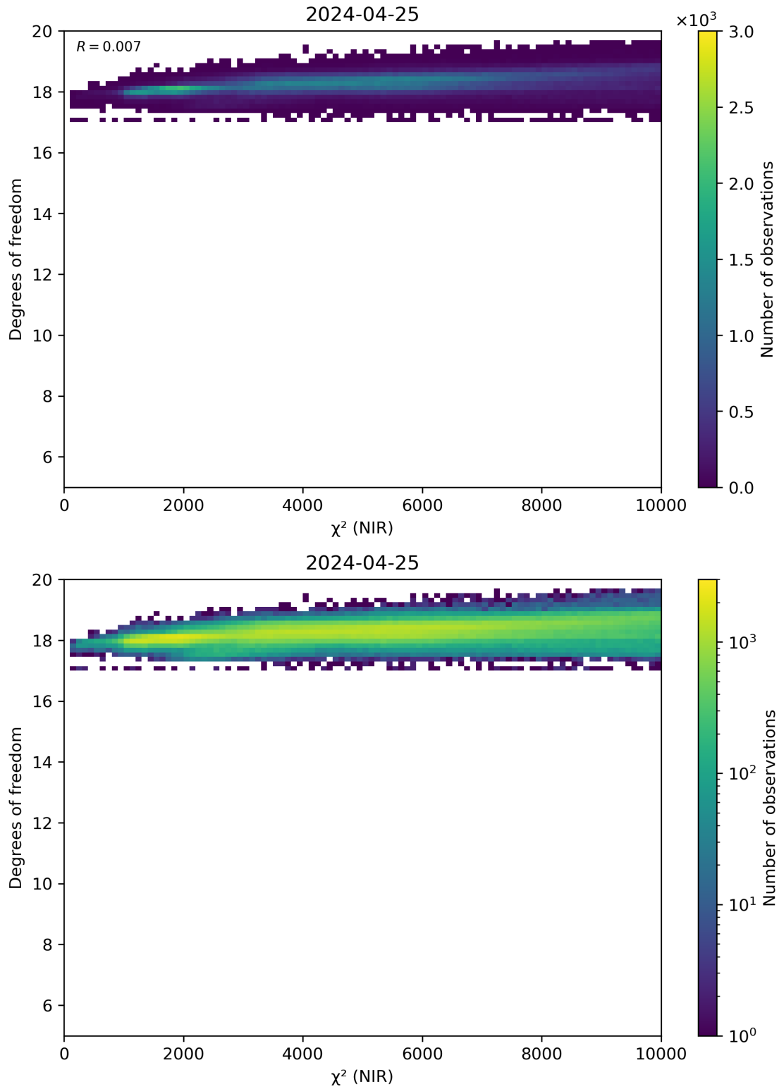
Figure 44: Scatter density plot of “ \chi^2 (NIR)” against “Degrees of freedom” for 2024-04-24 to 2024-04-26.
