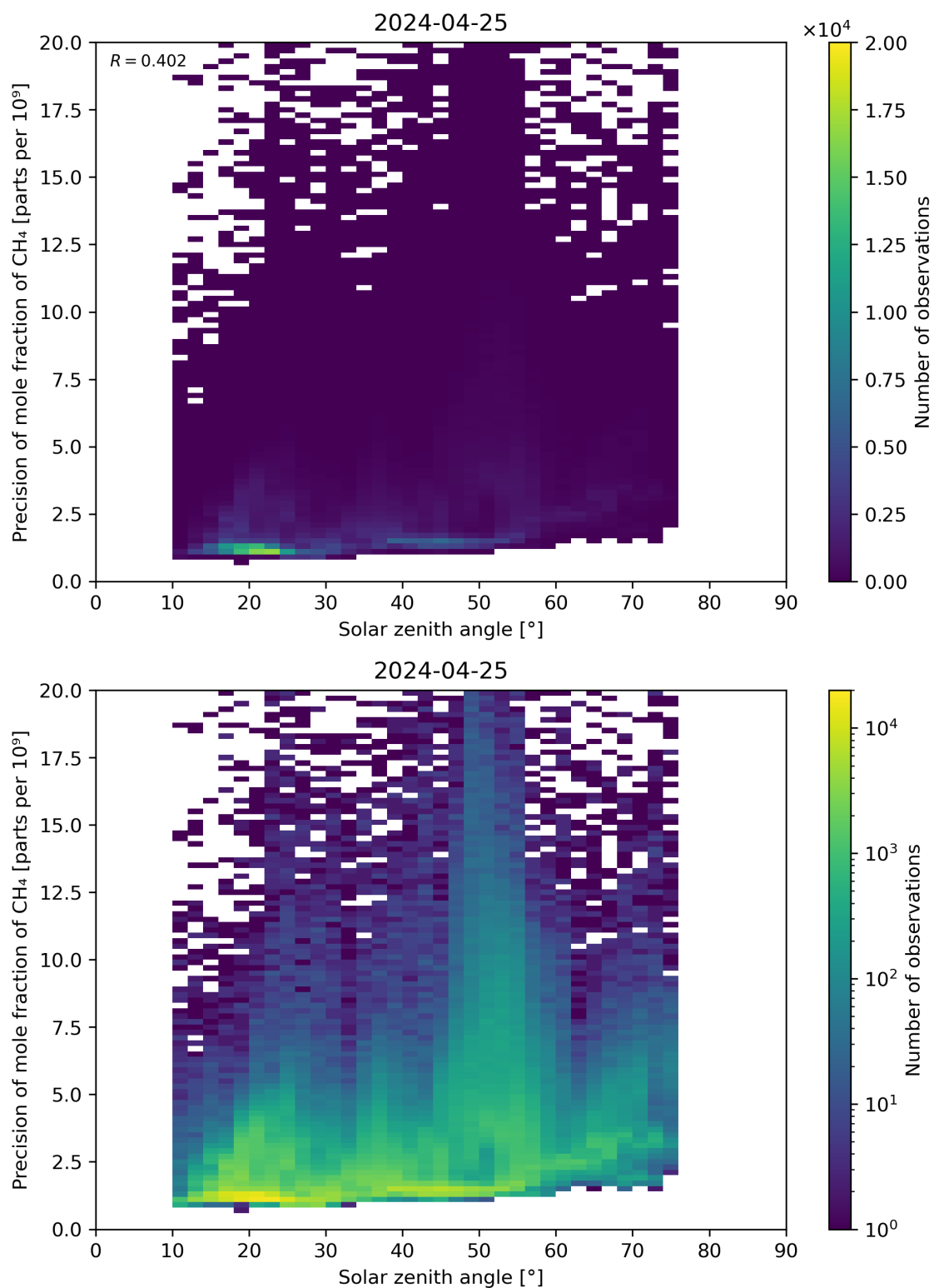
Figure 101: Scatter density plot of “Solar zenith angle” against “Precision of mole fraction of CH 4 ” for 2024-04-24 to 2024-04-26.
