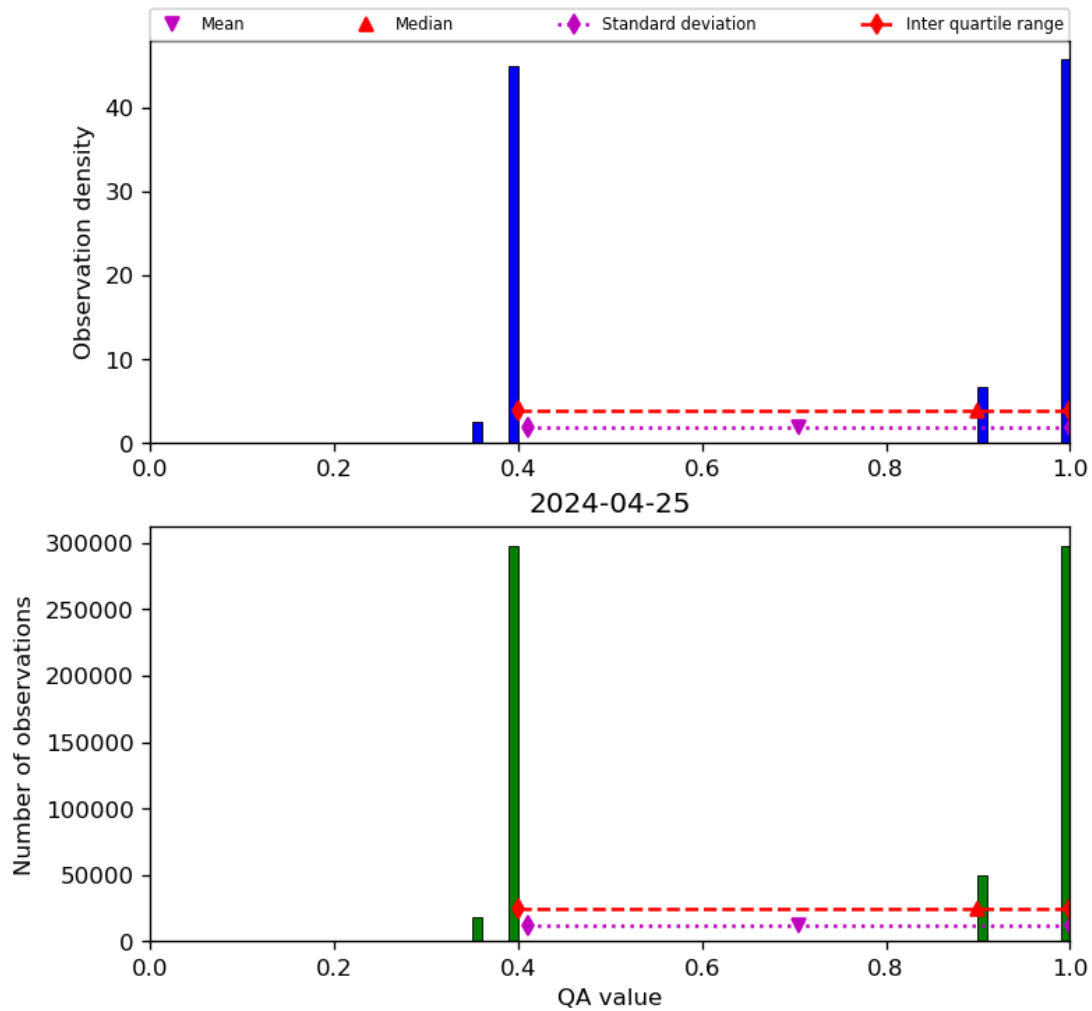
Figure 22: Histogram of “QA value” for 2024-04-24 to 2024-04-26
