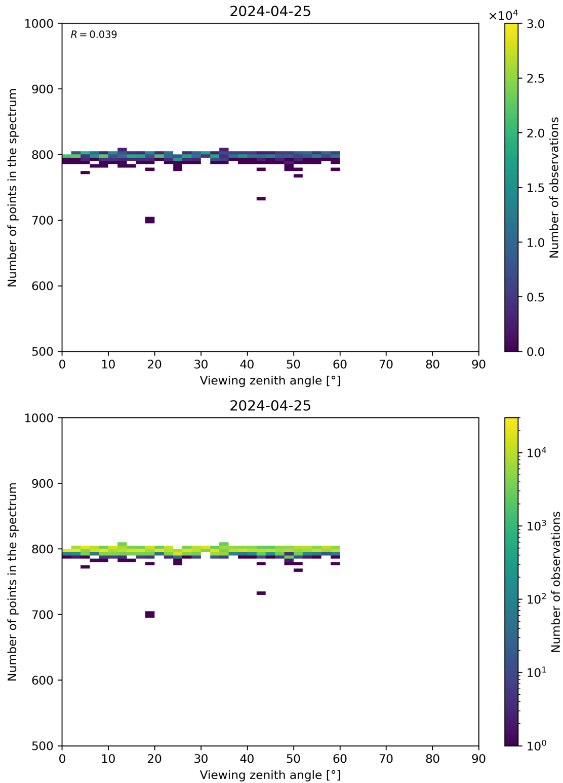
Figure 114: Scatter density plot of “Viewing zenith angle” against “Number of points in the spectrum” for 2024-04-24 to 2024-04-26.
