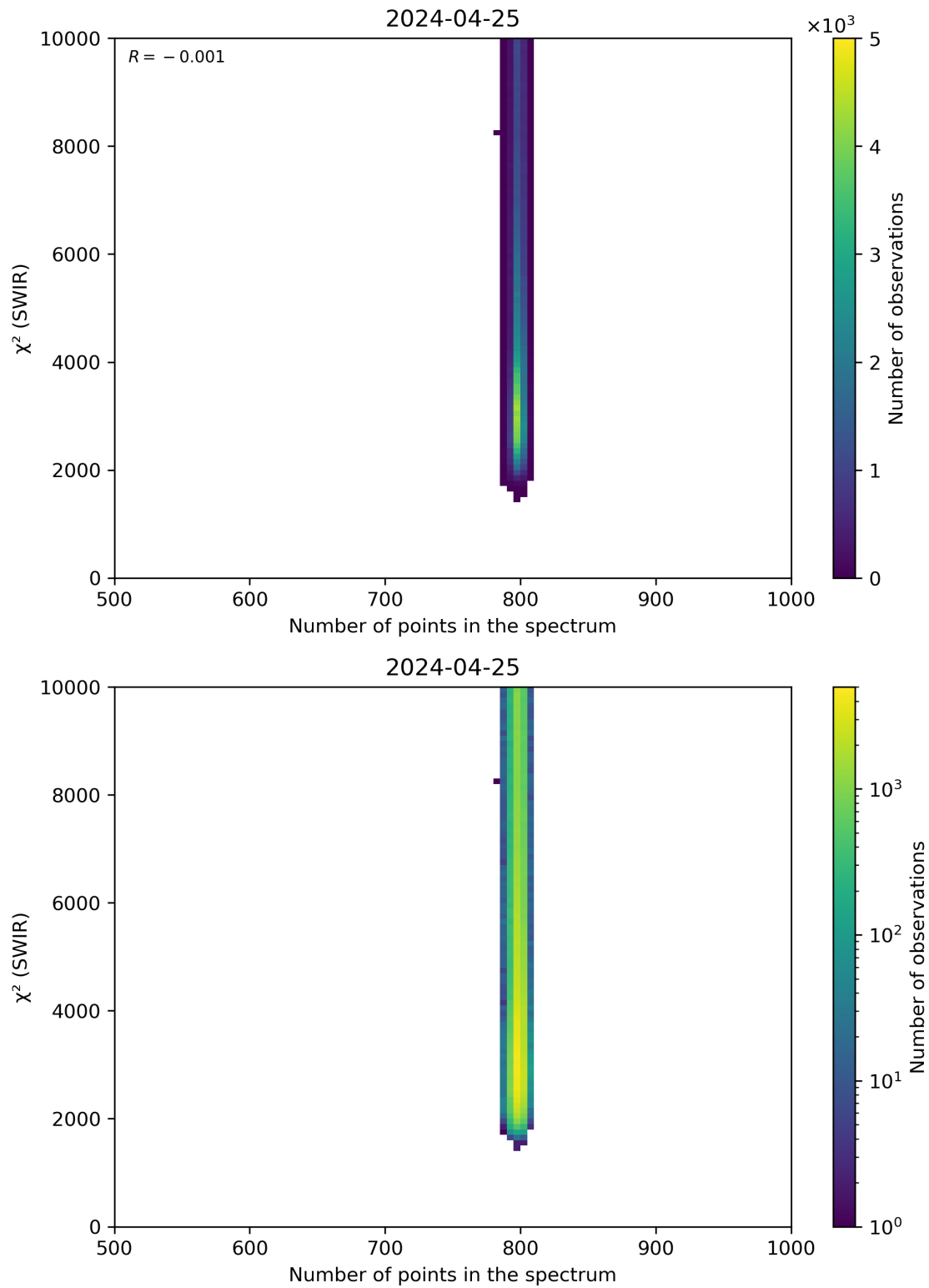
Figure 89: Scatter density plot of “Number of points in the spectrum” against “ \chi^2 (SWIR)” for 2024-04-24 to 2024-04-26.
