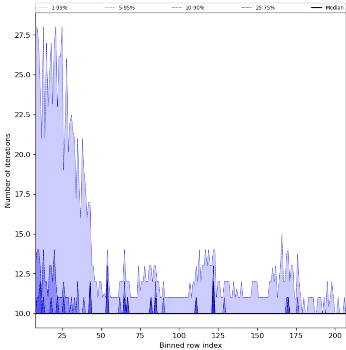
Figure 42: Along track statistics of “Number of iterations” for 2024-04-24 to 2024-04-26
