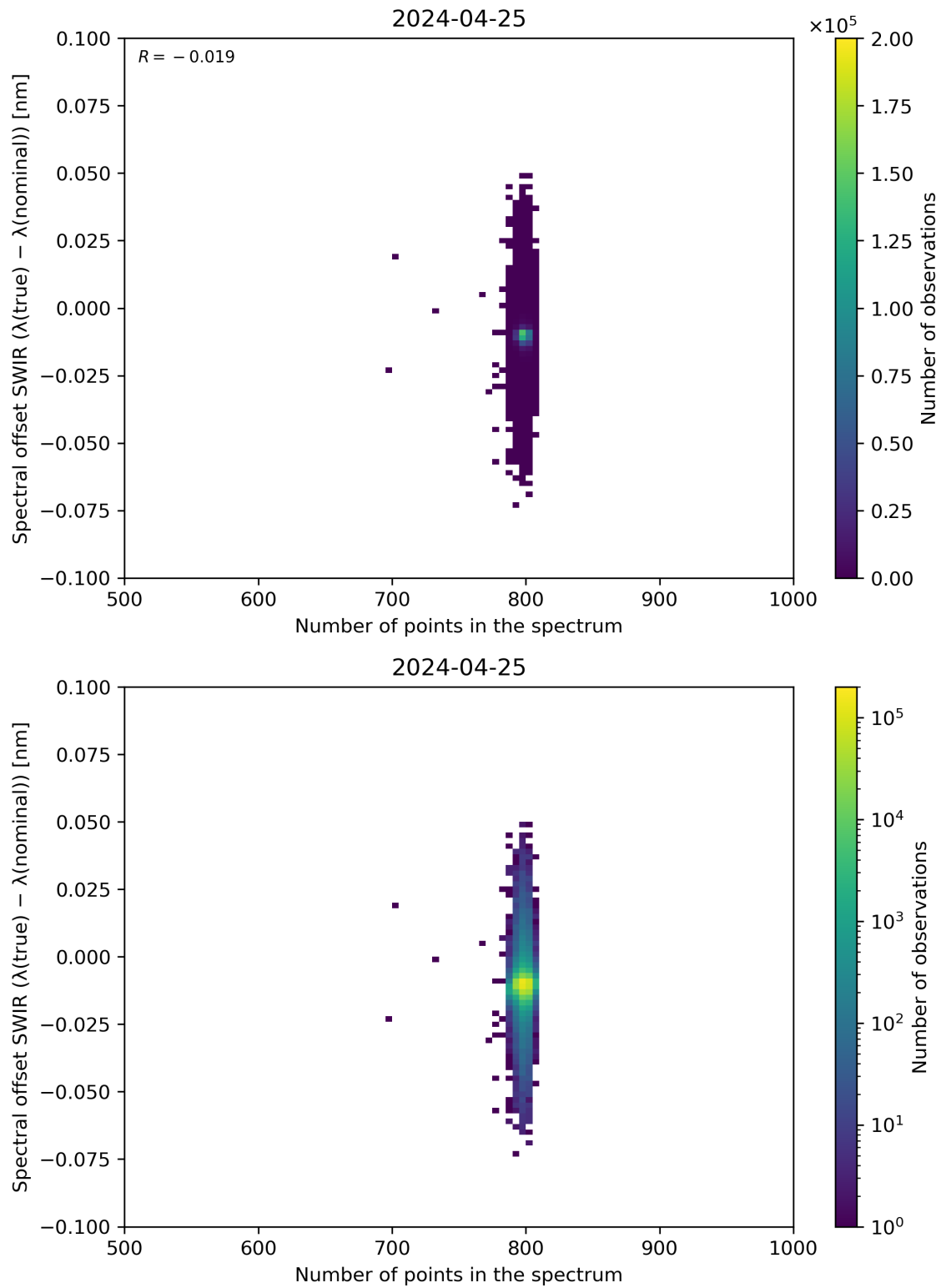
Figure 93: Scatter density plot of “Number of points in the spectrum” against “Spectral offset SWIR ( \lambda(\text{true}) - \lambda(\text{nominal}) )” for 2024-04-24 to 2024-04-26.
