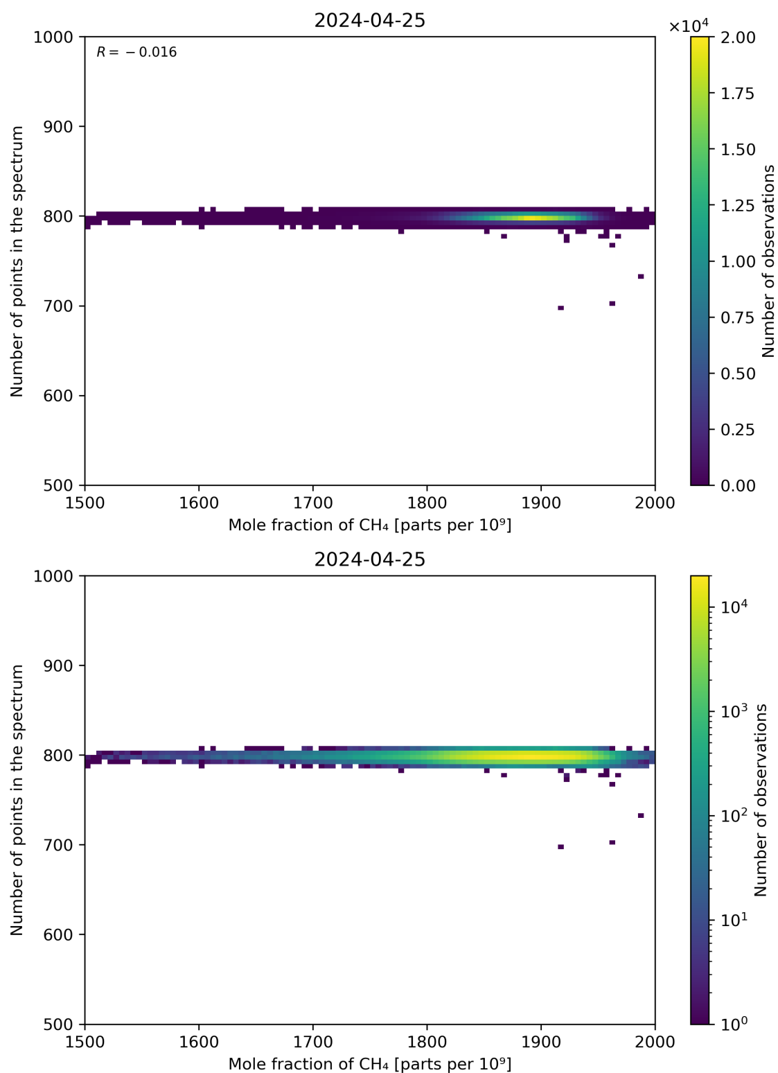
Figure 77: Scatter density plot of “Mole fraction of CH 4 ” against “Number of points in the spectrum” for 2024-04-24 to 2024-04-26.
