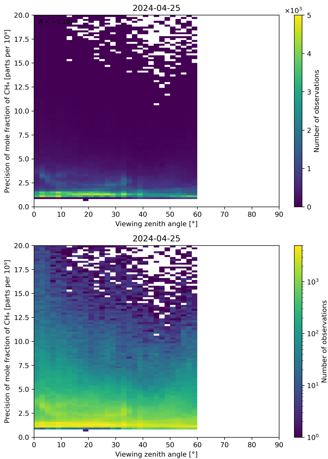
Figure 112: Scatter density plot of “Viewing zenith angle” against “Precision of mole fraction of CH 4 ” for 2024-04-24 to 2024-04-26.
