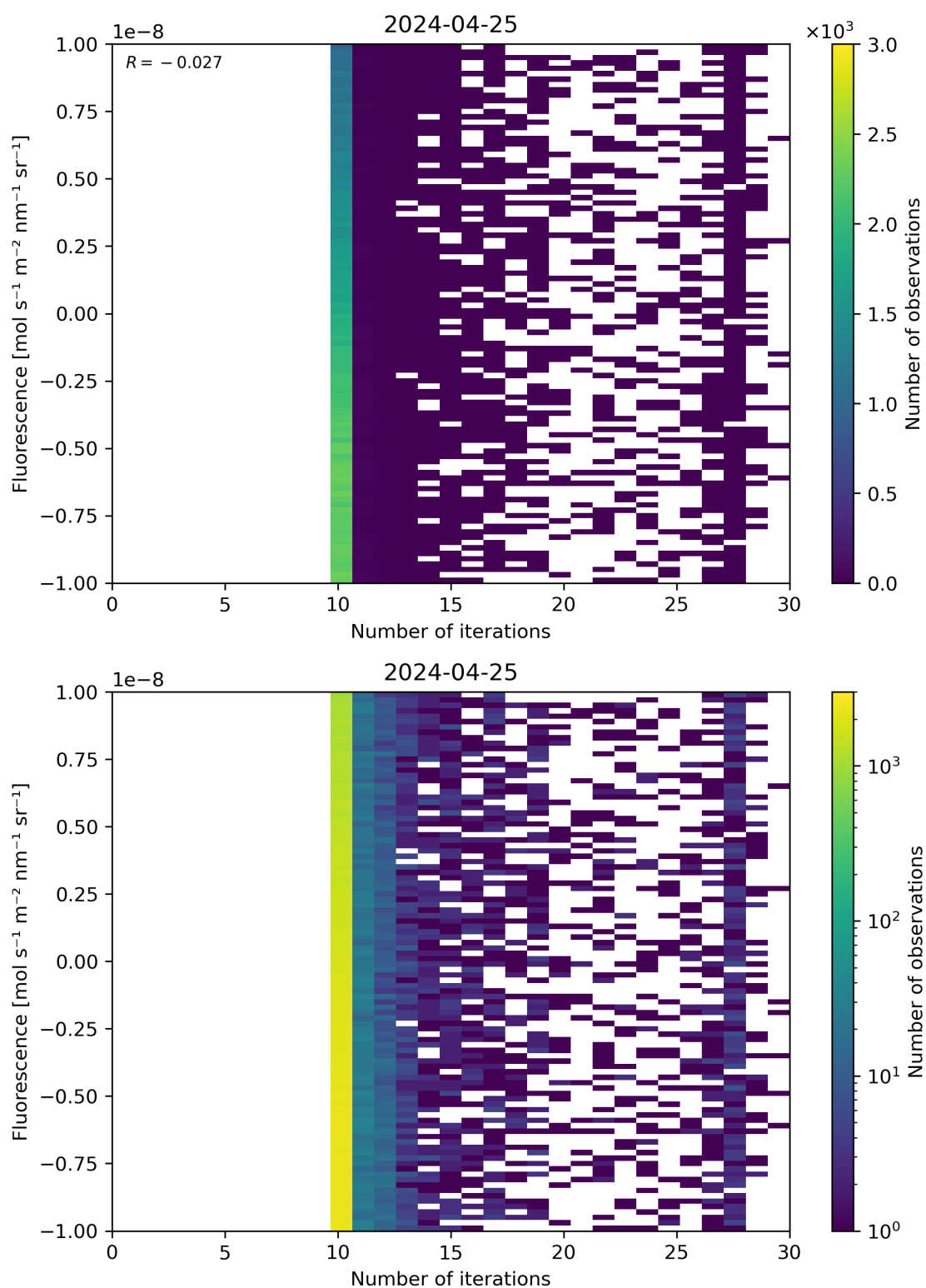
Figure 87: Scatter density plot of “Number of iterations” against “Fluorescence” for 2024-04-24 to 2024-04-26.
