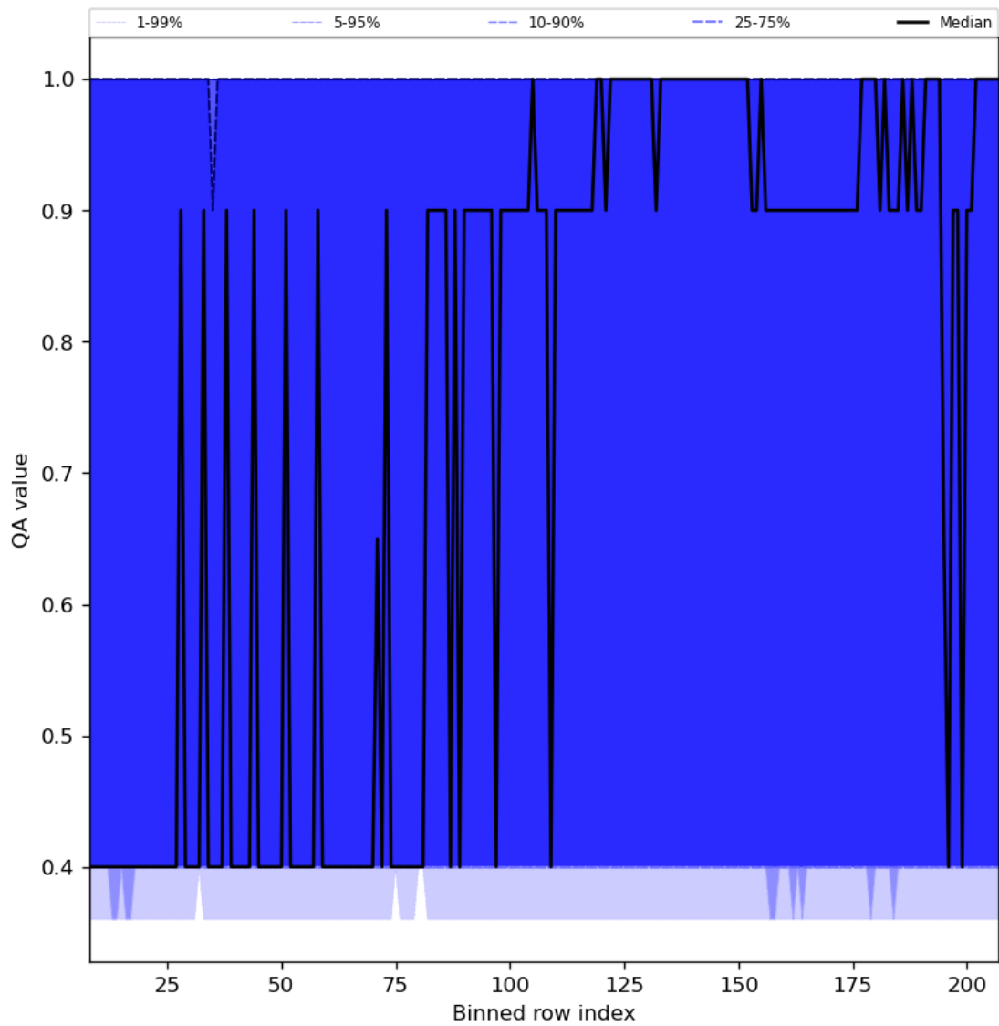
Figure 33: Along track statistics of “QA value” for 2024-04-24 to 2024-04-26
