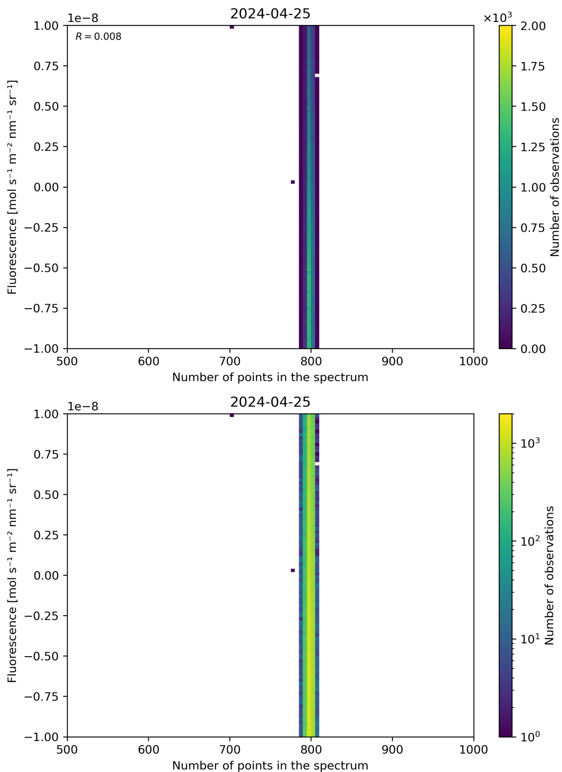
Figure 91: Scatter density plot of “Number of points in the spectrum” against “Fluorescence” for 2024-04-24 to 2024-04-26.
