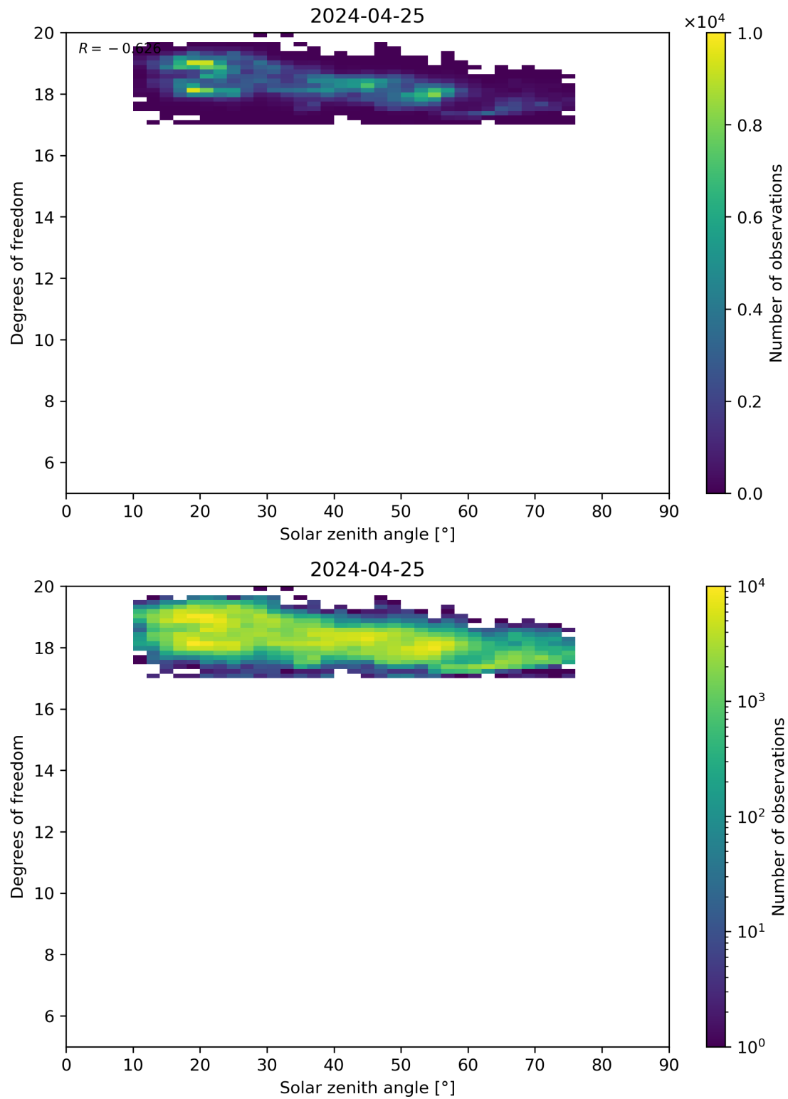
Figure 96: Scatter density plot of “Solar zenith angle” against “Degrees of freedom” for 2024-04-24 to 2024-04-26.
