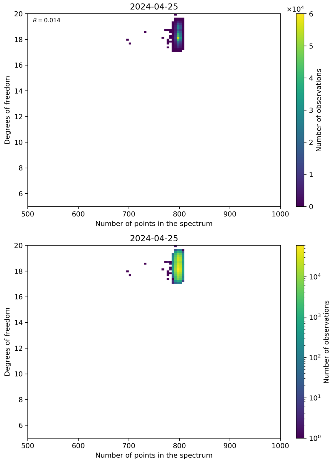
Figure 90: Scatter density plot of “Number of points in the spectrum” against “Degrees of freedom” for 2024-04-24 to 2024-04-26.
