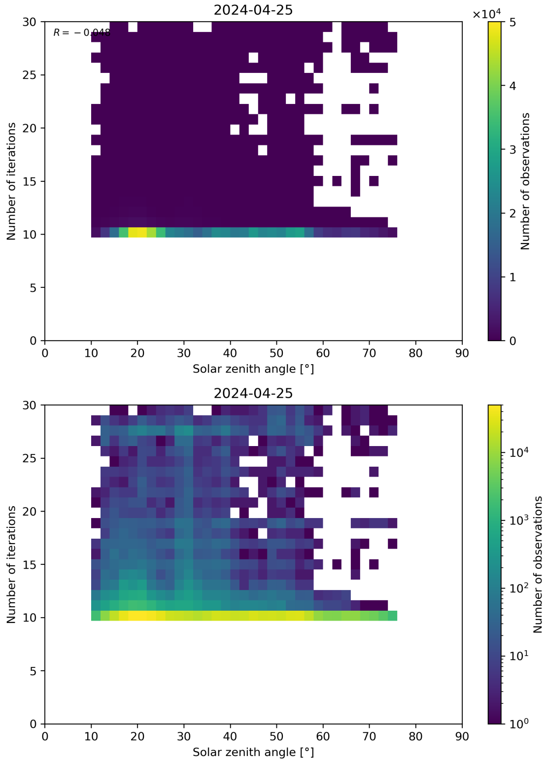
Figure 102: Scatter density plot of “Solar zenith angle” against “Number of iterations” for 2024-04-24 to 2024-04-26.
