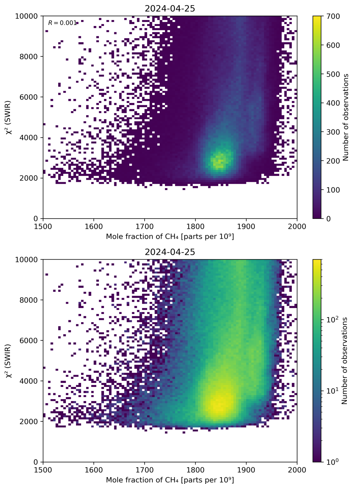
Figure 71: Scatter density plot of “Mole fraction of \text{CH}_4 ” against “ \chi^2 (SWIR)” for 2024-04-24 to 2024-04-26.
