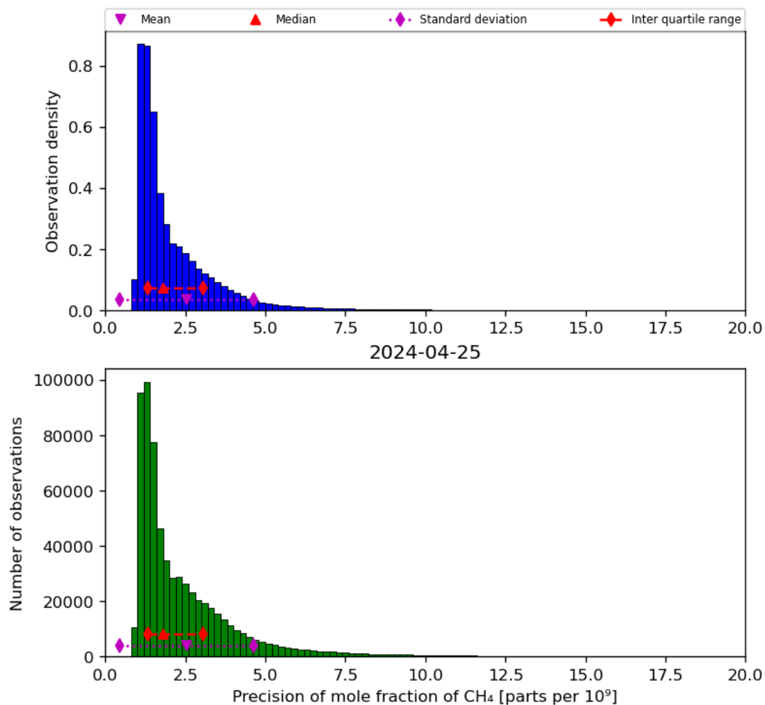
Figure 24: Histogram of “Precision of mole fraction of CH 4 ” for 2024-04-24 to 2024-04-26
