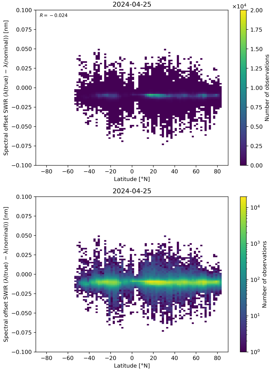
Figure 62: Scatter density plot of “Latitude” against “Spectral offset SWIR ( \lambda(\text{true}) - \lambda(\text{nominal}) )” for 2024-04-24 to 2024-04-26.
