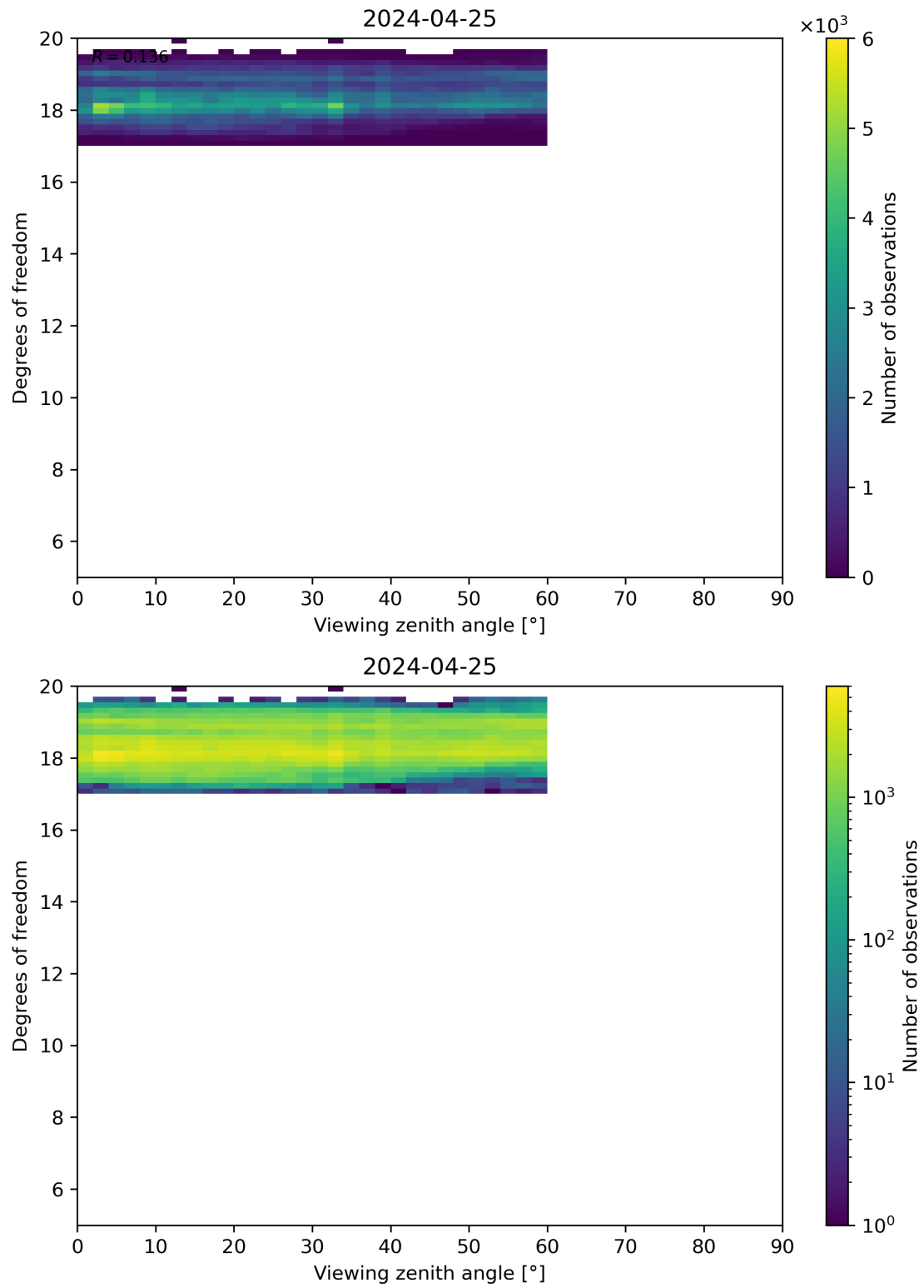
Figure 107: Scatter density plot of “Viewing zenith angle” against “Degrees of freedom” for 2024-04-24 to 2024-04-26.
