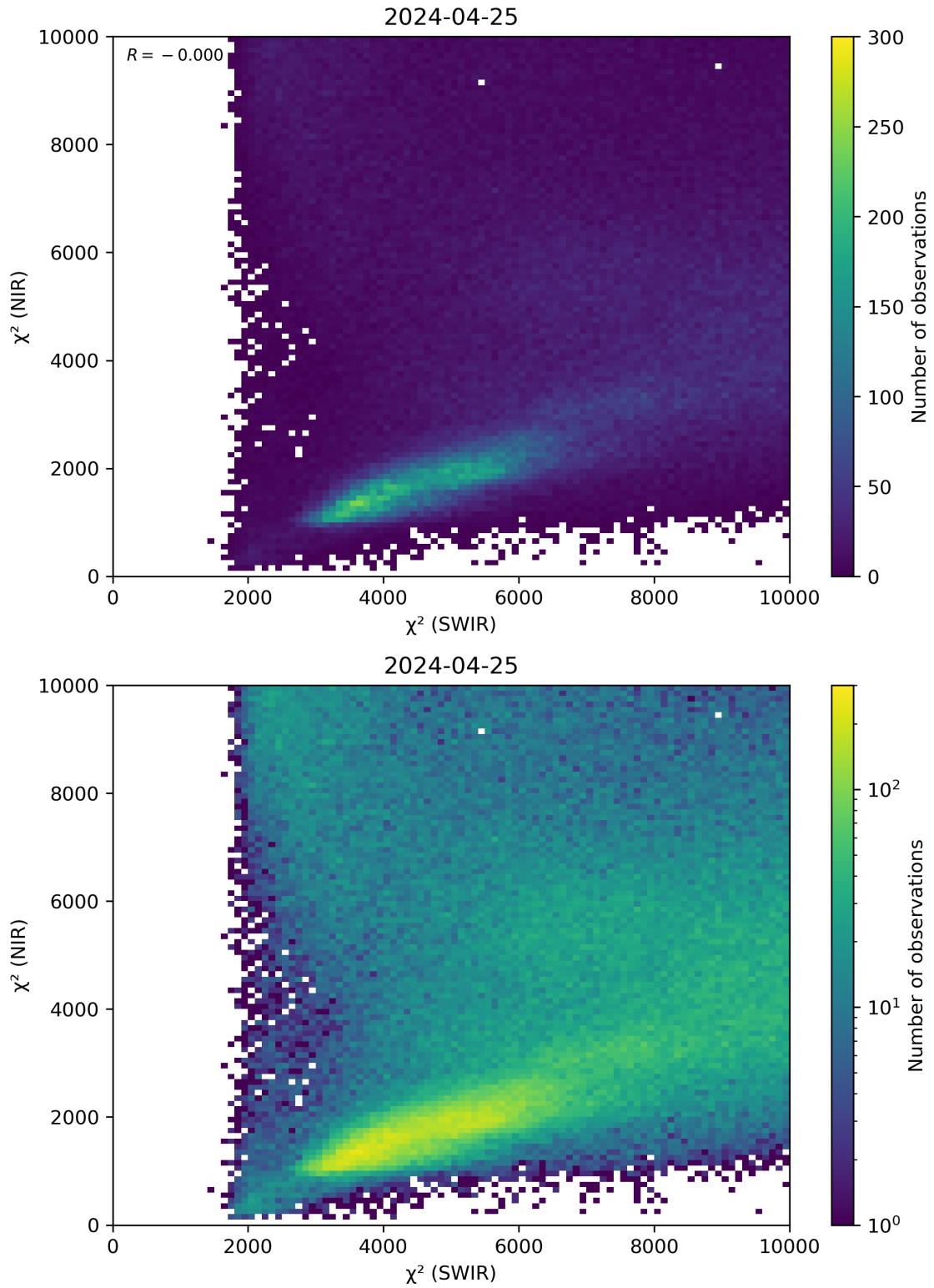
Figure 47: Scatter density plot of “ \chi^2 (SWIR)” against “ \chi^2 (NIR)” for 2024-04-24 to 2024-04-26.
