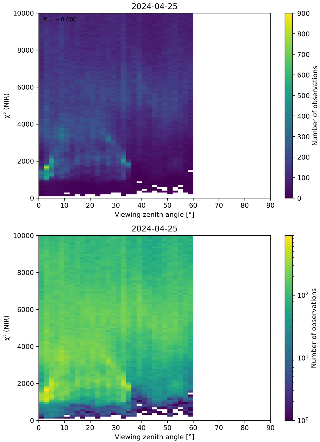
Figure 105: Scatter density plot of “Viewing zenith angle” against “ \chi^2 (NIR)” for 2024-04-24 to 2024-04-26.
