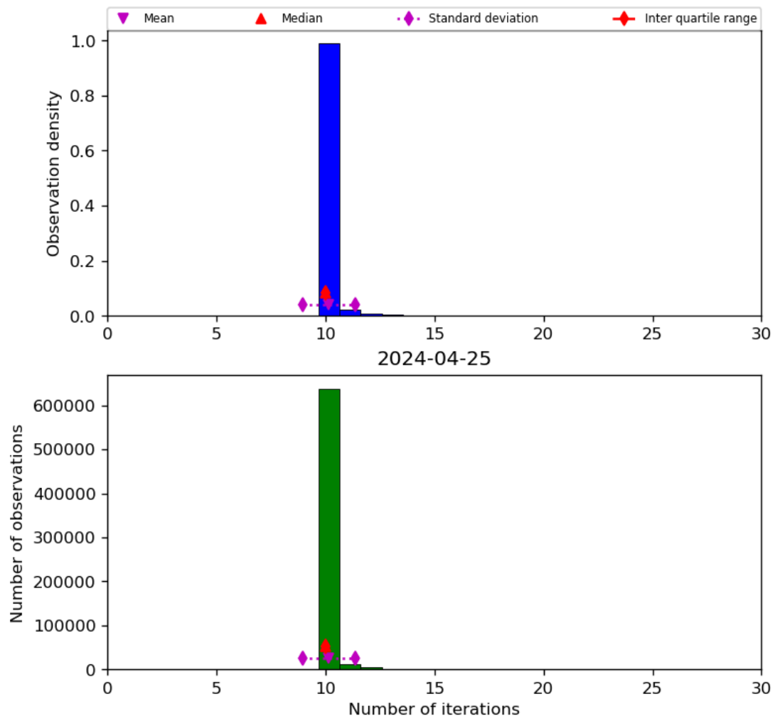
Figure 31: Histogram of “Number of iterations” for 2024-04-24 to 2024-04-26
