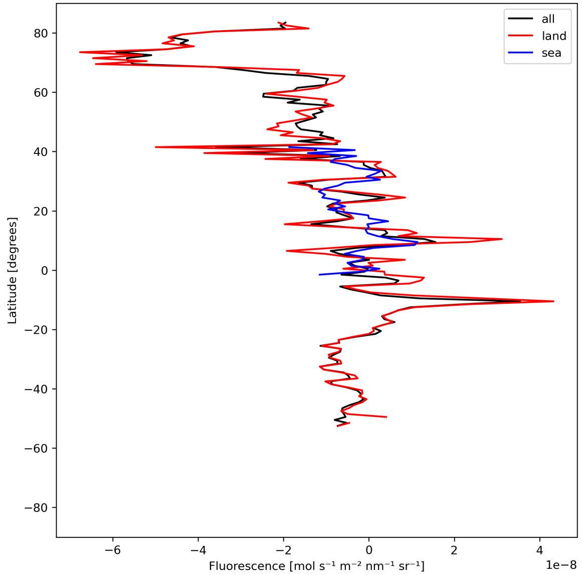
Figure 21: Zonal average of “Fluorescence” for 2024-04-24 to 2024-04-26.
