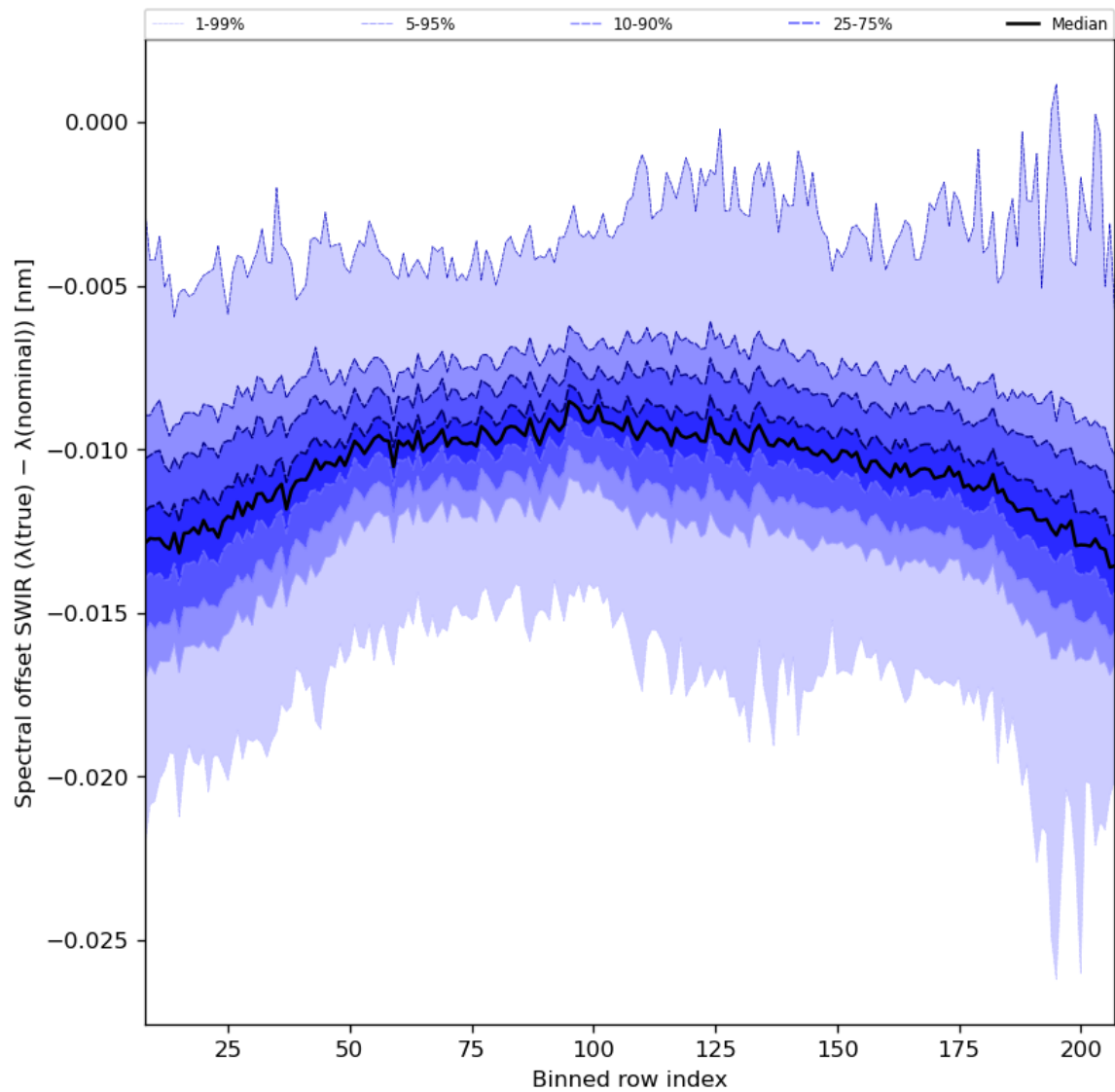
Figure 38: Along track statistics of “Spectral offset SWIR ( \lambda(\text{true}) - \lambda(\text{nominal}) )” for 2024-04-24 to 2024-04-26
