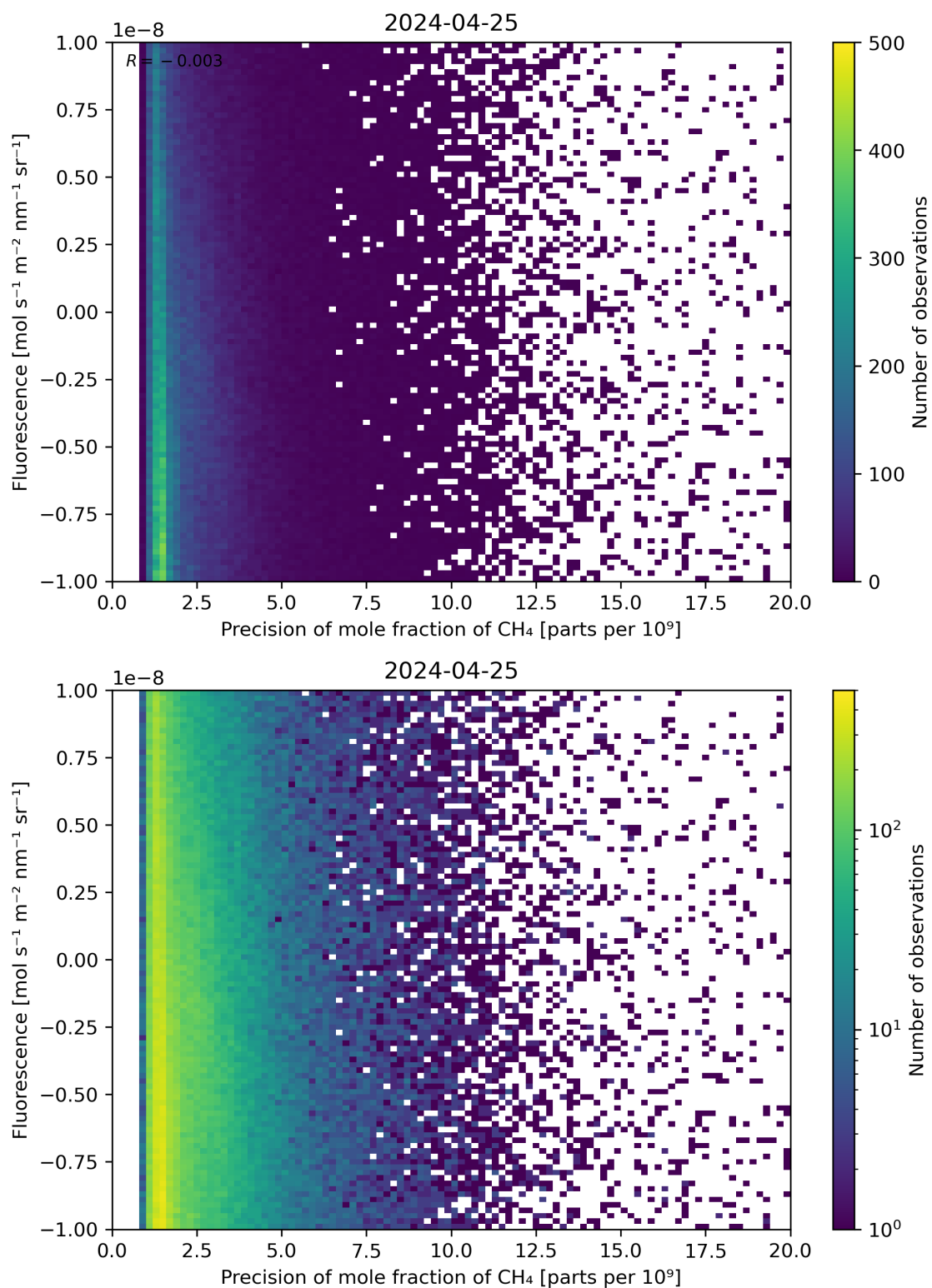
Figure 81: Scatter density plot of “Precision of mole fraction of \text{CH}_4 ” against “Fluorescence” for 2024-04-24 to 2024-04-26.
