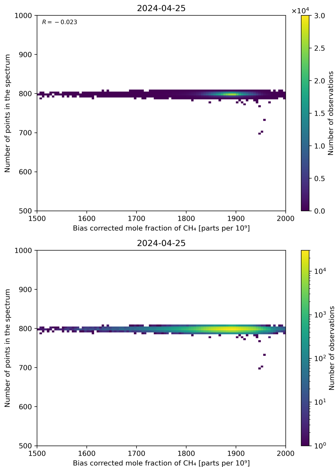
Figure 68: Scatter density plot of “Bias corrected mole fraction of CH 4 ” against “Number of points in the spectrum” for 2024-04-24 to 2024-04-26.
