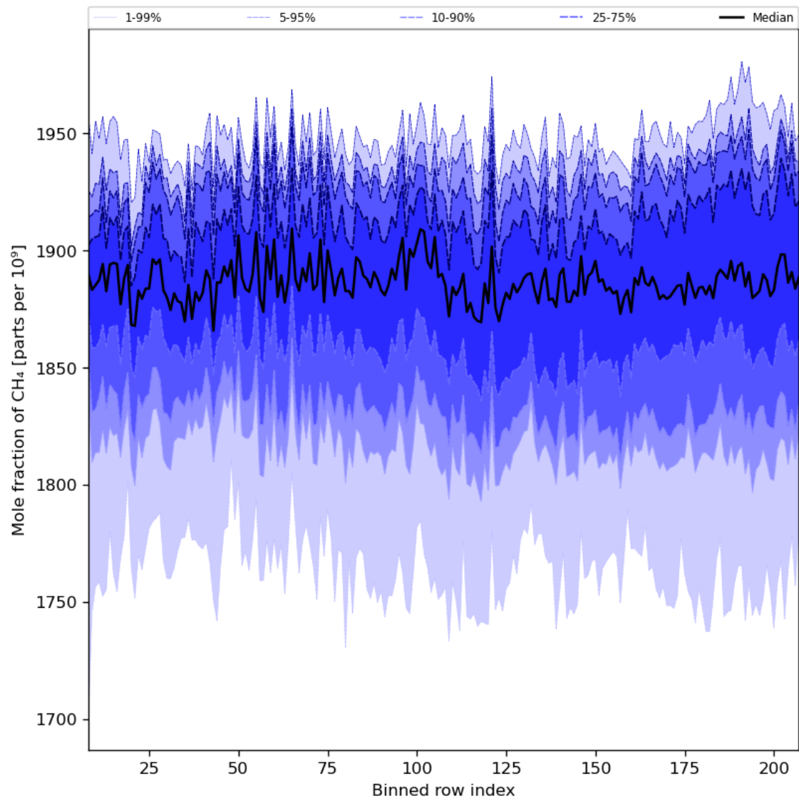
Figure 34: Along track statistics of “Mole fraction of CH 4 ” for 2024-04-24 to 2024-04-26
