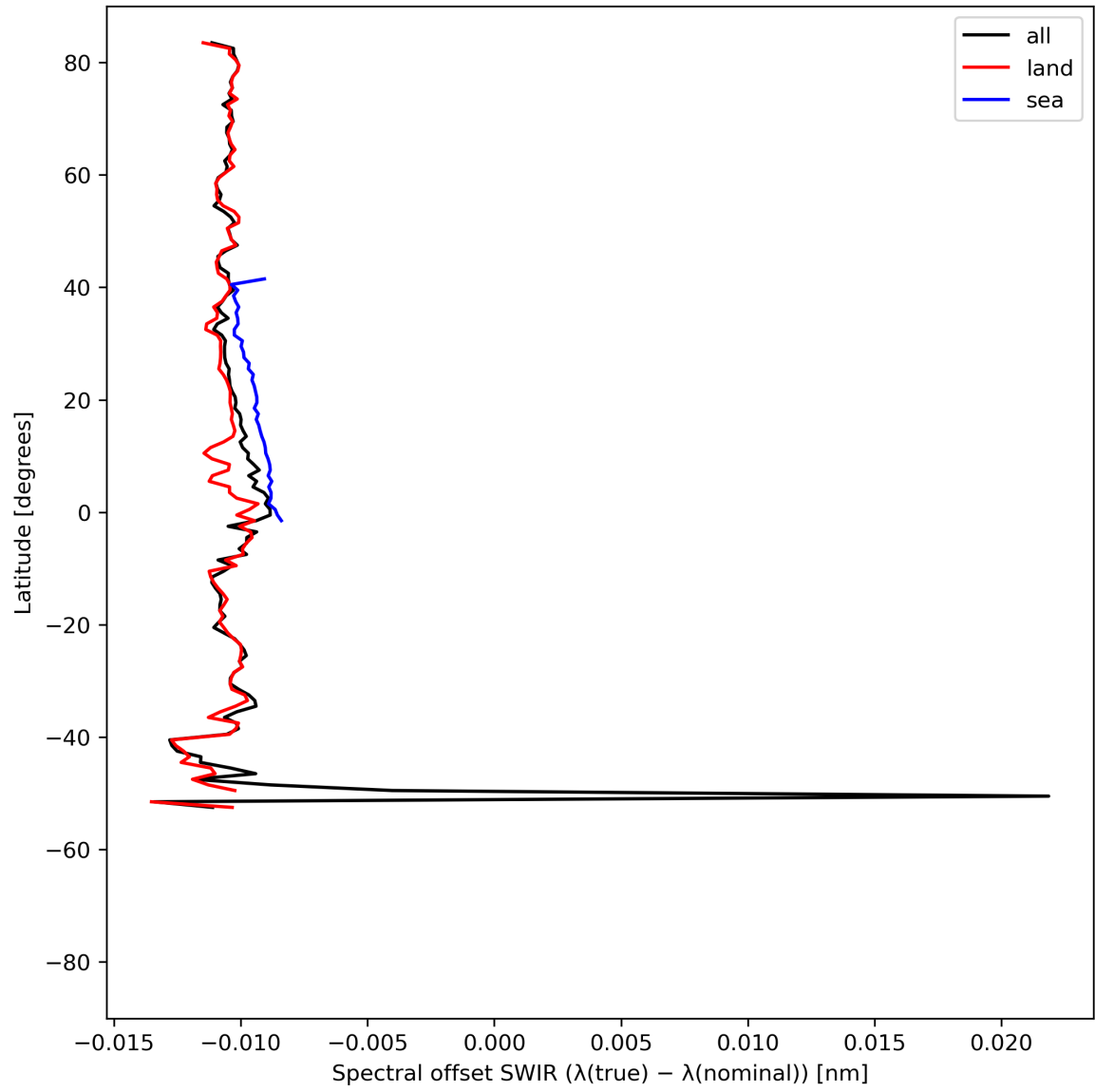
Figure 16: Zonal average of “Spectral offset SWIR ( \lambda(\text{true}) - \lambda(\text{nominal}) )” for 2024-04-24 to 2024-04-26.
