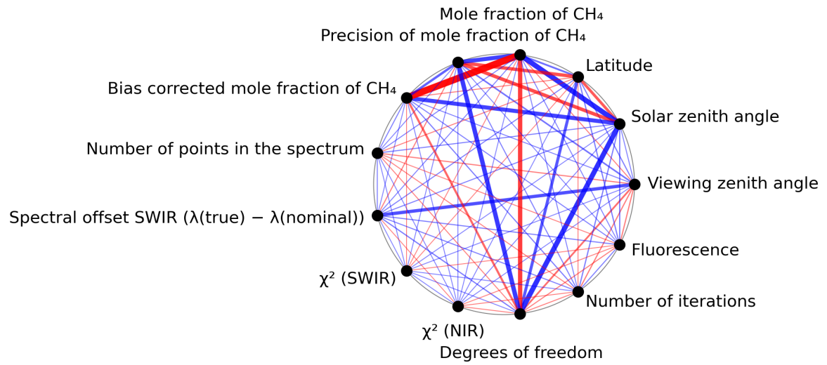
Figure 1: Map of correlation graph for 2024-04-24 to 2024-04-26.
