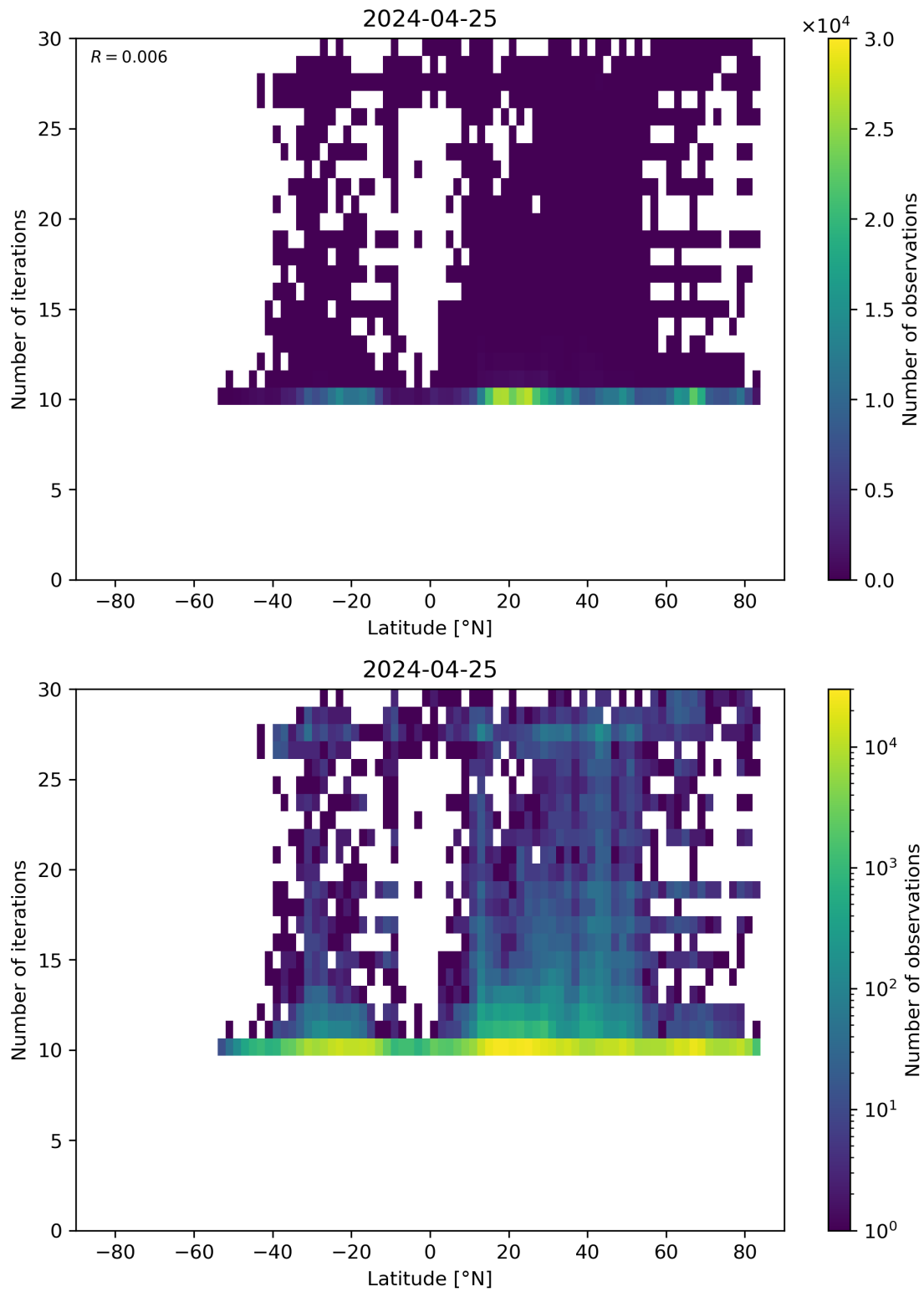
Figure 60: Scatter density plot of “Latitude” against “Number of iterations” for 2024-04-24 to 2024-04-26.
