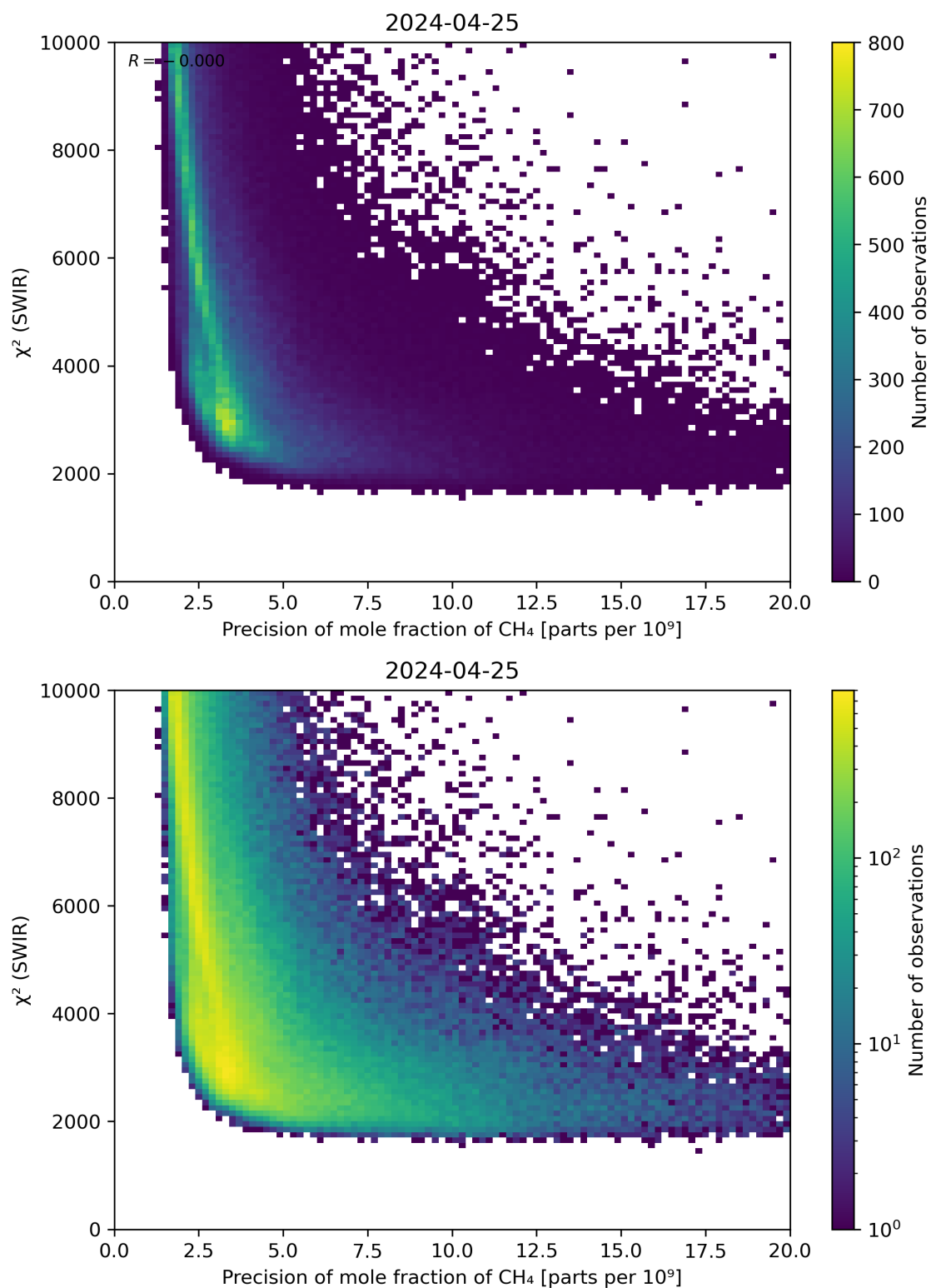
Figure 79: Scatter density plot of “Precision of mole fraction of \text{CH}_4 ” against “ \chi^2 (SWIR)” for 2024-04-24 to 2024-04-26.
