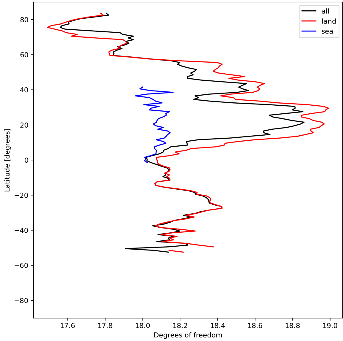
Figure 19: Zonal average of “Degrees of freedom” for 2024-04-24 to 2024-04-26.
