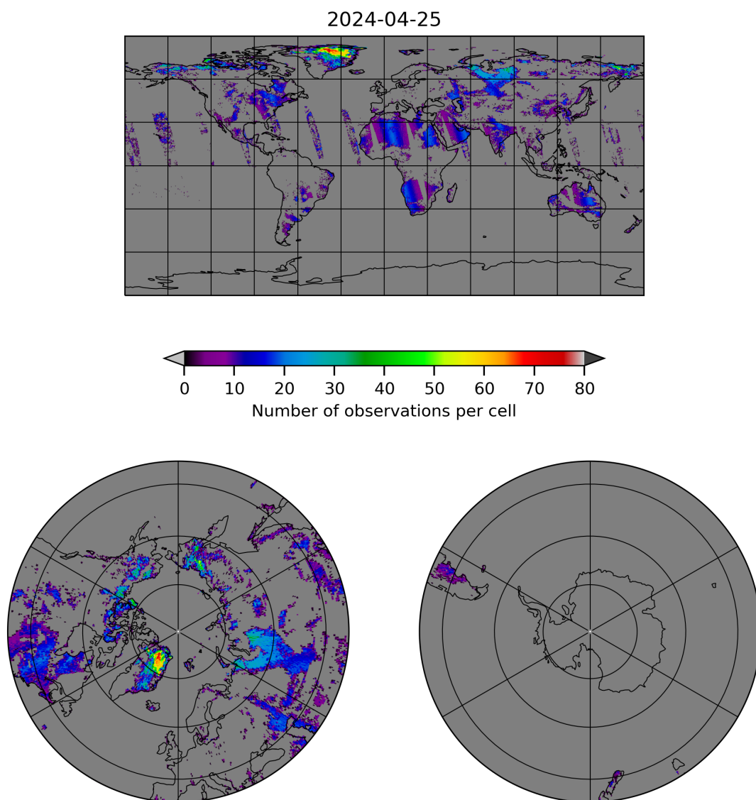
Figure 10: Map of the number of observations for 2024-04-24 to 2024-04-26
