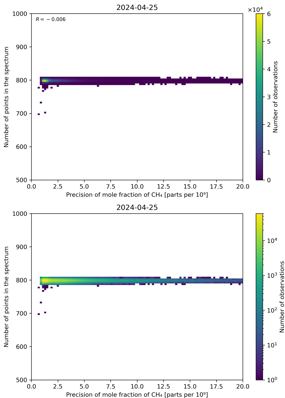
Figure 84: Scatter density plot of “Precision of mole fraction of CH 4 ” against “Number of points in the spectrum” for 2024-04-24 to 2024-04-26.
