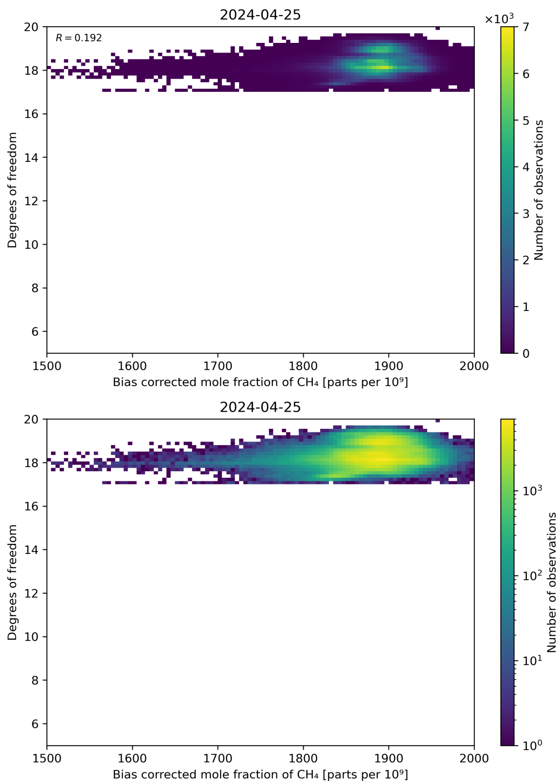
Figure 65: Scatter density plot of “Bias corrected mole fraction of CH 4 ” against “Degrees of freedom” for 2024-04-24 to 2024-04-26.
