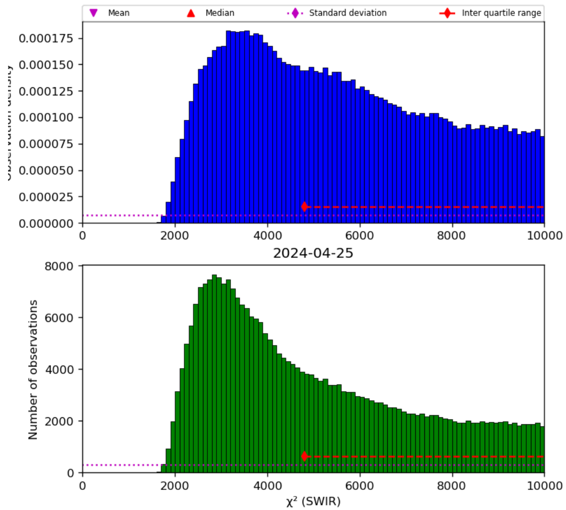
Figure 28: Histogram of “ \chi^2 (SWIR)” for 2024-04-24 to 2024-04-26
