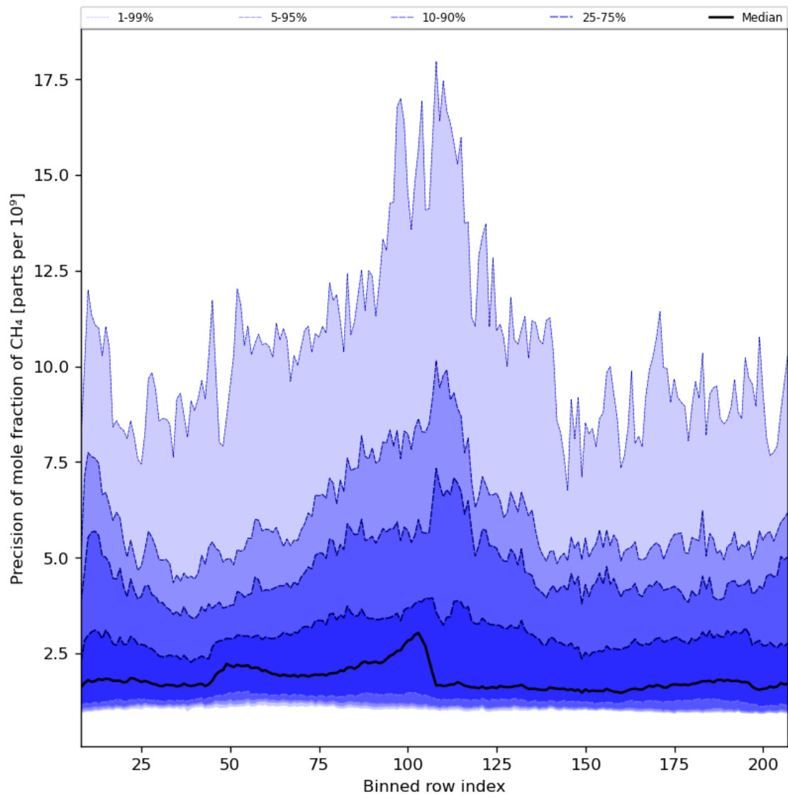
Figure 35: Along track statistics of “Precision of mole fraction of CH 4 ” for 2024-04-24 to 2024-04-26
