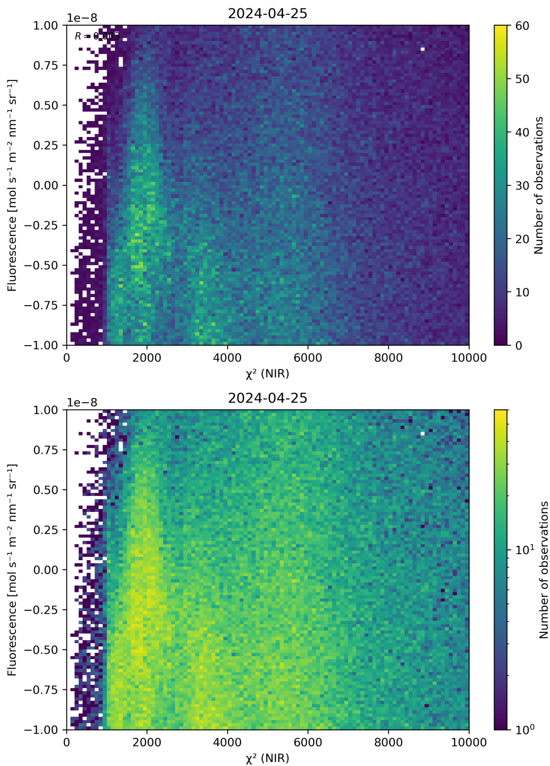
Figure 45: Scatter density plot of “ \chi^2 (NIR)” against “Fluorescence” for 2024-04-24 to 2024-04-26.
