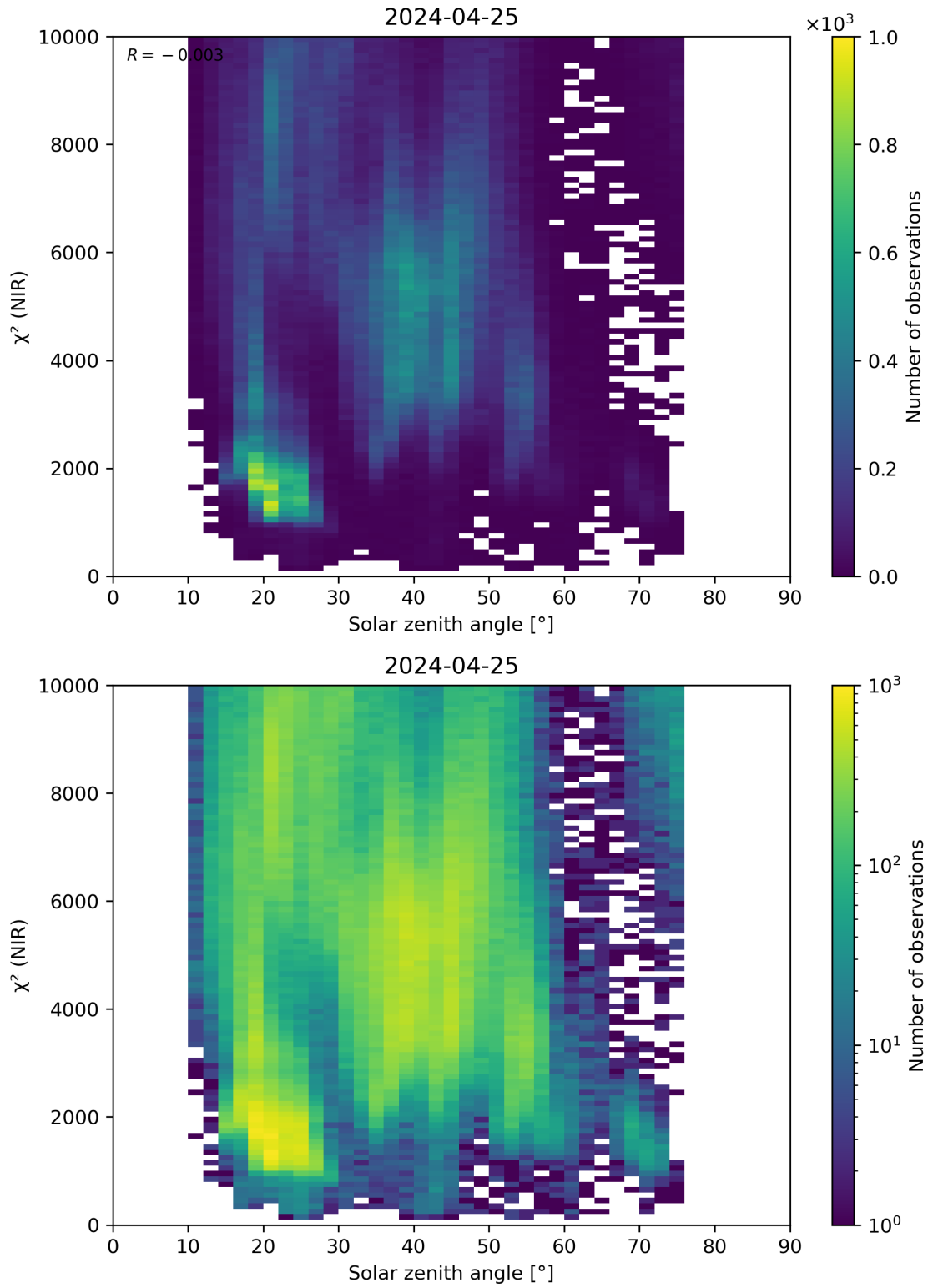
Figure 94: Scatter density plot of “Solar zenith angle” against “ \chi^2 (NIR)” for 2024-04-24 to 2024-04-26.
