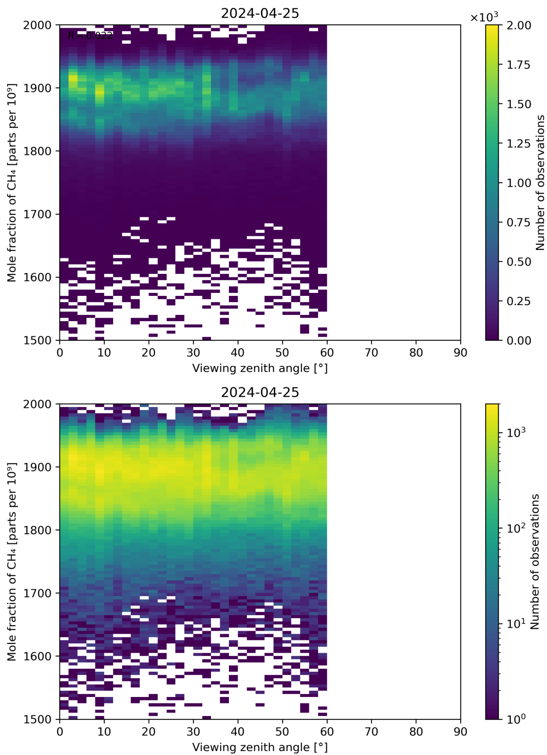
Figure 110: Scatter density plot of “Viewing zenith angle” against “Mole fraction of CH 4 ” for 2024-04-24 to 2024-04-26.
