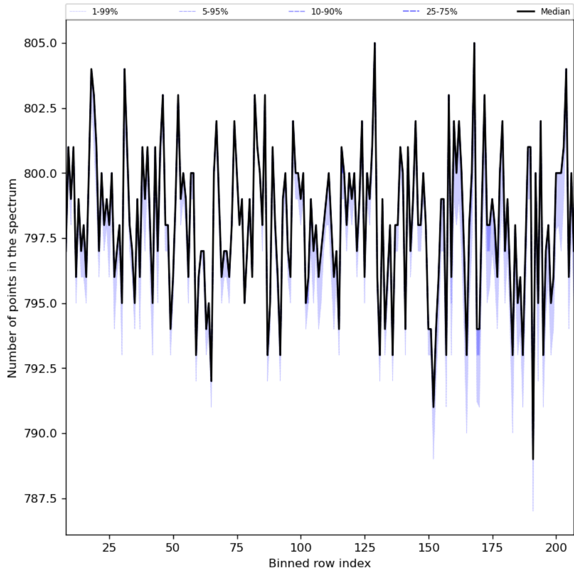
Figure 37: Along track statistics of “Number of points in the spectrum” for 2024-04-24 to 2024-04-26
