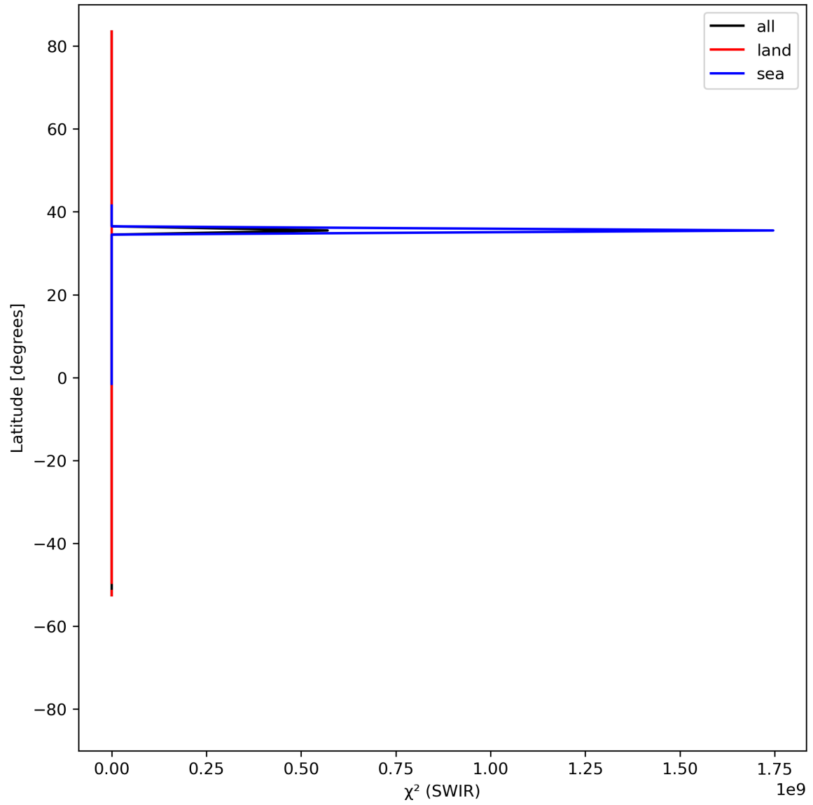
Figure 17: Zonal average of “ \chi^2 (SWIR)” for 2024-04-24 to 2024-04-26.
