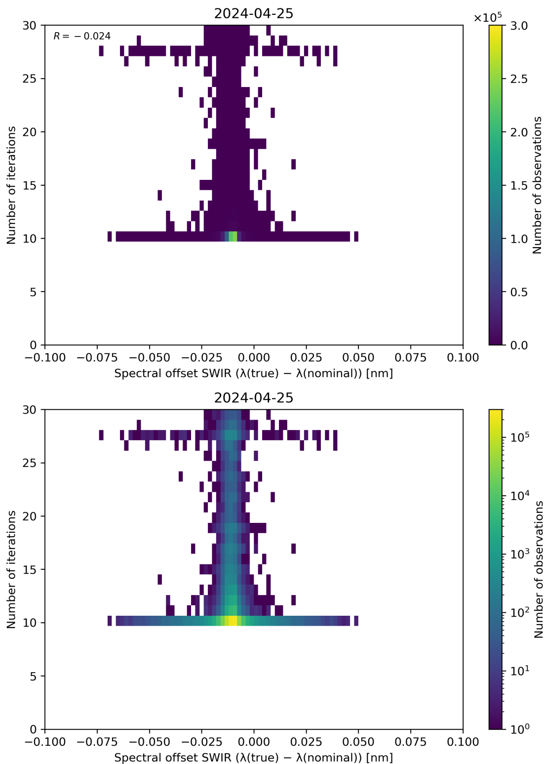
Figure 121: Scatter density plot of “Spectral offset SWIR ( \lambda(\text{true}) - \lambda(\text{nominal}) )” against “Number of iterations” for 2024-04-24 to 2024-04-26.
