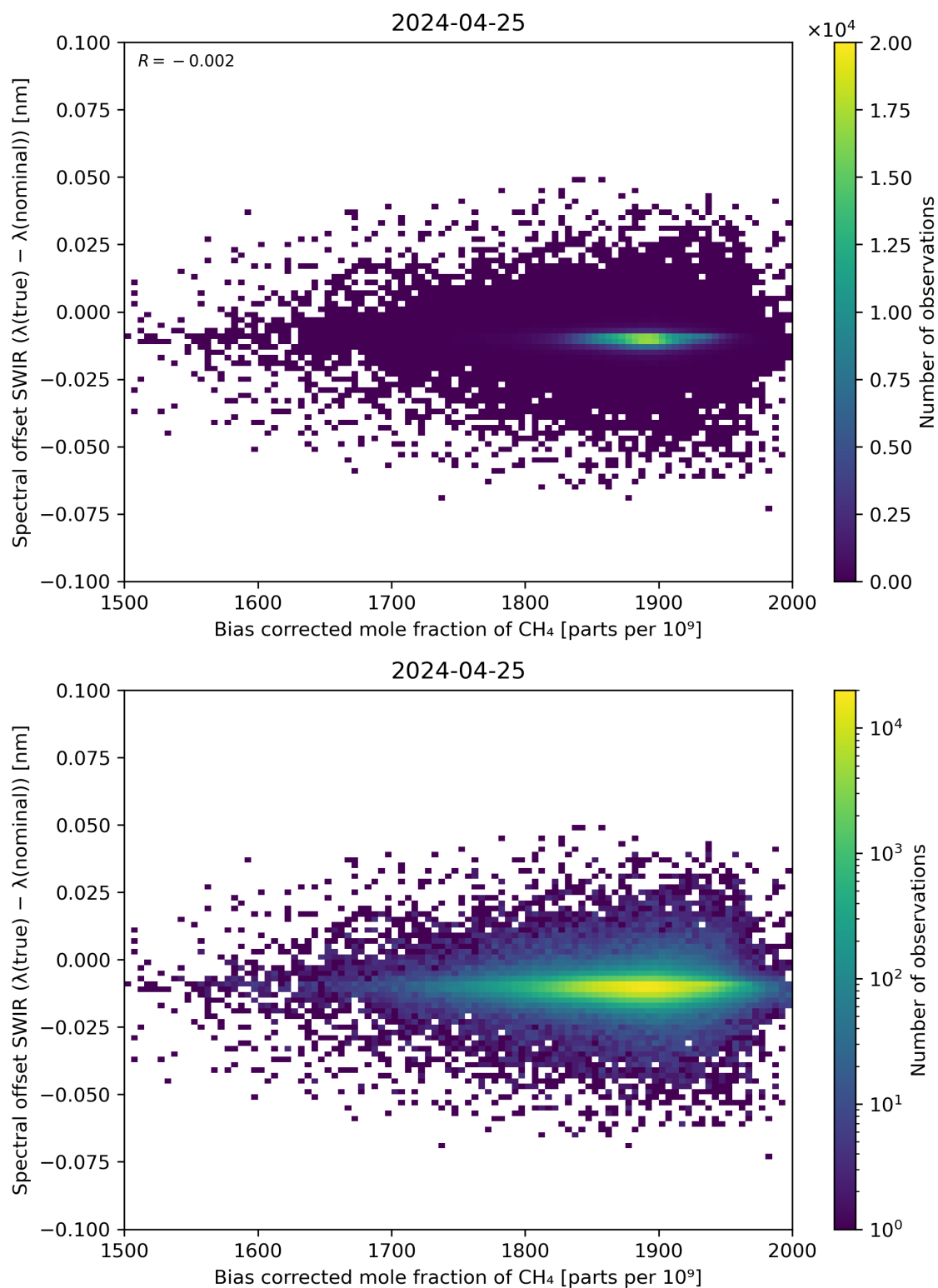
Figure 69: Scatter density plot of “Bias corrected mole fraction of \text{CH}_4 ” against “Spectral offset SWIR ( \lambda(\text{true}) - \lambda(\text{nominal}) )” for 2024-04-24 to 2024-04-26.
