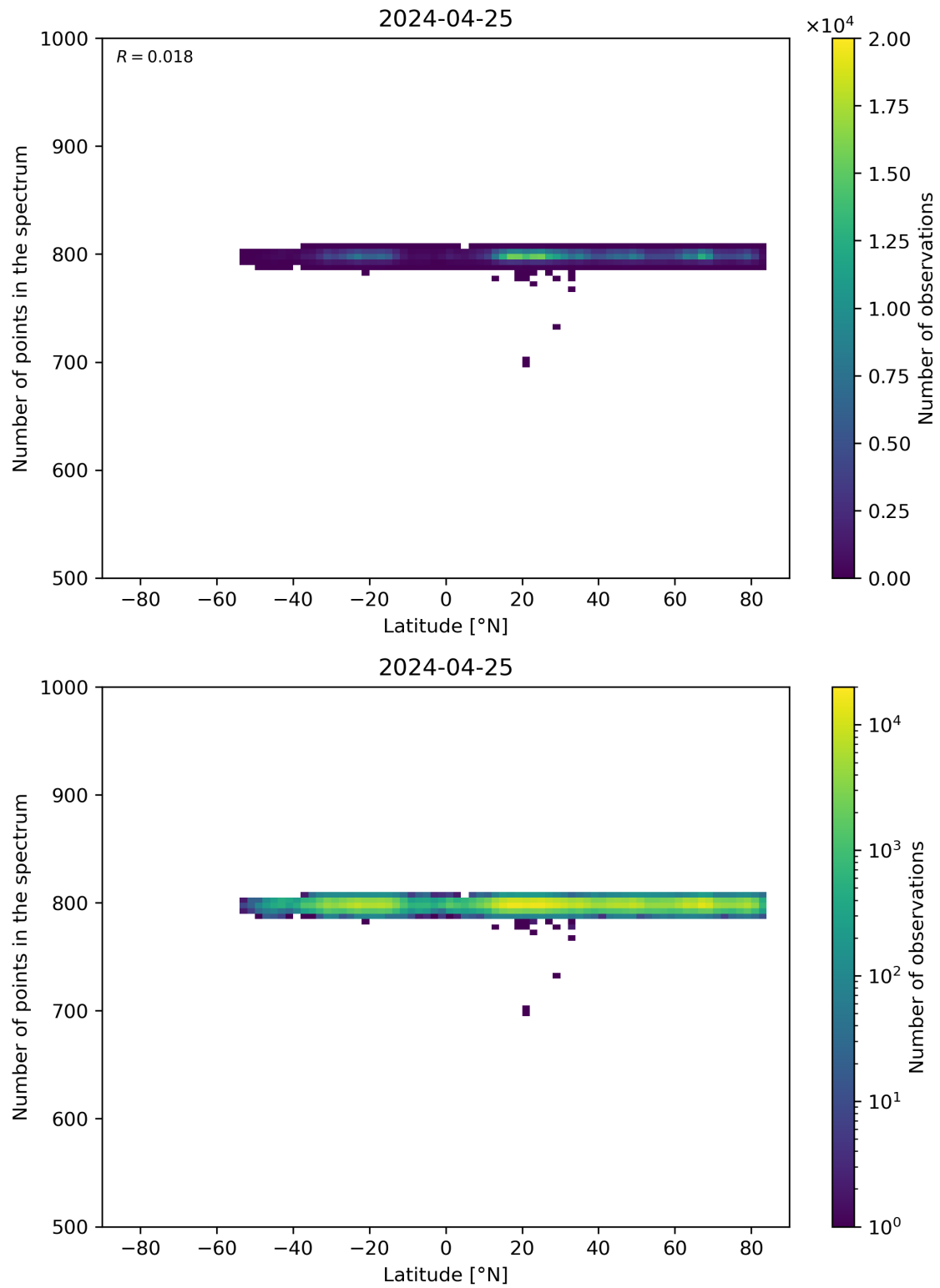
Figure 61: Scatter density plot of “Latitude” against “Number of points in the spectrum” for 2024-04-24 to 2024-04-26.
