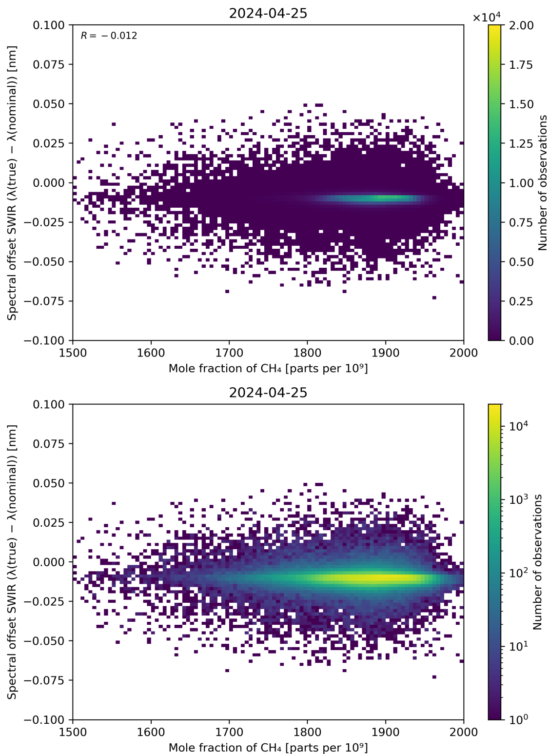
Figure 86: Scatter density plot of “Mole fraction of CH 4 ” against “Spectral offset SWIR ( \lambda(\text{true}) - \lambda(\text{nominal}) )” for 2024-04-24 to 2024-04-26.
