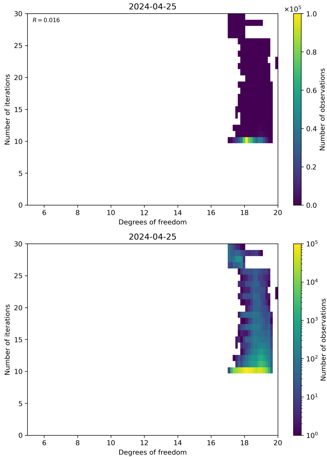
Figure 52: Scatter density plot of “Degrees of freedom” against “Number of iterations” for 2024-04-24 to 2024-04-26.
