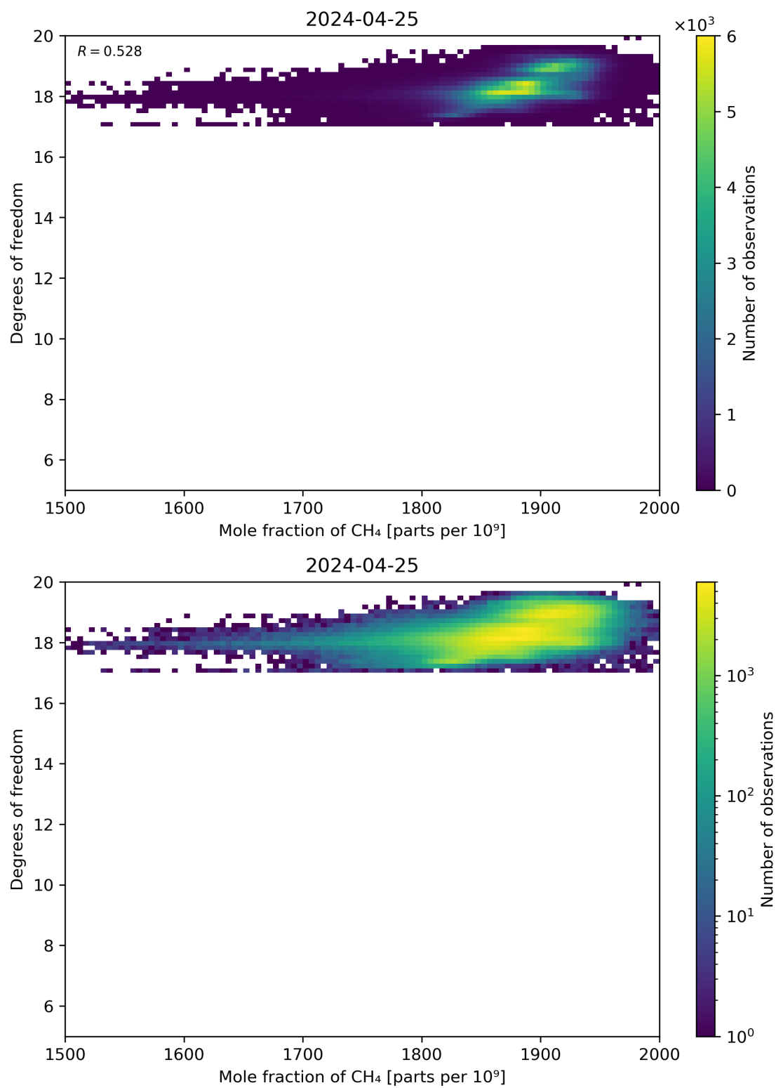
Figure 72: Scatter density plot of “Mole fraction of CH 4 ” against “Degrees of freedom” for 2024-04-24 to 2024-04-26.
