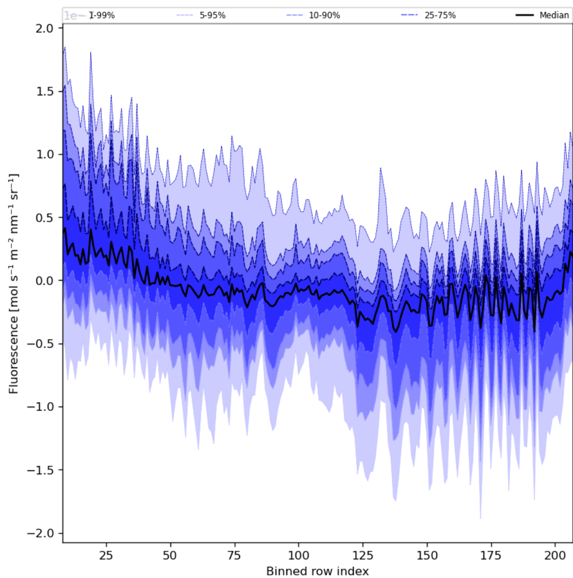
Figure 43: Along track statistics of “Fluorescence” for 2024-04-24 to 2024-04-26
