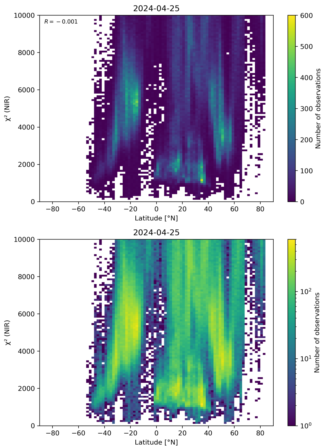
Figure 53: Scatter density plot of “Latitude” against “ \chi^2 (NIR)” for 2024-04-24 to 2024-04-26.
