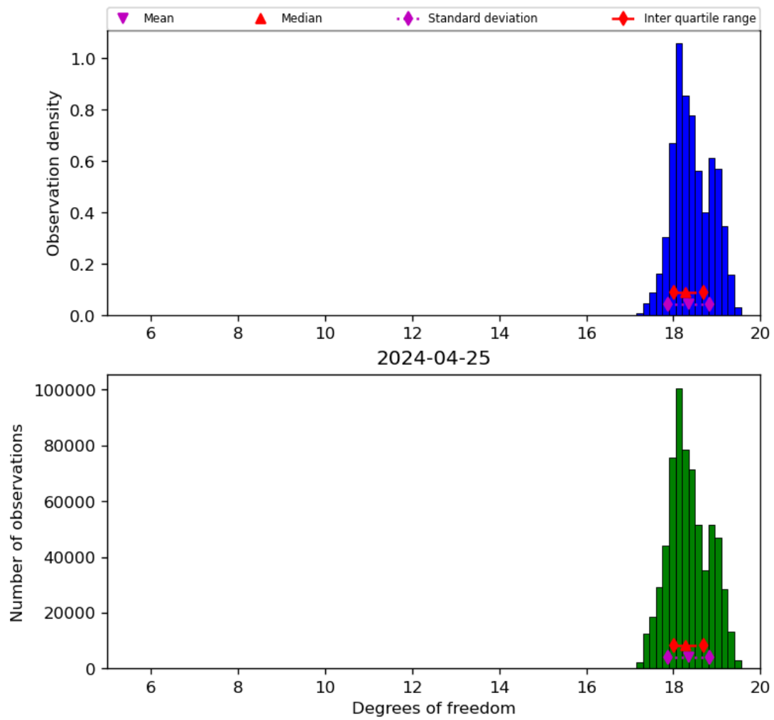
Figure 30: Histogram of “Degrees of freedom” for 2024-04-24 to 2024-04-26
