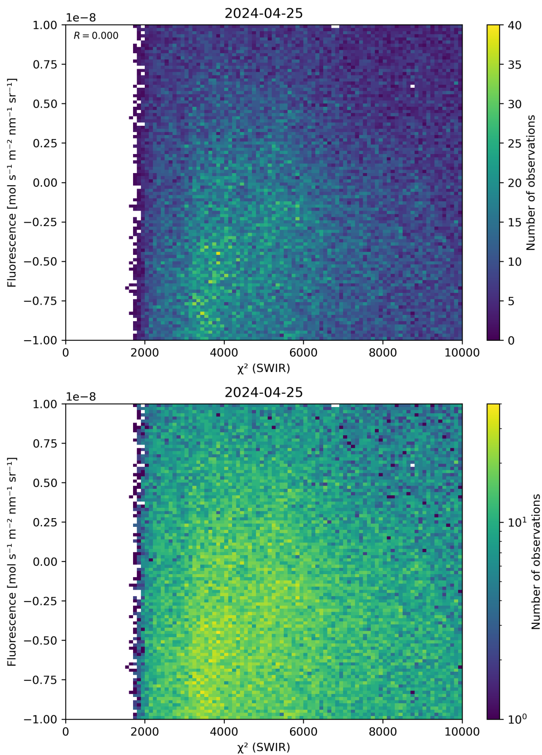
Figure 49: Scatter density plot of “ \chi^2 (SWIR)” against “Fluorescence” for 2024-04-24 to 2024-04-26.
