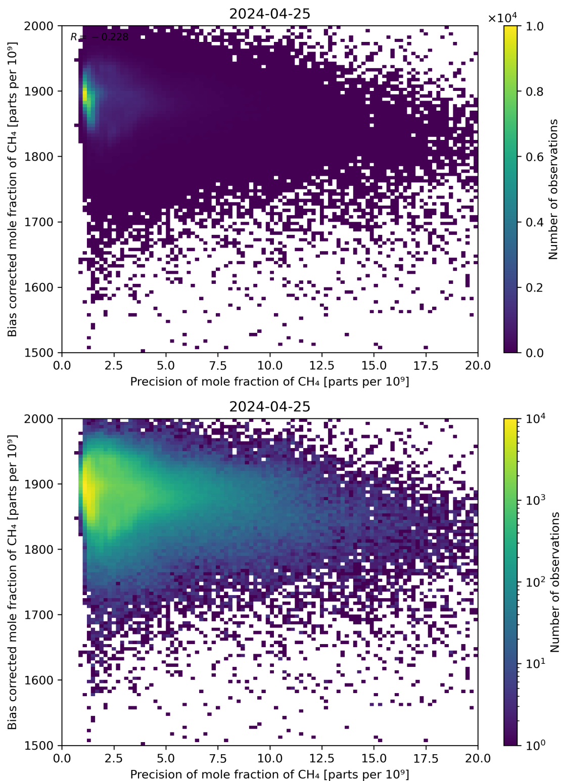
Figure 82: Scatter density plot of “Precision of mole fraction of CH 4 ” against “Bias corrected mole fraction of CH 4 ” for 2024-04-24 to 2024-04-26.
