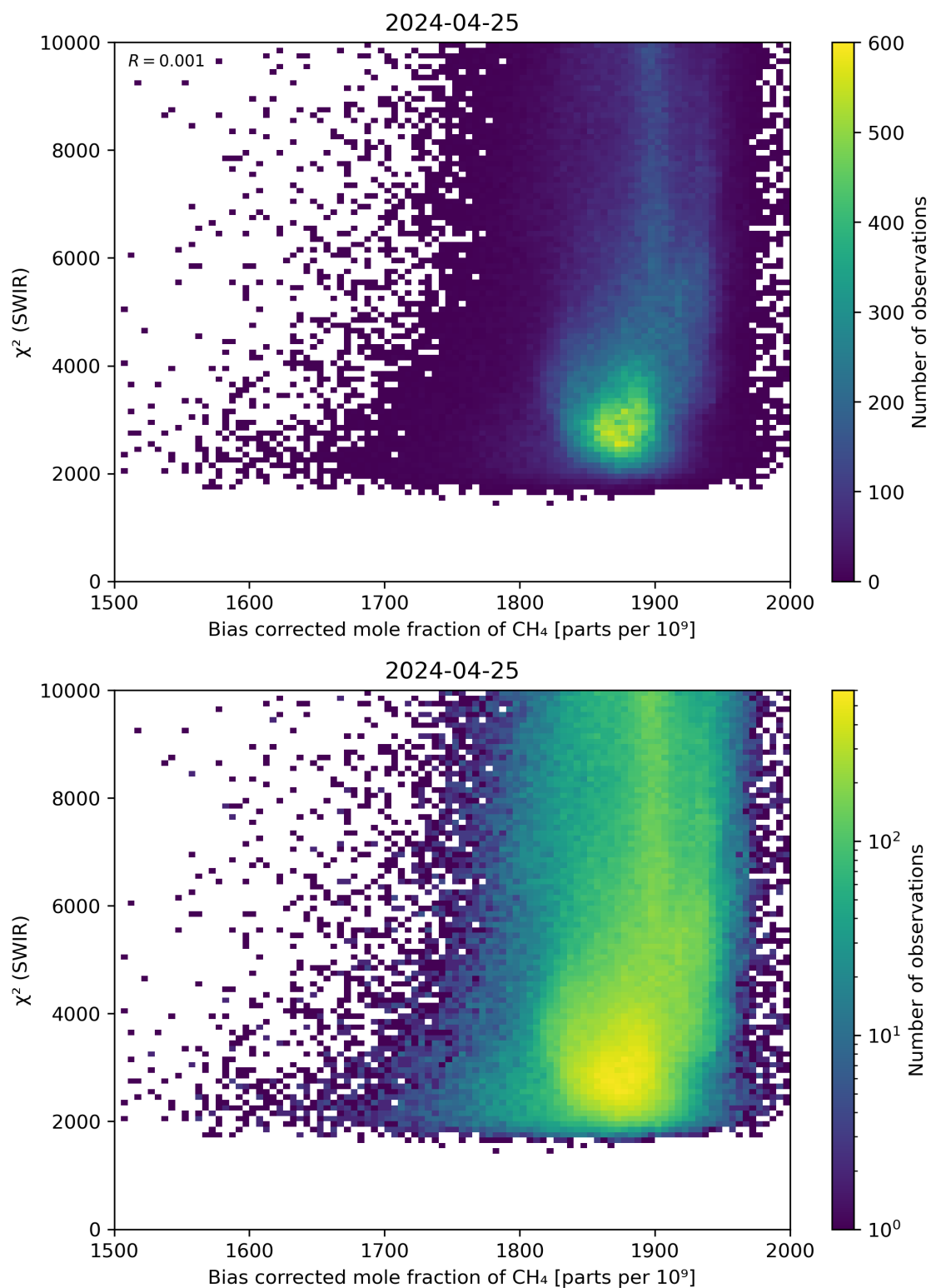
Figure 64: Scatter density plot of “Bias corrected mole fraction of CH 4 ” against “ \chi^2 (SWIR)” for 2024-04-24 to 2024-04-26.
