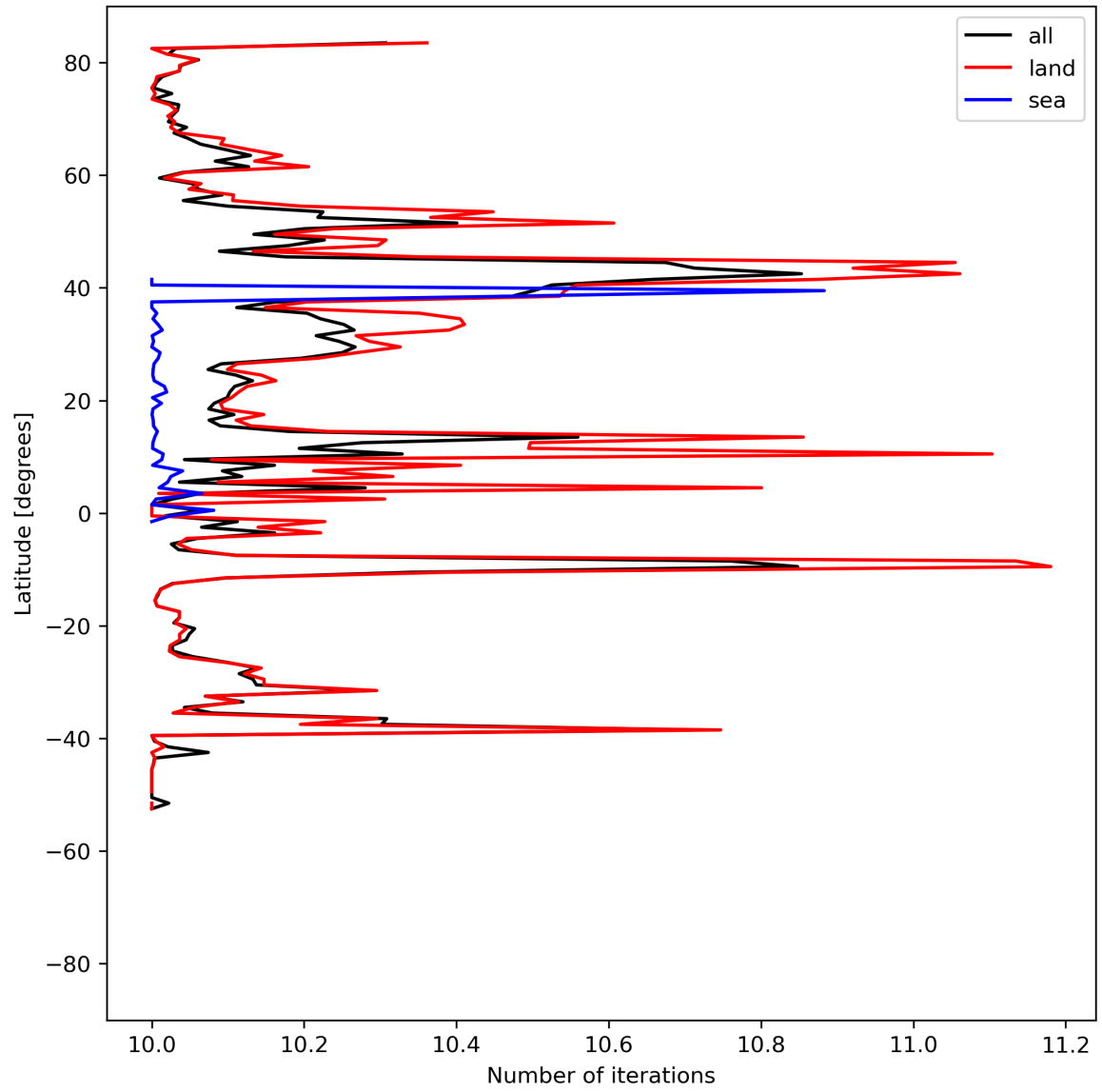
Figure 20: Zonal average of “Number of iterations” for 2024-04-24 to 2024-04-26.
