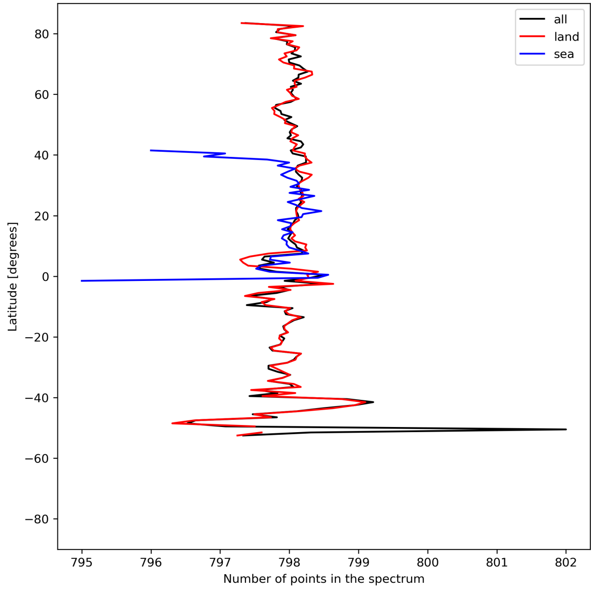
Figure 15: Zonal average of “Number of points in the spectrum” for 2024-04-24 to 2024-04-26.
