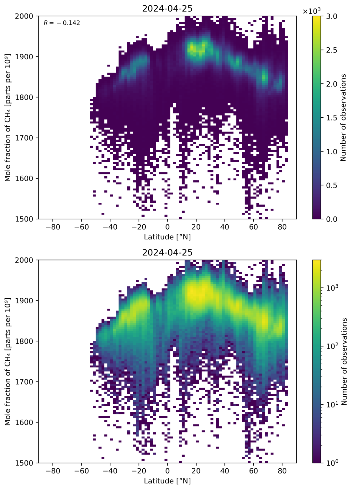
Figure 57: Scatter density plot of “Latitude” against “Mole fraction of \text{CH}_4 ” for 2024-04-24 to 2024-04-26.
