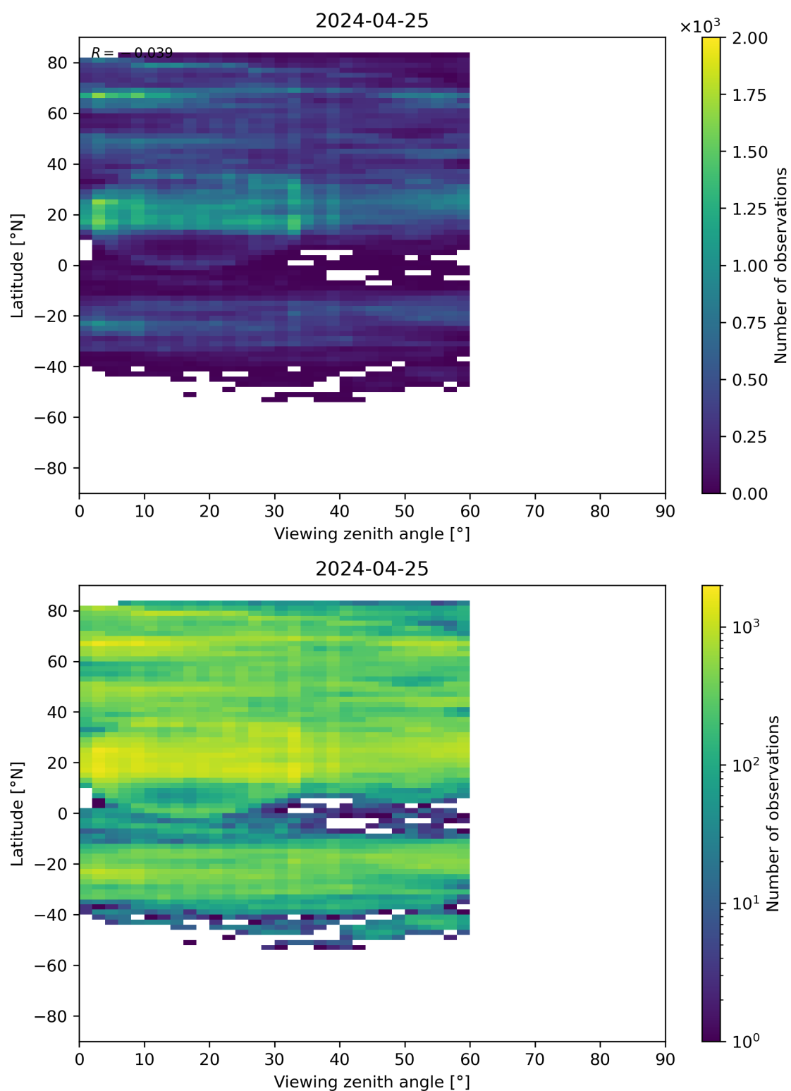
Figure 109: Scatter density plot of “Viewing zenith angle” against “Latitude” for 2024-04-24 to 2024-04-26.
