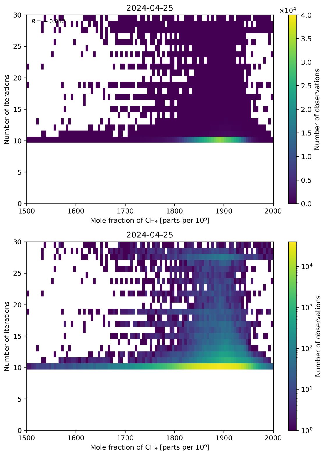
Figure 76: Scatter density plot of “Mole fraction of CH 4 ” against “Number of iterations” for 2024-04-24 to 2024-04-26.
