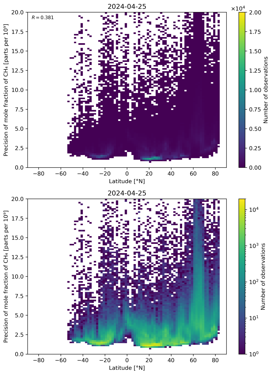
Figure 59: Scatter density plot of “Latitude” against “Precision of mole fraction of \text{CH}_4 ” for 2024-04-24 to 2024-04-26.
