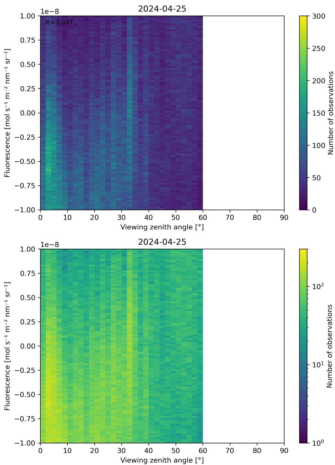
Figure 108: Scatter density plot of “Viewing zenith angle” against “Fluorescence” for 2024-04-24 to 2024-04-26.
