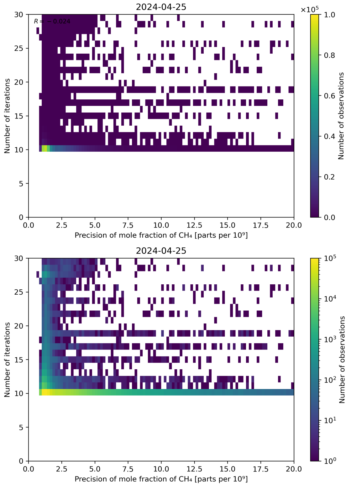
Figure 83: Scatter density plot of “Precision of mole fraction of CH 4 ” against “Number of iterations” for 2024-04-24 to 2024-04-26.
