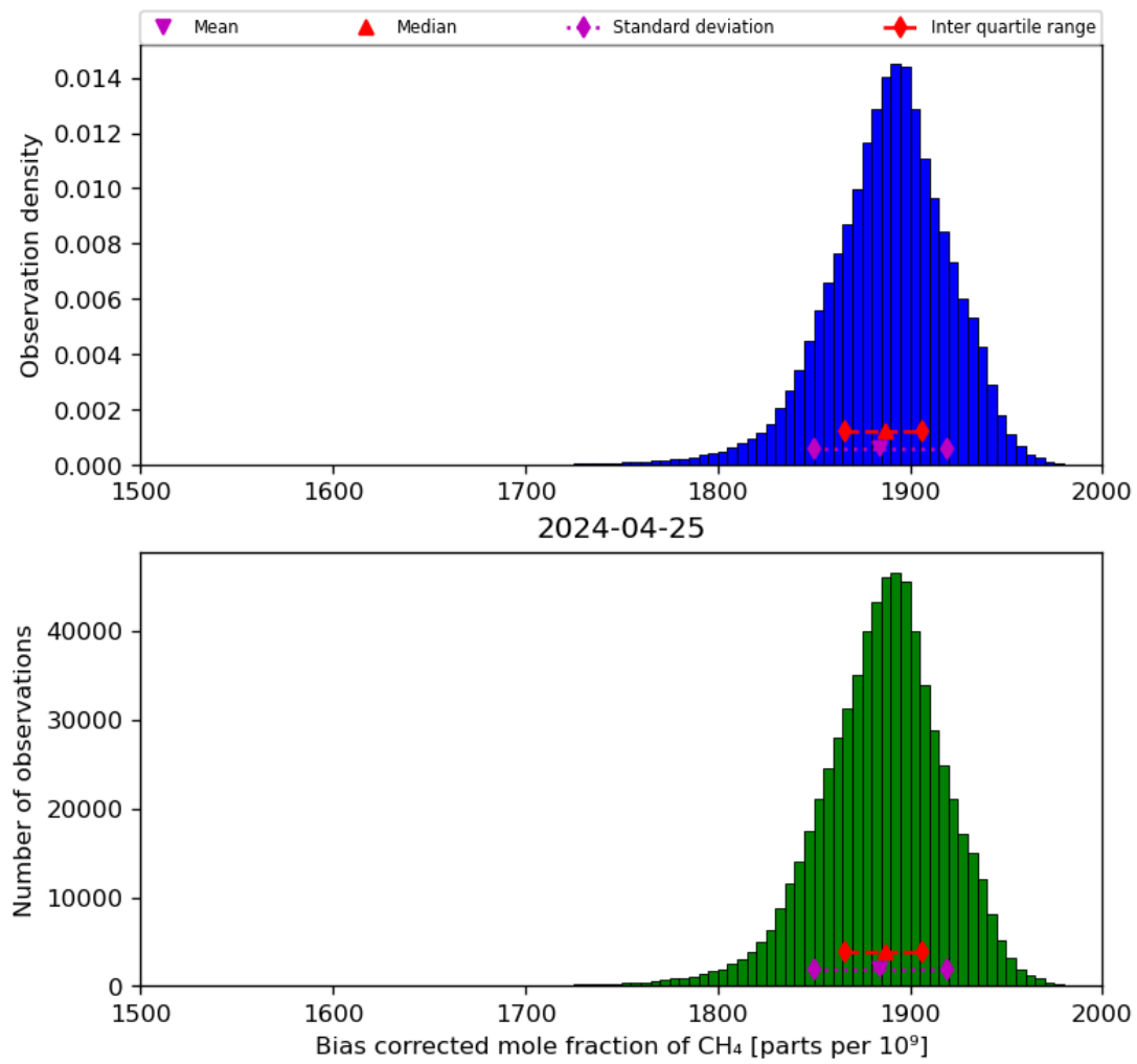
Figure 25: Histogram of “Bias corrected mole fraction of CH 4 ” for 2024-04-24 to 2024-04-26
