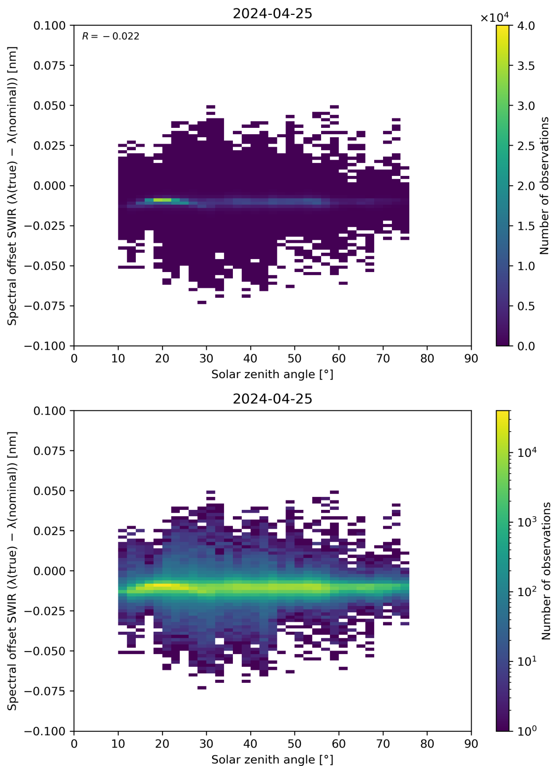
Figure 104: Scatter density plot of “Solar zenith angle” against “Spectral offset SWIR ( \lambda(\text{true}) - \lambda(\text{nominal}) )” for 2024-04-24 to 2024-04-26.
