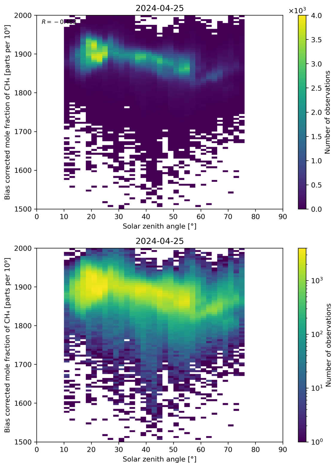
Figure 100: Scatter density plot of “Solar zenith angle” against “Bias corrected mole fraction of \text{CH}_4 ” for 2024-04-24 to 2024-04-26.
