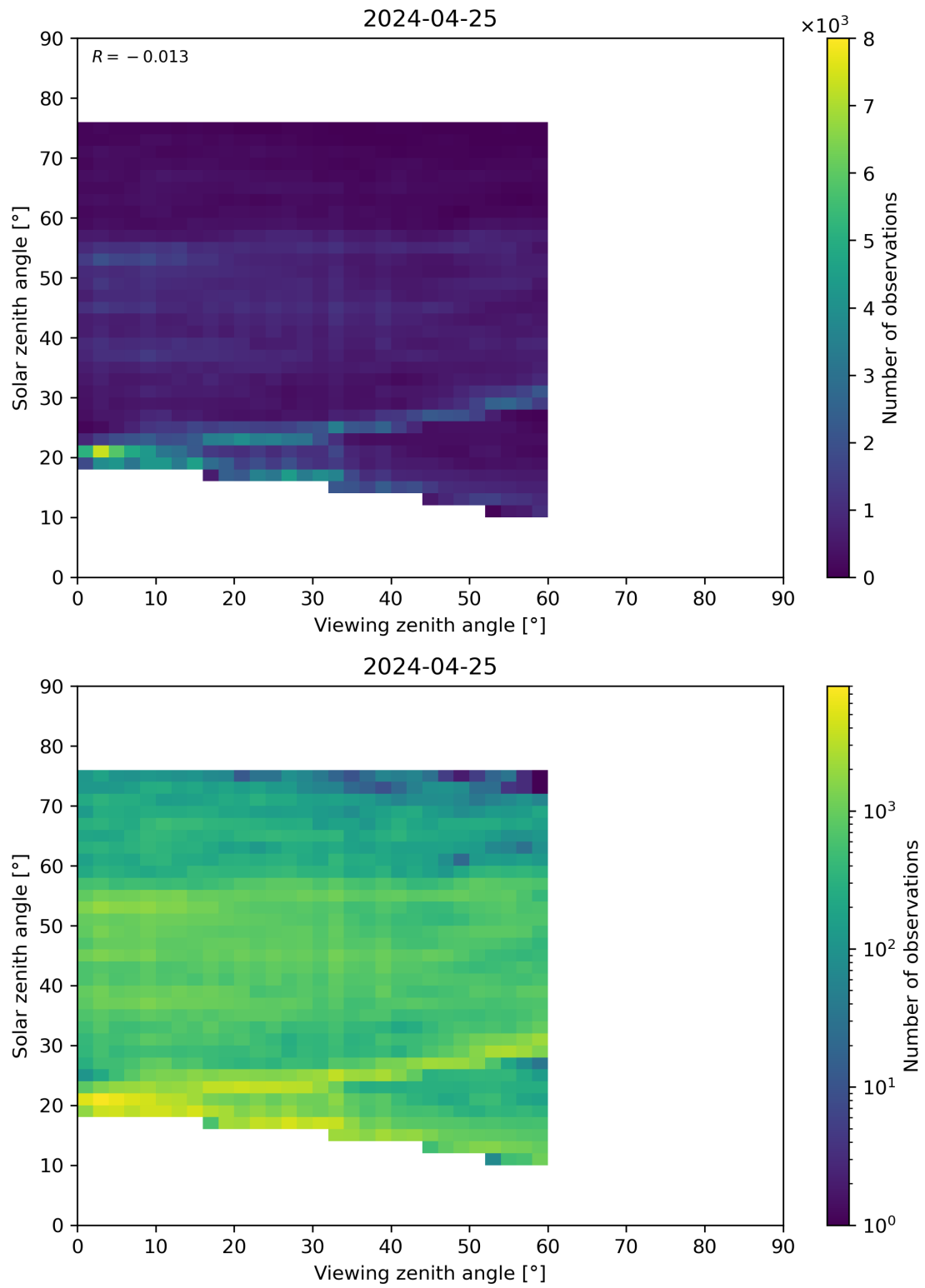
Figure 115: Scatter density plot of “Viewing zenith angle” against “Solar zenith angle” for 2024-04-24 to 2024-04-26.
