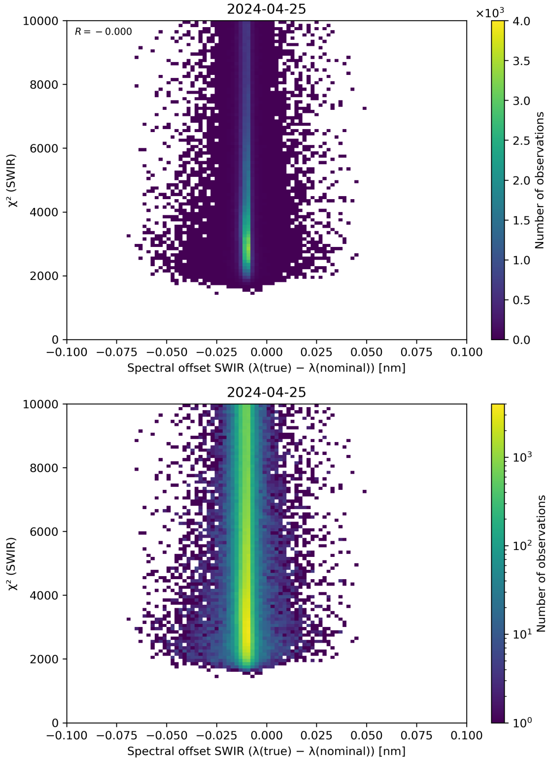
Figure 118: Scatter density plot of “Spectral offset SWIR ( \lambda(\text{true}) - \lambda(\text{nominal}) )” against “ \chi^2 (SWIR)” for 2024-04-24 to 2024-04-26.
