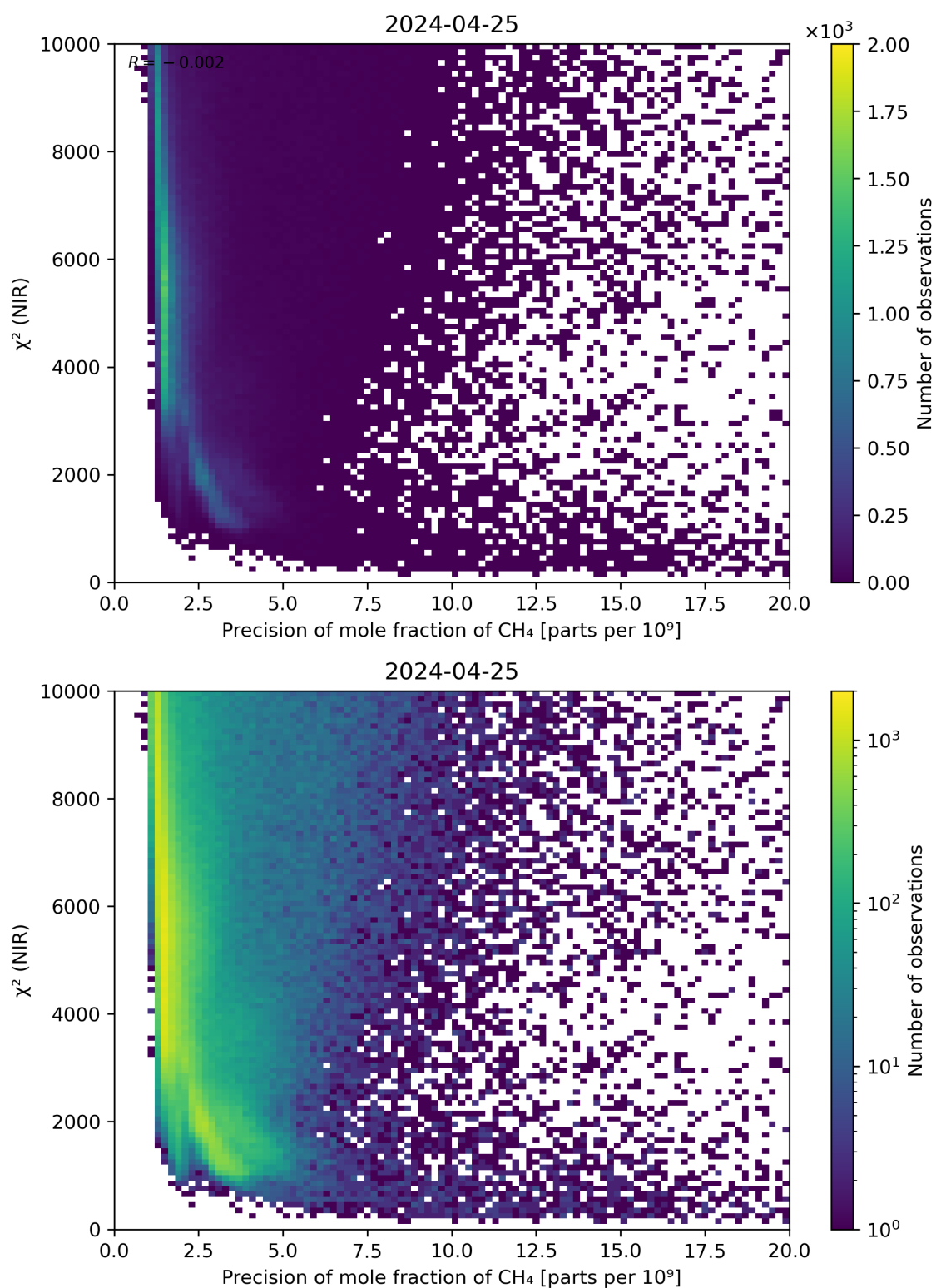
Figure 78: Scatter density plot of “Precision of mole fraction of CH 4 ” against “ \chi^2 (NIR)” for 2024-04-24 to 2024-04-26.
