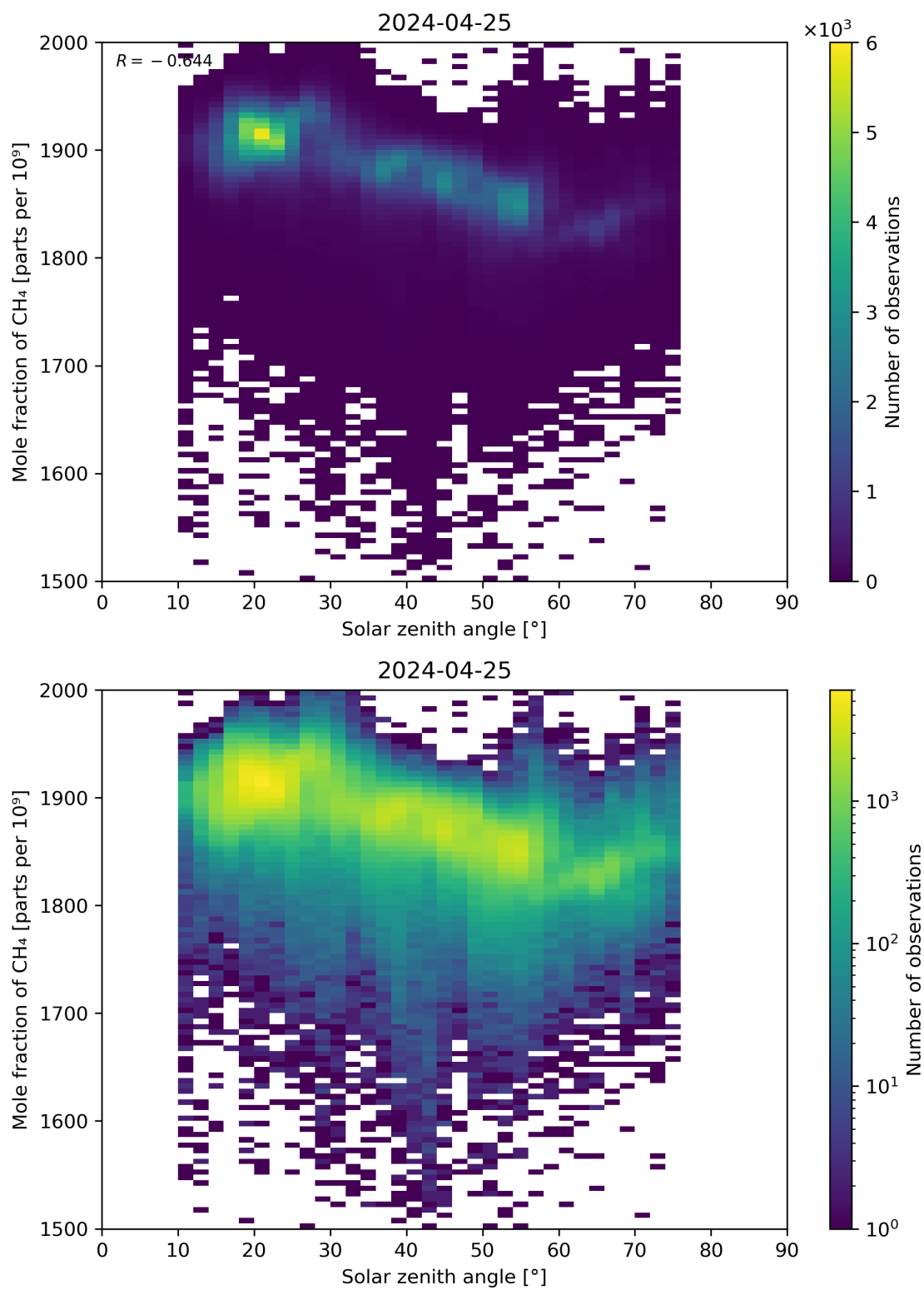
Figure 99: Scatter density plot of “Solar zenith angle” against “Mole fraction of CH 4 ” for 2024-04-24 to 2024-04-26.
