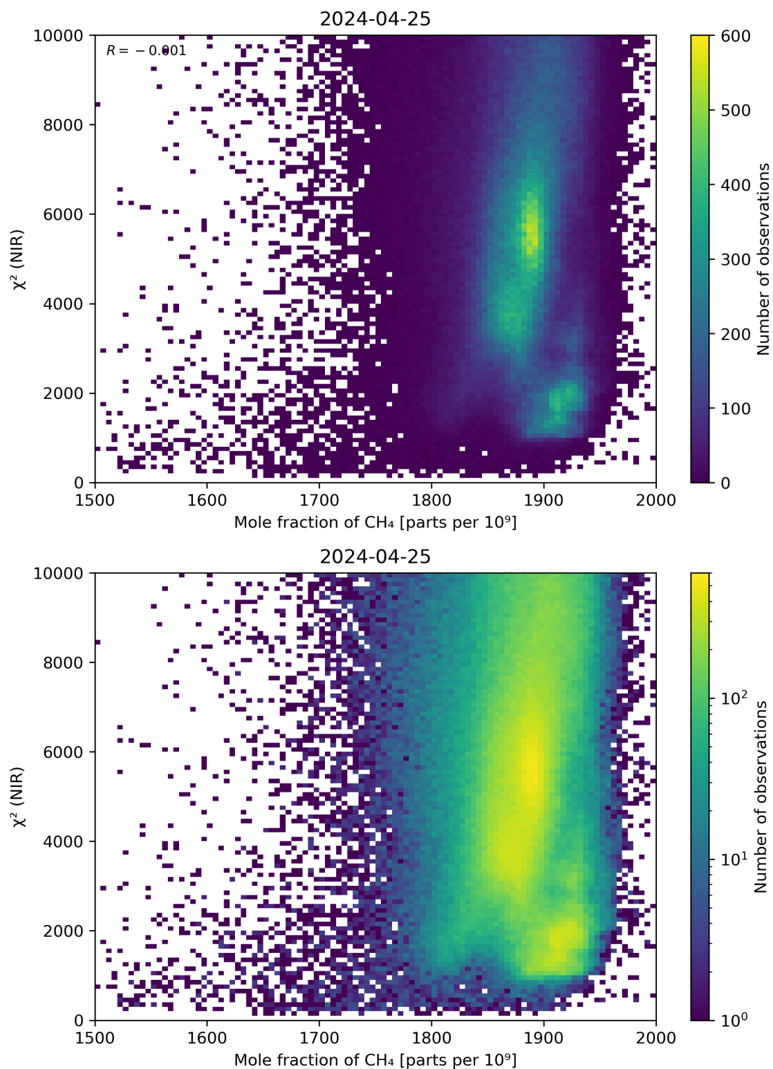
Figure 70: Scatter density plot of “Mole fraction of CH 4 ” against “ \chi^2 (NIR)” for 2024-04-24 to 2024-04-26.
