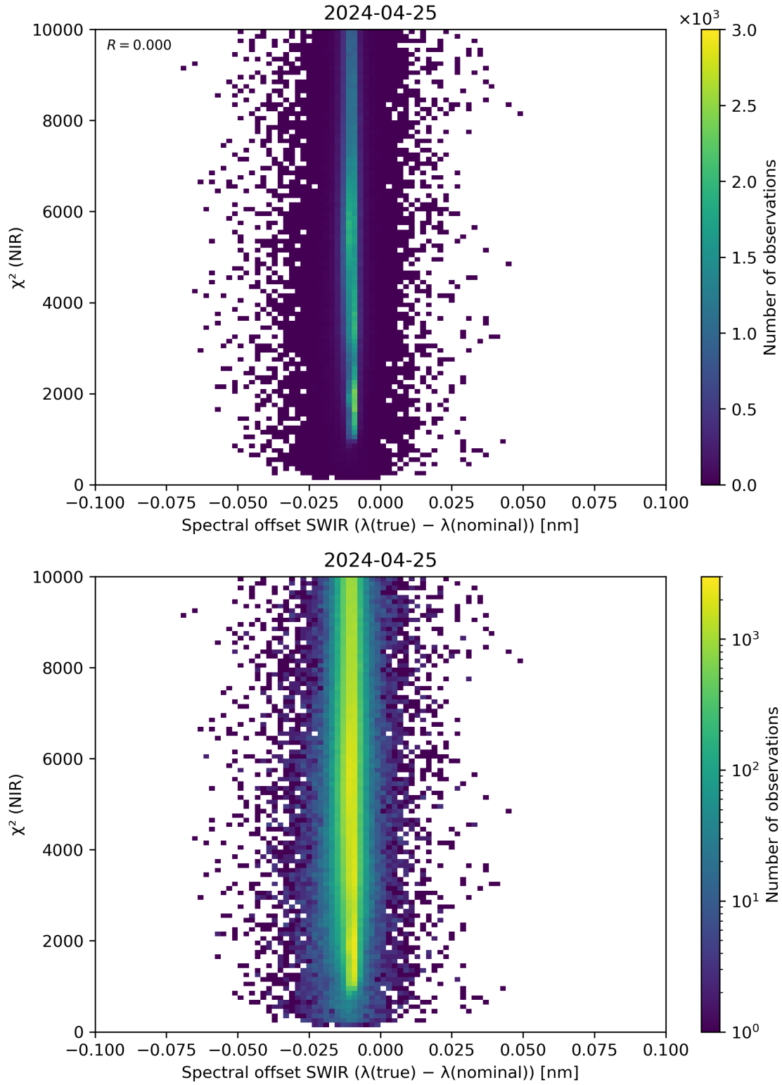
Figure 117: Scatter density plot of “Spectral offset SWIR ( \lambda(\text{true}) - \lambda(\text{nominal}) )” against “ \chi^2 (NIR)” for 2024-04-24 to 2024-04-26.
