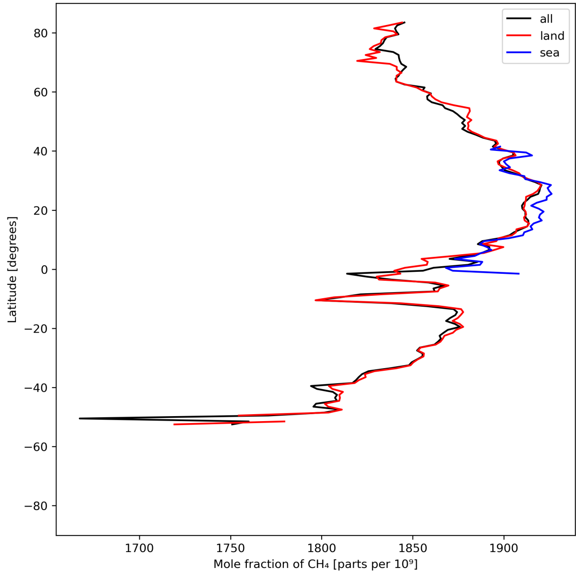
Figure 12: Zonal average of “Mole fraction of \text{CH}_4 ” for 2024-04-24 to 2024-04-26.
