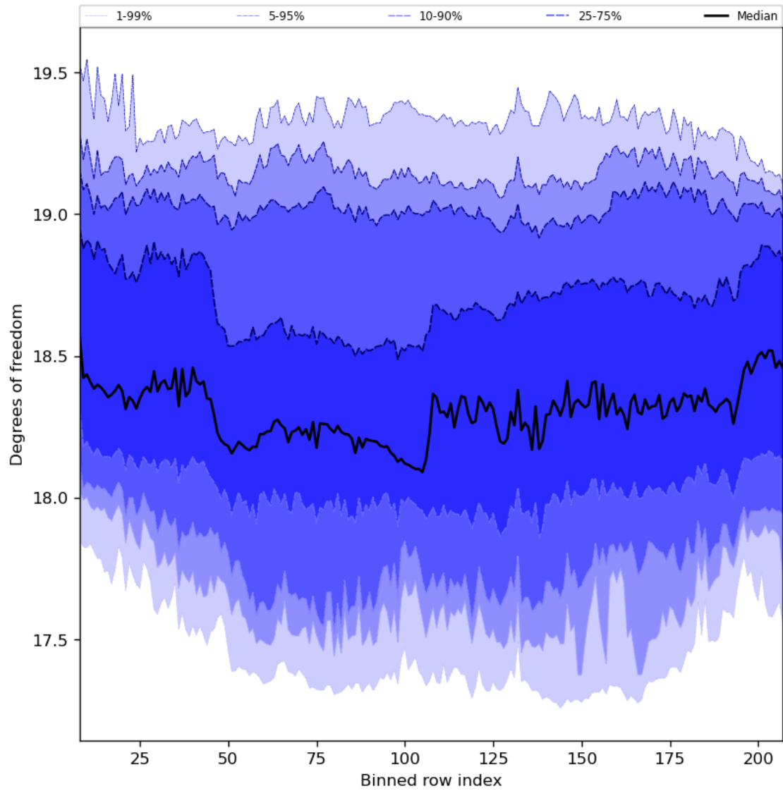
Figure 41: Along track statistics of “Degrees of freedom” for 2024-04-24 to 2024-04-26
