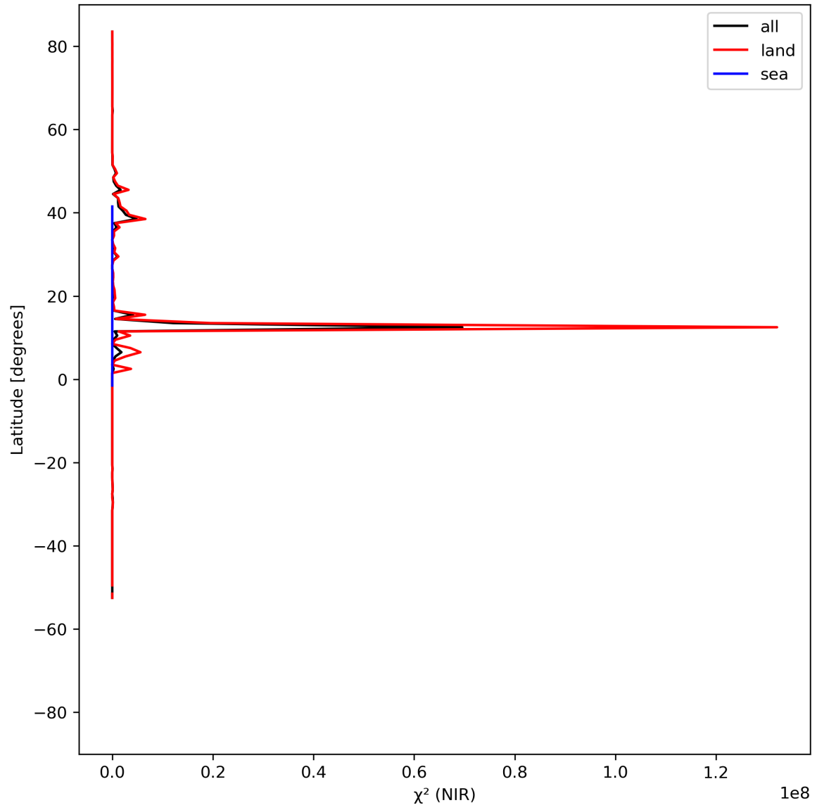
Figure 18: Zonal average of “ \chi^2 (NIR)” for 2024-04-24 to 2024-04-26.
