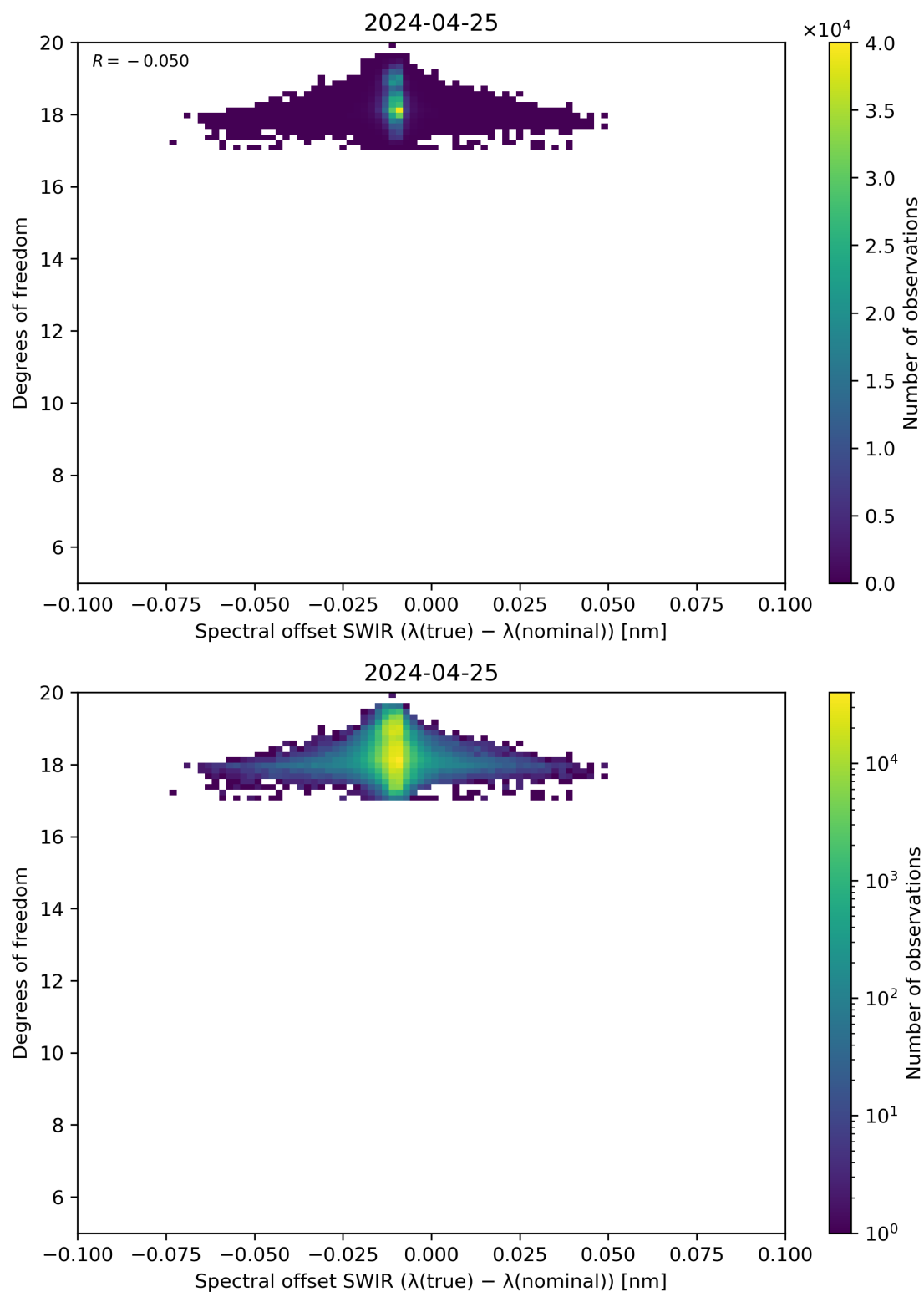
Figure 119: Scatter density plot of “Spectral offset SWIR ( \lambda(\text{true}) - \lambda(\text{nominal}) )” against “Degrees of freedom” for 2024-04-24 to 2024-04-26.
