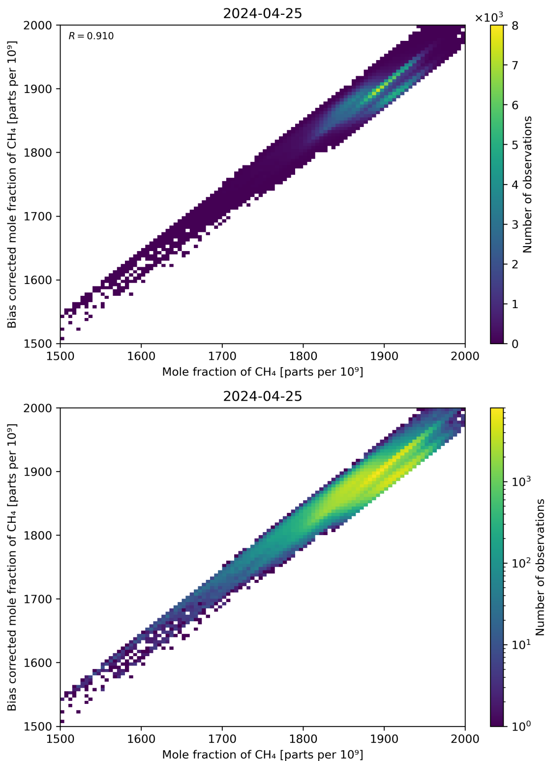
Figure 74: Scatter density plot of “Mole fraction of CH 4 ” against “Bias corrected mole fraction of CH 4 ” for 2024-04-24 to 2024-04-26.
