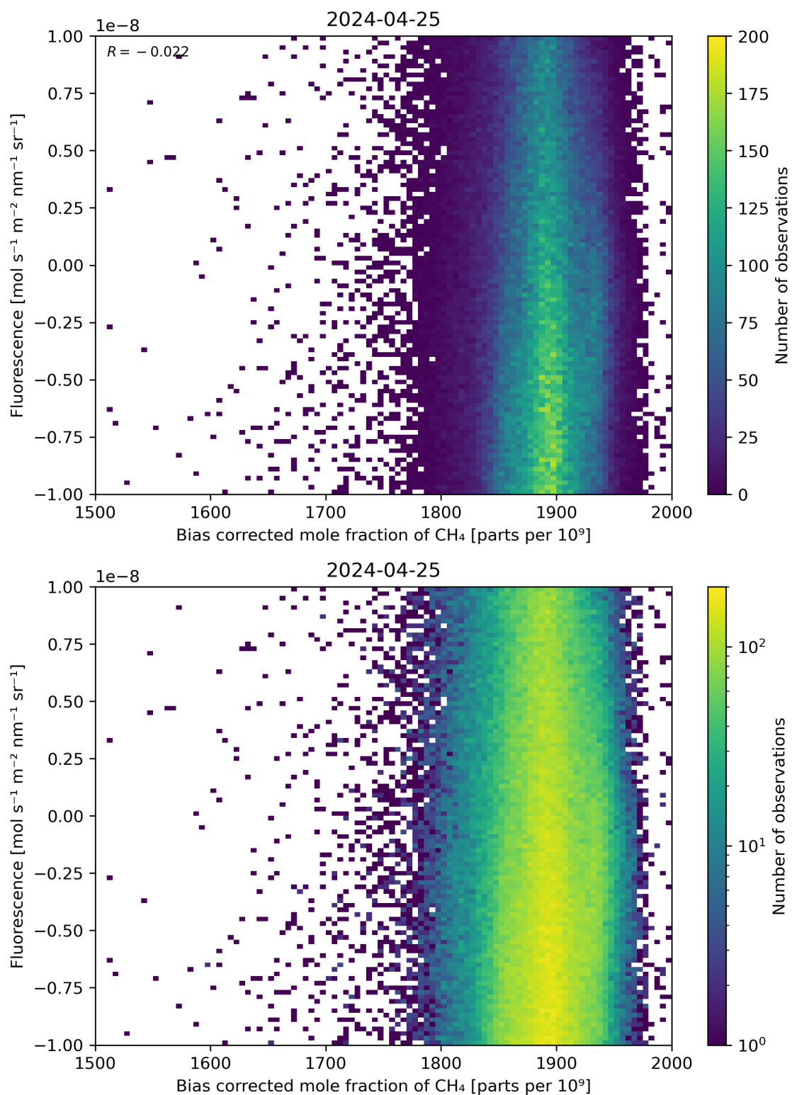
Figure 66: Scatter density plot of “Bias corrected mole fraction of \text{CH}_4 ” against “Fluorescence” for 2024-04-24 to 2024-04-26.
