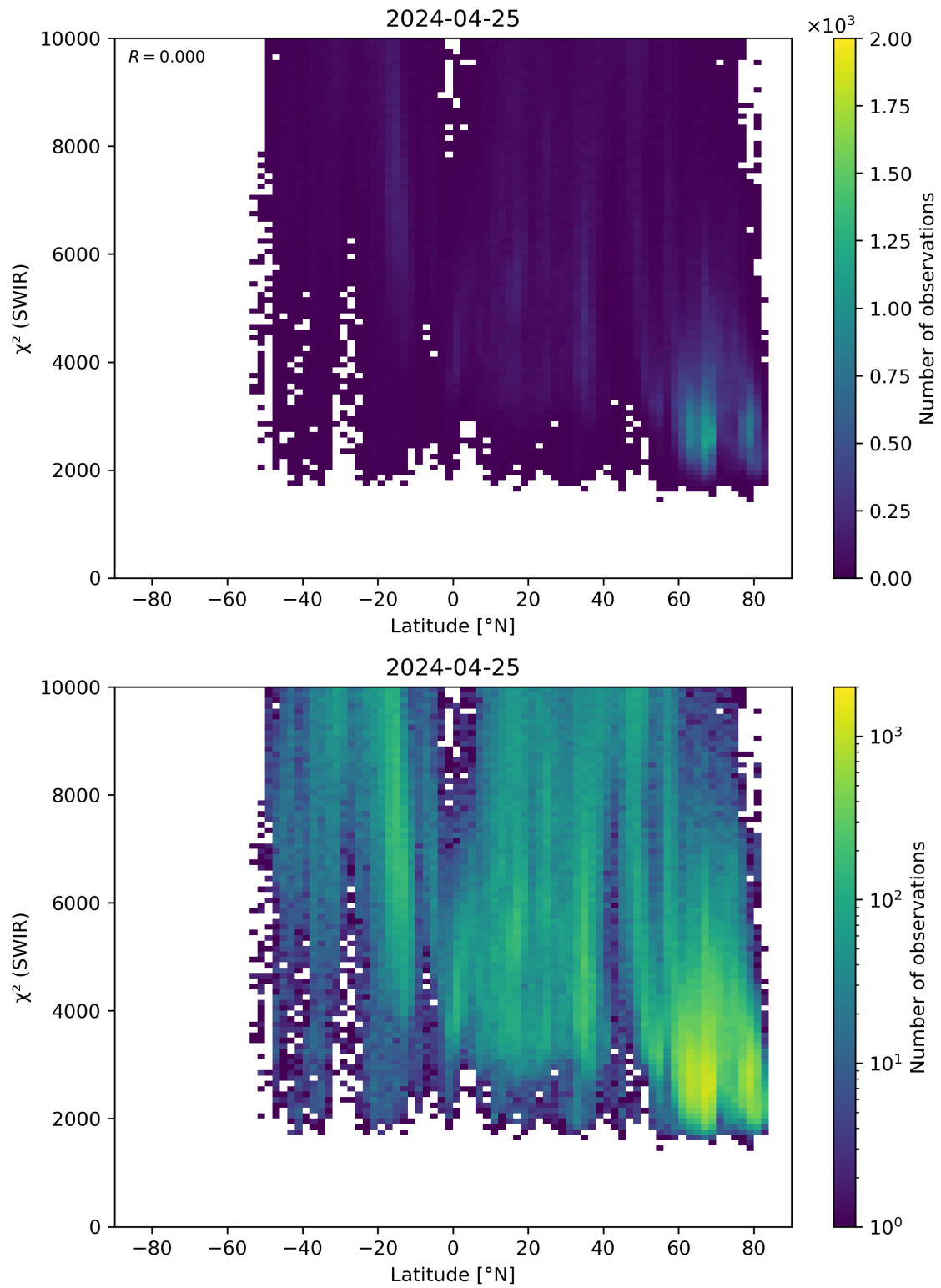
Figure 54: Scatter density plot of “Latitude” against “ \chi^2 (SWIR)” for 2024-04-24 to 2024-04-26.
