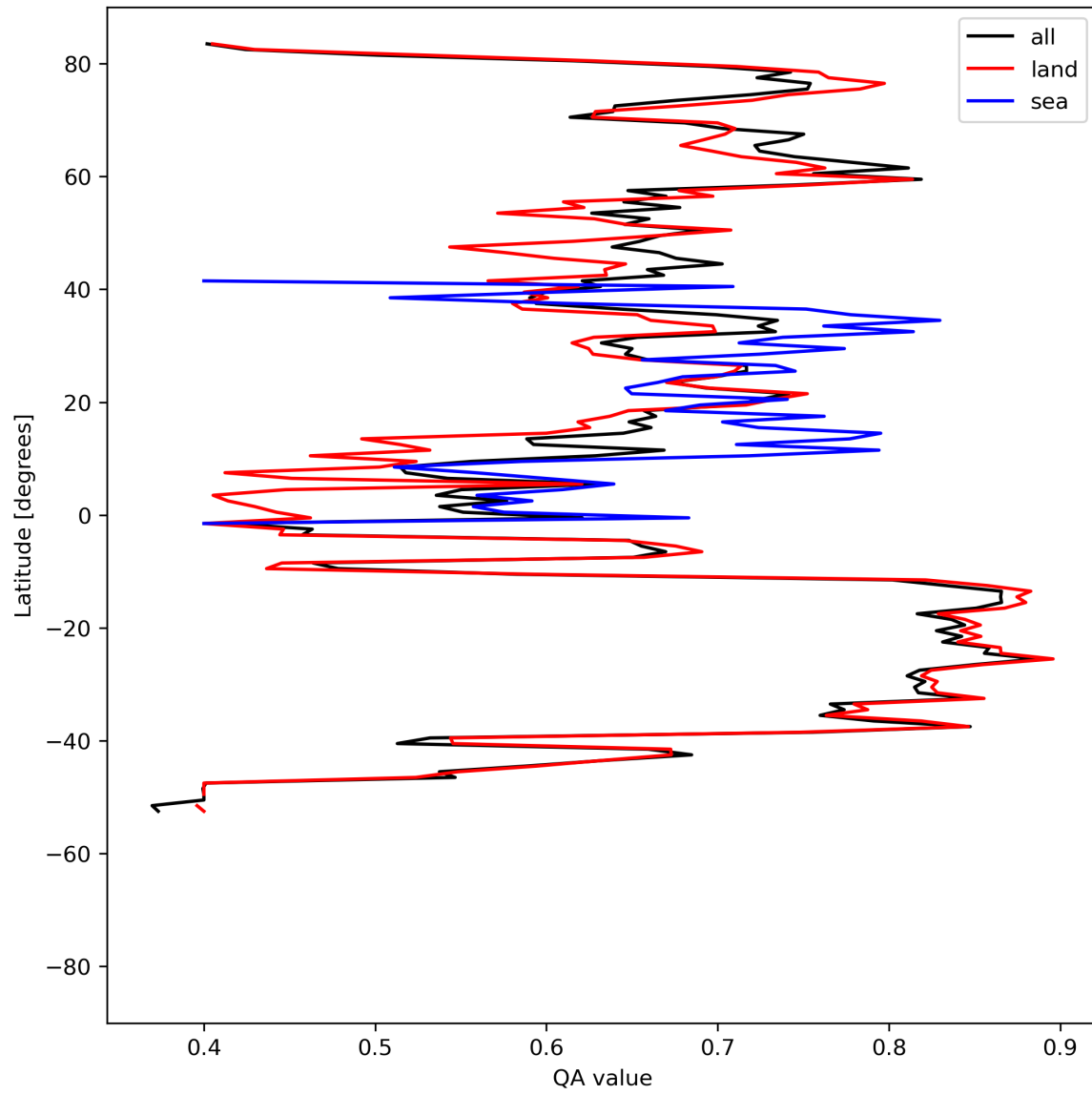
Figure 11: Zonal average of “QA value” for 2024-04-24 to 2024-04-26.
