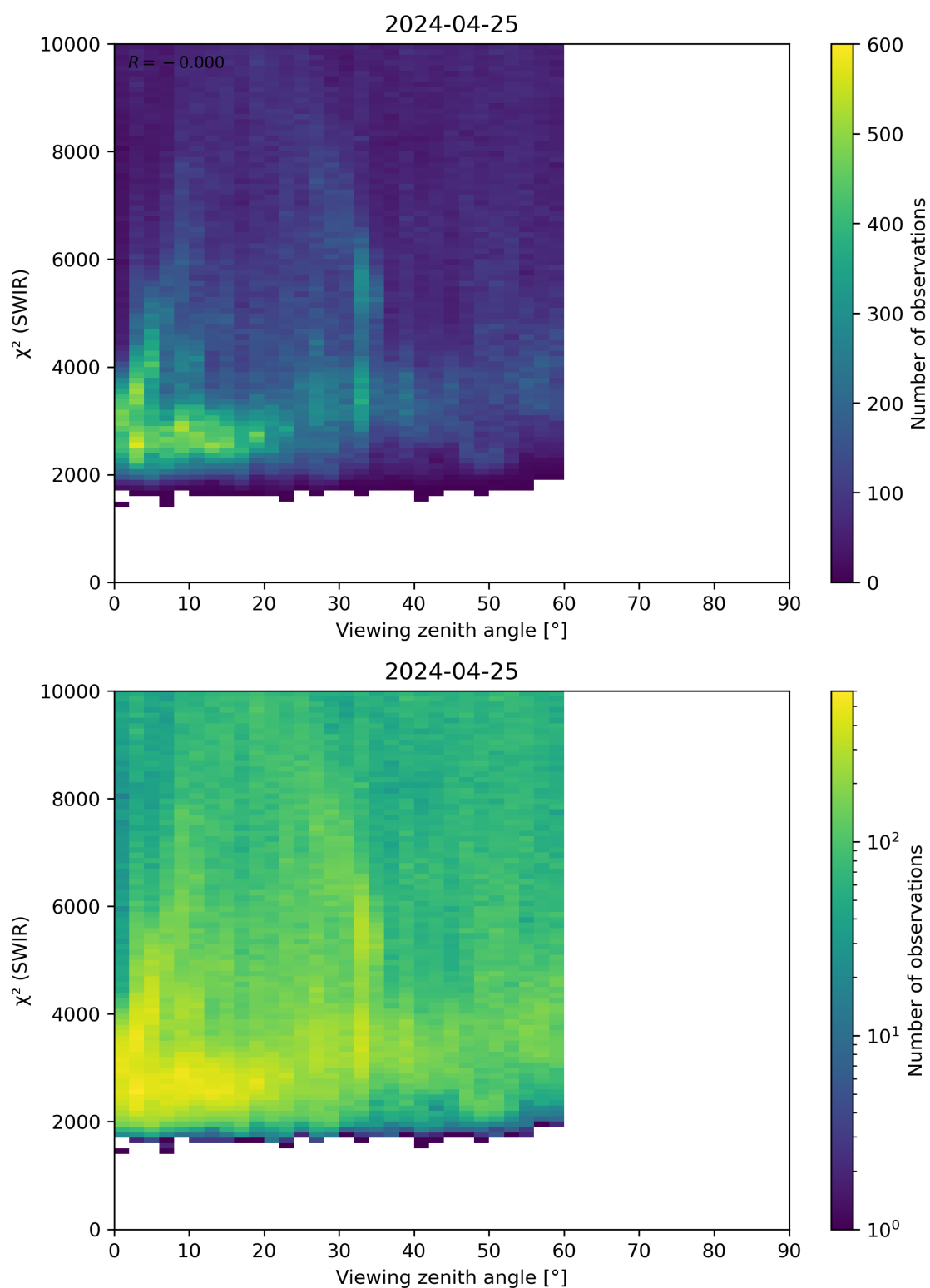
Figure 106: Scatter density plot of “Viewing zenith angle” against “ \chi^2 (SWIR)” for 2024-04-24 to 2024-04-26.
