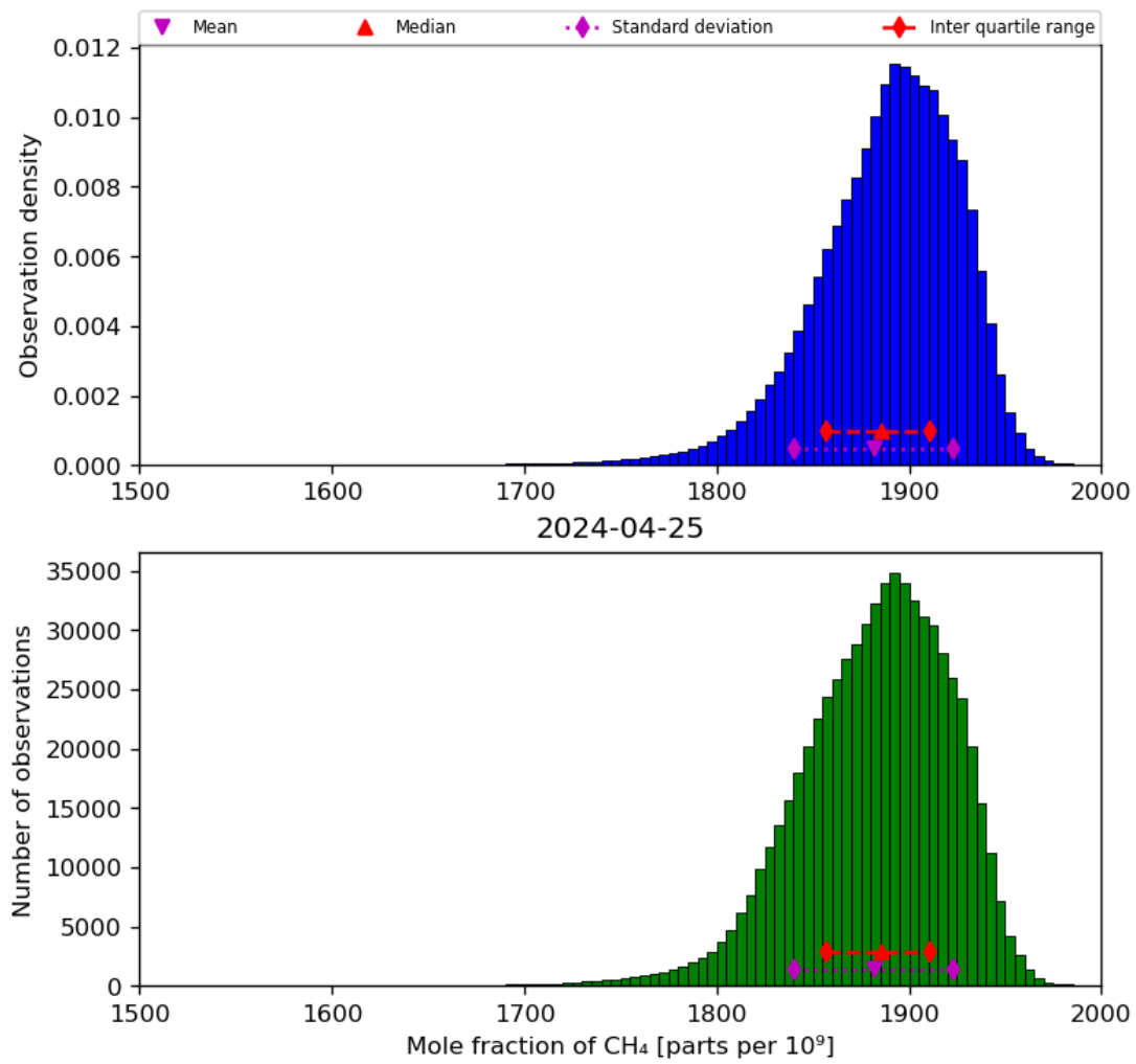
Figure 23: Histogram of “Mole fraction of CH 4 ” for 2024-04-24 to 2024-04-26
