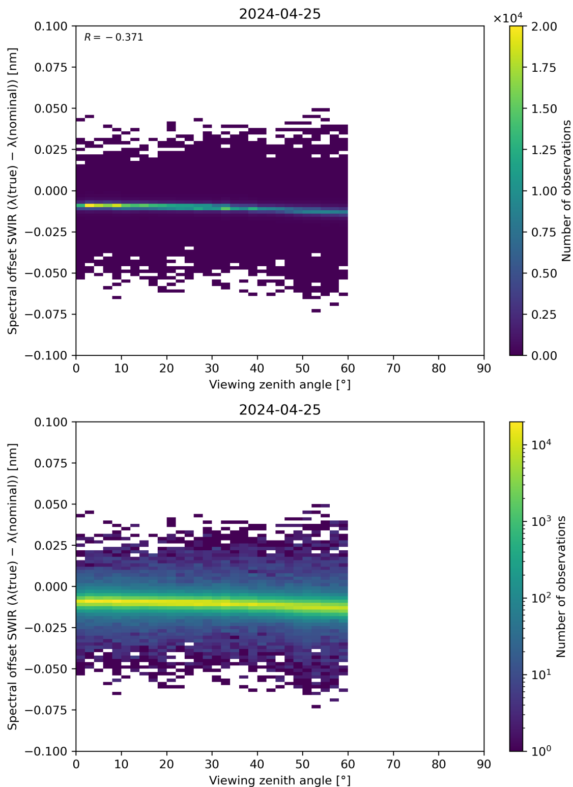
Figure 116: Scatter density plot of “Viewing zenith angle” against “Spectral offset SWIR ( \lambda(\text{true}) - \lambda(\text{nominal}) )” for 2024-04-24 to 2024-04-26.
