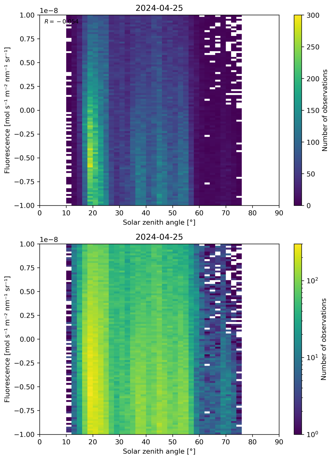
Figure 97: Scatter density plot of “Solar zenith angle” against “Fluorescence” for 2024-04-24 to 2024-04-26.
