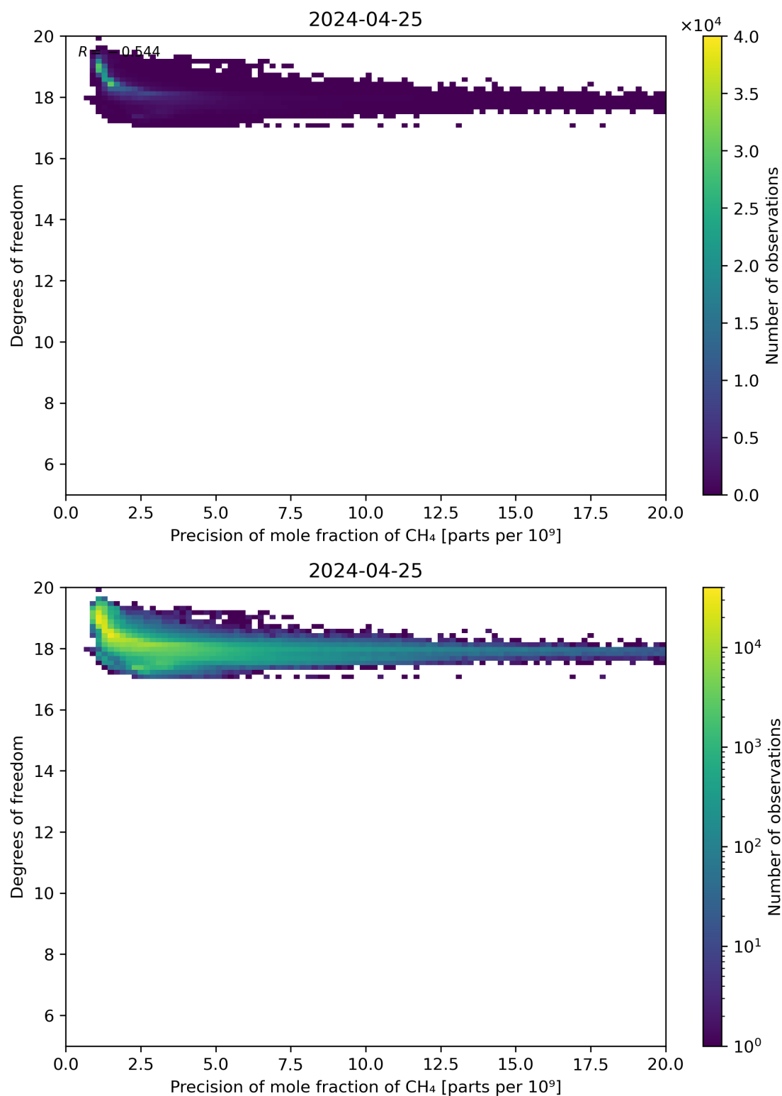
Figure 80: Scatter density plot of “Precision of mole fraction of CH 4 ” against “Degrees of freedom” for 2024-04-24 to 2024-04-26.
