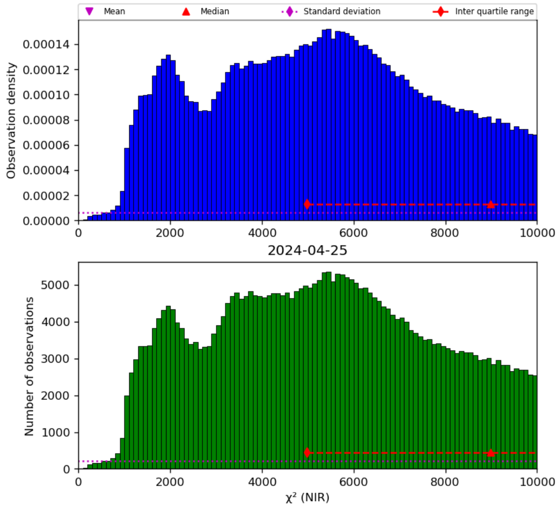
Figure 29: Histogram of “ \chi^2 (NIR)” for 2024-04-24 to 2024-04-26
