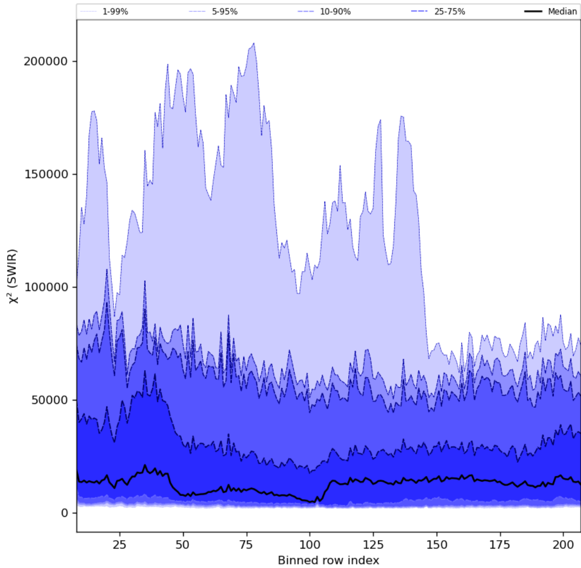
Figure 39: Along track statistics of “ \chi^2 (SWIR)” for 2024-04-24 to 2024-04-26
