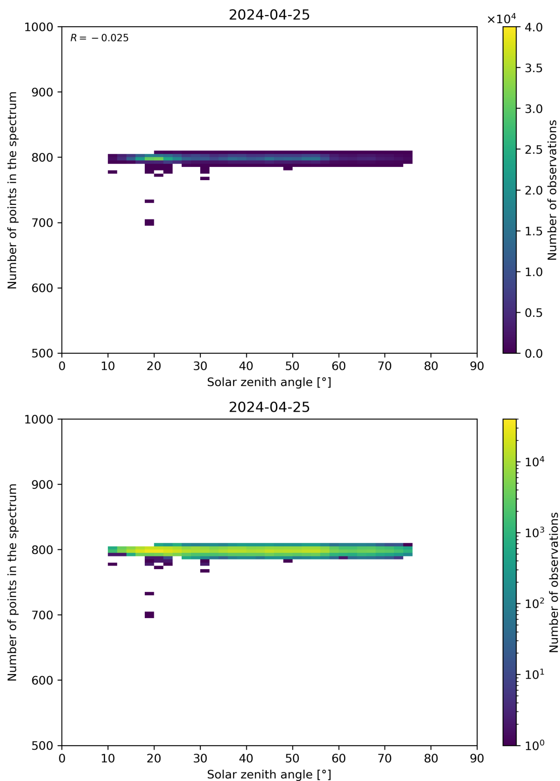
Figure 103: Scatter density plot of “Solar zenith angle” against “Number of points in the spectrum” for 2024-04-24 to 2024-04-26.
