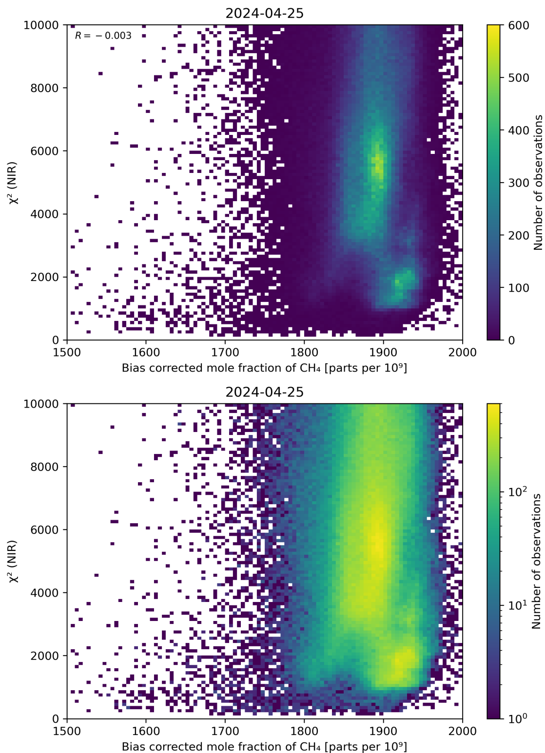
Figure 63: Scatter density plot of “Bias corrected mole fraction of CH 4 ” against “ \chi^2 (NIR)” for 2024-04-24 to 2024-04-26.
