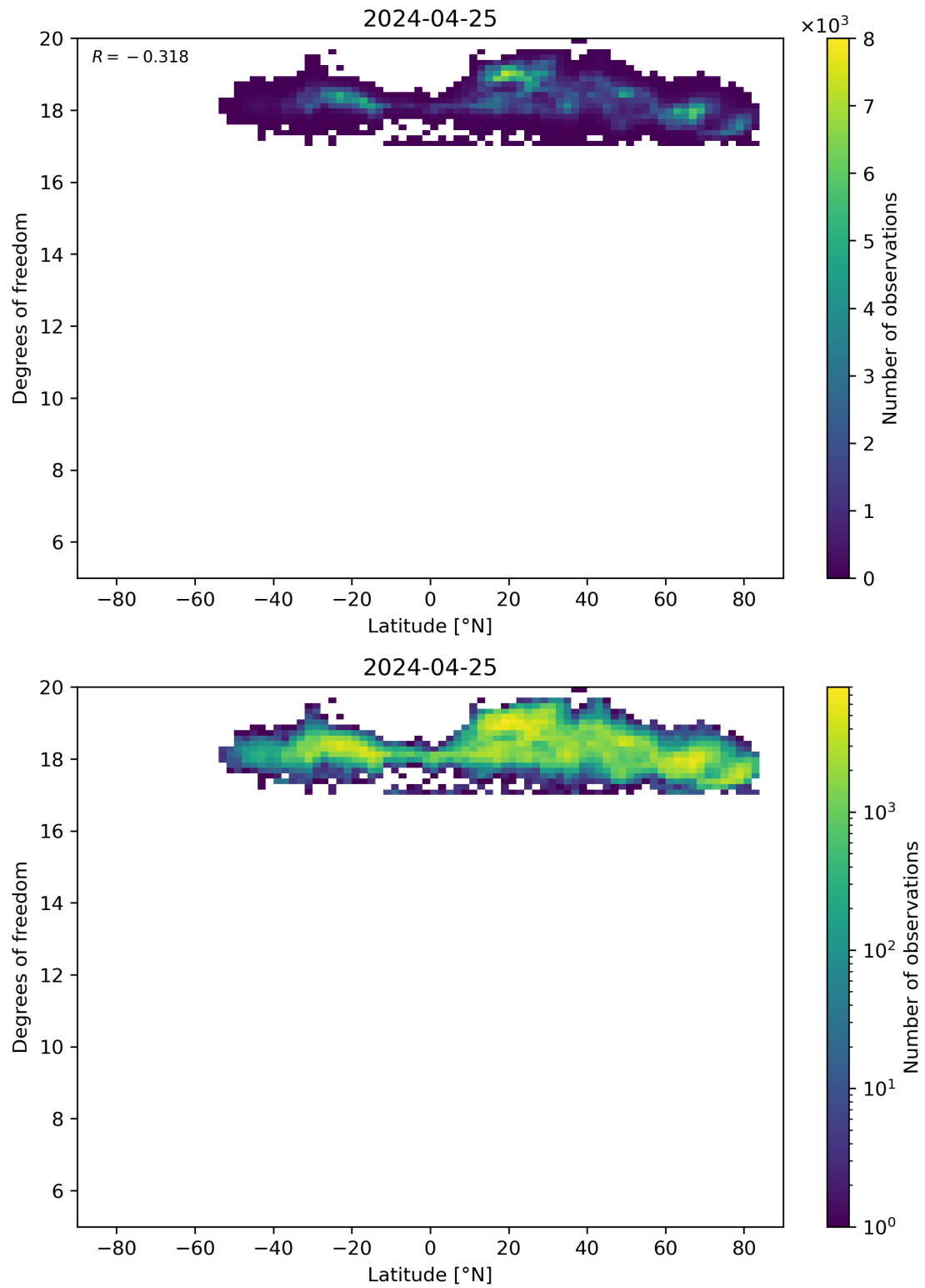
Figure 55: Scatter density plot of “Latitude” against “Degrees of freedom” for 2024-04-24 to 2024-04-26.
