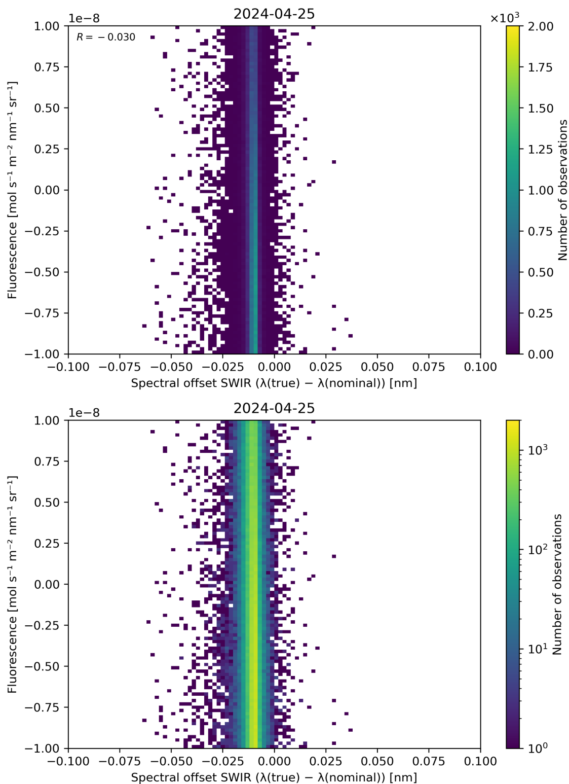
Figure 120: Scatter density plot of “Spectral offset SWIR ( \lambda(\text{true}) - \lambda(\text{nominal}) )” against “Fluorescence” for 2024-04-24 to 2024-04-26.
