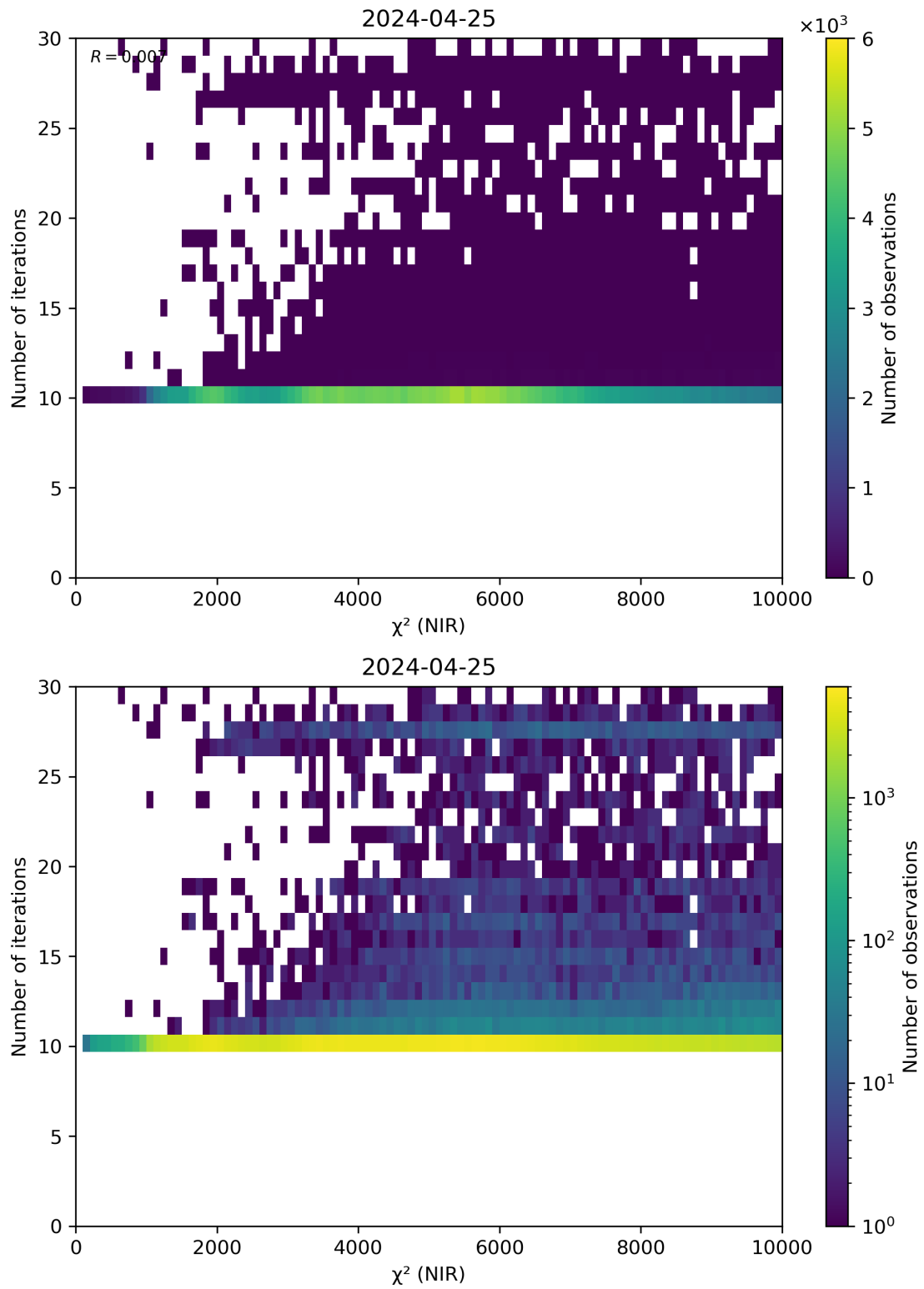
Figure 46: Scatter density plot of “ \chi^2 (NIR)” against “Number of iterations” for 2024-04-24 to 2024-04-26.
