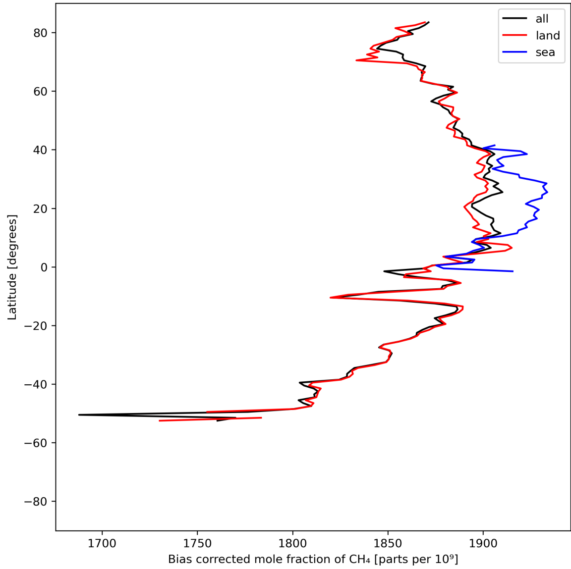
Figure 14: Zonal average of “Bias corrected mole fraction of \text{CH}_4 ” for 2024-04-24 to 2024-04-26.
