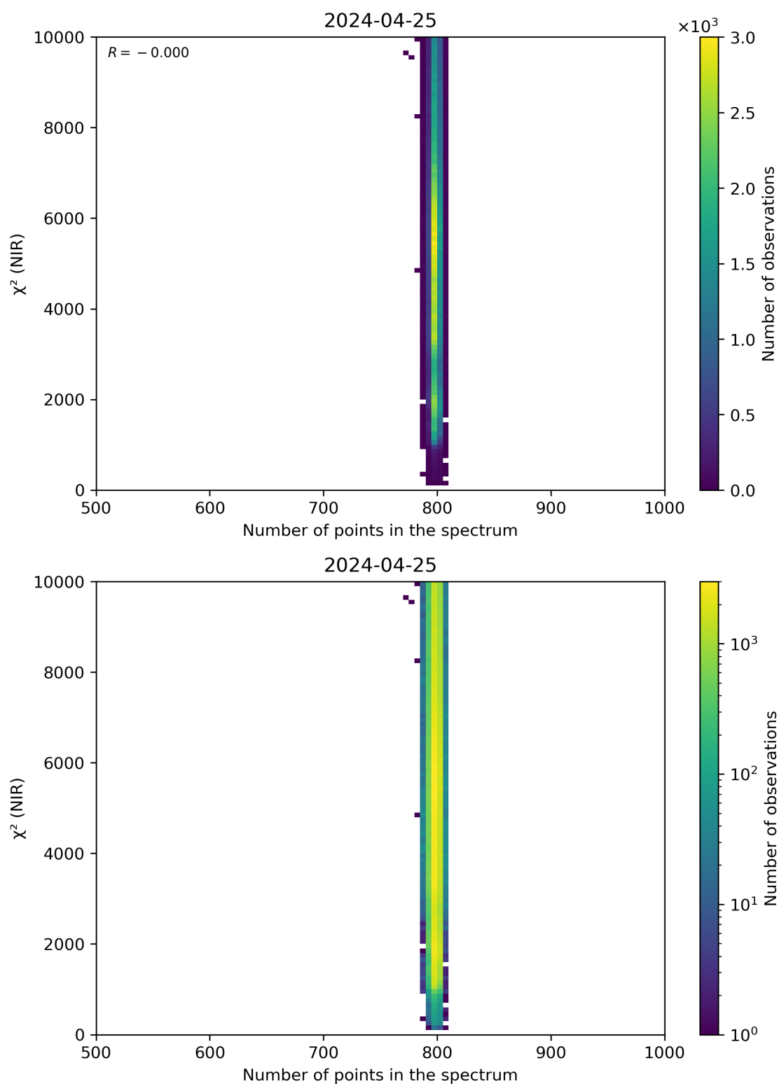
Figure 88: Scatter density plot of “Number of points in the spectrum” against “ \chi^2 (NIR)” for 2024-04-24 to 2024-04-26.
