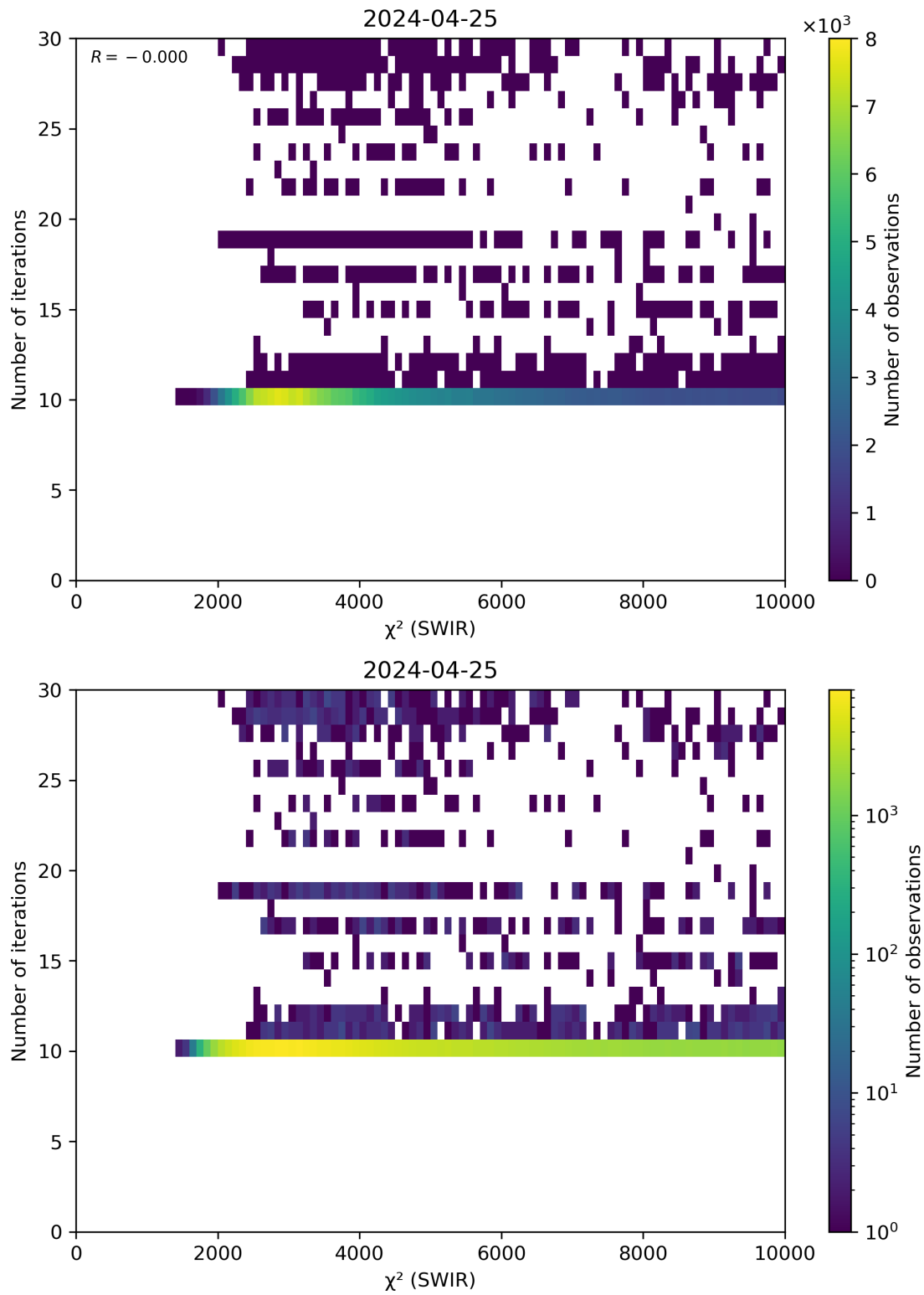
Figure 50: Scatter density plot of “ \chi^2 (SWIR)” against “Number of iterations” for 2024-04-24 to 2024-04-26.
