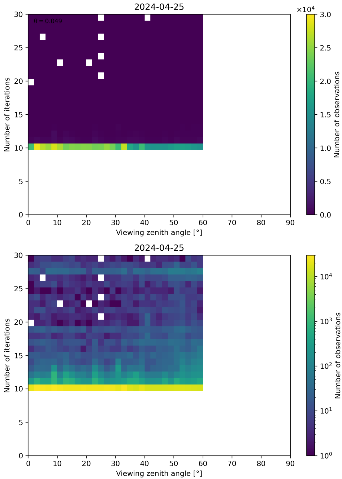
Figure 113: Scatter density plot of “Viewing zenith angle” against “Number of iterations” for 2024-04-24 to 2024-04-26.
