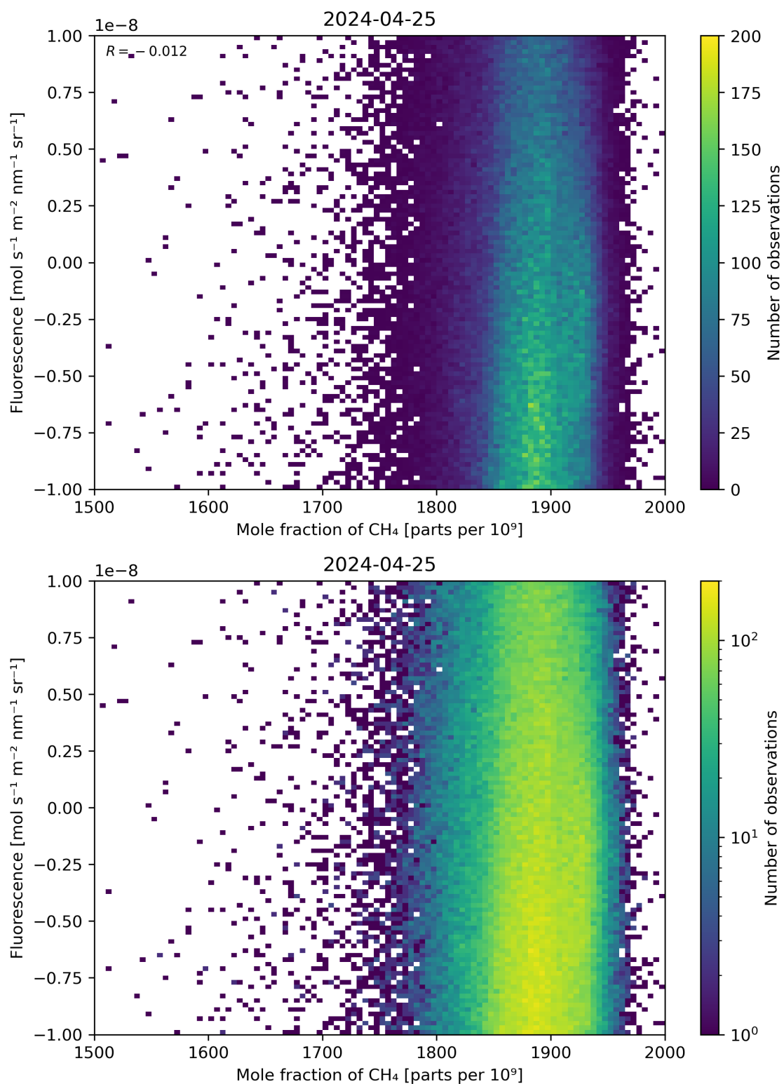
Figure 73: Scatter density plot of “Mole fraction of \text{CH}_4 ” against “Fluorescence” for 2024-04-24 to 2024-04-26.
