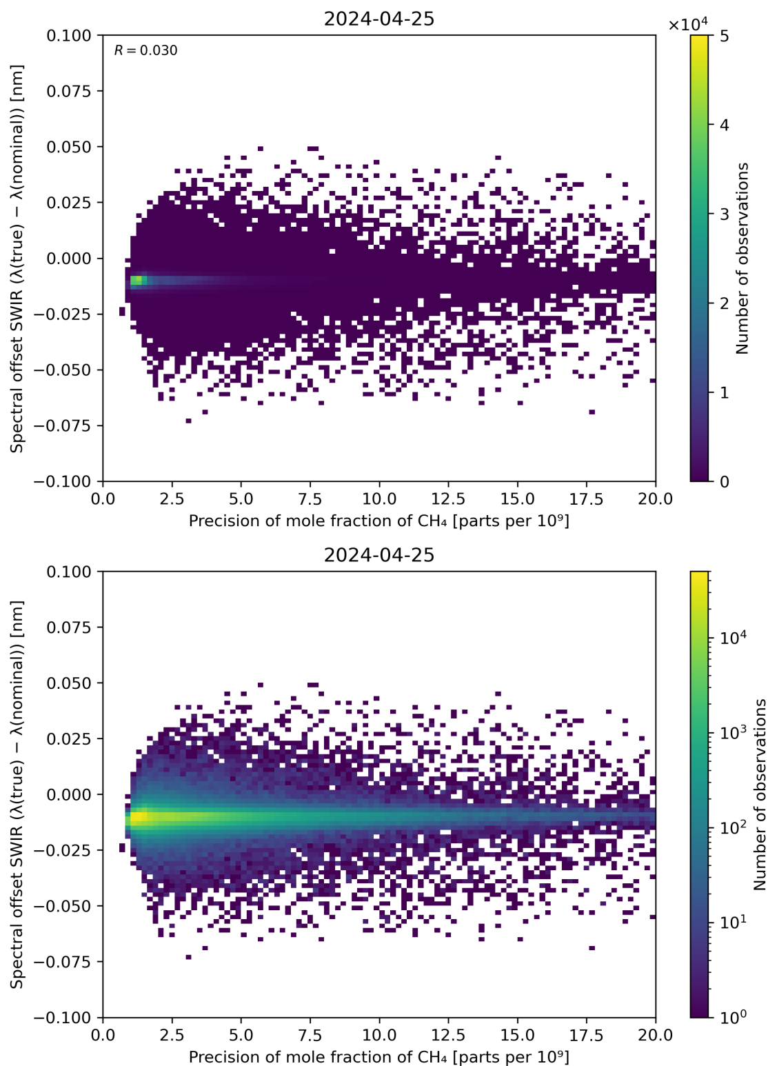
Figure 85: Scatter density plot of “Precision of mole fraction of \text{CH}_4 ” against “Spectral offset SWIR ( \lambda(\text{true}) - \lambda(\text{nominal}) )” for 2024-04-24 to 2024-04-26.
