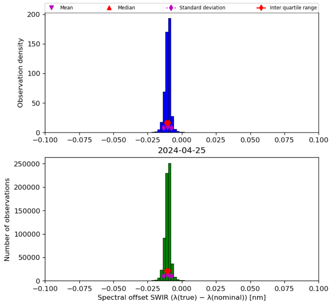
Figure 27: Histogram of “Spectral offset SWIR ( \lambda(\text{true}) - \lambda(\text{nominal}) )” for 2024-04-24 to 2024-04-26
