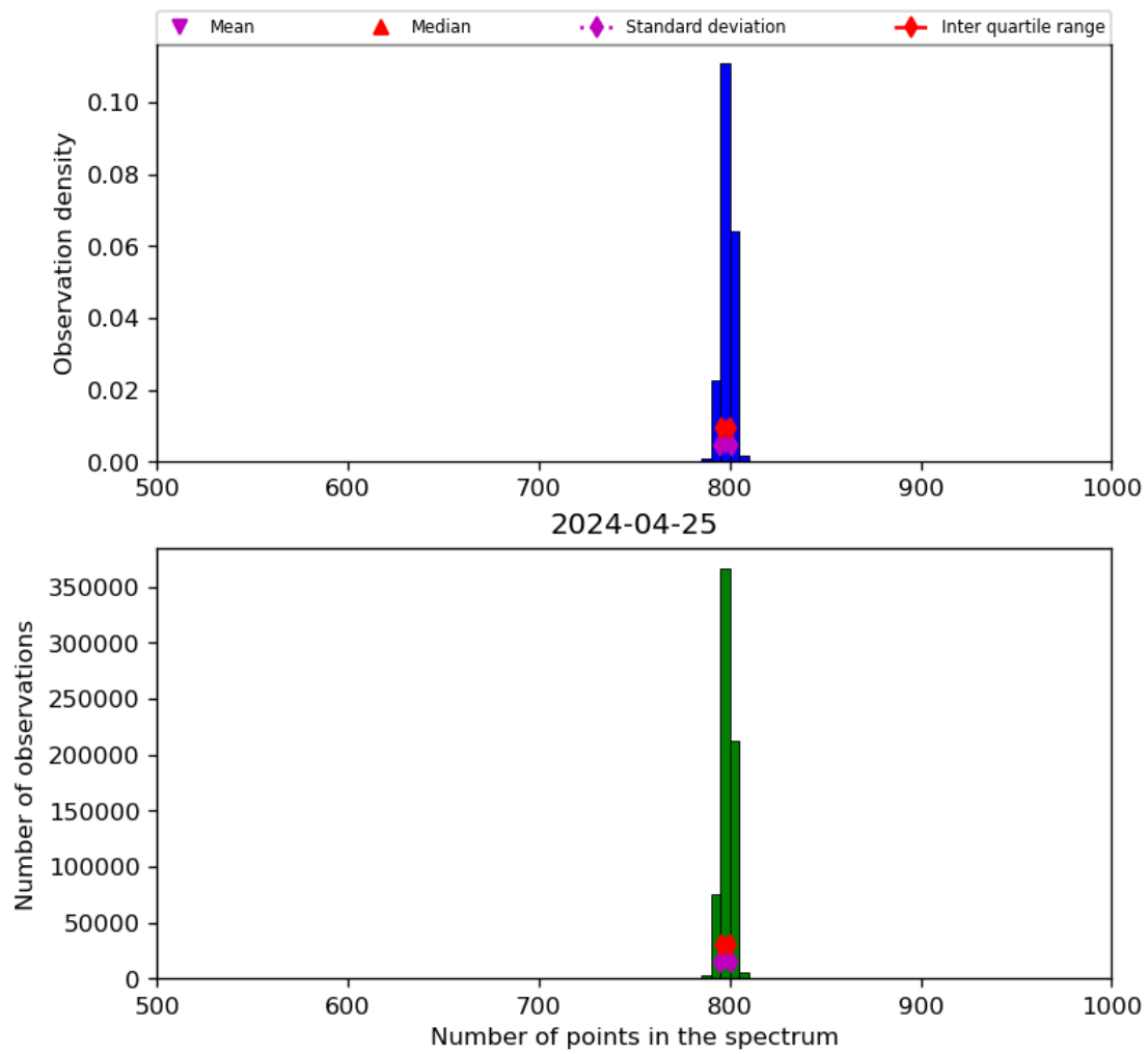
Figure 26: Histogram of “Number of points in the spectrum” for 2024-04-24 to 2024-04-26
