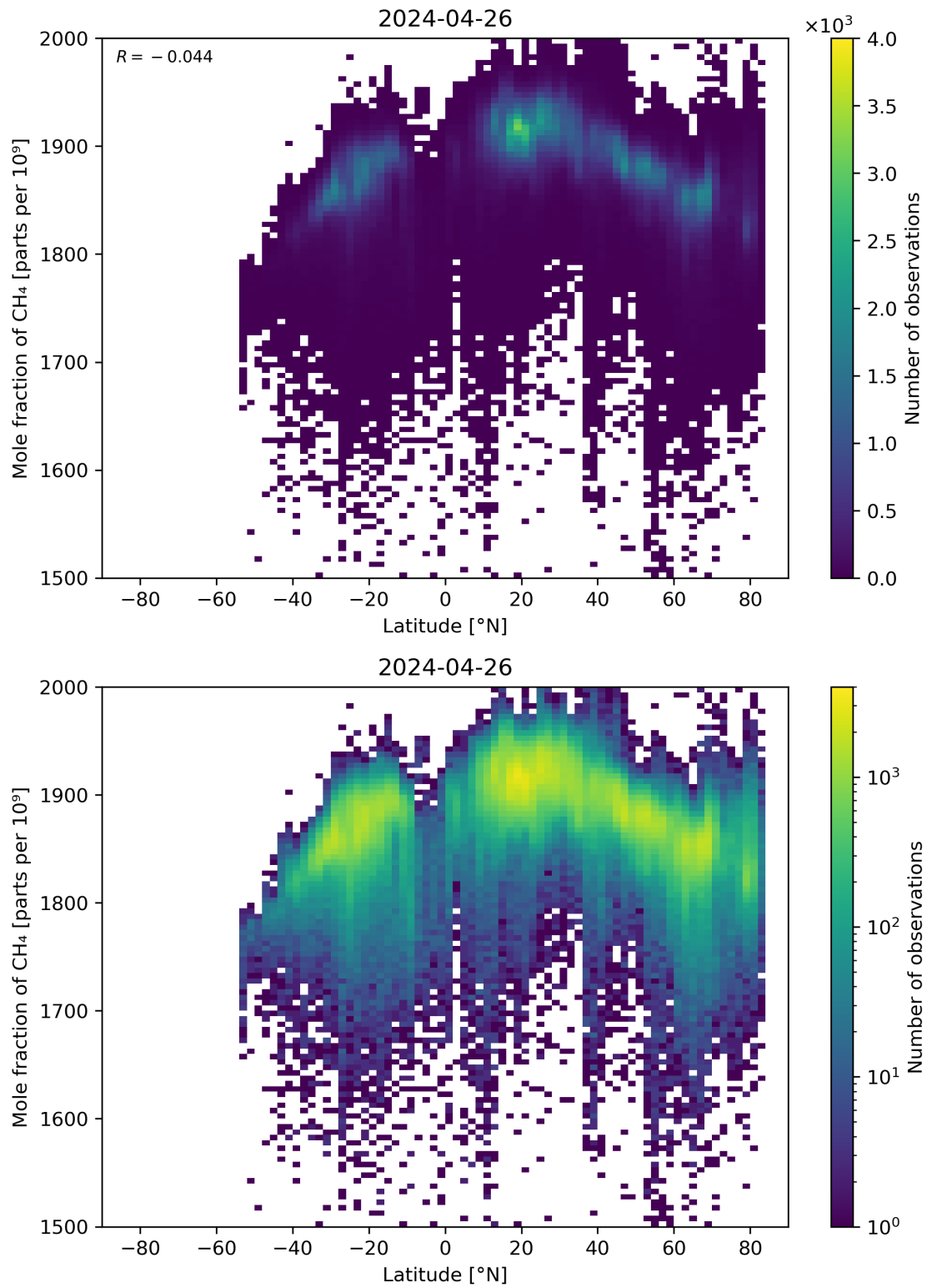
Figure 57: Scatter density plot of “Latitude” against “Mole fraction of \text{CH}_4 ” for 2024-04-26 to 2024-04-27.
