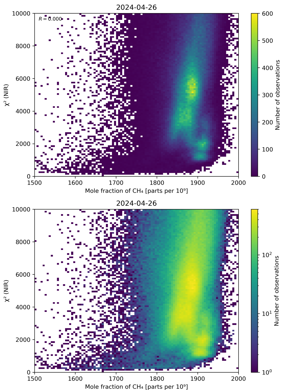
Figure 70: Scatter density plot of “Mole fraction of \text{CH}_4 ” against “ \chi^2 (NIR)” for 2024-04-26 to 2024-04-27.
