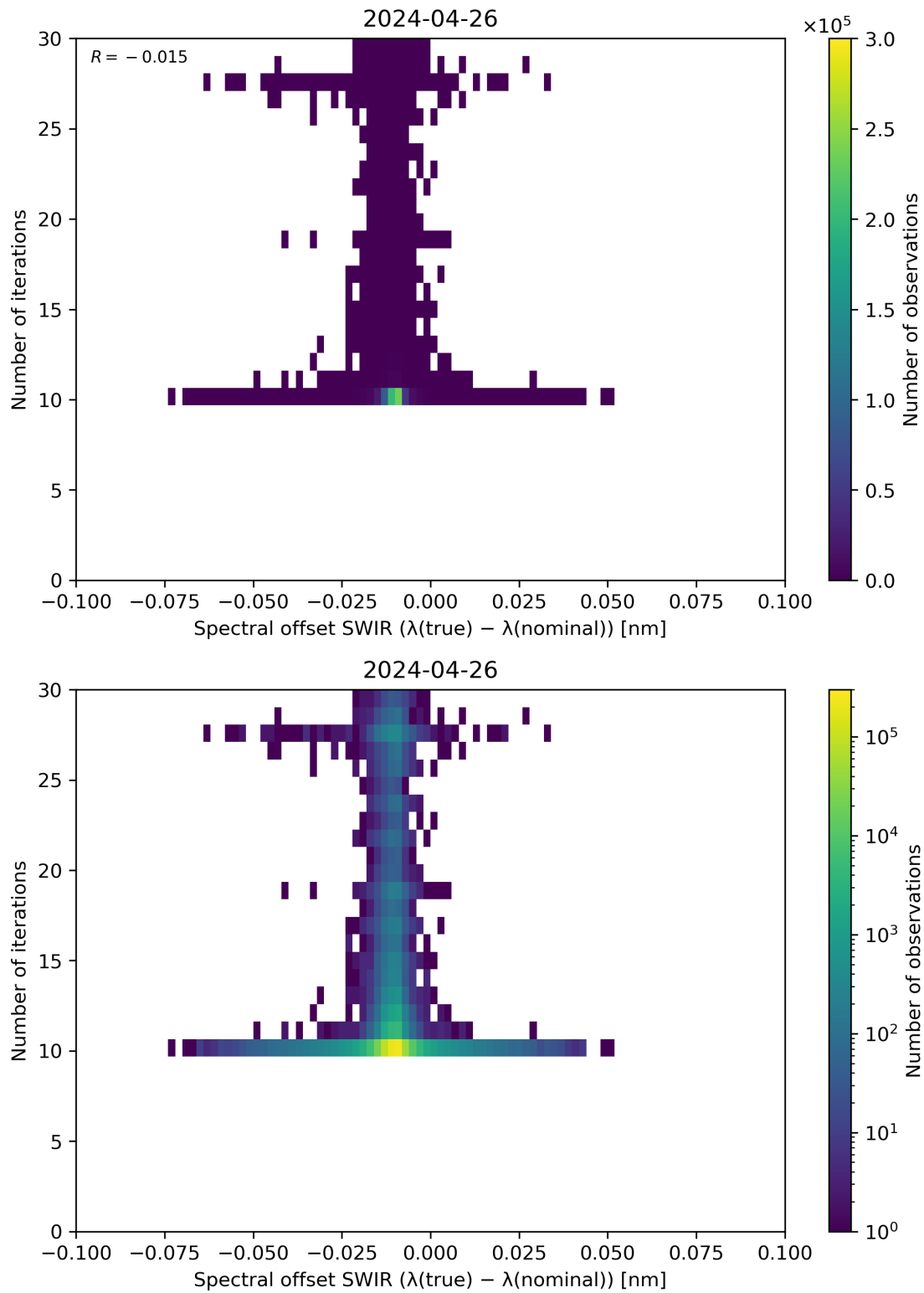
Figure 121: Scatter density plot of “Spectral offset SWIR ( \lambda(\text{true}) - \lambda(\text{nominal}) )” against “Number of iterations” for 2024-04-26 to 2024-04-27.
