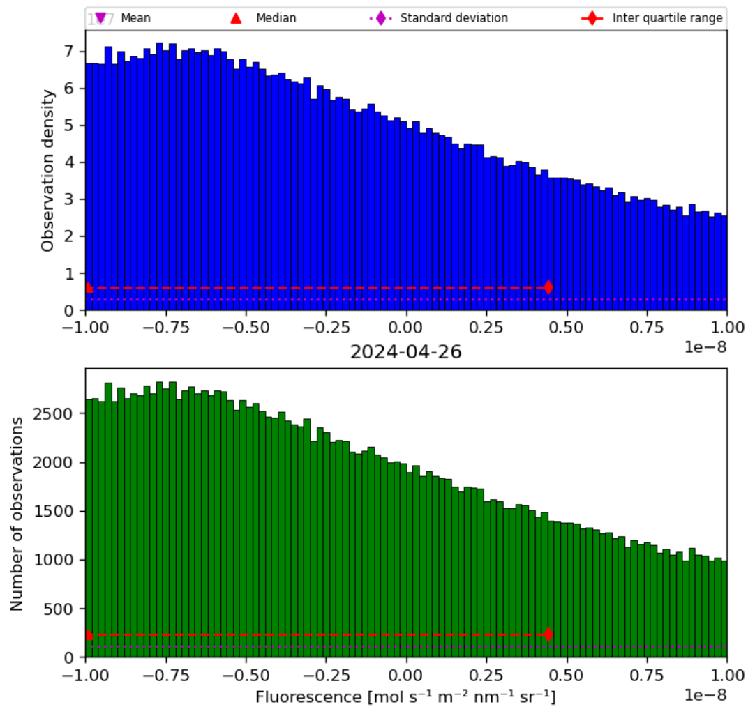
Figure 32: Histogram of “Fluorescence” for 2024-04-26 to 2024-04-27
