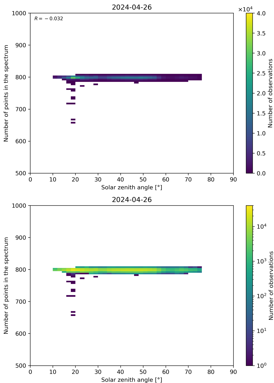
Figure 103: Scatter density plot of “Solar zenith angle” against “Number of points in the spectrum” for 2024-04-26 to 2024-04-27.
