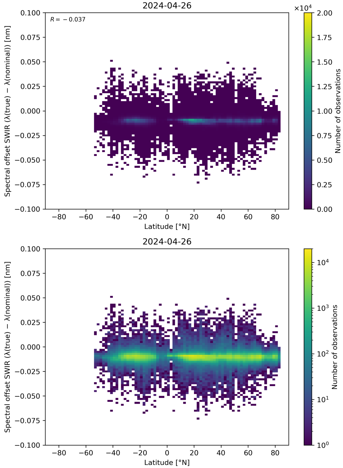
Figure 62: Scatter density plot of “Latitude” against “Spectral offset SWIR ( \lambda(\text{true}) - \lambda(\text{nominal}) )” for 2024-04-26 to 2024-04-27.
