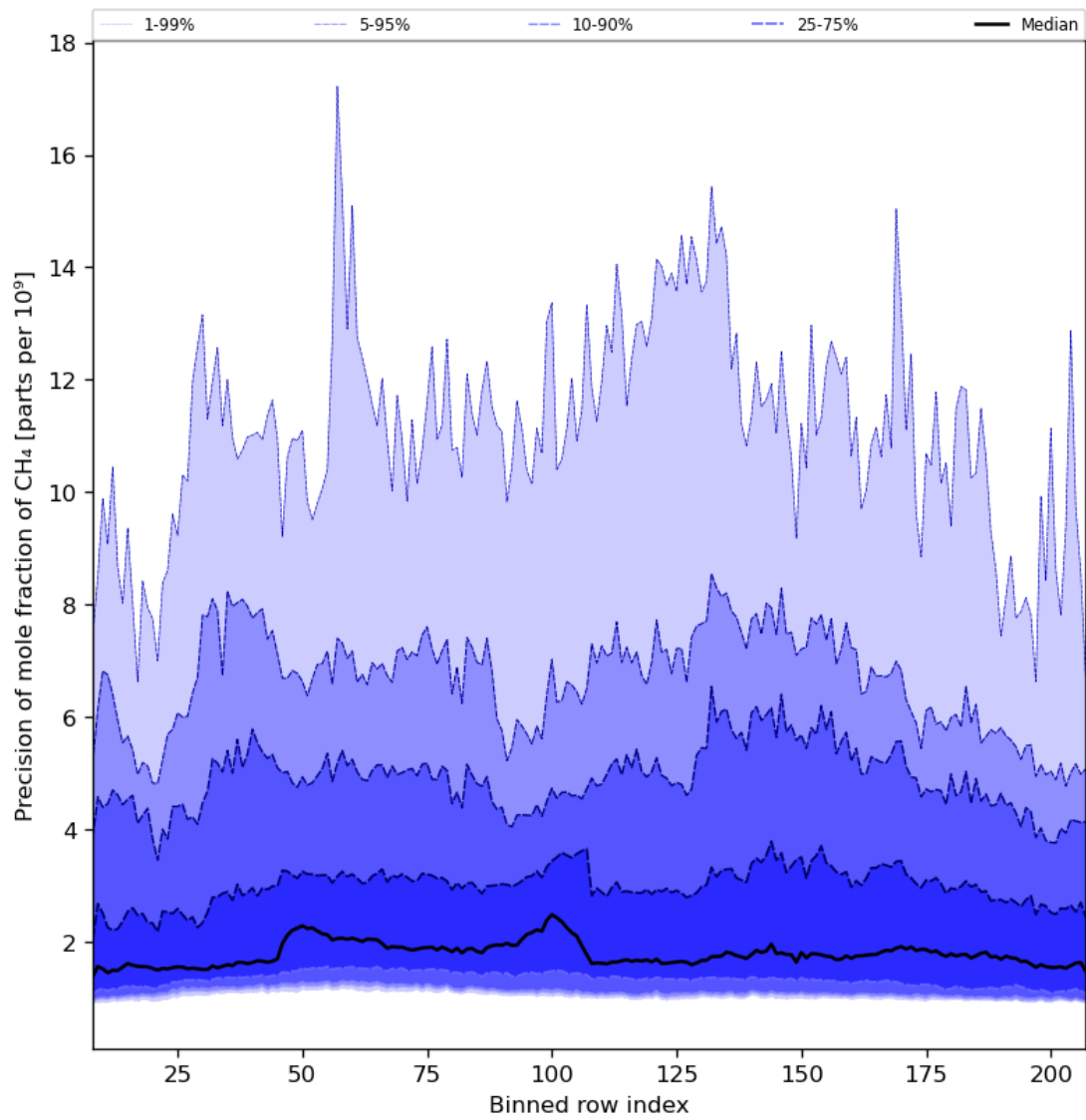
Figure 35: Along track statistics of “Precision of mole fraction of CH 4 ” for 2024-04-26 to 2024-04-27
