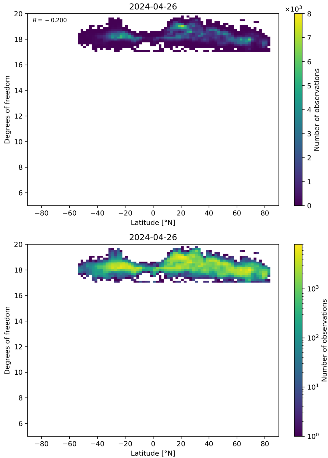
Figure 55: Scatter density plot of “Latitude” against “Degrees of freedom” for 2024-04-26 to 2024-04-27.
