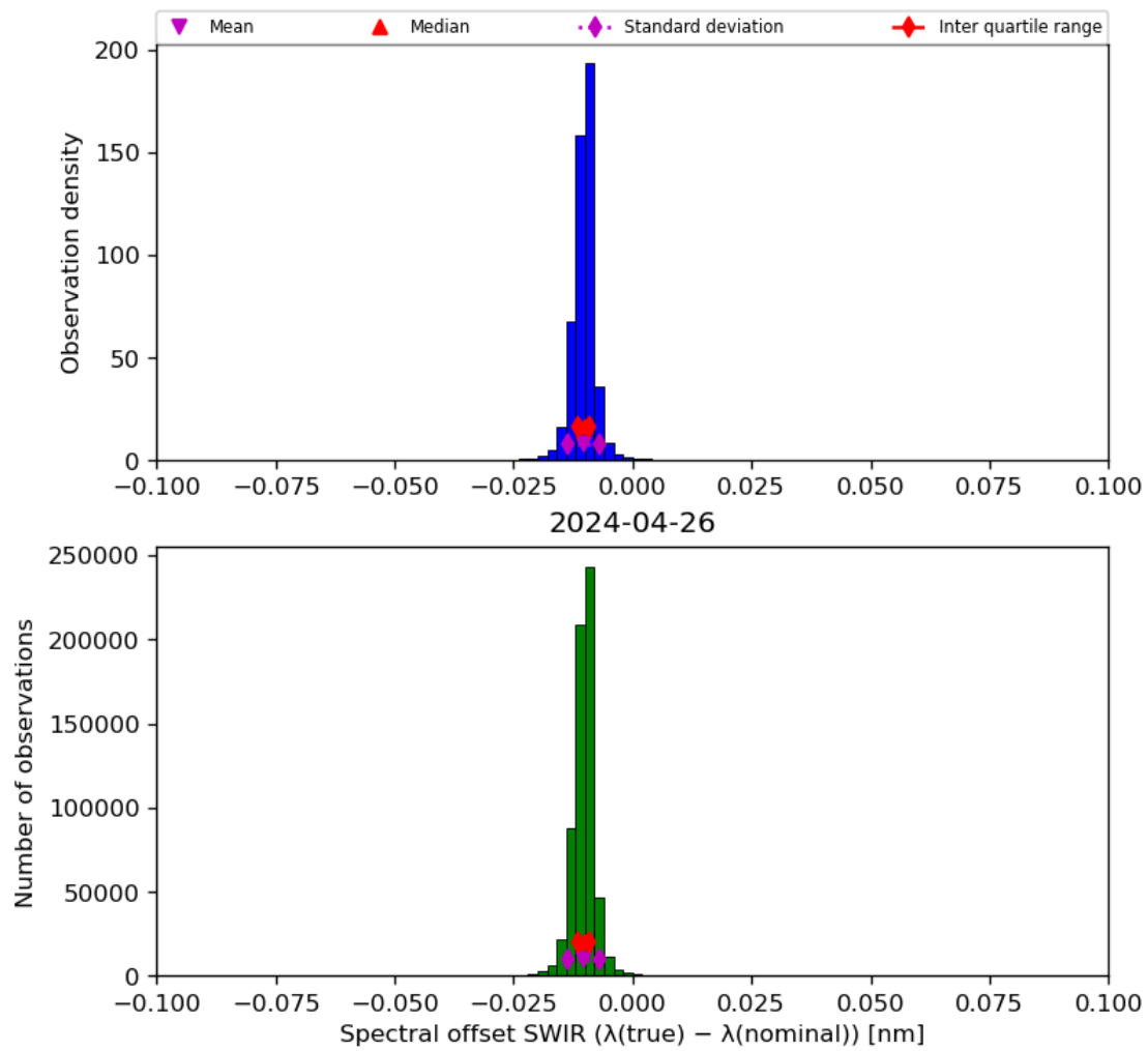
Figure 27: Histogram of “Spectral offset SWIR ( \lambda(\text{true}) - \lambda(\text{nominal}) )” for 2024-04-26 to 2024-04-27
