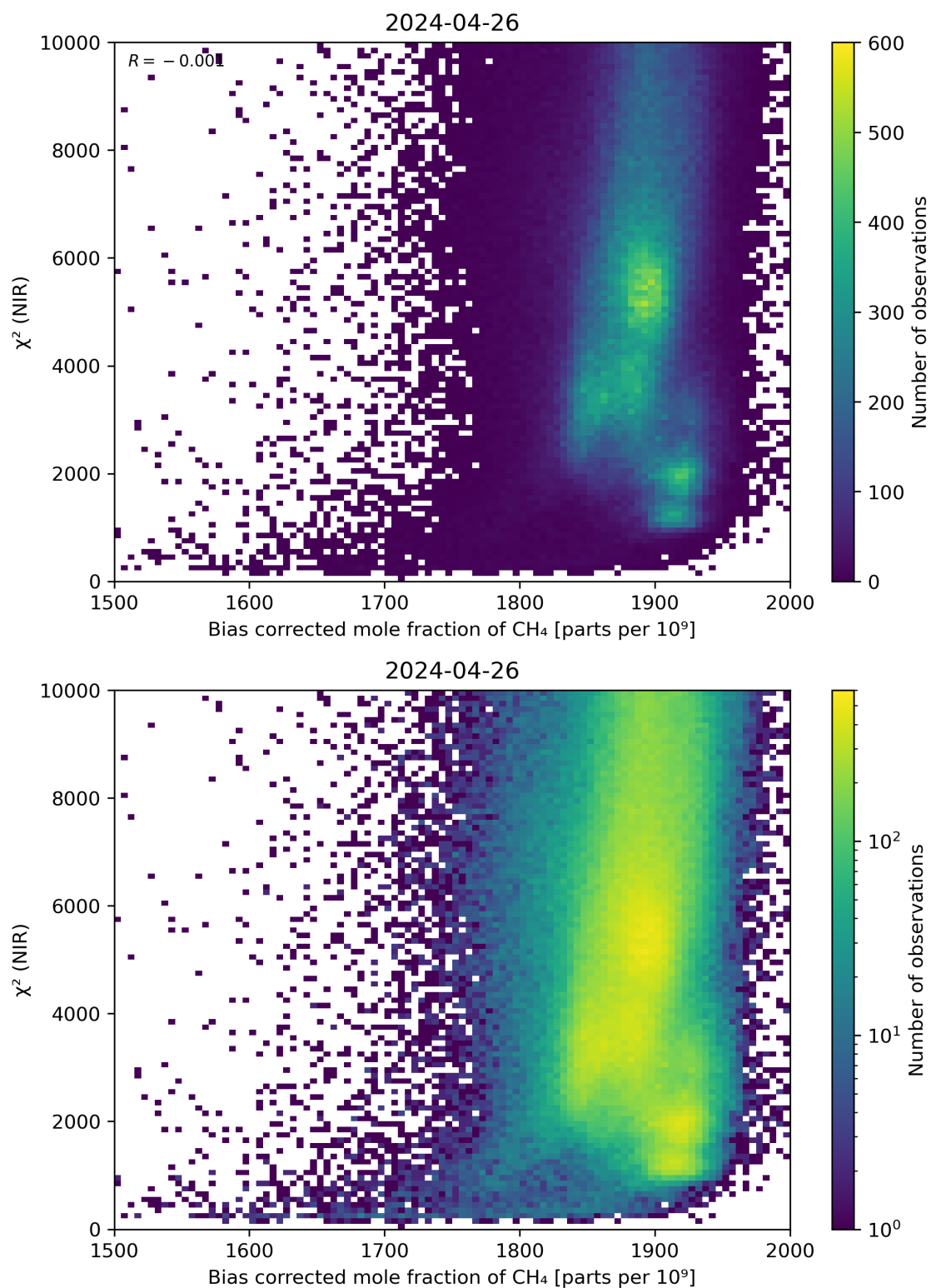
Figure 63: Scatter density plot of “Bias corrected mole fraction of CH 4 ” against “ \chi^2 (NIR)” for 2024-04-26 to 2024-04-27.
