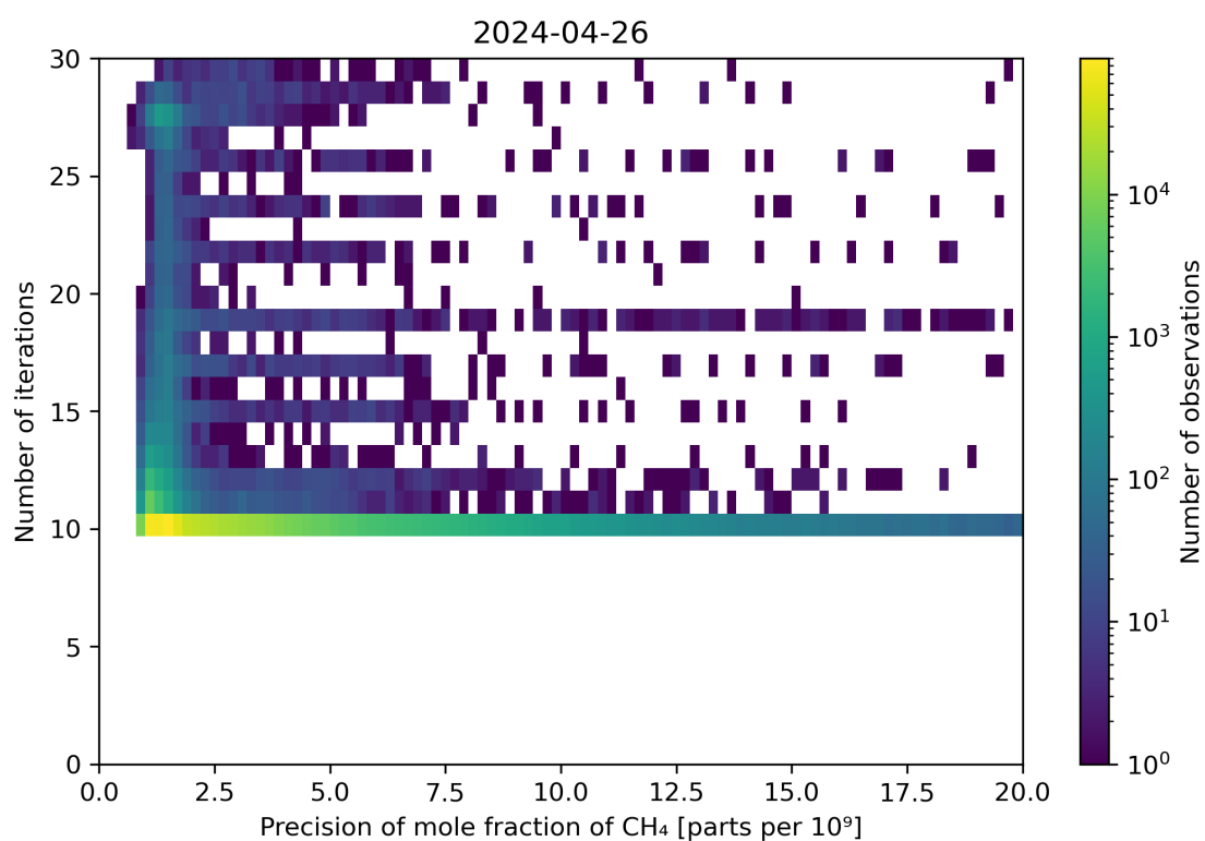
Figure 83: Scatter density plot of “Precision of mole fraction of \text{CH}_4 ” against “Number of iterations” for 2024-04-26 to 2024-04-27.
