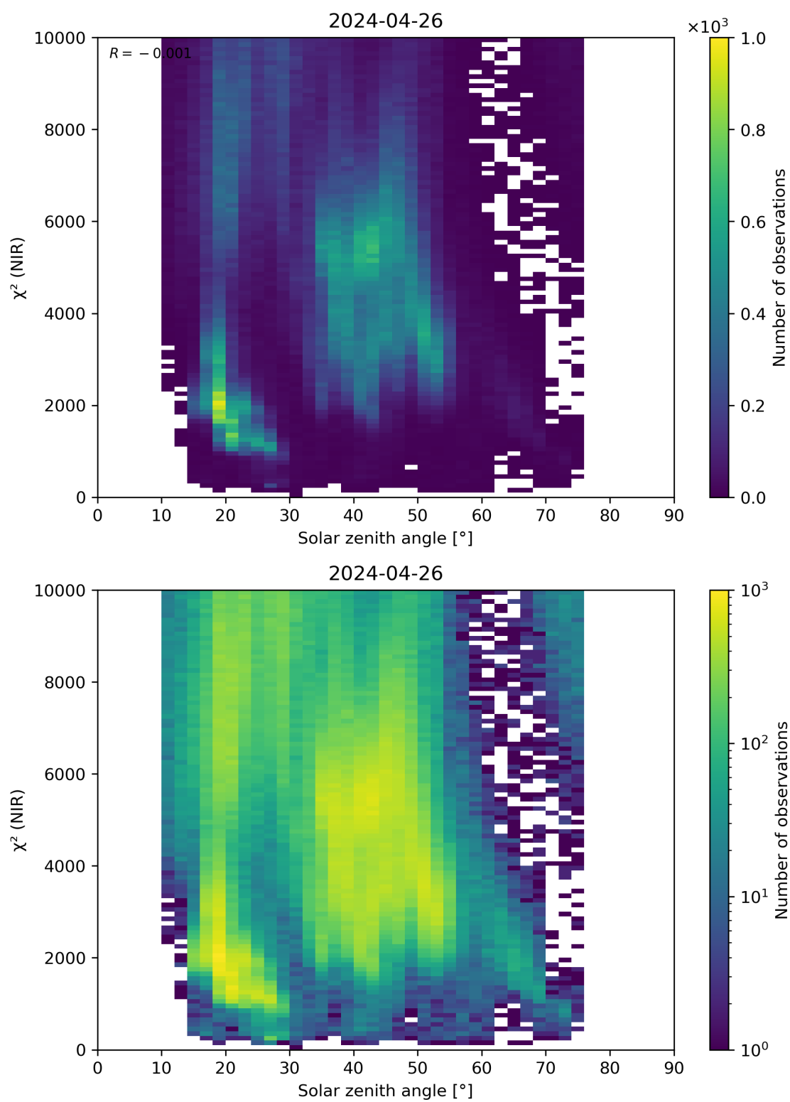
Figure 94: Scatter density plot of “Solar zenith angle” against “ \chi^2 (NIR)” for 2024-04-26 to 2024-04-27.
