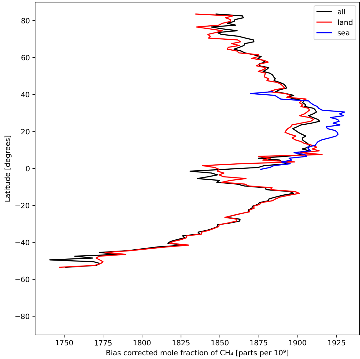
Figure 14: Zonal average of “Bias corrected mole fraction of CH 4 ” for 2024-04-26 to 2024-04-27.
