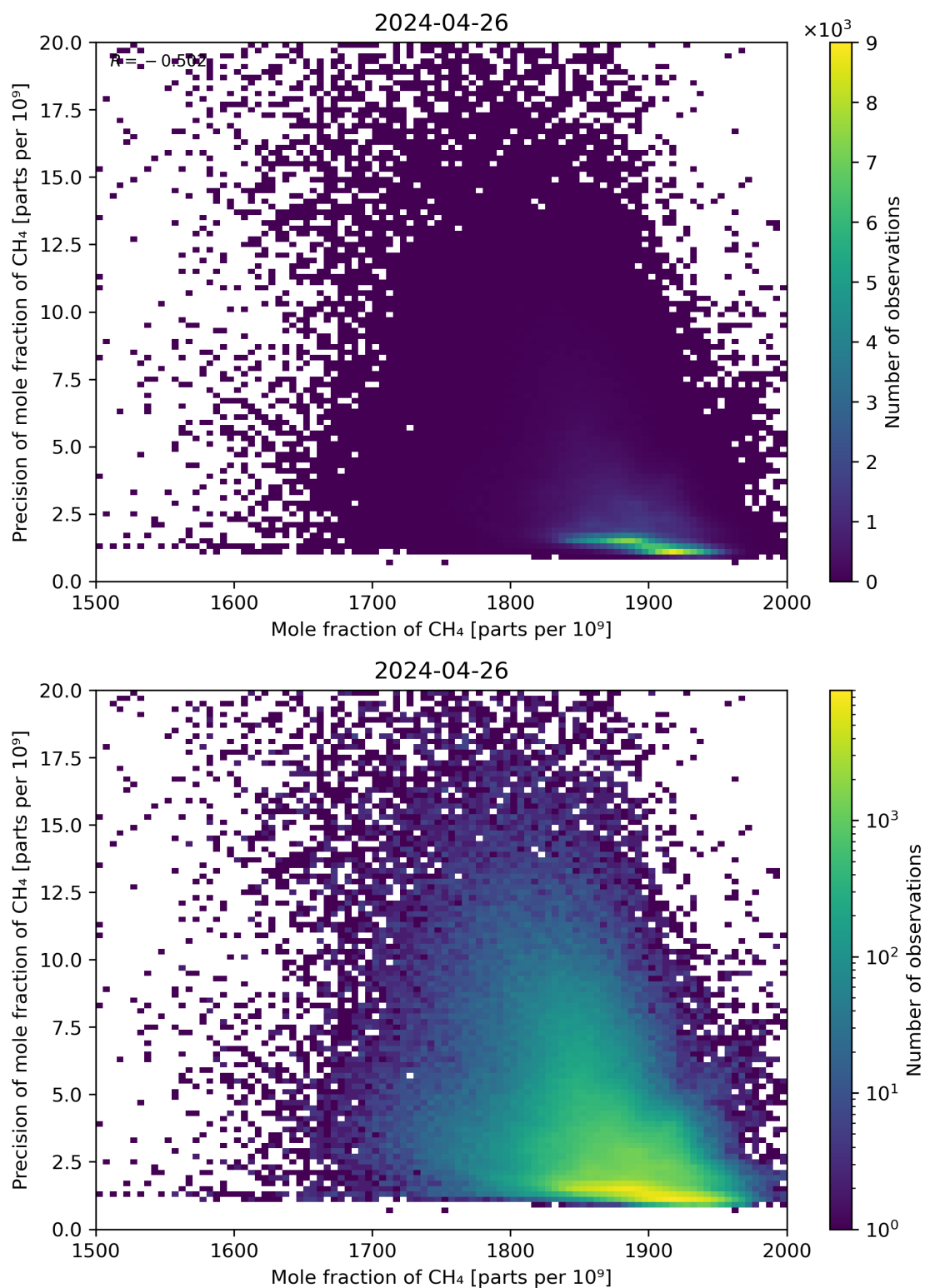
Figure 75: Scatter density plot of “Mole fraction of CH 4 ” against “Precision of mole fraction of CH 4 ” for 2024-04-26 to 2024-04-27.
