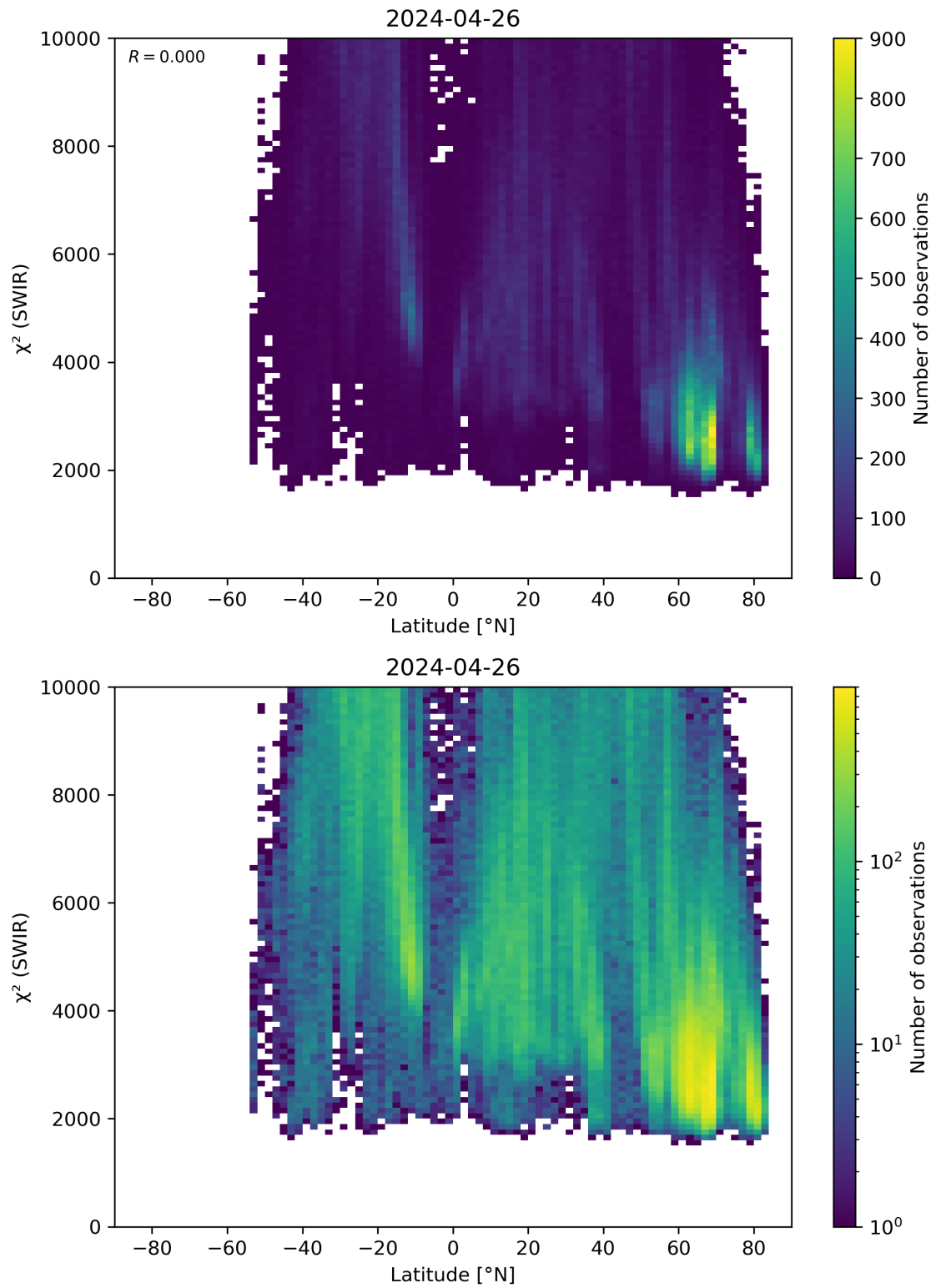
Figure 54: Scatter density plot of “Latitude” against “ \chi^2 (SWIR)” for 2024-04-26 to 2024-04-27.
