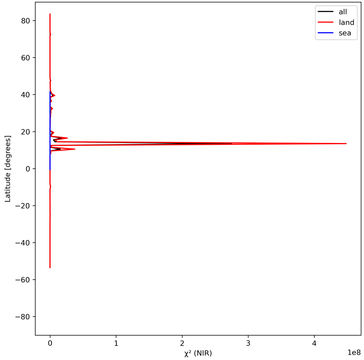
Figure 18: Zonal average of “ \chi^2 (NIR)” for 2024-04-26 to 2024-04-27.
