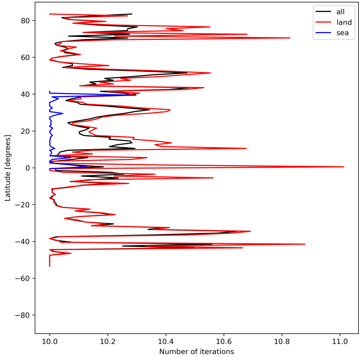
Figure 20: Zonal average of “Number of iterations” for 2024-04-26 to 2024-04-27.
