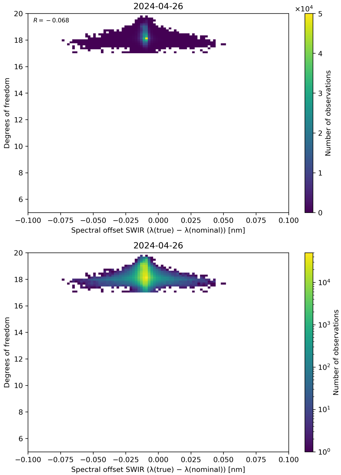
Figure 119: Scatter density plot of “Spectral offset SWIR ( \lambda(\text{true}) - \lambda(\text{nominal}) )” against “Degrees of freedom” for 2024-04-26 to 2024-04-27.
