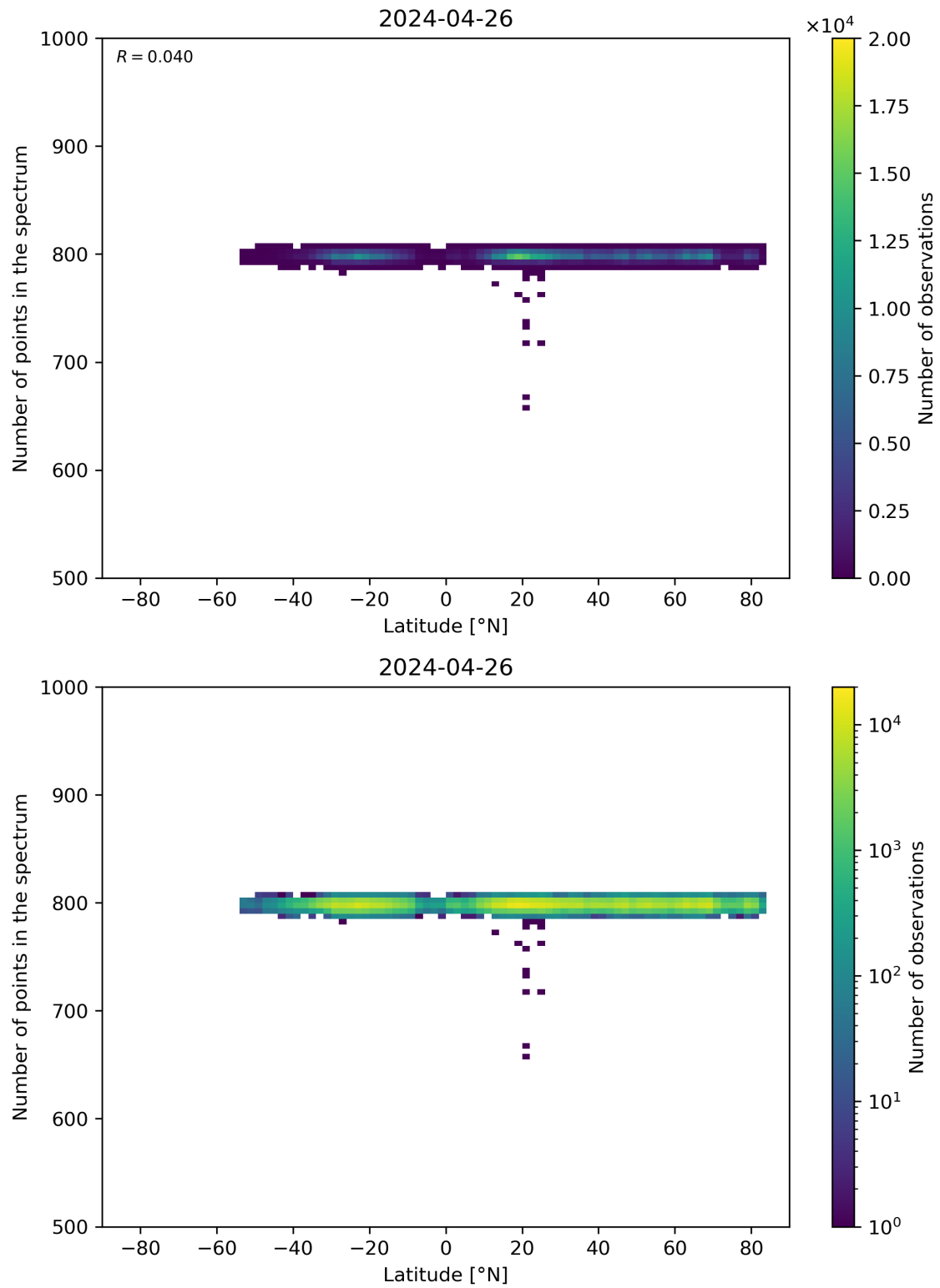
Figure 61: Scatter density plot of “Latitude” against “Number of points in the spectrum” for 2024-04-26 to 2024-04-27.
