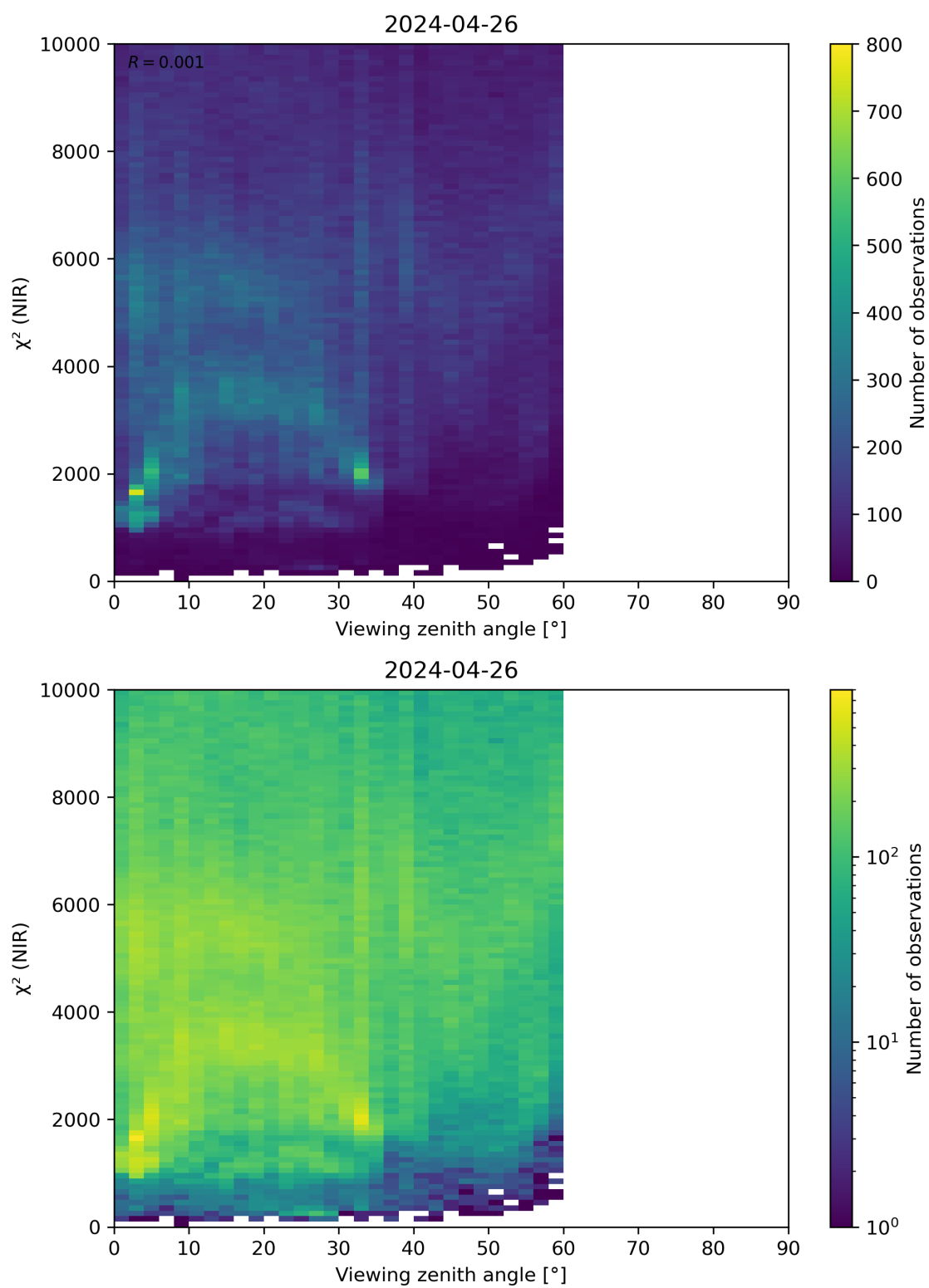
Figure 105: Scatter density plot of “Viewing zenith angle” against “ \chi^2 (NIR)” for 2024-04-26 to 2024-04-27.
