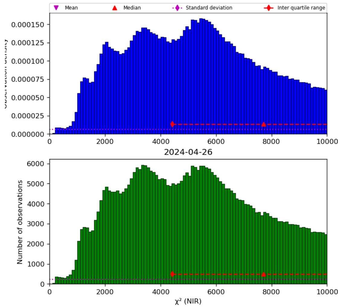
Figure 29: Histogram of “ \chi^2 (NIR)” for 2024-04-26 to 2024-04-27
