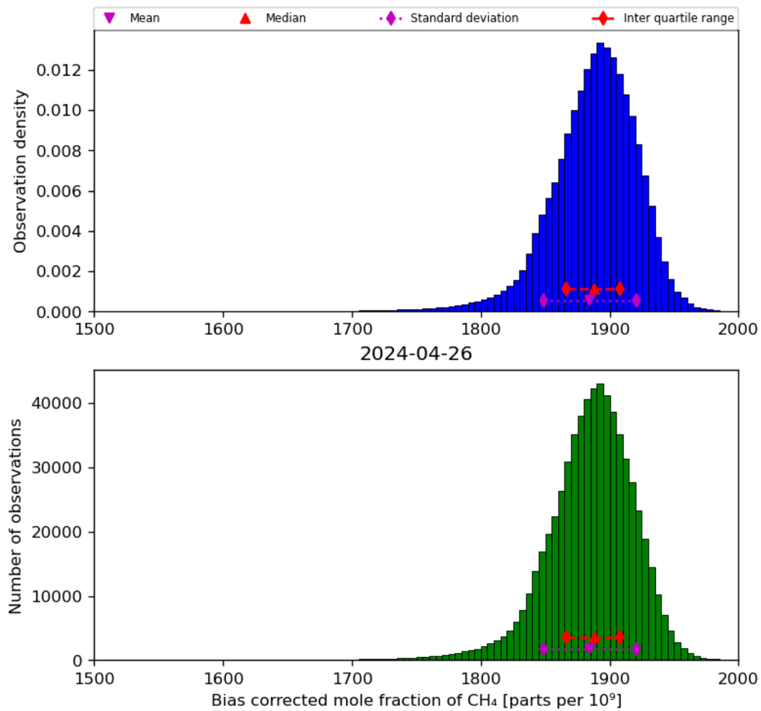
Figure 25: Histogram of “Bias corrected mole fraction of CH 4 ” for 2024-04-26 to 2024-04-27
