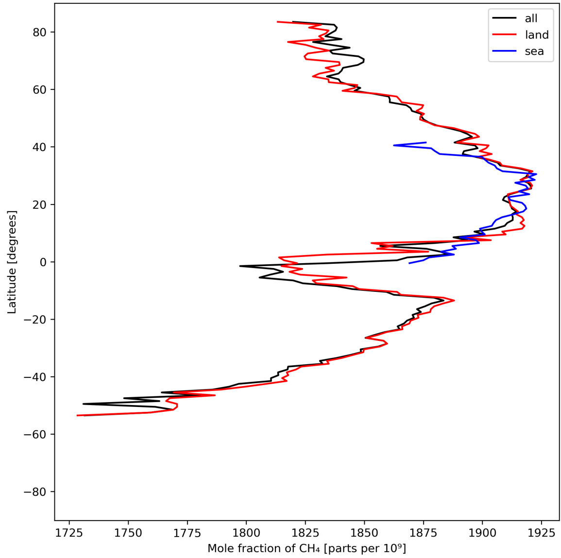
Figure 12: Zonal average of “Mole fraction of \text{CH}_4 ” for 2024-04-26 to 2024-04-27.
