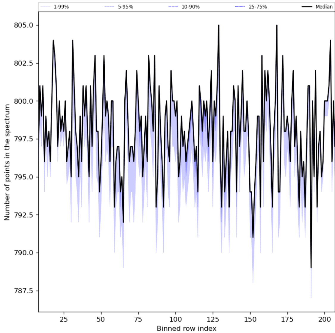
Figure 37: Along track statistics of “Number of points in the spectrum” for 2024-04-26 to 2024-04-27
