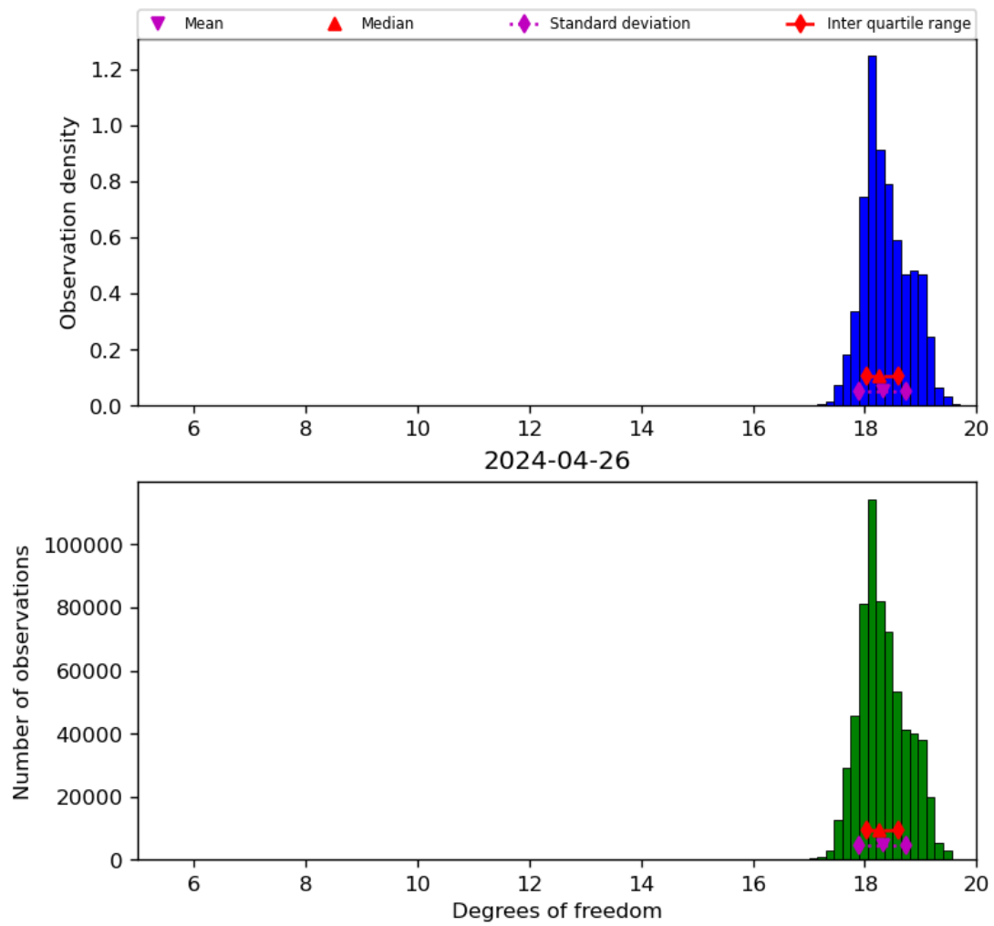
Figure 30: Histogram of “Degrees of freedom” for 2024-04-26 to 2024-04-27
