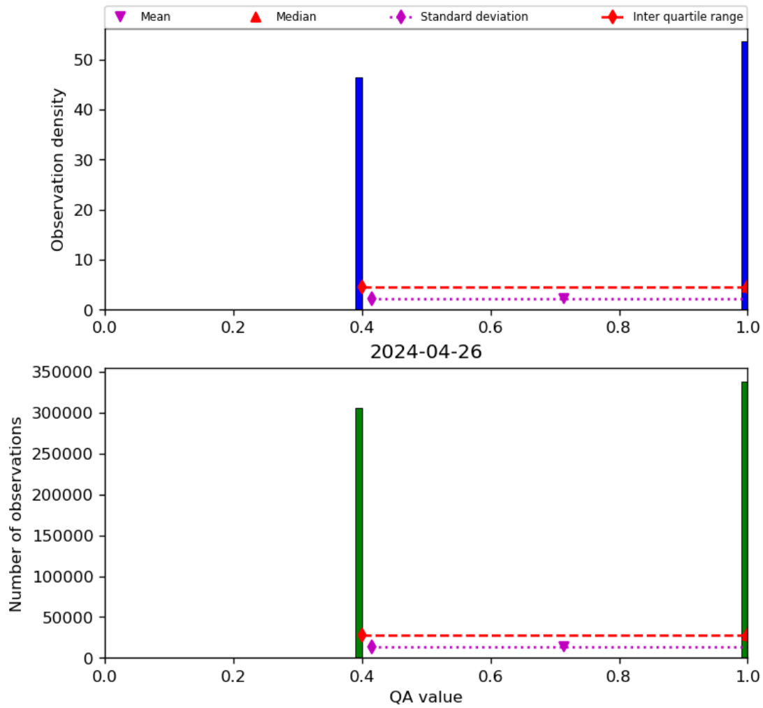
Figure 22: Histogram of “QA value” for 2024-04-26 to 2024-04-27
