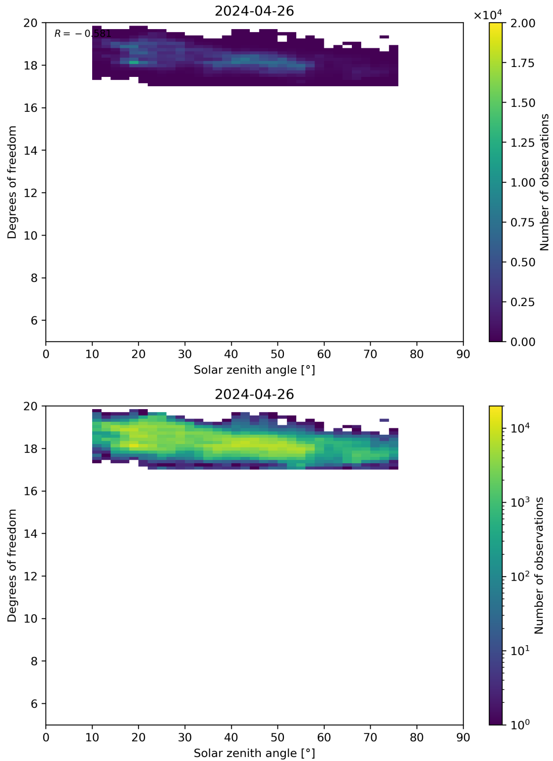
Figure 96: Scatter density plot of “Solar zenith angle” against “Degrees of freedom” for 2024-04-26 to 2024-04-27.
