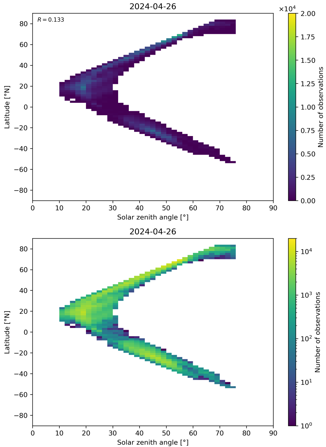
Figure 98: Scatter density plot of “Solar zenith angle” against “Latitude” for 2024-04-26 to 2024-04-27.
