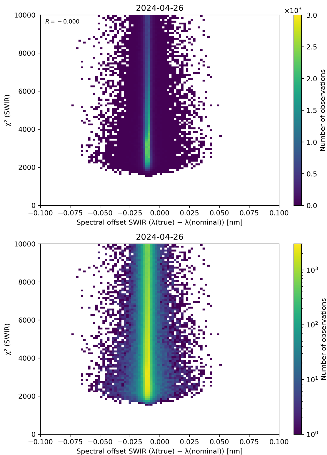
Figure 118: Scatter density plot of “Spectral offset SWIR ( \lambda(\text{true}) - \lambda(\text{nominal}) )” against “ \chi^2 (SWIR)” for 2024-04-26 to 2024-04-27.
