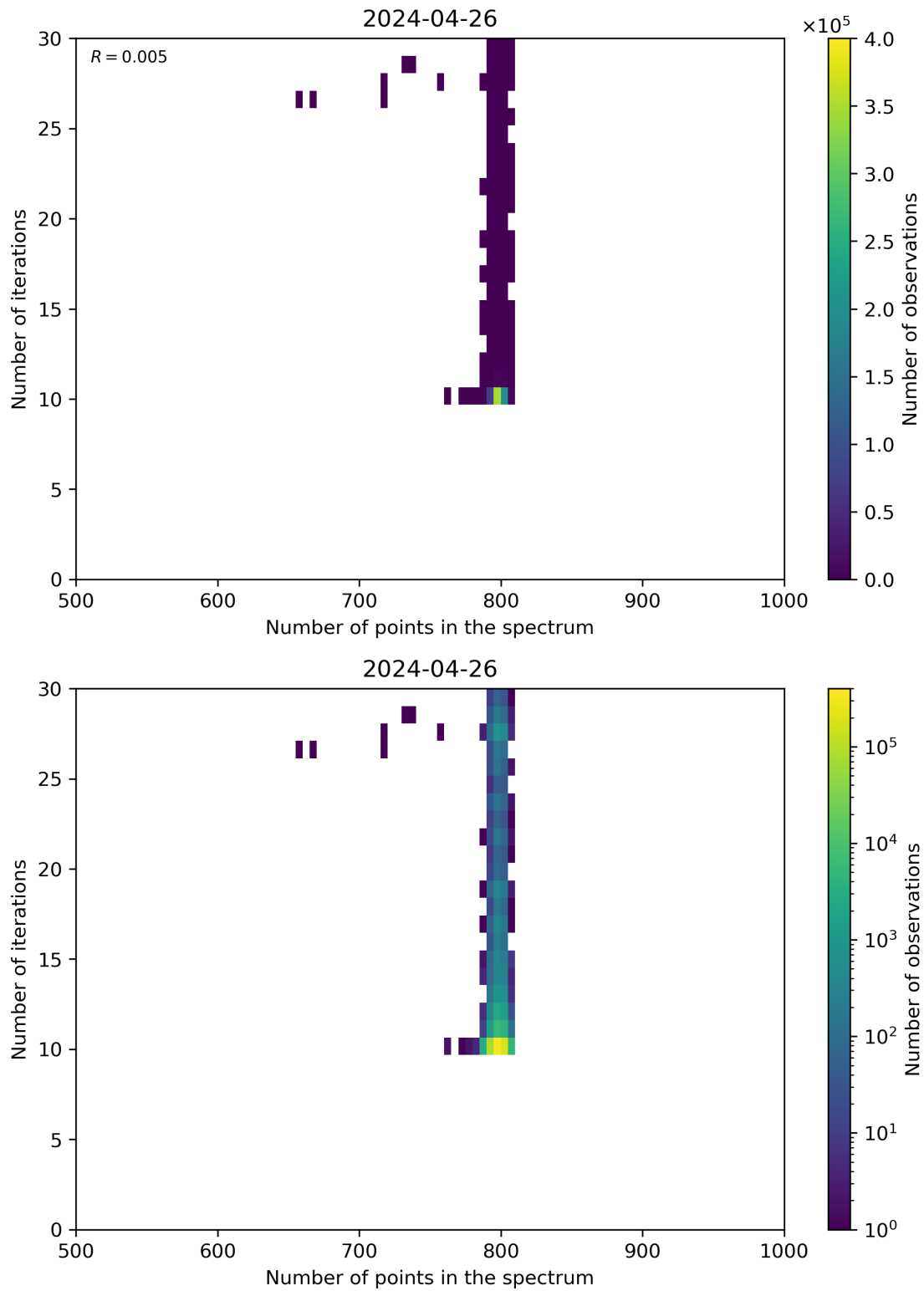
Figure 92: Scatter density plot of “Number of points in the spectrum” against “Number of iterations” for 2024-04-26 to 2024-04-27.
