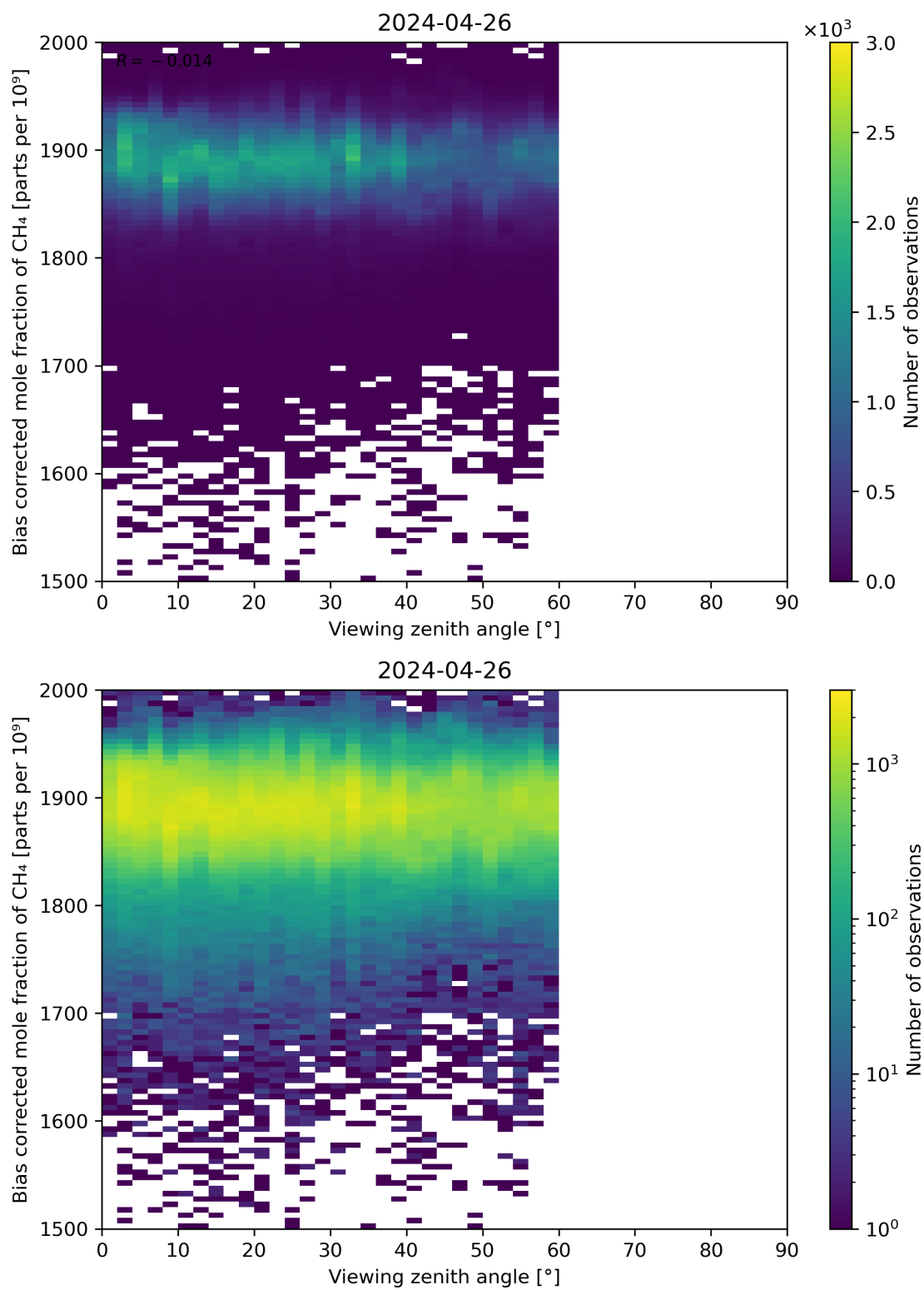
Figure 111: Scatter density plot of “Viewing zenith angle” against “Bias corrected mole fraction of CH 4 ” for 2024-04-26 to 2024-04-27.
