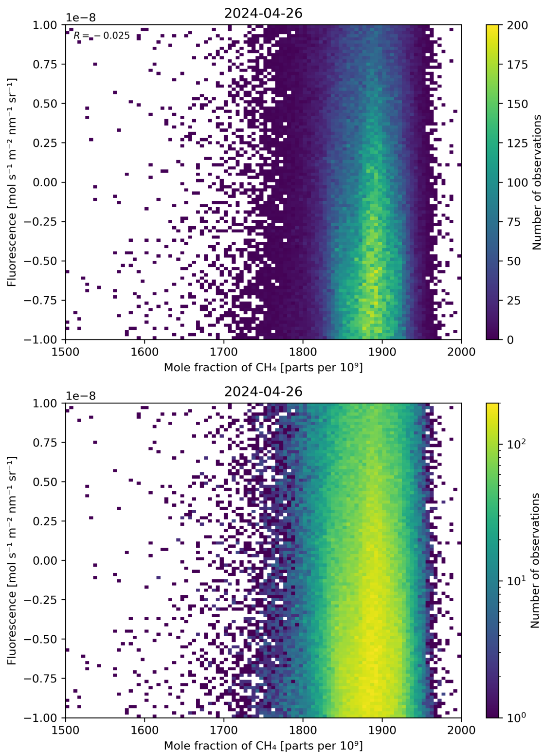
Figure 73: Scatter density plot of “Mole fraction of \text{CH}_4 ” against “Fluorescence” for 2024-04-26 to 2024-04-27.
