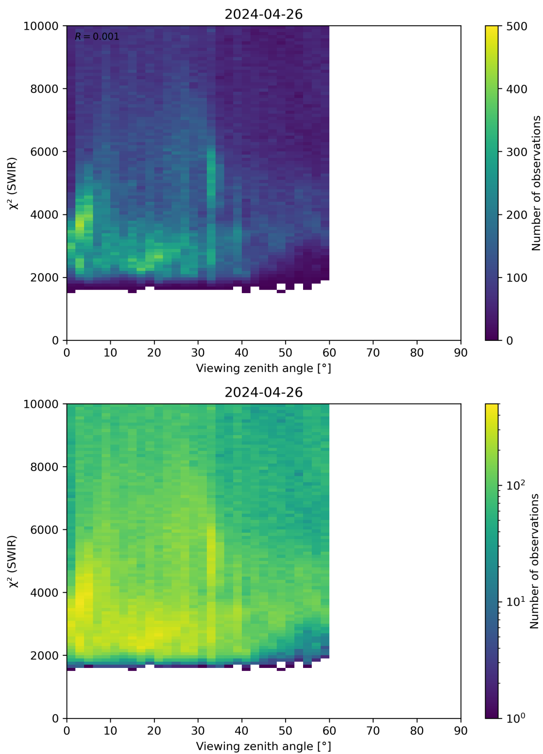
Figure 106: Scatter density plot of “Viewing zenith angle” against “ \chi^2 (SWIR)” for 2024-04-26 to 2024-04-27.
