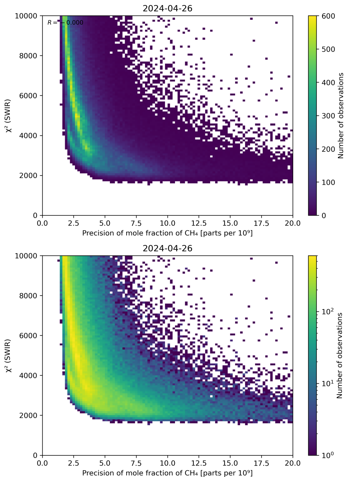
Figure 79: Scatter density plot of “Precision of mole fraction of CH 4 ” against “ \chi^2 (SWIR)” for 2024-04-26 to 2024-04-27.
