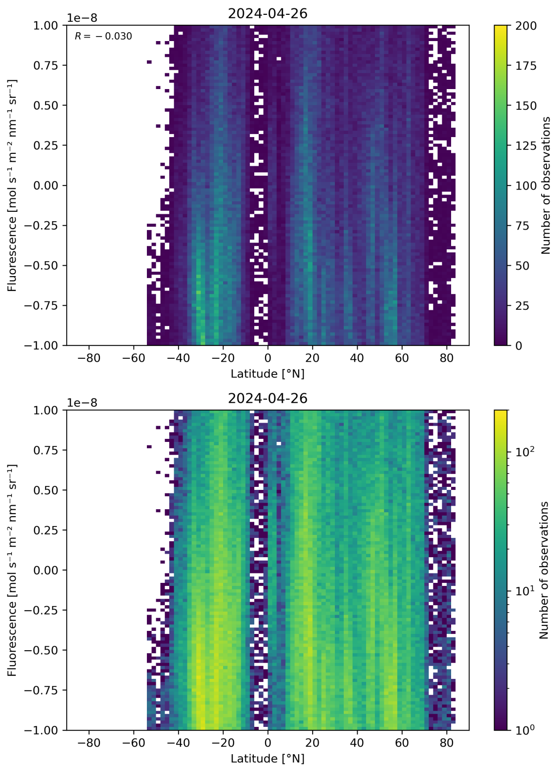
Figure 56: Scatter density plot of “Latitude” against “Fluorescence” for 2024-04-26 to 2024-04-27.
