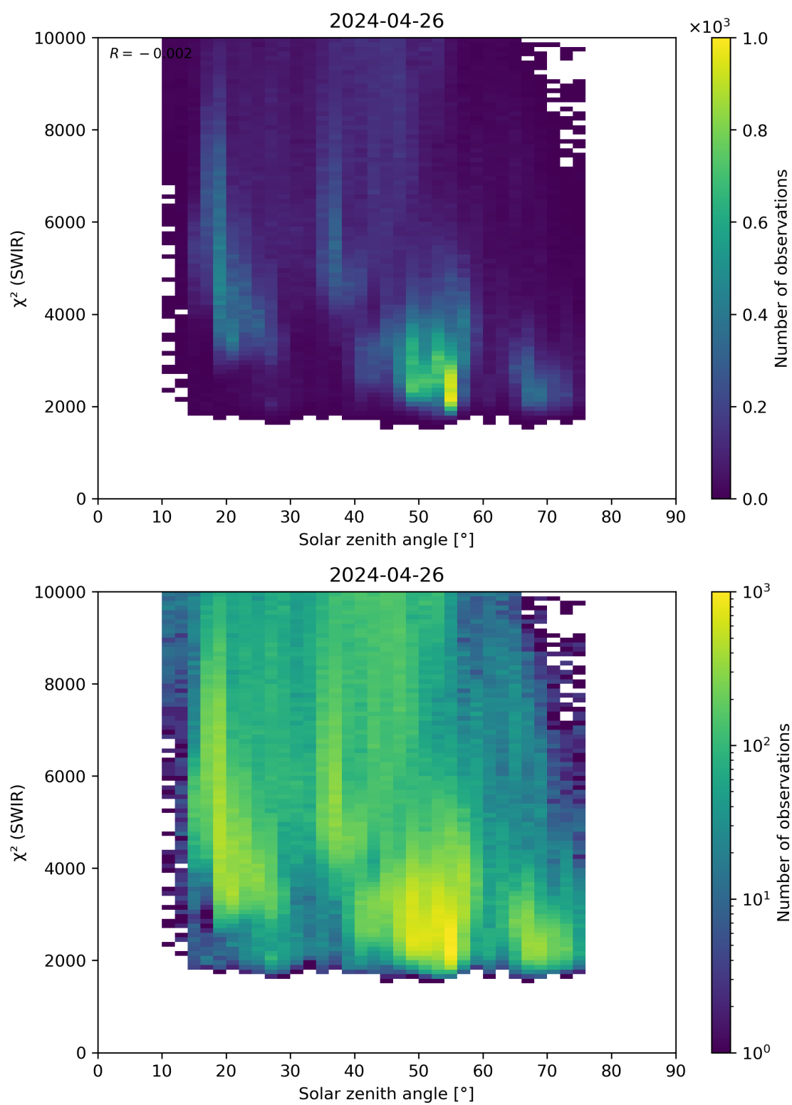
Figure 95: Scatter density plot of “Solar zenith angle” against “ \chi^2 (SWIR)” for 2024-04-26 to 2024-04-27.
