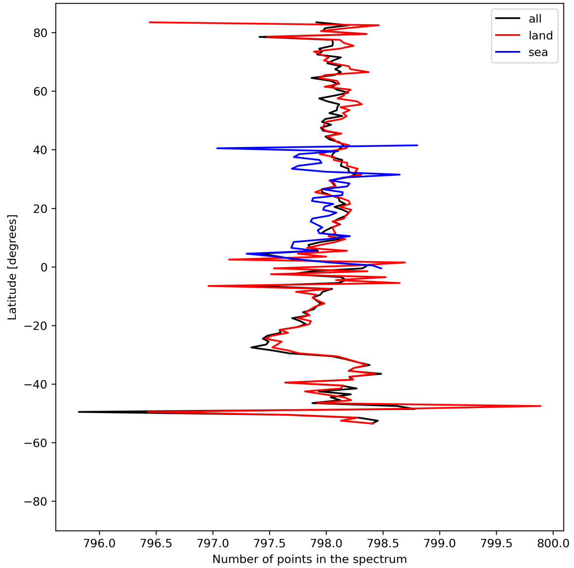
Figure 15: Zonal average of “Number of points in the spectrum” for 2024-04-26 to 2024-04-27.
