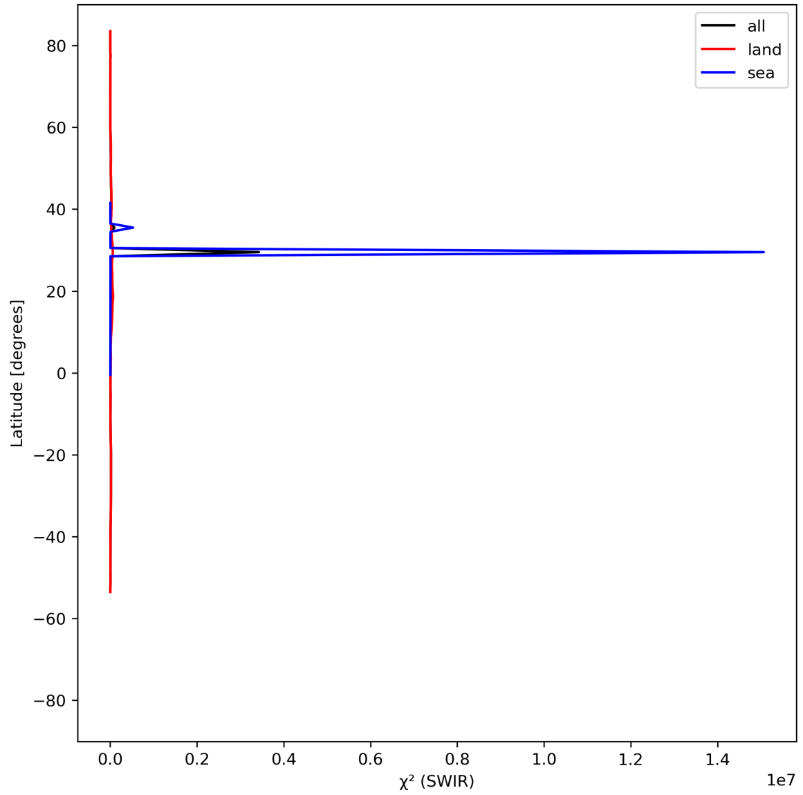
Figure 17: Zonal average of “ \chi^2 (SWIR)” for 2024-04-26 to 2024-04-27.
