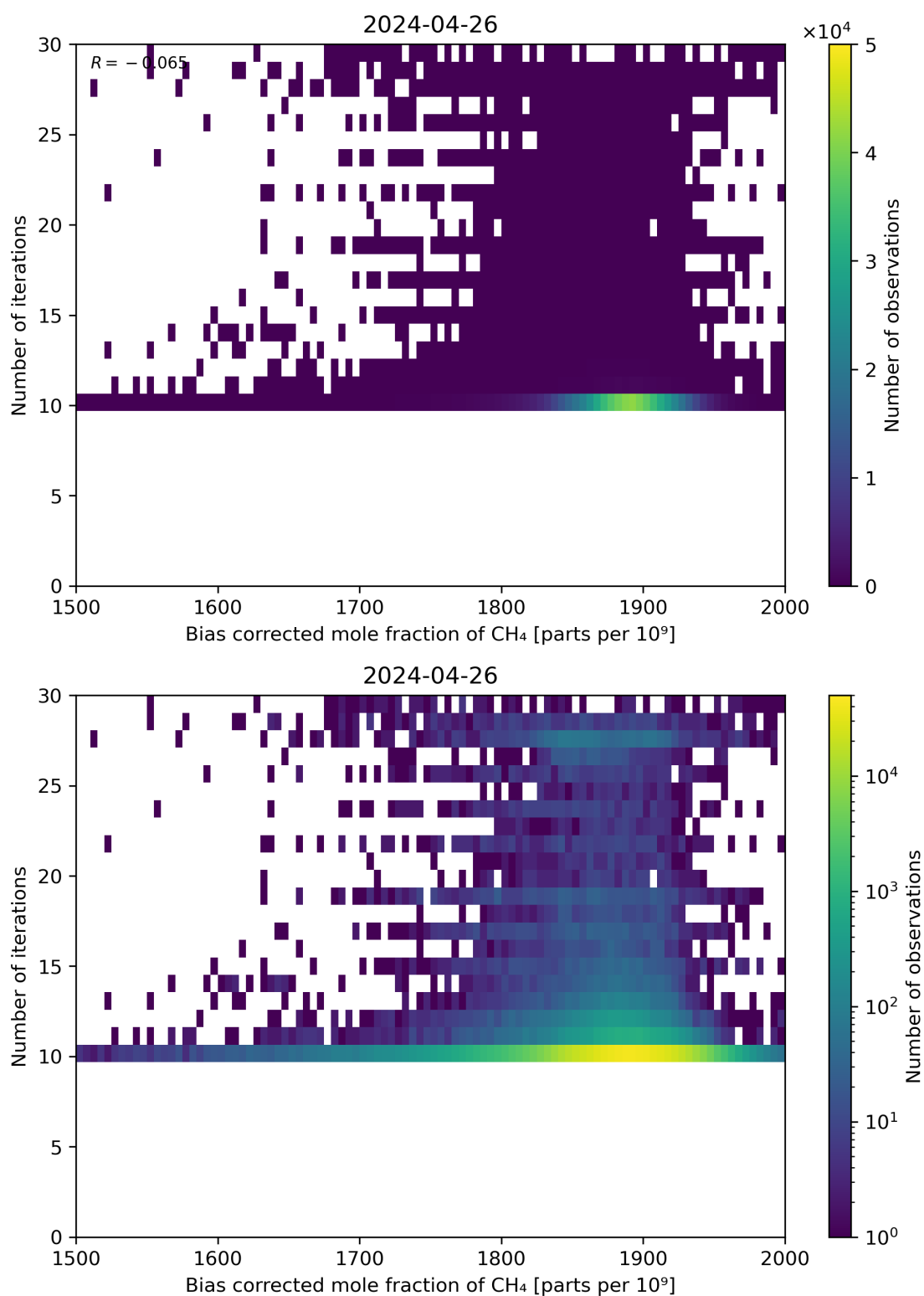
Figure 67: Scatter density plot of “Bias corrected mole fraction of \text{CH}_4 ” against “Number of iterations” for 2024-04-26 to 2024-04-27.
