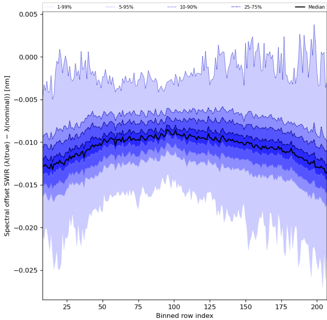
Figure 38: Along track statistics of “Spectral offset SWIR ( \lambda(\text{true}) - \lambda(\text{nominal}) )” for 2024-04-26 to 2024-04-27
