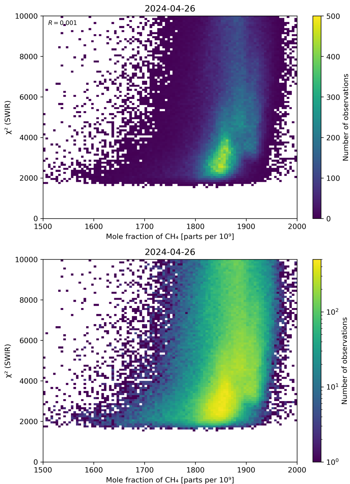
Figure 71: Scatter density plot of “Mole fraction of \text{CH}_4 ” against “ \chi^2 (SWIR)” for 2024-04-26 to 2024-04-27.
