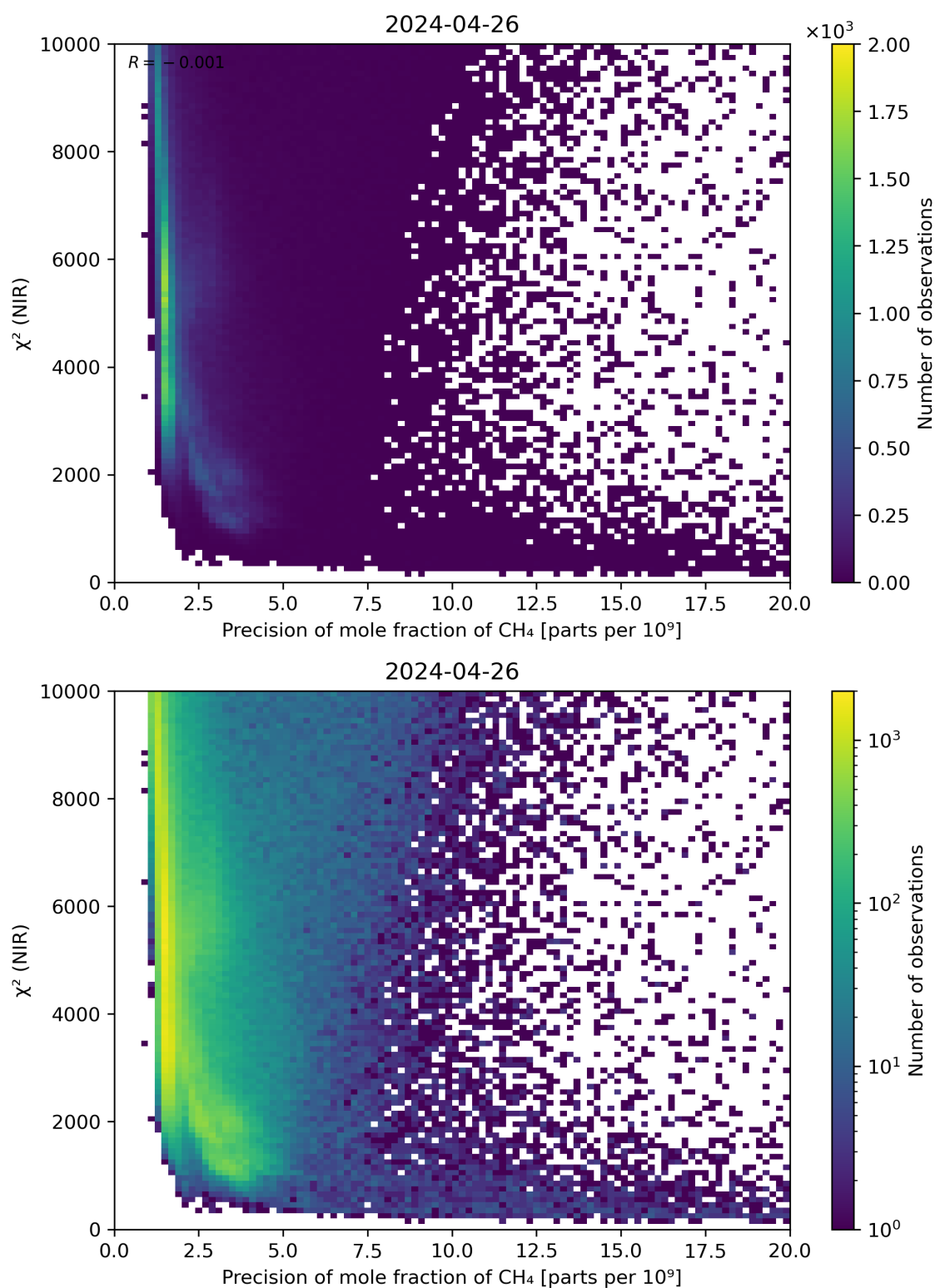
Figure 78: Scatter density plot of “Precision of mole fraction of CH 4 ” against “ \chi^2 (NIR)” for 2024-04-26 to 2024-04-27.
