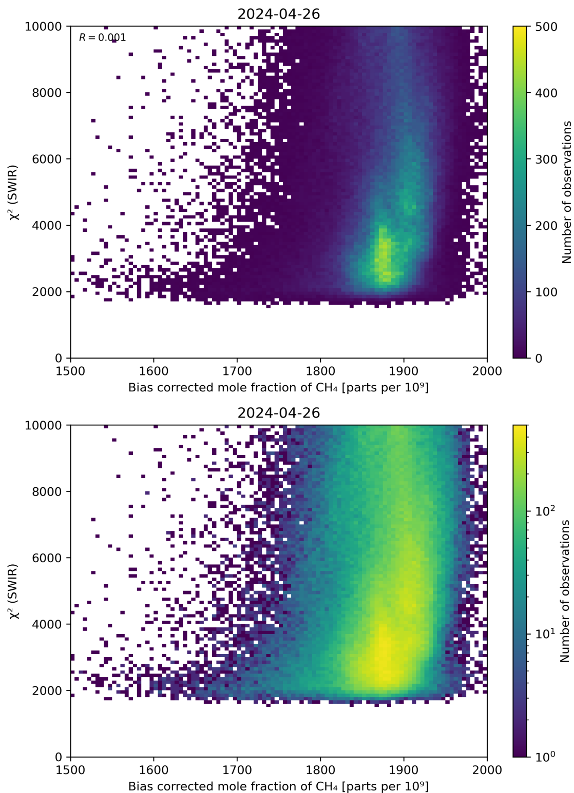
Figure 64: Scatter density plot of “Bias corrected mole fraction of CH 4 ” against “ \chi^2 (SWIR)” for 2024-04-26 to 2024-04-27.
