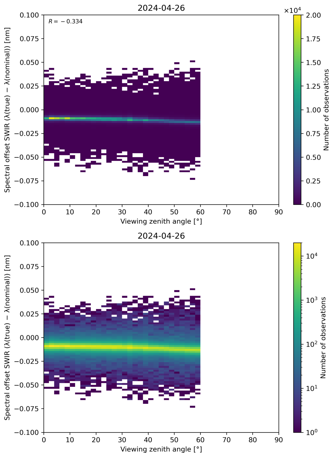
Figure 116: Scatter density plot of “Viewing zenith angle” against “Spectral offset SWIR ( \lambda(\text{true}) - \lambda(\text{nominal}) )” for 2024-04-26 to 2024-04-27.
