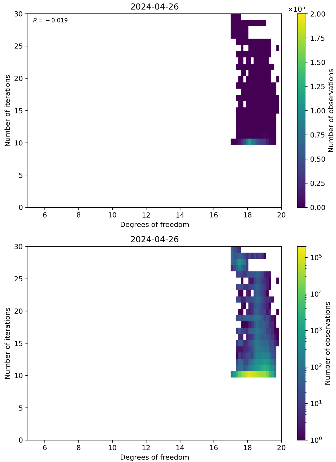
Figure 52: Scatter density plot of “Degrees of freedom” against “Number of iterations” for 2024-04-26 to 2024-04-27.
