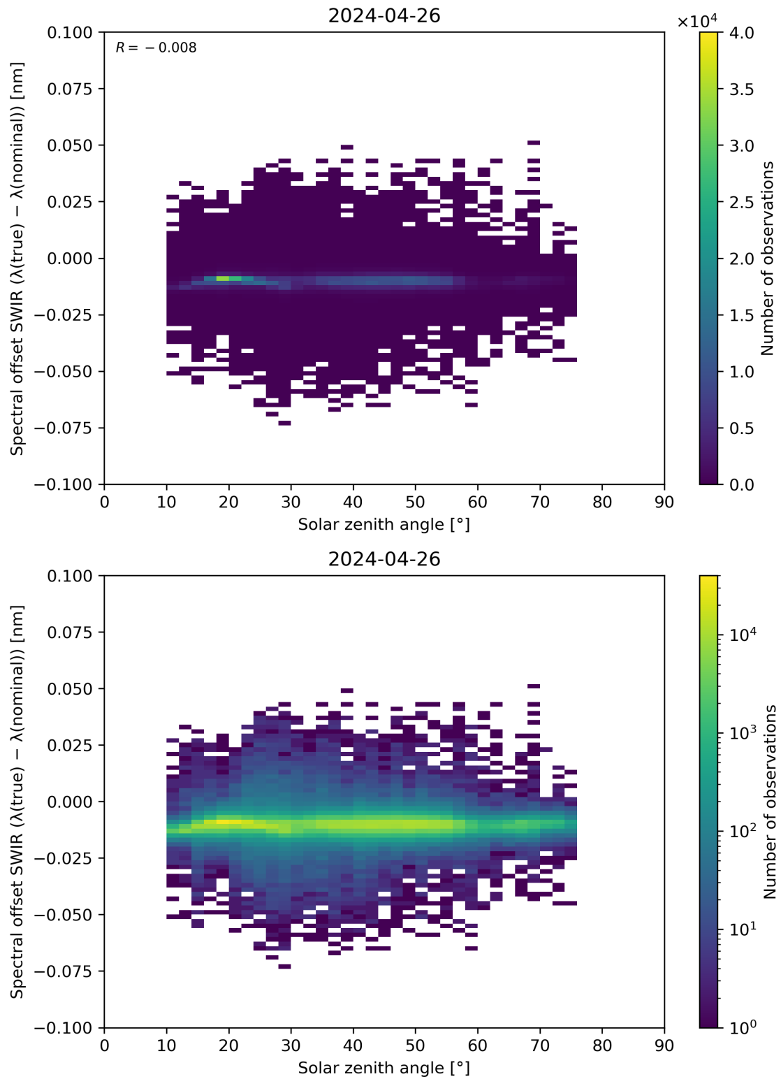
Figure 104: Scatter density plot of “Solar zenith angle” against “Spectral offset SWIR ( \lambda(\text{true}) - \lambda(\text{nominal}) )” for 2024-04-26 to 2024-04-27.
