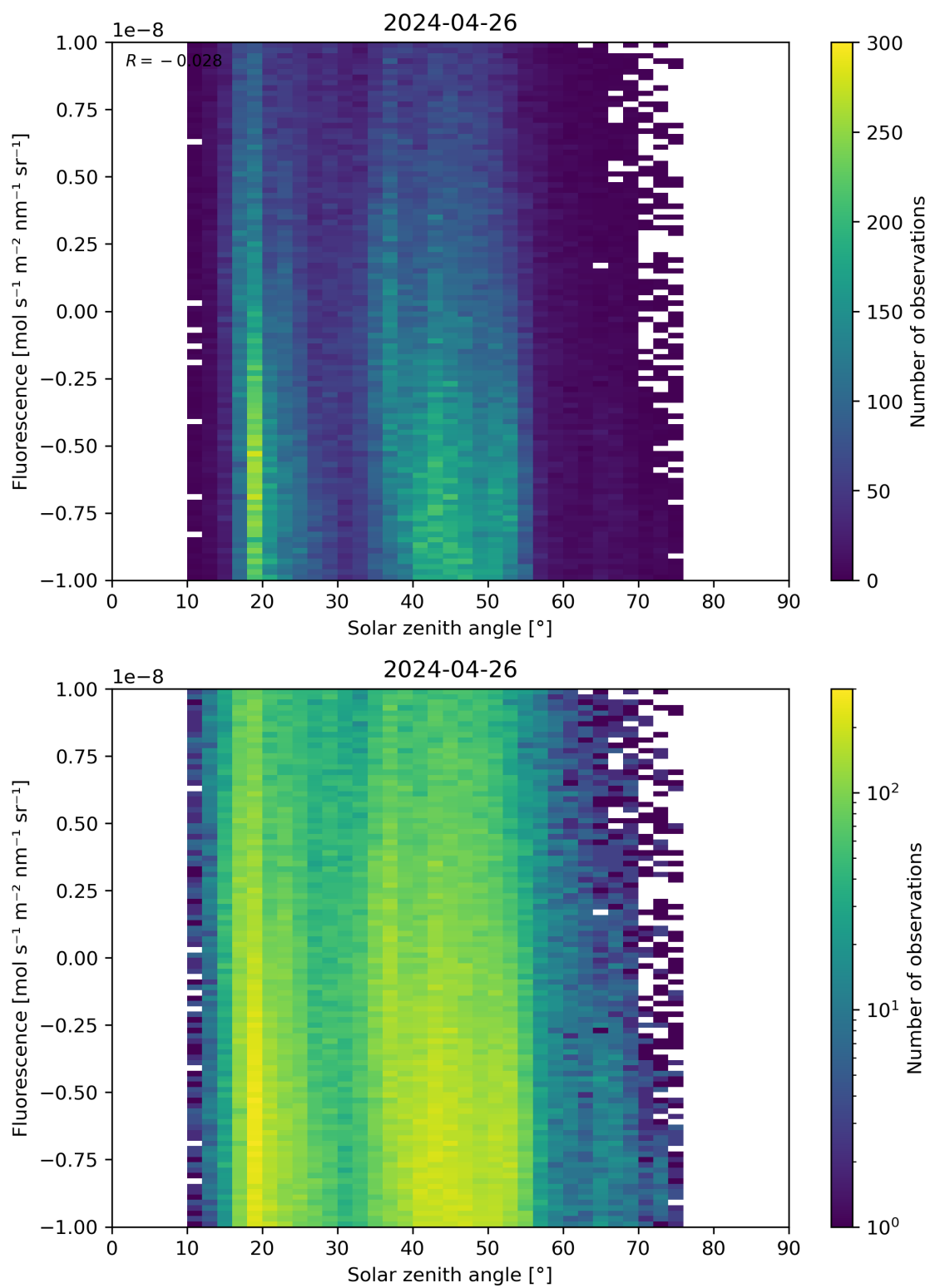
Figure 97: Scatter density plot of “Solar zenith angle” against “Fluorescence” for 2024-04-26 to 2024-04-27.
