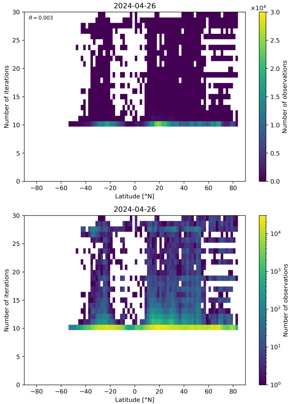
Figure 60: Scatter density plot of “Latitude” against “Number of iterations” for 2024-04-26 to 2024-04-27.
