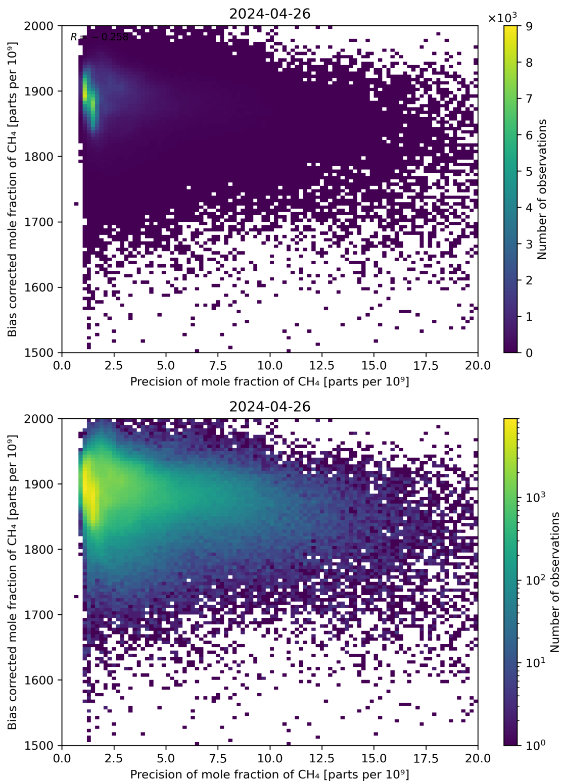
Figure 82: Scatter density plot of “Precision of mole fraction of CH 4 ” against “Bias corrected mole fraction of CH 4 ” for 2024-04-26 to 2024-04-27.
