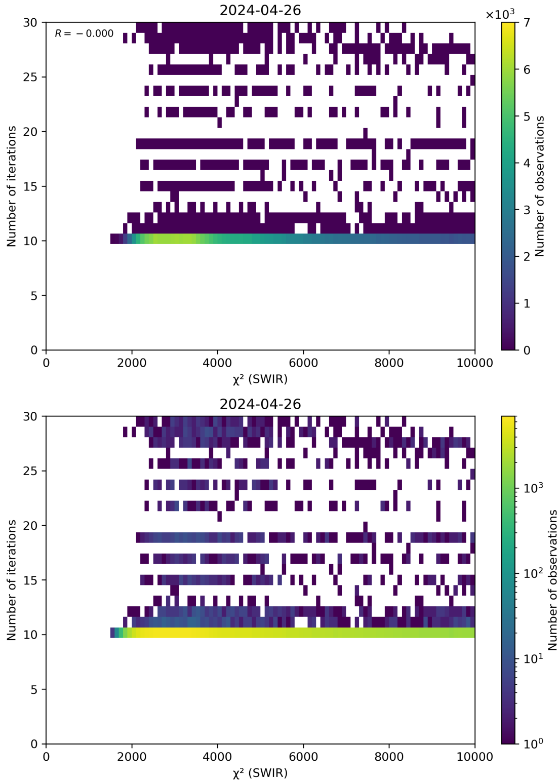
Figure 50: Scatter density plot of “ \chi^2 (SWIR)” against “Number of iterations” for 2024-04-26 to 2024-04-27.
