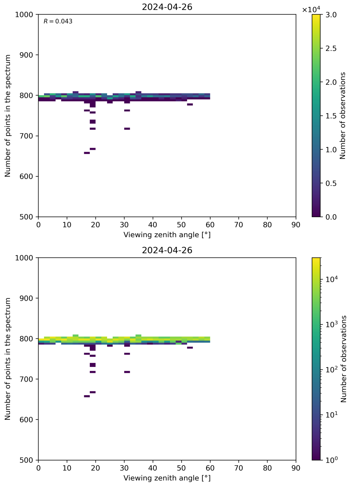
Figure 114: Scatter density plot of “Viewing zenith angle” against “Number of points in the spectrum” for 2024-04-26 to 2024-04-27.
