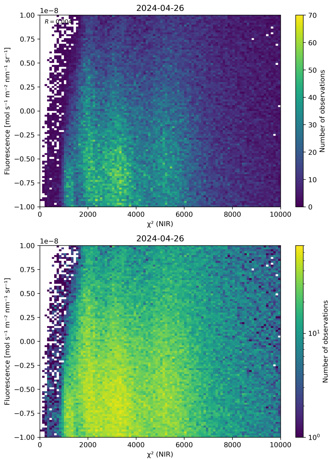
Figure 45: Scatter density plot of “ \chi^2 (NIR)” against “Fluorescence” for 2024-04-26 to 2024-04-27.
