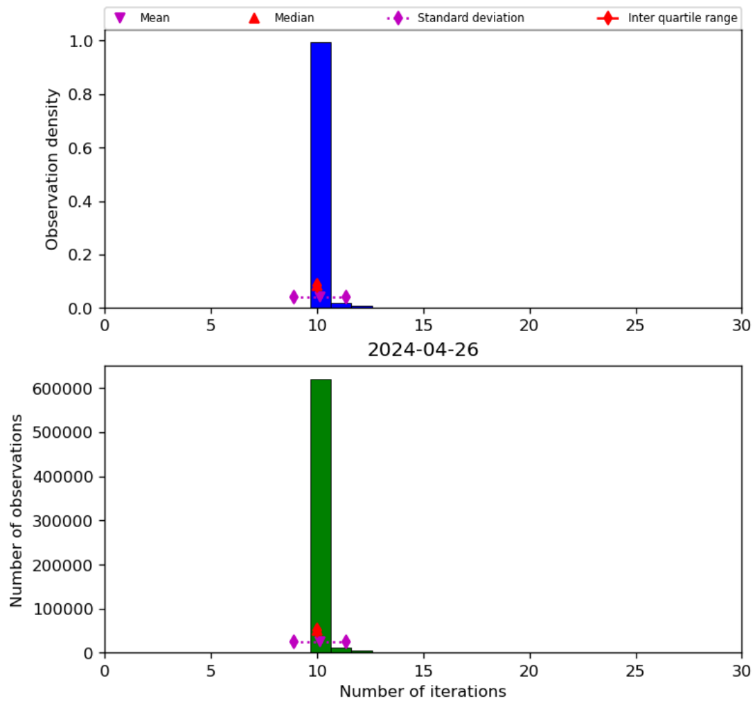
Figure 31: Histogram of “Number of iterations” for 2024-04-26 to 2024-04-27
