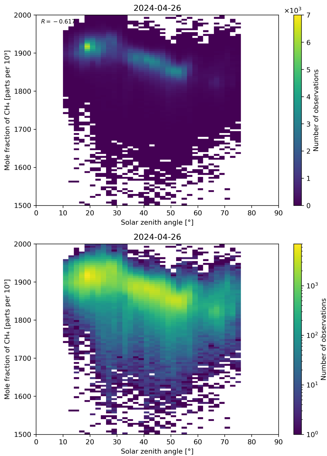
Figure 99: Scatter density plot of “Solar zenith angle” against “Mole fraction of \text{CH}_4 ” for 2024-04-26 to 2024-04-27.
