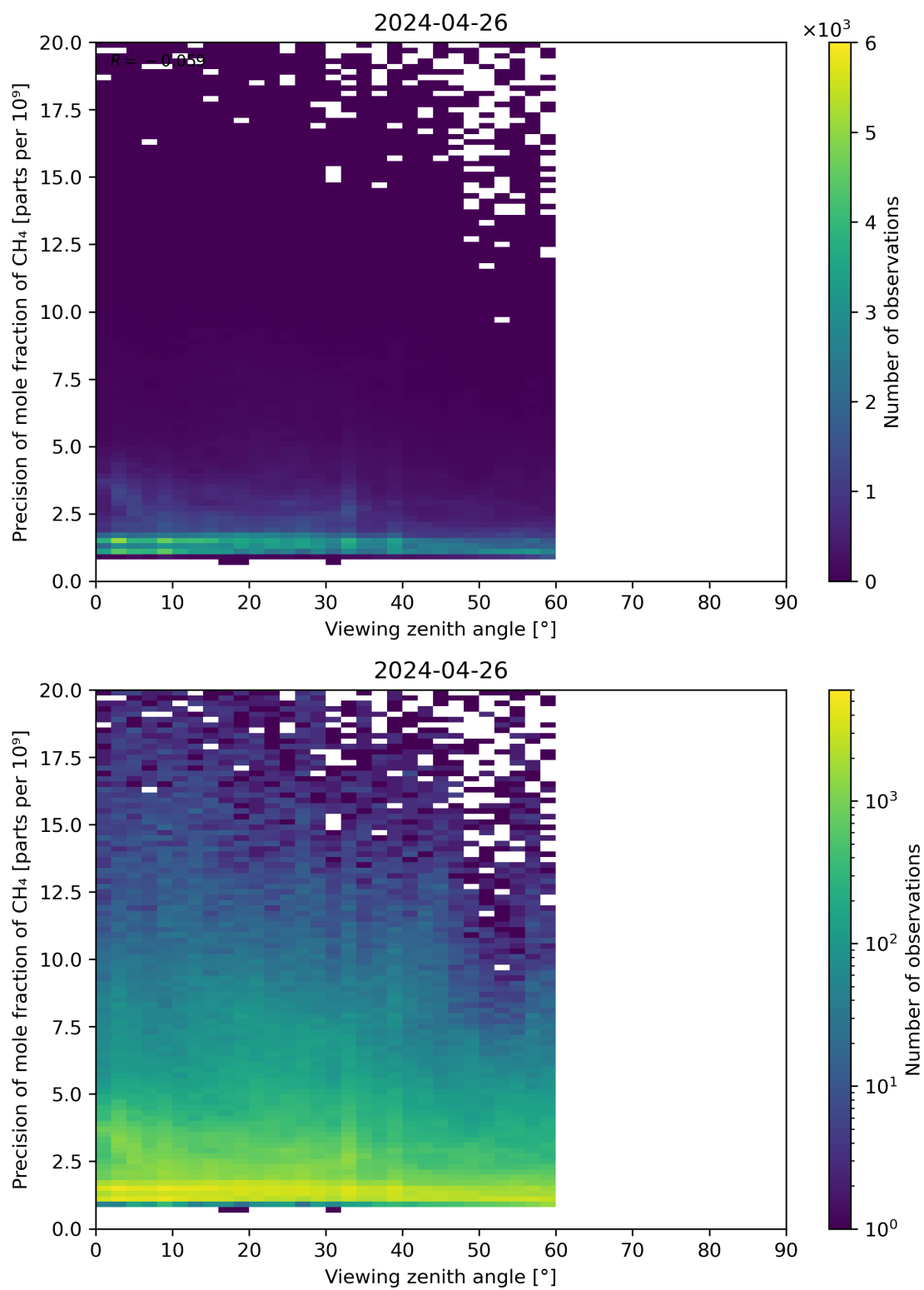
Figure 112: Scatter density plot of “Viewing zenith angle” against “Precision of mole fraction of CH 4 ” for 2024-04-26 to 2024-04-27.
