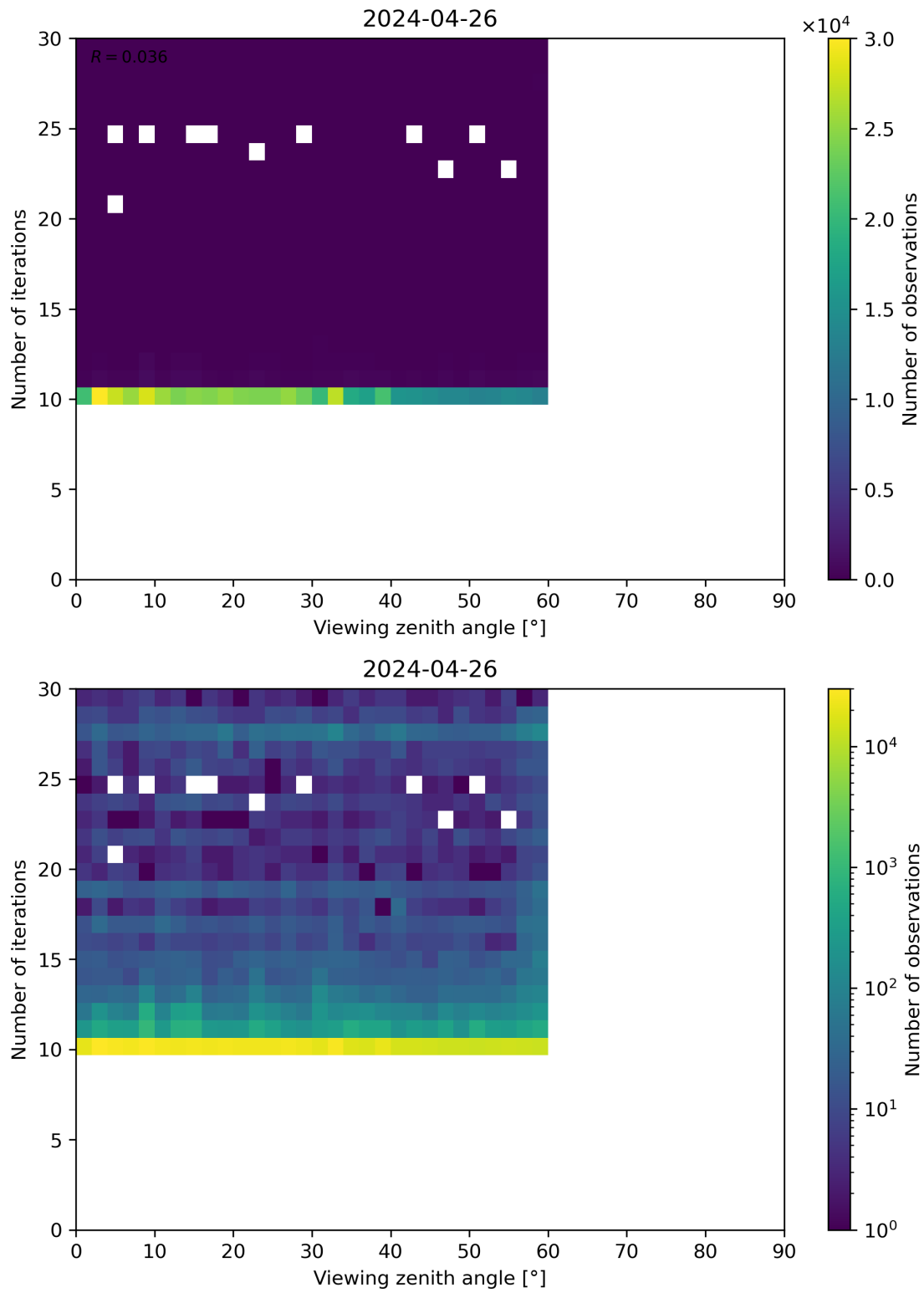
Figure 113: Scatter density plot of “Viewing zenith angle” against “Number of iterations” for 2024-04-26 to 2024-04-27.
