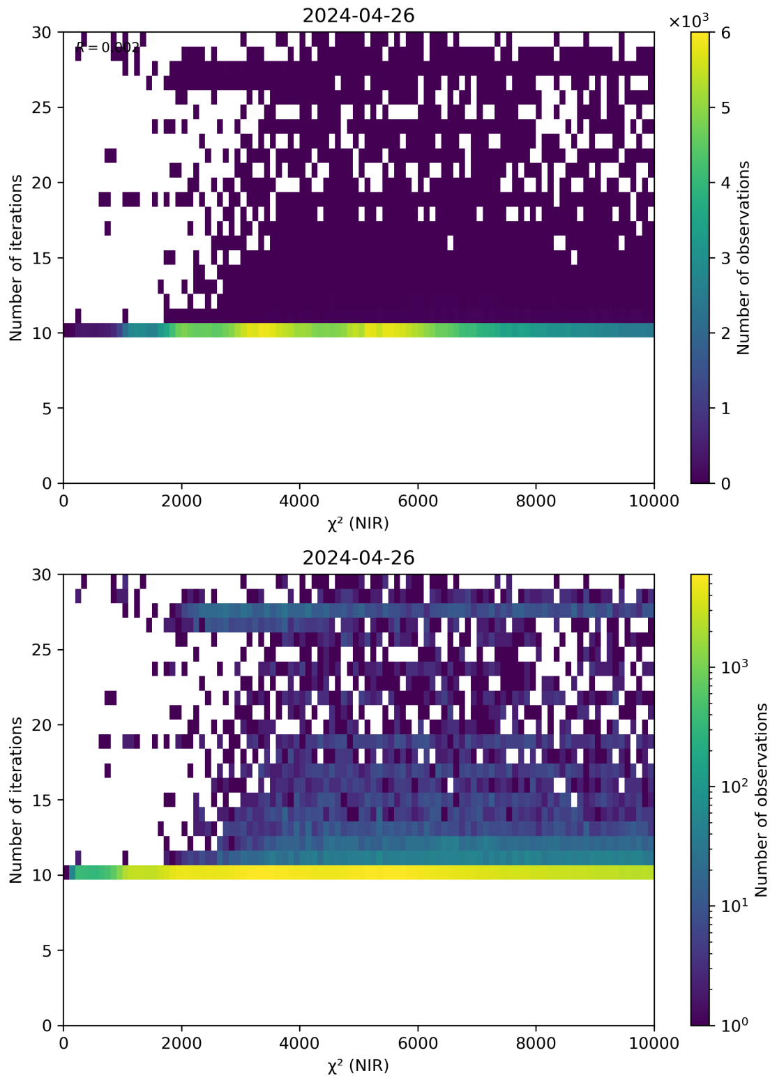
Figure 46: Scatter density plot of “ \chi^2 (NIR)” against “Number of iterations” for 2024-04-26 to 2024-04-27.
