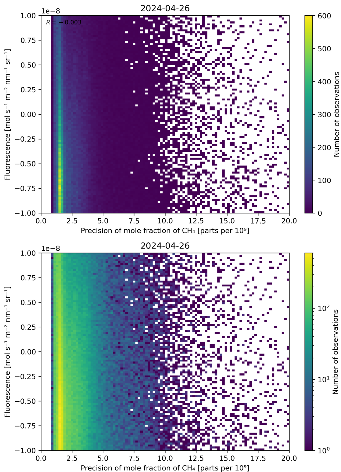
Figure 81: Scatter density plot of “Precision of mole fraction of CH 4 ” against “Fluorescence” for 2024-04-26 to 2024-04-27.
