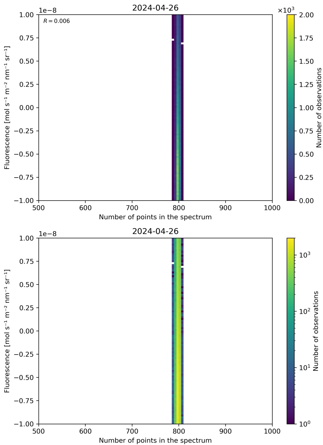
Figure 91: Scatter density plot of “Number of points in the spectrum” against “Fluorescence” for 2024-04-26 to 2024-04-27.
