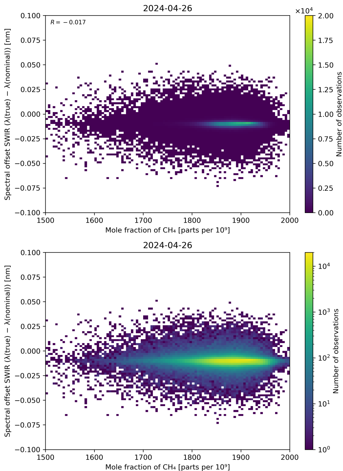
Figure 86: Scatter density plot of “Mole fraction of CH 4 ” against “Spectral offset SWIR ( \lambda(\text{true}) - \lambda(\text{nominal}) )” for 2024-04-26 to 2024-04-27.
