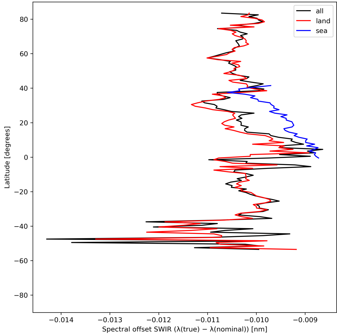
Figure 16: Zonal average of “Spectral offset SWIR ( \lambda(\text{true}) - \lambda(\text{nominal}) )” for 2024-04-26 to 2024-04-27.
