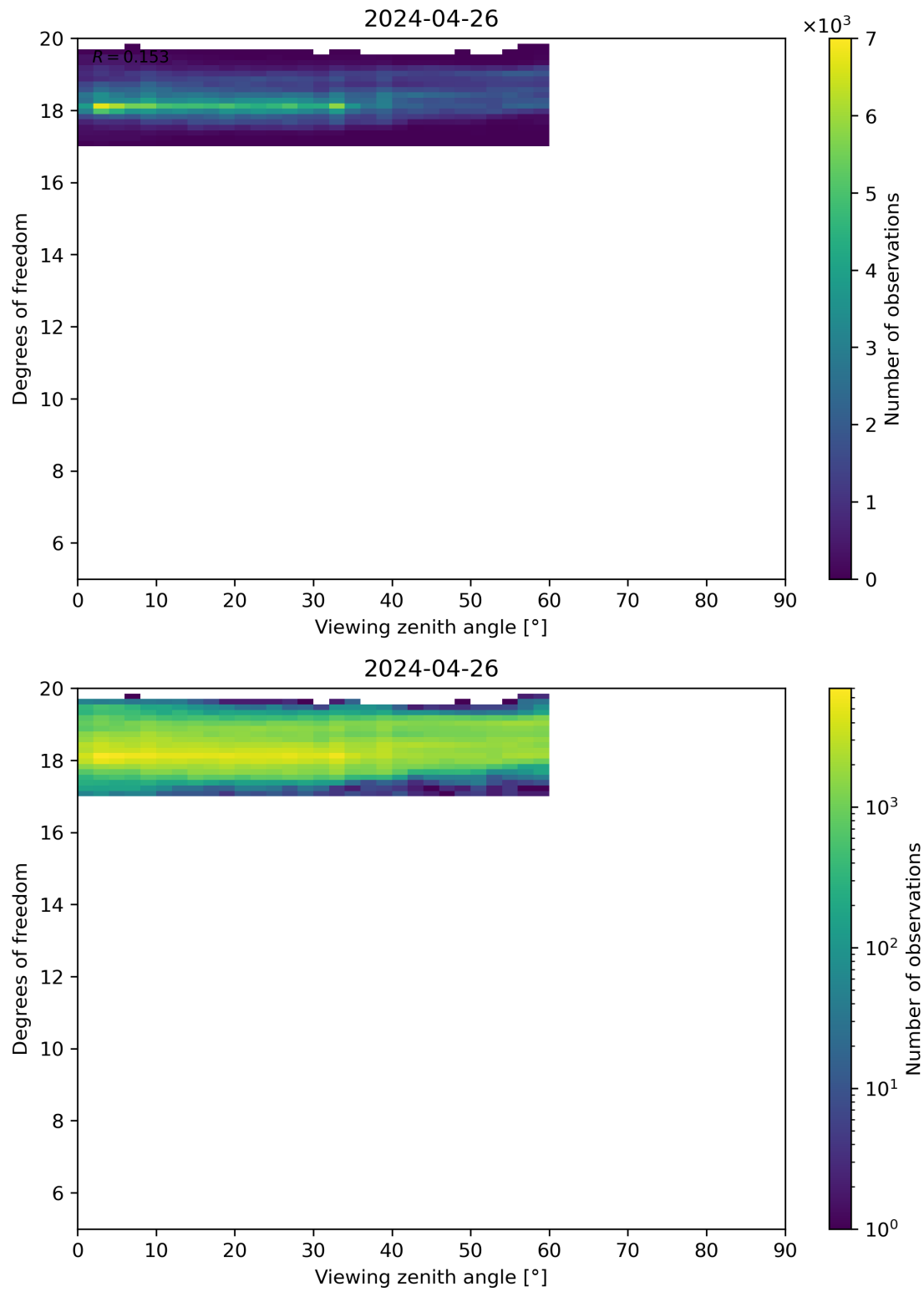
Figure 107: Scatter density plot of “Viewing zenith angle” against “Degrees of freedom” for 2024-04-26 to 2024-04-27.
