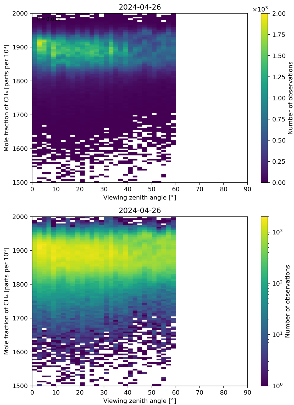
Figure 110: Scatter density plot of “Viewing zenith angle” against “Mole fraction of CH 4 ” for 2024-04-26 to 2024-04-27.
