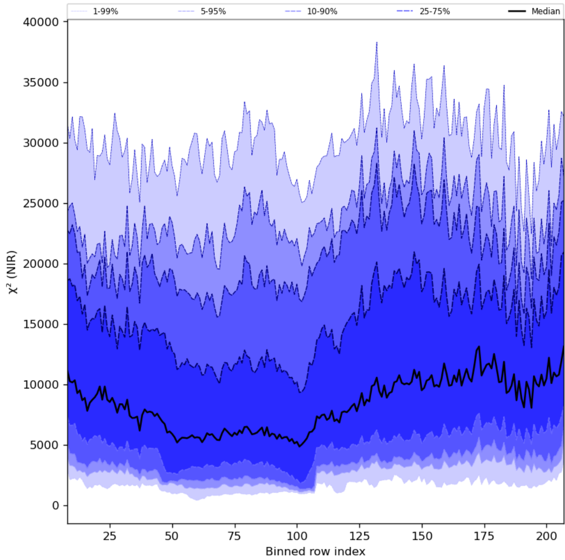
Figure 40: Along track statistics of “ \chi^2 (NIR)” for 2024-04-26 to 2024-04-27
