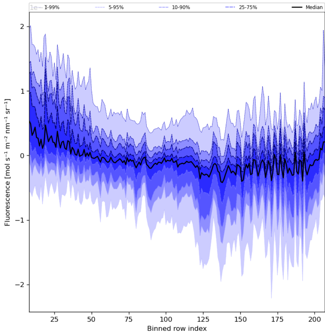
Figure 43: Along track statistics of “Fluorescence” for 2024-04-26 to 2024-04-27
