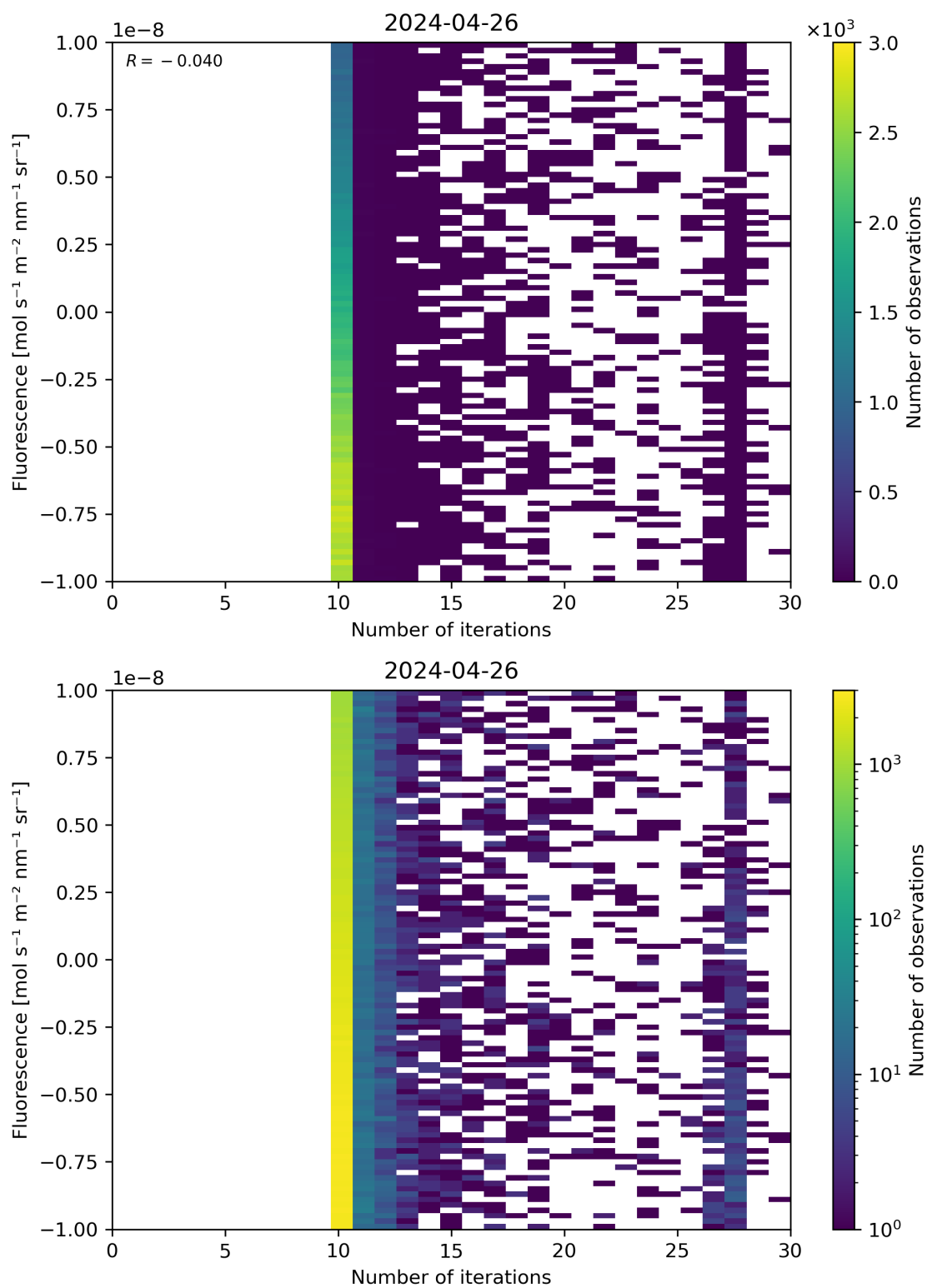
Figure 87: Scatter density plot of “Number of iterations” against “Fluorescence” for 2024-04-26 to 2024-04-27.
