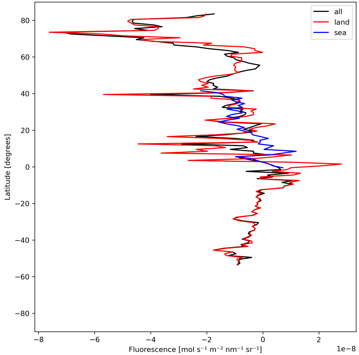
Figure 21: Zonal average of “Fluorescence” for 2024-04-26 to 2024-04-27.
