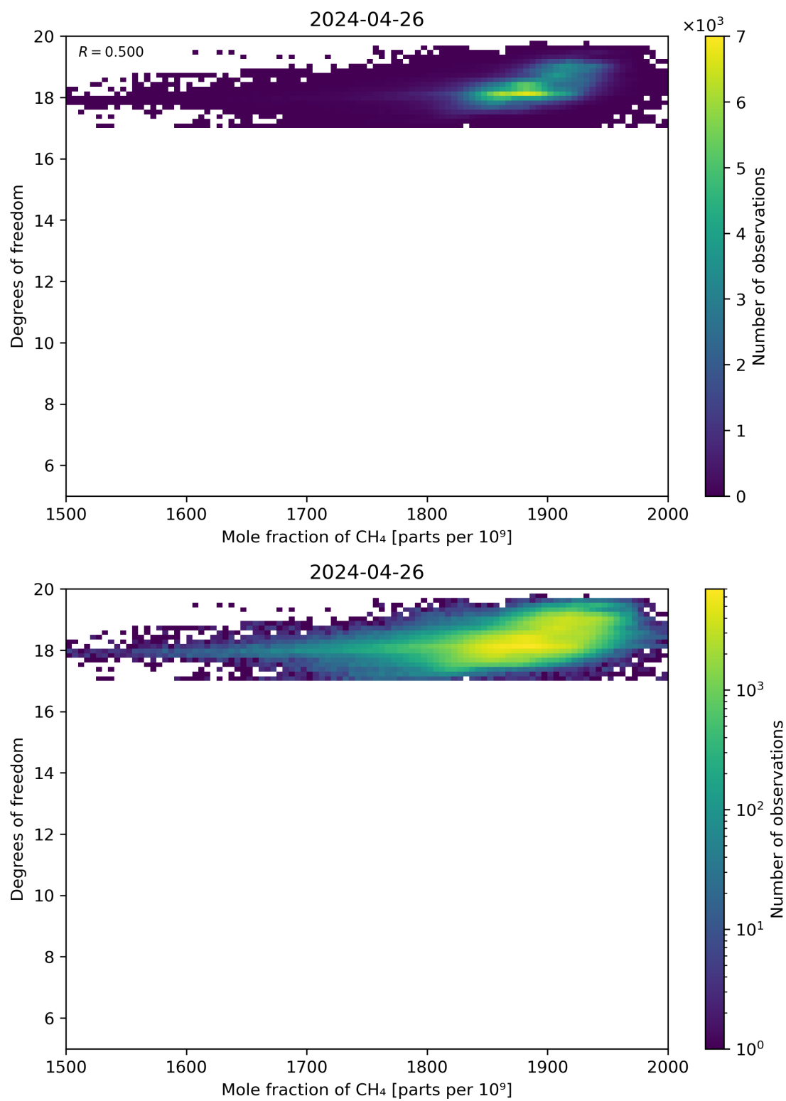
Figure 72: Scatter density plot of “Mole fraction of CH 4 ” against “Degrees of freedom” for 2024-04-26 to 2024-04-27.
