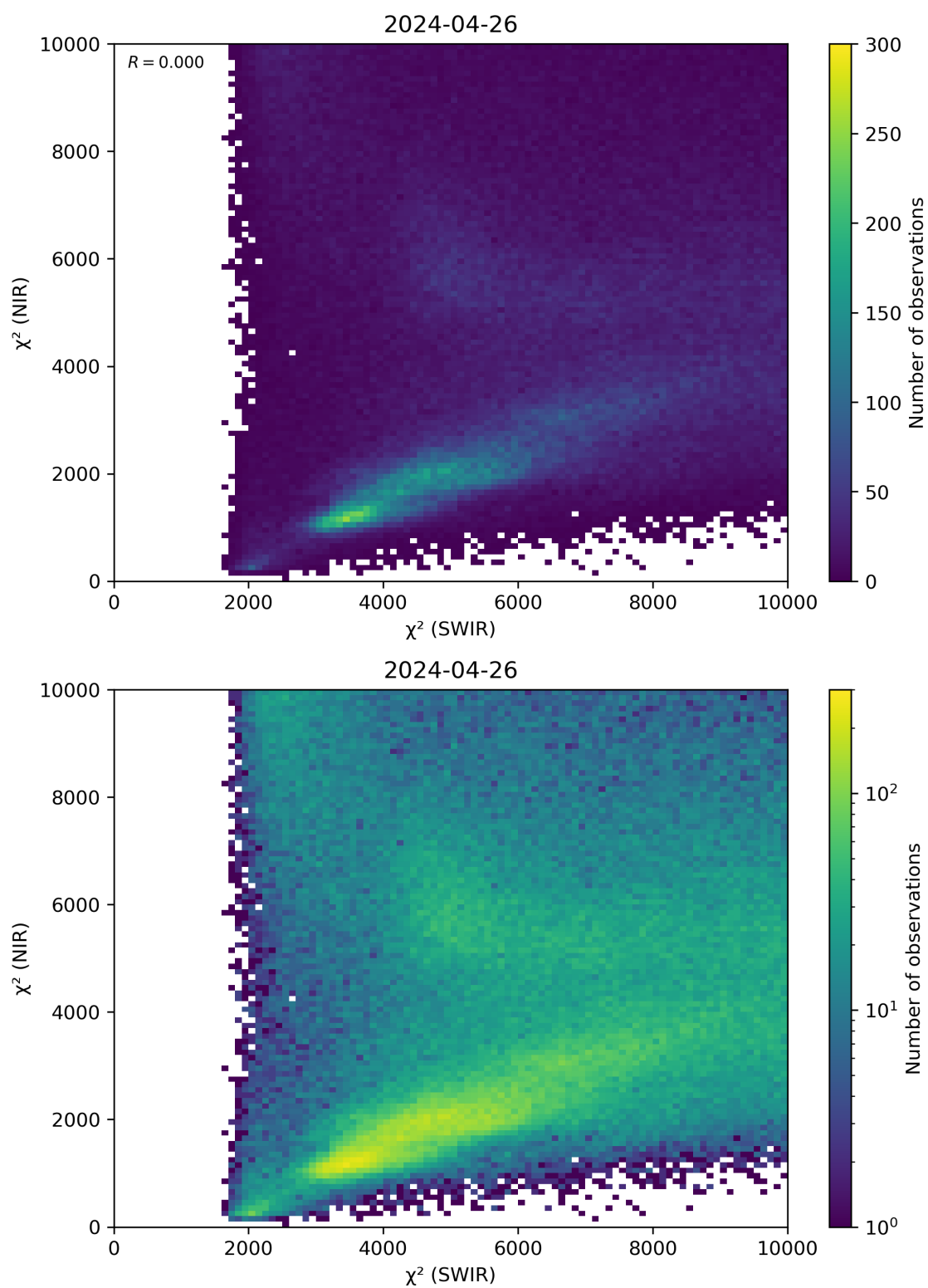
Figure 47: Scatter density plot of “ \chi^2 (SWIR)” against “ \chi^2 (NIR)” for 2024-04-26 to 2024-04-27.
