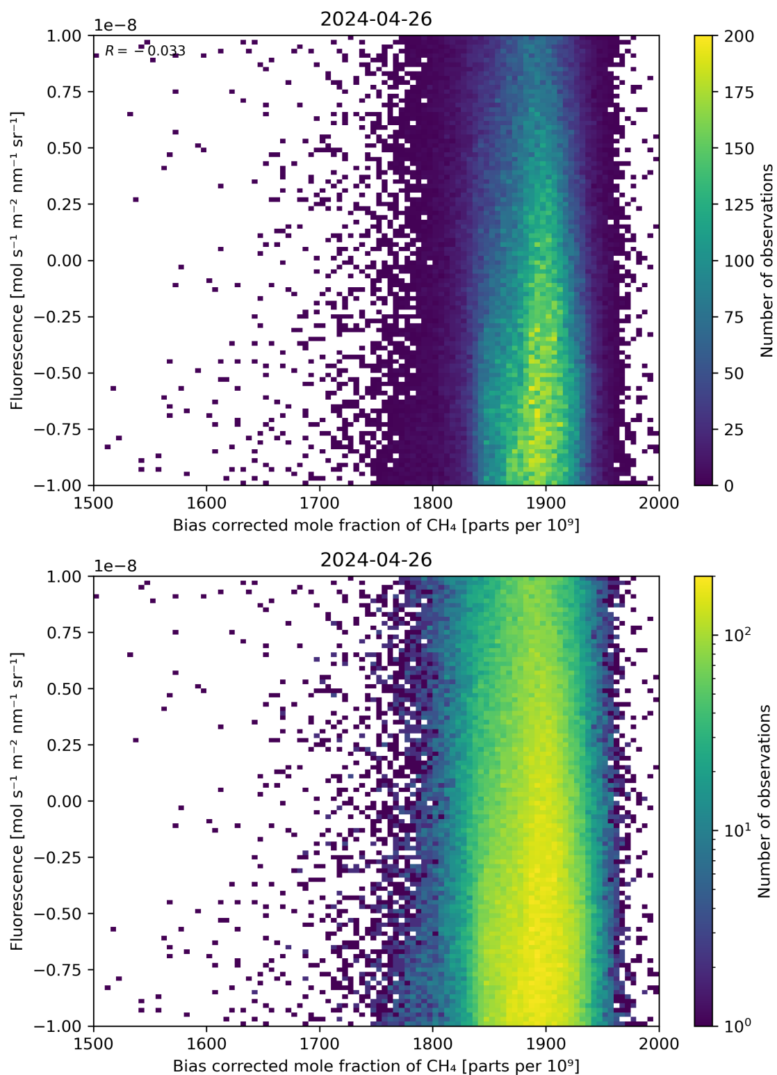
Figure 66: Scatter density plot of “Bias corrected mole fraction of \text{CH}_4 ” against “Fluorescence” for 2024-04-26 to 2024-04-27.
