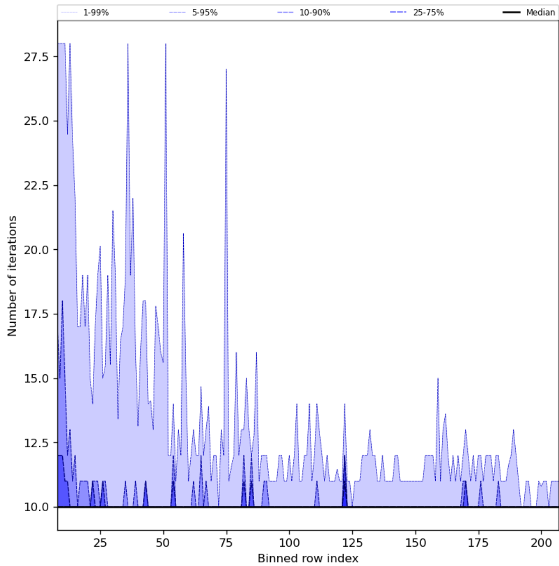
Figure 42: Along track statistics of “Number of iterations” for 2024-04-26 to 2024-04-27
