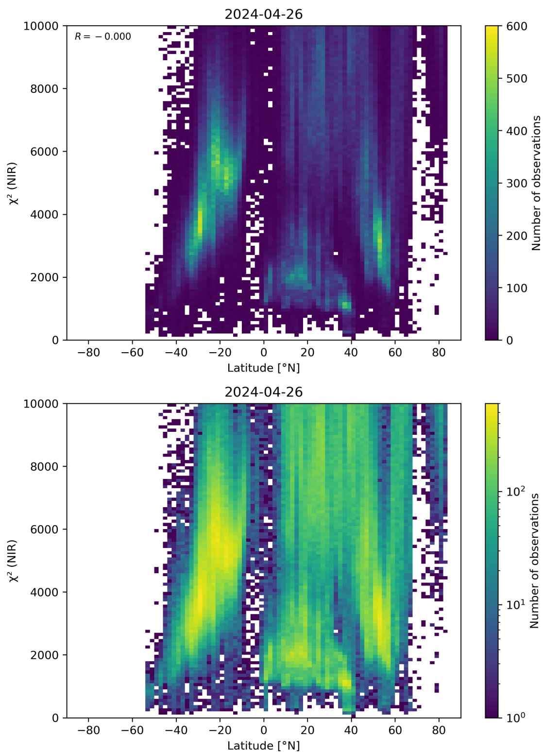
Figure 53: Scatter density plot of “Latitude” against “ \chi^2 (NIR)” for 2024-04-26 to 2024-04-27.
