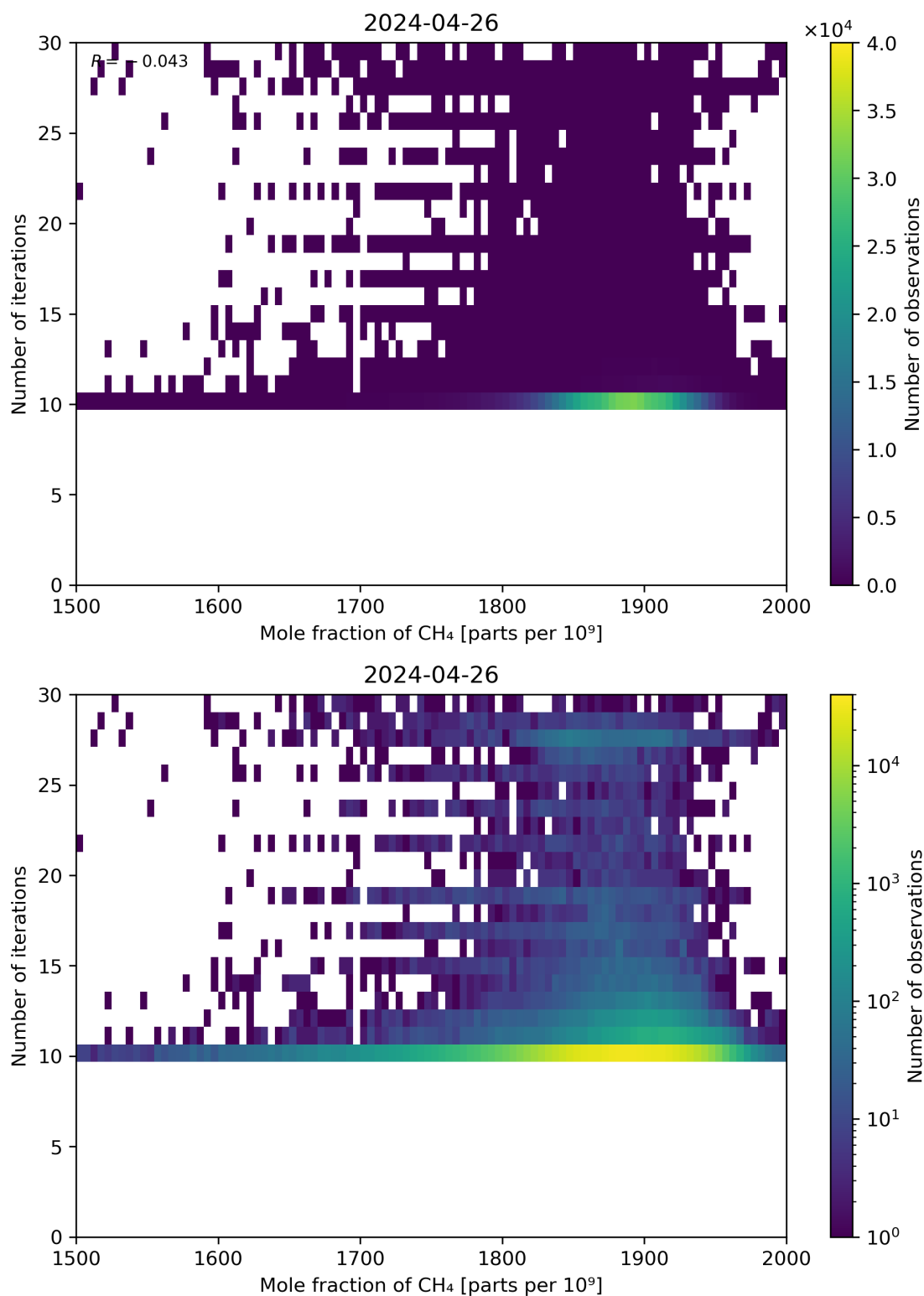
Figure 76: Scatter density plot of “Mole fraction of CH 4 ” against “Number of iterations” for 2024-04-26 to 2024-04-27.
