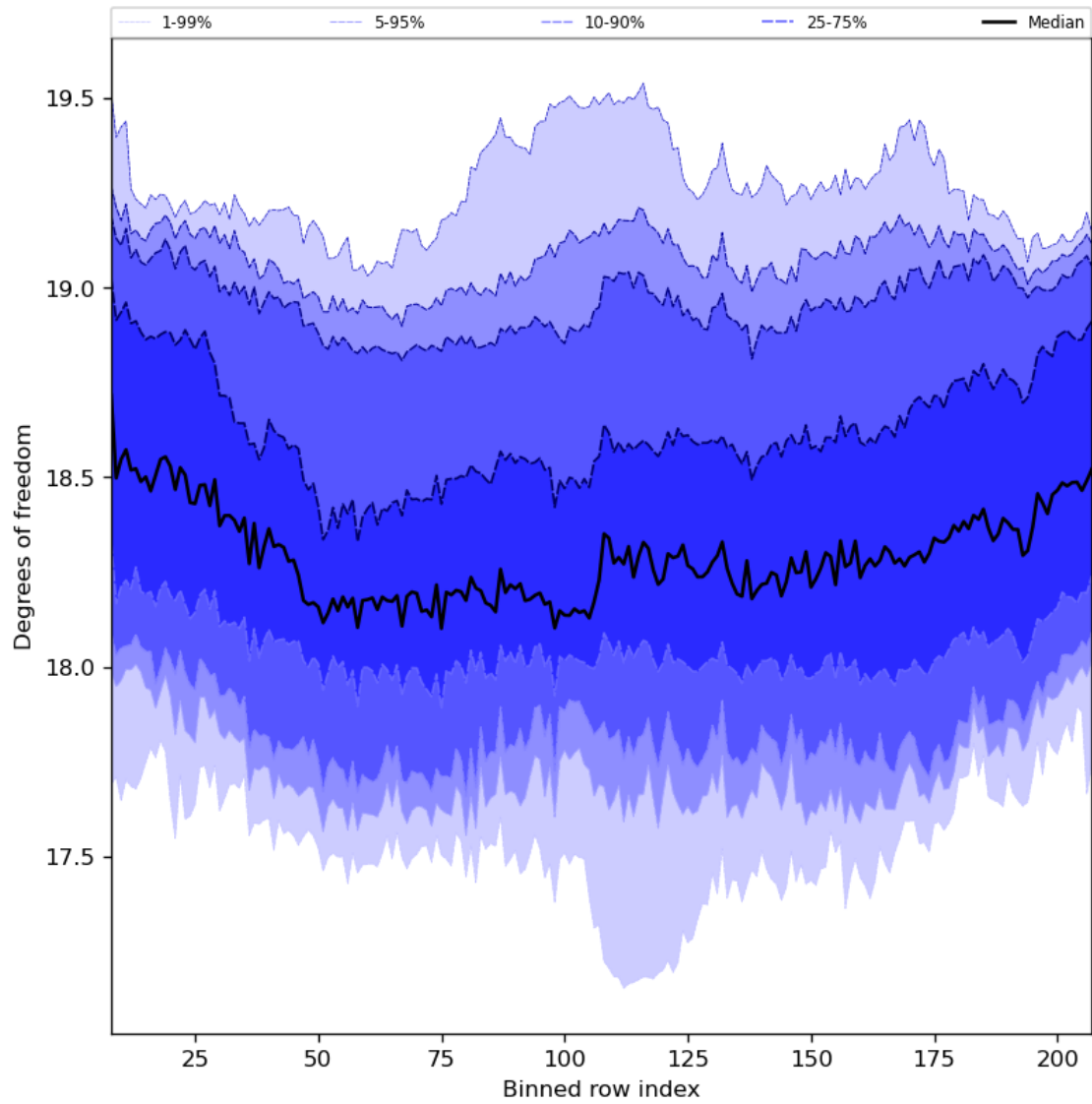
Figure 41: Along track statistics of “Degrees of freedom” for 2024-04-26 to 2024-04-27
