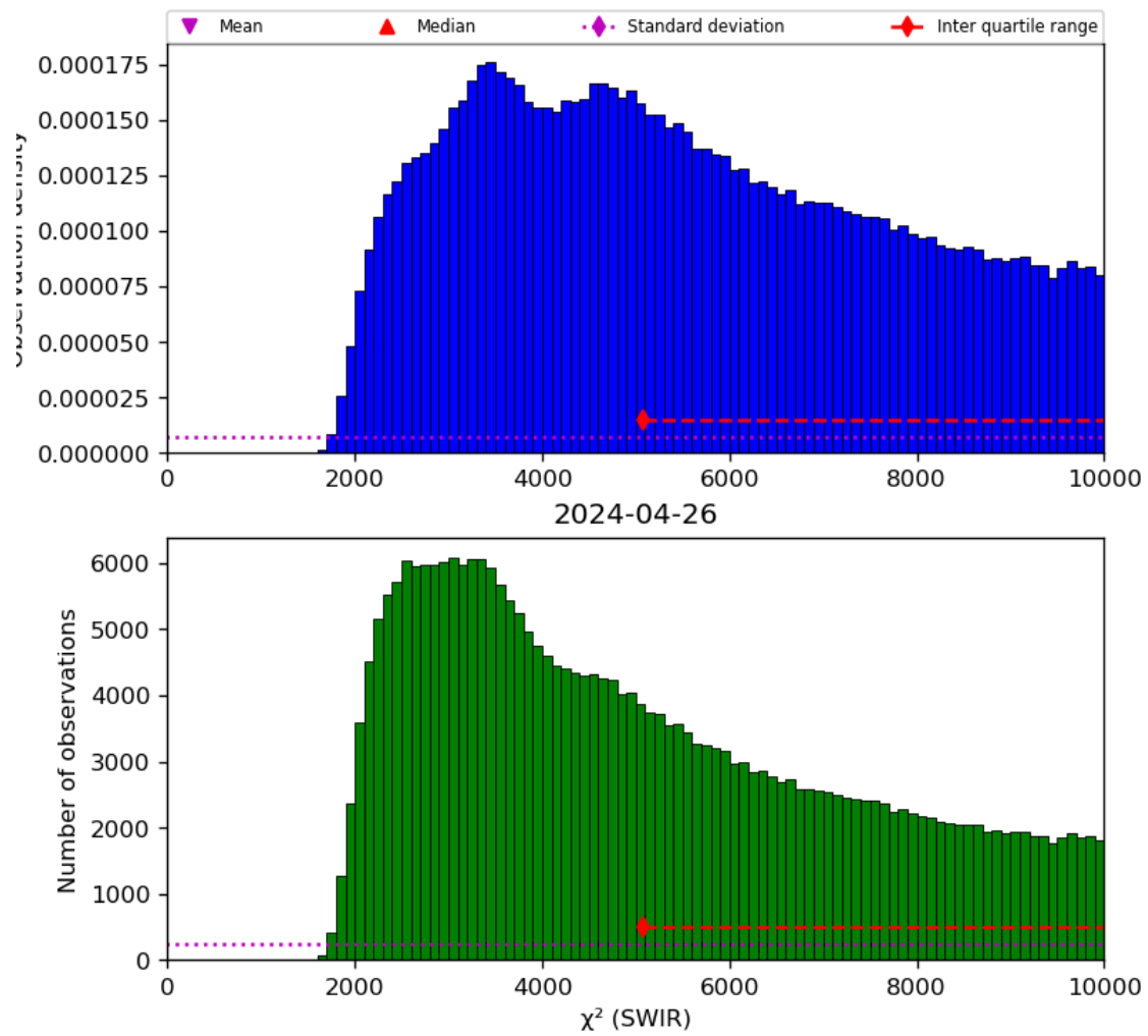
Figure 28: Histogram of “ \chi^2 (SWIR)” for 2024-04-26 to 2024-04-27
