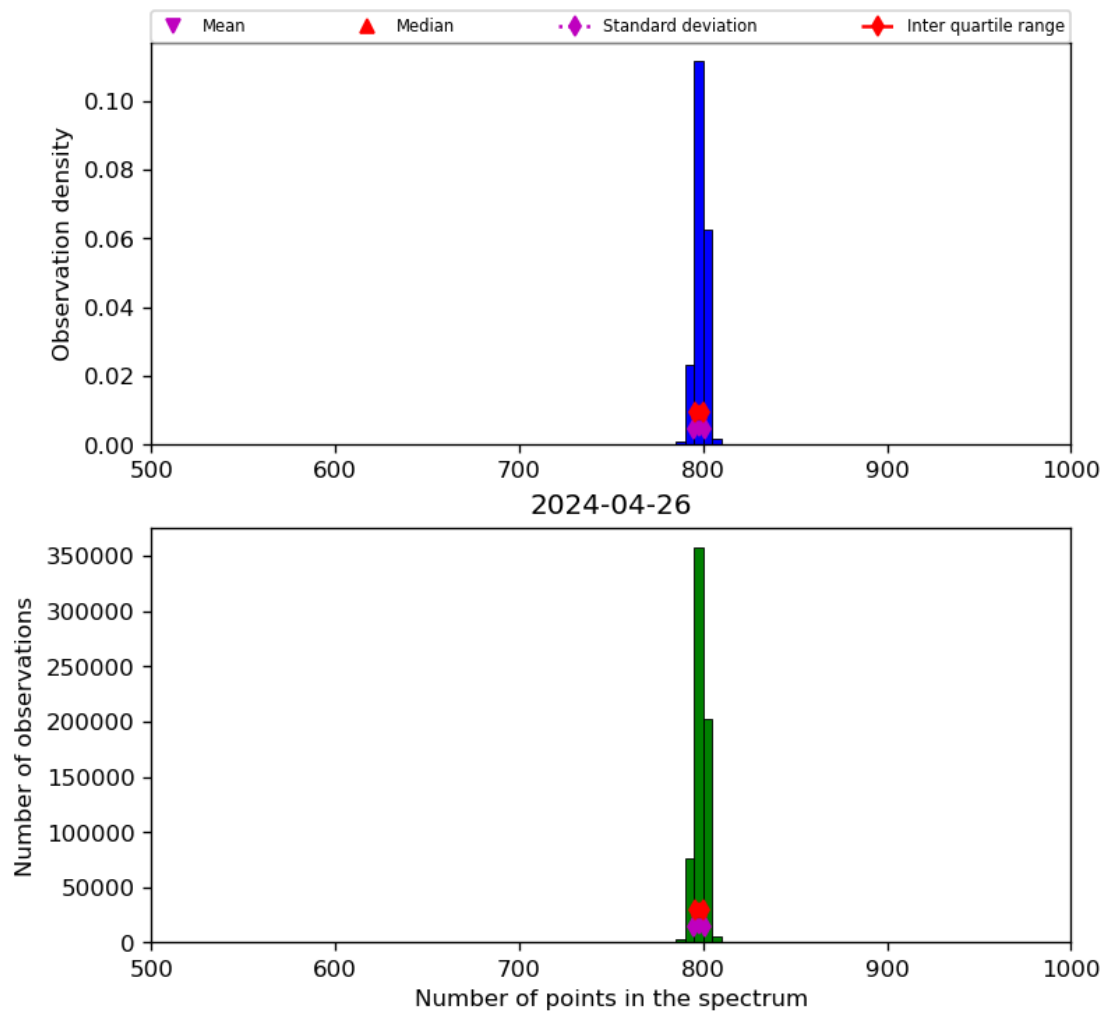
Figure 26: Histogram of “Number of points in the spectrum” for 2024-04-26 to 2024-04-27
