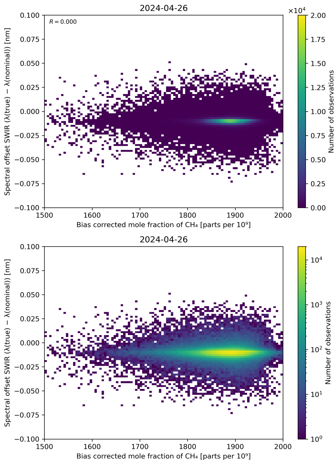
Figure 69: Scatter density plot of “Bias corrected mole fraction of \text{CH}_4 ” against “Spectral offset SWIR ( \lambda(\text{true}) - \lambda(\text{nominal}) )” for 2024-04-26 to 2024-04-27.
