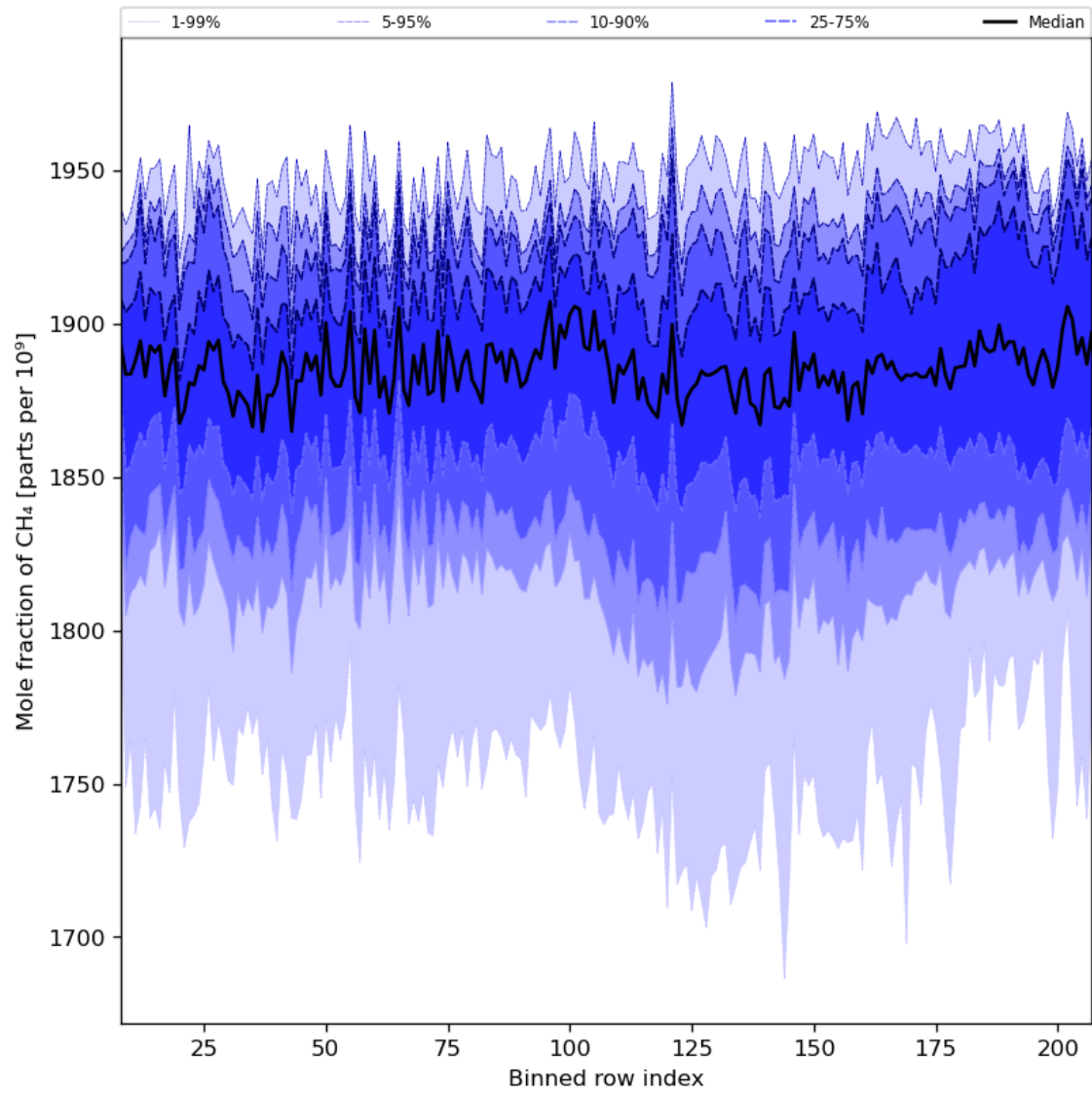
Figure 34: Along track statistics of “Mole fraction of CH 4 ” for 2024-04-26 to 2024-04-27
