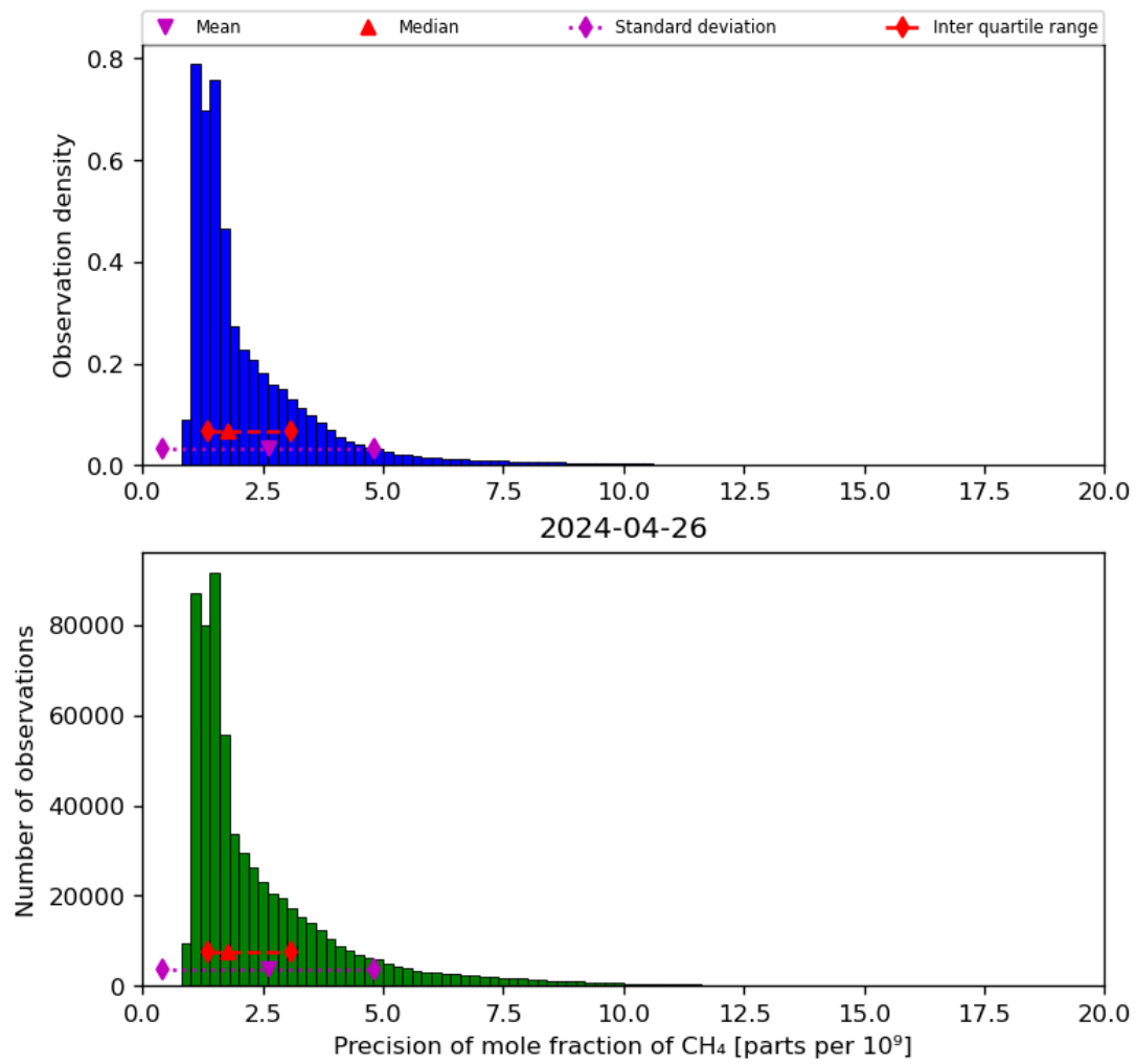
Figure 24: Histogram of “Precision of mole fraction of CH 4 ” for 2024-04-26 to 2024-04-27
