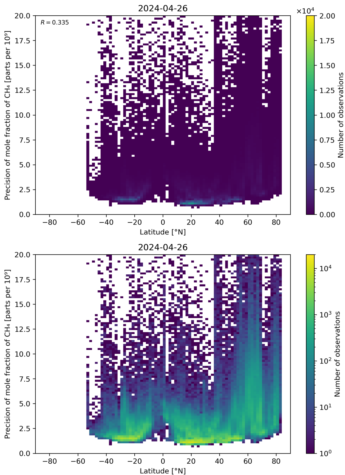
Figure 59: Scatter density plot of “Latitude” against “Precision of mole fraction of \text{CH}_4 ” for 2024-04-26 to 2024-04-27.
