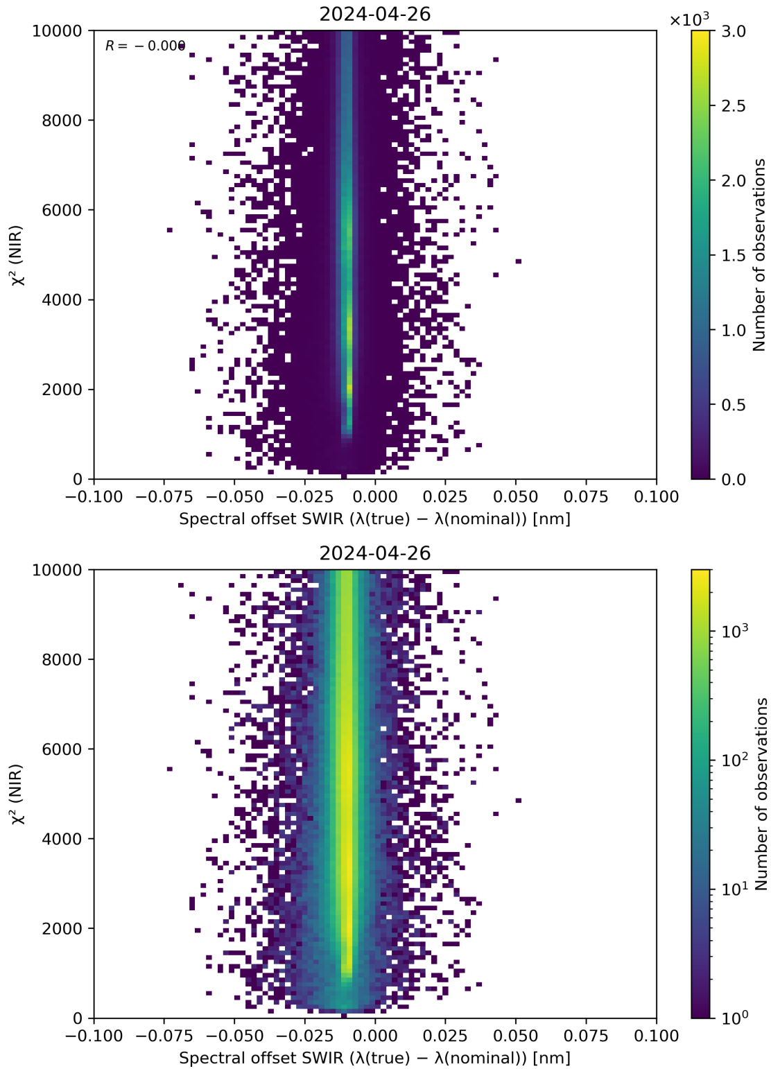
Figure 117: Scatter density plot of “Spectral offset SWIR ( \lambda(\text{true}) - \lambda(\text{nominal}) )” against “ \chi^2 (NIR)” for 2024-04-26 to 2024-04-27.
