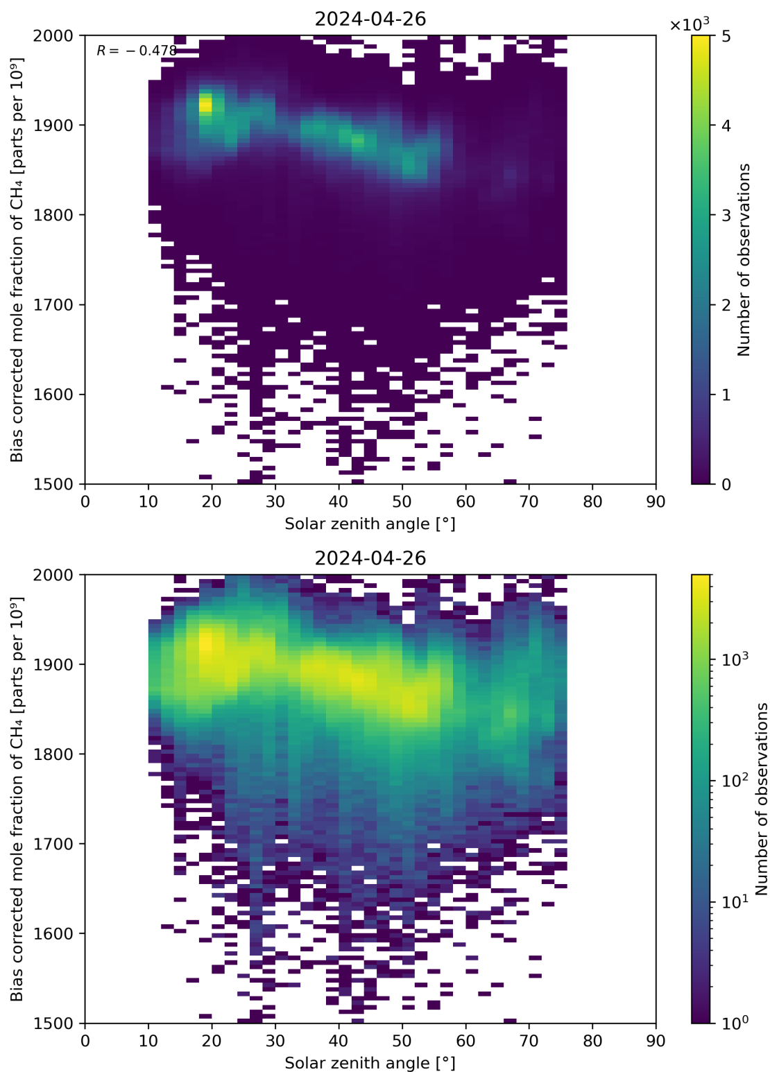
Figure 100: Scatter density plot of “Solar zenith angle” against “Bias corrected mole fraction of CH 4 ” for 2024-04-26 to 2024-04-27.
