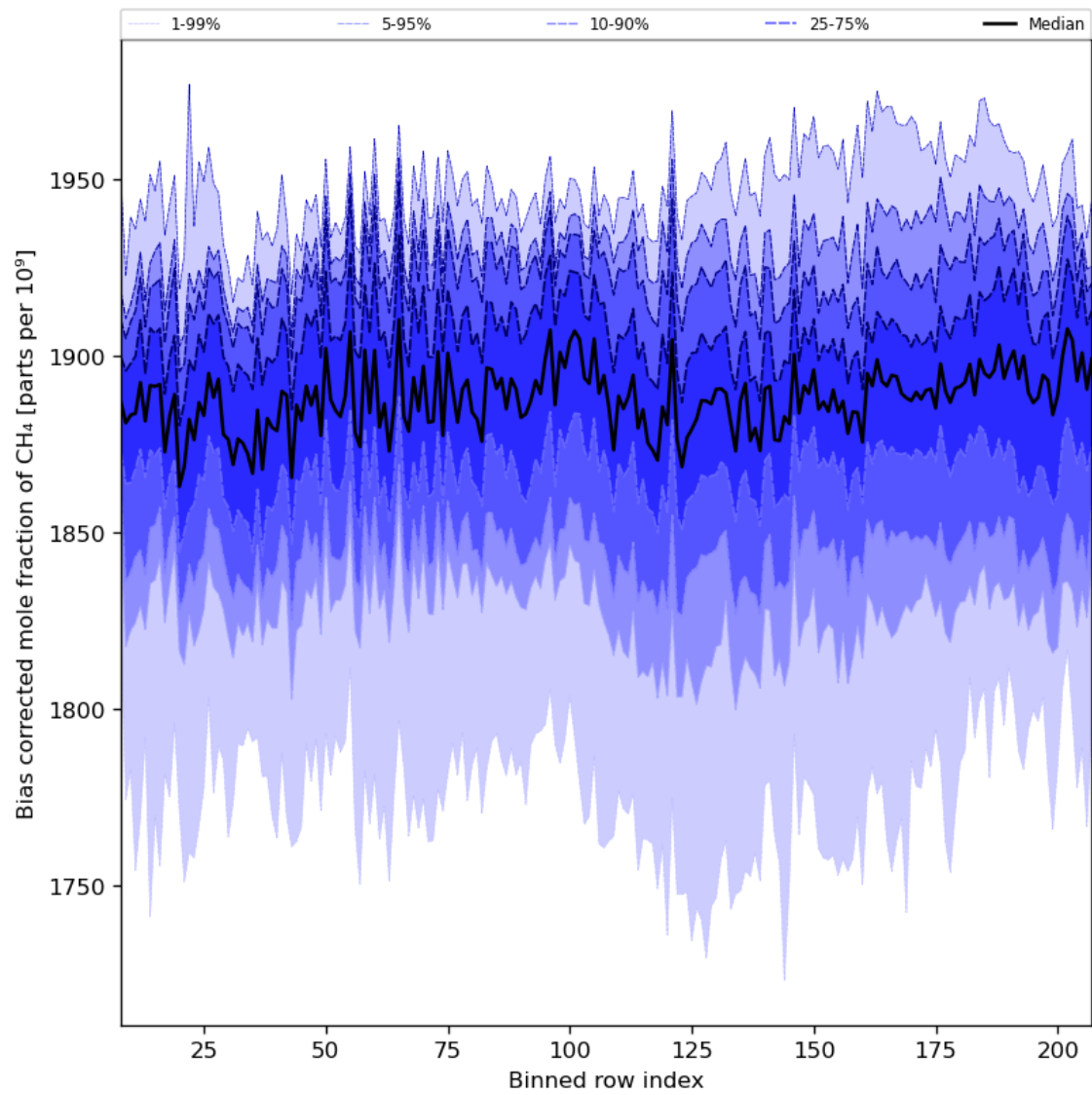
Figure 36: Along track statistics of “Bias corrected mole fraction of CH 4 ” for 2024-04-26 to 2024-04-27
