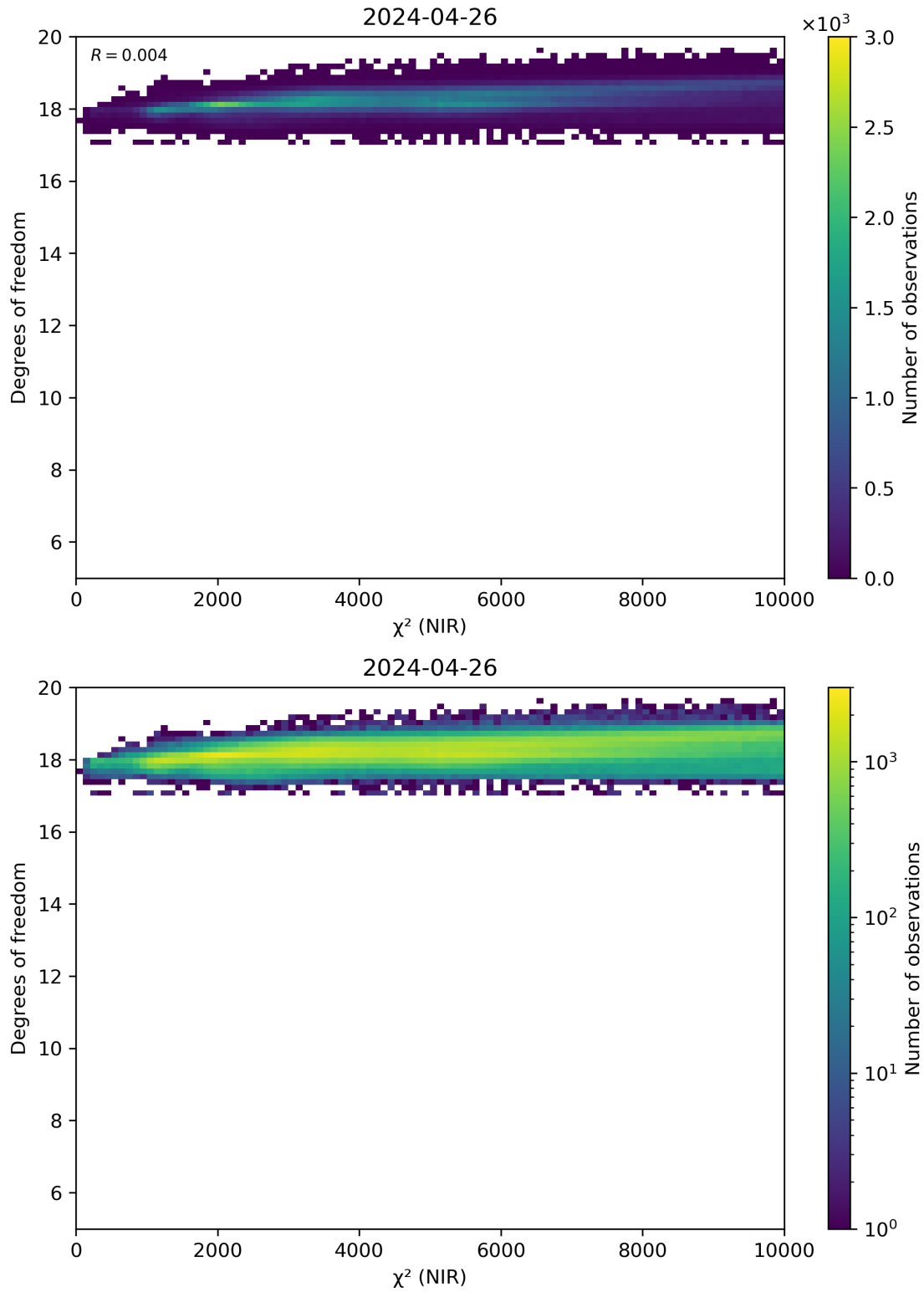
Figure 44: Scatter density plot of “ \chi^2 (NIR)” against “Degrees of freedom” for 2024-04-26 to 2024-04-27.
