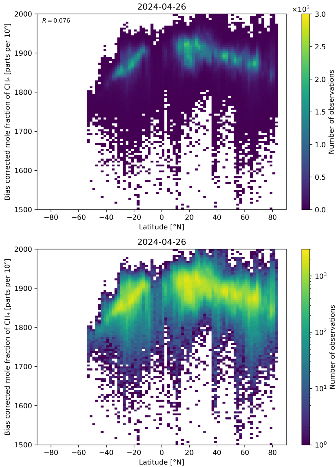
Figure 58: Scatter density plot of “Latitude” against “Bias corrected mole fraction of CH 4 ” for 2024-04-26 to 2024-04-27.
