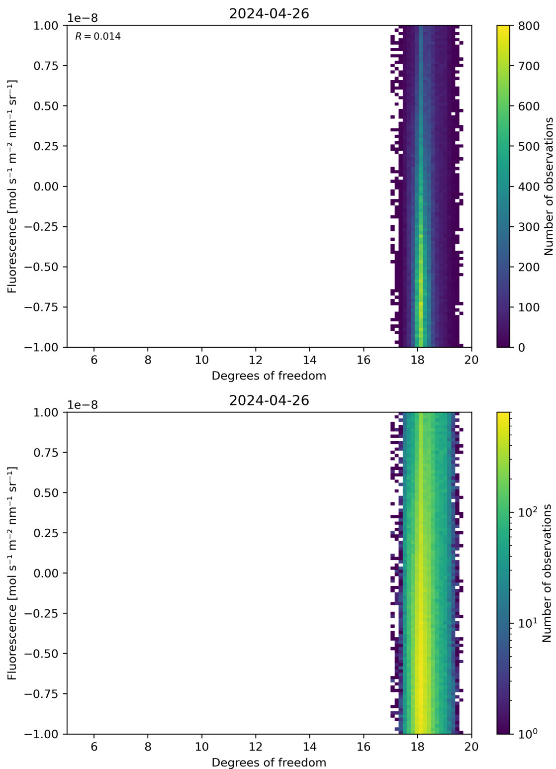
Figure 51: Scatter density plot of “Degrees of freedom” against “Fluorescence” for 2024-04-26 to 2024-04-27.
