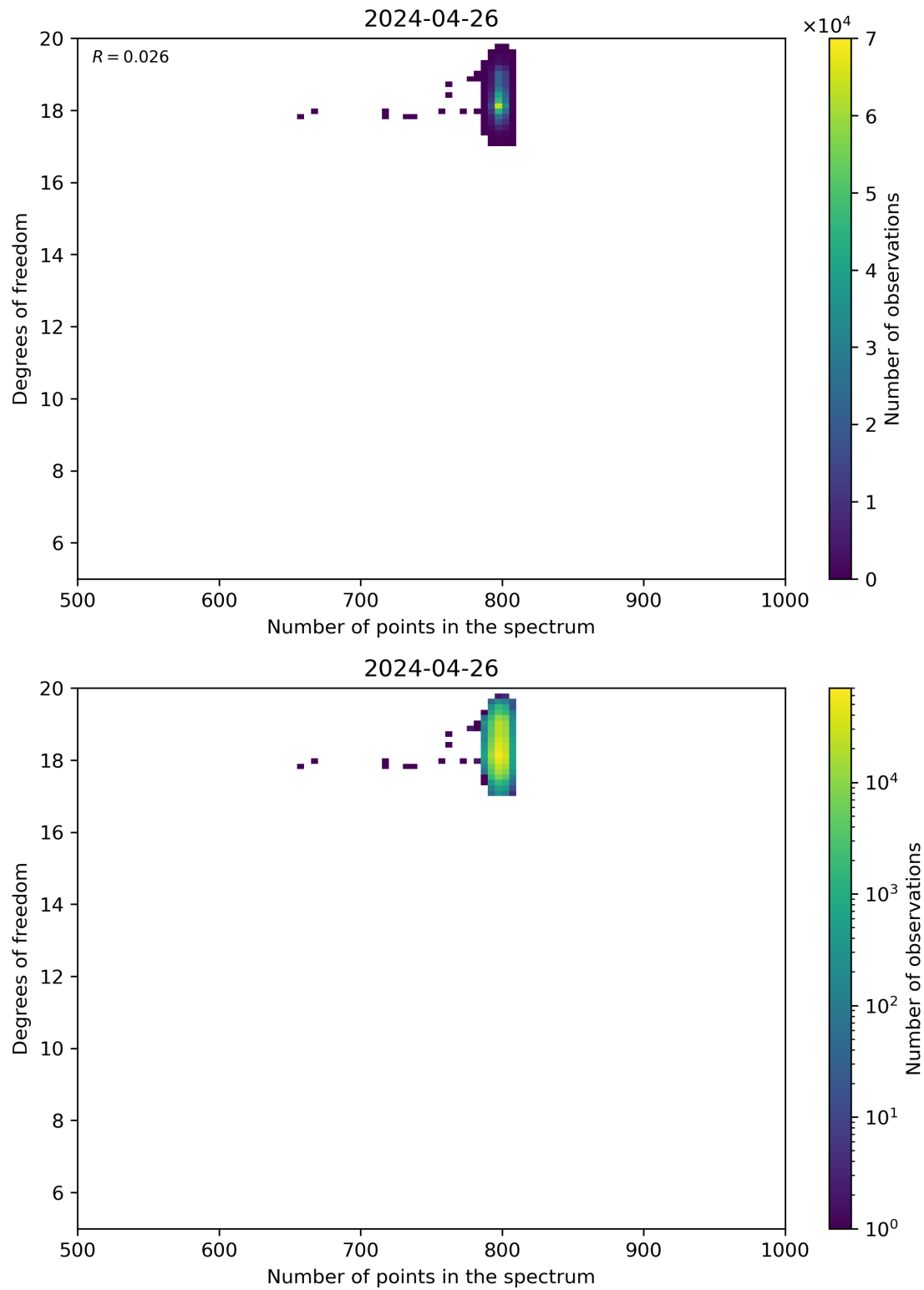
Figure 90: Scatter density plot of “Number of points in the spectrum” against “Degrees of freedom” for 2024-04-26 to 2024-04-27.
