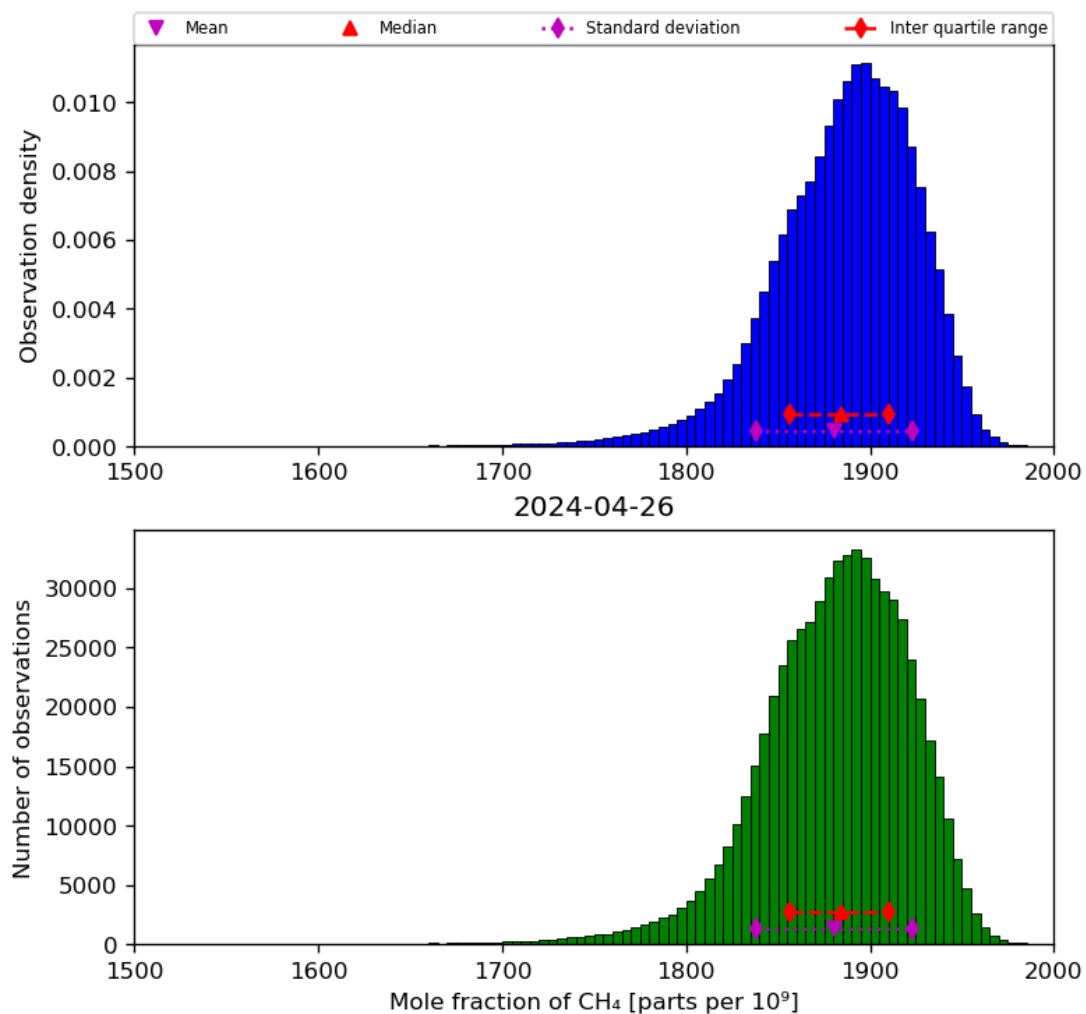
Figure 23: Histogram of “Mole fraction of CH 4 ” for 2024-04-26 to 2024-04-27
