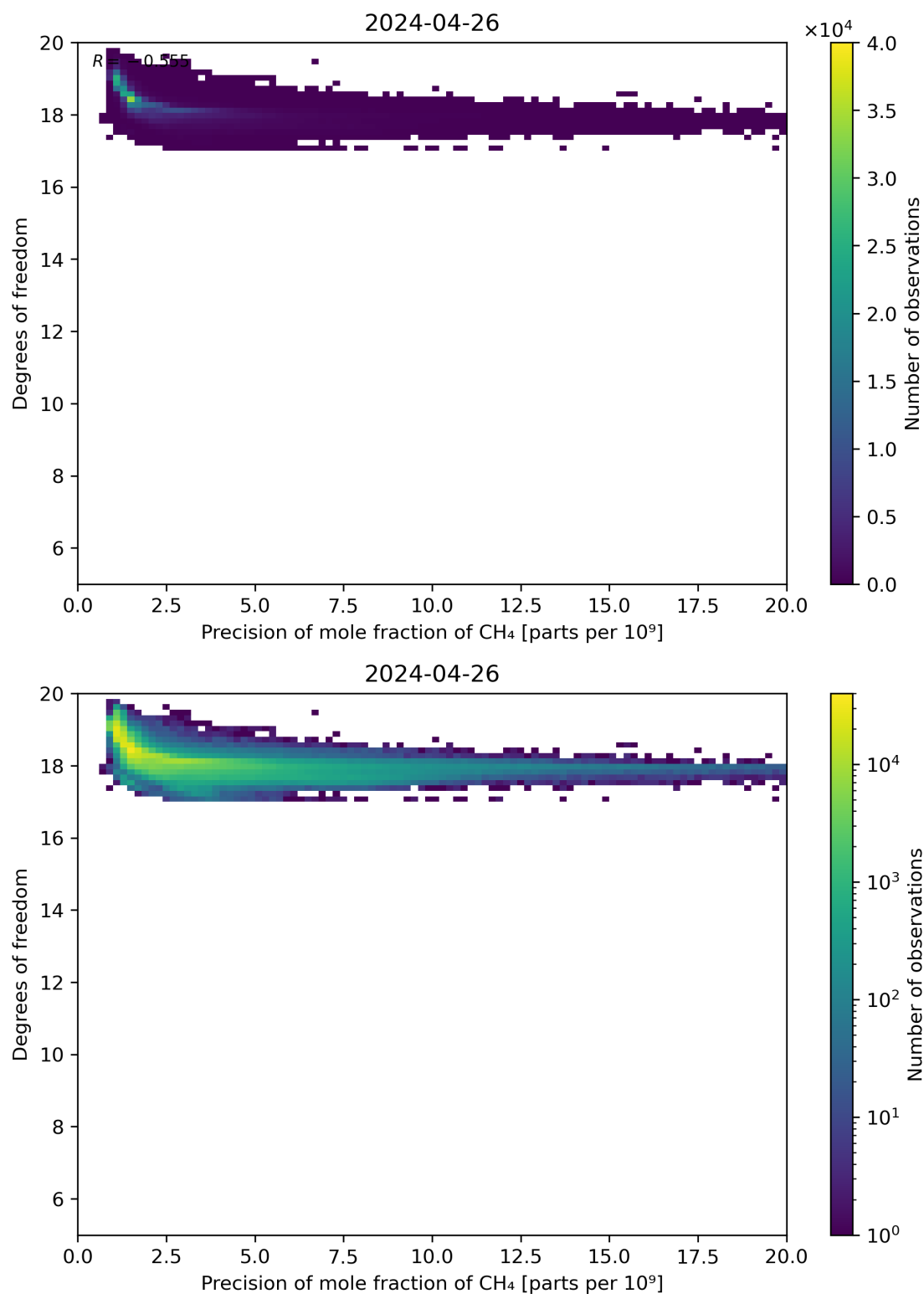
Figure 80: Scatter density plot of “Precision of mole fraction of CH 4 ” against “Degrees of freedom” for 2024-04-26 to 2024-04-27.
