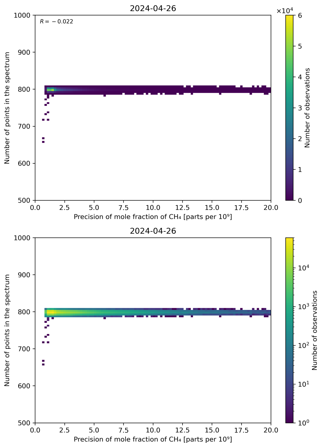
Figure 84: Scatter density plot of “Precision of mole fraction of CH 4 ” against “Number of points in the spectrum” for 2024-04-26 to 2024-04-27.
