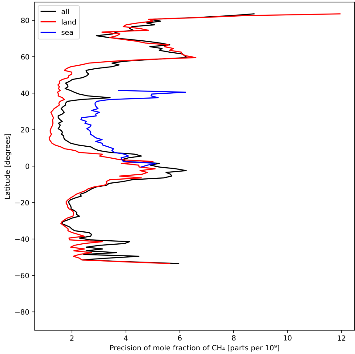
Figure 13: Zonal average of “Precision of mole fraction of CH 4 ” for 2024-04-26 to 2024-04-27.
