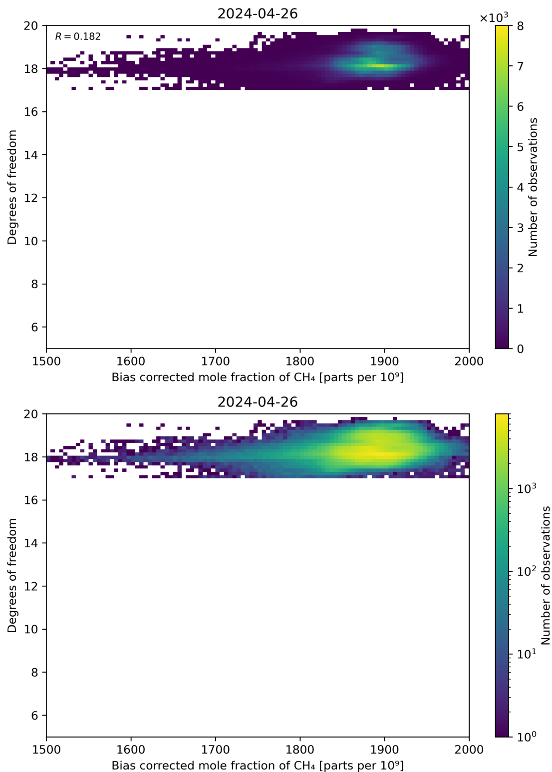
Figure 65: Scatter density plot of “Bias corrected mole fraction of CH 4 ” against “Degrees of freedom” for 2024-04-26 to 2024-04-27.
