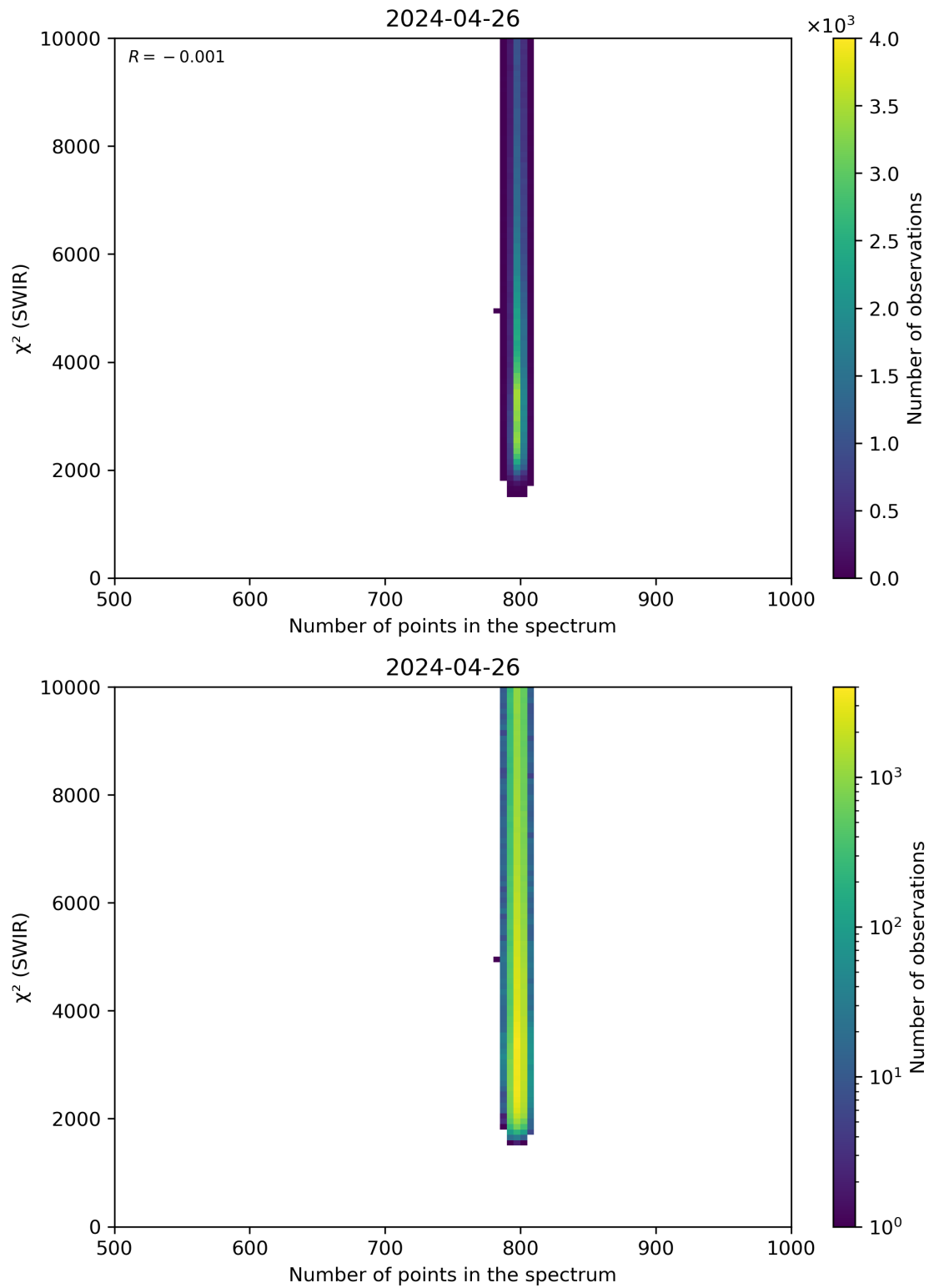
Figure 89: Scatter density plot of “Number of points in the spectrum” against “ \chi^2 (SWIR)” for 2024-04-26 to 2024-04-27.
