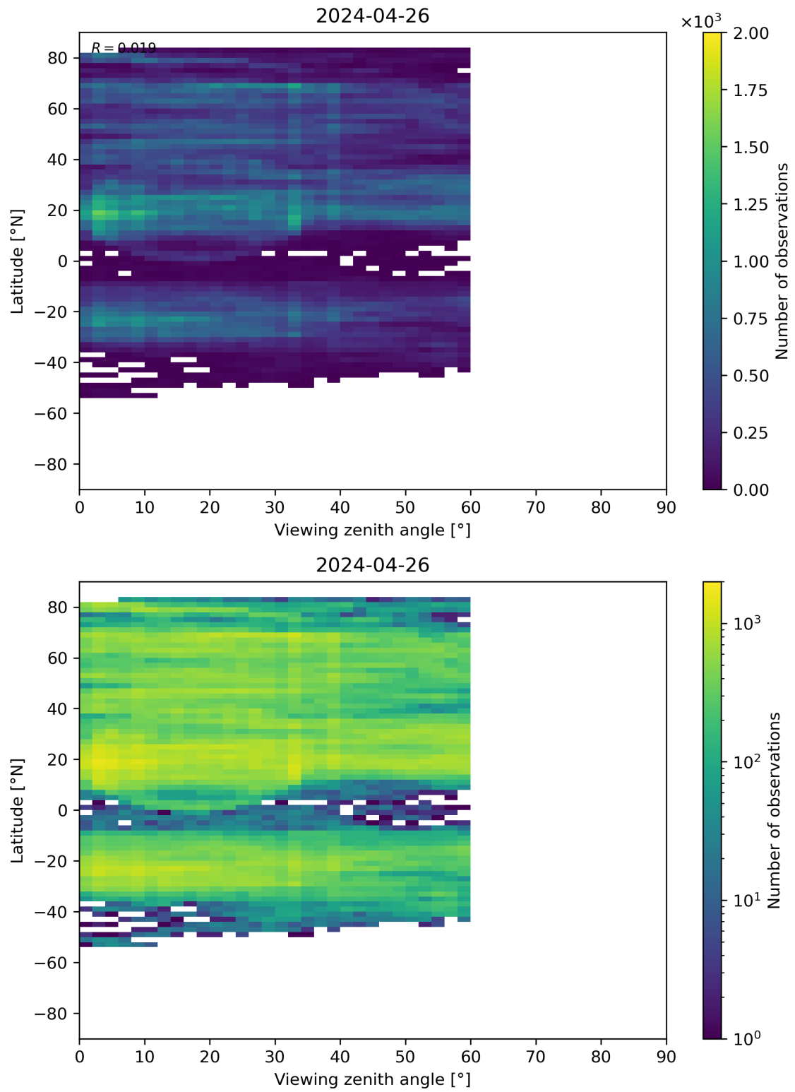
Figure 109: Scatter density plot of “Viewing zenith angle” against “Latitude” for 2024-04-26 to 2024-04-27.
