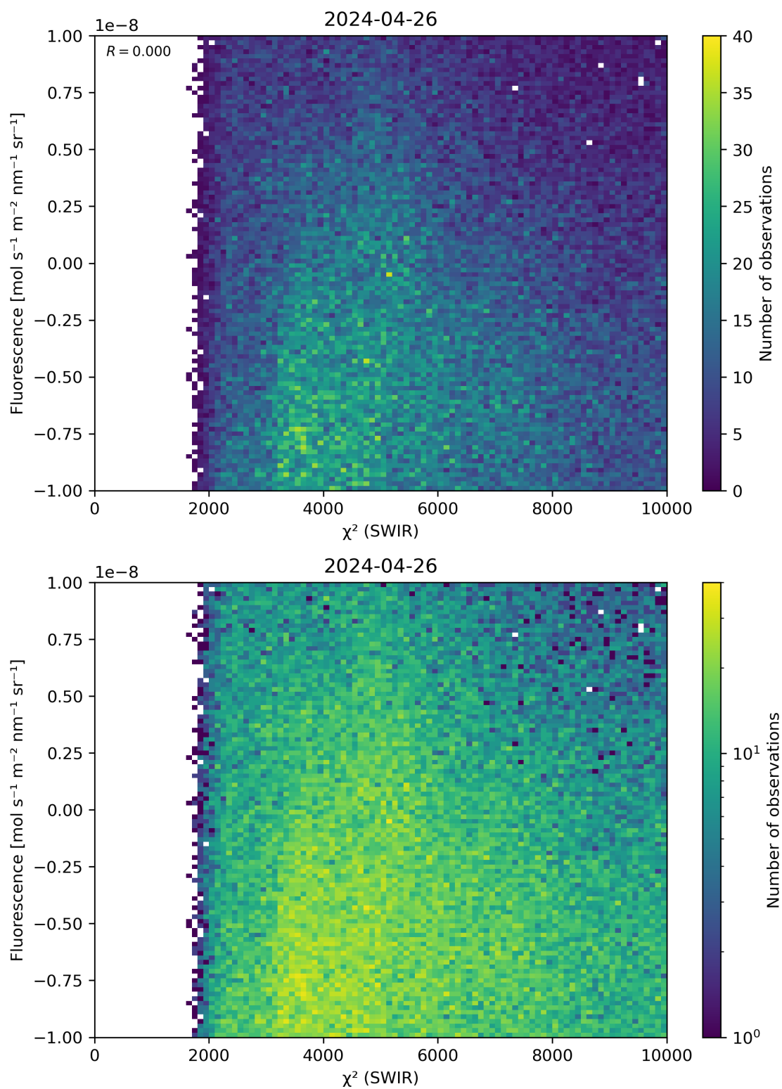
Figure 49: Scatter density plot of “ \chi^2 (SWIR)” against “Fluorescence” for 2024-04-26 to 2024-04-27.
