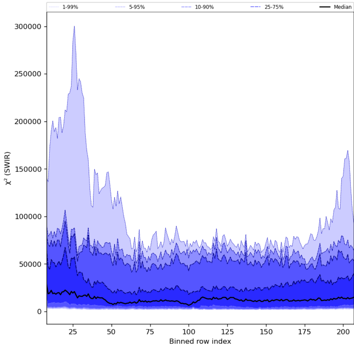
Figure 39: Along track statistics of “ \chi^2 (SWIR)” for 2024-04-26 to 2024-04-27
