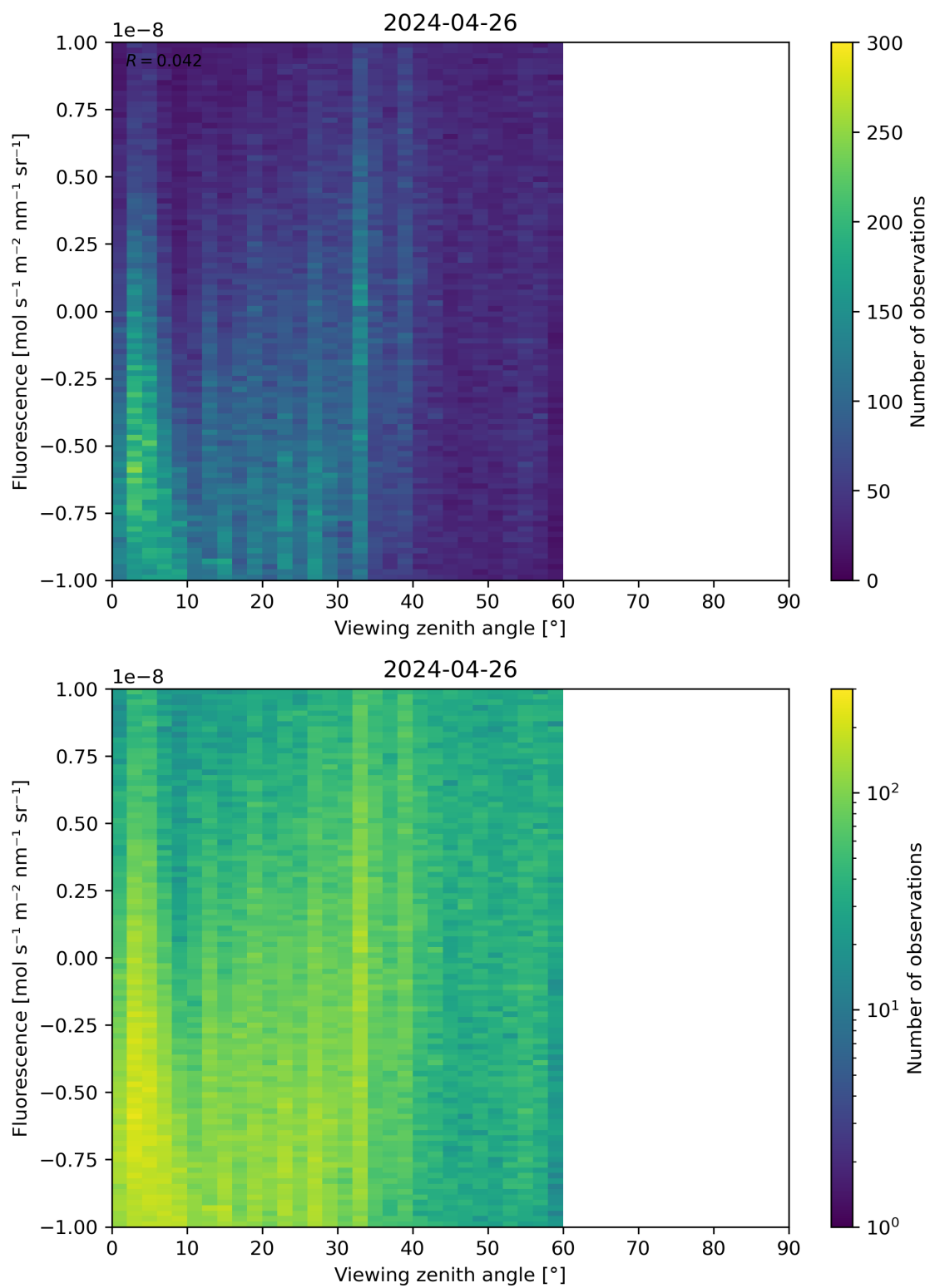
Figure 108: Scatter density plot of “Viewing zenith angle” against “Fluorescence” for 2024-04-26 to 2024-04-27.
