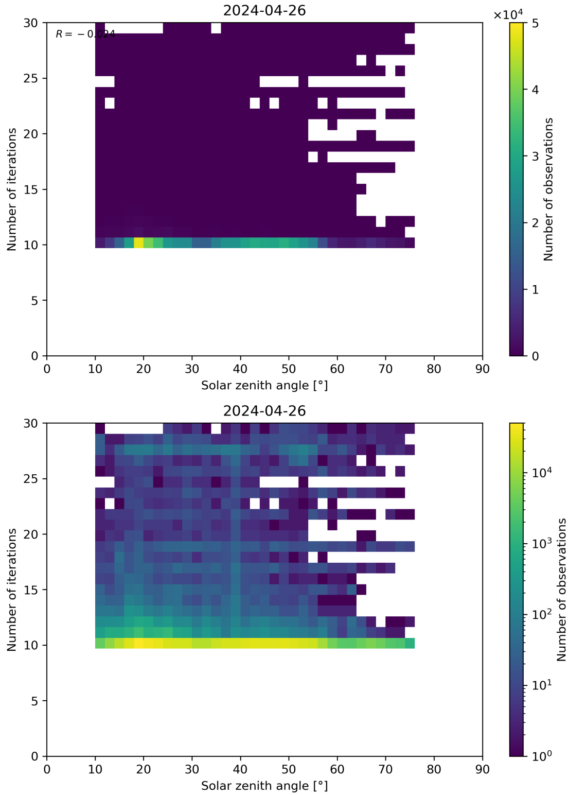
Figure 102: Scatter density plot of “Solar zenith angle” against “Number of iterations” for 2024-04-26 to 2024-04-27.
