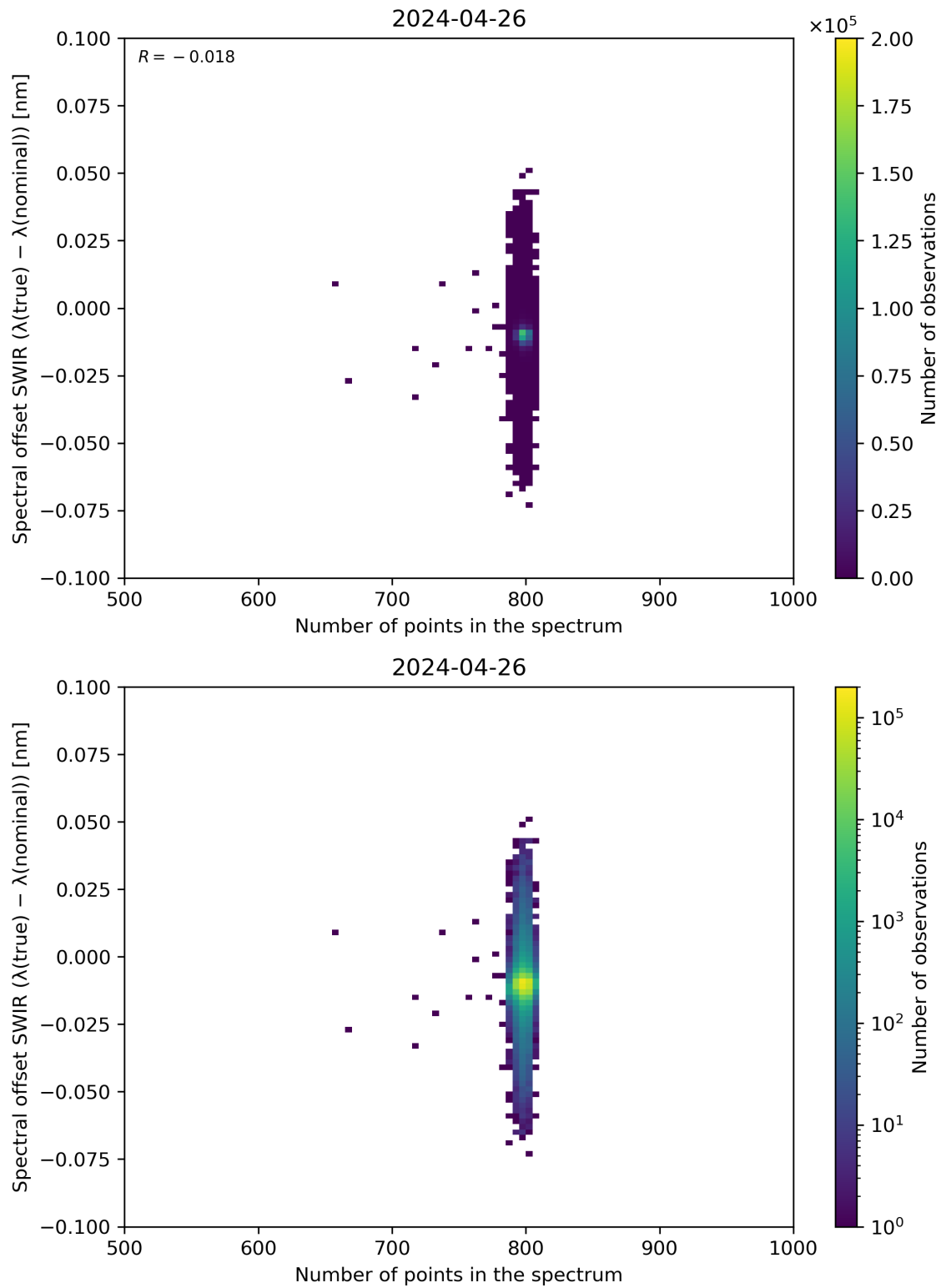
Figure 93: Scatter density plot of “Number of points in the spectrum” against “Spectral offset SWIR ( \lambda(\text{true}) - \lambda(\text{nominal}) )” for 2024-04-26 to 2024-04-27.
