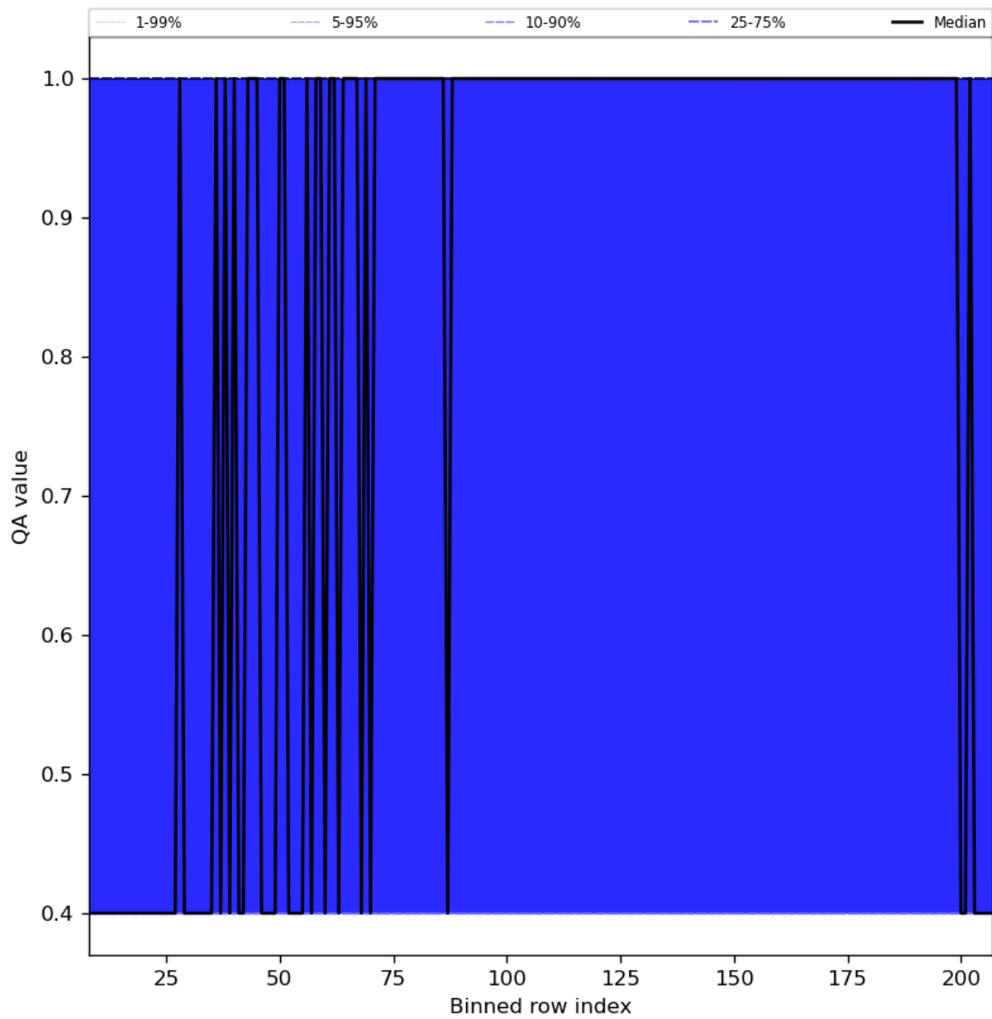
Figure 33: Along track statistics of “QA value” for 2024-04-26 to 2024-04-27
