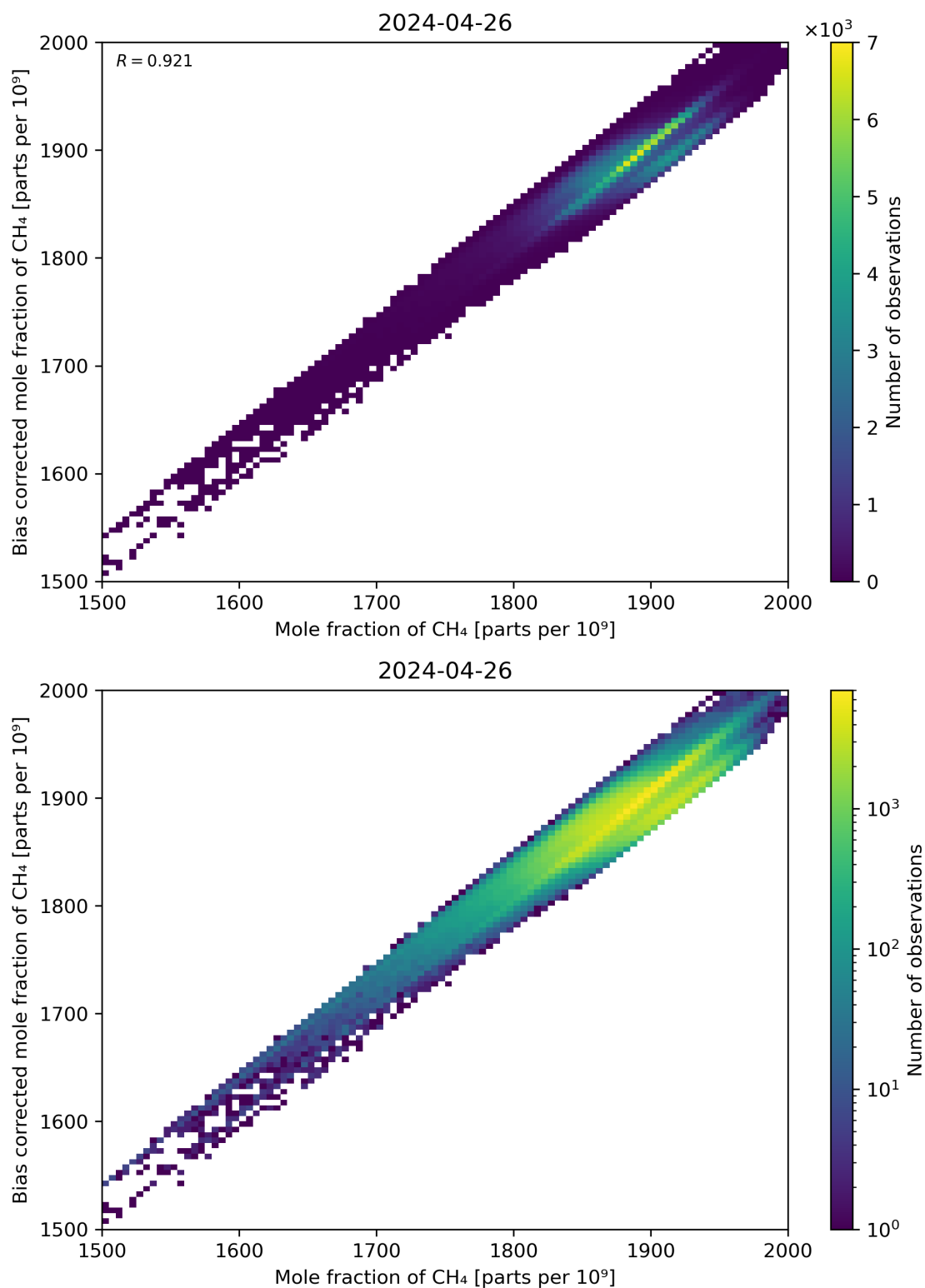
Figure 74: Scatter density plot of “Mole fraction of CH 4 ” against “Bias corrected mole fraction of CH 4 ” for 2024-04-26 to 2024-04-27.
