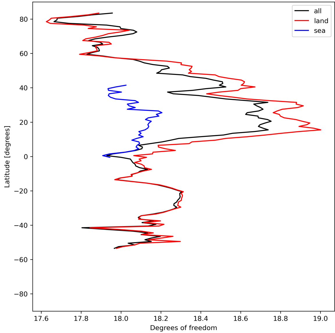
Figure 19: Zonal average of “Degrees of freedom” for 2024-04-26 to 2024-04-27.
