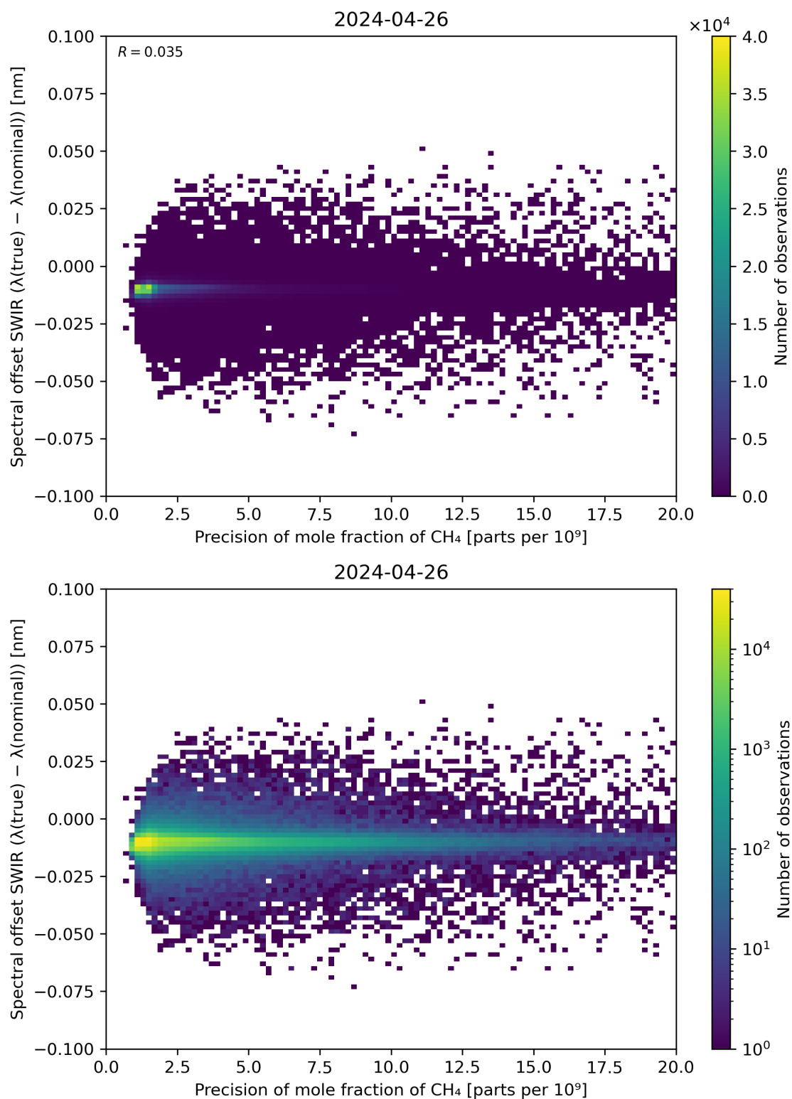
Figure 85: Scatter density plot of “Precision of mole fraction of \text{CH}_4 ” against “Spectral offset SWIR ( \lambda(\text{true}) - \lambda(\text{nominal}) )” for 2024-04-26 to 2024-04-27.
