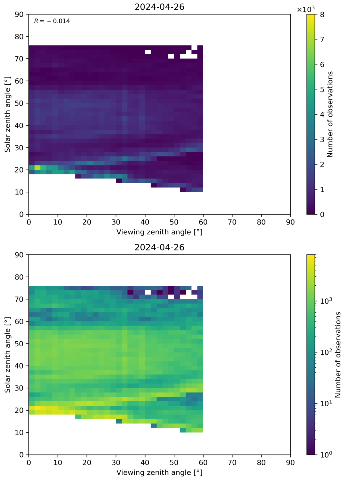
Figure 115: Scatter density plot of “Viewing zenith angle” against “Solar zenith angle” for 2024-04-26 to 2024-04-27.
