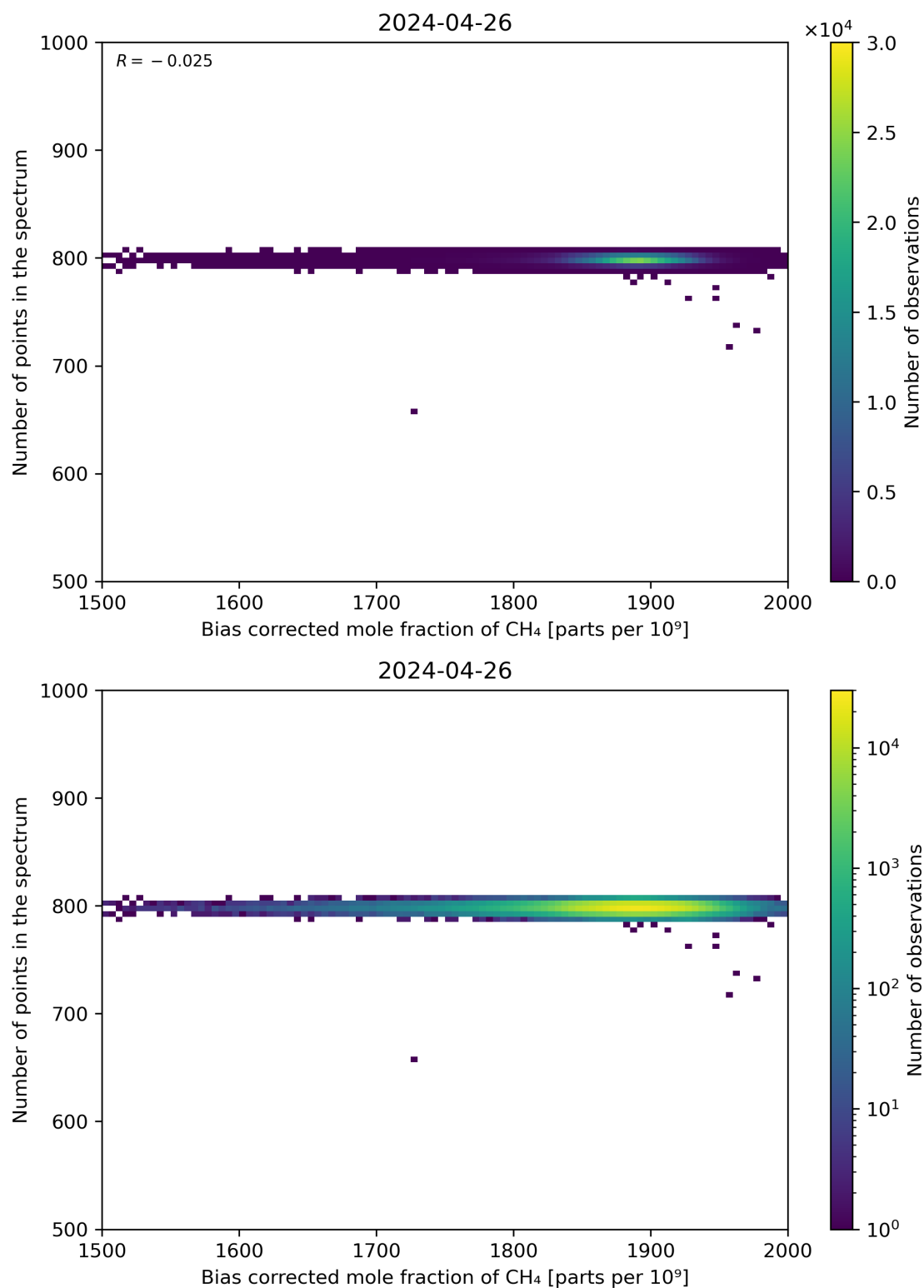
Figure 68: Scatter density plot of “Bias corrected mole fraction of CH 4 ” against “Number of points in the spectrum” for 2024-04-26 to 2024-04-27.
