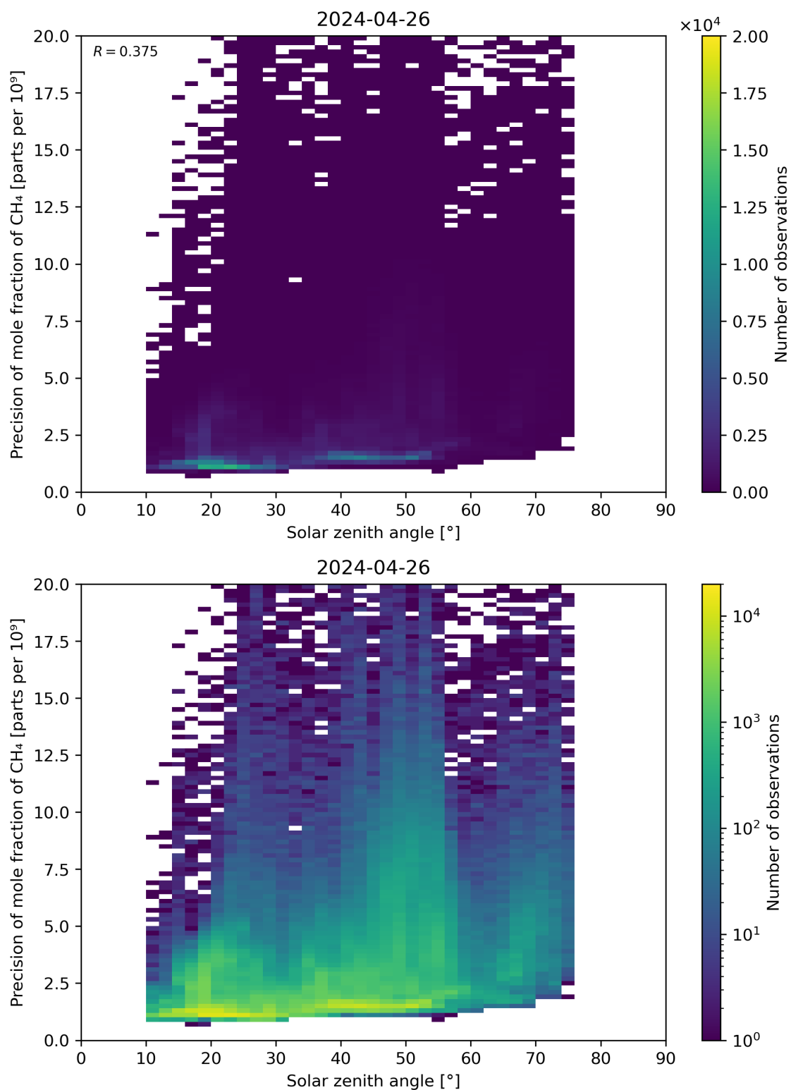
Figure 101: Scatter density plot of “Solar zenith angle” against “Precision of mole fraction of CH 4 ” for 2024-04-26 to 2024-04-27.
