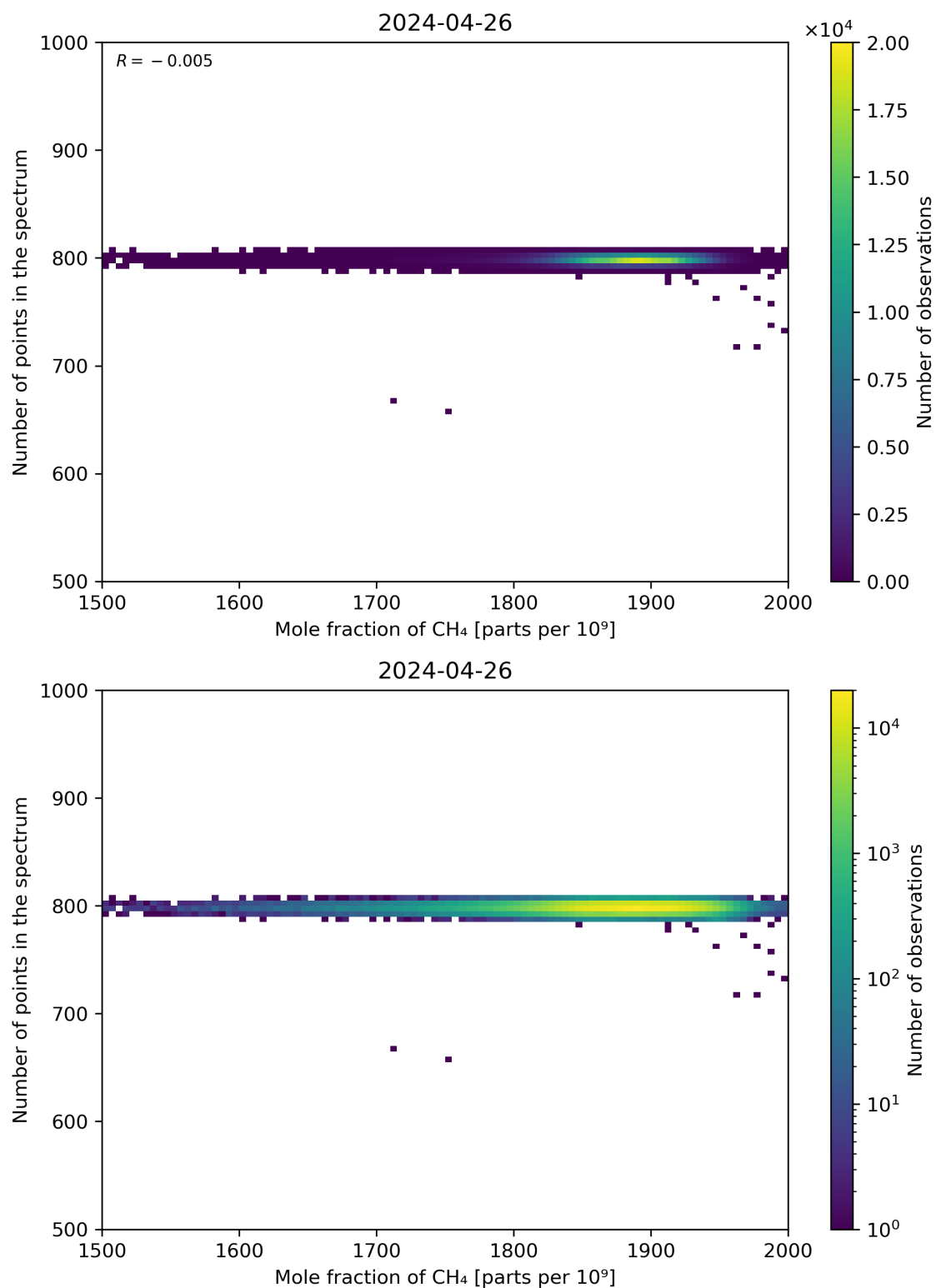
Figure 77: Scatter density plot of “Mole fraction of CH 4 ” against “Number of points in the spectrum” for 2024-04-26 to 2024-04-27.
