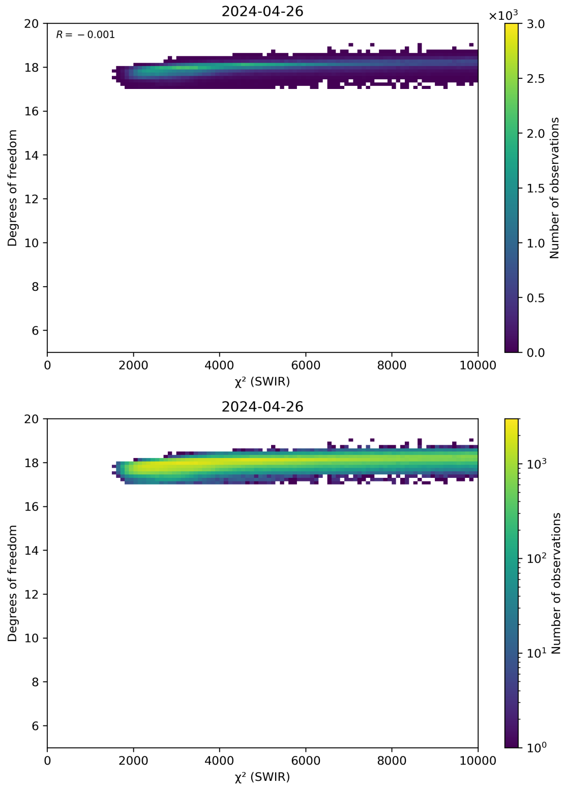
Figure 48: Scatter density plot of “ \chi^2 (SWIR)” against “Degrees of freedom” for 2024-04-26 to 2024-04-27.
