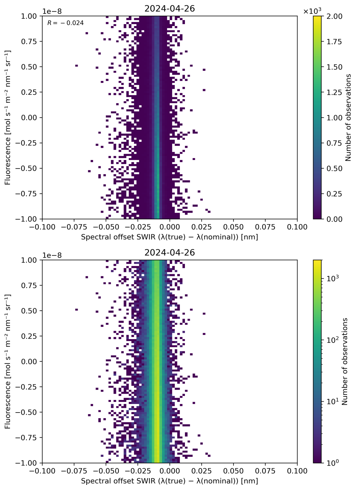
Figure 120: Scatter density plot of “Spectral offset SWIR ( \lambda(\text{true}) - \lambda(\text{nominal}) )” against “Fluorescence” for 2024-04-26 to 2024-04-27.
