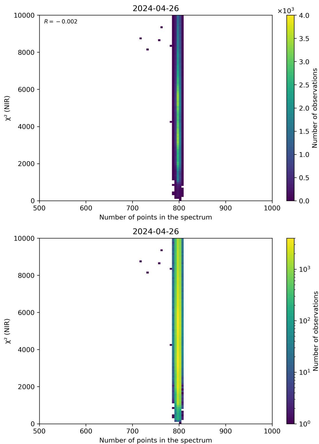
Figure 88: Scatter density plot of “Number of points in the spectrum” against “ \chi^2 (NIR)” for 2024-04-26 to 2024-04-27.
