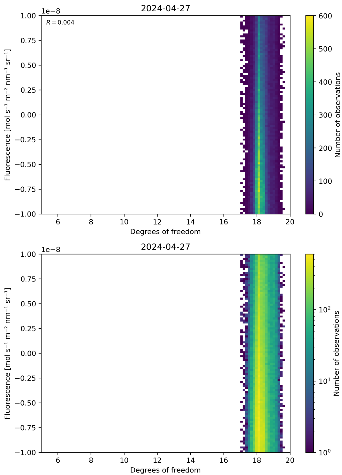
Figure 51: Scatter density plot of “Degrees of freedom” against “Fluorescence” for 2024-04-26 to 2024-04-28.
