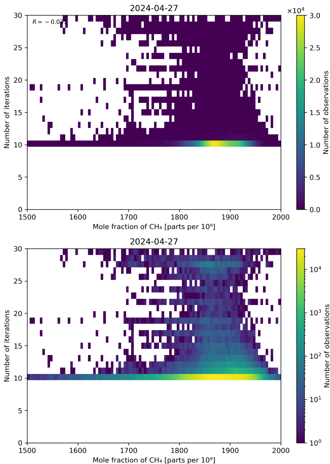
Figure 76: Scatter density plot of “Mole fraction of CH 4 ” against “Number of iterations” for 2024-04-26 to 2024-04-28.
