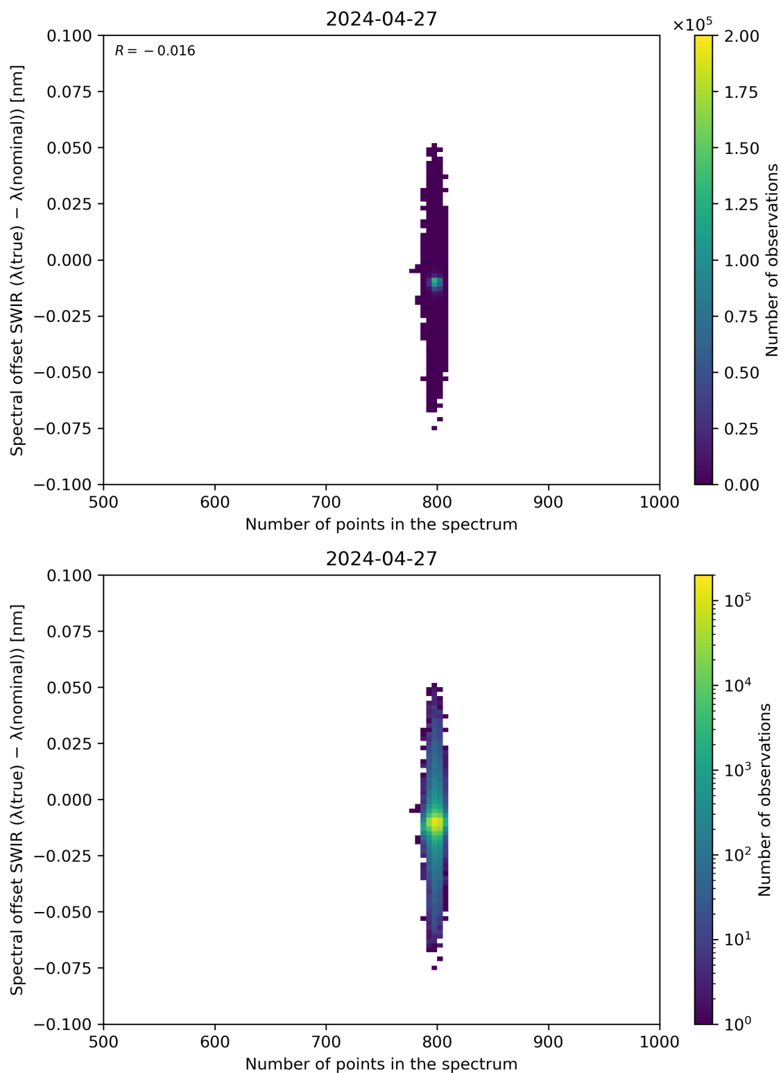
Figure 93: Scatter density plot of “Number of points in the spectrum” against “Spectral offset SWIR ( \lambda(\text{true}) - \lambda(\text{nominal}) )” for 2024-04-26 to 2024-04-28.
