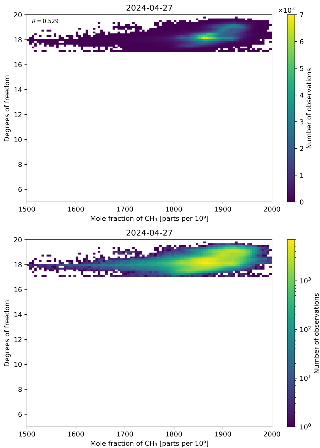
Figure 72: Scatter density plot of “Mole fraction of CH 4 ” against “Degrees of freedom” for 2024-04-26 to 2024-04-28.
