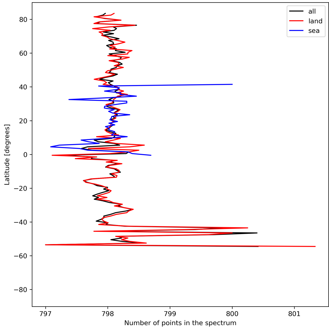
Figure 15: Zonal average of “Number of points in the spectrum” for 2024-04-26 to 2024-04-28.
