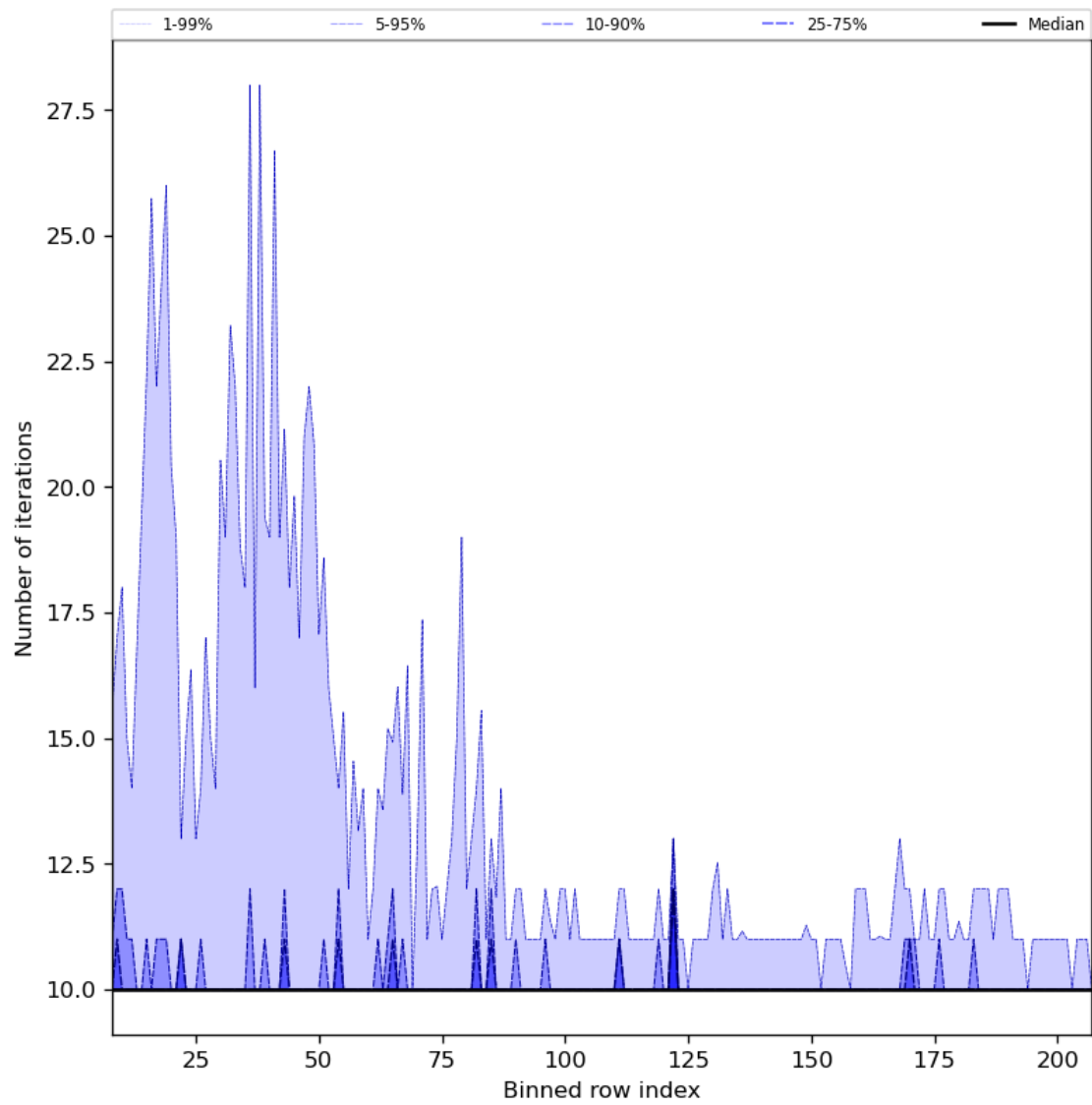
Figure 42: Along track statistics of “Number of iterations” for 2024-04-26 to 2024-04-28
