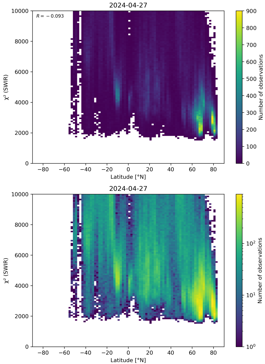
Figure 54: Scatter density plot of “Latitude” against “ \chi^2 (SWIR)” for 2024-04-26 to 2024-04-28.
