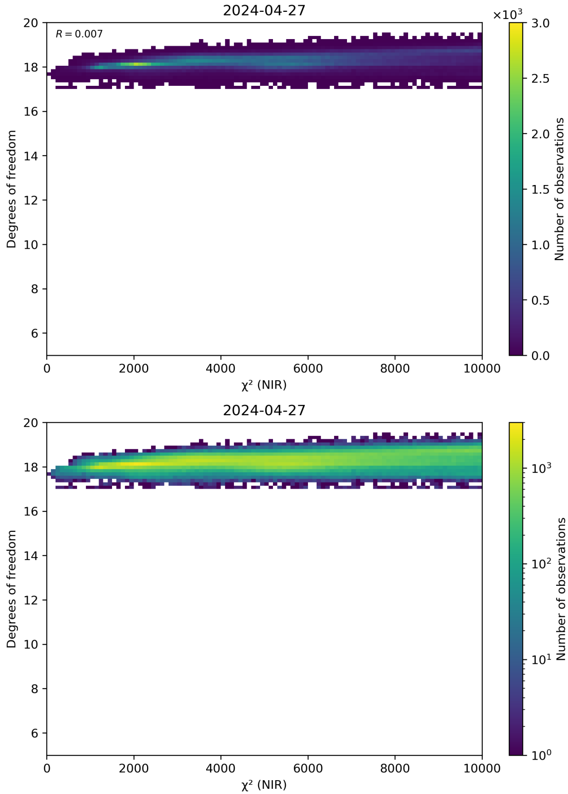
Figure 44: Scatter density plot of “ \chi^2 (NIR)” against “Degrees of freedom” for 2024-04-26 to 2024-04-28.
