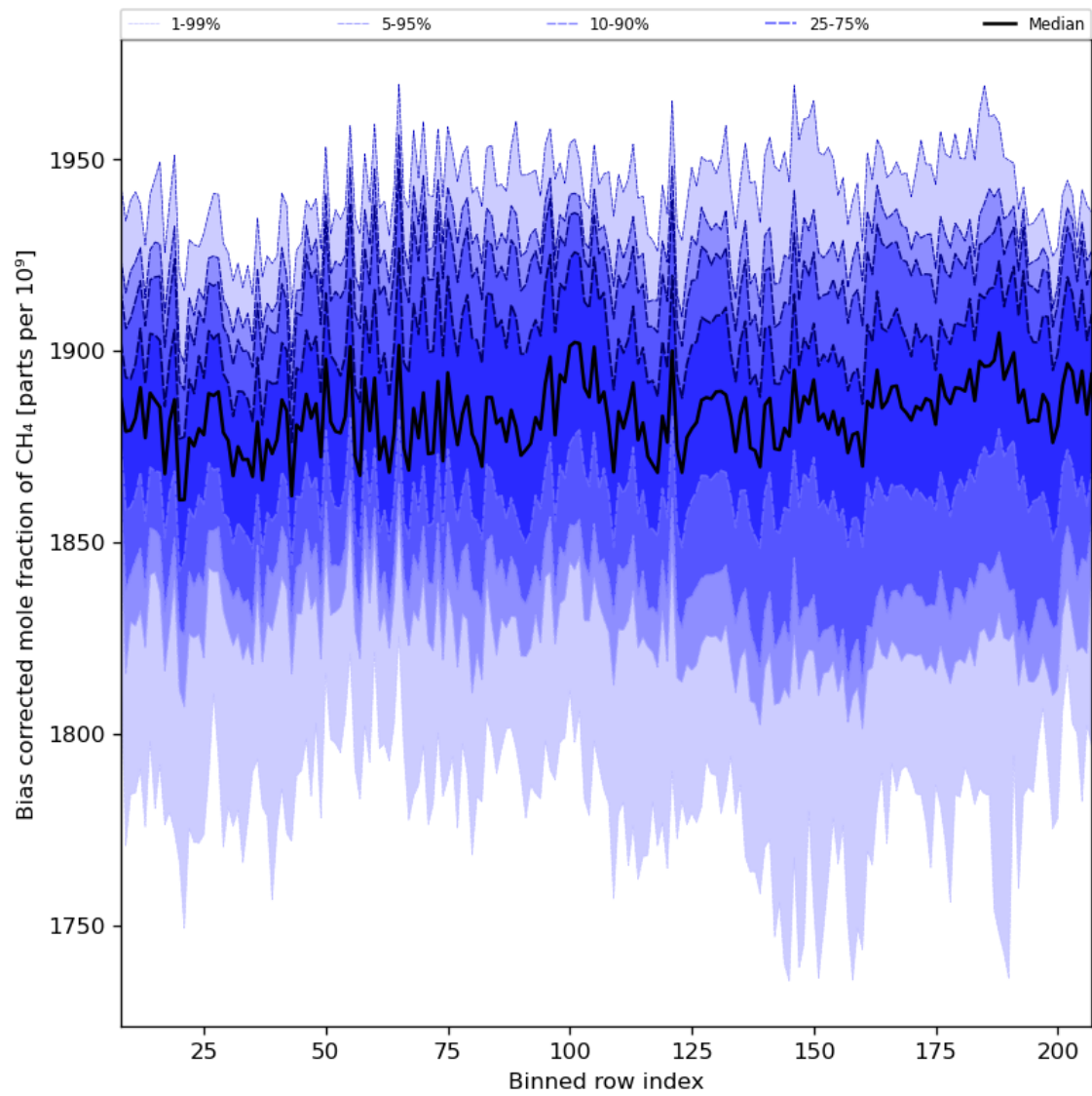
Figure 36: Along track statistics of “Bias corrected mole fraction of CH 4 ” for 2024-04-26 to 2024-04-28
