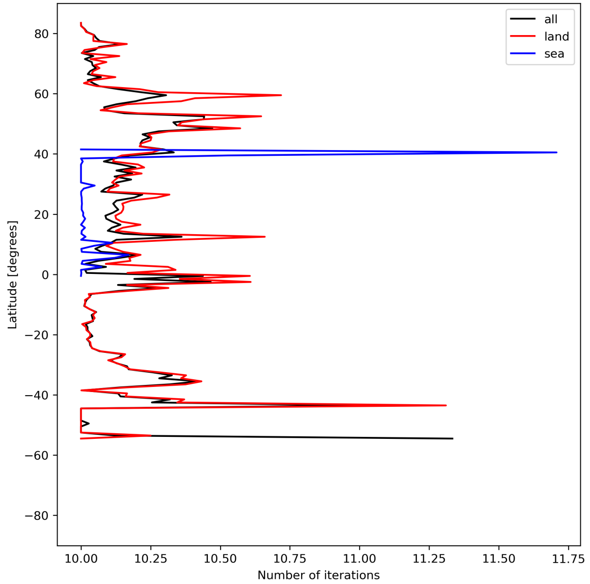
Figure 20: Zonal average of “Number of iterations” for 2024-04-26 to 2024-04-28.
