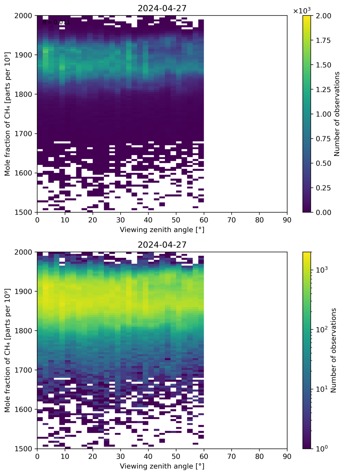
Figure 110: Scatter density plot of “Viewing zenith angle” against “Mole fraction of CH 4 ” for 2024-04-26 to 2024-04-28.
