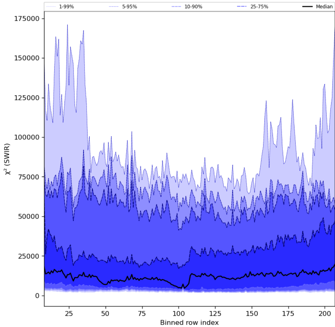
Figure 39: Along track statistics of “ \chi^2 (SWIR)” for 2024-04-26 to 2024-04-28
