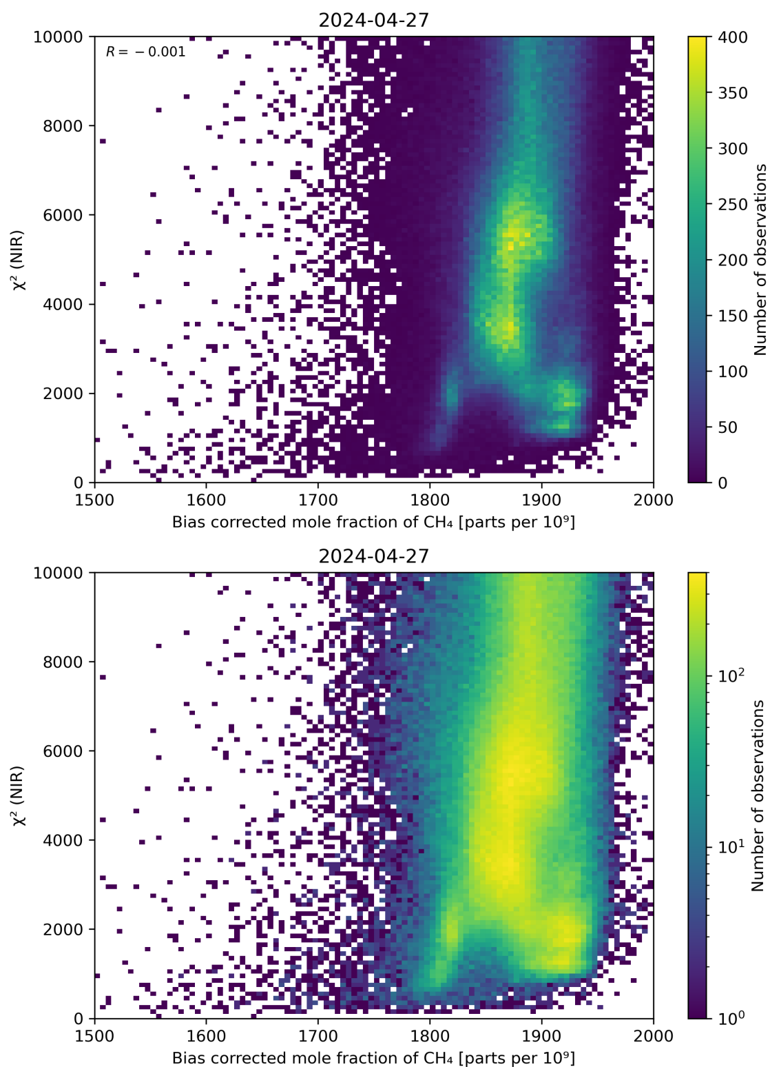
Figure 63: Scatter density plot of “Bias corrected mole fraction of CH 4 ” against “ \chi^2 (NIR)” for 2024-04-26 to 2024-04-28.
