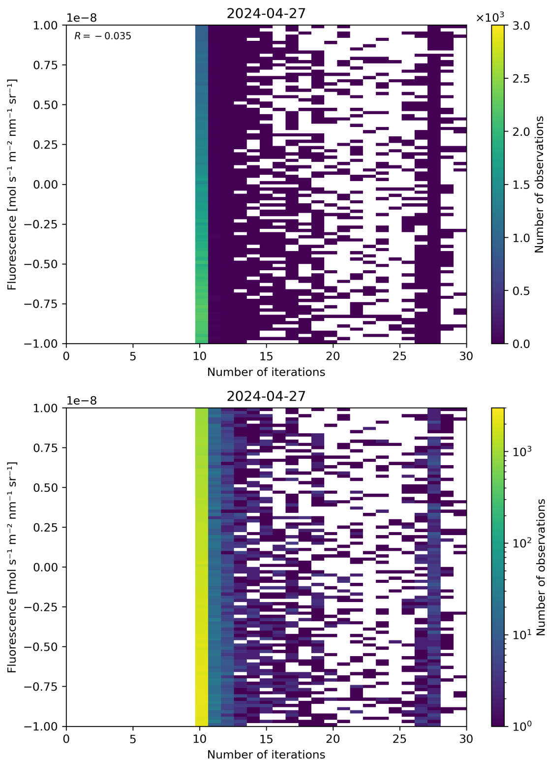
Figure 87: Scatter density plot of “Number of iterations” against “Fluorescence” for 2024-04-26 to 2024-04-28.
