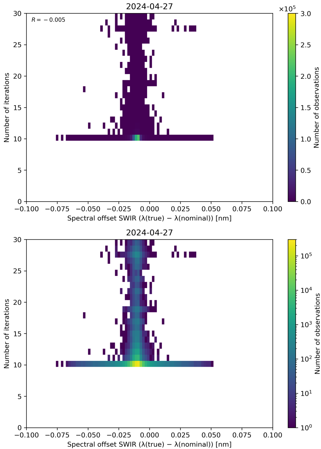
Figure 121: Scatter density plot of “Spectral offset SWIR ( \lambda(\text{true}) - \lambda(\text{nominal}) )” against “Number of iterations” for 2024-04-26 to 2024-04-28.
