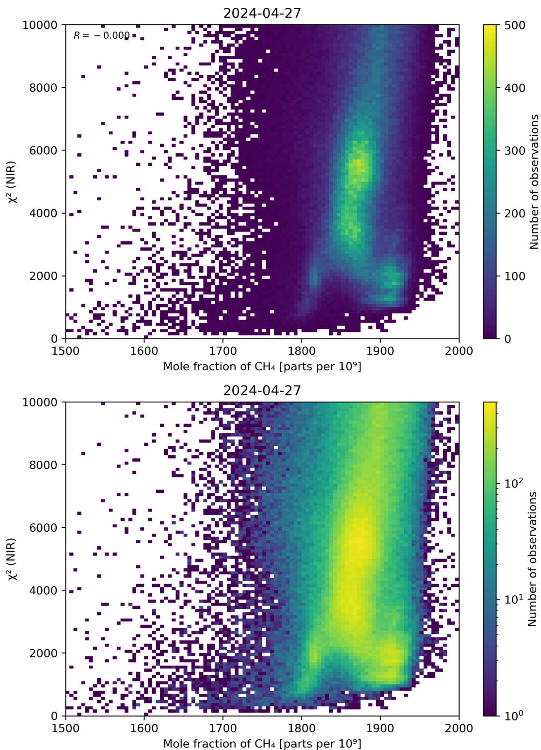
Figure 70: Scatter density plot of “Mole fraction of CH 4 ” against “ \chi^2 (NIR)” for 2024-04-26 to 2024-04-28.
