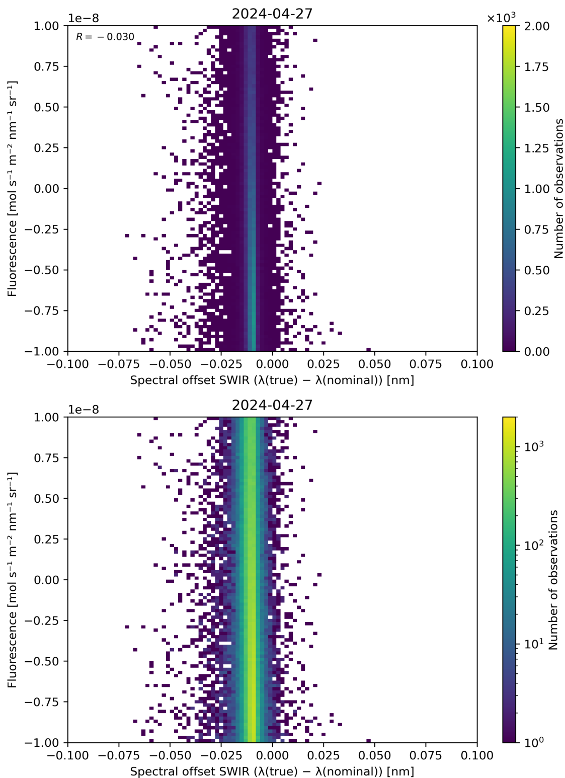
Figure 120: Scatter density plot of “Spectral offset SWIR ( \lambda(\text{true}) - \lambda(\text{nominal}) )” against “Fluorescence” for 2024-04-26 to 2024-04-28.
