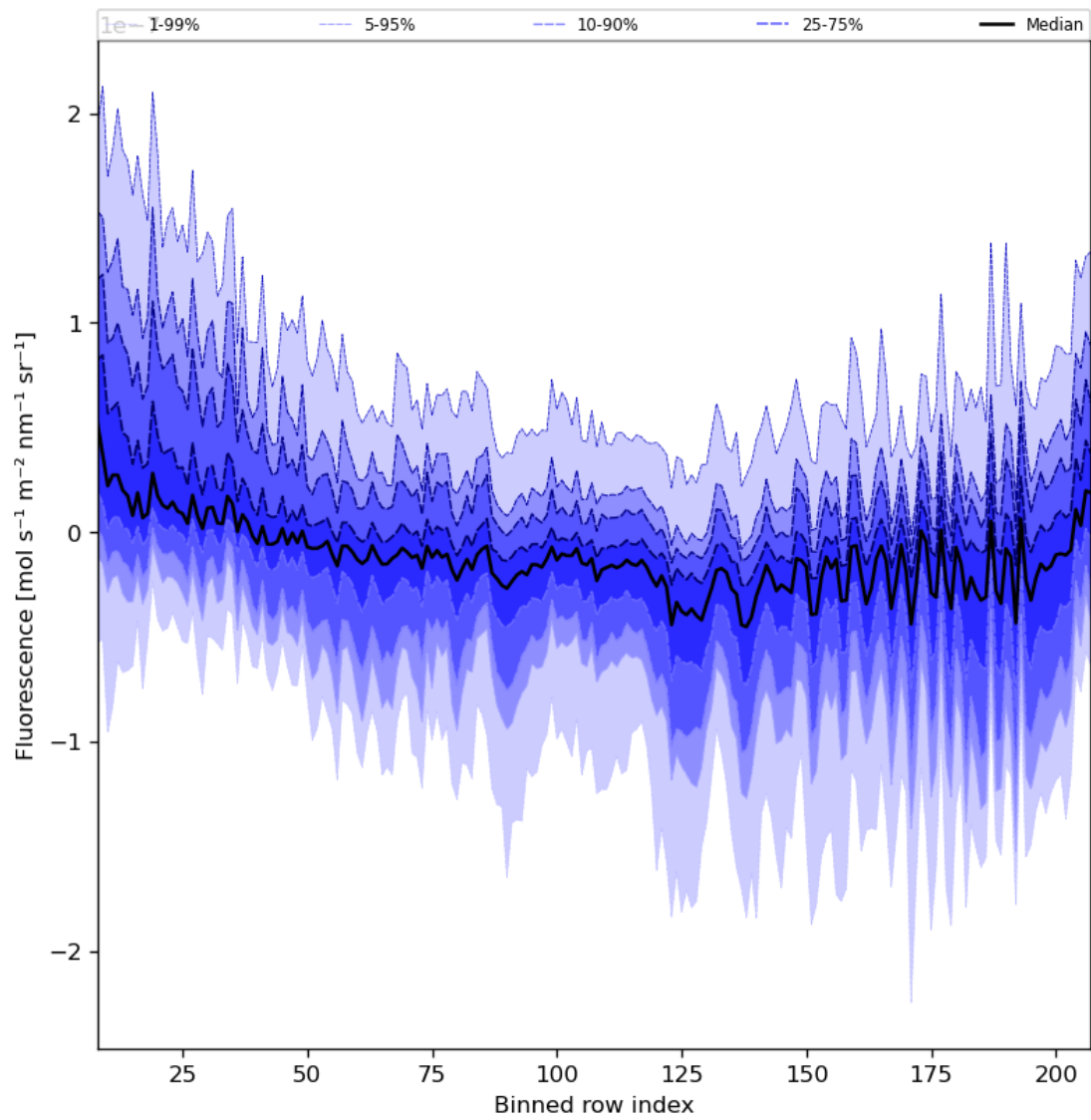
Figure 43: Along track statistics of "Fluorescence" for 2024-04-26 to 2024-04-28
