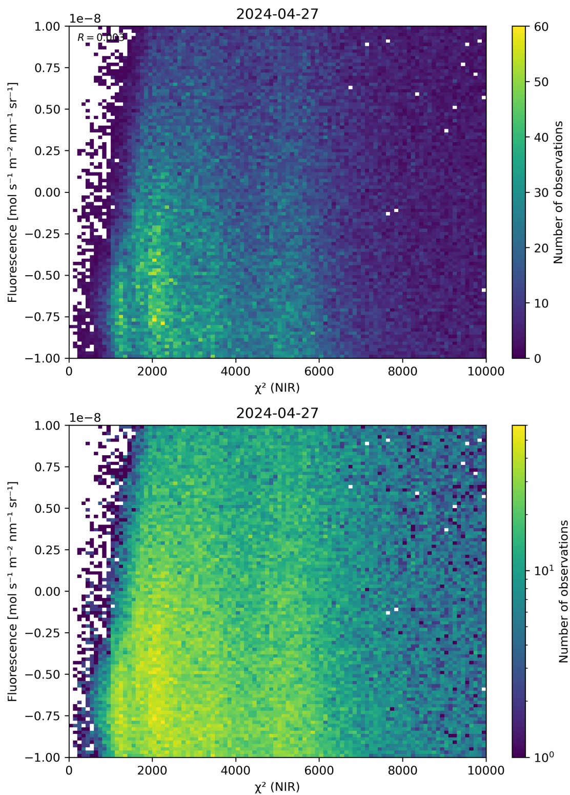
Figure 45: Scatter density plot of “ \chi^2 (NIR)” against “Fluorescence” for 2024-04-26 to 2024-04-28.
