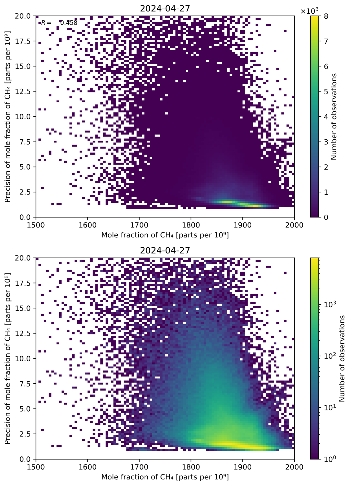
Figure 75: Scatter density plot of “Mole fraction of CH 4 ” against “Precision of mole fraction of CH 4 ” for 2024-04-26 to 2024-04-28.
