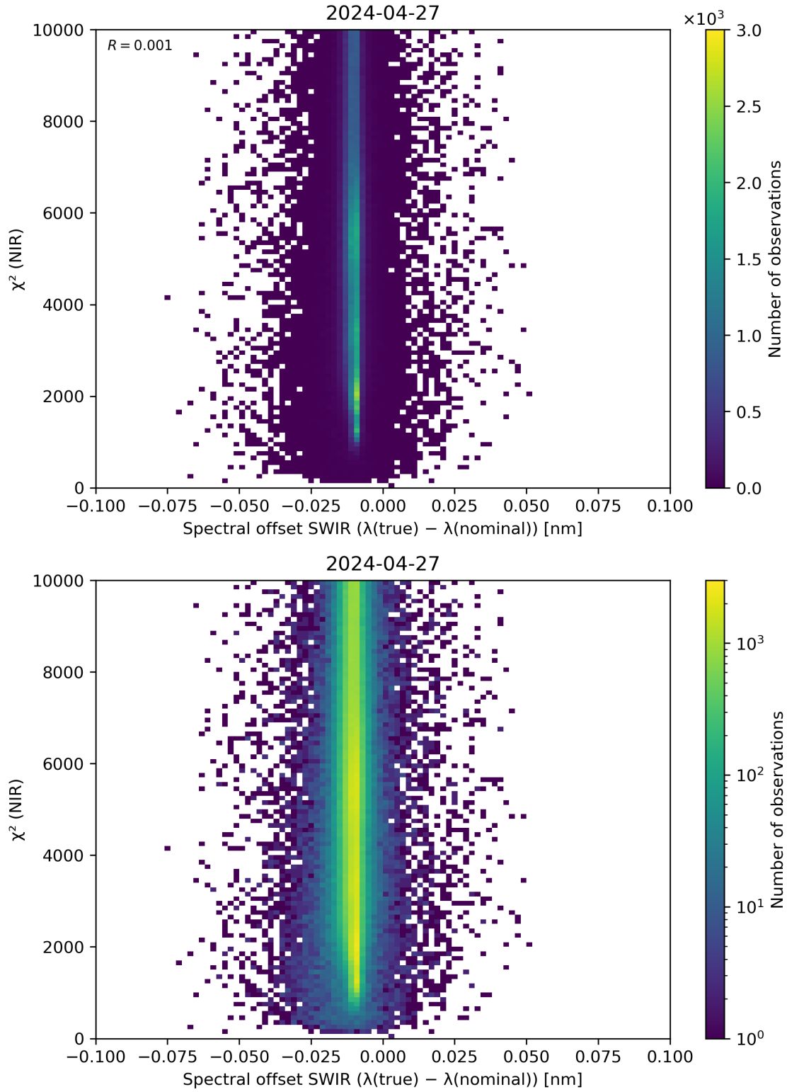
Figure 117: Scatter density plot of “Spectral offset SWIR ( \lambda(\text{true}) - \lambda(\text{nominal}) )” against “ \chi^2 (NIR)” for 2024-04-26 to 2024-04-28.
