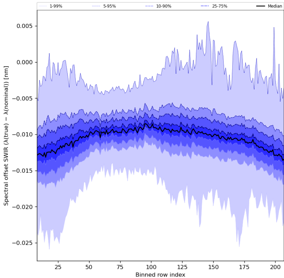
Figure 38: Along track statistics of “Spectral offset SWIR ( \lambda(\text{true}) - \lambda(\text{nominal}) )” for 2024-04-26 to 2024-04-28
