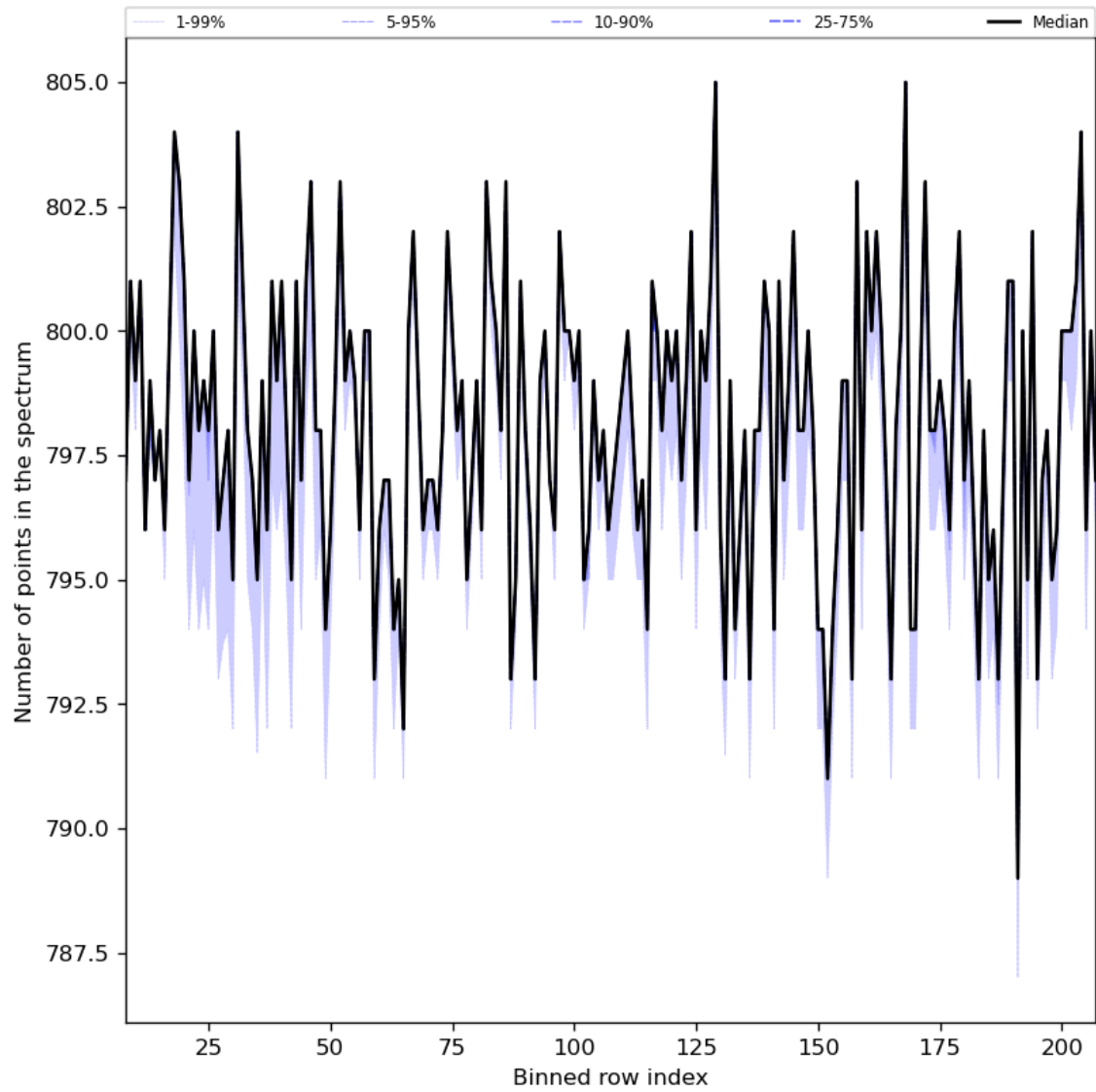
Figure 37: Along track statistics of “Number of points in the spectrum” for 2024-04-26 to 2024-04-28
