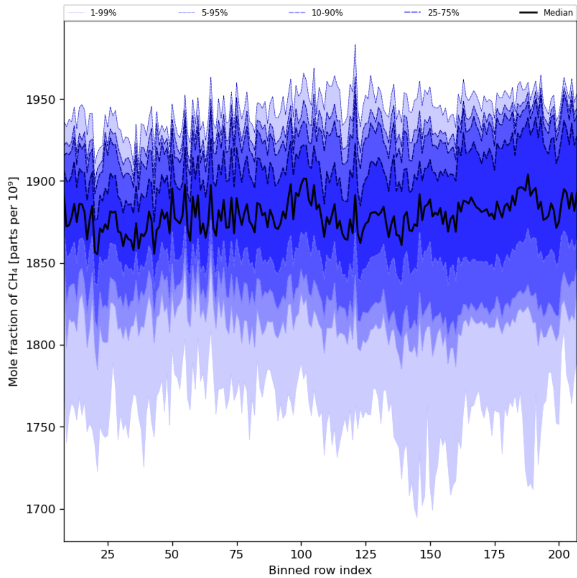
Figure 34: Along track statistics of “Mole fraction of CH 4 ” for 2024-04-26 to 2024-04-28
