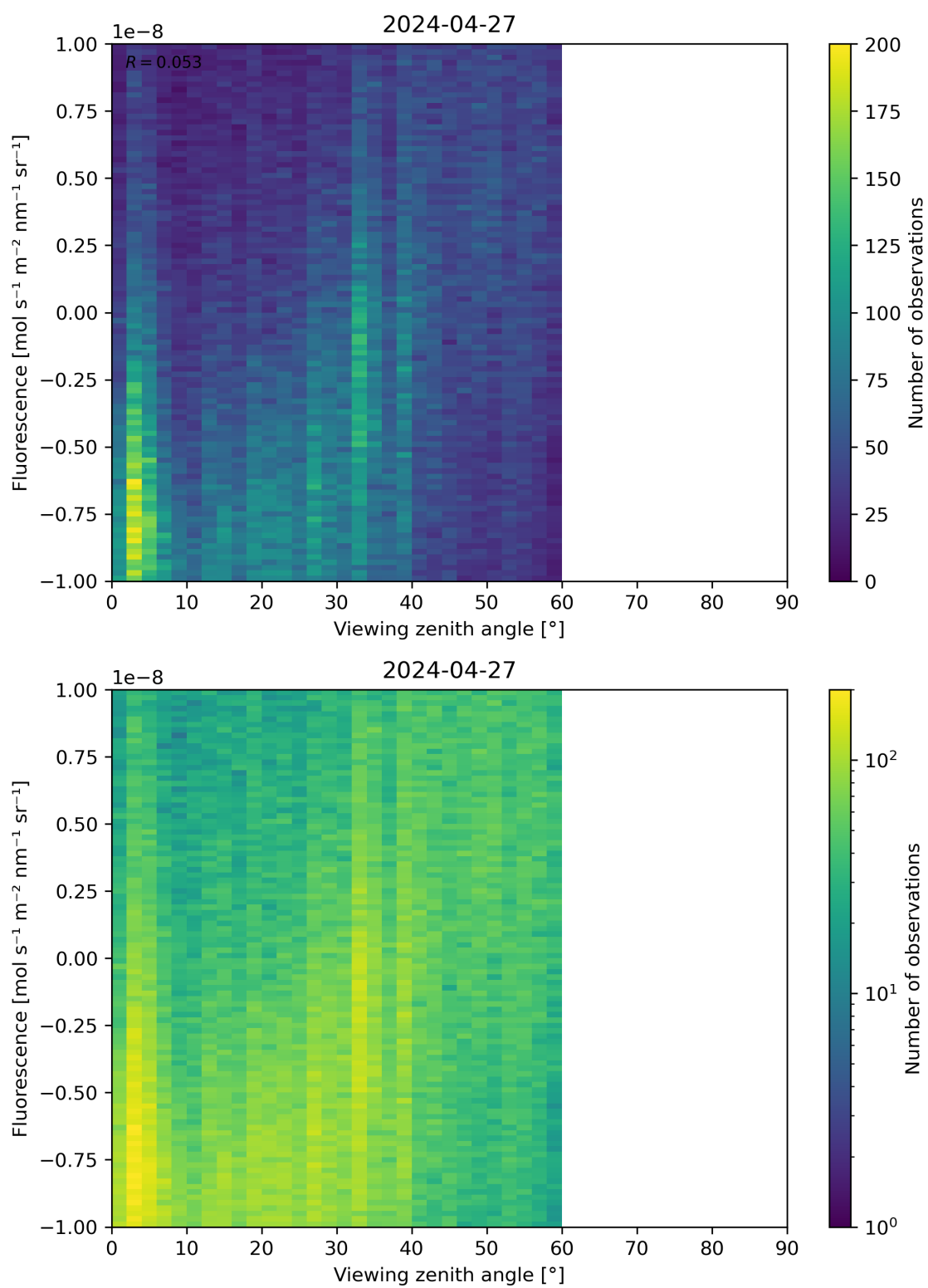
Figure 108: Scatter density plot of “Viewing zenith angle” against “Fluorescence” for 2024-04-26 to 2024-04-28.
