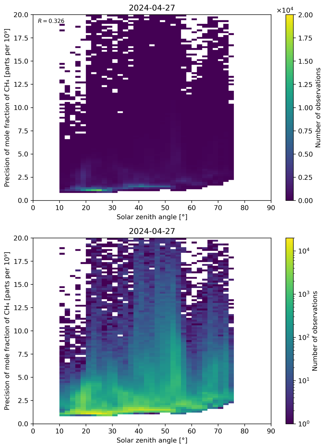
Figure 101: Scatter density plot of “Solar zenith angle” against “Precision of mole fraction of \text{CH}_4 ” for 2024-04-26 to 2024-04-28.
