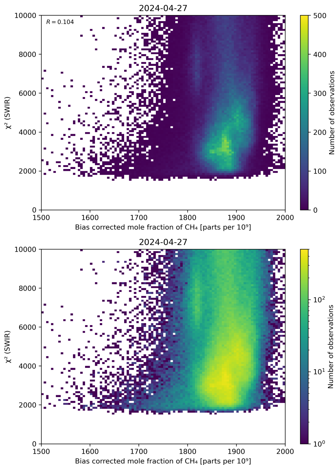
Figure 64: Scatter density plot of “Bias corrected mole fraction of \text{CH}_4 ” against “ \chi^2 (SWIR)” for 2024-04-26 to 2024-04-28.
