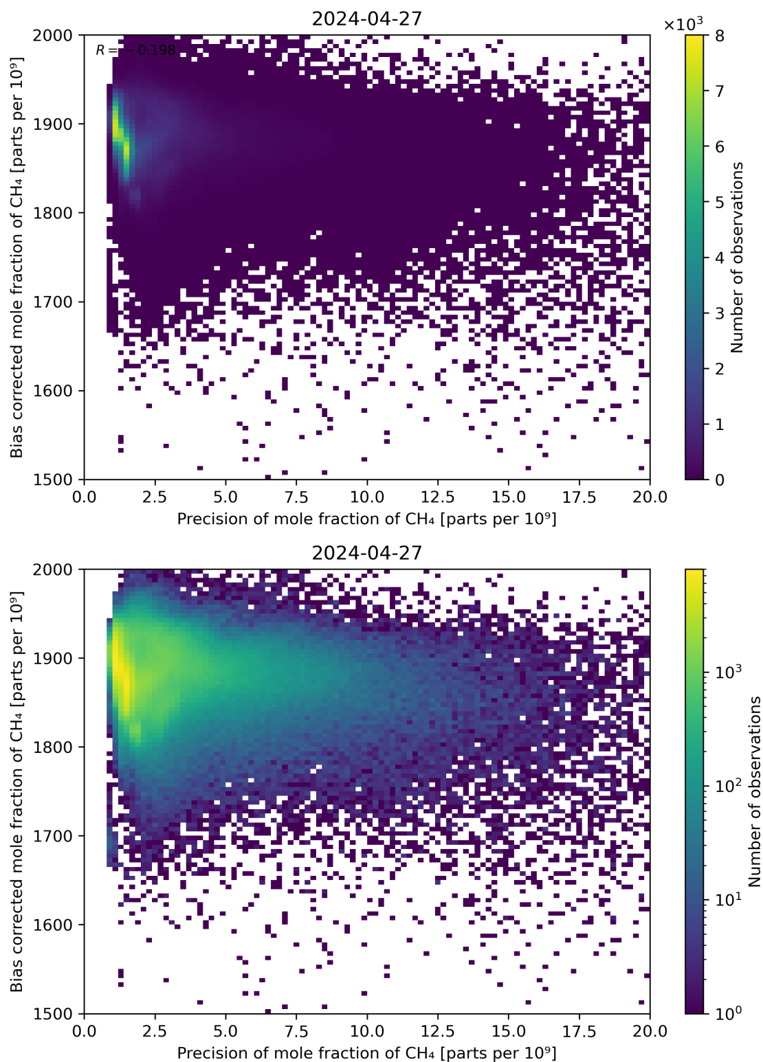
Figure 82: Scatter density plot of “Precision of mole fraction of CH 4 ” against “Bias corrected mole fraction of CH 4 ” for 2024-04-26 to 2024-04-28.
