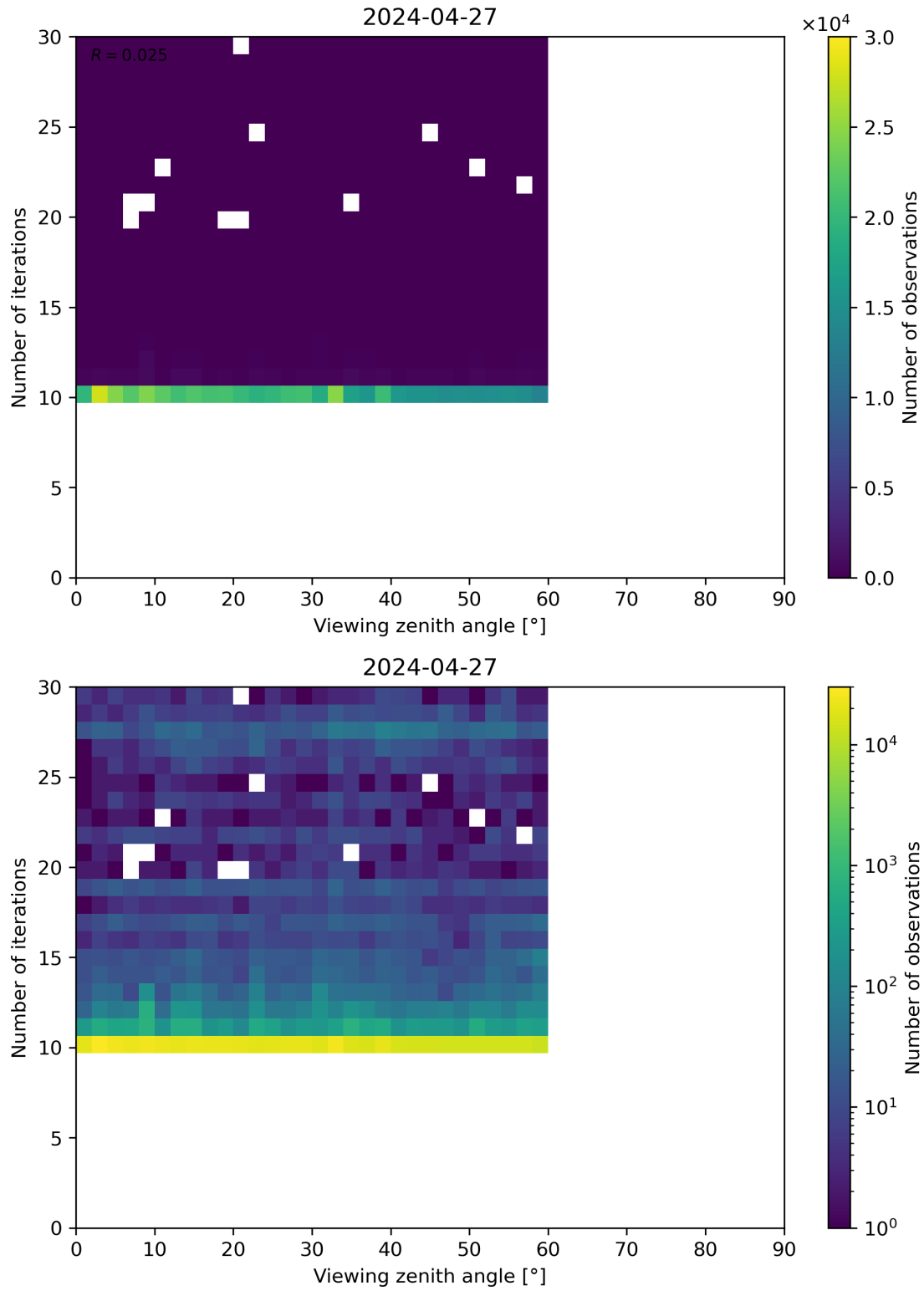
Figure 113: Scatter density plot of “Viewing zenith angle” against “Number of iterations” for 2024-04-26 to 2024-04-28.
