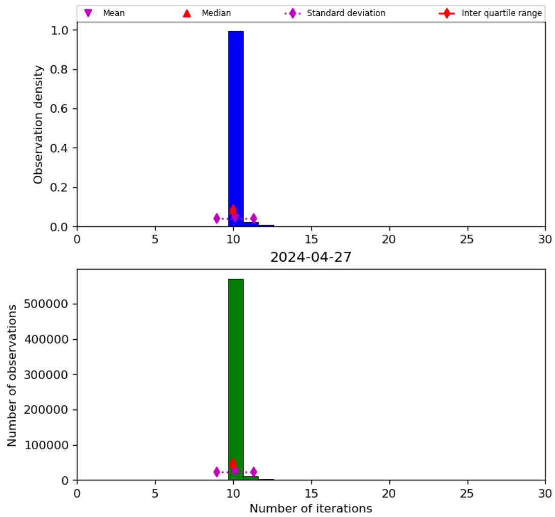
Figure 31: Histogram of “Number of iterations” for 2024-04-26 to 2024-04-28
