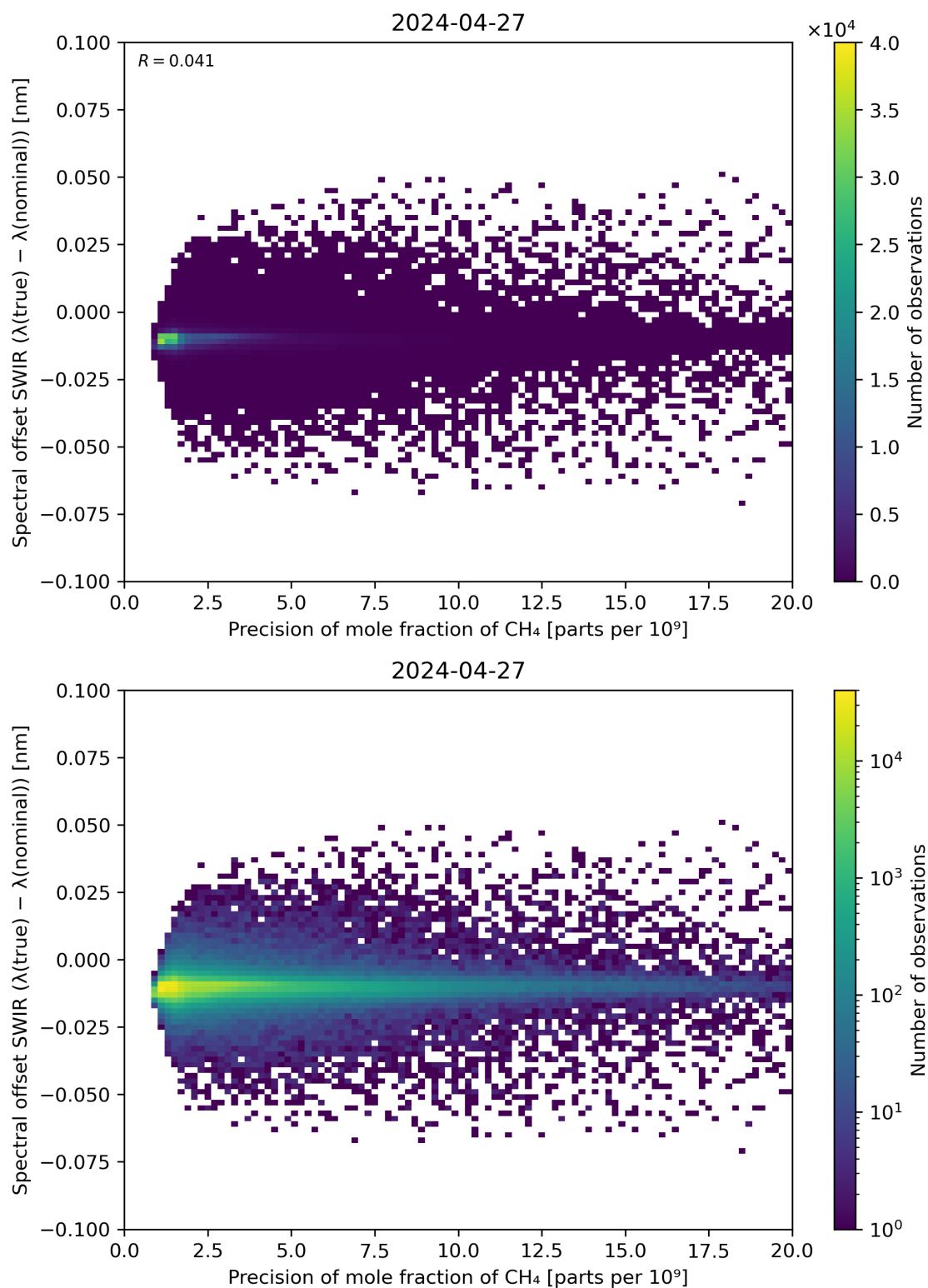
Figure 85: Scatter density plot of “Precision of mole fraction of CH 4 ” against “Spectral offset SWIR ( \lambda(\text{true}) - \lambda(\text{nominal}) )” for 2024-04-26 to 2024-04-28.
