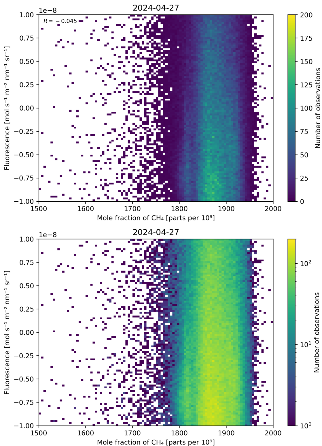
Figure 73: Scatter density plot of “Mole fraction of \text{CH}_4 ” against “Fluorescence” for 2024-04-26 to 2024-04-28.
