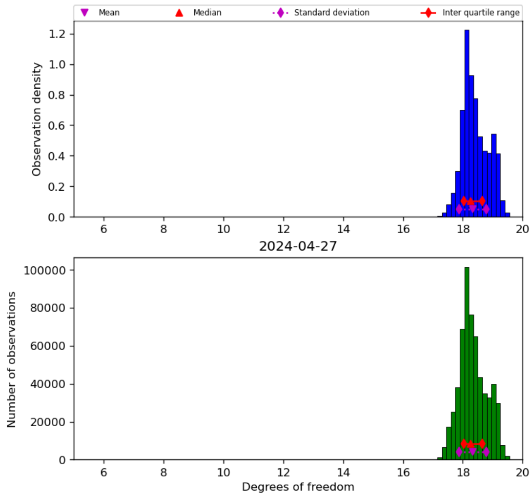
Figure 30: Histogram of “Degrees of freedom” for 2024-04-26 to 2024-04-28
