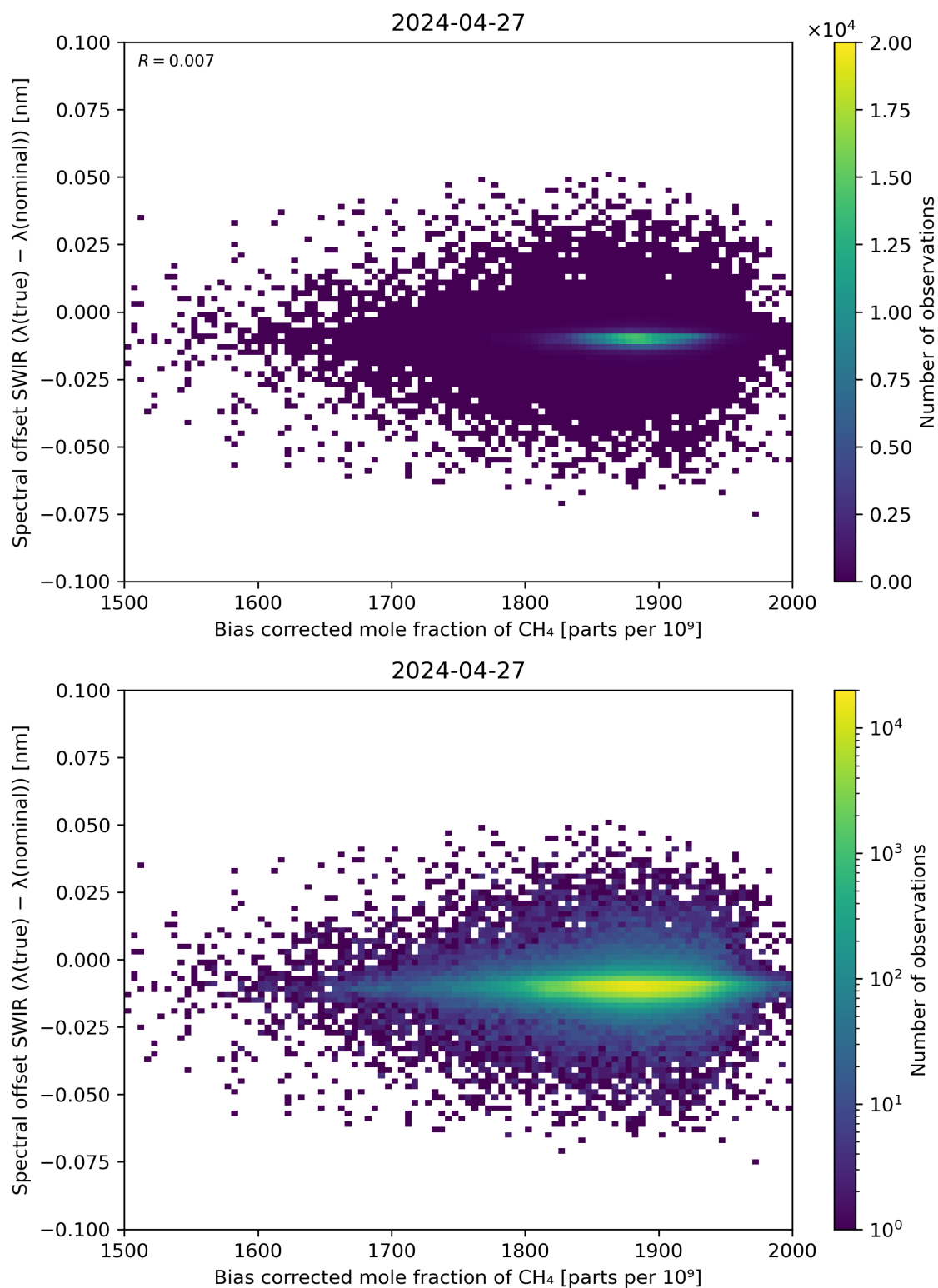
Figure 69: Scatter density plot of “Bias corrected mole fraction of \text{CH}_4 ” against “Spectral offset SWIR ( \lambda(\text{true}) - \lambda(\text{nominal}) )” for 2024-04-26 to 2024-04-28.
