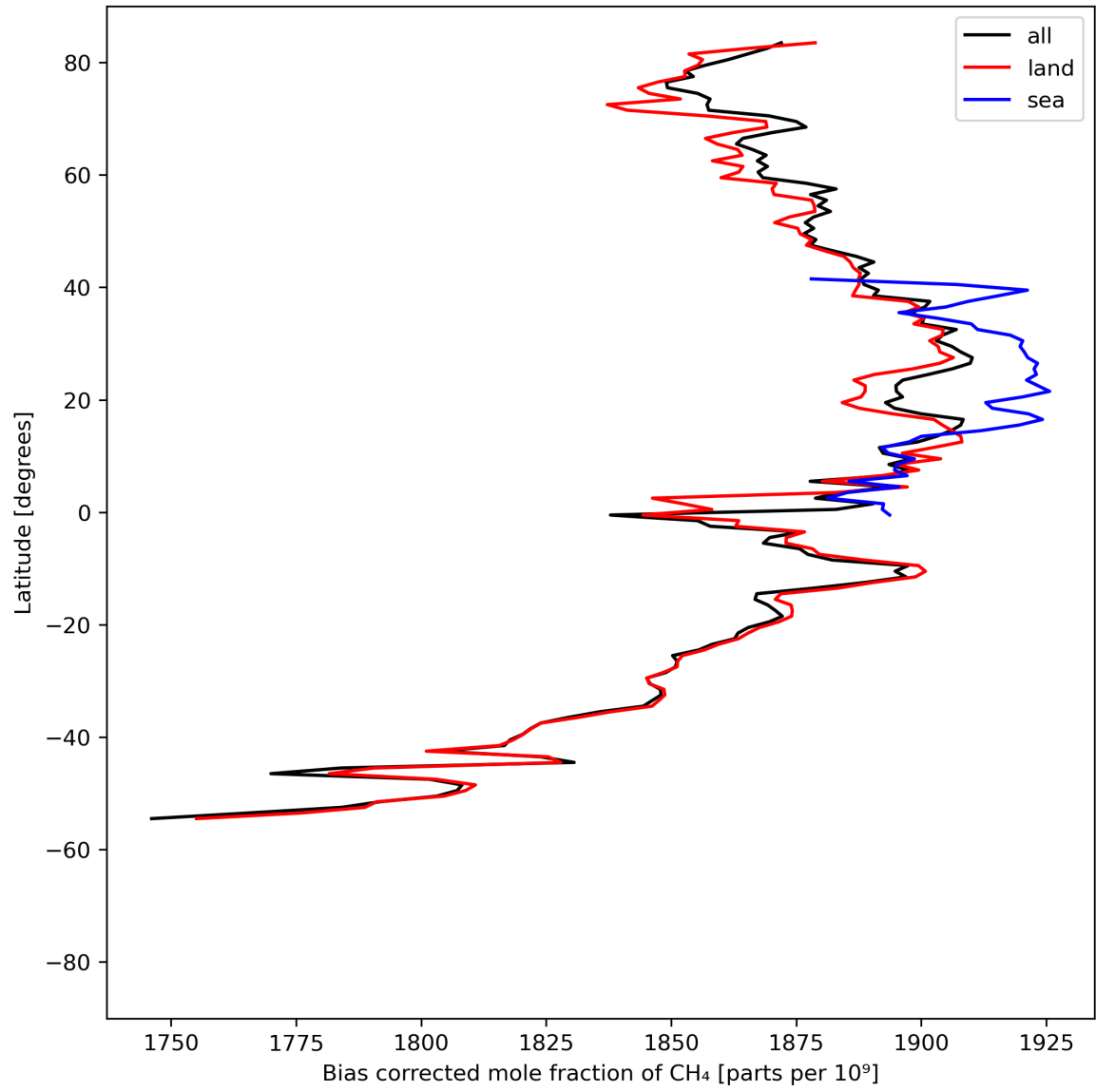
Figure 14: Zonal average of “Bias corrected mole fraction of \text{CH}_4 ” for 2024-04-26 to 2024-04-28.
