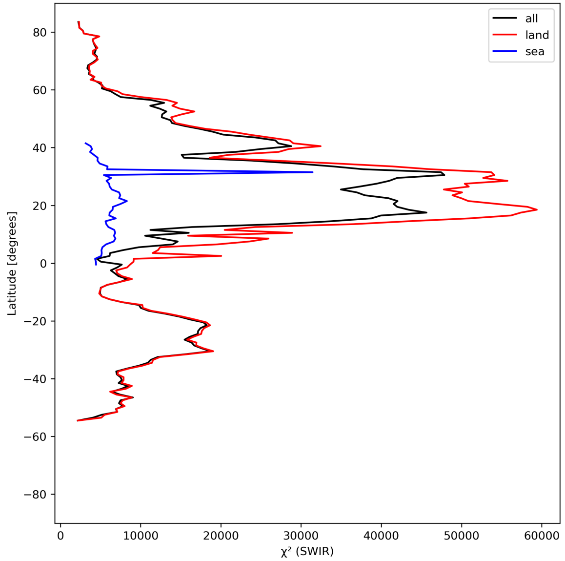
Figure 17: Zonal average of “ \chi^2 (SWIR)” for 2024-04-26 to 2024-04-28.
