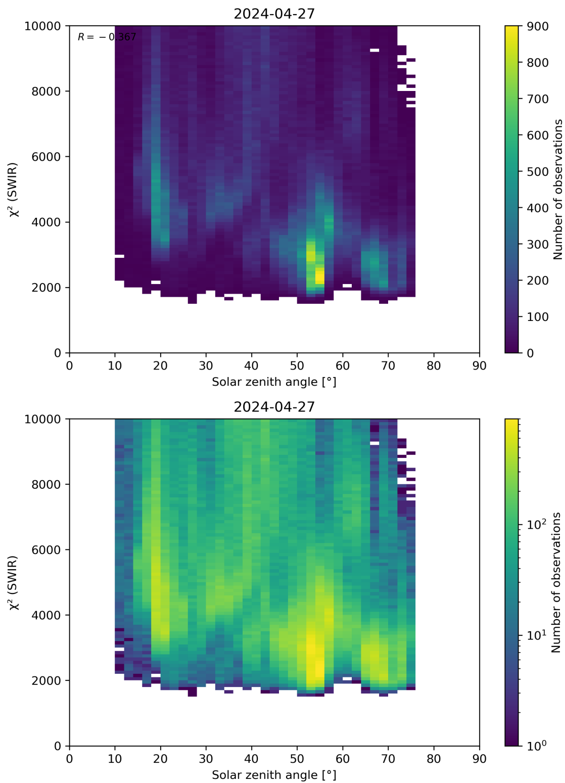
Figure 95: Scatter density plot of “Solar zenith angle” against “ \chi^2 (SWIR)” for 2024-04-26 to 2024-04-28.
