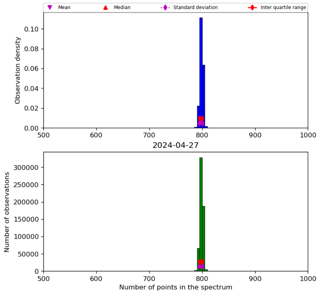
Figure 26: Histogram of “Number of points in the spectrum” for 2024-04-26 to 2024-04-28
