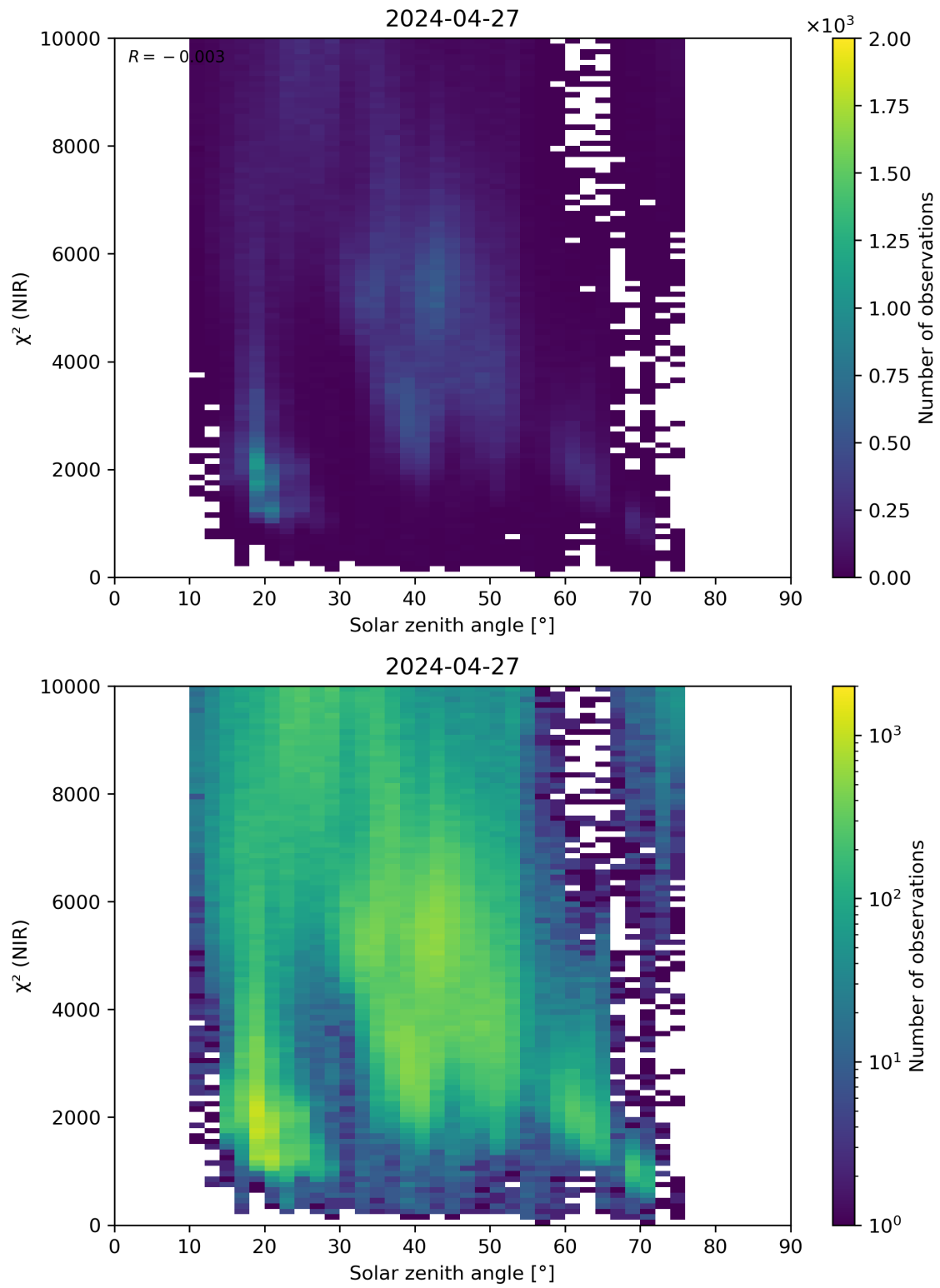
Figure 94: Scatter density plot of “Solar zenith angle” against “ \chi^2 (NIR)” for 2024-04-26 to 2024-04-28.
