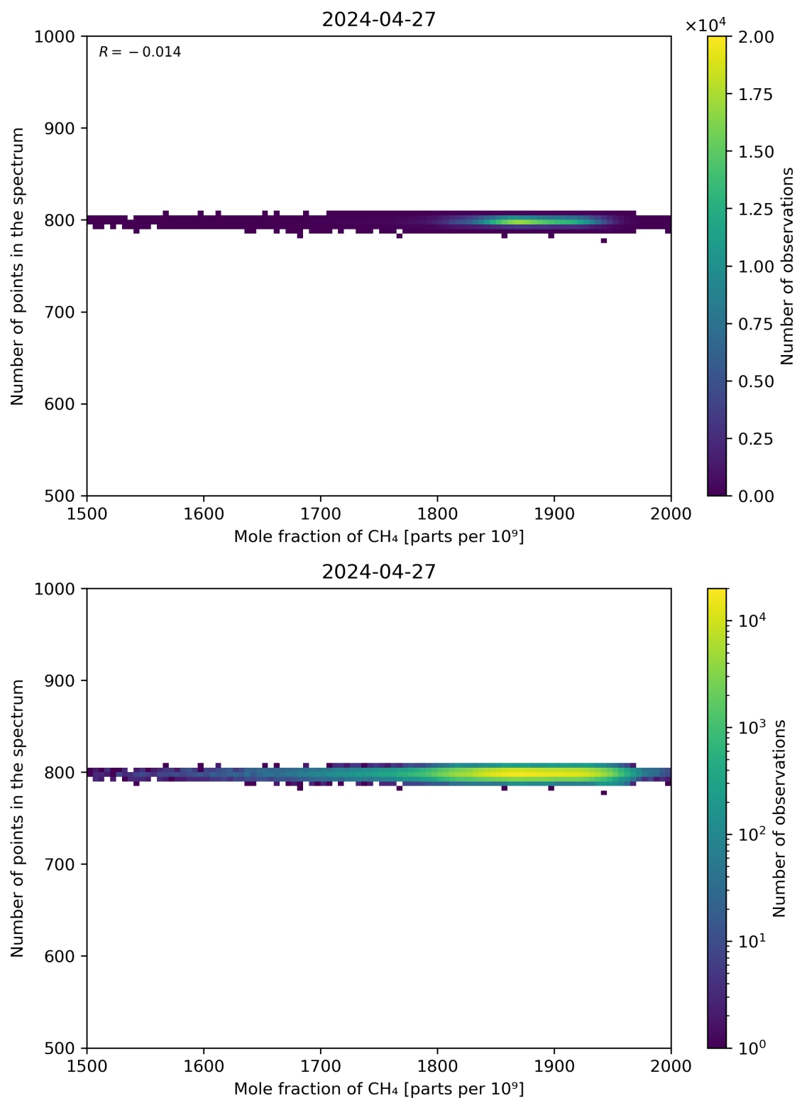
Figure 77: Scatter density plot of “Mole fraction of CH 4 ” against “Number of points in the spectrum” for 2024-04-26 to 2024-04-28.
