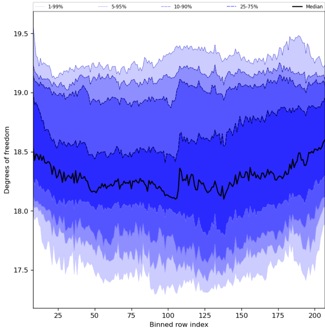
Figure 41: Along track statistics of “Degrees of freedom” for 2024-04-26 to 2024-04-28
