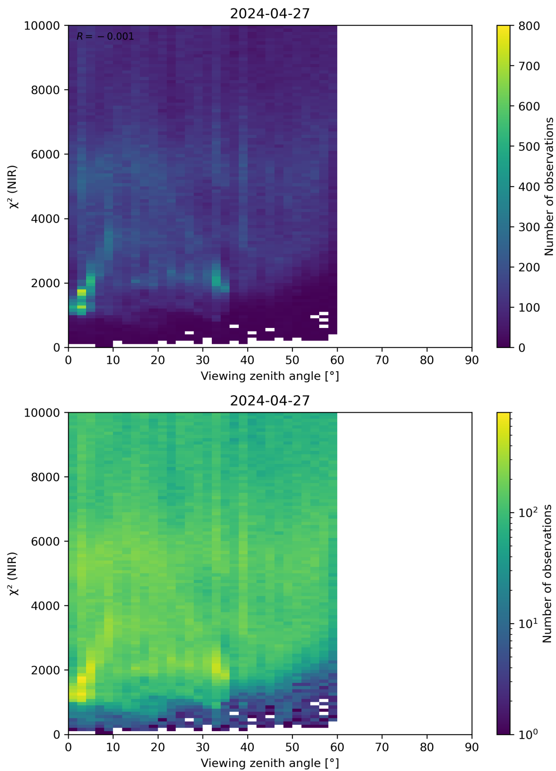
Figure 105: Scatter density plot of “Viewing zenith angle” against “ \chi^2 (NIR)” for 2024-04-26 to 2024-04-28.
