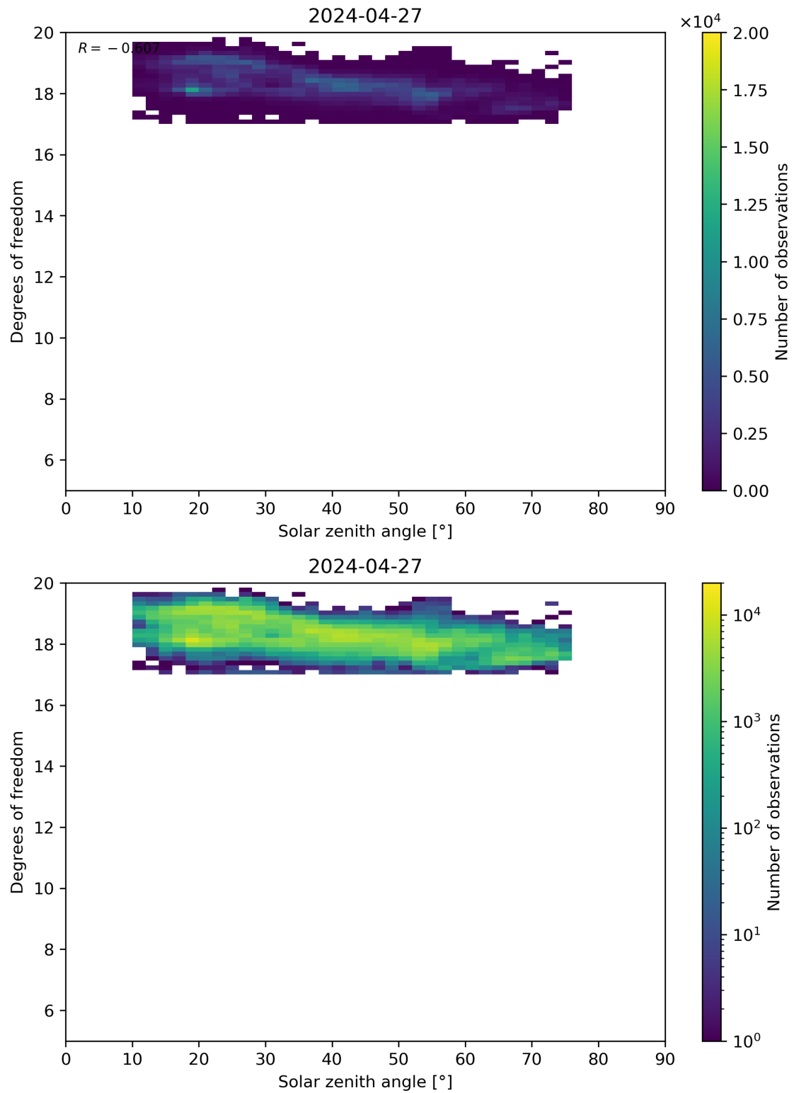
Figure 96: Scatter density plot of “Solar zenith angle” against “Degrees of freedom” for 2024-04-26 to 2024-04-28.
