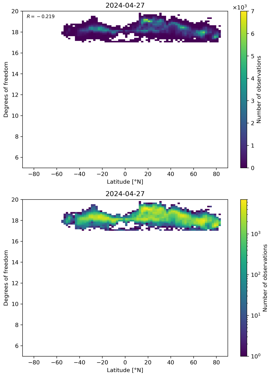
Figure 55: Scatter density plot of “Latitude” against “Degrees of freedom” for 2024-04-26 to 2024-04-28.
