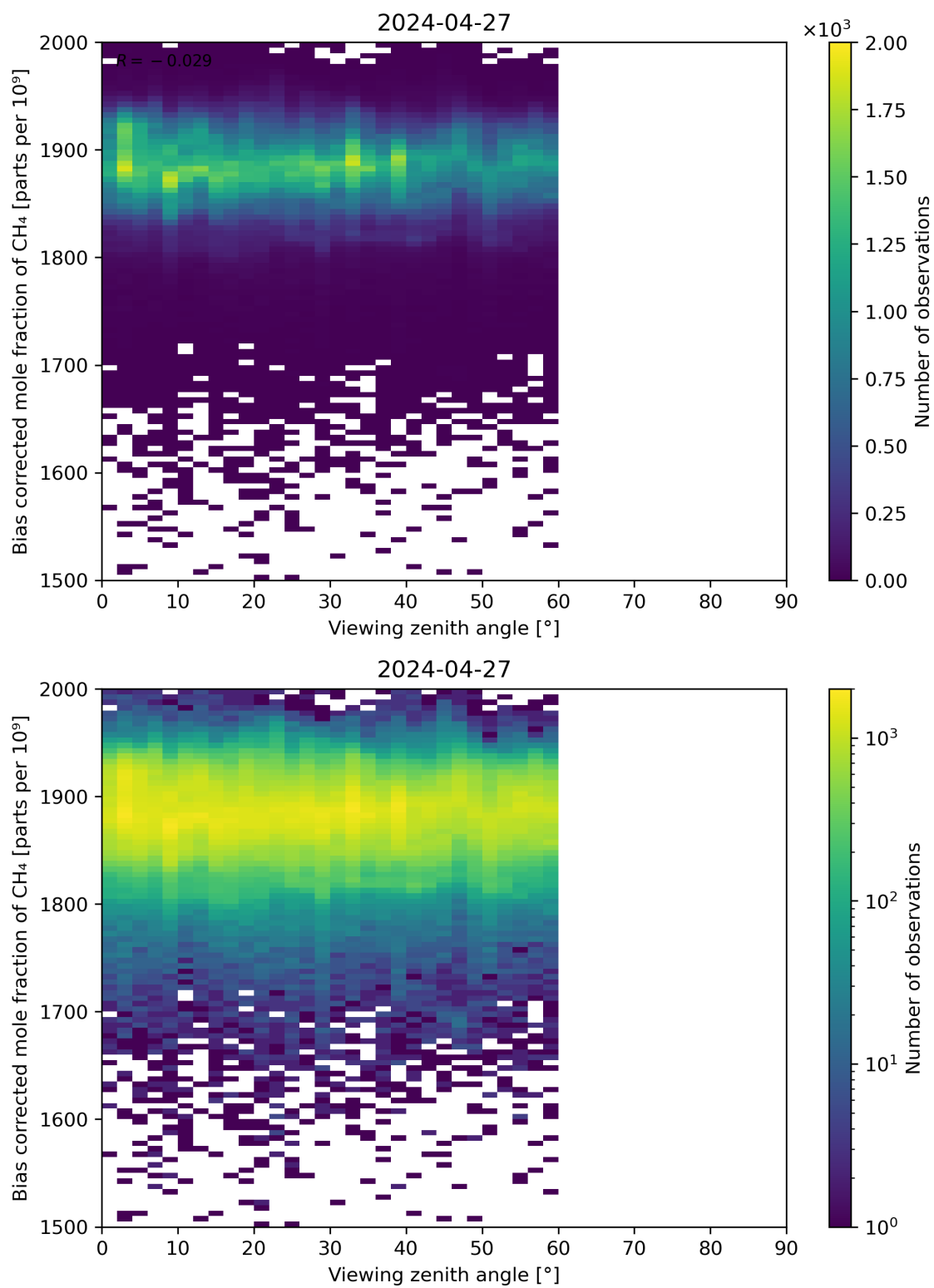
Figure 111: Scatter density plot of “Viewing zenith angle” against “Bias corrected mole fraction of CH 4 ” for 2024-04-26 to 2024-04-28.
