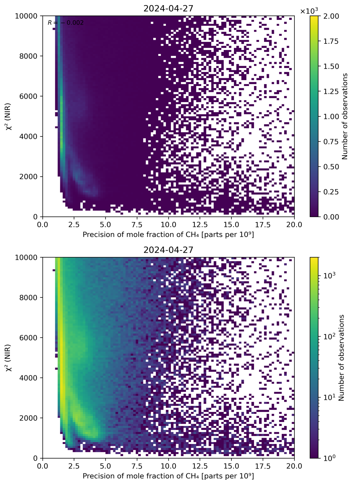
Figure 78: Scatter density plot of “Precision of mole fraction of CH 4 ” against “ \chi^2 (NIR)” for 2024-04-26 to 2024-04-28.
