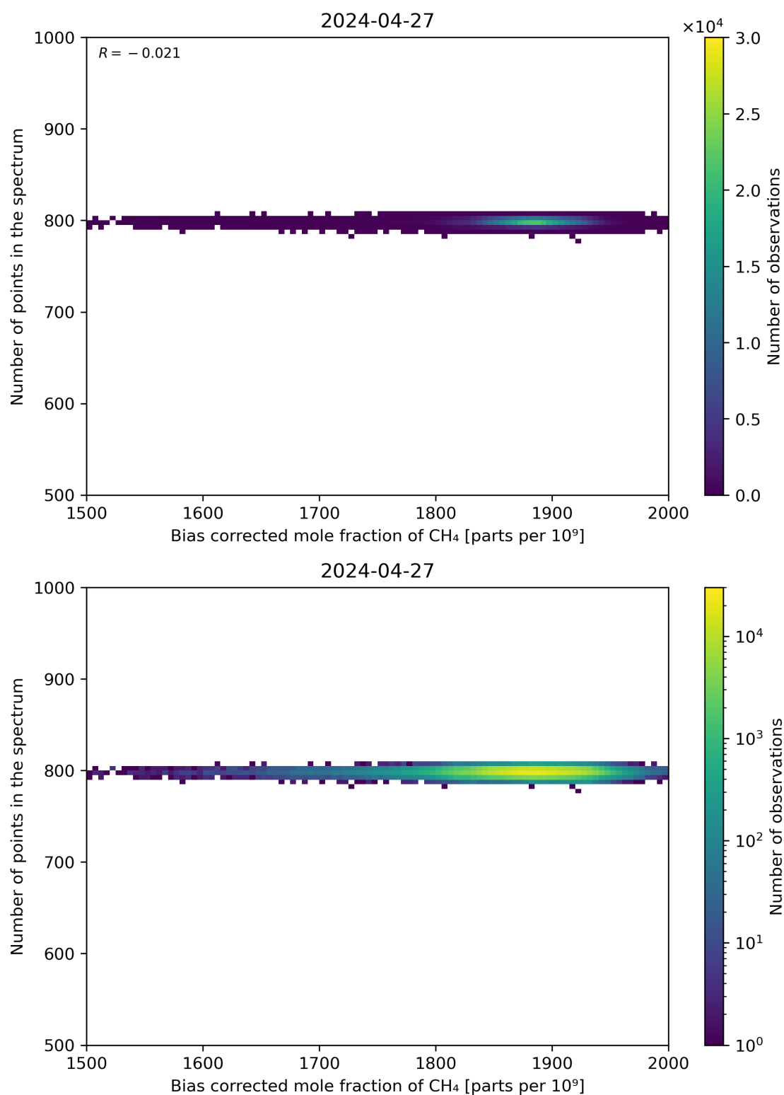
Figure 68: Scatter density plot of “Bias corrected mole fraction of CH 4 ” against “Number of points in the spectrum” for 2024-04-26 to 2024-04-28.
