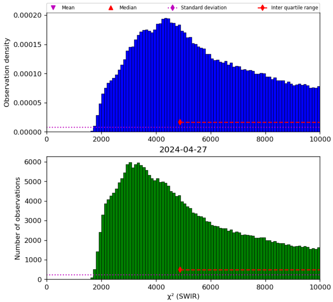
Figure 28: Histogram of “ \chi^2 (SWIR)” for 2024-04-26 to 2024-04-28
