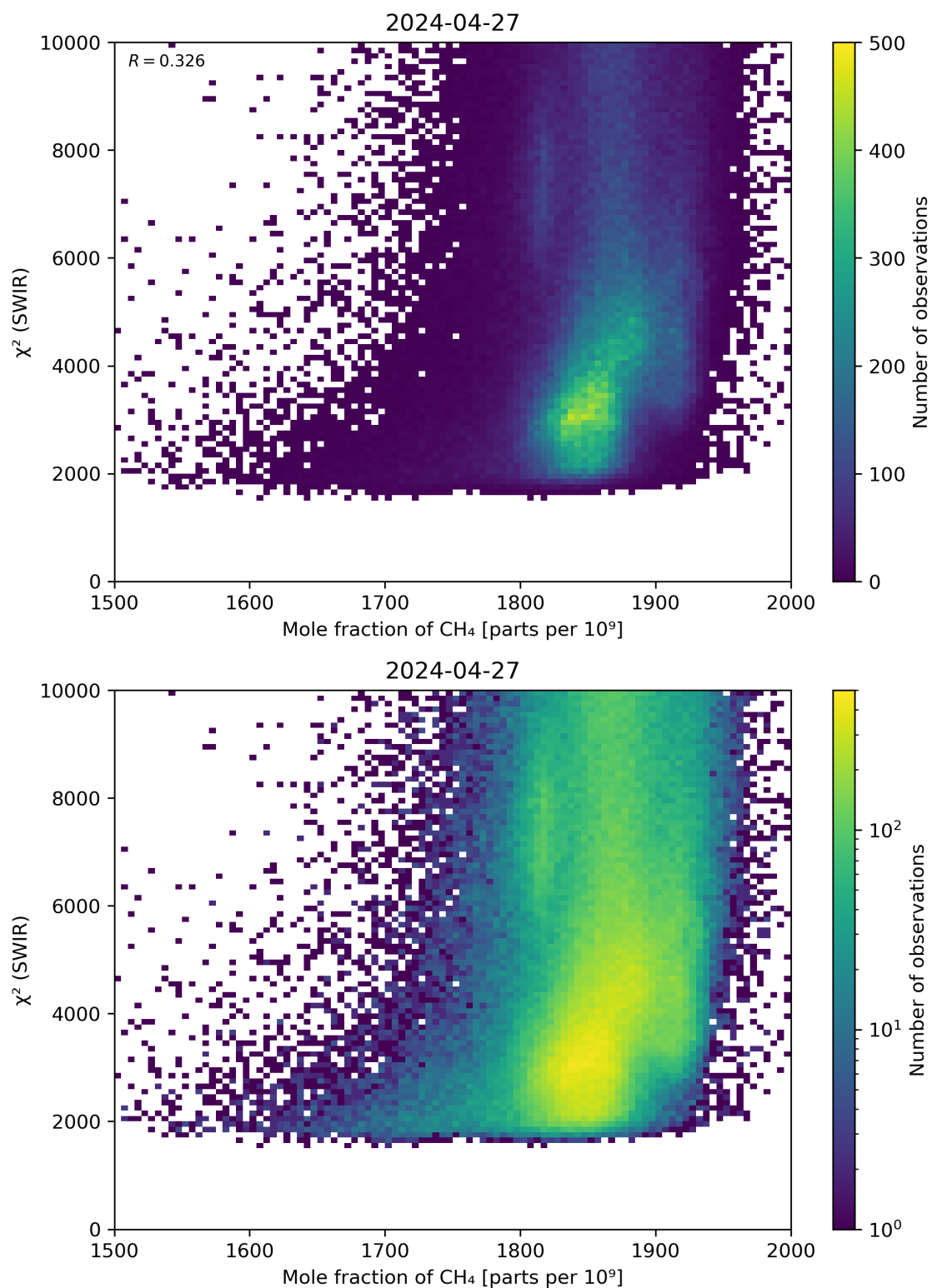
Figure 71: Scatter density plot of “Mole fraction of \text{CH}_4 ” against “ \chi^2 (SWIR)” for 2024-04-26 to 2024-04-28.
