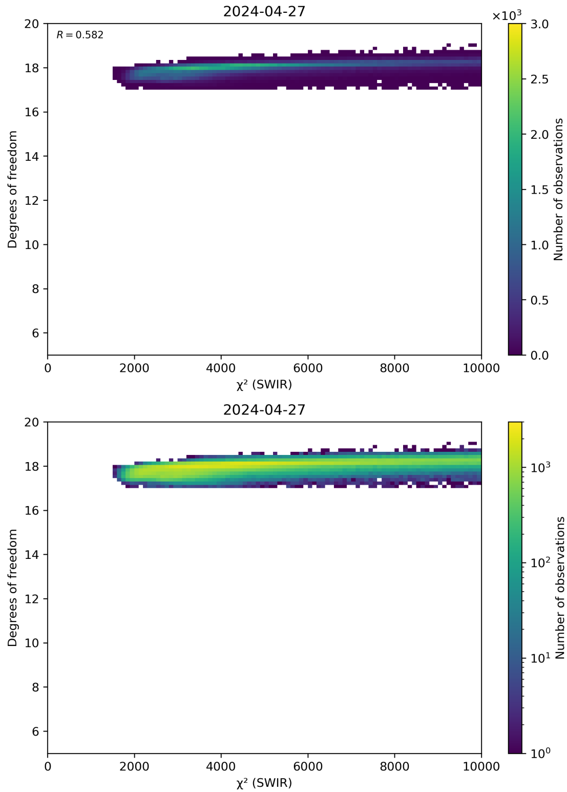
Figure 48: Scatter density plot of “ \chi^2 (SWIR)” against “Degrees of freedom” for 2024-04-26 to 2024-04-28.
