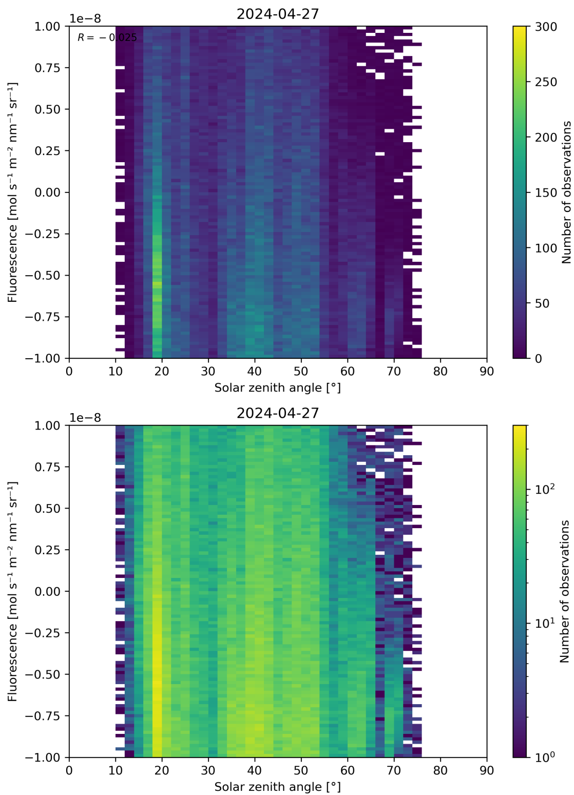
Figure 97: Scatter density plot of “Solar zenith angle” against “Fluorescence” for 2024-04-26 to 2024-04-28.
