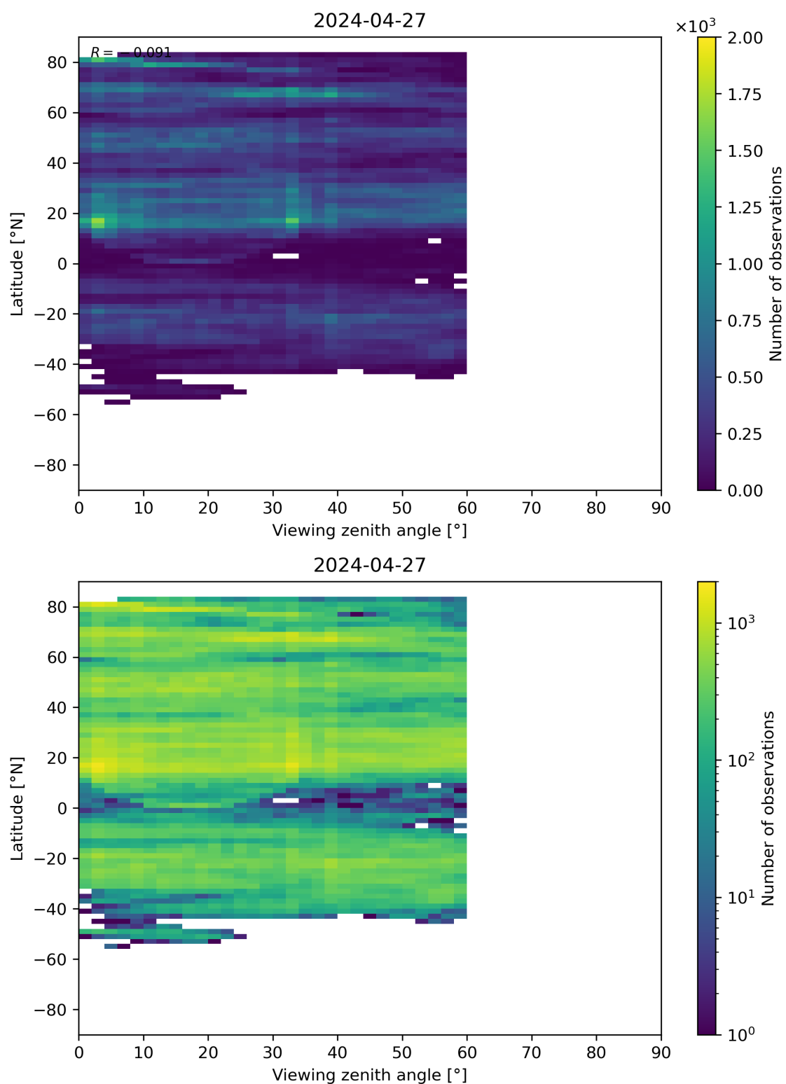
Figure 109: Scatter density plot of “Viewing zenith angle” against “Latitude” for 2024-04-26 to 2024-04-28.
