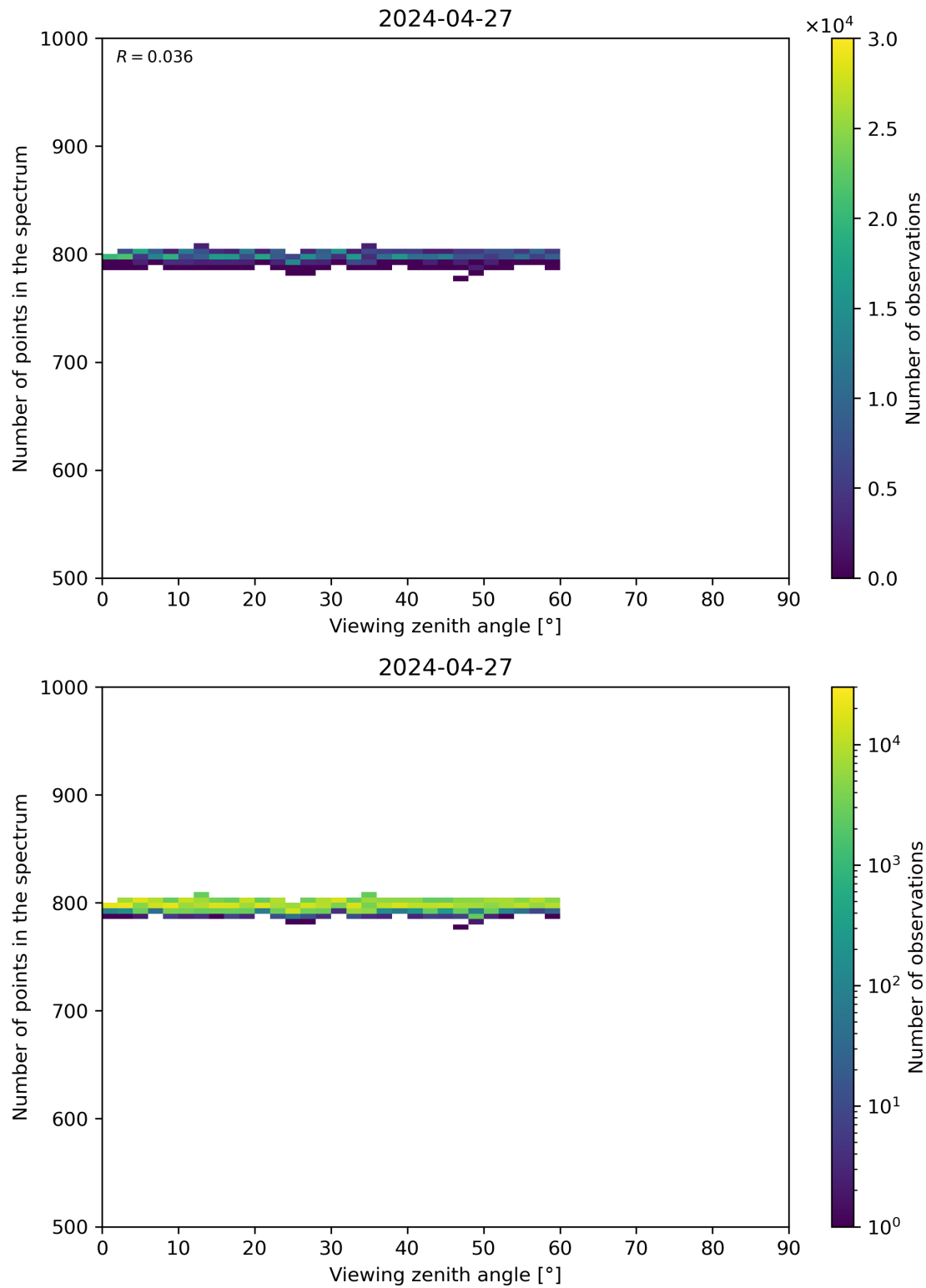
Figure 114: Scatter density plot of “Viewing zenith angle” against “Number of points in the spectrum” for 2024-04-26 to 2024-04-28.
