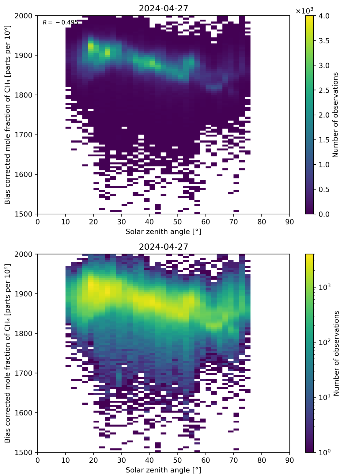
Figure 100: Scatter density plot of “Solar zenith angle” against “Bias corrected mole fraction of CH 4 ” for 2024-04-26 to 2024-04-28.
