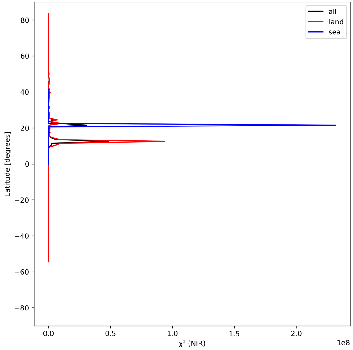
Figure 18: Zonal average of “ \chi^2 (NIR)” for 2024-04-26 to 2024-04-28.
