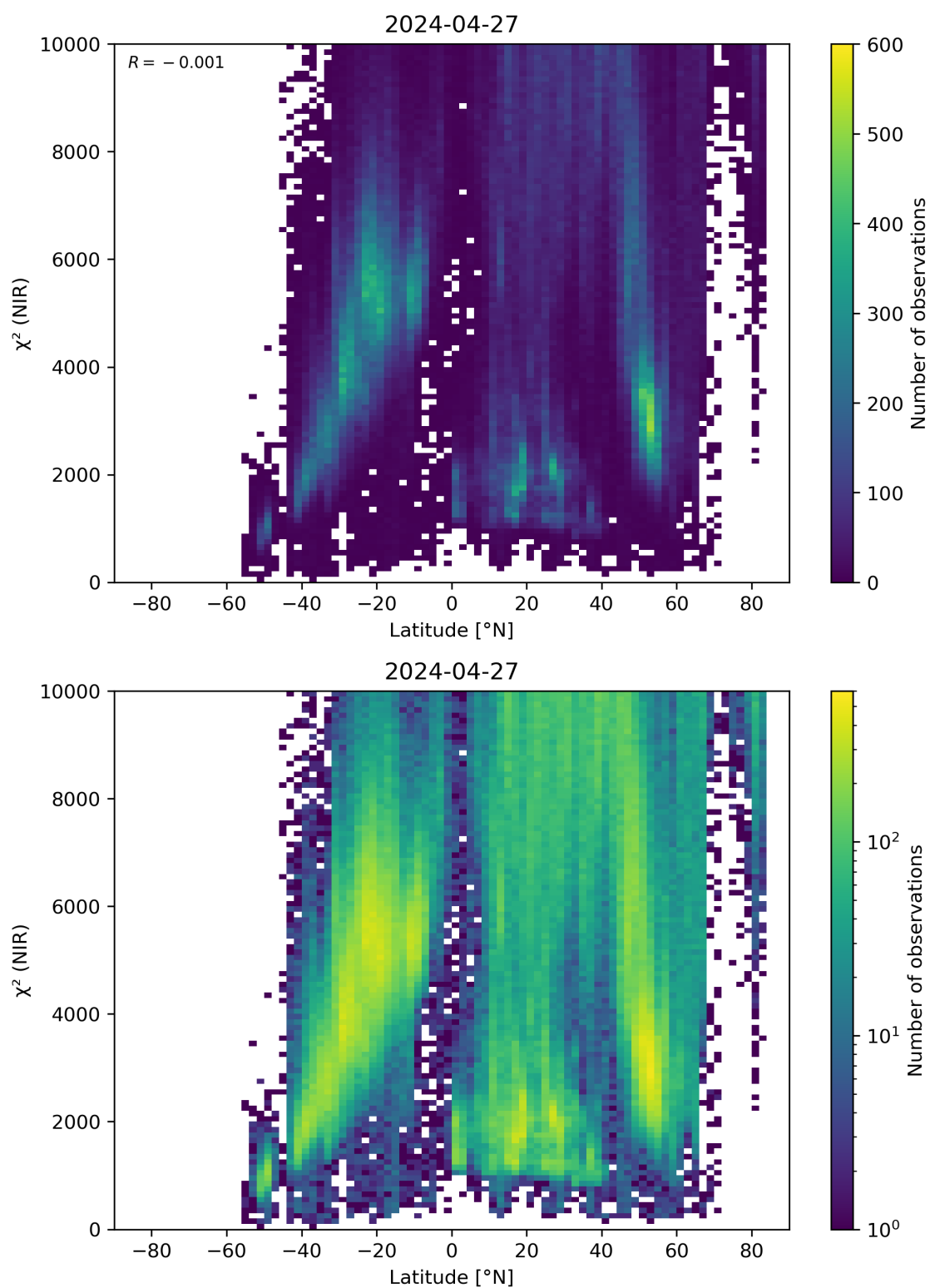
Figure 53: Scatter density plot of “Latitude” against “ \chi^2 (NIR)” for 2024-04-26 to 2024-04-28.
