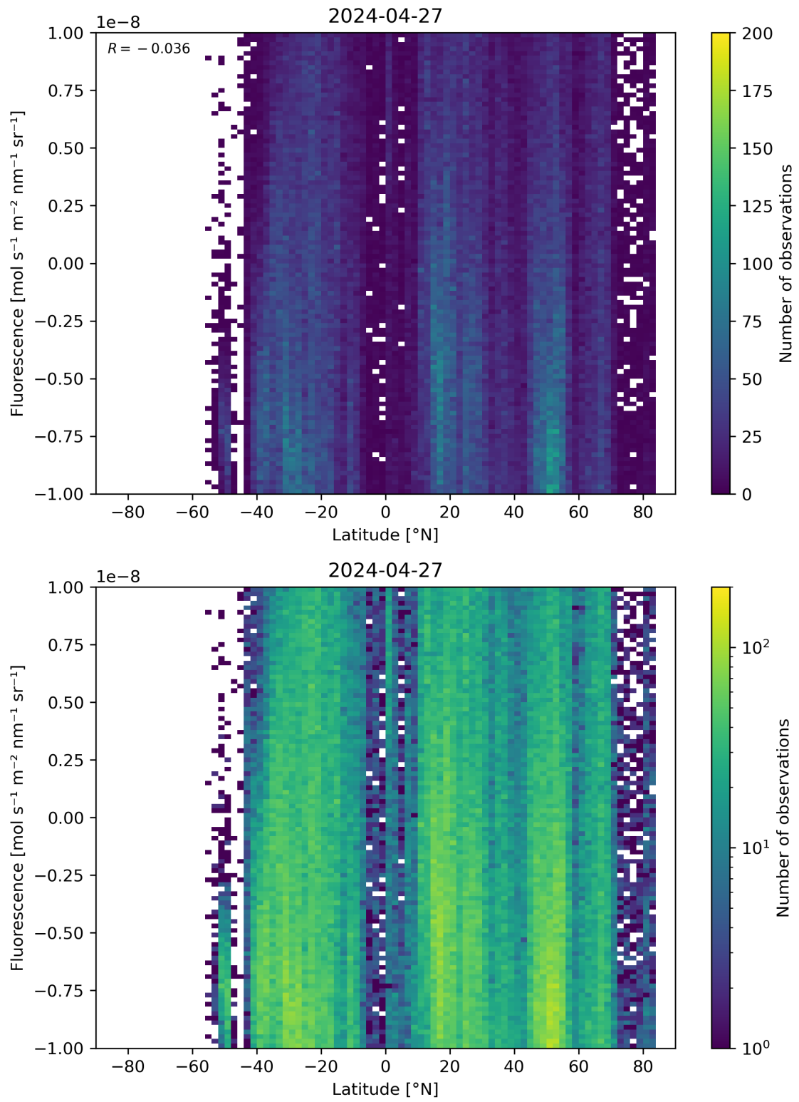
Figure 56: Scatter density plot of “Latitude” against “Fluorescence” for 2024-04-26 to 2024-04-28.
