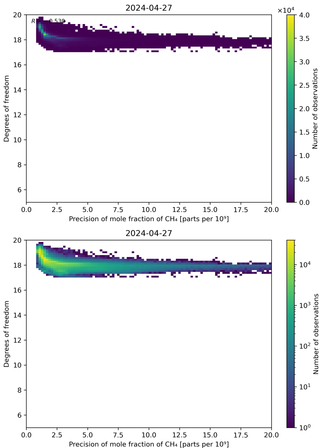
Figure 80: Scatter density plot of “Precision of mole fraction of CH 4 ” against “Degrees of freedom” for 2024-04-26 to 2024-04-28.
