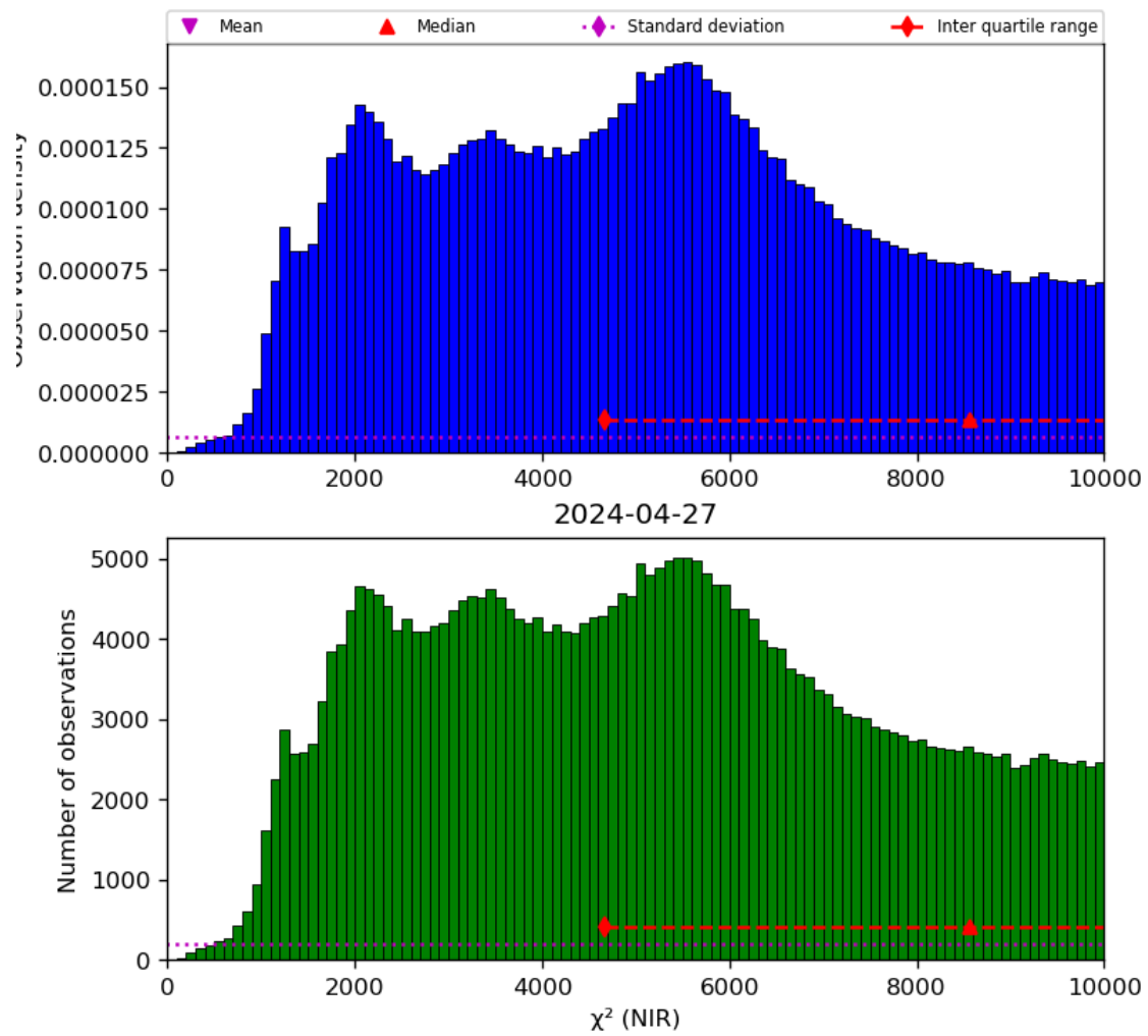
Figure 29: Histogram of “ \chi^2 (NIR)” for 2024-04-26 to 2024-04-28
