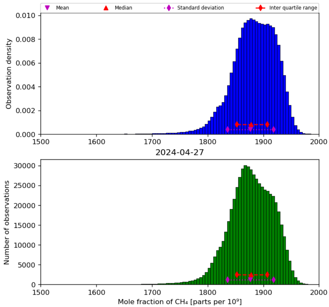
Figure 23: Histogram of “Mole fraction of CH 4 ” for 2024-04-26 to 2024-04-28
