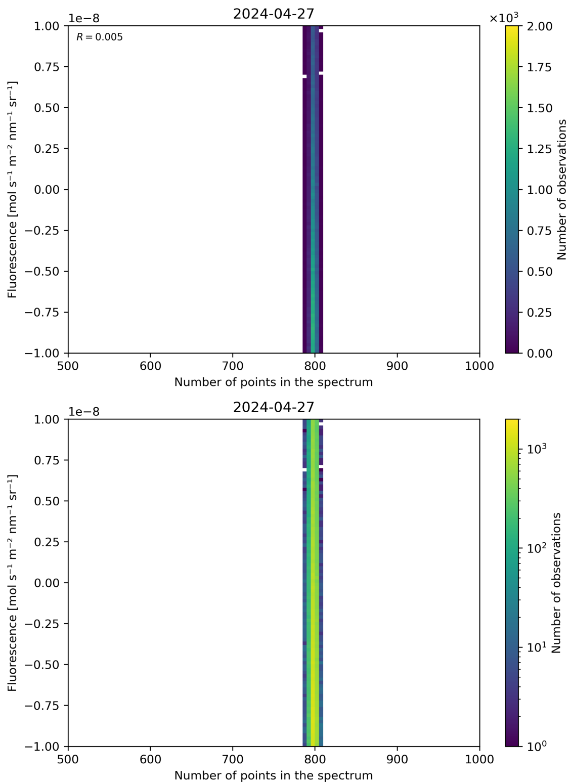
Figure 91: Scatter density plot of “Number of points in the spectrum” against “Fluorescence” for 2024-04-26 to 2024-04-28.
