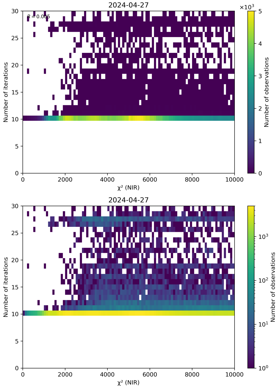
Figure 46: Scatter density plot of “ \chi^2 (NIR)” against “Number of iterations” for 2024-04-26 to 2024-04-28.
