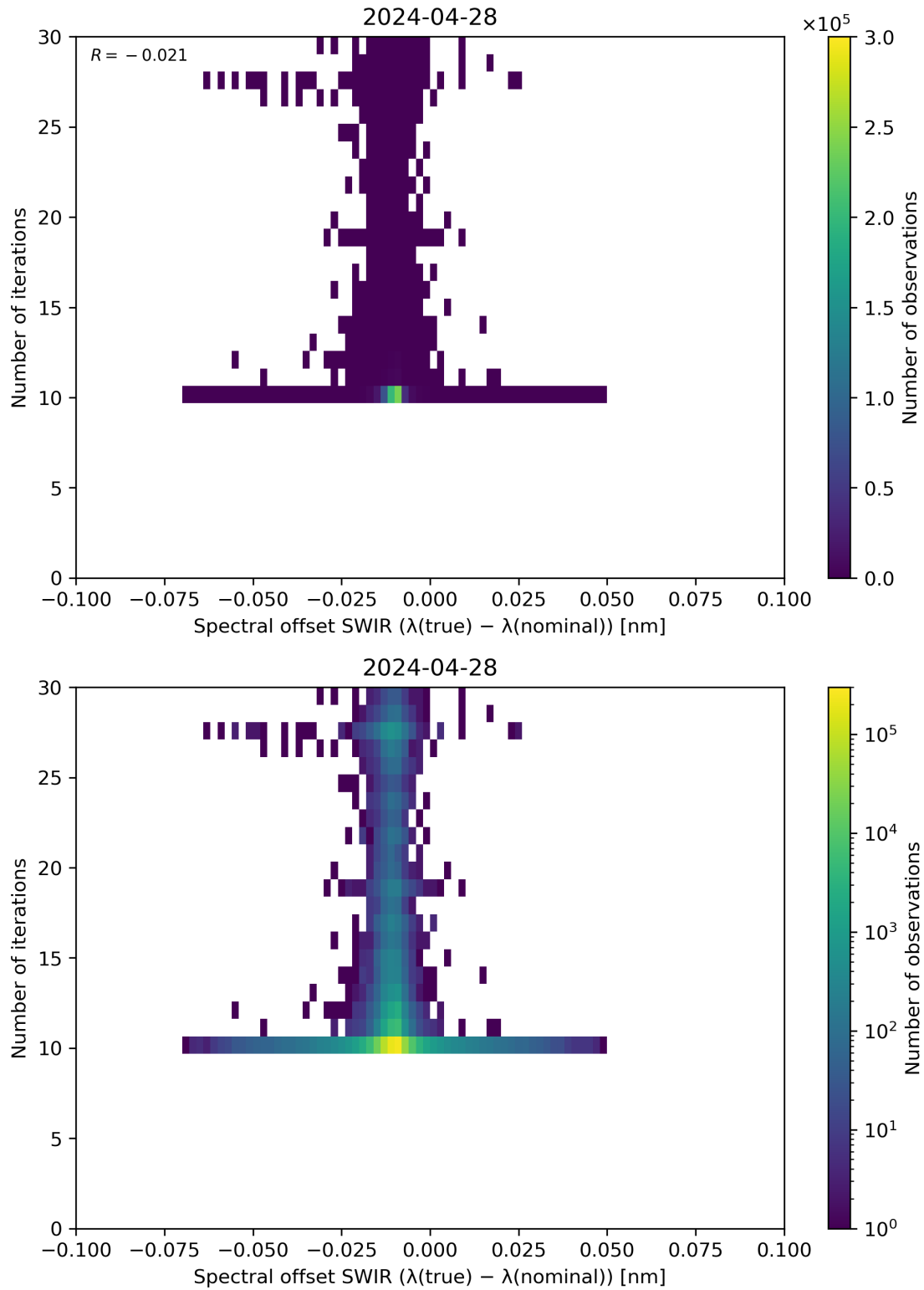
Figure 121: Scatter density plot of “Spectral offset SWIR ( \lambda(\text{true}) - \lambda(\text{nominal}) )” against “Number of iterations” for 2024-04-27 to 2024-04-29.
