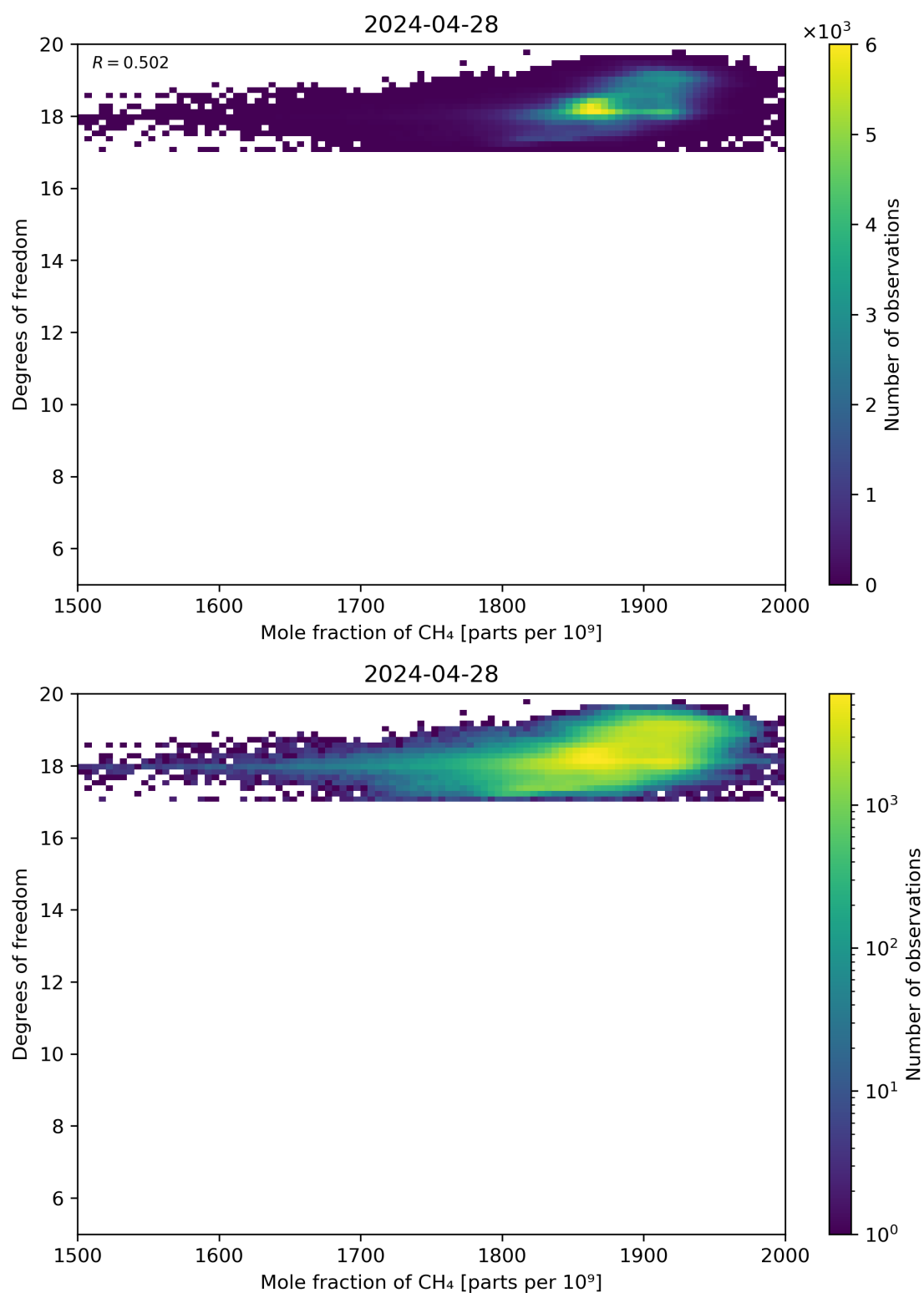
Figure 72: Scatter density plot of “Mole fraction of CH 4 ” against “Degrees of freedom” for 2024-04-27 to 2024-04-29.
