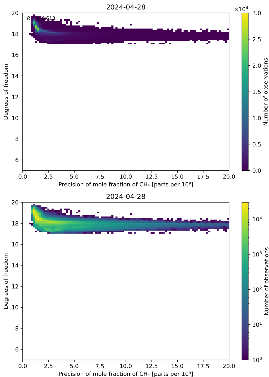
Figure 80: Scatter density plot of “Precision of mole fraction of CH 4 ” against “Degrees of freedom” for 2024-04-27 to 2024-04-29.
