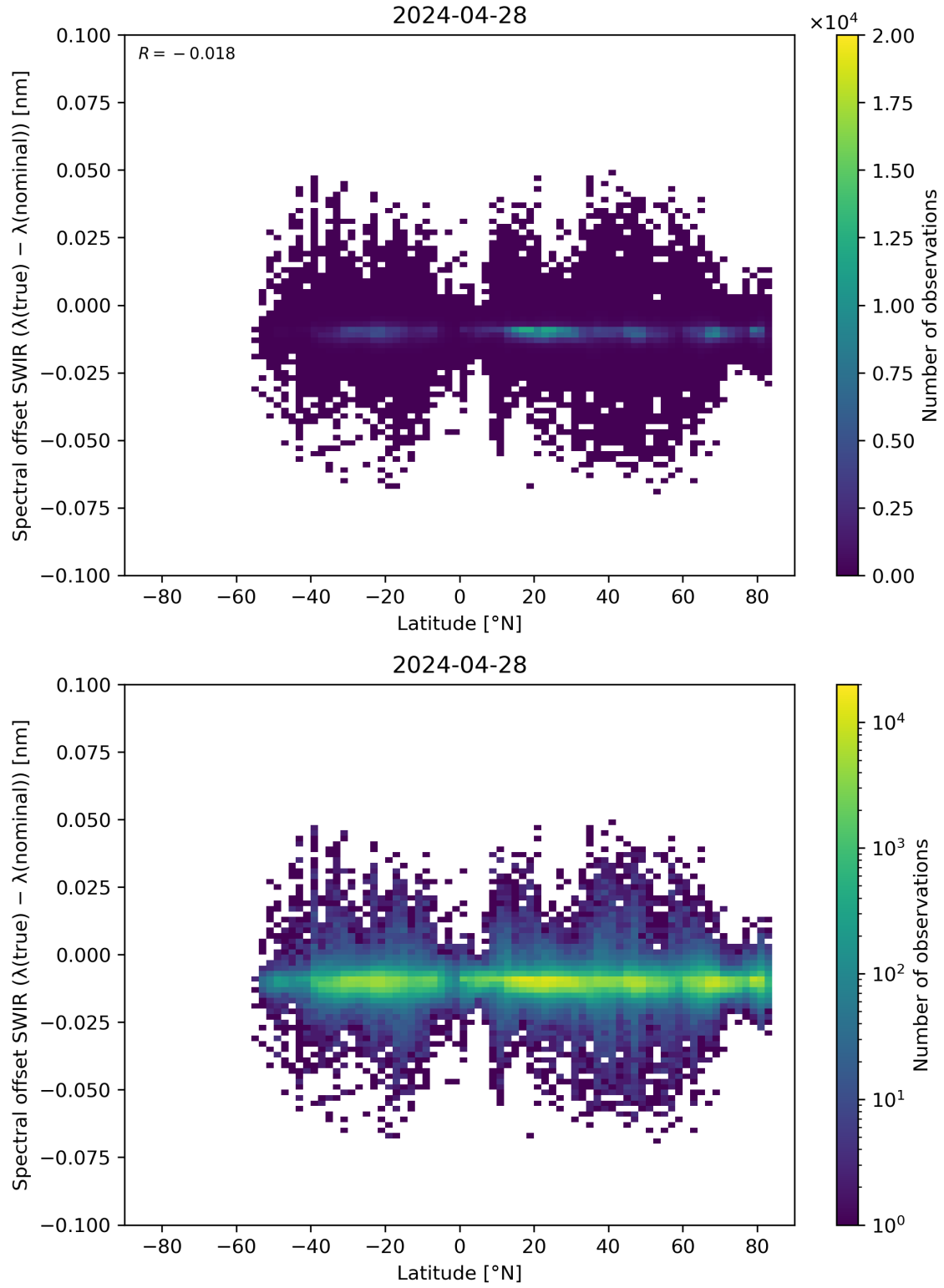
Figure 62: Scatter density plot of “Latitude” against “Spectral offset SWIR ( \lambda(\text{true}) - \lambda(\text{nominal}) )” for 2024-04-27 to 2024-04-29.
