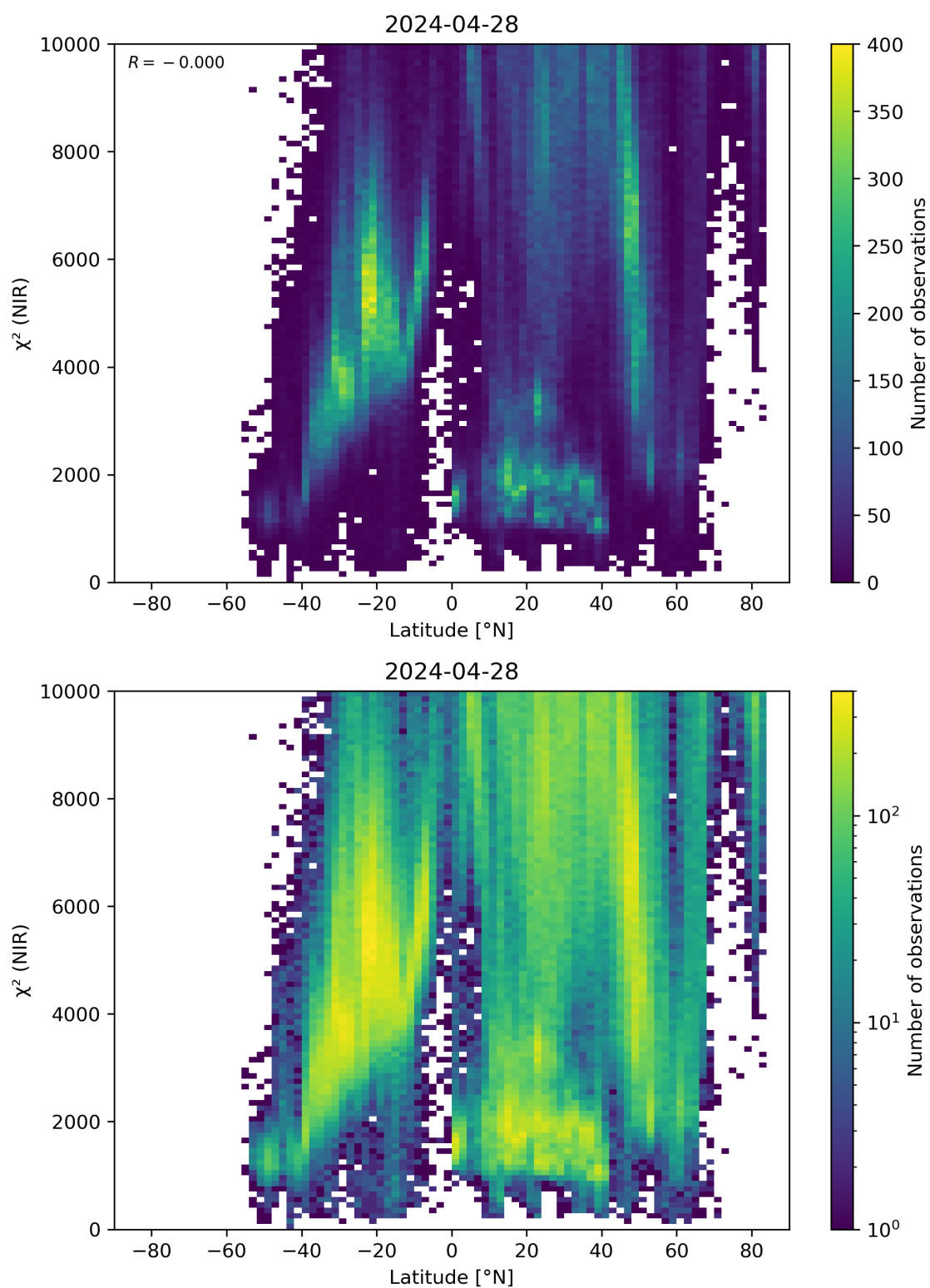
Figure 53: Scatter density plot of “Latitude” against “ \chi^2 (NIR)” for 2024-04-27 to 2024-04-29.
