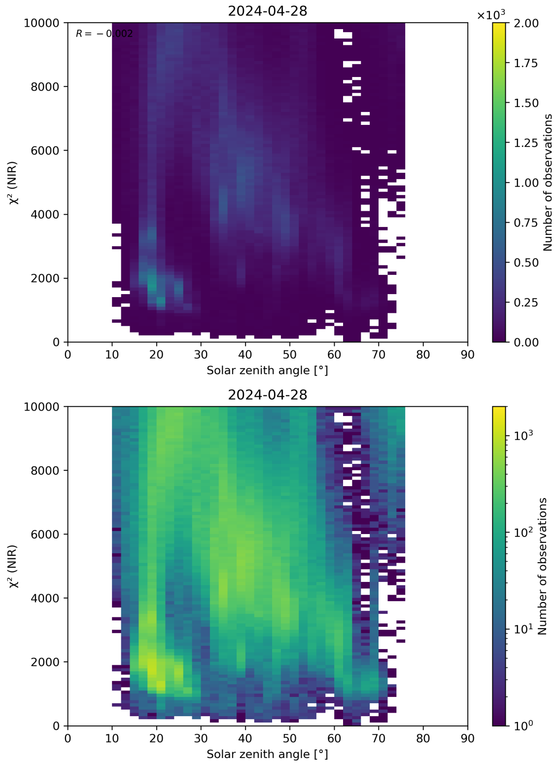
Figure 94: Scatter density plot of “Solar zenith angle” against “ \chi^2 (NIR)” for 2024-04-27 to 2024-04-29.
