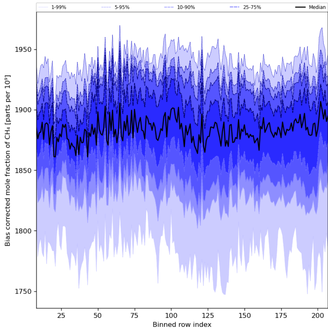
Figure 36: Along track statistics of “Bias corrected mole fraction of CH 4 ” for 2024-04-27 to 2024-04-29
