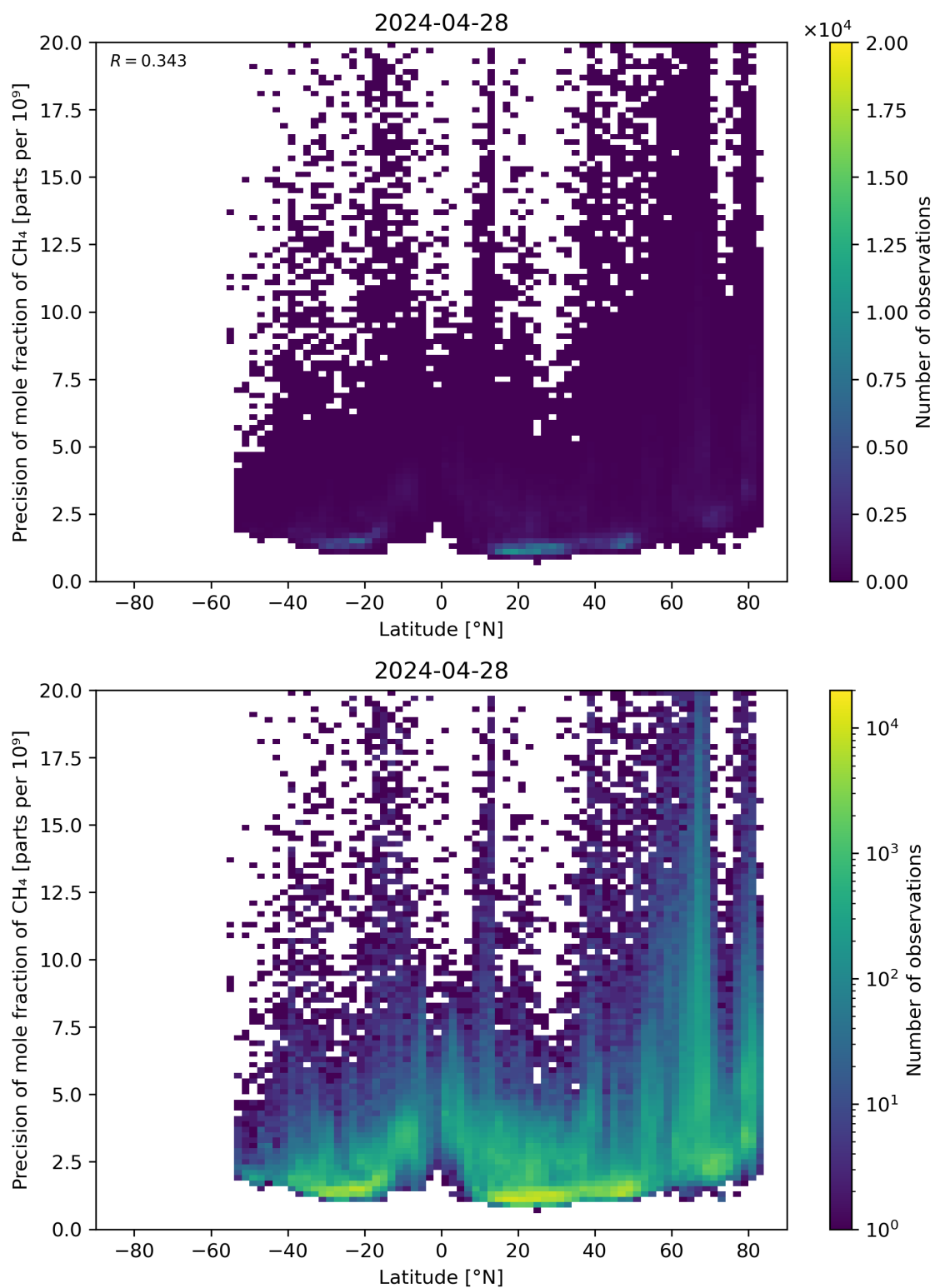
Figure 59: Scatter density plot of “Latitude” against “Precision of mole fraction of \text{CH}_4 ” for 2024-04-27 to 2024-04-29.
