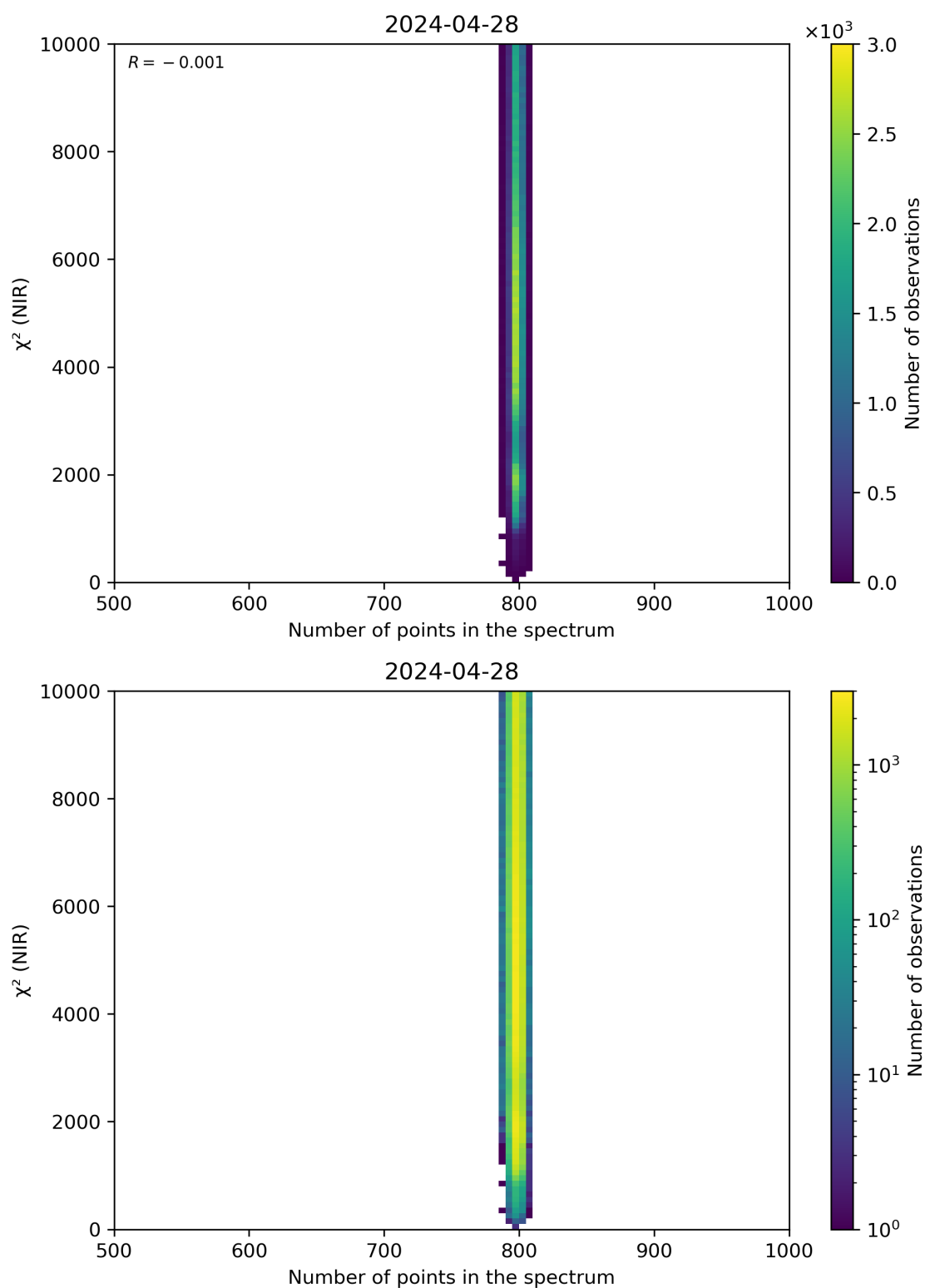
Figure 88: Scatter density plot of “Number of points in the spectrum” against “ \chi^2 (NIR)” for 2024-04-27 to 2024-04-29.
