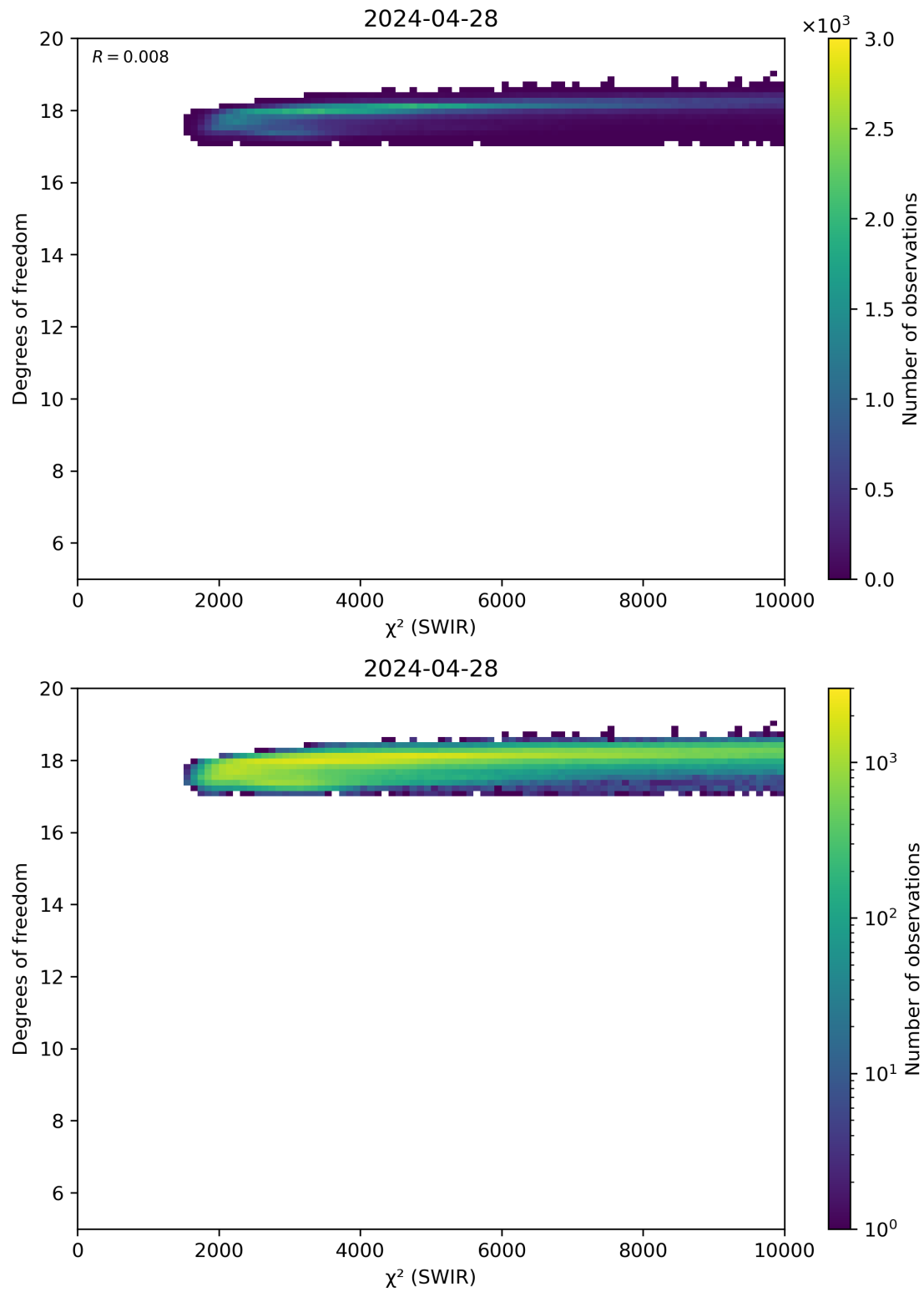
Figure 48: Scatter density plot of “ \chi^2 (SWIR)” against “Degrees of freedom” for 2024-04-27 to 2024-04-29.
