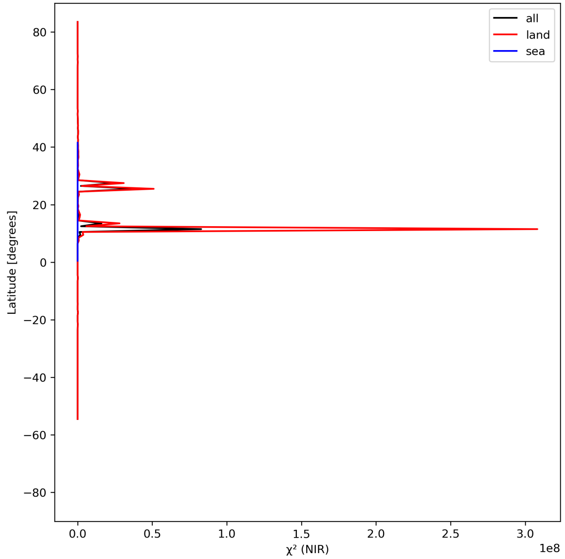
Figure 18: Zonal average of “ \chi^2 (NIR)” for 2024-04-27 to 2024-04-29.
