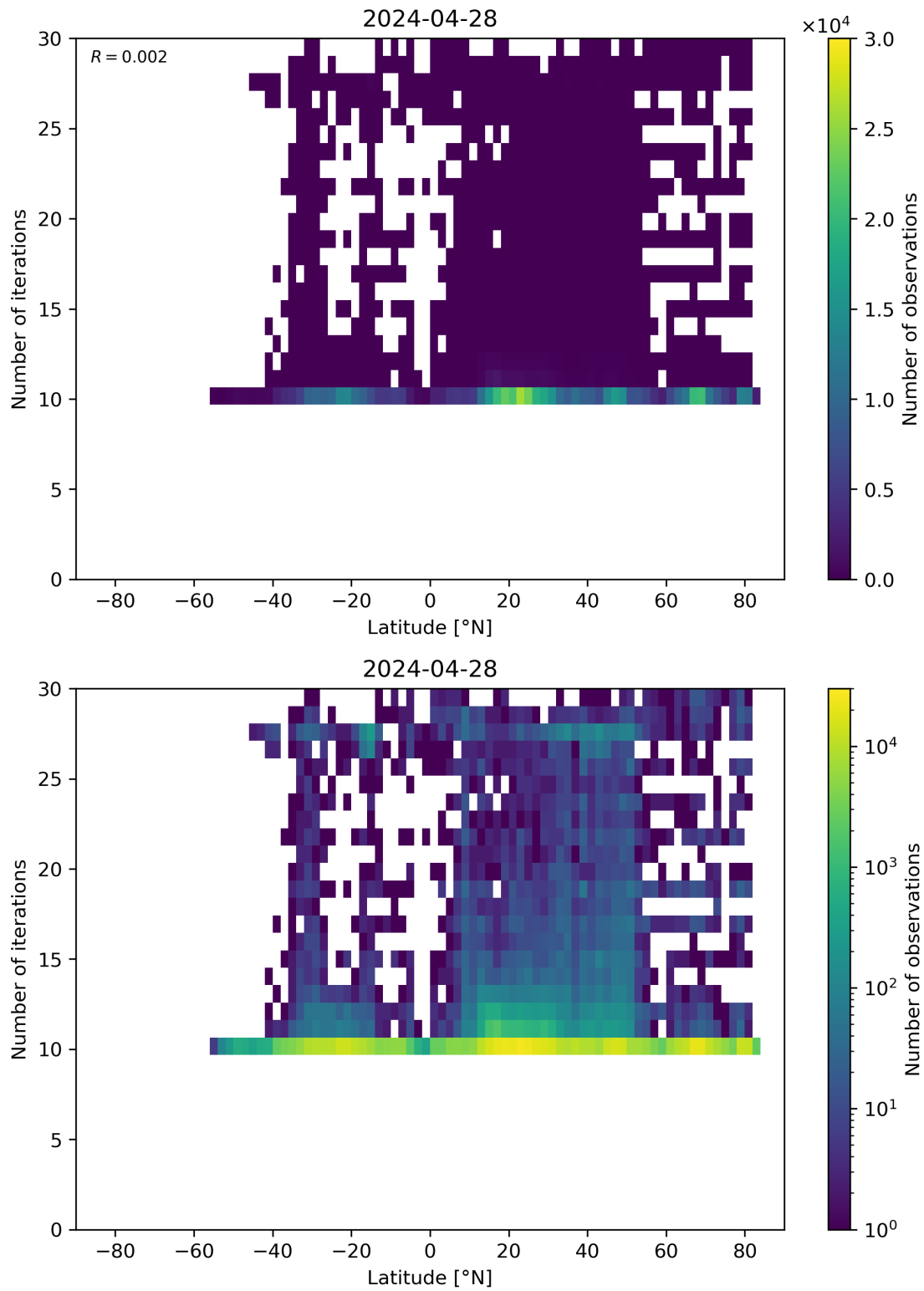
Figure 60: Scatter density plot of “Latitude” against “Number of iterations” for 2024-04-27 to 2024-04-29.
