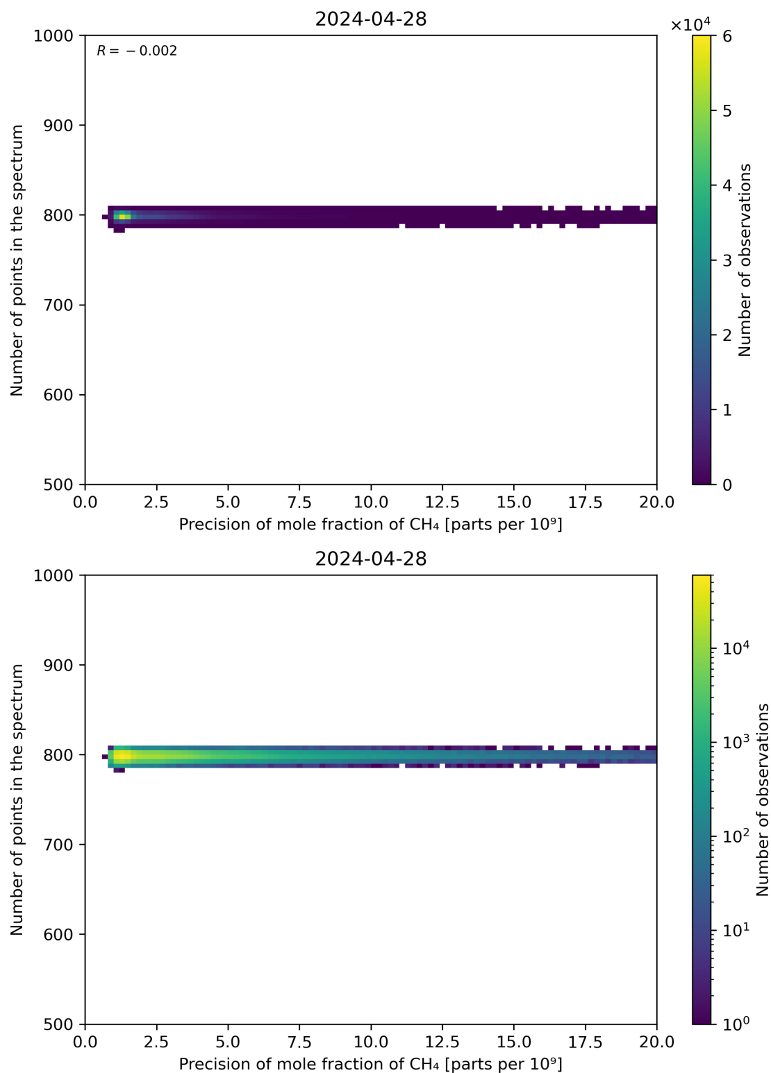
Figure 84: Scatter density plot of “Precision of mole fraction of CH 4 ” against “Number of points in the spectrum” for 2024-04-27 to 2024-04-29.
