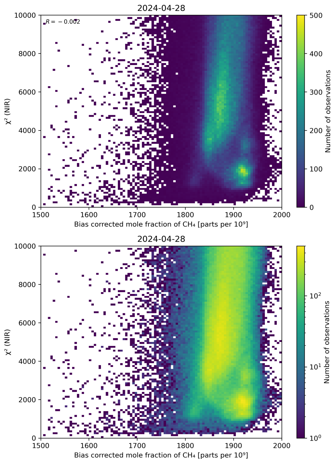
Figure 63: Scatter density plot of “Bias corrected mole fraction of CH 4 ” against “ \chi^2 (NIR)” for 2024-04-27 to 2024-04-29.
