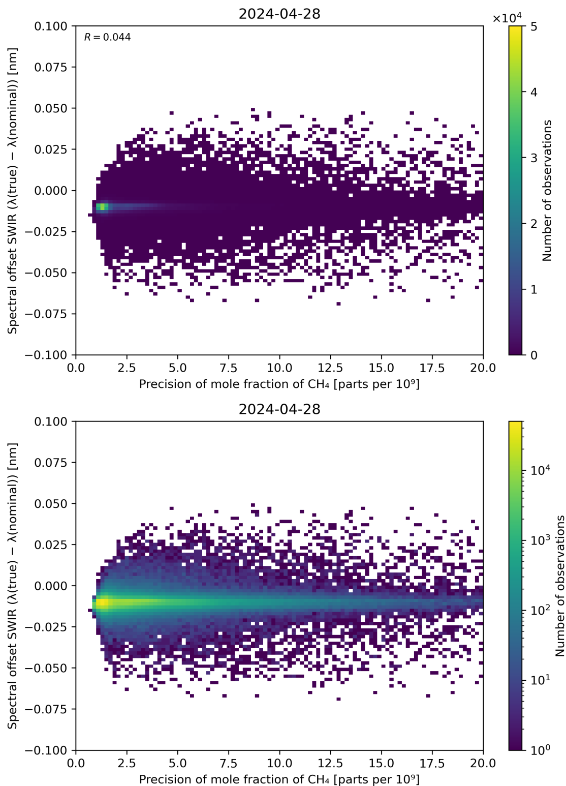
Figure 85: Scatter density plot of “Precision of mole fraction of \text{CH}_4 ” against “Spectral offset SWIR ( \lambda(\text{true}) - \lambda(\text{nominal}) )” for 2024-04-27 to 2024-04-29.
