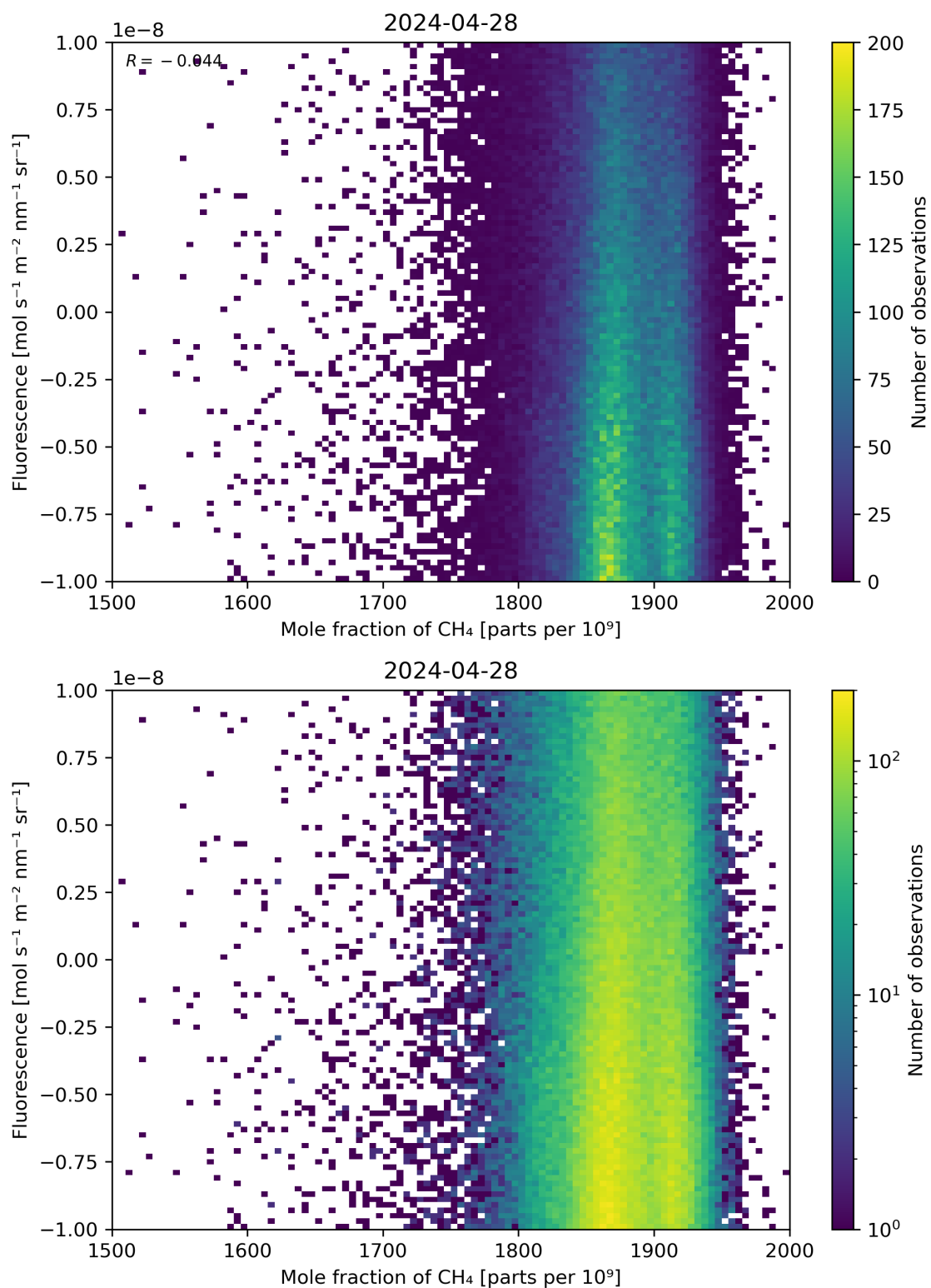
Figure 73: Scatter density plot of “Mole fraction of \text{CH}_4 ” against “Fluorescence” for 2024-04-27 to 2024-04-29.
