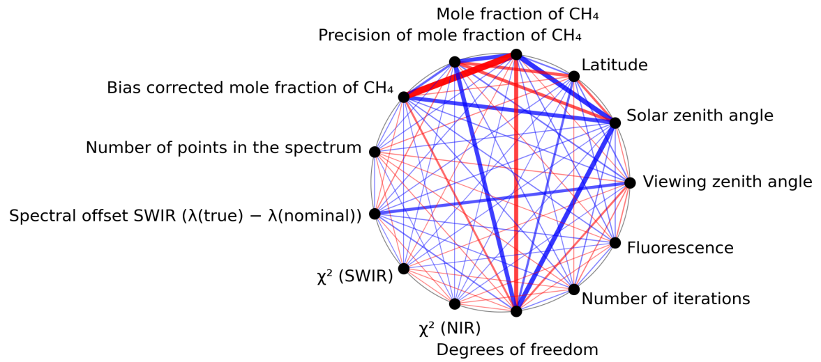
Figure 1: Map of correlation graph for 2024-04-27 to 2024-04-29.
