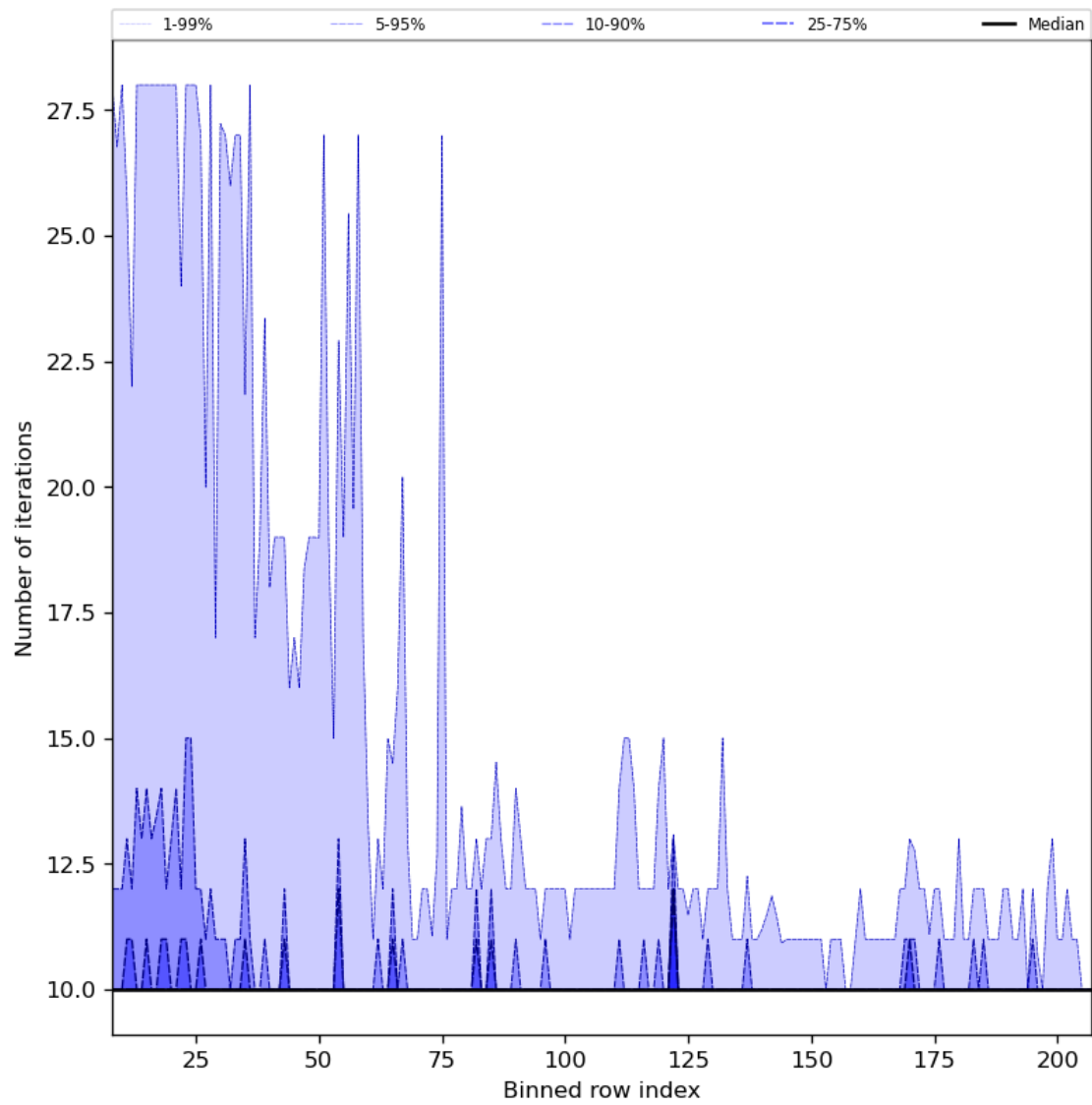
Figure 42: Along track statistics of “Number of iterations” for 2024-04-27 to 2024-04-29
