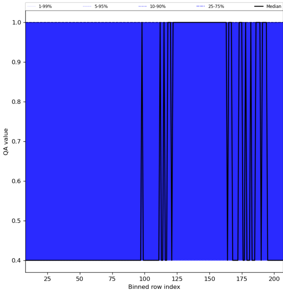
Figure 33: Along track statistics of “QA value” for 2024-04-27 to 2024-04-29
