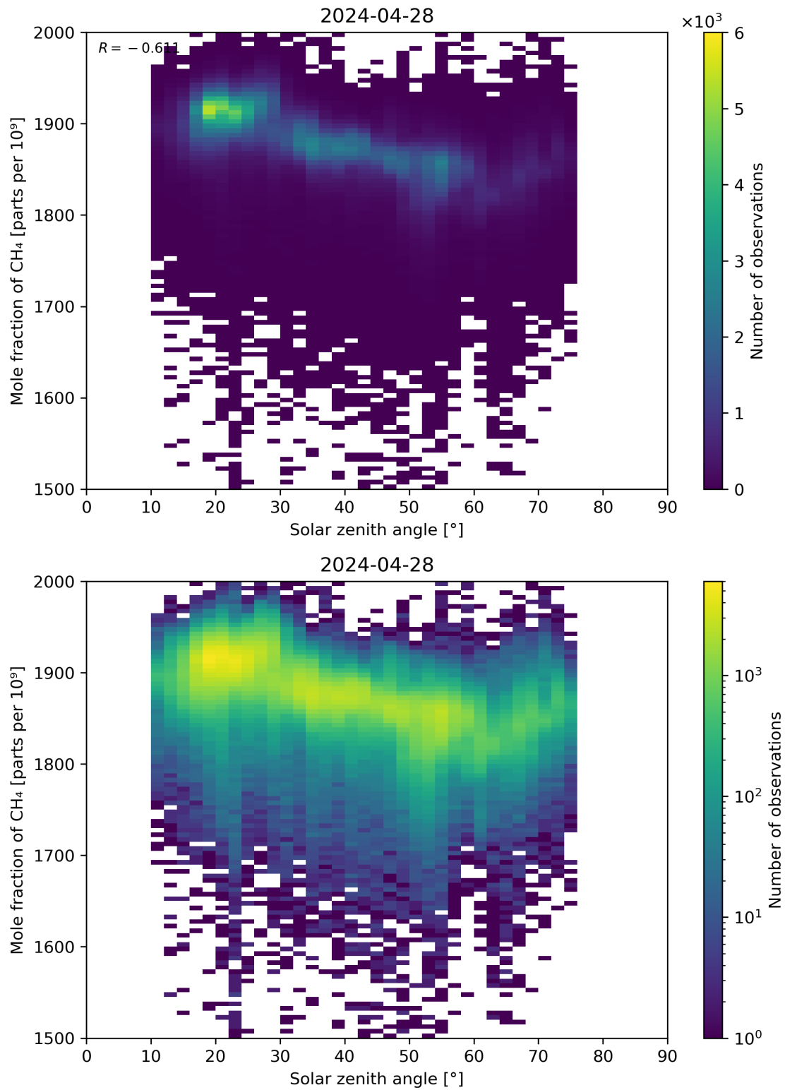
Figure 99: Scatter density plot of “Solar zenith angle” against “Mole fraction of CH 4 ” for 2024-04-27 to 2024-04-29.
