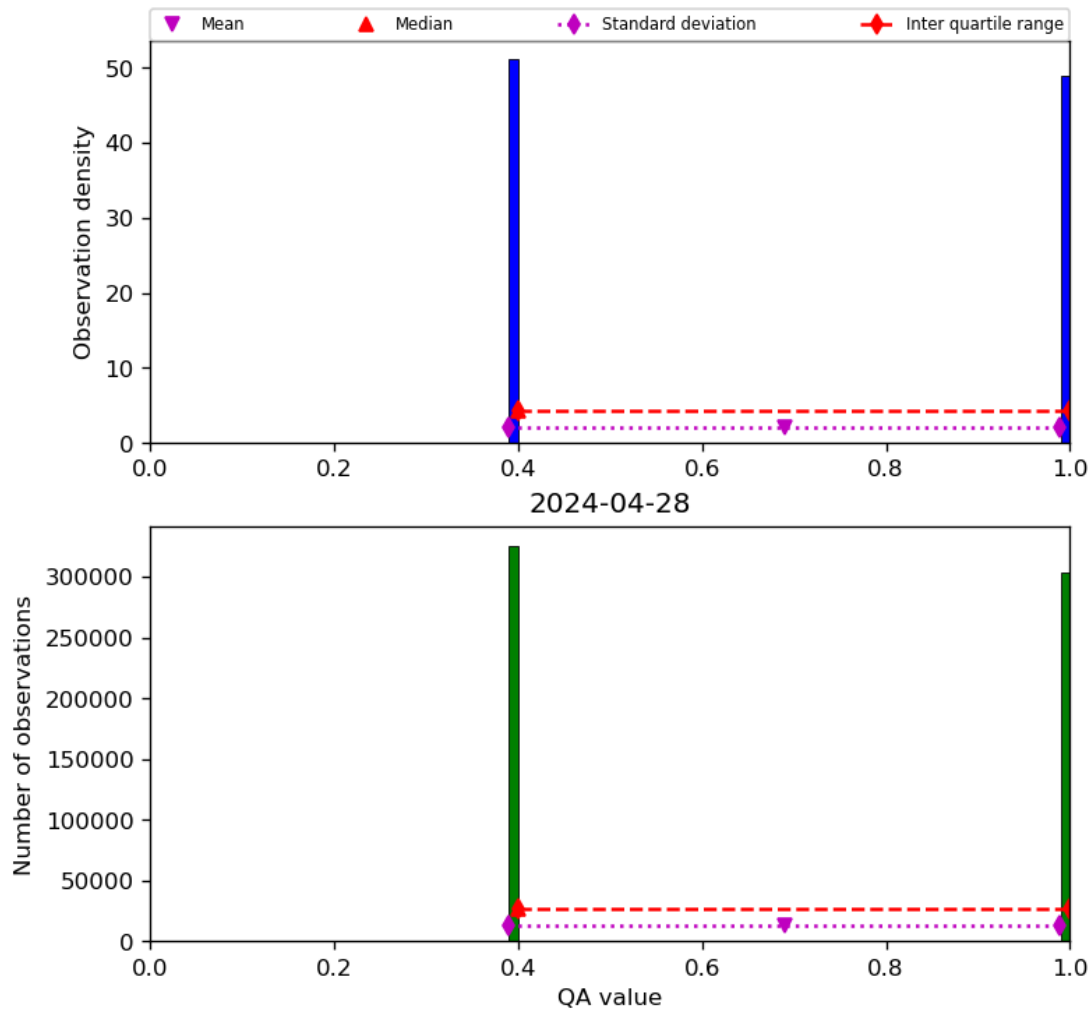
Figure 22: Histogram of “QA value” for 2024-04-27 to 2024-04-29
