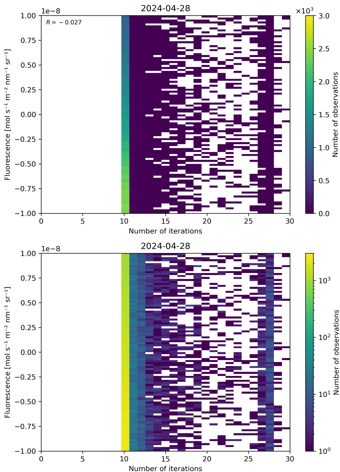
Figure 87: Scatter density plot of “Number of iterations” against “Fluorescence” for 2024-04-27 to 2024-04-29.
