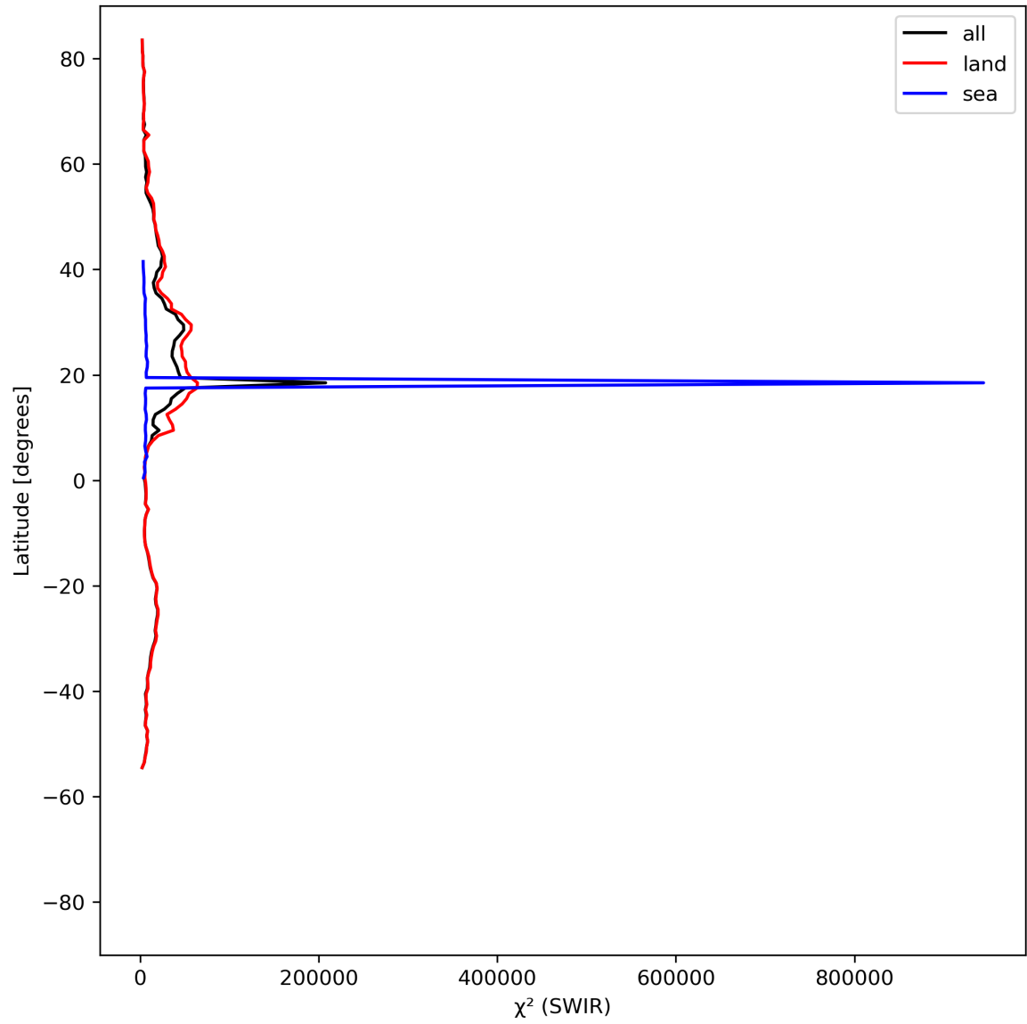
Figure 17: Zonal average of “ \chi^2 (SWIR)” for 2024-04-27 to 2024-04-29.
