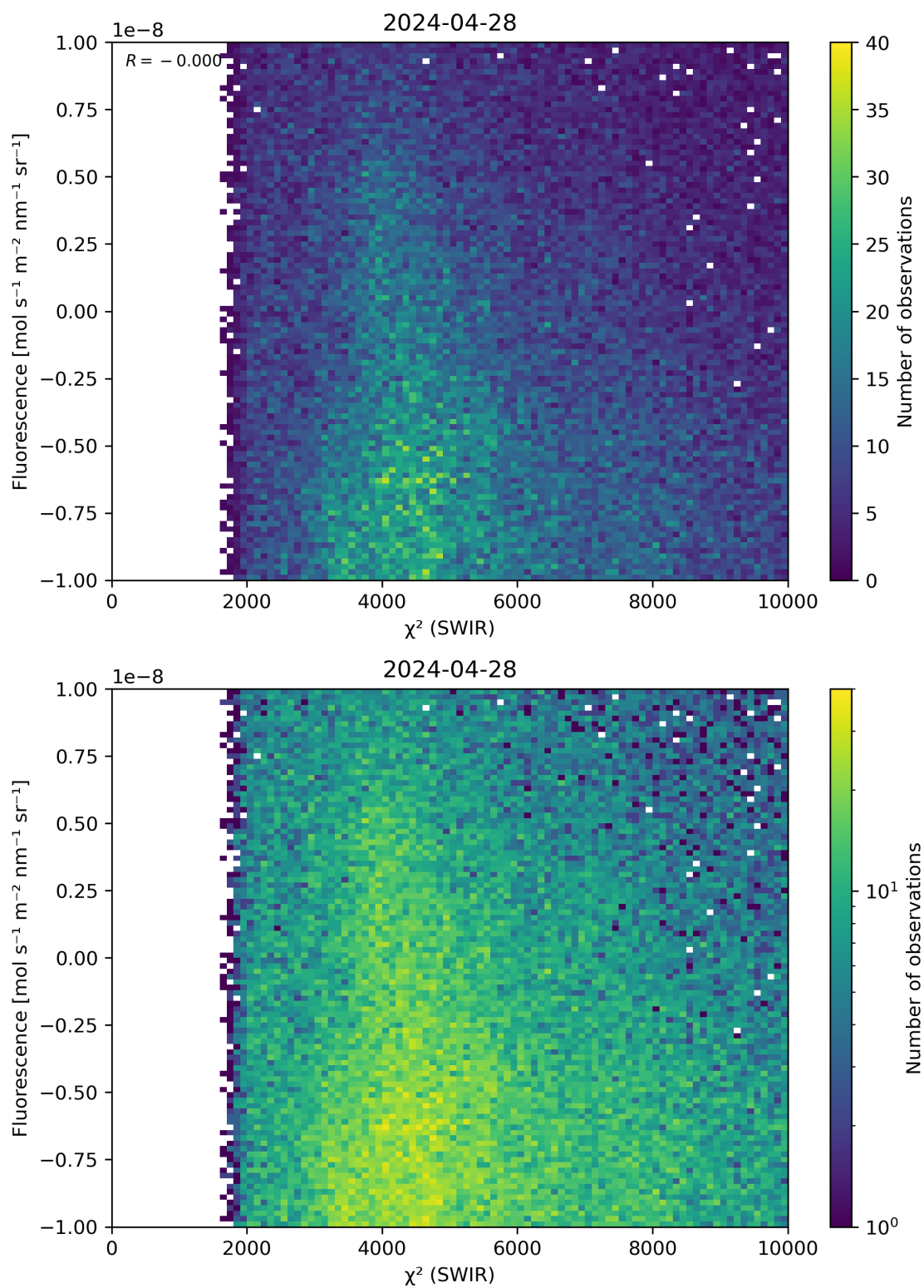
Figure 49: Scatter density plot of “ \chi^2 (SWIR)” against “Fluorescence” for 2024-04-27 to 2024-04-29.
