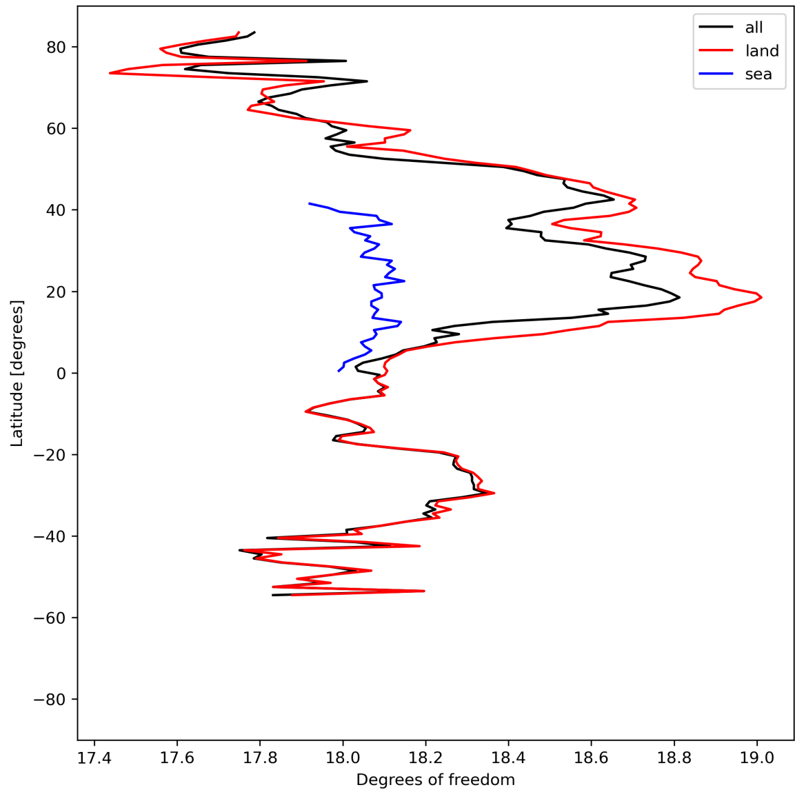
Figure 19: Zonal average of “Degrees of freedom” for 2024-04-27 to 2024-04-29.
