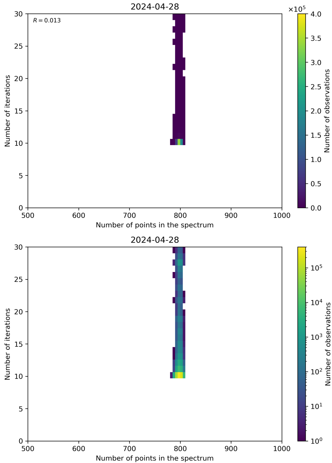
Figure 92: Scatter density plot of “Number of points in the spectrum” against “Number of iterations” for 2024-04-27 to 2024-04-29.
