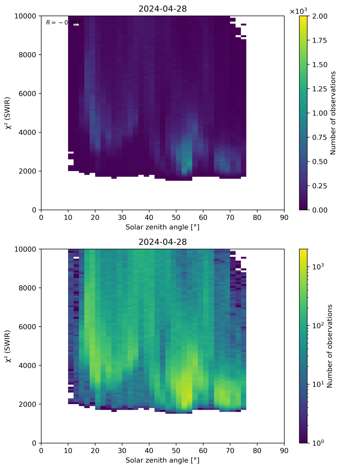
Figure 95: Scatter density plot of “Solar zenith angle” against “ \chi^2 (SWIR)” for 2024-04-27 to 2024-04-29.
