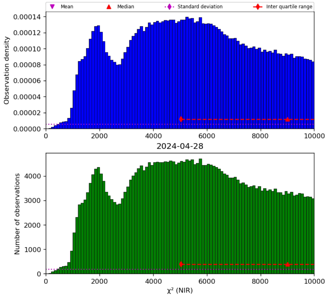
Figure 29: Histogram of “ \chi^2 (NIR)” for 2024-04-27 to 2024-04-29
