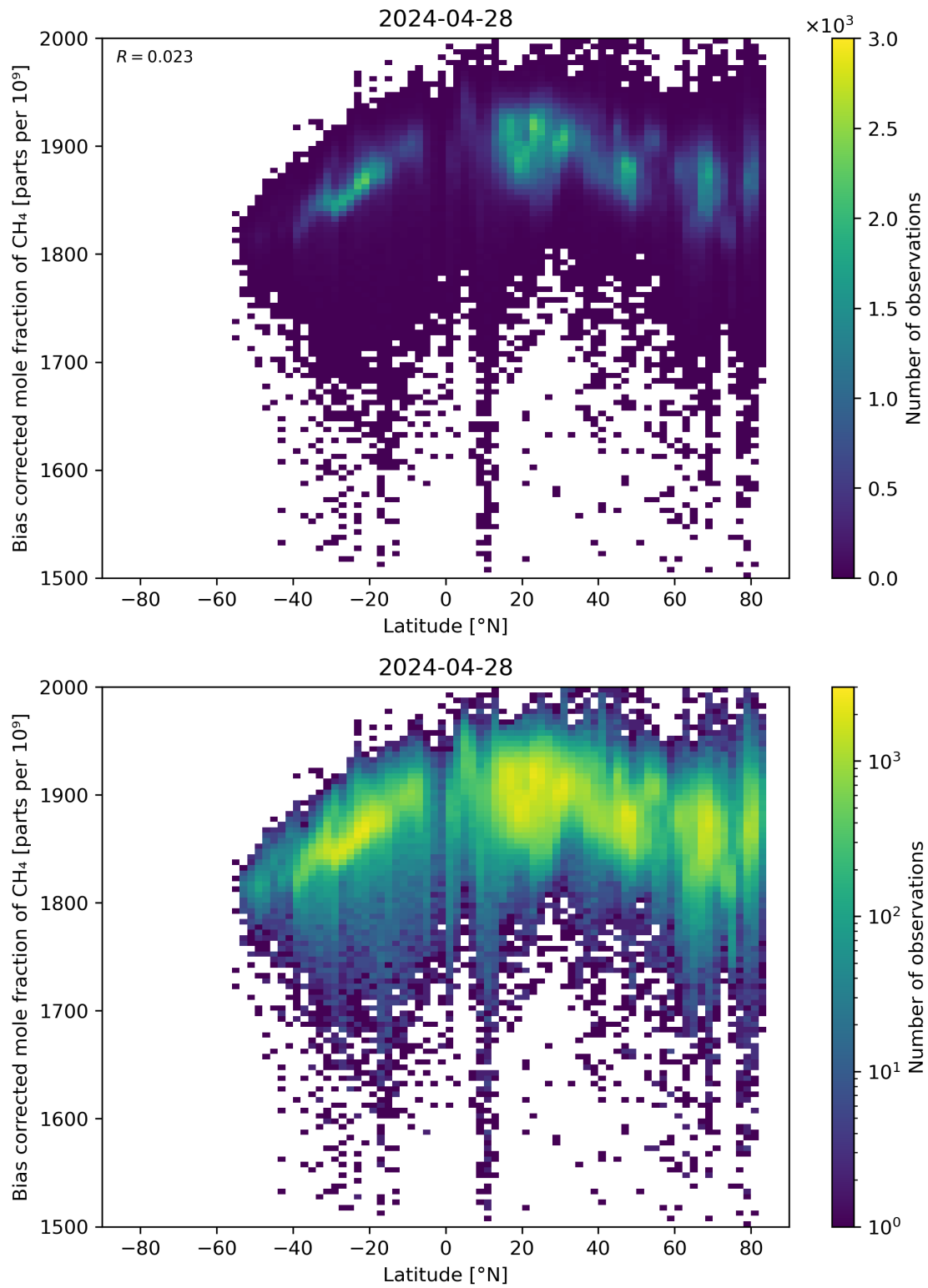
Figure 58: Scatter density plot of “Latitude” against “Bias corrected mole fraction of CH 4 ” for 2024-04-27 to 2024-04-29.
