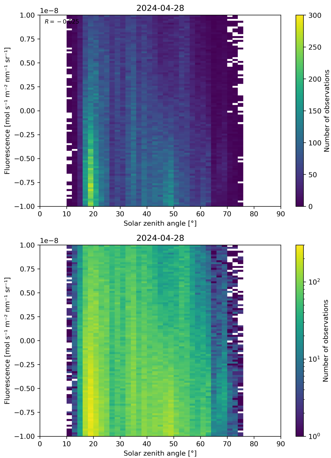
Figure 97: Scatter density plot of “Solar zenith angle” against “Fluorescence” for 2024-04-27 to 2024-04-29.
