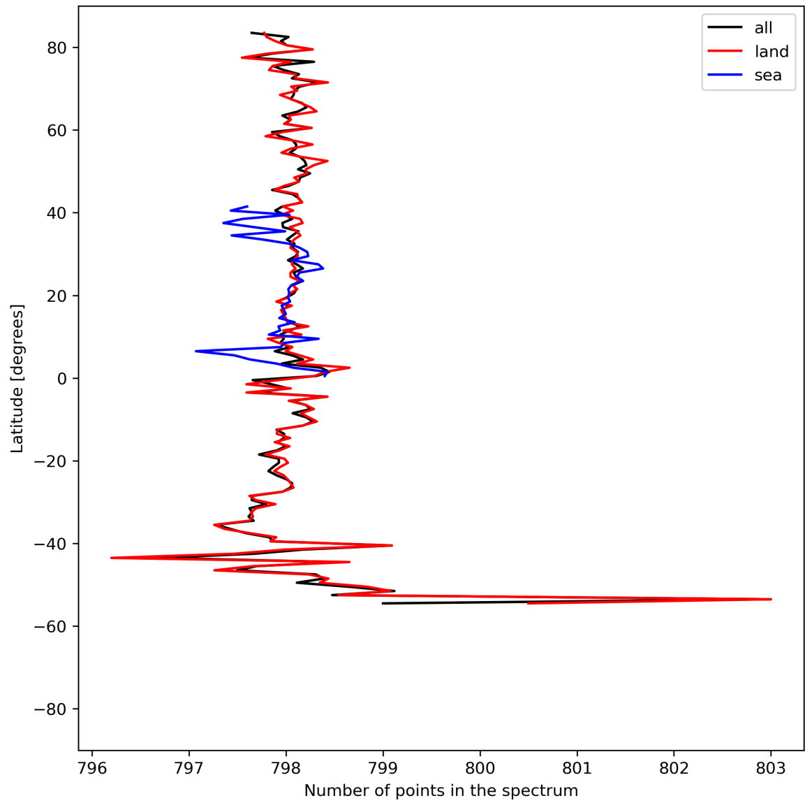
Figure 15: Zonal average of “Number of points in the spectrum” for 2024-04-27 to 2024-04-29.
