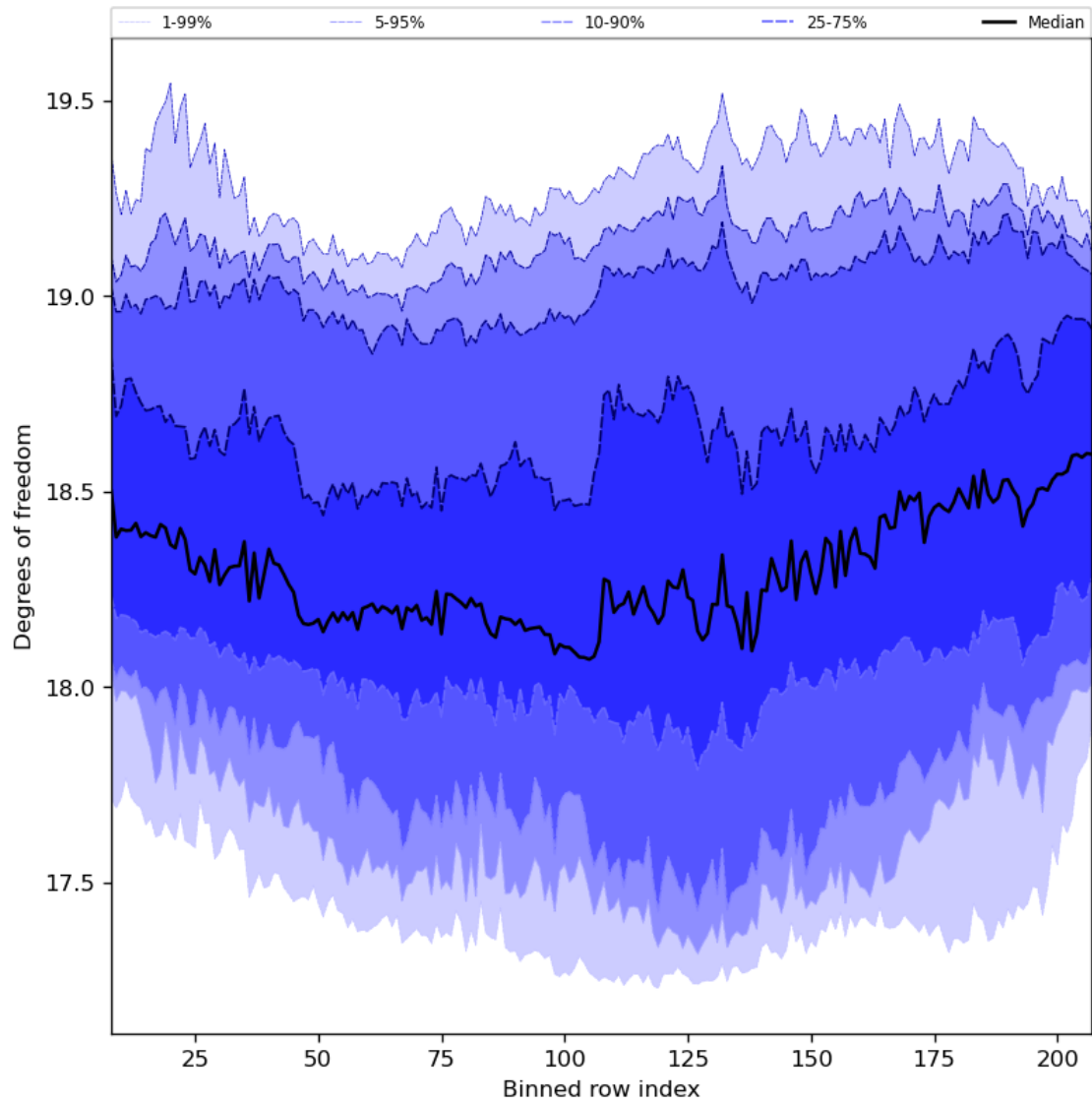
Figure 41: Along track statistics of “Degrees of freedom” for 2024-04-27 to 2024-04-29
