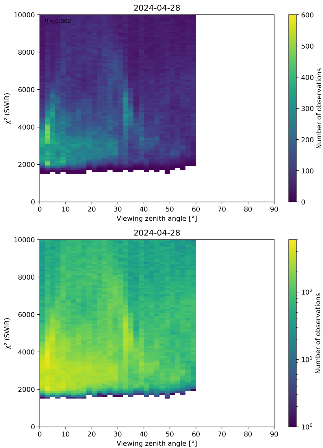
Figure 106: Scatter density plot of “Viewing zenith angle” against “ \chi^2 (SWIR)” for 2024-04-27 to 2024-04-29.
