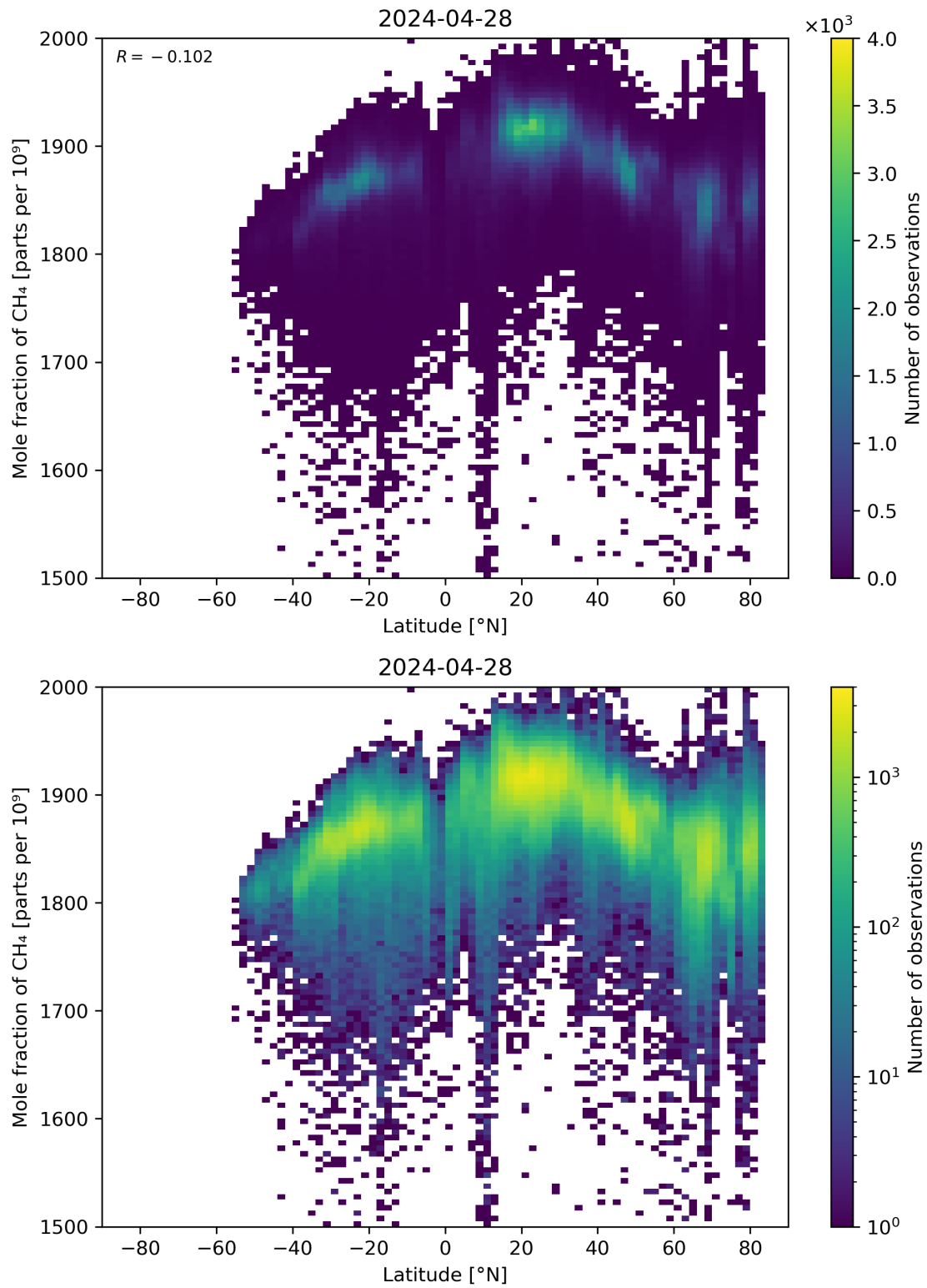
Figure 57: Scatter density plot of “Latitude” against “Mole fraction of \text{CH}_4 ” for 2024-04-27 to 2024-04-29.
