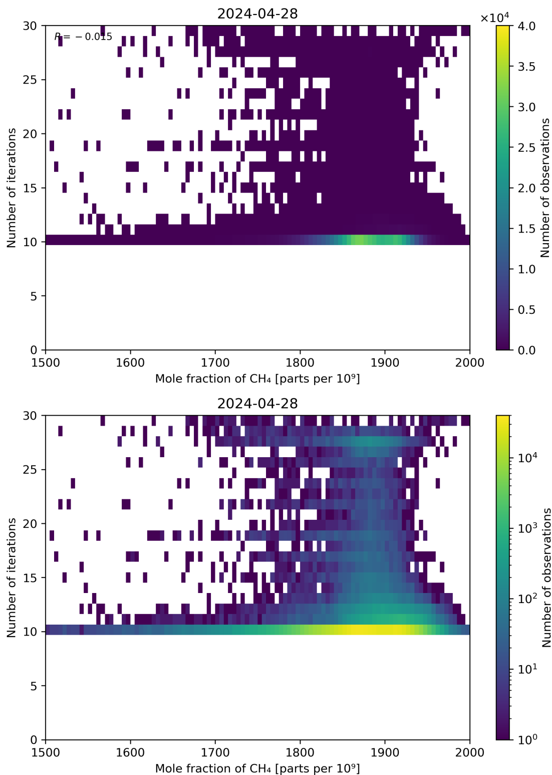
Figure 76: Scatter density plot of “Mole fraction of CH 4 ” against “Number of iterations” for 2024-04-27 to 2024-04-29.
