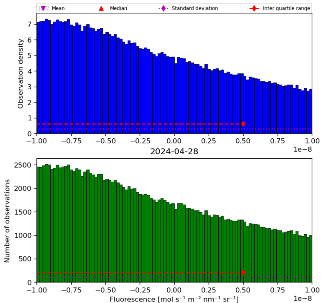
Figure 32: Histogram of “Fluorescence” for 2024-04-27 to 2024-04-29
