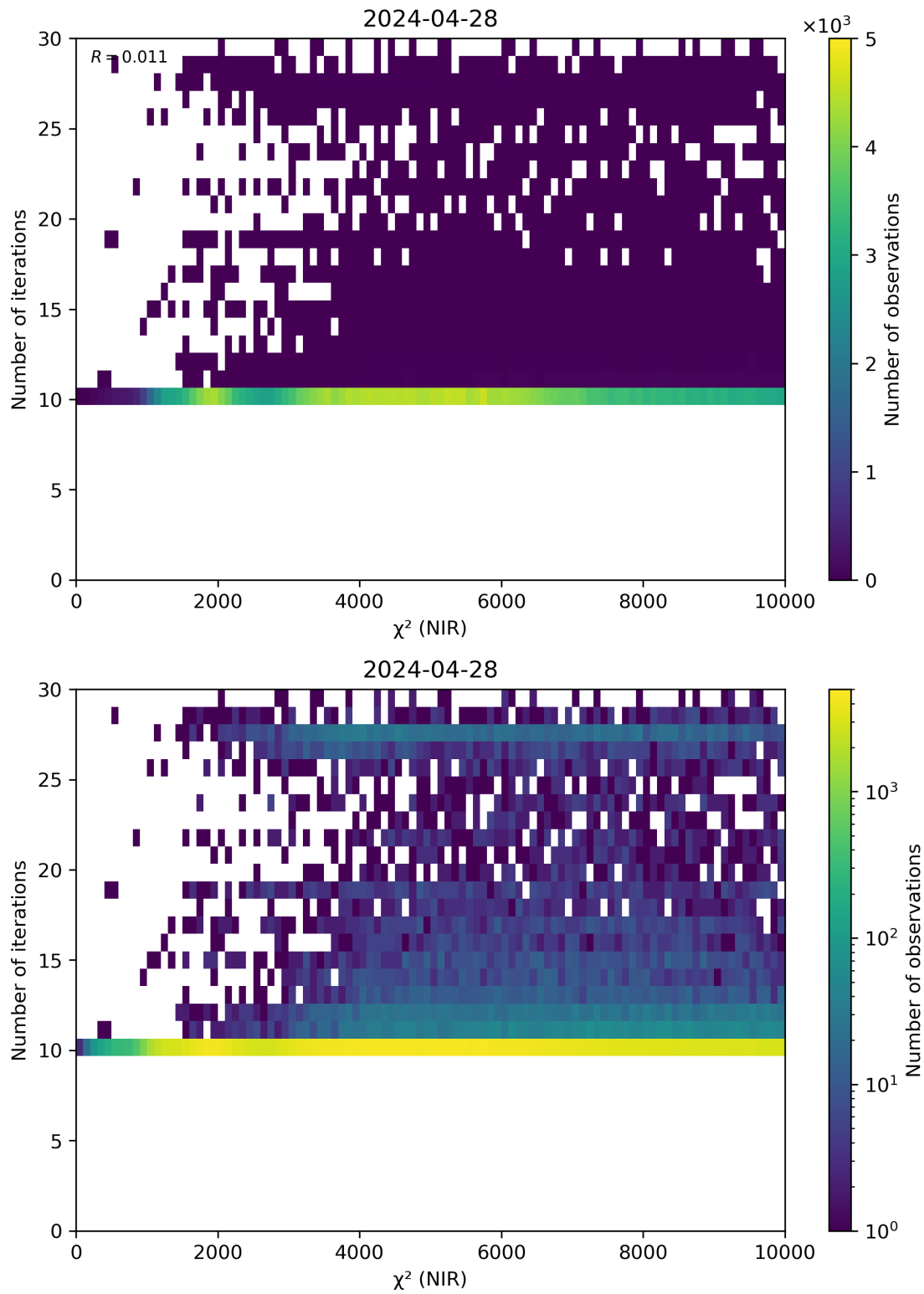
Figure 46: Scatter density plot of “ \chi^2 (NIR)” against “Number of iterations” for 2024-04-27 to 2024-04-29.
