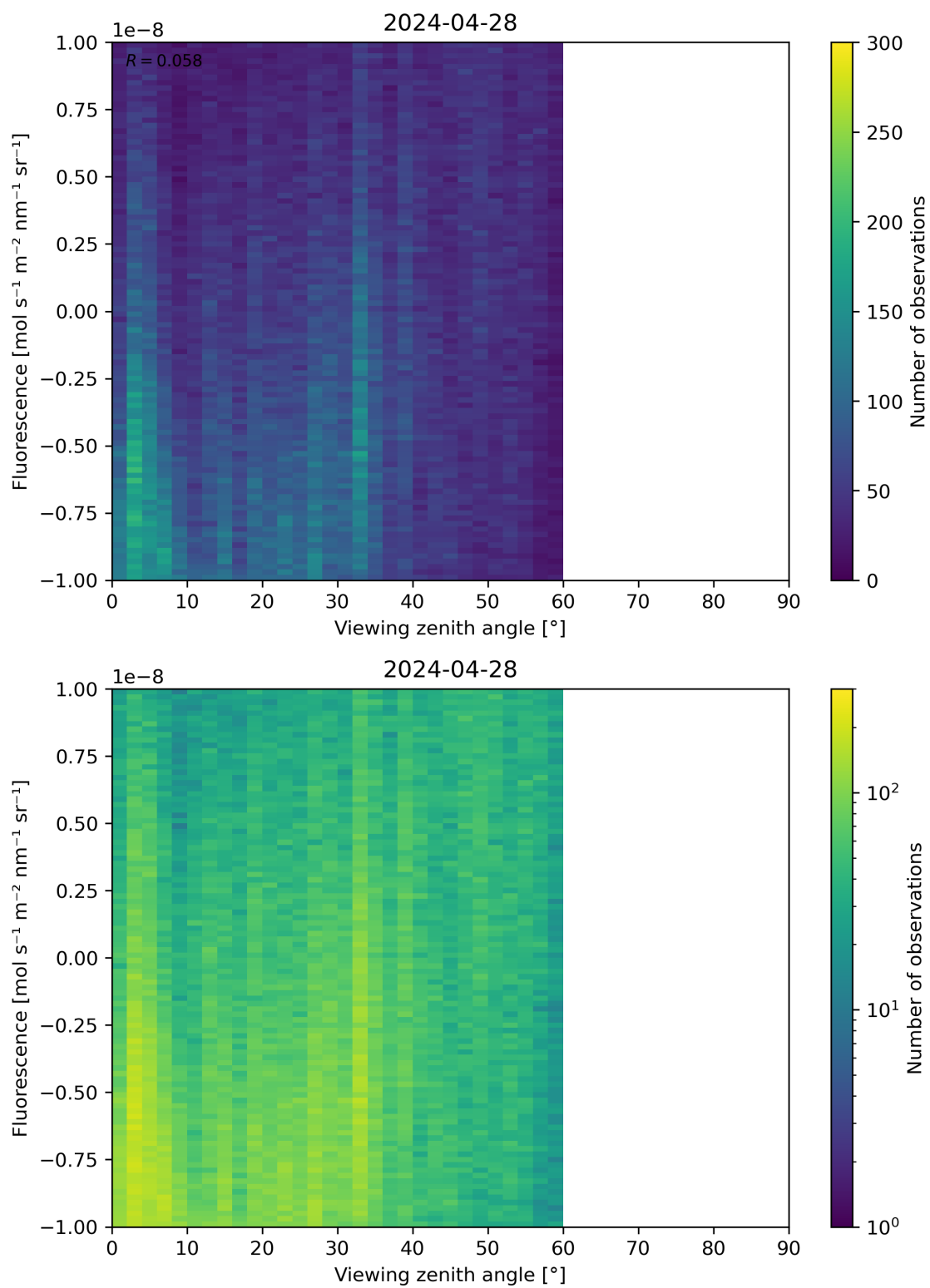
Figure 108: Scatter density plot of “Viewing zenith angle” against “Fluorescence” for 2024-04-27 to 2024-04-29.
