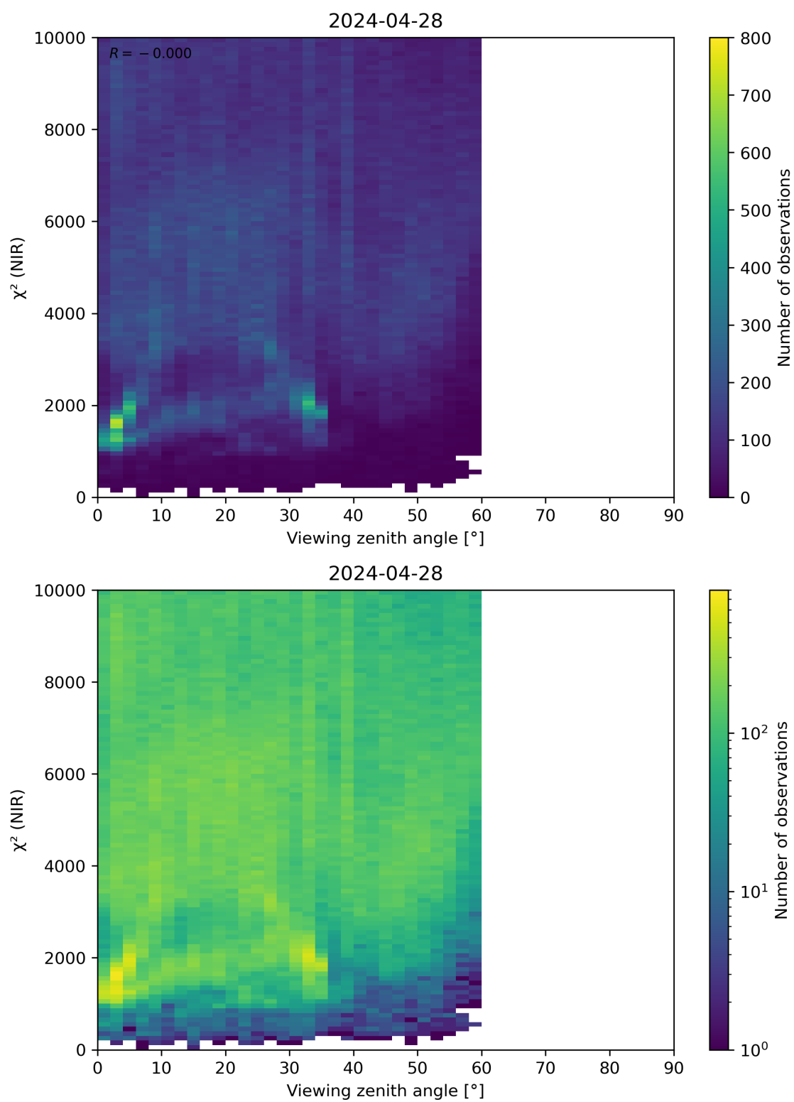
Figure 105: Scatter density plot of “Viewing zenith angle” against “ \chi^2 (NIR)” for 2024-04-27 to 2024-04-29.
