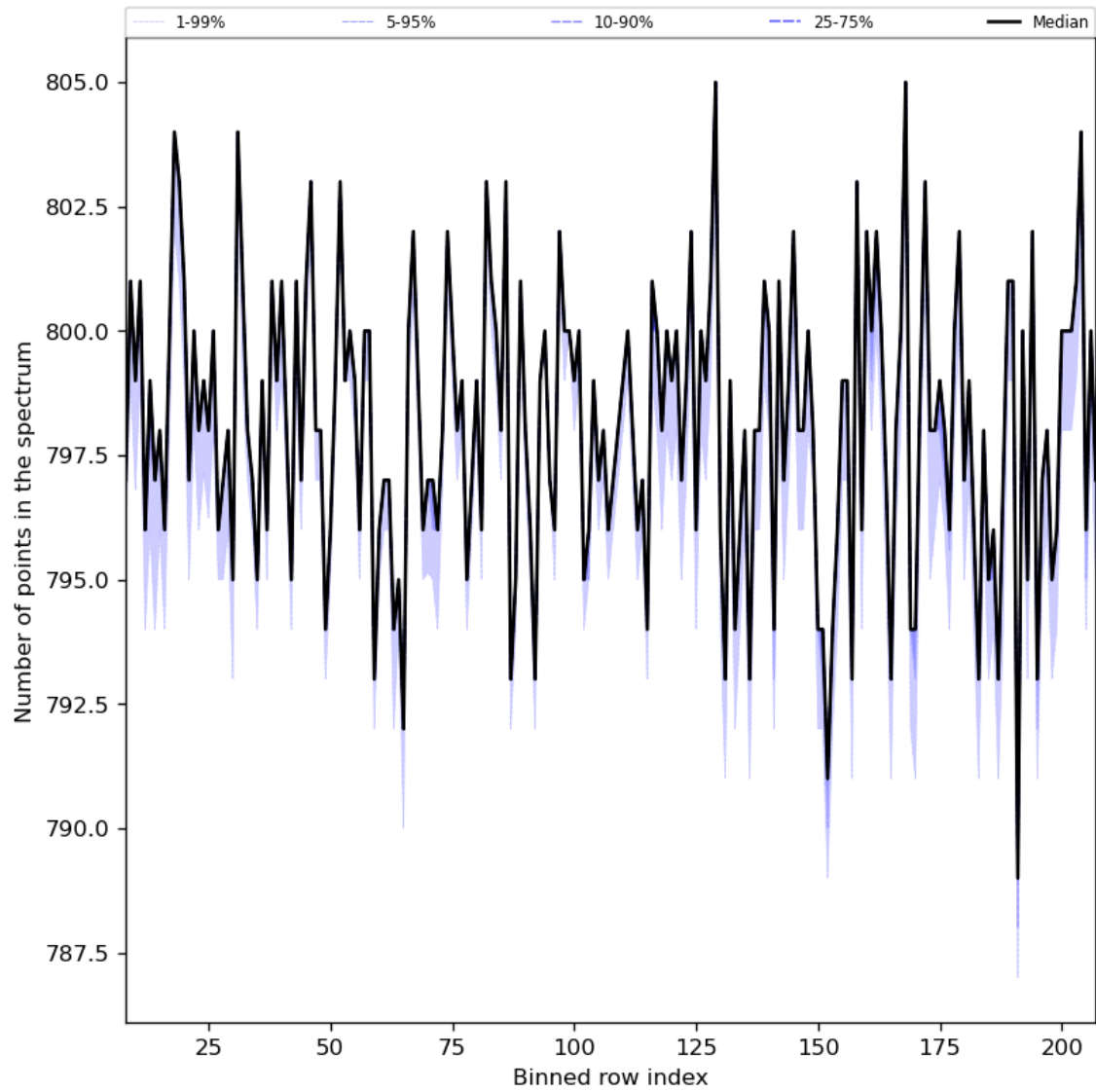
Figure 37: Along track statistics of “Number of points in the spectrum” for 2024-04-27 to 2024-04-29
