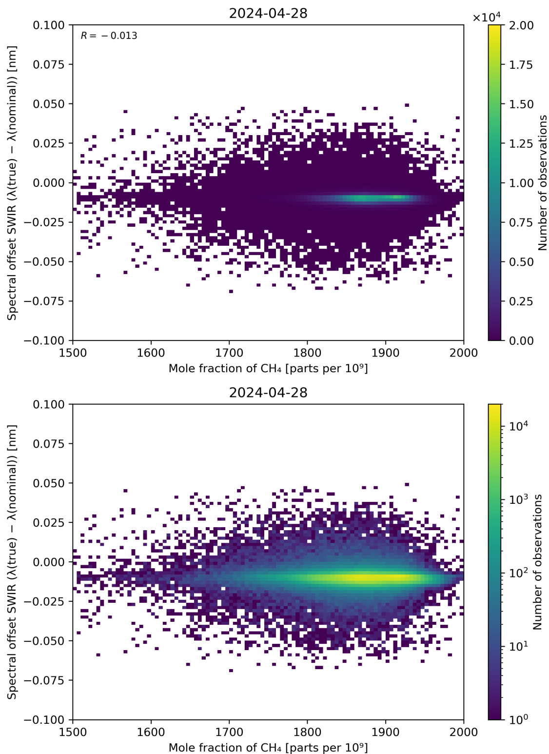
Figure 86: Scatter density plot of “Mole fraction of CH 4 ” against “Spectral offset SWIR ( \lambda(\text{true}) - \lambda(\text{nominal}) )” for 2024-04-27 to 2024-04-29.
