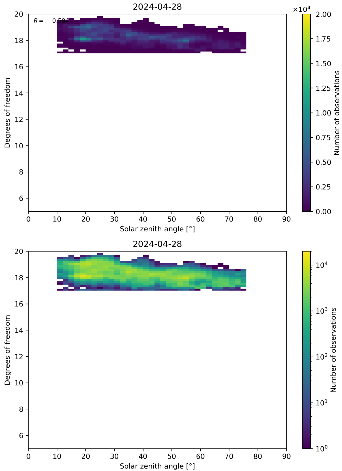
Figure 96: Scatter density plot of “Solar zenith angle” against “Degrees of freedom” for 2024-04-27 to 2024-04-29.
