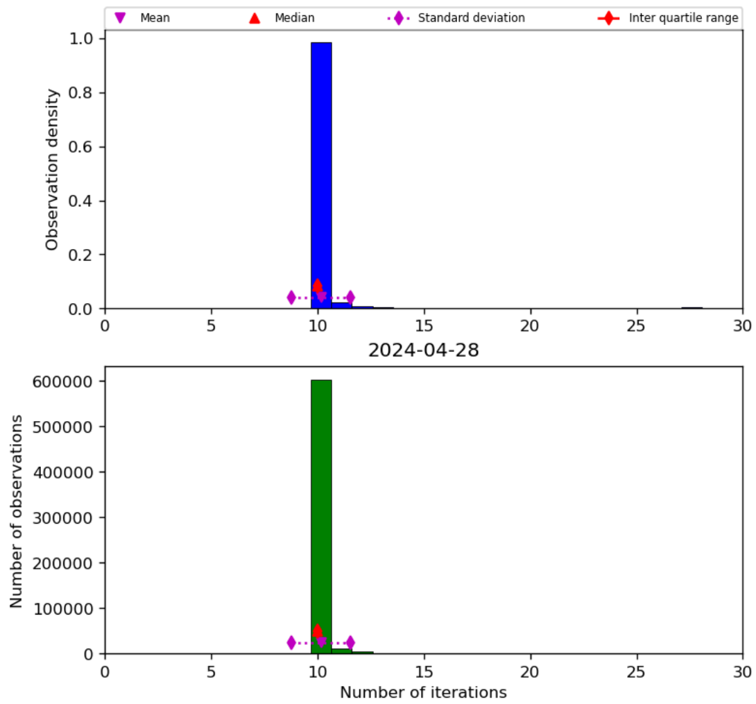
Figure 31: Histogram of “Number of iterations” for 2024-04-27 to 2024-04-29
