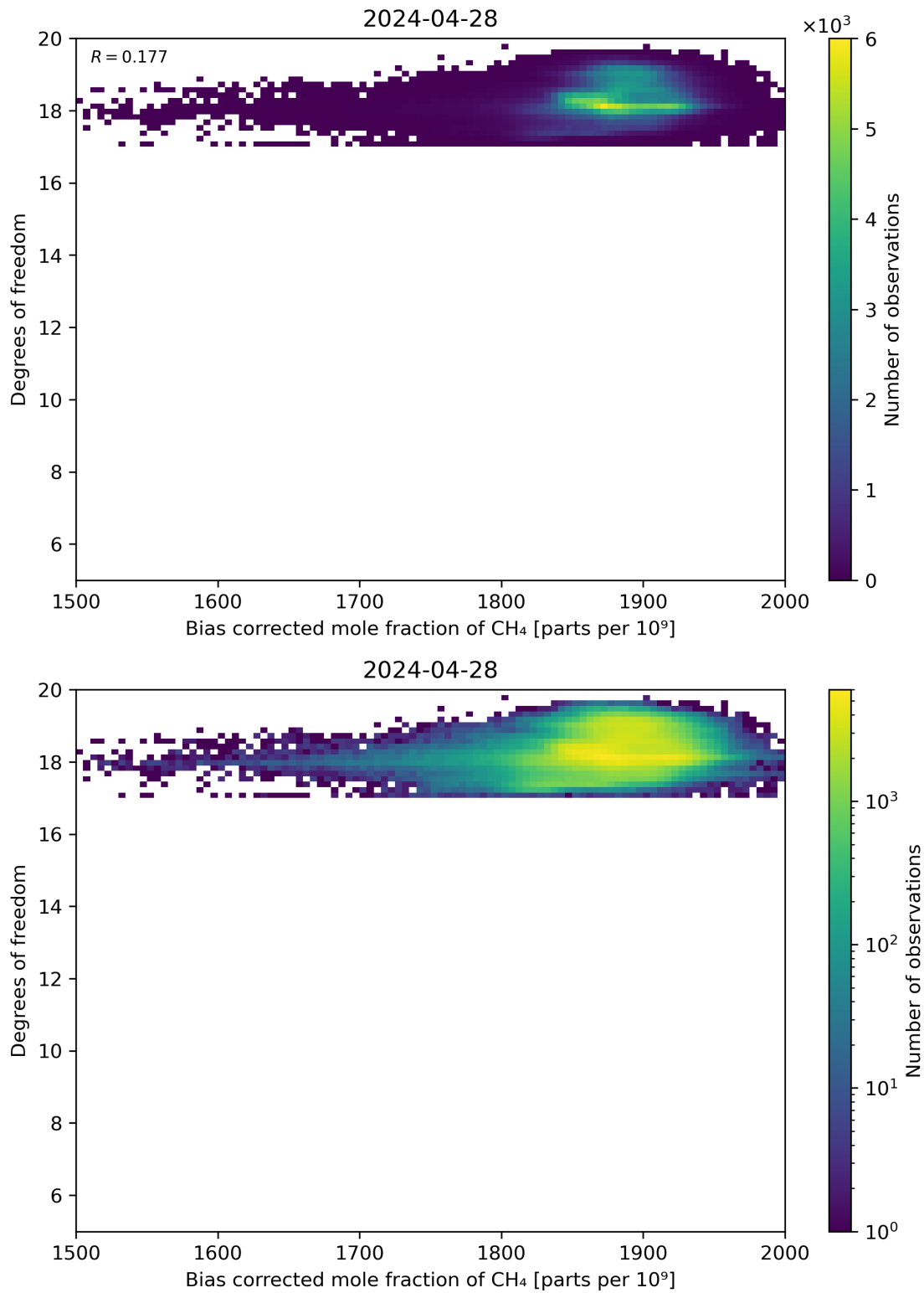
Figure 65: Scatter density plot of “Bias corrected mole fraction of CH 4 ” against “Degrees of freedom” for 2024-04-27 to 2024-04-29.
