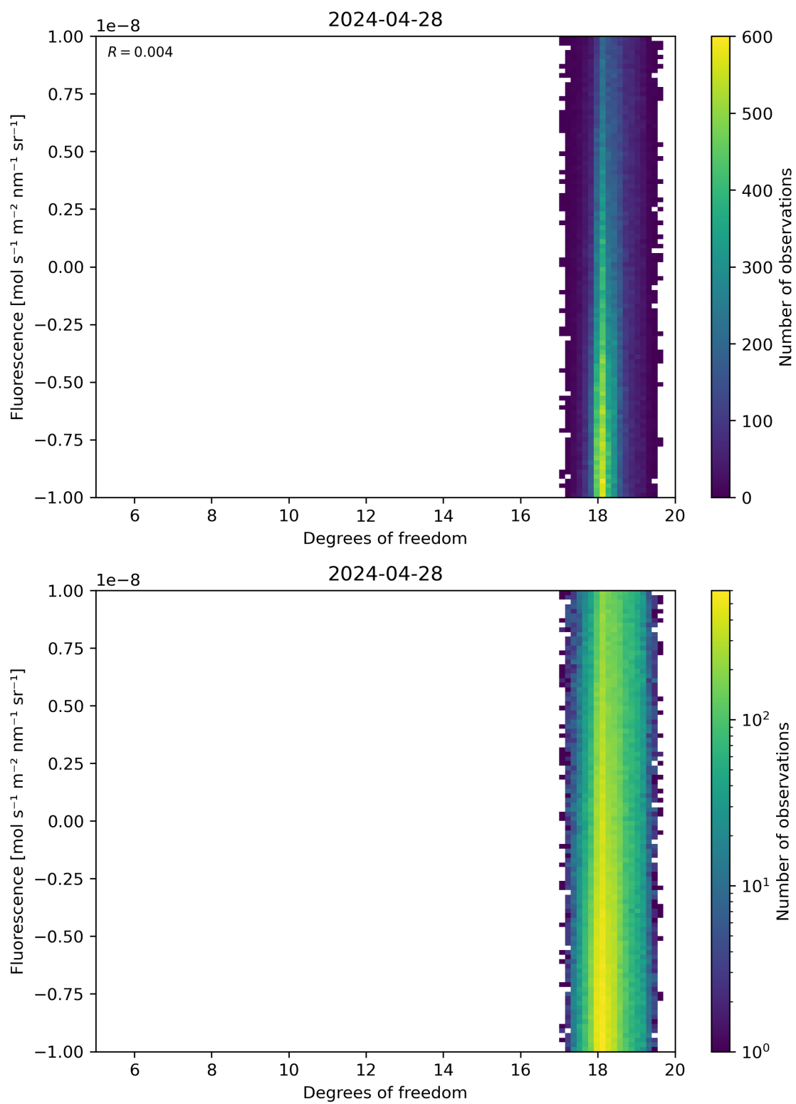
Figure 51: Scatter density plot of “Degrees of freedom” against “Fluorescence” for 2024-04-27 to 2024-04-29.
