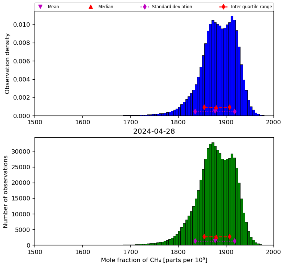
Figure 23: Histogram of “Mole fraction of CH 4 ” for 2024-04-27 to 2024-04-29
