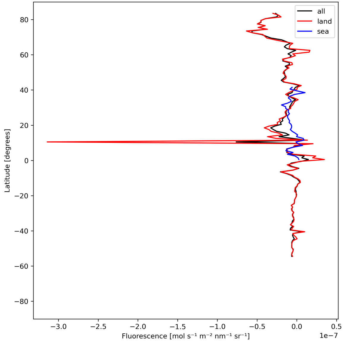
Figure 21: Zonal average of “Fluorescence” for 2024-04-27 to 2024-04-29.
