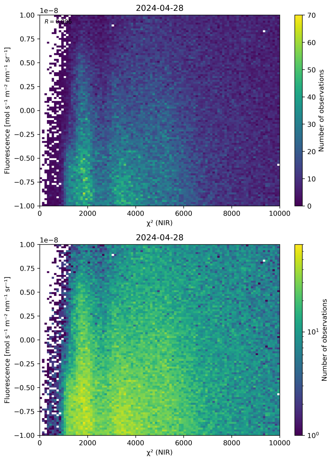
Figure 45: Scatter density plot of “ \chi^2 (NIR)” against “Fluorescence” for 2024-04-27 to 2024-04-29.
