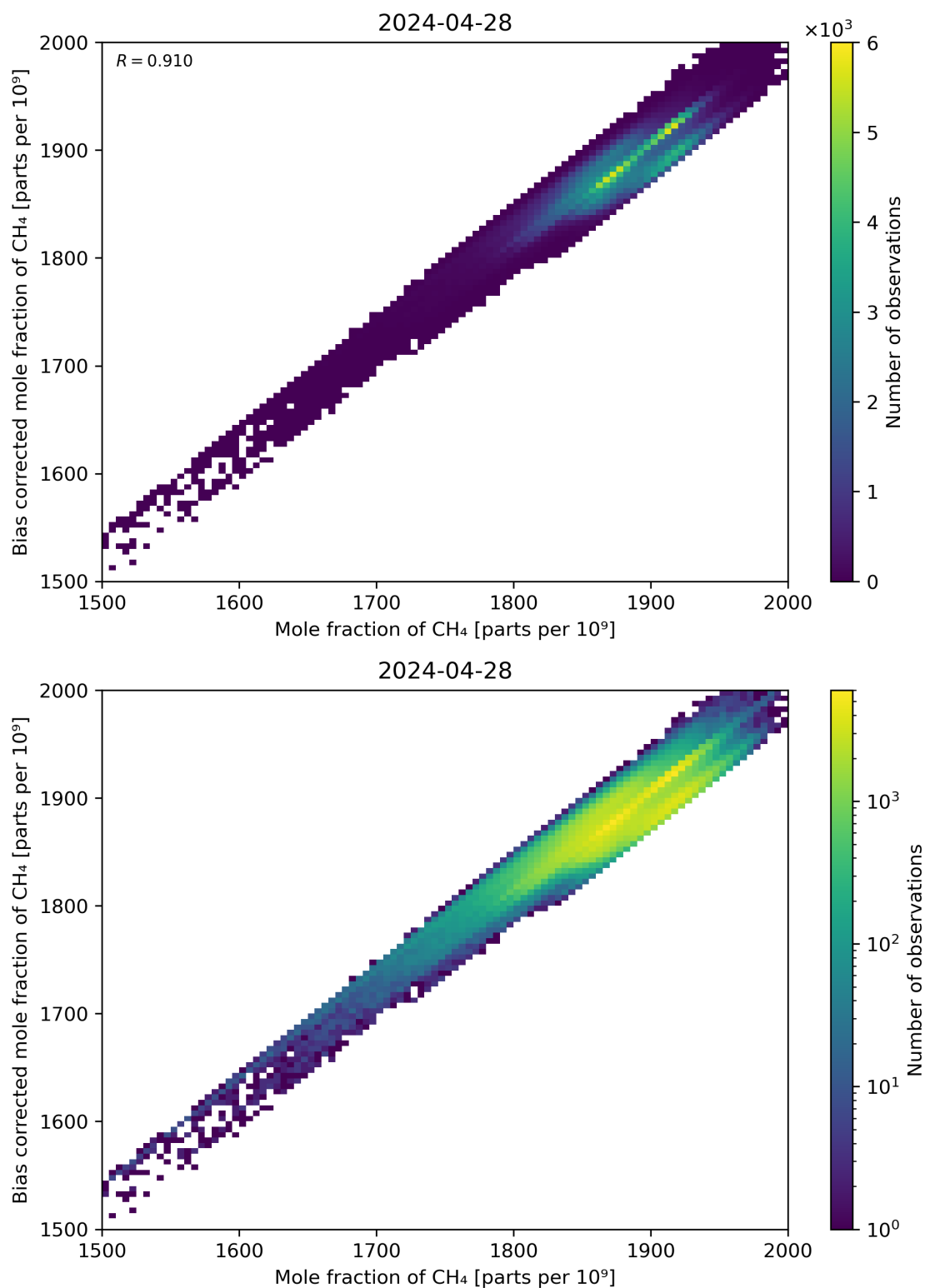
Figure 74: Scatter density plot of “Mole fraction of CH 4 ” against “Bias corrected mole fraction of CH 4 ” for 2024-04-27 to 2024-04-29.
