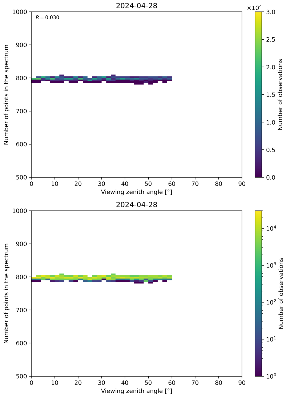
Figure 114: Scatter density plot of “Viewing zenith angle” against “Number of points in the spectrum” for 2024-04-27 to 2024-04-29.
