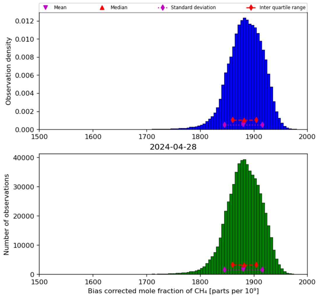
Figure 25: Histogram of “Bias corrected mole fraction of CH 4 ” for 2024-04-27 to 2024-04-29
