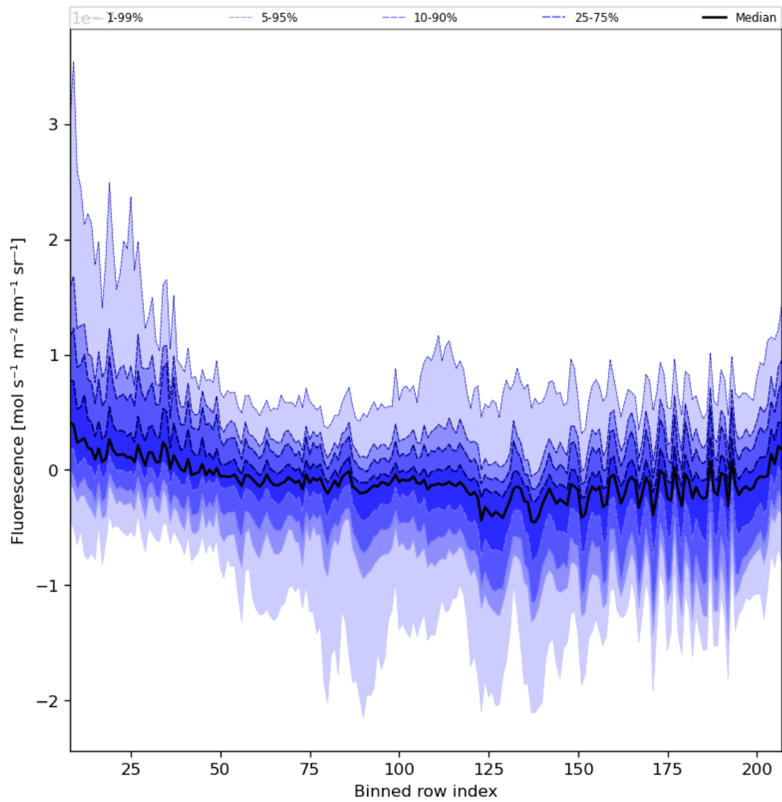
Figure 43: Along track statistics of “Fluorescence” for 2024-04-27 to 2024-04-29
