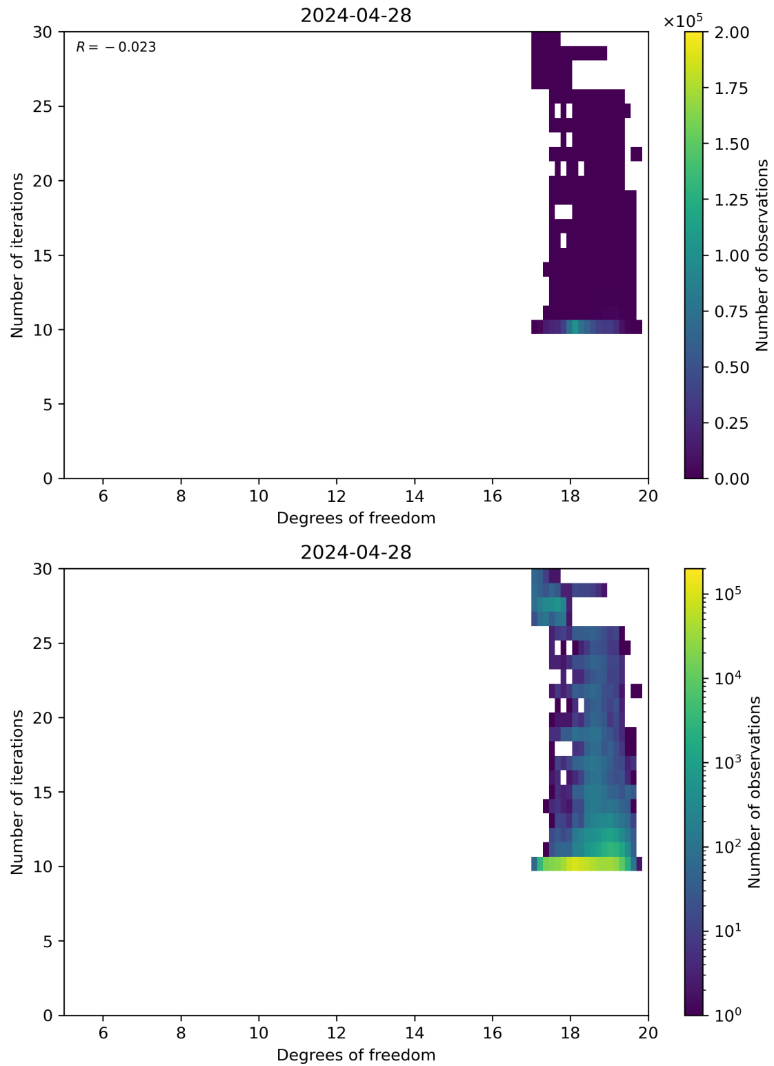
Figure 52: Scatter density plot of “Degrees of freedom” against “Number of iterations” for 2024-04-27 to 2024-04-29.
