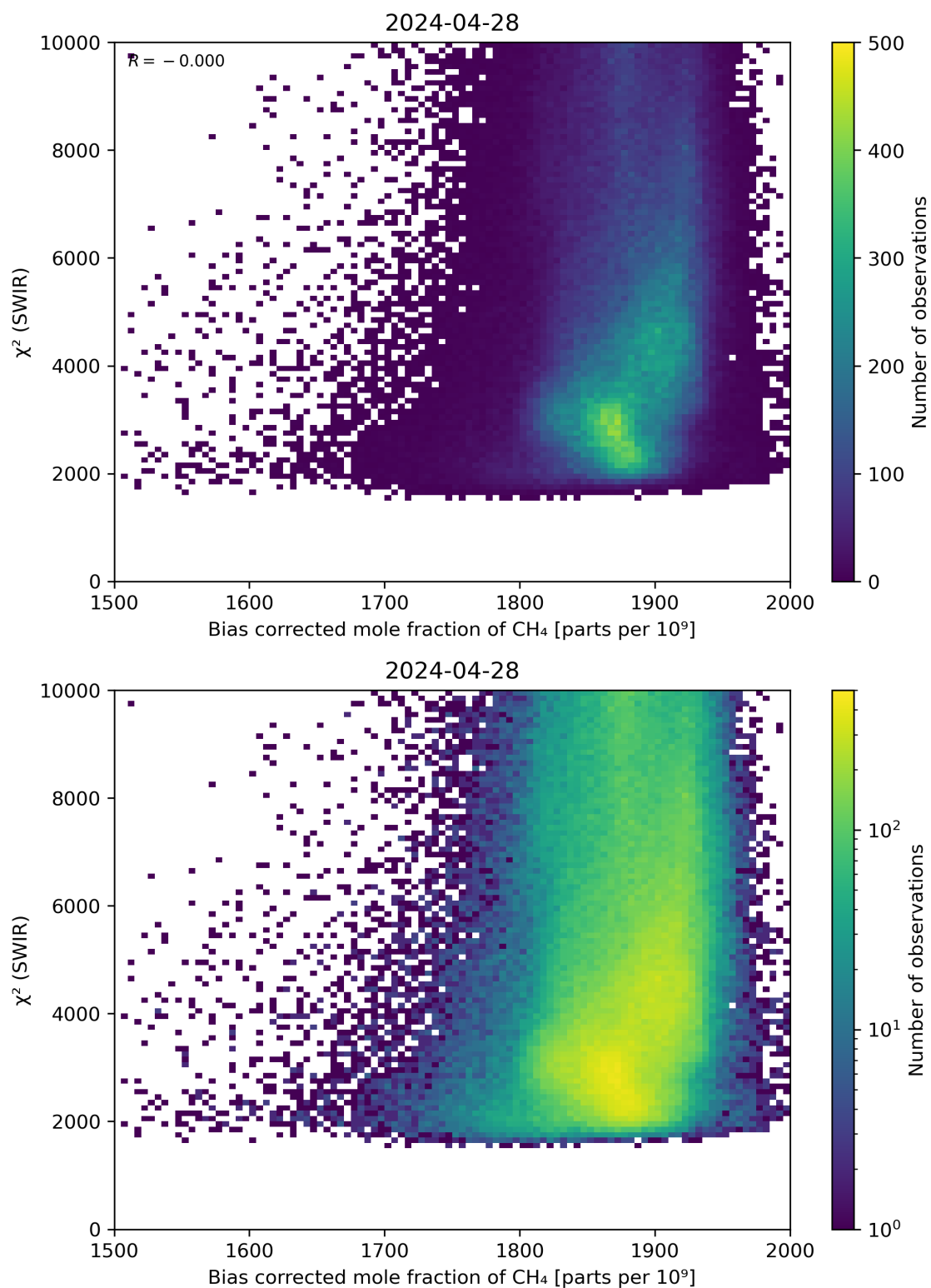
Figure 64: Scatter density plot of “Bias corrected mole fraction of CH 4 ” against “ \chi^2 (SWIR)” for 2024-04-27 to 2024-04-29.
