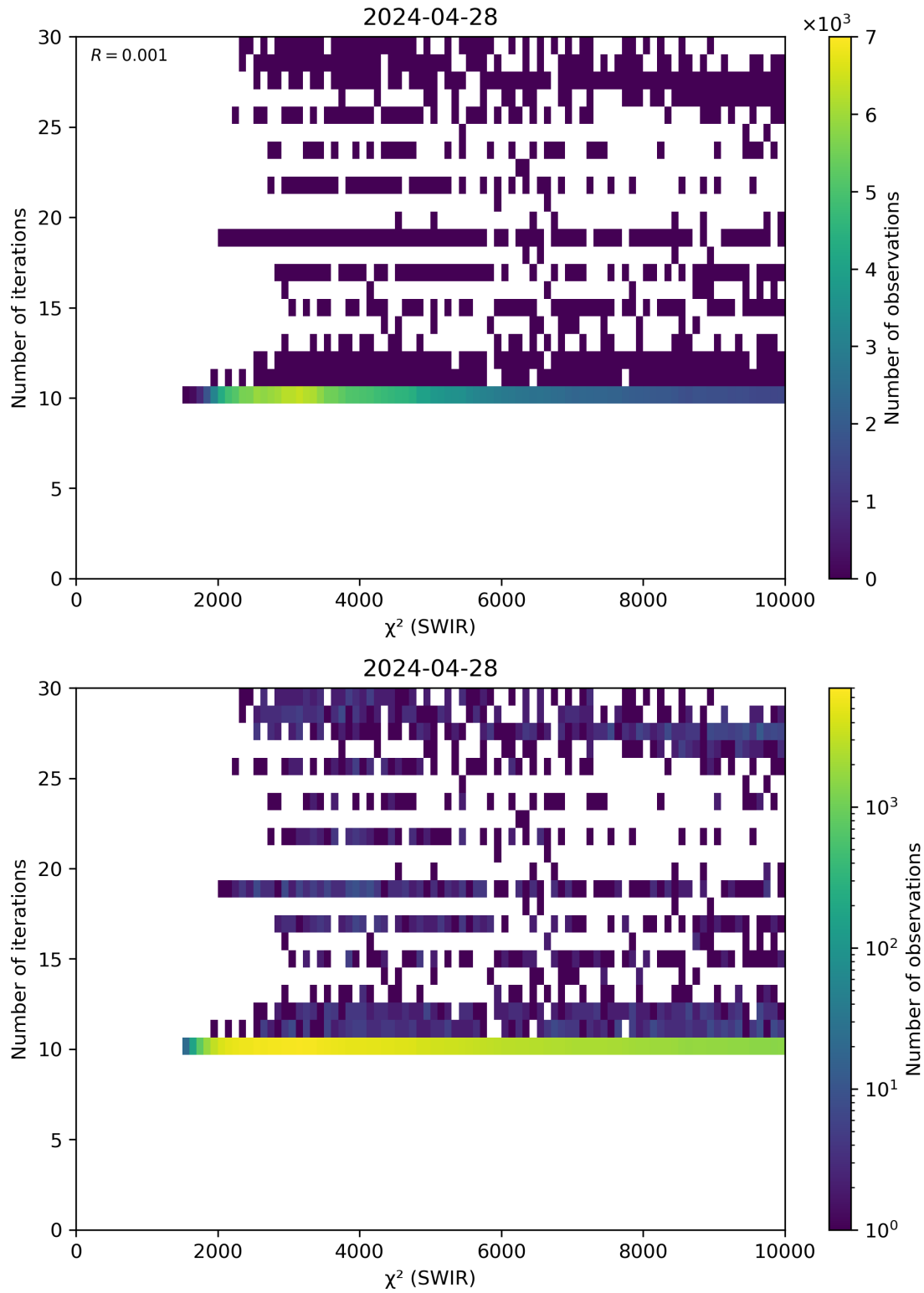
Figure 50: Scatter density plot of “ \chi^2 (SWIR)” against “Number of iterations” for 2024-04-27 to 2024-04-29.
