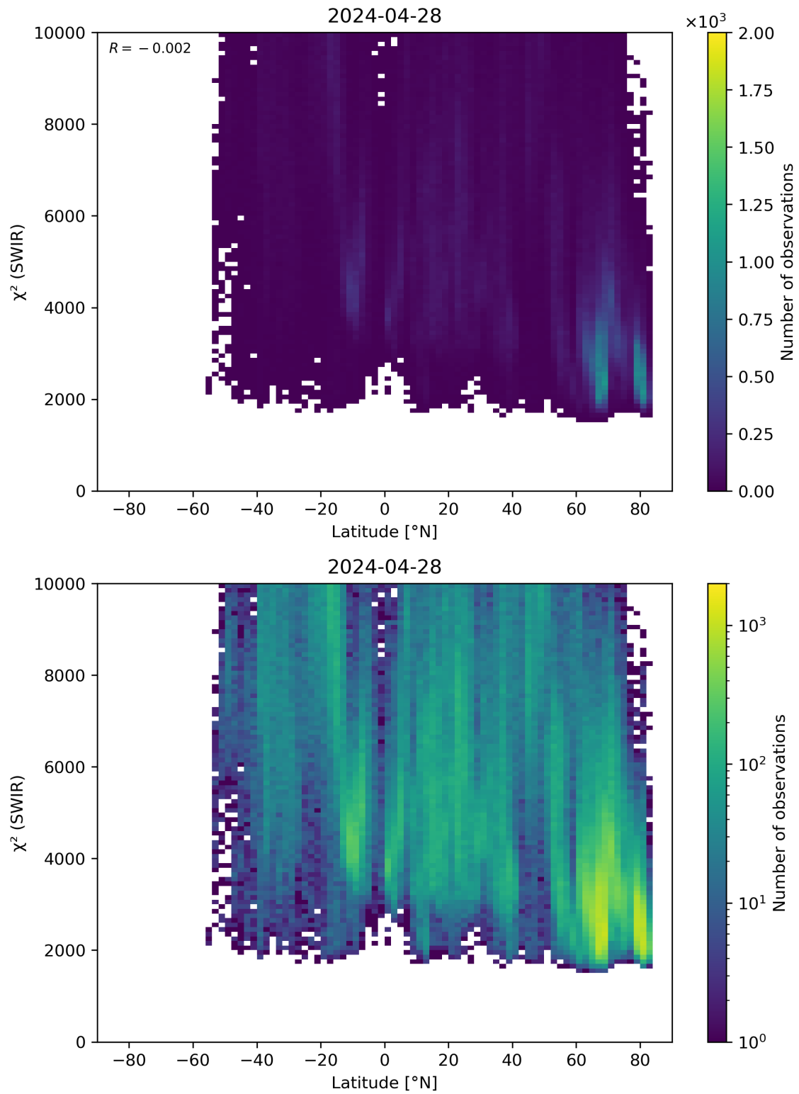
Figure 54: Scatter density plot of “Latitude” against “ \chi^2 (SWIR)” for 2024-04-27 to 2024-04-29.
