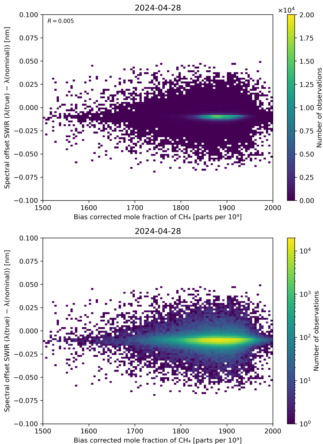
Figure 69: Scatter density plot of “Bias corrected mole fraction of \text{CH}_4 ” against “Spectral offset SWIR ( \lambda(\text{true}) - \lambda(\text{nominal}) )” for 2024-04-27 to 2024-04-29.
