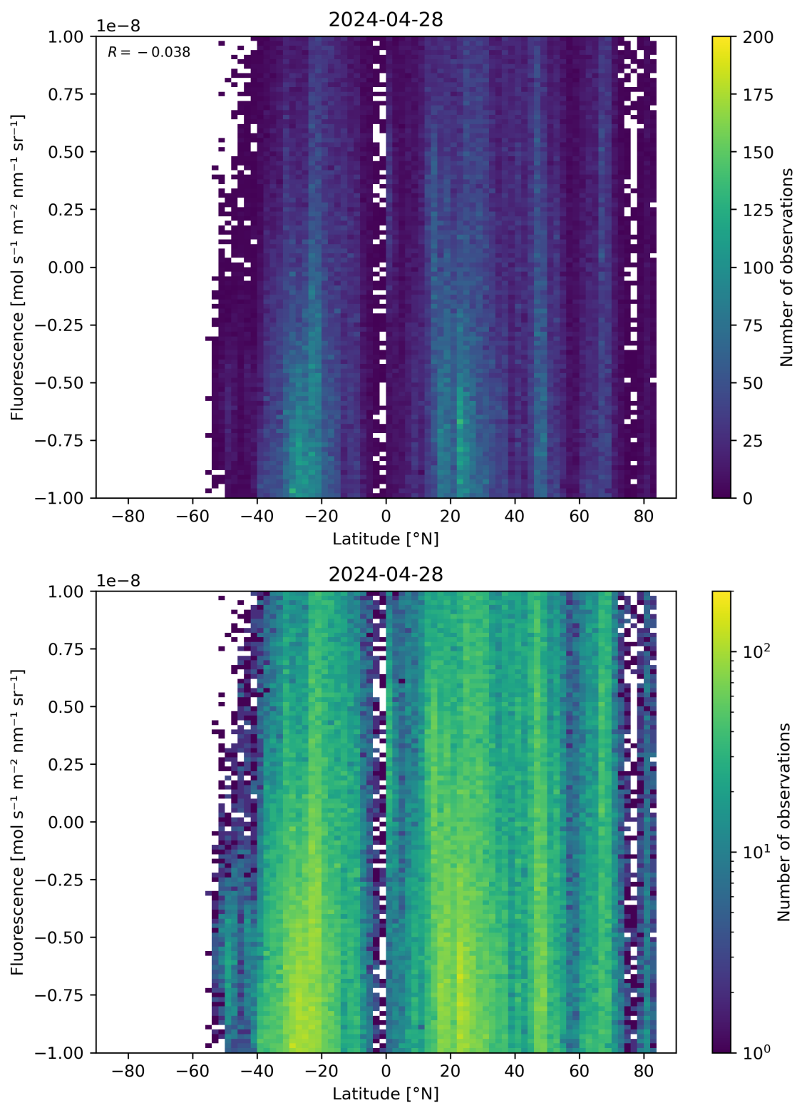
Figure 56: Scatter density plot of “Latitude” against “Fluorescence” for 2024-04-27 to 2024-04-29.
