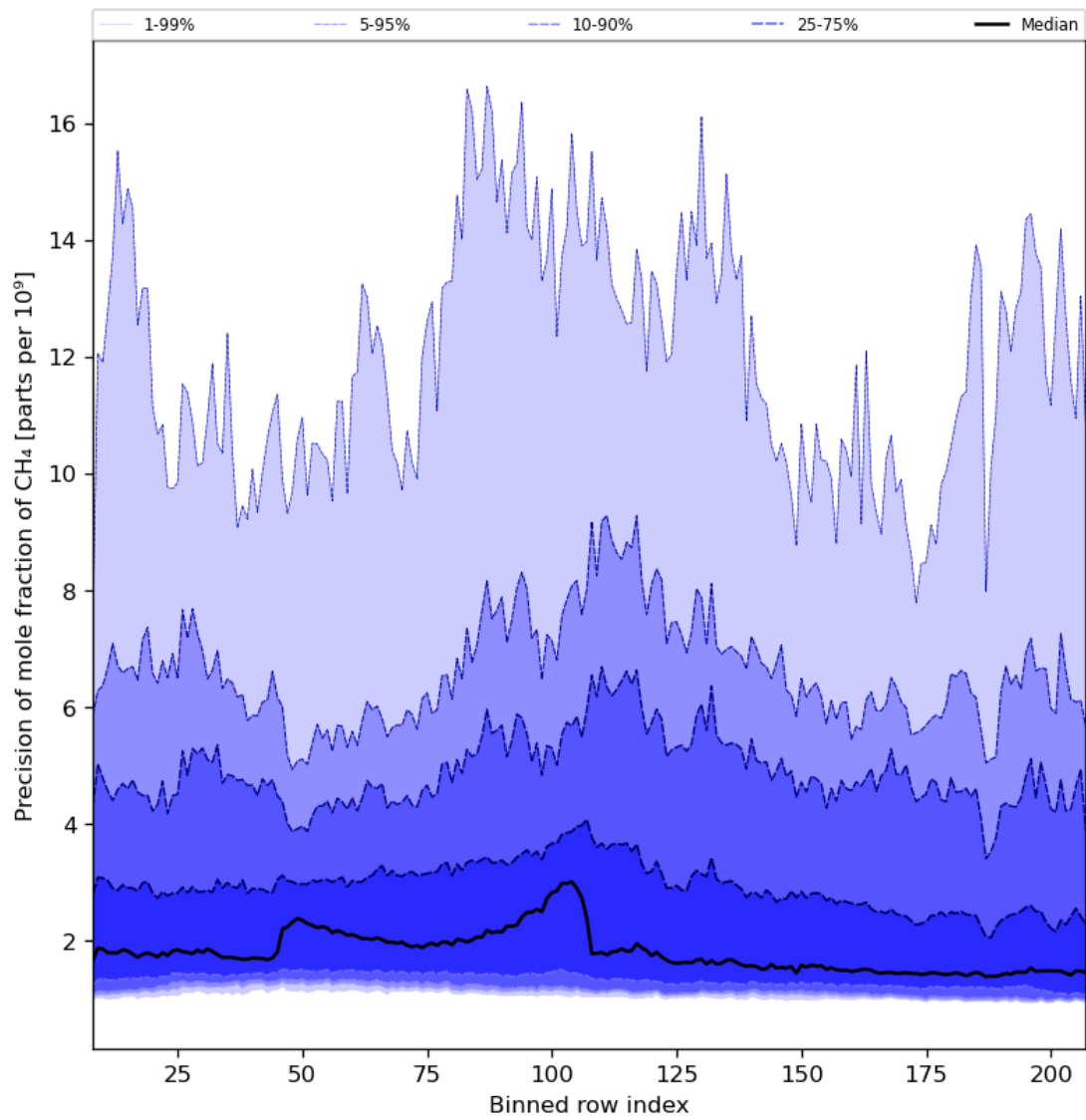
Figure 35: Along track statistics of “Precision of mole fraction of CH 4 ” for 2024-04-27 to 2024-04-29
