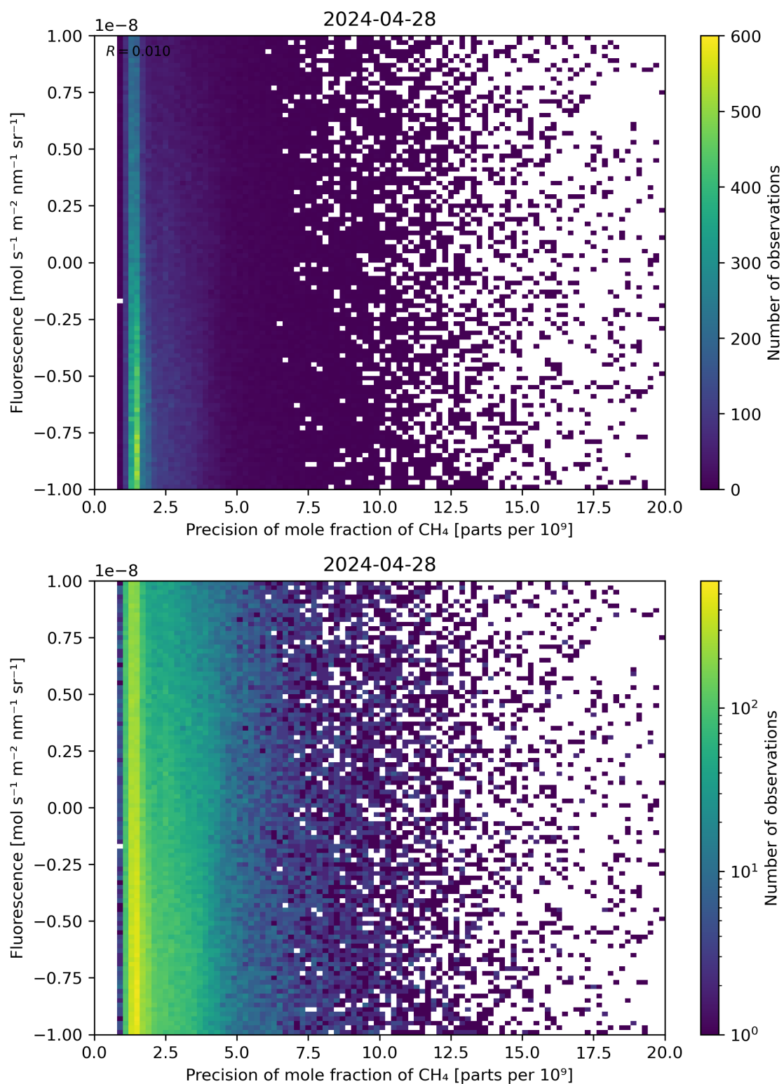
Figure 81: Scatter density plot of “Precision of mole fraction of CH 4 ” against “Fluorescence” for 2024-04-27 to 2024-04-29.
