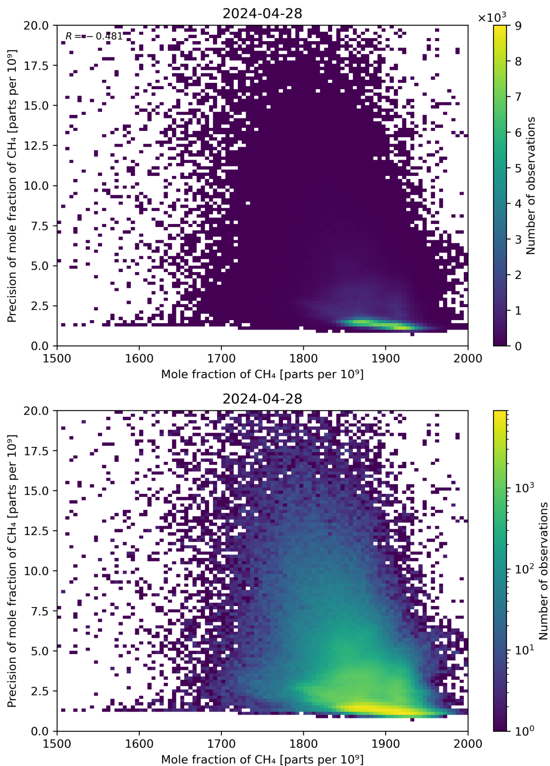
Figure 75: Scatter density plot of “Mole fraction of CH 4 ” against “Precision of mole fraction of CH 4 ” for 2024-04-27 to 2024-04-29.
