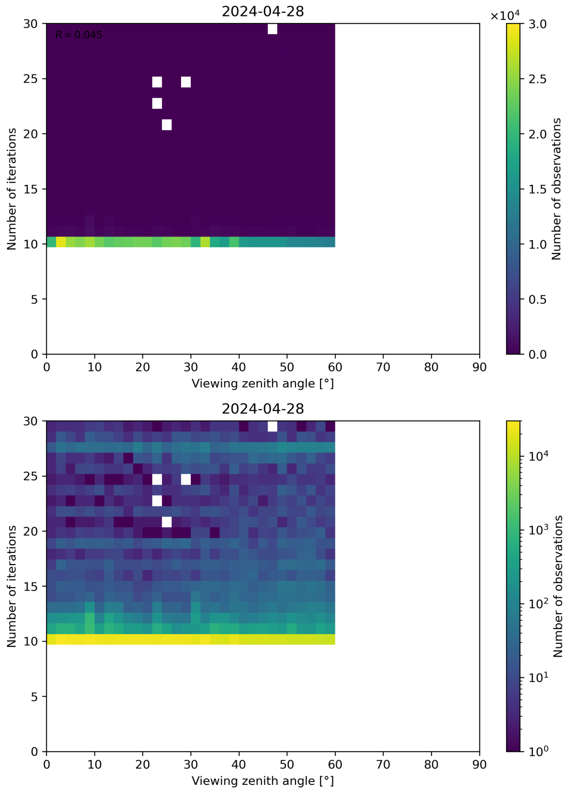
Figure 113: Scatter density plot of “Viewing zenith angle” against “Number of iterations” for 2024-04-27 to 2024-04-29.
