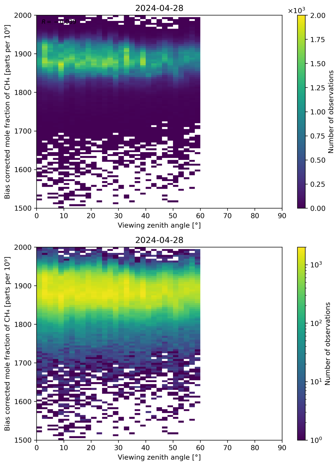
Figure 111: Scatter density plot of “Viewing zenith angle” against “Bias corrected mole fraction of CH 4 ” for 2024-04-27 to 2024-04-29.
