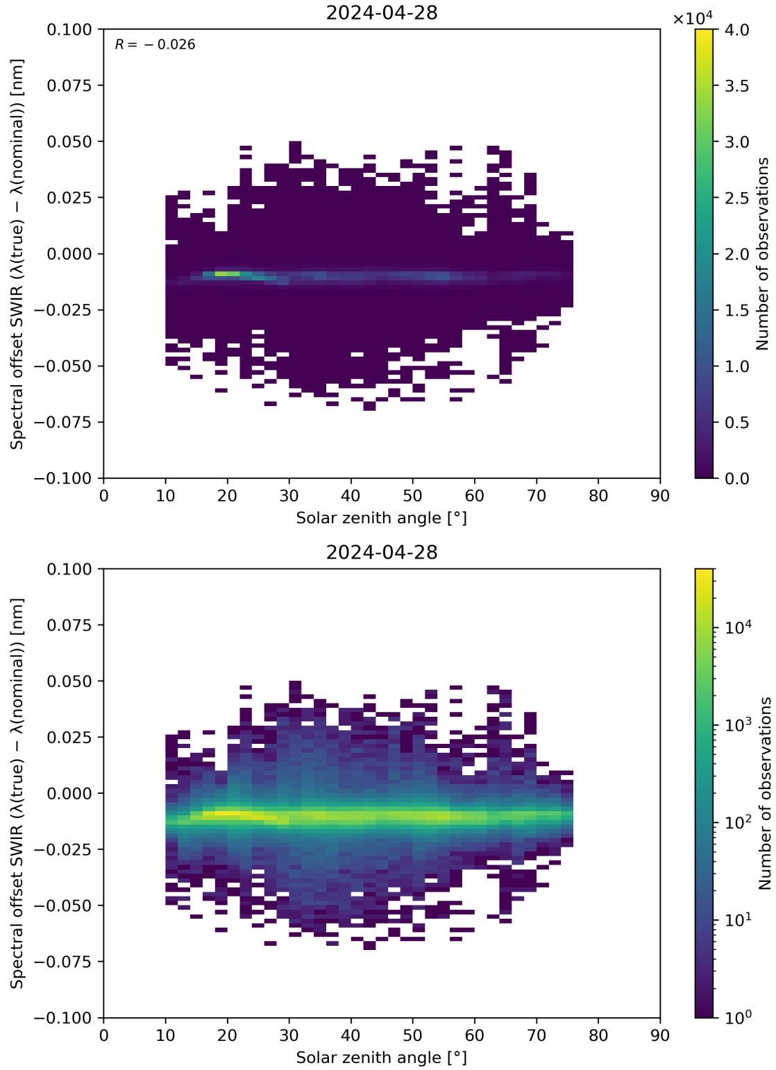
Figure 104: Scatter density plot of “Solar zenith angle” against “Spectral offset SWIR ( \lambda(\text{true}) - \lambda(\text{nominal}) )” for 2024-04-27 to 2024-04-29.
