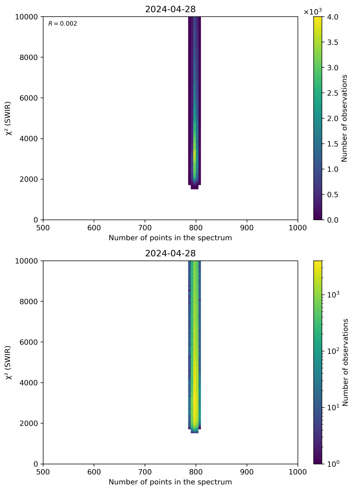
Figure 89: Scatter density plot of “Number of points in the spectrum” against “ \chi^2 (SWIR)” for 2024-04-27 to 2024-04-29.
