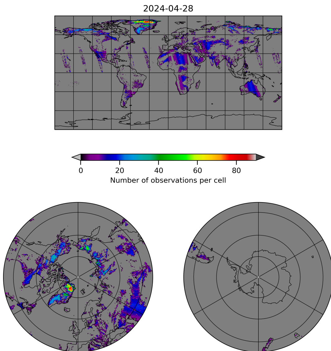
Figure 10: Map of the number of observations for 2024-04-27 to 2024-04-29
