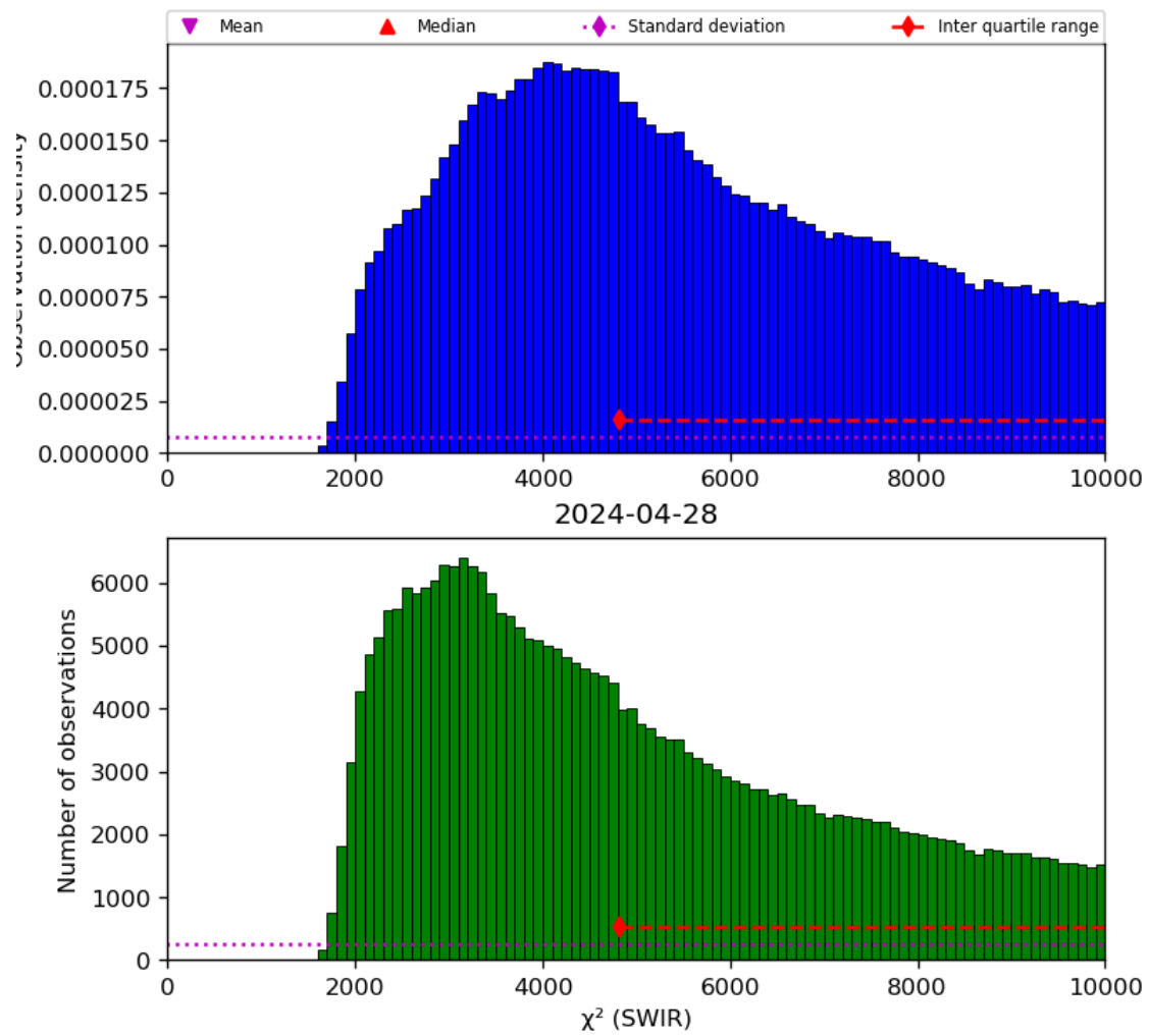
Figure 28: Histogram of “ \chi^2 (SWIR)” for 2024-04-27 to 2024-04-29
