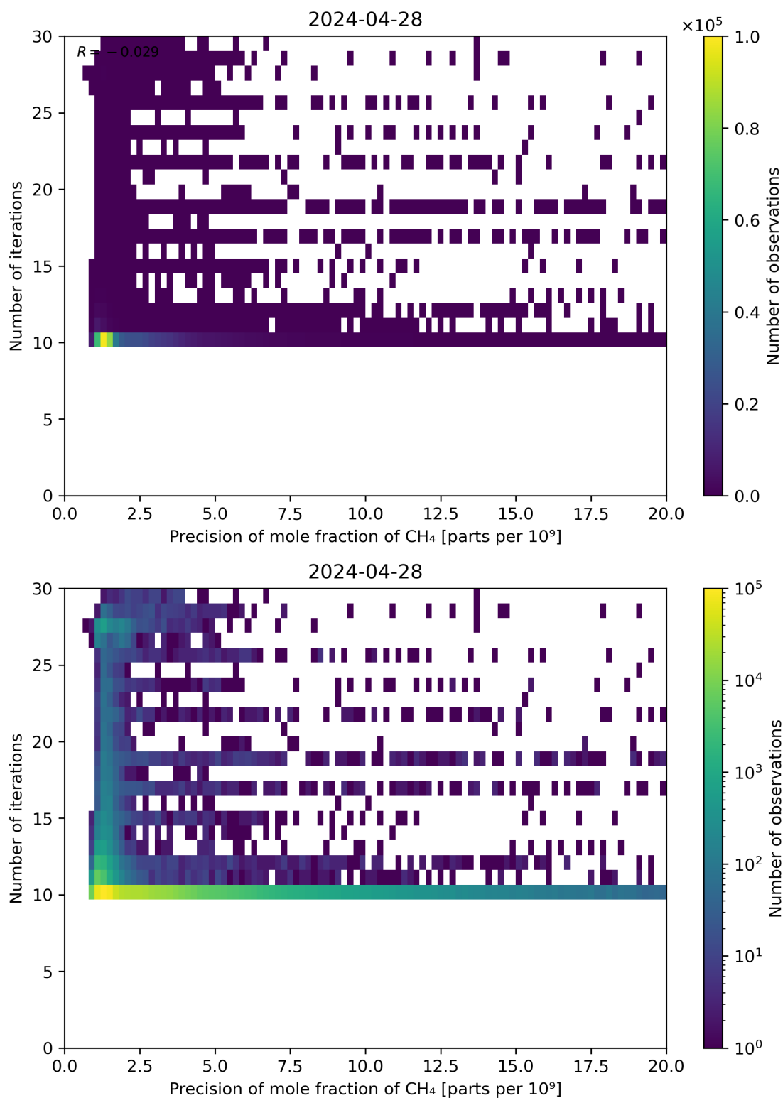
Figure 83: Scatter density plot of “Precision of mole fraction of CH 4 ” against “Number of iterations” for 2024-04-27 to 2024-04-29.
