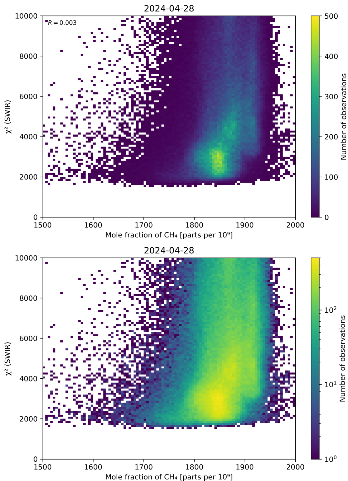
Figure 71: Scatter density plot of “Mole fraction of \text{CH}_4 ” against “ \chi^2 (SWIR)” for 2024-04-27 to 2024-04-29.
