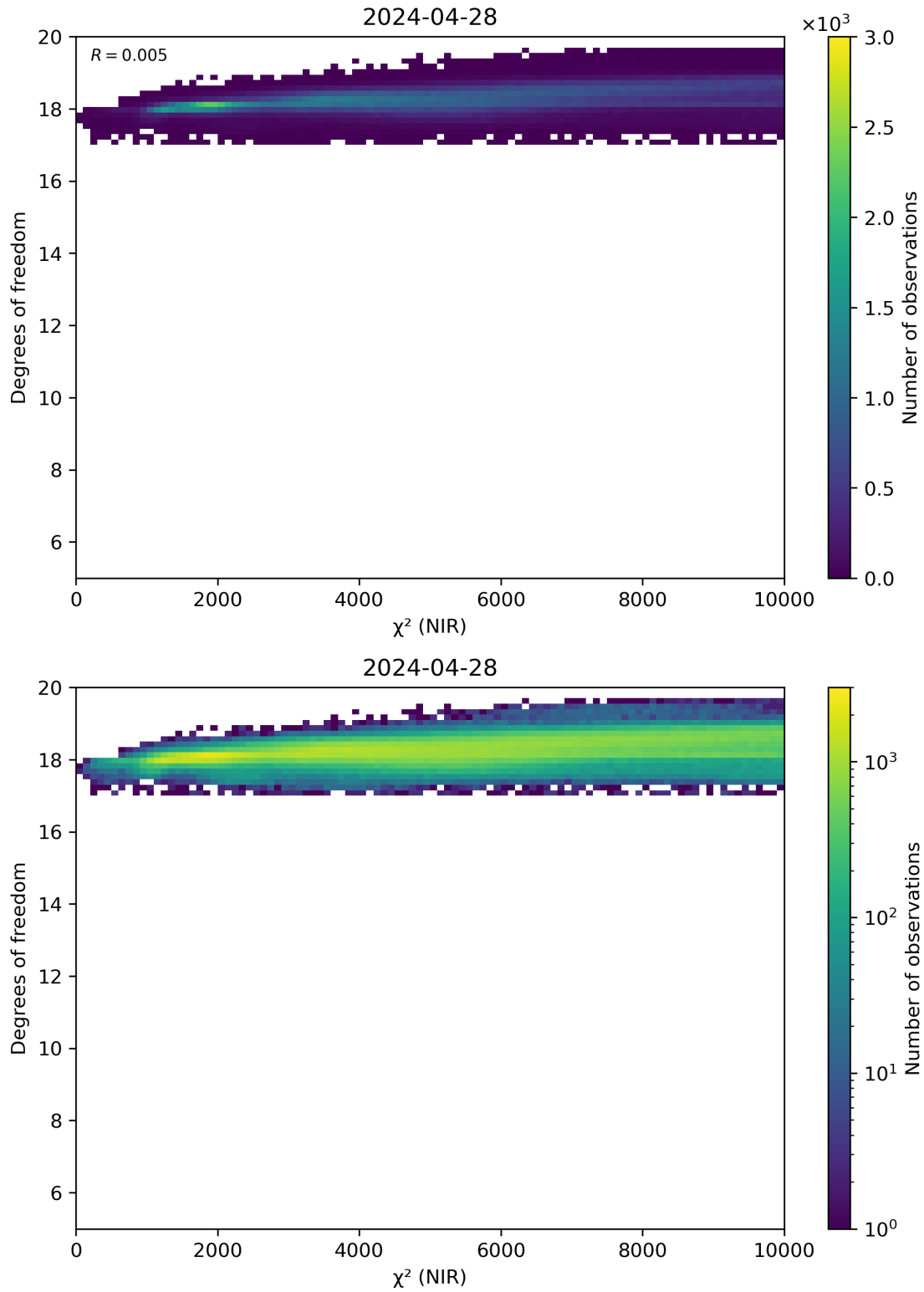
Figure 44: Scatter density plot of “ \chi^2 (NIR)” against “Degrees of freedom” for 2024-04-27 to 2024-04-29.
