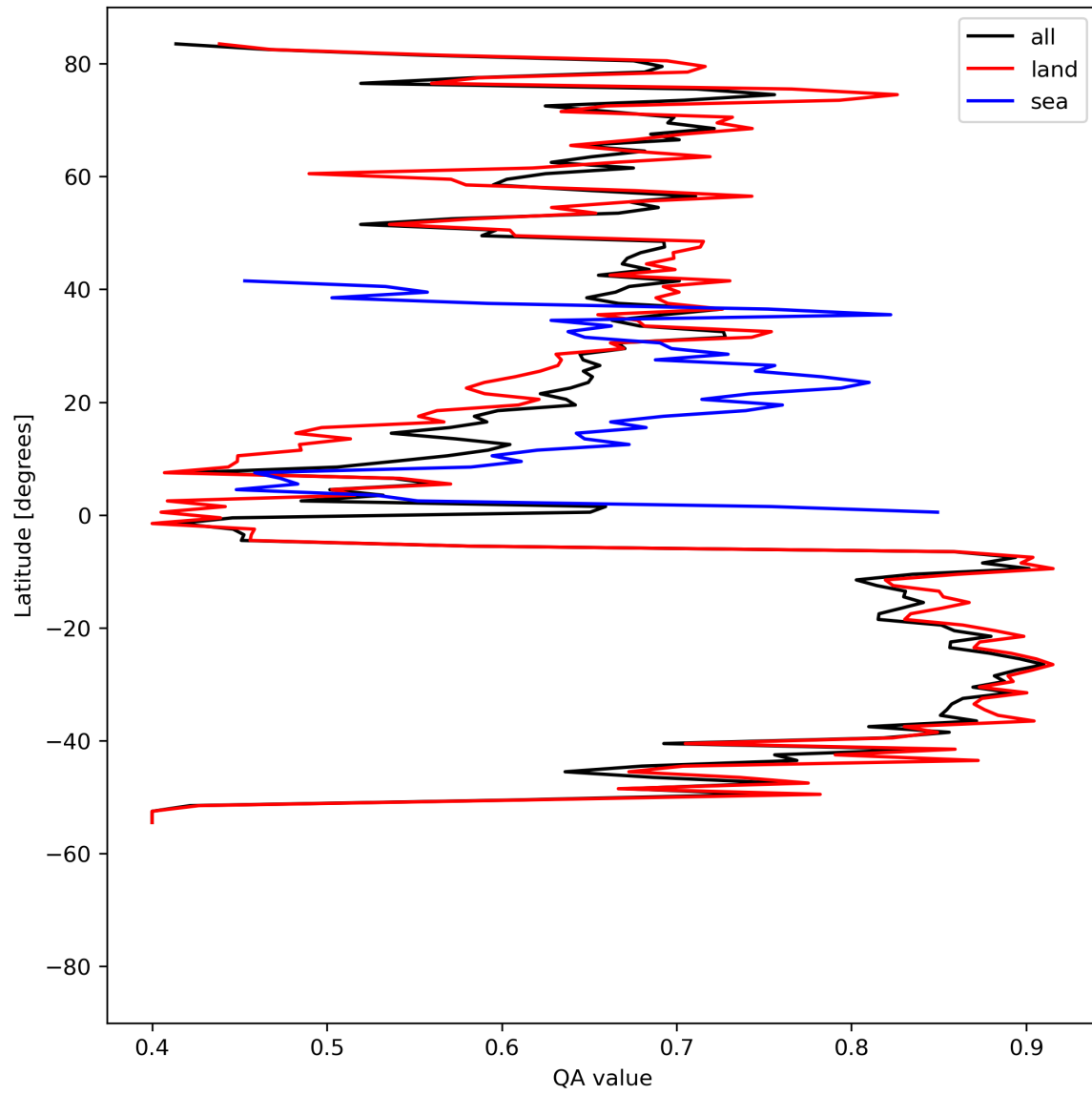
Figure 11: Zonal average of “QA value” for 2024-04-27 to 2024-04-29.
