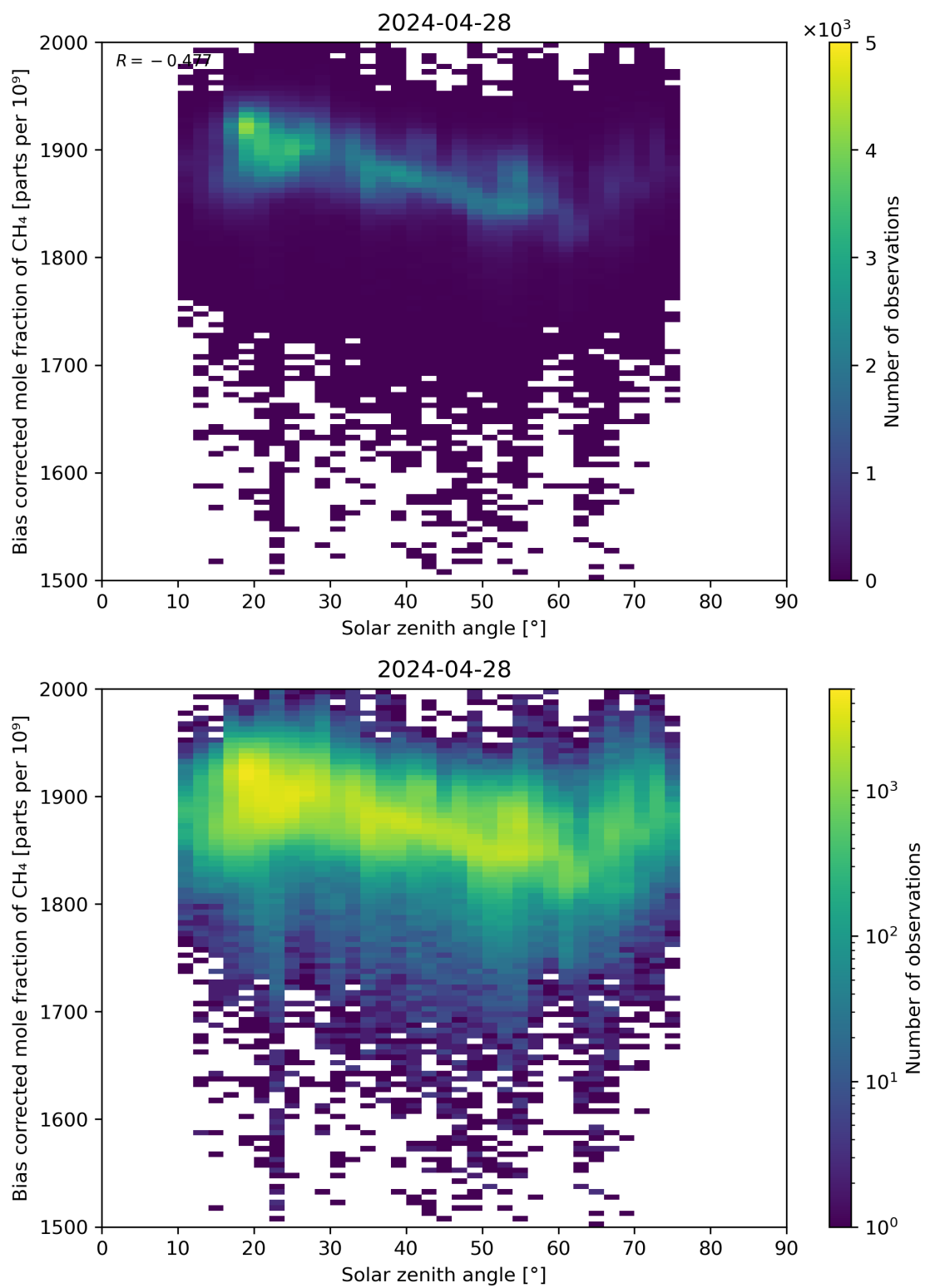
Figure 100: Scatter density plot of “Solar zenith angle” against “Bias corrected mole fraction of CH 4 ” for 2024-04-27 to 2024-04-29.
