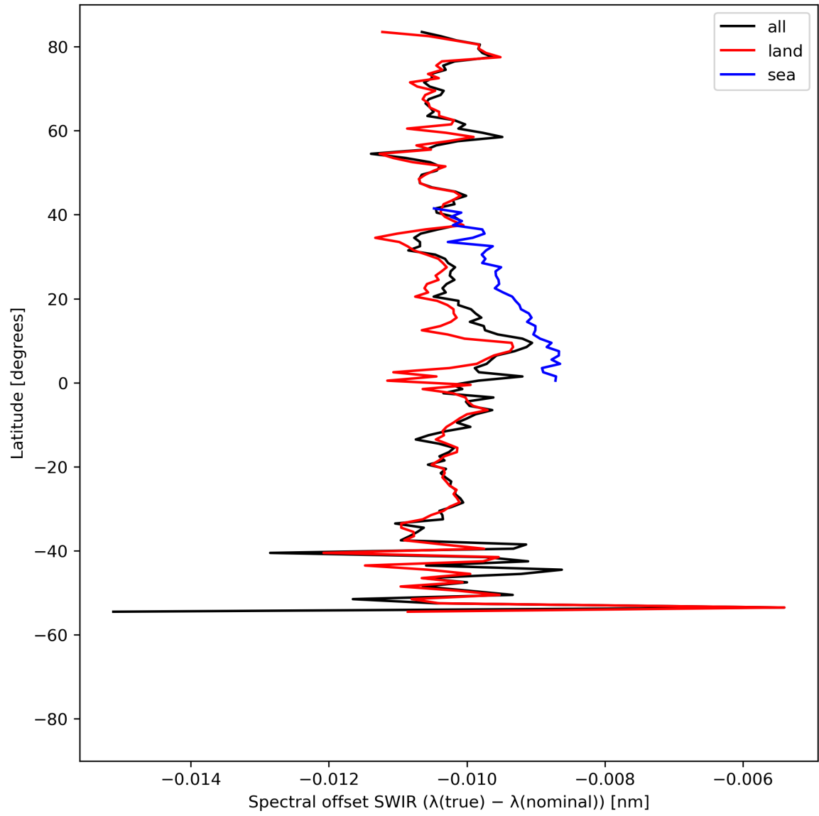
Figure 16: Zonal average of “Spectral offset SWIR ( \lambda(\text{true}) - \lambda(\text{nominal}) )” for 2024-04-27 to 2024-04-29.
