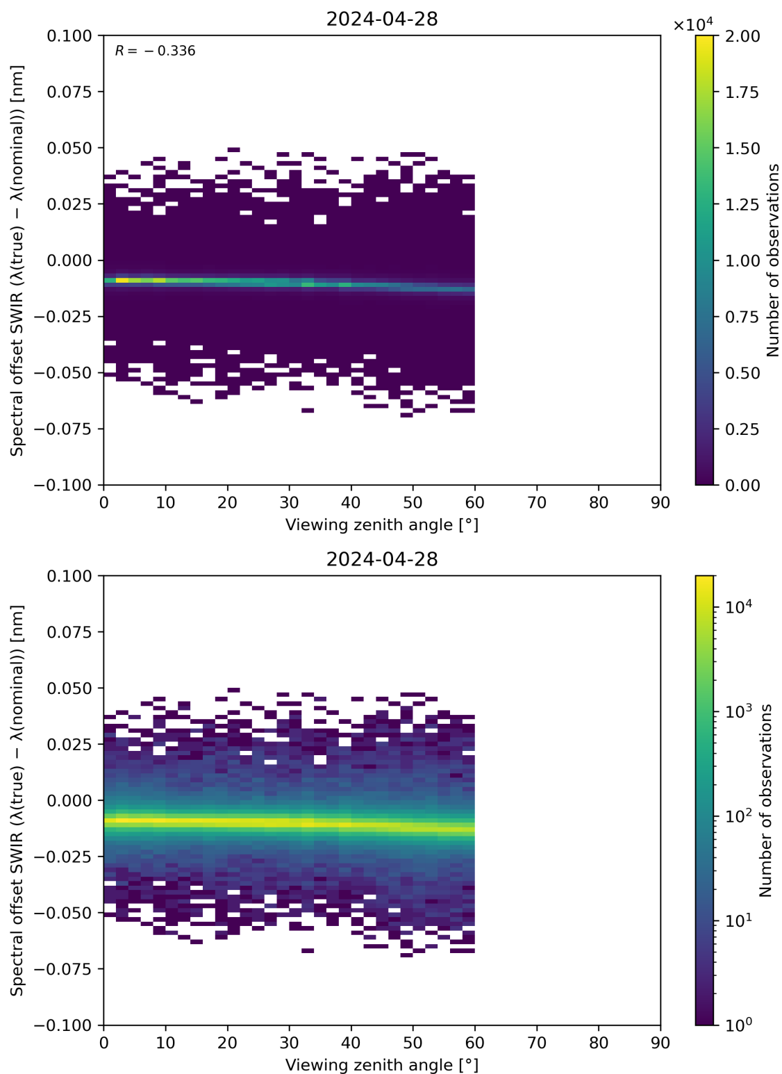
Figure 116: Scatter density plot of “Viewing zenith angle” against “Spectral offset SWIR ( \lambda(\text{true}) - \lambda(\text{nominal}) )” for 2024-04-27 to 2024-04-29.
