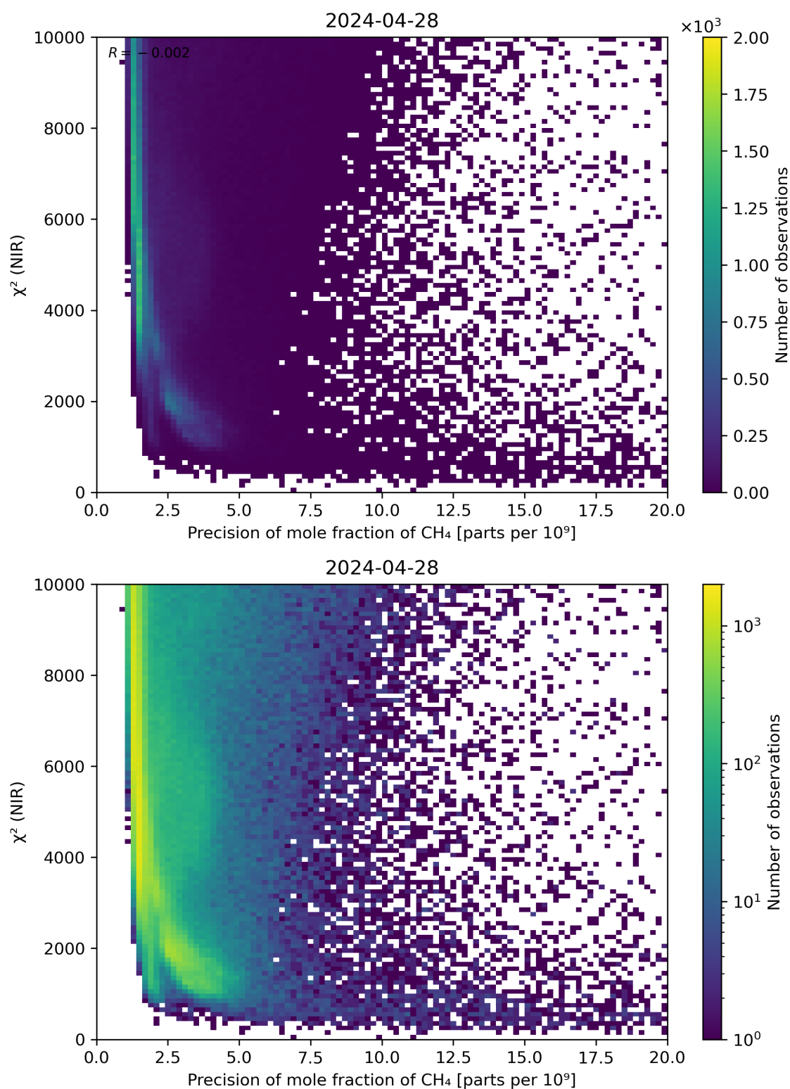
Figure 78: Scatter density plot of “Precision of mole fraction of CH 4 ” against “ \chi^2 (NIR)” for 2024-04-27 to 2024-04-29.
