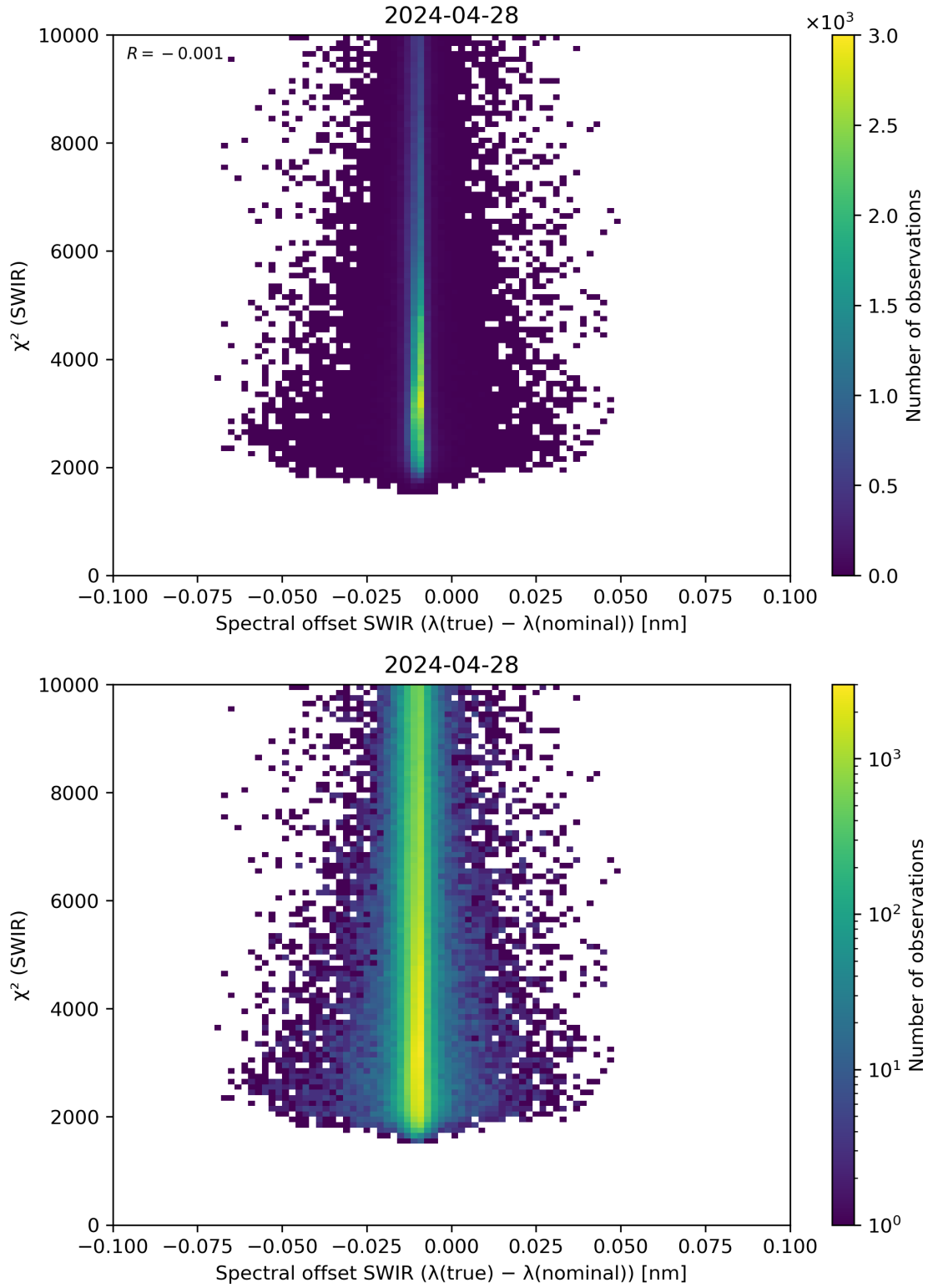
Figure 118: Scatter density plot of “Spectral offset SWIR ( \lambda(\text{true}) - \lambda(\text{nominal}) )” against “ \chi^2 (SWIR)” for 2024-04-27 to 2024-04-29.
