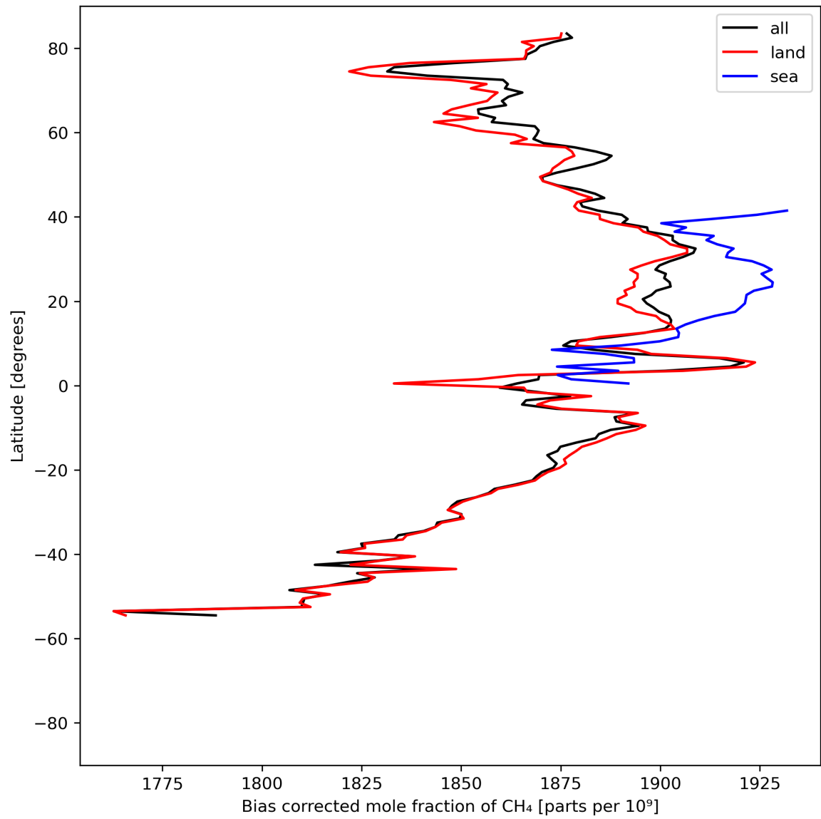
Figure 14: Zonal average of “Bias corrected mole fraction of \text{CH}_4 ” for 2024-04-27 to 2024-04-29.
