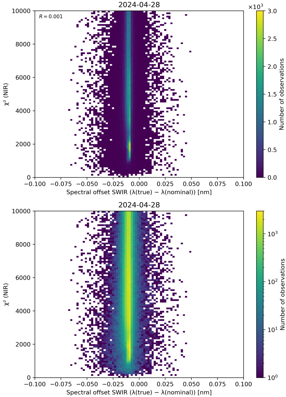
Figure 117: Scatter density plot of “Spectral offset SWIR ( \lambda(\text{true}) - \lambda(\text{nominal}) )” against “ \chi^2 (NIR)” for 2024-04-27 to 2024-04-29.
