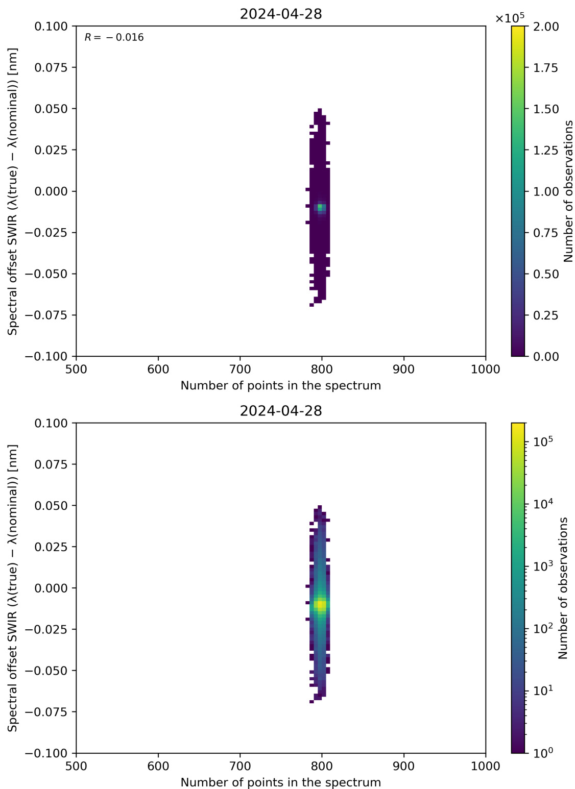
Figure 93: Scatter density plot of “Number of points in the spectrum” against “Spectral offset SWIR ( \lambda(\text{true}) - \lambda(\text{nominal}) )” for 2024-04-27 to 2024-04-29.
