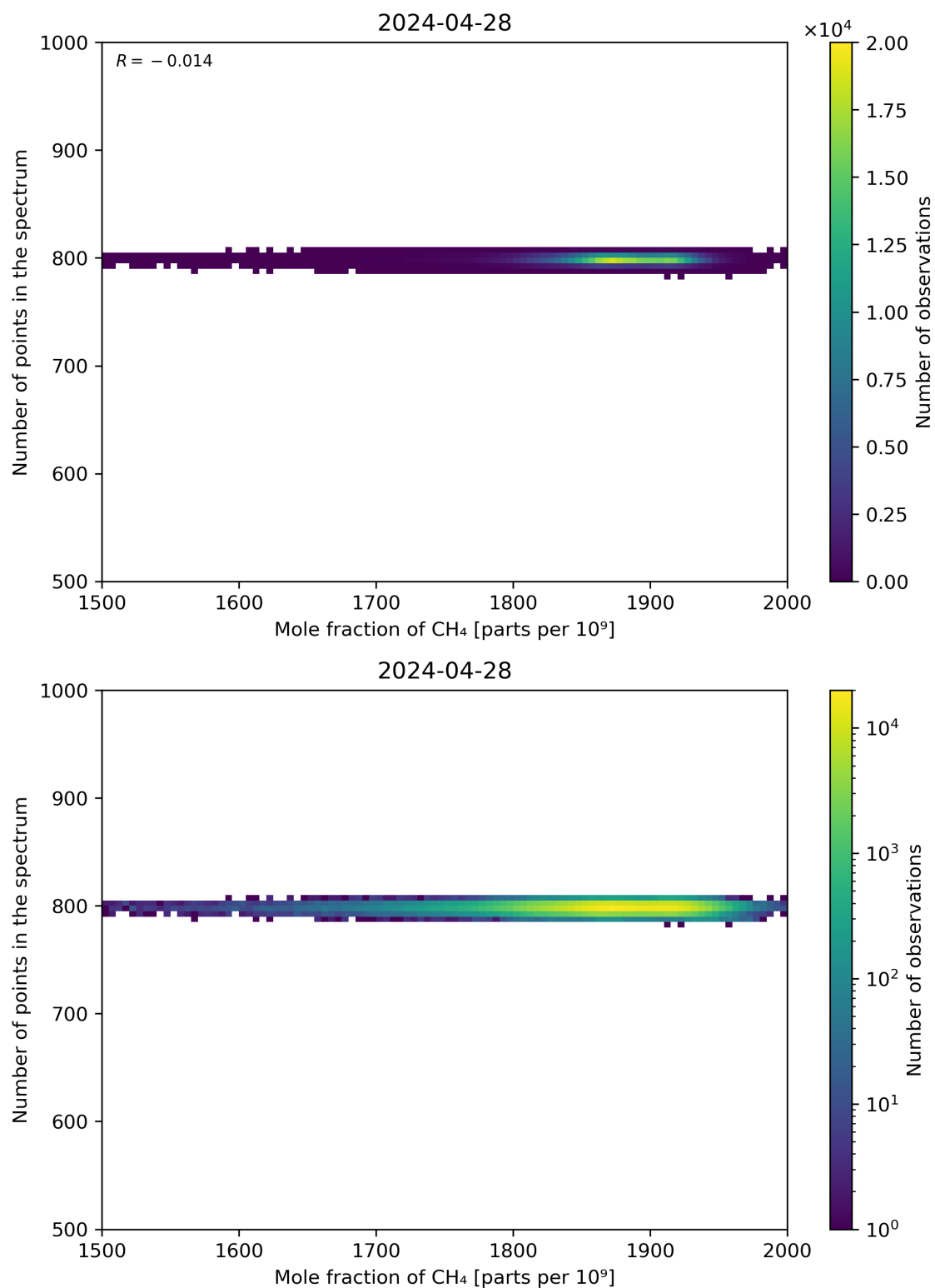
Figure 77: Scatter density plot of “Mole fraction of CH 4 ” against “Number of points in the spectrum” for 2024-04-27 to 2024-04-29.
