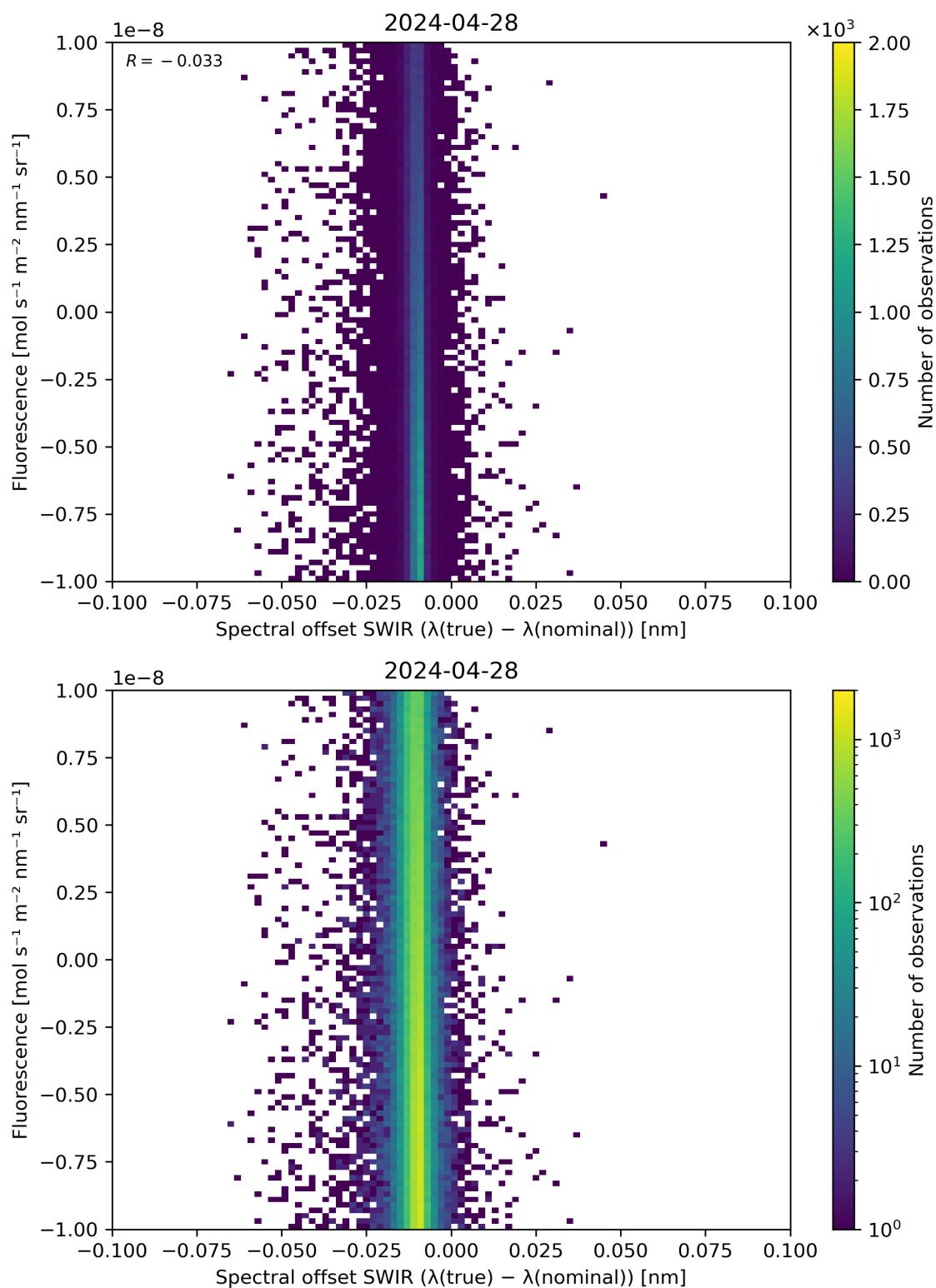
Figure 120: Scatter density plot of “Spectral offset SWIR ( \lambda(\text{true}) - \lambda(\text{nominal}) )” against “Fluorescence” for 2024-04-27 to 2024-04-29.
