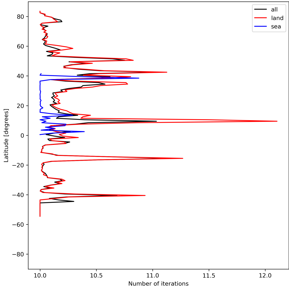
Figure 20: Zonal average of “Number of iterations” for 2024-04-27 to 2024-04-29.
