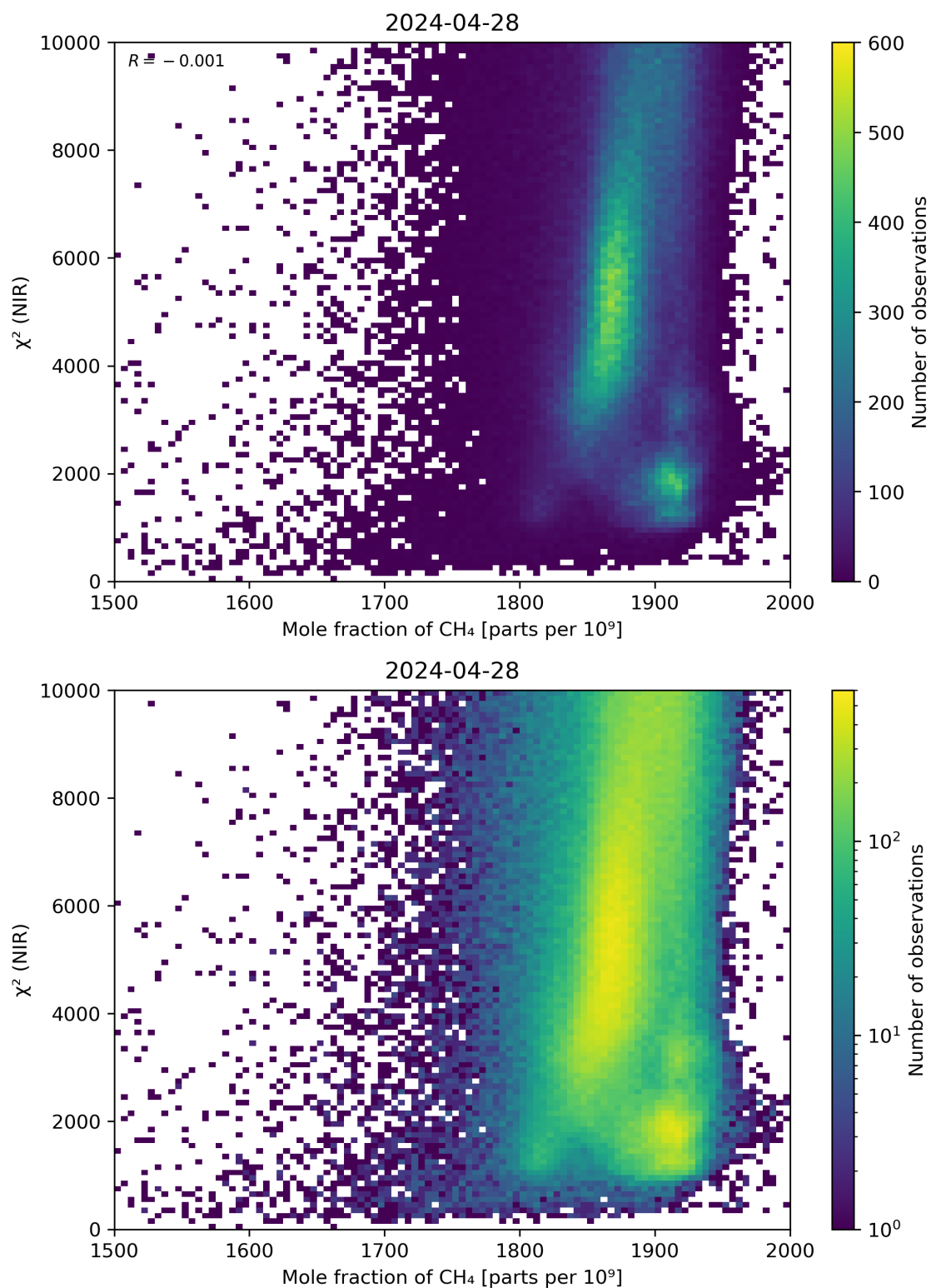
Figure 70: Scatter density plot of “Mole fraction of CH 4 ” against “ \chi^2 (NIR)” for 2024-04-27 to 2024-04-29.
