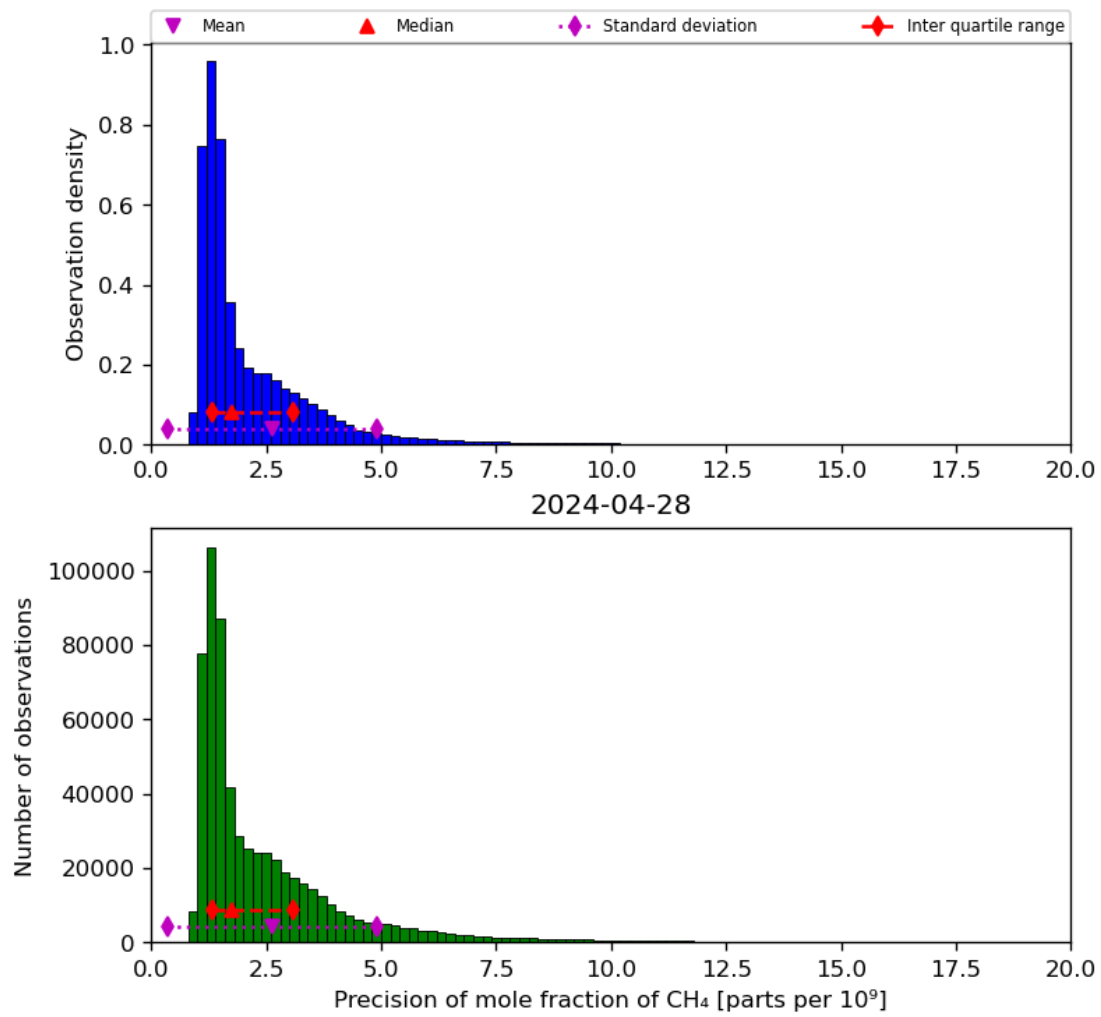
Figure 24: Histogram of “Precision of mole fraction of CH 4 ” for 2024-04-27 to 2024-04-29
