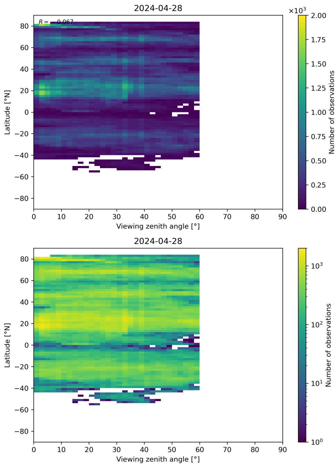
Figure 109: Scatter density plot of “Viewing zenith angle” against “Latitude” for 2024-04-27 to 2024-04-29.
