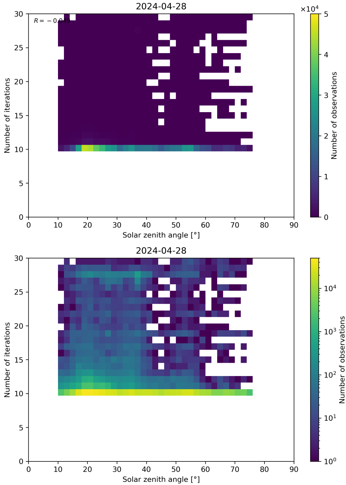
Figure 102: Scatter density plot of “Solar zenith angle” against “Number of iterations” for 2024-04-27 to 2024-04-29.
