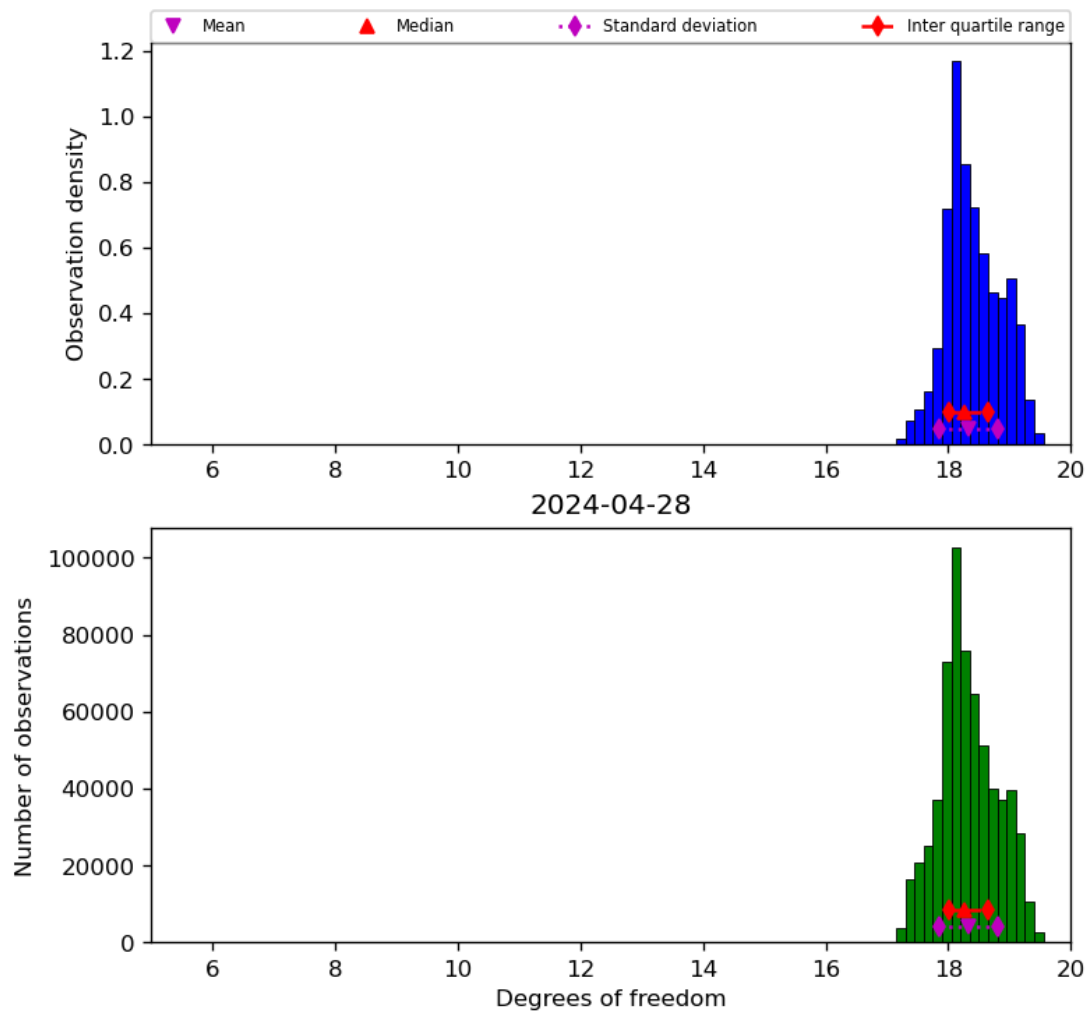
Figure 30: Histogram of “Degrees of freedom” for 2024-04-27 to 2024-04-29
