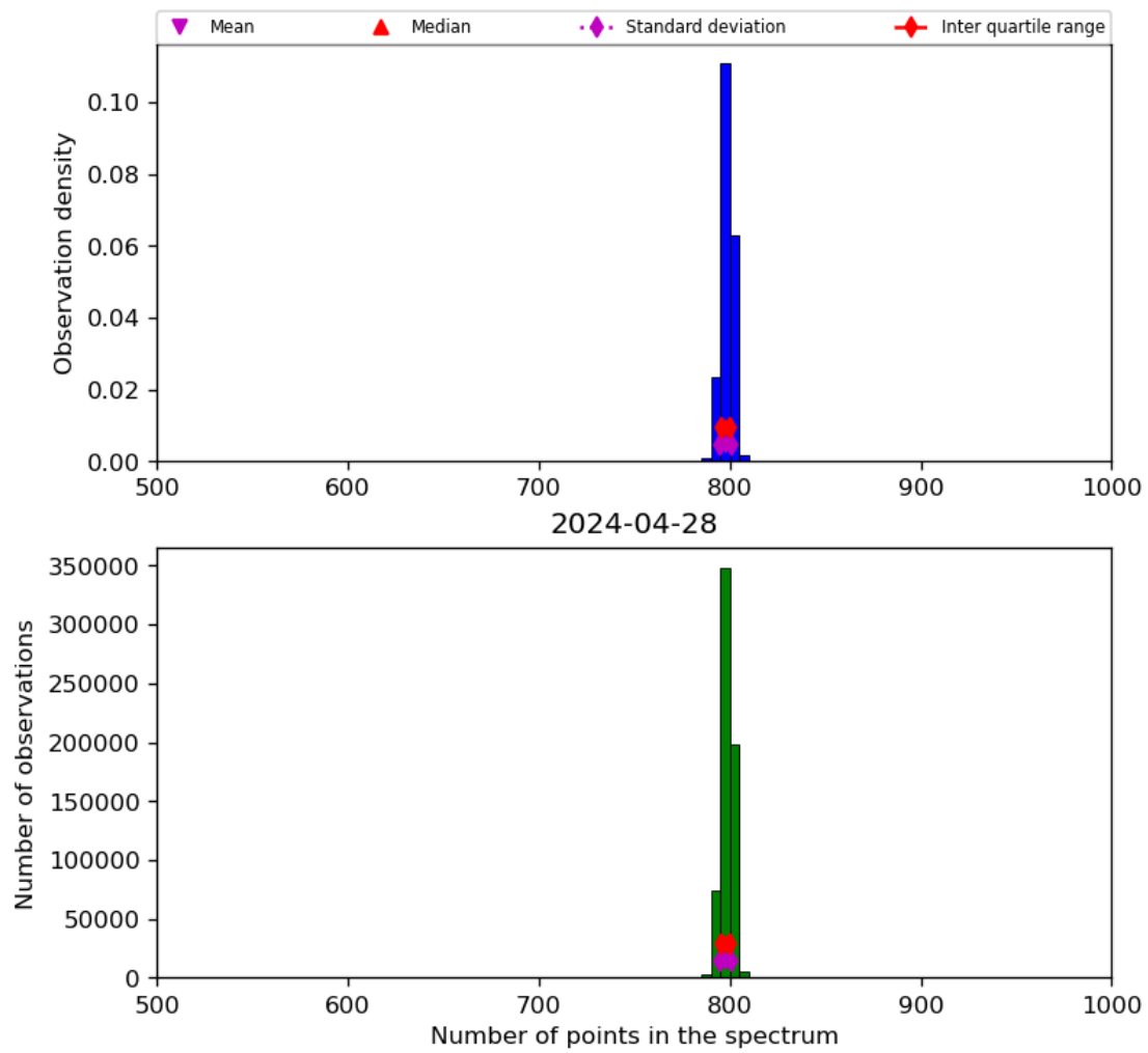
Figure 26: Histogram of “Number of points in the spectrum” for 2024-04-27 to 2024-04-29
