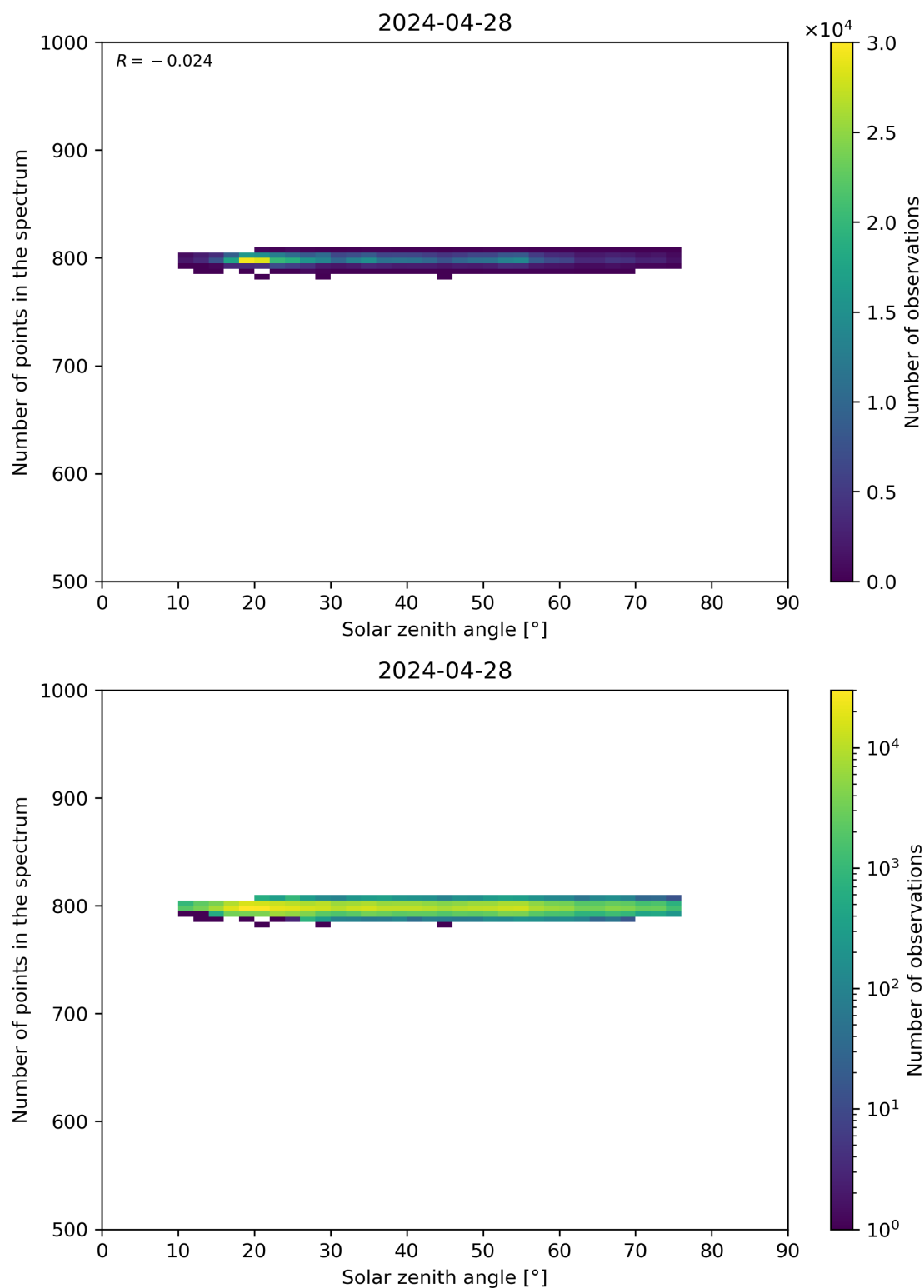
Figure 103: Scatter density plot of “Solar zenith angle” against “Number of points in the spectrum” for 2024-04-27 to 2024-04-29.
