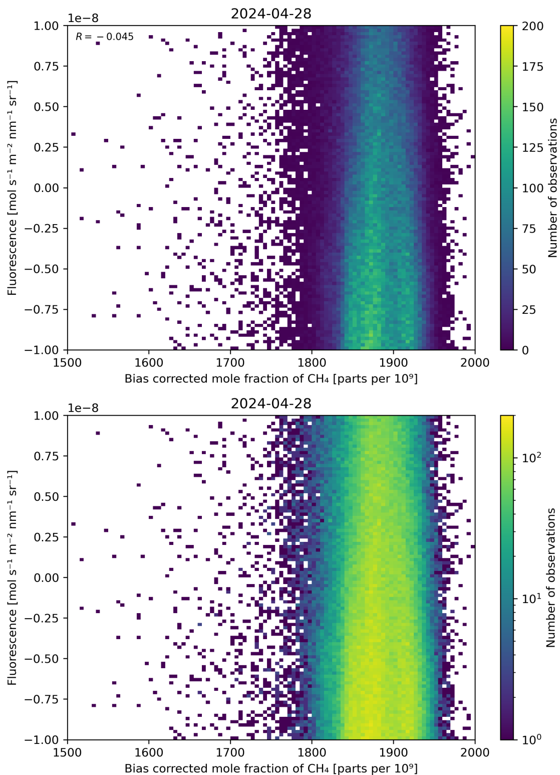
Figure 66: Scatter density plot of “Bias corrected mole fraction of \text{CH}_4 ” against “Fluorescence” for 2024-04-27 to 2024-04-29.
