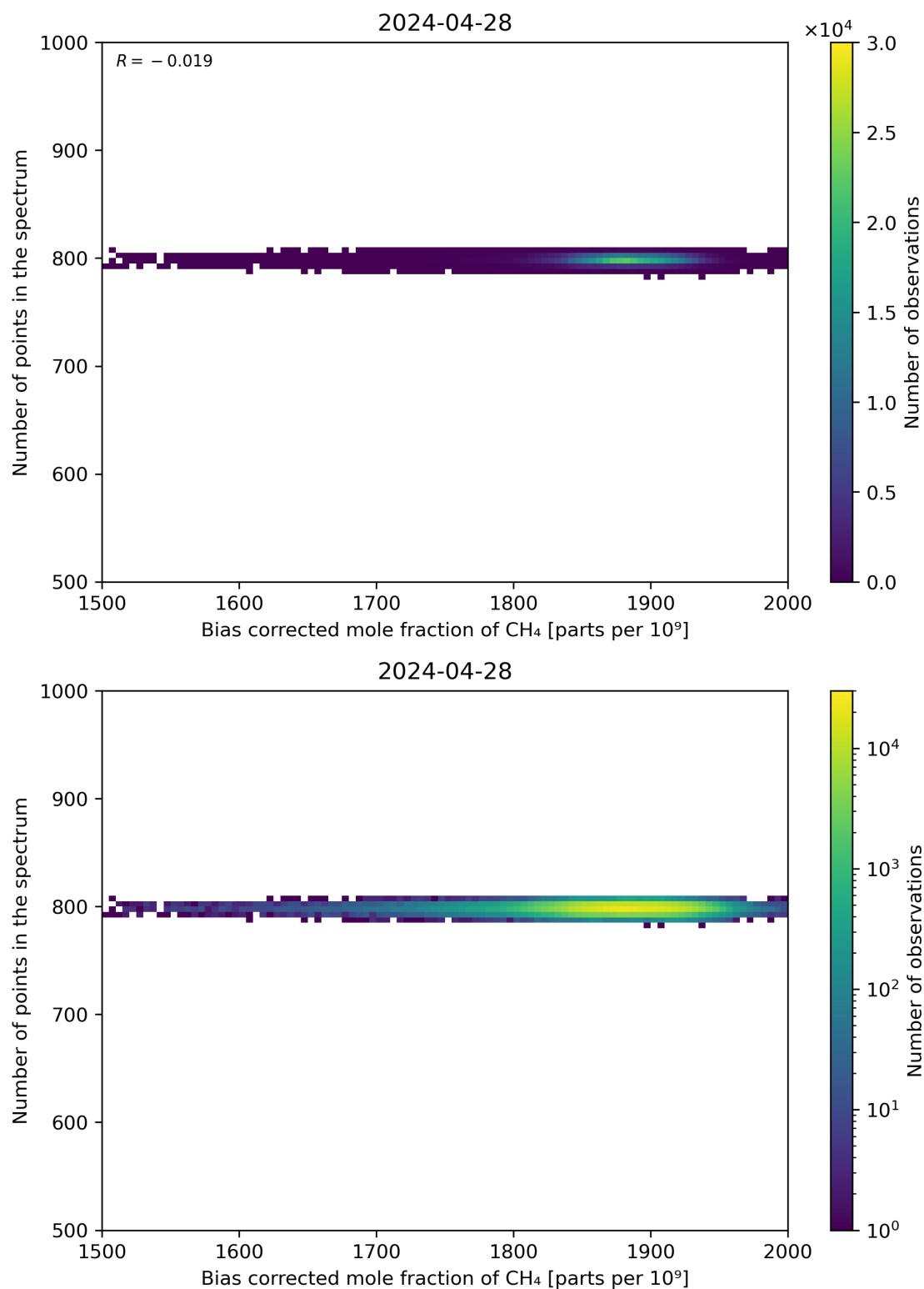
Figure 68: Scatter density plot of “Bias corrected mole fraction of CH 4 ” against “Number of points in the spectrum” for 2024-04-27 to 2024-04-29.
