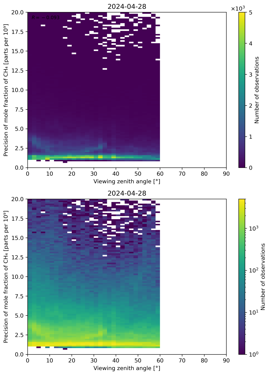
Figure 112: Scatter density plot of “Viewing zenith angle” against “Precision of mole fraction of \text{CH}_4 ” for 2024-04-27 to 2024-04-29.
