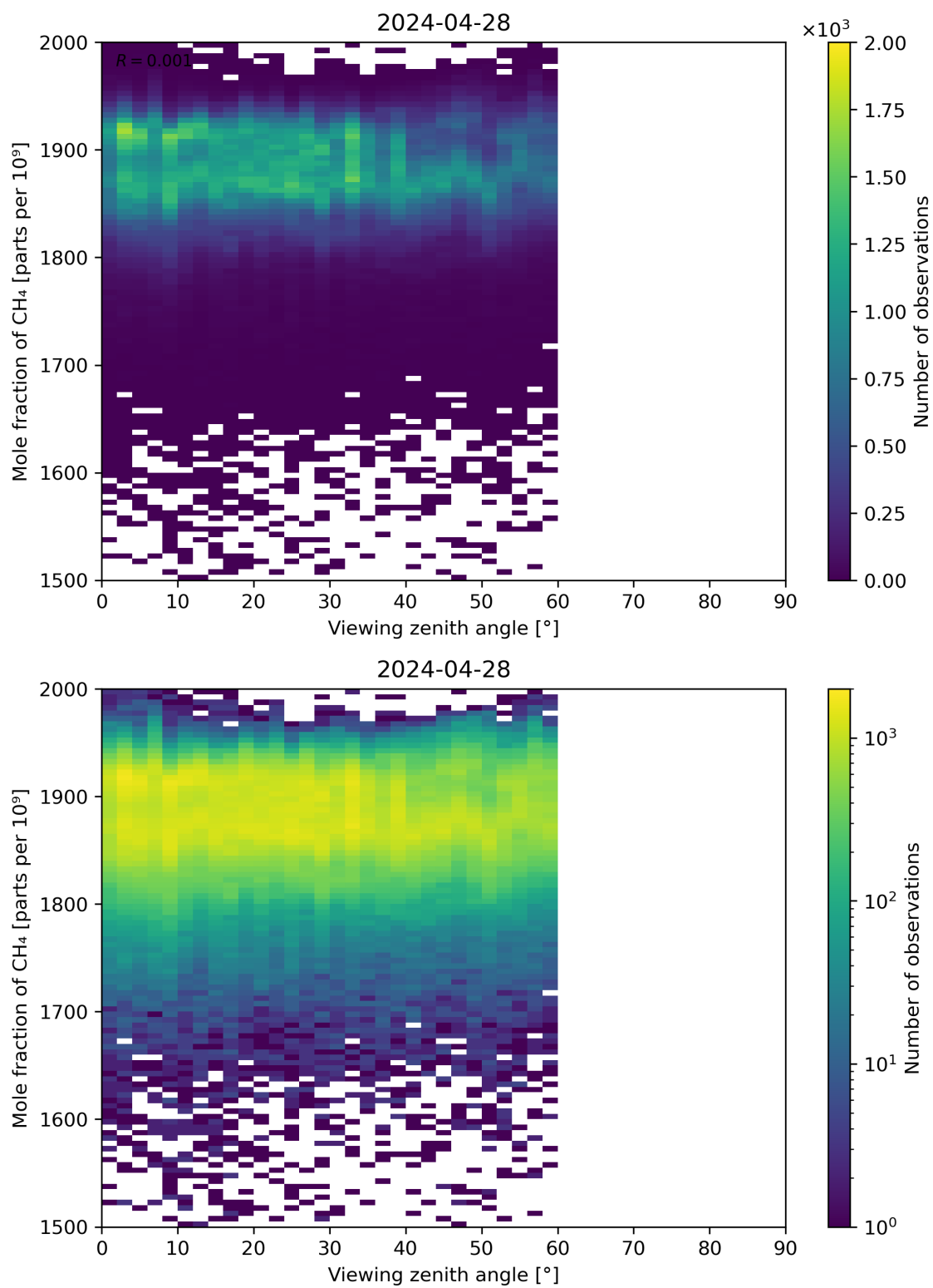
Figure 110: Scatter density plot of “Viewing zenith angle” against “Mole fraction of CH 4 ” for 2024-04-27 to 2024-04-29.
