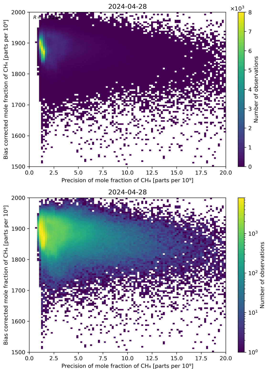
Figure 82: Scatter density plot of “Precision of mole fraction of CH 4 ” against “Bias corrected mole fraction of CH 4 ” for 2024-04-27 to 2024-04-29.
