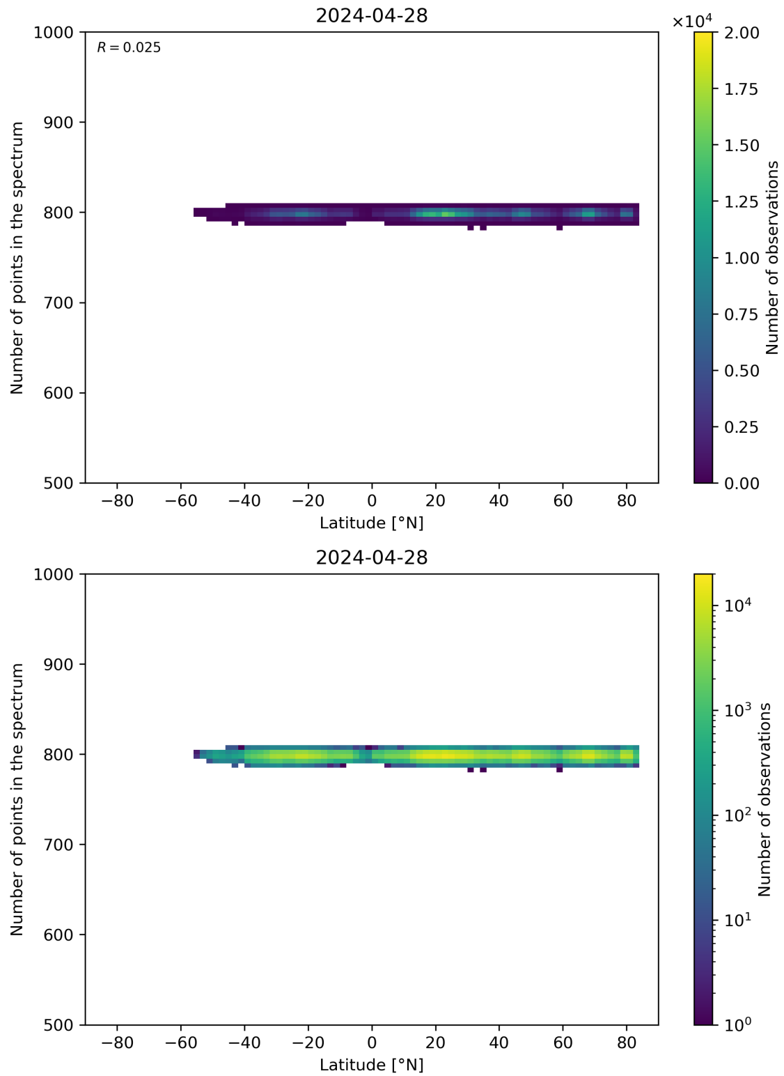
Figure 61: Scatter density plot of “Latitude” against “Number of points in the spectrum” for 2024-04-27 to 2024-04-29.
