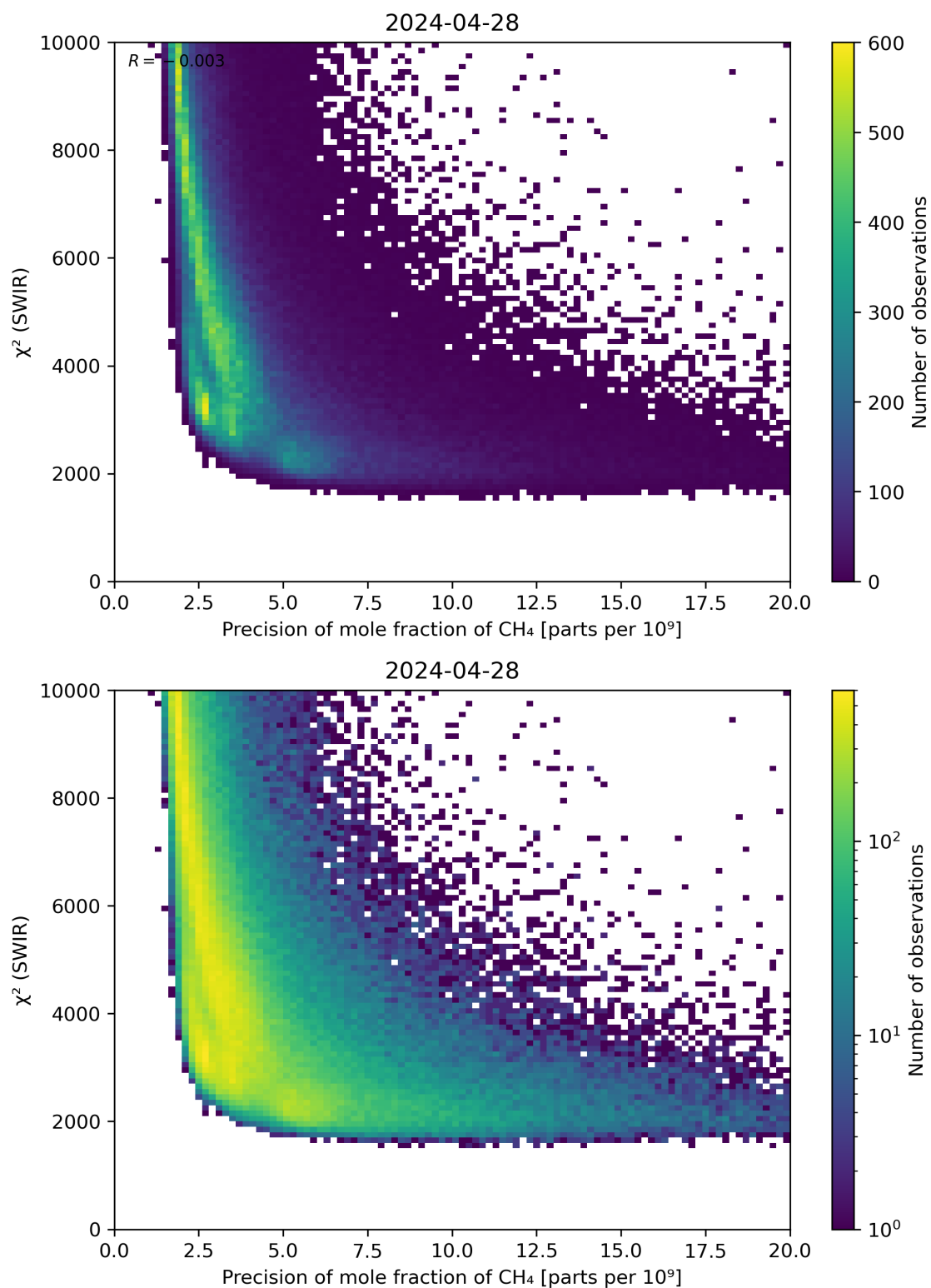
Figure 79: Scatter density plot of “Precision of mole fraction of CH 4 ” against “ \chi^2 (SWIR)” for 2024-04-27 to 2024-04-29.
