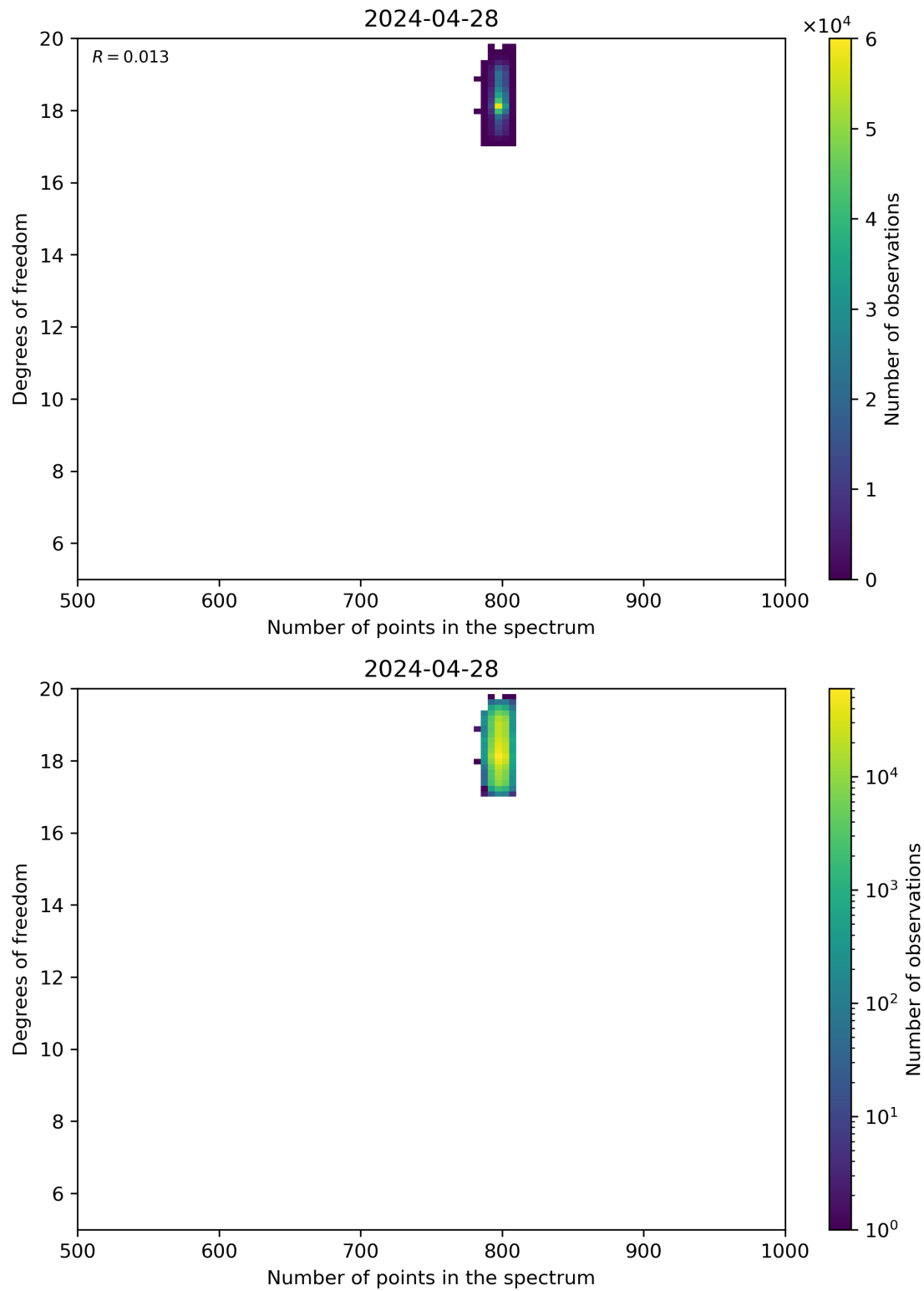
Figure 90: Scatter density plot of “Number of points in the spectrum” against “Degrees of freedom” for 2024-04-27 to 2024-04-29.
