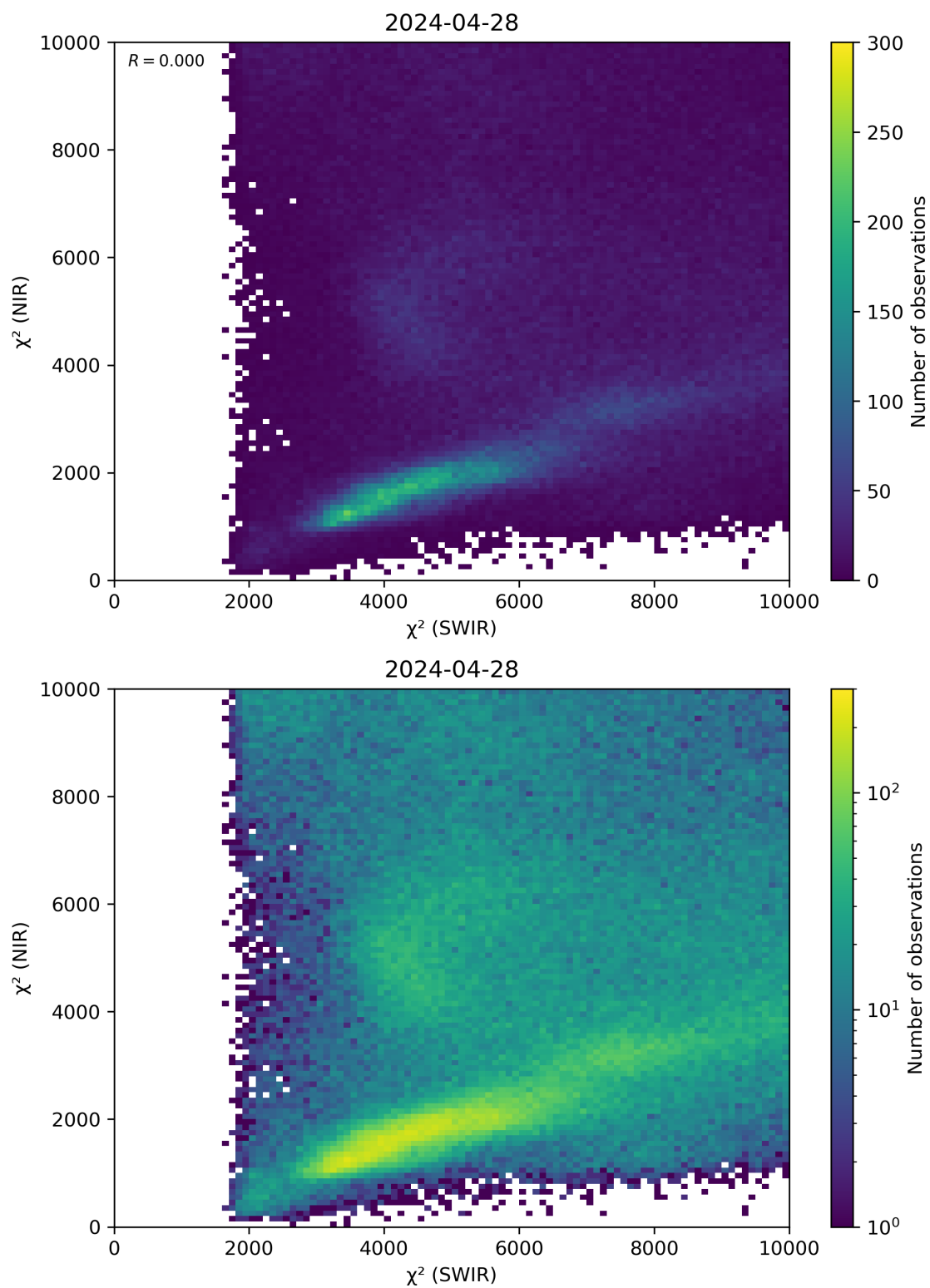
Figure 47: Scatter density plot of “ \chi^2 (SWIR)” against “ \chi^2 (NIR)” for 2024-04-27 to 2024-04-29.
