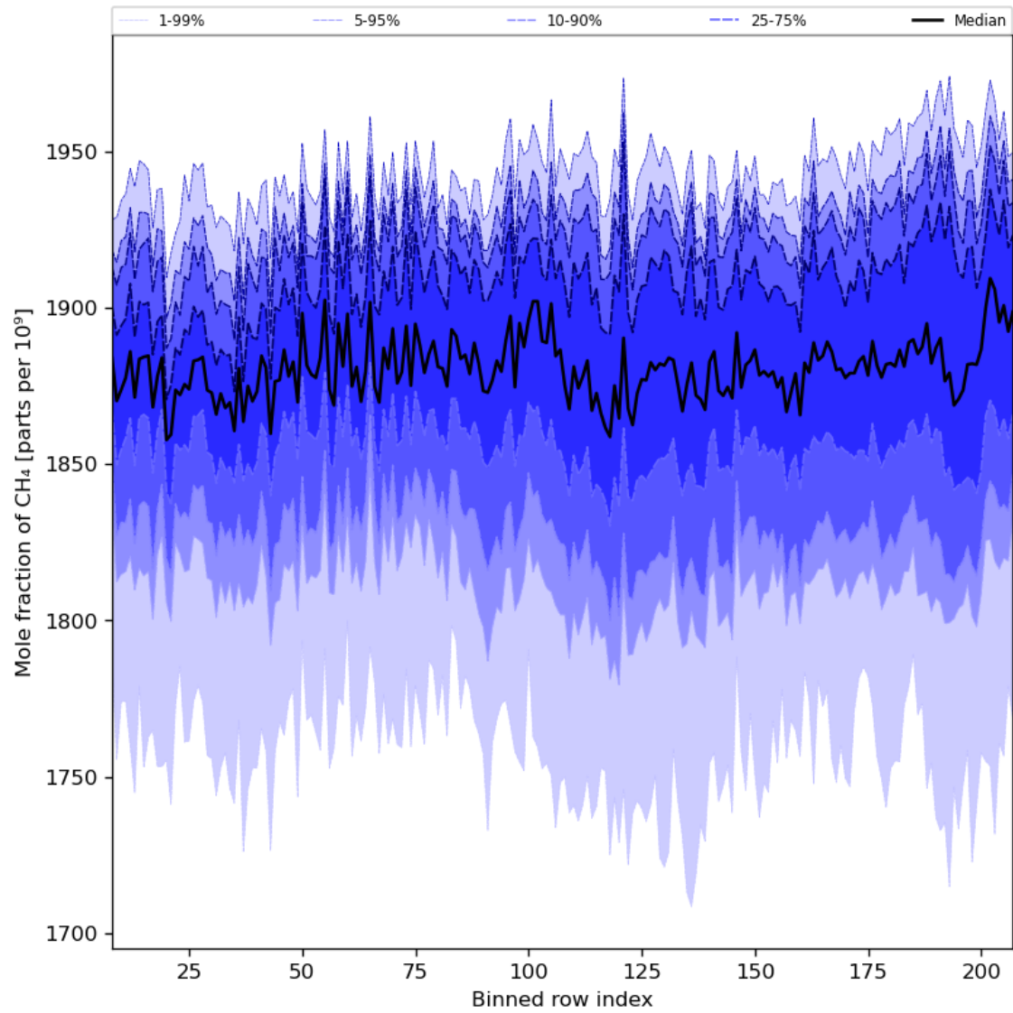
Figure 34: Along track statistics of “Mole fraction of CH 4 ” for 2024-04-27 to 2024-04-29
