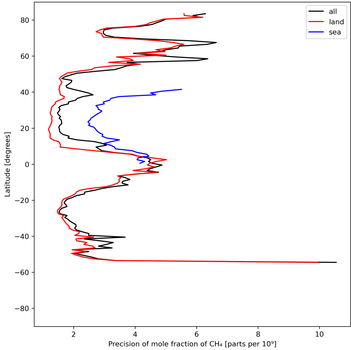
Figure 13: Zonal average of “Precision of mole fraction of CH 4 ” for 2024-04-27 to 2024-04-29.
