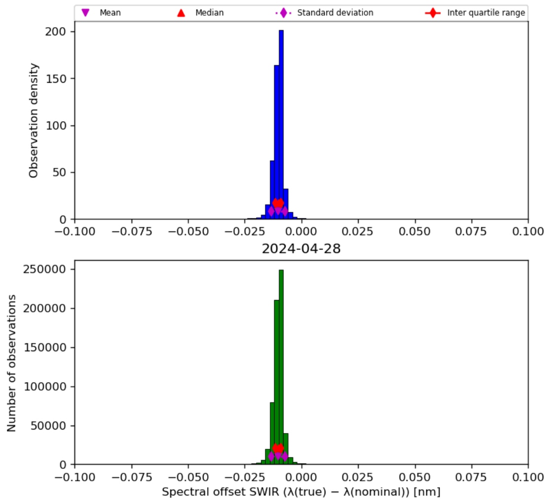
Figure 27: Histogram of “Spectral offset SWIR ( \lambda(\text{true}) - \lambda(\text{nominal}) )” for 2024-04-27 to 2024-04-29
