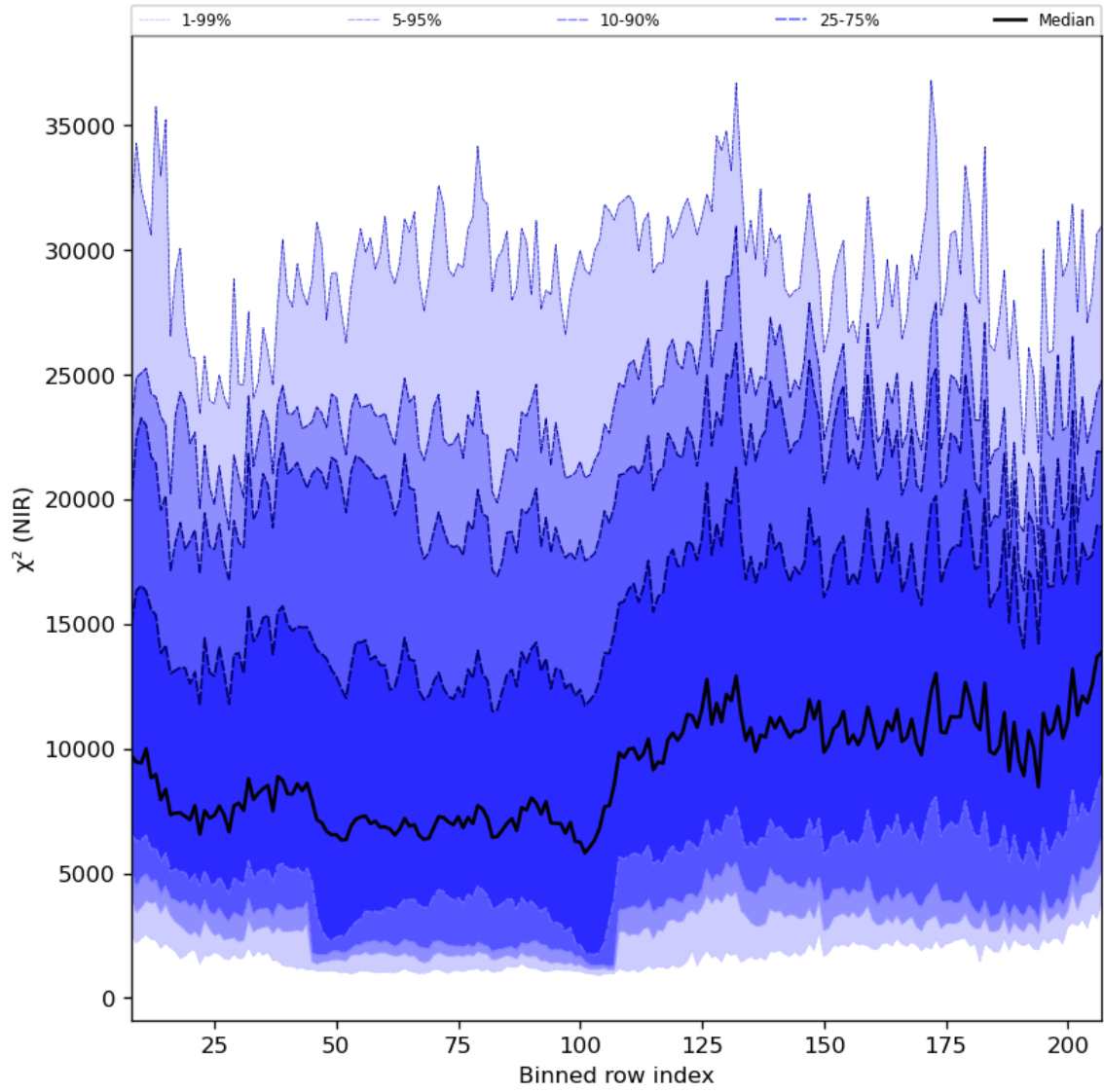
Figure 40: Along track statistics of “ \chi^2 (NIR)” for 2024-04-27 to 2024-04-29
