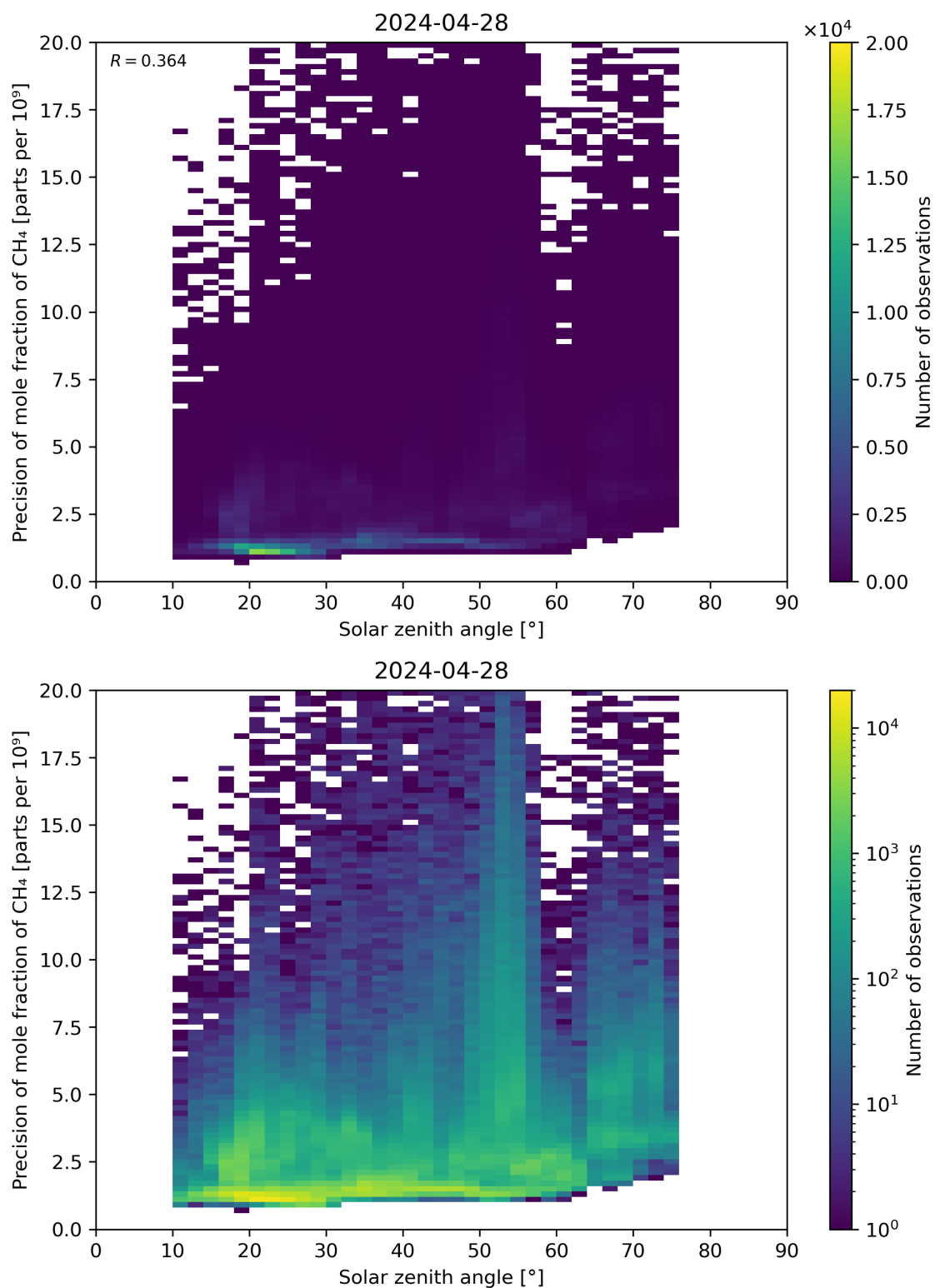
Figure 101: Scatter density plot of “Solar zenith angle” against “Precision of mole fraction of CH 4 ” for 2024-04-27 to 2024-04-29.
