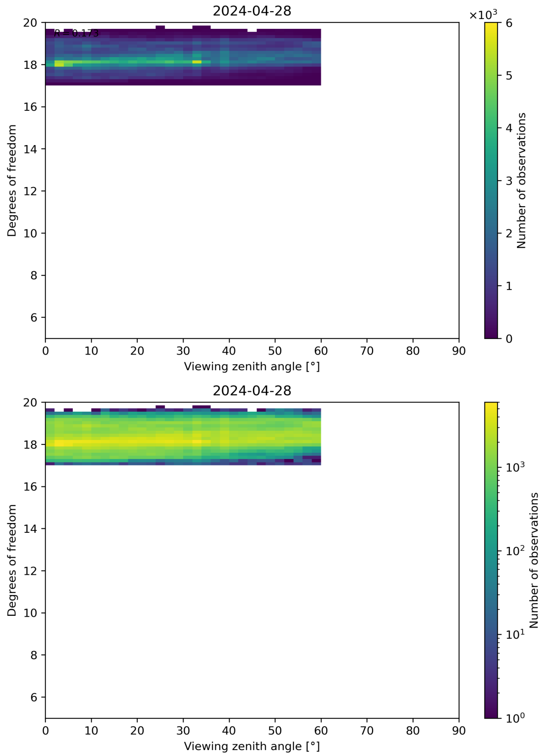
Figure 107: Scatter density plot of “Viewing zenith angle” against “Degrees of freedom” for 2024-04-27 to 2024-04-29.
