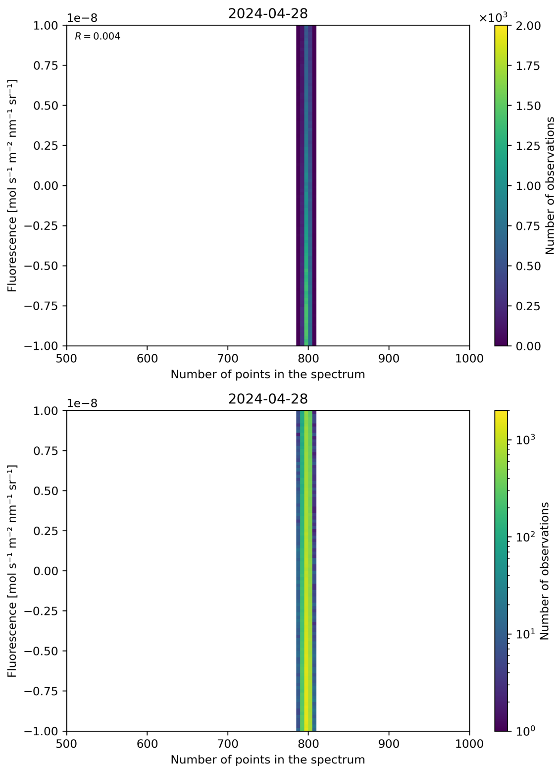
Figure 91: Scatter density plot of “Number of points in the spectrum” against “Fluorescence” for 2024-04-27 to 2024-04-29.
