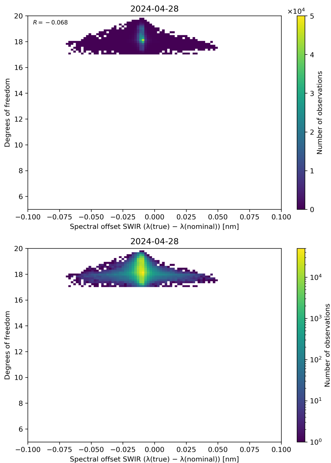
Figure 119: Scatter density plot of “Spectral offset SWIR ( \lambda(\text{true}) - \lambda(\text{nominal}) )” against “Degrees of freedom” for 2024-04-27 to 2024-04-29.
