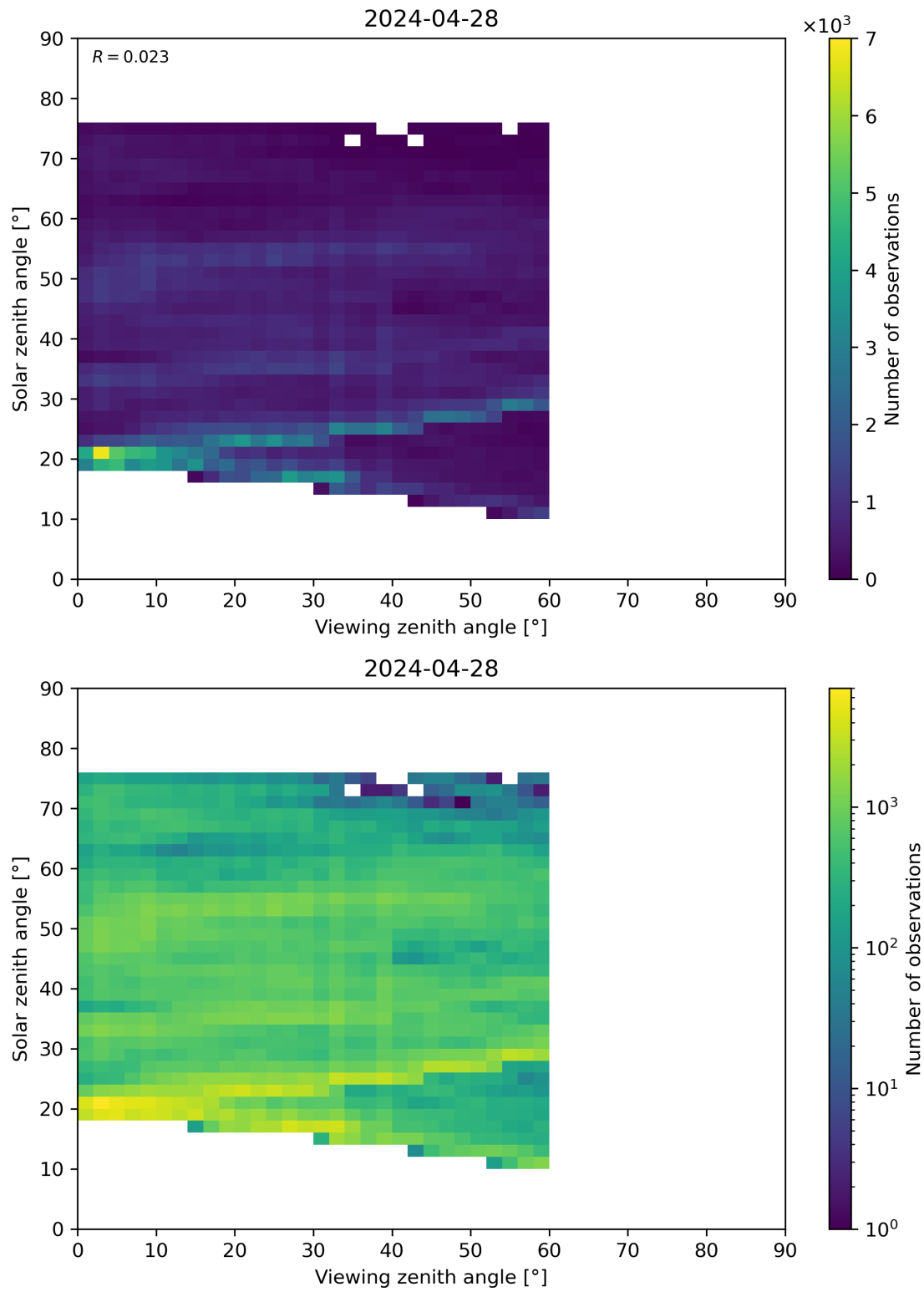
Figure 115: Scatter density plot of “Viewing zenith angle” against “Solar zenith angle” for 2024-04-27 to 2024-04-29.
