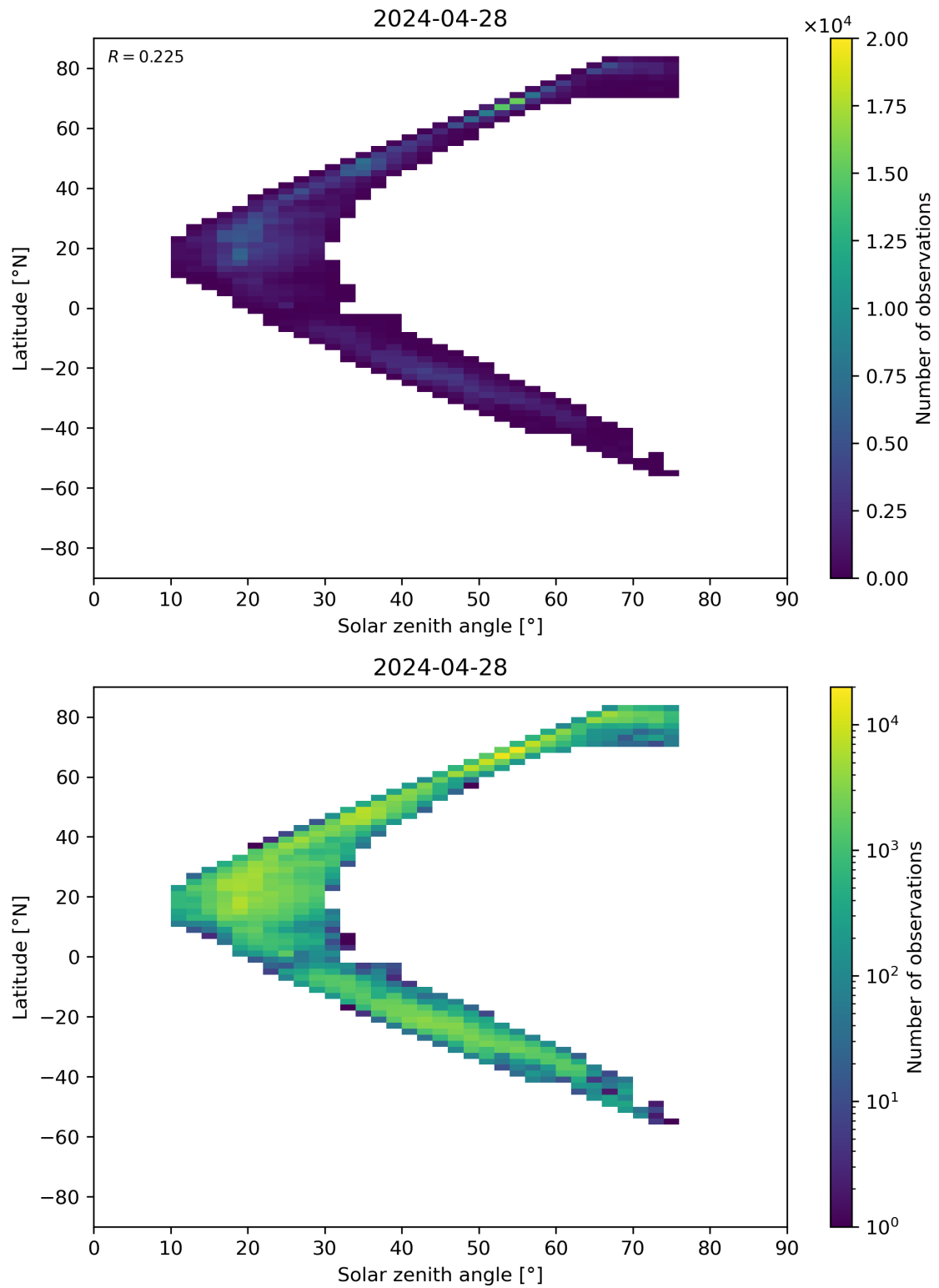
Figure 98: Scatter density plot of “Solar zenith angle” against “Latitude” for 2024-04-27 to 2024-04-29.
