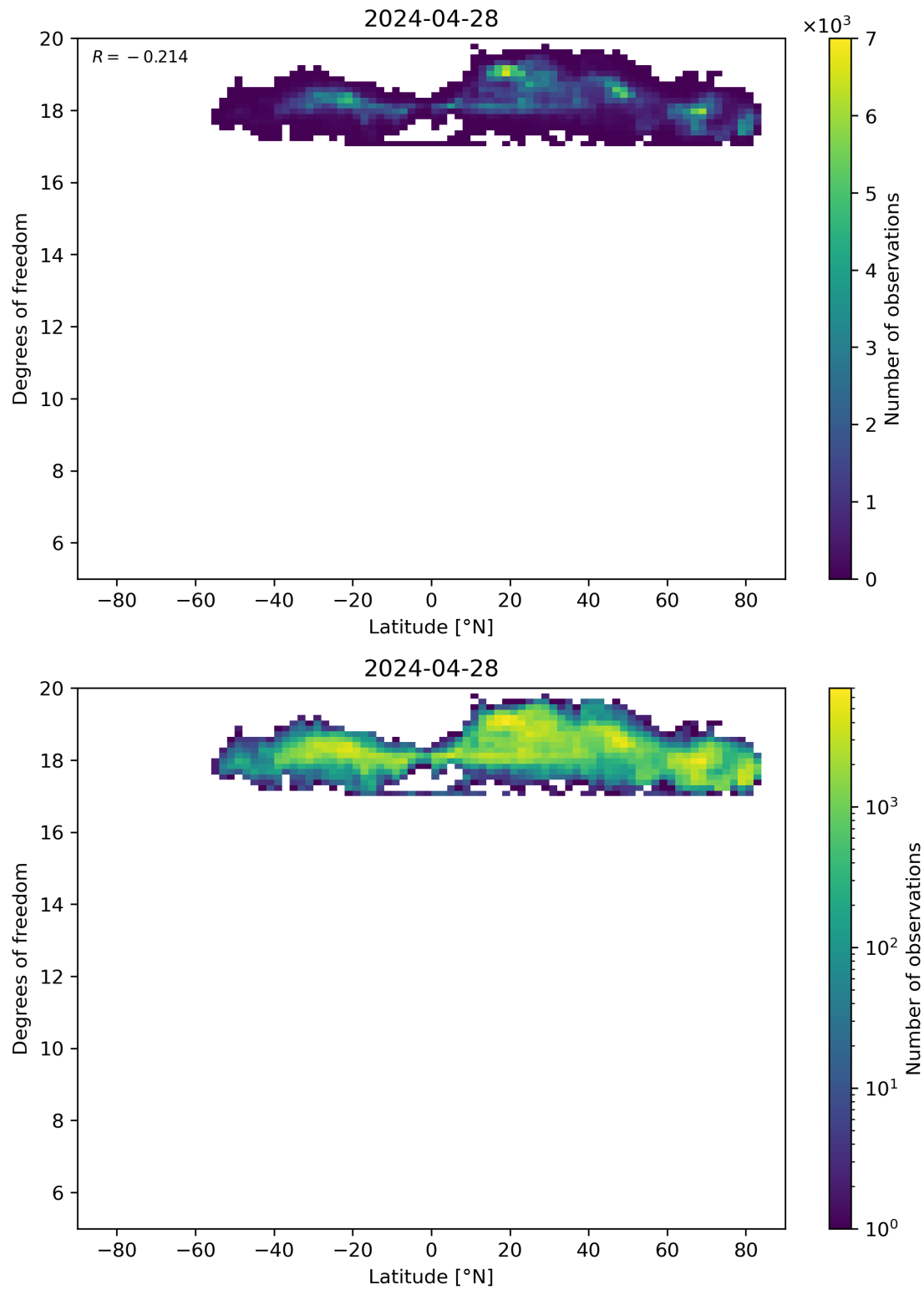
Figure 55: Scatter density plot of “Latitude” against “Degrees of freedom” for 2024-04-27 to 2024-04-29.
