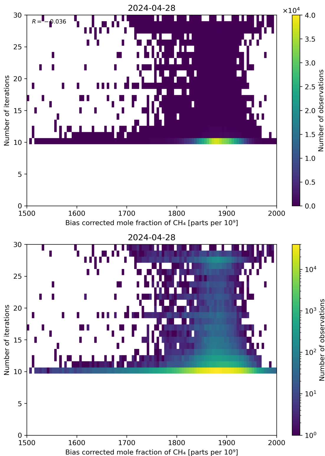
Figure 67: Scatter density plot of “Bias corrected mole fraction of CH 4 ” against “Number of iterations” for 2024-04-27 to 2024-04-29.
