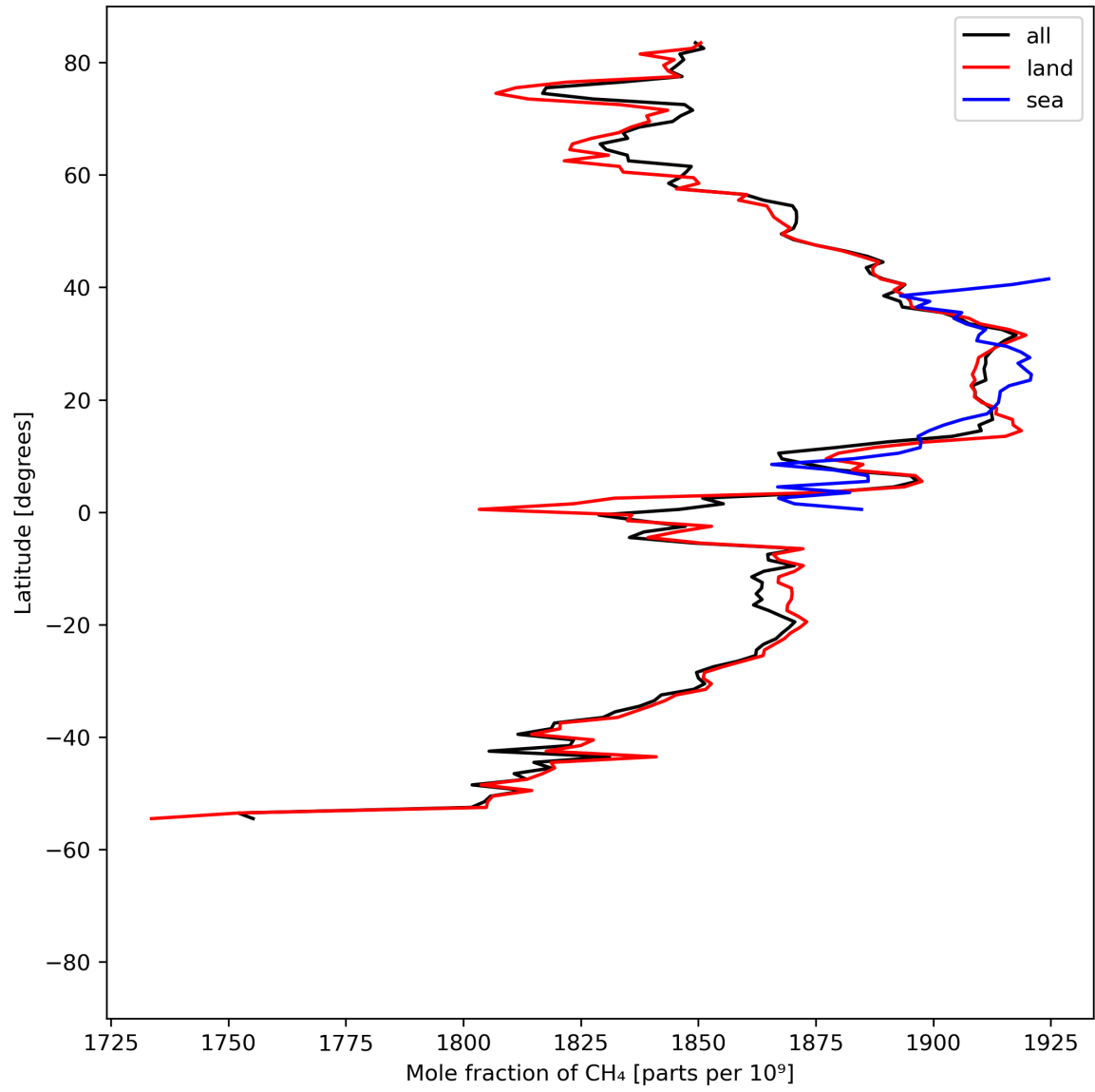
Figure 12: Zonal average of “Mole fraction of CH 4 ” for 2024-04-27 to 2024-04-29.
