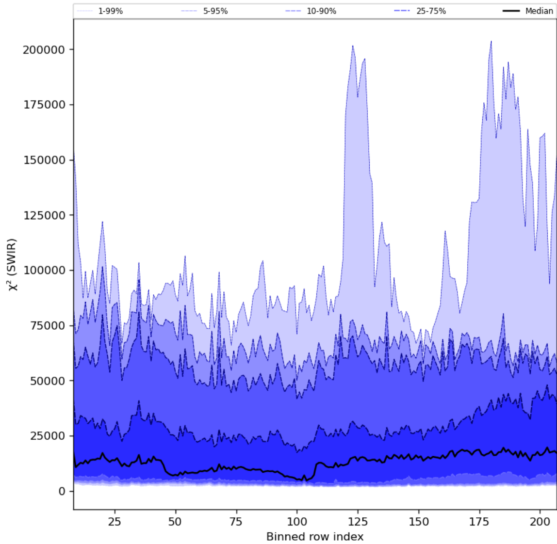
Figure 39: Along track statistics of “ \chi^2 (SWIR)” for 2024-04-27 to 2024-04-29
