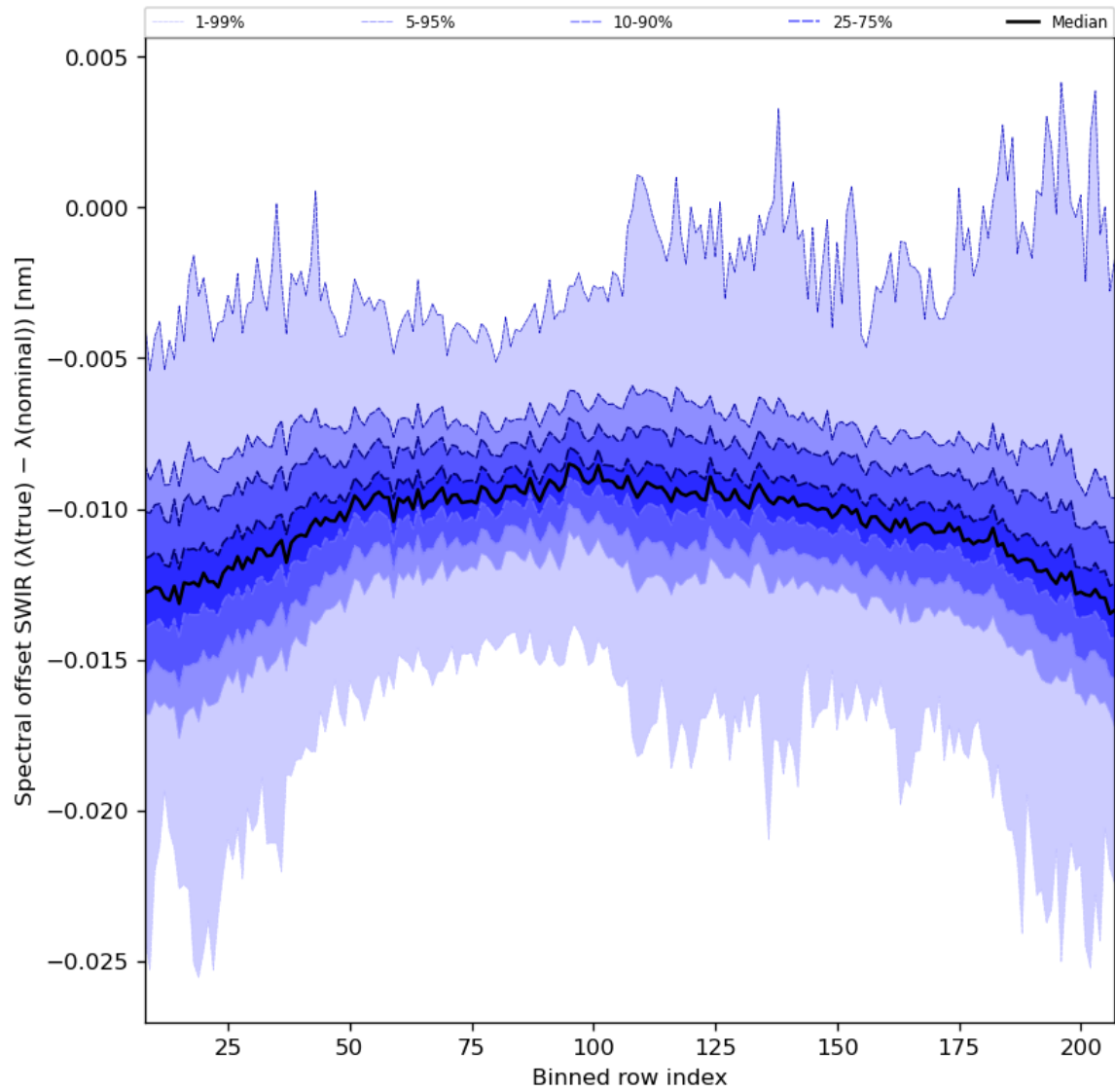
Figure 38: Along track statistics of “Spectral offset SWIR ( \lambda(\text{true}) - \lambda(\text{nominal}) )” for 2024-04-27 to 2024-04-29
