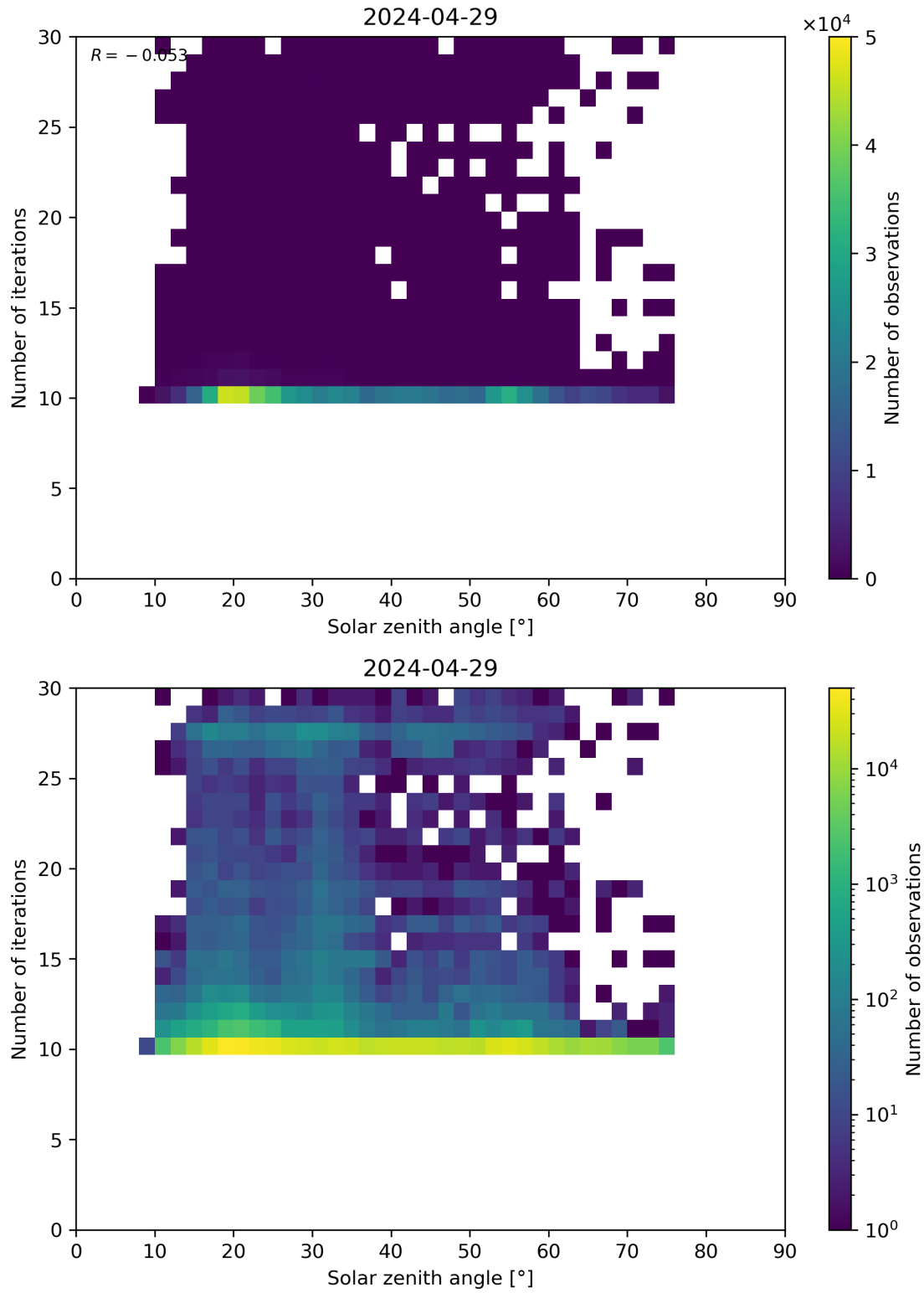
Figure 102: Scatter density plot of “Solar zenith angle” against “Number of iterations” for 2024-04-28 to 2024-04-30.
