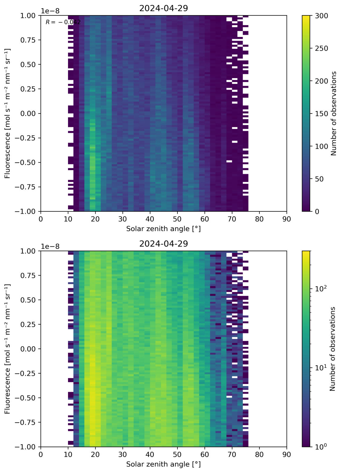
Figure 97: Scatter density plot of “Solar zenith angle” against “Fluorescence” for 2024-04-28 to 2024-04-30.
