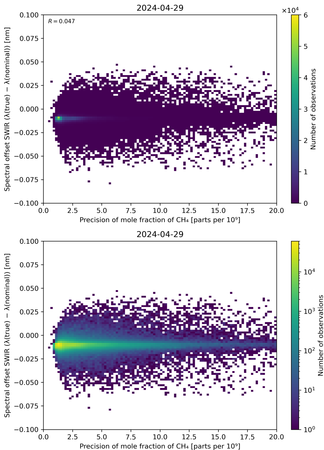
Figure 85: Scatter density plot of “Precision of mole fraction of \text{CH}_4 ” against “Spectral offset SWIR ( \lambda(\text{true}) - \lambda(\text{nominal}) )” for 2024-04-28 to 2024-04-30.
