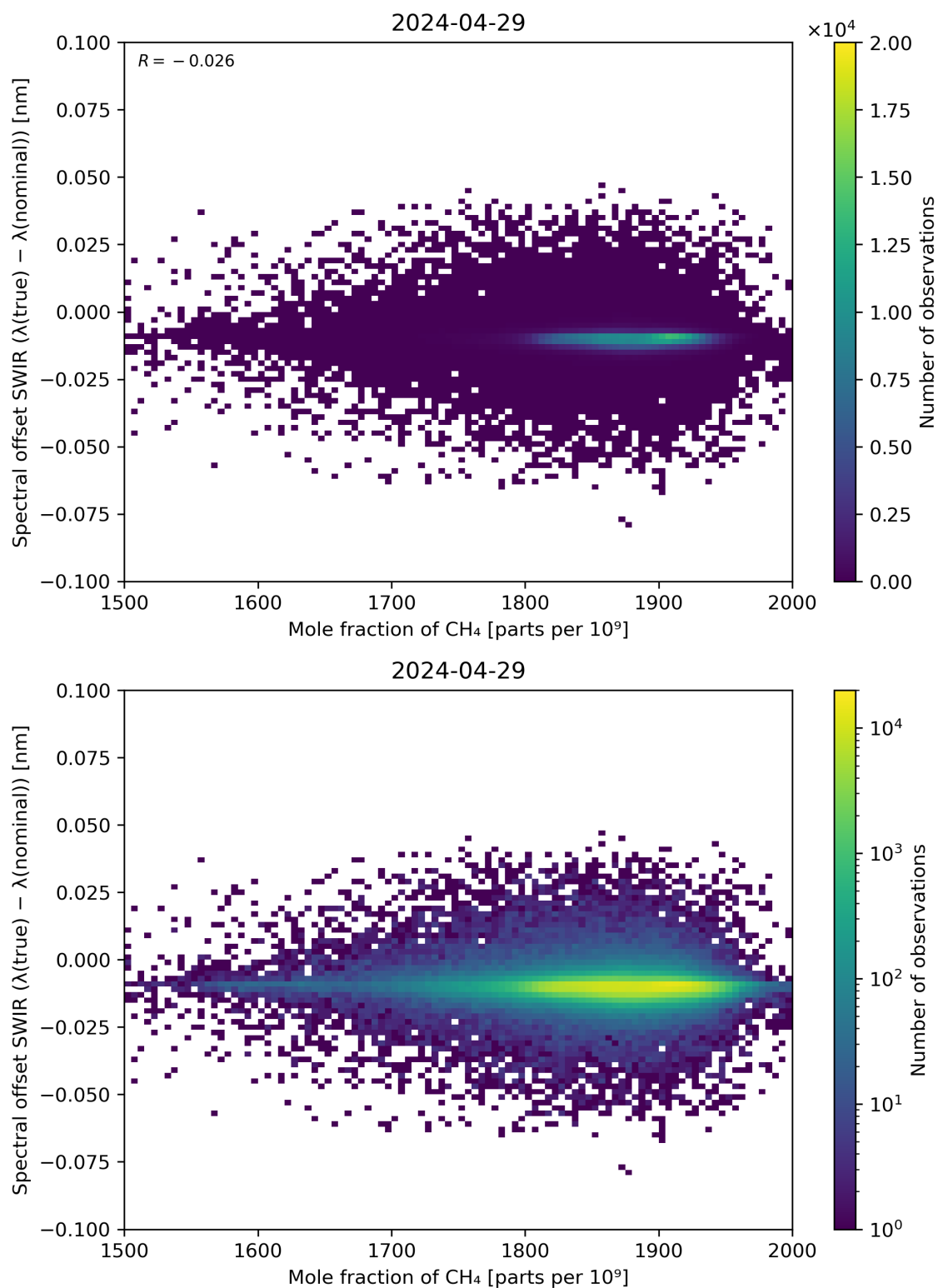
Figure 86: Scatter density plot of “Mole fraction of CH 4 ” against “Spectral offset SWIR ( \lambda(\text{true}) - \lambda(\text{nominal}) )” for 2024-04-28 to 2024-04-30.
