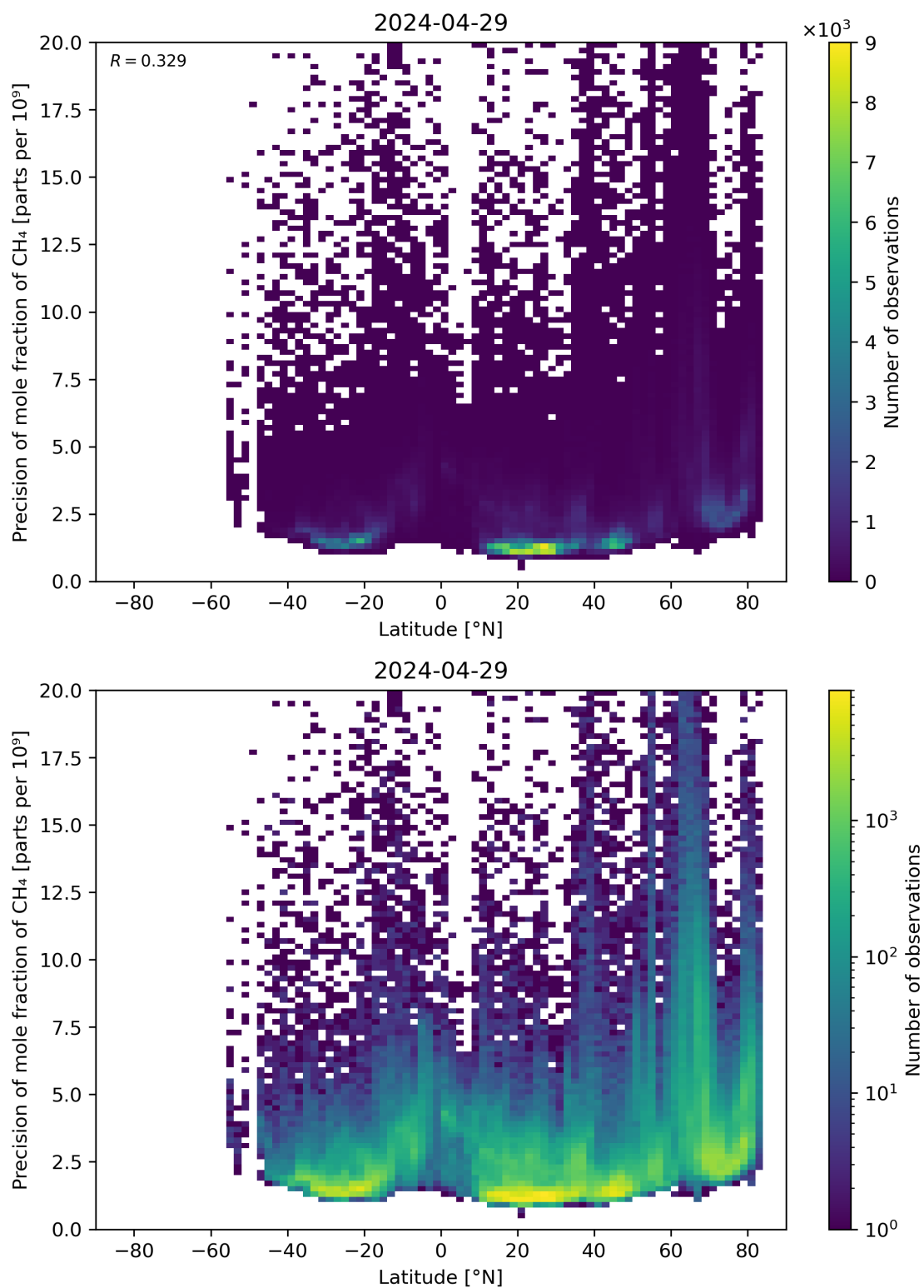
Figure 59: Scatter density plot of “Latitude” against “Precision of mole fraction of CH 4 ” for 2024-04-28 to 2024-04-30.
