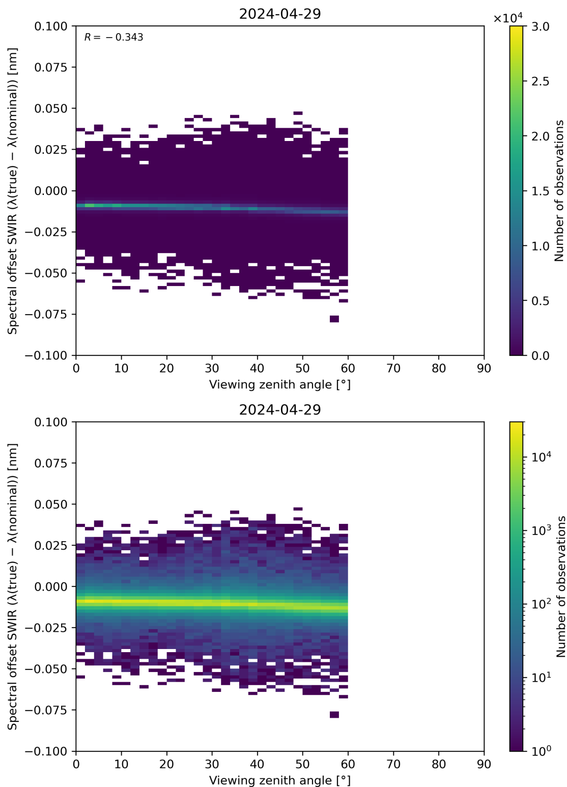
Figure 116: Scatter density plot of “Viewing zenith angle” against “Spectral offset SWIR ( \lambda(\text{true}) - \lambda(\text{nominal}) )” for 2024-04-28 to 2024-04-30.
