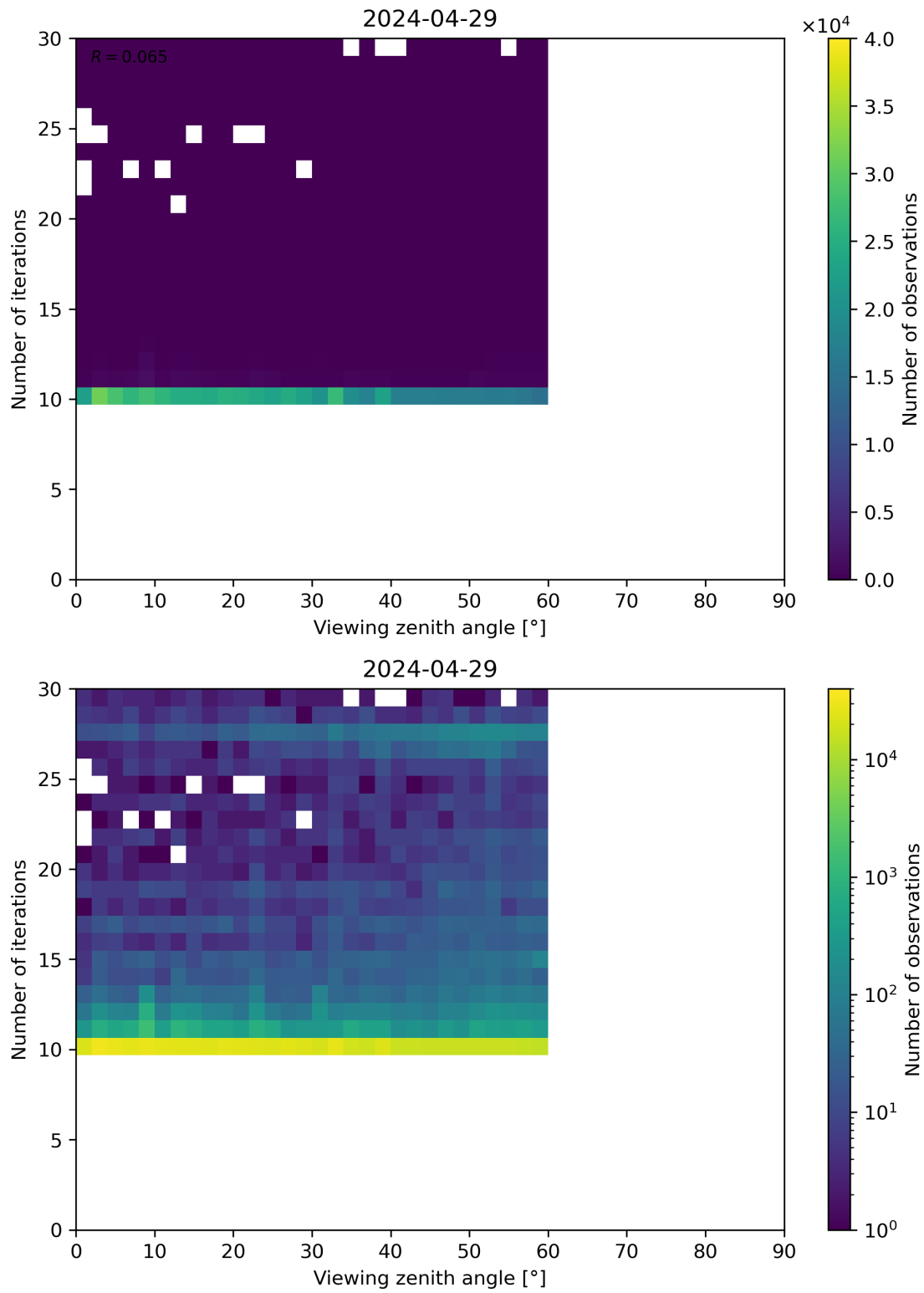
Figure 113: Scatter density plot of “Viewing zenith angle” against “Number of iterations” for 2024-04-28 to 2024-04-30.
