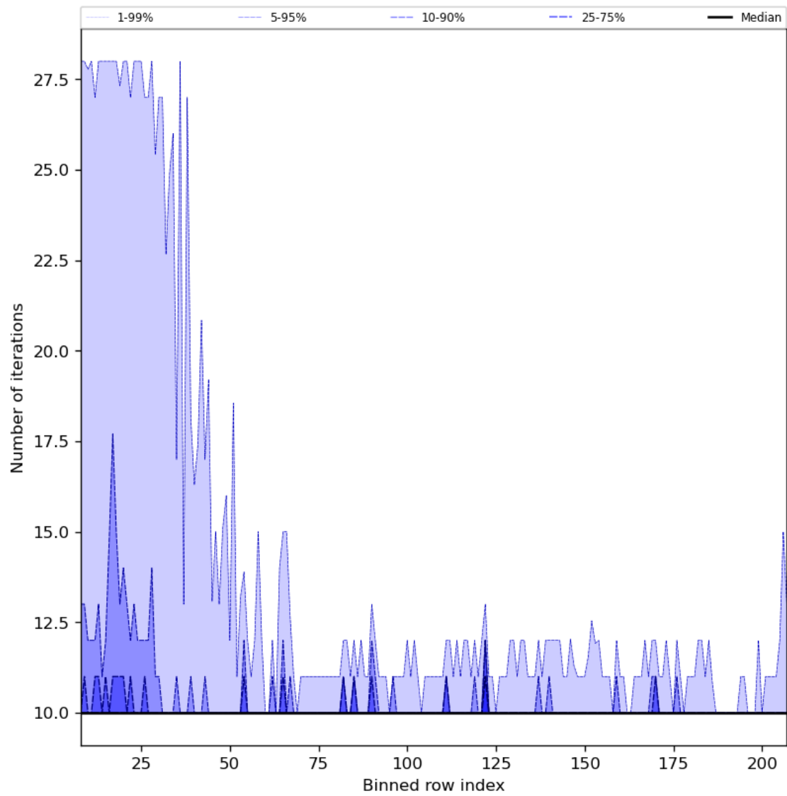
Figure 42: Along track statistics of “Number of iterations” for 2024-04-28 to 2024-04-30
