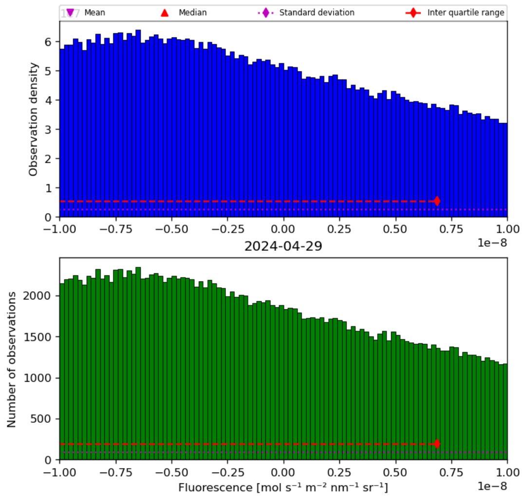
Figure 32: Histogram of “Fluorescence” for 2024-04-28 to 2024-04-30
