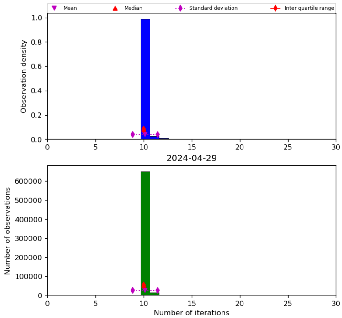
Figure 31: Histogram of "Number of iterations" for 2024-04-28 to 2024-04-30
