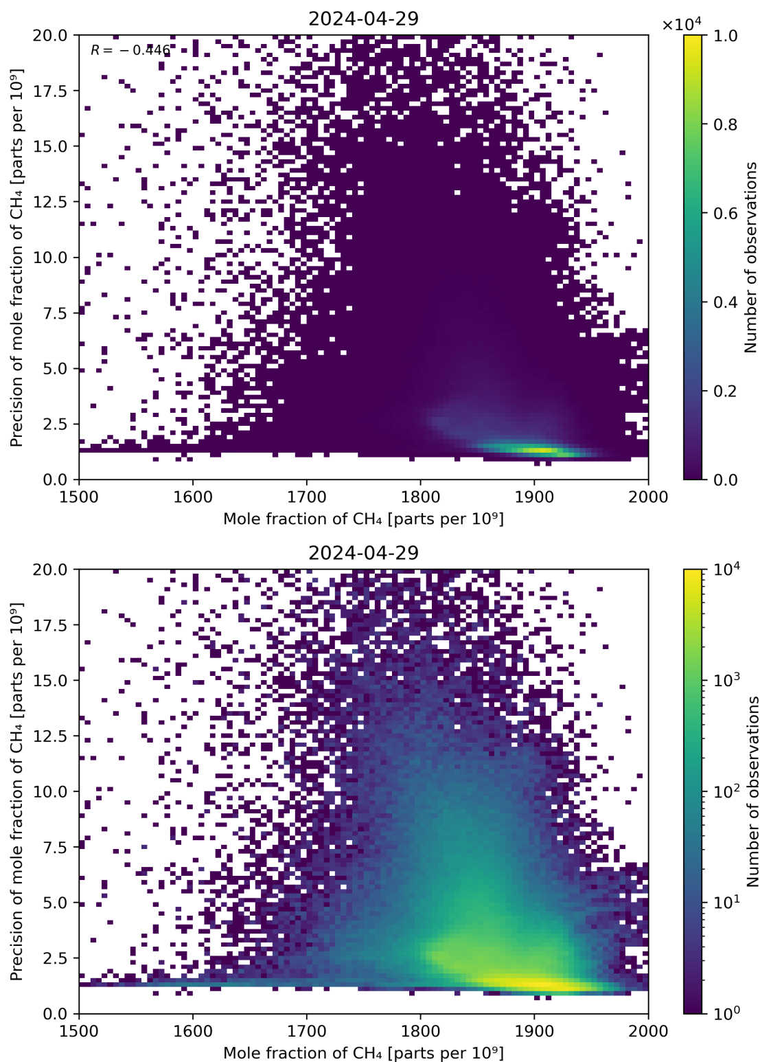
Figure 75: Scatter density plot of “Mole fraction of CH 4 ” against “Precision of mole fraction of CH 4 ” for 2024-04-28 to 2024-04-30.
