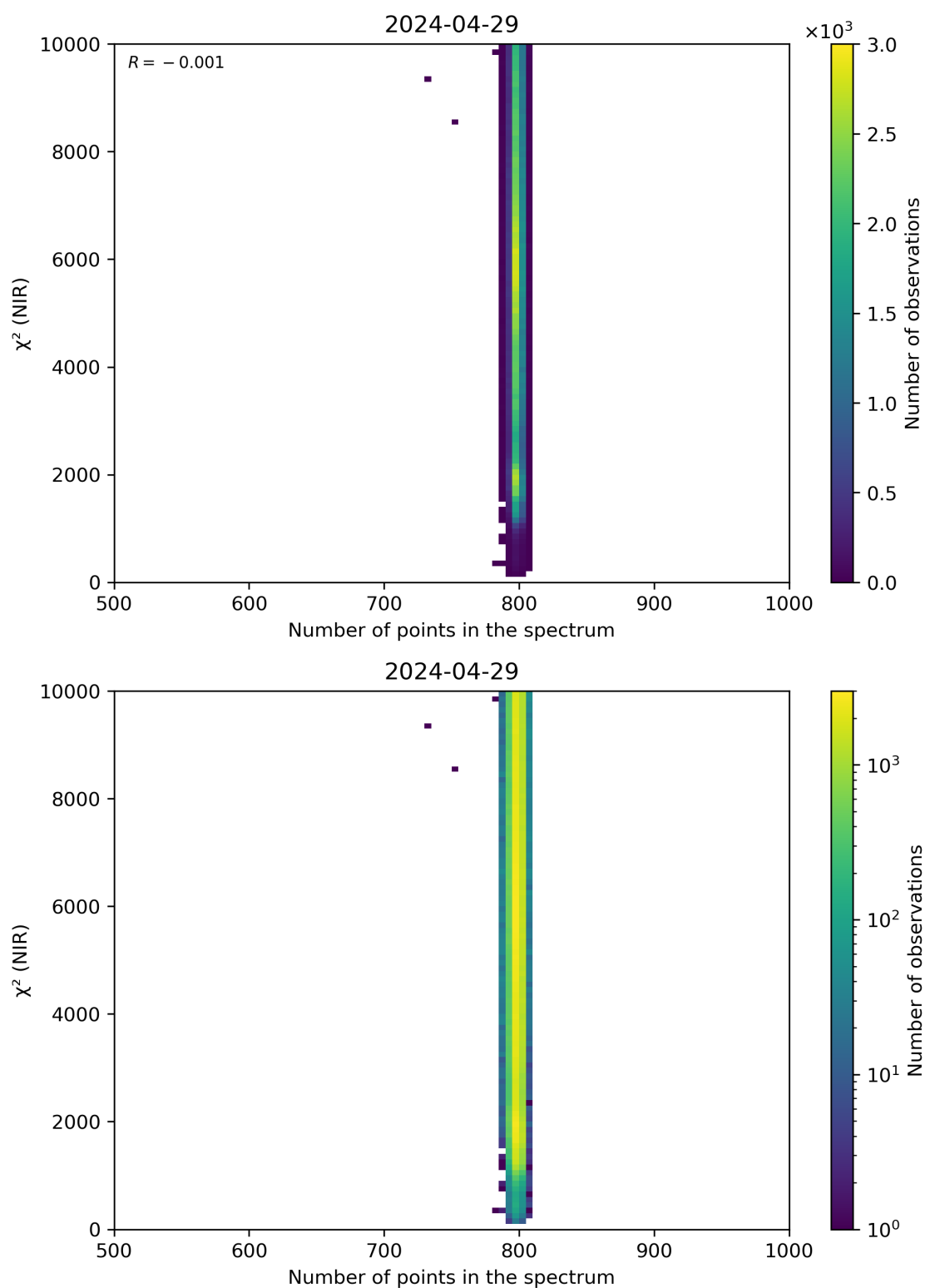
Figure 88: Scatter density plot of “Number of points in the spectrum” against “ \chi^2 (NIR)” for 2024-04-28 to 2024-04-30.
