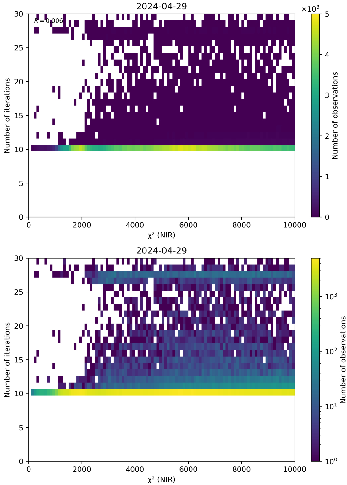
Figure 46: Scatter density plot of “ \chi^2 (NIR)” against “Number of iterations” for 2024-04-28 to 2024-04-30.
