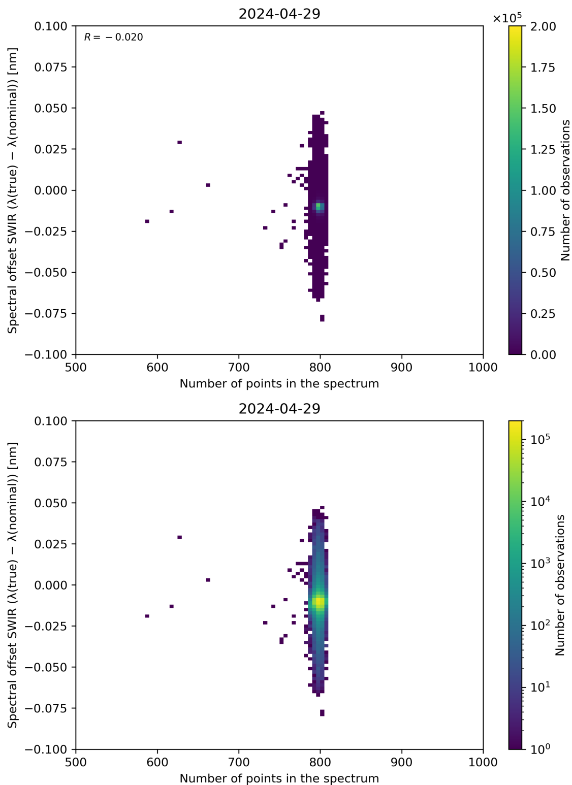
Figure 93: Scatter density plot of “Number of points in the spectrum” against “Spectral offset SWIR ( \lambda(\text{true}) - \lambda(\text{nominal}) )” for 2024-04-28 to 2024-04-30.
