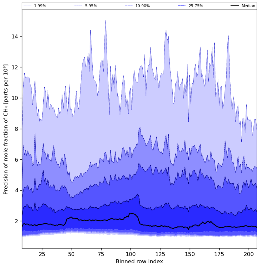
Figure 35: Along track statistics of “Precision of mole fraction of CH 4 ” for 2024-04-28 to 2024-04-30
