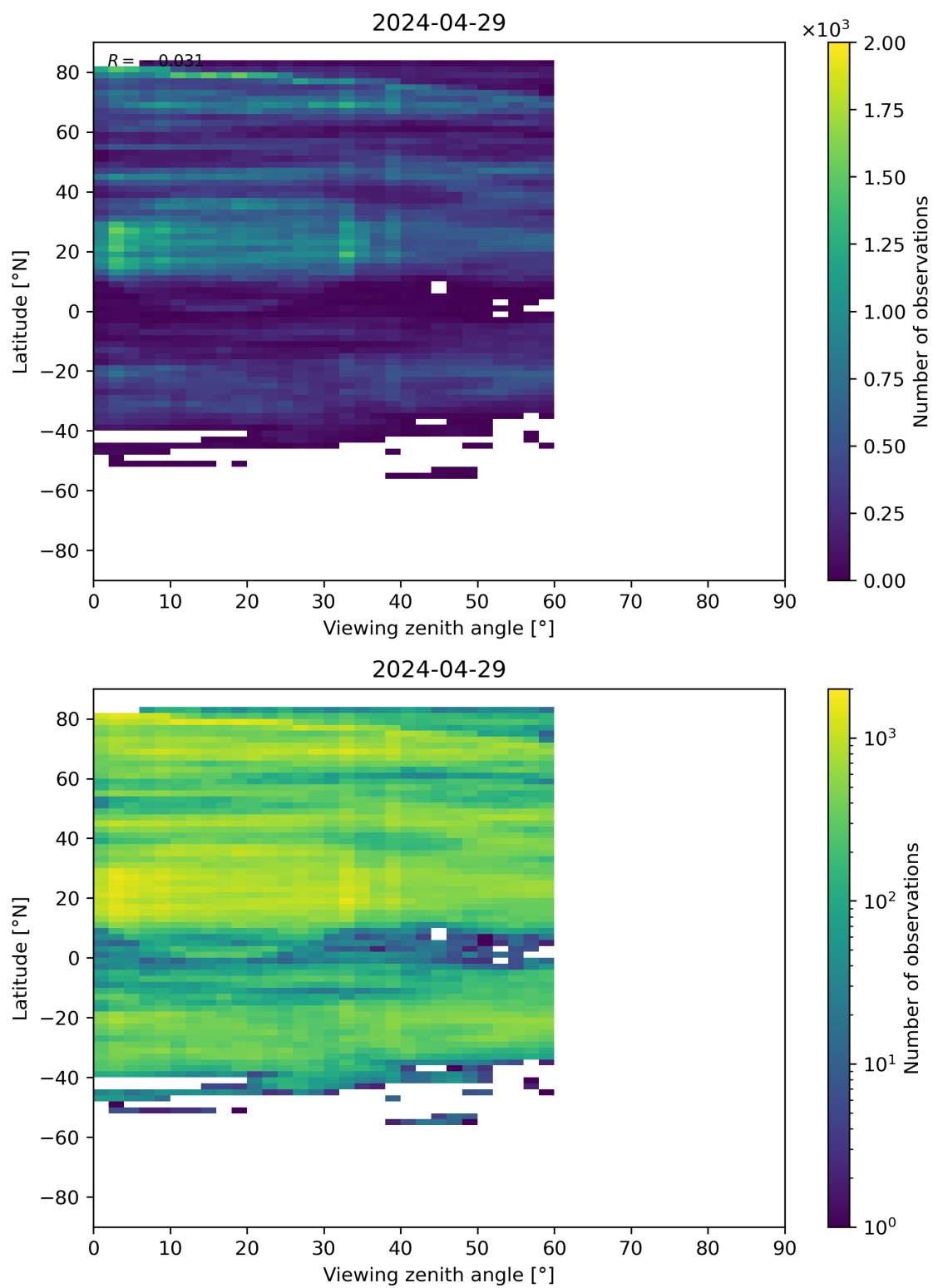
Figure 109: Scatter density plot of “Viewing zenith angle” against “Latitude” for 2024-04-28 to 2024-04-30.
