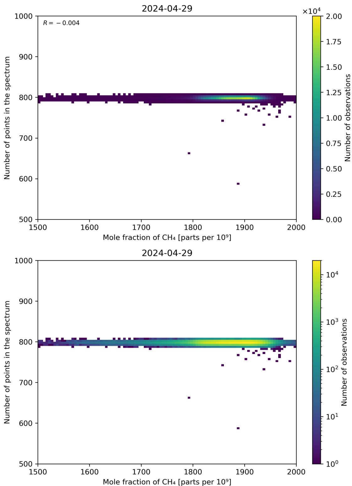
Figure 77: Scatter density plot of “Mole fraction of CH 4 ” against “Number of points in the spectrum” for 2024-04-28 to 2024-04-30.
