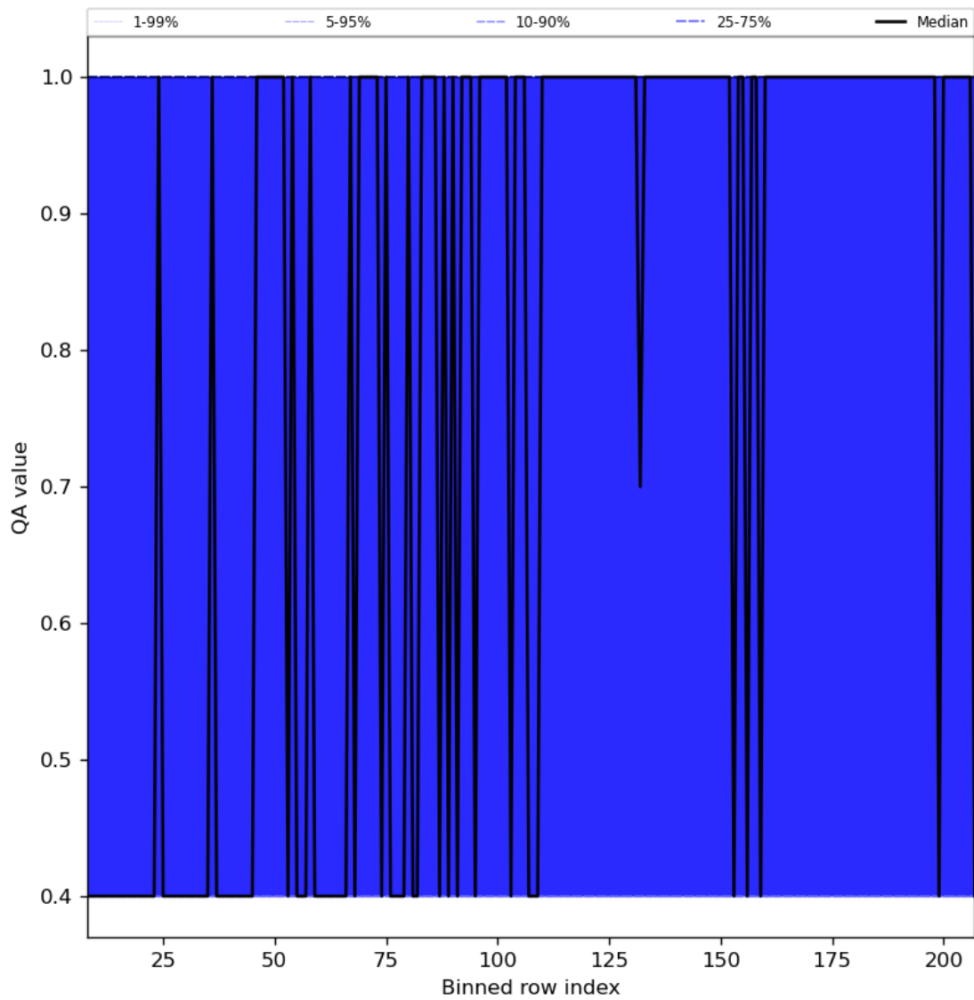
Figure 33: Along track statistics of “QA value” for 2024-04-28 to 2024-04-30
