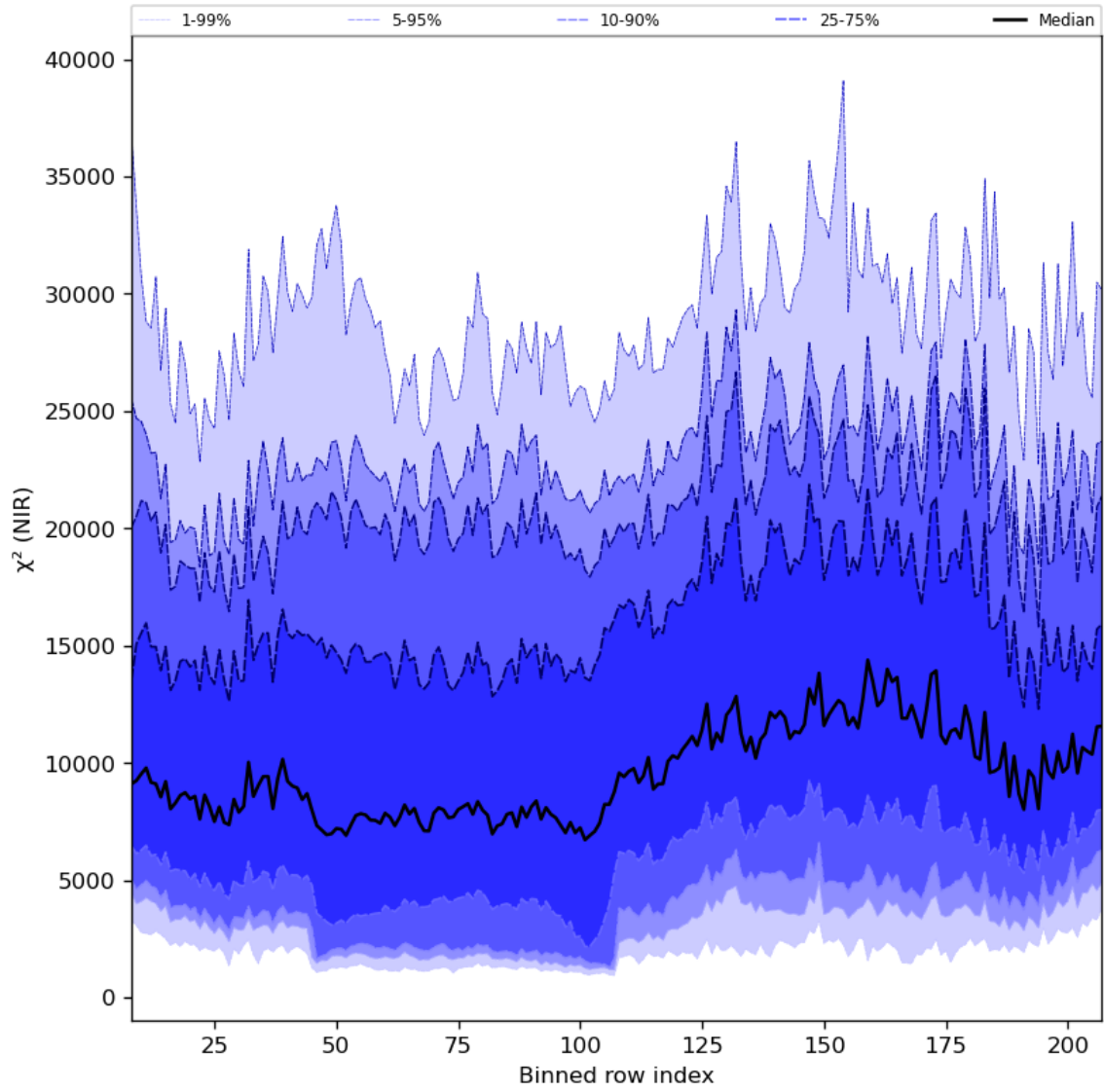
Figure 40: Along track statistics of “ \chi^2 (NIR)” for 2024-04-28 to 2024-04-30
