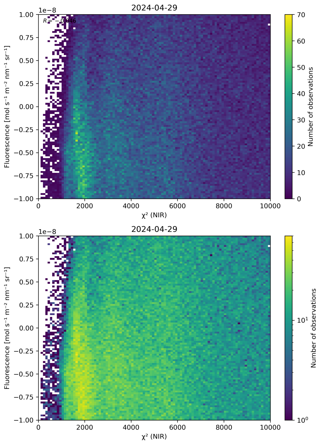
Figure 45: Scatter density plot of “ \chi^2 (NIR)” against “Fluorescence” for 2024-04-28 to 2024-04-30.
