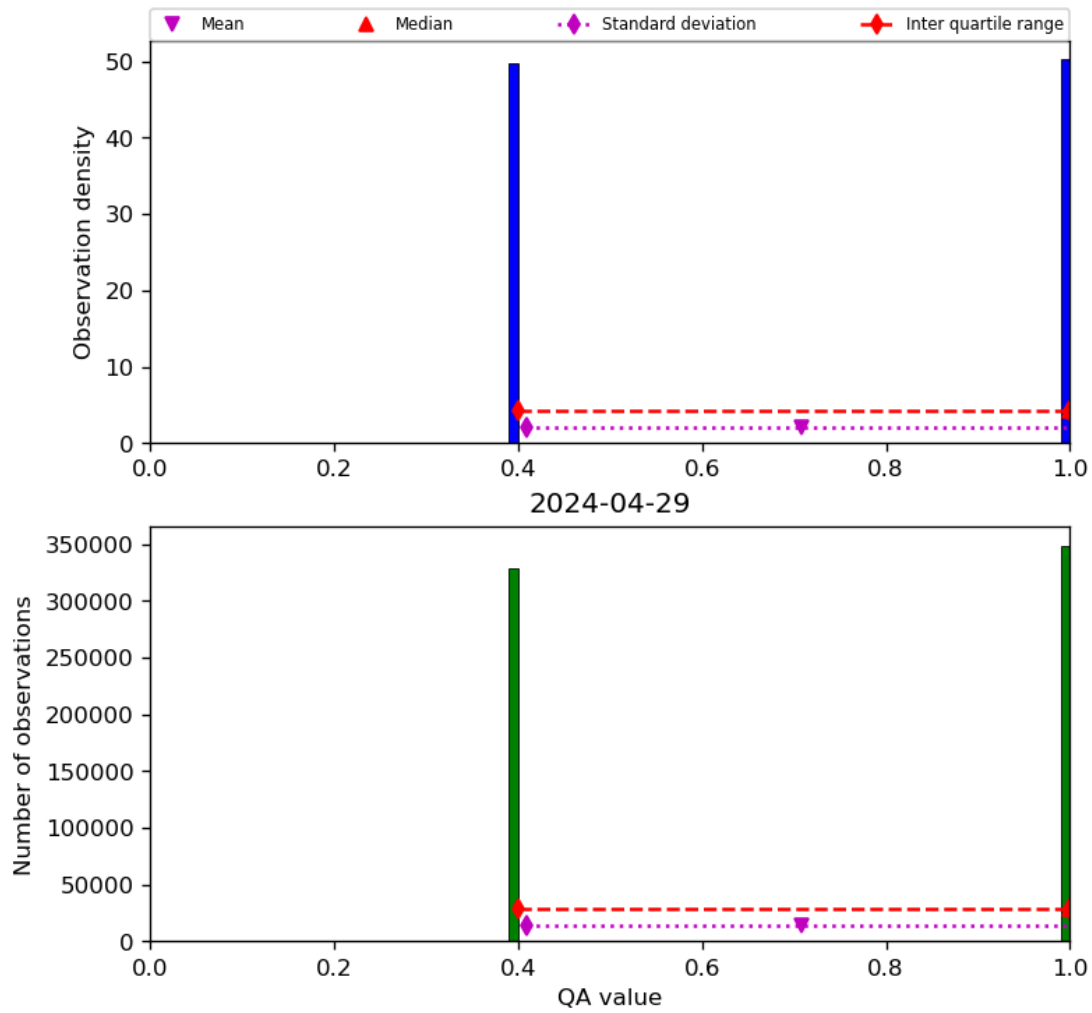
Figure 22: Histogram of “QA value” for 2024-04-28 to 2024-04-30
