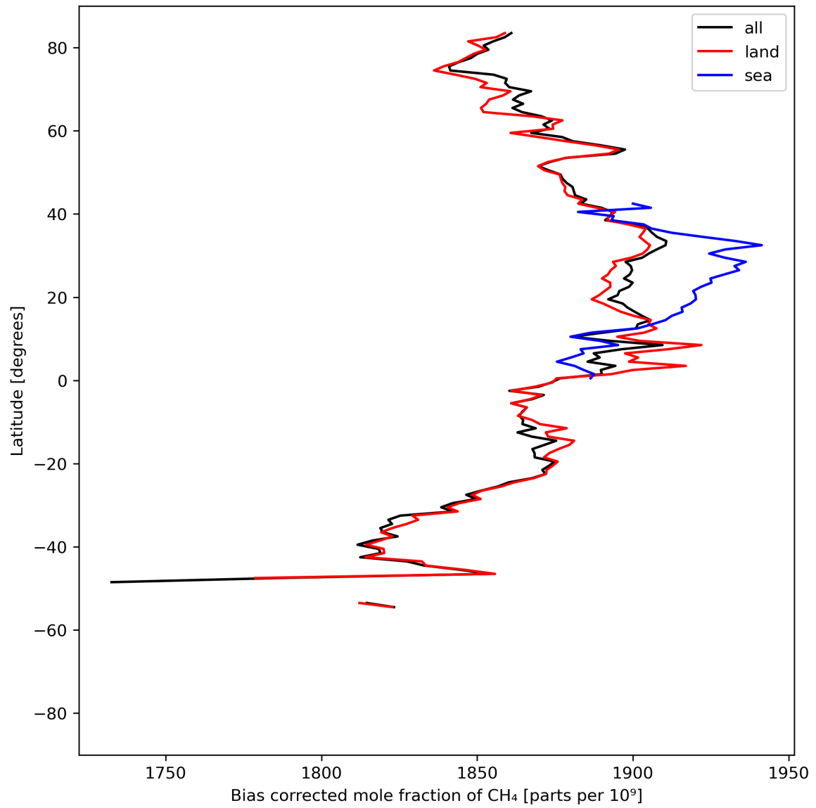
Figure 14: Zonal average of “Bias corrected mole fraction of \text{CH}_4 ” for 2024-04-28 to 2024-04-30.
