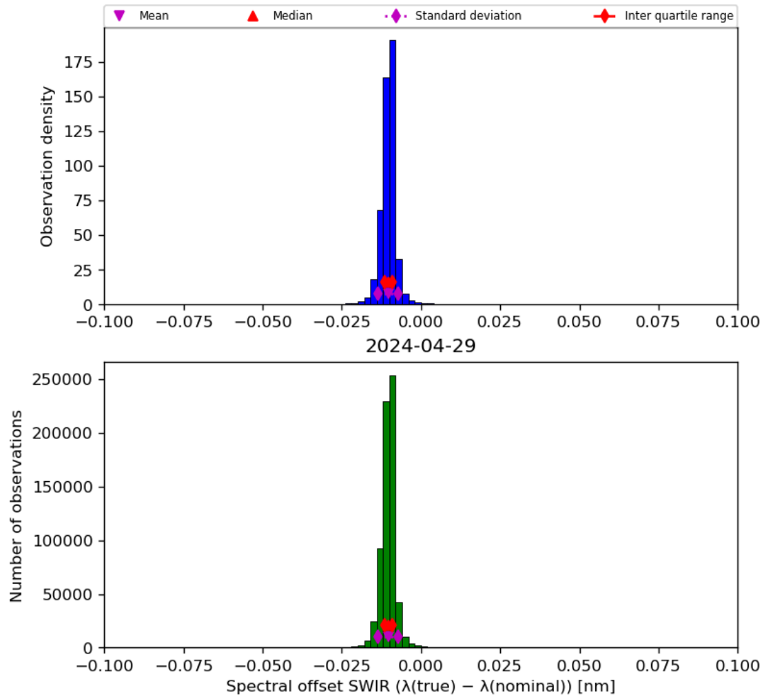
Figure 27: Histogram of “Spectral offset SWIR ( \lambda(\text{true}) - \lambda(\text{nominal}) )” for 2024-04-28 to 2024-04-30
