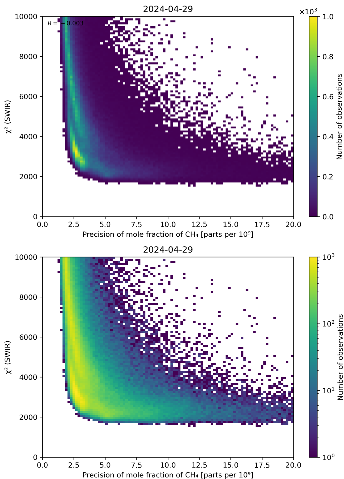
Figure 79: Scatter density plot of “Precision of mole fraction of CH 4 ” against “ \chi^2 (SWIR)” for 2024-04-28 to 2024-04-30.
