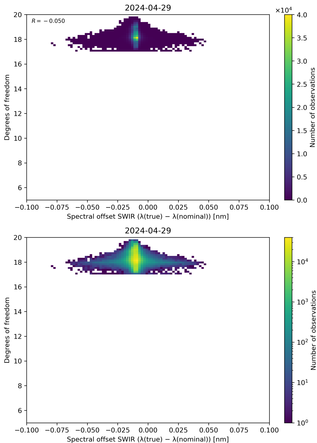
Figure 119: Scatter density plot of “Spectral offset SWIR ( \lambda(\text{true}) - \lambda(\text{nominal}) )” against “Degrees of freedom” for 2024-04-28 to 2024-04-30.
