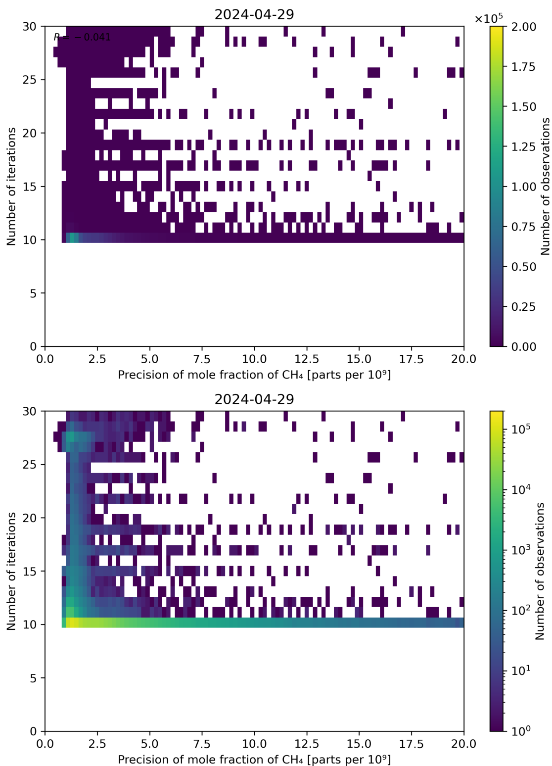
Figure 83: Scatter density plot of “Precision of mole fraction of CH 4 ” against “Number of iterations” for 2024-04-28 to 2024-04-30.
