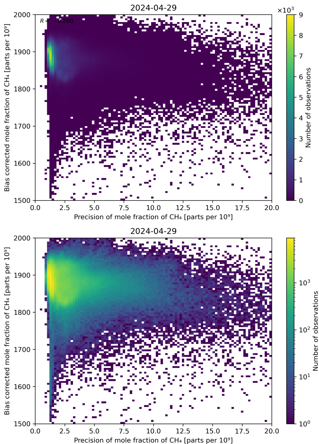
Figure 82: Scatter density plot of “Precision of mole fraction of CH 4 ” against “Bias corrected mole fraction of CH 4 ” for 2024-04-28 to 2024-04-30.
