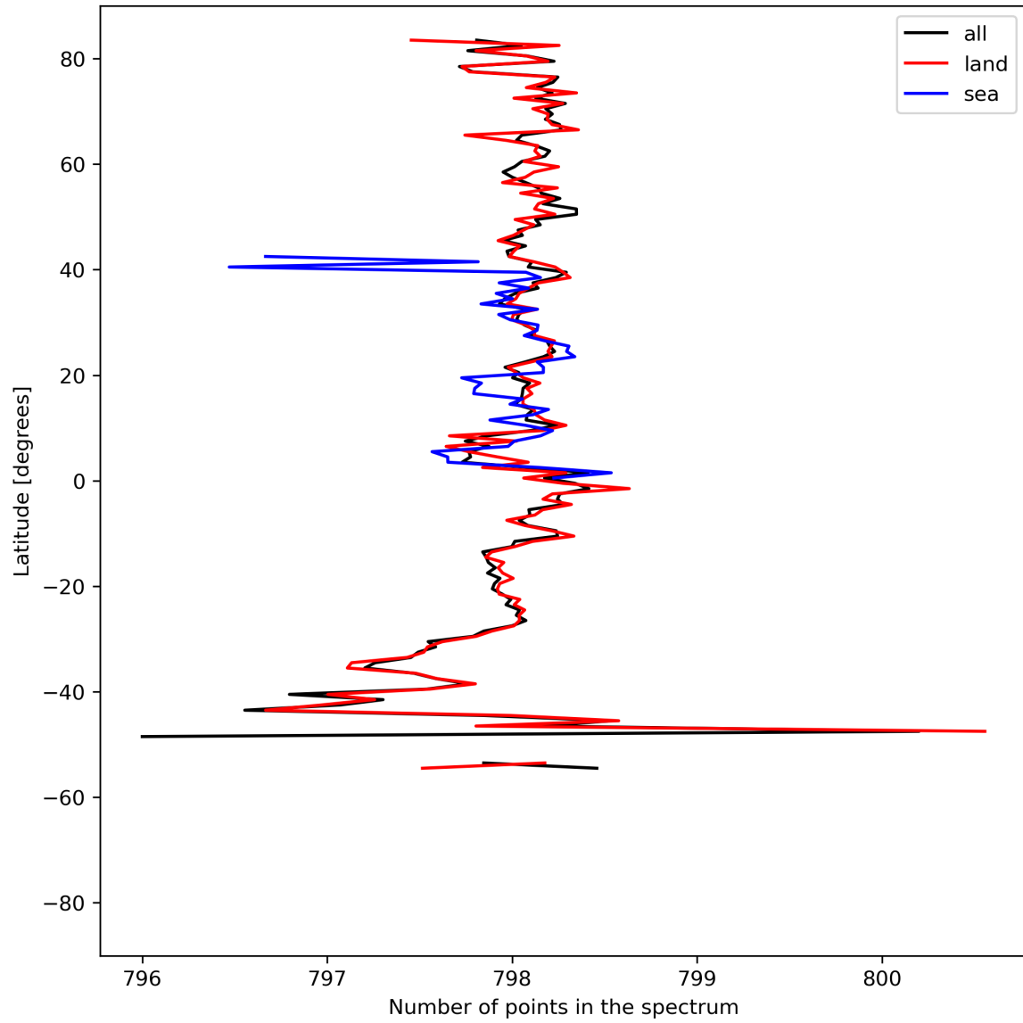
Figure 15: Zonal average of “Number of points in the spectrum” for 2024-04-28 to 2024-04-30.
