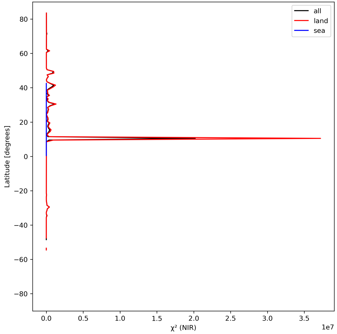
Figure 18: Zonal average of “ \chi^2 (NIR)” for 2024-04-28 to 2024-04-30.
