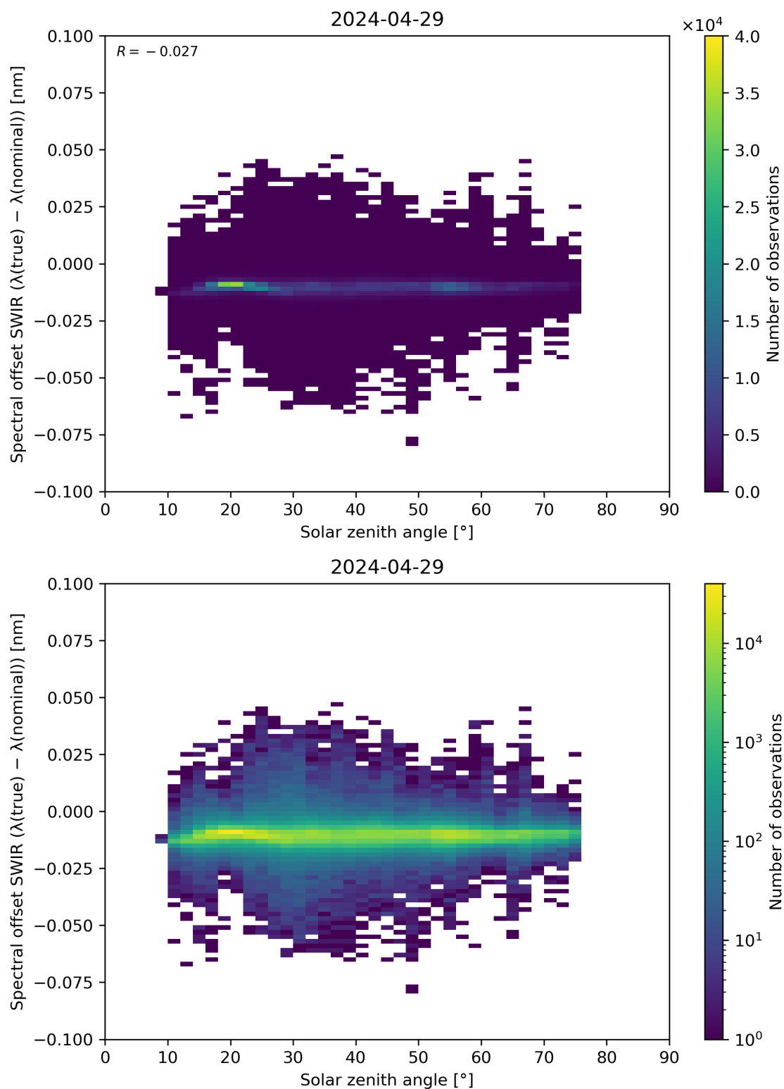
Figure 104: Scatter density plot of “Solar zenith angle” against “Spectral offset SWIR ( \lambda(\text{true}) - \lambda(\text{nominal}) )” for 2024-04-28 to 2024-04-30.
