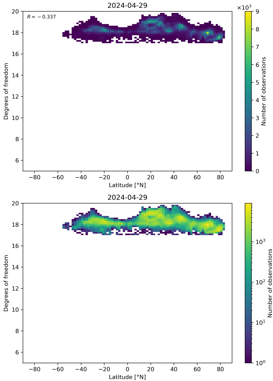
Figure 55: Scatter density plot of “Latitude” against “Degrees of freedom” for 2024-04-28 to 2024-04-30.
