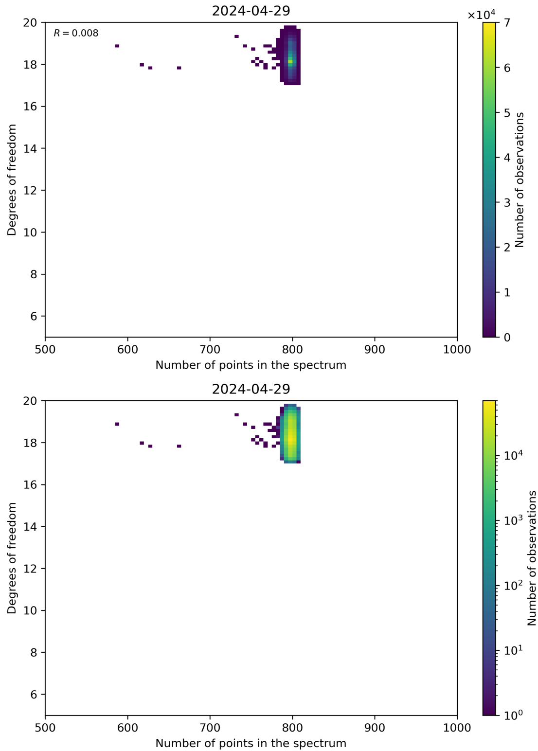
Figure 90: Scatter density plot of “Number of points in the spectrum” against “Degrees of freedom” for 2024-04-28 to 2024-04-30.
