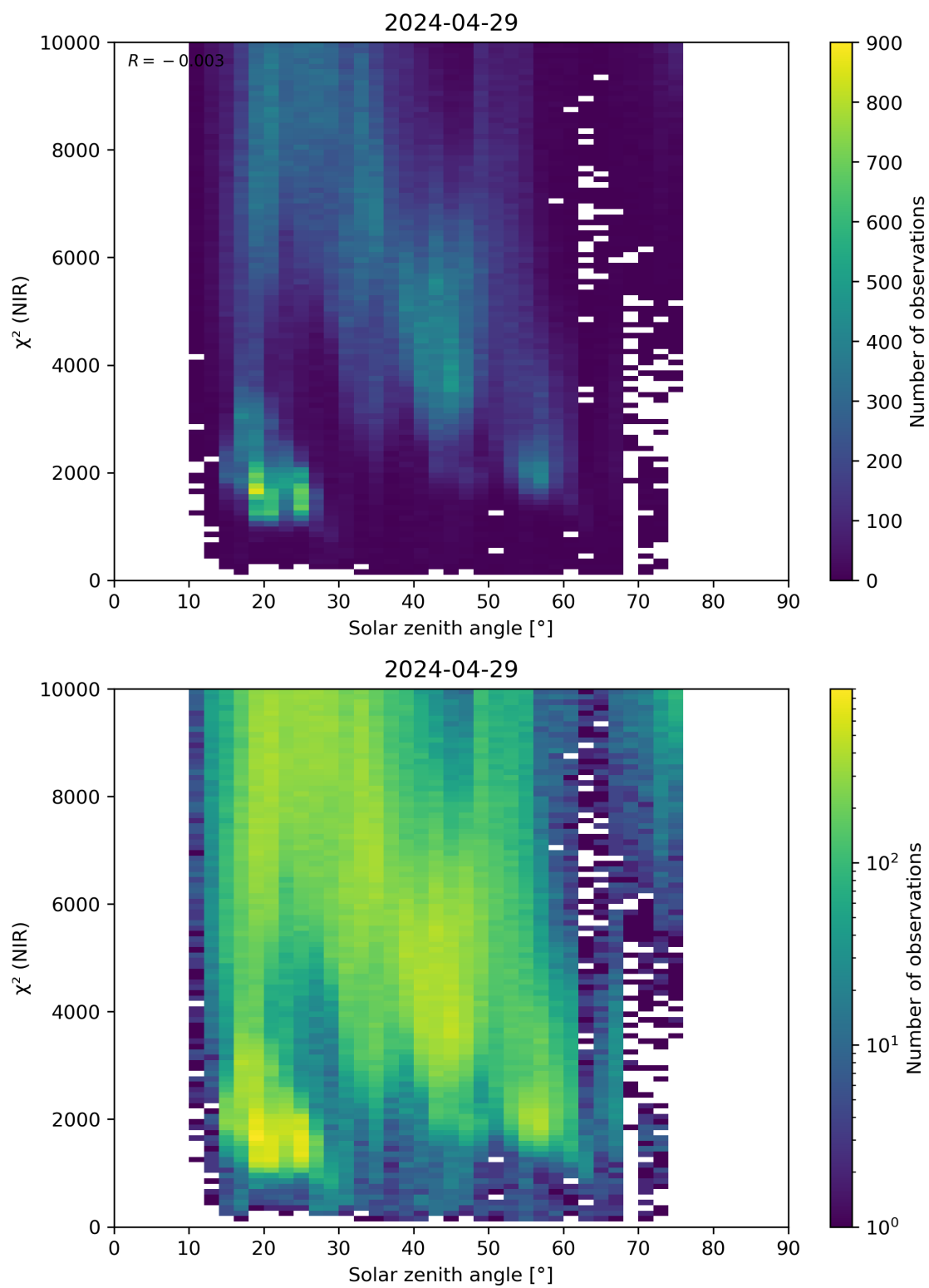
Figure 94: Scatter density plot of “Solar zenith angle” against “ \chi^2 (NIR)” for 2024-04-28 to 2024-04-30.
