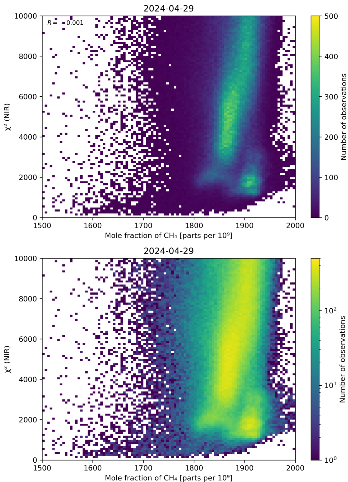
Figure 70: Scatter density plot of “Mole fraction of CH 4 ” against “ \chi^2 (NIR)” for 2024-04-28 to 2024-04-30.
