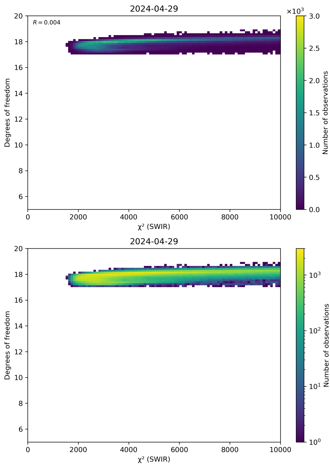
Figure 48: Scatter density plot of “ \chi^2 (SWIR)” against “Degrees of freedom” for 2024-04-28 to 2024-04-30.
