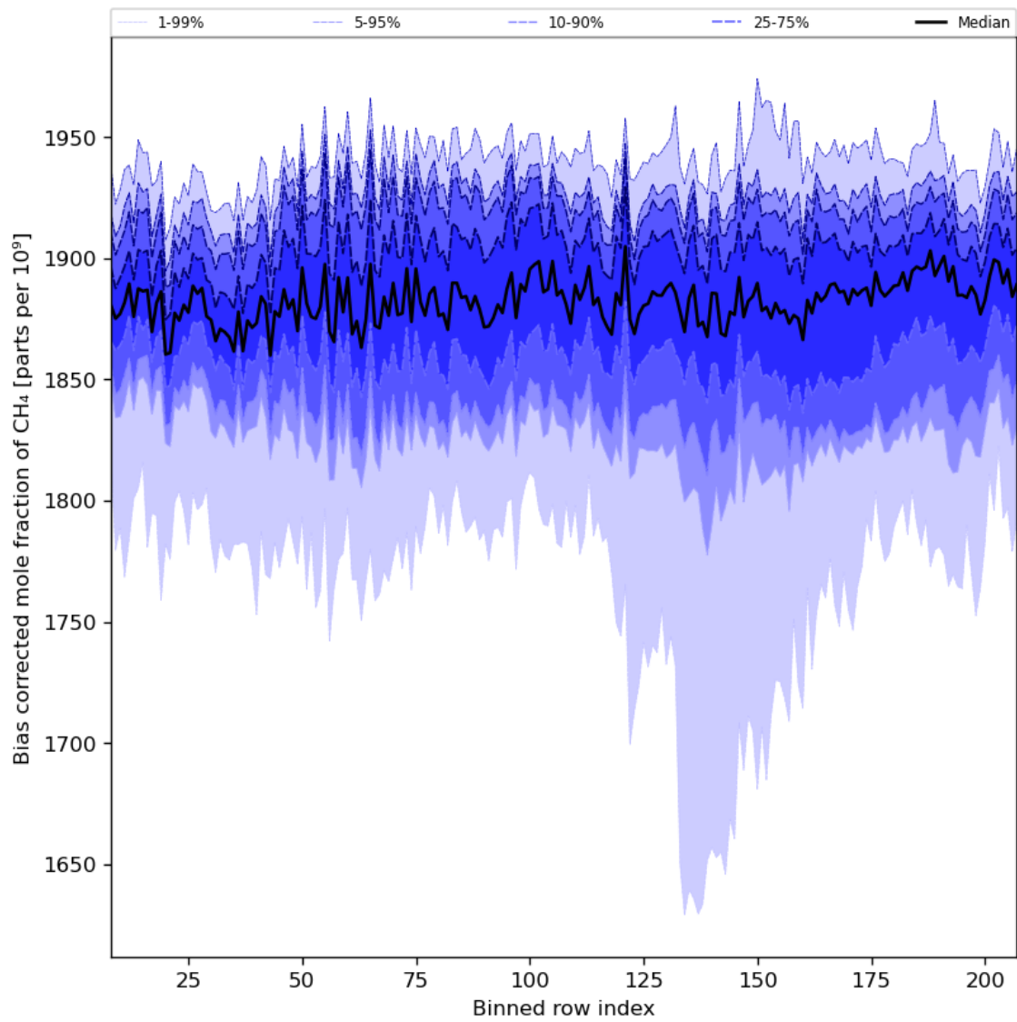
Figure 36: Along track statistics of “Bias corrected mole fraction of CH 4 ” for 2024-04-28 to 2024-04-30
