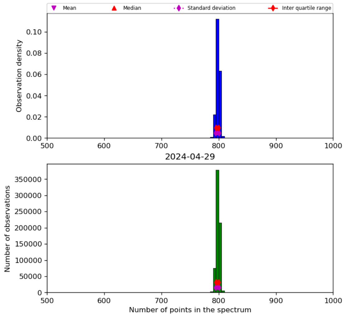
Figure 26: Histogram of “Number of points in the spectrum” for 2024-04-28 to 2024-04-30
