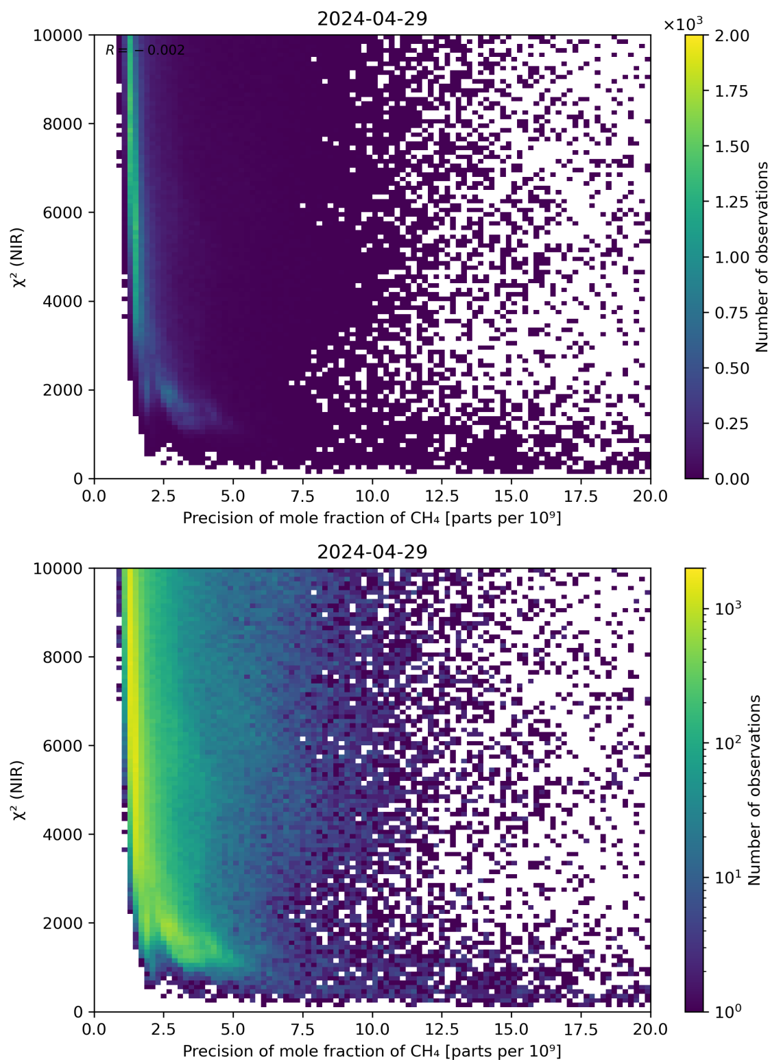
Figure 78: Scatter density plot of “Precision of mole fraction of CH 4 ” against “ \chi^2 (NIR)” for 2024-04-28 to 2024-04-30.
