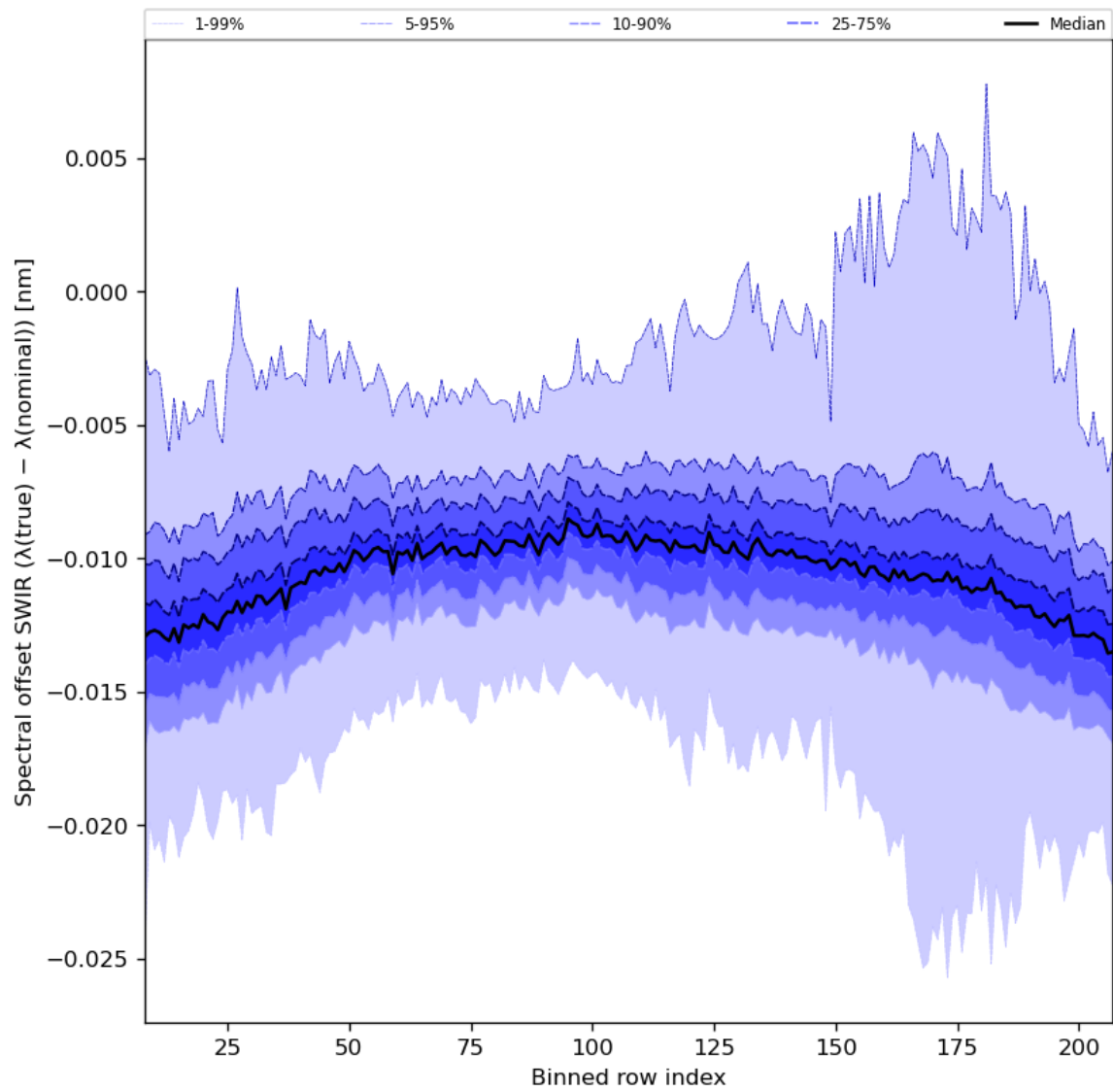
Figure 38: Along track statistics of “Spectral offset SWIR ( \lambda(\text{true}) - \lambda(\text{nominal}) )” for 2024-04-28 to 2024-04-30
