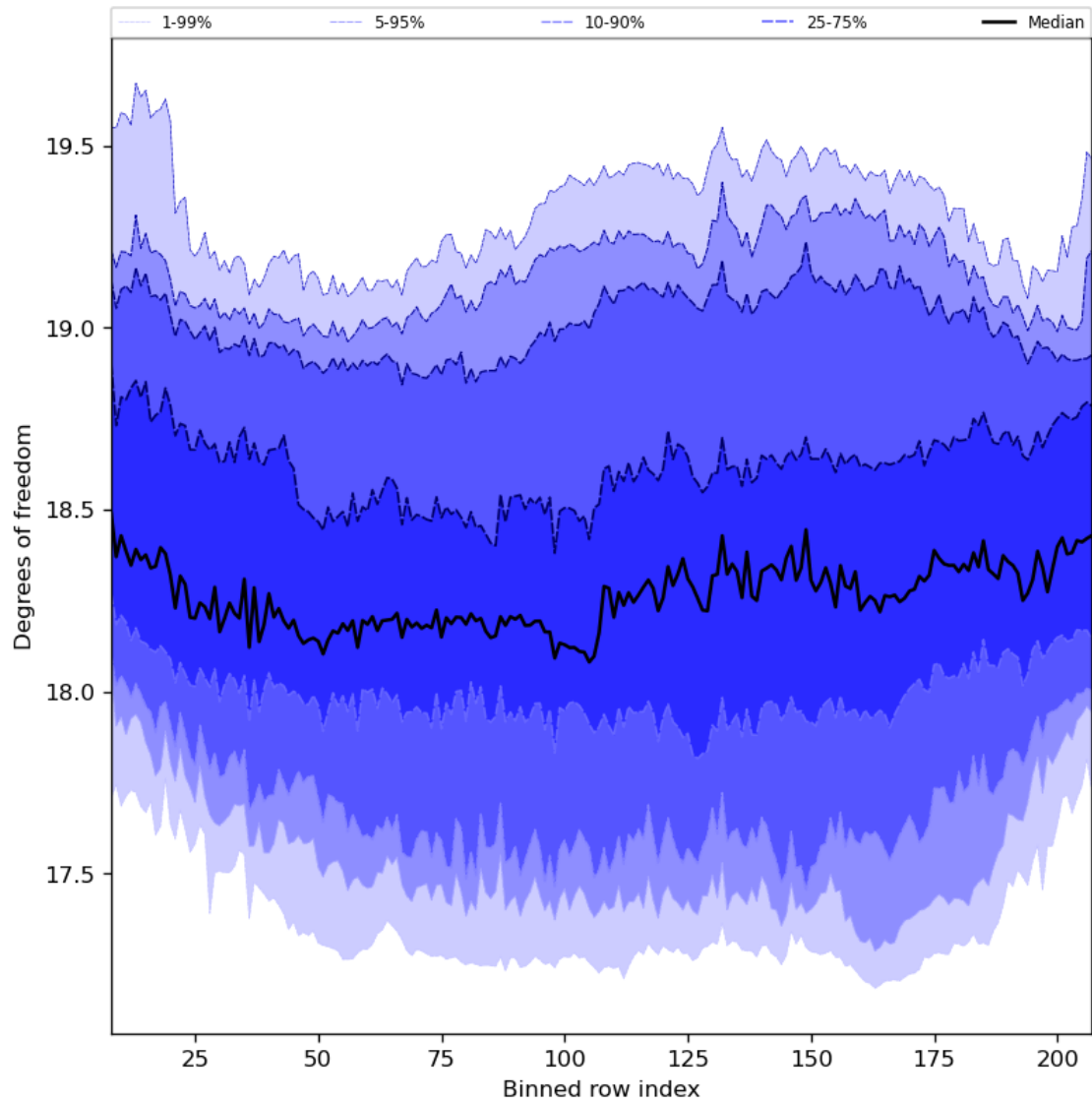
Figure 41: Along track statistics of “Degrees of freedom” for 2024-04-28 to 2024-04-30
