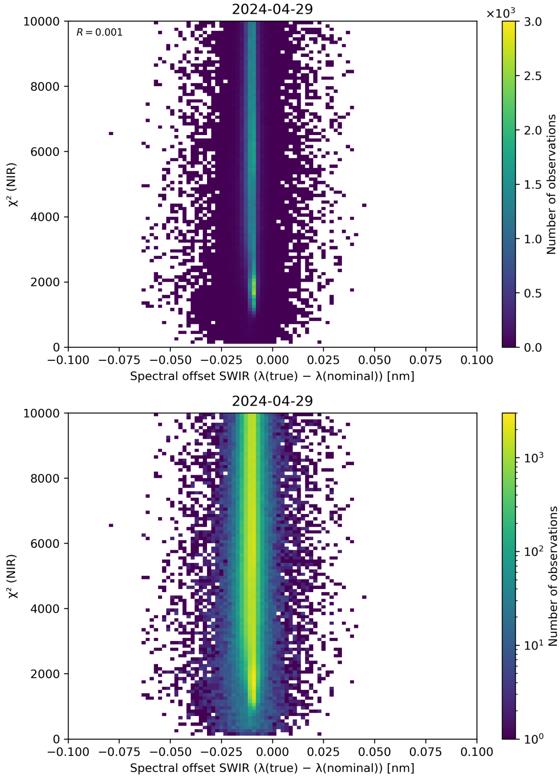
Figure 117: Scatter density plot of “Spectral offset SWIR ( \lambda(\text{true}) - \lambda(\text{nominal}) )” against “ \chi^2 (NIR)” for 2024-04-28 to 2024-04-30.
