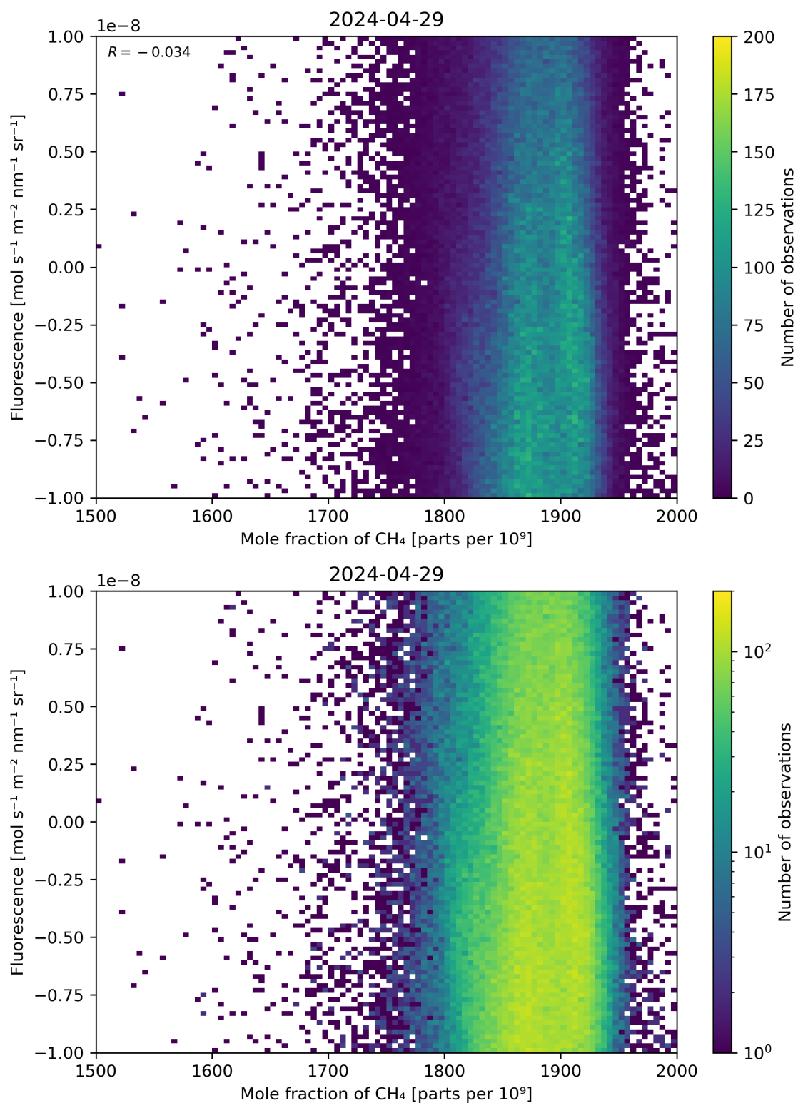
Figure 73: Scatter density plot of “Mole fraction of \text{CH}_4 ” against “Fluorescence” for 2024-04-28 to 2024-04-30.
