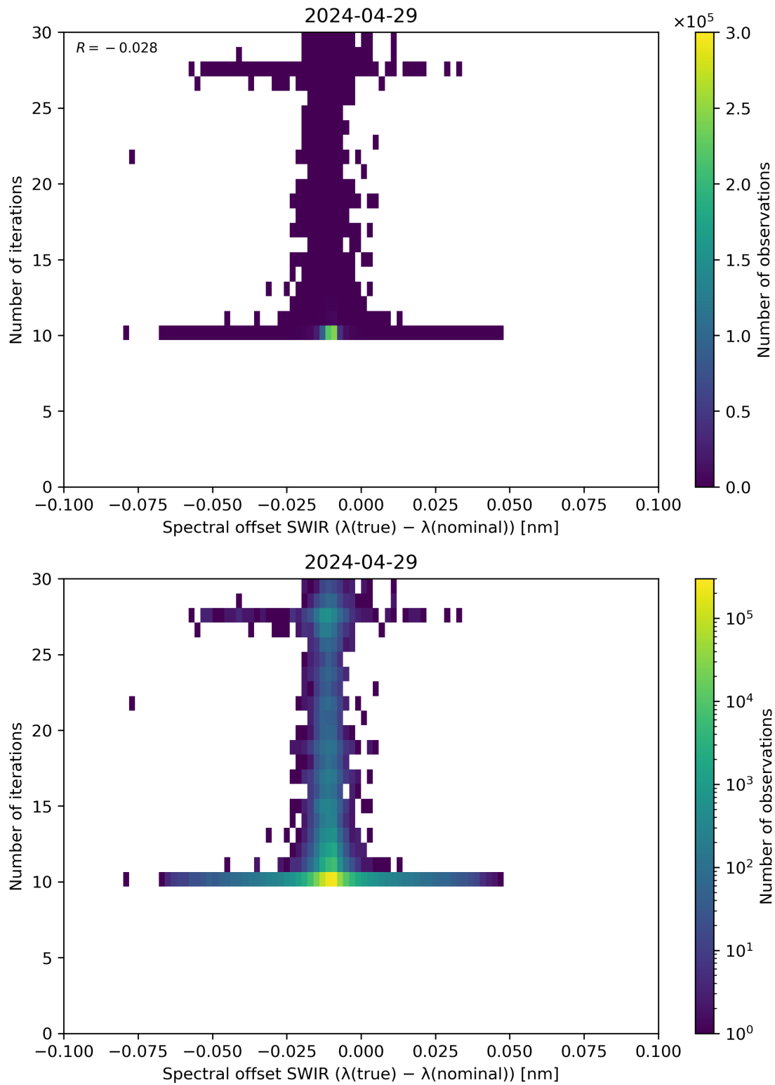
Figure 121: Scatter density plot of “Spectral offset SWIR ( \lambda(\text{true}) - \lambda(\text{nominal}) )” against “Number of iterations” for 2024-04-28 to 2024-04-30.
