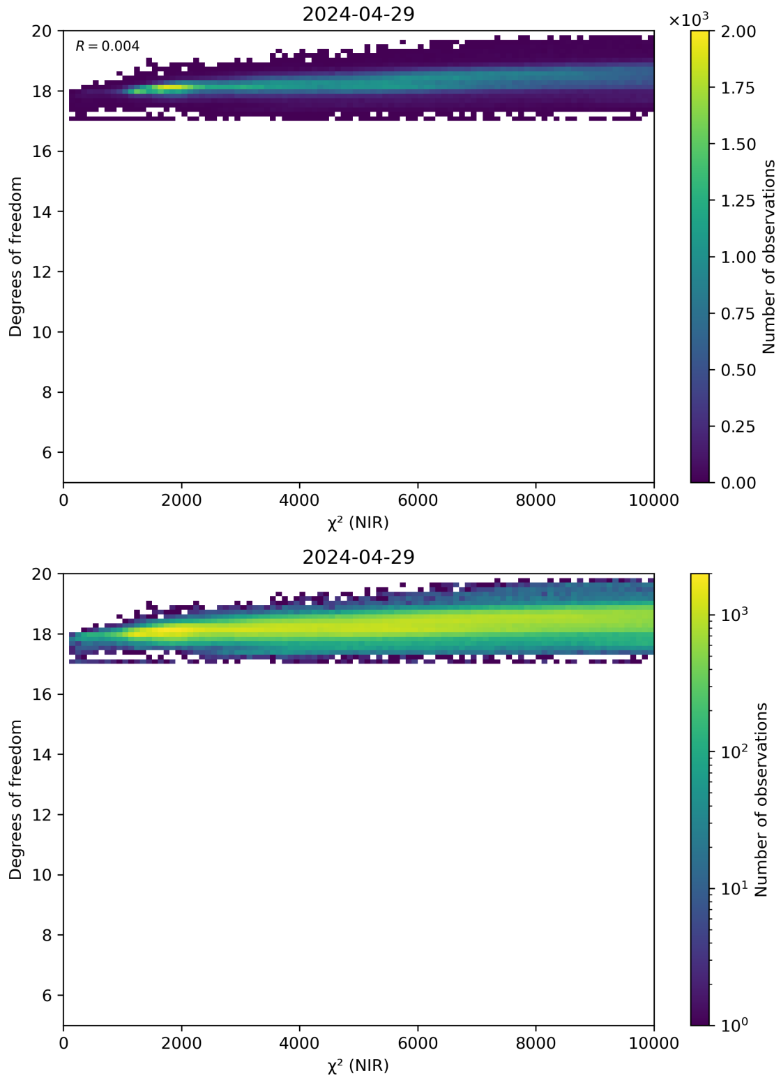
Figure 44: Scatter density plot of “ \chi^2 (NIR)” against “Degrees of freedom” for 2024-04-28 to 2024-04-30.
