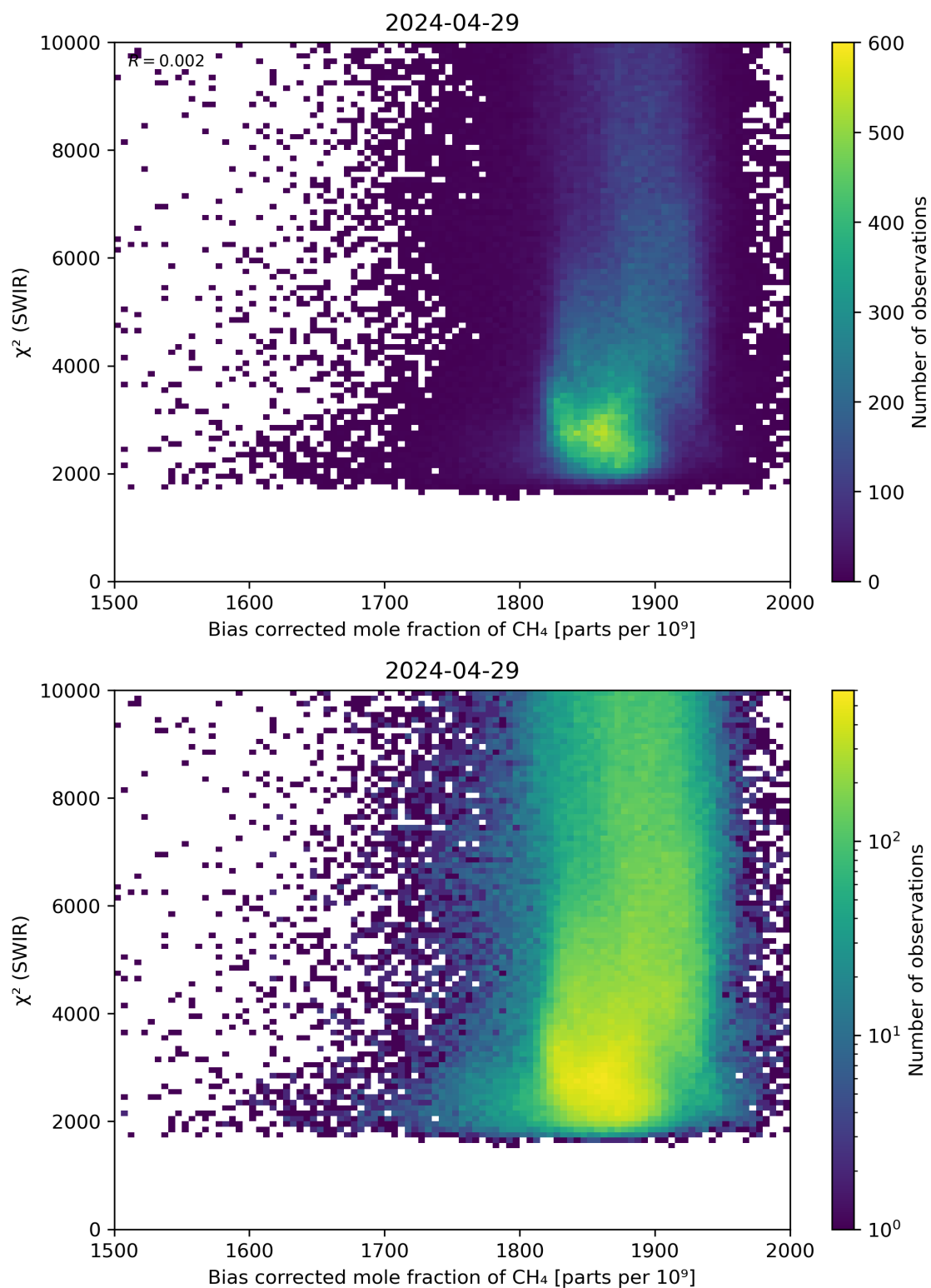
Figure 64: Scatter density plot of “Bias corrected mole fraction of \text{CH}_4 ” against “ \chi^2 (SWIR)” for 2024-04-28 to 2024-04-30.
