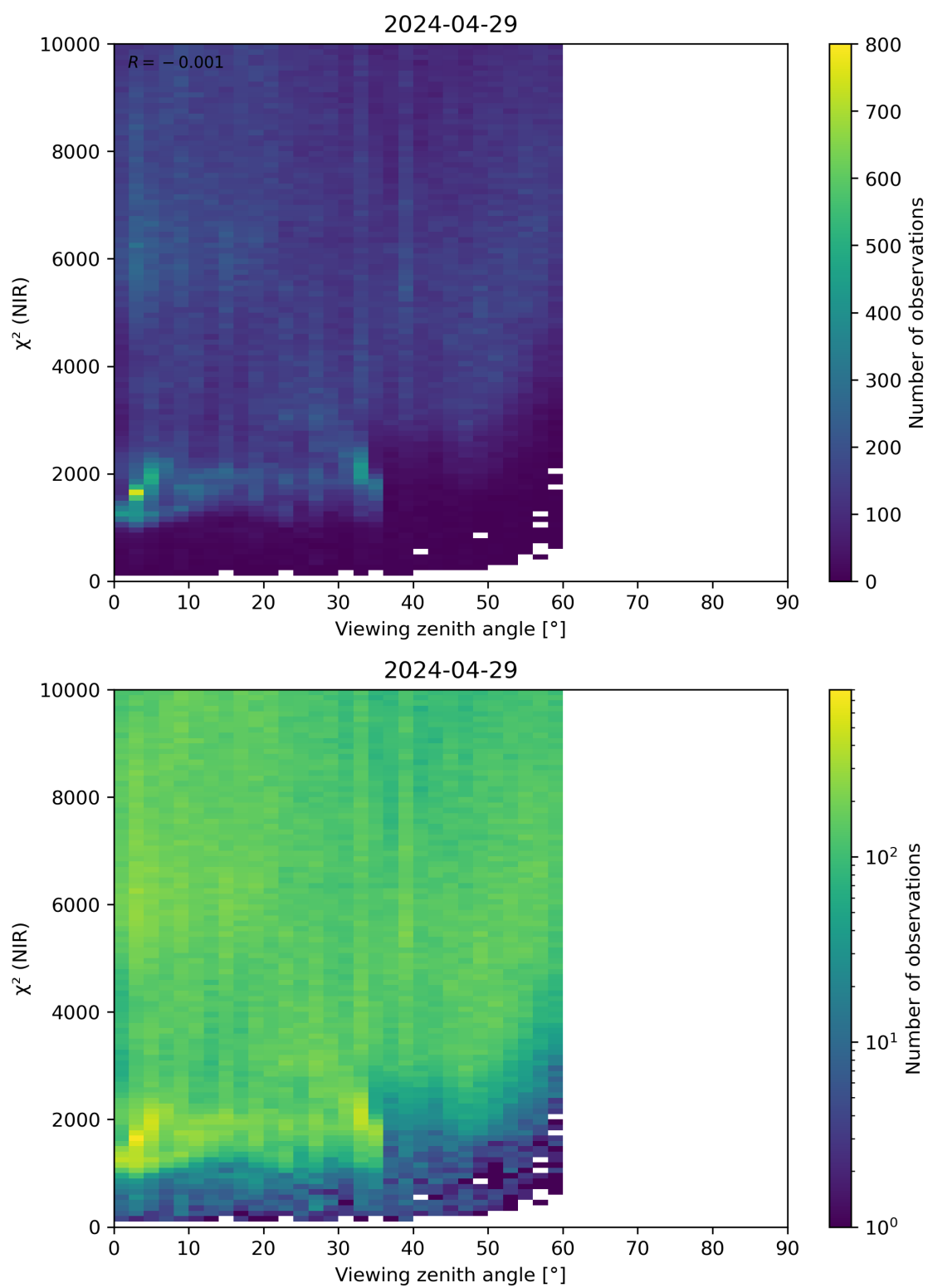
Figure 105: Scatter density plot of “Viewing zenith angle” against “ \chi^2 (NIR)” for 2024-04-28 to 2024-04-30.
