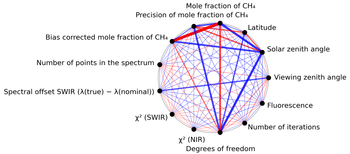
Figure 1: Map of correlation graph for 2024-04-28 to 2024-04-30.
