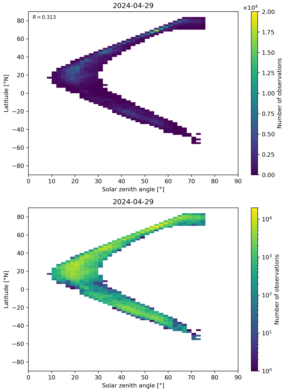
Figure 98: Scatter density plot of “Solar zenith angle” against “Latitude” for 2024-04-28 to 2024-04-30.
