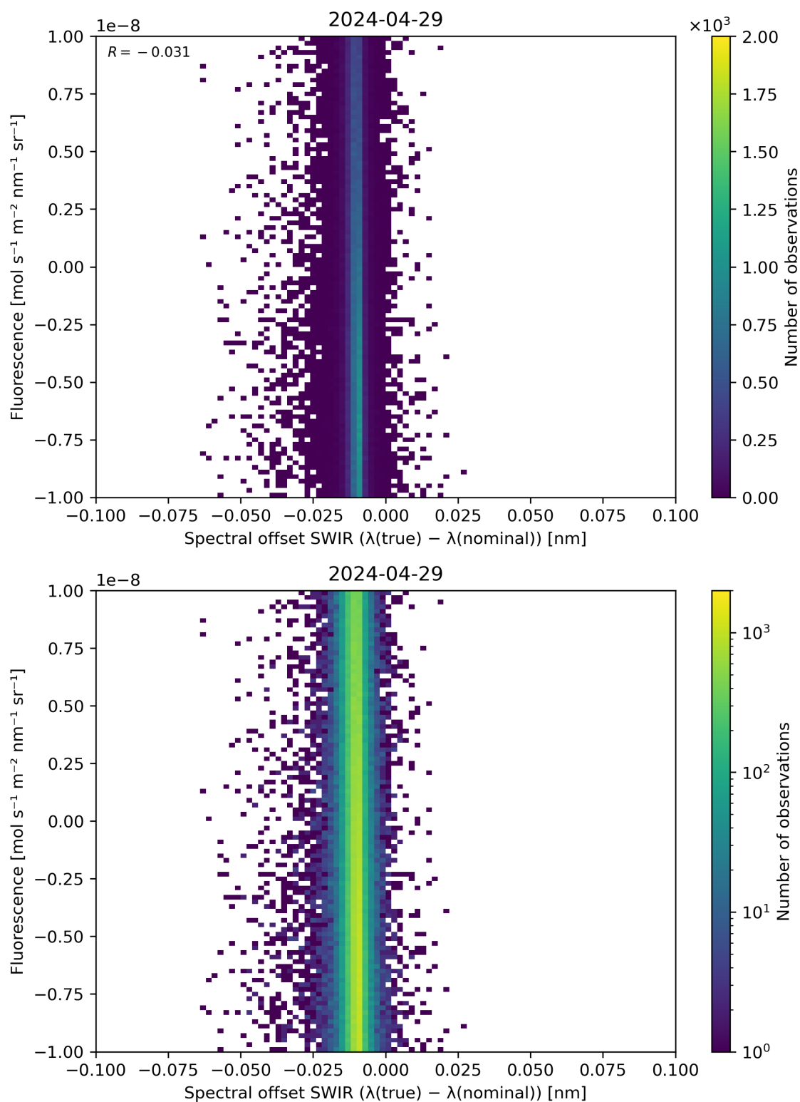
Figure 120: Scatter density plot of “Spectral offset SWIR ( \lambda(\text{true}) - \lambda(\text{nominal}) )” against “Fluorescence” for 2024-04-28 to 2024-04-30.
