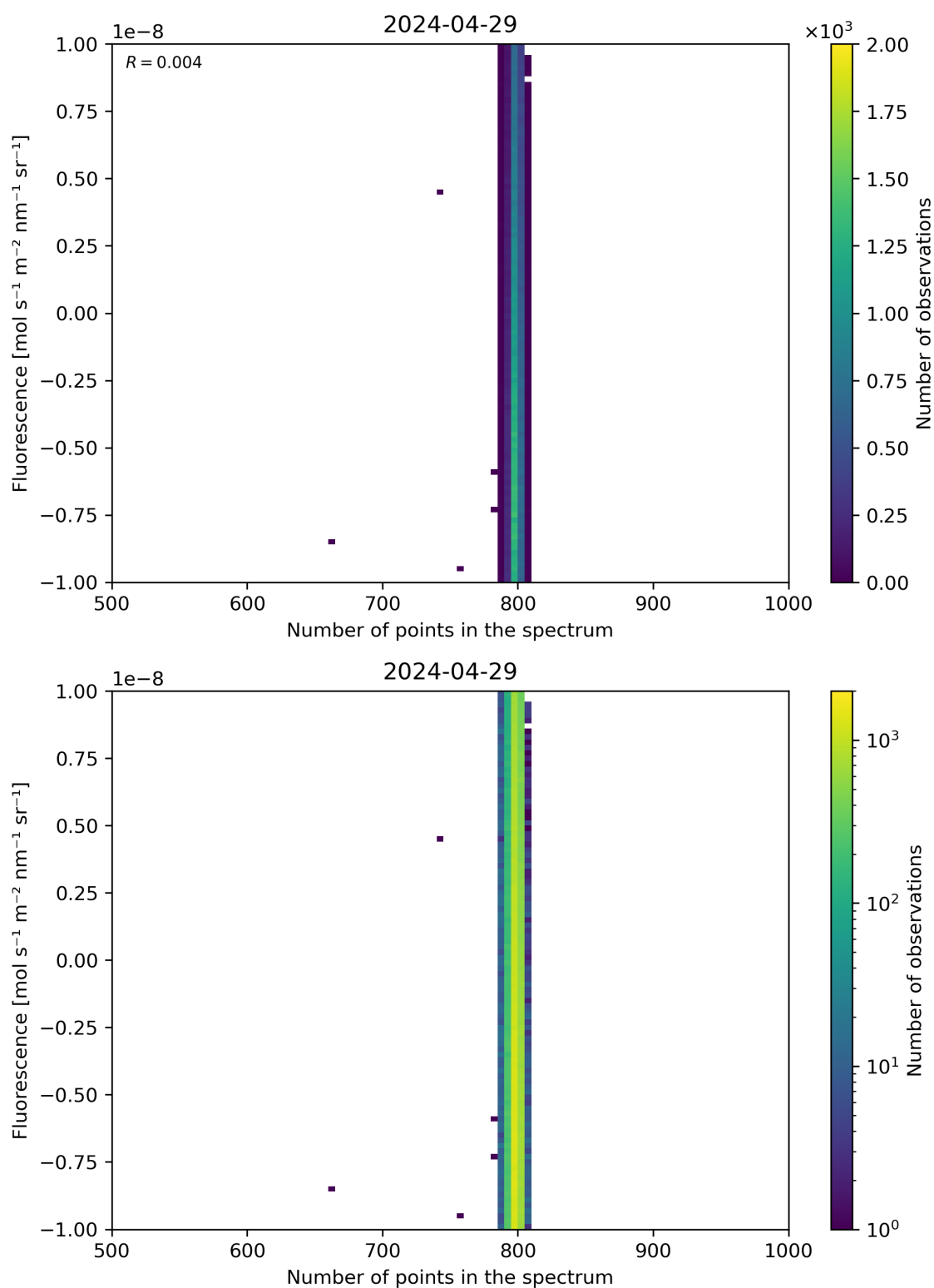
Figure 91: Scatter density plot of “Number of points in the spectrum” against “Fluorescence” for 2024-04-28 to 2024-04-30.
