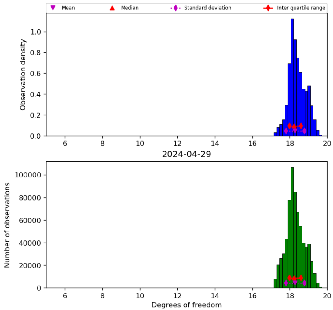
Figure 30: Histogram of “Degrees of freedom” for 2024-04-28 to 2024-04-30
