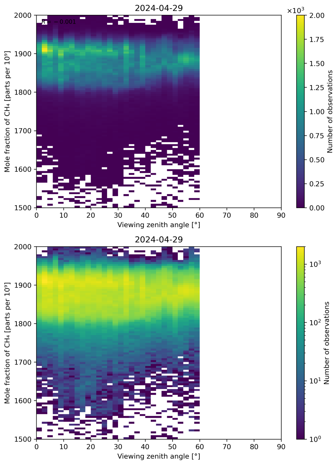
Figure 110: Scatter density plot of “Viewing zenith angle” against “Mole fraction of CH 4 ” for 2024-04-28 to 2024-04-30.
