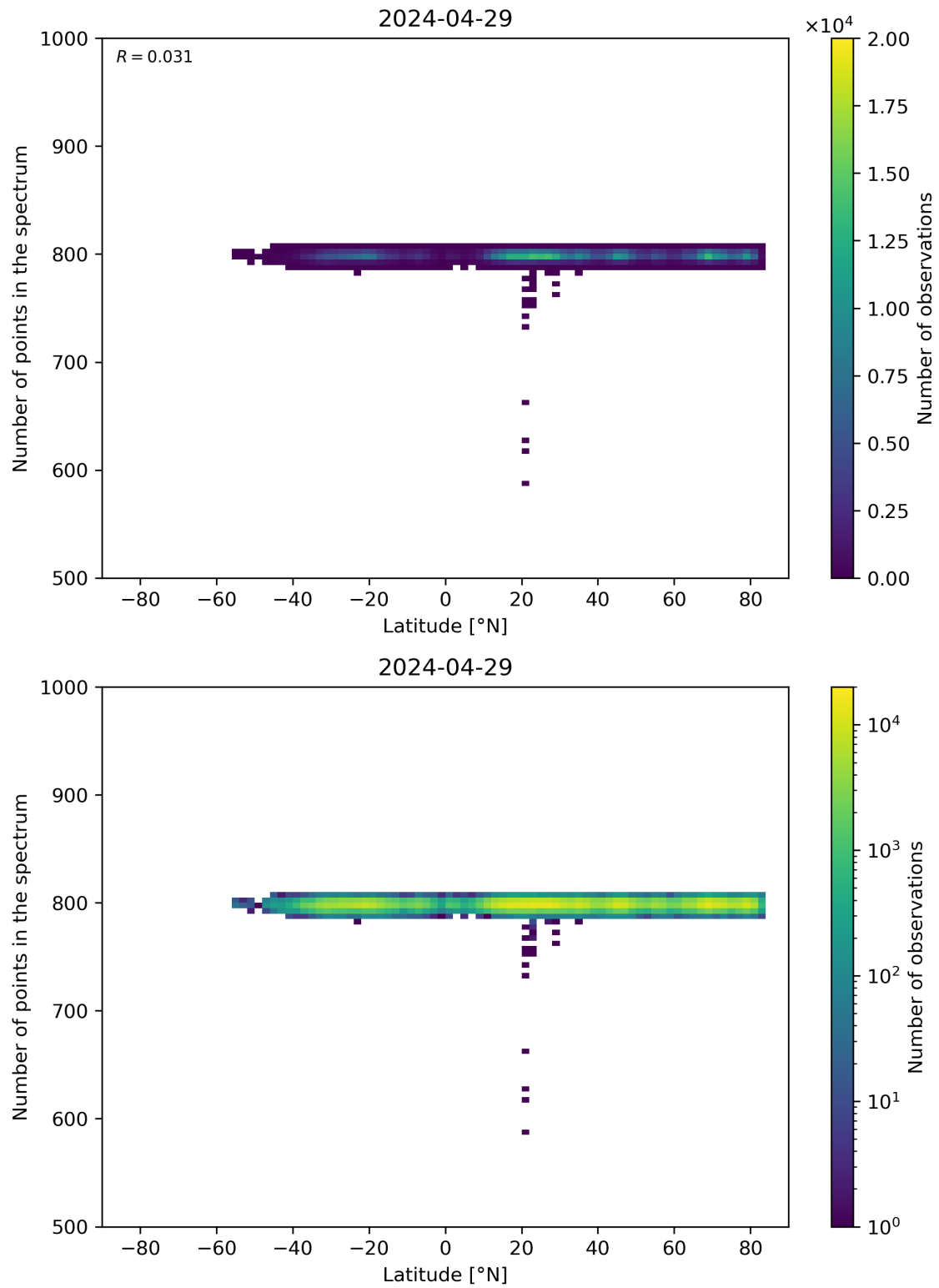
Figure 61: Scatter density plot of “Latitude” against “Number of points in the spectrum” for 2024-04-28 to 2024-04-30.
