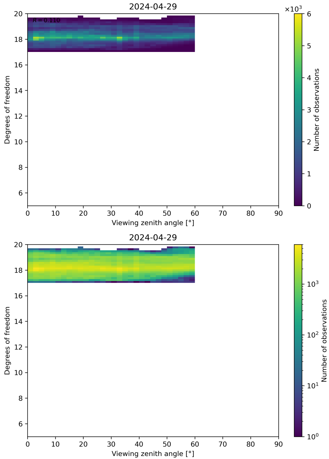
Figure 107: Scatter density plot of “Viewing zenith angle” against “Degrees of freedom” for 2024-04-28 to 2024-04-30.
