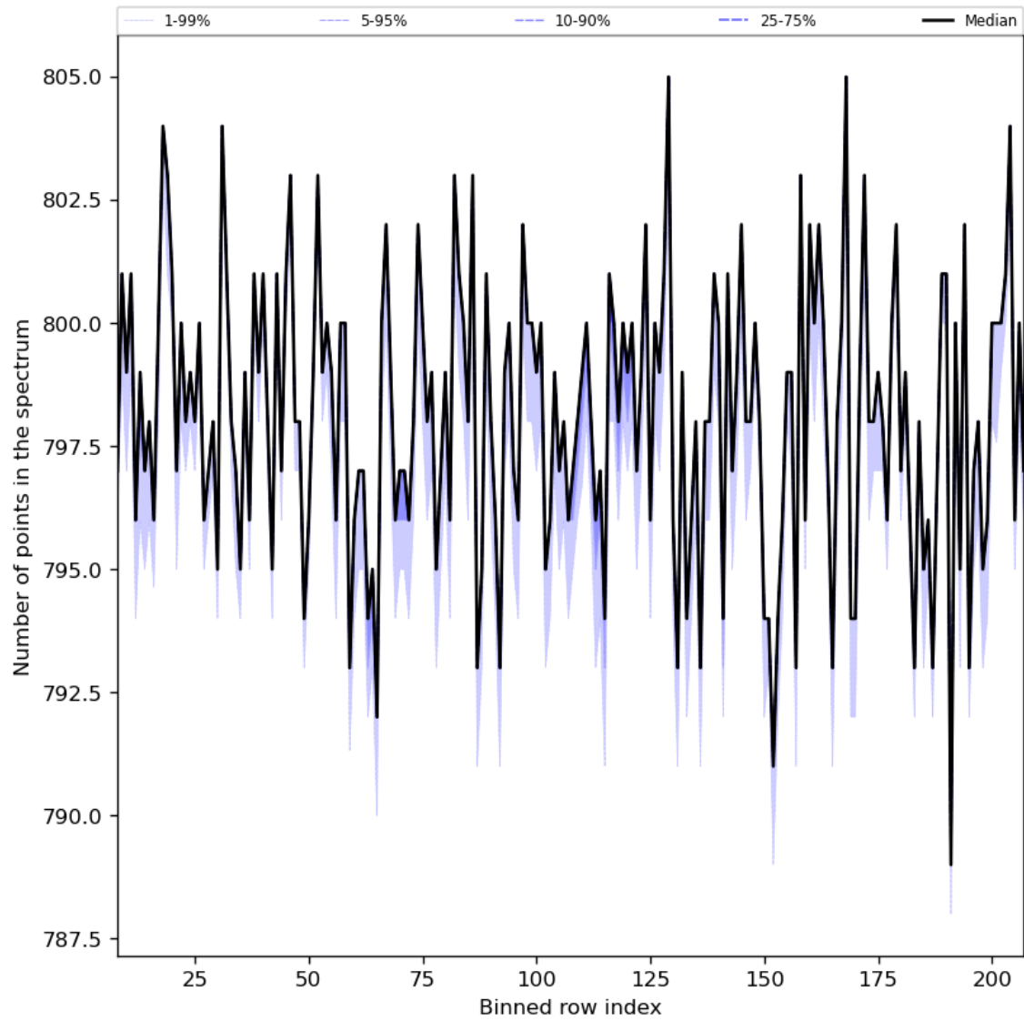
Figure 37: Along track statistics of “Number of points in the spectrum” for 2024-04-28 to 2024-04-30
