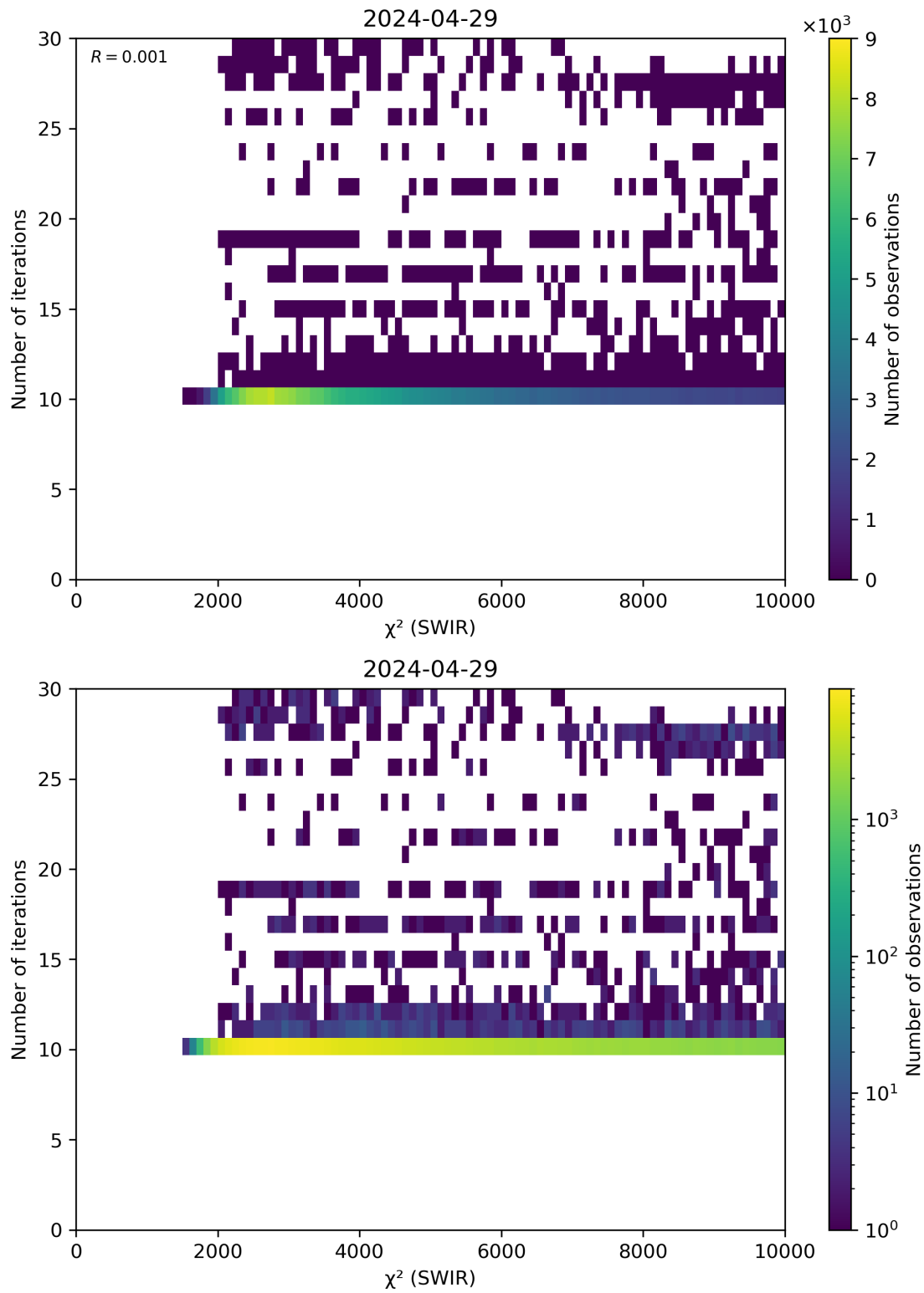
Figure 50: Scatter density plot of “ \chi^2 (SWIR)” against “Number of iterations” for 2024-04-28 to 2024-04-30.
