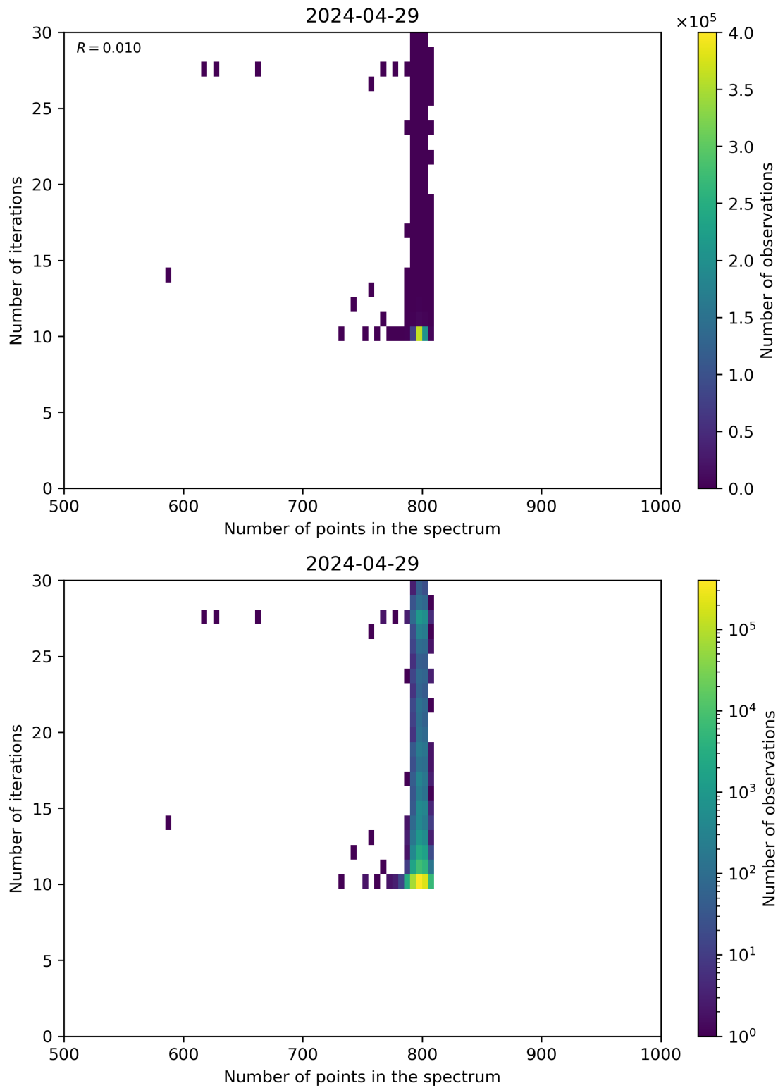
Figure 92: Scatter density plot of “Number of points in the spectrum” against “Number of iterations” for 2024-04-28 to 2024-04-30.
