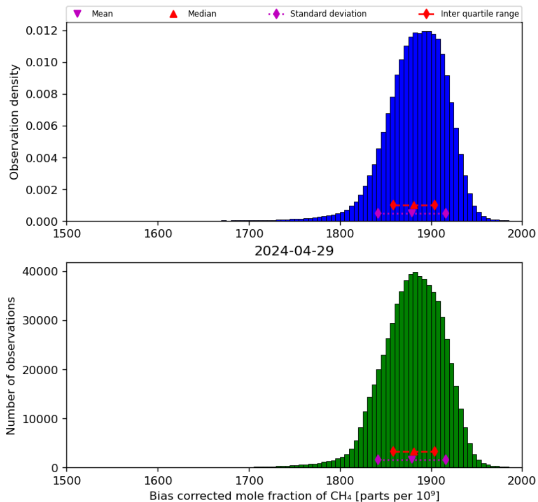
Figure 25: Histogram of “Bias corrected mole fraction of CH 4 ” for 2024-04-28 to 2024-04-30
