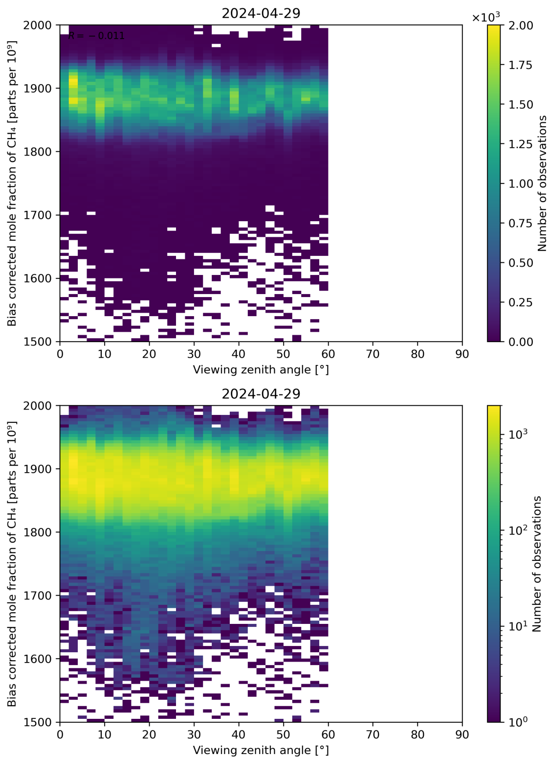
Figure 111: Scatter density plot of “Viewing zenith angle” against “Bias corrected mole fraction of CH 4 ” for 2024-04-28 to 2024-04-30.
