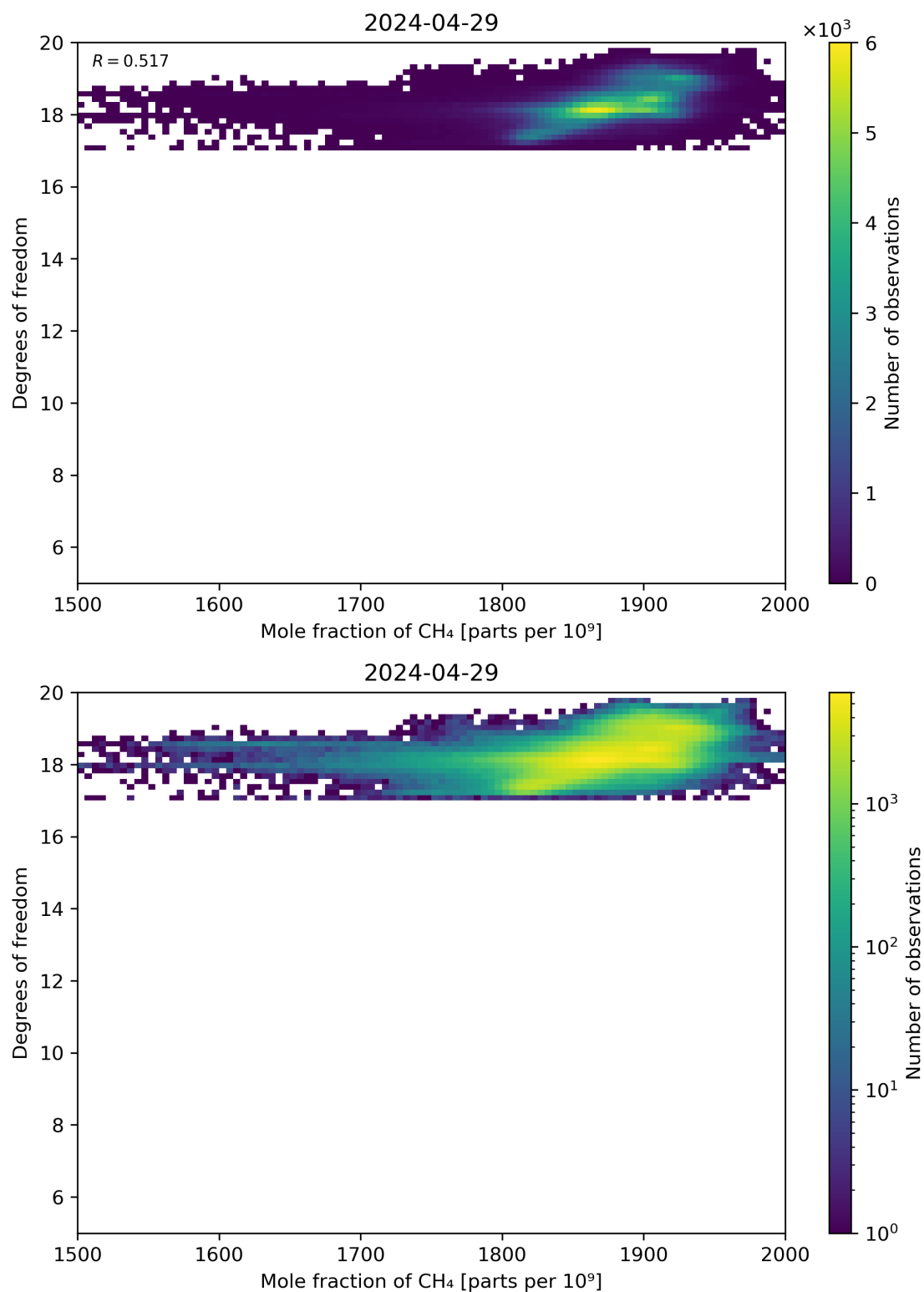
Figure 72: Scatter density plot of “Mole fraction of CH 4 ” against “Degrees of freedom” for 2024-04-28 to 2024-04-30.
