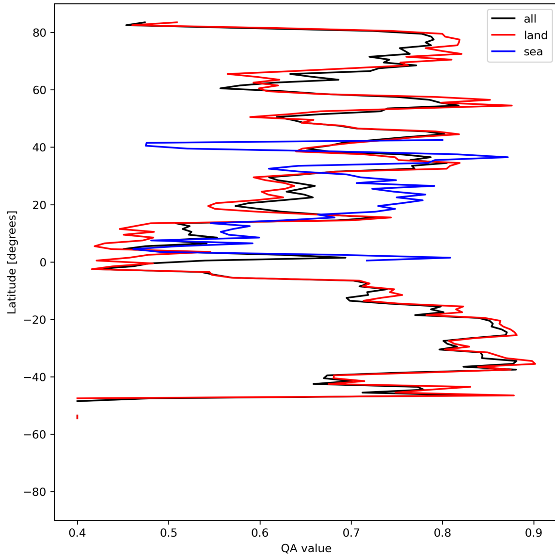
Figure 11: Zonal average of “QA value” for 2024-04-28 to 2024-04-30.
