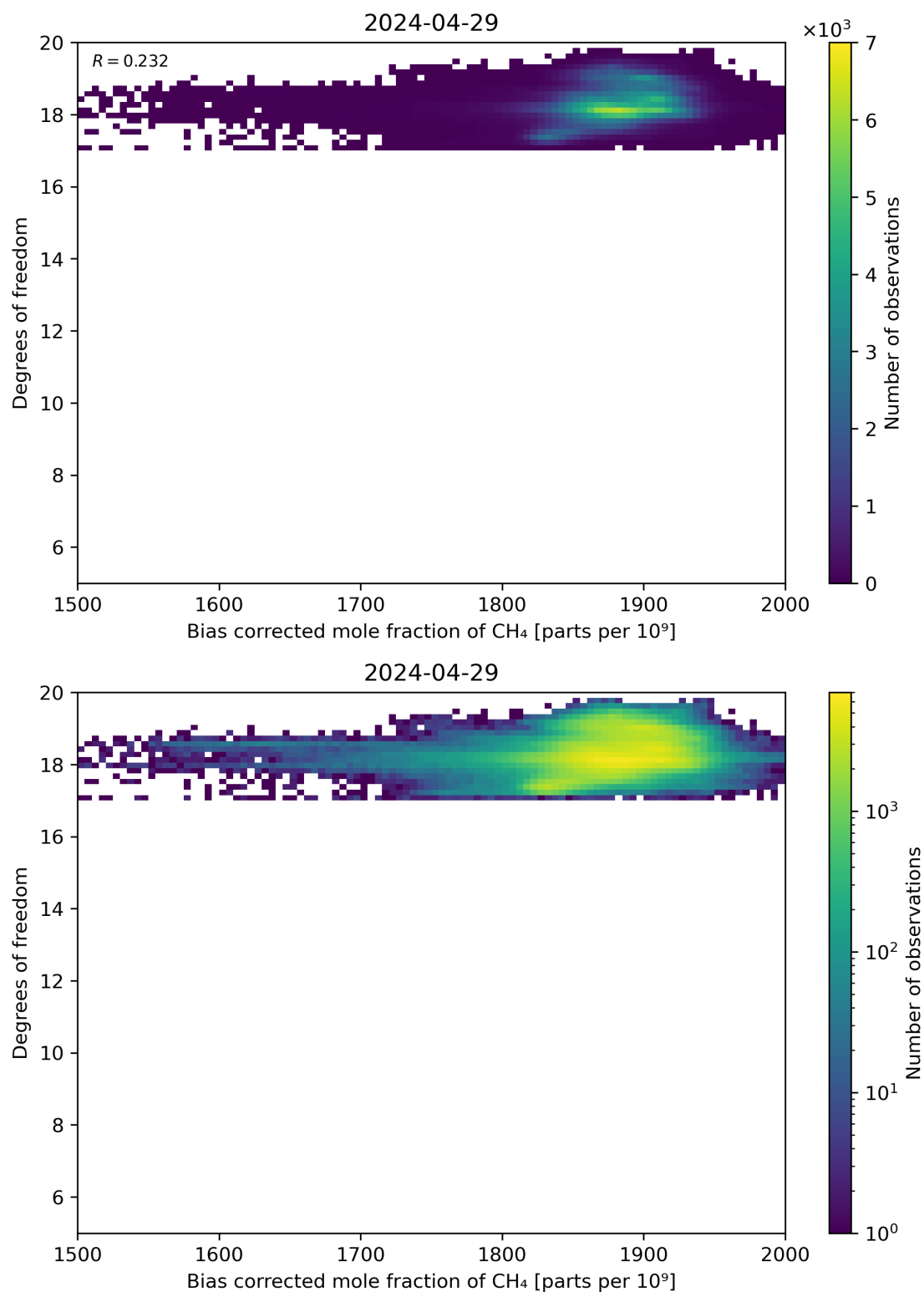
Figure 65: Scatter density plot of “Bias corrected mole fraction of CH 4 ” against “Degrees of freedom” for 2024-04-28 to 2024-04-30.
