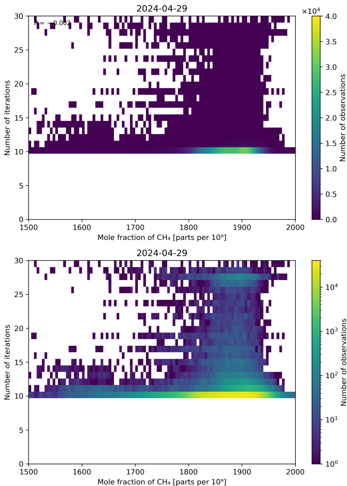
Figure 76: Scatter density plot of “Mole fraction of CH 4 ” against “Number of iterations” for 2024-04-28 to 2024-04-30.
