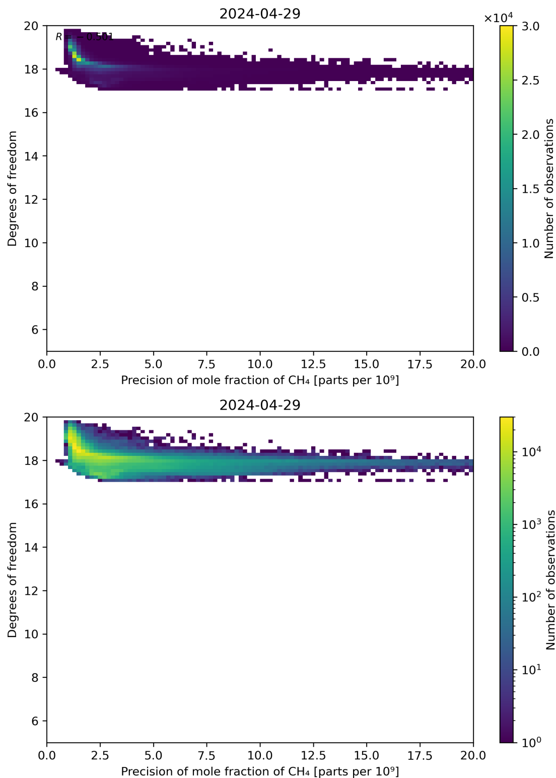
Figure 80: Scatter density plot of “Precision of mole fraction of CH 4 ” against “Degrees of freedom” for 2024-04-28 to 2024-04-30.
