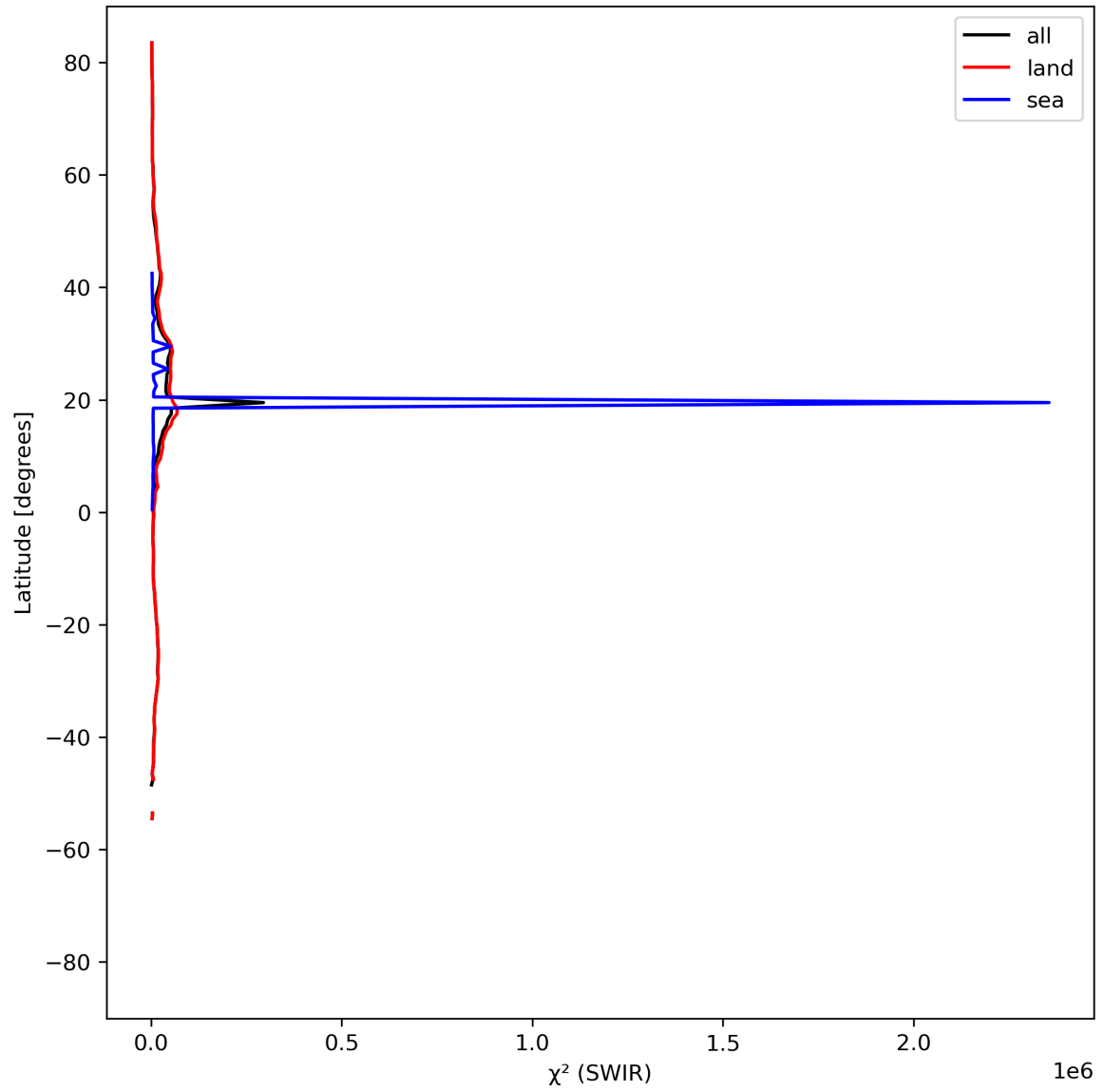
Figure 17: Zonal average of “ \chi^2 (SWIR)” for 2024-04-28 to 2024-04-30.
