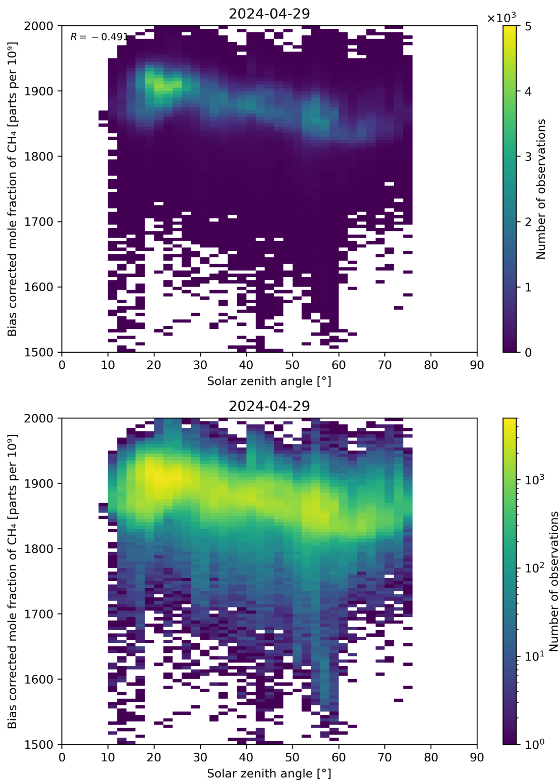
Figure 100: Scatter density plot of “Solar zenith angle” against “Bias corrected mole fraction of \text{CH}_4 ” for 2024-04-28 to 2024-04-30.
