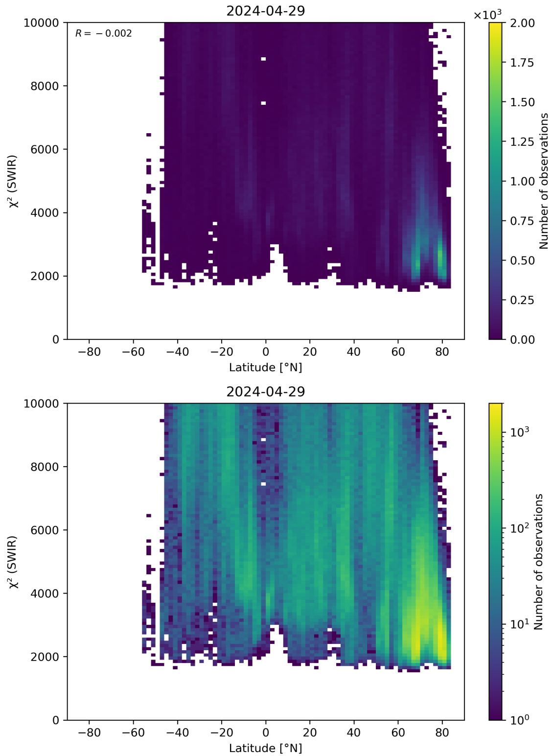
Figure 54: Scatter density plot of “Latitude” against “ \chi^2 (SWIR)” for 2024-04-28 to 2024-04-30.
