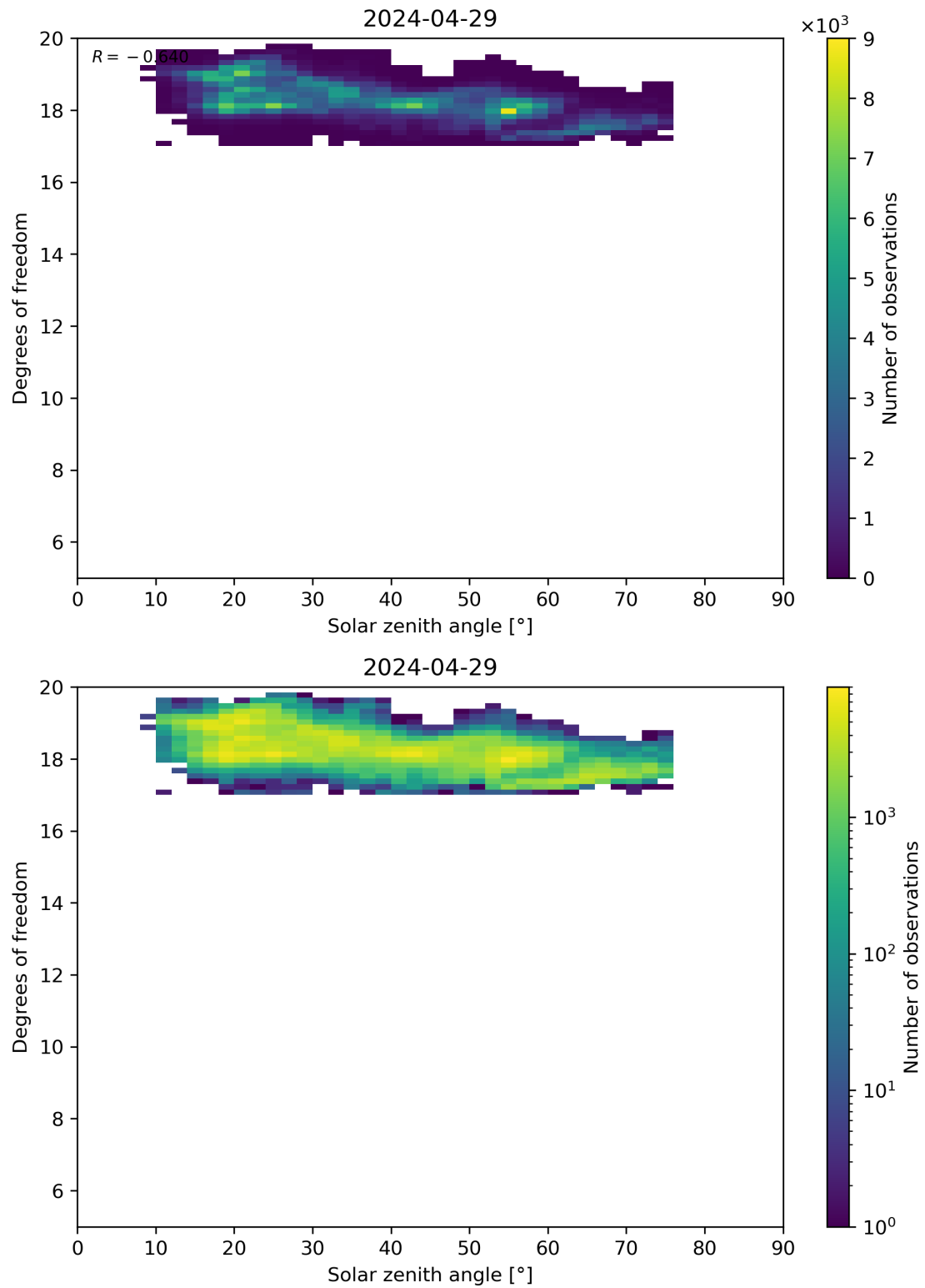
Figure 96: Scatter density plot of “Solar zenith angle” against “Degrees of freedom” for 2024-04-28 to 2024-04-30.
