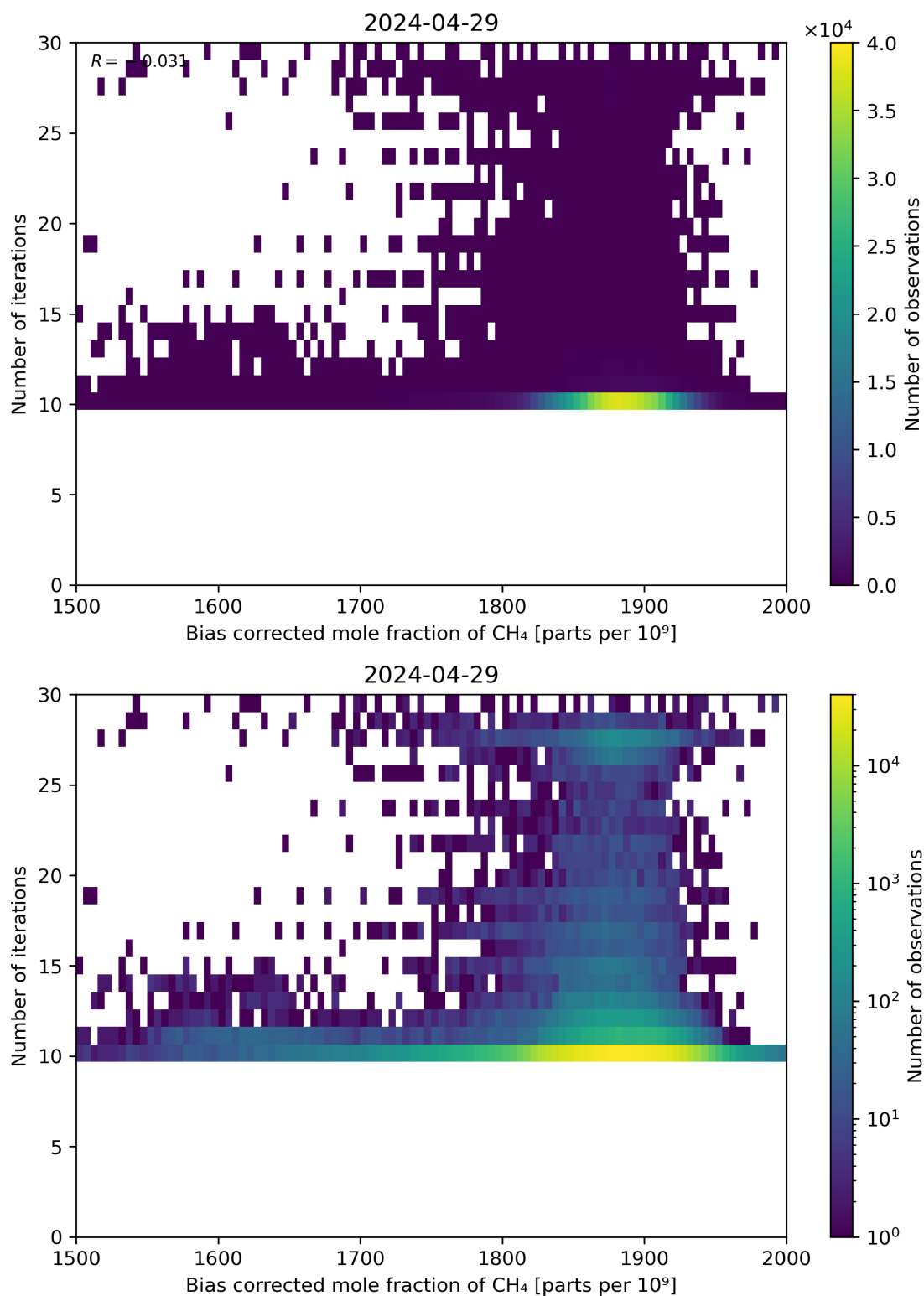
Figure 67: Scatter density plot of “Bias corrected mole fraction of CH 4 ” against “Number of iterations” for 2024-04-28 to 2024-04-30.
