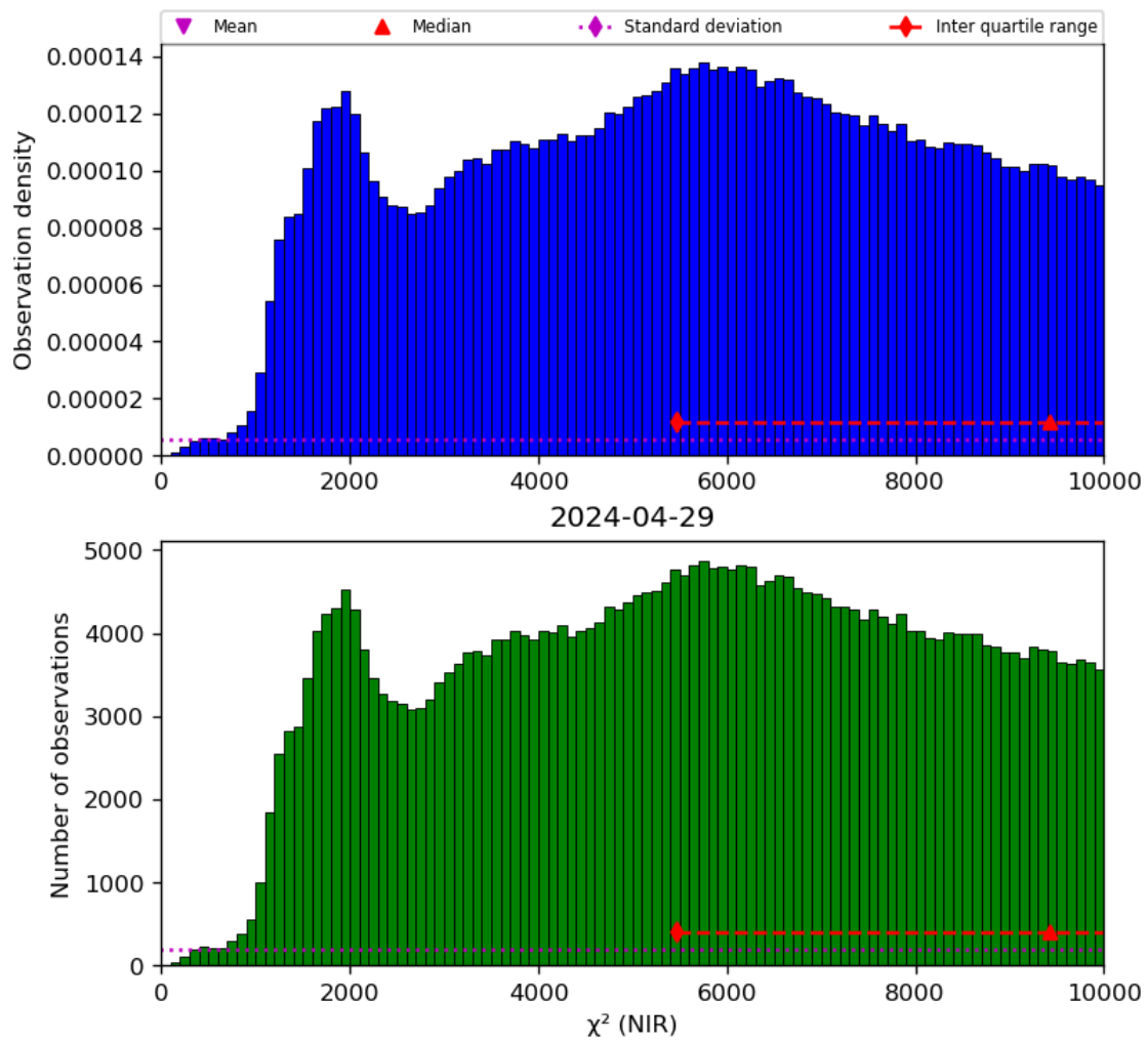
Figure 29: Histogram of “ \chi^2 (NIR)” for 2024-04-28 to 2024-04-30
