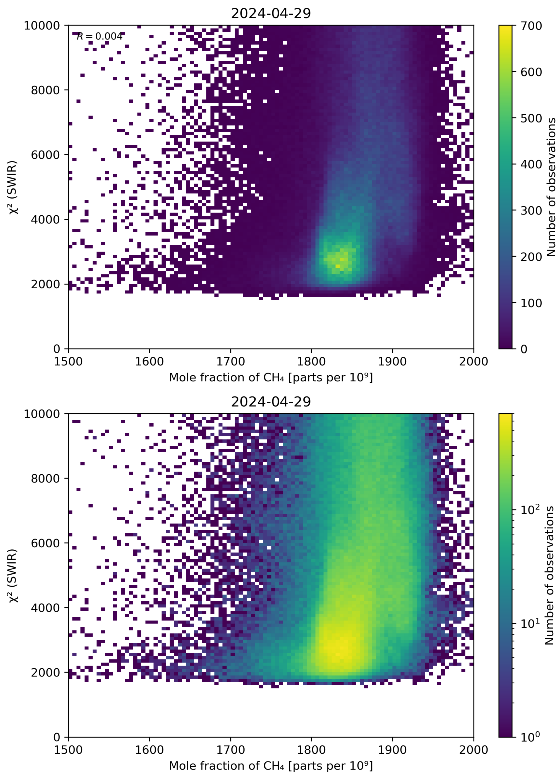
Figure 71: Scatter density plot of “Mole fraction of \text{CH}_4 ” against “ \chi^2 (SWIR)” for 2024-04-28 to 2024-04-30.
