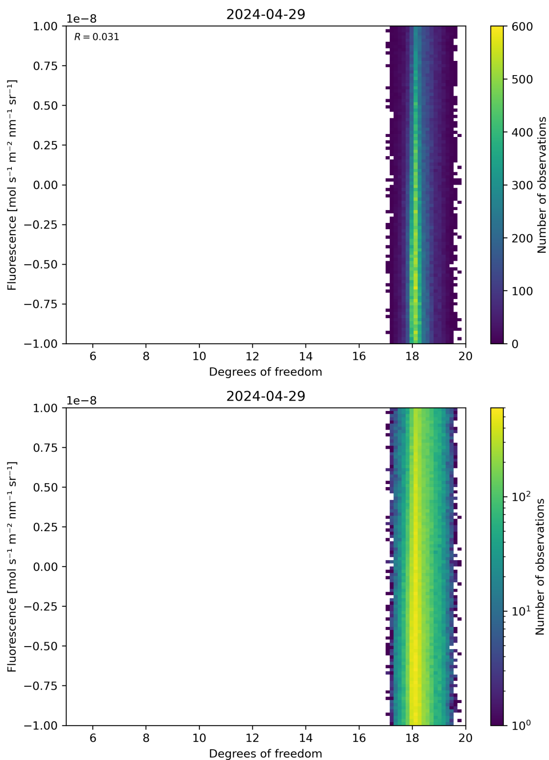
Figure 51: Scatter density plot of “Degrees of freedom” against “Fluorescence” for 2024-04-28 to 2024-04-30.
