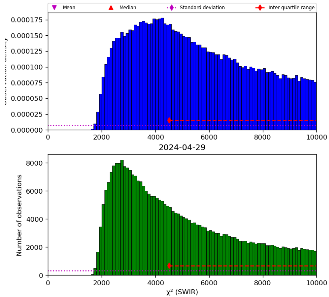
Figure 28: Histogram of “ \chi^2 (SWIR)” for 2024-04-28 to 2024-04-30
