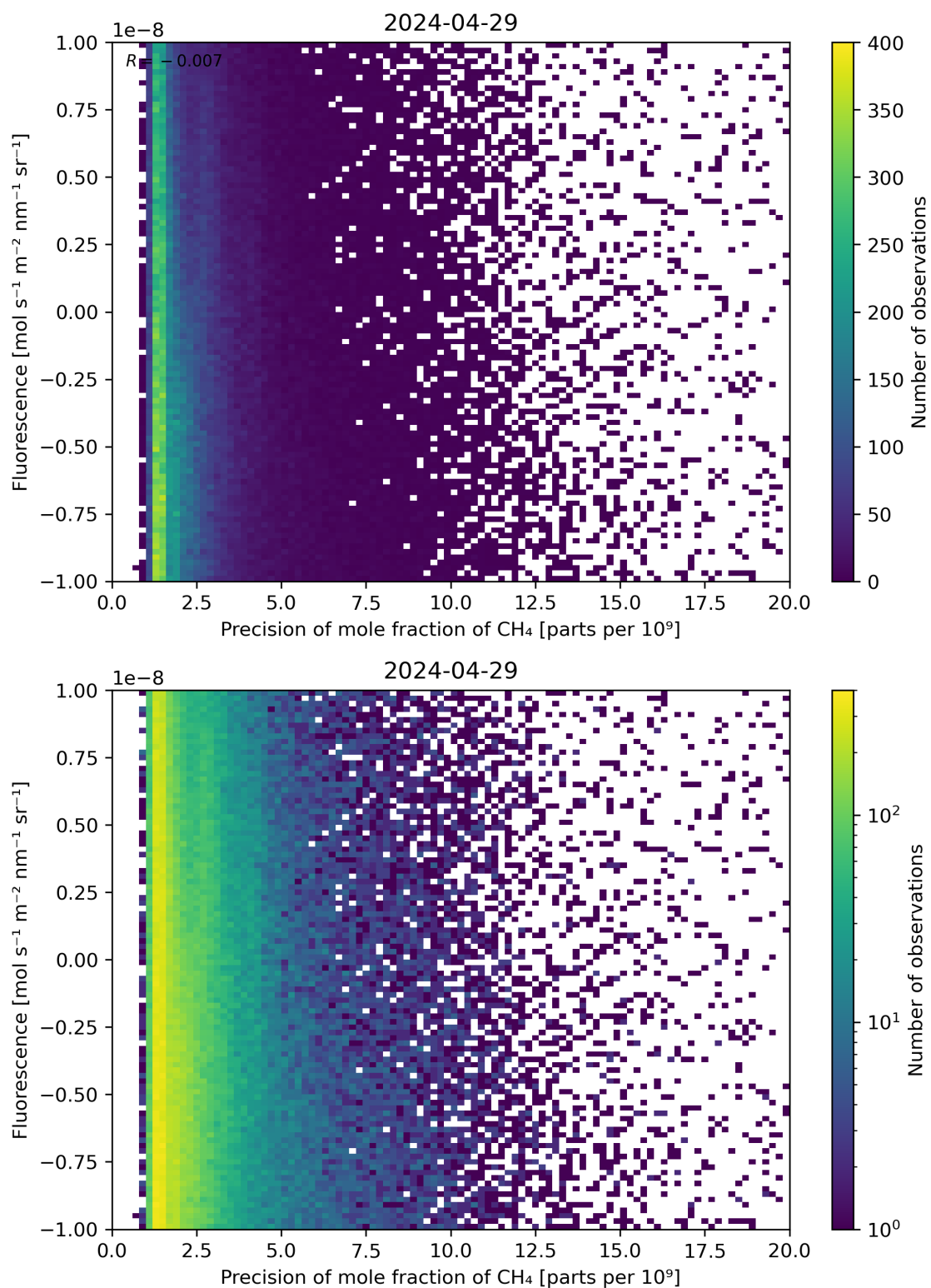
Figure 81: Scatter density plot of “Precision of mole fraction of \text{CH}_4 ” against “Fluorescence” for 2024-04-28 to 2024-04-30.
