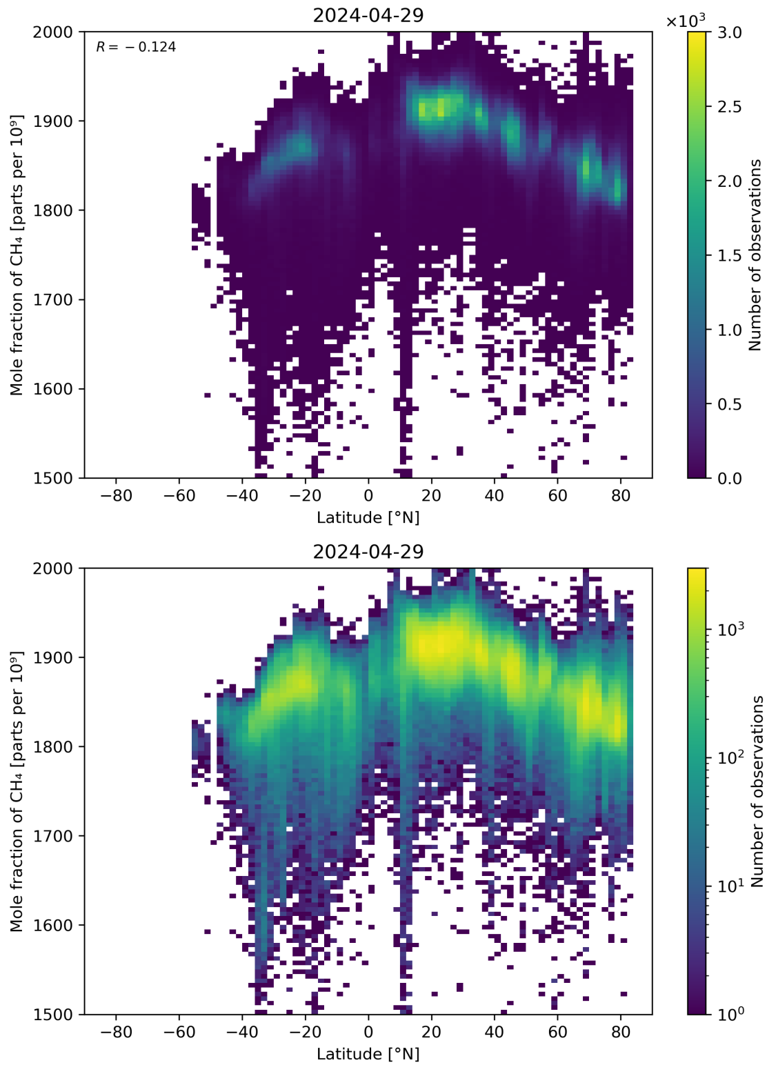
Figure 57: Scatter density plot of “Latitude” against “Mole fraction of \text{CH}_4 ” for 2024-04-28 to 2024-04-30.
