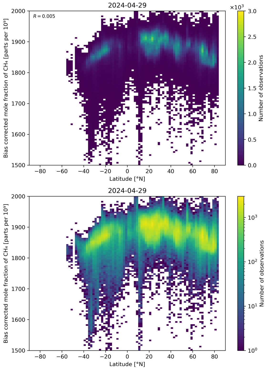
Figure 58: Scatter density plot of “Latitude” against “Bias corrected mole fraction of \text{CH}_4 ” for 2024-04-28 to 2024-04-30.
