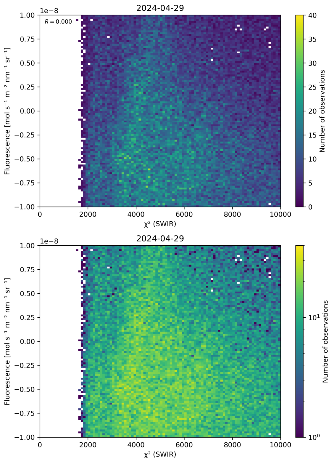
Figure 49: Scatter density plot of “ \chi^2 (SWIR)” against “Fluorescence” for 2024-04-28 to 2024-04-30.
