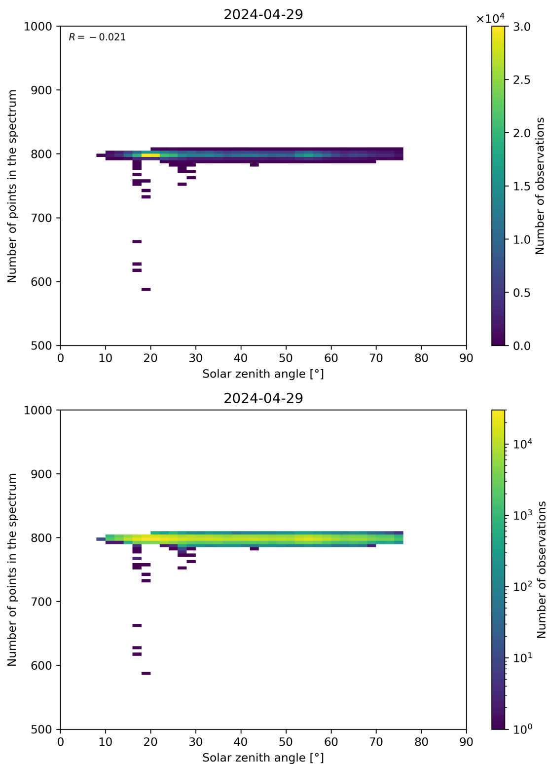
Figure 103: Scatter density plot of “Solar zenith angle” against “Number of points in the spectrum” for 2024-04-28 to 2024-04-30.
