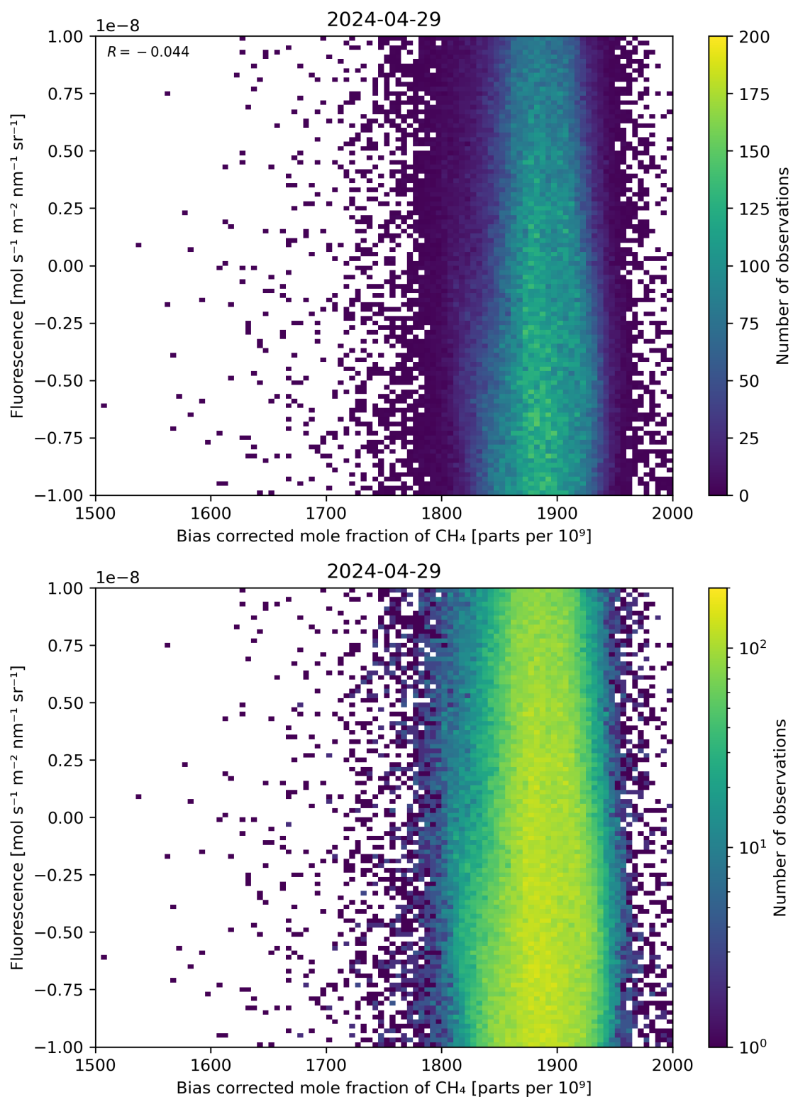
Figure 66: Scatter density plot of “Bias corrected mole fraction of \text{CH}_4 ” against “Fluorescence” for 2024-04-28 to 2024-04-30.
