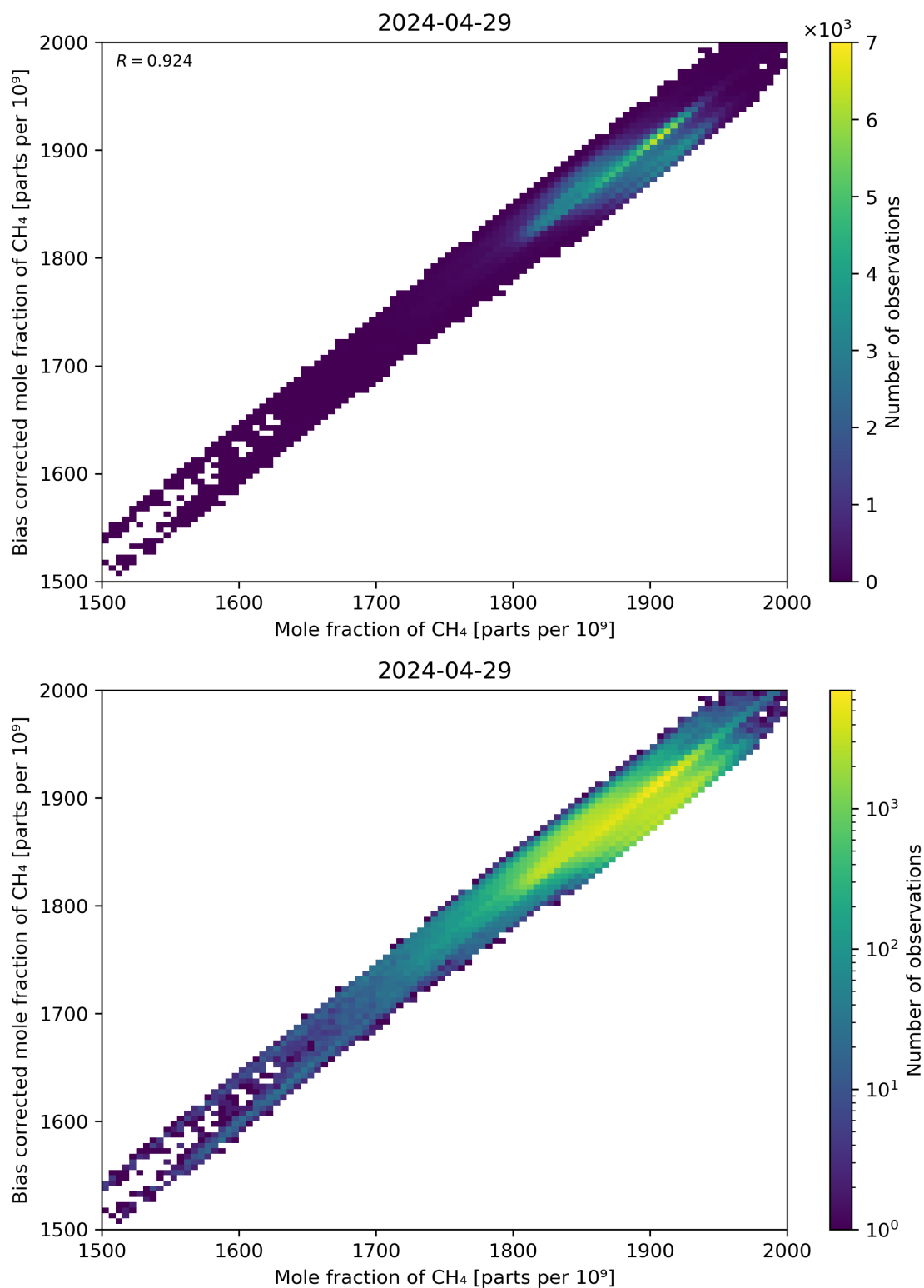
Figure 74: Scatter density plot of “Mole fraction of CH 4 ” against “Bias corrected mole fraction of CH 4 ” for 2024-04-28 to 2024-04-30.
