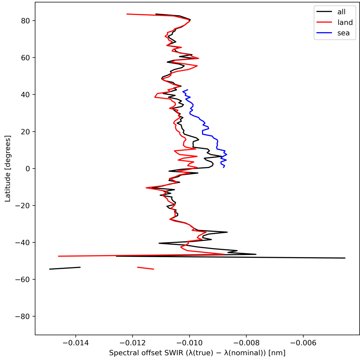
Figure 16: Zonal average of “Spectral offset SWIR ( \lambda(\text{true}) - \lambda(\text{nominal}) )” for 2024-04-28 to 2024-04-30.
