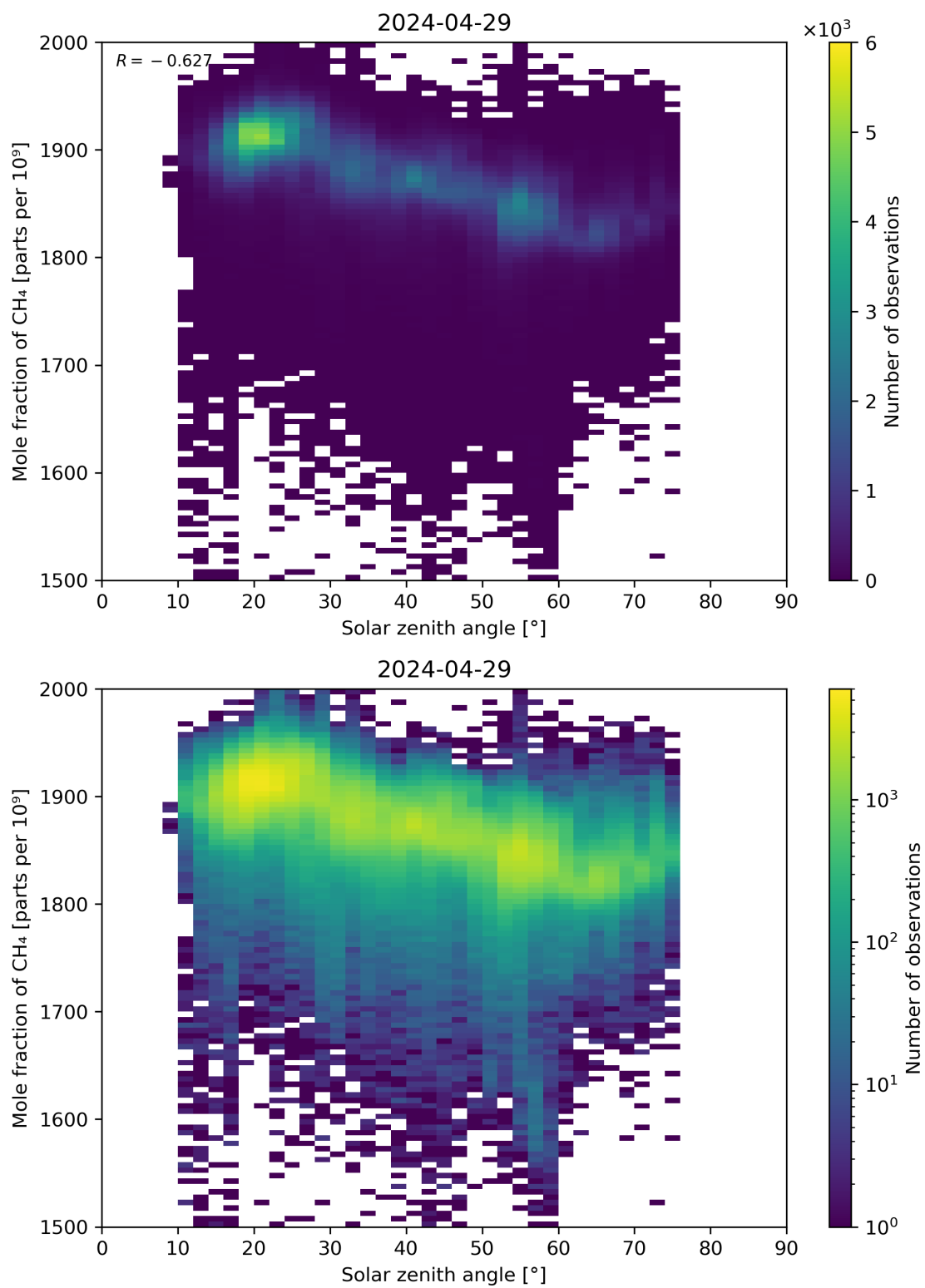
Figure 99: Scatter density plot of “Solar zenith angle” against “Mole fraction of CH 4 ” for 2024-04-28 to 2024-04-30.
