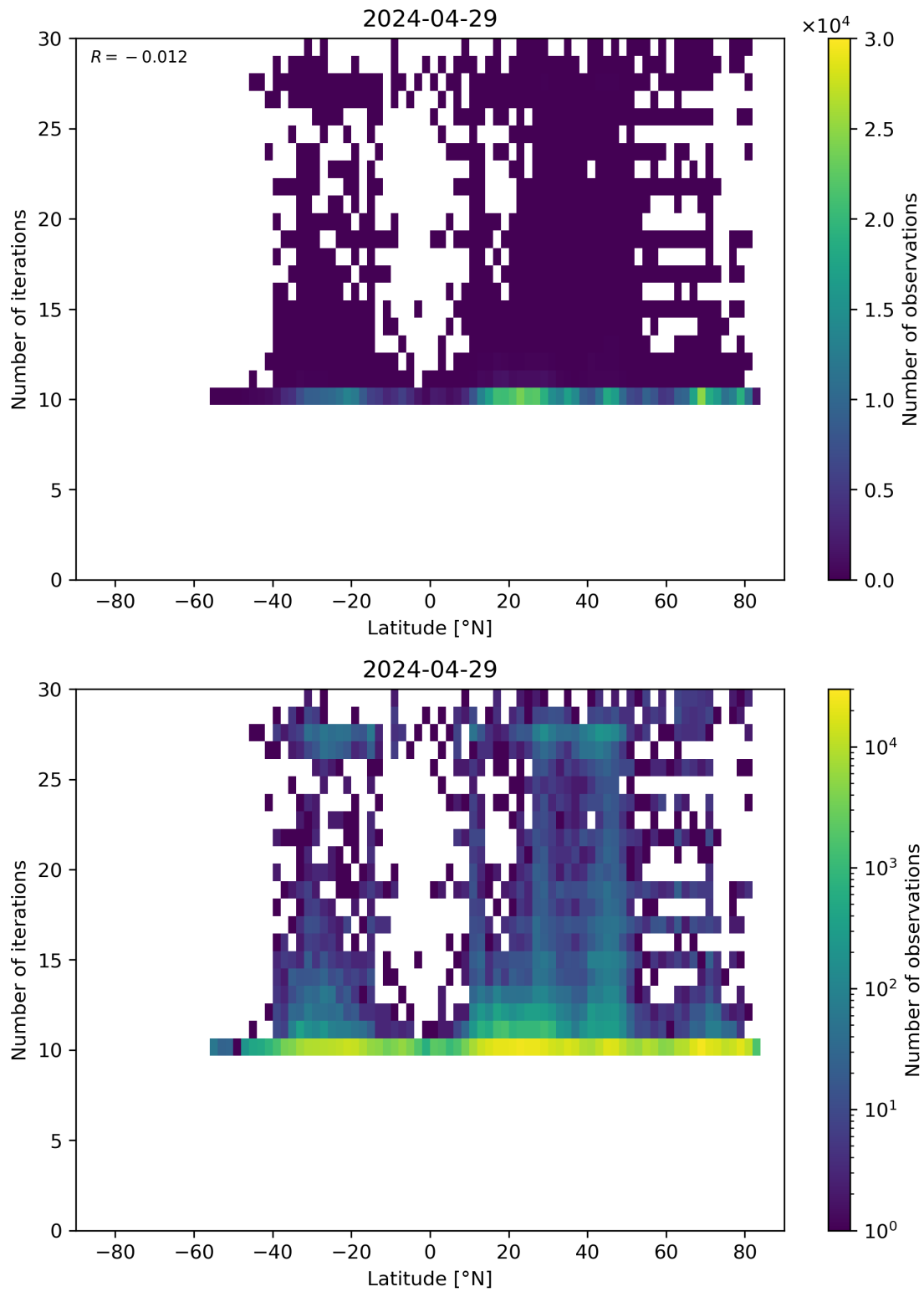
Figure 60: Scatter density plot of “Latitude” against “Number of iterations” for 2024-04-28 to 2024-04-30.
