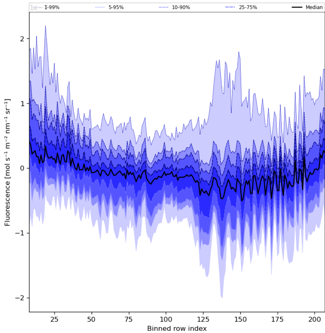
Figure 43: Along track statistics of “Fluorescence” for 2024-04-28 to 2024-04-30
