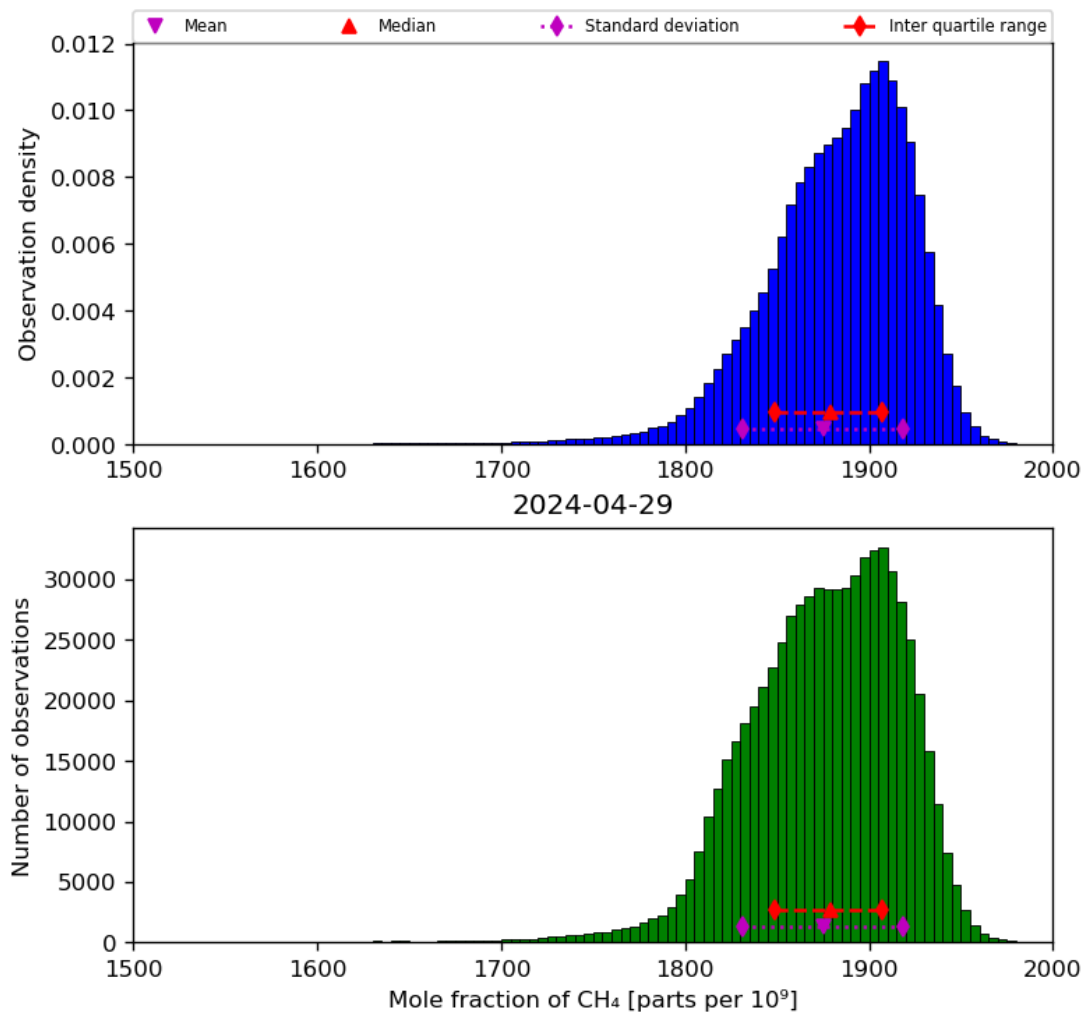
Figure 23: Histogram of “Mole fraction of CH 4 ” for 2024-04-28 to 2024-04-30
