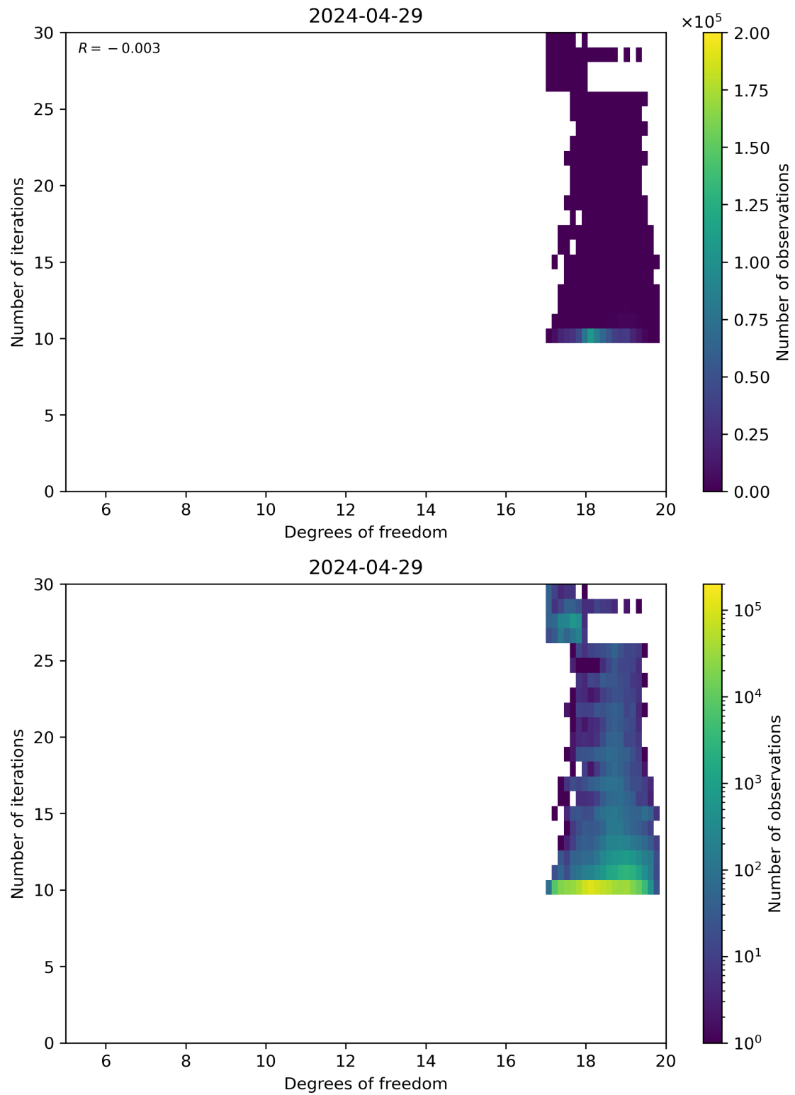
Figure 52: Scatter density plot of “Degrees of freedom” against “Number of iterations” for 2024-04-28 to 2024-04-30.
