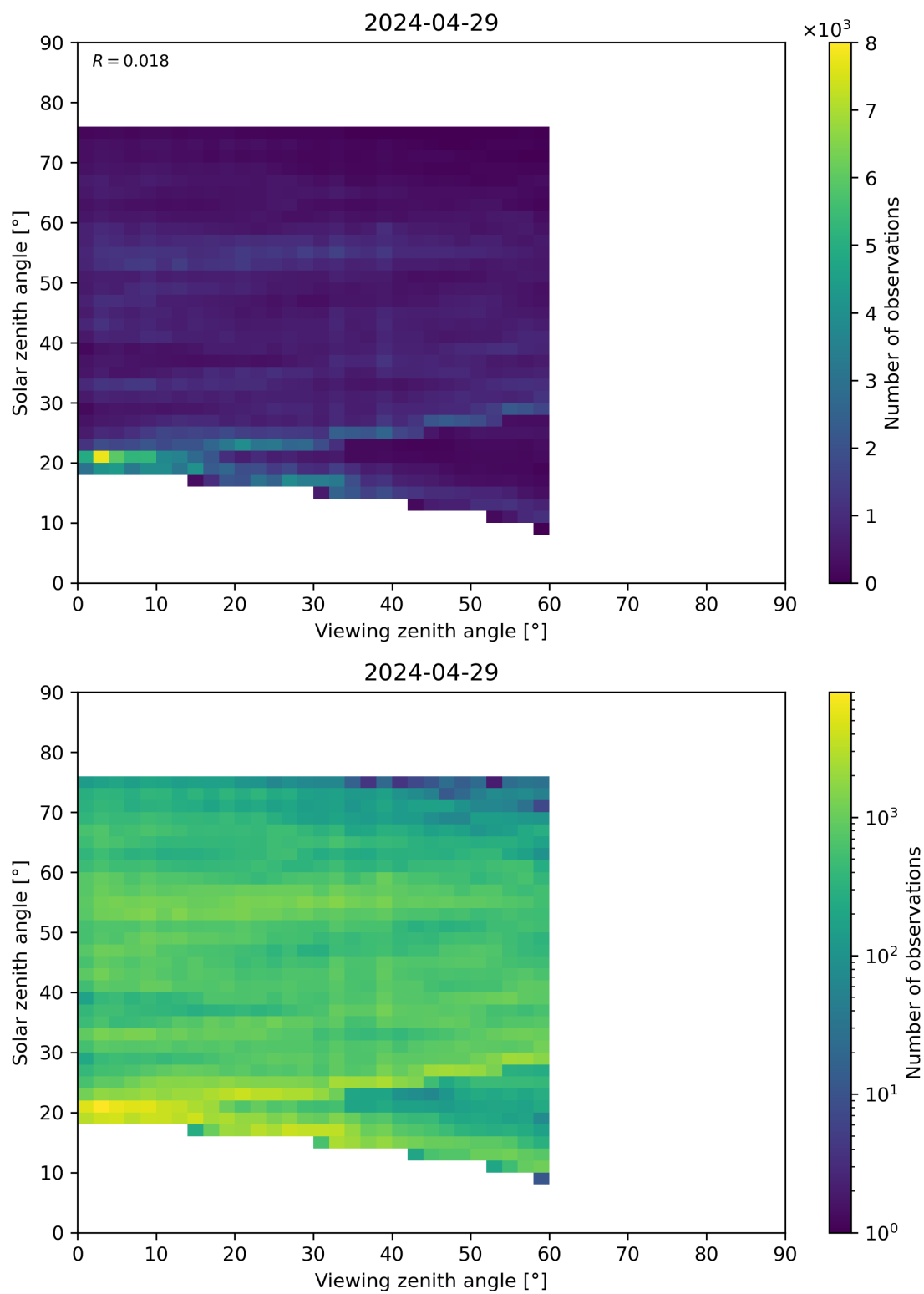
Figure 115: Scatter density plot of “Viewing zenith angle” against “Solar zenith angle” for 2024-04-28 to 2024-04-30.
