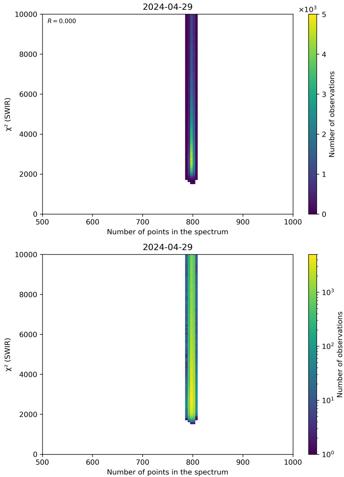
Figure 89: Scatter density plot of “Number of points in the spectrum” against “ \chi^2 (SWIR)” for 2024-04-28 to 2024-04-30.
