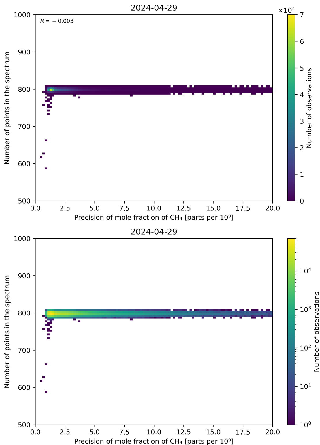
Figure 84: Scatter density plot of “Precision of mole fraction of CH 4 ” against “Number of points in the spectrum” for 2024-04-28 to 2024-04-30.
