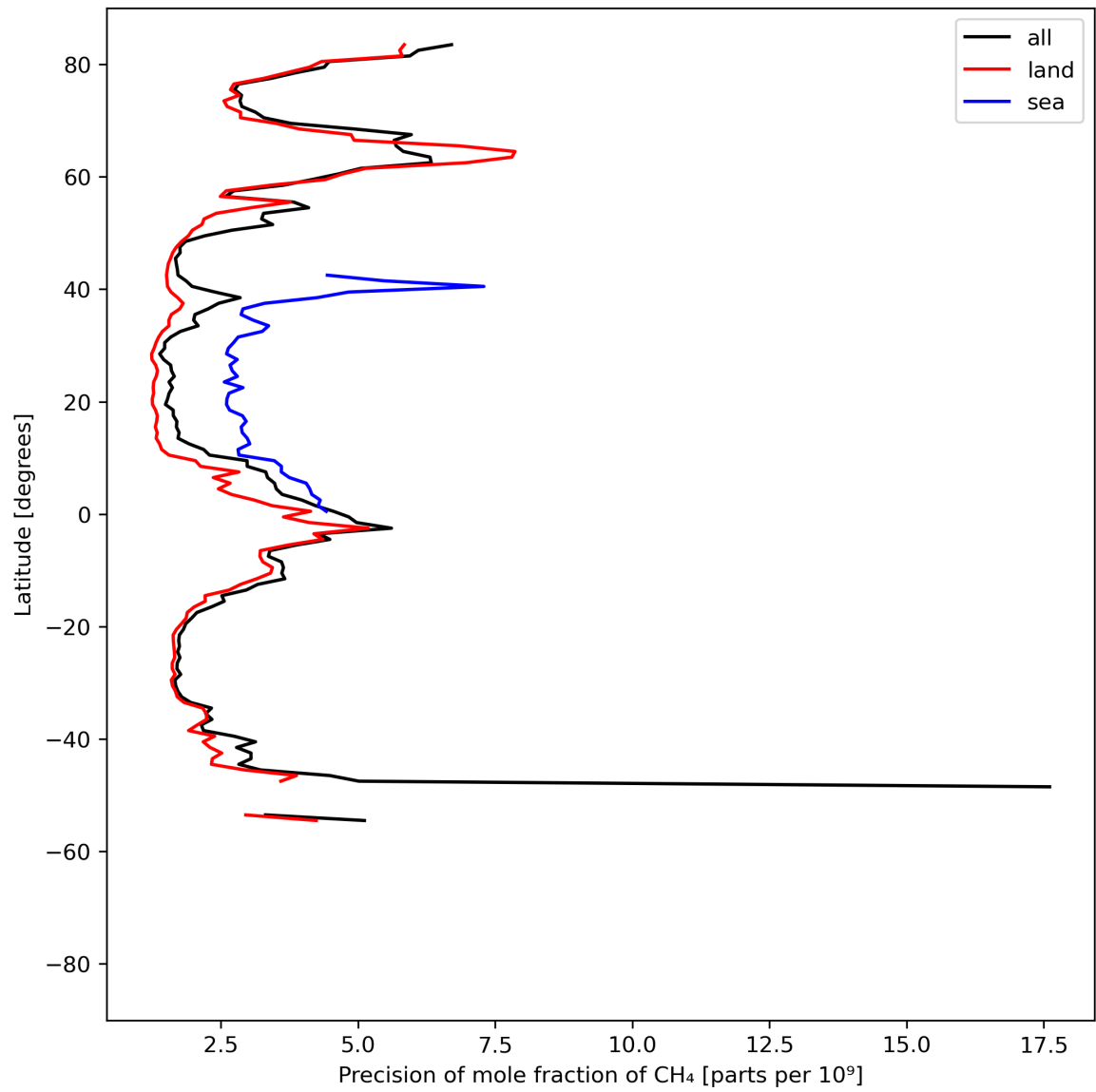
Figure 13: Zonal average of “Precision of mole fraction of CH 4 ” for 2024-04-28 to 2024-04-30.
