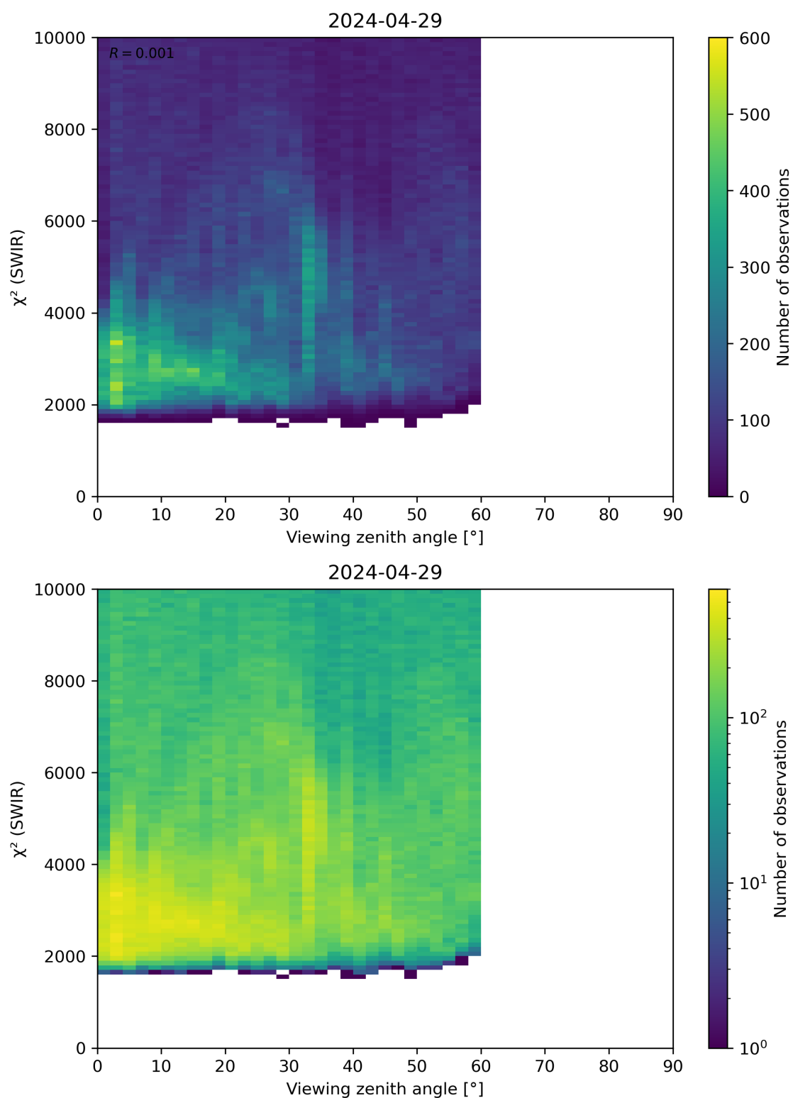
Figure 106: Scatter density plot of “Viewing zenith angle” against “ \chi^2 (SWIR)” for 2024-04-28 to 2024-04-30.
