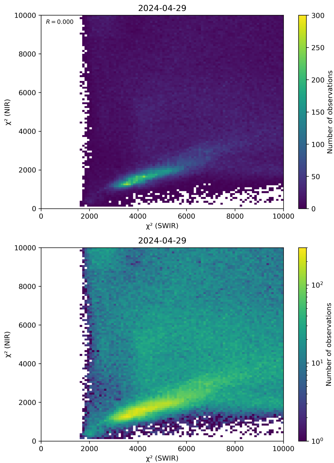
Figure 47: Scatter density plot of “ \chi^2 (SWIR)” against “ \chi^2 (NIR)” for 2024-04-28 to 2024-04-30.
