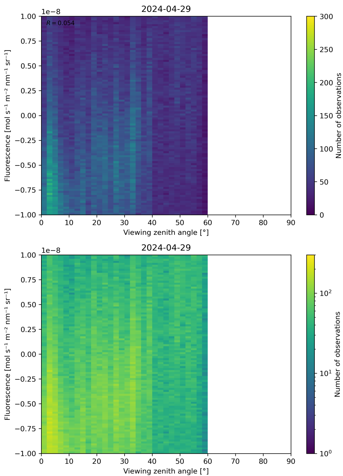
Figure 108: Scatter density plot of “Viewing zenith angle” against “Fluorescence” for 2024-04-28 to 2024-04-30.
