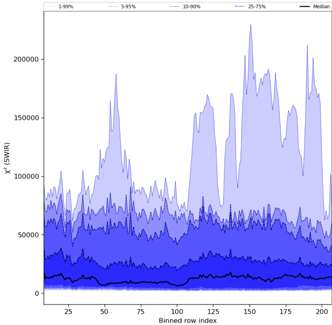
Figure 39: Along track statistics of " \chi^2 (SWIR)" for 2024-04-28 to 2024-04-30
