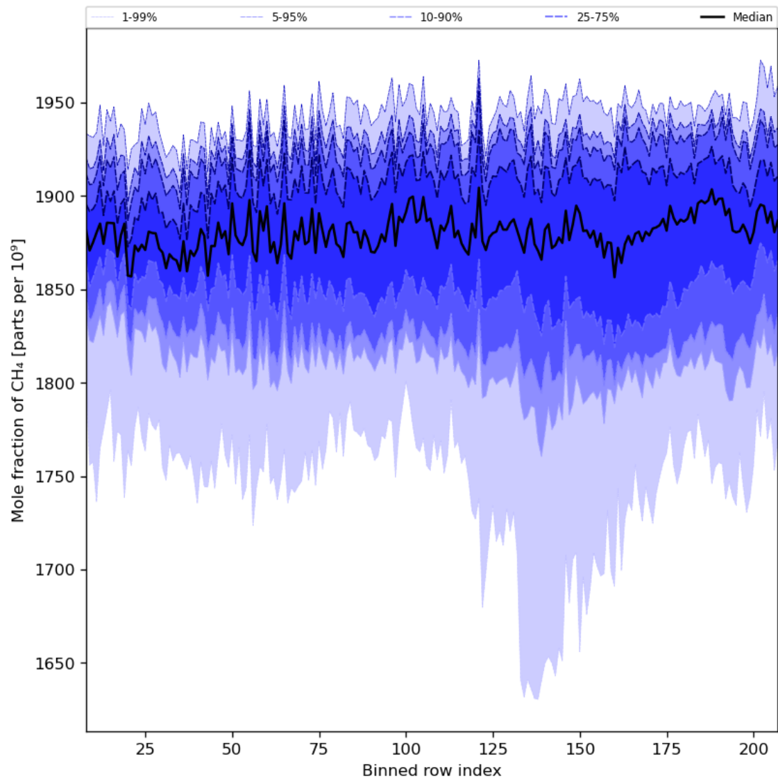
Figure 34: Along track statistics of “Mole fraction of CH 4 ” for 2024-04-28 to 2024-04-30
