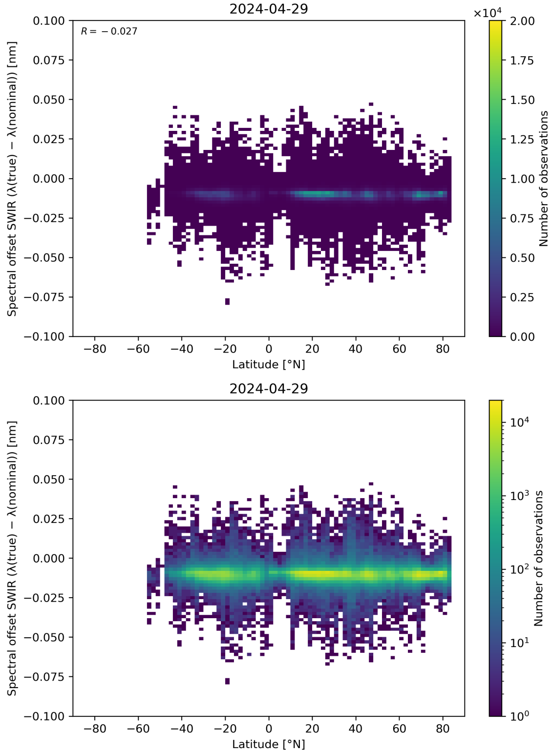
Figure 62: Scatter density plot of “Latitude” against “Spectral offset SWIR ( \lambda(\text{true}) - \lambda(\text{nominal}) )” for 2024-04-28 to 2024-04-30.
