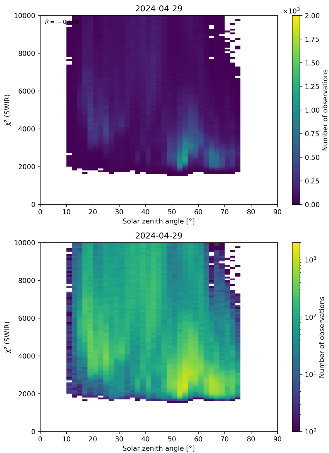
Figure 95: Scatter density plot of “Solar zenith angle” against “ \chi^2 (SWIR)” for 2024-04-28 to 2024-04-30.
