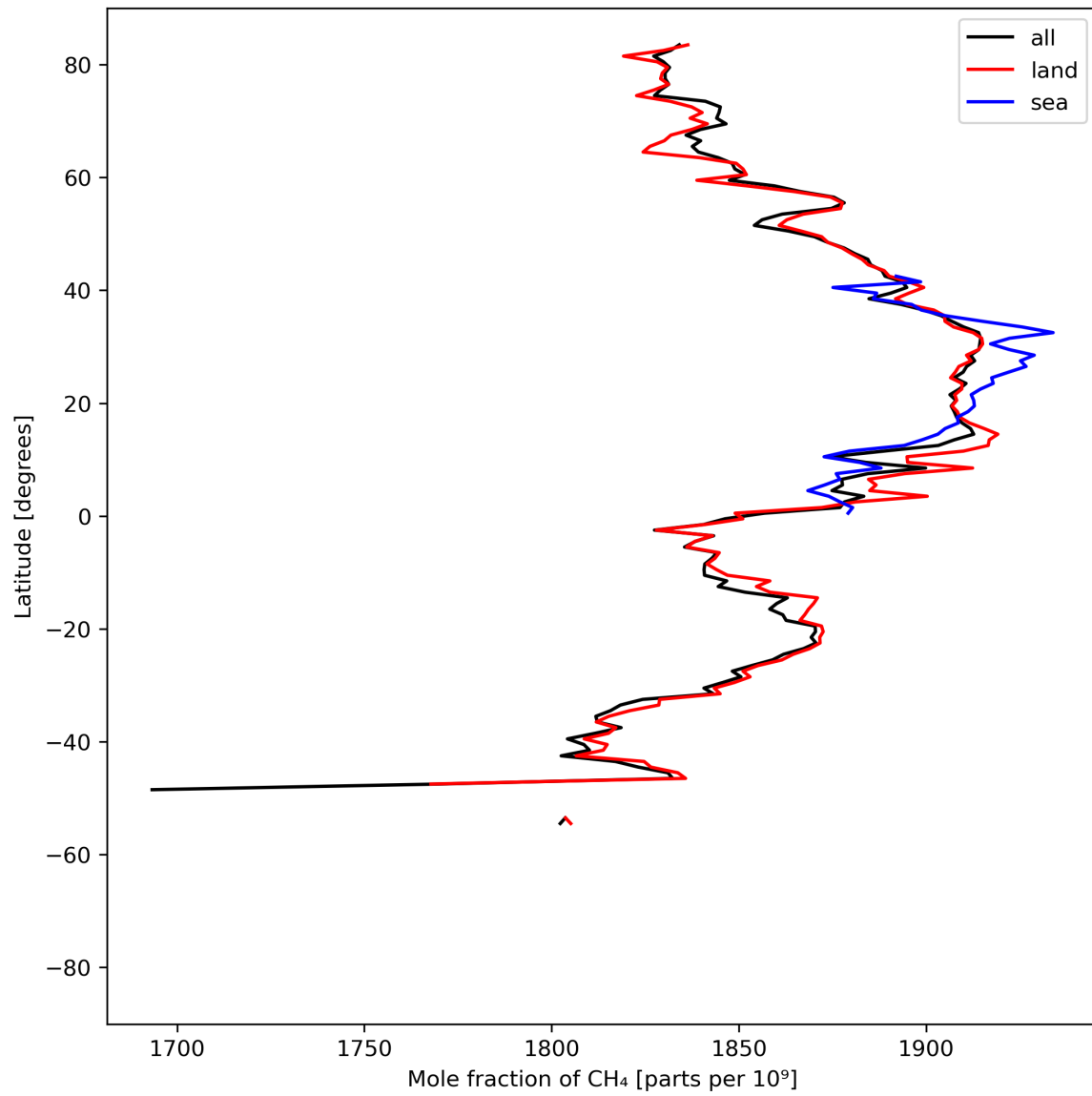
Figure 12: Zonal average of “Mole fraction of \text{CH}_4 ” for 2024-04-28 to 2024-04-30.
