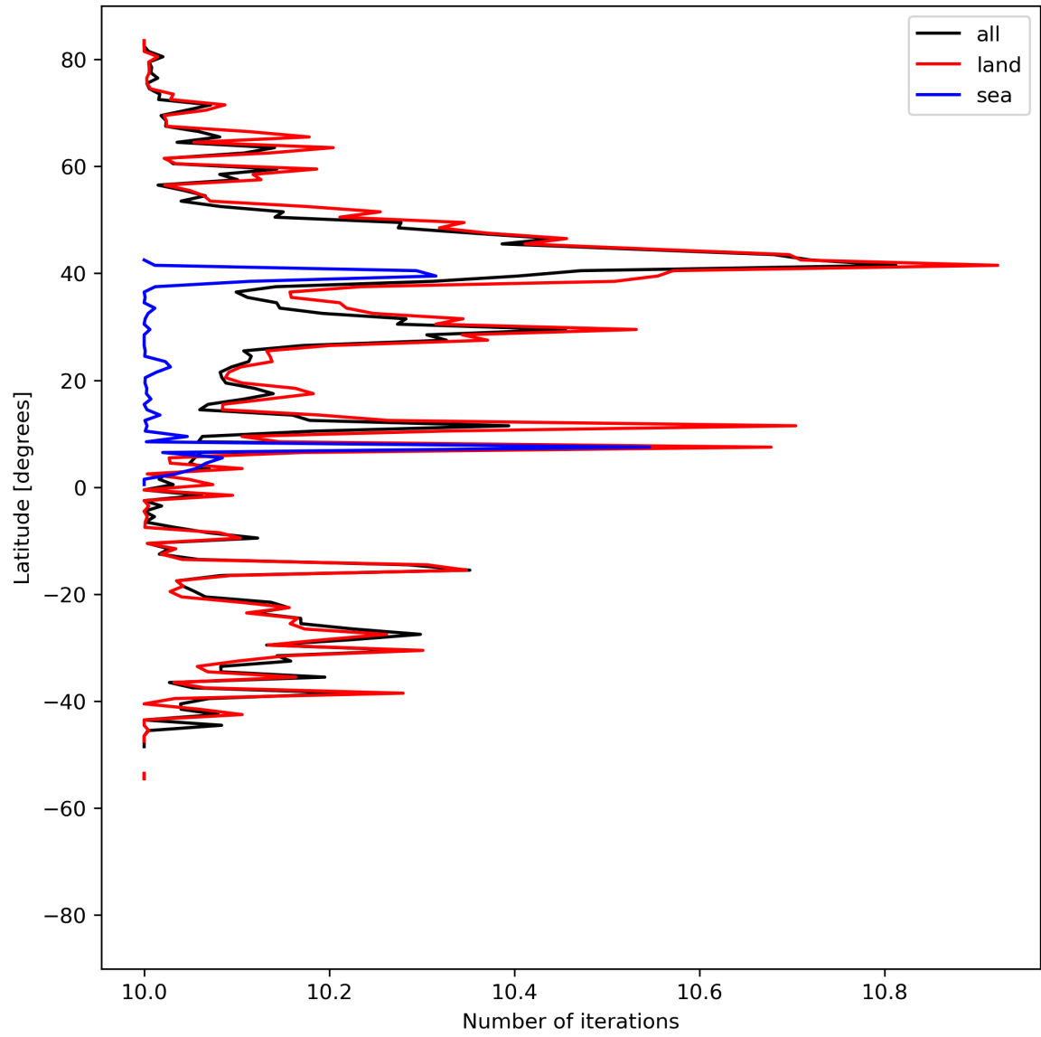
Figure 20: Zonal average of “Number of iterations” for 2024-04-28 to 2024-04-30.
