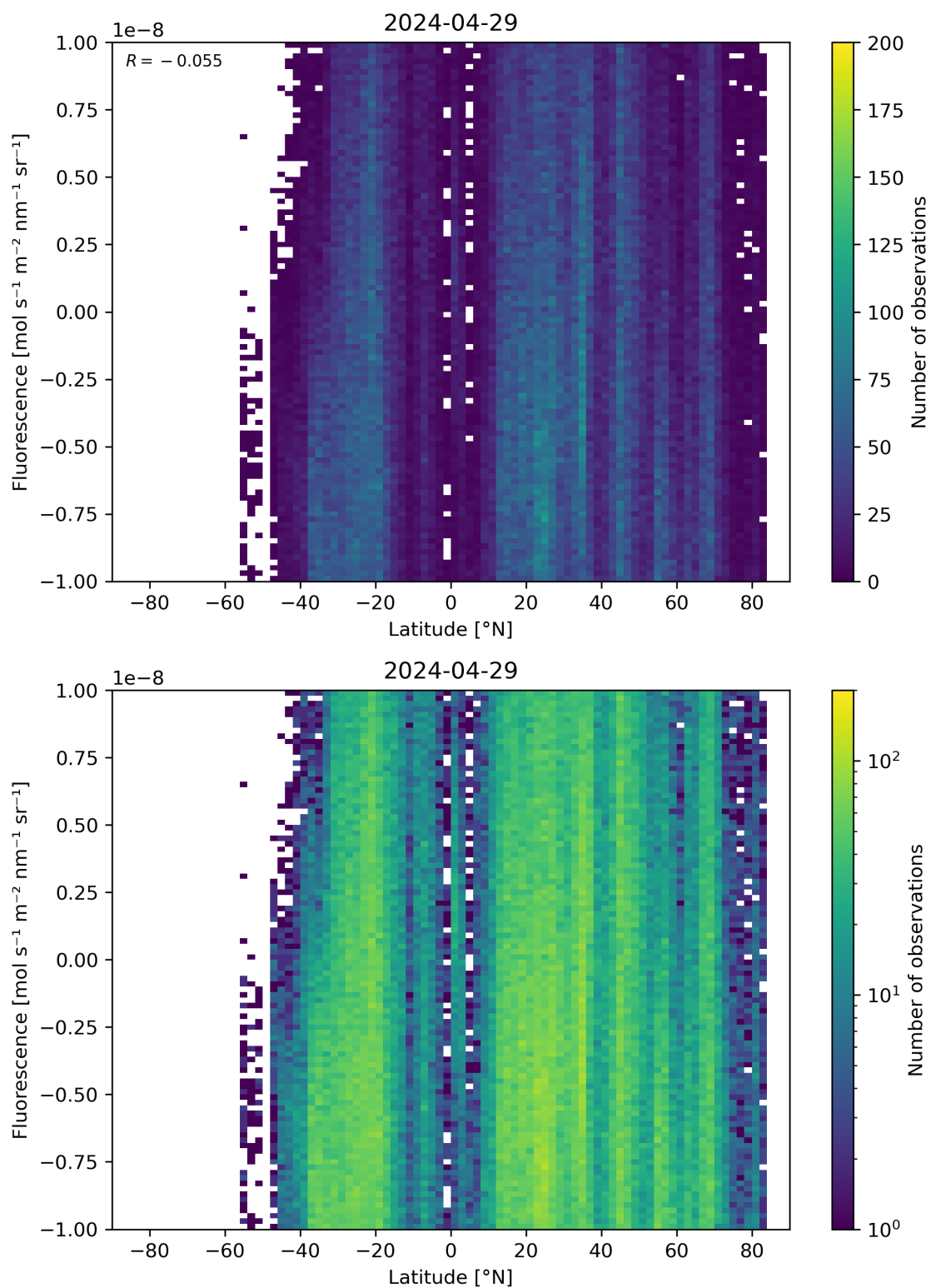
Figure 56: Scatter density plot of “Latitude” against “Fluorescence” for 2024-04-28 to 2024-04-30.
