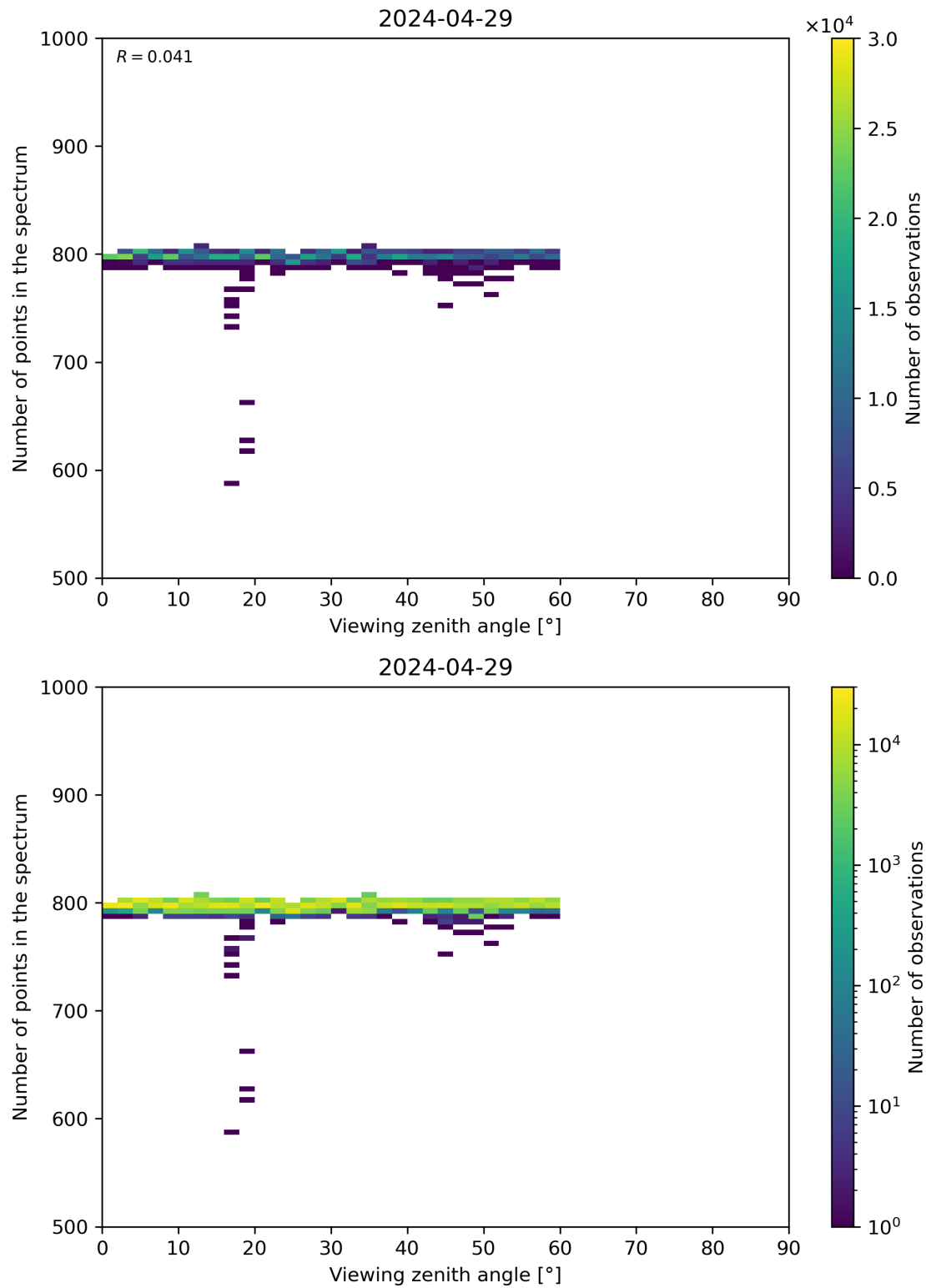
Figure 114: Scatter density plot of “Viewing zenith angle” against “Number of points in the spectrum” for 2024-04-28 to 2024-04-30.
