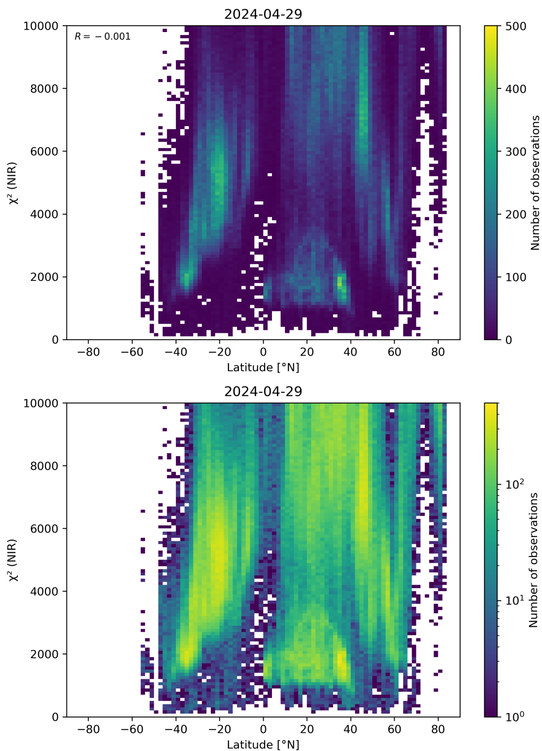
Figure 53: Scatter density plot of “Latitude” against “ \chi^2 (NIR)” for 2024-04-28 to 2024-04-30.
