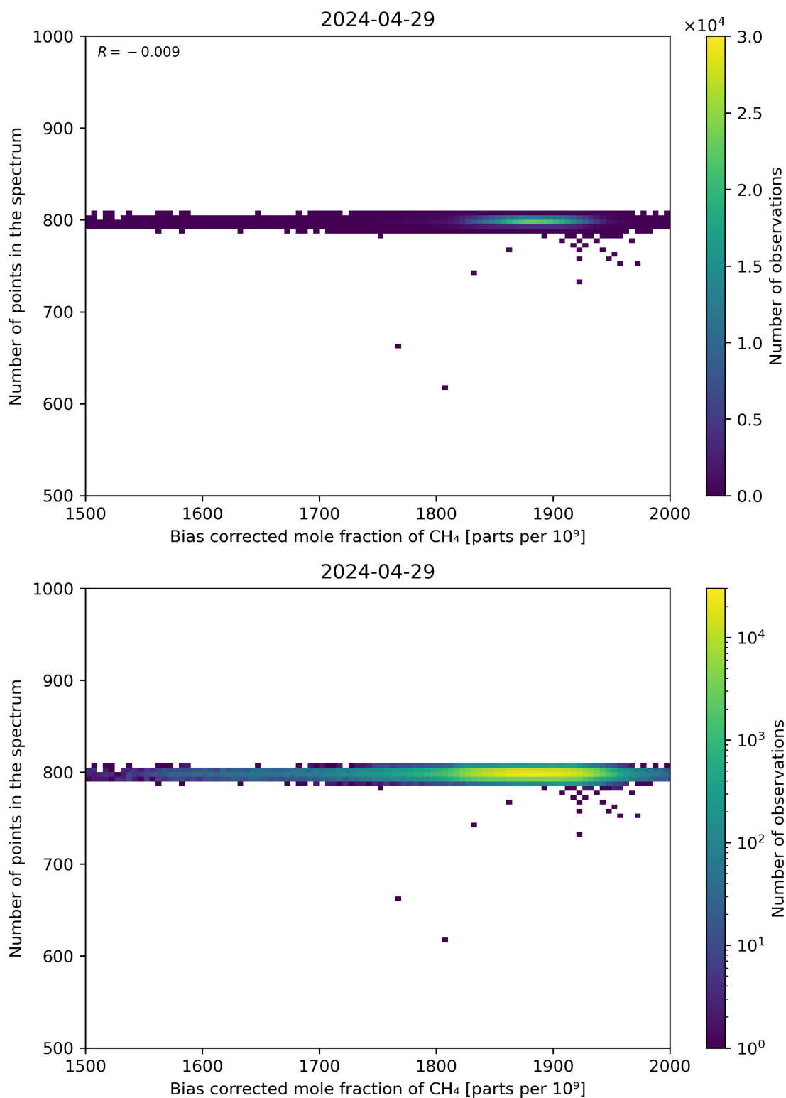
Figure 68: Scatter density plot of “Bias corrected mole fraction of CH 4 ” against “Number of points in the spectrum” for 2024-04-28 to 2024-04-30.
