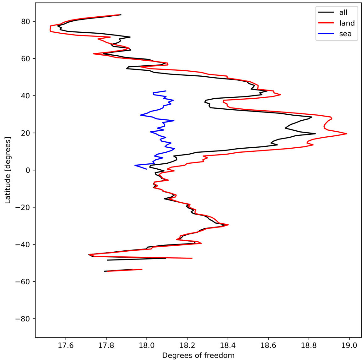
Figure 19: Zonal average of “Degrees of freedom” for 2024-04-28 to 2024-04-30.
