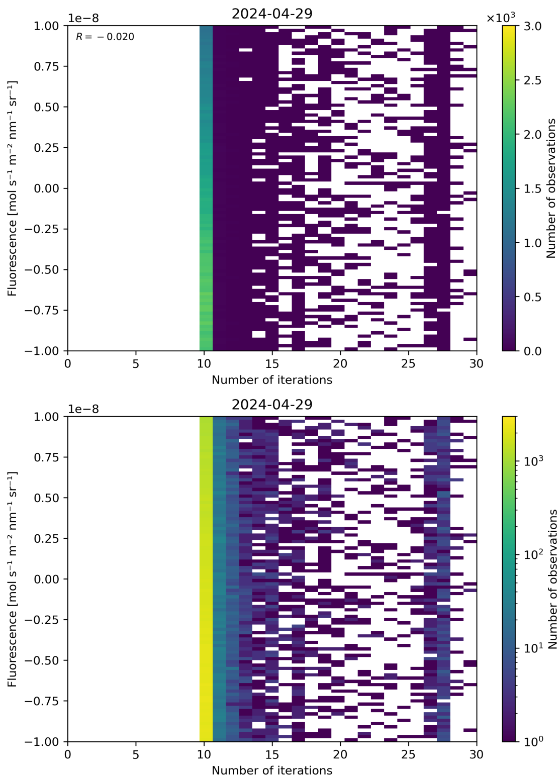
Figure 87: Scatter density plot of “Number of iterations” against “Fluorescence” for 2024-04-28 to 2024-04-30.
