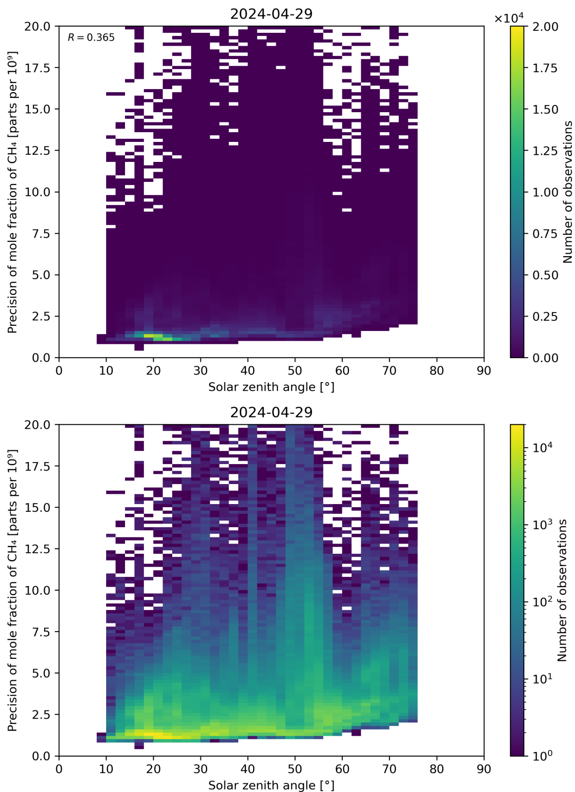
Figure 101: Scatter density plot of “Solar zenith angle” against “Precision of mole fraction of CH 4 ” for 2024-04-28 to 2024-04-30.
