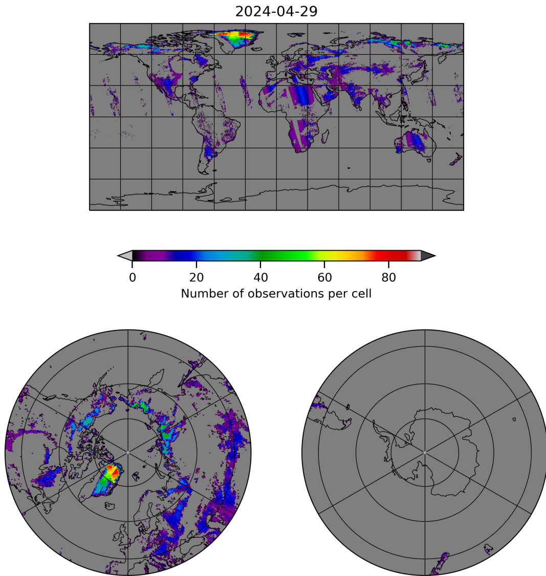
Figure 10: Map of the number of observations for 2024-04-28 to 2024-04-30
