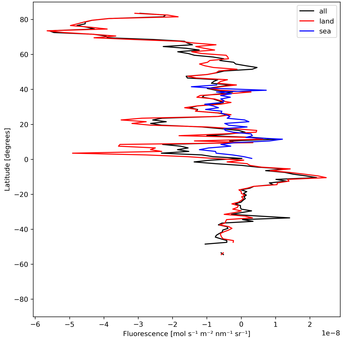
Figure 21: Zonal average of "Fluorescence" for 2024-04-28 to 2024-04-30.
