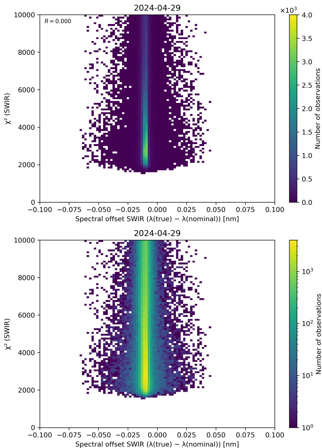
Figure 118: Scatter density plot of “Spectral offset SWIR ( \lambda(\text{true}) - \lambda(\text{nominal}) )” against “ \chi^2 (SWIR)” for 2024-04-28 to 2024-04-30.
