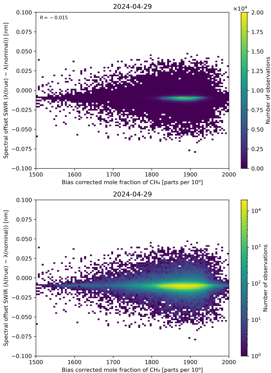
Figure 69: Scatter density plot of “Bias corrected mole fraction of \text{CH}_4 ” against “Spectral offset SWIR ( \lambda(\text{true}) - \lambda(\text{nominal}) )” for 2024-04-28 to 2024-04-30.
