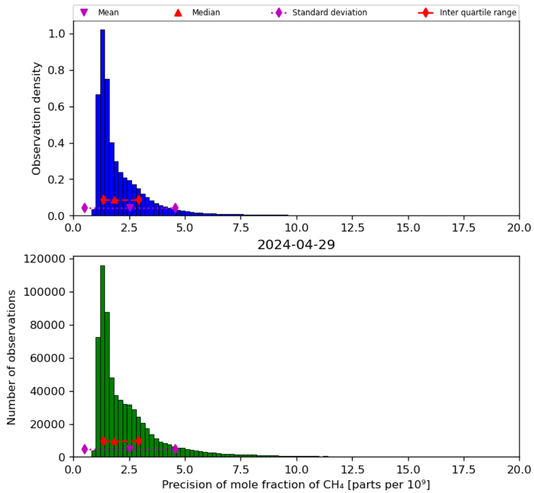
Figure 24: Histogram of “Precision of mole fraction of CH 4 ” for 2024-04-28 to 2024-04-30
