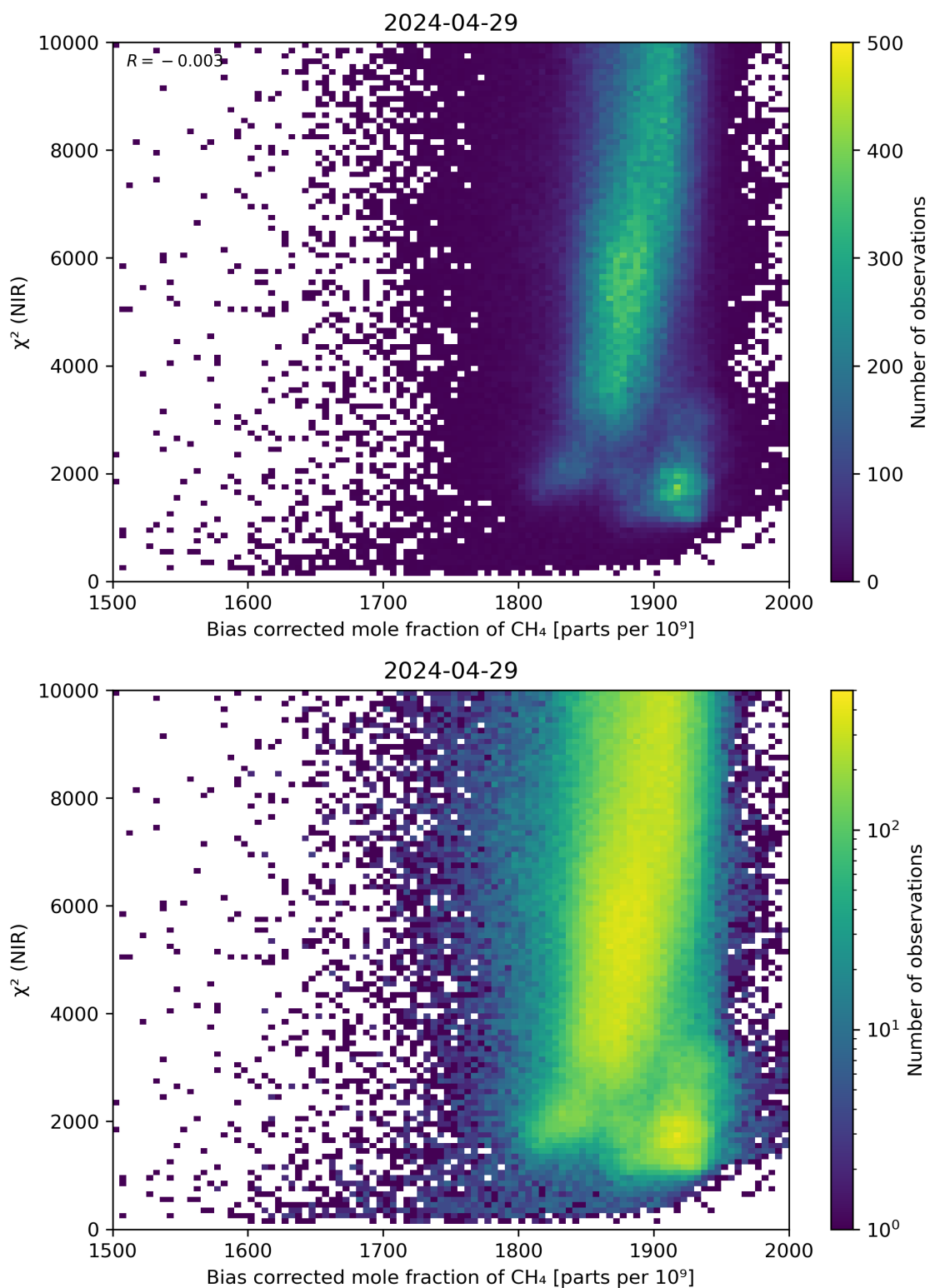
Figure 63: Scatter density plot of “Bias corrected mole fraction of CH 4 ” against “ \chi^2 (NIR)” for 2024-04-28 to 2024-04-30.
