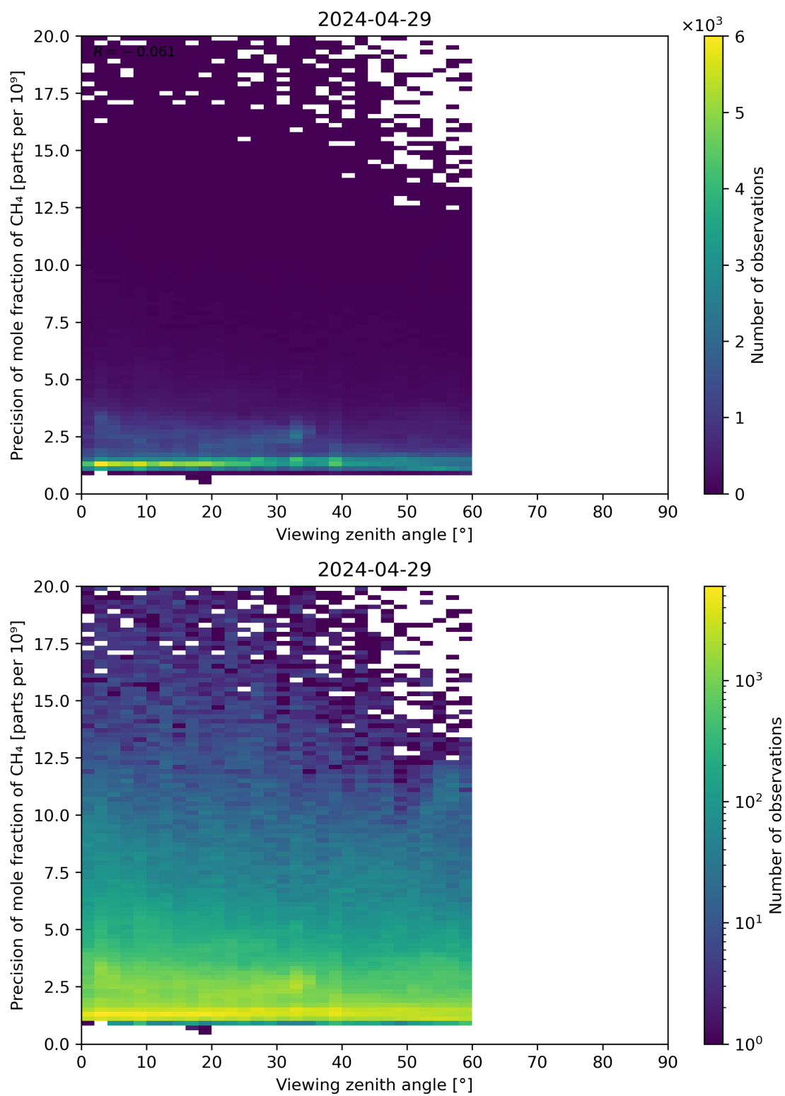
Figure 112: Scatter density plot of “Viewing zenith angle” against “Precision of mole fraction of CH 4 ” for 2024-04-28 to 2024-04-30.
