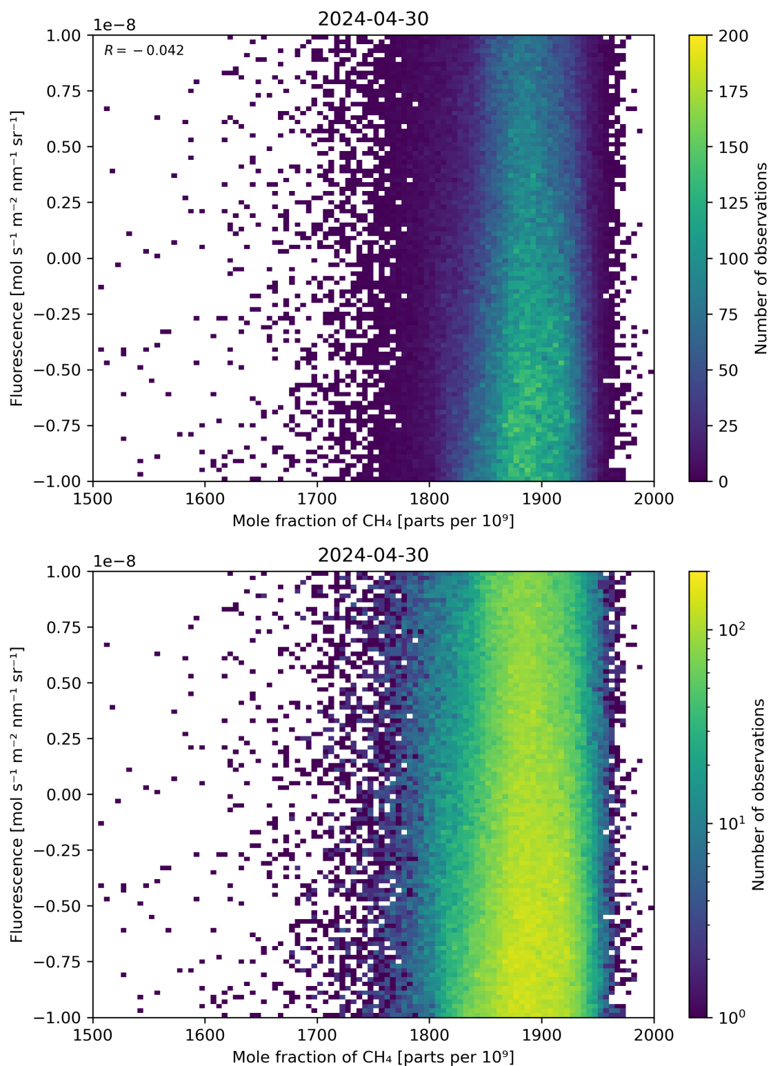
Figure 73: Scatter density plot of “Mole fraction of \text{CH}_4 ” against “Fluorescence” for 2024-04-29 to 2024-05-01.
