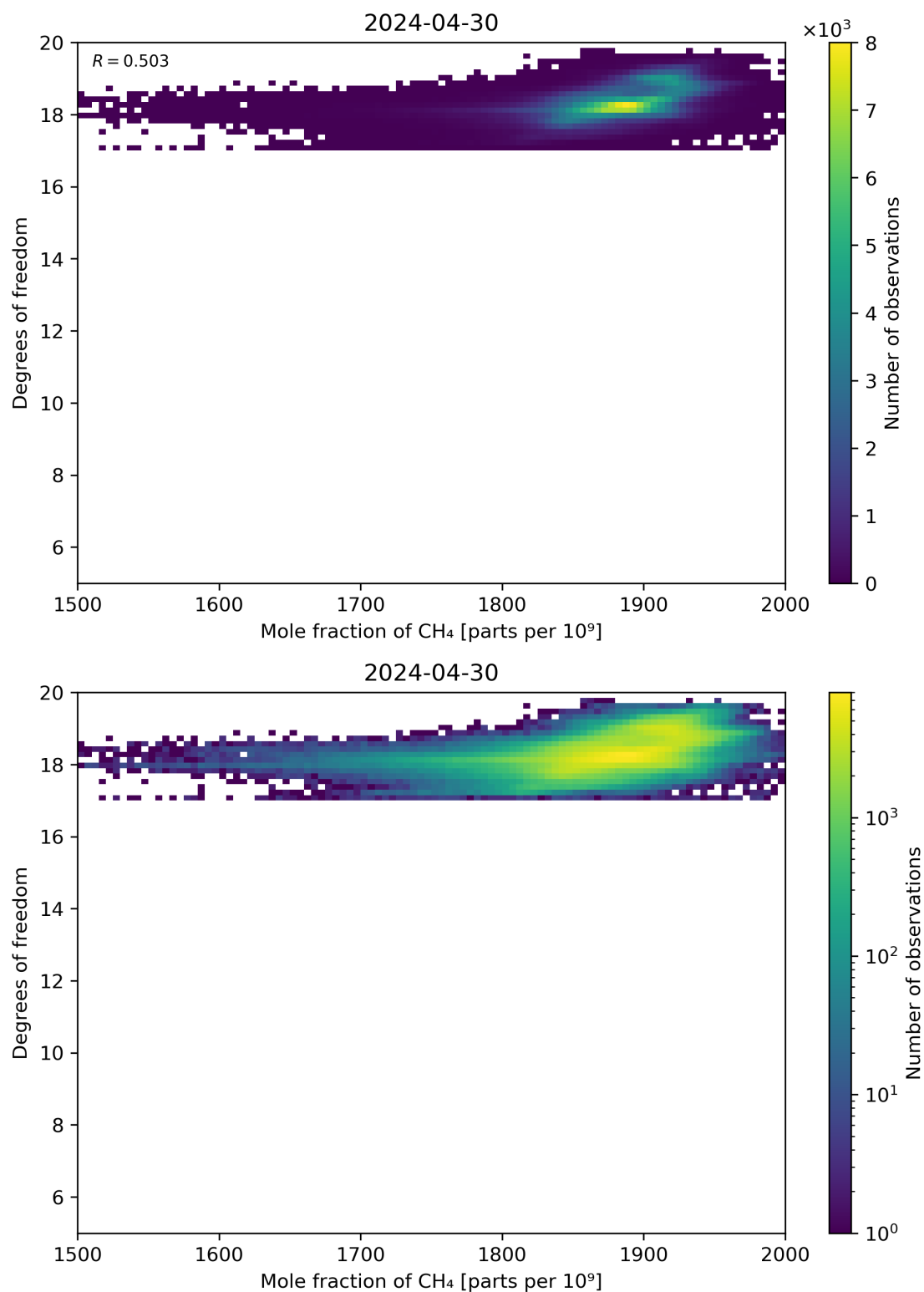
Figure 72: Scatter density plot of “Mole fraction of CH 4 ” against “Degrees of freedom” for 2024-04-29 to 2024-05-01.
