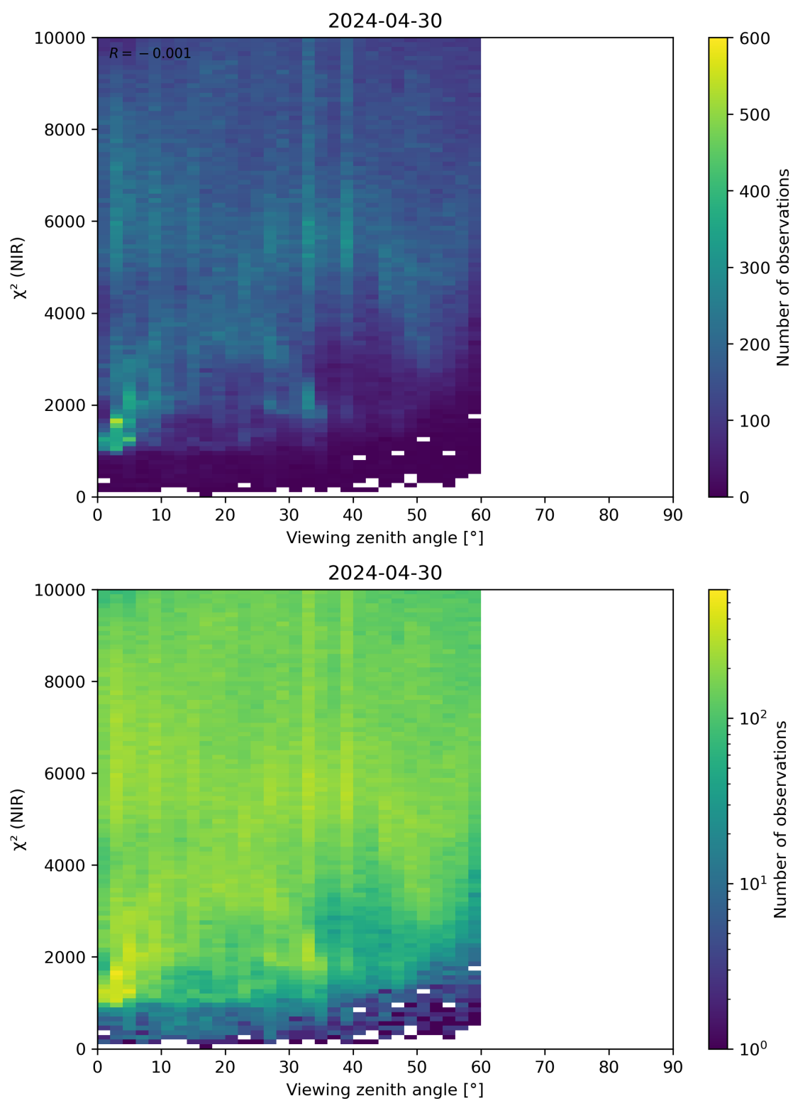
Figure 105: Scatter density plot of “Viewing zenith angle” against “ \chi^2 (NIR)” for 2024-04-29 to 2024-05-01.
