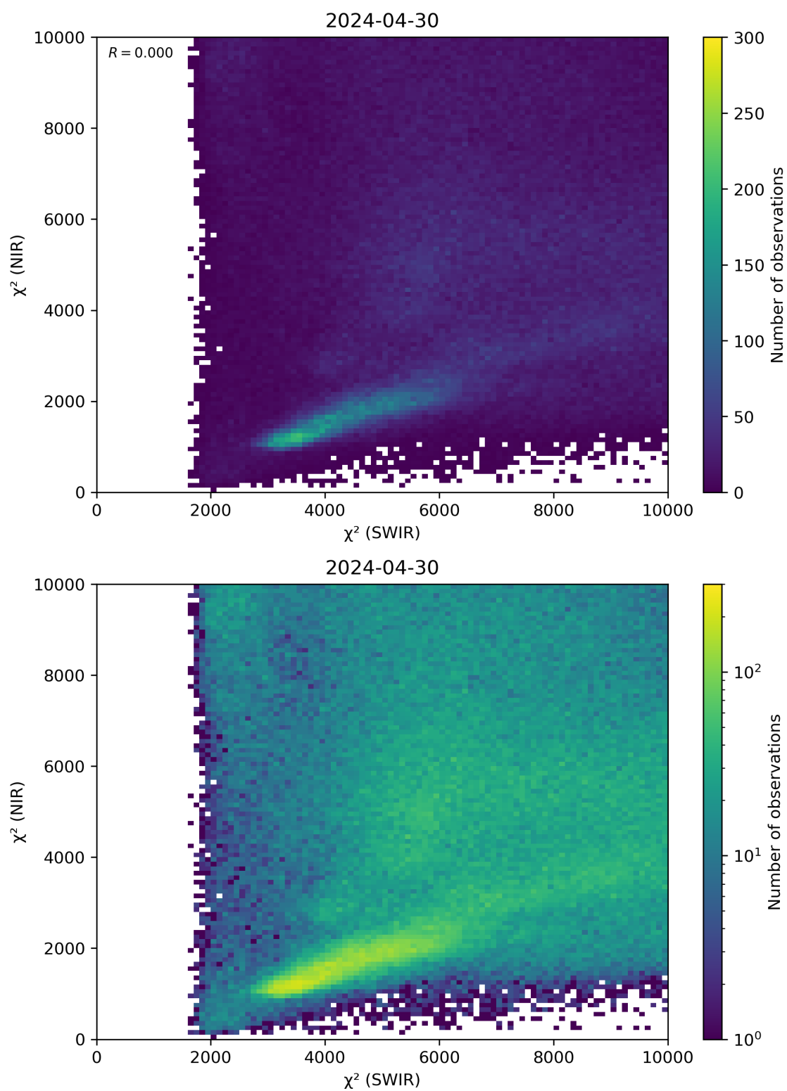
Figure 47: Scatter density plot of “ \chi^2 (SWIR)” against “ \chi^2 (NIR)” for 2024-04-29 to 2024-05-01.
