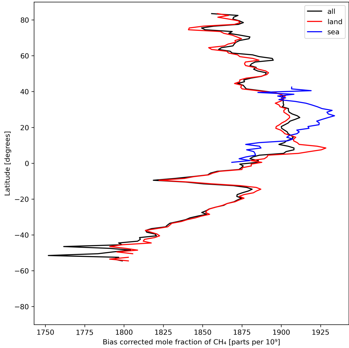
Figure 14: Zonal average of “Bias corrected mole fraction of CH 4 ” for 2024-04-29 to 2024-05-01.
