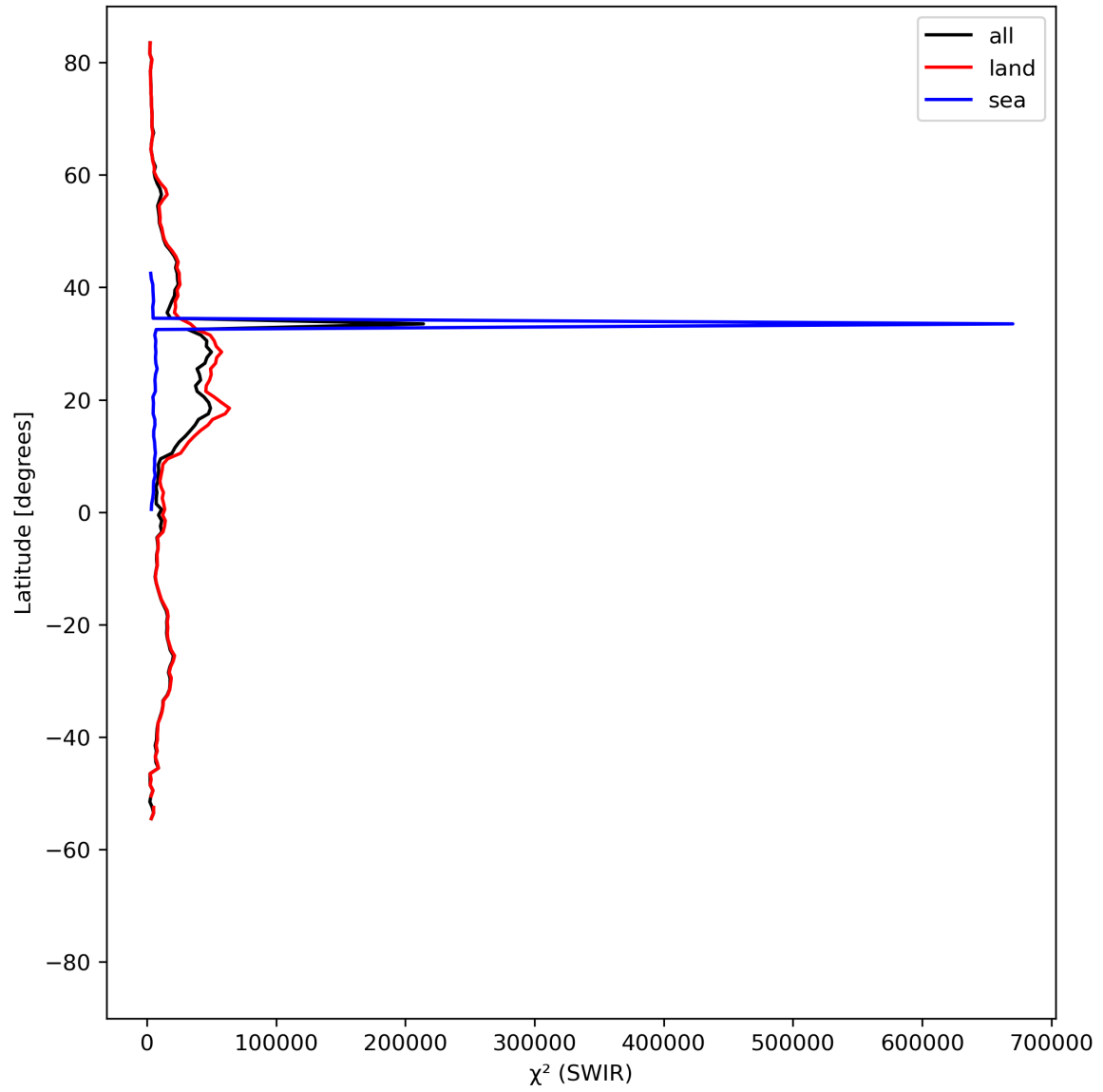
Figure 17: Zonal average of “ \chi^2 (SWIR)” for 2024-04-29 to 2024-05-01.
