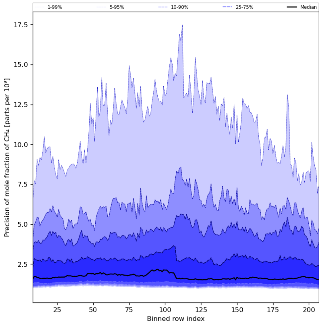
Figure 35: Along track statistics of “Precision of mole fraction of CH 4 ” for 2024-04-29 to 2024-05-01
