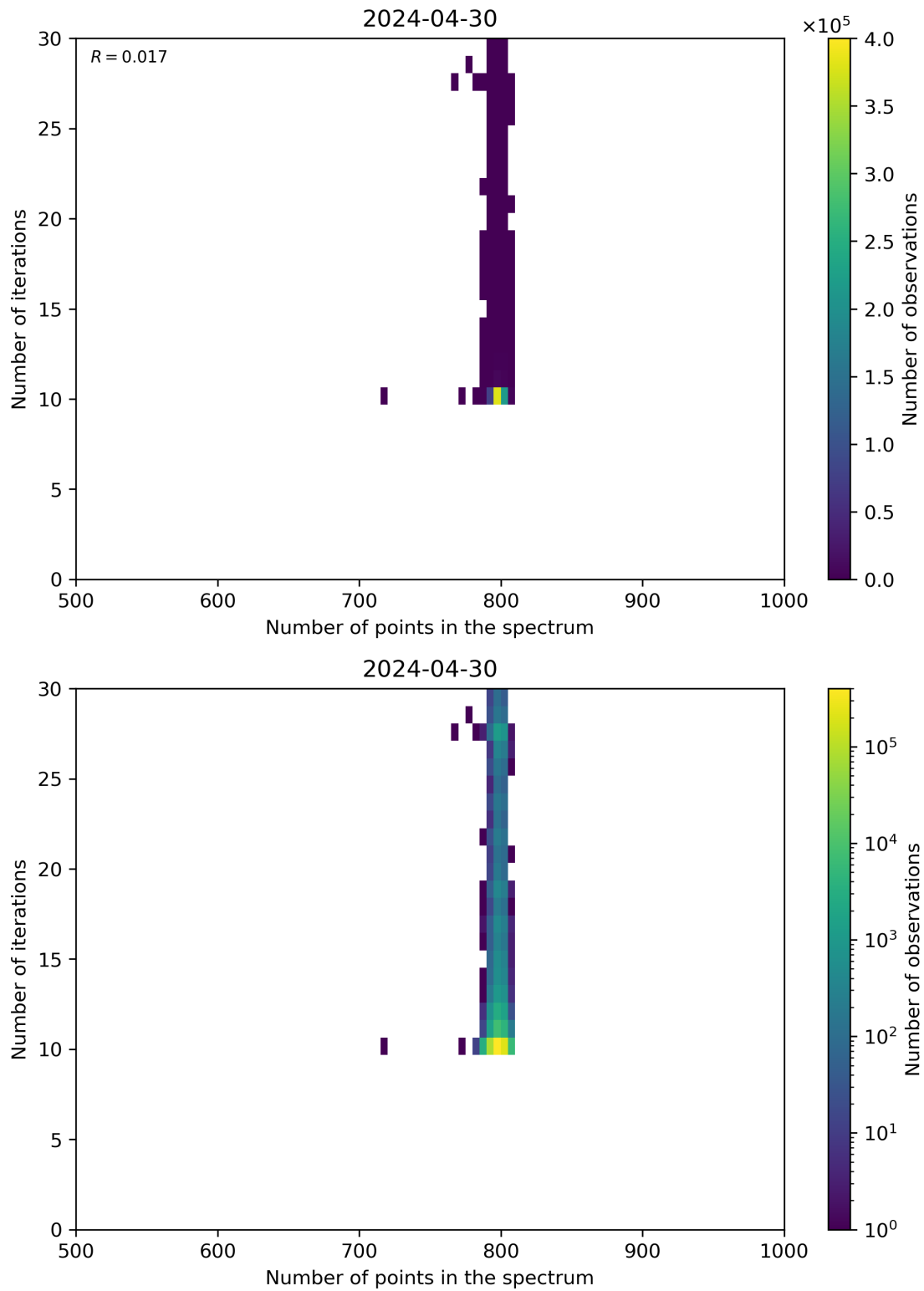
Figure 92: Scatter density plot of “Number of points in the spectrum” against “Number of iterations” for 2024-04-29 to 2024-05-01.
