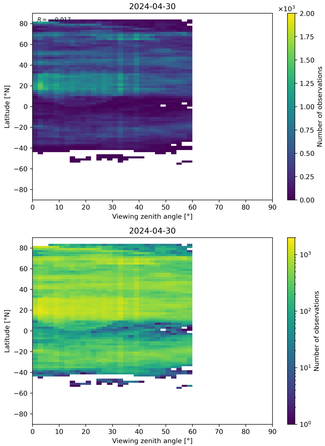
Figure 109: Scatter density plot of “Viewing zenith angle” against “Latitude” for 2024-04-29 to 2024-05-01.
