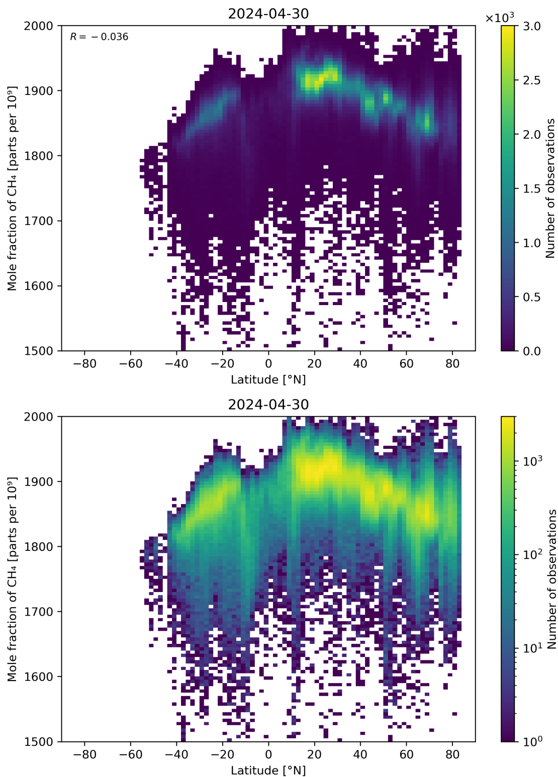
Figure 57: Scatter density plot of “Latitude” against “Mole fraction of \text{CH}_4 ” for 2024-04-29 to 2024-05-01.
