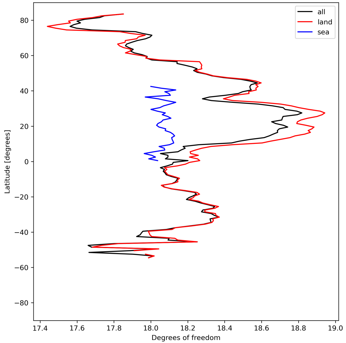
Figure 19: Zonal average of “Degrees of freedom” for 2024-04-29 to 2024-05-01.
