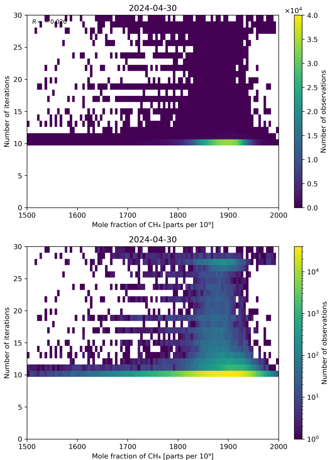
Figure 76: Scatter density plot of “Mole fraction of CH 4 ” against “Number of iterations” for 2024-04-29 to 2024-05-01.
