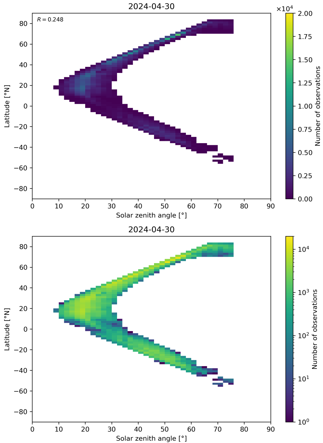
Figure 98: Scatter density plot of “Solar zenith angle” against “Latitude” for 2024-04-29 to 2024-05-01.
