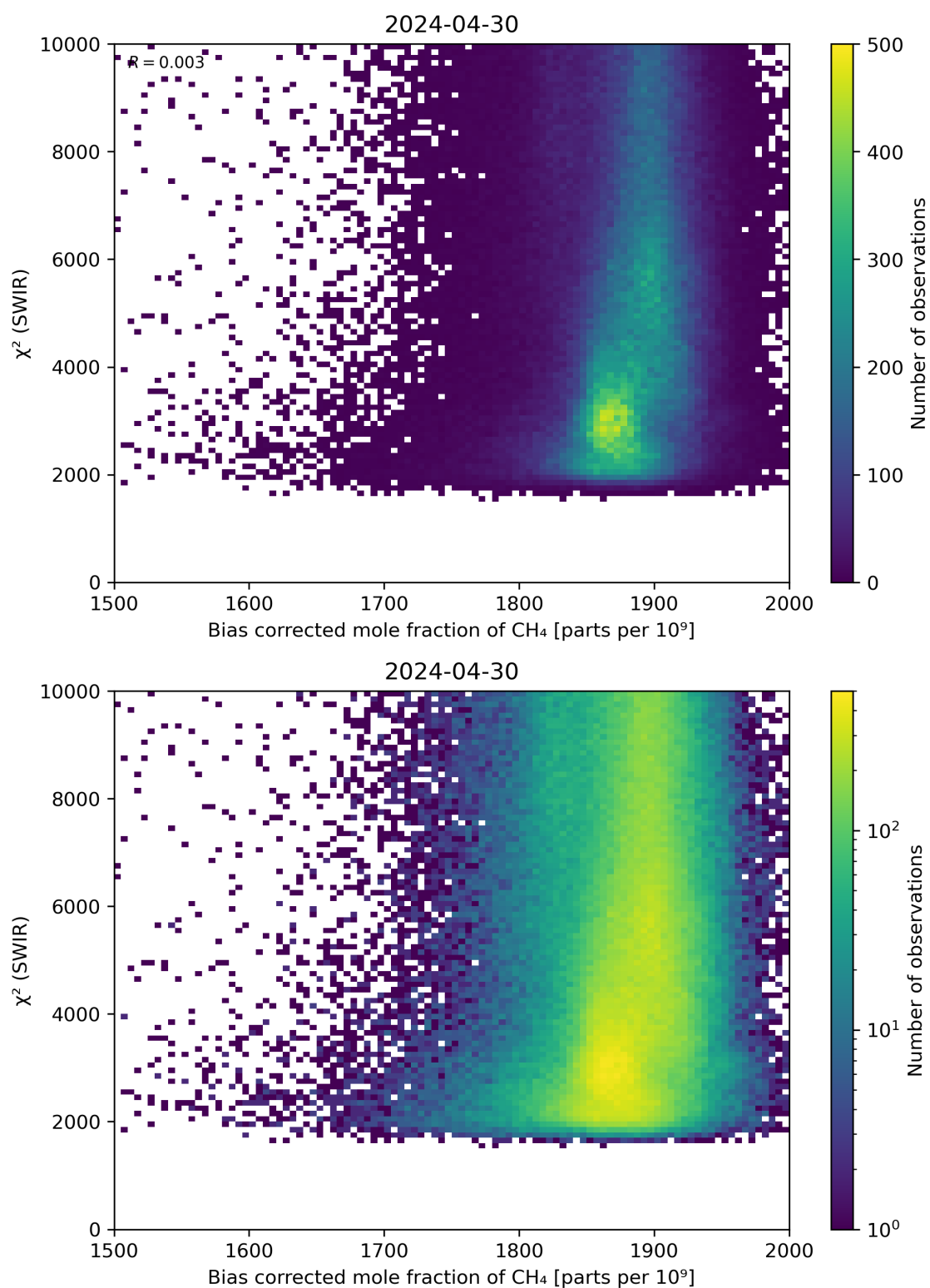
Figure 64: Scatter density plot of “Bias corrected mole fraction of CH 4 ” against “ \chi^2 (SWIR)” for 2024-04-29 to 2024-05-01.
