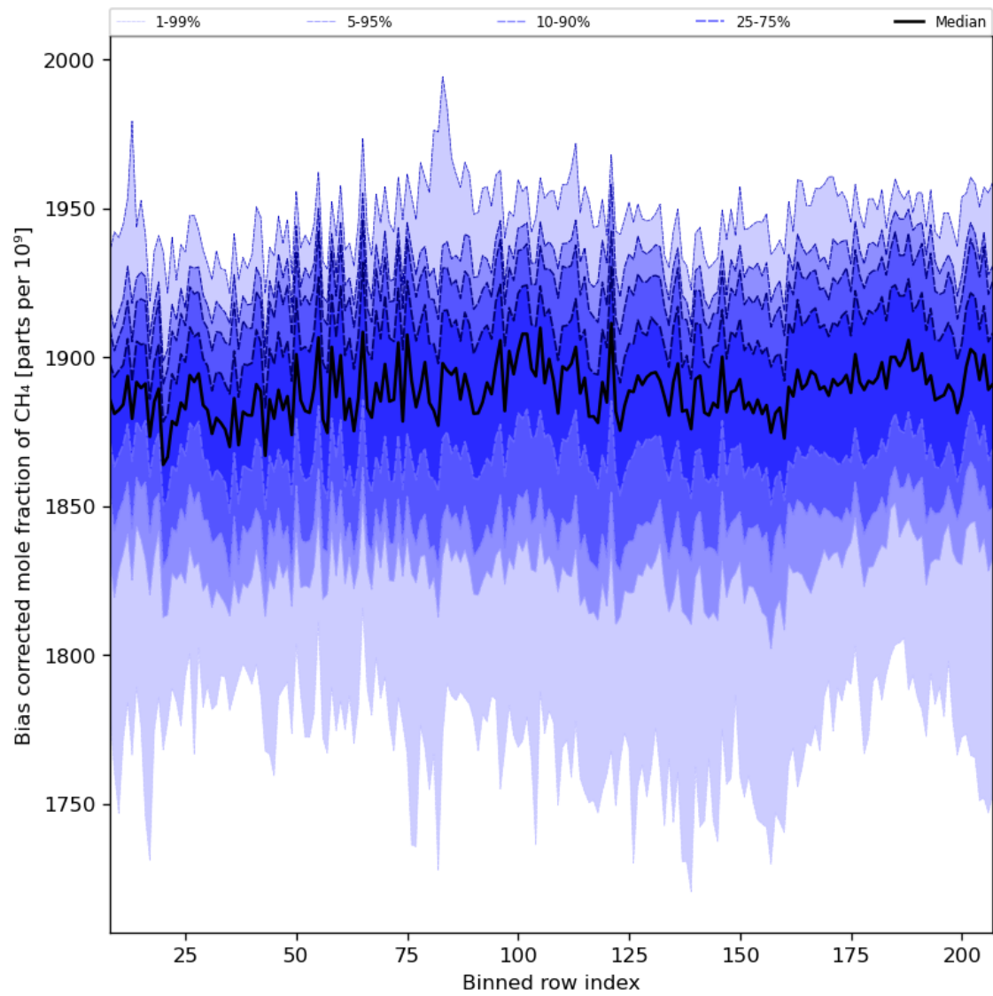
Figure 36: Along track statistics of “Bias corrected mole fraction of CH 4 ” for 2024-04-29 to 2024-05-01
