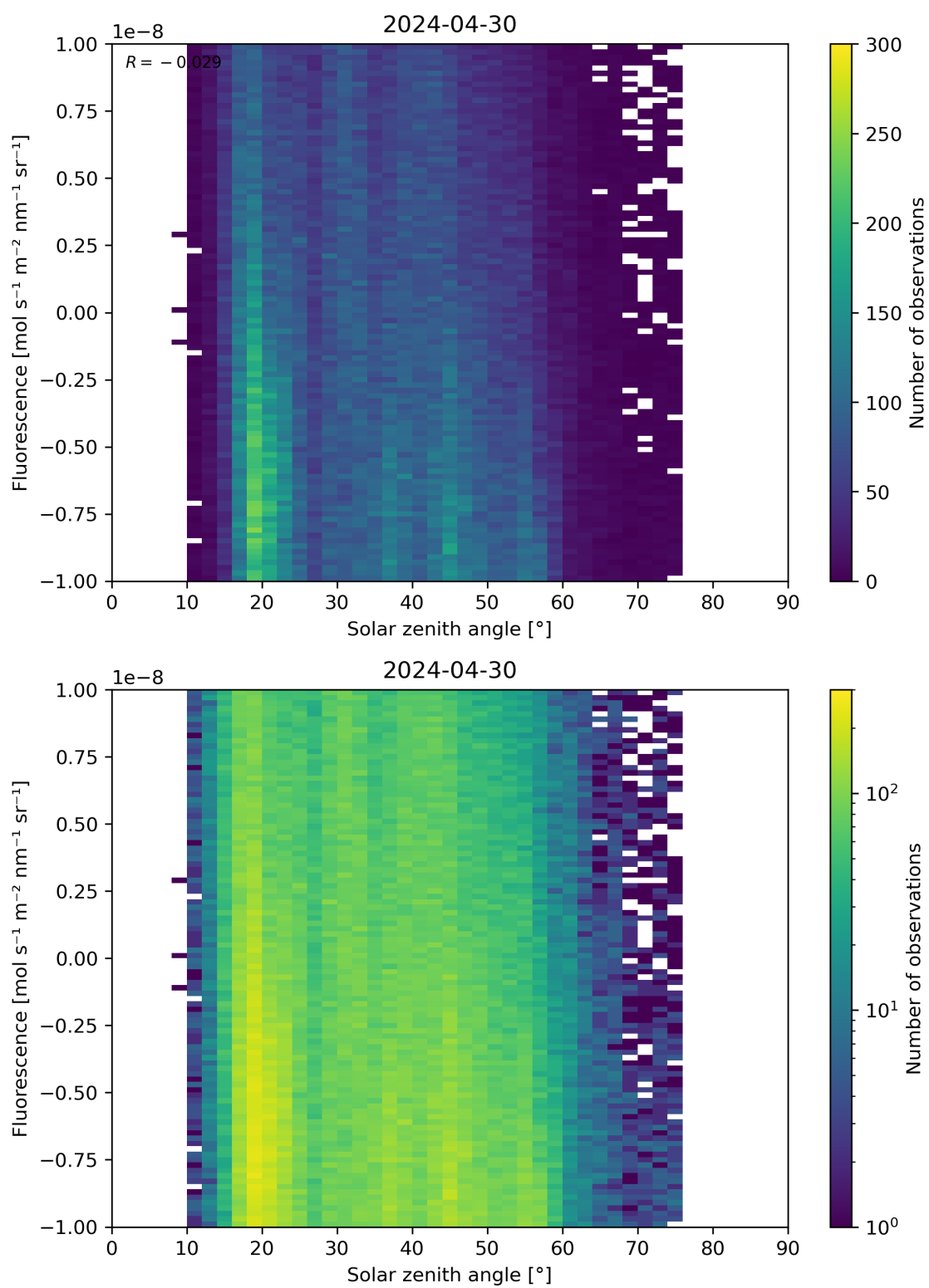
Figure 97: Scatter density plot of “Solar zenith angle” against “Fluorescence” for 2024-04-29 to 2024-05-01.
