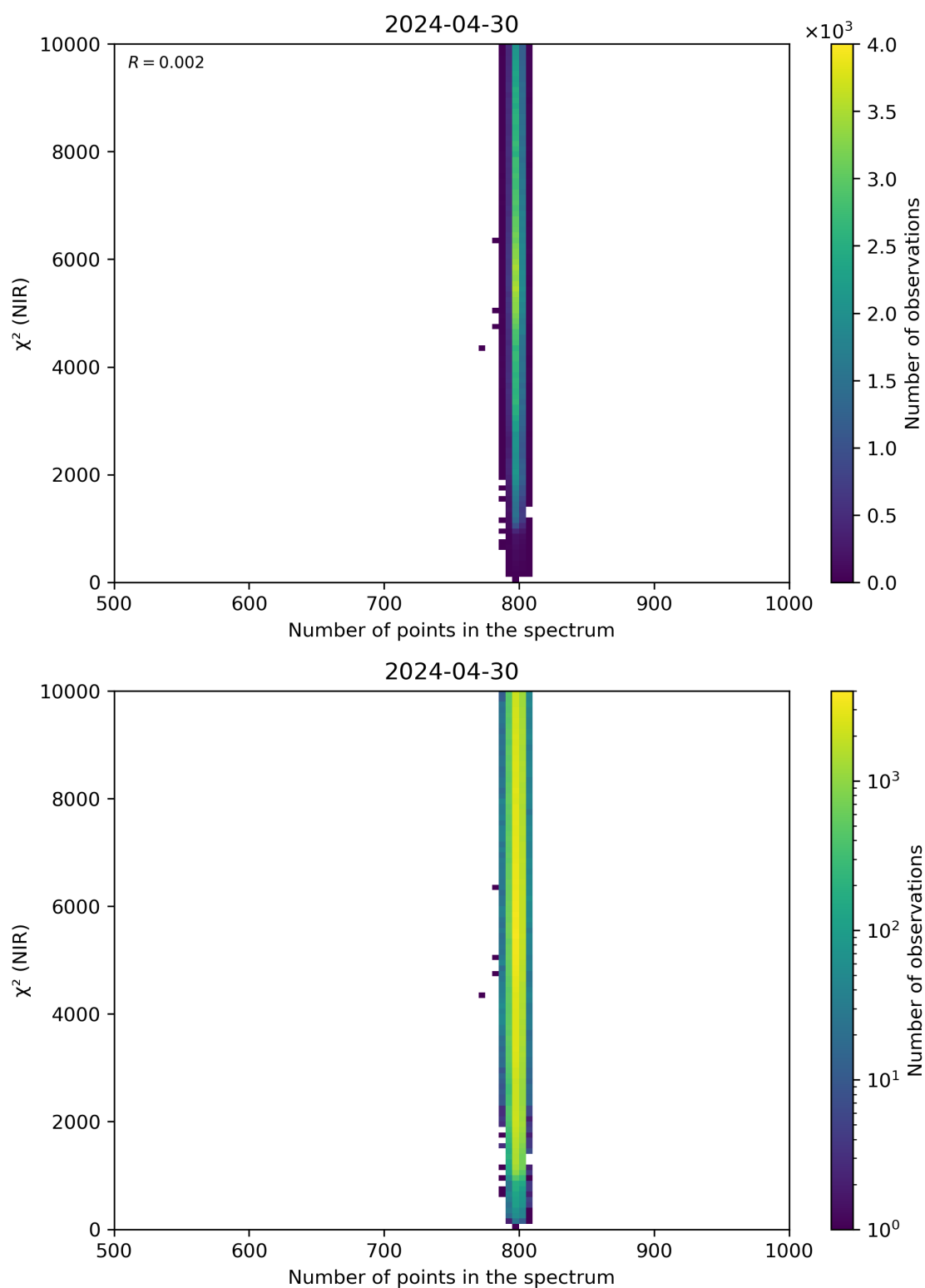
Figure 88: Scatter density plot of “Number of points in the spectrum” against “ \chi^2 (NIR)” for 2024-04-29 to 2024-05-01.
