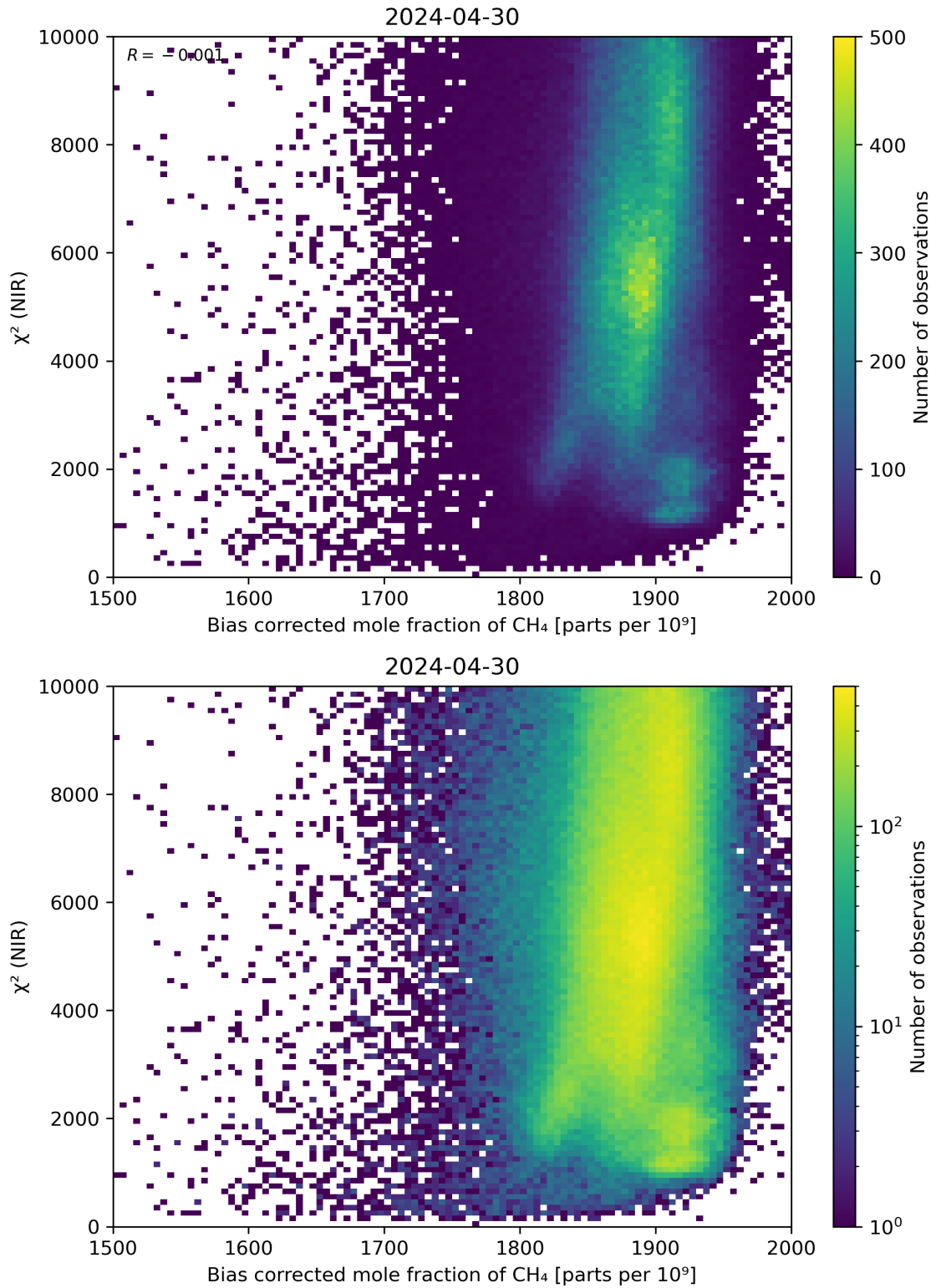
Figure 63: Scatter density plot of “Bias corrected mole fraction of CH 4 ” against “ \chi^2 (NIR)” for 2024-04-29 to 2024-05-01.
