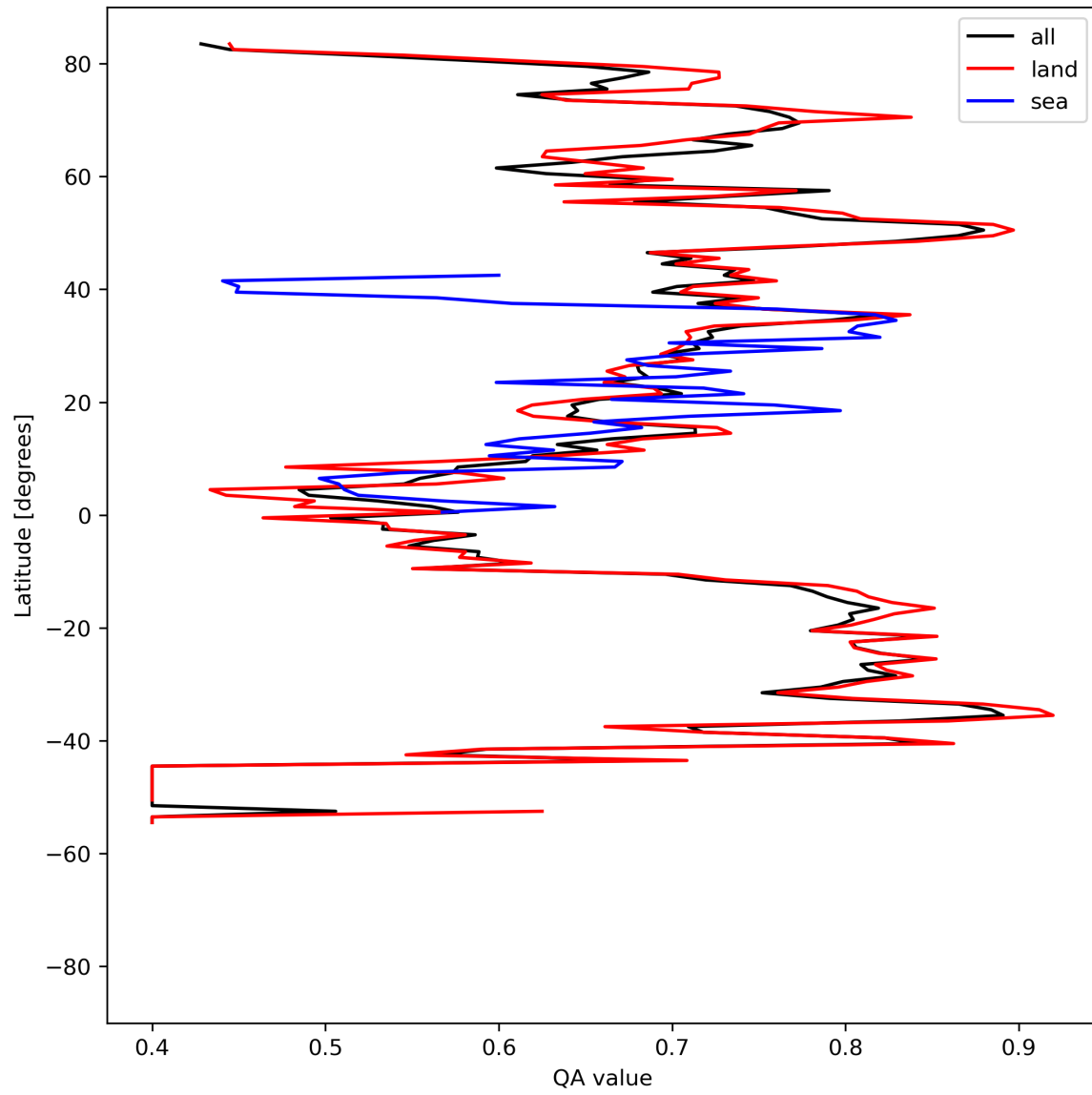
Figure 11: Zonal average of “QA value” for 2024-04-29 to 2024-05-01.
