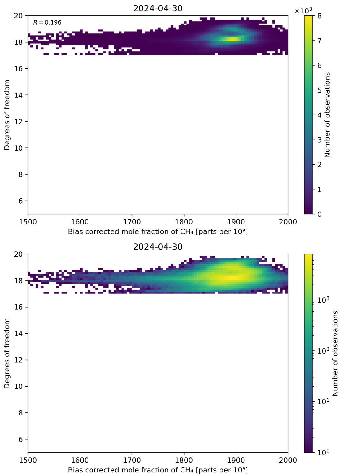
Figure 65: Scatter density plot of “Bias corrected mole fraction of CH 4 ” against “Degrees of freedom” for 2024-04-29 to 2024-05-01.
