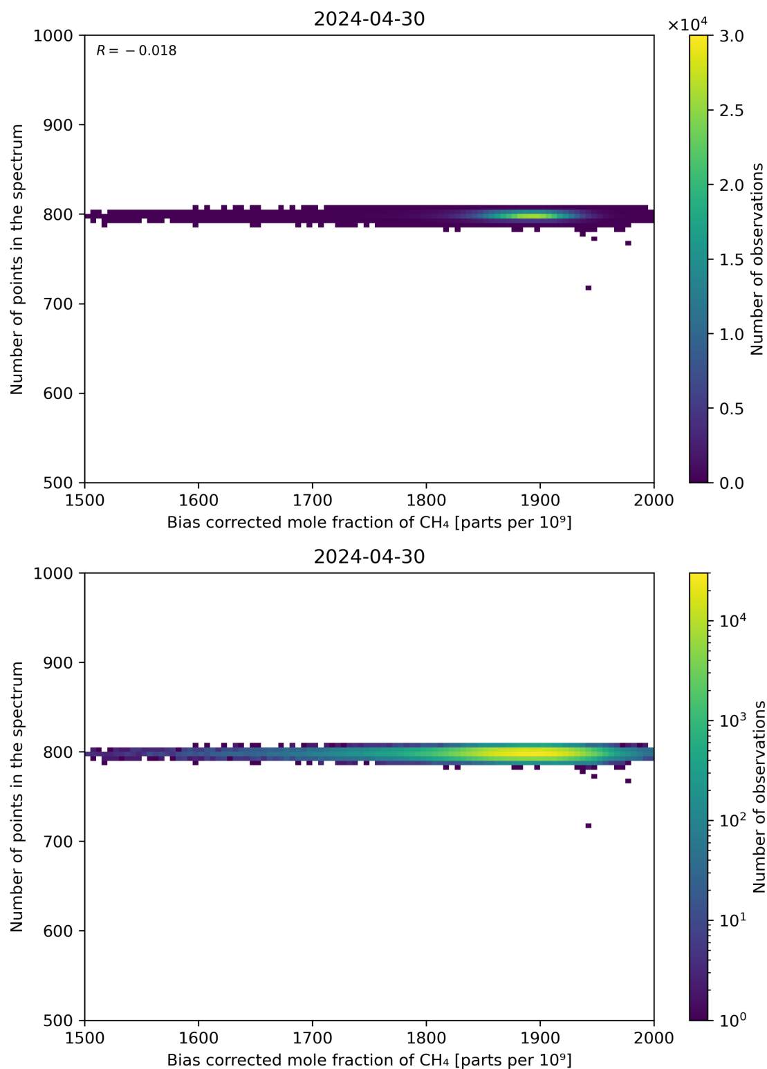
Figure 68: Scatter density plot of “Bias corrected mole fraction of CH 4 ” against “Number of points in the spectrum” for 2024-04-29 to 2024-05-01.
