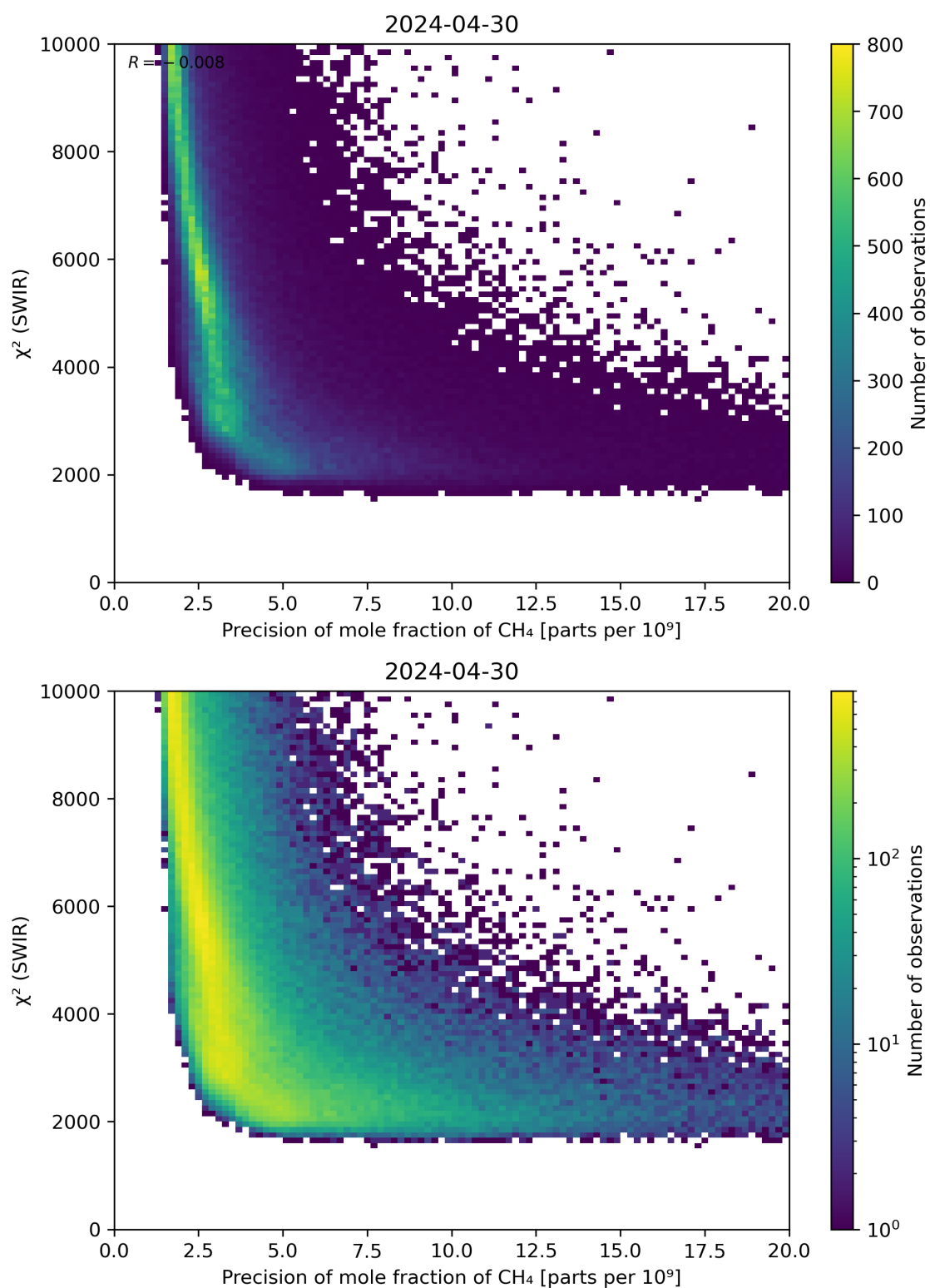
Figure 79: Scatter density plot of “Precision of mole fraction of CH 4 ” against “ \chi^2 (SWIR)” for 2024-04-29 to 2024-05-01.
