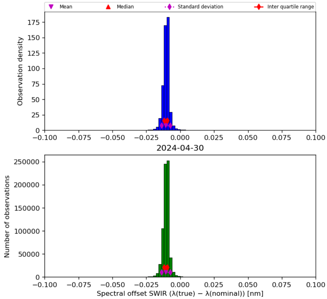
Figure 27: Histogram of “Spectral offset SWIR ( \lambda(\text{true}) - \lambda(\text{nominal}) )” for 2024-04-29 to 2024-05-01
