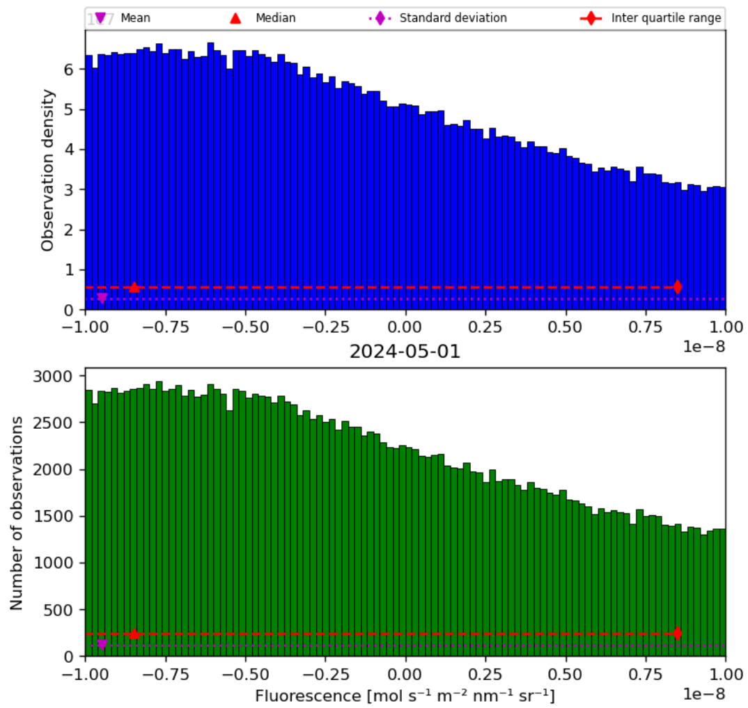
Figure 32: Histogram of “Fluorescence” for 2024-04-30 to 2024-05-02
