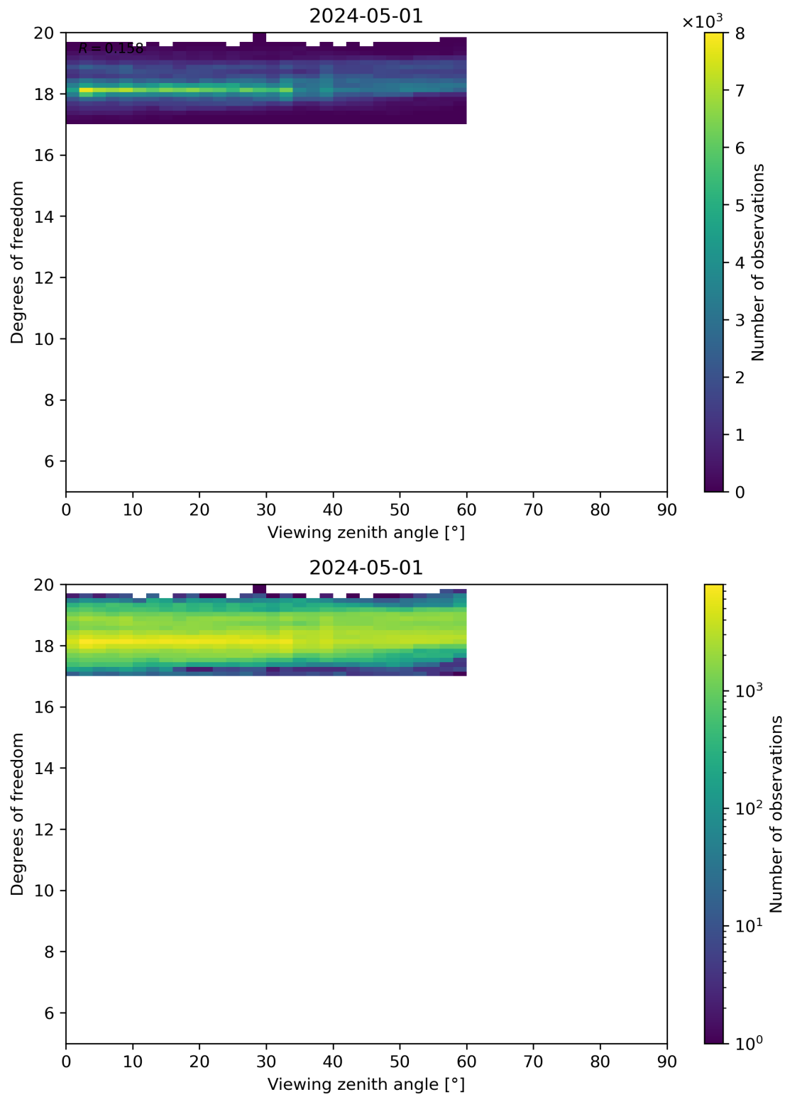
Figure 107: Scatter density plot of “Viewing zenith angle” against “Degrees of freedom” for 2024-04-30 to 2024-05-02.
