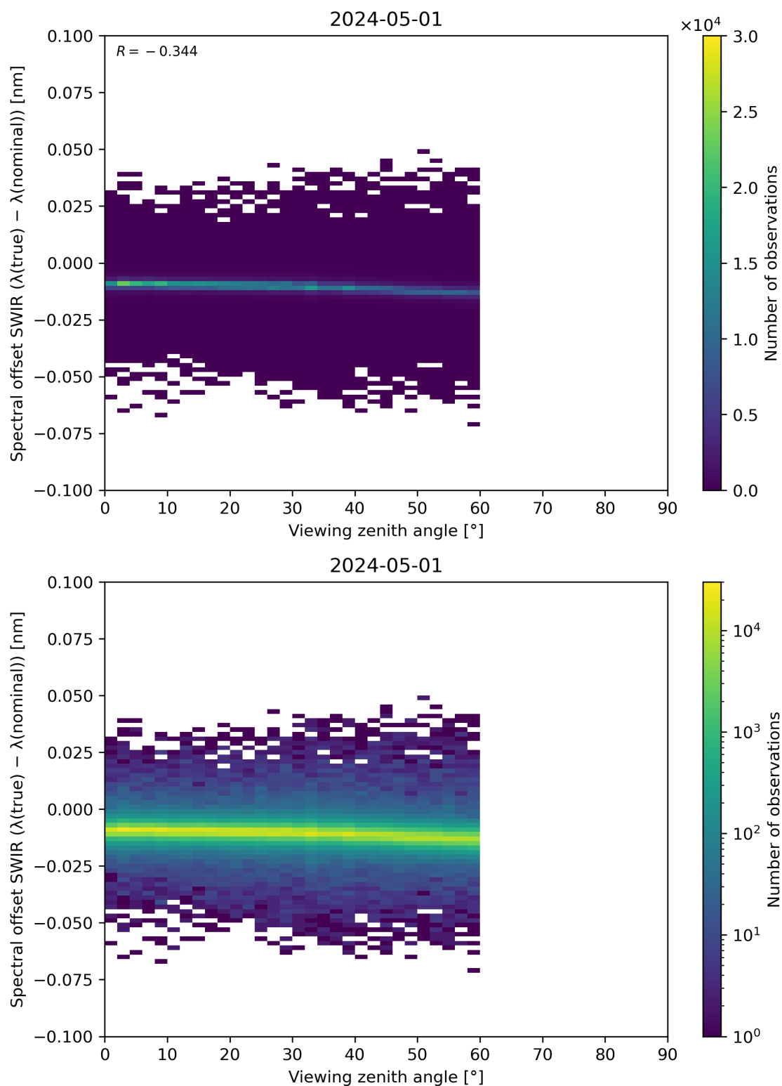
Figure 116: Scatter density plot of “Viewing zenith angle” against “Spectral offset SWIR ( \lambda(\text{true}) - \lambda(\text{nominal}) )” for 2024-04-30 to 2024-05-02.
