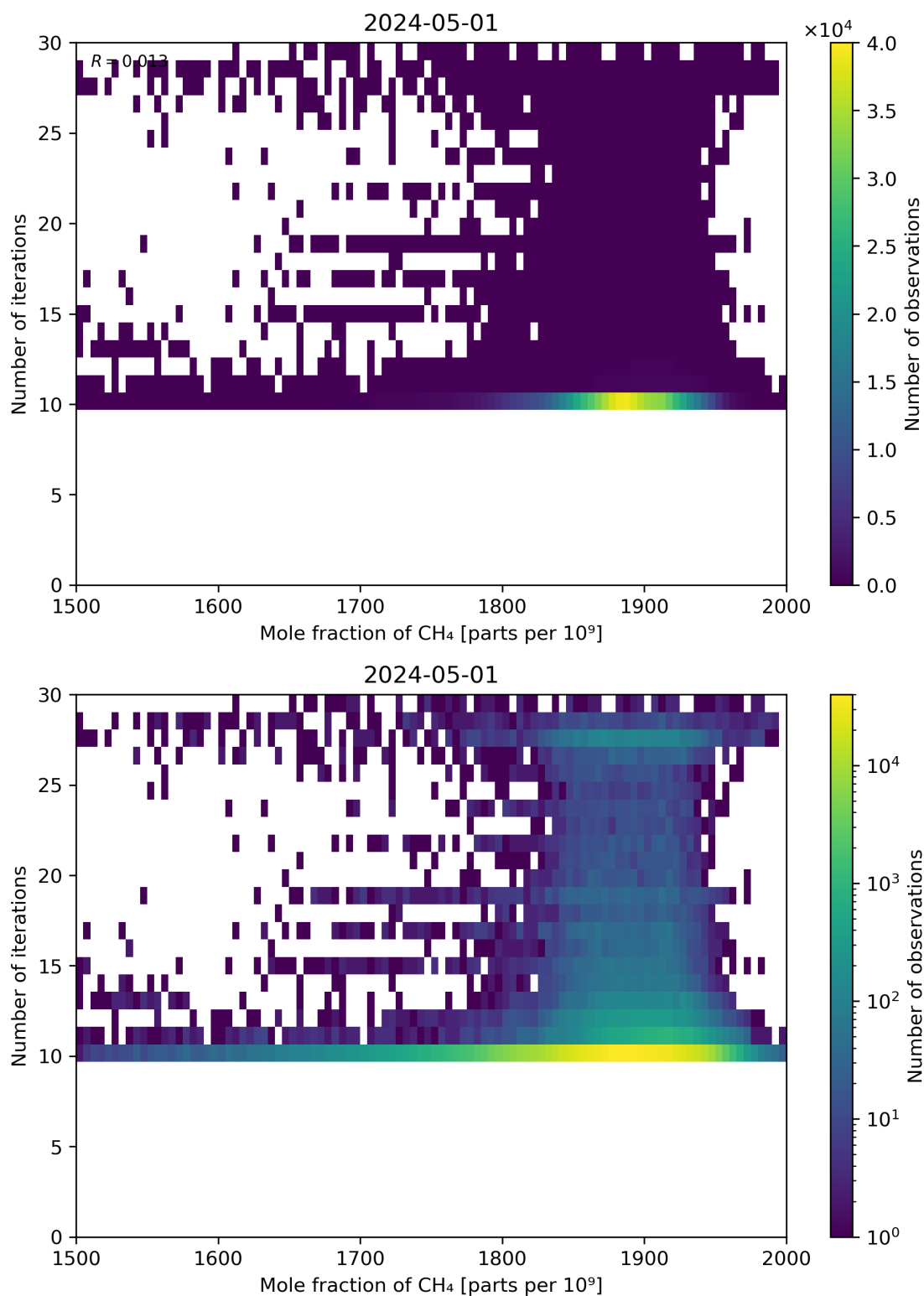
Figure 76: Scatter density plot of “Mole fraction of CH 4 ” against “Number of iterations” for 2024-04-30 to 2024-05-02.
