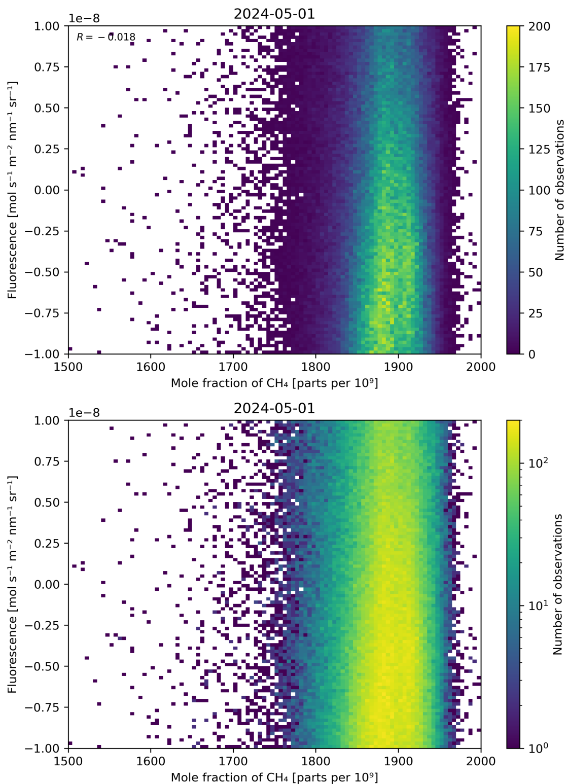
Figure 73: Scatter density plot of “Mole fraction of \text{CH}_4 ” against “Fluorescence” for 2024-04-30 to 2024-05-02.
