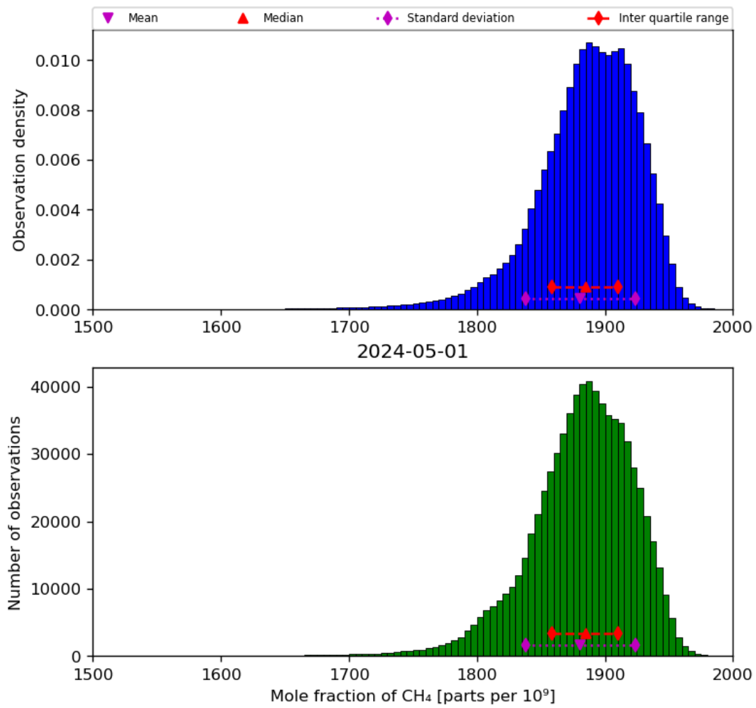
Figure 23: Histogram of “Mole fraction of CH 4 ” for 2024-04-30 to 2024-05-02
