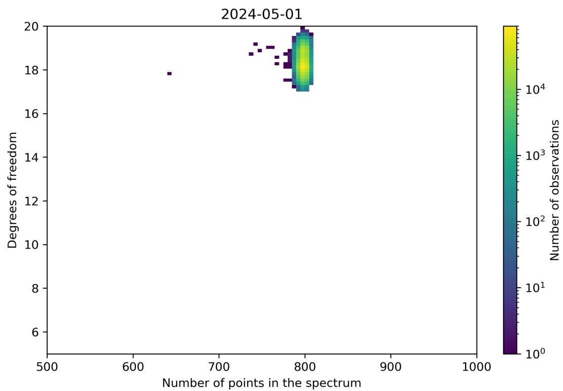
Figure 90: Scatter density plot of “Number of points in the spectrum” against “Degrees of freedom” for 2024-04-30 to 2024-05-02.
