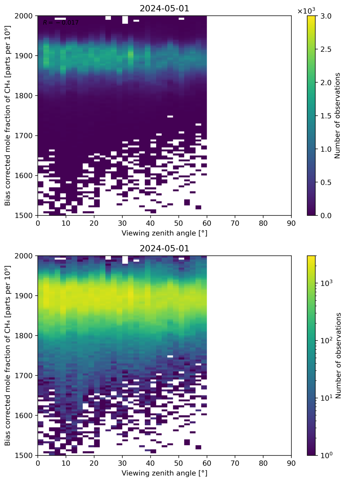
Figure 111: Scatter density plot of “Viewing zenith angle” against “Bias corrected mole fraction of CH 4 ” for 2024-04-30 to 2024-05-02.
