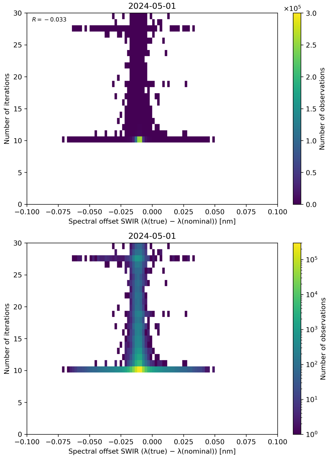
Figure 121: Scatter density plot of “Spectral offset SWIR ( \lambda(\text{true}) - \lambda(\text{nominal}) )” against “Number of iterations” for 2024-04-30 to 2024-05-02.
