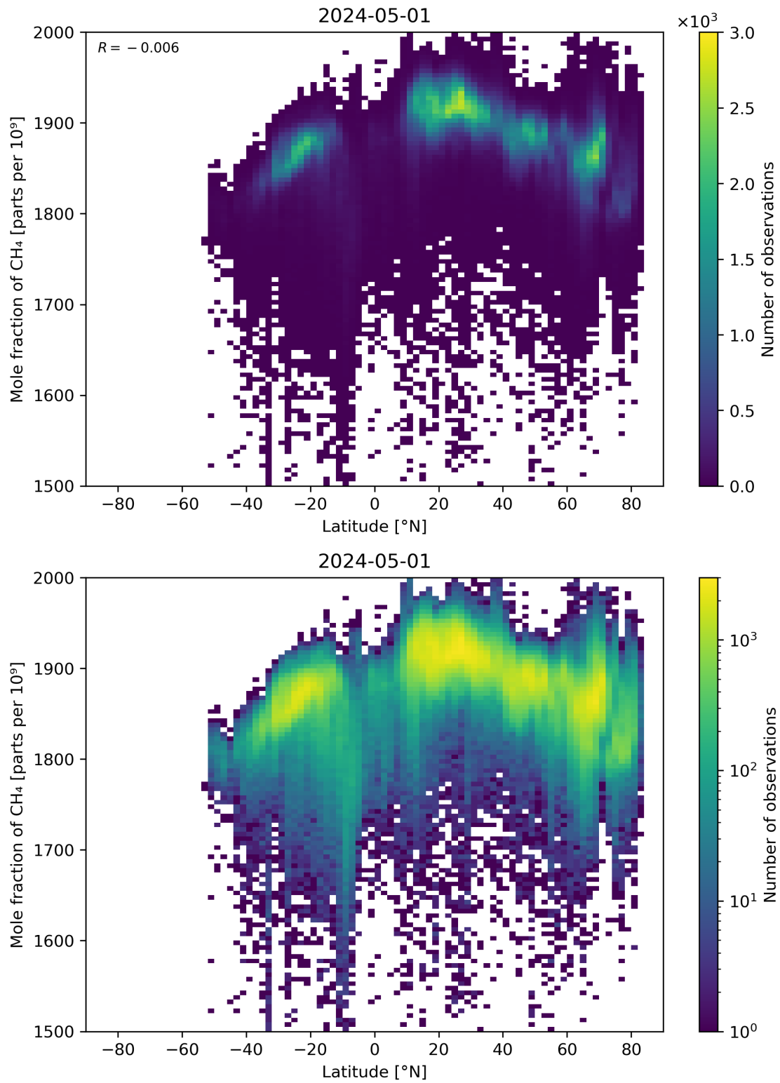
Figure 57: Scatter density plot of “Latitude” against “Mole fraction of CH 4 ” for 2024-04-30 to 2024-05-02.
