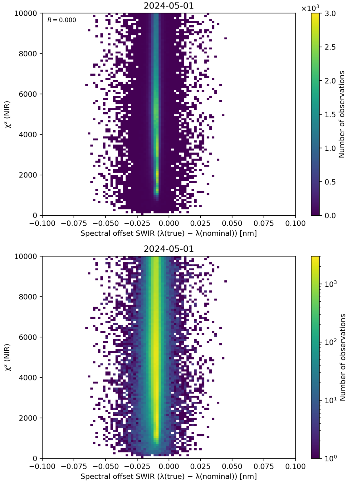
Figure 117: Scatter density plot of “Spectral offset SWIR ( \lambda(\text{true}) - \lambda(\text{nominal}) )” against “ \chi^2 (NIR)” for 2024-04-30 to 2024-05-02.
