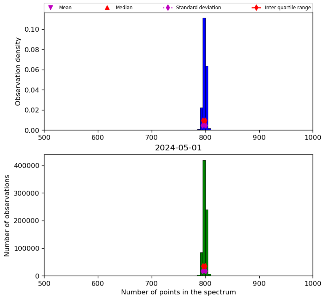
Figure 26: Histogram of “Number of points in the spectrum” for 2024-04-30 to 2024-05-02
