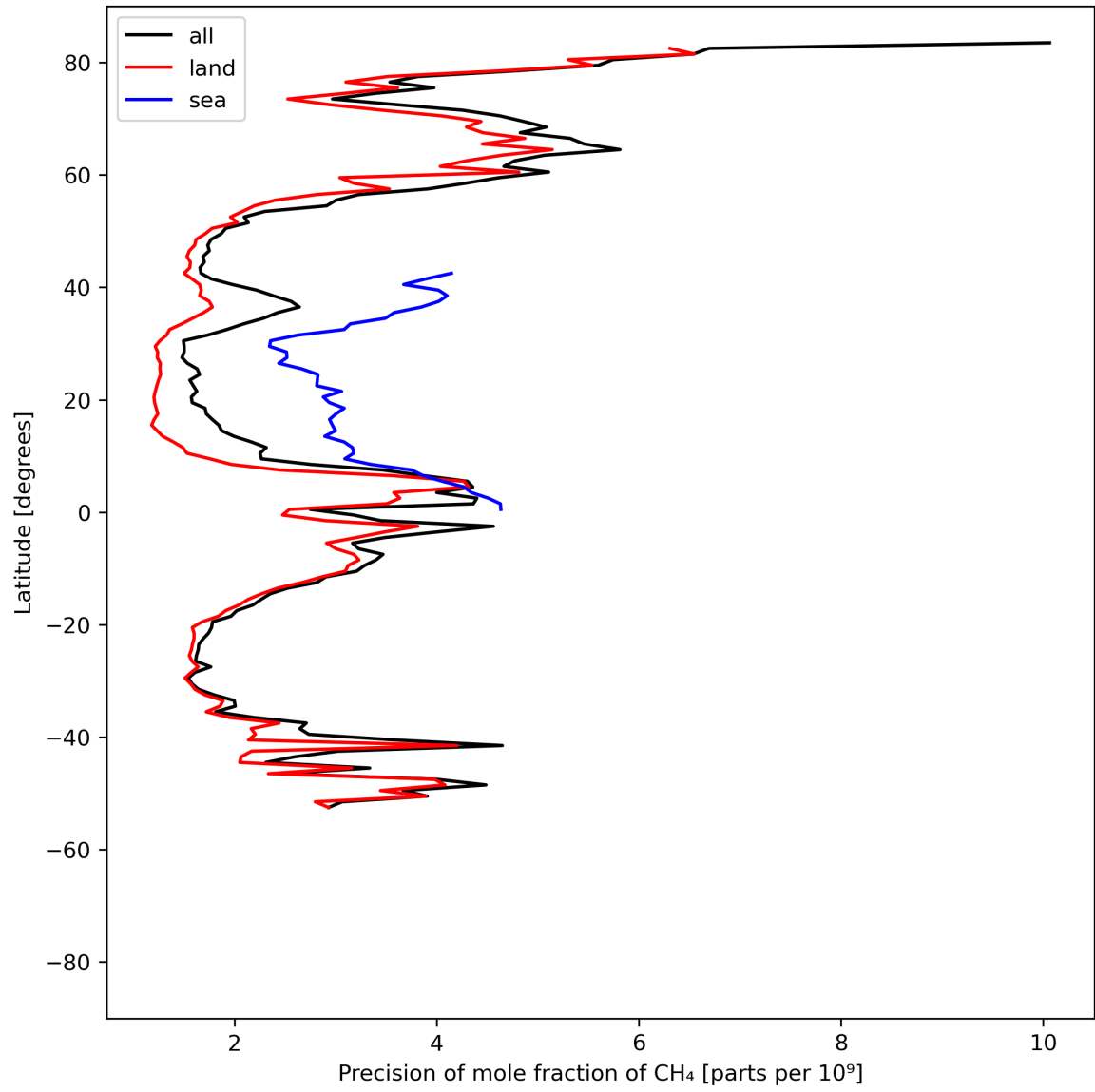
Figure 13: Zonal average of “Precision of mole fraction of CH 4 ” for 2024-04-30 to 2024-05-02.
