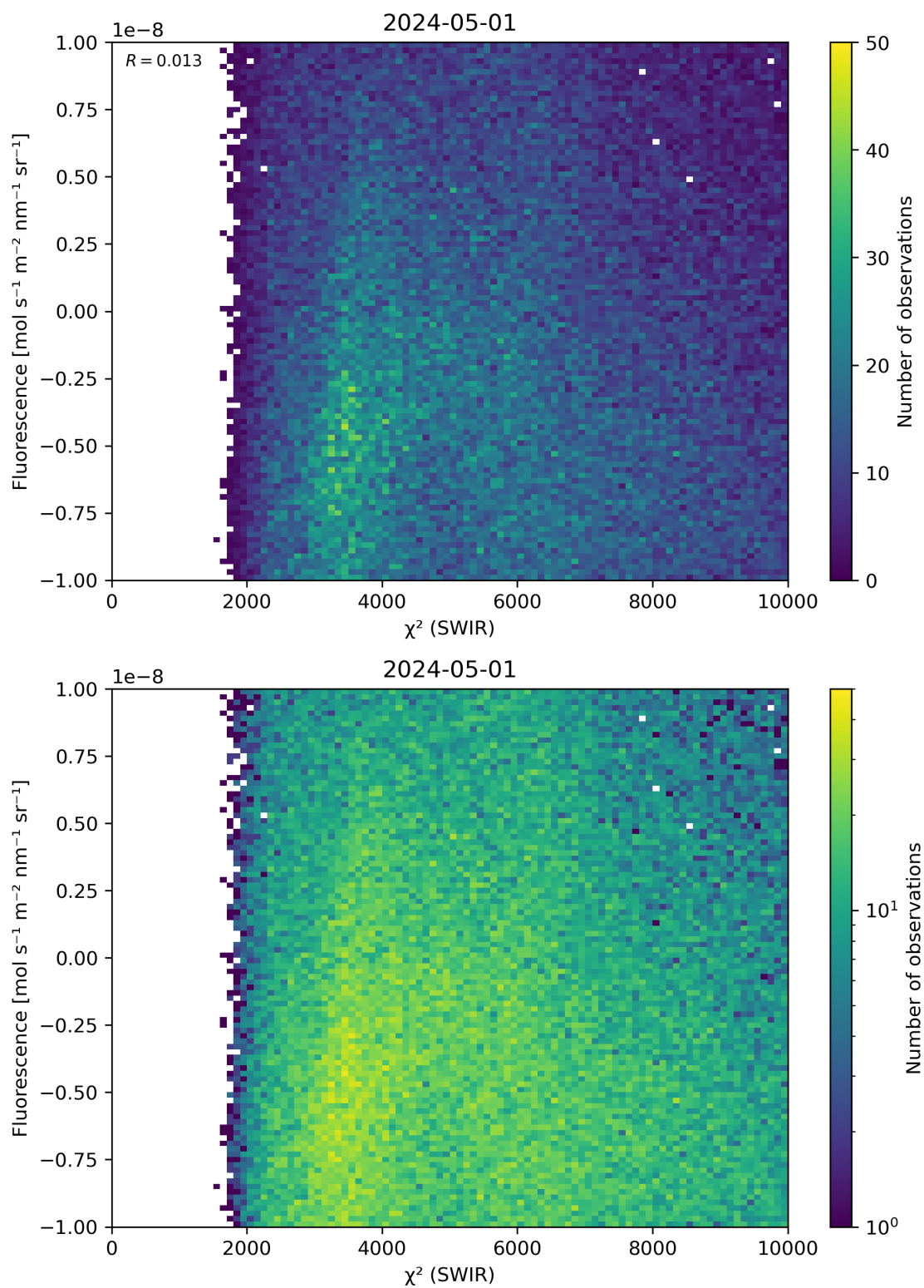
Figure 49: Scatter density plot of “ \chi^2 (SWIR)” against “Fluorescence” for 2024-04-30 to 2024-05-02.
