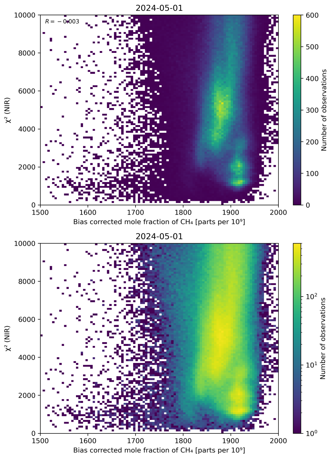
Figure 63: Scatter density plot of “Bias corrected mole fraction of CH 4 ” against “ \chi^2 (NIR)” for 2024-04-30 to 2024-05-02.
