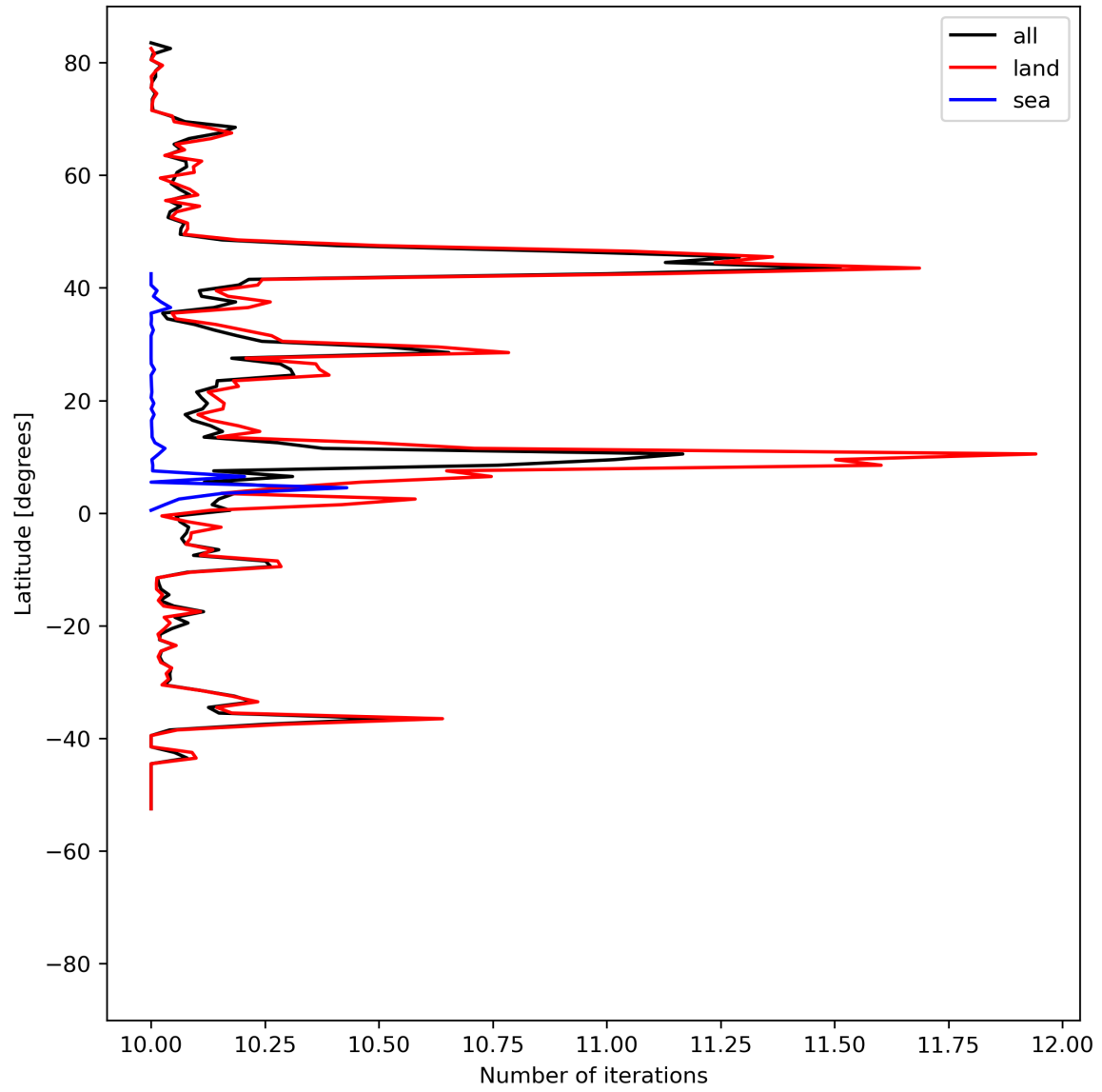
Figure 20: Zonal average of “Number of iterations” for 2024-04-30 to 2024-05-02.
