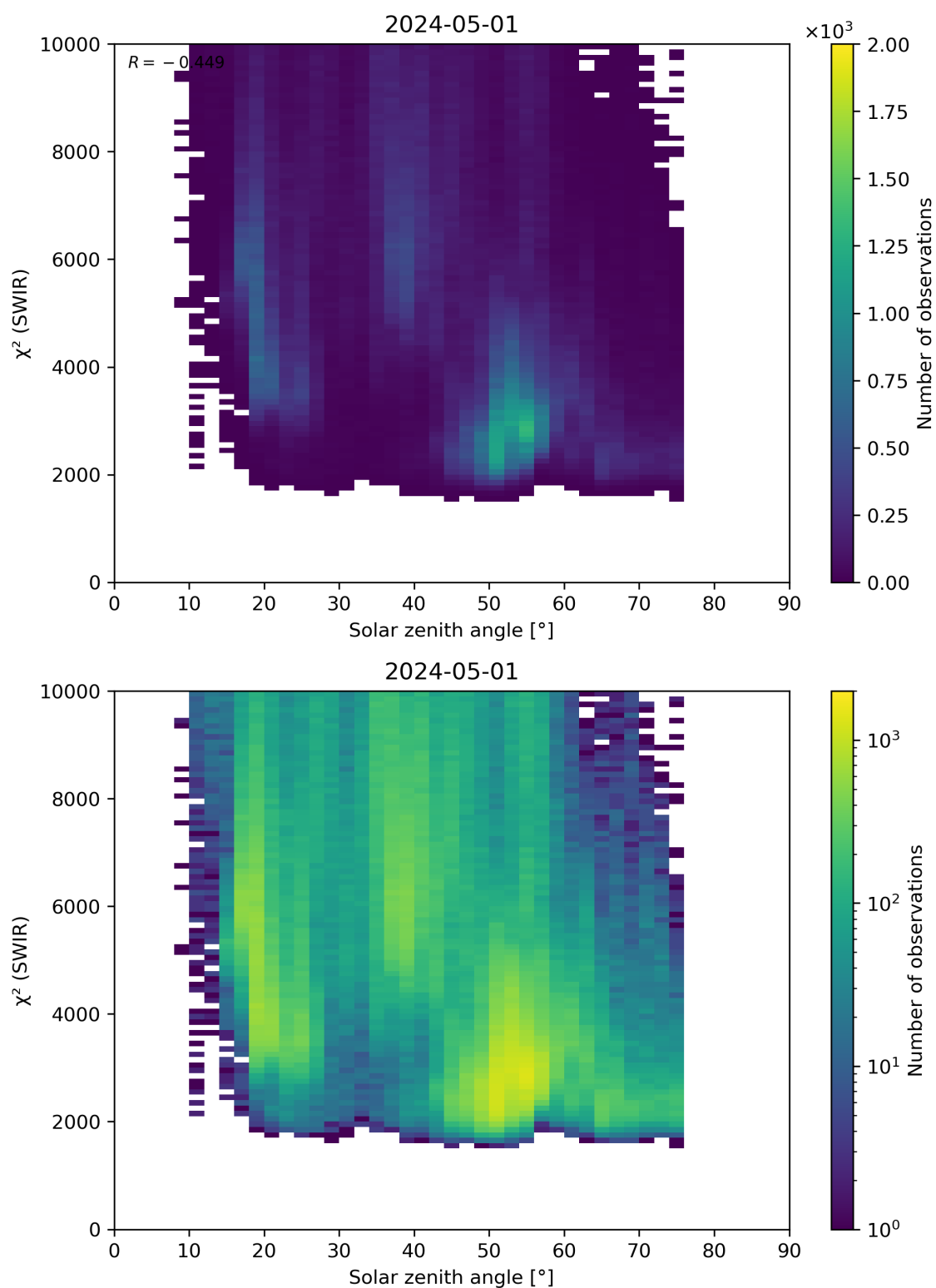
Figure 95: Scatter density plot of “Solar zenith angle” against “ \chi^2 (SWIR)” for 2024-04-30 to 2024-05-02.
