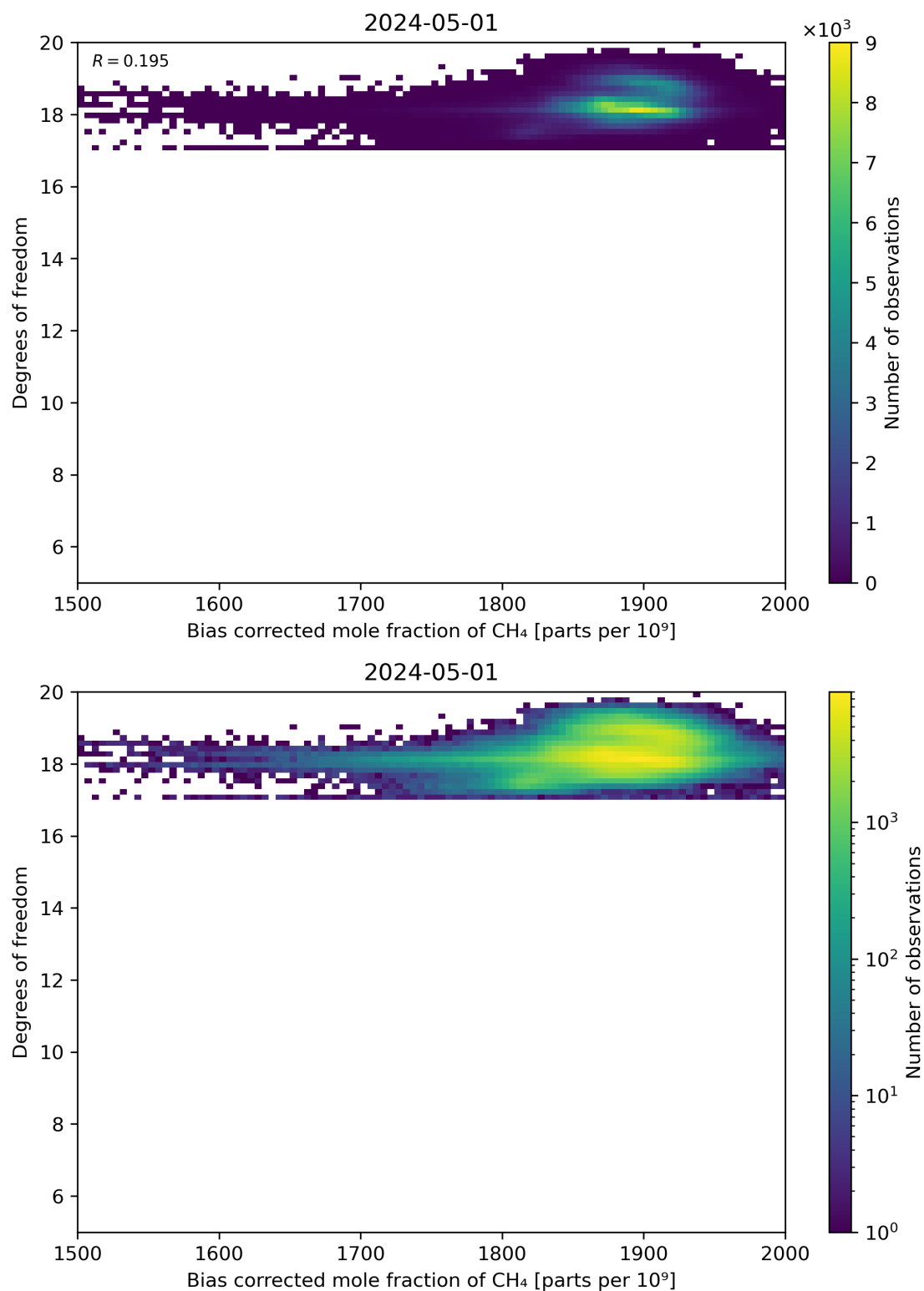
Figure 65: Scatter density plot of “Bias corrected mole fraction of CH 4 ” against “Degrees of freedom” for 2024-04-30 to 2024-05-02.
