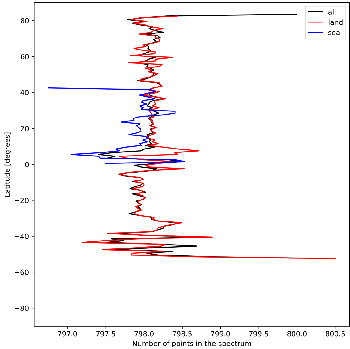
Figure 15: Zonal average of “Number of points in the spectrum” for 2024-04-30 to 2024-05-02.
