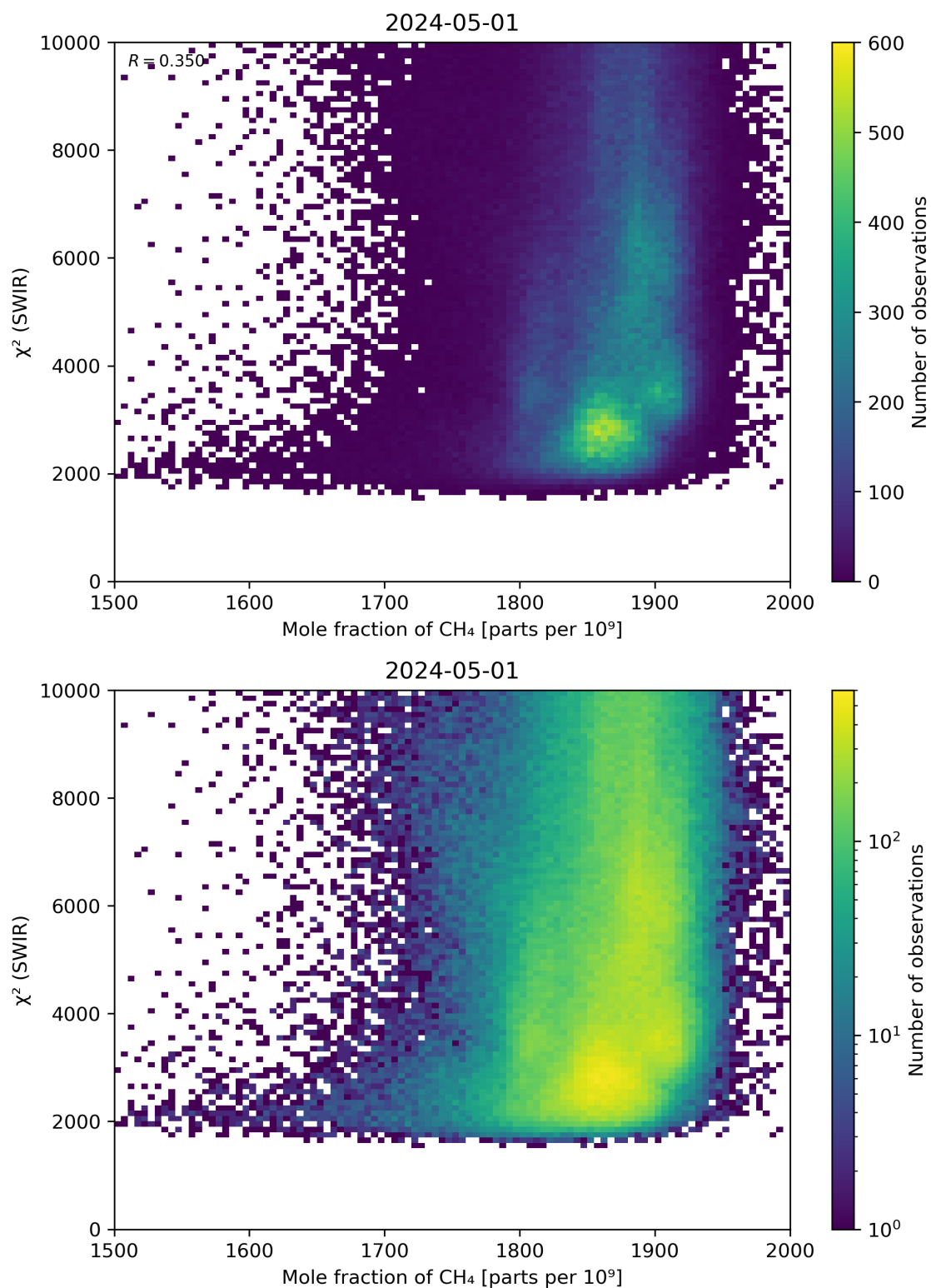
Figure 71: Scatter density plot of “Mole fraction of \text{CH}_4 ” against “ \chi^2 (SWIR)” for 2024-04-30 to 2024-05-02.
