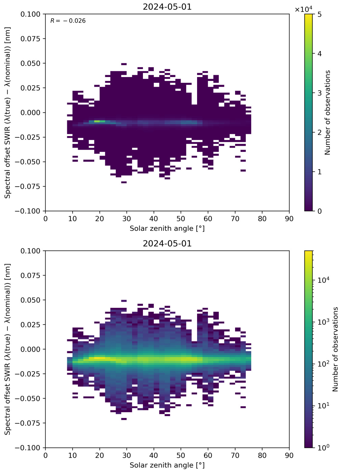
Figure 104: Scatter density plot of “Solar zenith angle” against “Spectral offset SWIR ( \lambda(\text{true}) - \lambda(\text{nominal}) )” for 2024-04-30 to 2024-05-02.
