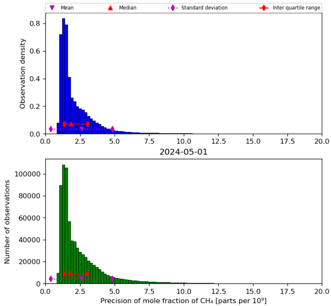
Figure 24: Histogram of “Precision of mole fraction of CH 4 ” for 2024-04-30 to 2024-05-02
