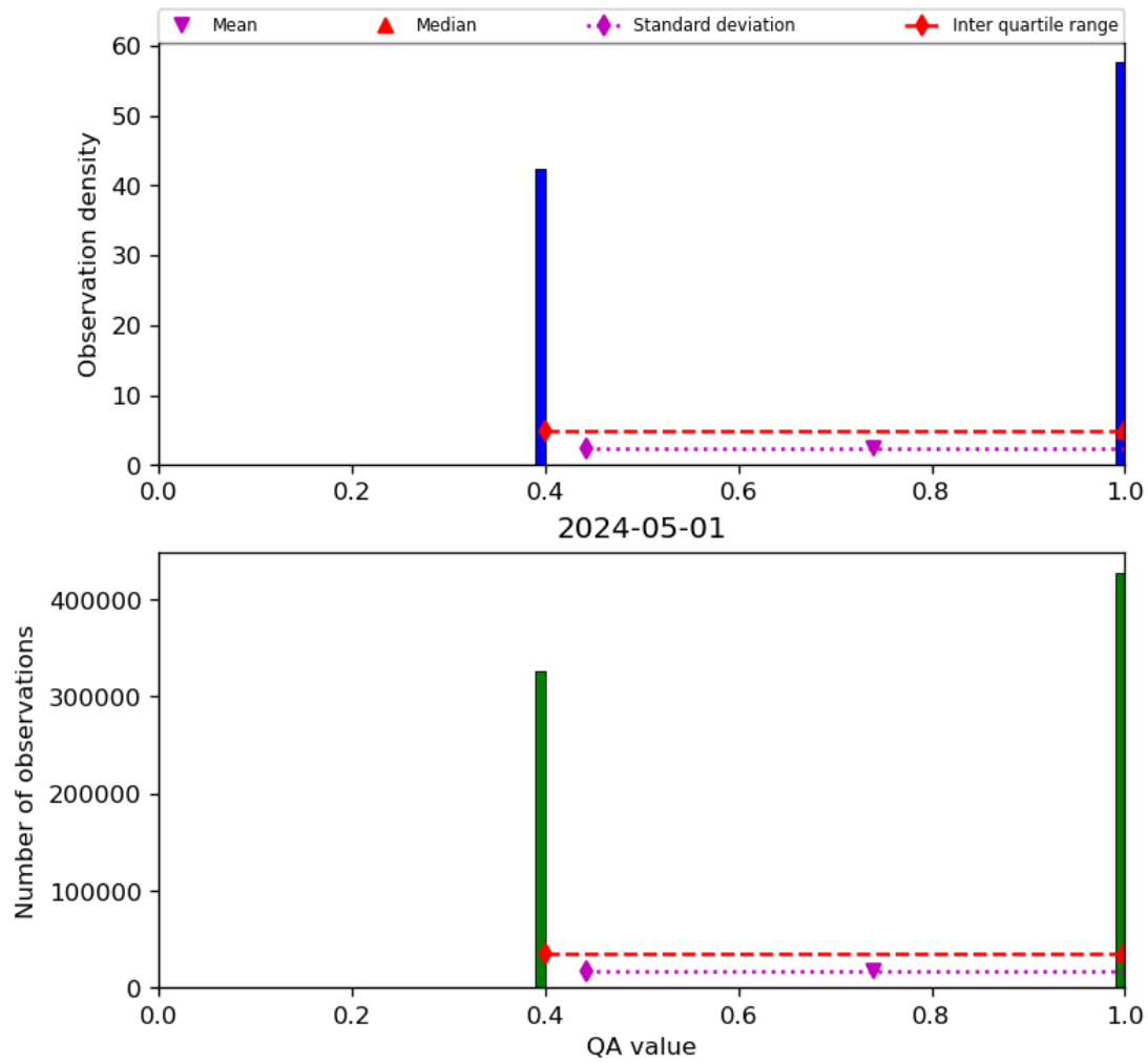
Figure 22: Histogram of “QA value” for 2024-04-30 to 2024-05-02
