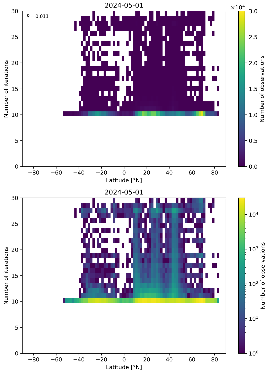
Figure 60: Scatter density plot of “Latitude” against “Number of iterations” for 2024-04-30 to 2024-05-02.
