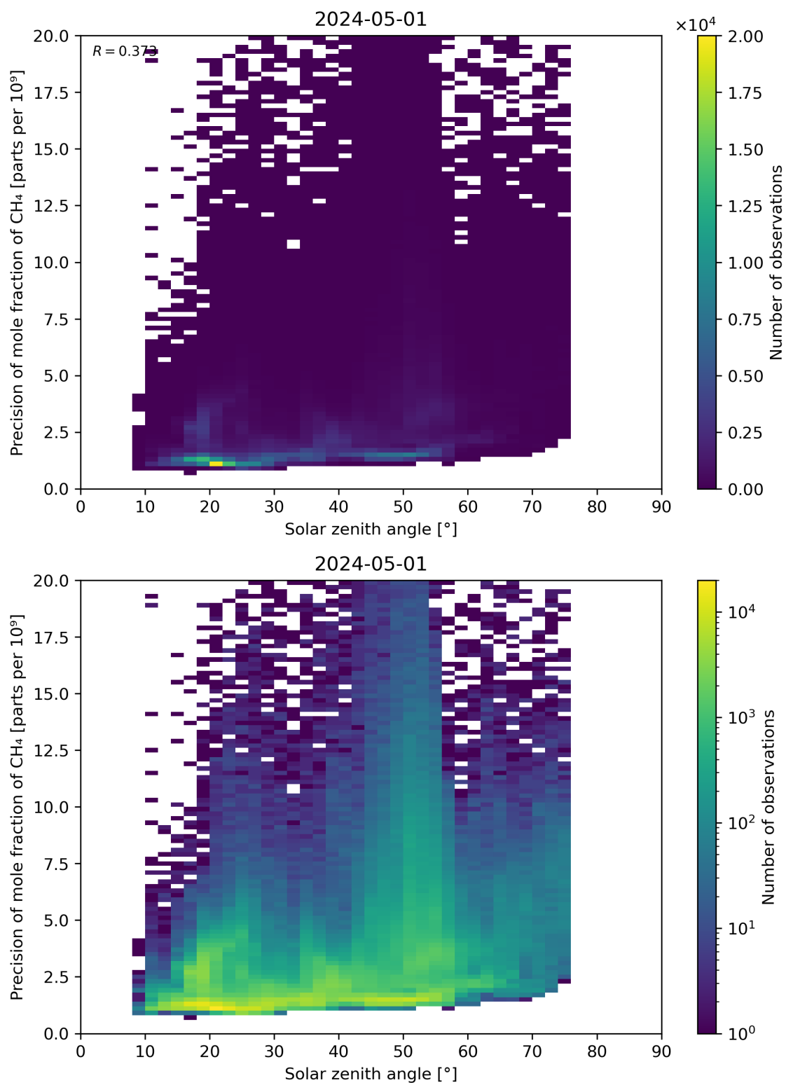
Figure 101: Scatter density plot of “Solar zenith angle” against “Precision of mole fraction of CH 4 ” for 2024-04-30 to 2024-05-02.
