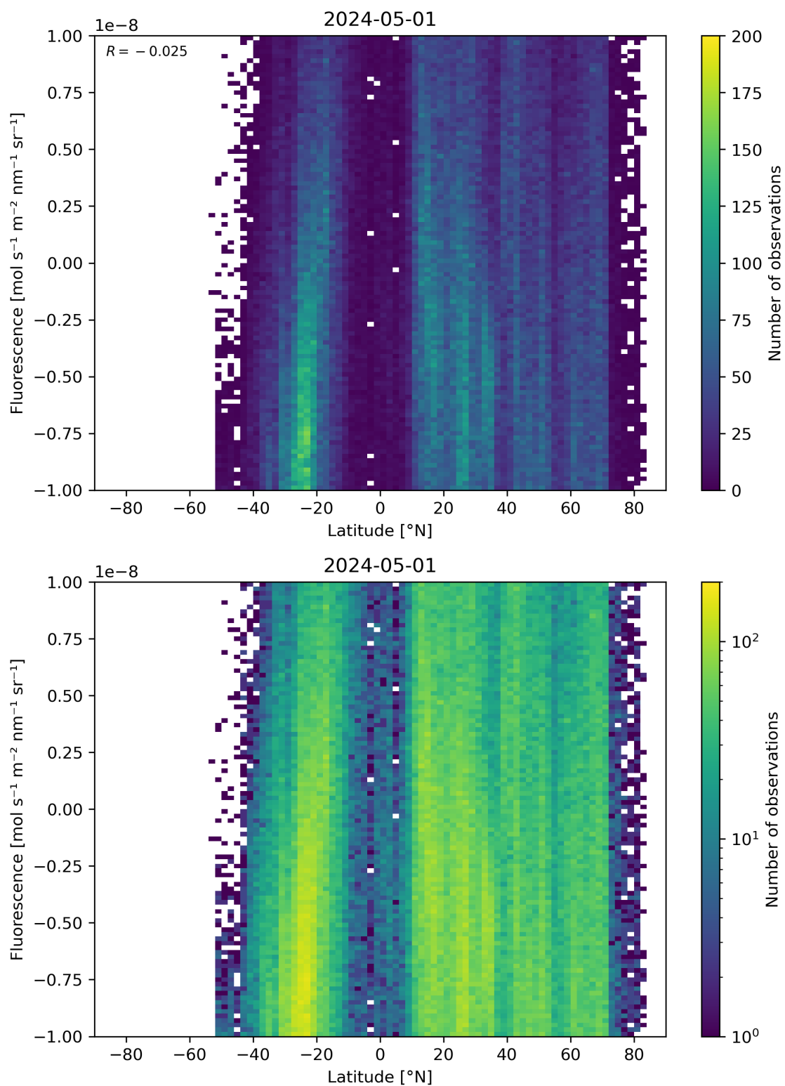
Figure 56: Scatter density plot of “Latitude” against “Fluorescence” for 2024-04-30 to 2024-05-02.
