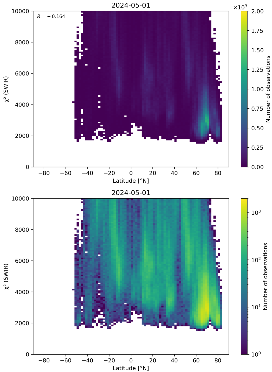
Figure 54: Scatter density plot of “Latitude” against “ \chi^2 (SWIR)” for 2024-04-30 to 2024-05-02.
