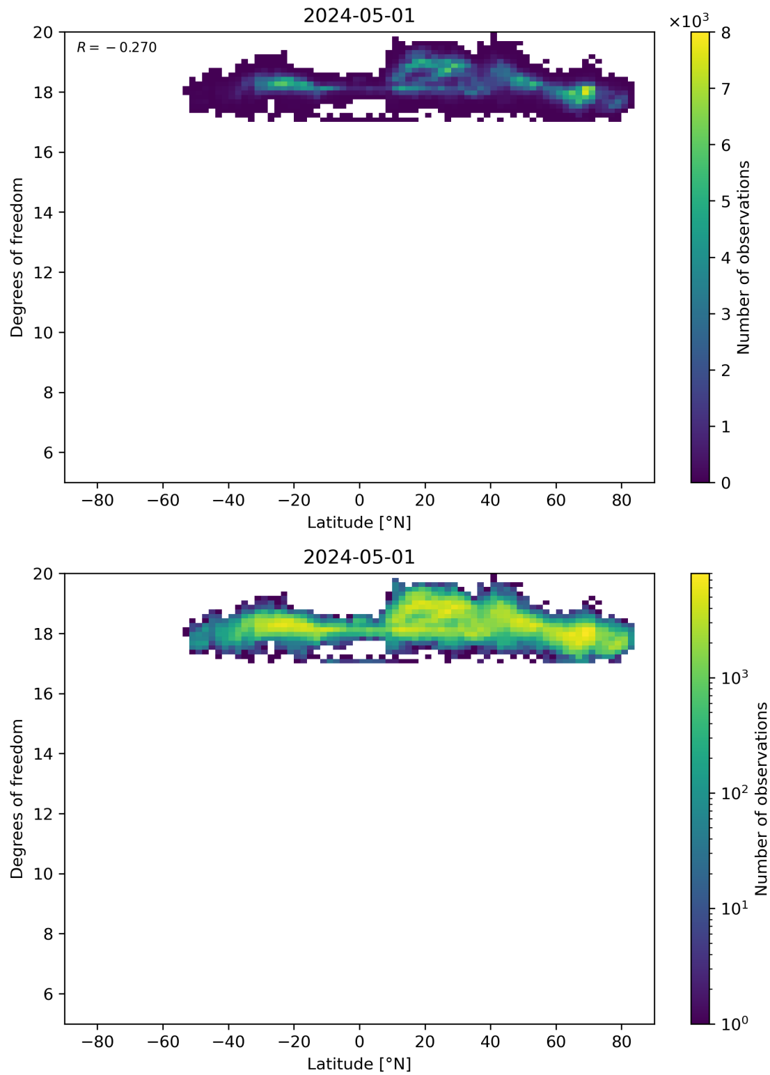
Figure 55: Scatter density plot of “Latitude” against “Degrees of freedom” for 2024-04-30 to 2024-05-02.
