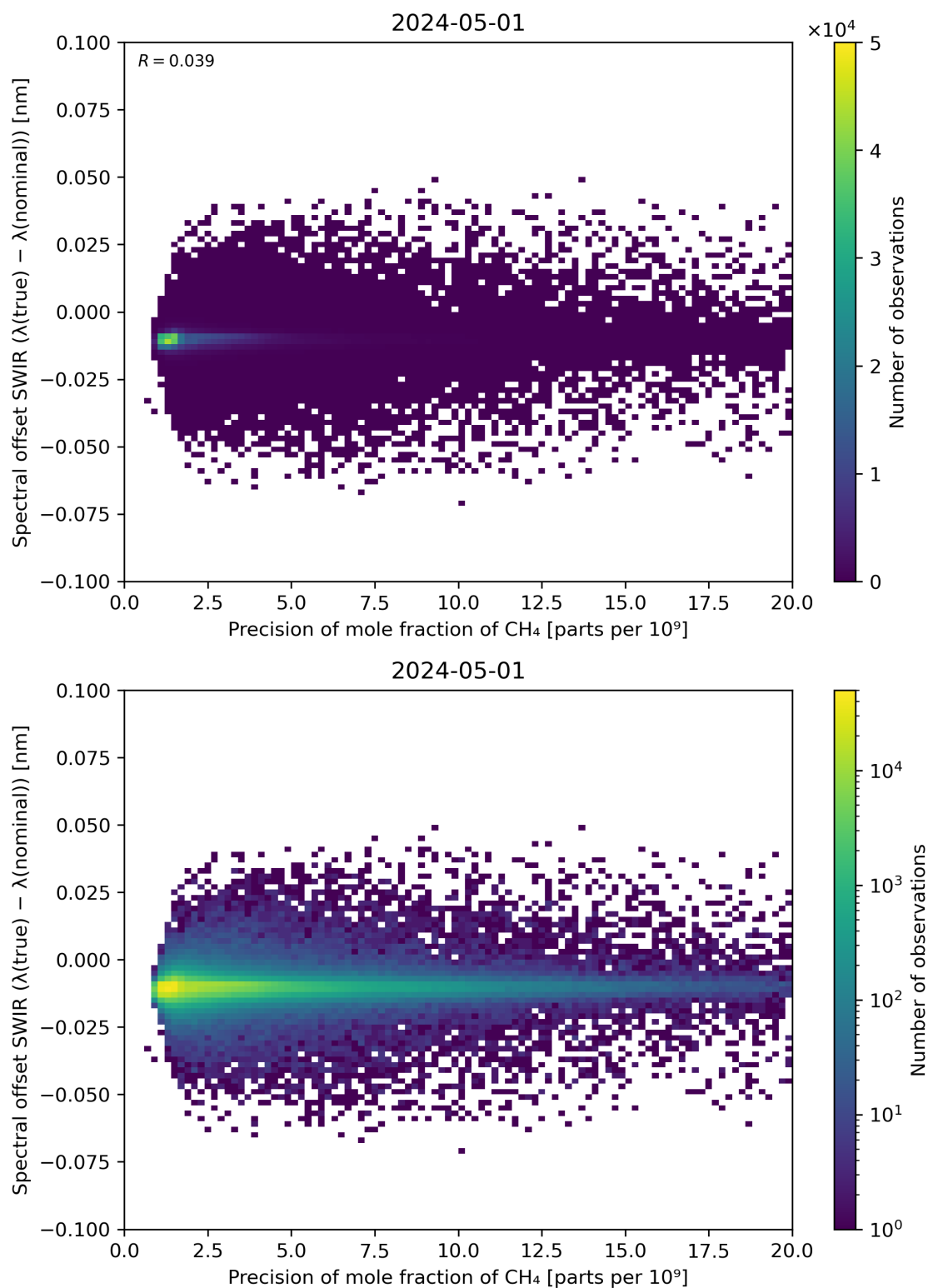
Figure 85: Scatter density plot of “Precision of mole fraction of CH 4 ” against “Spectral offset SWIR ( \lambda(\text{true}) - \lambda(\text{nominal}) )” for 2024-04-30 to 2024-05-02.
