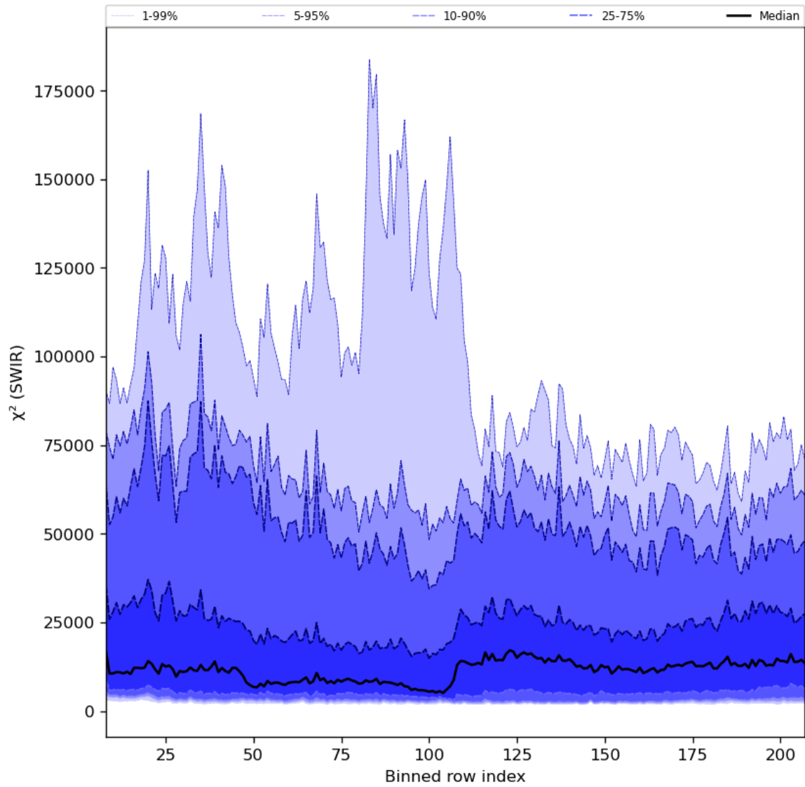
Figure 39: Along track statistics of " \chi^2 (SWIR)" for 2024-04-30 to 2024-05-02
