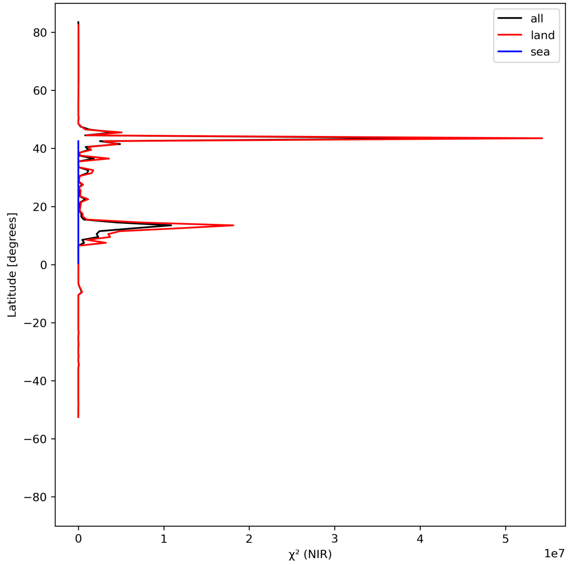
Figure 18: Zonal average of “ \chi^2 (NIR)” for 2024-04-30 to 2024-05-02.
