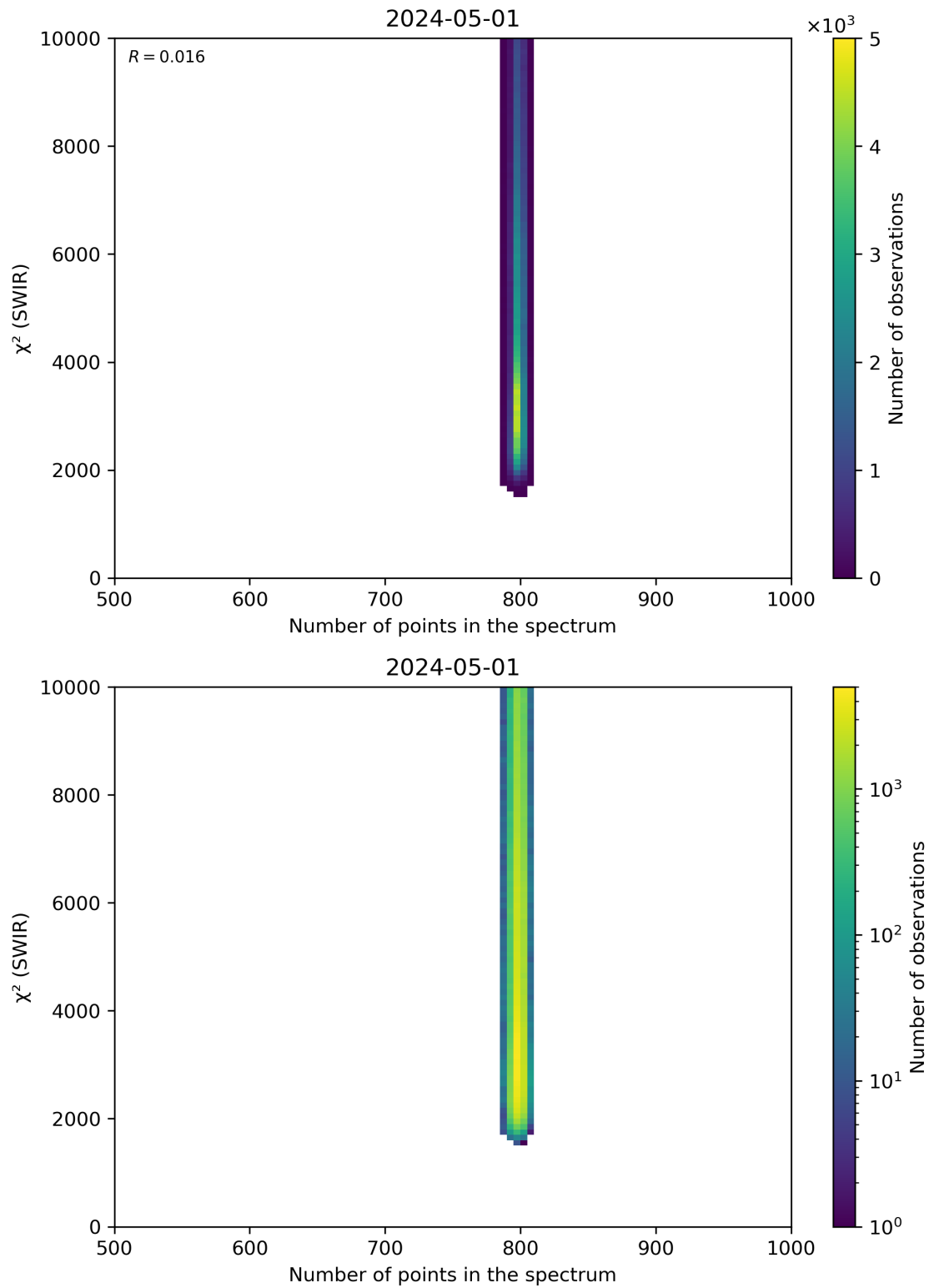
Figure 89: Scatter density plot of “Number of points in the spectrum” against “ \chi^2 (SWIR)” for 2024-04-30 to 2024-05-02.
