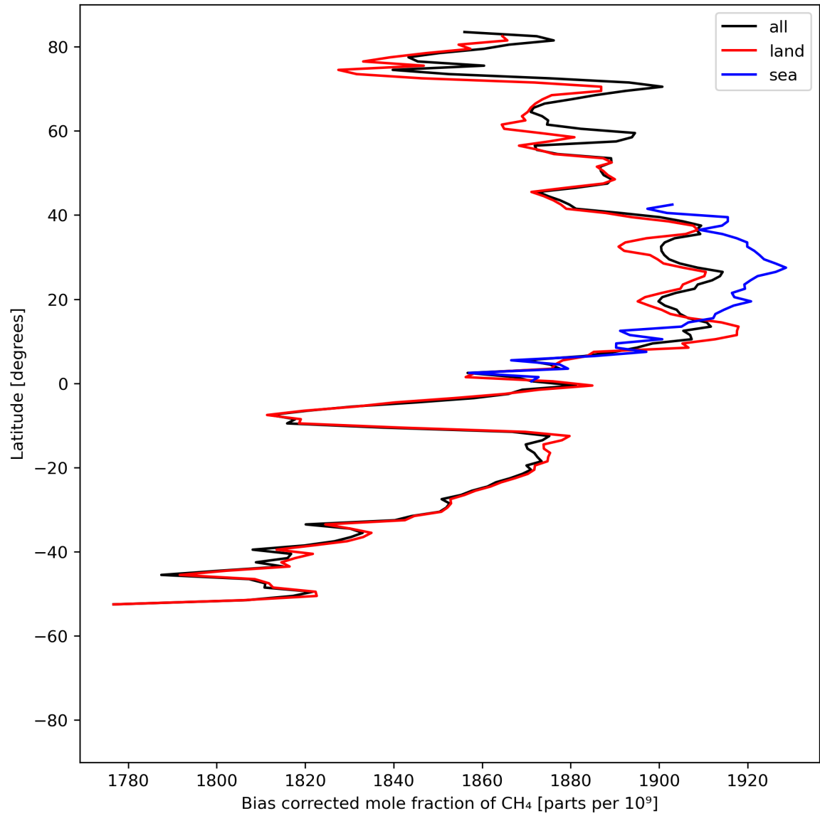
Figure 14: Zonal average of “Bias corrected mole fraction of \text{CH}_4 ” for 2024-04-30 to 2024-05-02.
