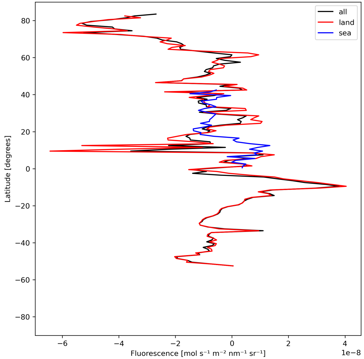
Figure 21: Zonal average of “Fluorescence” for 2024-04-30 to 2024-05-02.
