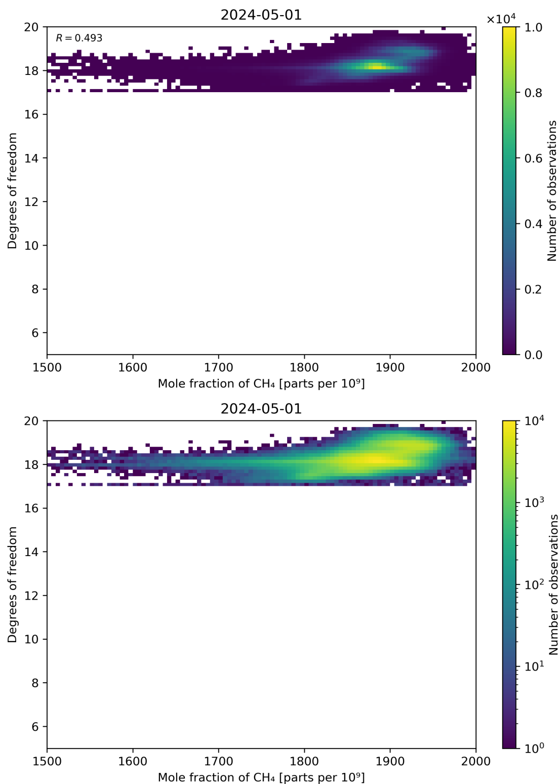
Figure 72: Scatter density plot of “Mole fraction of CH 4 ” against “Degrees of freedom” for 2024-04-30 to 2024-05-02.
