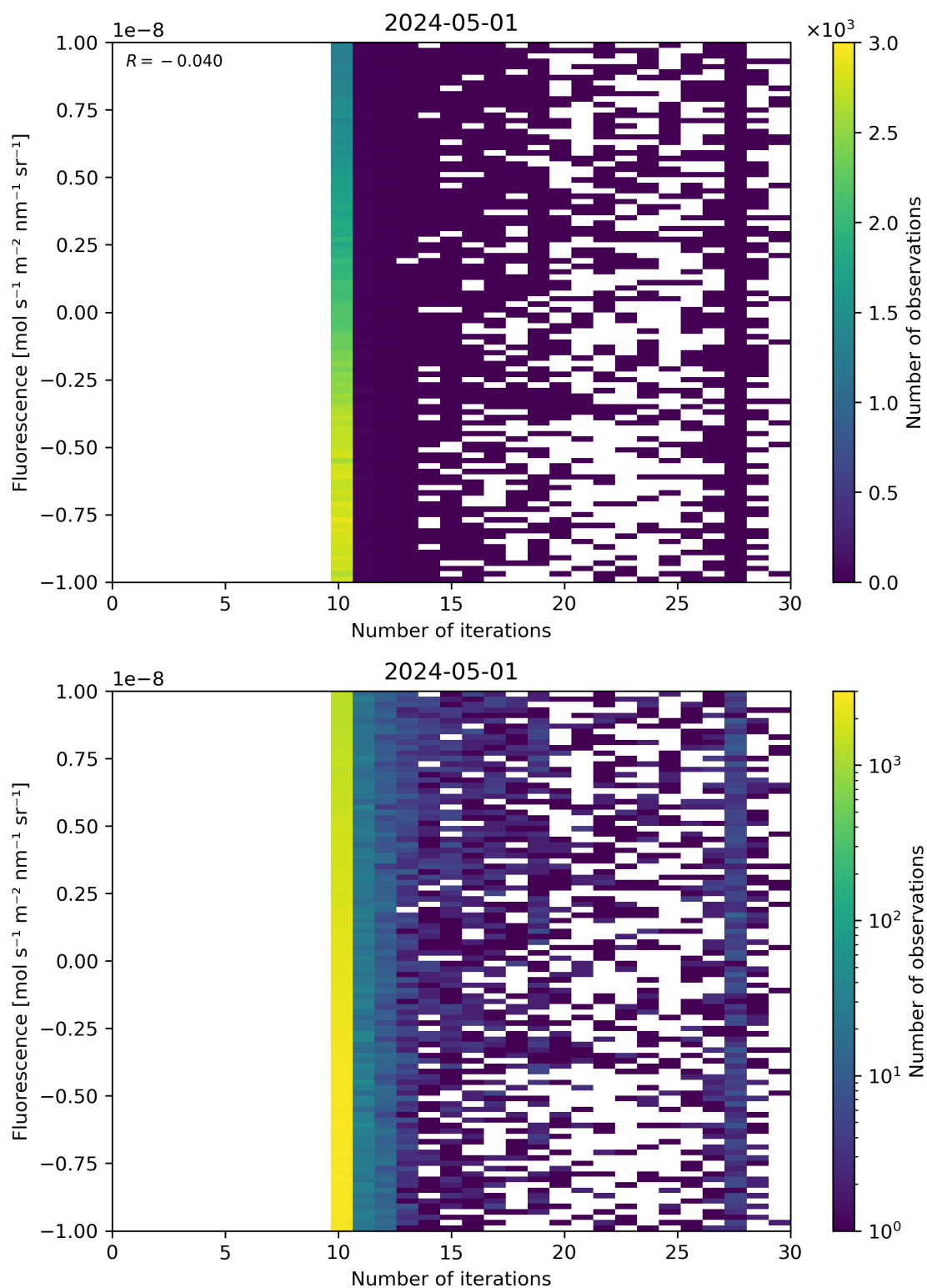
Figure 87: Scatter density plot of “Number of iterations” against “Fluorescence” for 2024-04-30 to 2024-05-02.
