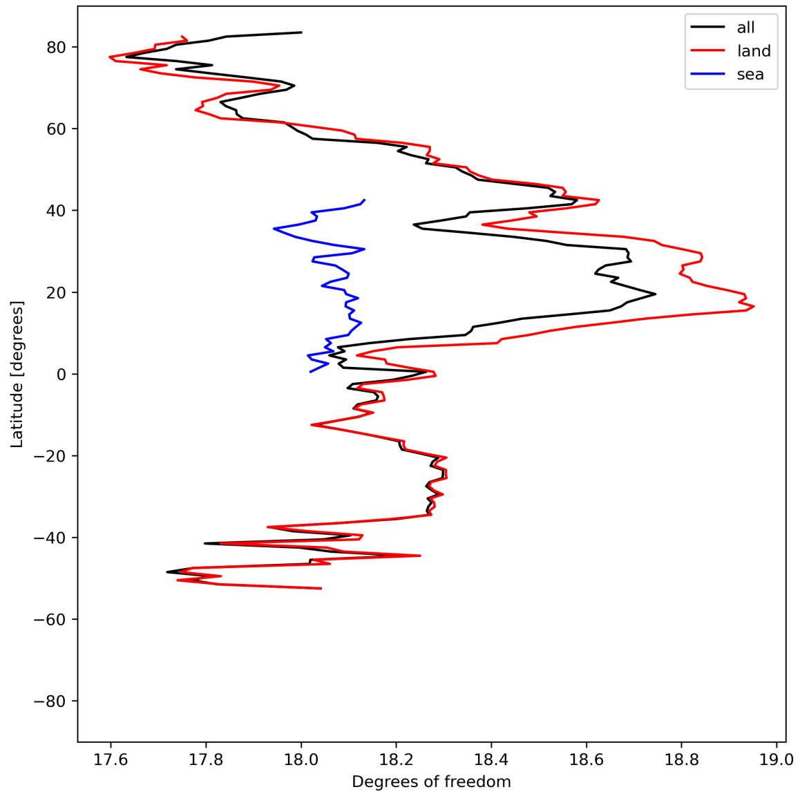
Figure 19: Zonal average of “Degrees of freedom” for 2024-04-30 to 2024-05-02.
