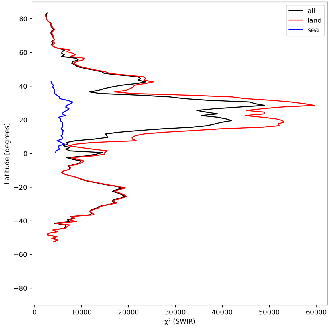
Figure 17: Zonal average of “ \chi^2 (SWIR)” for 2024-04-30 to 2024-05-02.
