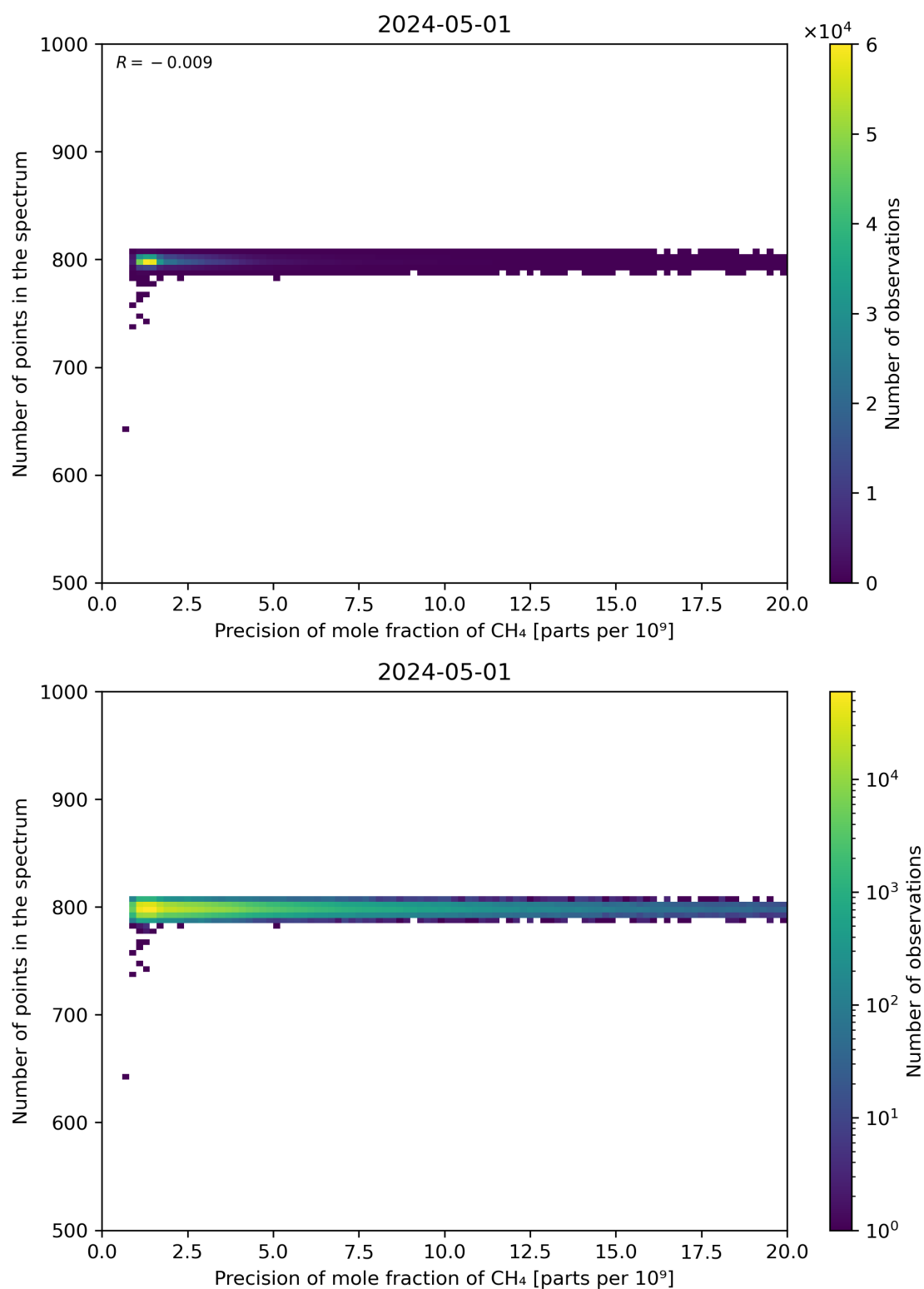
Figure 84: Scatter density plot of “Precision of mole fraction of CH 4 ” against “Number of points in the spectrum” for 2024-04-30 to 2024-05-02.
