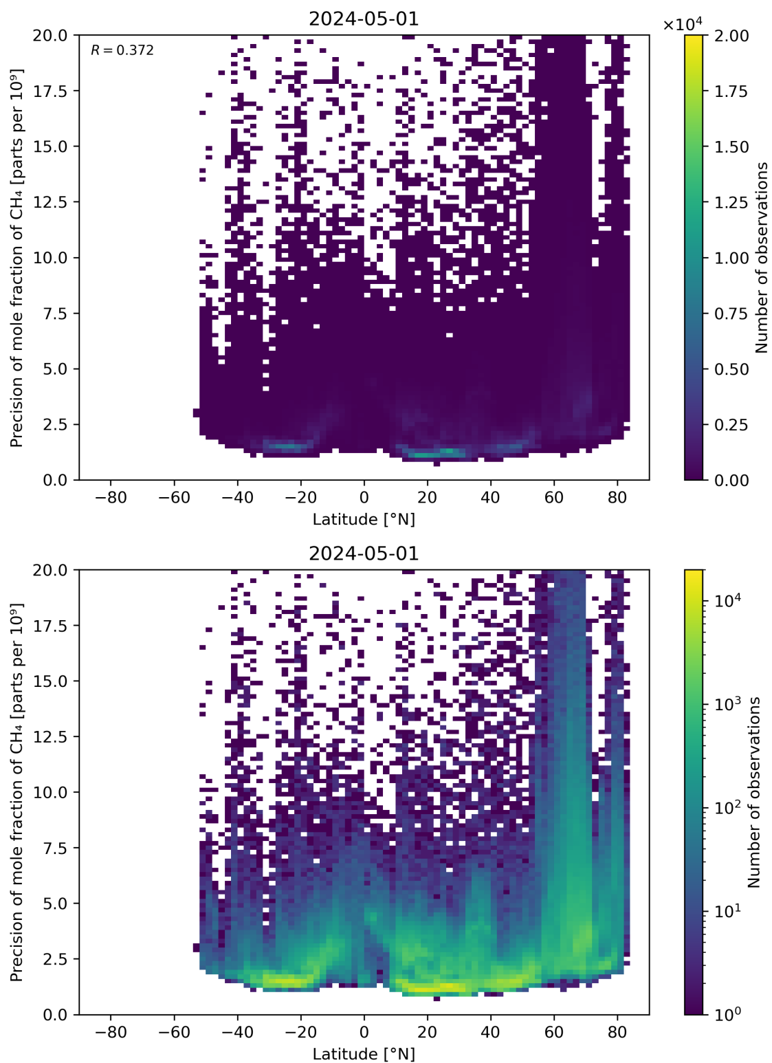
Figure 59: Scatter density plot of “Latitude” against “Precision of mole fraction of \text{CH}_4 ” for 2024-04-30 to 2024-05-02.
