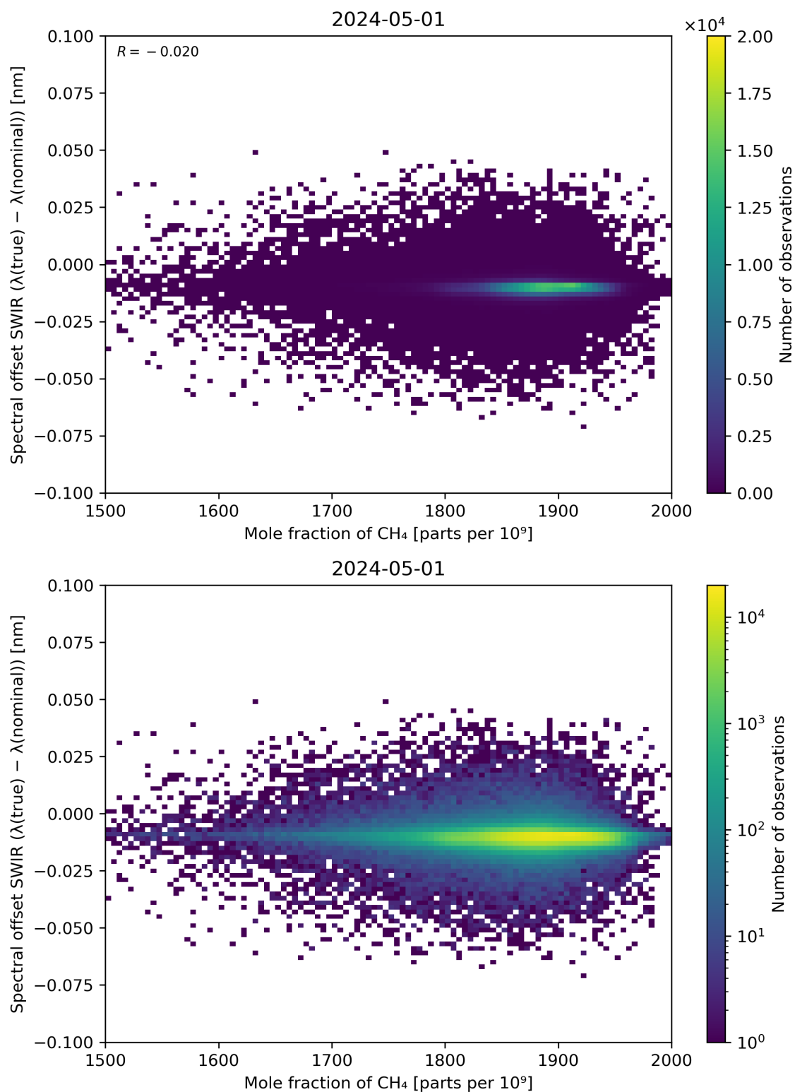
Figure 86: Scatter density plot of “Mole fraction of CH 4 ” against “Spectral offset SWIR ( \lambda(\text{true}) - \lambda(\text{nominal}) )” for 2024-04-30 to 2024-05-02.
