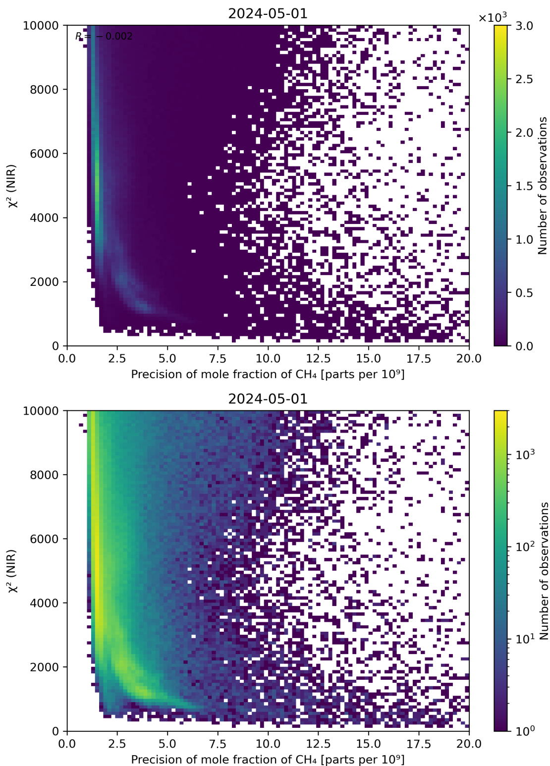
Figure 78: Scatter density plot of “Precision of mole fraction of CH 4 ” against “ \chi^2 (NIR)” for 2024-04-30 to 2024-05-02.
