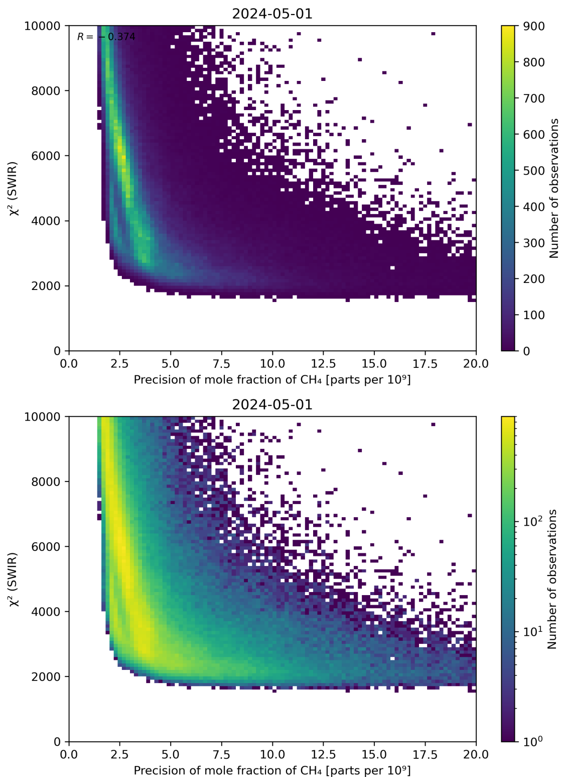
Figure 79: Scatter density plot of “Precision of mole fraction of CH 4 ” against “ \chi^2 (SWIR)” for 2024-04-30 to 2024-05-02.
