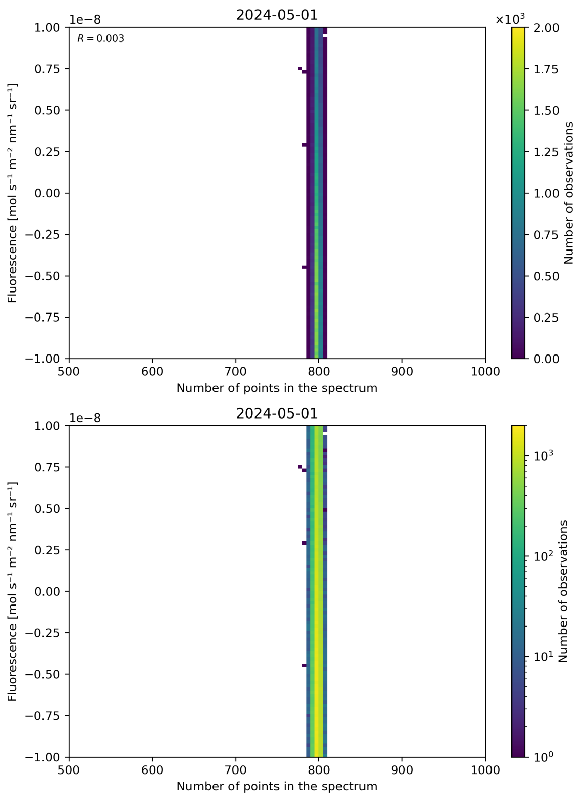
Figure 91: Scatter density plot of “Number of points in the spectrum” against “Fluorescence” for 2024-04-30 to 2024-05-02.
