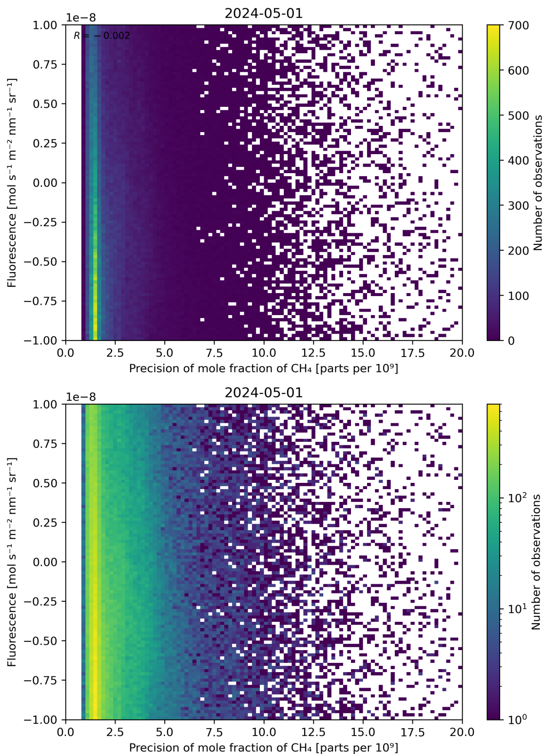
Figure 81: Scatter density plot of “Precision of mole fraction of \text{CH}_4 ” against “Fluorescence” for 2024-04-30 to 2024-05-02.
