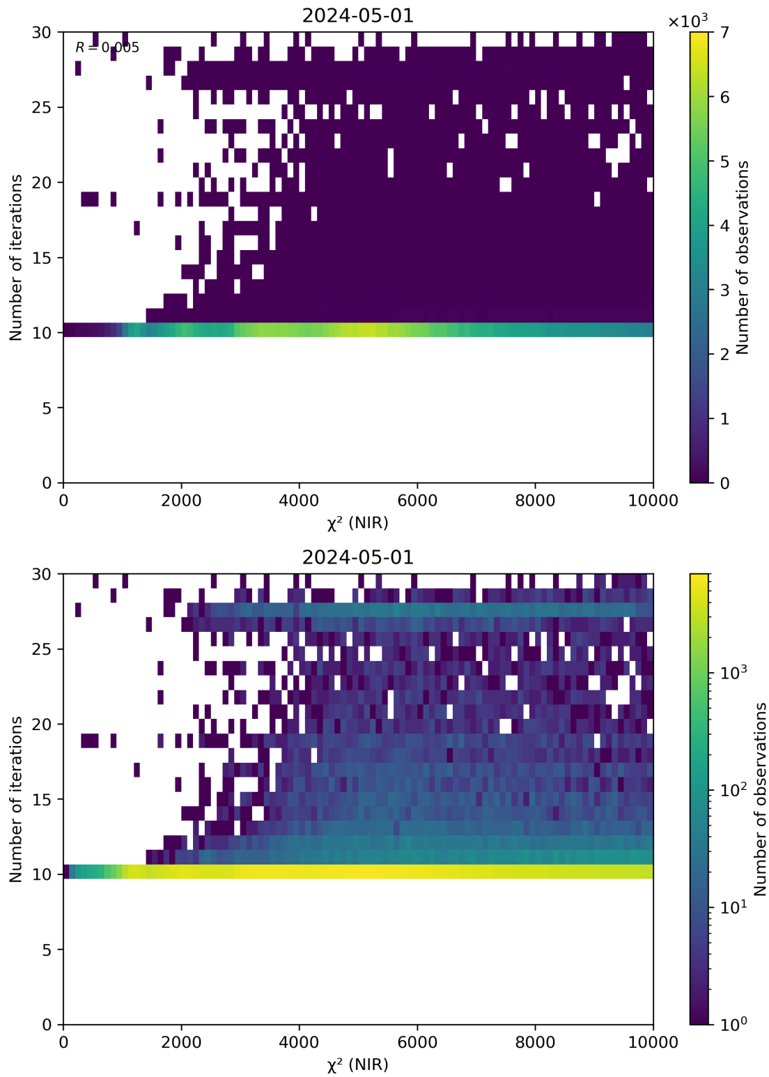
Figure 46: Scatter density plot of “ \chi^2 (NIR)” against “Number of iterations” for 2024-04-30 to 2024-05-02.
