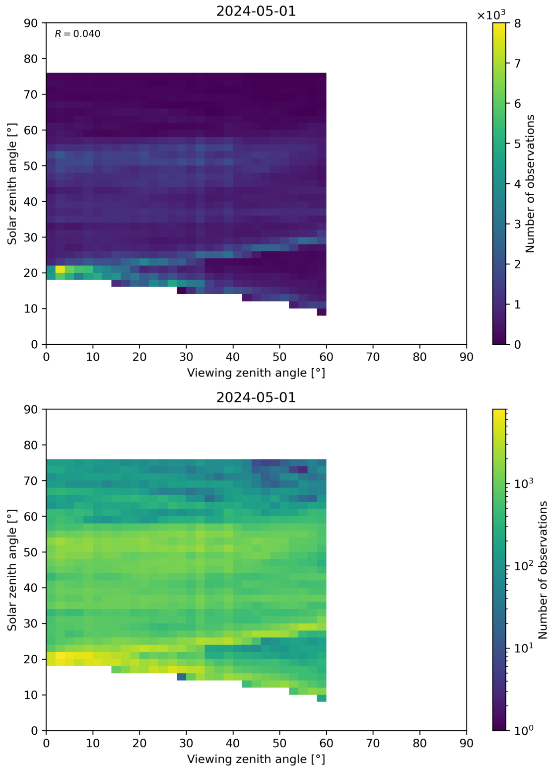
Figure 115: Scatter density plot of “Viewing zenith angle” against “Solar zenith angle” for 2024-04-30 to 2024-05-02.
