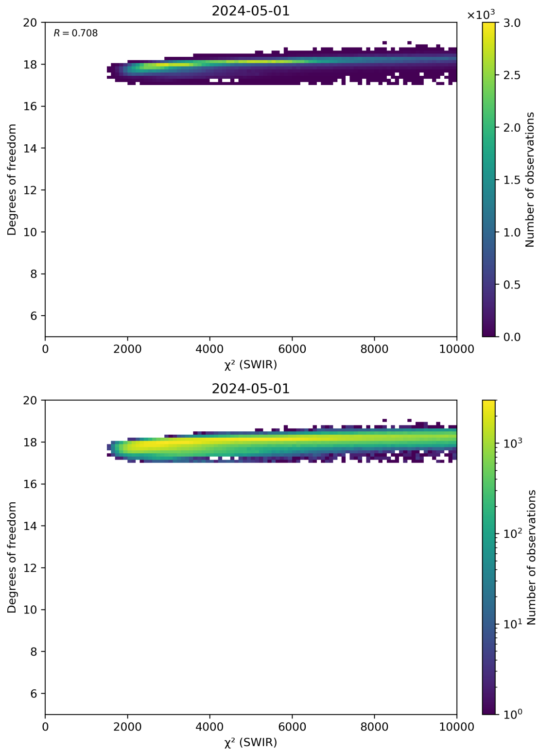
Figure 48: Scatter density plot of " \chi^2 (SWIR)" against "Degrees of freedom" for 2024-04-30 to 2024-05-02.
