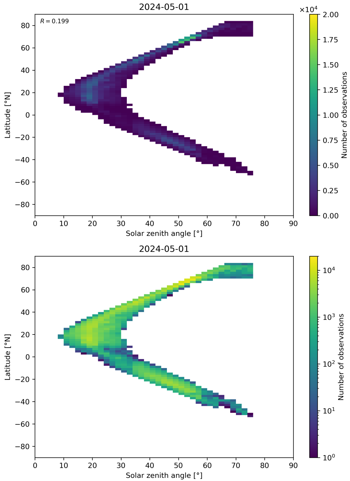
Figure 98: Scatter density plot of “Solar zenith angle” against “Latitude” for 2024-04-30 to 2024-05-02.
