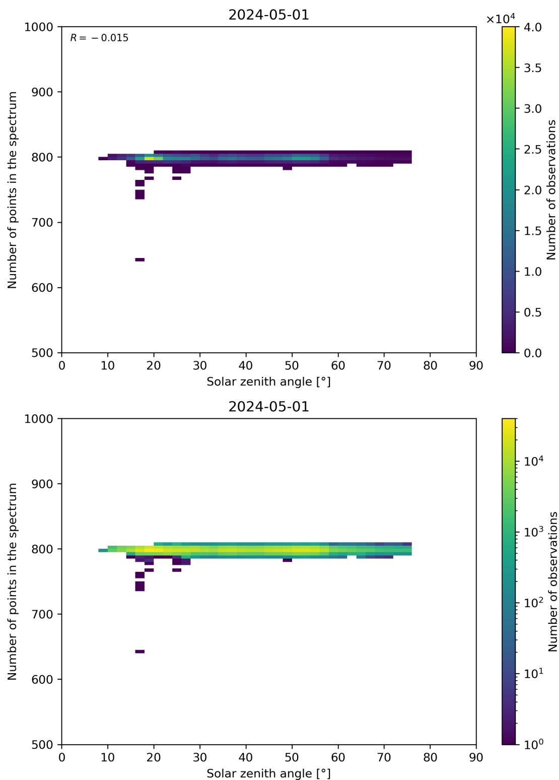
Figure 103: Scatter density plot of “Solar zenith angle” against “Number of points in the spectrum” for 2024-04-30 to 2024-05-02.
