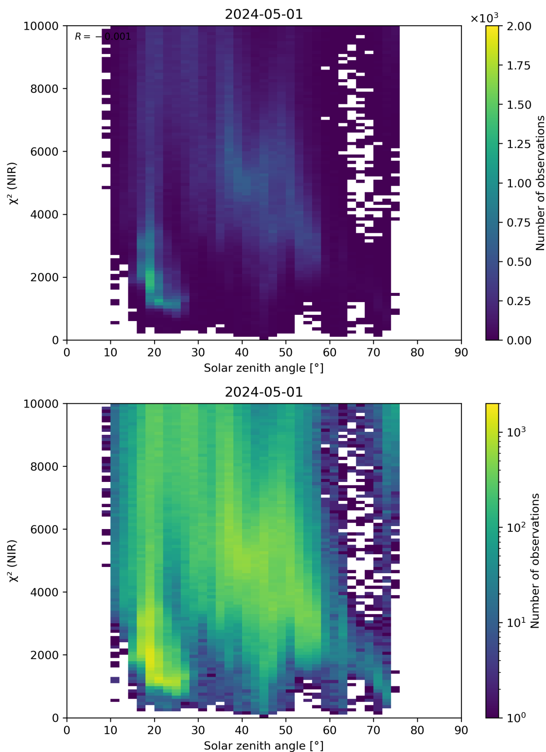
Figure 94: Scatter density plot of “Solar zenith angle” against “ \chi^2 (NIR)” for 2024-04-30 to 2024-05-02.
