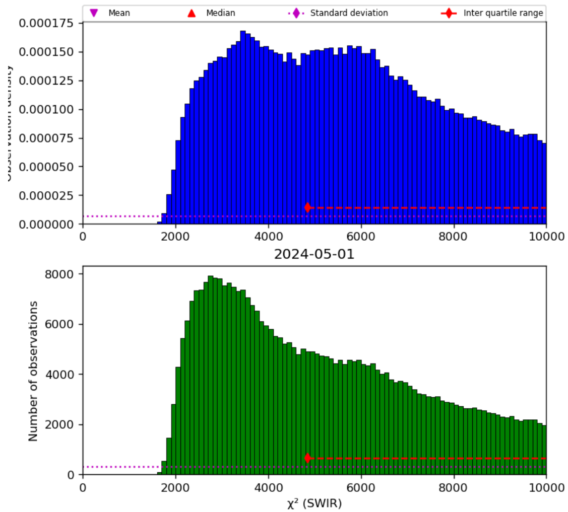
Figure 28: Histogram of “ \chi^2 (SWIR)” for 2024-04-30 to 2024-05-02
