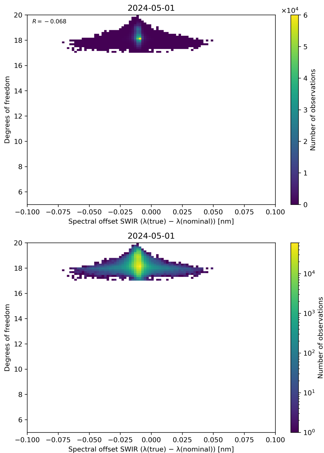
Figure 119: Scatter density plot of “Spectral offset SWIR ( \lambda(\text{true}) - \lambda(\text{nominal}) )” against “Degrees of freedom” for 2024-04-30 to 2024-05-02.
