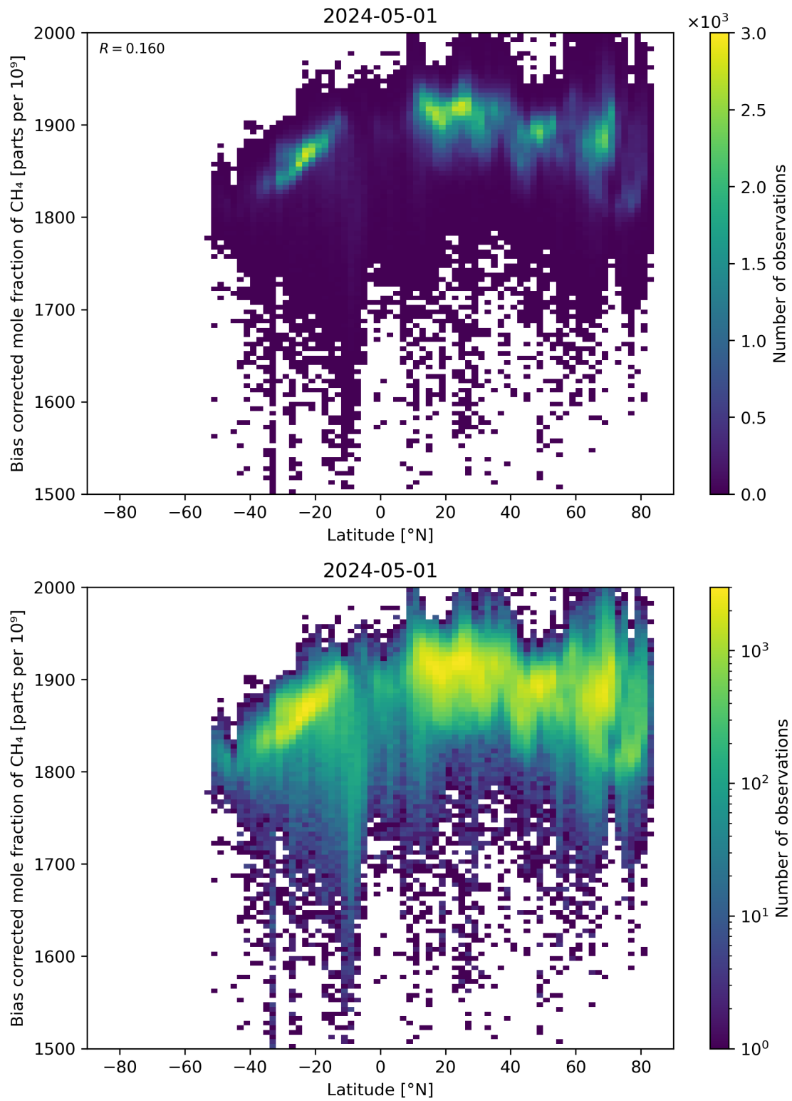
Figure 58: Scatter density plot of “Latitude” against “Bias corrected mole fraction of CH 4 ” for 2024-04-30 to 2024-05-02.
