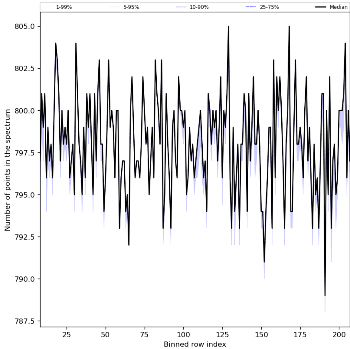
Figure 37: Along track statistics of “Number of points in the spectrum” for 2024-04-30 to 2024-05-02
