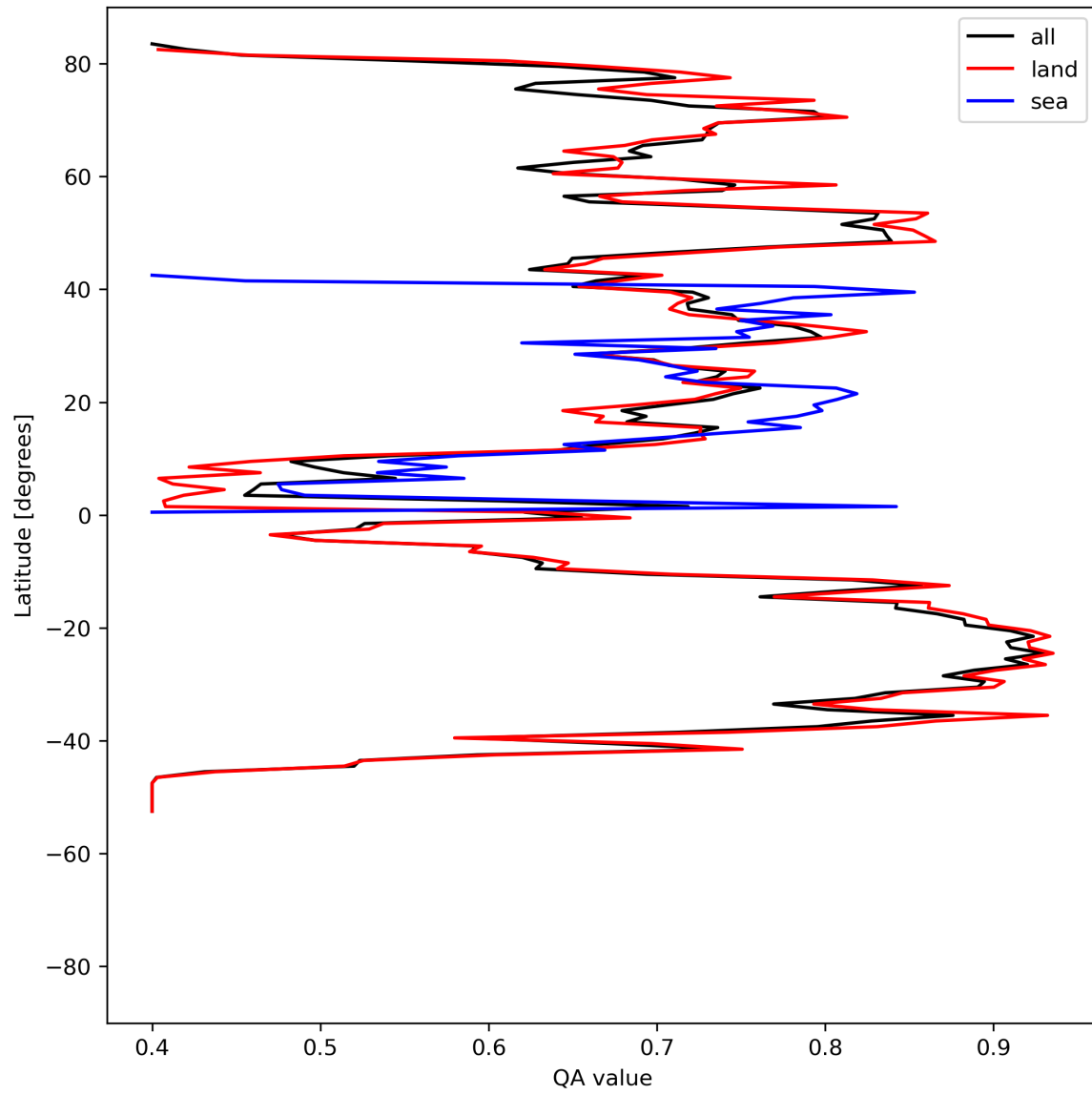
Figure 11: Zonal average of “QA value” for 2024-04-30 to 2024-05-02.
