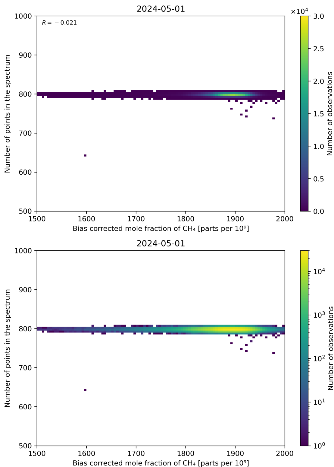
Figure 68: Scatter density plot of “Bias corrected mole fraction of CH 4 ” against “Number of points in the spectrum” for 2024-04-30 to 2024-05-02.
