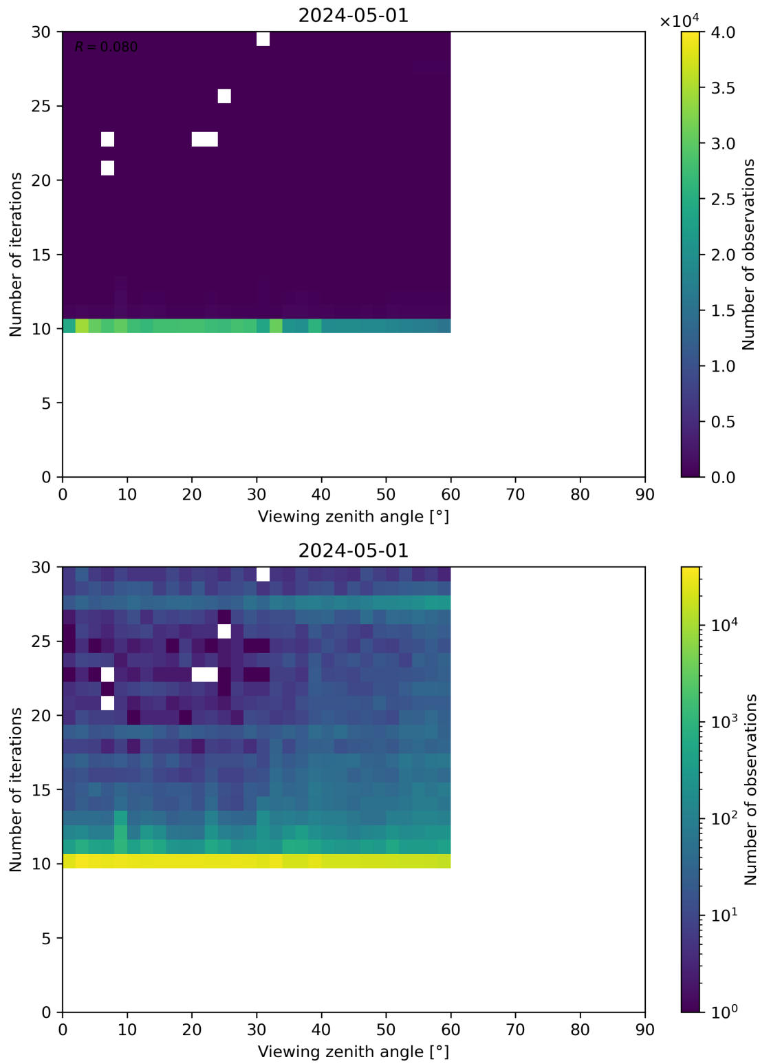
Figure 113: Scatter density plot of “Viewing zenith angle” against “Number of iterations” for 2024-04-30 to 2024-05-02.
