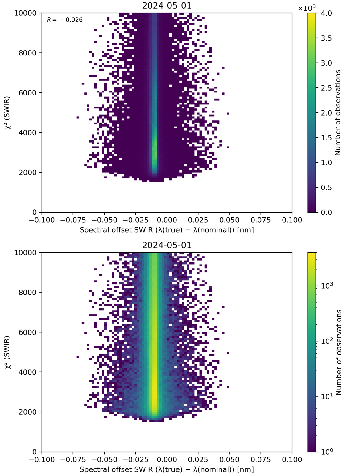
Figure 118: Scatter density plot of “Spectral offset SWIR ( \lambda(\text{true}) - \lambda(\text{nominal}) )” against “ \chi^2 (SWIR)” for 2024-04-30 to 2024-05-02.
