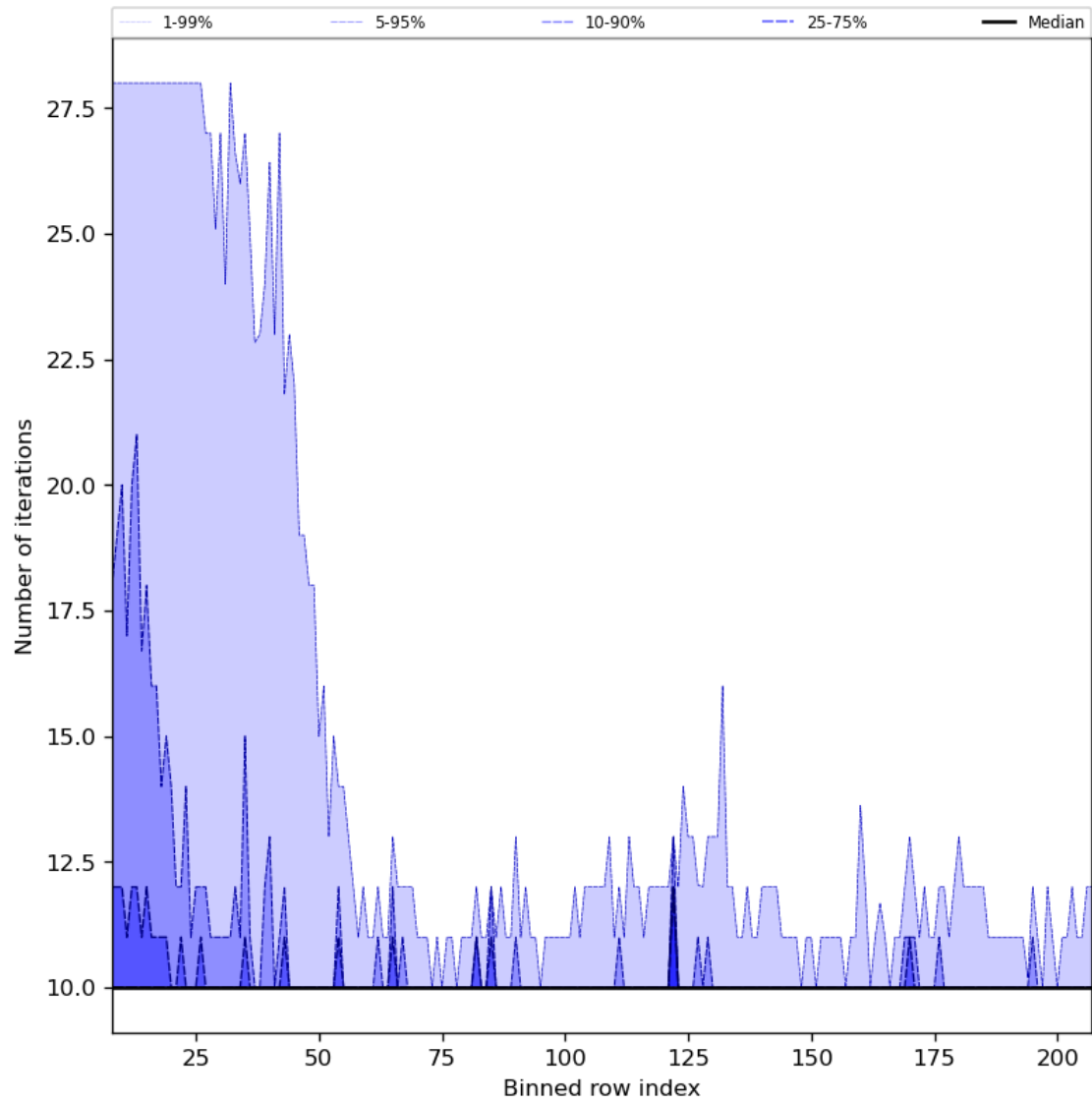
Figure 42: Along track statistics of “Number of iterations” for 2024-04-30 to 2024-05-02
