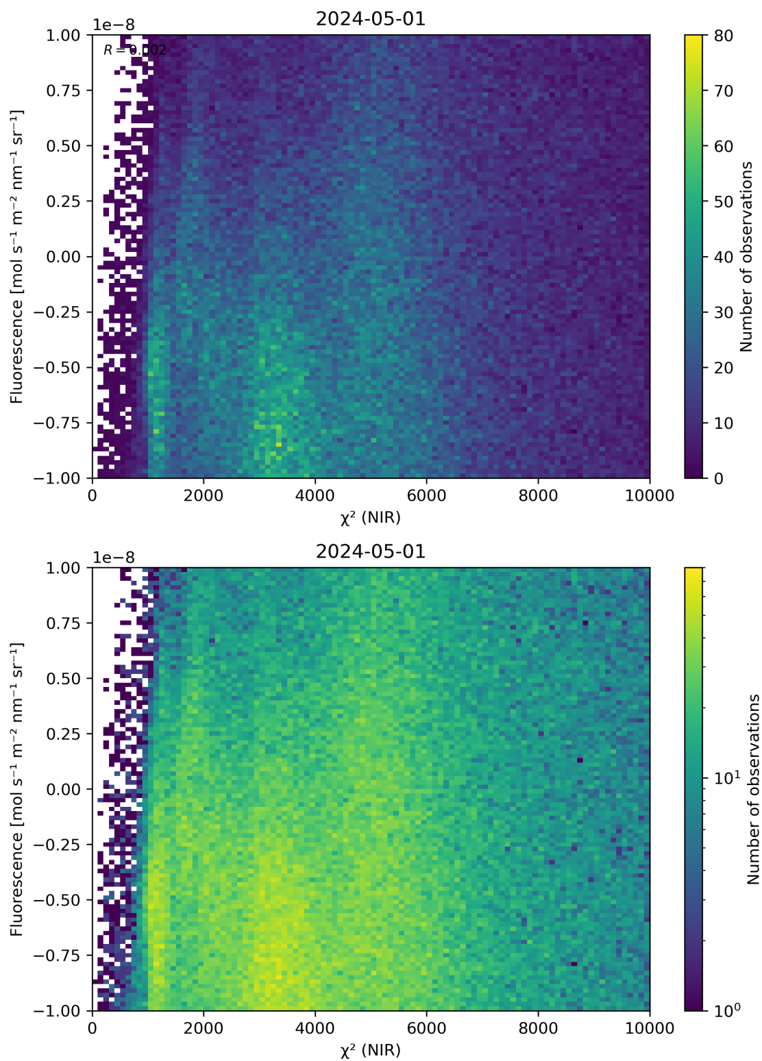
Figure 45: Scatter density plot of “ \chi^2 (NIR)” against “Fluorescence” for 2024-04-30 to 2024-05-02.
