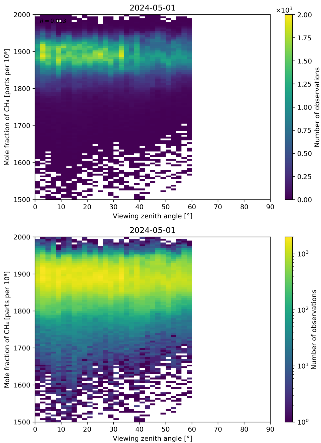
Figure 110: Scatter density plot of “Viewing zenith angle” against “Mole fraction of CH 4 ” for 2024-04-30 to 2024-05-02.
