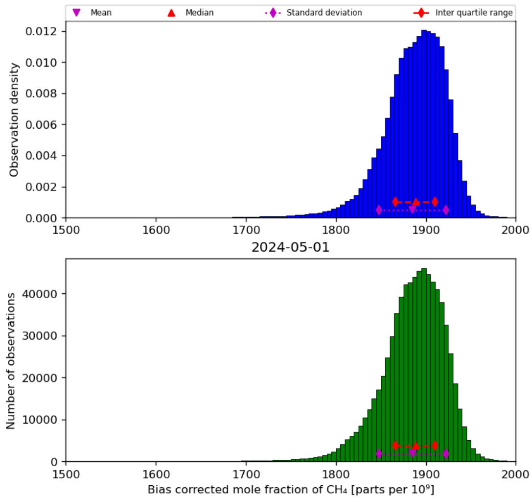
Figure 25: Histogram of “Bias corrected mole fraction of CH 4 ” for 2024-04-30 to 2024-05-02
