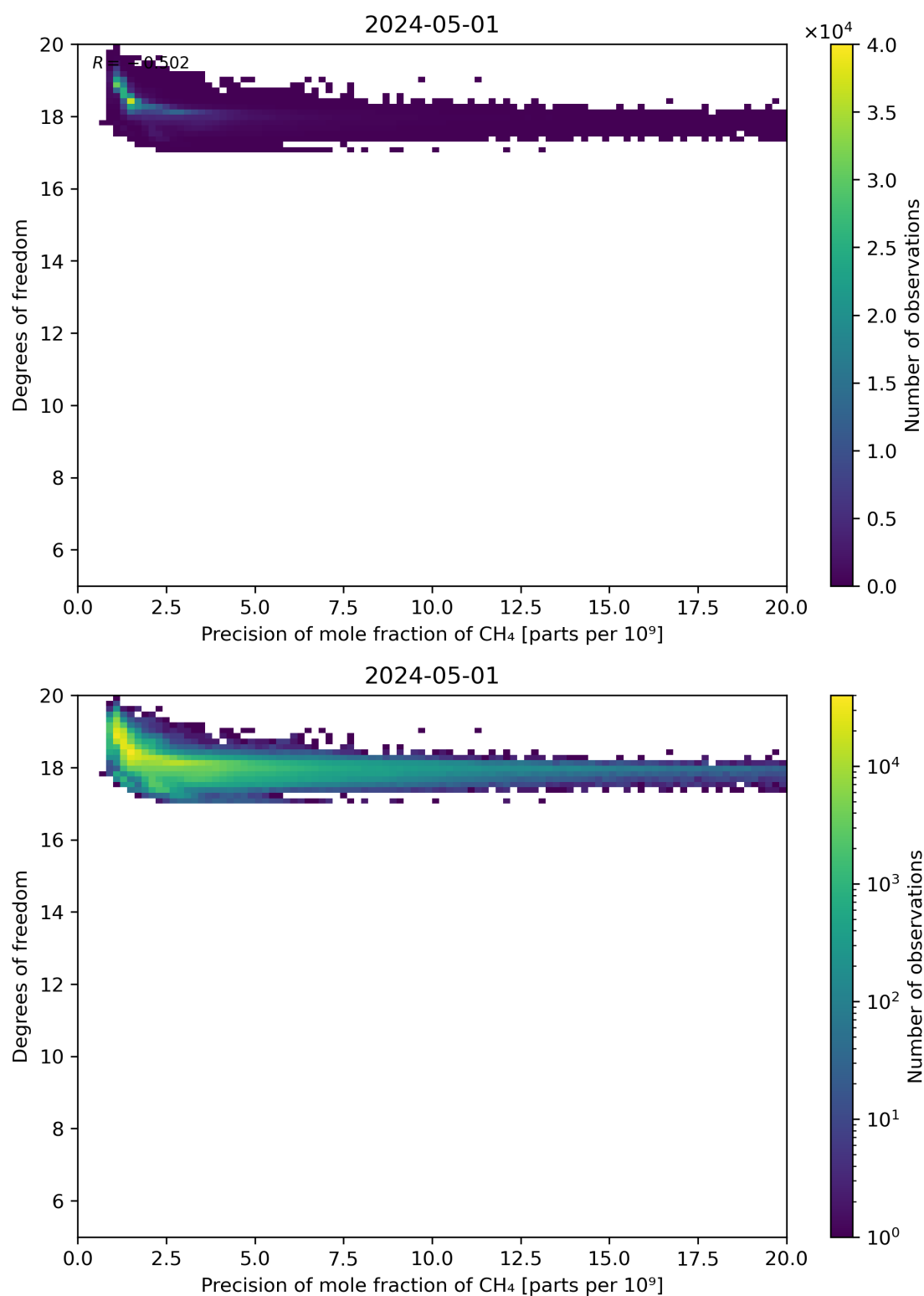
Figure 80: Scatter density plot of “Precision of mole fraction of CH 4 ” against “Degrees of freedom” for 2024-04-30 to 2024-05-02.
