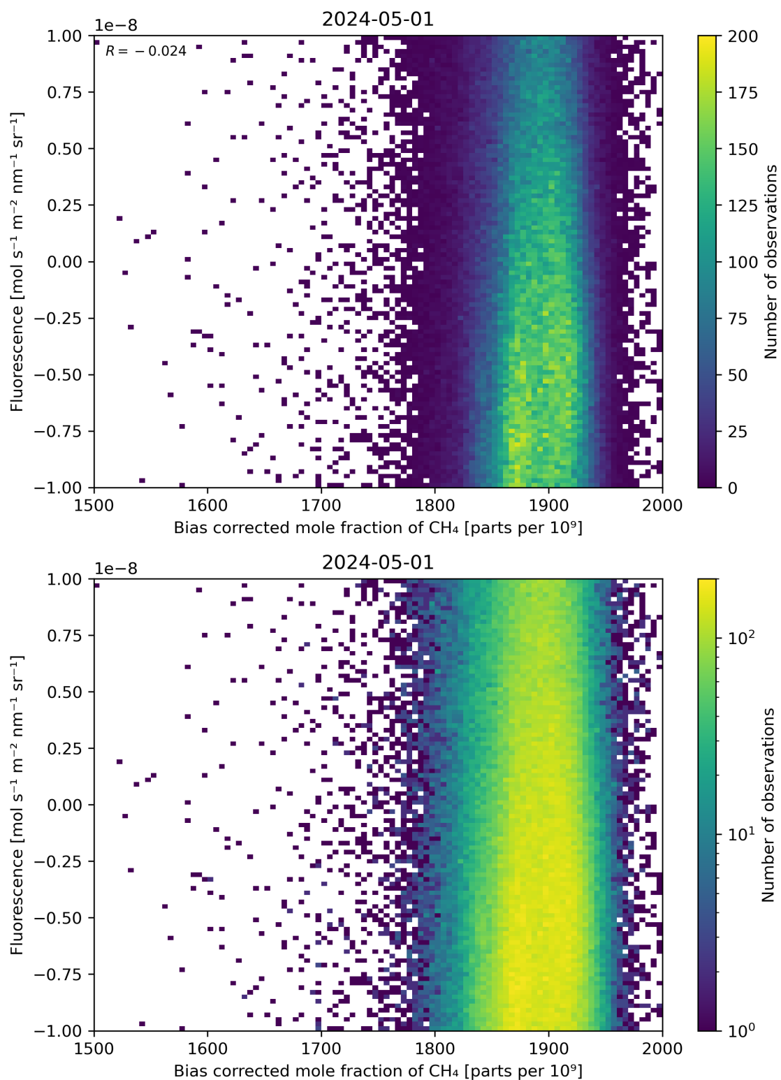
Figure 66: Scatter density plot of “Bias corrected mole fraction of \text{CH}_4 ” against “Fluorescence” for 2024-04-30 to 2024-05-02.
