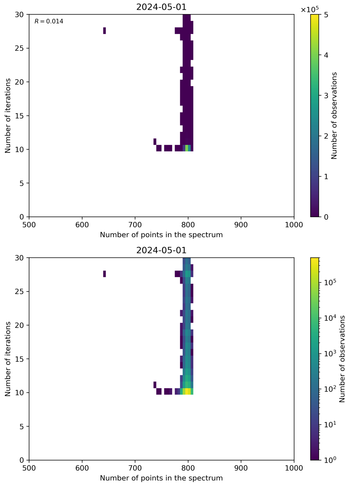
Figure 92: Scatter density plot of “Number of points in the spectrum” against “Number of iterations” for 2024-04-30 to 2024-05-02.
