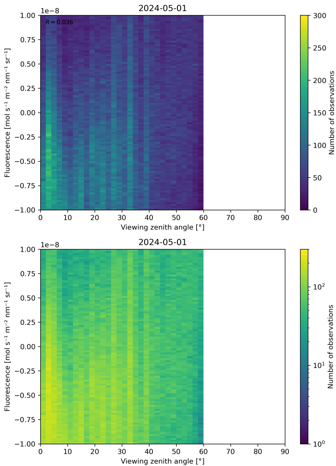
Figure 108: Scatter density plot of “Viewing zenith angle” against “Fluorescence” for 2024-04-30 to 2024-05-02.
