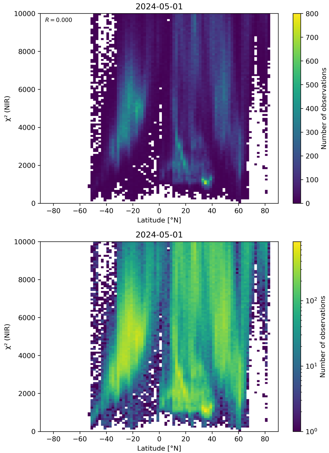
Figure 53: Scatter density plot of “Latitude” against “ \chi^2 (NIR)” for 2024-04-30 to 2024-05-02.
