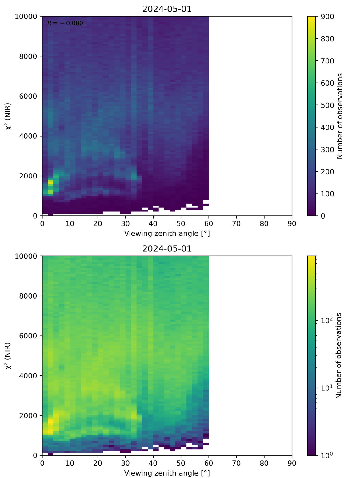
Figure 105: Scatter density plot of “Viewing zenith angle” against “ \chi^2 (NIR)” for 2024-04-30 to 2024-05-02.
