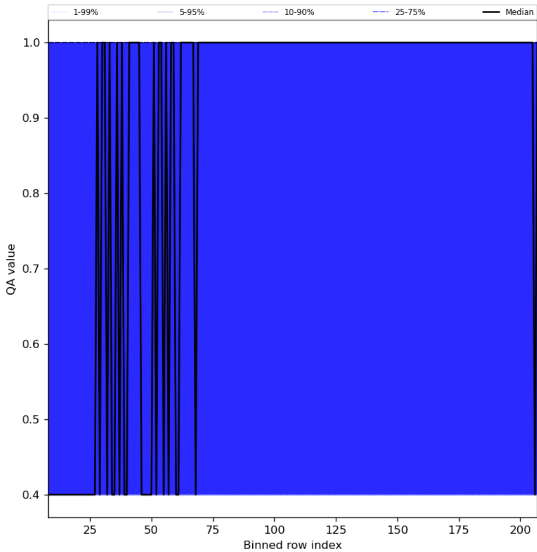
Figure 33: Along track statistics of “QA value” for 2024-04-30 to 2024-05-02
