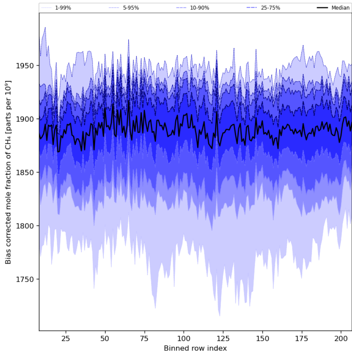
Figure 36: Along track statistics of “Bias corrected mole fraction of CH 4 ” for 2024-04-30 to 2024-05-02
