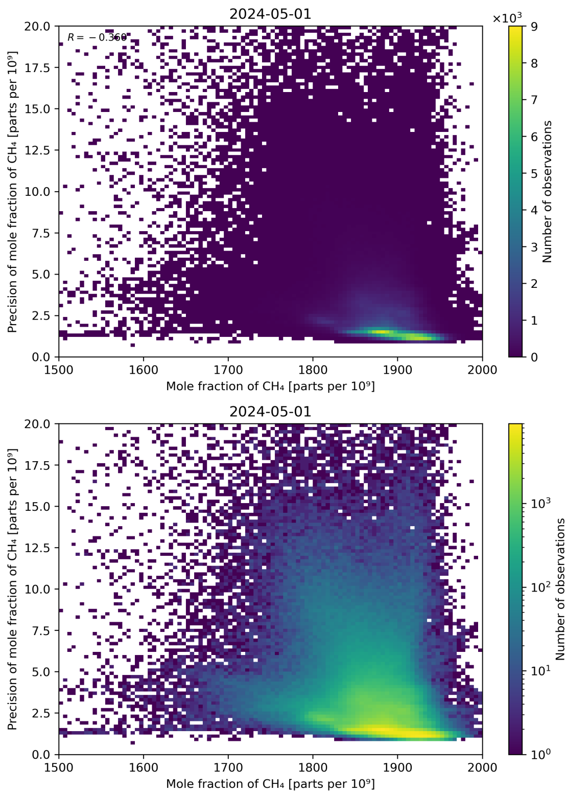
Figure 75: Scatter density plot of “Mole fraction of CH 4 ” against “Precision of mole fraction of CH 4 ” for 2024-04-30 to 2024-05-02.
