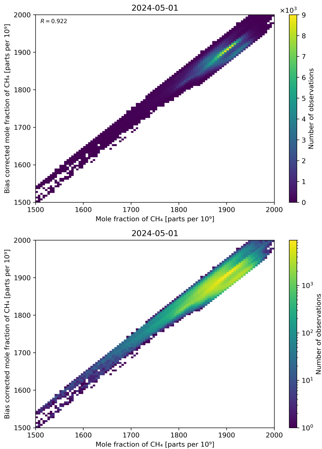
Figure 74: Scatter density plot of “Mole fraction of CH 4 ” against “Bias corrected mole fraction of CH 4 ” for 2024-04-30 to 2024-05-02.
