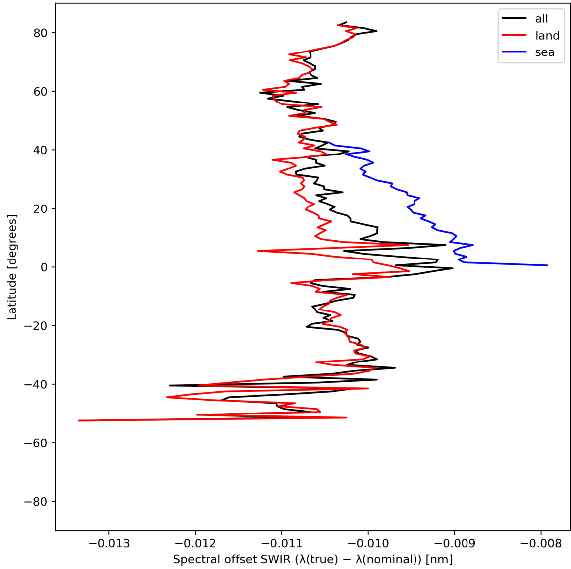
Figure 16: Zonal average of “Spectral offset SWIR ( \lambda(\text{true}) - \lambda(\text{nominal}) )” for 2024-04-30 to 2024-05-02.
