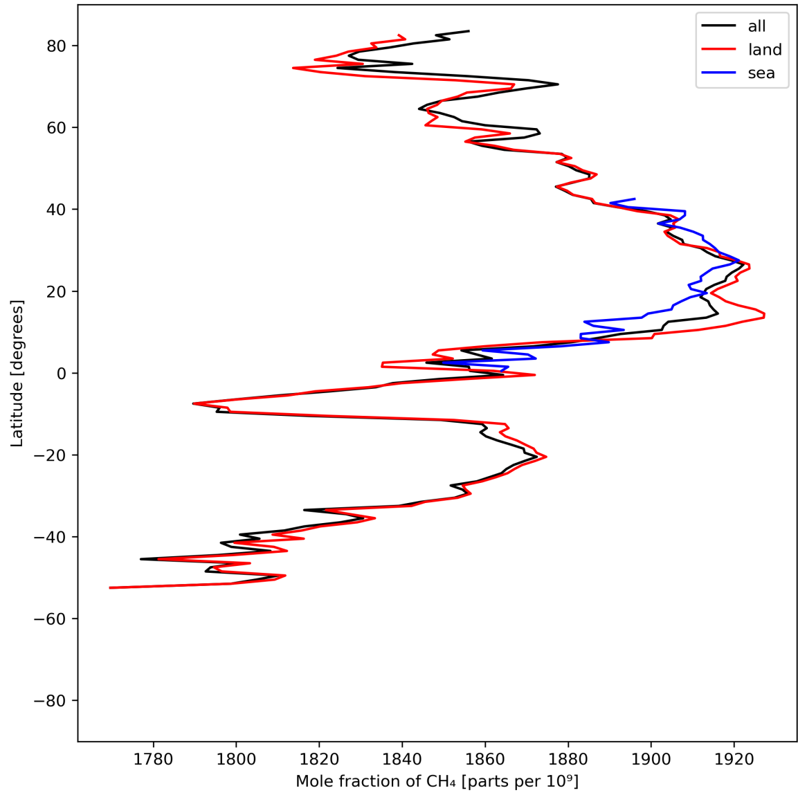
Figure 12: Zonal average of “Mole fraction of \text{CH}_4 ” for 2024-04-30 to 2024-05-02.
