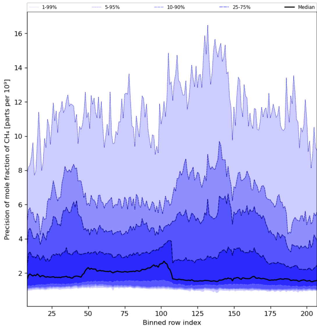
Figure 35: Along track statistics of “Precision of mole fraction of CH 4 ” for 2024-04-30 to 2024-05-02
