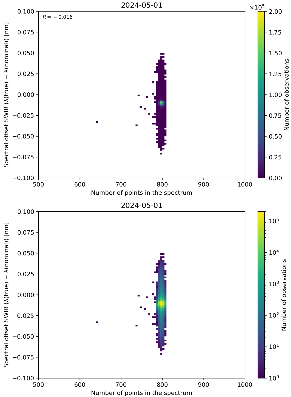
Figure 93: Scatter density plot of “Number of points in the spectrum” against “Spectral offset SWIR ( \lambda(\text{true}) - \lambda(\text{nominal}) )” for 2024-04-30 to 2024-05-02.
