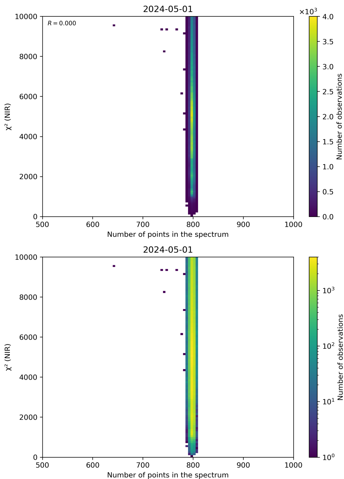
Figure 88: Scatter density plot of “Number of points in the spectrum” against “ \chi^2 (NIR)” for 2024-04-30 to 2024-05-02.
