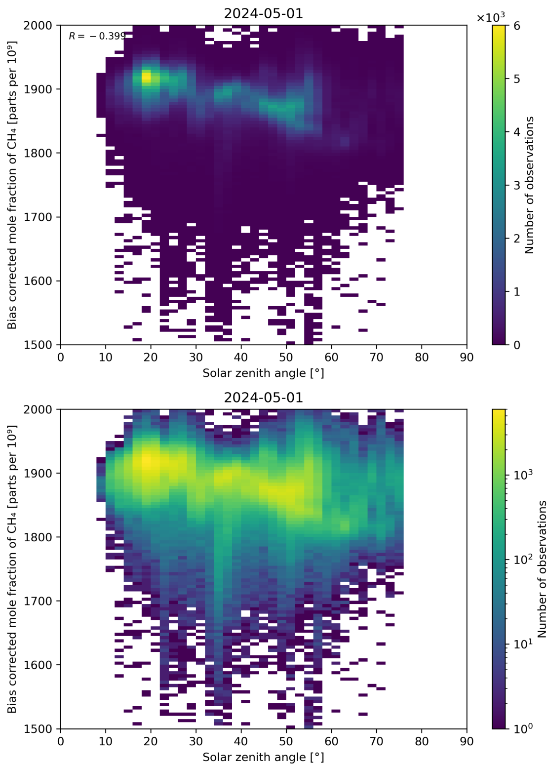
Figure 100: Scatter density plot of “Solar zenith angle” against “Bias corrected mole fraction of \text{CH}_4 ” for 2024-04-30 to 2024-05-02.
