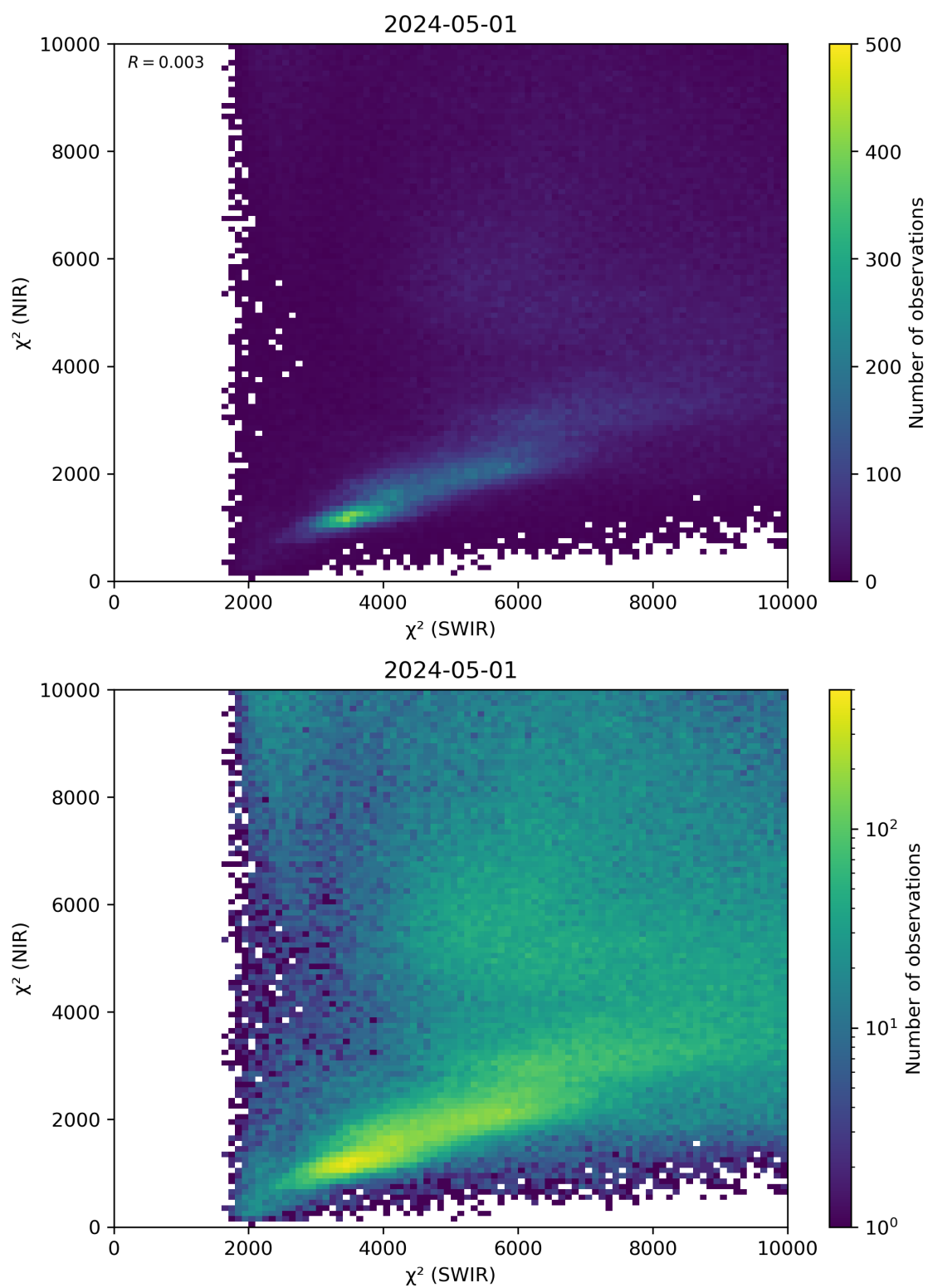
Figure 47: Scatter density plot of “ \chi^2 (SWIR)” against “ \chi^2 (NIR)” for 2024-04-30 to 2024-05-02.
