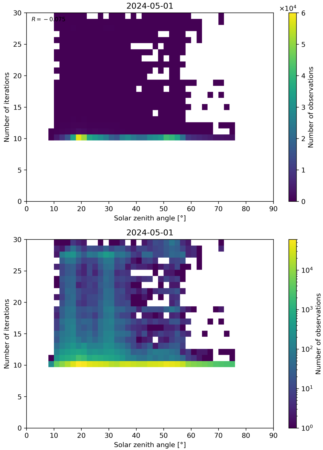
Figure 102: Scatter density plot of “Solar zenith angle” against “Number of iterations” for 2024-04-30 to 2024-05-02.
