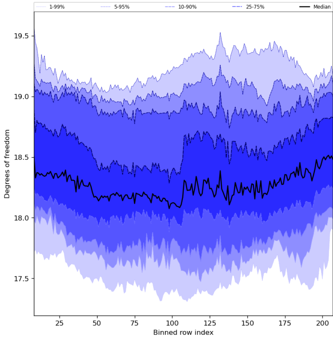
Figure 41: Along track statistics of “Degrees of freedom” for 2024-04-30 to 2024-05-02
