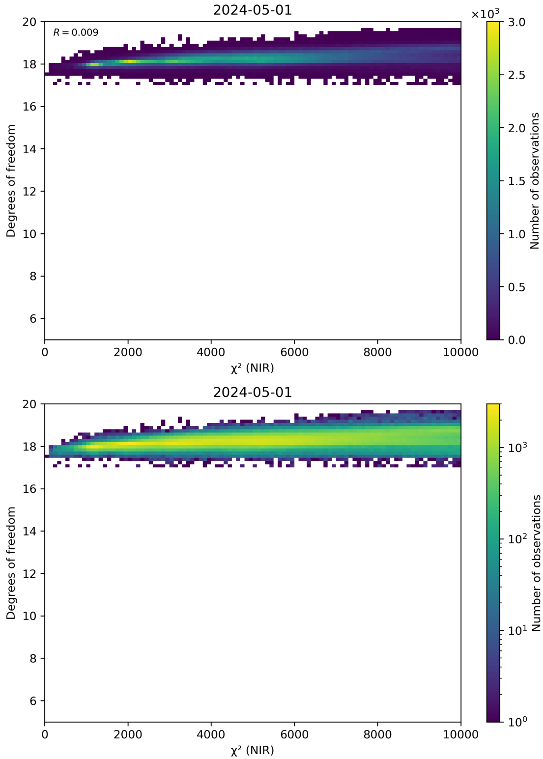
Figure 44: Scatter density plot of “ \chi^2 (NIR)” against “Degrees of freedom” for 2024-04-30 to 2024-05-02.
