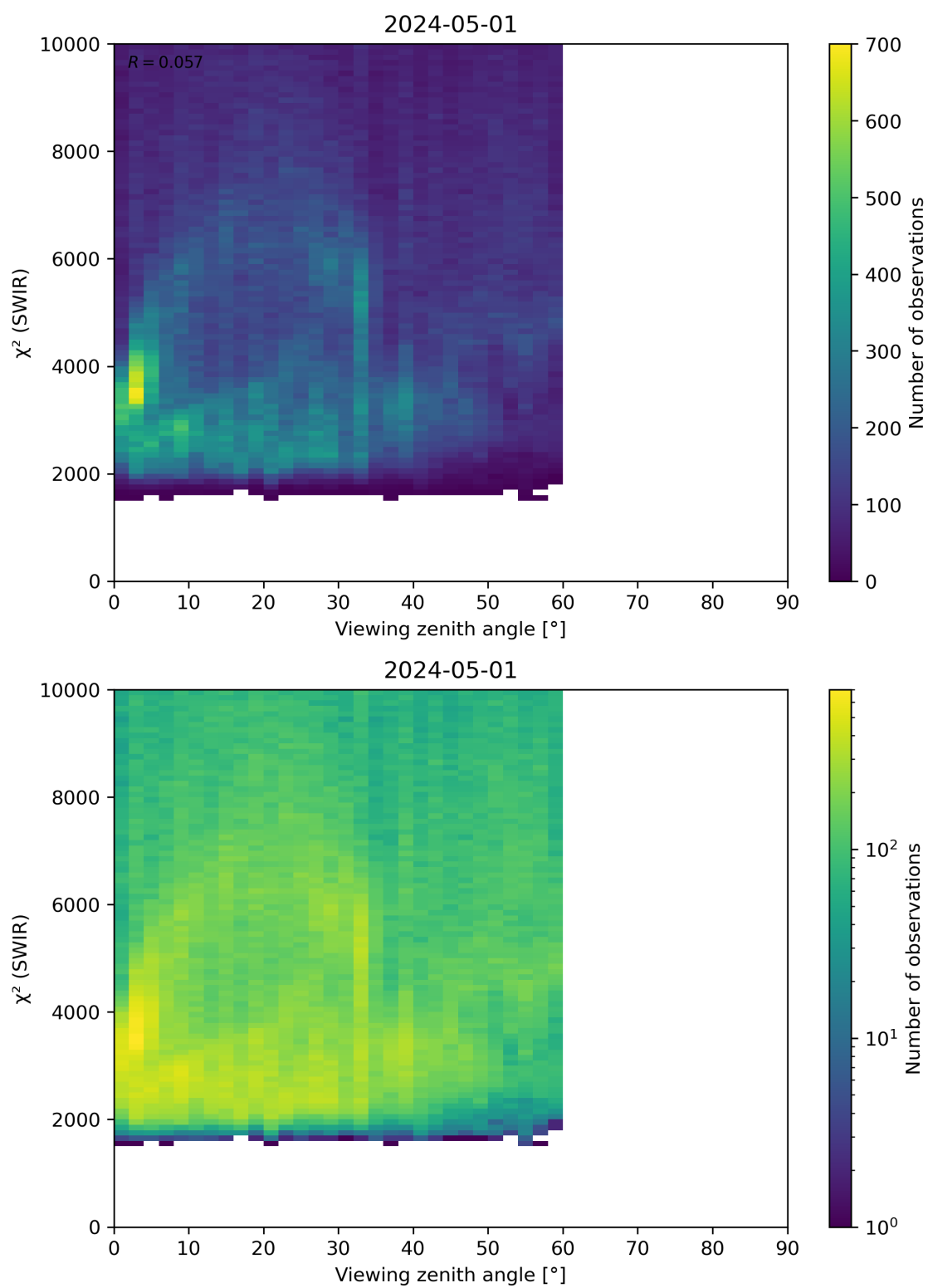
Figure 106: Scatter density plot of “Viewing zenith angle” against “ \chi^2 (SWIR)” for 2024-04-30 to 2024-05-02.
