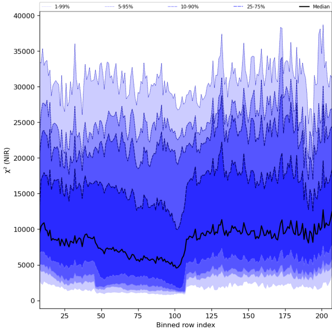
Figure 40: Along track statistics of “ \chi^2 (NIR)” for 2024-04-30 to 2024-05-02
