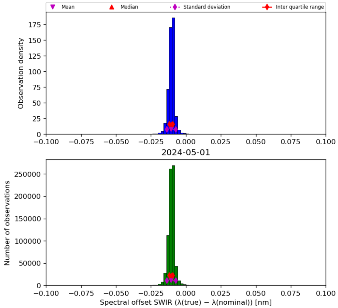
Figure 27: Histogram of “Spectral offset SWIR ( \lambda(\text{true}) - \lambda(\text{nominal}) )” for 2024-04-30 to 2024-05-02
