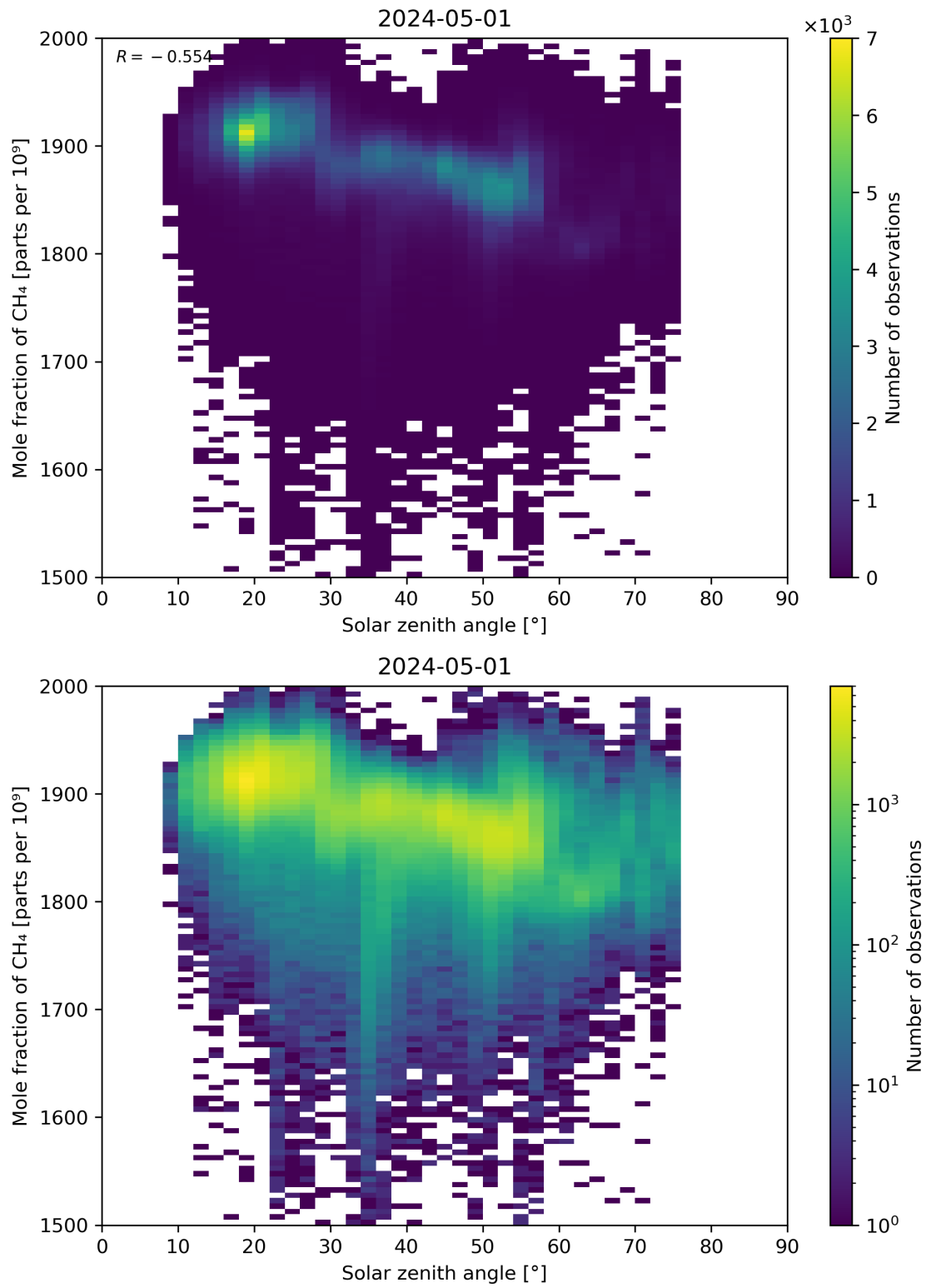
Figure 99: Scatter density plot of “Solar zenith angle” against “Mole fraction of CH 4 ” for 2024-04-30 to 2024-05-02.
