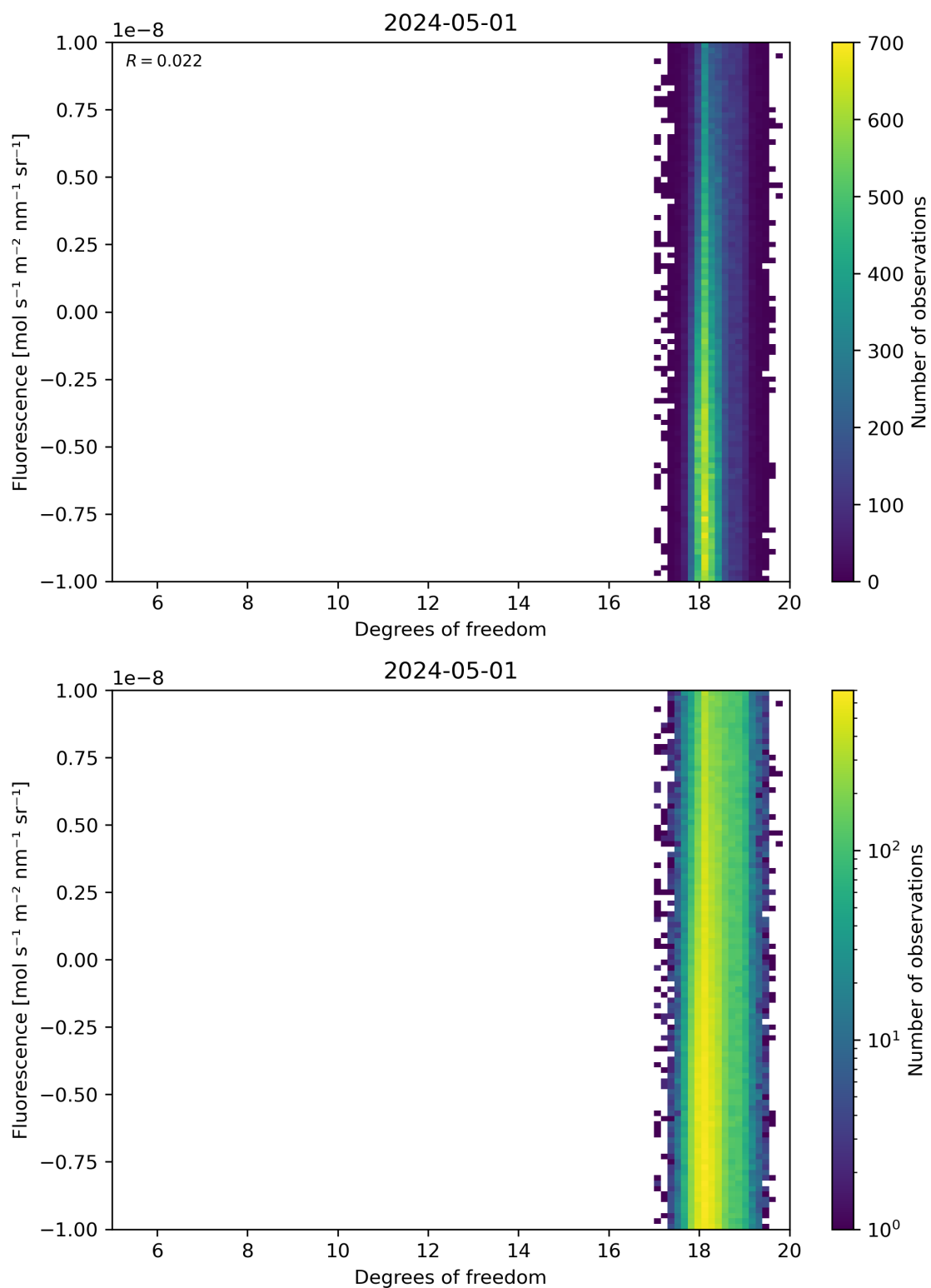
Figure 51: Scatter density plot of “Degrees of freedom” against “Fluorescence” for 2024-04-30 to 2024-05-02.
