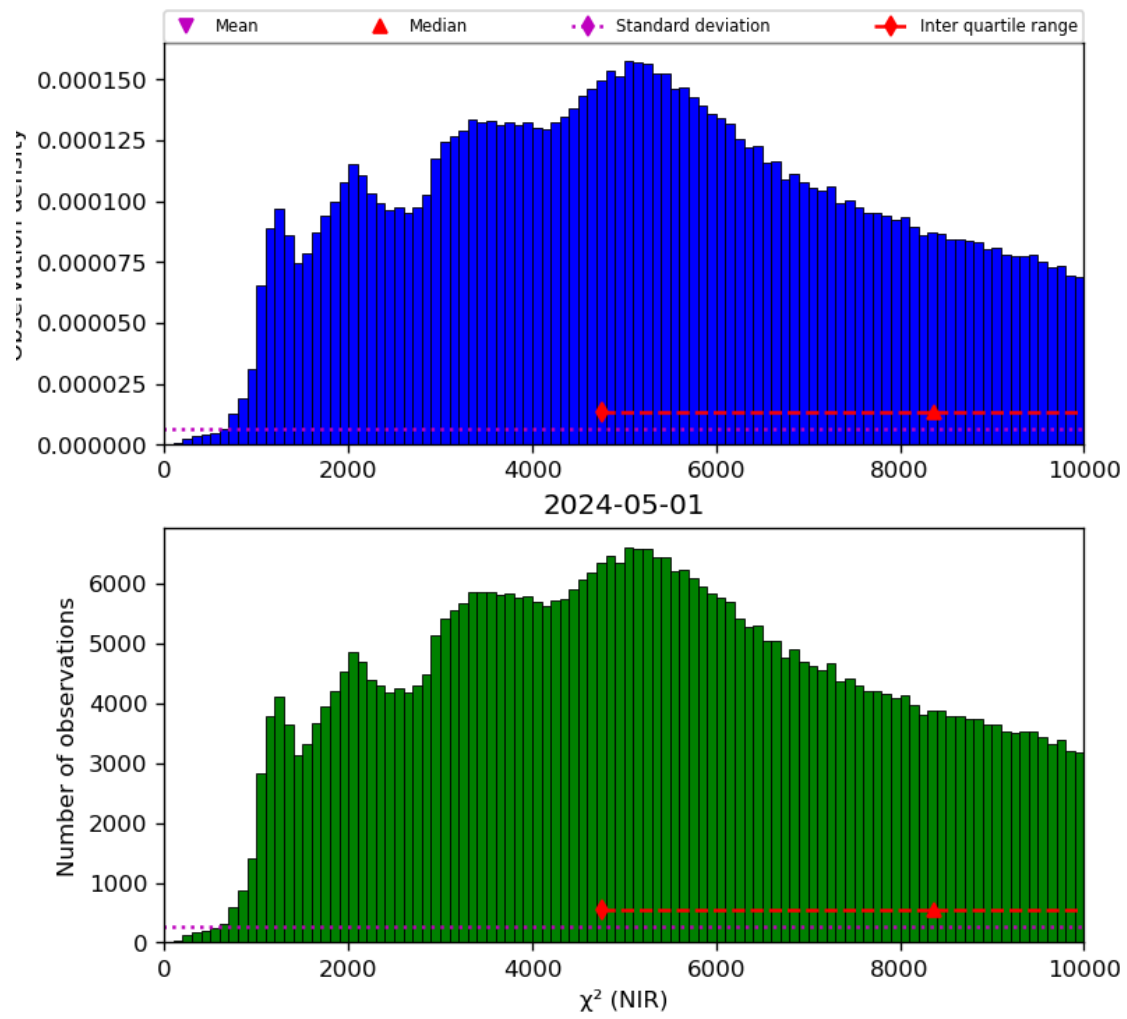
Figure 29: Histogram of “ \chi^2 (NIR)” for 2024-04-30 to 2024-05-02
