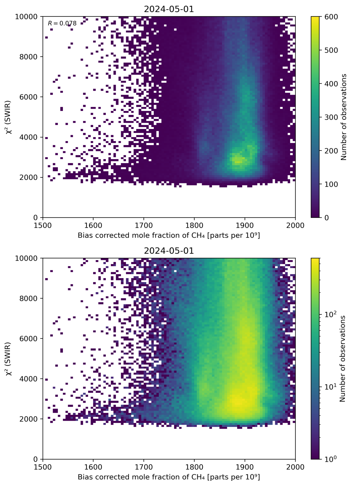
Figure 64: Scatter density plot of “Bias corrected mole fraction of \text{CH}_4 ” against “ \chi^2 (SWIR)” for 2024-04-30 to 2024-05-02.
