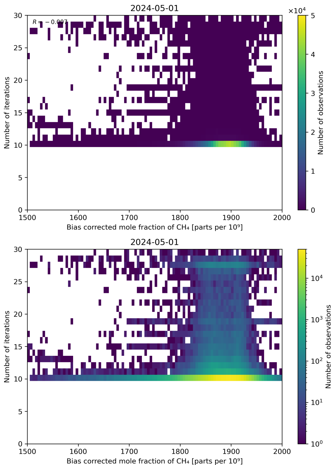
Figure 67: Scatter density plot of “Bias corrected mole fraction of CH 4 ” against “Number of iterations” for 2024-04-30 to 2024-05-02.
