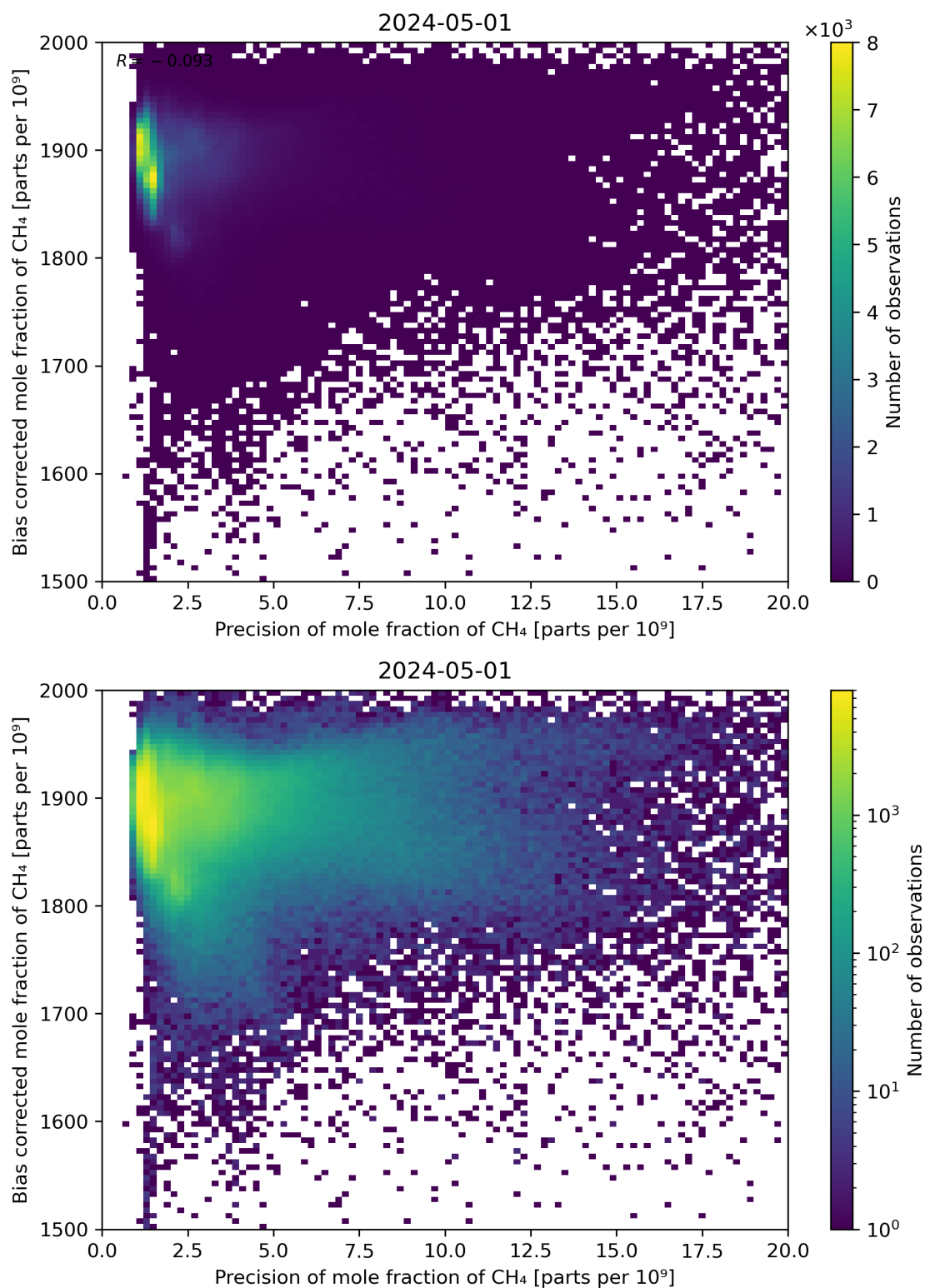
Figure 82: Scatter density plot of “Precision of mole fraction of CH 4 ” against “Bias corrected mole fraction of CH 4 ” for 2024-04-30 to 2024-05-02.
