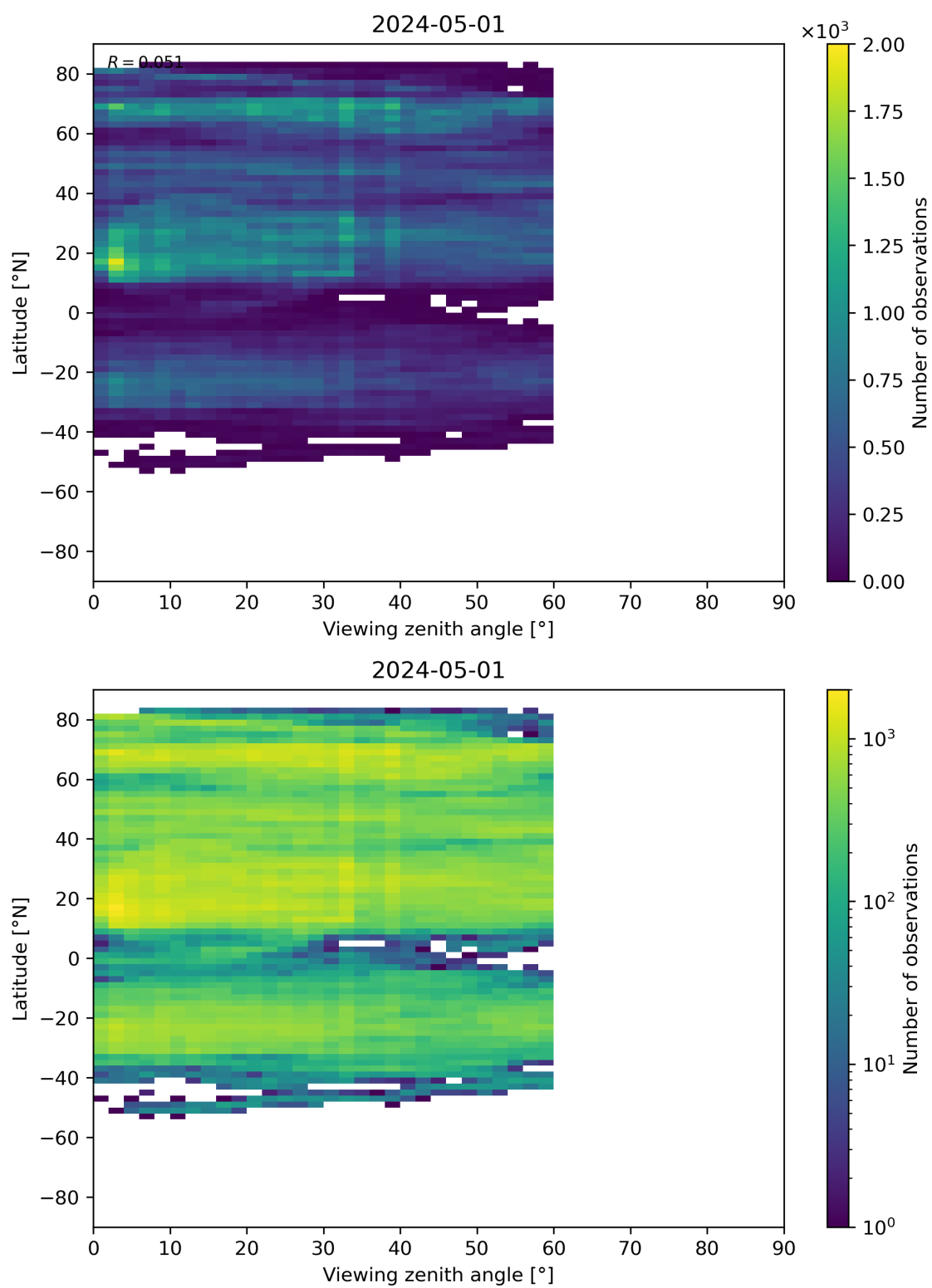
Figure 109: Scatter density plot of “Viewing zenith angle” against “Latitude” for 2024-04-30 to 2024-05-02.
