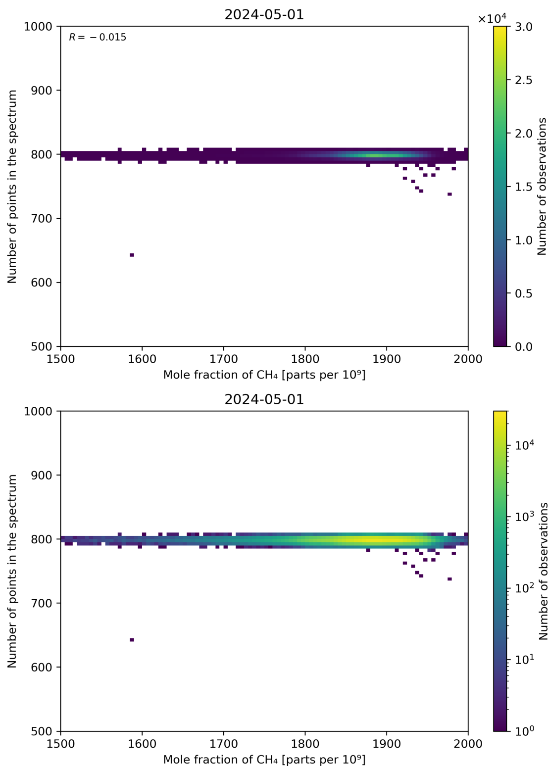
Figure 77: Scatter density plot of “Mole fraction of CH 4 ” against “Number of points in the spectrum” for 2024-04-30 to 2024-05-02.
