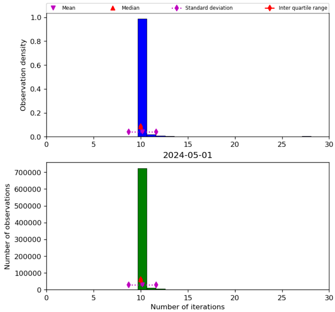
Figure 31: Histogram of “Number of iterations” for 2024-04-30 to 2024-05-02
