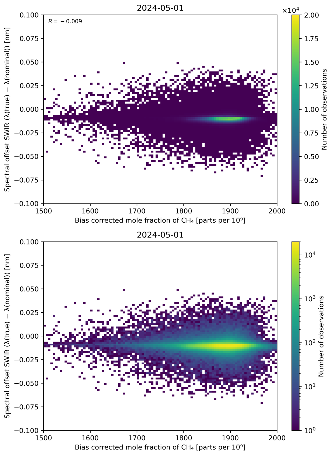
Figure 69: Scatter density plot of “Bias corrected mole fraction of \text{CH}_4 ” against “Spectral offset SWIR ( \lambda(\text{true}) - \lambda(\text{nominal}) )” for 2024-04-30 to 2024-05-02.
