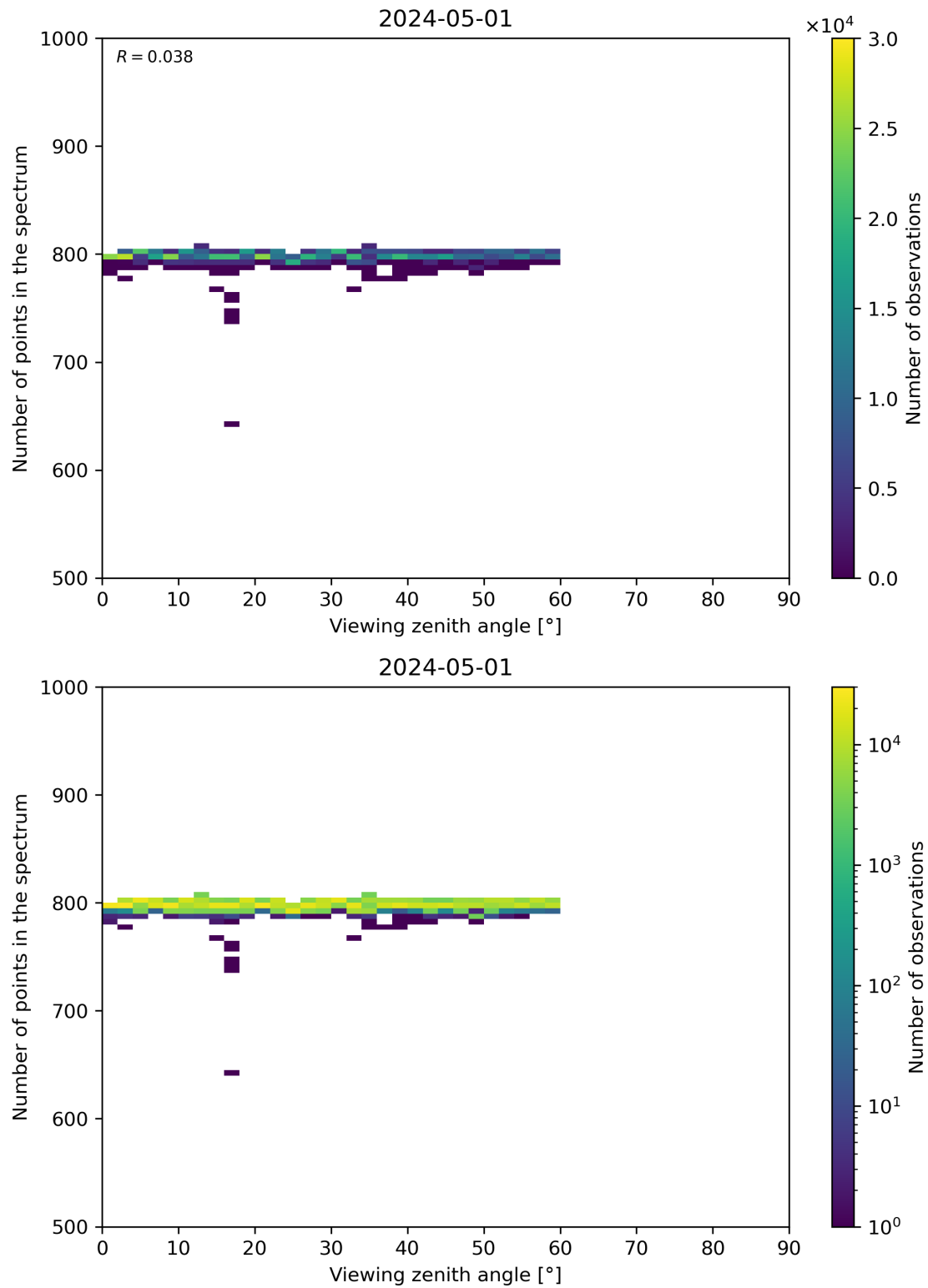
Figure 114: Scatter density plot of “Viewing zenith angle” against “Number of points in the spectrum” for 2024-04-30 to 2024-05-02.
