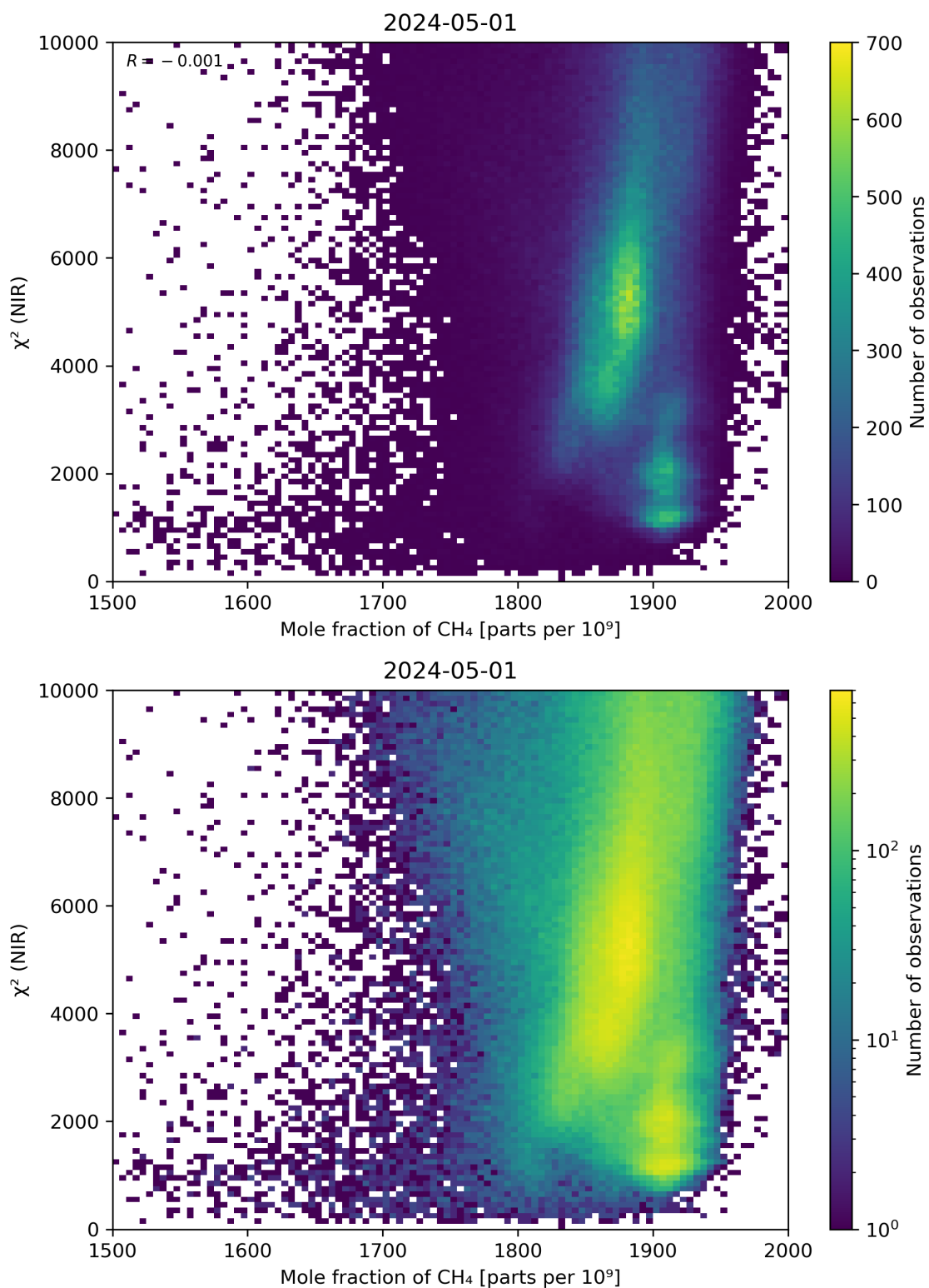
Figure 70: Scatter density plot of “Mole fraction of \text{CH}_4 ” against “ \chi^2 (NIR)” for 2024-04-30 to 2024-05-02.
