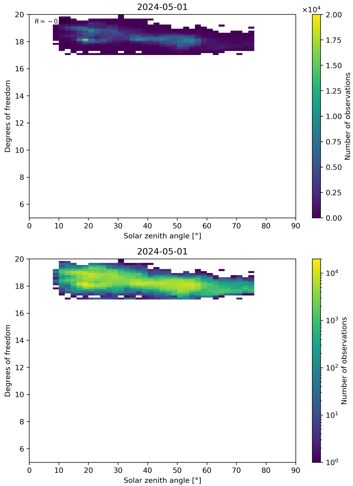
Figure 96: Scatter density plot of “Solar zenith angle” against “Degrees of freedom” for 2024-04-30 to 2024-05-02.
