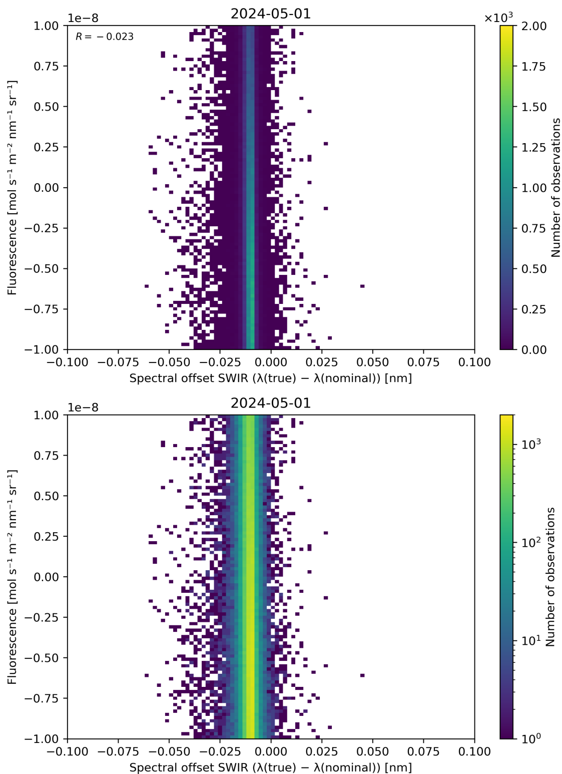
Figure 120: Scatter density plot of “Spectral offset SWIR ( \lambda(\text{true}) - \lambda(\text{nominal}) )” against “Fluorescence” for 2024-04-30 to 2024-05-02.
