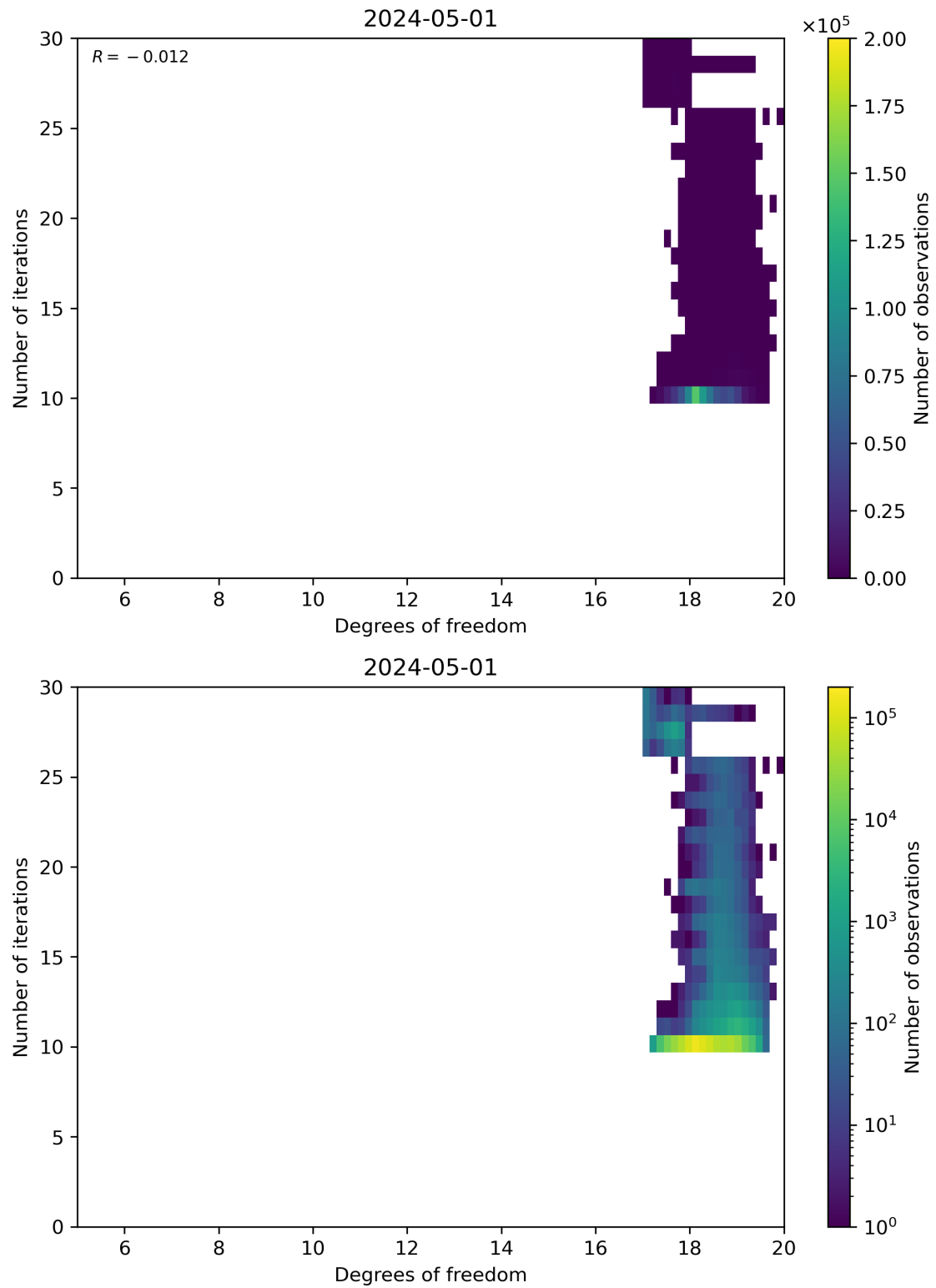
Figure 52: Scatter density plot of “Degrees of freedom” against “Number of iterations” for 2024-04-30 to 2024-05-02.
