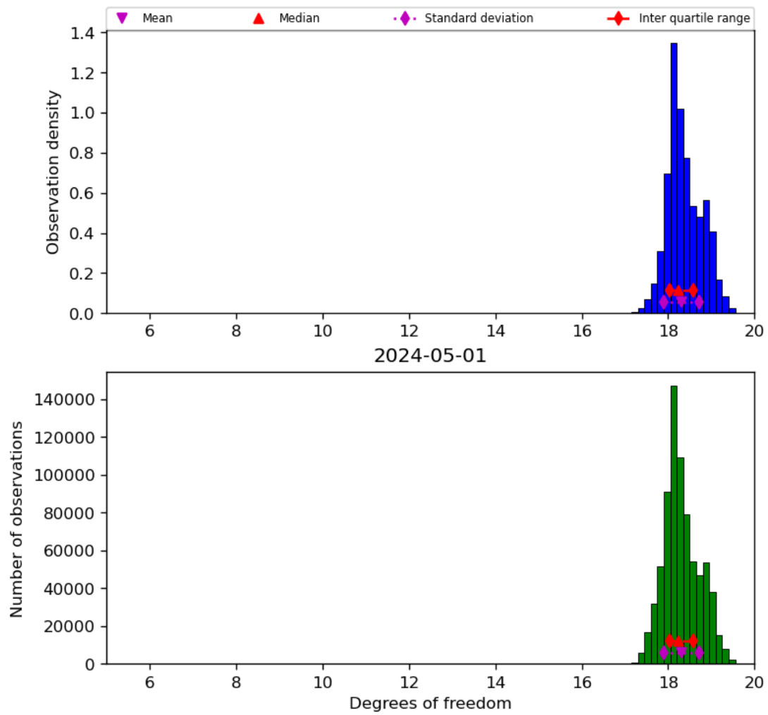
Figure 30: Histogram of “Degrees of freedom” for 2024-04-30 to 2024-05-02
