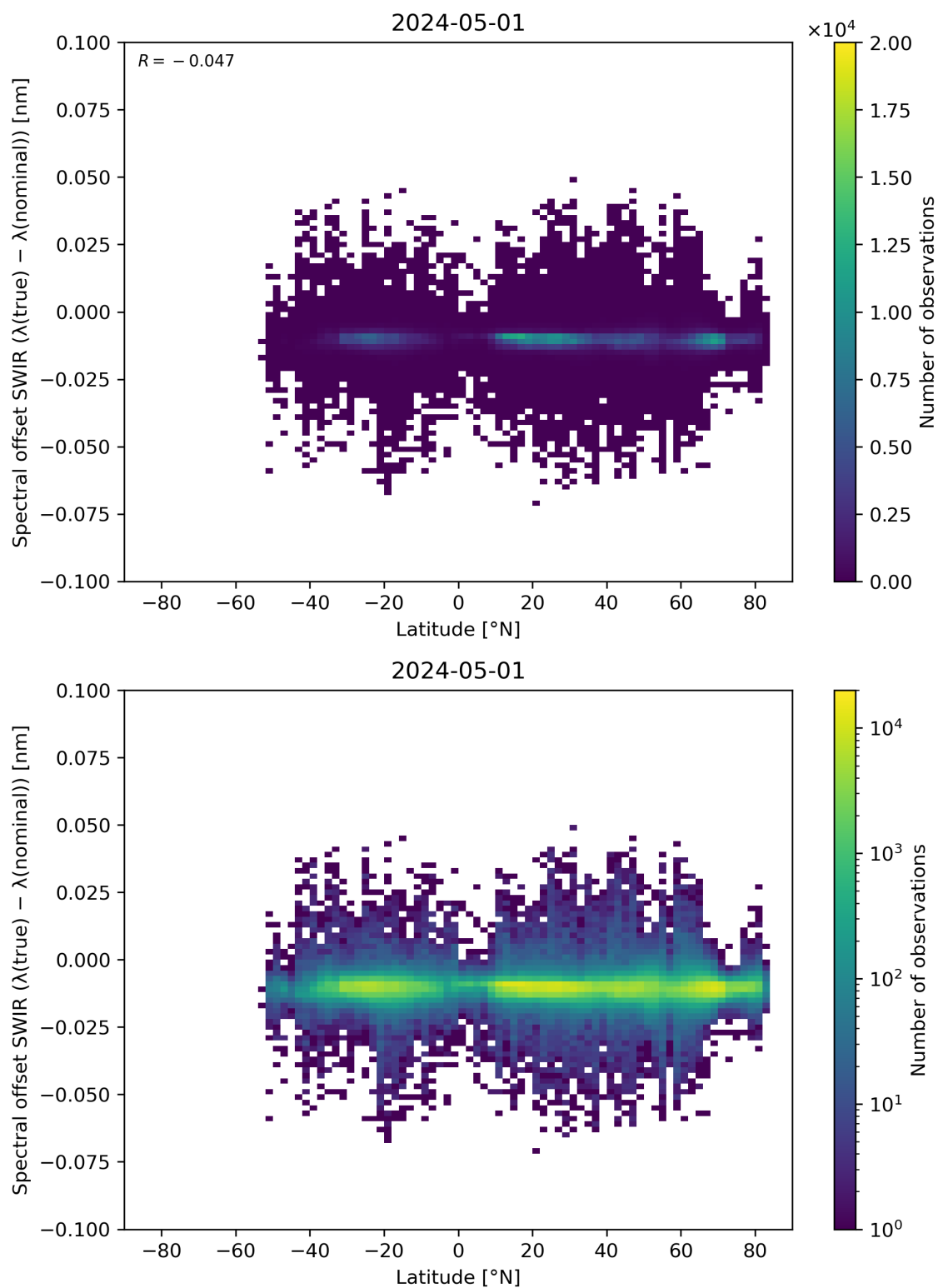
Figure 62: Scatter density plot of “Latitude” against “Spectral offset SWIR ( \lambda(\text{true}) - \lambda(\text{nominal}) )” for 2024-04-30 to 2024-05-02.
