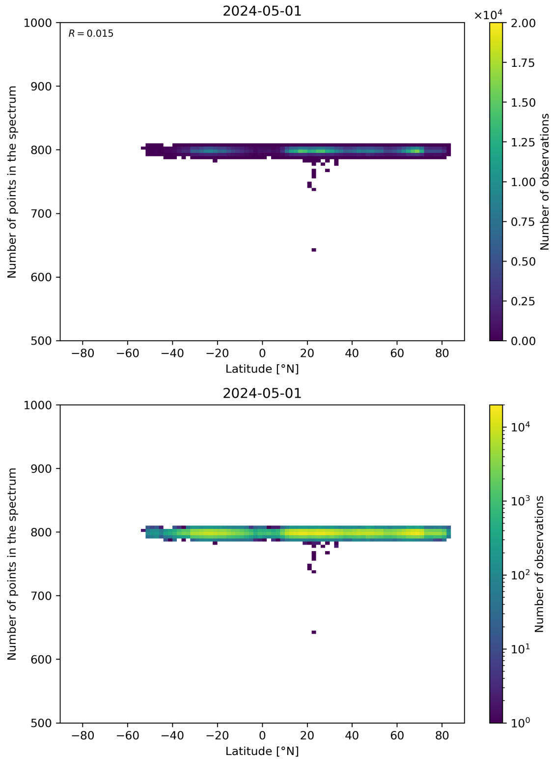
Figure 61: Scatter density plot of “Latitude” against “Number of points in the spectrum” for 2024-04-30 to 2024-05-02.
