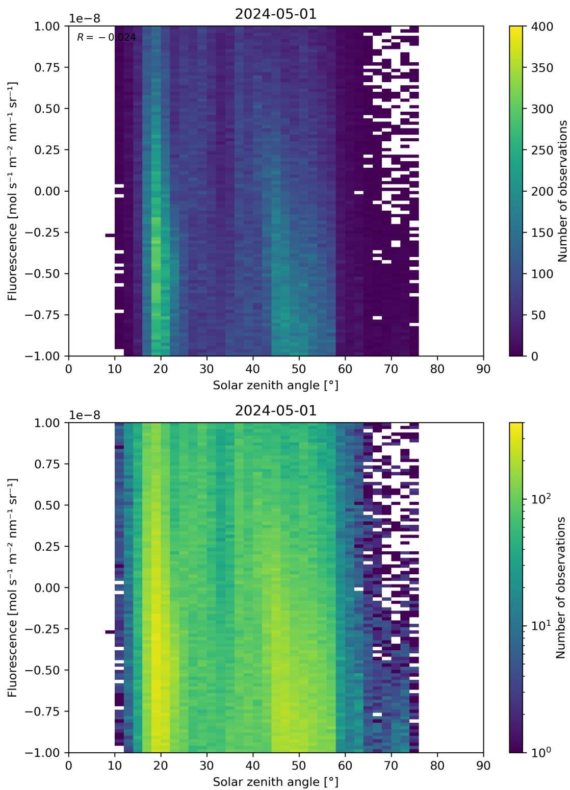
Figure 97: Scatter density plot of “Solar zenith angle” against “Fluorescence” for 2024-04-30 to 2024-05-02.
