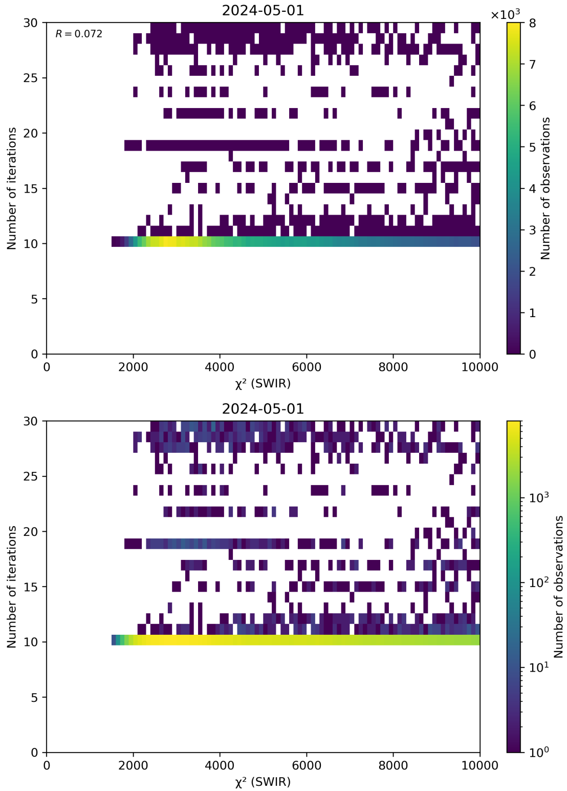
Figure 50: Scatter density plot of “ \chi^2 (SWIR)” against “Number of iterations” for 2024-04-30 to 2024-05-02.
