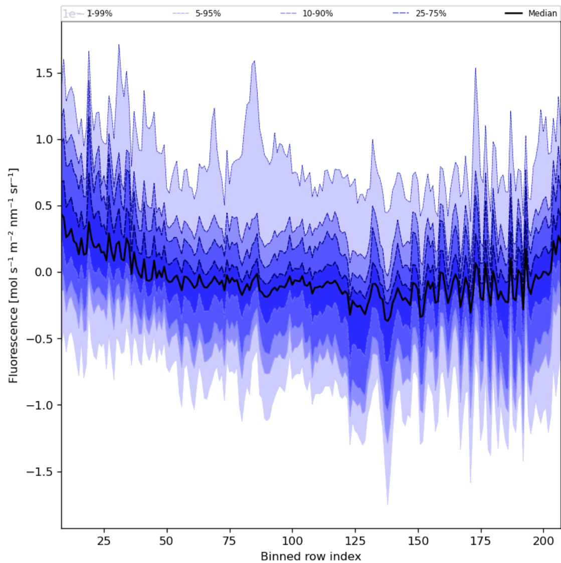
Figure 43: Along track statistics of “Fluorescence” for 2024-04-30 to 2024-05-02
