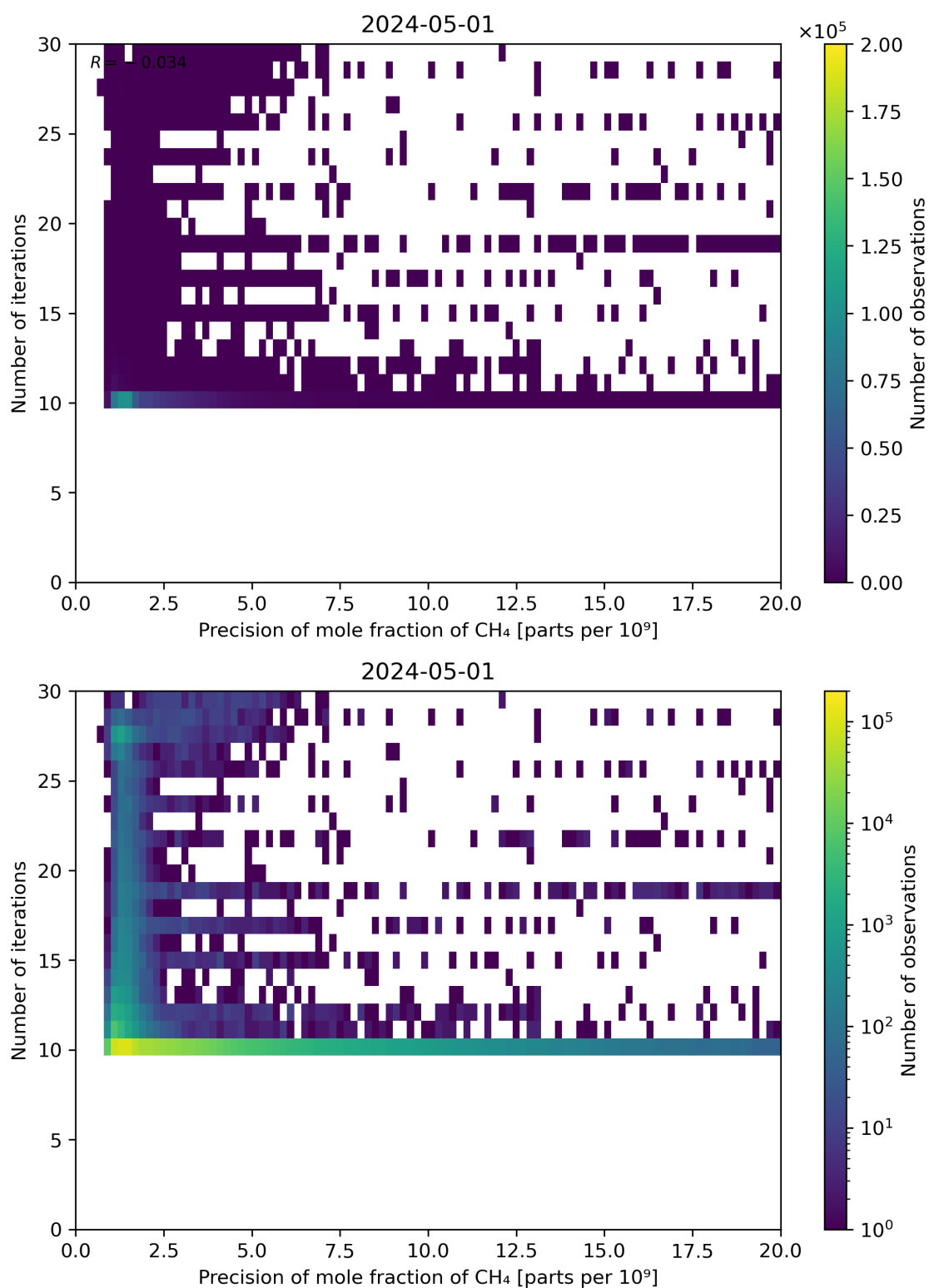
Figure 83: Scatter density plot of “Precision of mole fraction of CH 4 ” against “Number of iterations” for 2024-04-30 to 2024-05-02.
