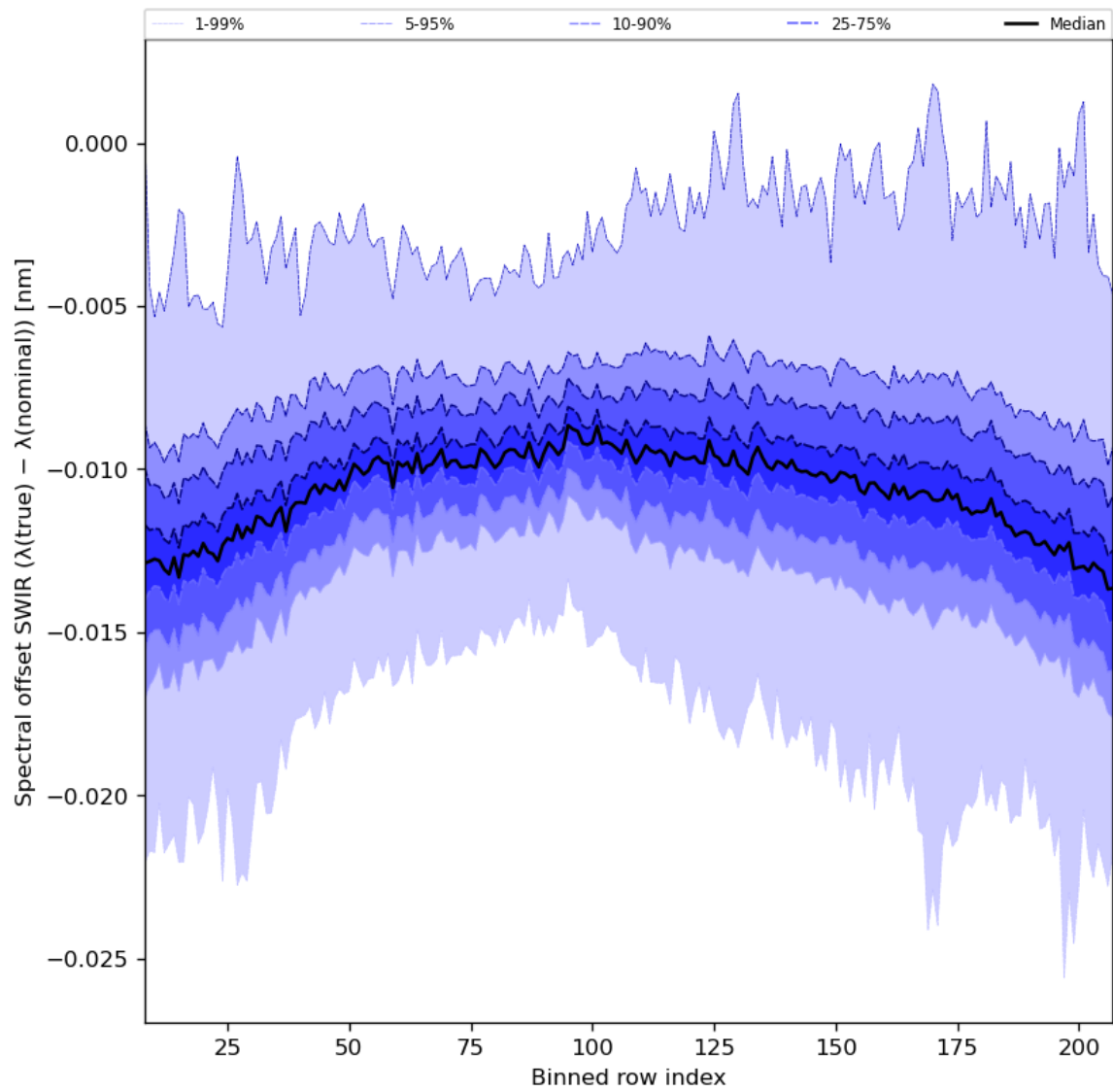
Figure 38: Along track statistics of “Spectral offset SWIR ( \lambda(\text{true}) - \lambda(\text{nominal}) )” for 2024-04-30 to 2024-05-02
