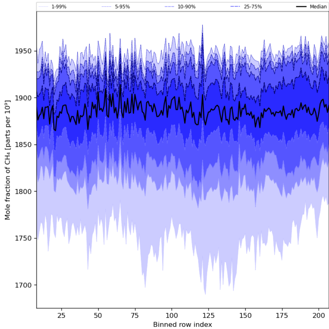
Figure 34: Along track statistics of “Mole fraction of CH 4 ” for 2024-04-30 to 2024-05-02
