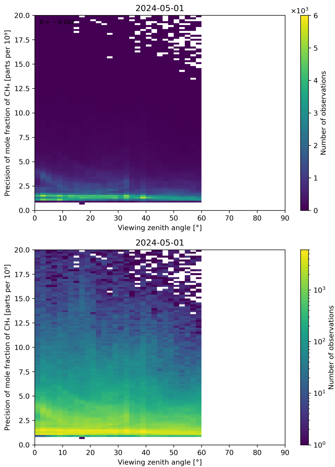
Figure 112: Scatter density plot of “Viewing zenith angle” against “Precision of mole fraction of CH 4 ” for 2024-04-30 to 2024-05-02.
