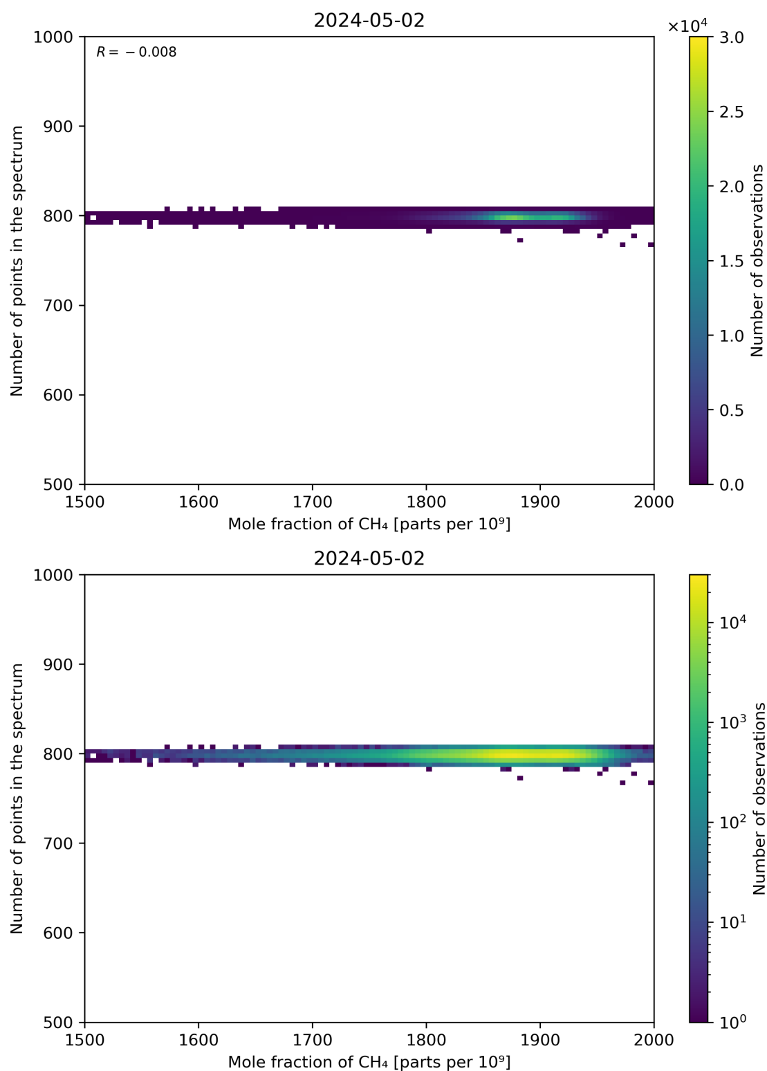
Figure 77: Scatter density plot of “Mole fraction of CH 4 ” against “Number of points in the spectrum” for 2024-05-02 to 2024-05-03.
