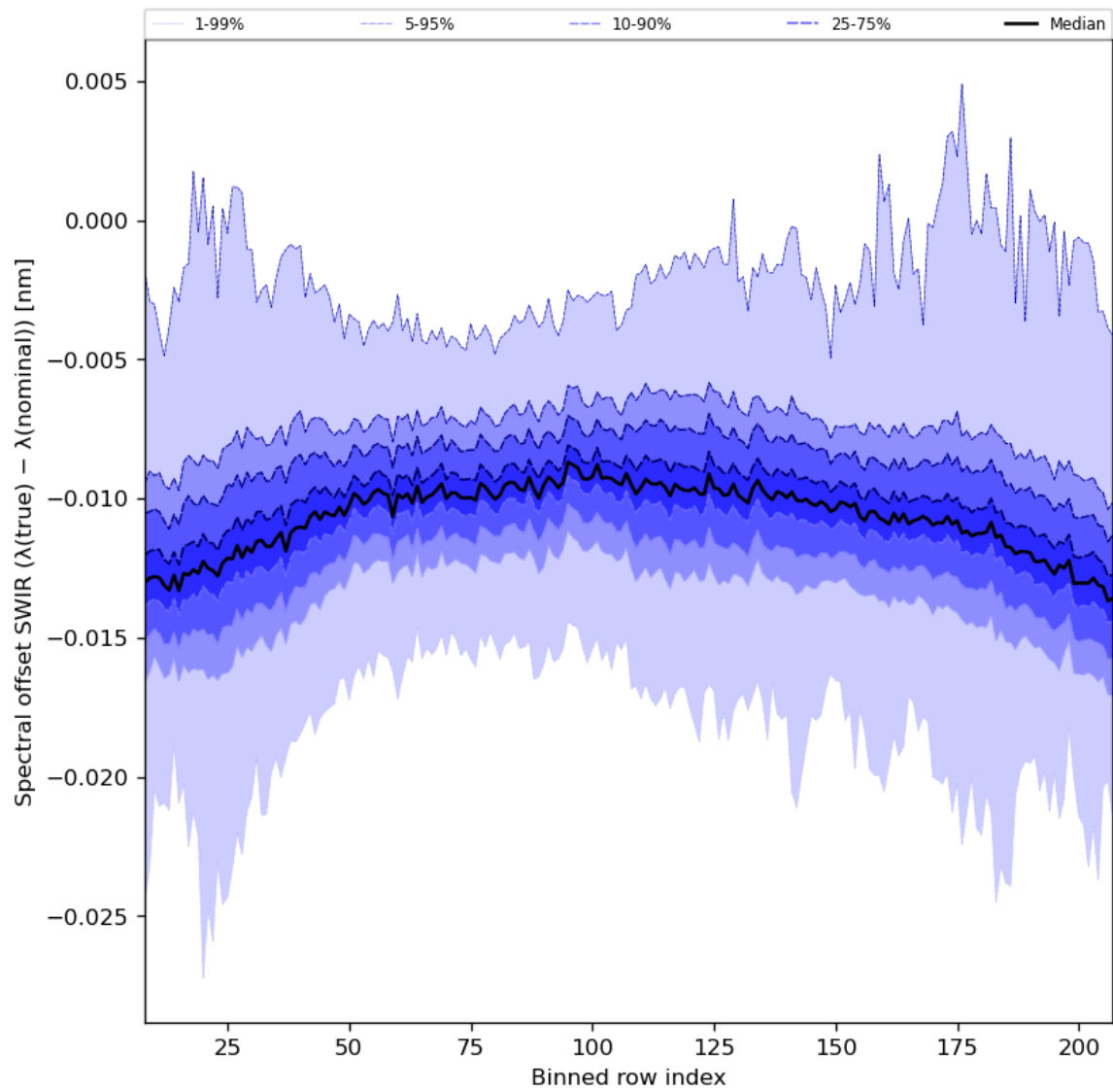
Figure 38: Along track statistics of “Spectral offset SWIR ( \lambda(\text{true}) - \lambda(\text{nominal}) )” for 2024-05-02 to 2024-05-03
