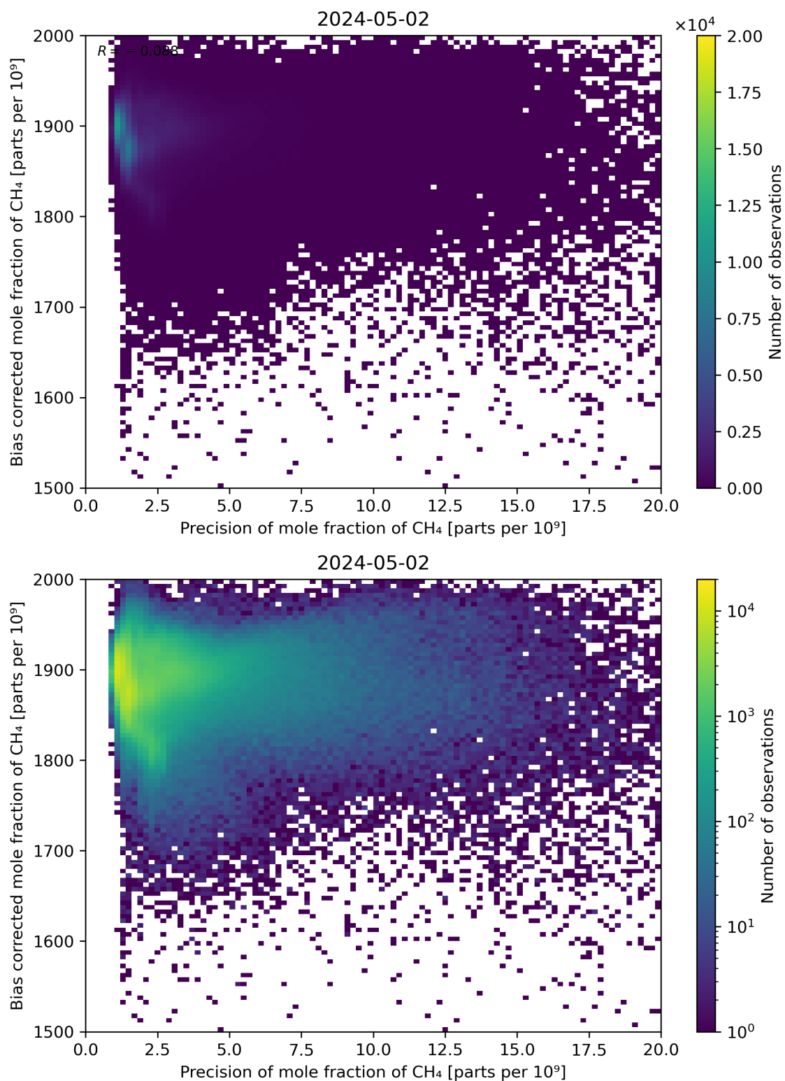
Figure 82: Scatter density plot of “Precision of mole fraction of \text{CH}_4 ” against “Bias corrected mole fraction of \text{CH}_4 ” for 2024-05-02 to 2024-05-03.
