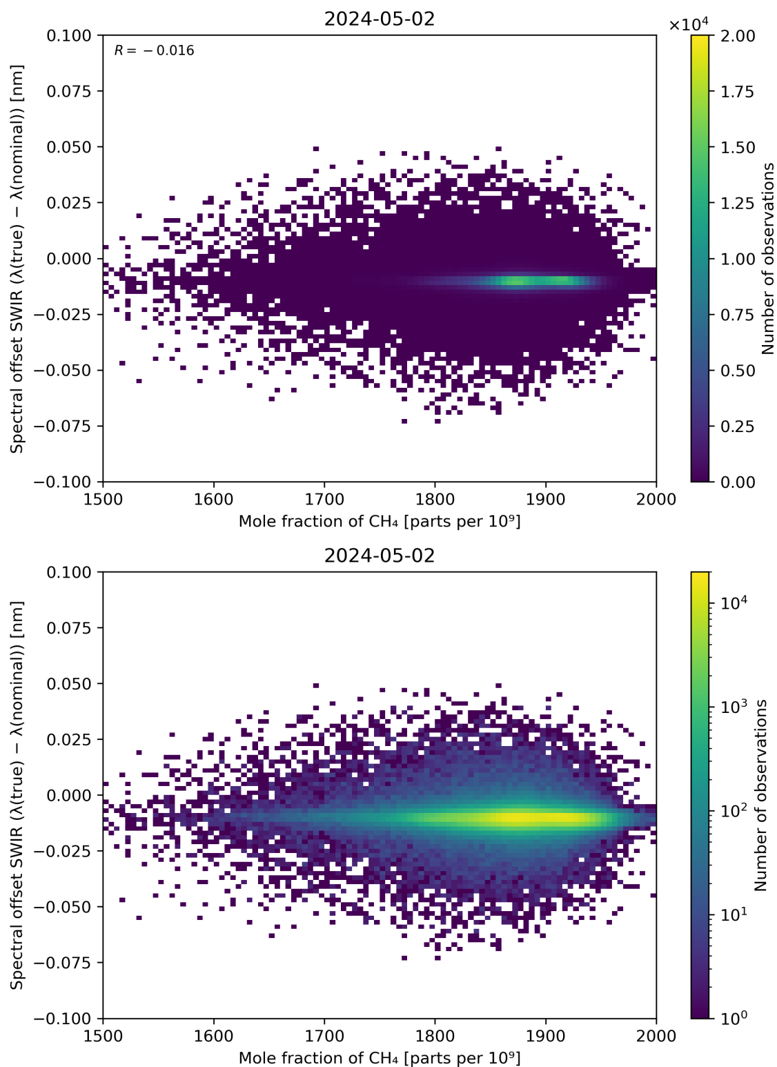
Figure 86: Scatter density plot of “Mole fraction of CH 4 ” against “Spectral offset SWIR ( \lambda(\text{true}) - \lambda(\text{nominal}) )” for 2024-05-02 to 2024-05-03.
