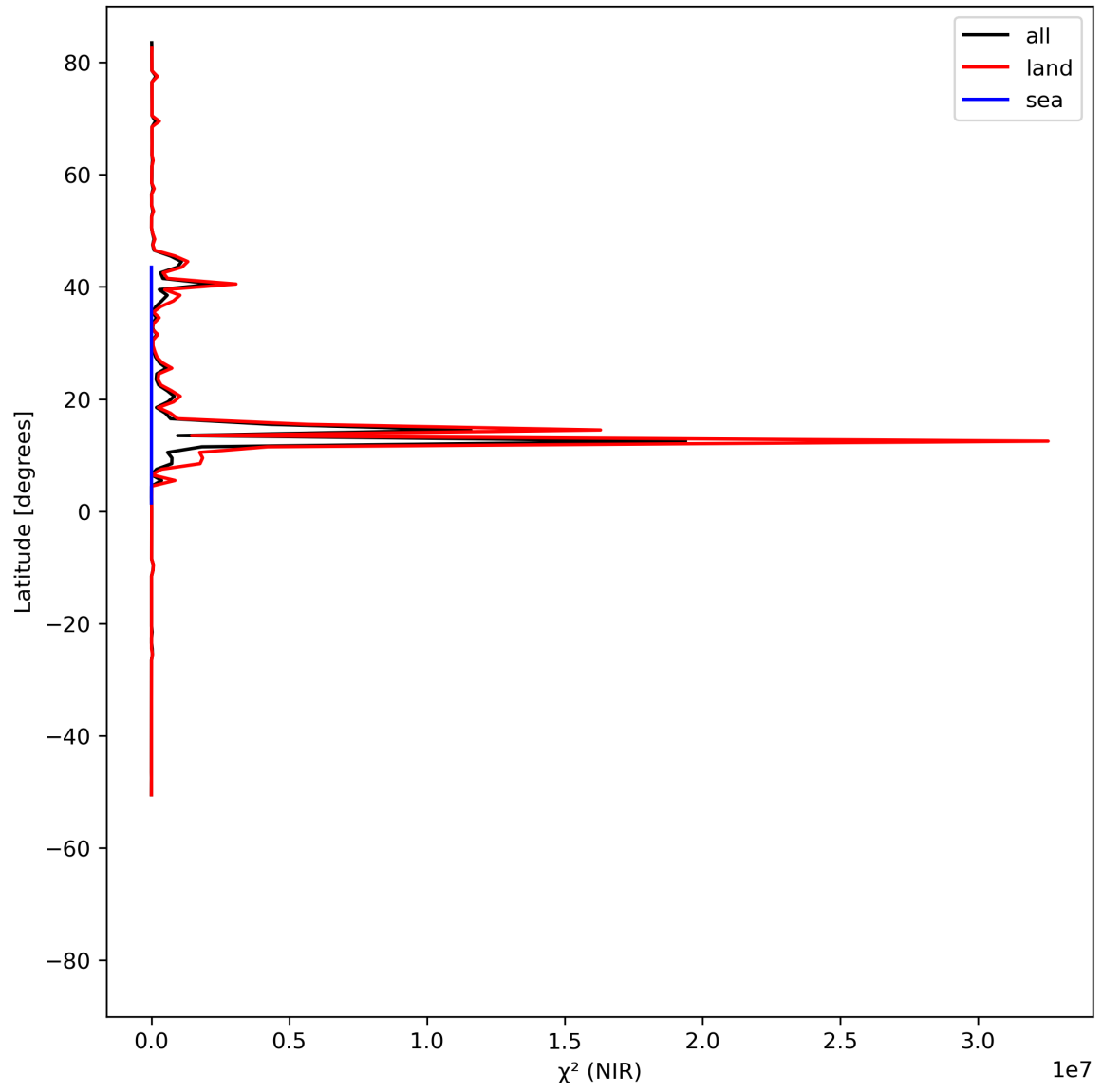
Figure 18: Zonal average of “ \chi^2 (NIR)” for 2024-05-02 to 2024-05-03.
