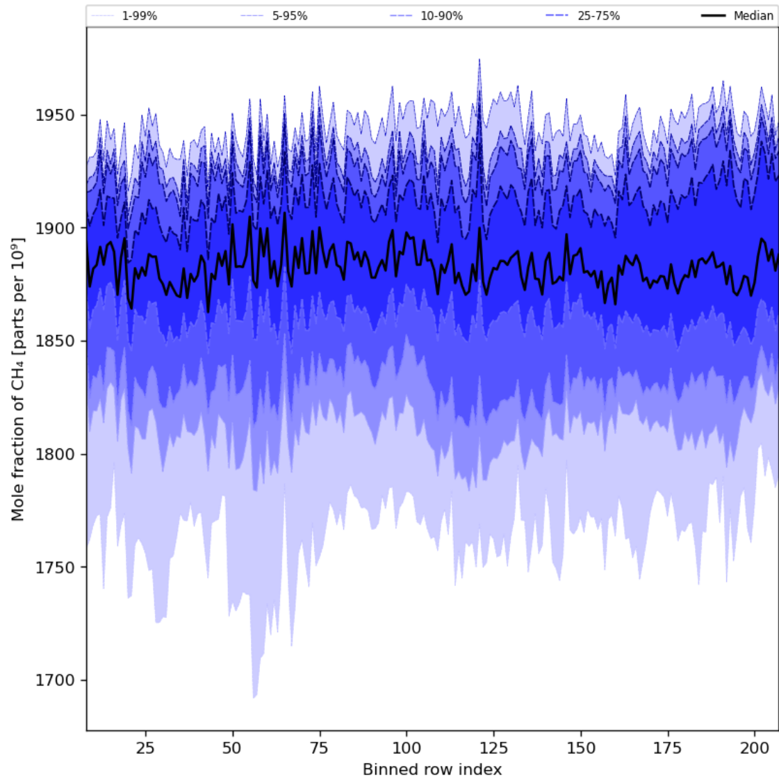
Figure 34: Along track statistics of “Mole fraction of CH 4 ” for 2024-05-02 to 2024-05-03
