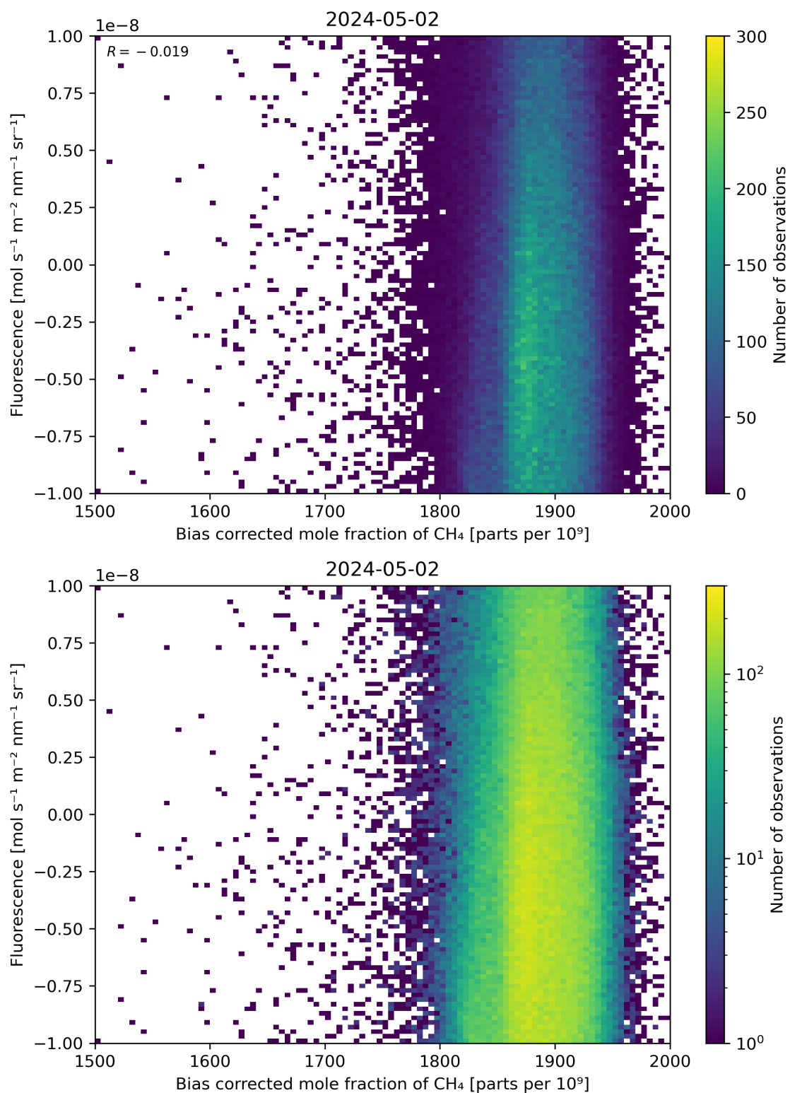
Figure 66: Scatter density plot of “Bias corrected mole fraction of \text{CH}_4 ” against “Fluorescence” for 2024-05-02 to 2024-05-03.
