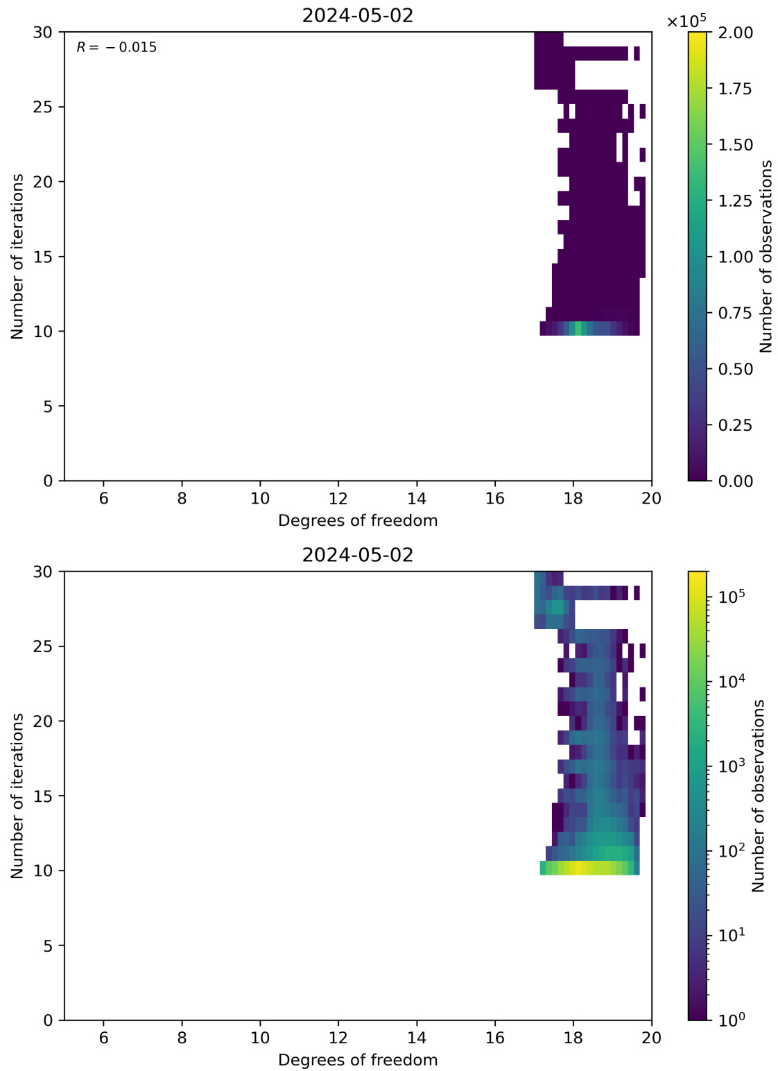
Figure 52: Scatter density plot of “Degrees of freedom” against “Number of iterations” for 2024-05-02 to 2024-05-03.
