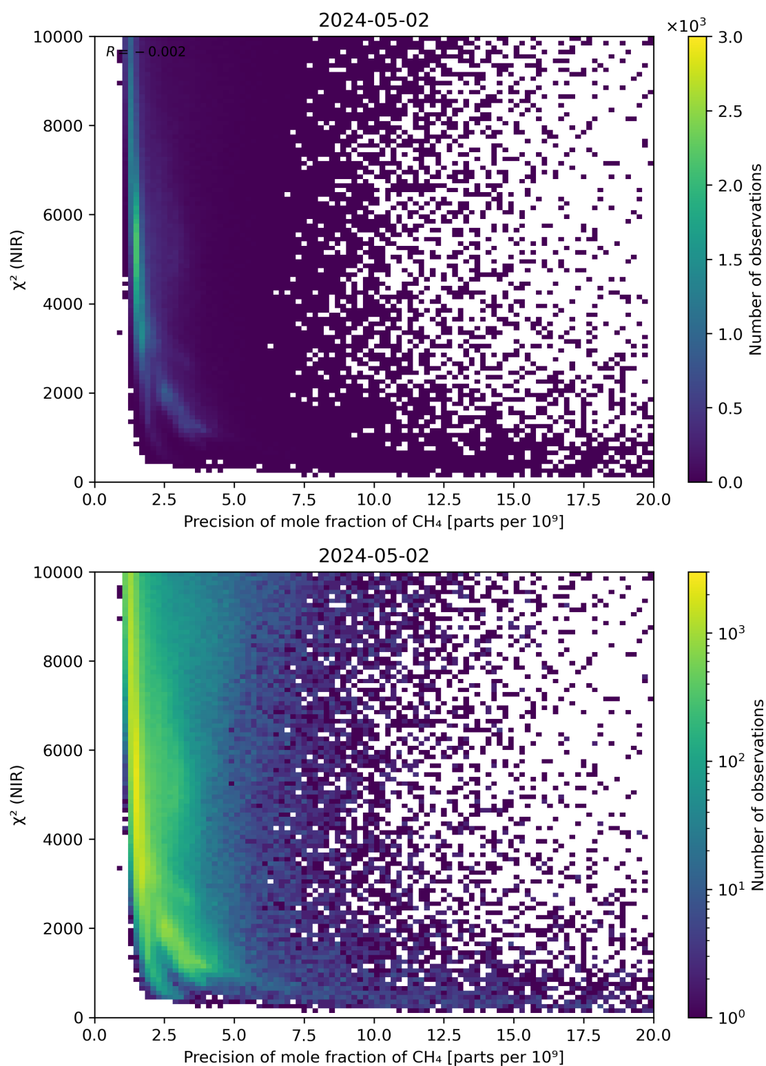
Figure 78: Scatter density plot of “Precision of mole fraction of CH 4 ” against “ \chi^2 (NIR)” for 2024-05-02 to 2024-05-03.
