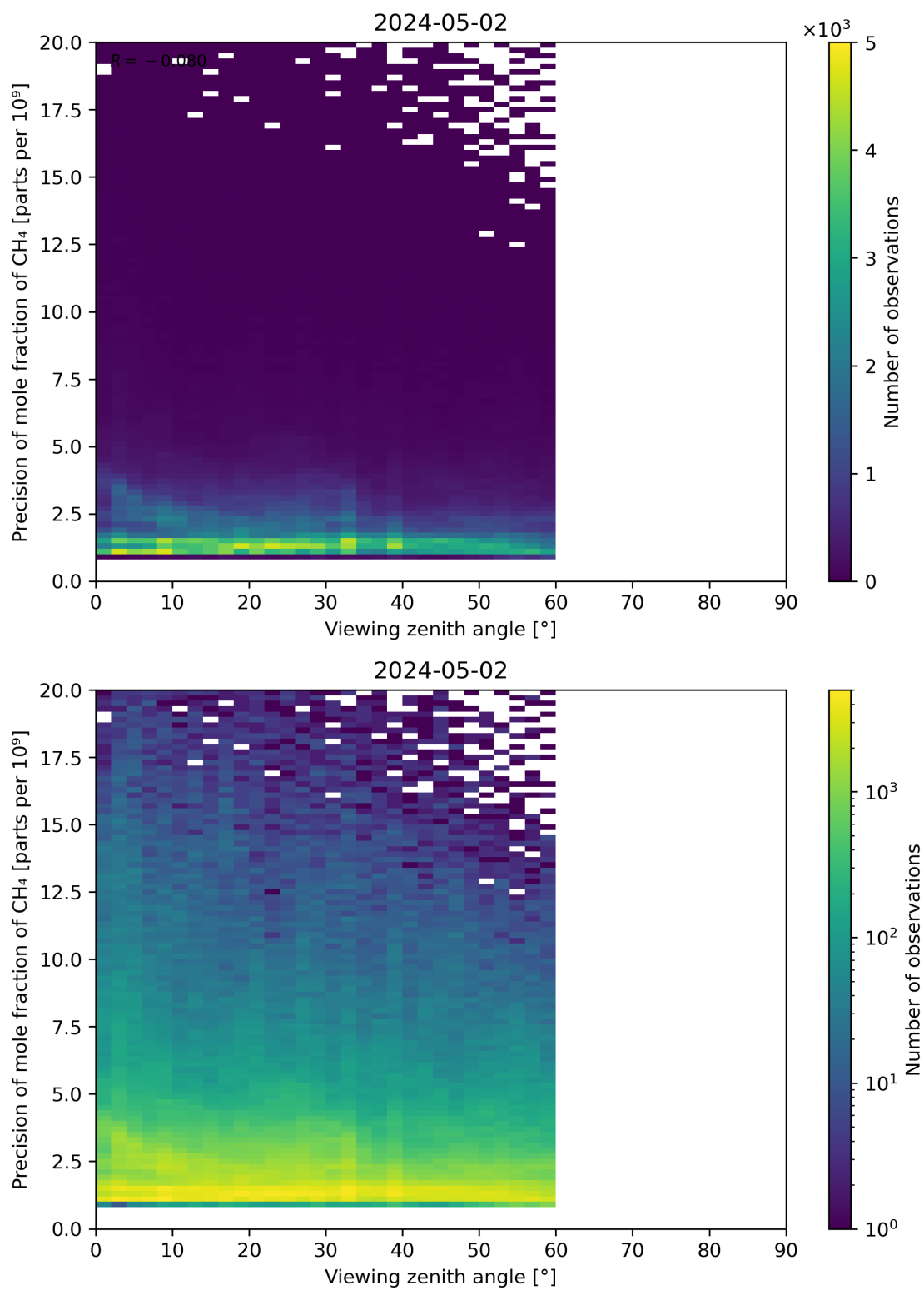
Figure 112: Scatter density plot of “Viewing zenith angle” against “Precision of mole fraction of CH 4 ” for 2024-05-02 to 2024-05-03.
