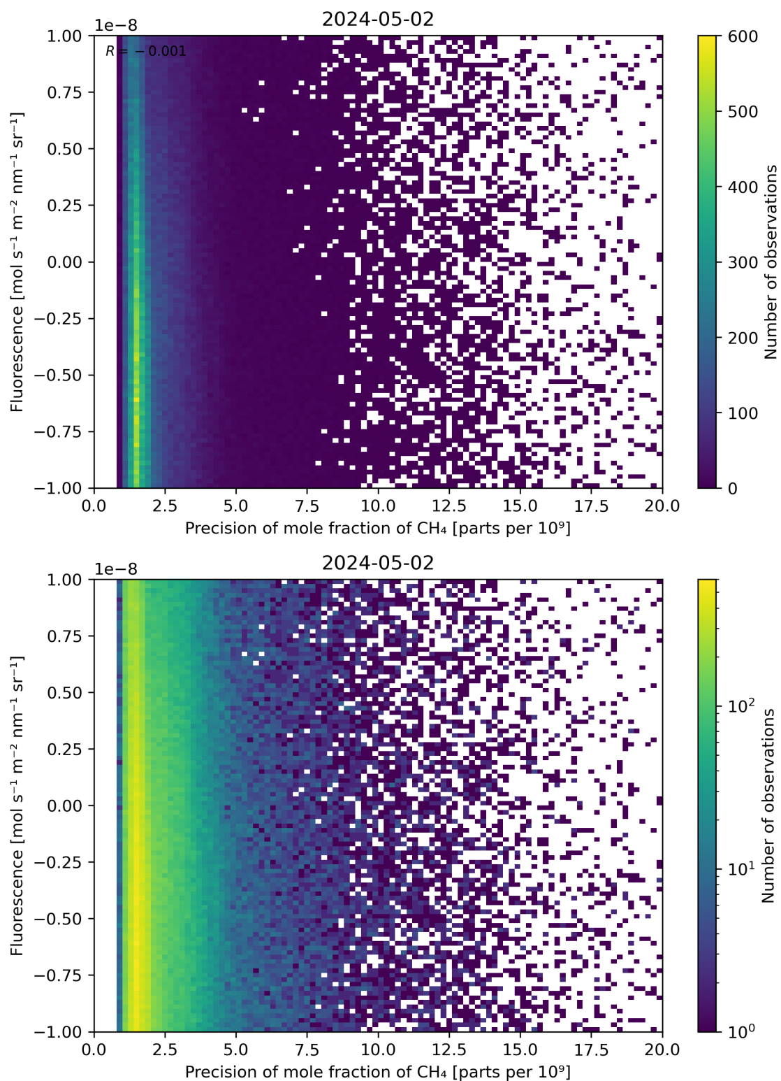
Figure 81: Scatter density plot of “Precision of mole fraction of \text{CH}_4 ” against “Fluorescence” for 2024-05-02 to 2024-05-03.
