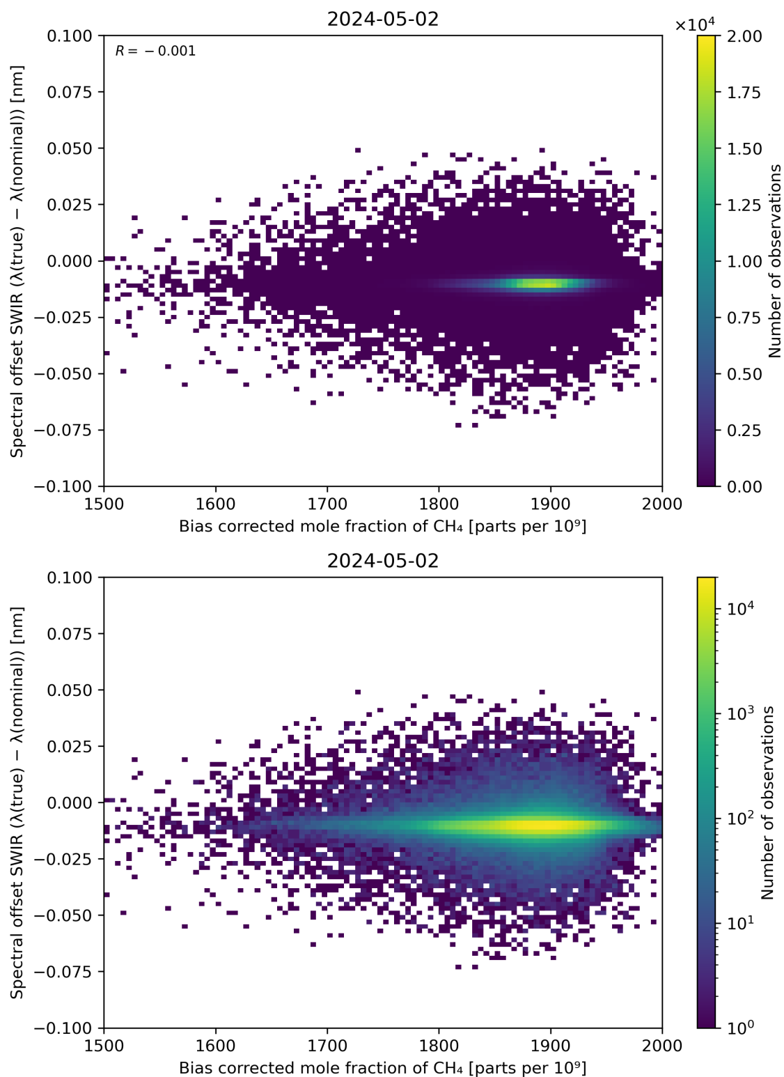
Figure 69: Scatter density plot of “Bias corrected mole fraction of \text{CH}_4 ” against “Spectral offset SWIR ( \lambda(\text{true}) - \lambda(\text{nominal}) )” for 2024-05-02 to 2024-05-03.
