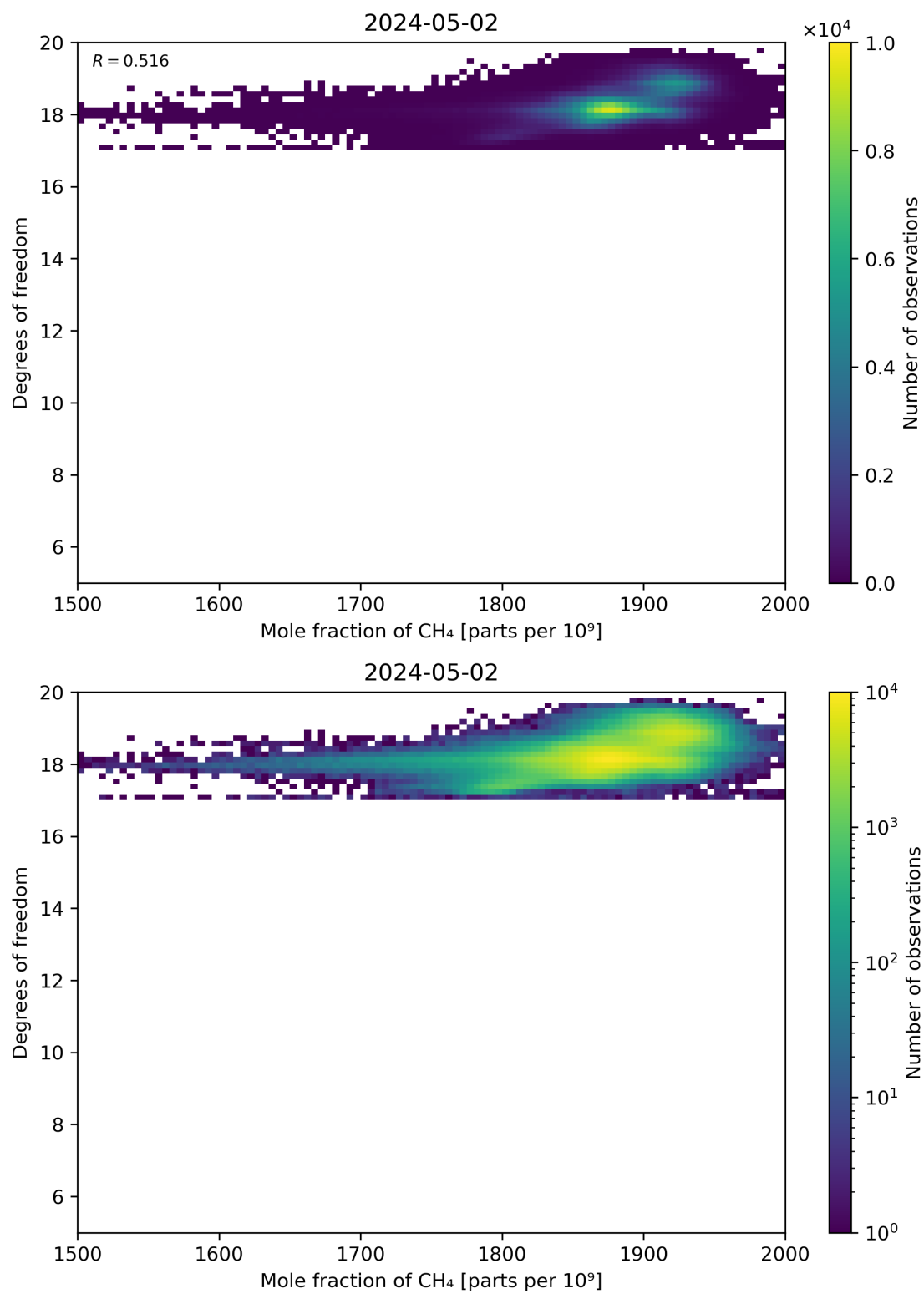
Figure 72: Scatter density plot of “Mole fraction of CH 4 ” against “Degrees of freedom” for 2024-05-02 to 2024-05-03.
