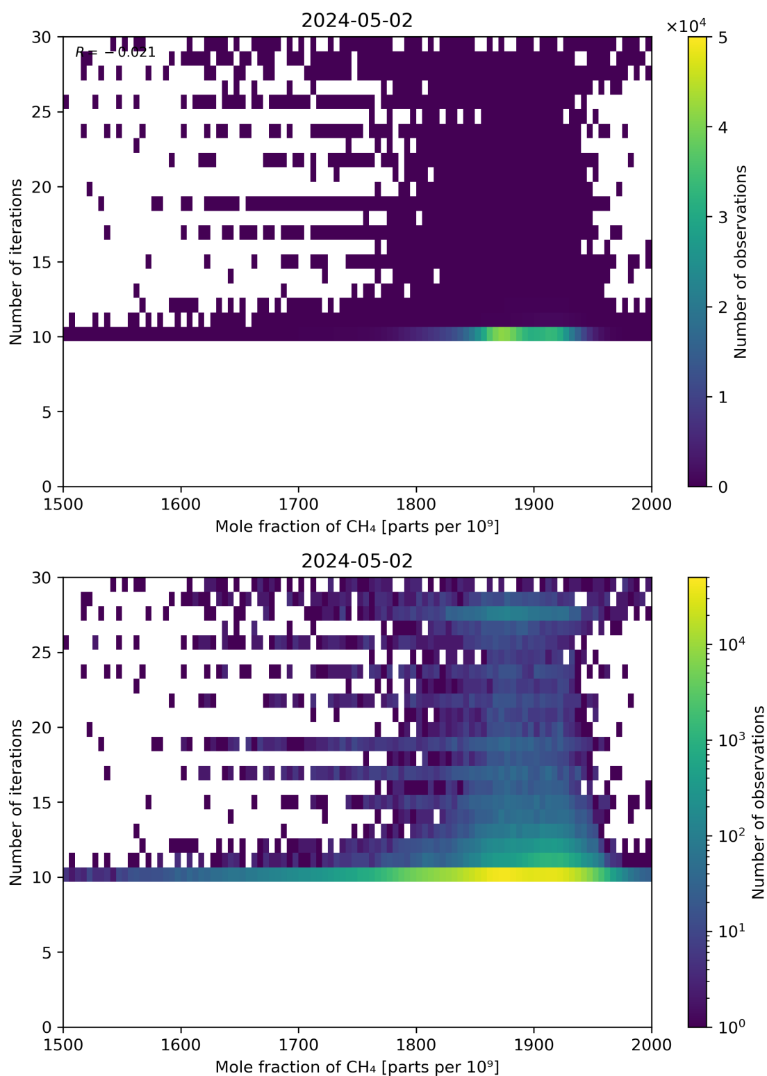
Figure 76: Scatter density plot of “Mole fraction of CH 4 ” against “Number of iterations” for 2024-05-02 to 2024-05-03.
