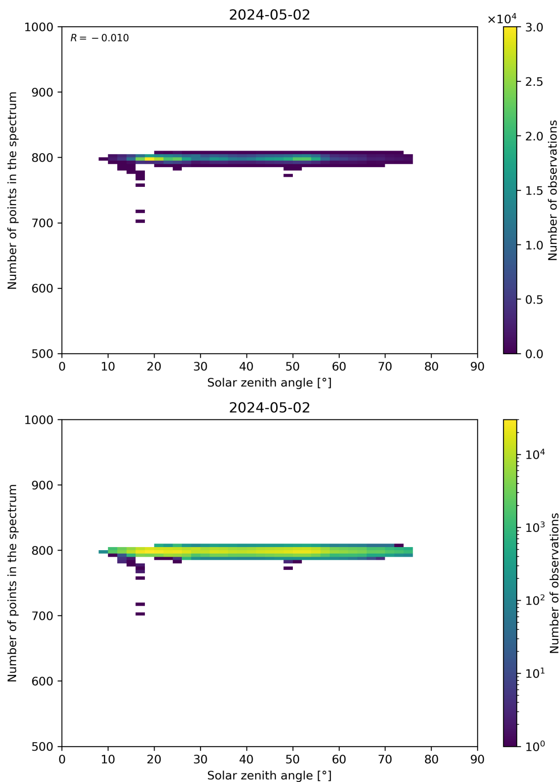
Figure 103: Scatter density plot of “Solar zenith angle” against “Number of points in the spectrum” for 2024-05-02 to 2024-05-03.
