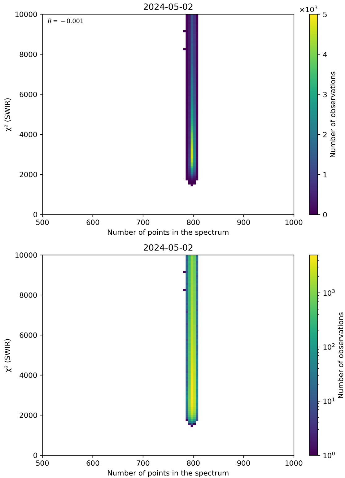
Figure 89: Scatter density plot of “Number of points in the spectrum” against “ \chi^2 (SWIR)” for 2024-05-02 to 2024-05-03.
