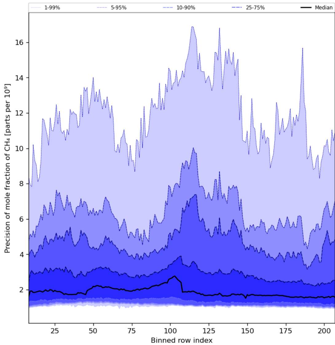
Figure 35: Along track statistics of “Precision of mole fraction of CH 4 ” for 2024-05-02 to 2024-05-03
