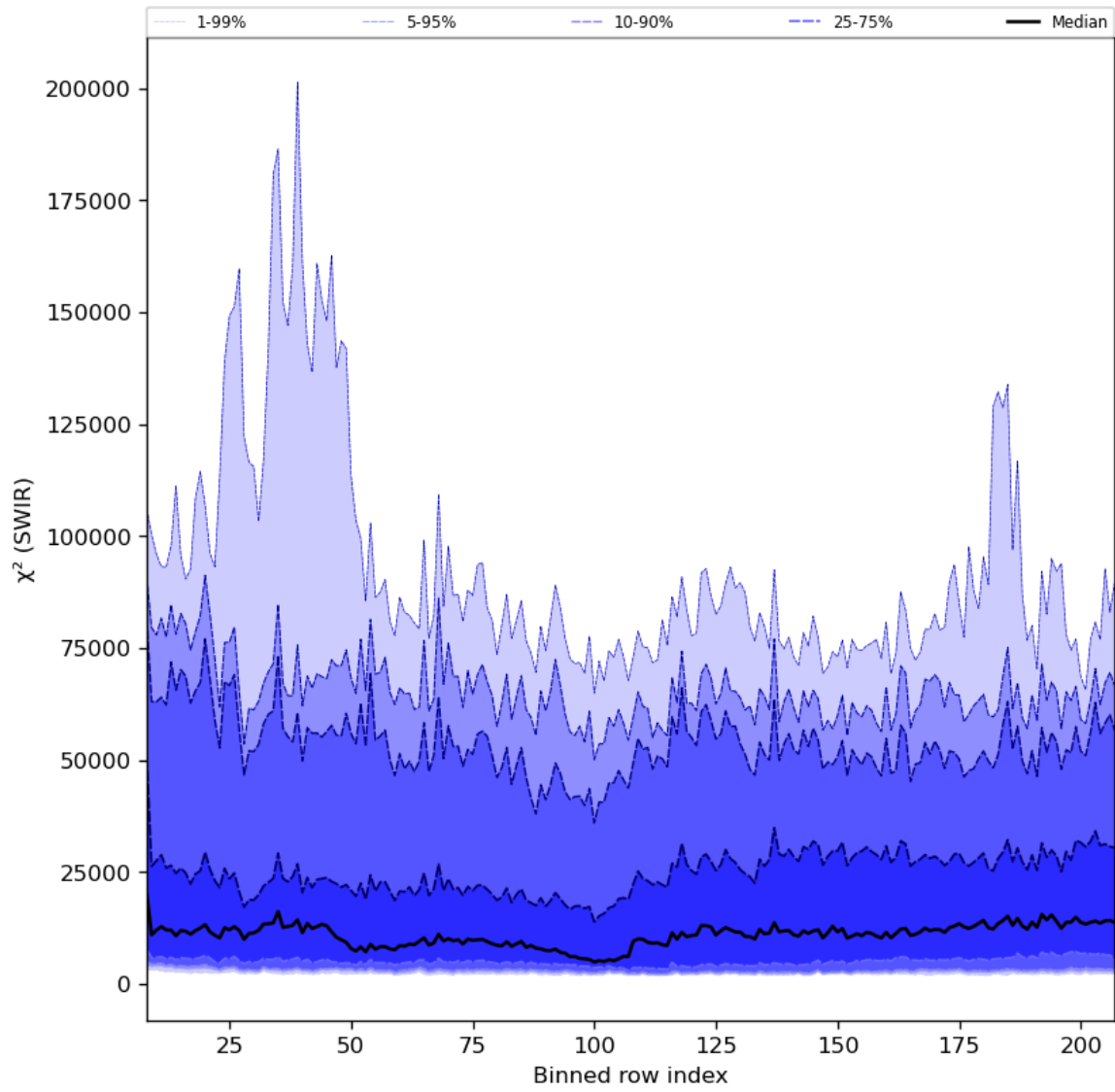
Figure 39: Along track statistics of “ \chi^2 (SWIR)” for 2024-05-02 to 2024-05-03
