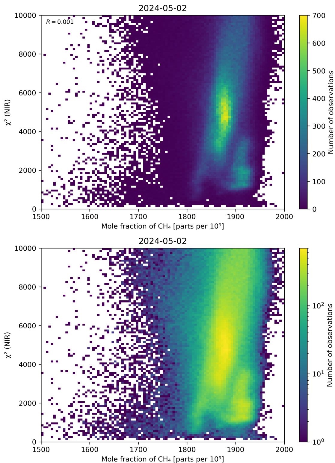
Figure 70: Scatter density plot of “Mole fraction of CH 4 ” against “ \chi^2 (NIR)” for 2024-05-02 to 2024-05-03.
