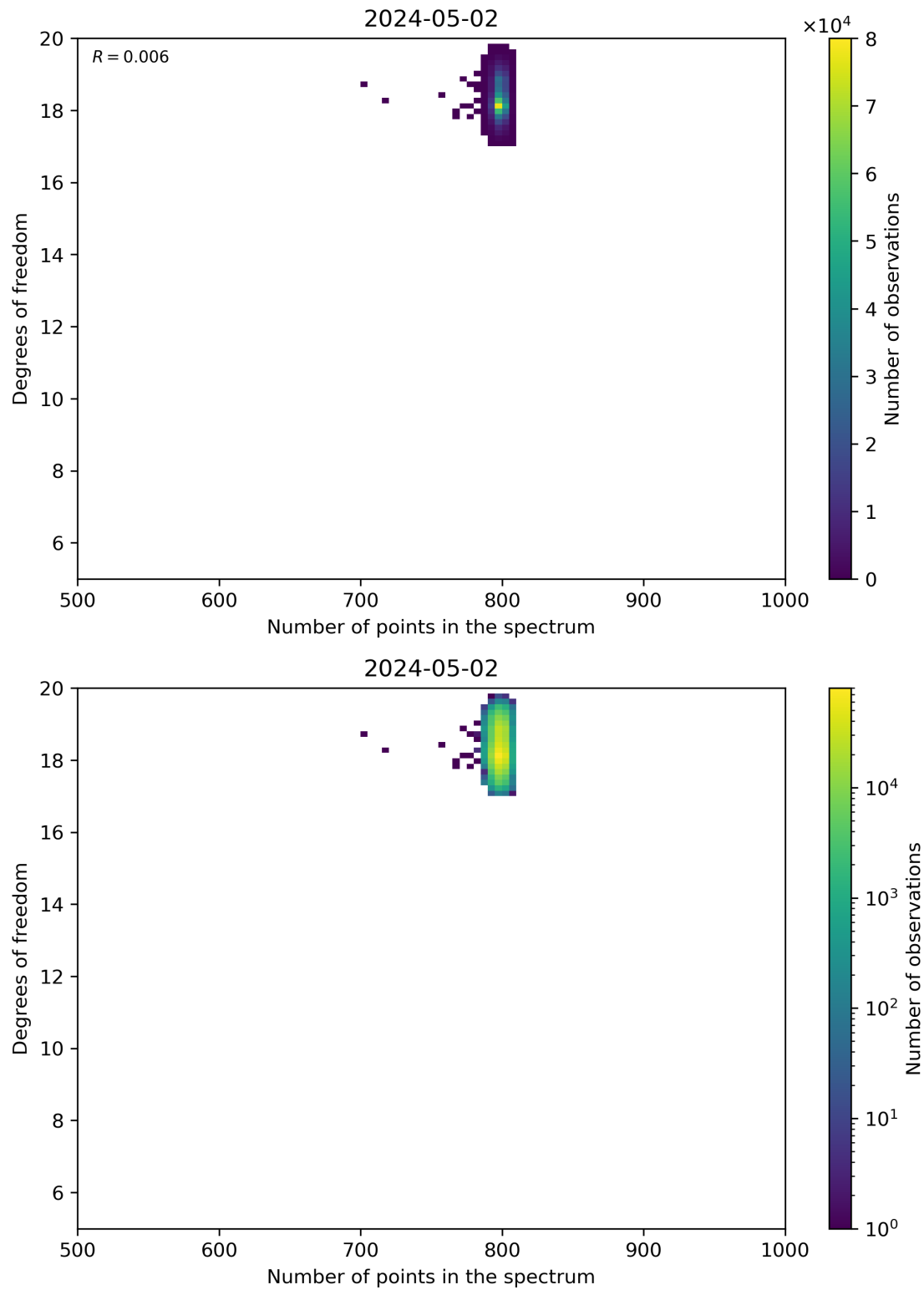
Figure 90: Scatter density plot of “Number of points in the spectrum” against “Degrees of freedom” for 2024-05-02 to 2024-05-03.
