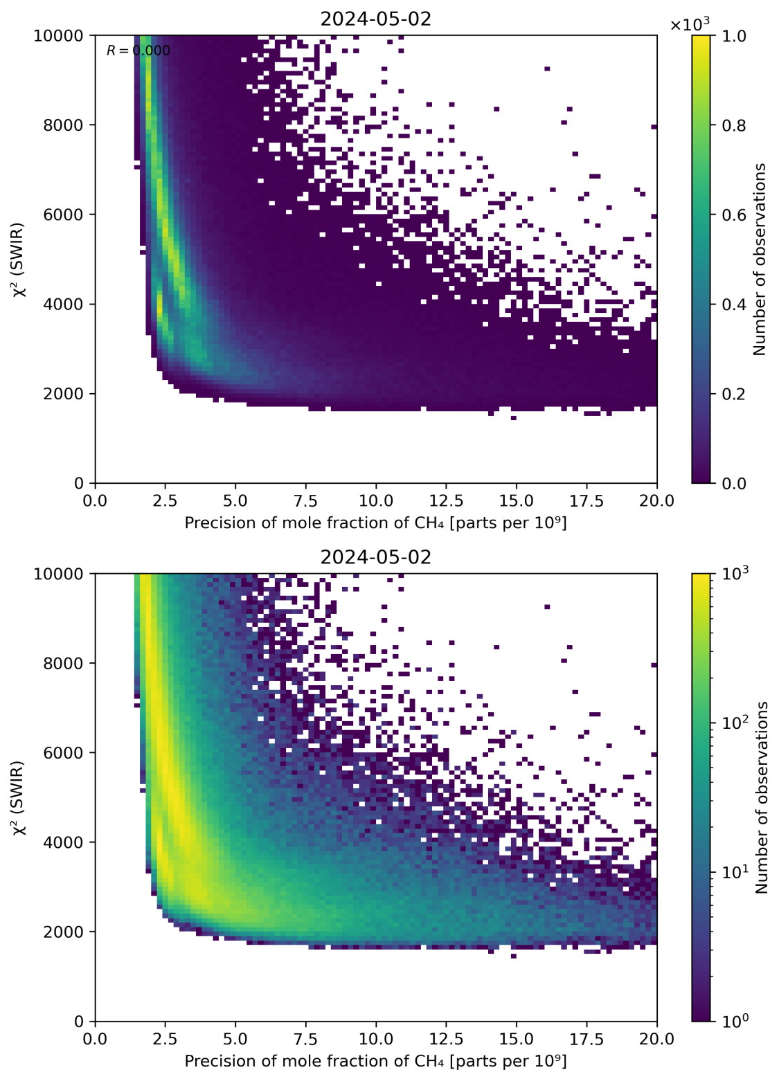
Figure 79: Scatter density plot of “Precision of mole fraction of \text{CH}_4 ” against “ \chi^2 (SWIR)” for 2024-05-02 to 2024-05-03.
