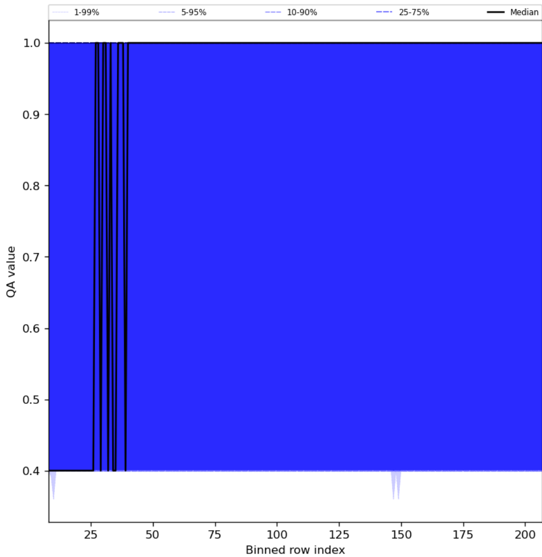
Figure 33: Along track statistics of “QA value” for 2024-05-02 to 2024-05-03
