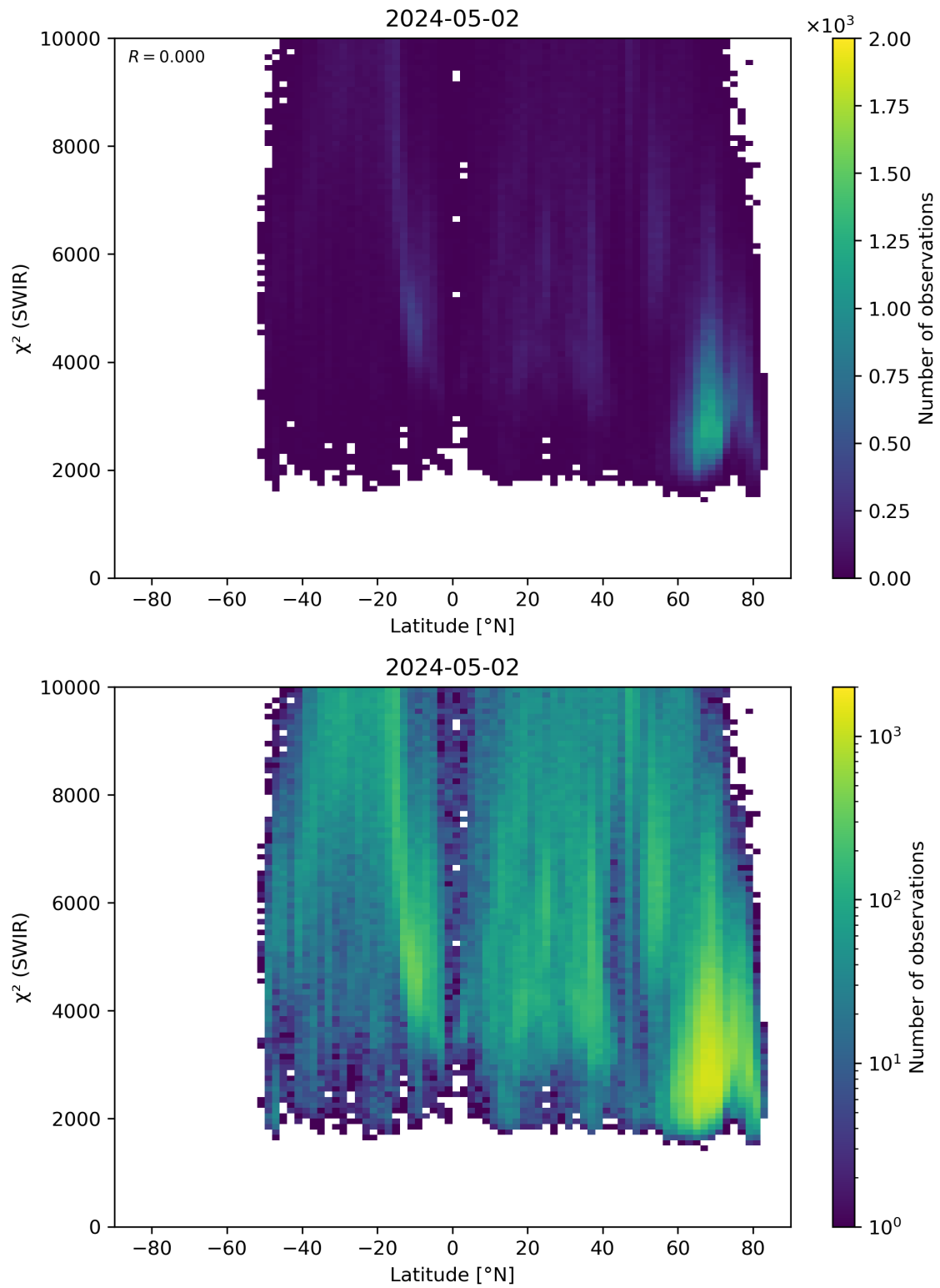
Figure 54: Scatter density plot of “Latitude” against “ \chi^2 (SWIR)” for 2024-05-02 to 2024-05-03.
