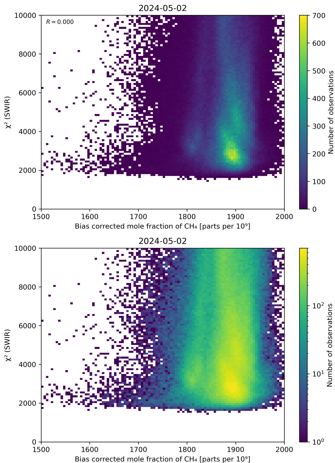
Figure 64: Scatter density plot of “Bias corrected mole fraction of CH 4 ” against “ \chi^2 (SWIR)” for 2024-05-02 to 2024-05-03.
