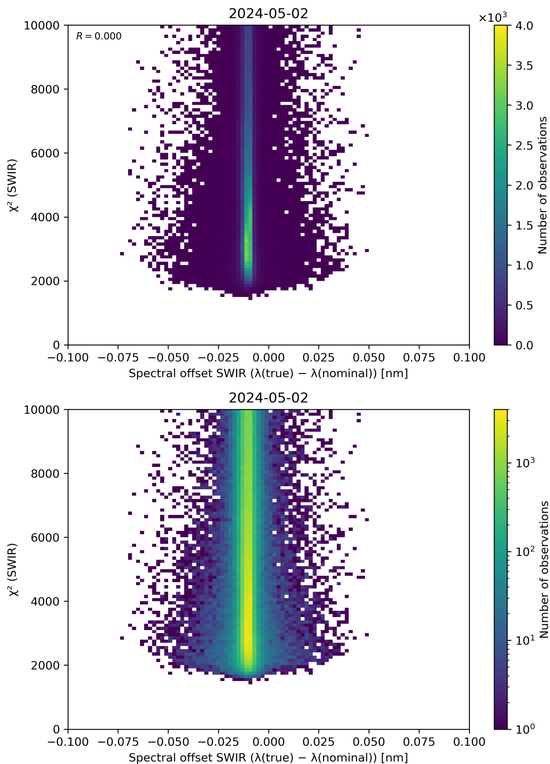
Figure 118: Scatter density plot of “Spectral offset SWIR ( \lambda(\text{true}) - \lambda(\text{nominal}) )” against “ \chi^2 (SWIR)” for 2024-05-02 to 2024-05-03.
