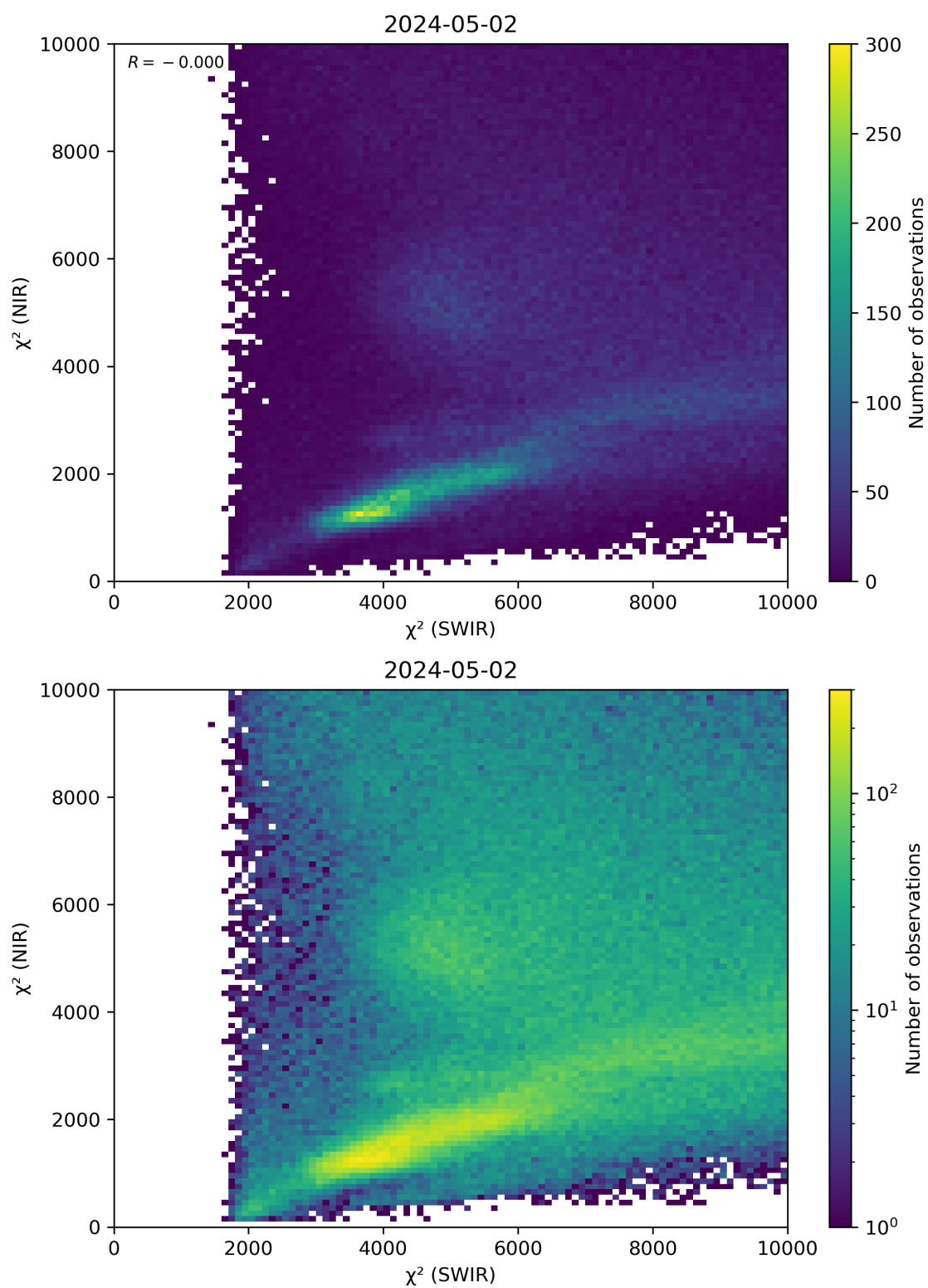
Figure 47: Scatter density plot of “ \chi^2 (SWIR)” against “ \chi^2 (NIR)” for 2024-05-02 to 2024-05-03.
