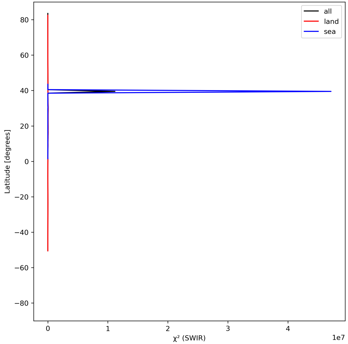
Figure 17: Zonal average of “ \chi^2 (SWIR)” for 2024-05-02 to 2024-05-03.
