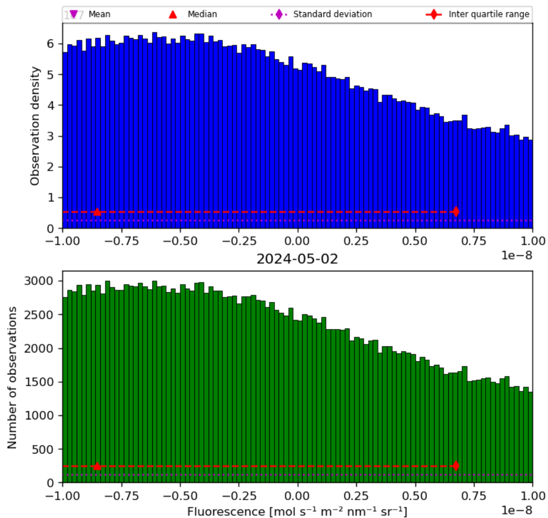
Figure 32: Histogram of “Fluorescence” for 2024-05-02 to 2024-05-03
