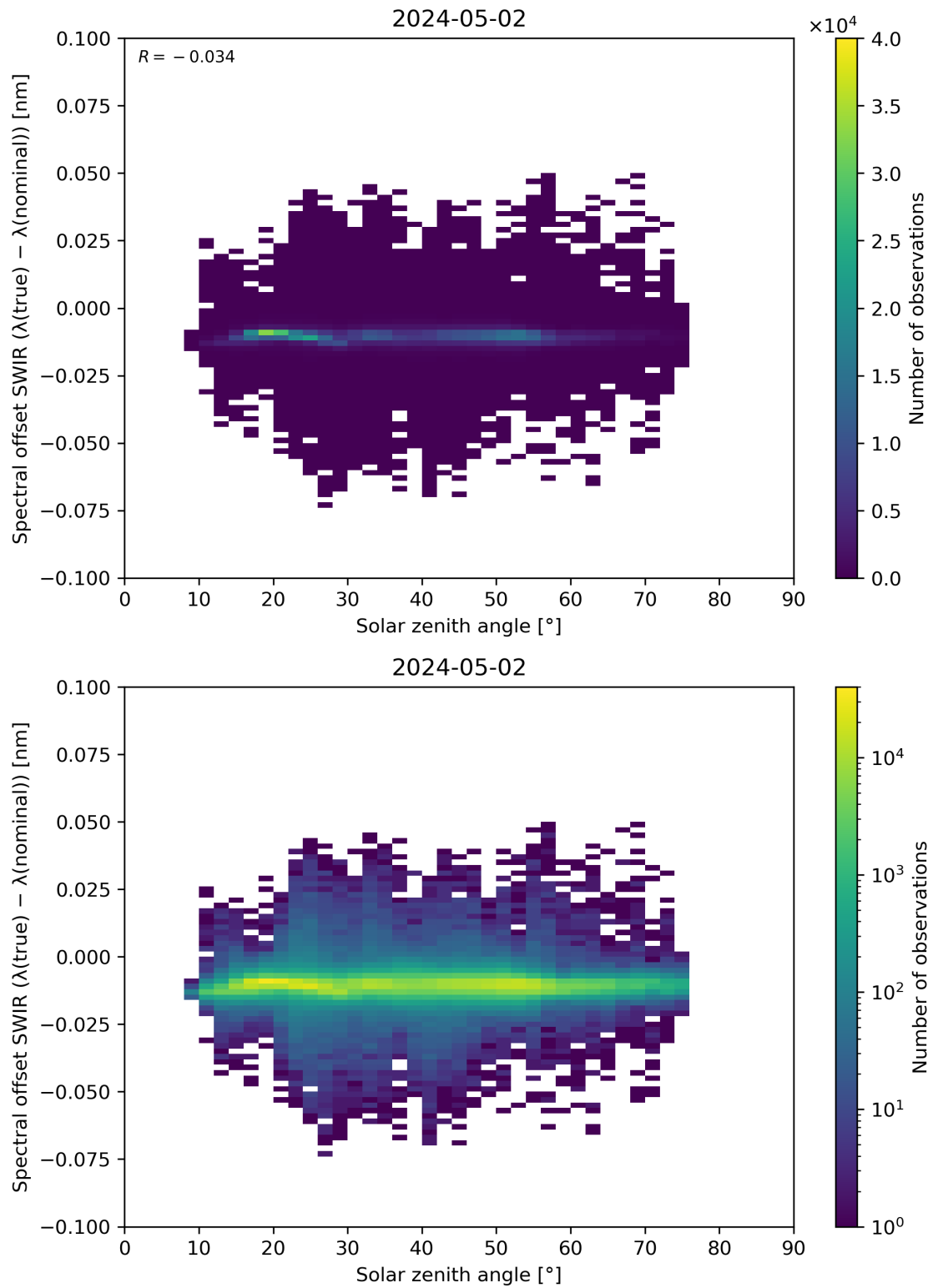
Figure 104: Scatter density plot of “Solar zenith angle” against “Spectral offset SWIR ( \lambda(\text{true}) - \lambda(\text{nominal}) )” for 2024-05-02 to 2024-05-03.
