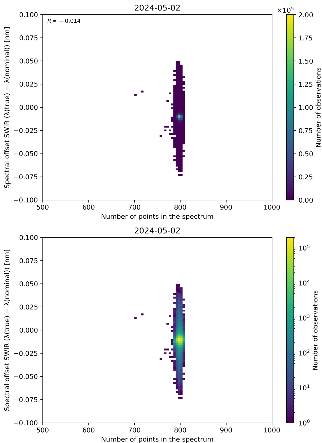
Figure 93: Scatter density plot of “Number of points in the spectrum” against “Spectral offset SWIR ( \lambda(\text{true}) - \lambda(\text{nominal}) )” for 2024-05-02 to 2024-05-03.
