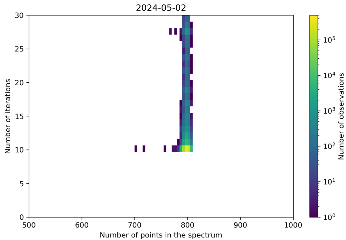
Figure 92: Scatter density plot of “Number of points in the spectrum” against “Number of iterations” for 2024-05-02 to 2024-05-03.
