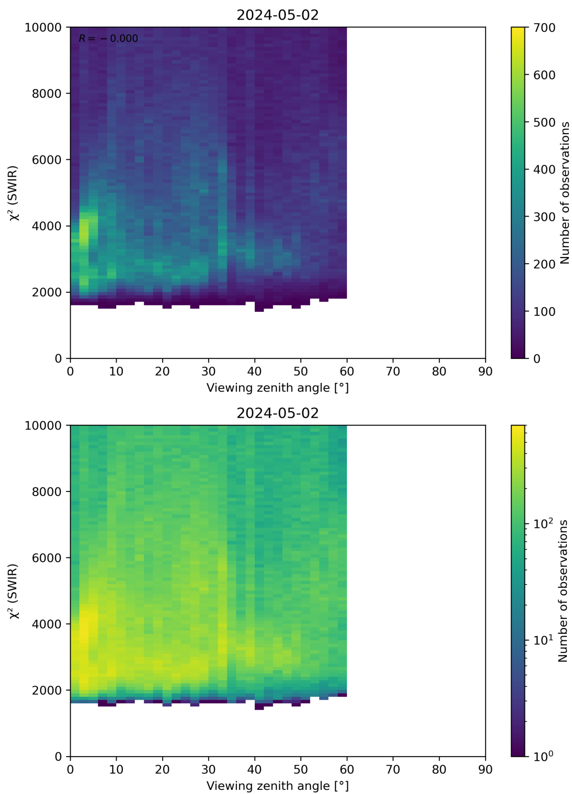
Figure 106: Scatter density plot of “Viewing zenith angle” against “ \chi^2 (SWIR)” for 2024-05-02 to 2024-05-03.
