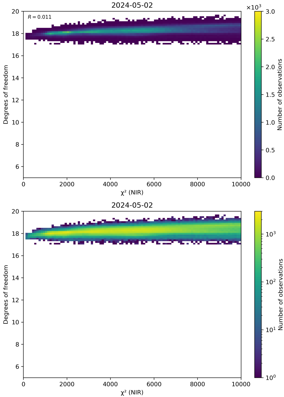
Figure 44: Scatter density plot of “ \chi^2 (NIR)” against “Degrees of freedom” for 2024-05-02 to 2024-05-03.
