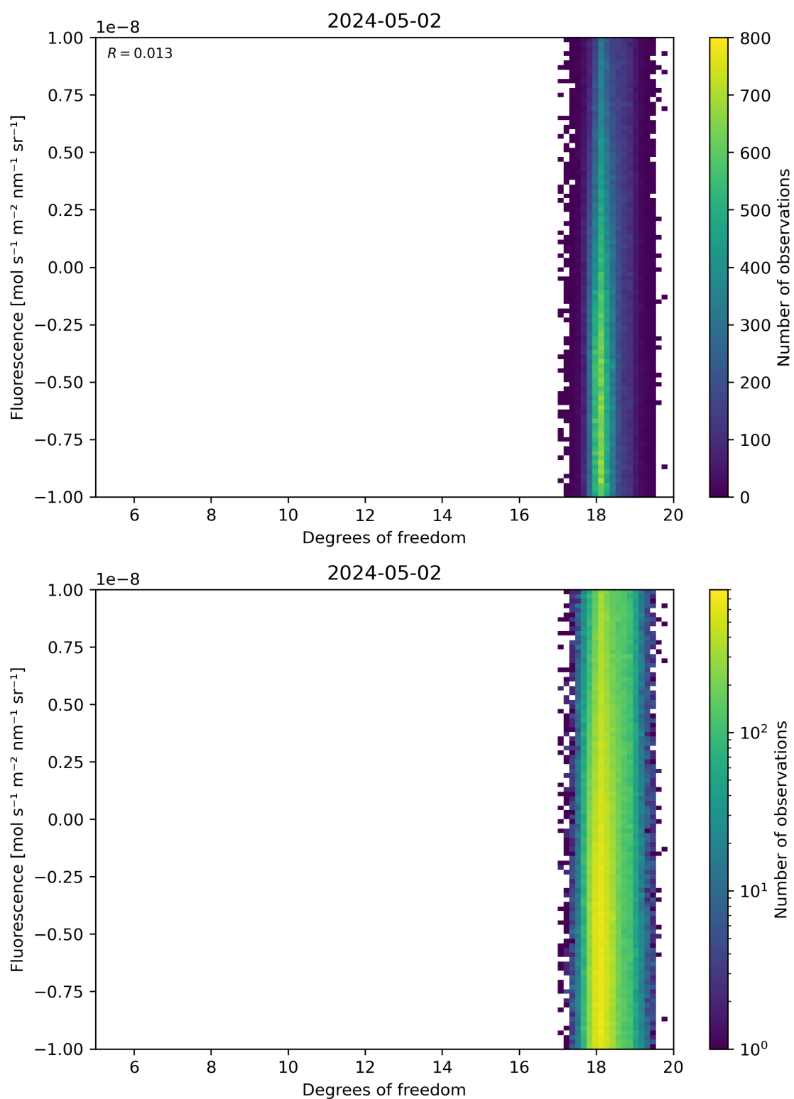
Figure 51: Scatter density plot of “Degrees of freedom” against “Fluorescence” for 2024-05-02 to 2024-05-03.
