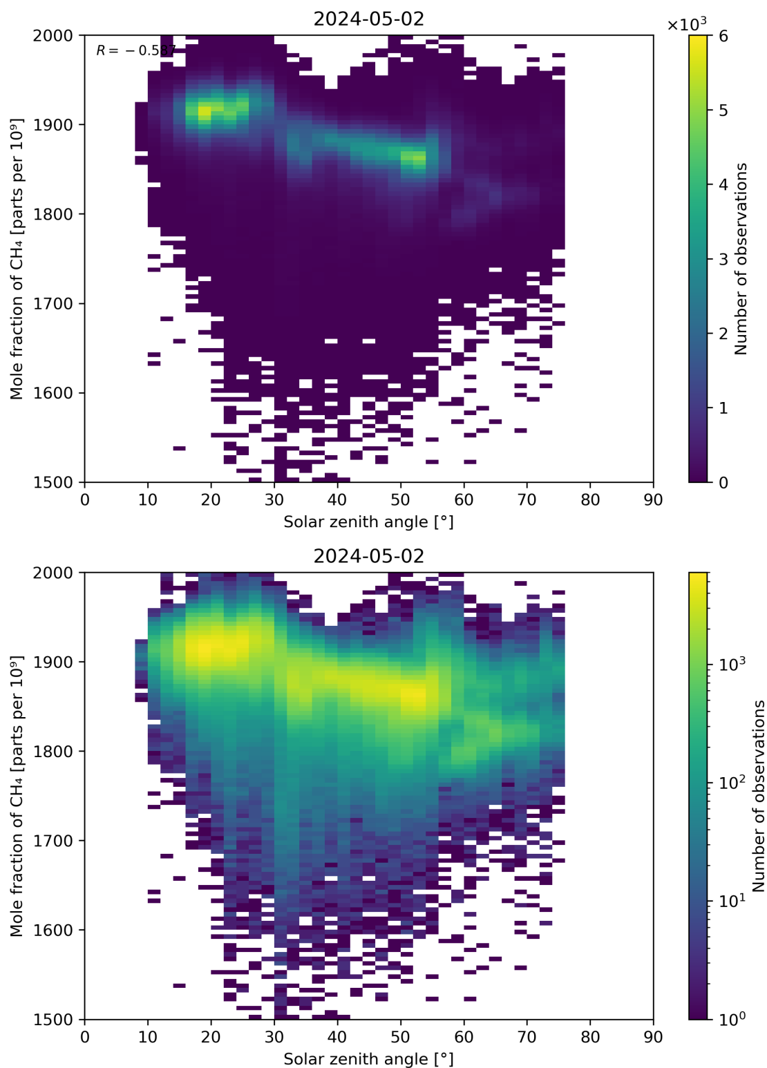
Figure 99: Scatter density plot of “Solar zenith angle” against “Mole fraction of CH 4 ” for 2024-05-02 to 2024-05-03.
