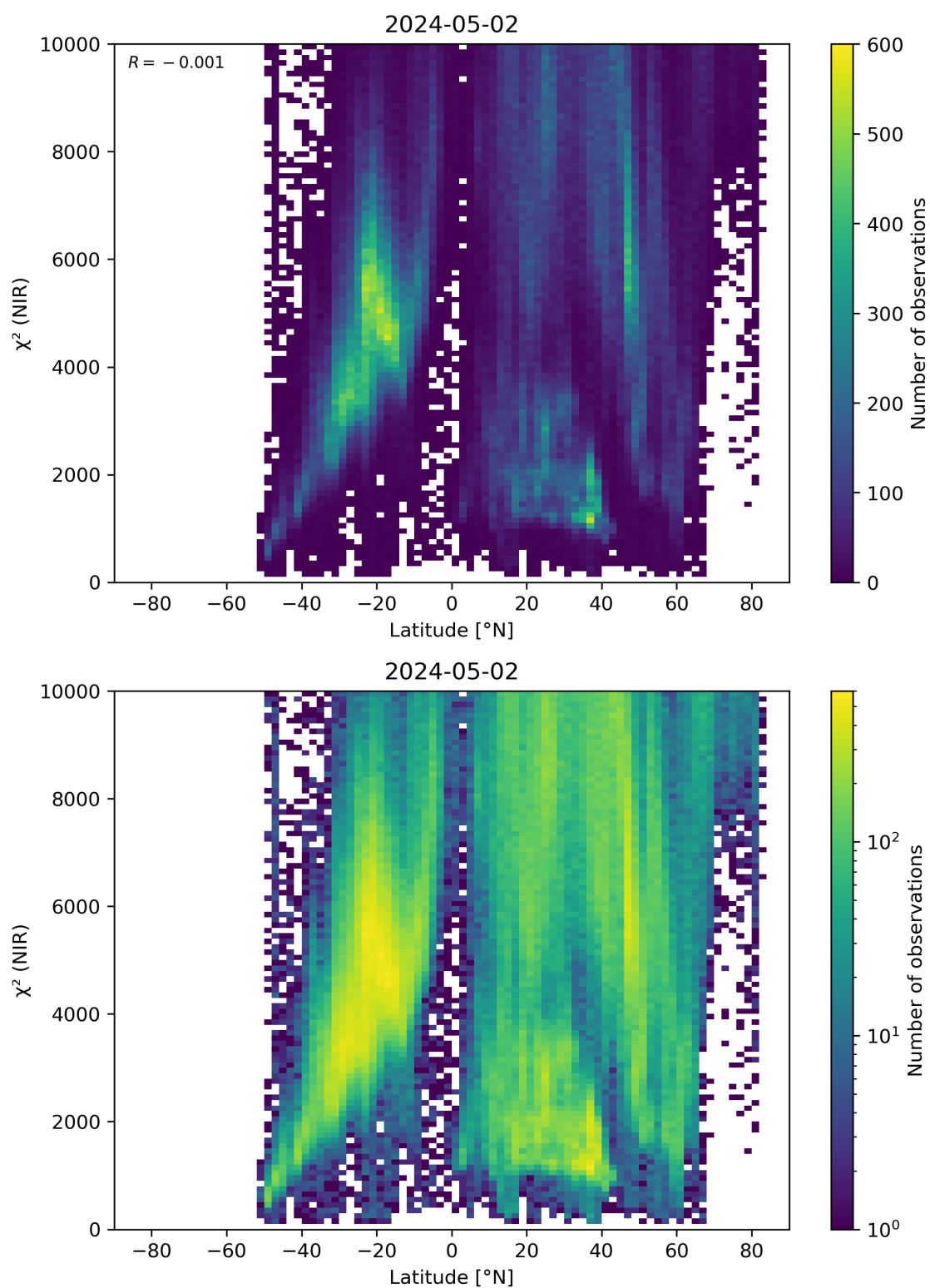
Figure 53: Scatter density plot of “Latitude” against “ \chi^2 (NIR)” for 2024-05-02 to 2024-05-03.
