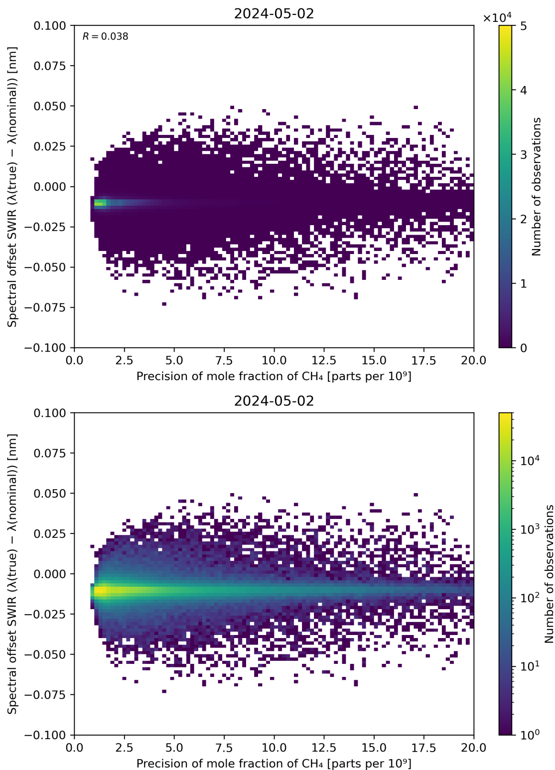
Figure 85: Scatter density plot of “Precision of mole fraction of \text{CH}_4 ” against “Spectral offset SWIR ( \lambda(\text{true}) - \lambda(\text{nominal}) )” for 2024-05-02 to 2024-05-03.
