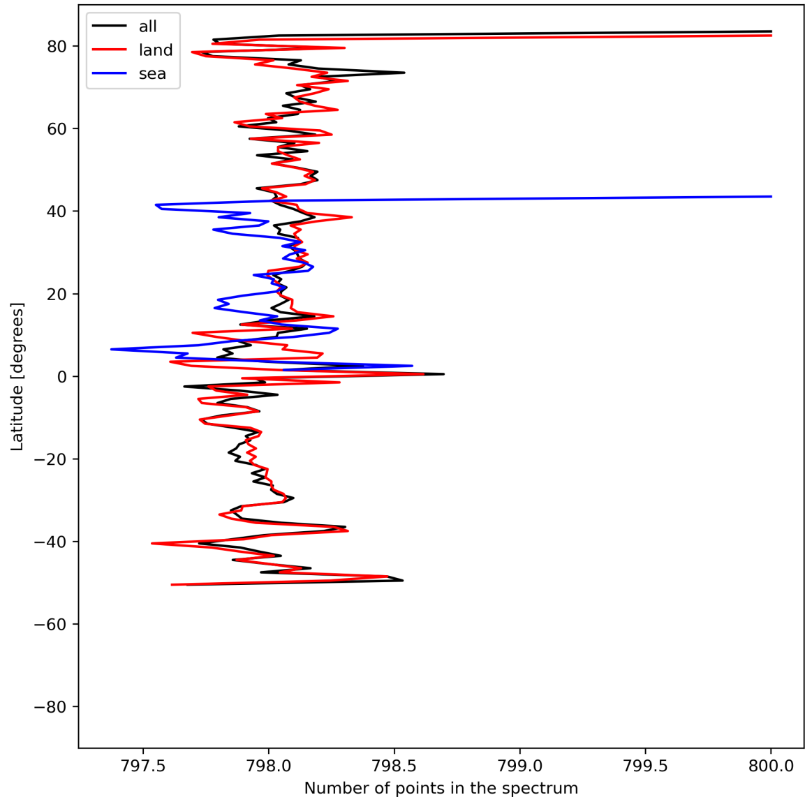
Figure 15: Zonal average of “Number of points in the spectrum” for 2024-05-02 to 2024-05-03.
