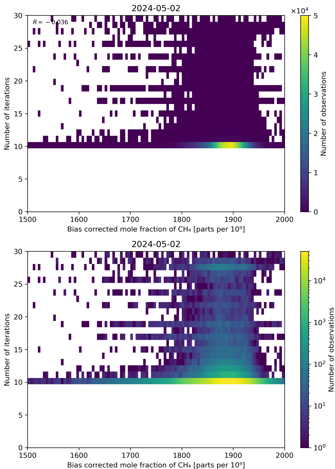
Figure 67: Scatter density plot of “Bias corrected mole fraction of CH 4 ” against “Number of iterations” for 2024-05-02 to 2024-05-03.
