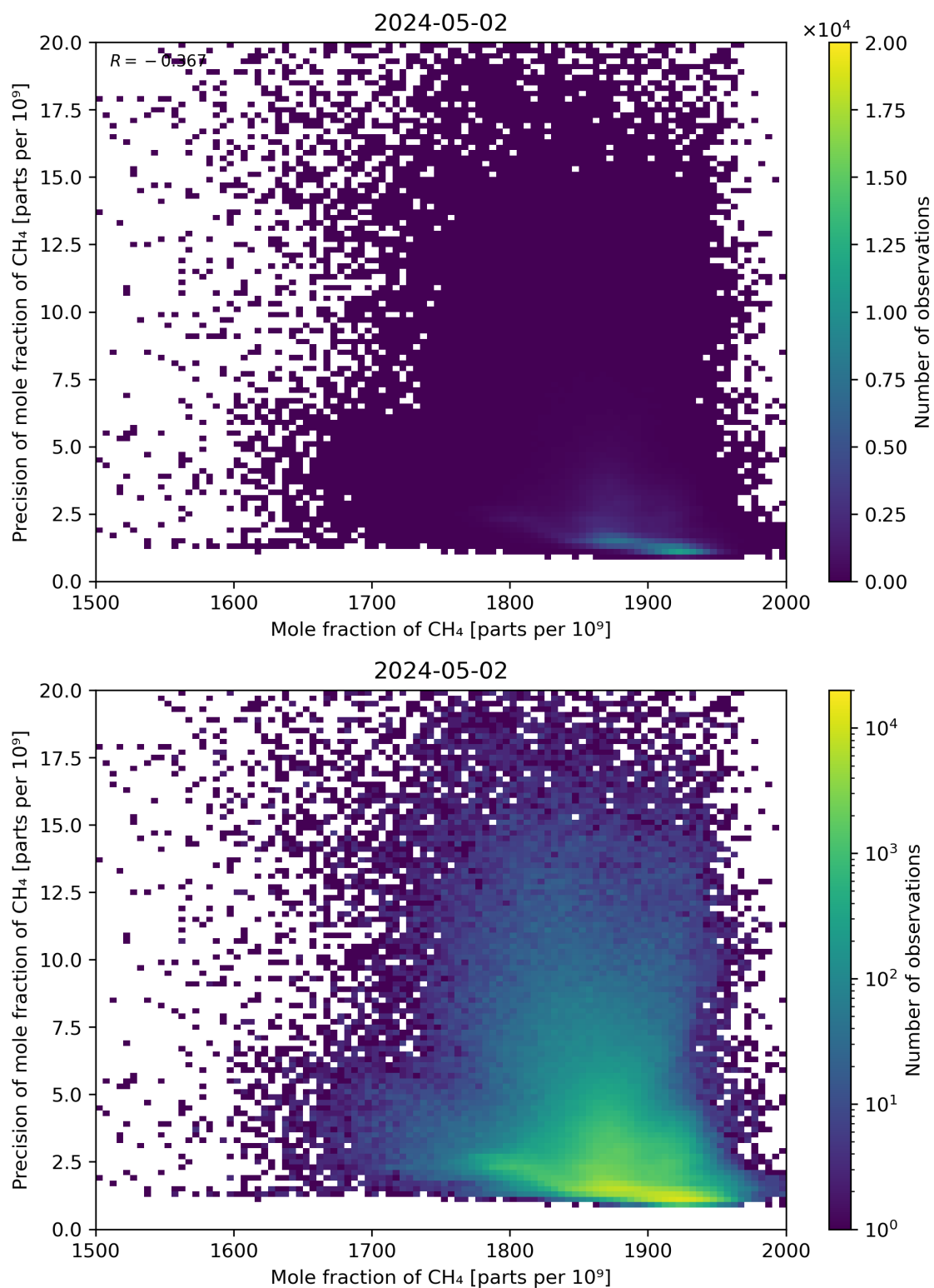
Figure 75: Scatter density plot of “Mole fraction of CH 4 ” against “Precision of mole fraction of CH 4 ” for 2024-05-02 to 2024-05-03.
