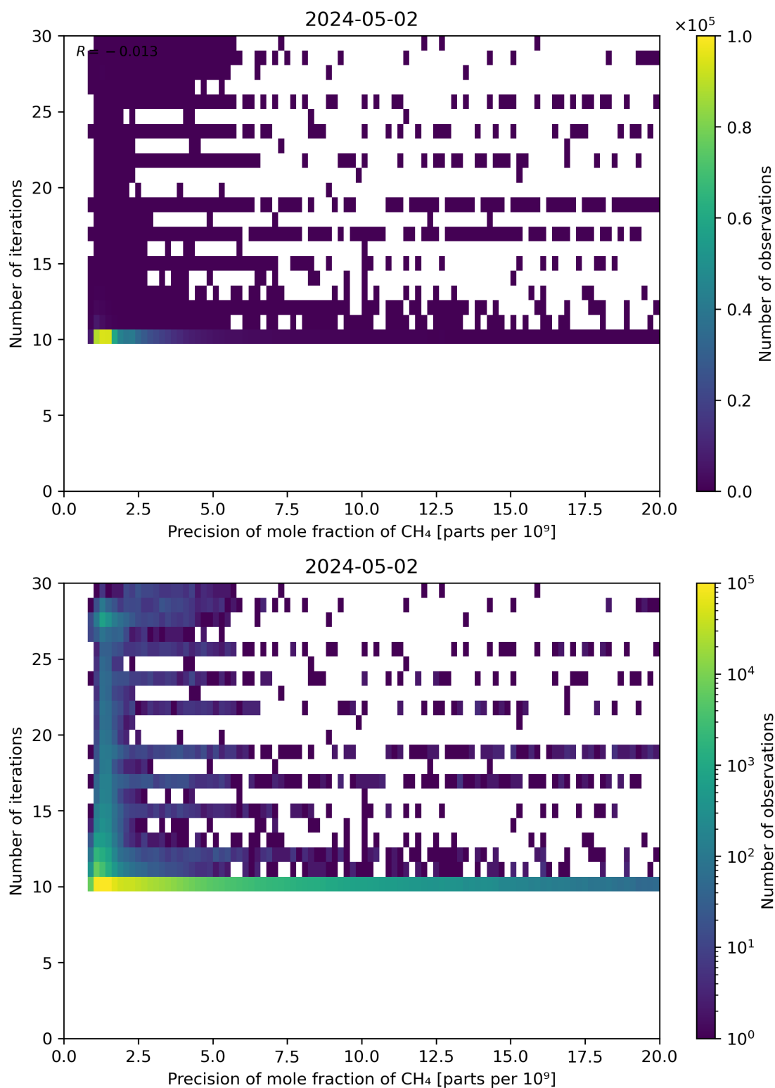
Figure 83: Scatter density plot of “Precision of mole fraction of CH 4 ” against “Number of iterations” for 2024-05-02 to 2024-05-03.
