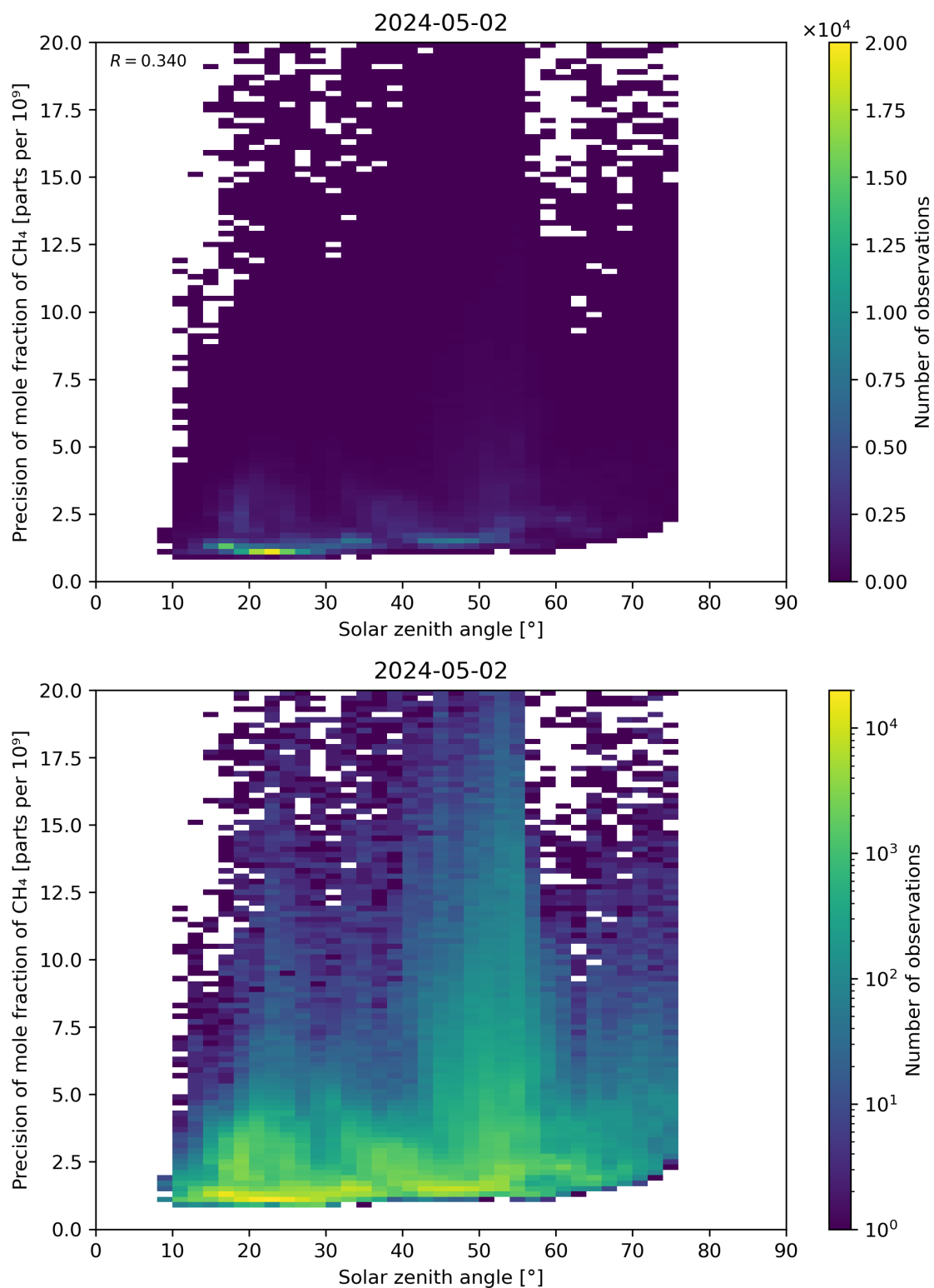
Figure 101: Scatter density plot of “Solar zenith angle” against “Precision of mole fraction of CH 4 ” for 2024-05-02 to 2024-05-03.
