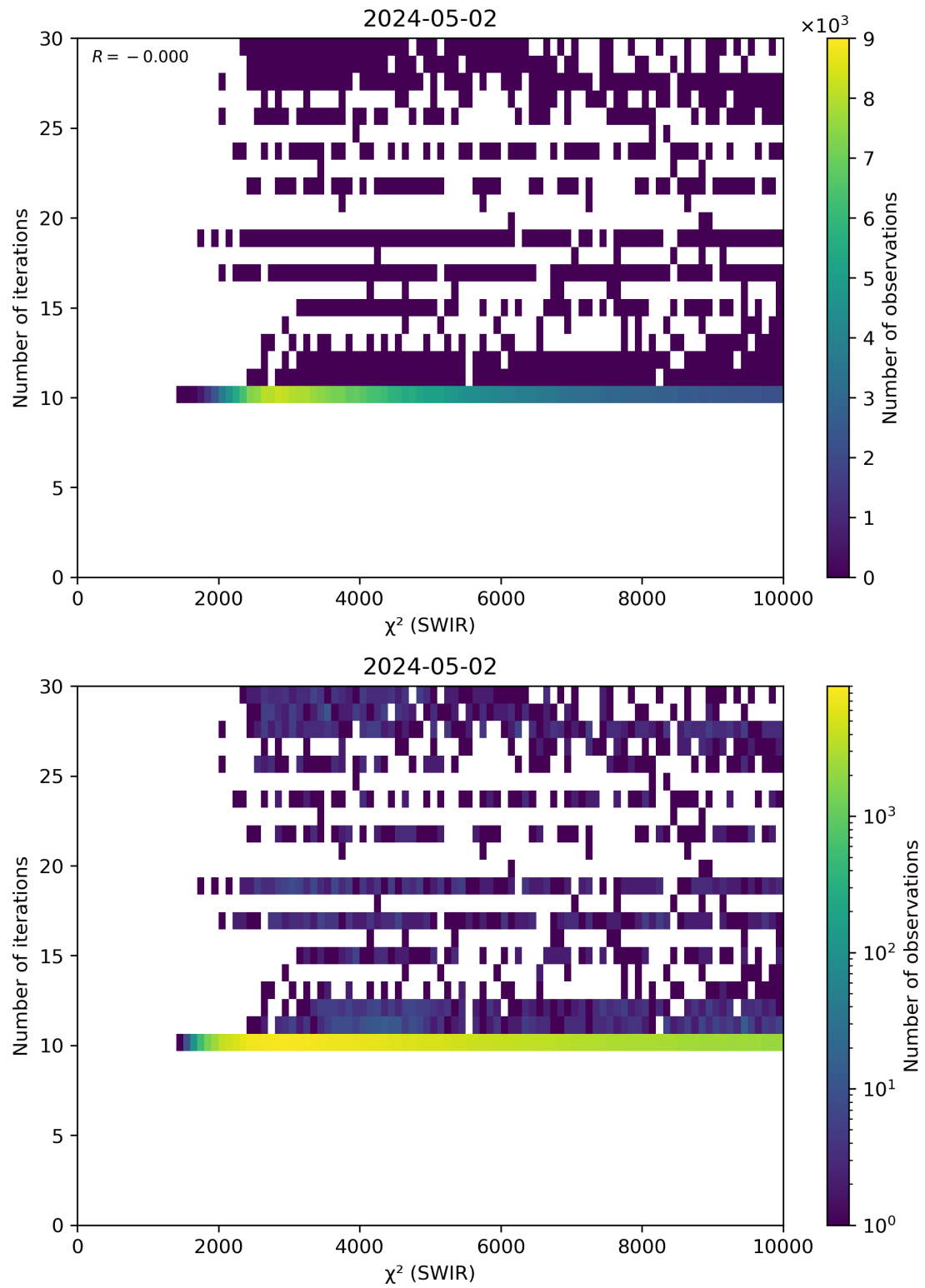
Figure 50: Scatter density plot of “ \chi^2 (SWIR)” against “Number of iterations” for 2024-05-02 to 2024-05-03.
