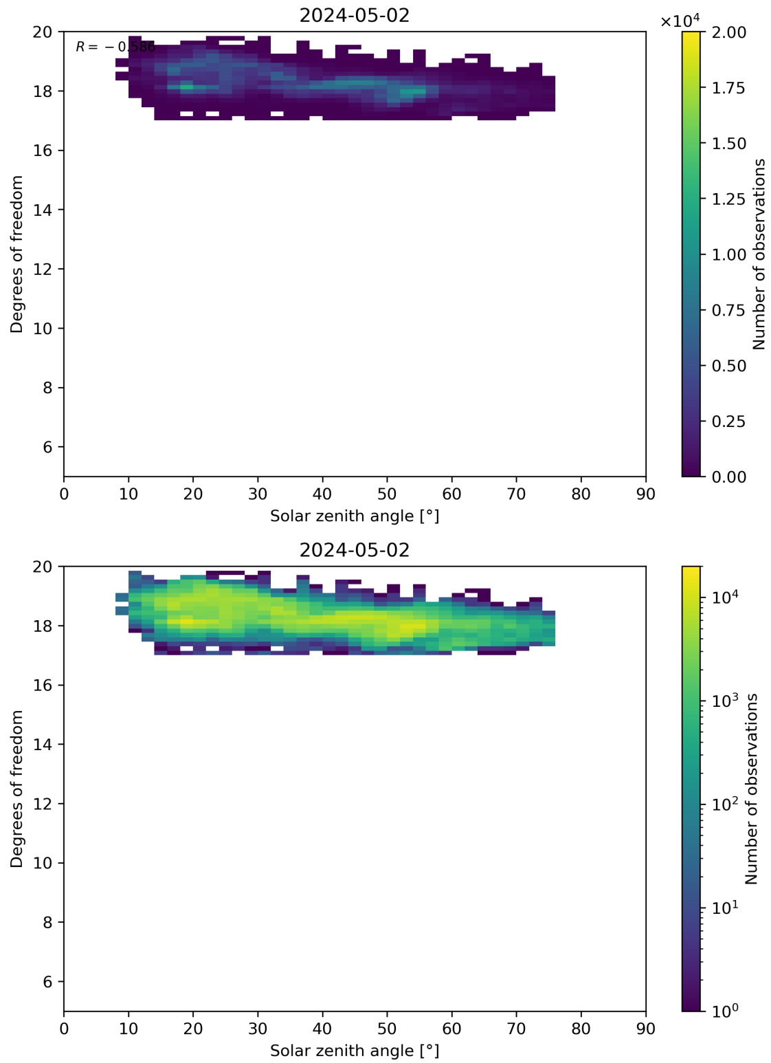
Figure 96: Scatter density plot of “Solar zenith angle” against “Degrees of freedom” for 2024-05-02 to 2024-05-03.
