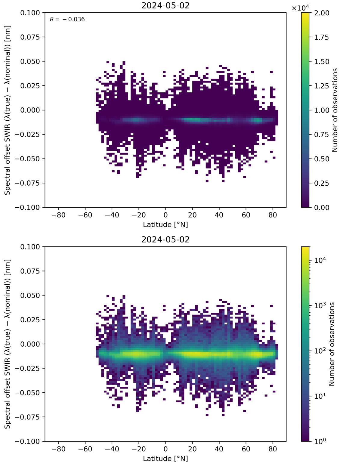
Figure 62: Scatter density plot of “Latitude” against “Spectral offset SWIR ( \lambda(\text{true}) - \lambda(\text{nominal}) )” for 2024-05-02 to 2024-05-03.
