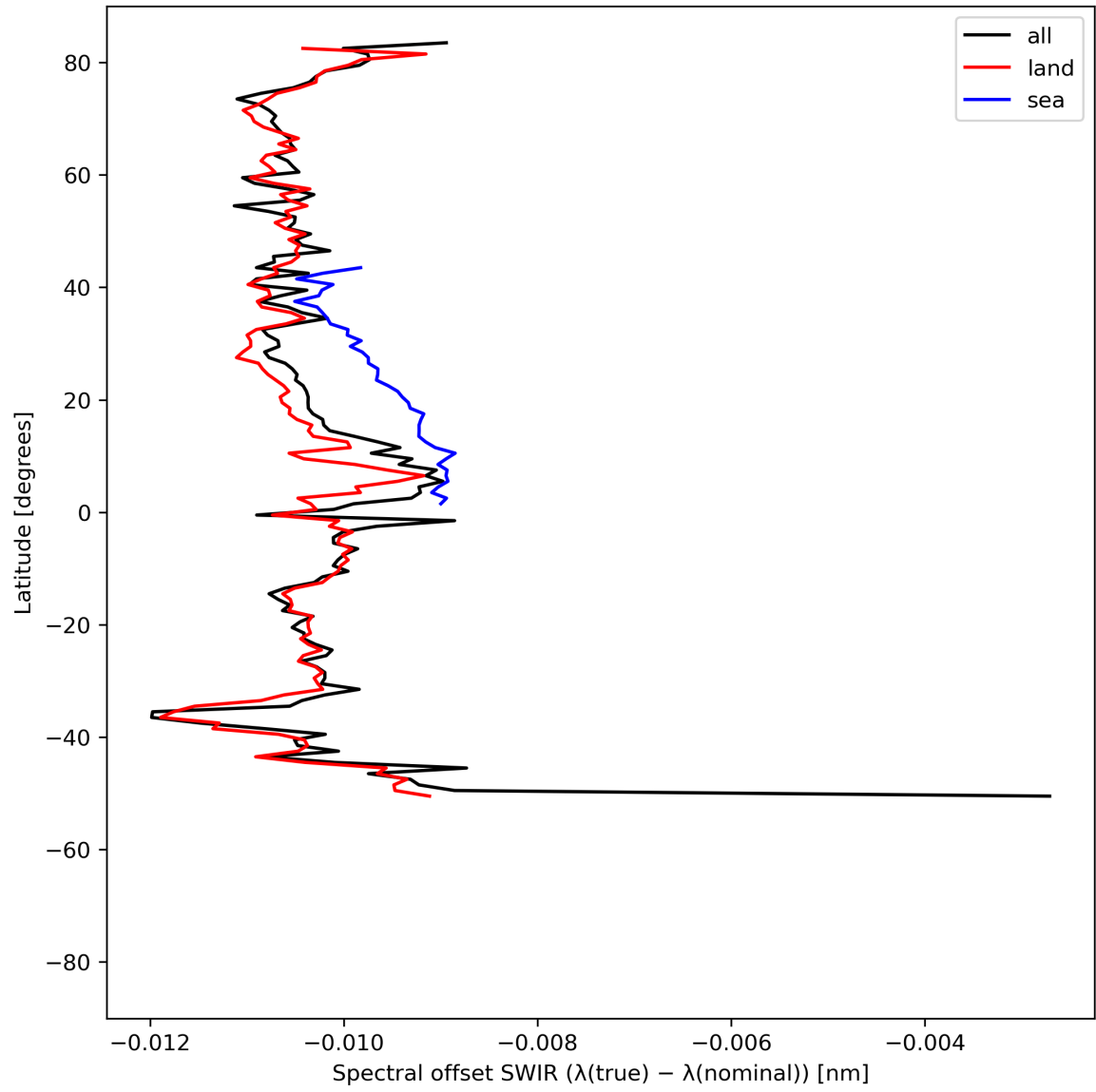
Figure 16: Zonal average of “Spectral offset SWIR ( \lambda(\text{true}) - \lambda(\text{nominal}) )” for 2024-05-02 to 2024-05-03.
