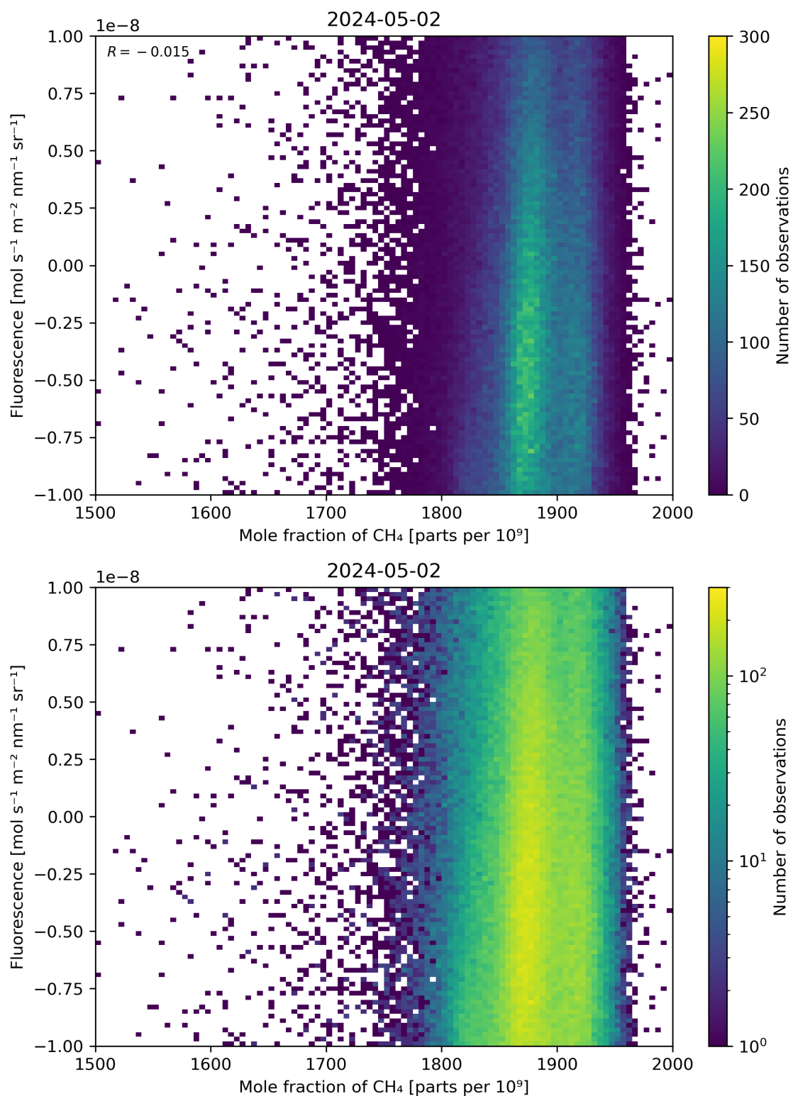
Figure 73: Scatter density plot of “Mole fraction of \text{CH}_4 ” against “Fluorescence” for 2024-05-02 to 2024-05-03.
