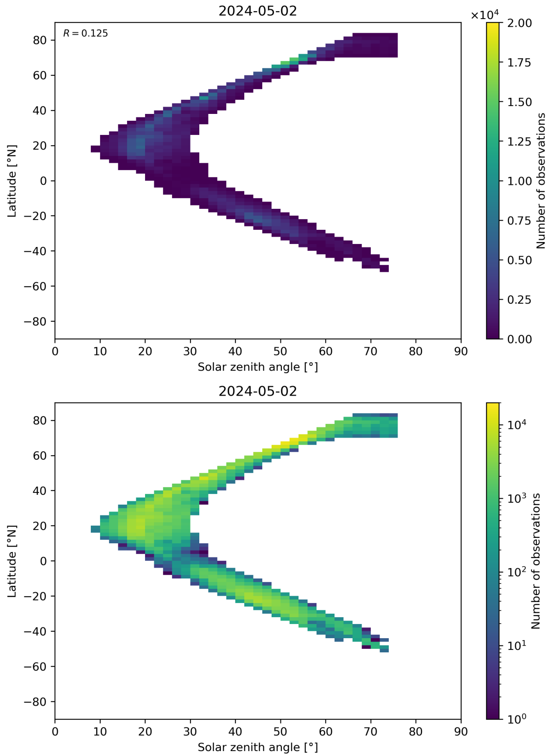
Figure 98: Scatter density plot of “Solar zenith angle” against “Latitude” for 2024-05-02 to 2024-05-03.
