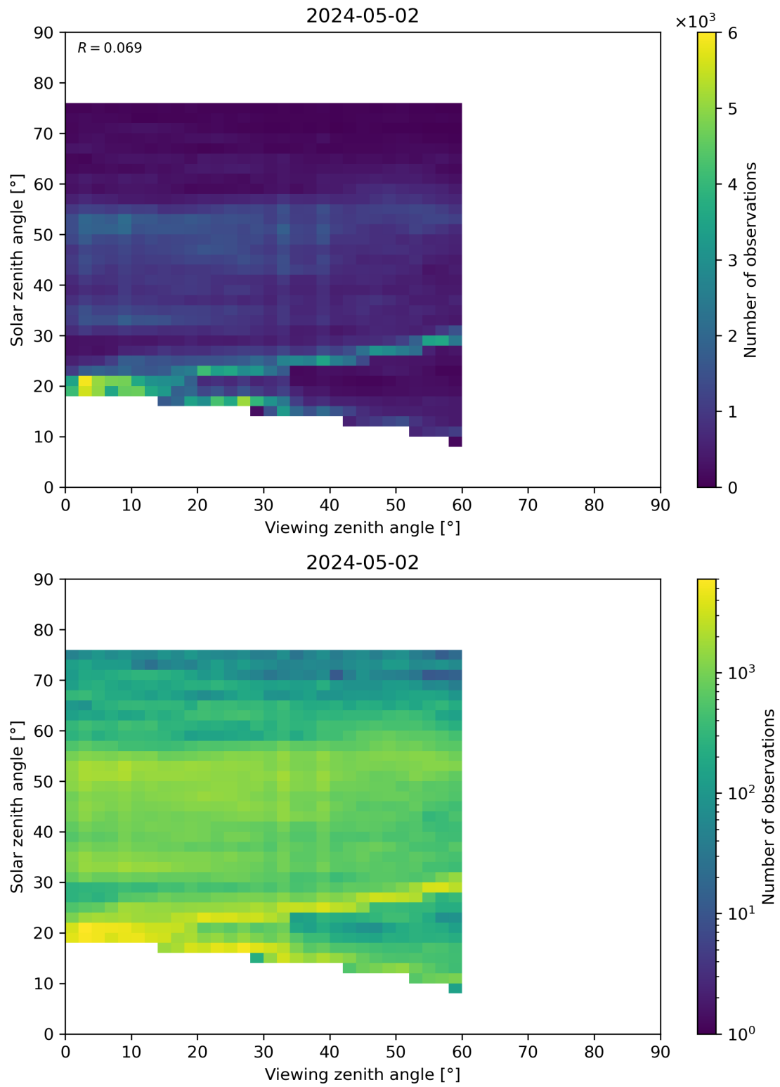
Figure 115: Scatter density plot of “Viewing zenith angle” against “Solar zenith angle” for 2024-05-02 to 2024-05-03.
