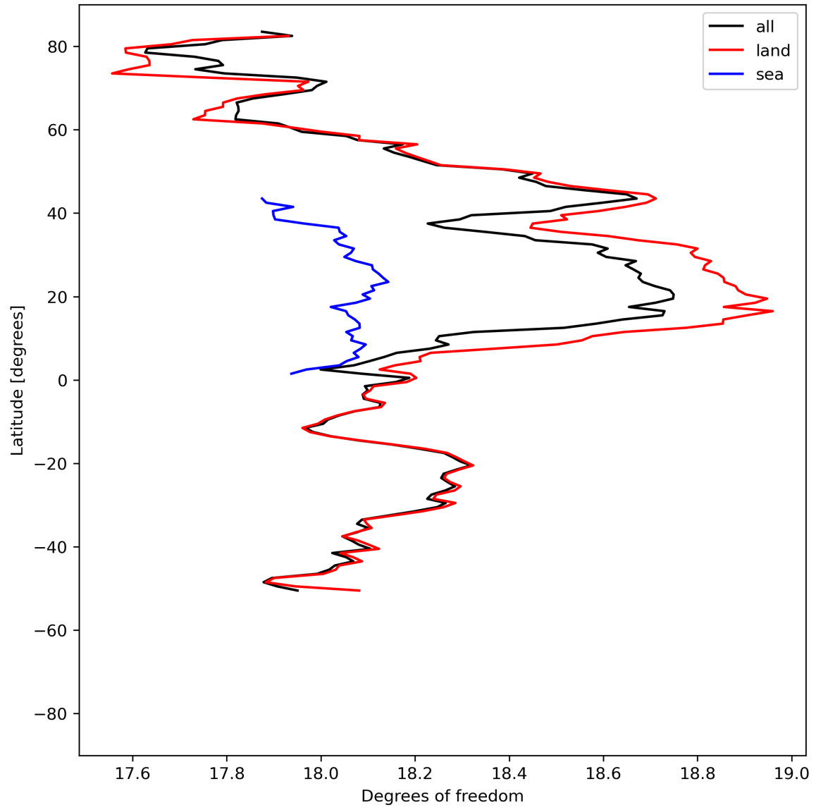
Figure 19: Zonal average of “Degrees of freedom” for 2024-05-02 to 2024-05-03.
