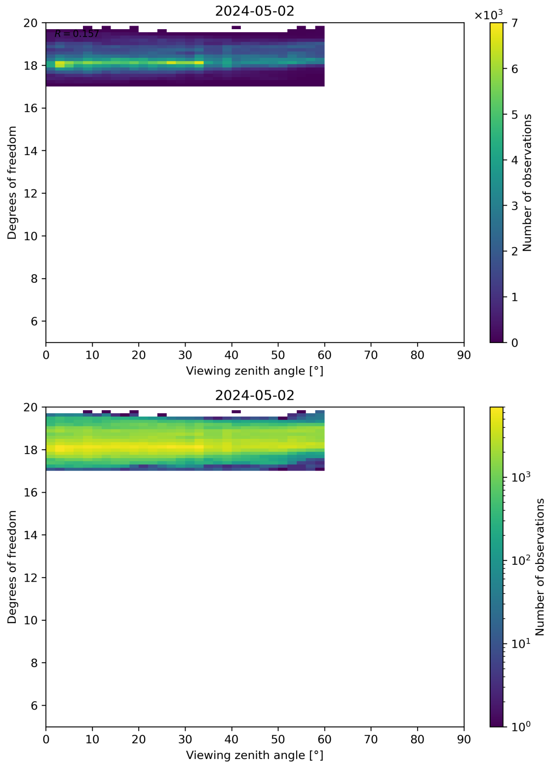
Figure 107: Scatter density plot of “Viewing zenith angle” against “Degrees of freedom” for 2024-05-02 to 2024-05-03.
