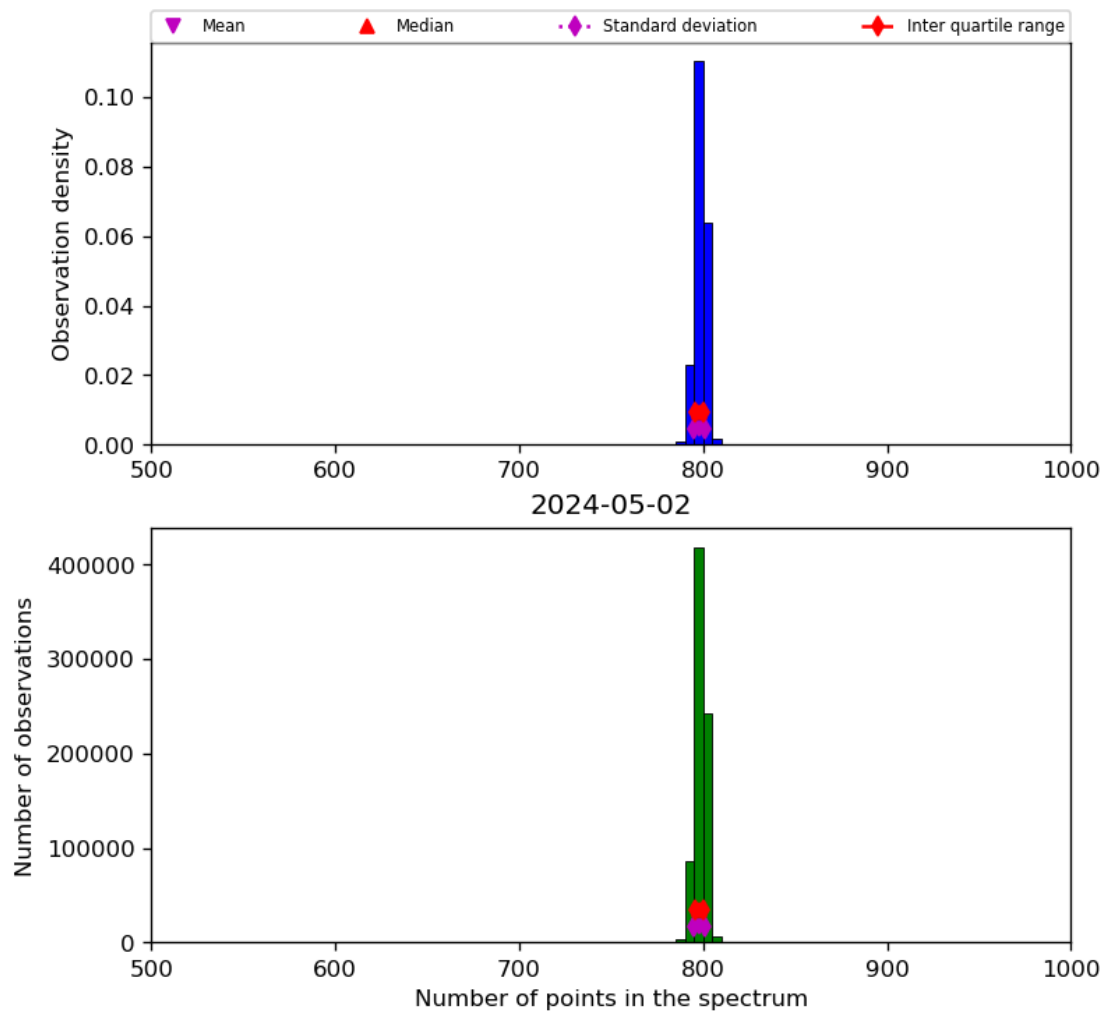
Figure 26: Histogram of “Number of points in the spectrum” for 2024-05-02 to 2024-05-03
