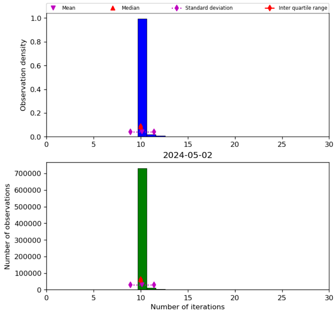
Figure 31: Histogram of “Number of iterations” for 2024-05-02 to 2024-05-03
