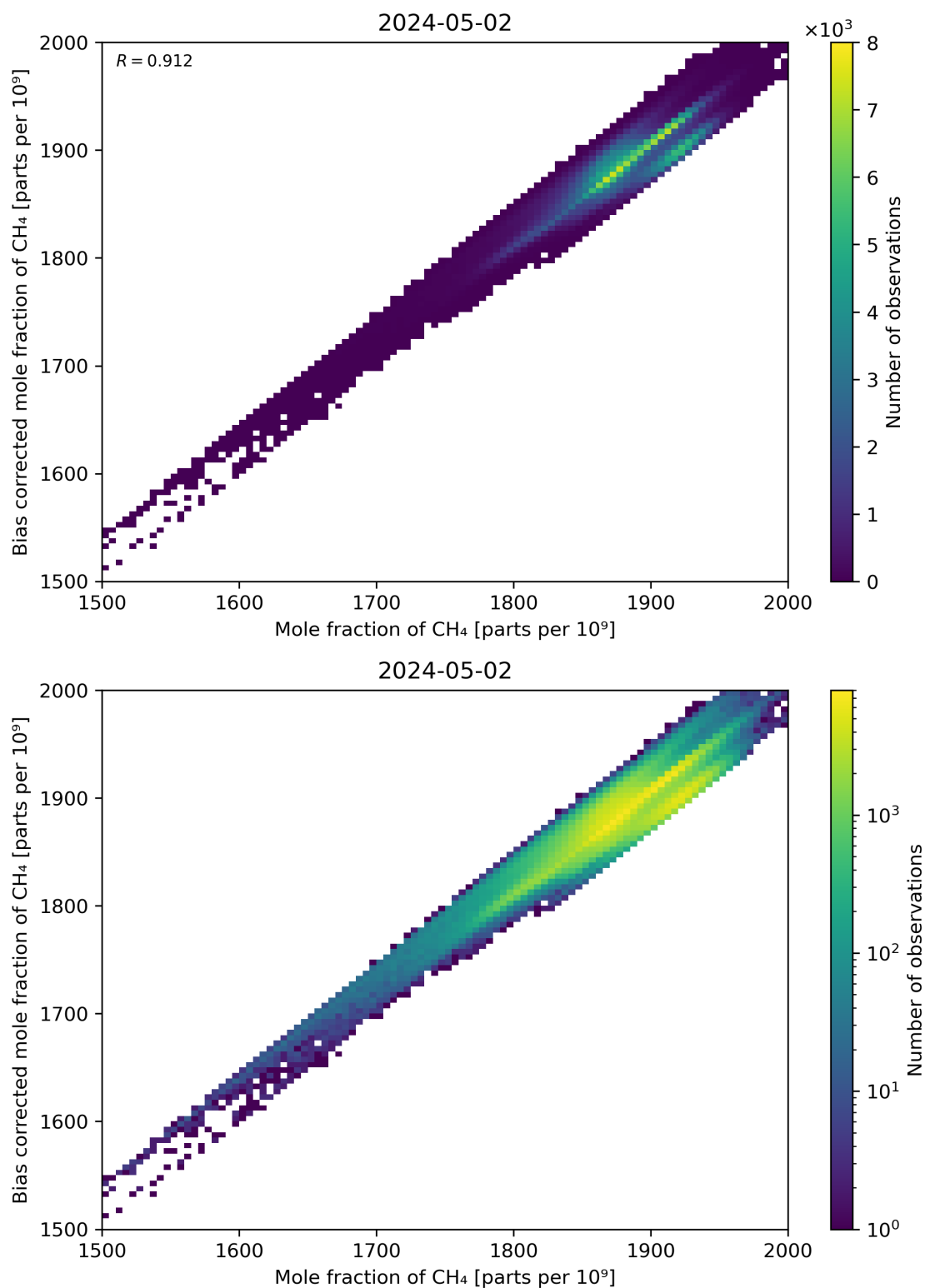
Figure 74: Scatter density plot of “Mole fraction of CH 4 ” against “Bias corrected mole fraction of CH 4 ” for 2024-05-02 to 2024-05-03.
