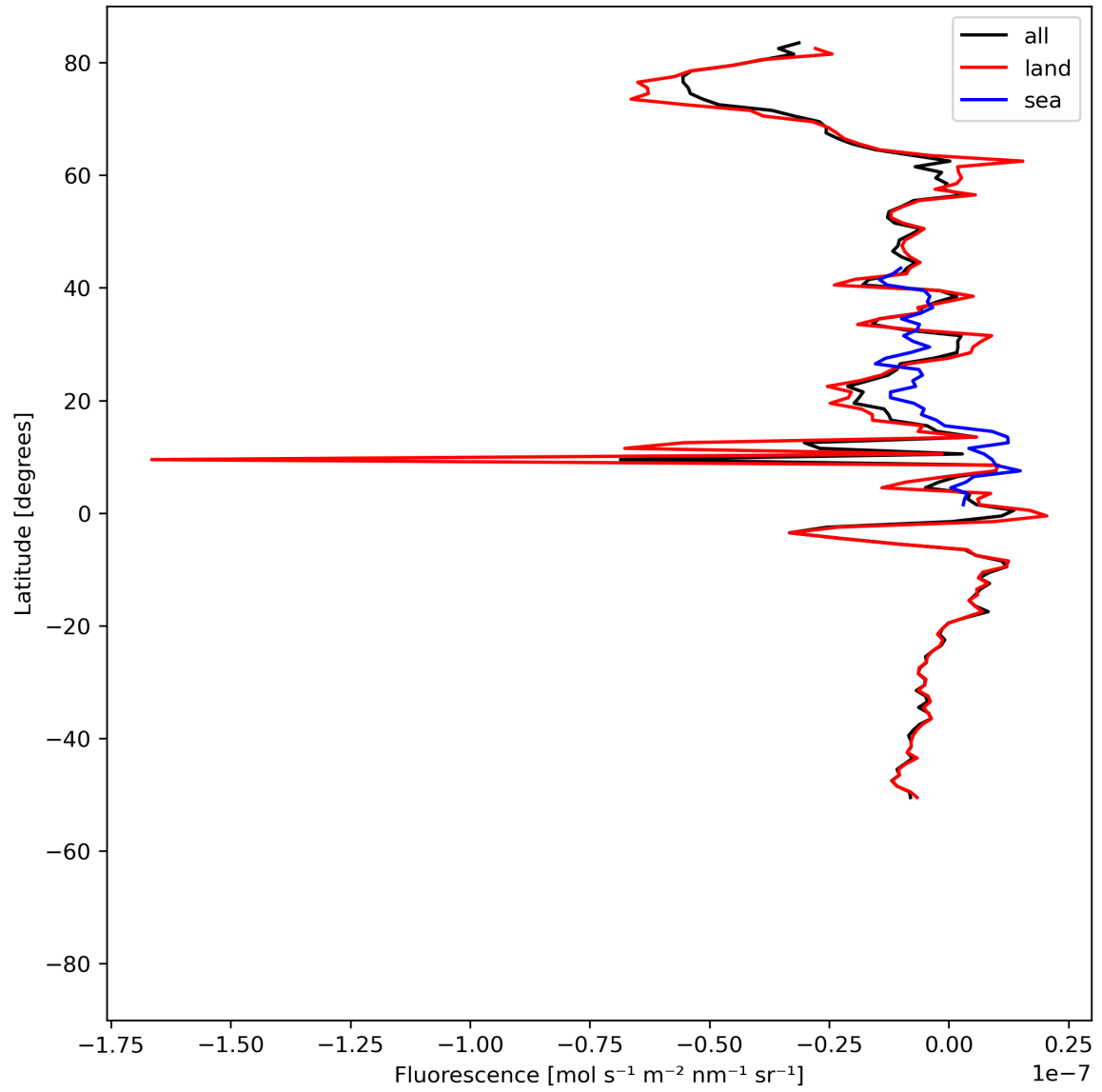
Figure 21: Zonal average of “Fluorescence” for 2024-05-02 to 2024-05-03.
