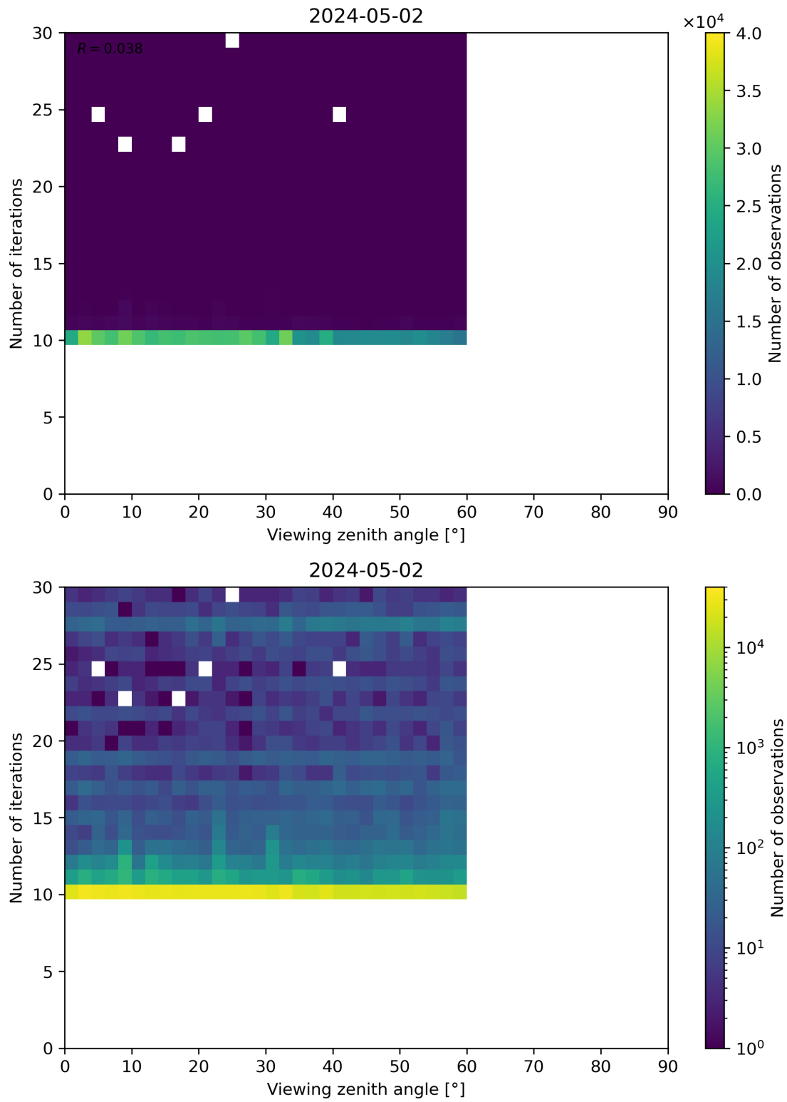
Figure 113: Scatter density plot of “Viewing zenith angle” against “Number of iterations” for 2024-05-02 to 2024-05-03.
