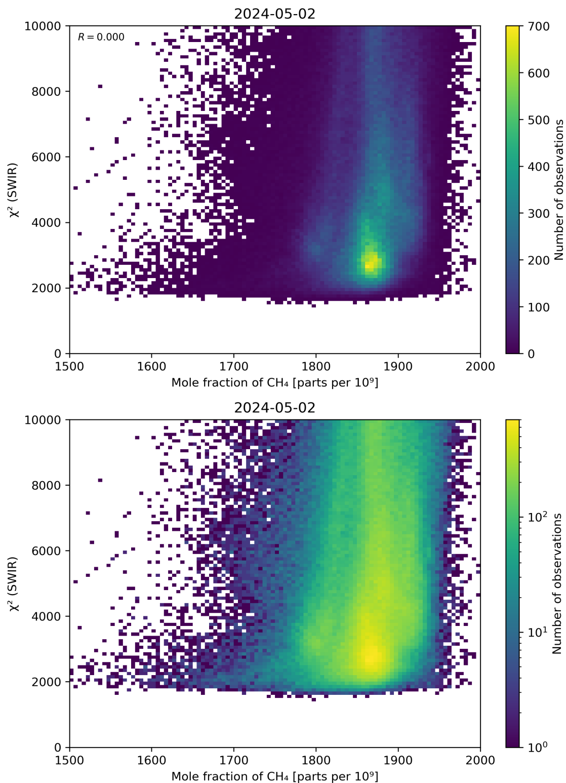
Figure 71: Scatter density plot of “Mole fraction of \text{CH}_4 ” against “ \chi^2 (SWIR)” for 2024-05-02 to 2024-05-03.
