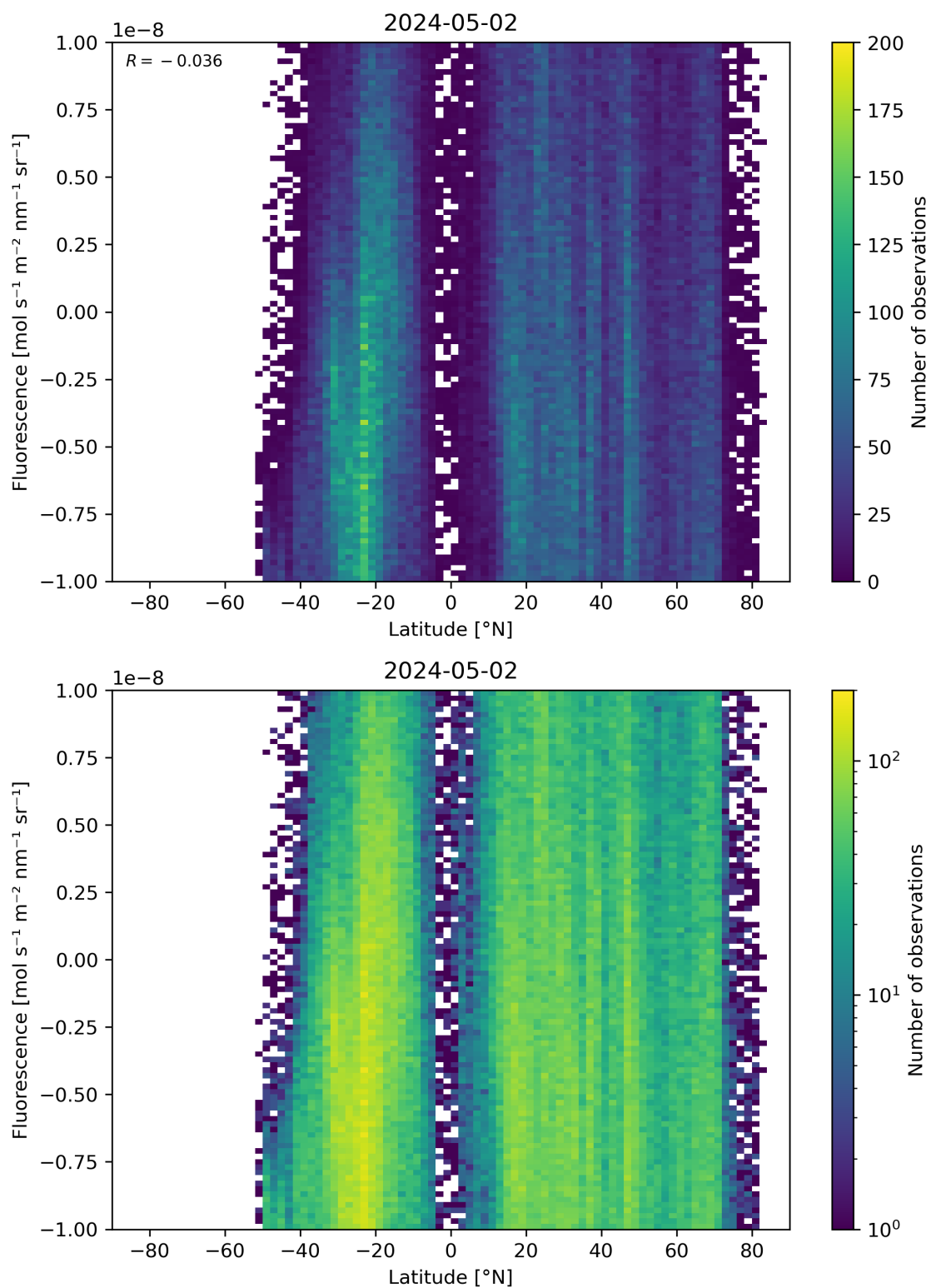
Figure 56: Scatter density plot of “Latitude” against “Fluorescence” for 2024-05-02 to 2024-05-03.
