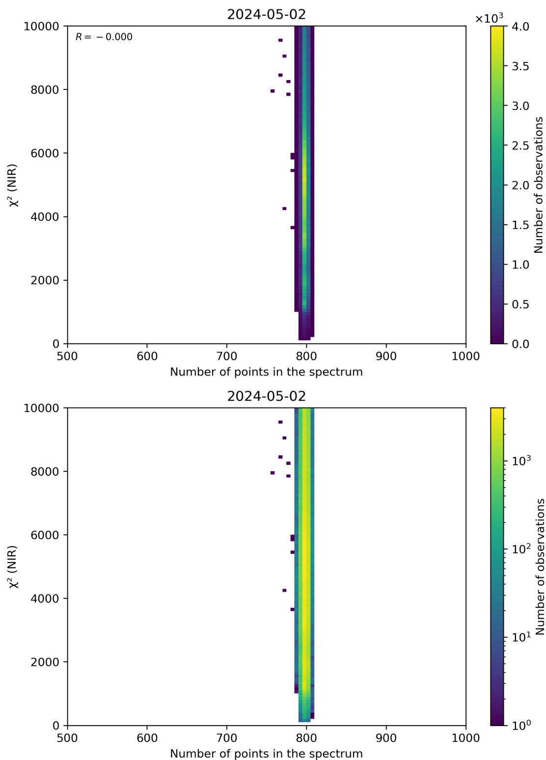
Figure 88: Scatter density plot of “Number of points in the spectrum” against “ \chi^2 (NIR)” for 2024-05-02 to 2024-05-03.
