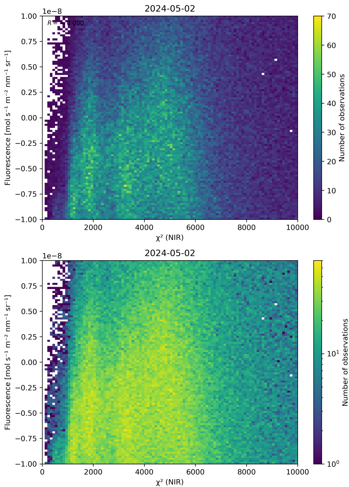
Figure 45: Scatter density plot of “ \chi^2 (NIR)” against “Fluorescence” for 2024-05-02 to 2024-05-03.
