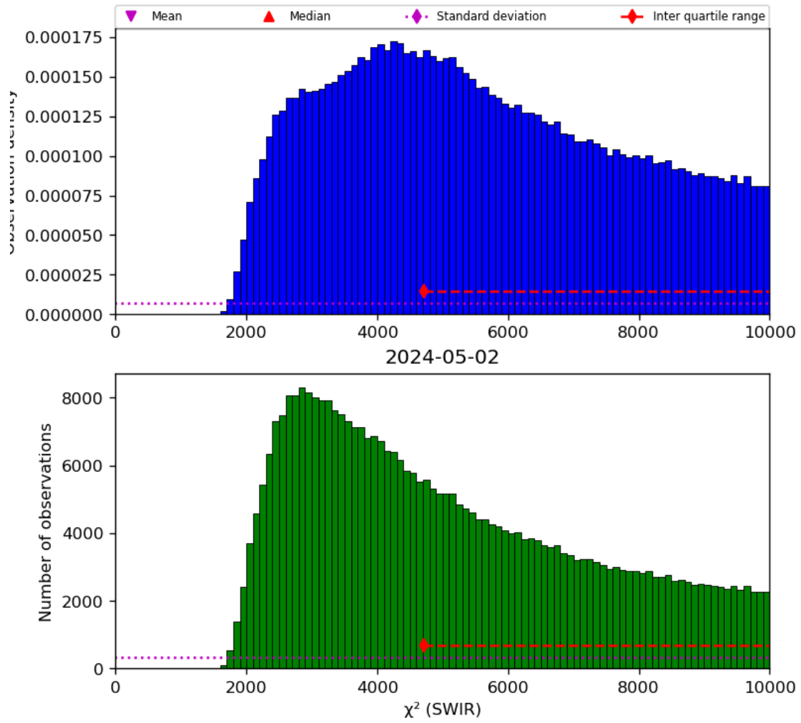
Figure 28: Histogram of “ \chi^2 (SWIR)” for 2024-05-02 to 2024-05-03
