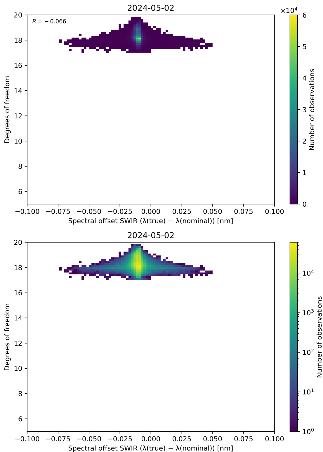
Figure 119: Scatter density plot of “Spectral offset SWIR ( \lambda(\text{true}) - \lambda(\text{nominal}) )” against “Degrees of freedom” for 2024-05-02 to 2024-05-03.
