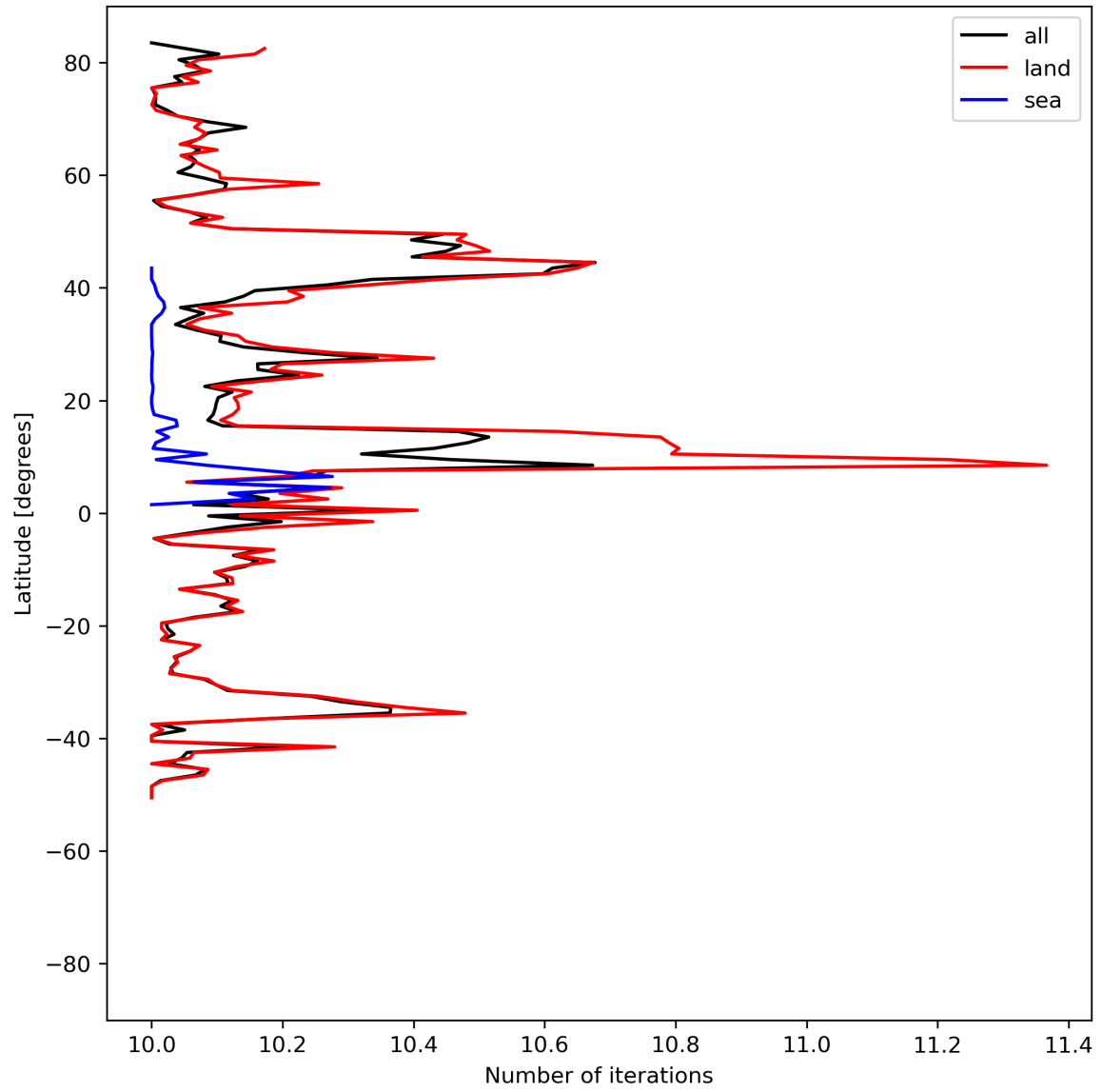
Figure 20: Zonal average of “Number of iterations” for 2024-05-02 to 2024-05-03.
