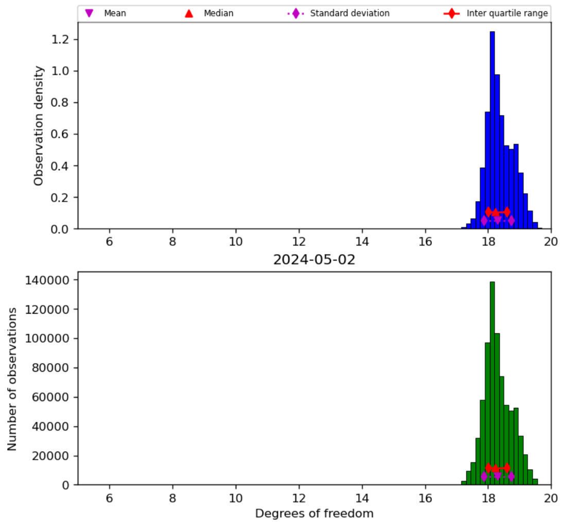
Figure 30: Histogram of “Degrees of freedom” for 2024-05-02 to 2024-05-03
