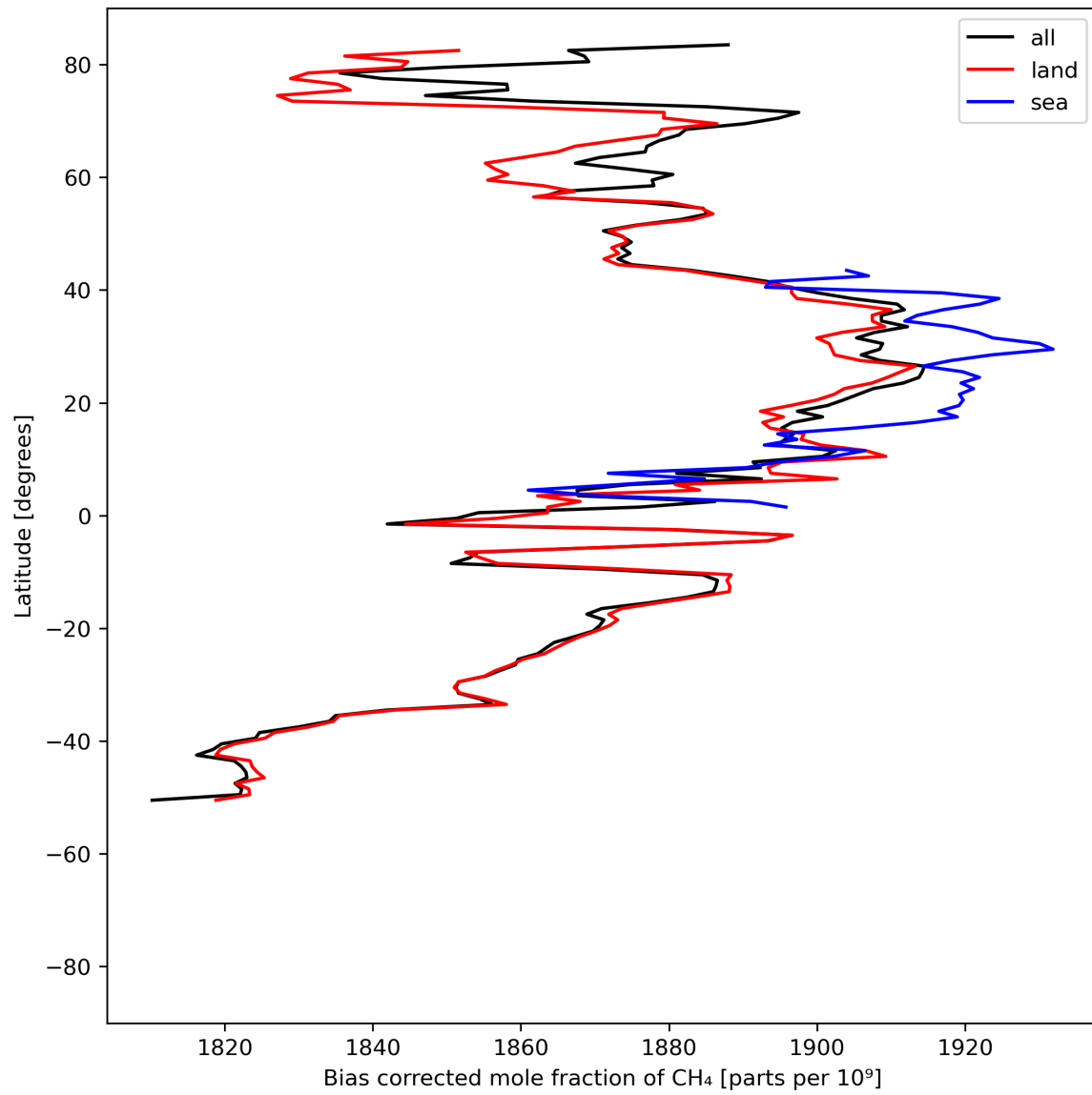
Figure 14: Zonal average of “Bias corrected mole fraction of \text{CH}_4 ” for 2024-05-02 to 2024-05-03.
