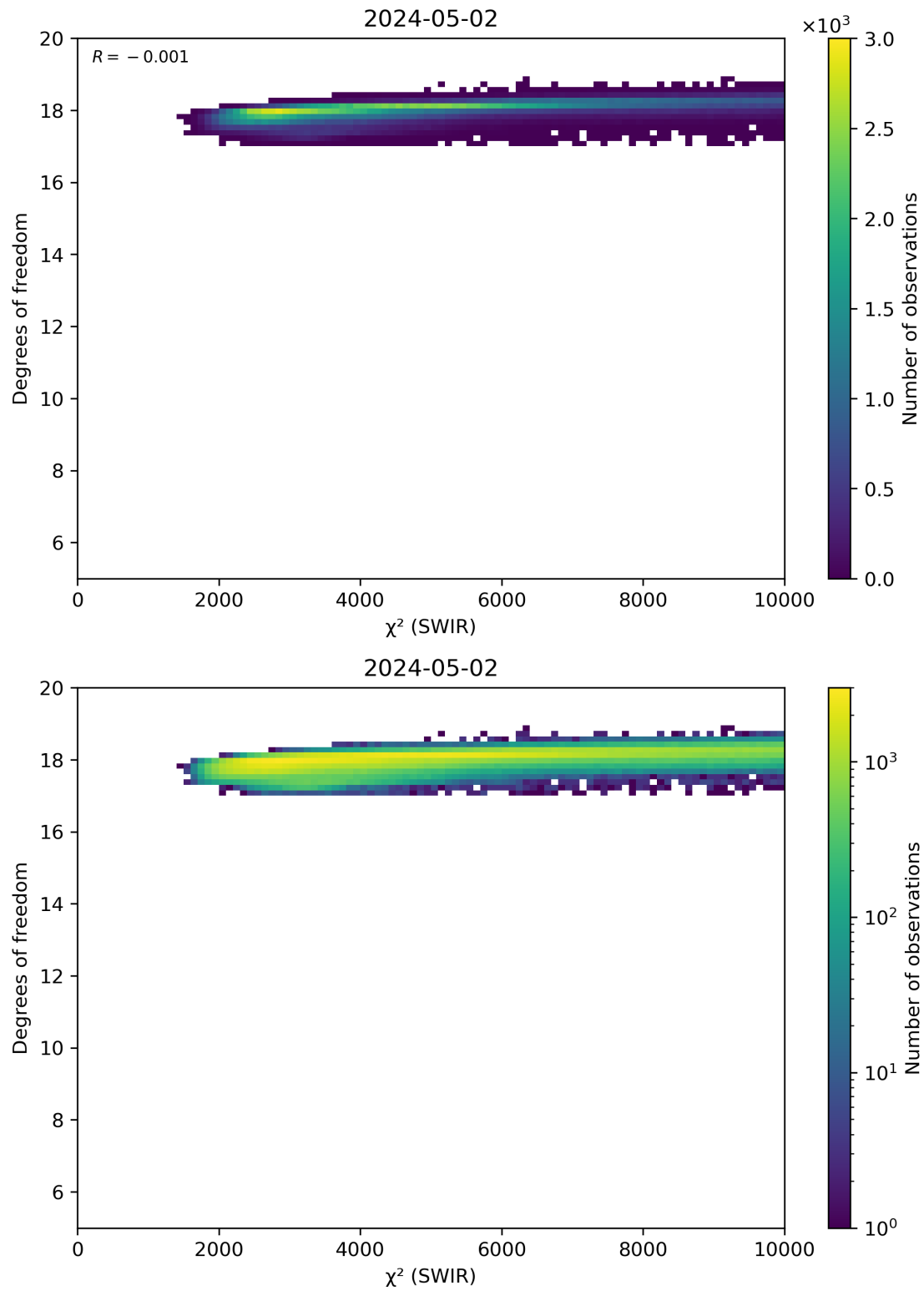
Figure 48: Scatter density plot of “ \chi^2 (SWIR)” against “Degrees of freedom” for 2024-05-02 to 2024-05-03.
