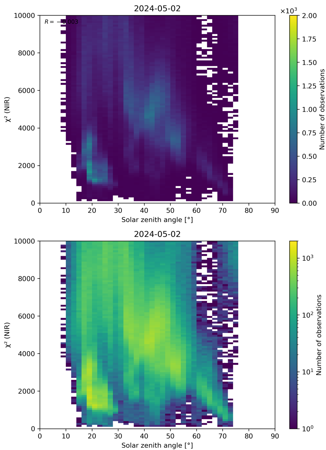
Figure 94: Scatter density plot of “Solar zenith angle” against “ \chi^2 (NIR)” for 2024-05-02 to 2024-05-03.
