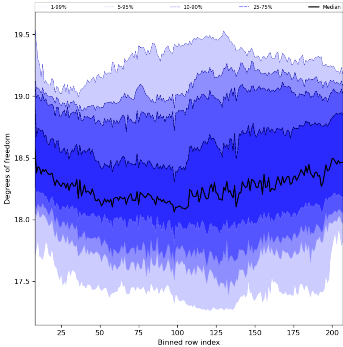
Figure 41: Along track statistics of “Degrees of freedom” for 2024-05-02 to 2024-05-03
