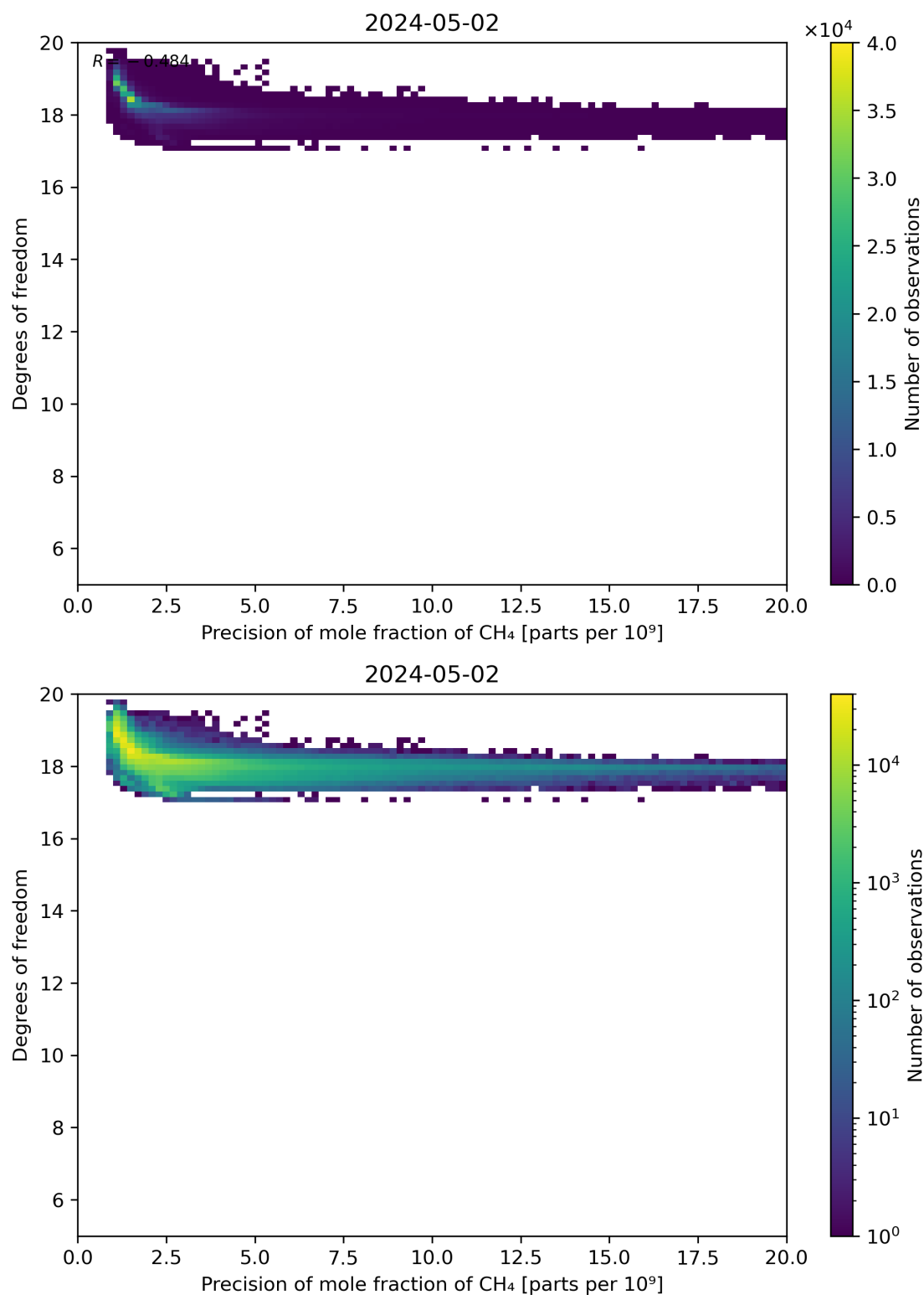
Figure 80: Scatter density plot of “Precision of mole fraction of CH 4 ” against “Degrees of freedom” for 2024-05-02 to 2024-05-03.
