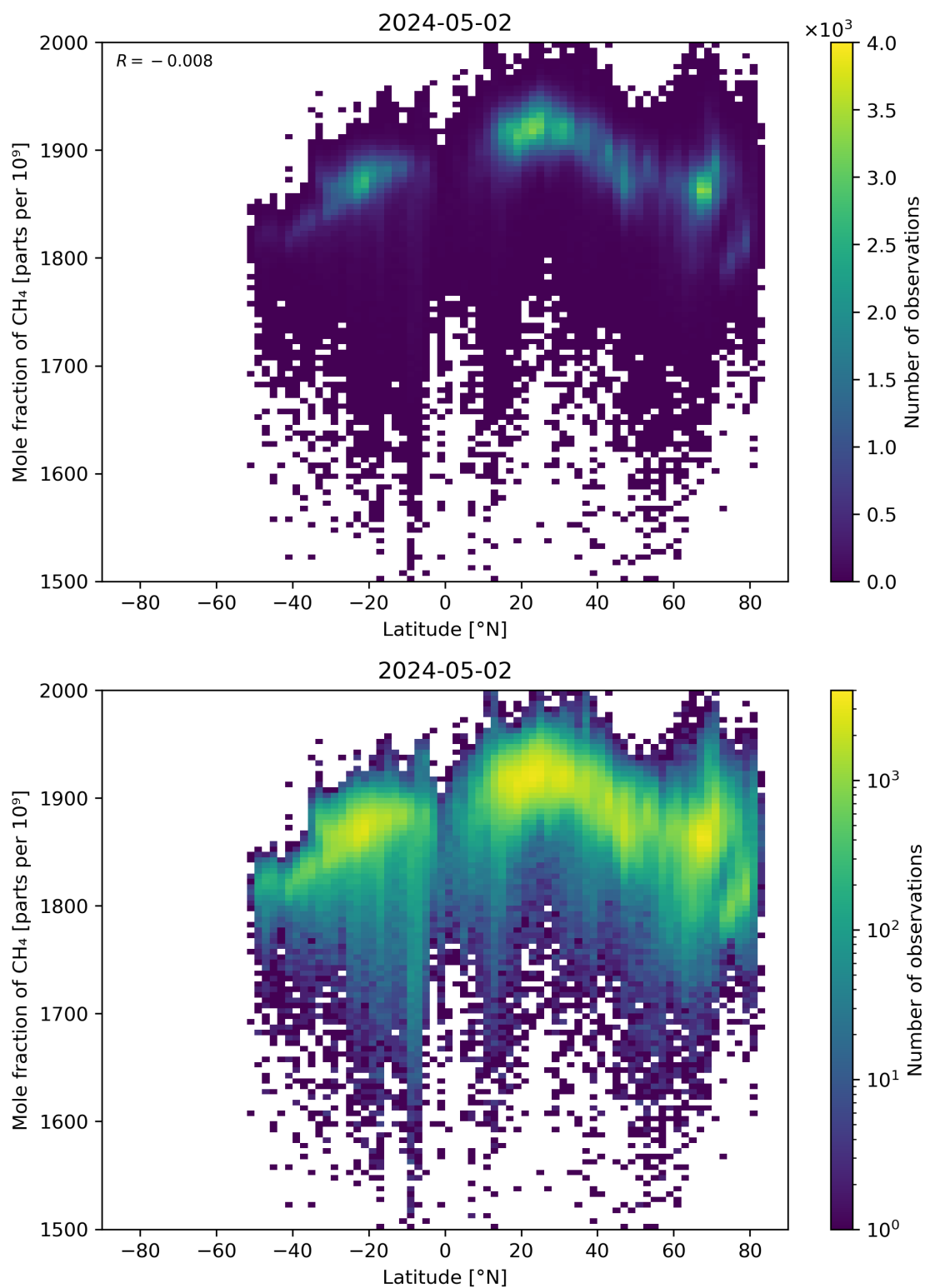
Figure 57: Scatter density plot of “Latitude” against “Mole fraction of CH 4 ” for 2024-05-02 to 2024-05-03.
