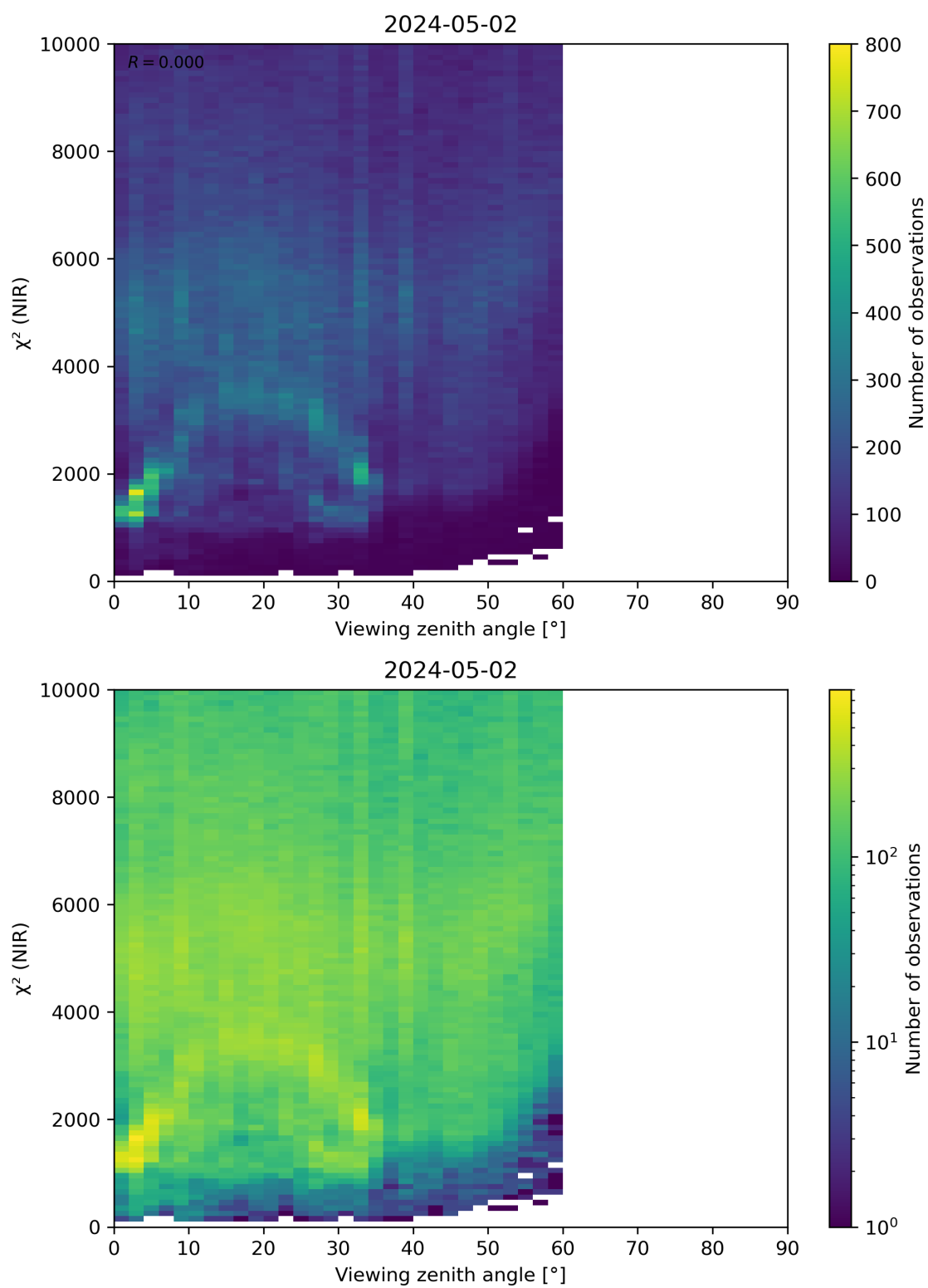
Figure 105: Scatter density plot of “Viewing zenith angle” against “ \chi^2 (NIR)” for 2024-05-02 to 2024-05-03.
