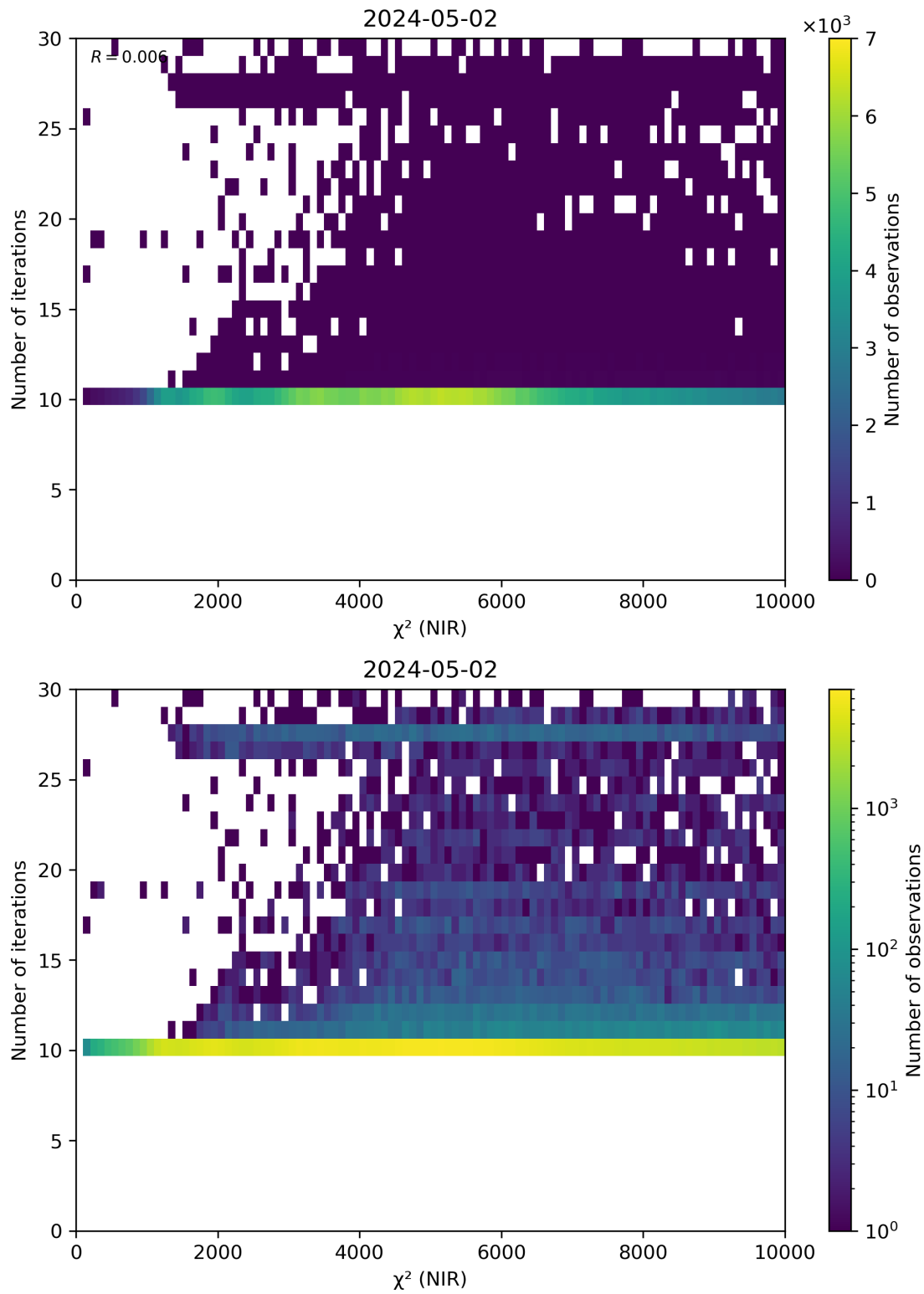
Figure 46: Scatter density plot of “ \chi^2 (NIR)” against “Number of iterations” for 2024-05-02 to 2024-05-03.
