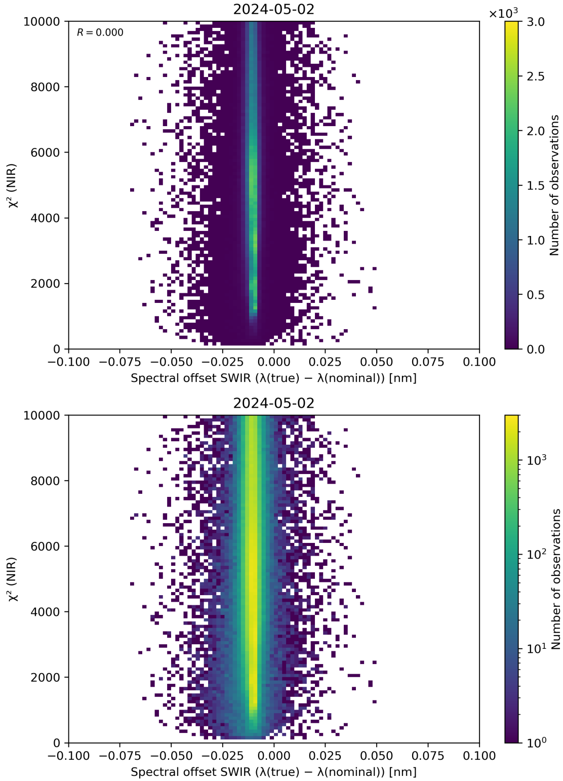
Figure 117: Scatter density plot of “Spectral offset SWIR ( \lambda(\text{true}) - \lambda(\text{nominal}) )” against “ \chi^2 (NIR)” for 2024-05-02 to 2024-05-03.
