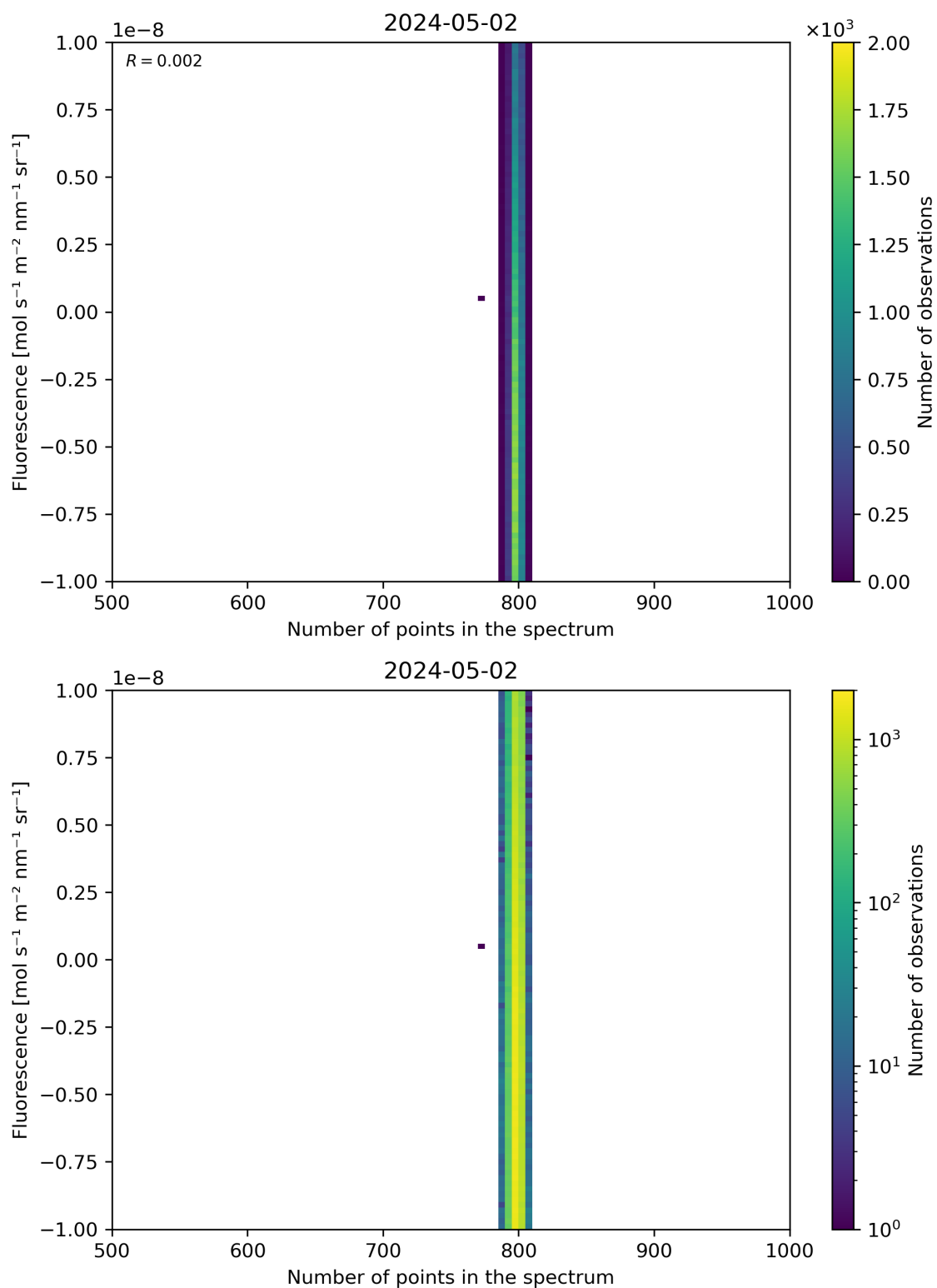
Figure 91: Scatter density plot of “Number of points in the spectrum” against “Fluorescence” for 2024-05-02 to 2024-05-03.
