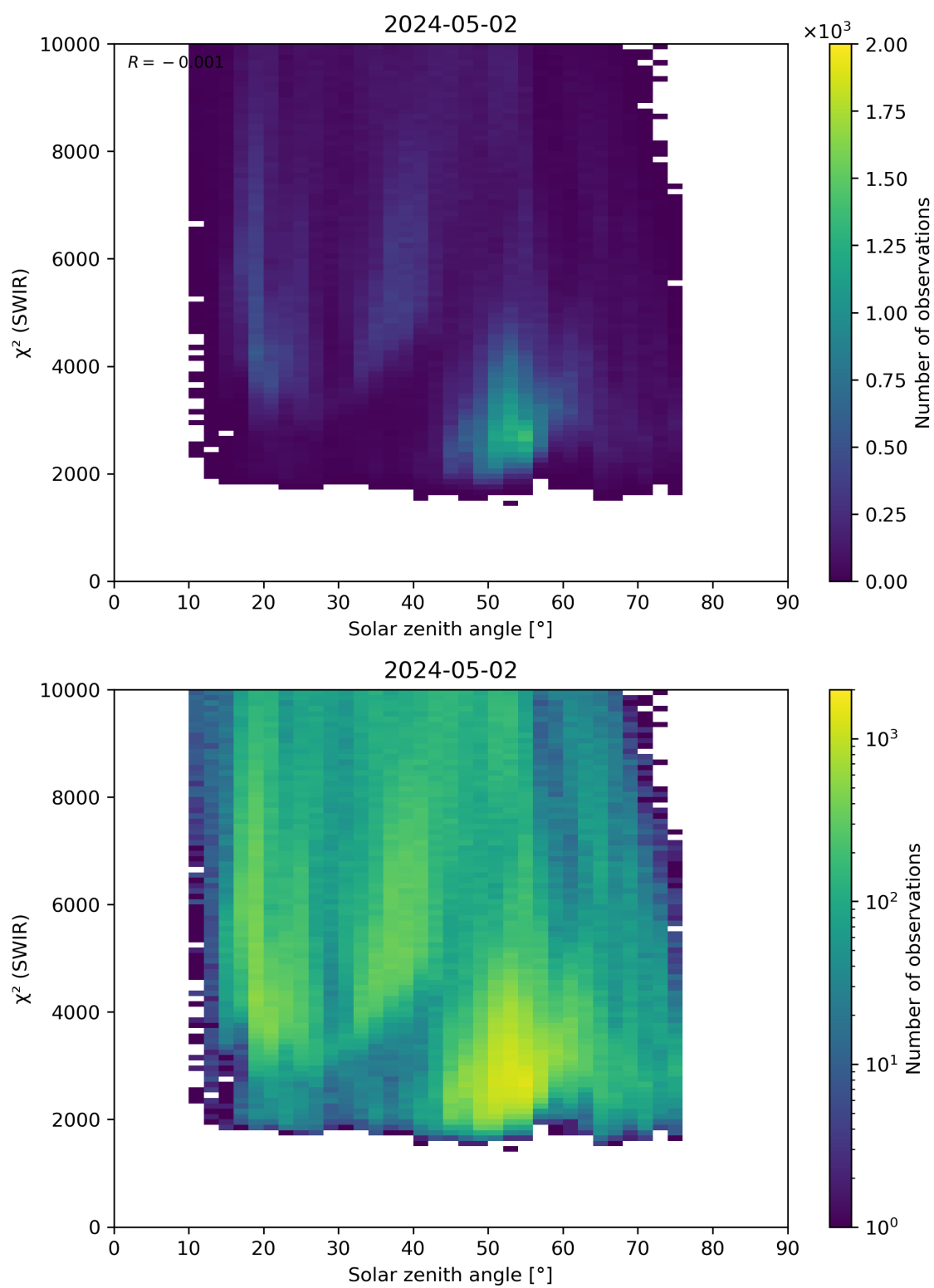
Figure 95: Scatter density plot of “Solar zenith angle” against “ \chi^2 (SWIR)” for 2024-05-02 to 2024-05-03.
