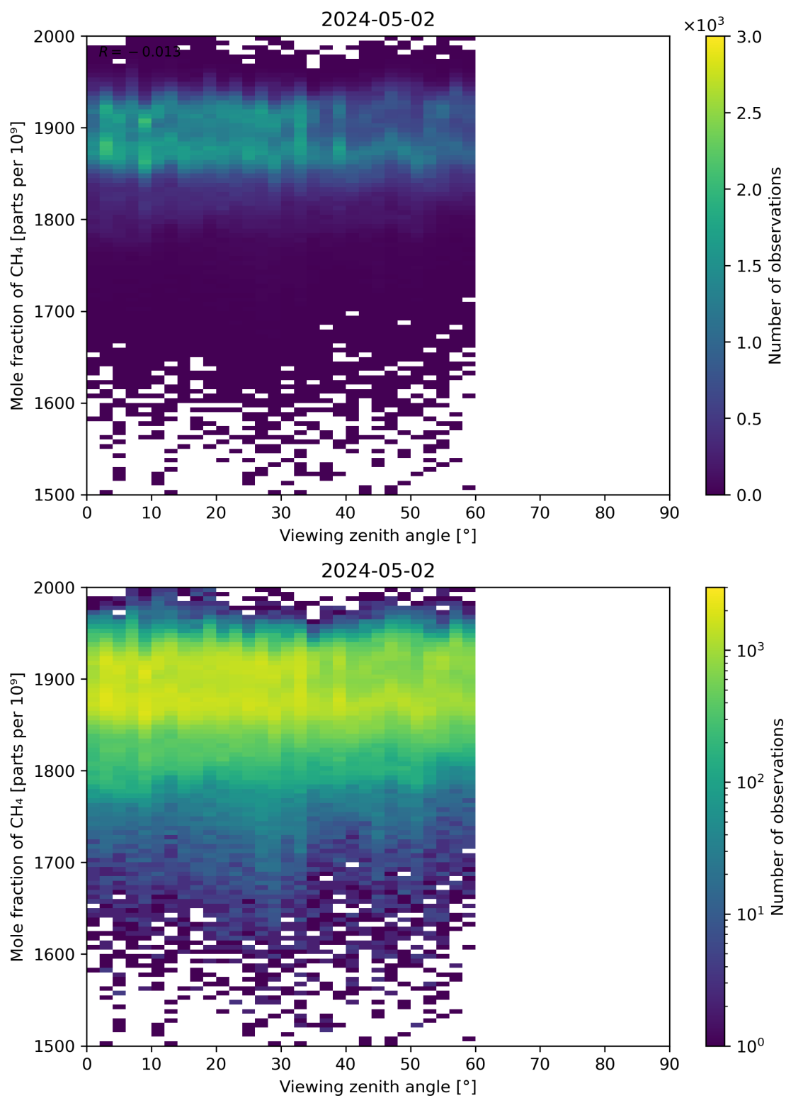
Figure 110: Scatter density plot of “Viewing zenith angle” against “Mole fraction of CH 4 ” for 2024-05-02 to 2024-05-03.
