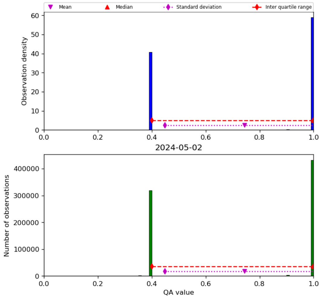
Figure 22: Histogram of “QA value” for 2024-05-02 to 2024-05-03
