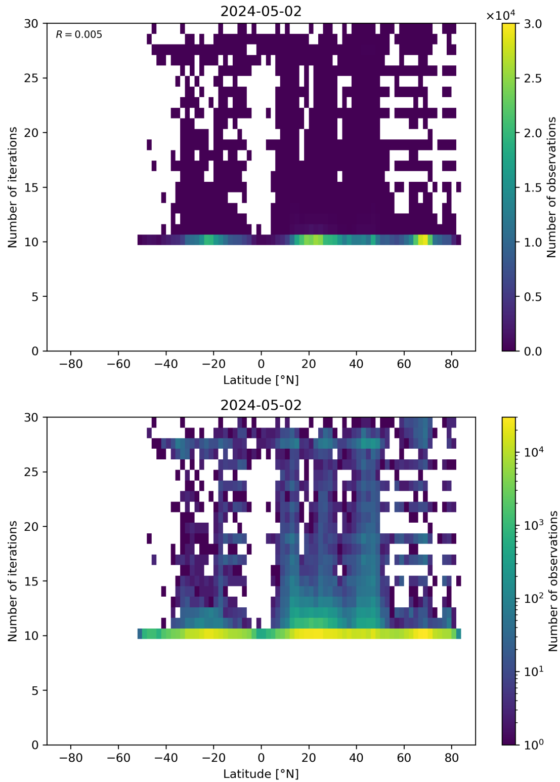
Figure 60: Scatter density plot of “Latitude” against “Number of iterations” for 2024-05-02 to 2024-05-03.
