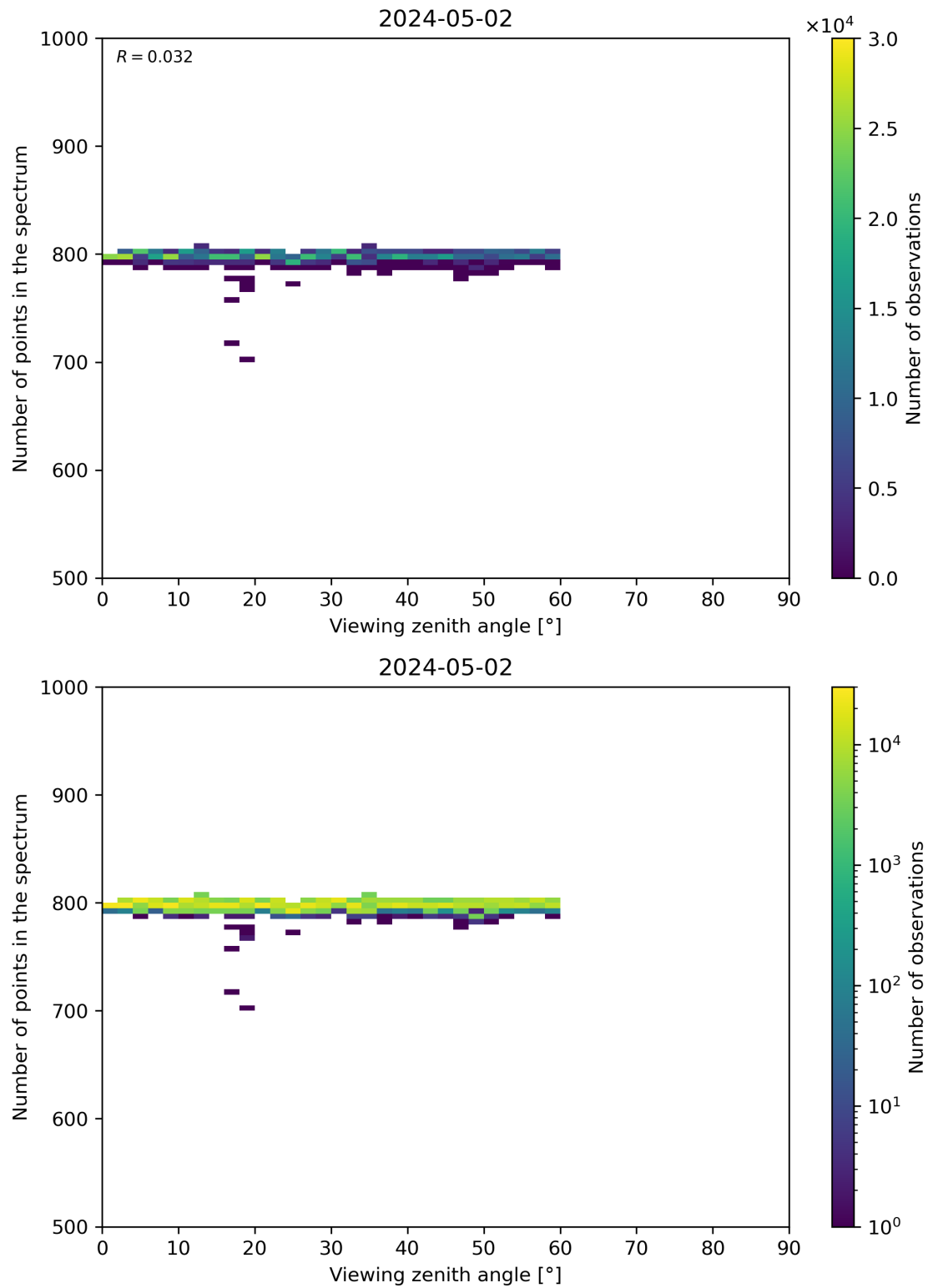
Figure 114: Scatter density plot of “Viewing zenith angle” against “Number of points in the spectrum” for 2024-05-02 to 2024-05-03.
