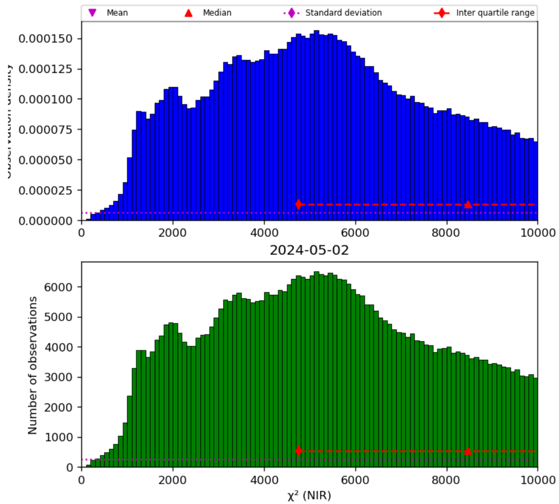
Figure 29: Histogram of “ \chi^2 (NIR)” for 2024-05-02 to 2024-05-03
