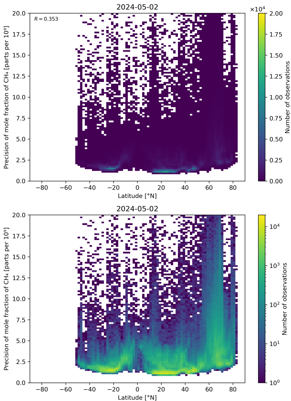
Figure 59: Scatter density plot of “Latitude” against “Precision of mole fraction of \text{CH}_4 ” for 2024-05-02 to 2024-05-03.
