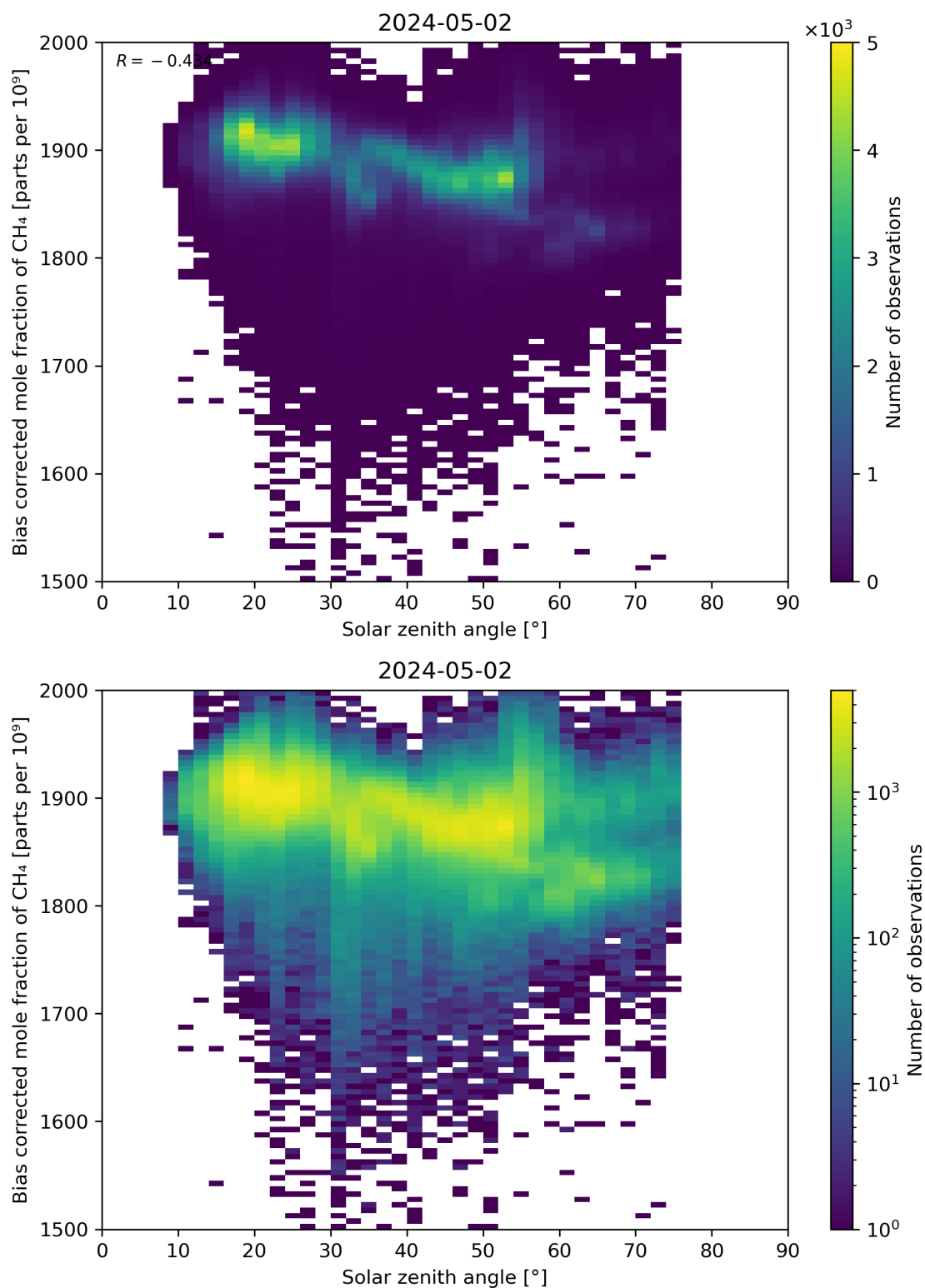
Figure 100: Scatter density plot of “Solar zenith angle” against “Bias corrected mole fraction of CH 4 ” for 2024-05-02 to 2024-05-03.
