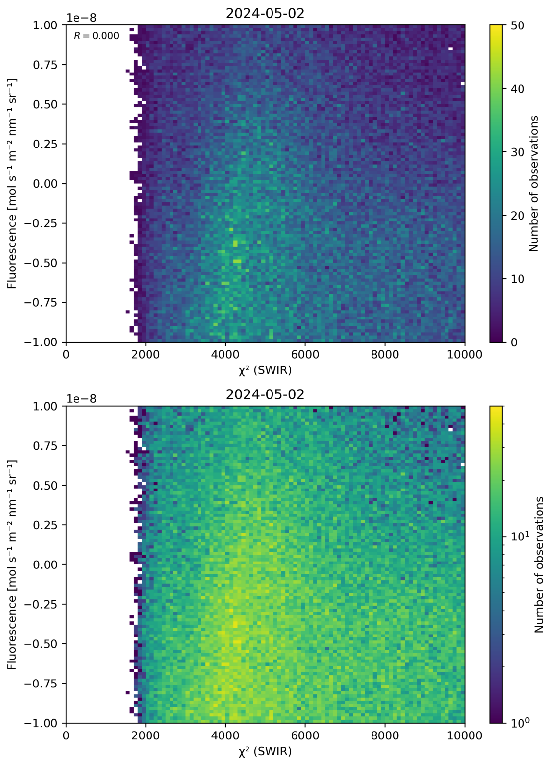
Figure 49: Scatter density plot of “ \chi^2 (SWIR)” against “Fluorescence” for 2024-05-02 to 2024-05-03.
