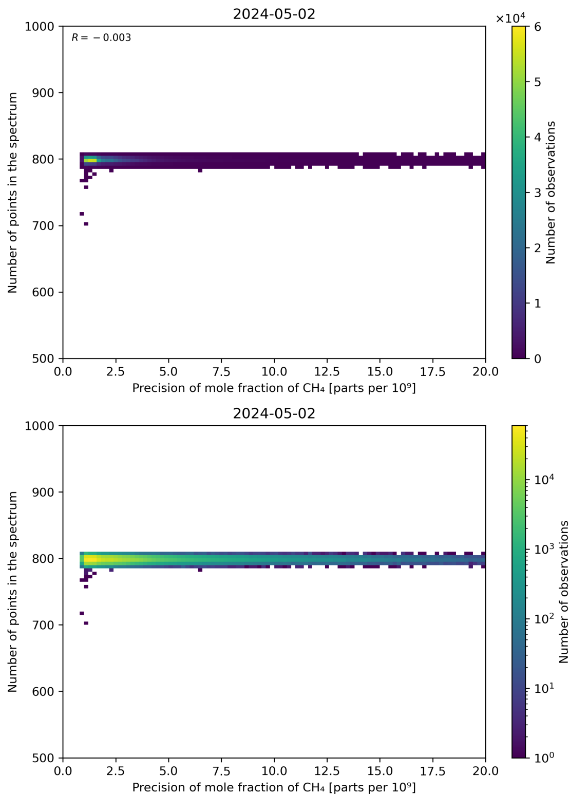
Figure 84: Scatter density plot of “Precision of mole fraction of CH 4 ” against “Number of points in the spectrum” for 2024-05-02 to 2024-05-03.
