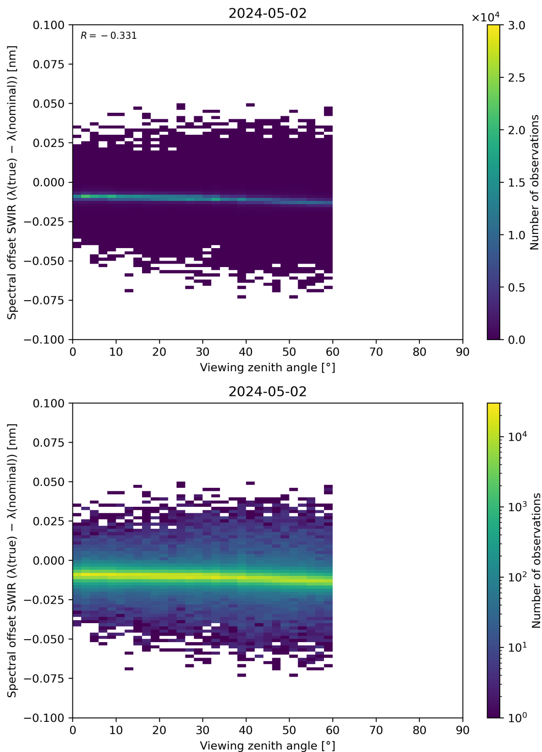
Figure 116: Scatter density plot of “Viewing zenith angle” against “Spectral offset SWIR ( \lambda(\text{true}) - \lambda(\text{nominal}) )” for 2024-05-02 to 2024-05-03.
