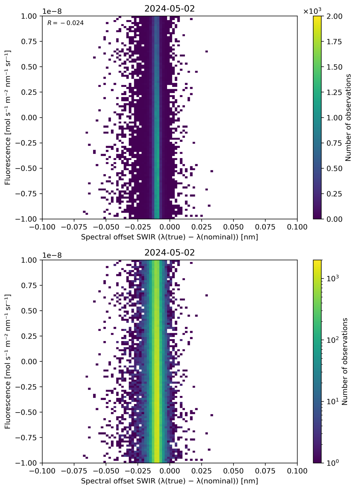
Figure 120: Scatter density plot of “Spectral offset SWIR ( \lambda(\text{true}) - \lambda(\text{nominal}) )” against “Fluorescence” for 2024-05-02 to 2024-05-03.
