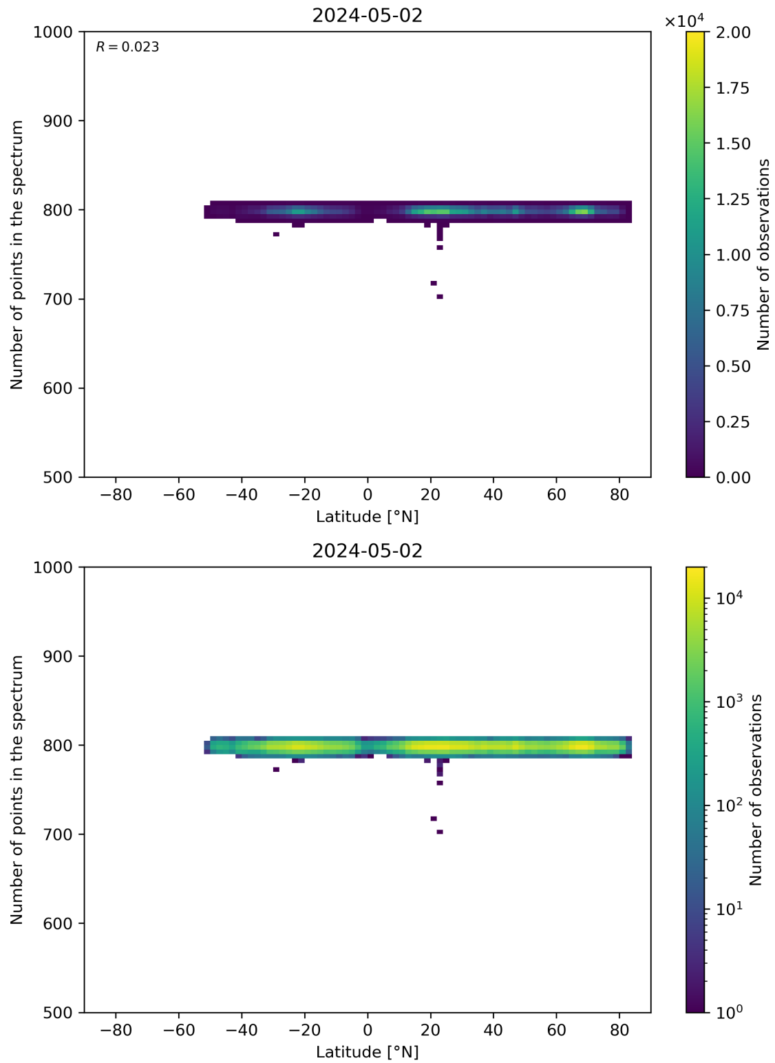
Figure 61: Scatter density plot of “Latitude” against “Number of points in the spectrum” for 2024-05-02 to 2024-05-03.
