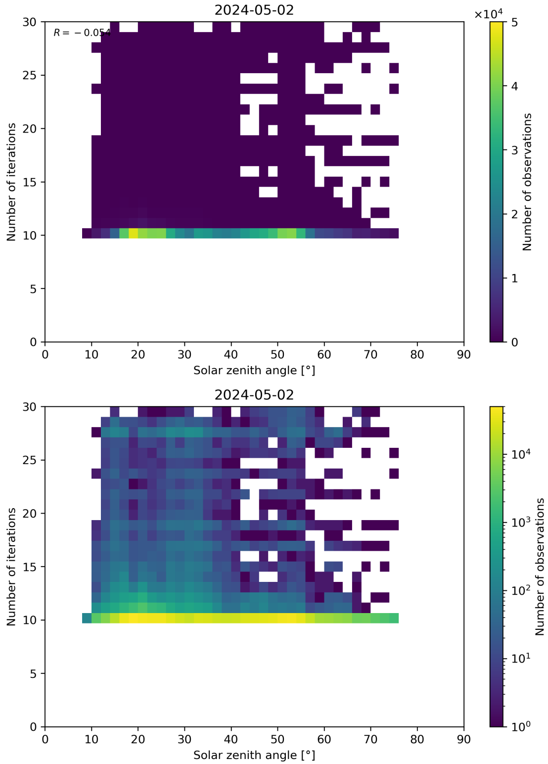
Figure 102: Scatter density plot of “Solar zenith angle” against “Number of iterations” for 2024-05-02 to 2024-05-03.
