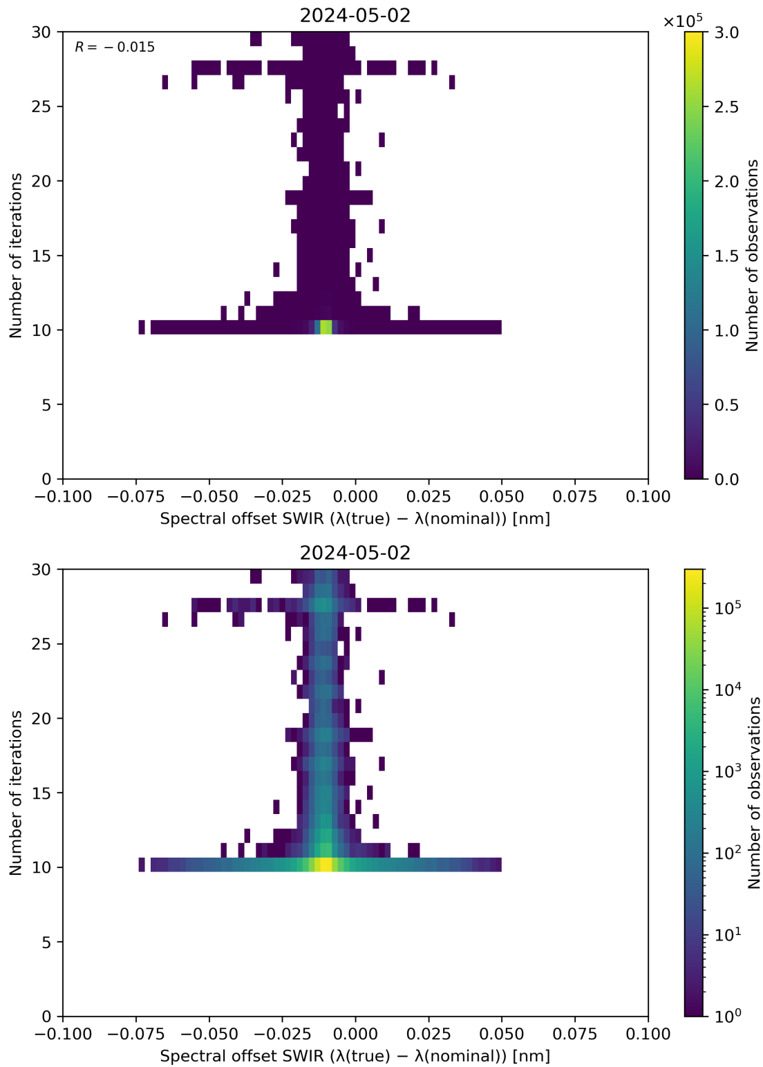
Figure 121: Scatter density plot of “Spectral offset SWIR ( \lambda(\text{true}) - \lambda(\text{nominal}) )” against “Number of iterations” for 2024-05-02 to 2024-05-03.
