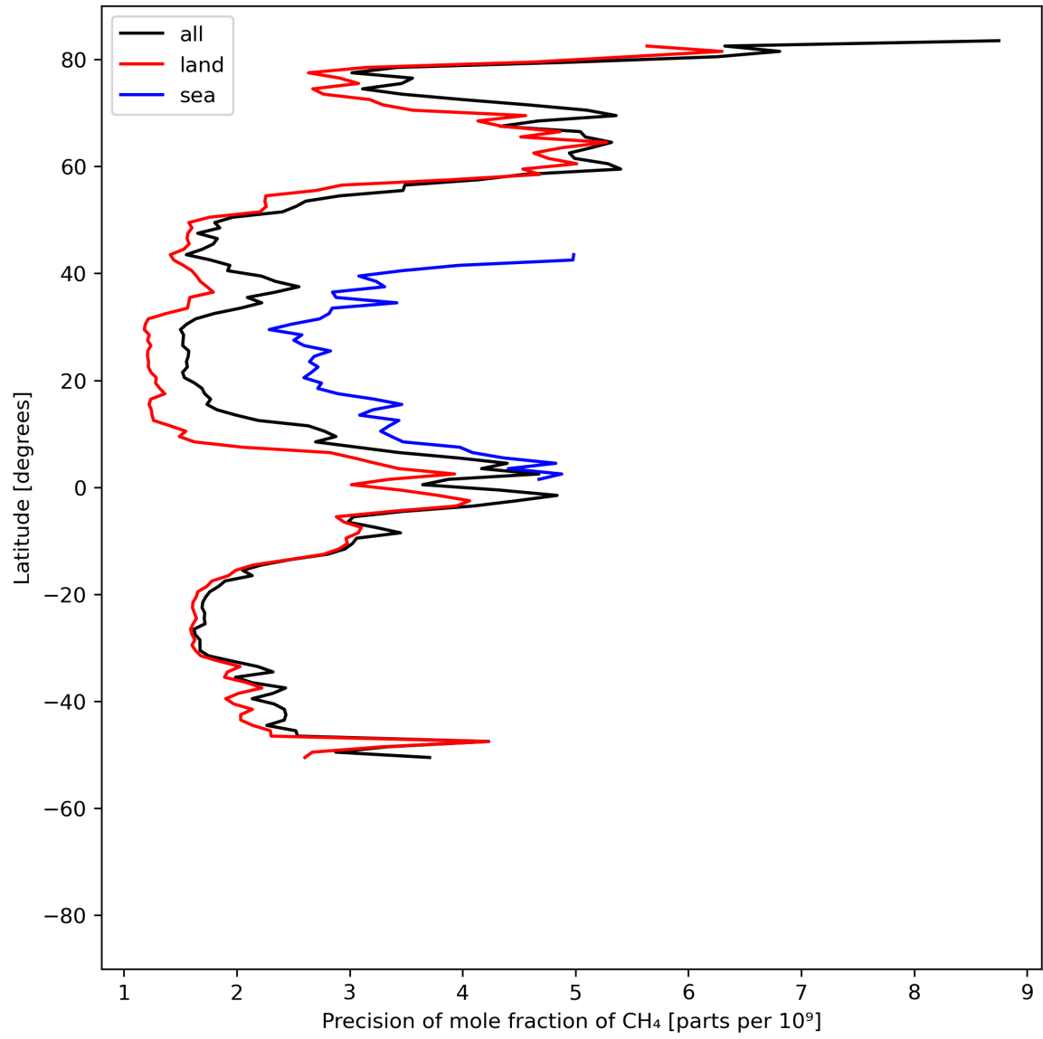
Figure 13: Zonal average of “Precision of mole fraction of \text{CH}_4 ” for 2024-05-02 to 2024-05-03.
