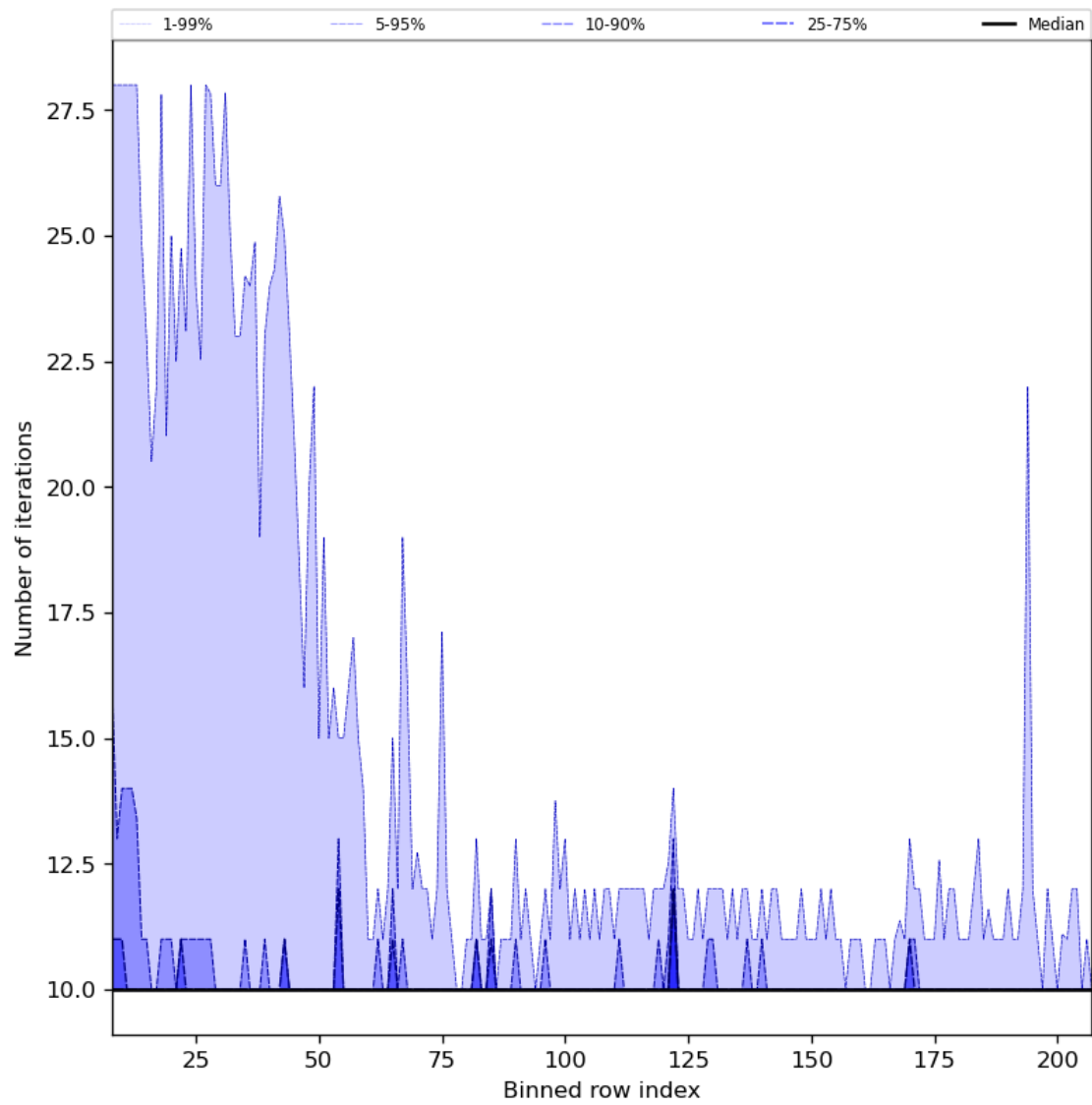
Figure 42: Along track statistics of “Number of iterations” for 2024-05-02 to 2024-05-03
