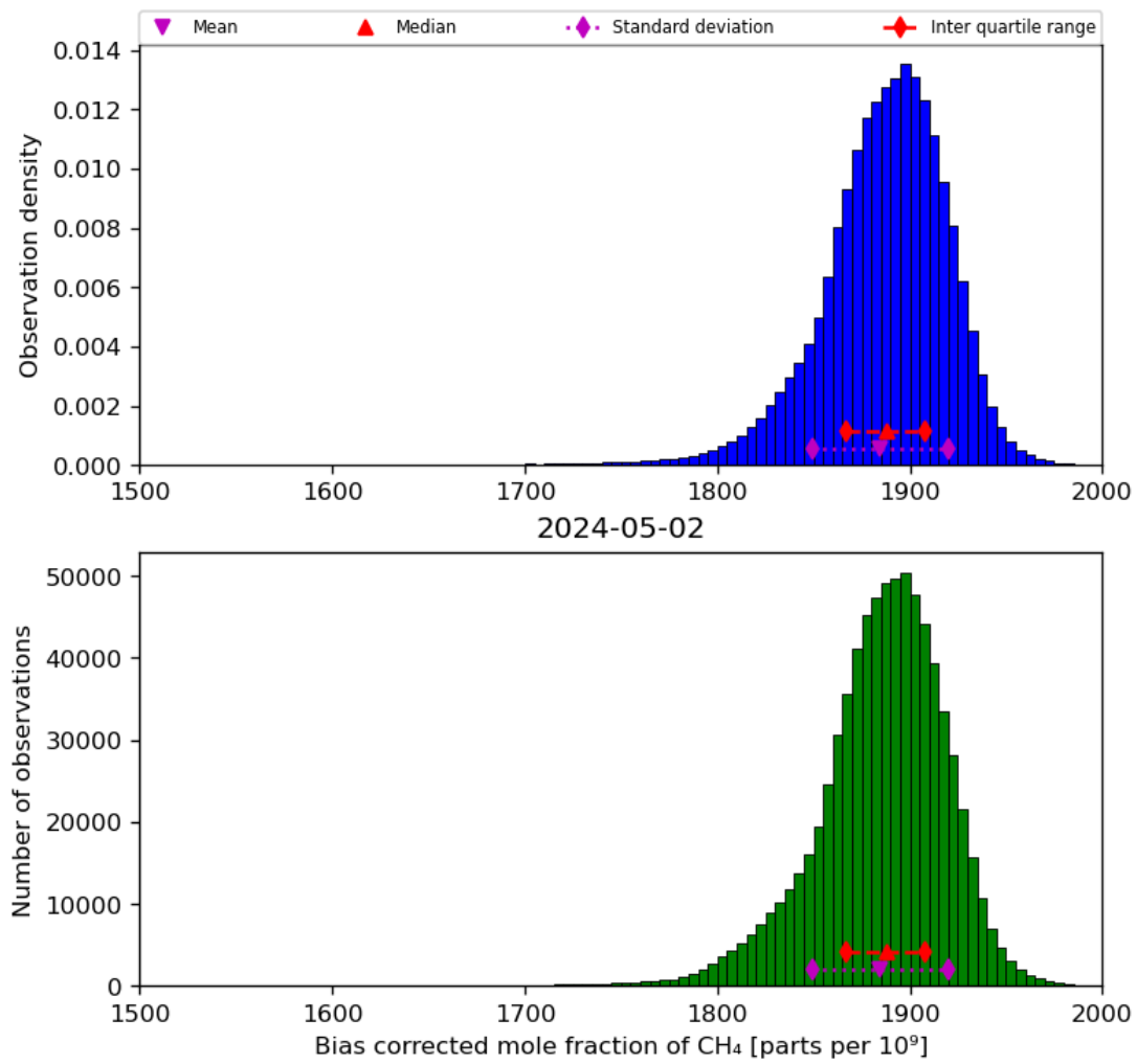
Figure 25: Histogram of “Bias corrected mole fraction of CH 4 ” for 2024-05-02 to 2024-05-03
