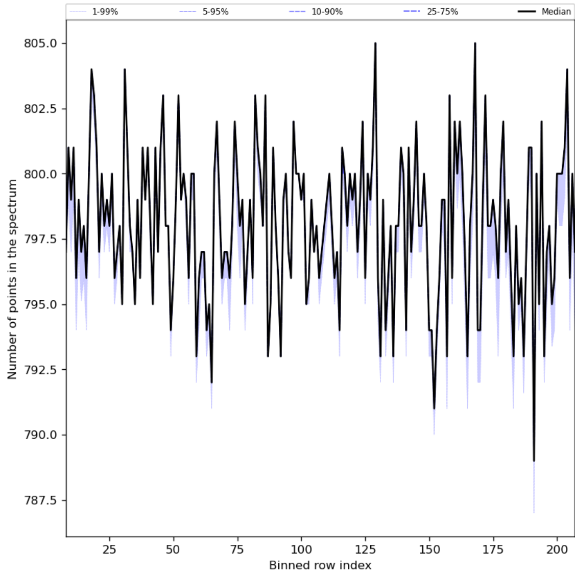
Figure 37: Along track statistics of “Number of points in the spectrum” for 2024-05-02 to 2024-05-03
