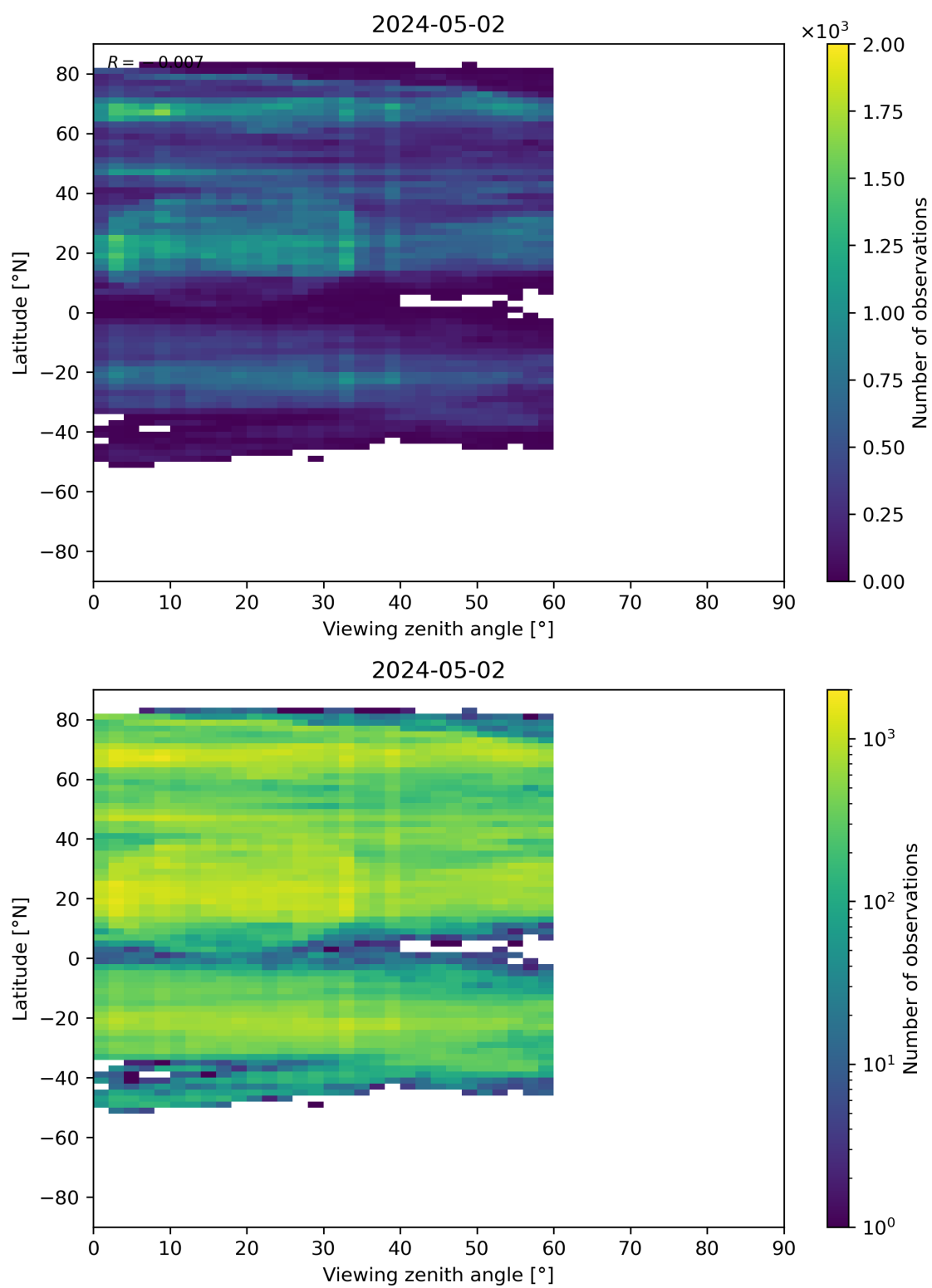
Figure 109: Scatter density plot of “Viewing zenith angle” against “Latitude” for 2024-05-02 to 2024-05-03.
