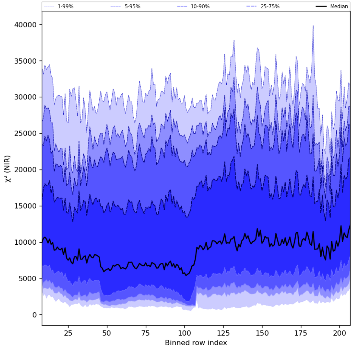
Figure 40: Along track statistics of “ \chi^2 (NIR)” for 2024-05-02 to 2024-05-03
