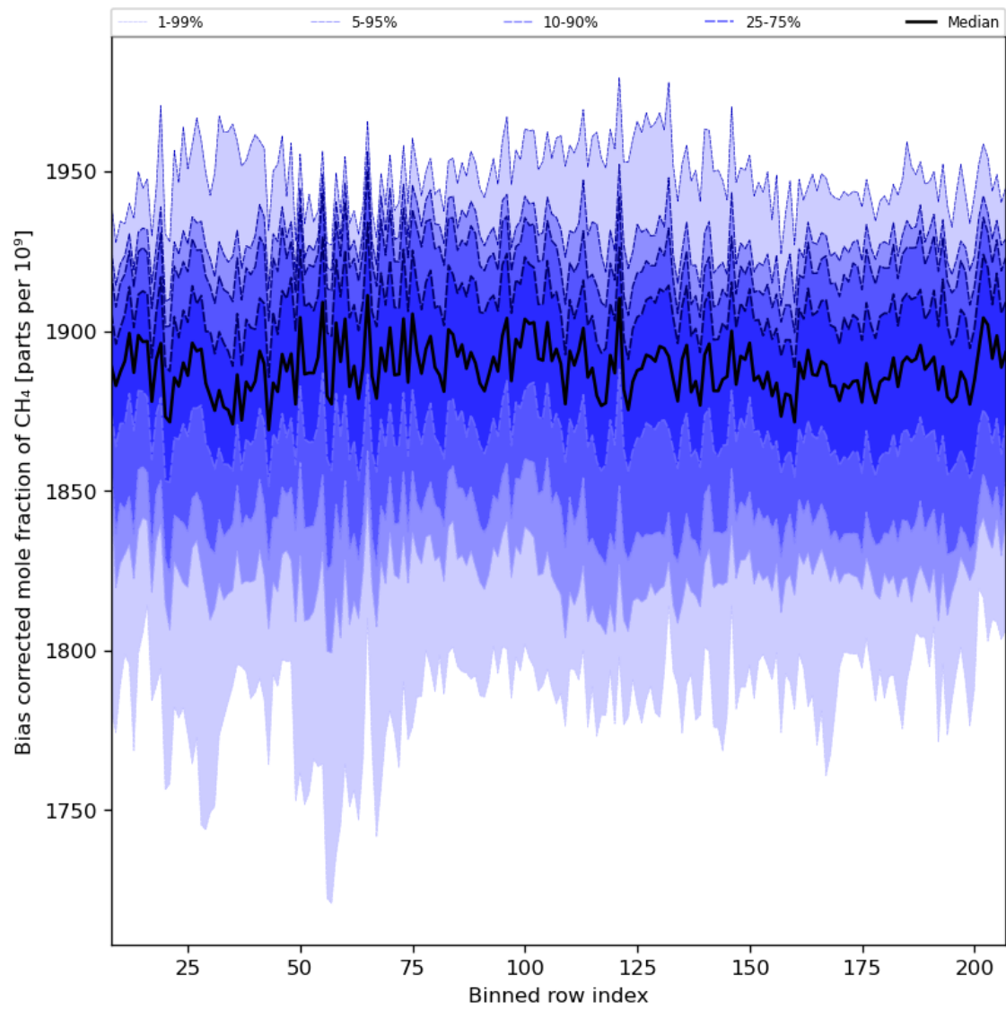
Figure 36: Along track statistics of “Bias corrected mole fraction of CH 4 ” for 2024-05-02 to 2024-05-03
