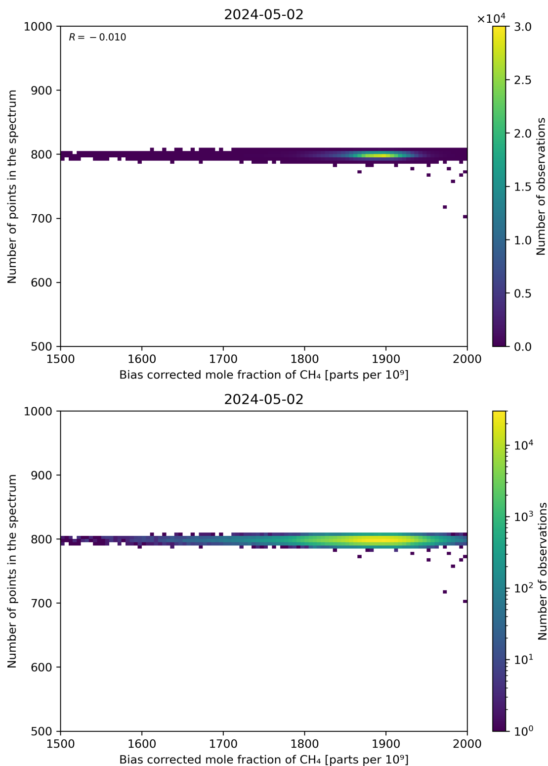
Figure 68: Scatter density plot of “Bias corrected mole fraction of CH 4 ” against “Number of points in the spectrum” for 2024-05-02 to 2024-05-03.
