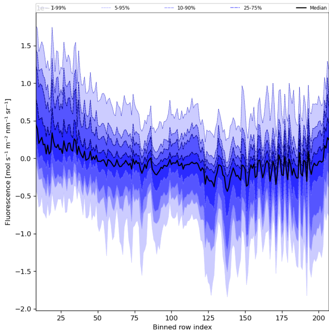
Figure 43: Along track statistics of “Fluorescence” for 2024-05-02 to 2024-05-03
