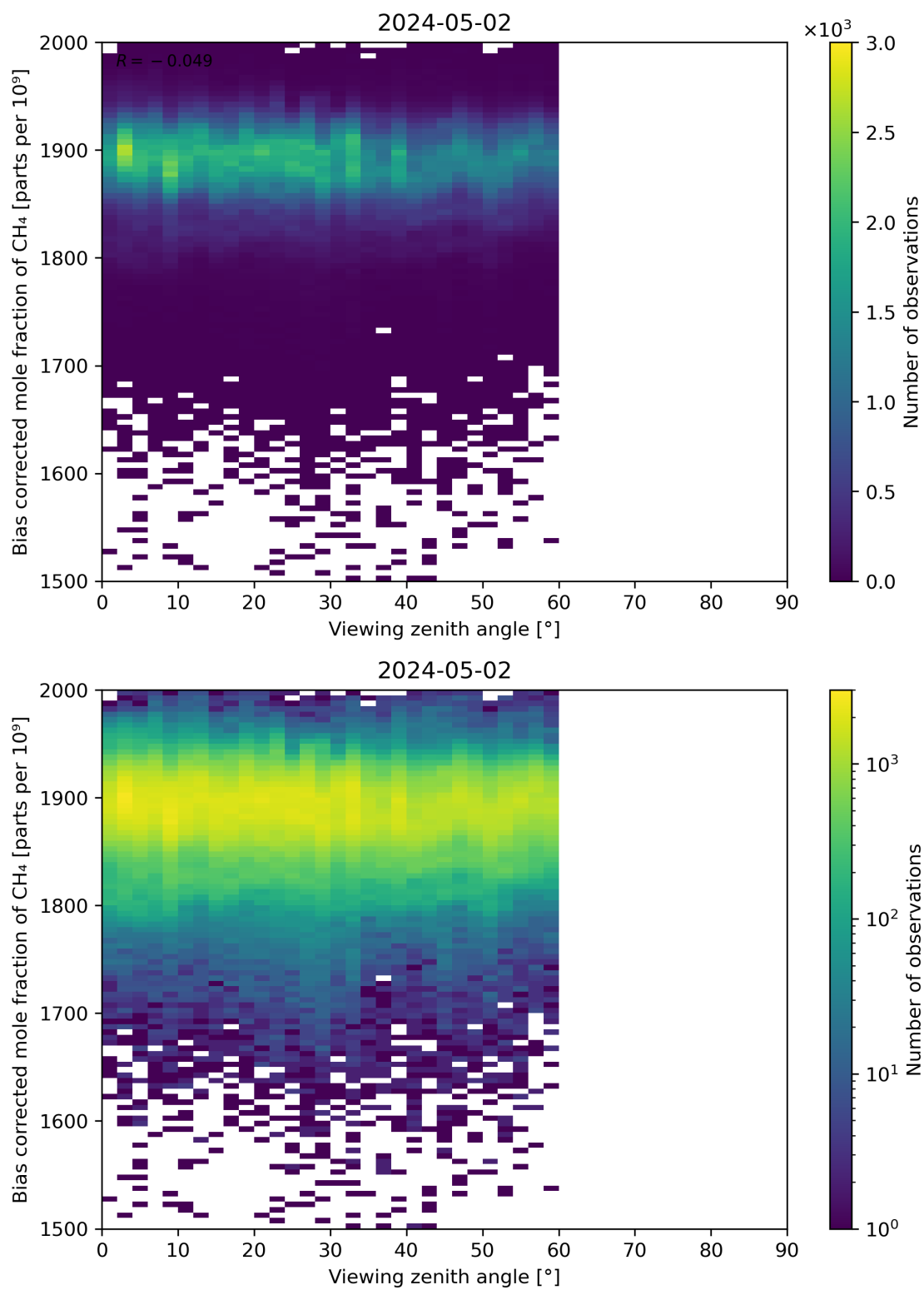
Figure 111: Scatter density plot of “Viewing zenith angle” against “Bias corrected mole fraction of CH 4 ” for 2024-05-02 to 2024-05-03.
