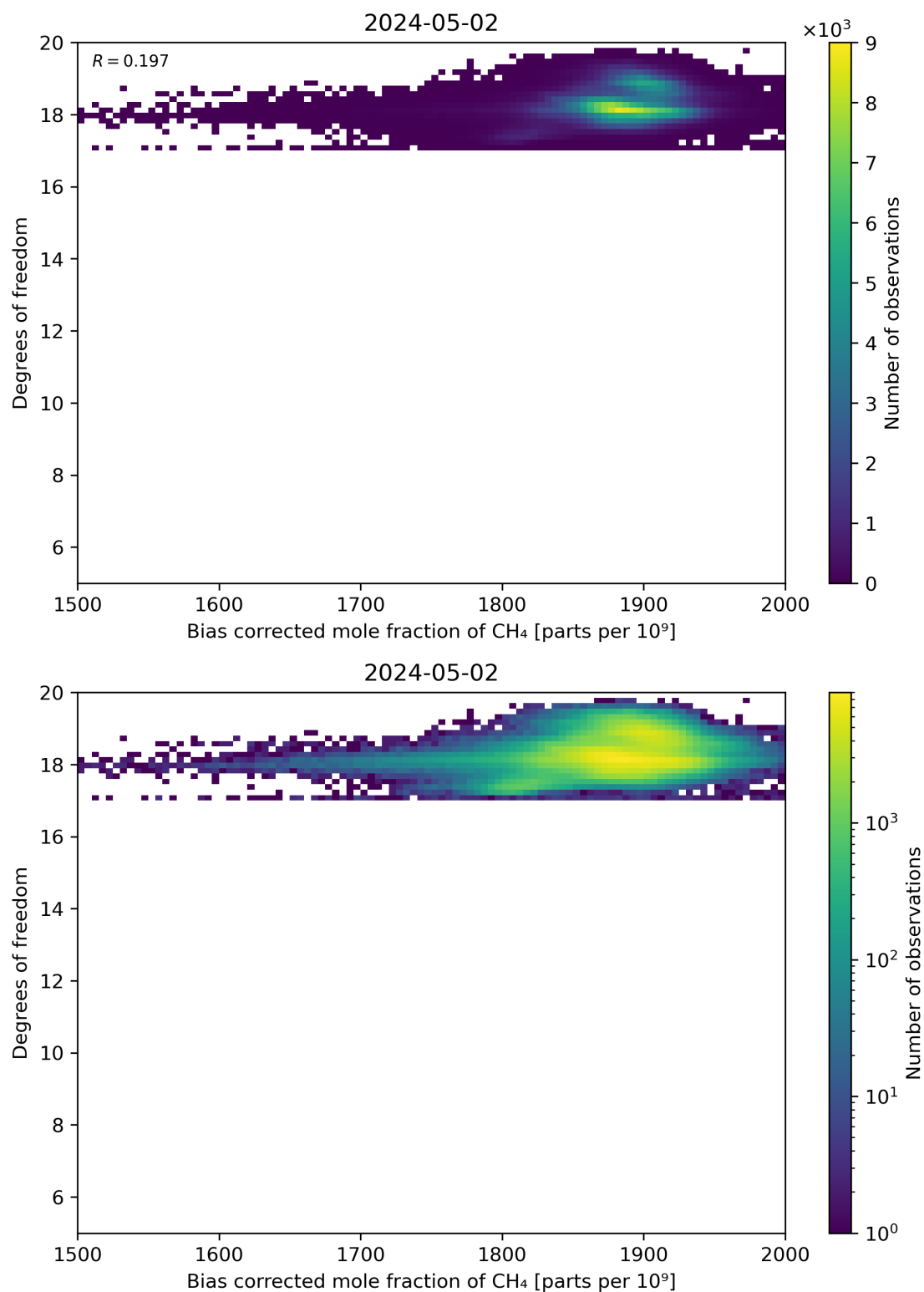
Figure 65: Scatter density plot of “Bias corrected mole fraction of CH 4 ” against “Degrees of freedom” for 2024-05-02 to 2024-05-03.
