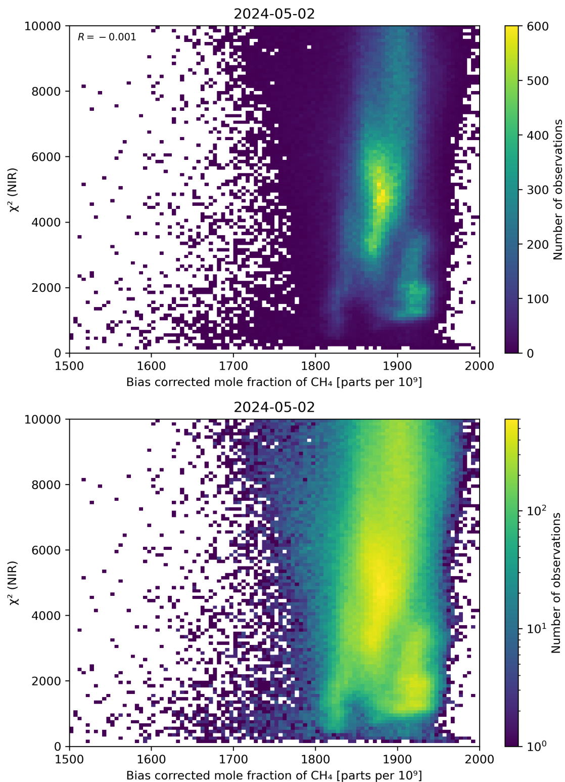
Figure 63: Scatter density plot of “Bias corrected mole fraction of CH 4 ” against “ \chi^2 (NIR)” for 2024-05-02 to 2024-05-03.
