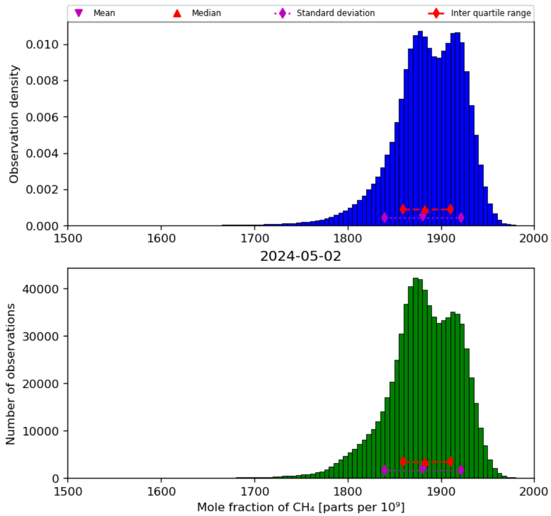
Figure 23: Histogram of “Mole fraction of CH 4 ” for 2024-05-02 to 2024-05-03
