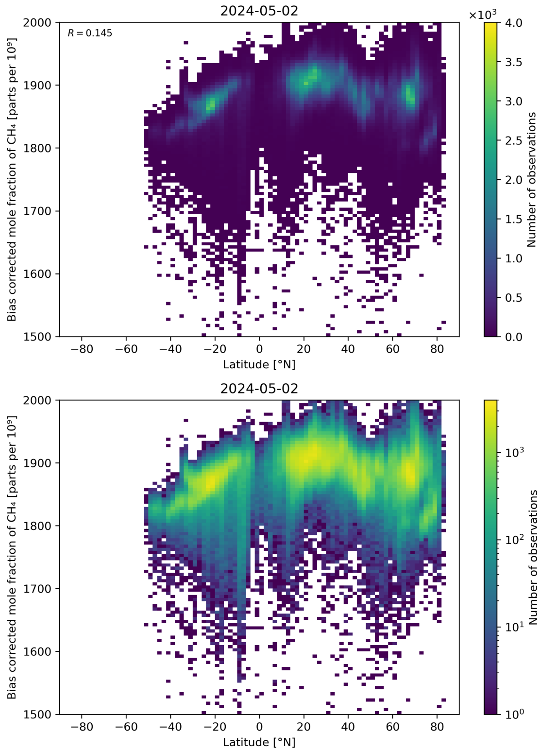
Figure 58: Scatter density plot of “Latitude” against “Bias corrected mole fraction of CH 4 ” for 2024-05-02 to 2024-05-03.
