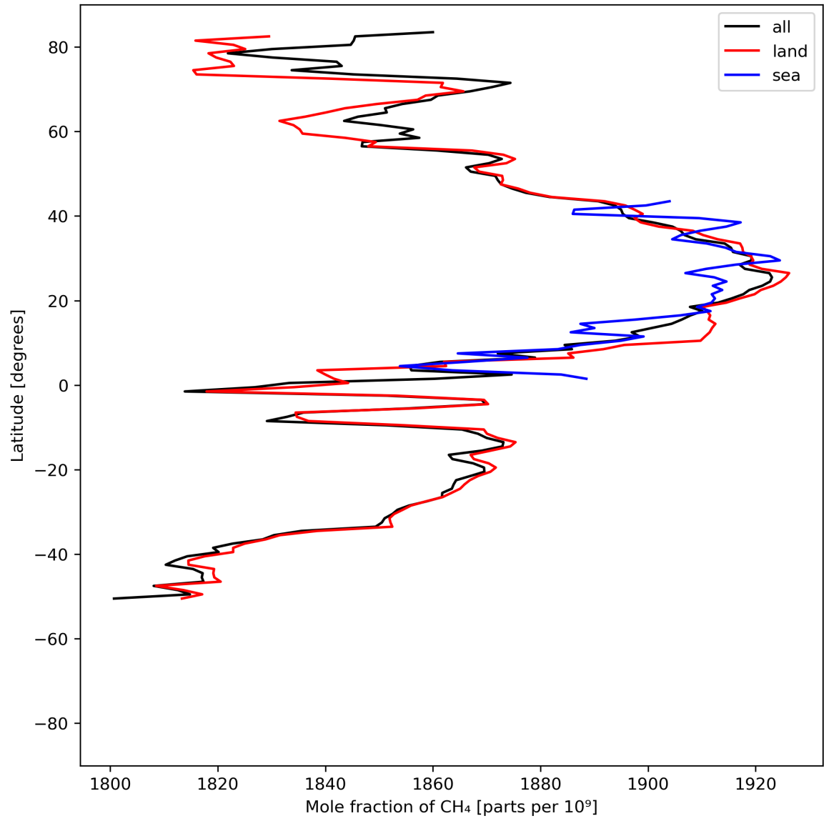
Figure 12: Zonal average of “Mole fraction of CH 4 ” for 2024-05-02 to 2024-05-03.
