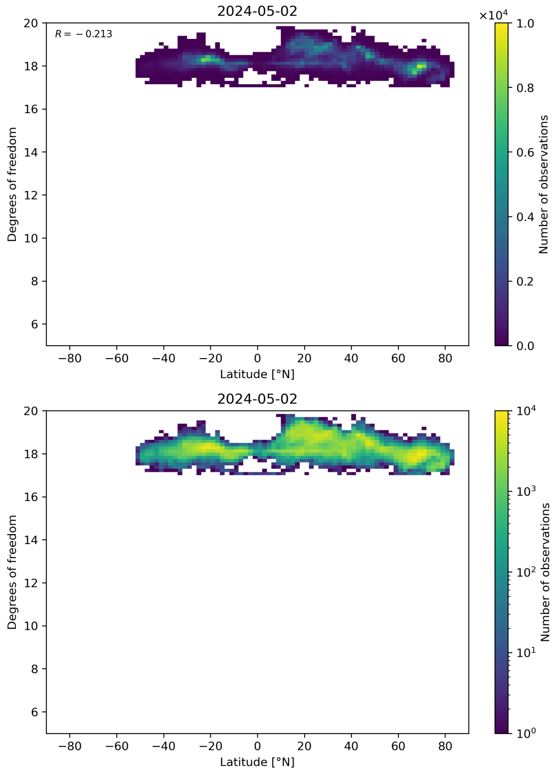
Figure 55: Scatter density plot of “Latitude” against “Degrees of freedom” for 2024-05-02 to 2024-05-03.
