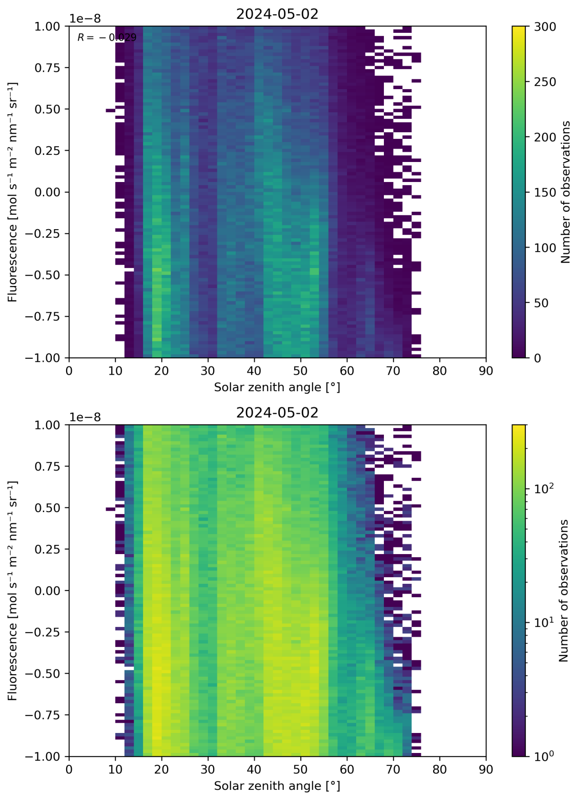
Figure 97: Scatter density plot of “Solar zenith angle” against “Fluorescence” for 2024-05-02 to 2024-05-03.
