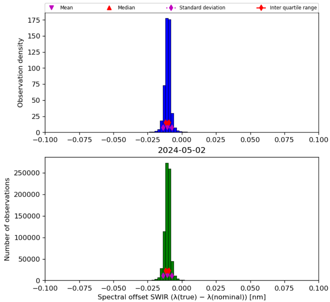
Figure 27: Histogram of “Spectral offset SWIR ( \lambda(\text{true}) - \lambda(\text{nominal}) )” for 2024-05-02 to 2024-05-03
