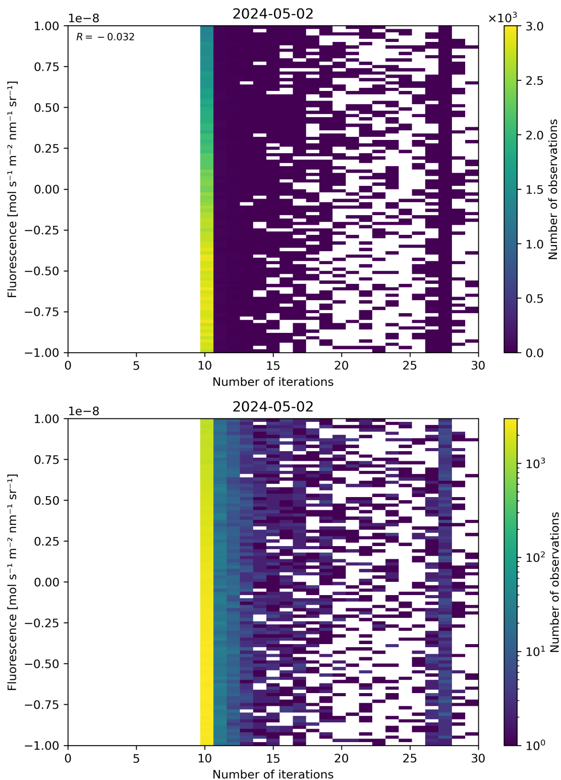
Figure 87: Scatter density plot of “Number of iterations” against “Fluorescence” for 2024-05-02 to 2024-05-03.
