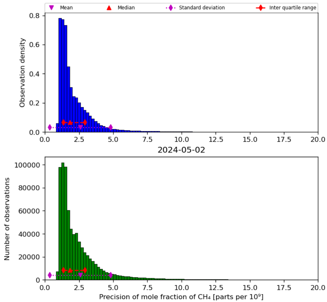
Figure 24: Histogram of “Precision of mole fraction of CH 4 ” for 2024-05-02 to 2024-05-03
