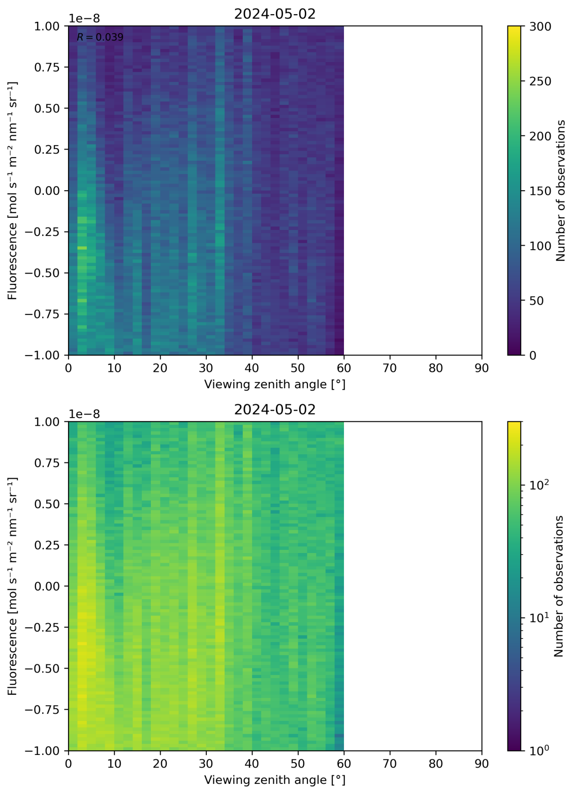
Figure 108: Scatter density plot of “Viewing zenith angle” against “Fluorescence” for 2024-05-02 to 2024-05-03.
