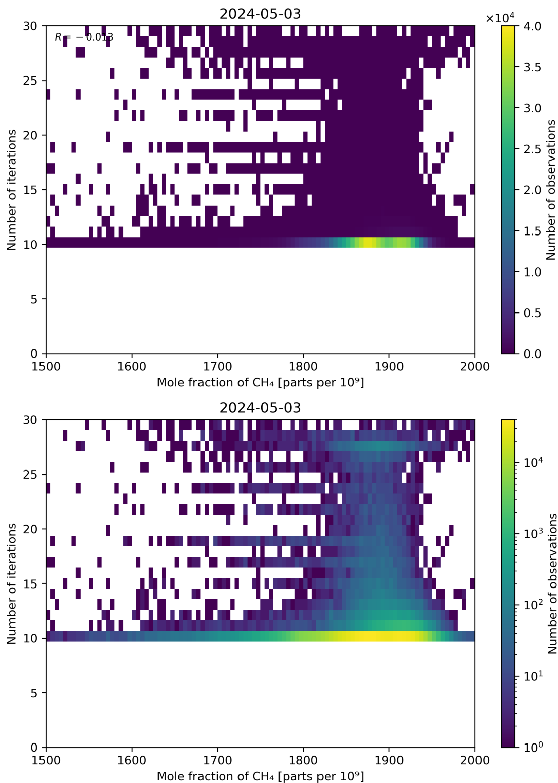
Figure 76: Scatter density plot of “Mole fraction of CH 4 ” against “Number of iterations” for 2024-05-02 to 2024-05-04.
