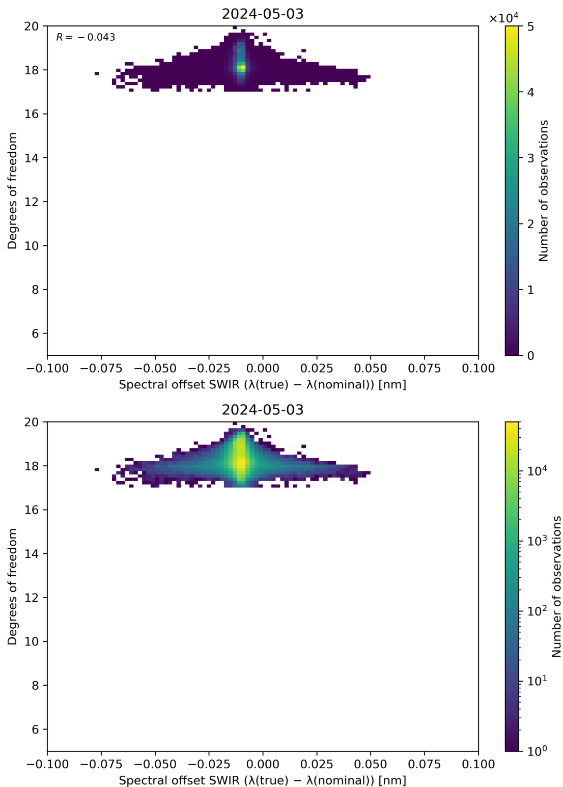
Figure 119: Scatter density plot of “Spectral offset SWIR ( \lambda(\text{true}) - \lambda(\text{nominal}) )” against “Degrees of freedom” for 2024-05-02 to 2024-05-04.
