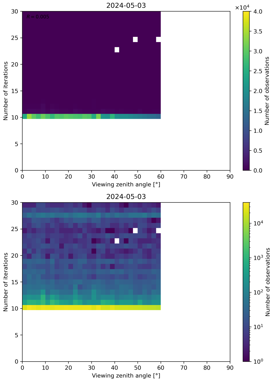
Figure 113: Scatter density plot of “Viewing zenith angle” against “Number of iterations” for 2024-05-02 to 2024-05-04.
