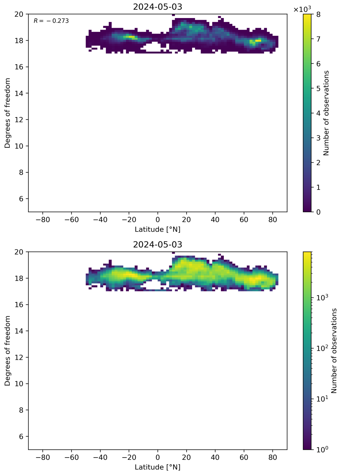
Figure 55: Scatter density plot of “Latitude” against “Degrees of freedom” for 2024-05-02 to 2024-05-04.
