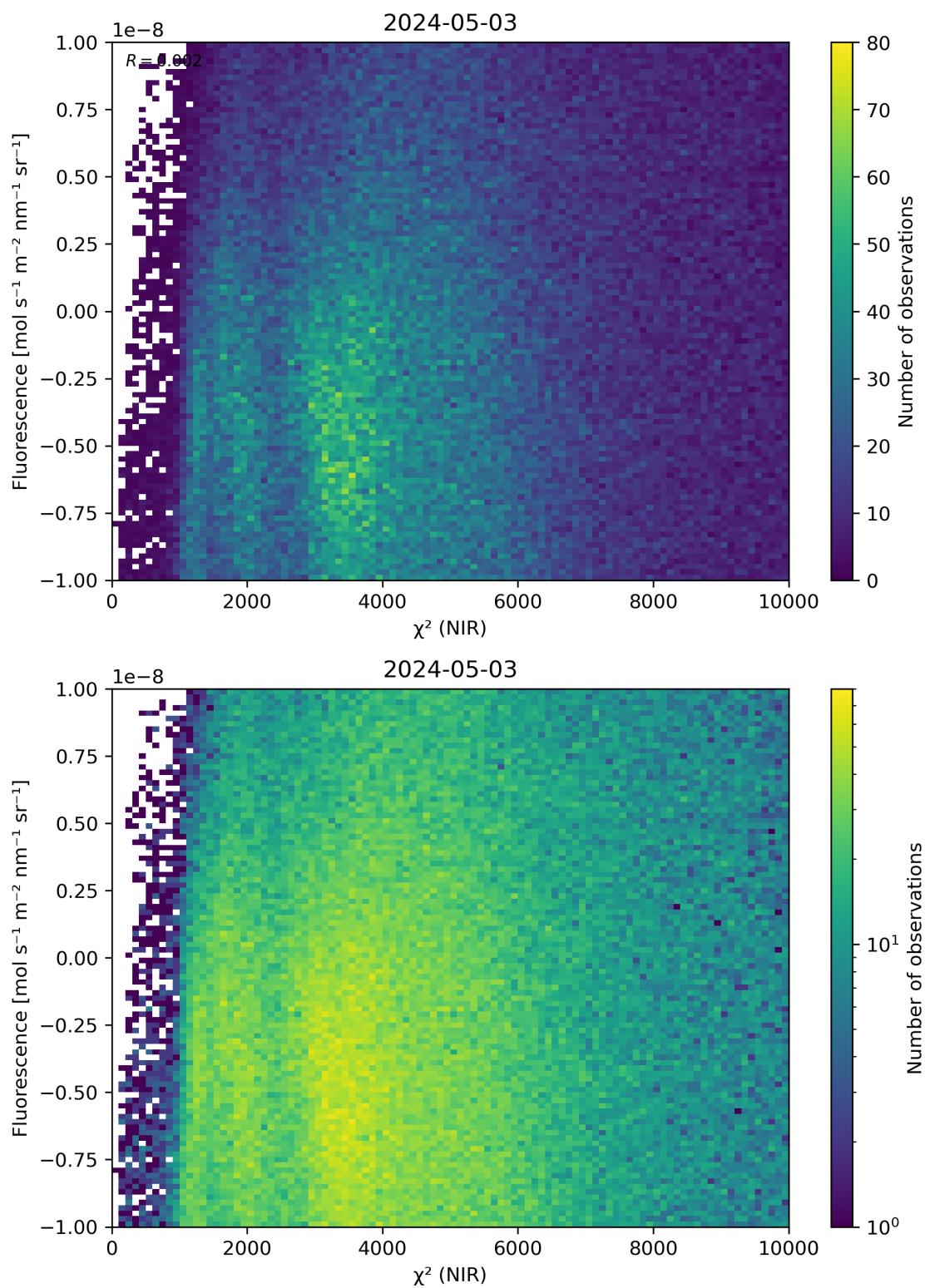
Figure 45: Scatter density plot of “ \chi^2 (NIR)” against “Fluorescence” for 2024-05-02 to 2024-05-04.
