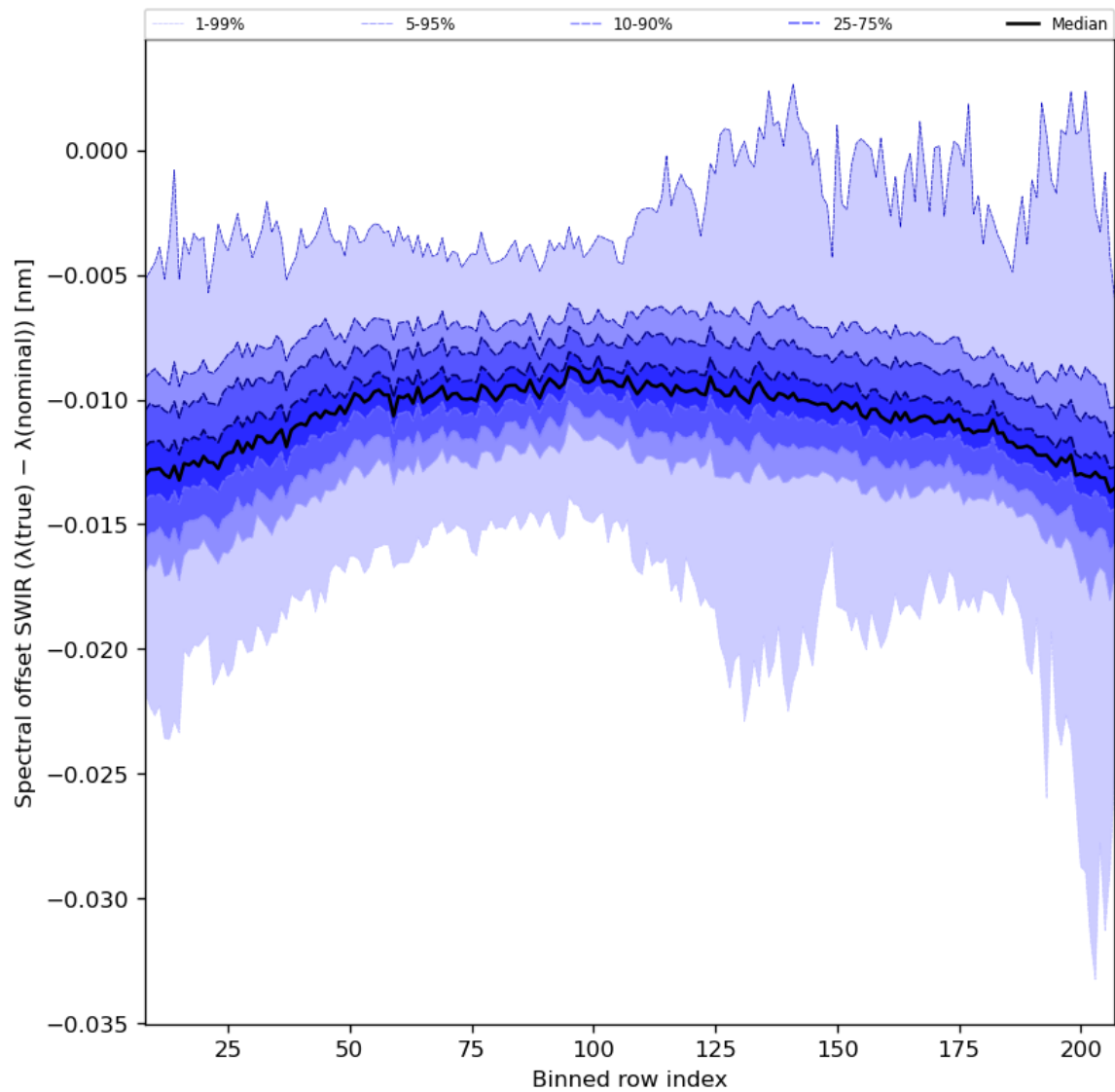
Figure 38: Along track statistics of “Spectral offset SWIR ( \lambda(\text{true}) - \lambda(\text{nominal}) )” for 2024-05-02 to 2024-05-04
