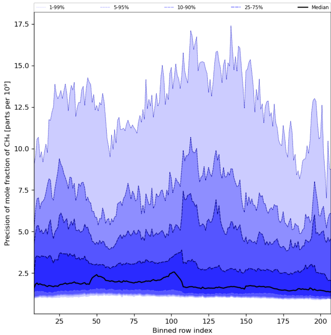
Figure 35: Along track statistics of “Precision of mole fraction of CH 4 ” for 2024-05-02 to 2024-05-04
