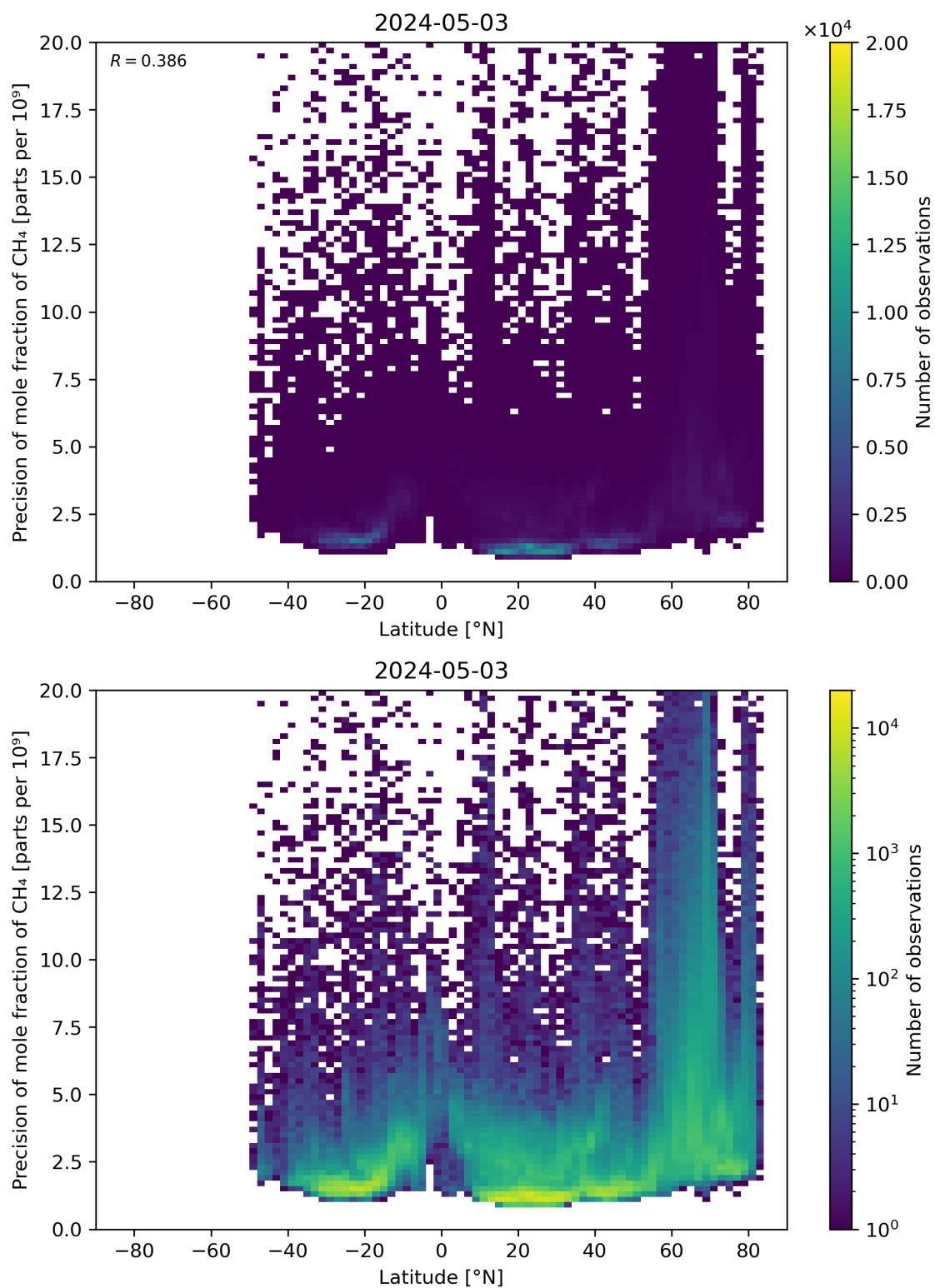
Figure 59: Scatter density plot of “Latitude” against “Precision of mole fraction of CH 4 ” for 2024-05-02 to 2024-05-04.
