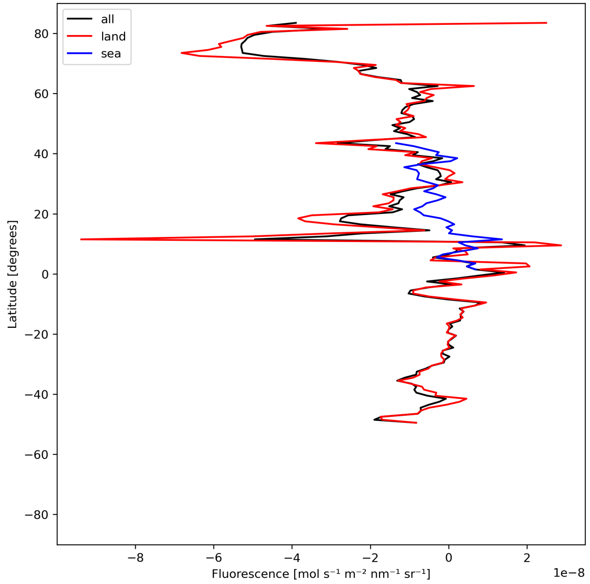
Figure 21: Zonal average of “Fluorescence” for 2024-05-02 to 2024-05-04.
