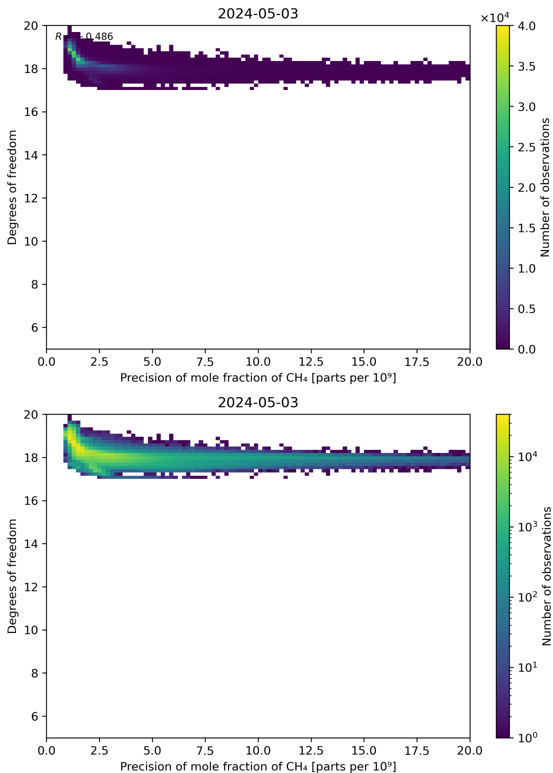
Figure 80: Scatter density plot of “Precision of mole fraction of CH 4 ” against “Degrees of freedom” for 2024-05-02 to 2024-05-04.
