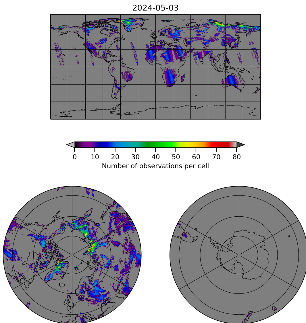
Figure 10: Map of the number of observations for 2024-05-02 to 2024-05-04
