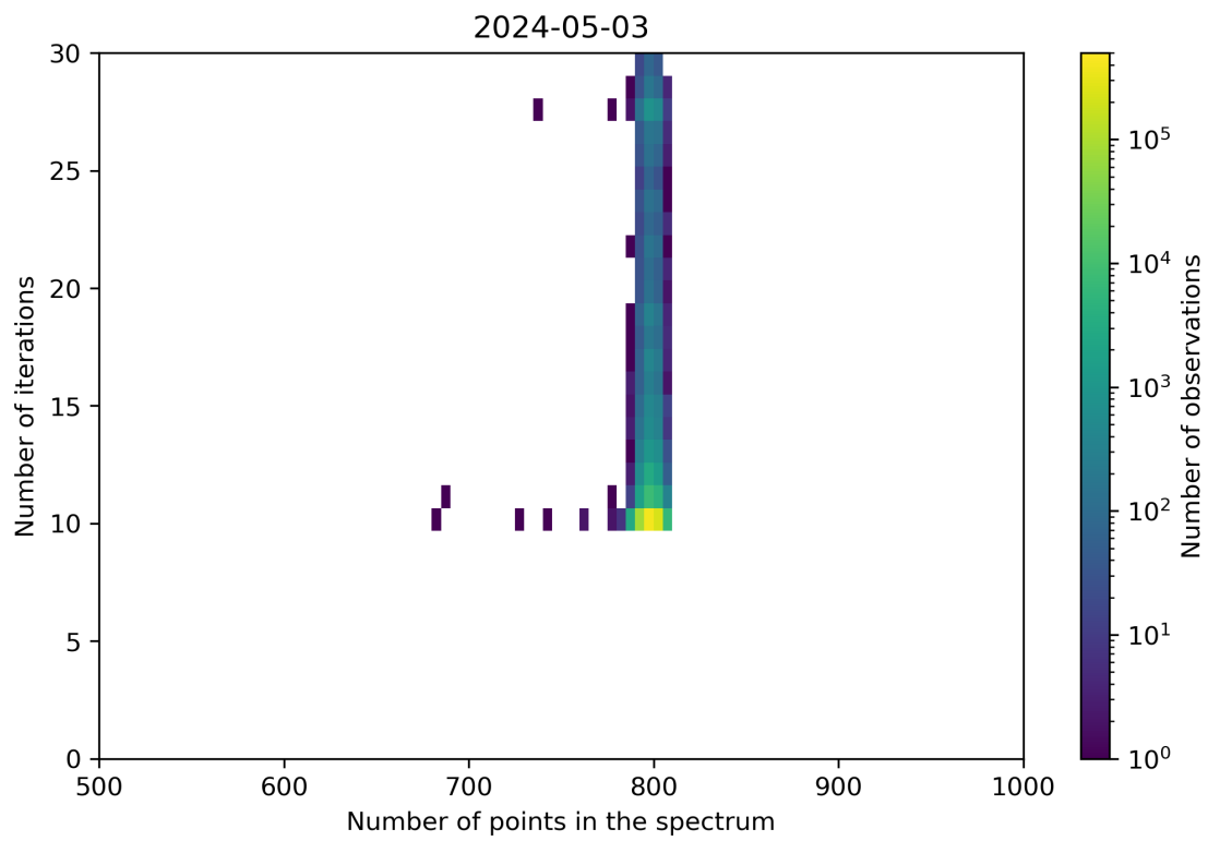
Figure 92: Scatter density plot of “Number of points in the spectrum” against “Number of iterations” for 2024-05-02 to 2024-05-04.
