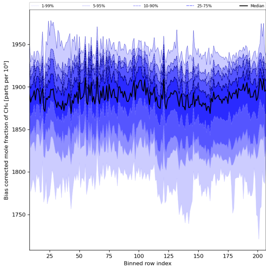
Figure 36: Along track statistics of “Bias corrected mole fraction of CH 4 ” for 2024-05-02 to 2024-05-04
