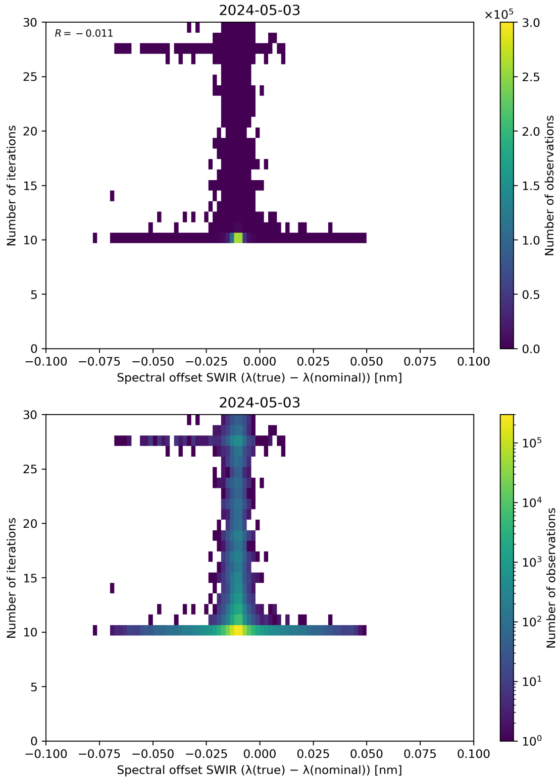
Figure 121: Scatter density plot of “Spectral offset SWIR ( \lambda(\text{true}) - \lambda(\text{nominal}) )” against “Number of iterations” for 2024-05-02 to 2024-05-04.
