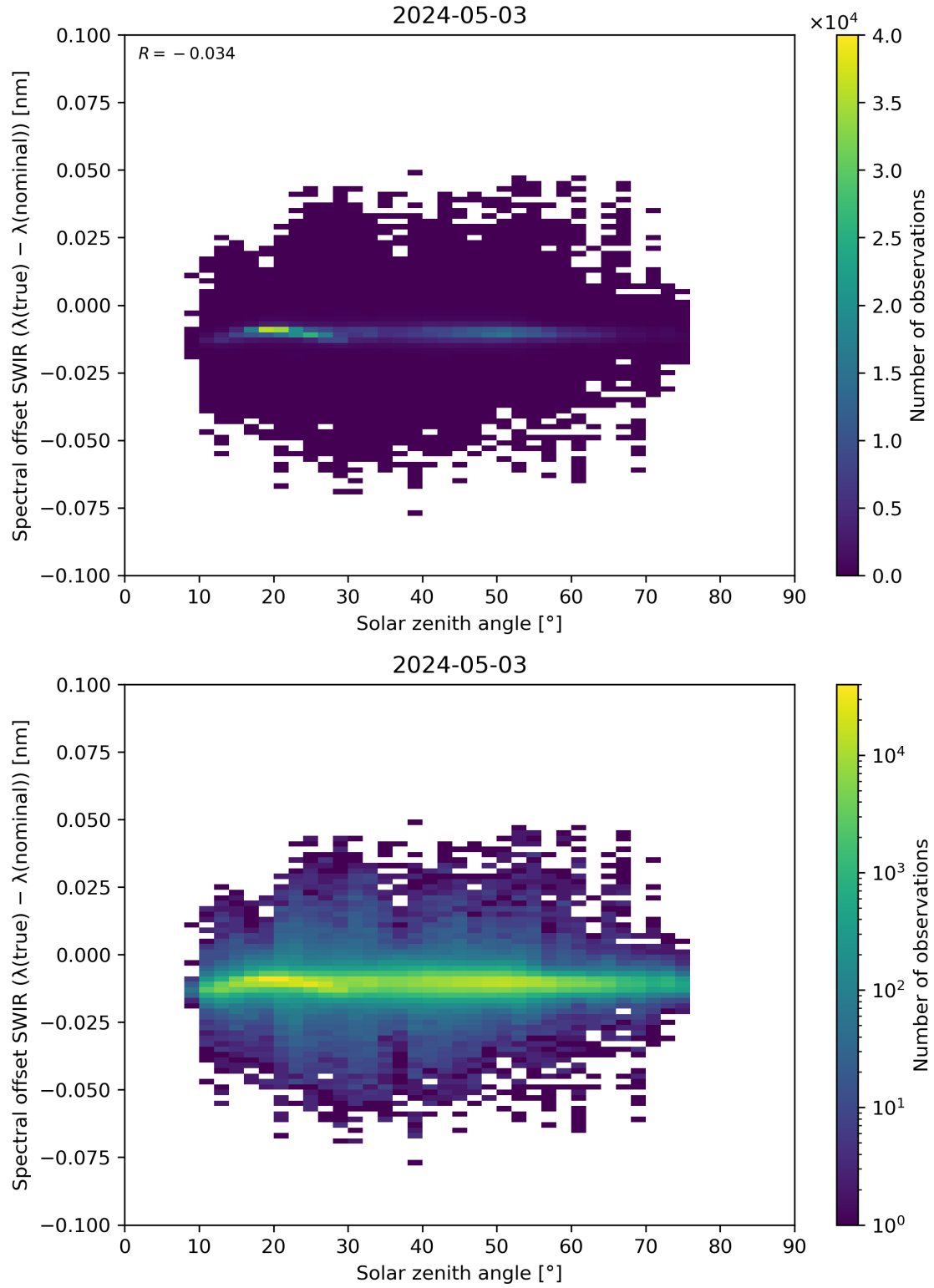
Figure 104: Scatter density plot of “Solar zenith angle” against “Spectral offset SWIR ( \lambda(\text{true}) - \lambda(\text{nominal}) )” for 2024-05-02 to 2024-05-04.
