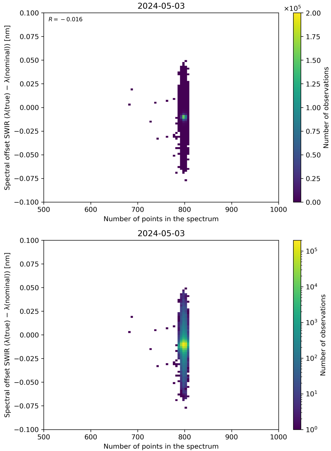
Figure 93: Scatter density plot of “Number of points in the spectrum” against “Spectral offset SWIR ( \lambda(\text{true}) - \lambda(\text{nominal}) )” for 2024-05-02 to 2024-05-04.
