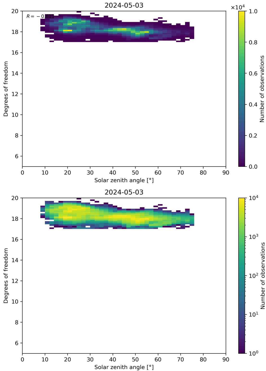
Figure 96: Scatter density plot of “Solar zenith angle” against “Degrees of freedom” for 2024-05-02 to 2024-05-04.
