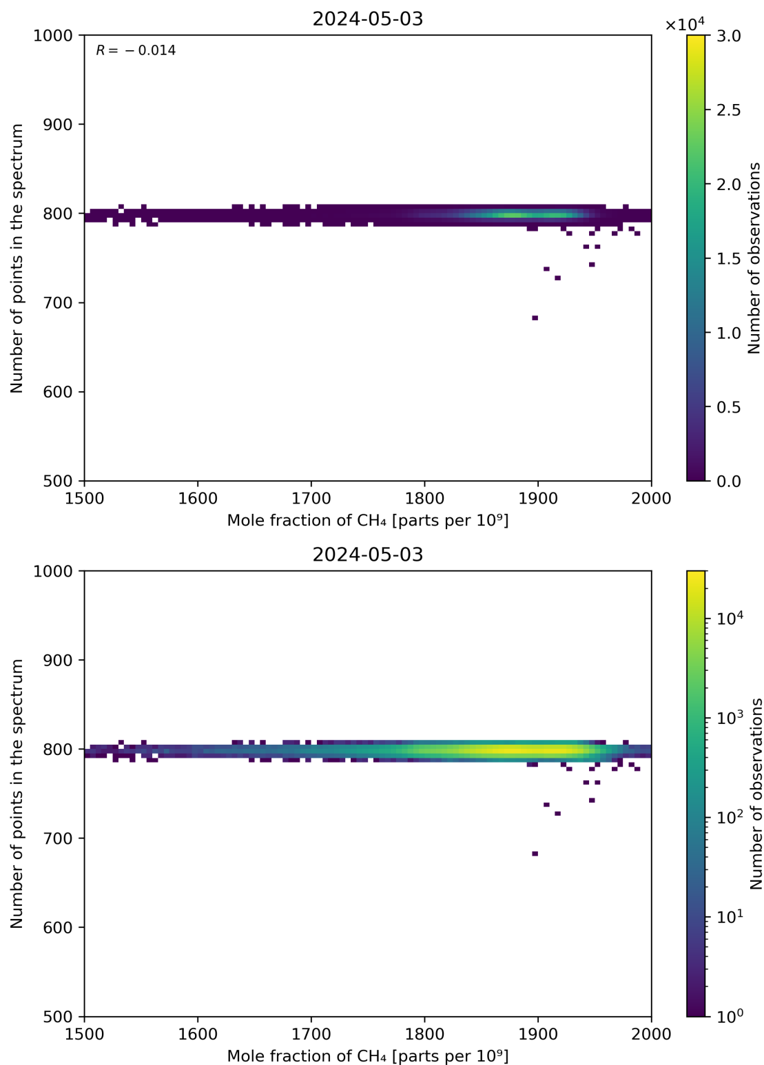
Figure 77: Scatter density plot of “Mole fraction of CH 4 ” against “Number of points in the spectrum” for 2024-05-02 to 2024-05-04.
