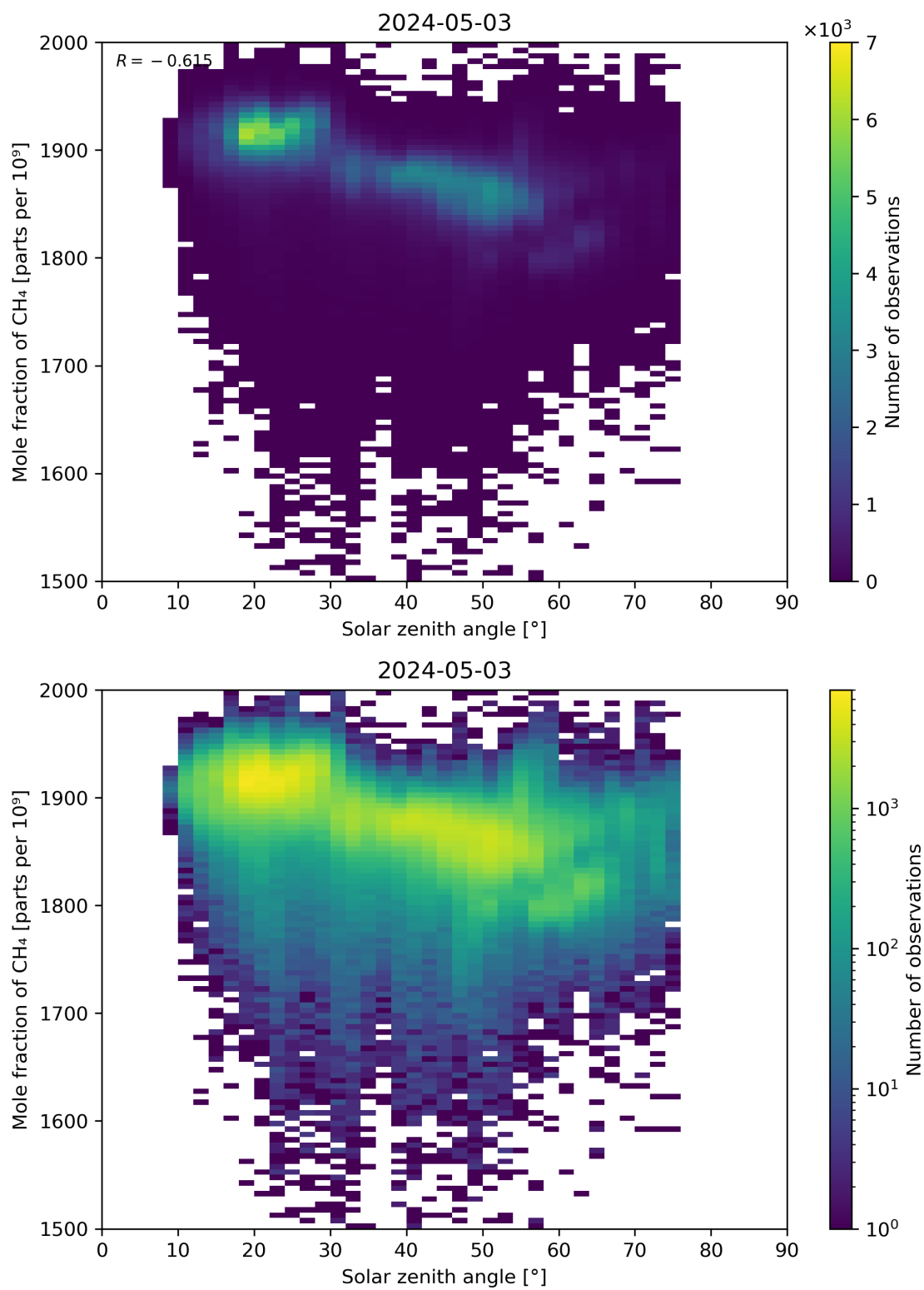
Figure 99: Scatter density plot of “Solar zenith angle” against “Mole fraction of CH 4 ” for 2024-05-02 to 2024-05-04.
