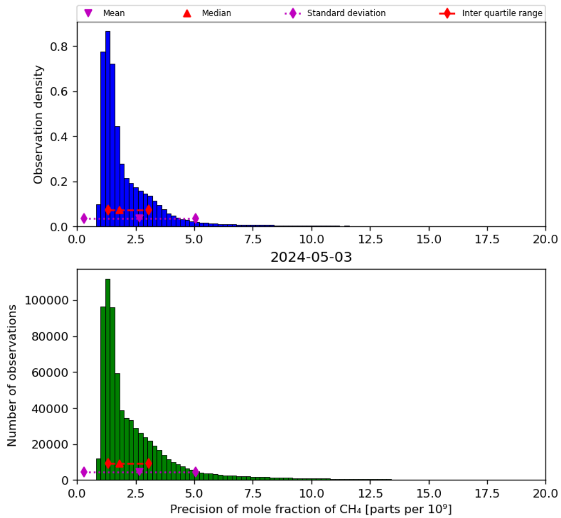
Figure 24: Histogram of “Precision of mole fraction of CH 4 ” for 2024-05-02 to 2024-05-04
