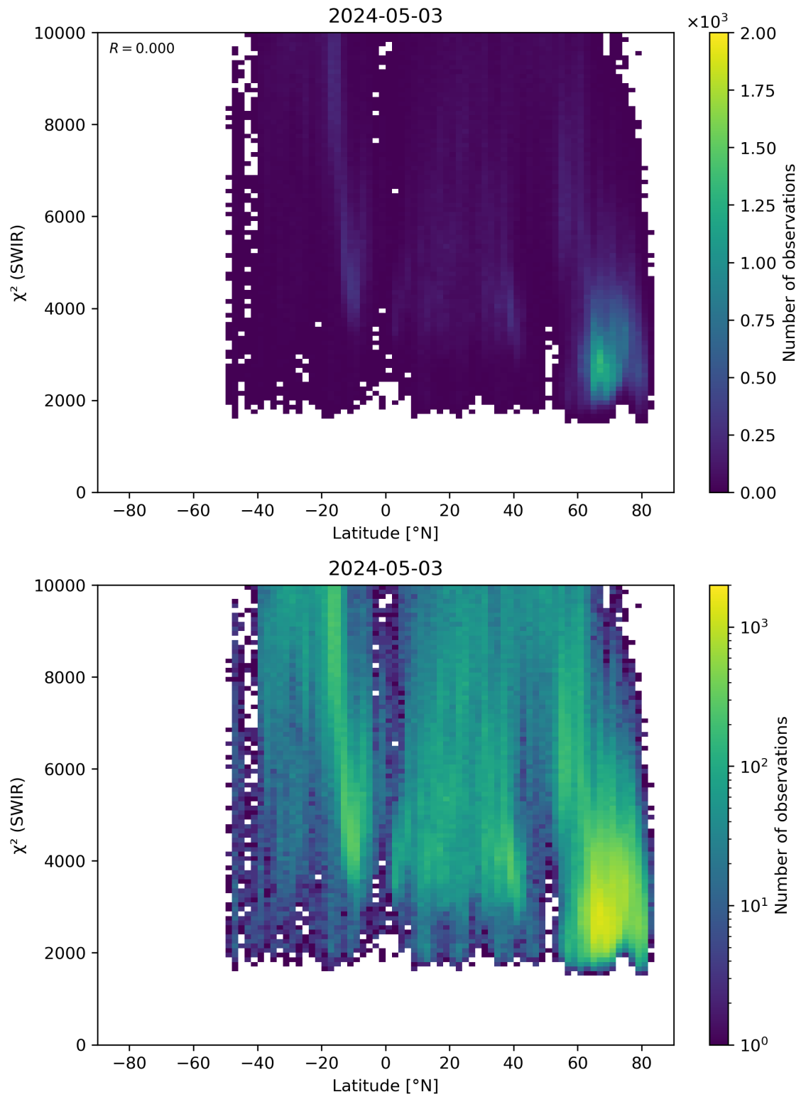
Figure 54: Scatter density plot of “Latitude” against “ \chi^2 (SWIR)” for 2024-05-02 to 2024-05-04.
