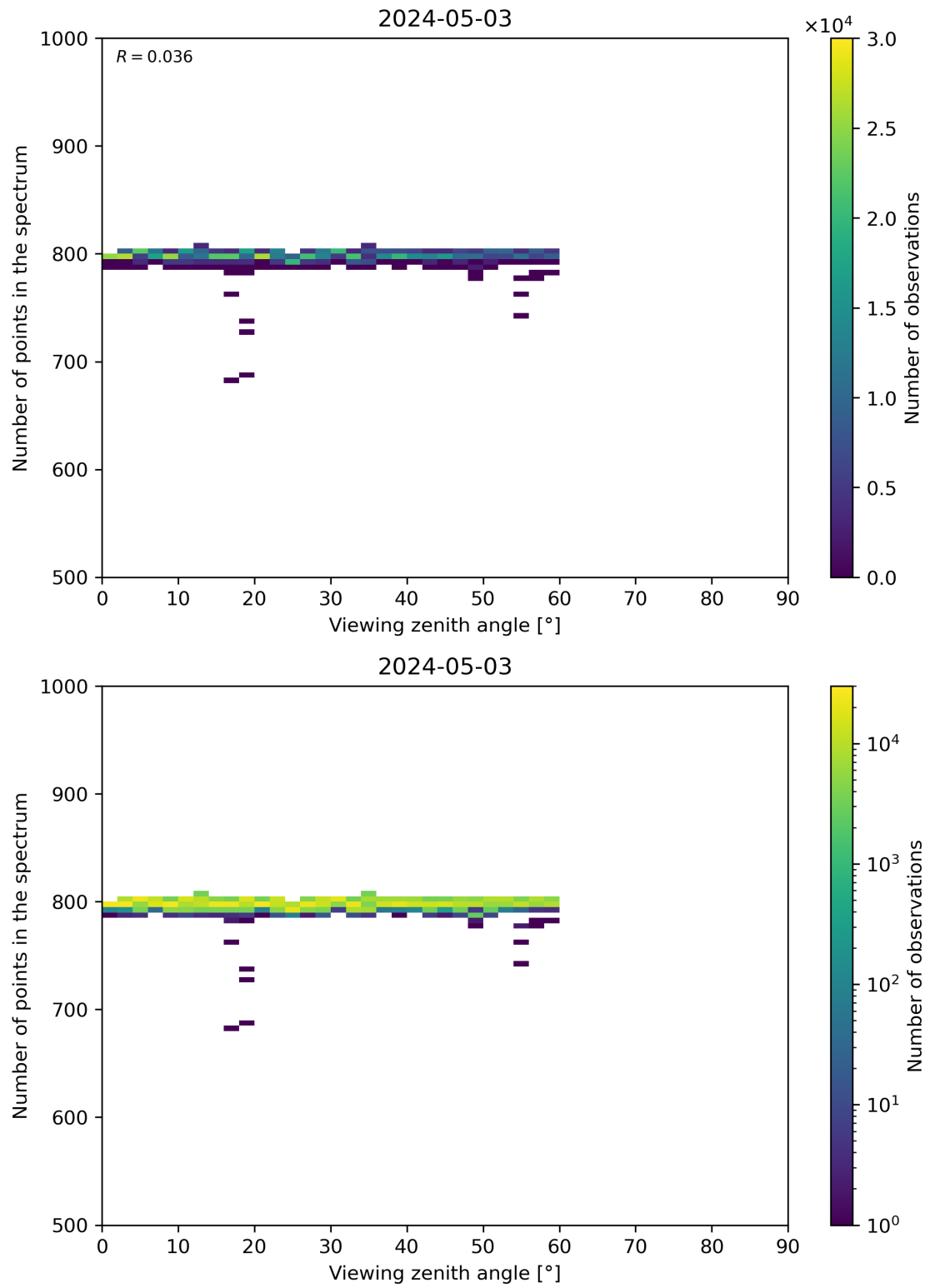
Figure 114: Scatter density plot of “Viewing zenith angle” against “Number of points in the spectrum” for 2024-05-02 to 2024-05-04.
