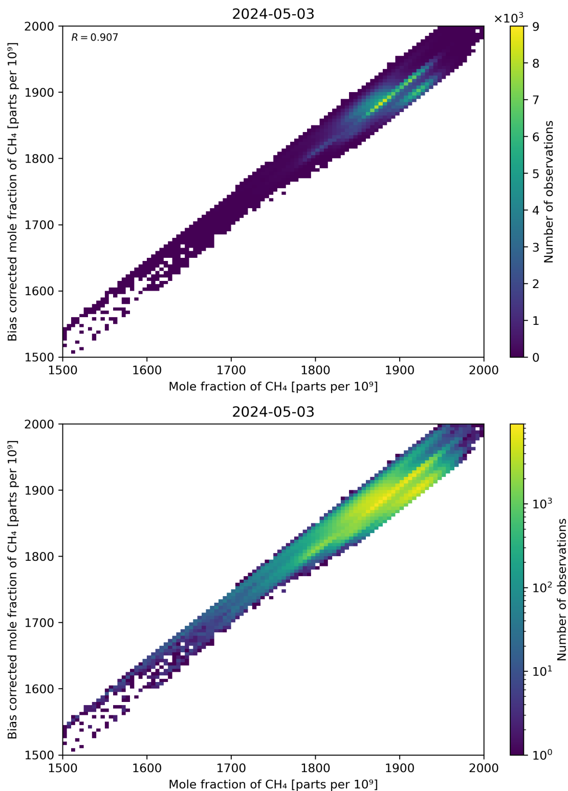
Figure 74: Scatter density plot of “Mole fraction of CH 4 ” against “Bias corrected mole fraction of CH 4 ” for 2024-05-02 to 2024-05-04.
