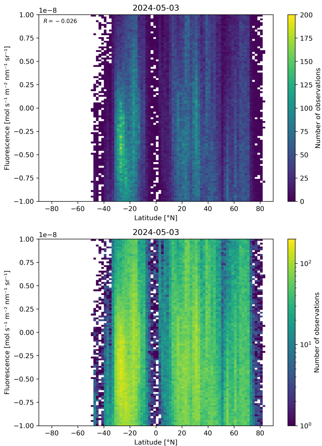
Figure 56: Scatter density plot of “Latitude” against “Fluorescence” for 2024-05-02 to 2024-05-04.
