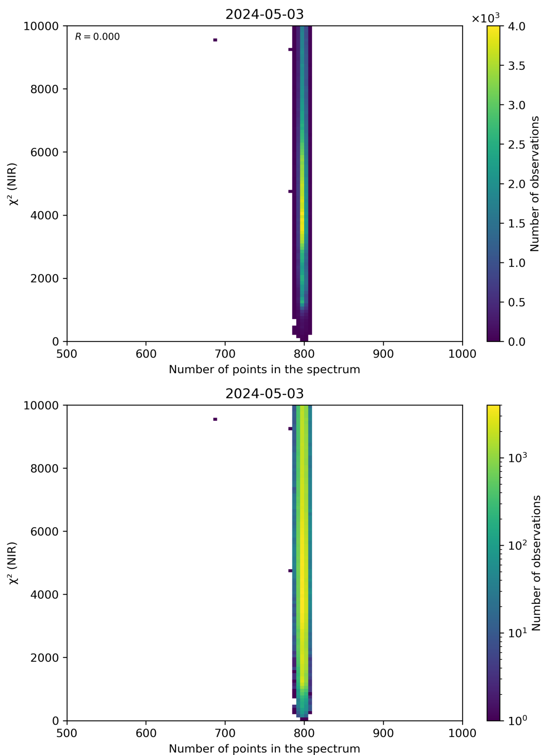
Figure 88: Scatter density plot of “Number of points in the spectrum” against “ \chi^2 (NIR)” for 2024-05-02 to 2024-05-04.
