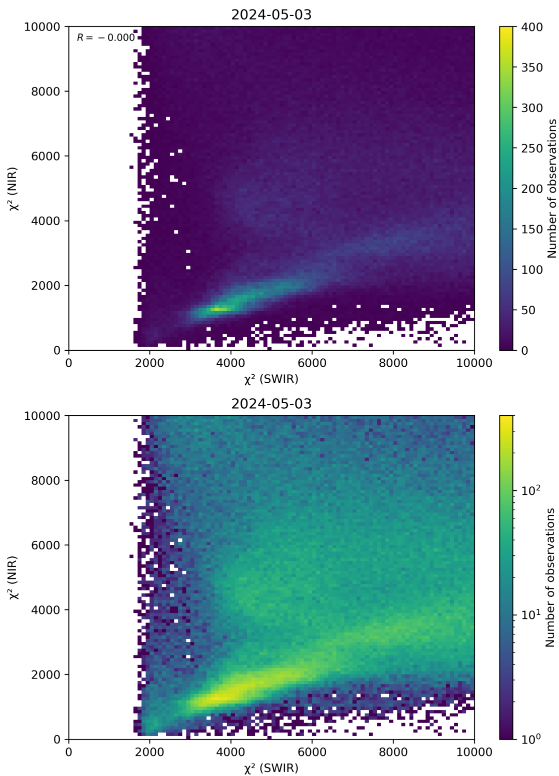
Figure 47: Scatter density plot of “ \chi^2 (SWIR)” against “ \chi^2 (NIR)” for 2024-05-02 to 2024-05-04.
