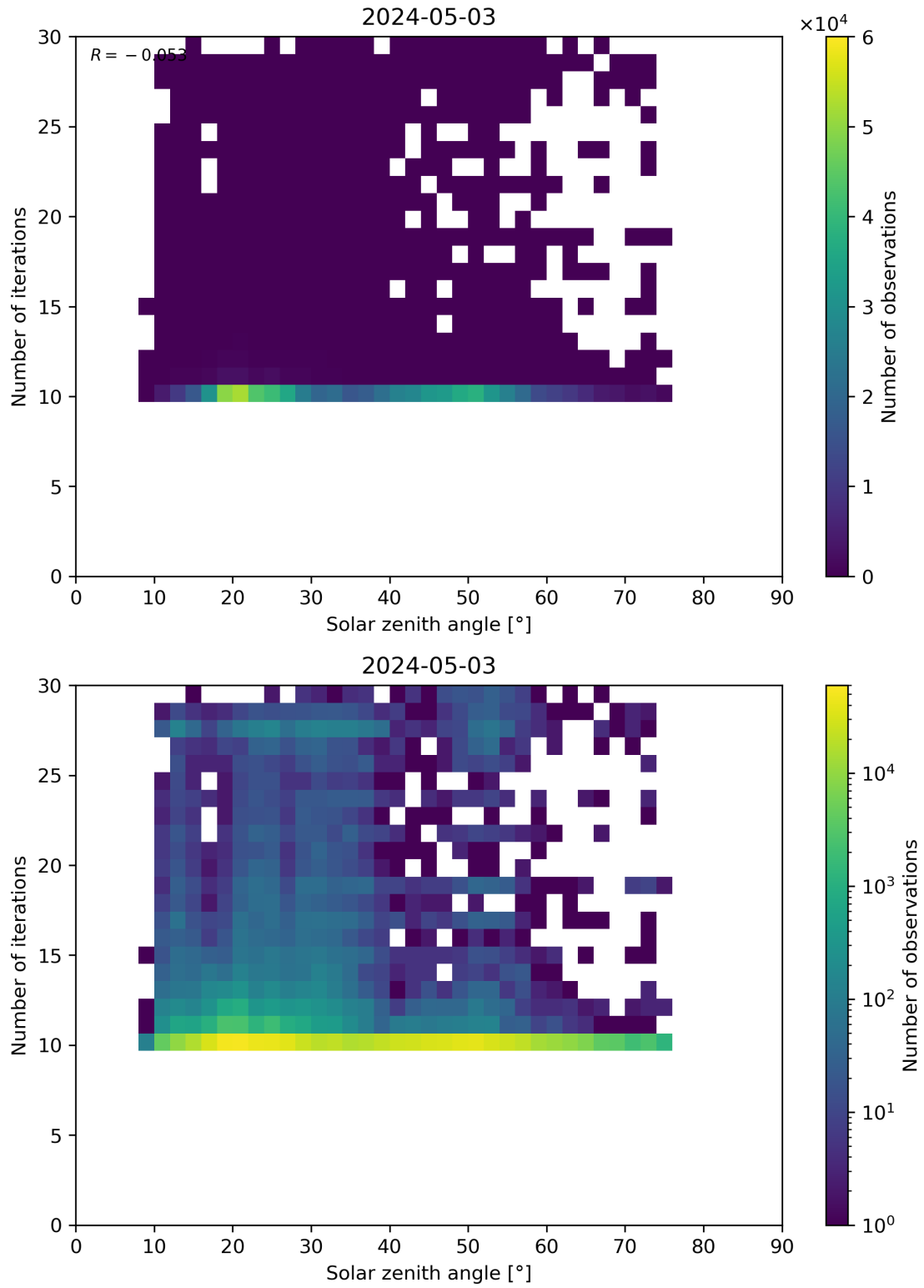
Figure 102: Scatter density plot of “Solar zenith angle” against “Number of iterations” for 2024-05-02 to 2024-05-04.
