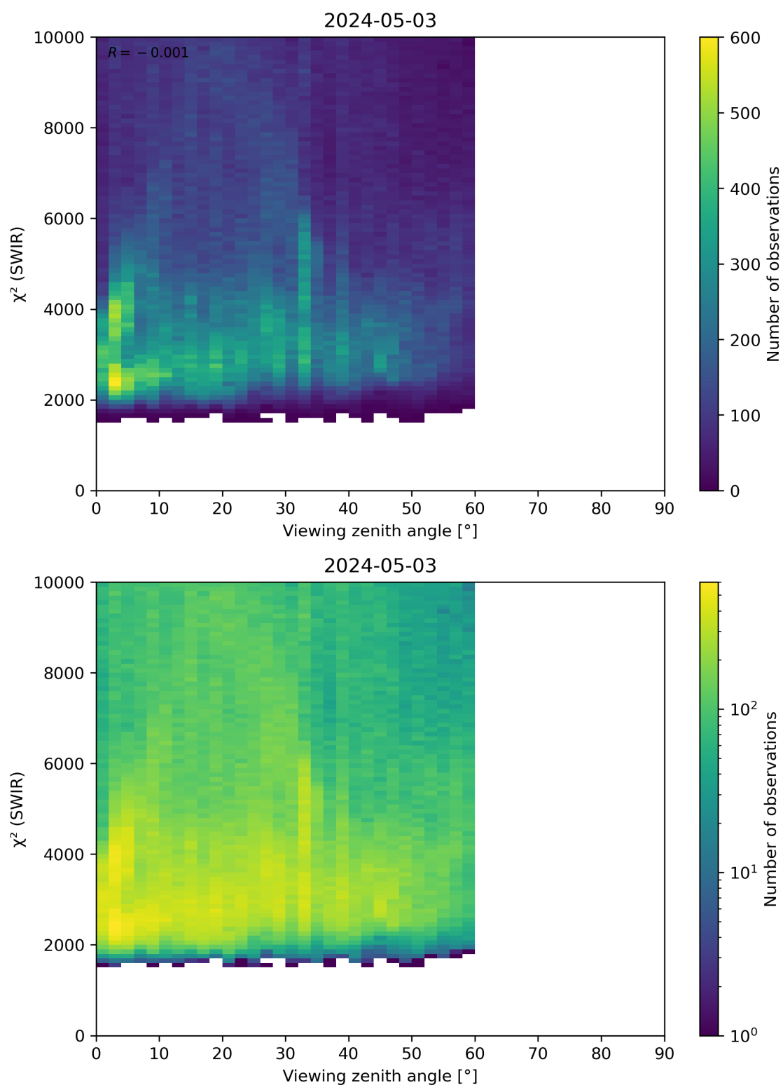
Figure 106: Scatter density plot of “Viewing zenith angle” against “ \chi^2 (SWIR)” for 2024-05-02 to 2024-05-04.
