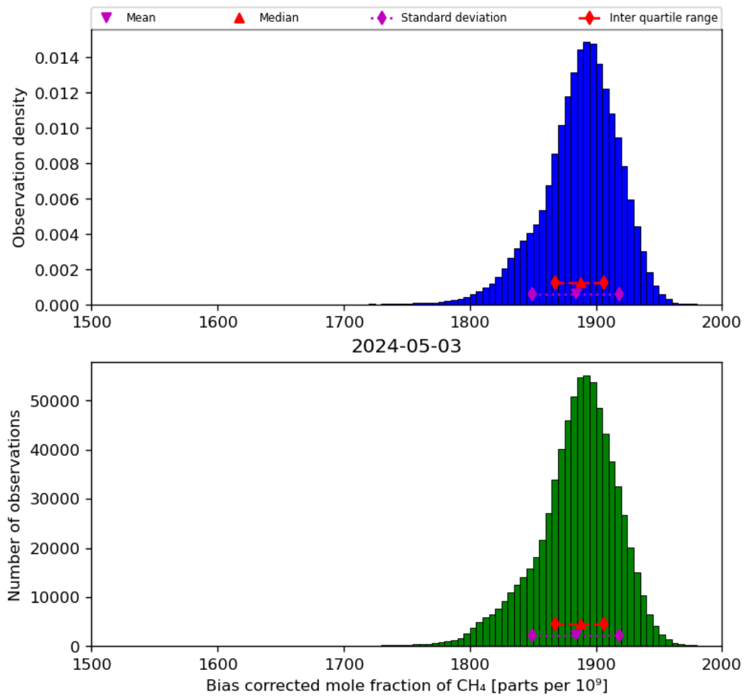
Figure 25: Histogram of “Bias corrected mole fraction of CH 4 ” for 2024-05-02 to 2024-05-04
