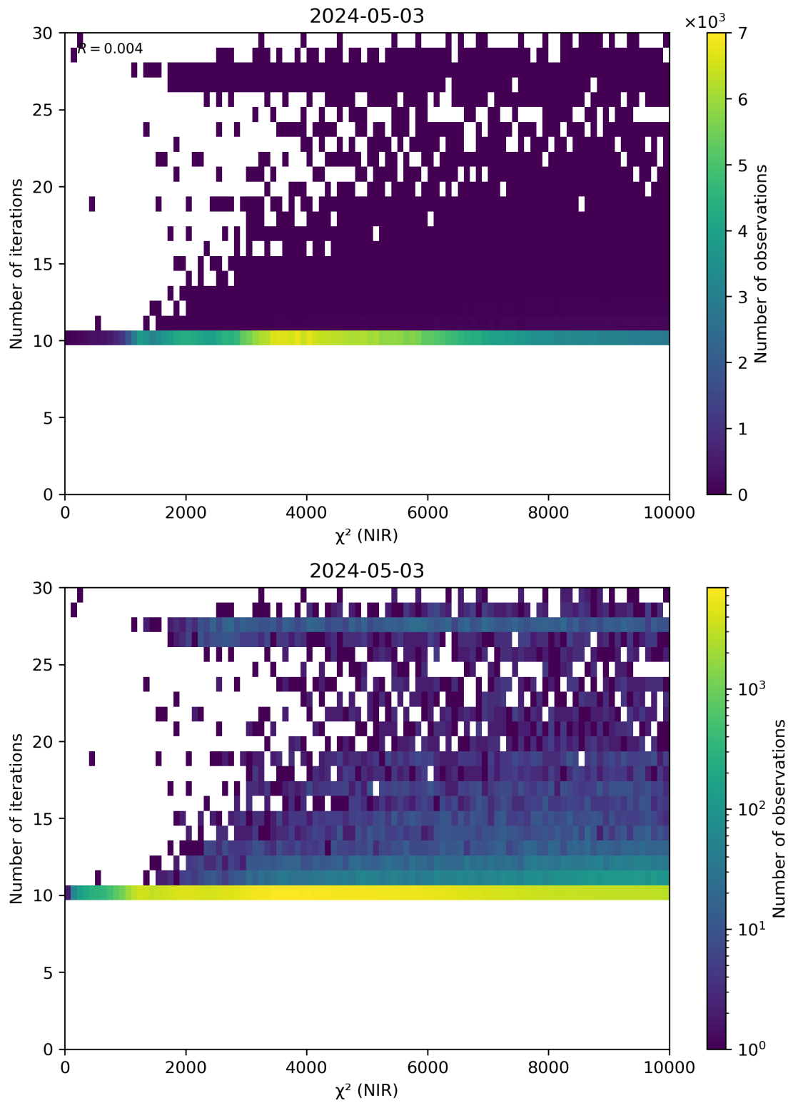
Figure 46: Scatter density plot of “ \chi^2 (NIR)” against “Number of iterations” for 2024-05-02 to 2024-05-04.
