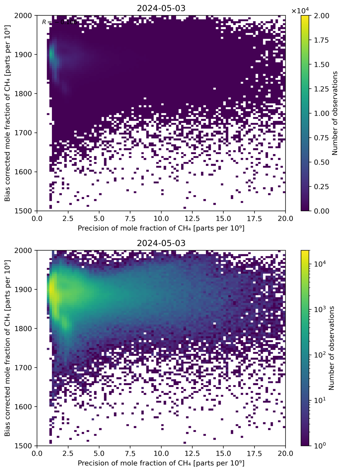
Figure 82: Scatter density plot of “Precision of mole fraction of CH 4 ” against “Bias corrected mole fraction of CH 4 ” for 2024-05-02 to 2024-05-04.
