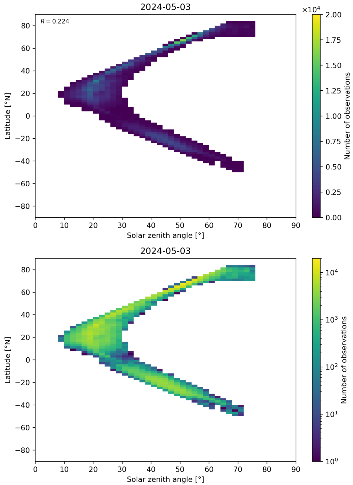
Figure 98: Scatter density plot of “Solar zenith angle” against “Latitude” for 2024-05-02 to 2024-05-04.
