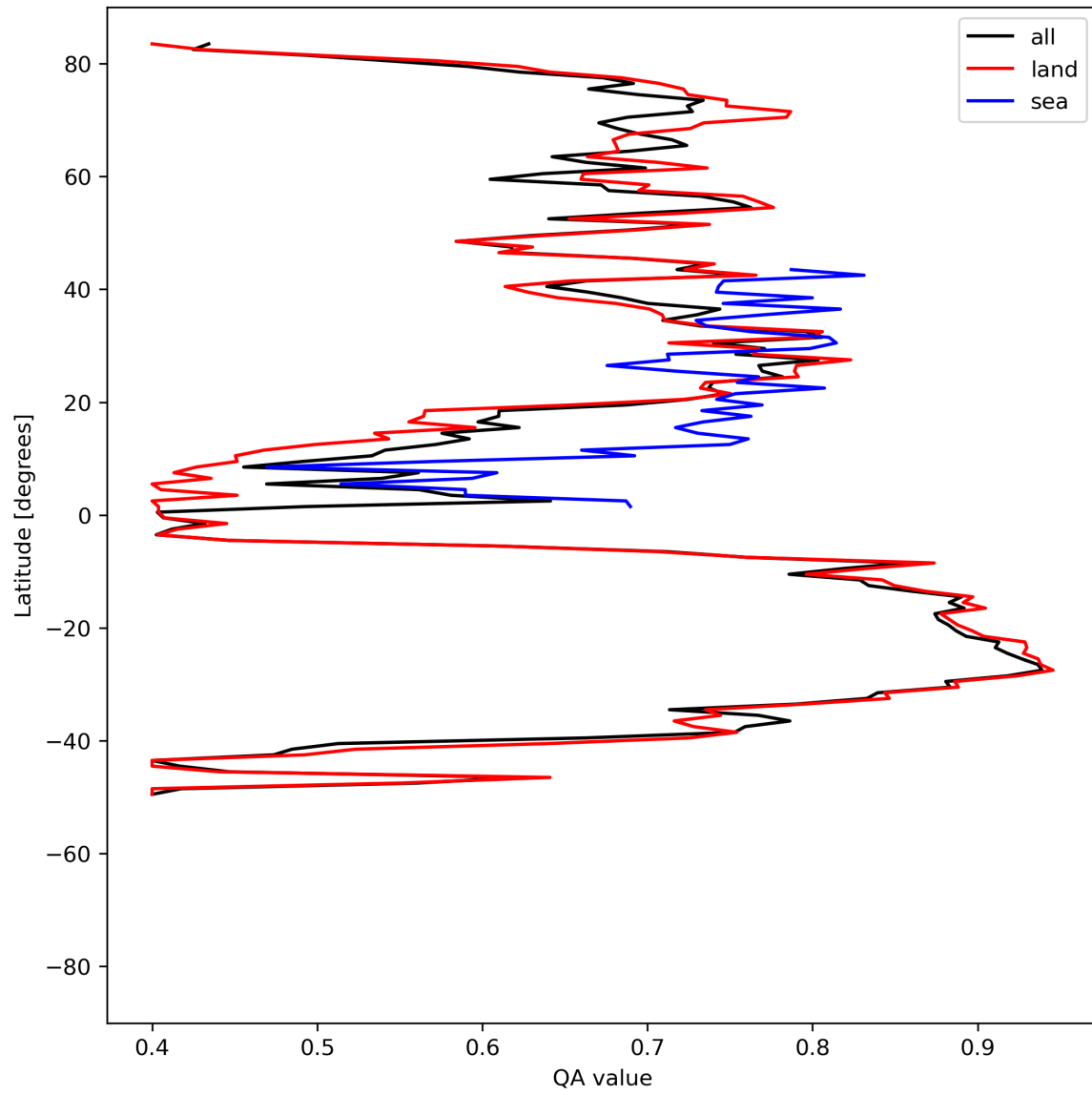
Figure 11: Zonal average of “QA value” for 2024-05-02 to 2024-05-04.
