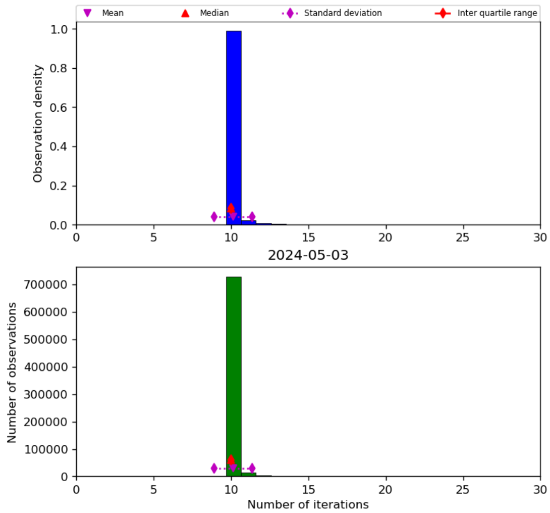
Figure 31: Histogram of “Number of iterations” for 2024-05-02 to 2024-05-04
