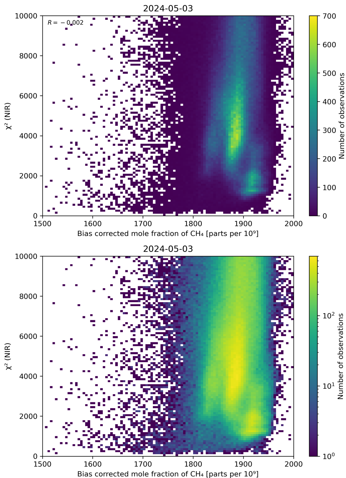
Figure 63: Scatter density plot of “Bias corrected mole fraction of CH 4 ” against “ \chi^2 (NIR)” for 2024-05-02 to 2024-05-04.
