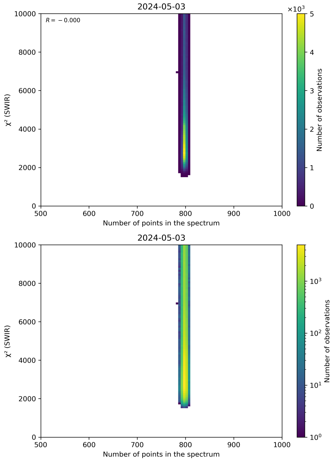
Figure 89: Scatter density plot of “Number of points in the spectrum” against “ \chi^2 (SWIR)” for 2024-05-02 to 2024-05-04.
