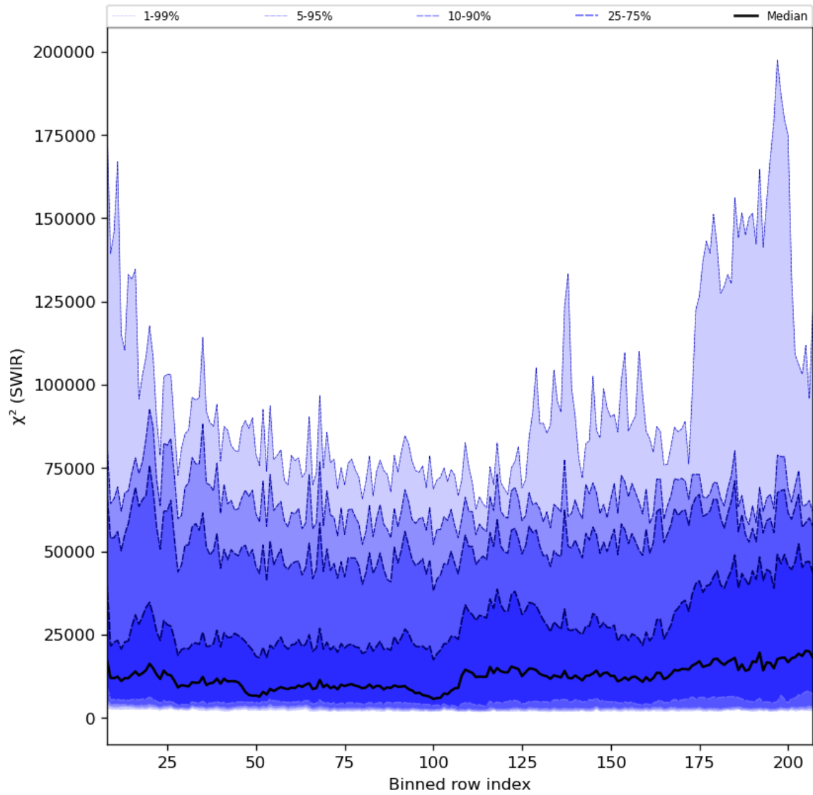
Figure 39: Along track statistics of “ \chi^2 (SWIR)” for 2024-05-02 to 2024-05-04
