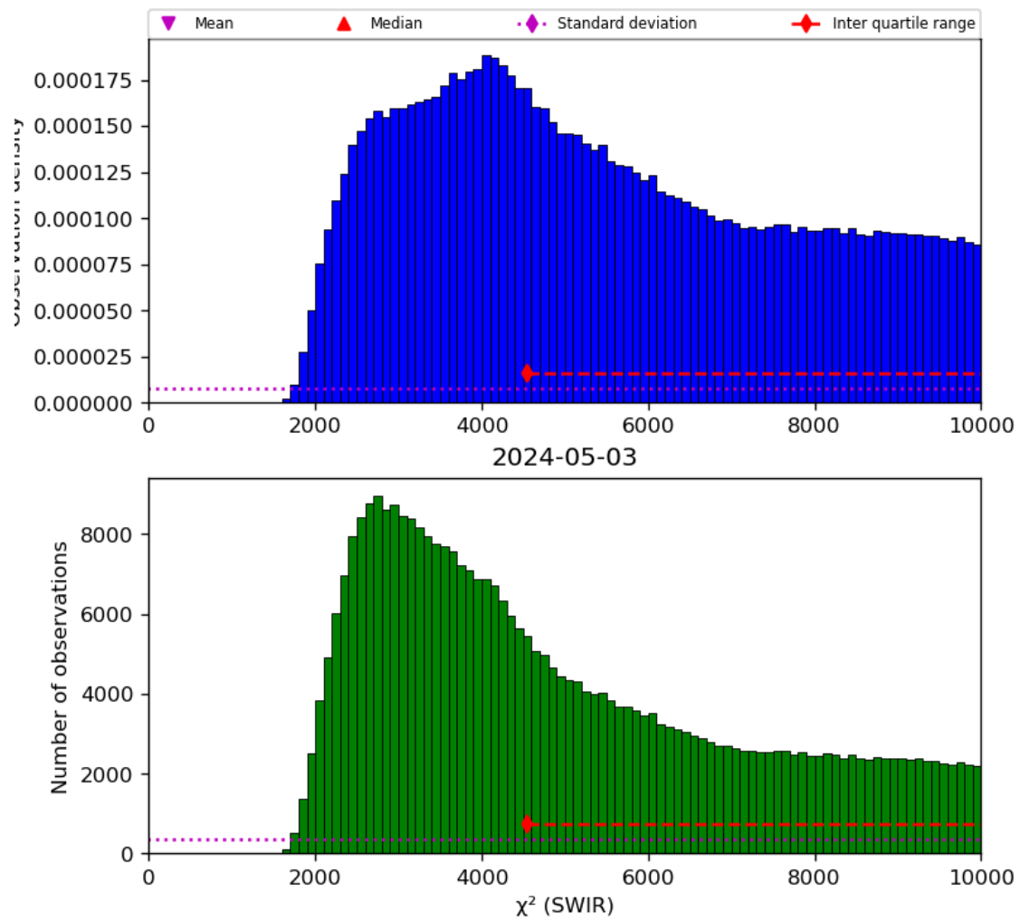
Figure 28: Histogram of “ \chi^2 (SWIR)” for 2024-05-02 to 2024-05-04
