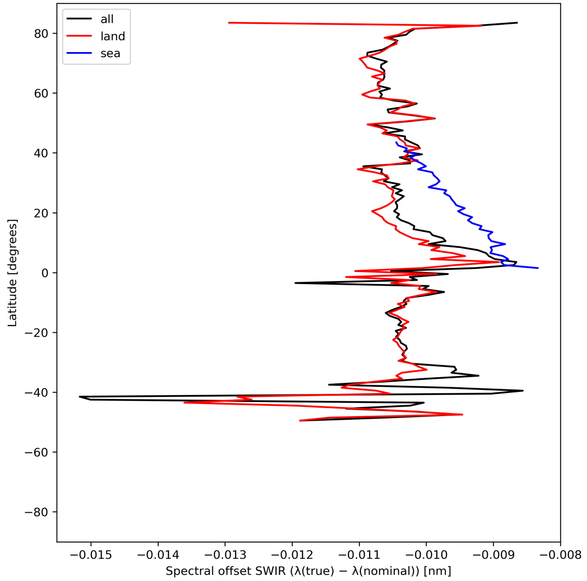
Figure 16: Zonal average of “Spectral offset SWIR ( \lambda(\text{true}) - \lambda(\text{nominal}) )” for 2024-05-02 to 2024-05-04.
