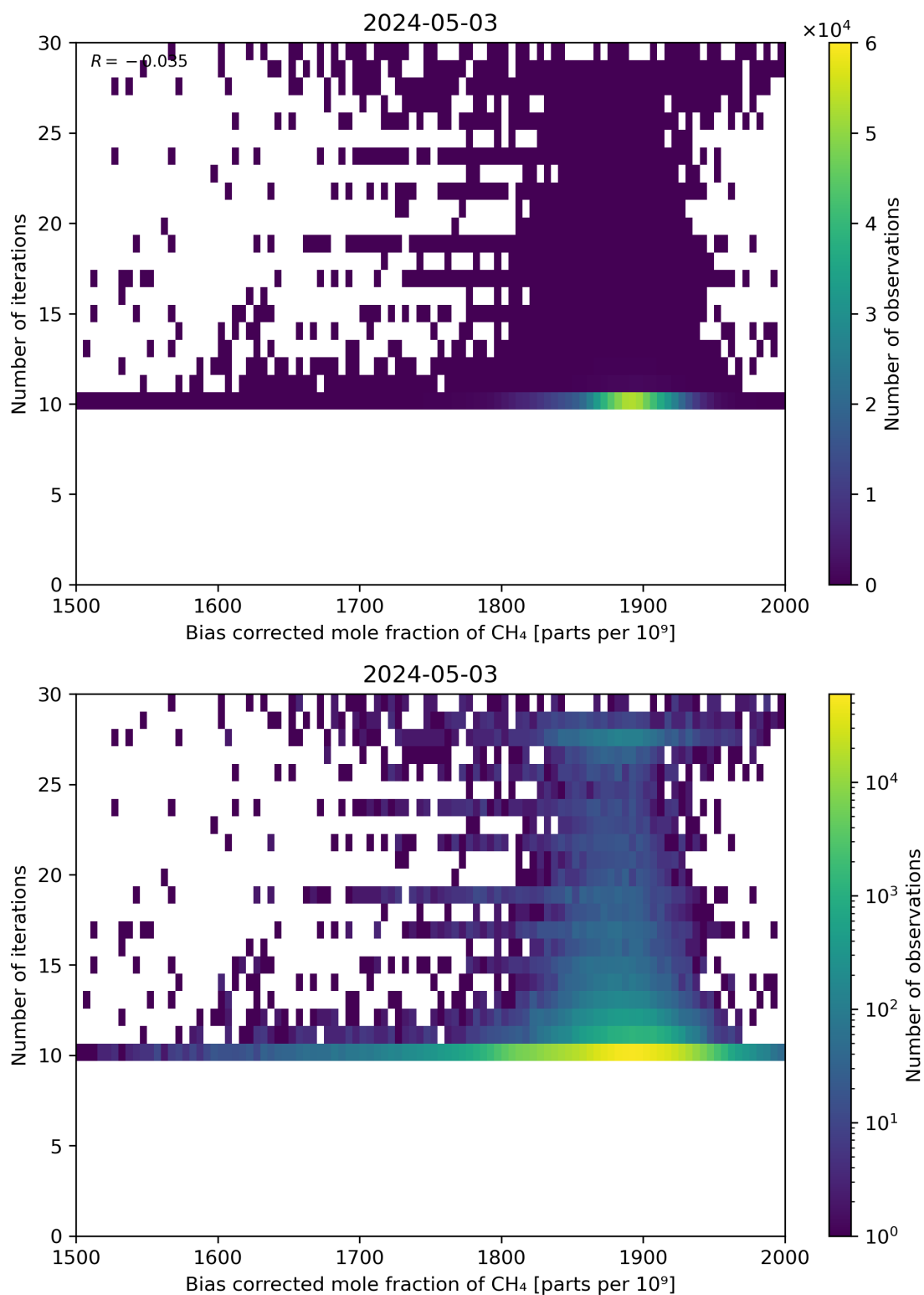
Figure 67: Scatter density plot of “Bias corrected mole fraction of CH 4 ” against “Number of iterations” for 2024-05-02 to 2024-05-04.
