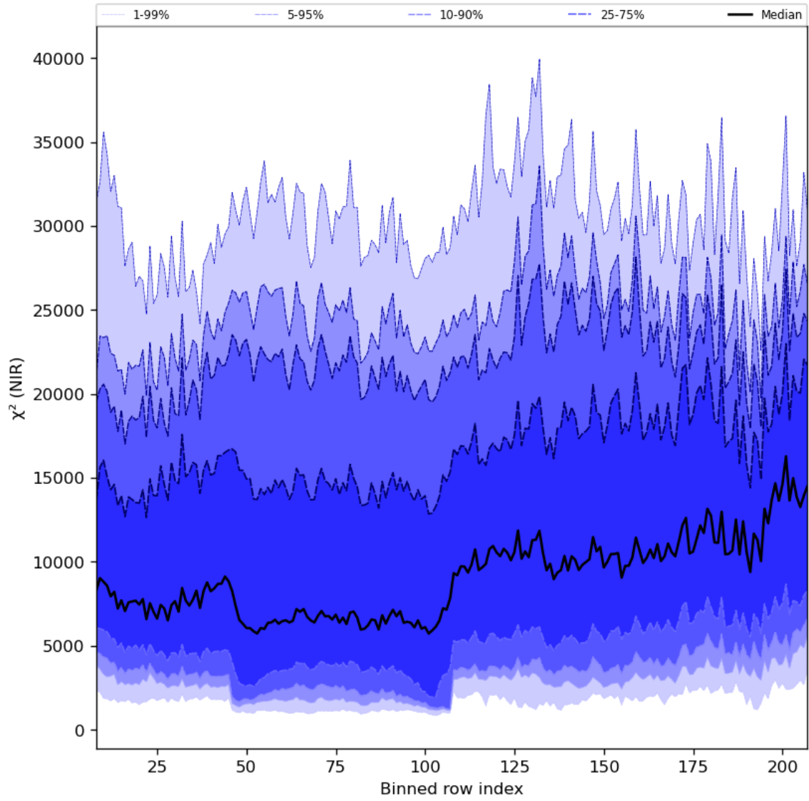
Figure 40: Along track statistics of “ \chi^2 (NIR)” for 2024-05-02 to 2024-05-04
