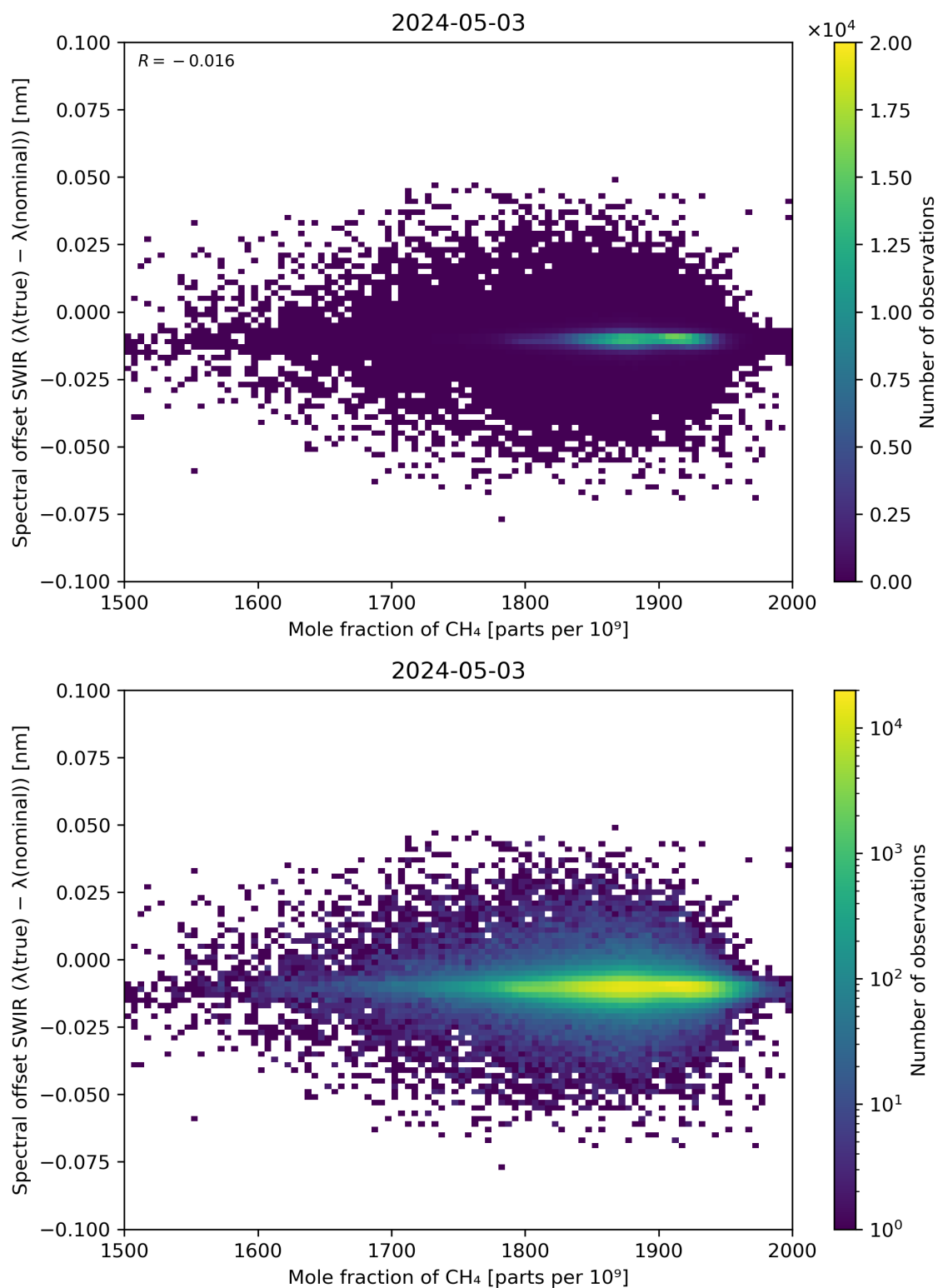
Figure 86: Scatter density plot of “Mole fraction of CH 4 ” against “Spectral offset SWIR ( \lambda(\text{true}) - \lambda(\text{nominal}) )” for 2024-05-02 to 2024-05-04.
