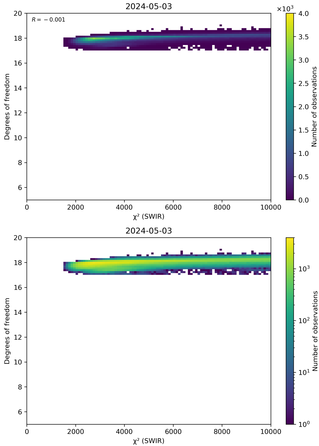
Figure 48: Scatter density plot of “ \chi^2 (SWIR)” against “Degrees of freedom” for 2024-05-02 to 2024-05-04.
