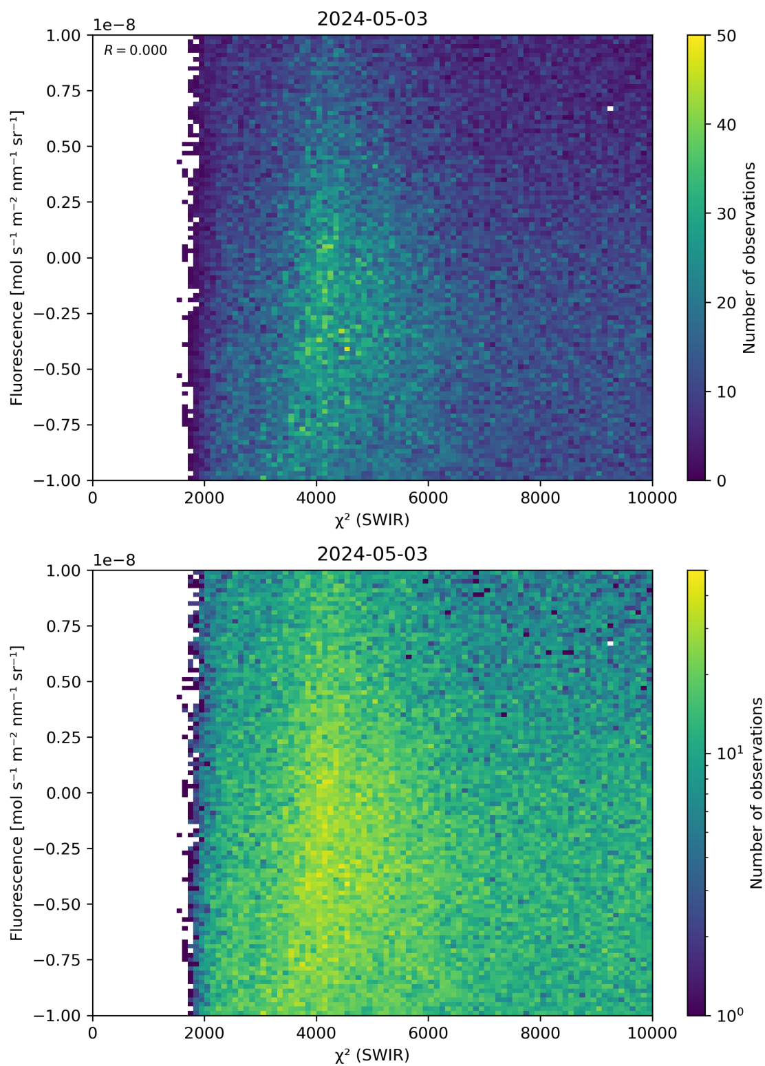
Figure 49: Scatter density plot of “ \chi^2 (SWIR)” against “Fluorescence” for 2024-05-02 to 2024-05-04.
