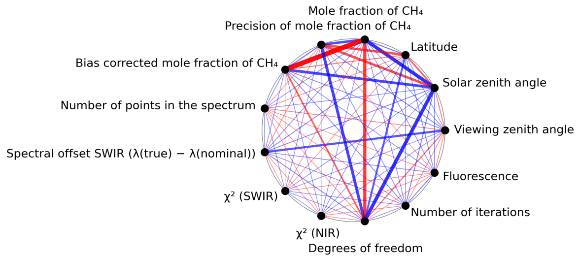
Figure 1: Map of correlation graph for 2024-05-02 to 2024-05-04.
