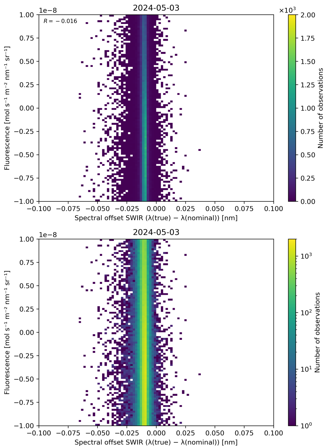
Figure 120: Scatter density plot of “Spectral offset SWIR ( \lambda(\text{true}) - \lambda(\text{nominal}) )” against “Fluorescence” for 2024-05-02 to 2024-05-04.
