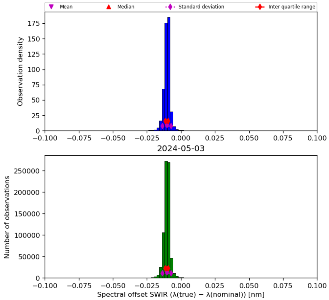
Figure 27: Histogram of “Spectral offset SWIR ( \lambda(\text{true}) - \lambda(\text{nominal}) )” for 2024-05-02 to 2024-05-04
