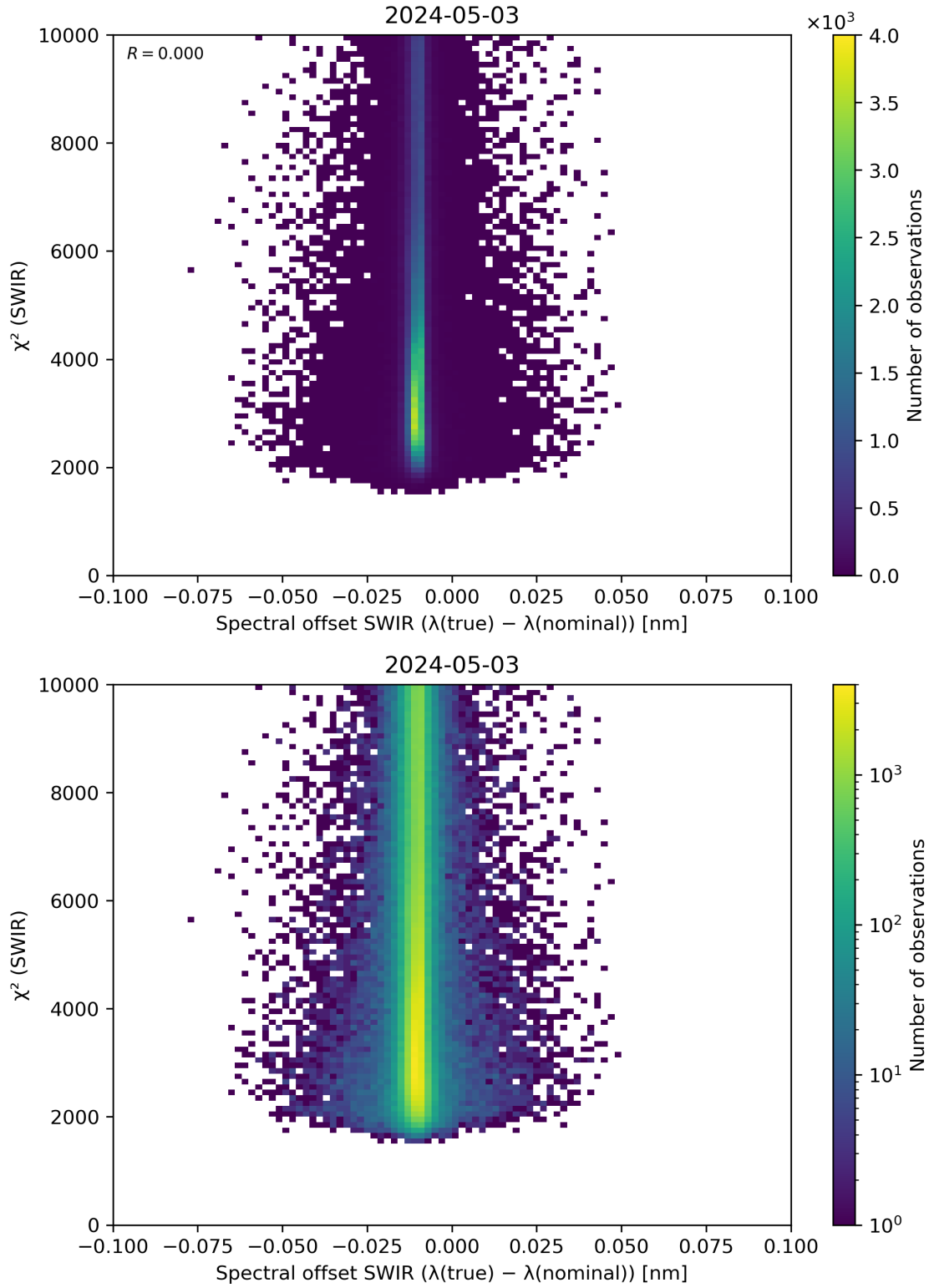
Figure 118: Scatter density plot of “Spectral offset SWIR ( \lambda(\text{true}) - \lambda(\text{nominal}) )” against “ \chi^2 (SWIR)” for 2024-05-02 to 2024-05-04.
