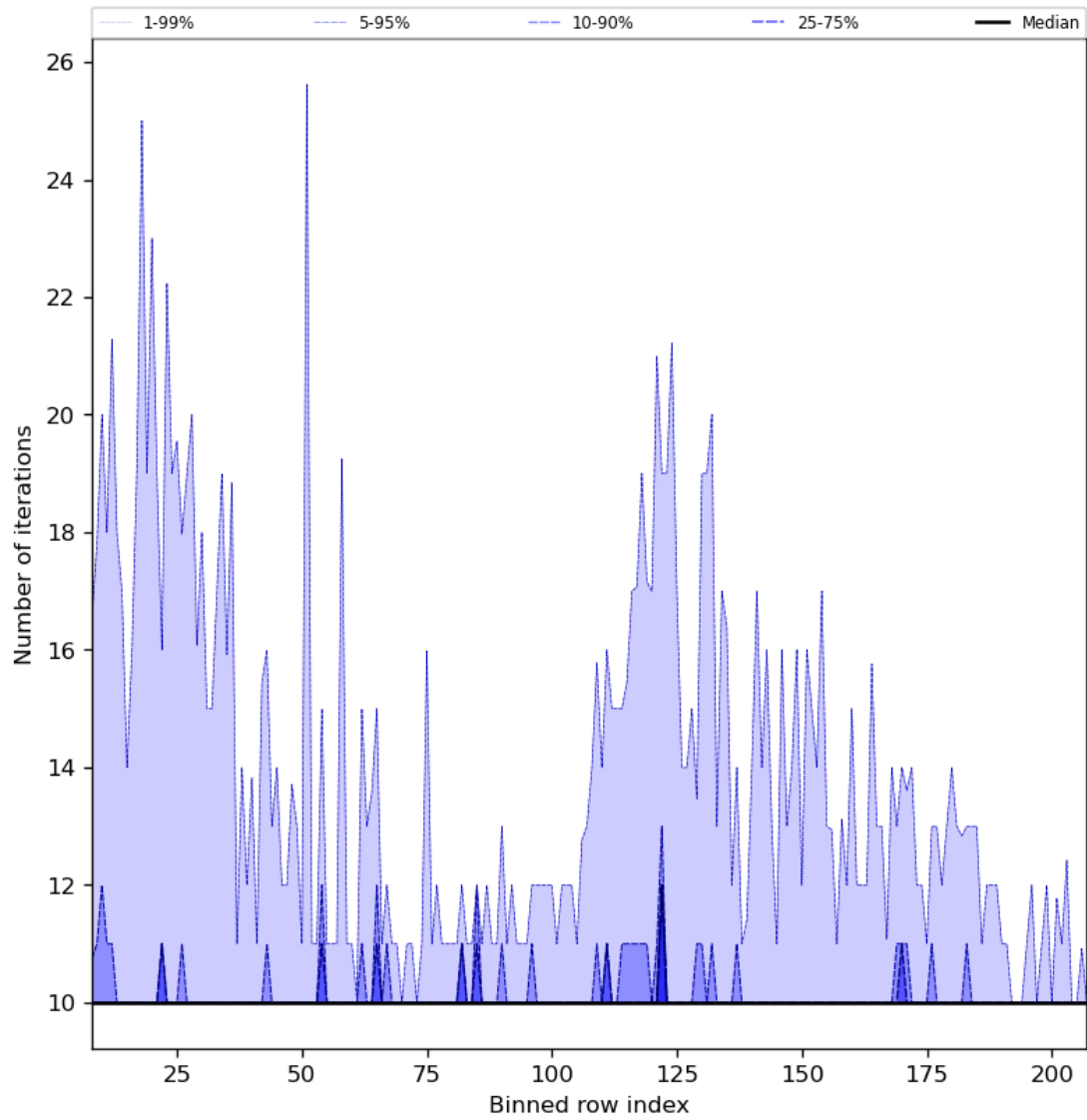
Figure 42: Along track statistics of “Number of iterations” for 2024-05-02 to 2024-05-04
