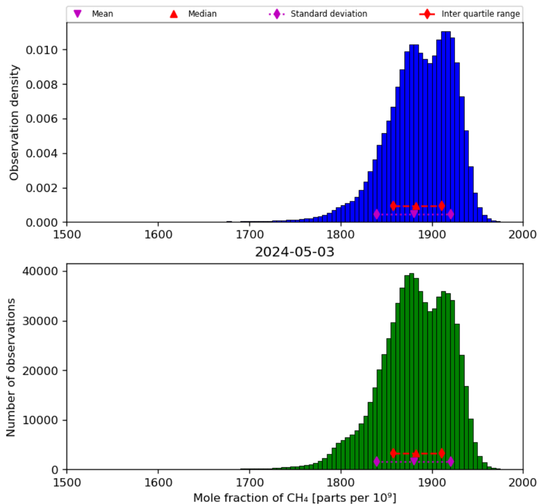
Figure 23: Histogram of “Mole fraction of CH 4 ” for 2024-05-02 to 2024-05-04
