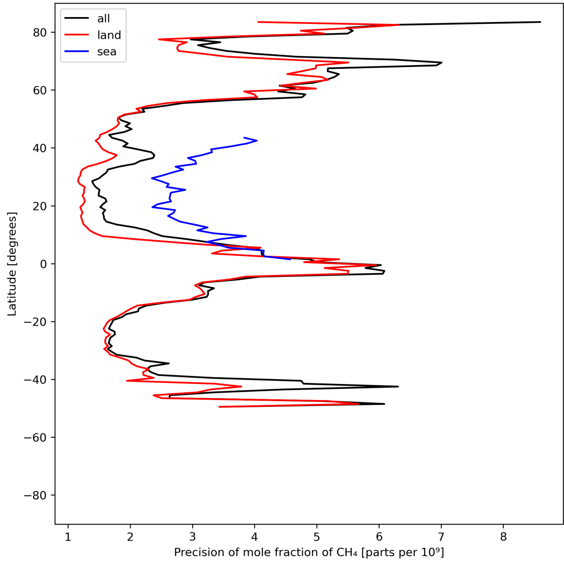
Figure 13: Zonal average of “Precision of mole fraction of CH 4 ” for 2024-05-02 to 2024-05-04.
