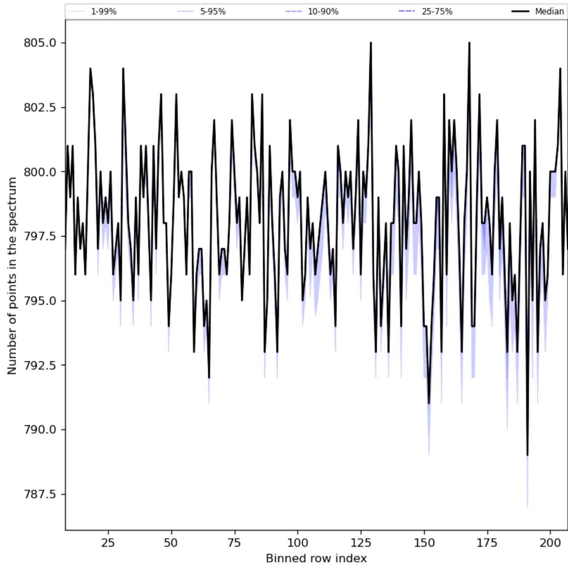
Figure 37: Along track statistics of “Number of points in the spectrum” for 2024-05-02 to 2024-05-04
