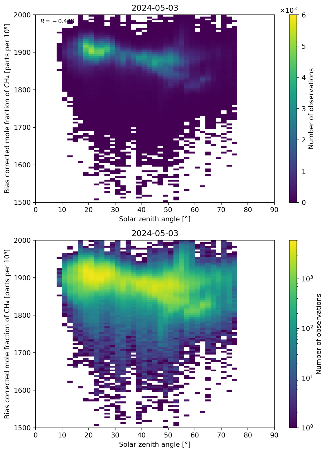
Figure 100: Scatter density plot of “Solar zenith angle” against “Bias corrected mole fraction of CH 4 ” for 2024-05-02 to 2024-05-04.
