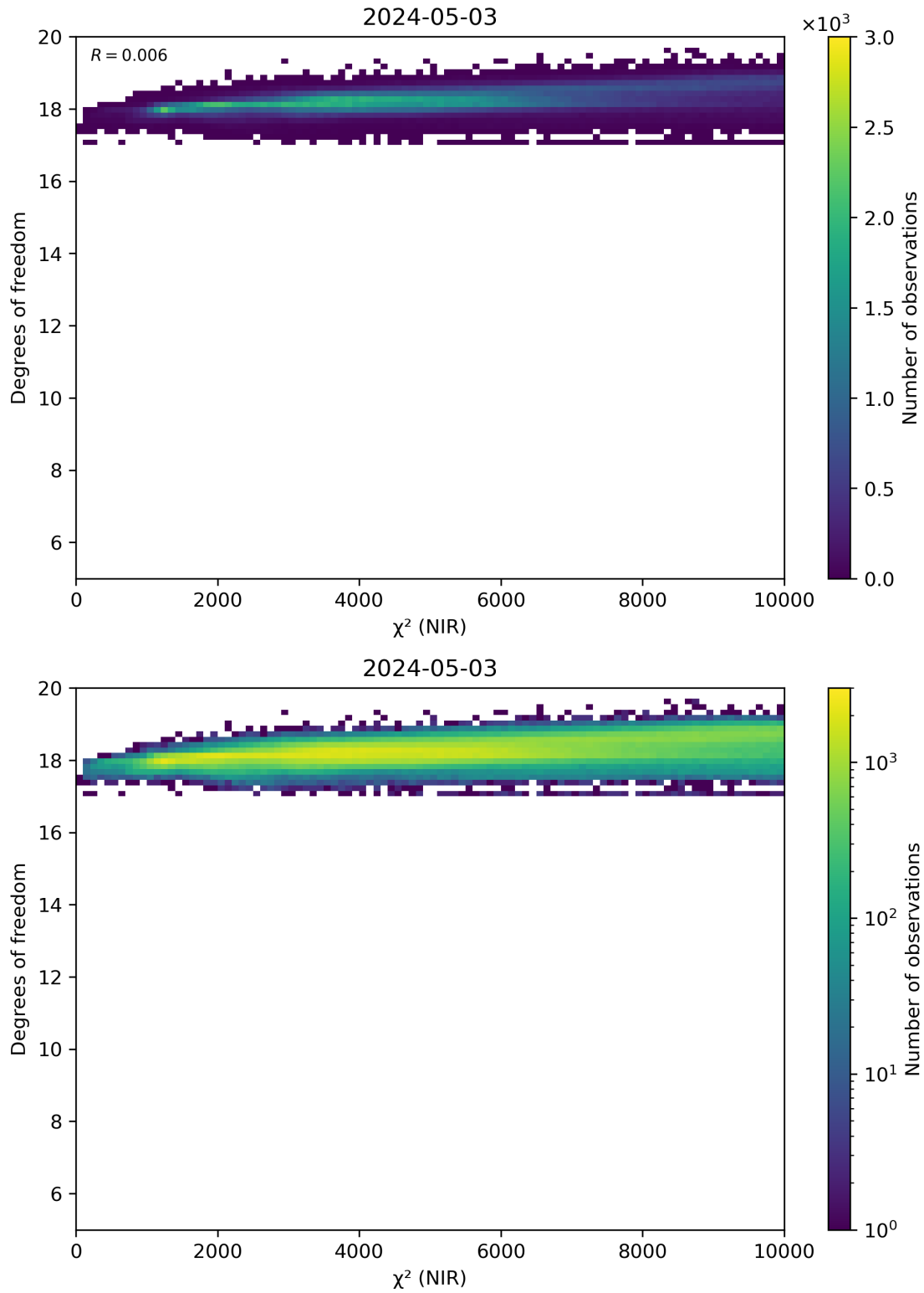
Figure 44: Scatter density plot of “ \chi^2 (NIR)” against “Degrees of freedom” for 2024-05-02 to 2024-05-04.
