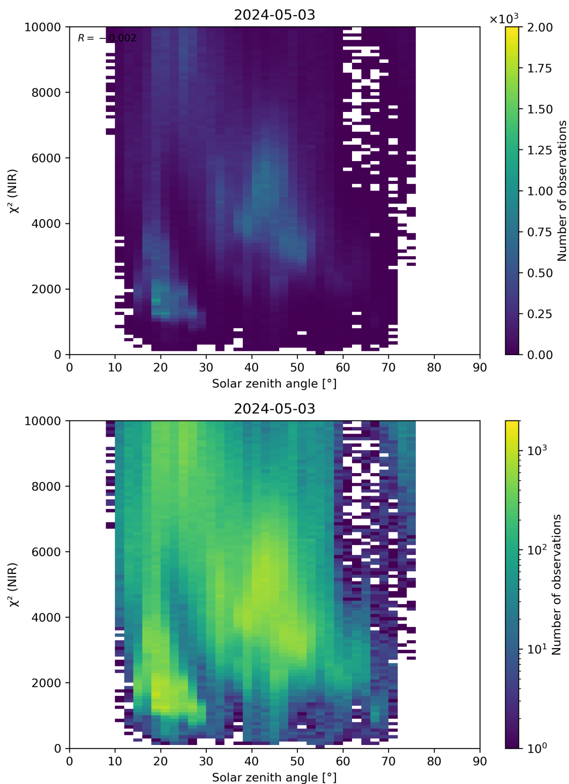
Figure 94: Scatter density plot of “Solar zenith angle” against “ \chi^2 (NIR)” for 2024-05-02 to 2024-05-04.
