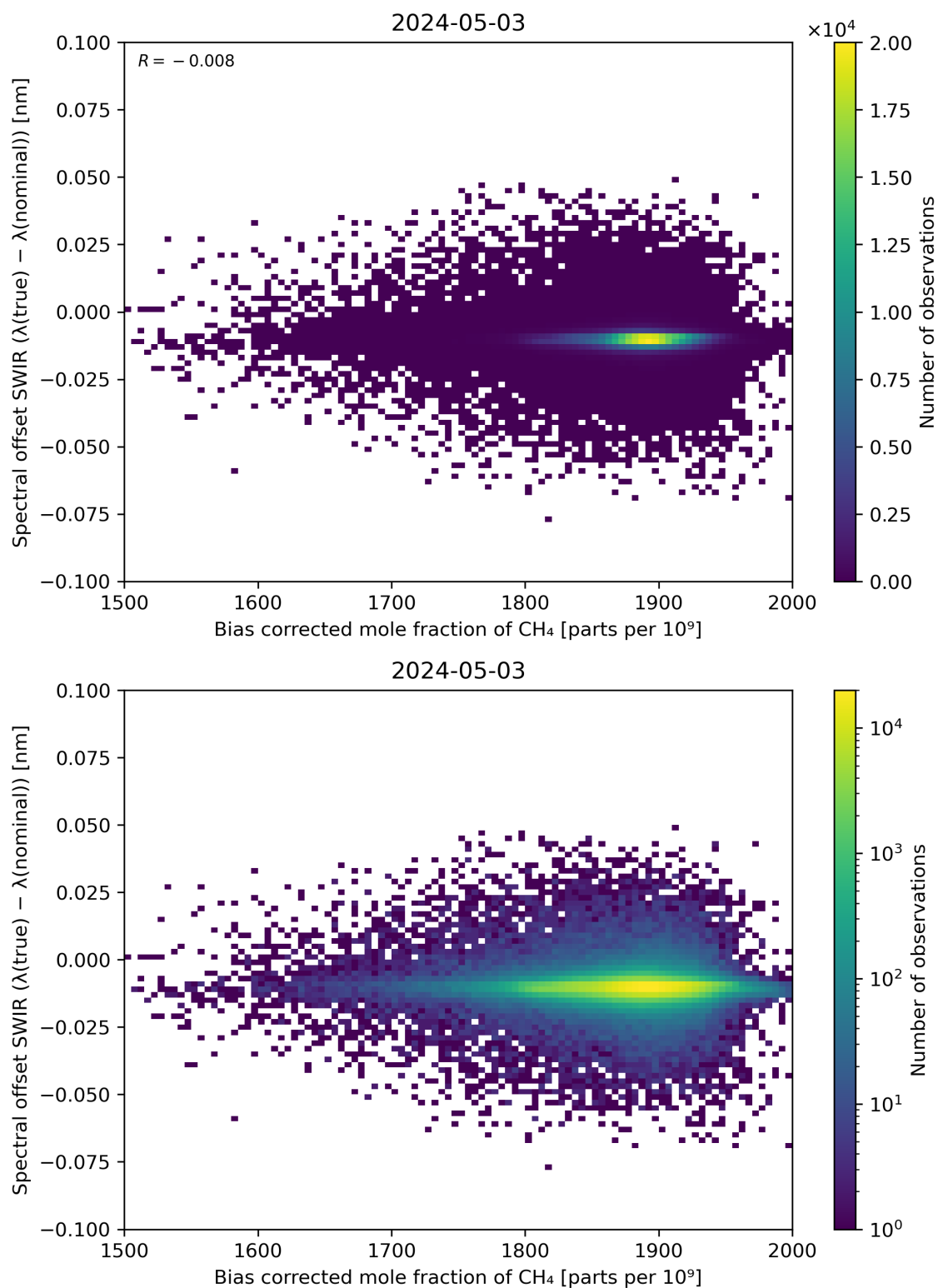
Figure 69: Scatter density plot of “Bias corrected mole fraction of \text{CH}_4 ” against “Spectral offset SWIR ( \lambda(\text{true}) - \lambda(\text{nominal}) )” for 2024-05-02 to 2024-05-04.
