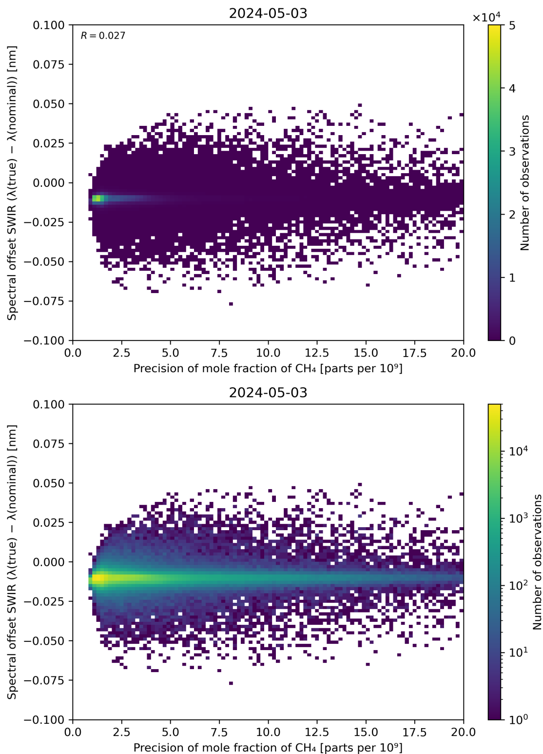
Figure 85: Scatter density plot of “Precision of mole fraction of CH 4 ” against “Spectral offset SWIR ( \lambda(\text{true}) - \lambda(\text{nominal}) )” for 2024-05-02 to 2024-05-04.
