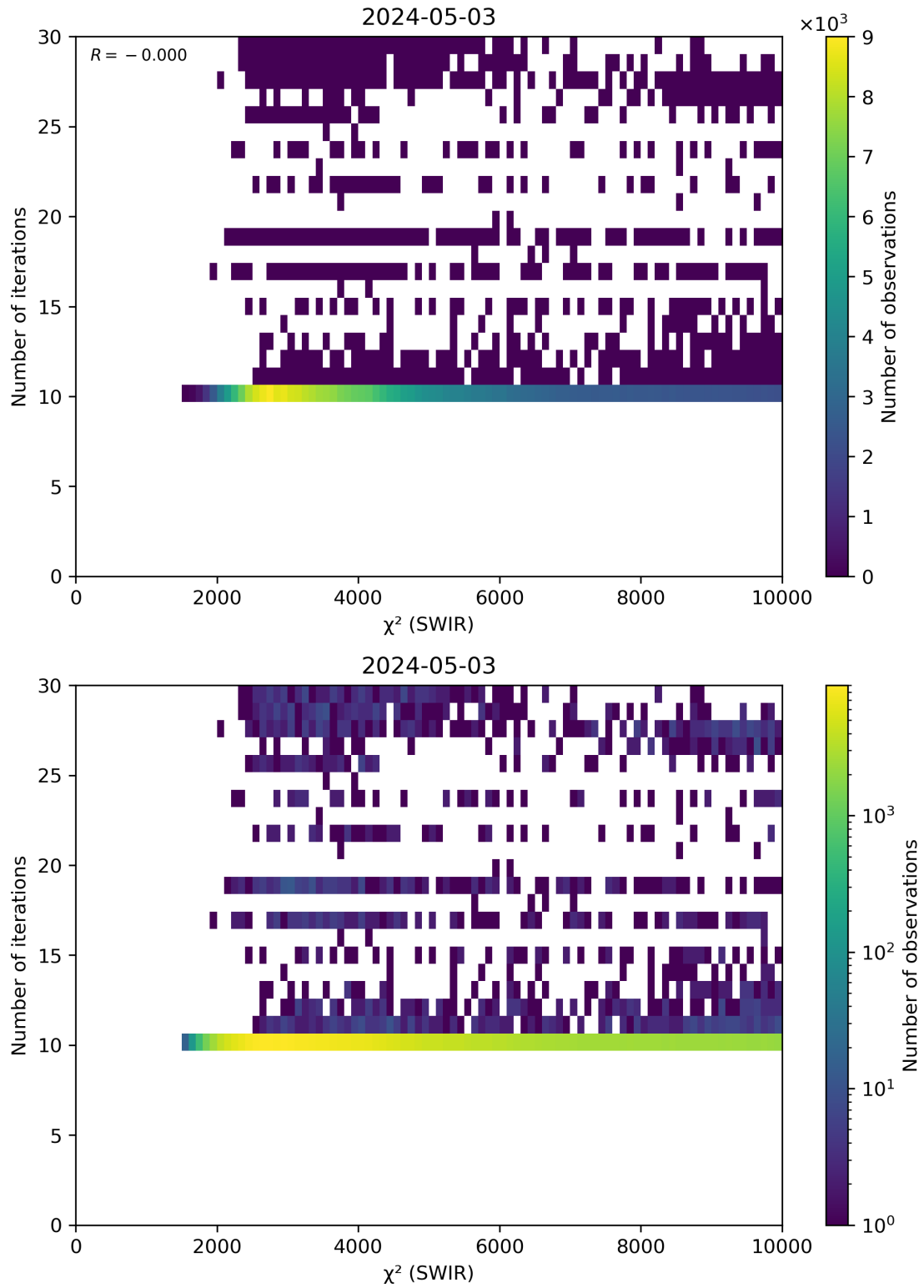
Figure 50: Scatter density plot of " \chi^2 (SWIR)" against "Number of iterations" for 2024-05-02 to 2024-05-04.
