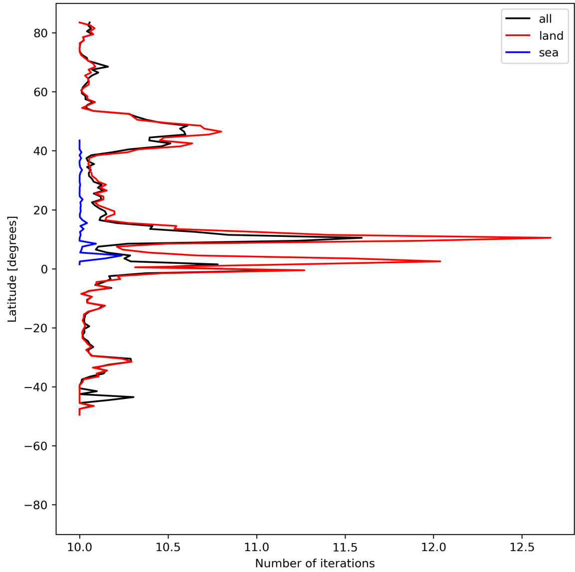
Figure 20: Zonal average of “Number of iterations” for 2024-05-02 to 2024-05-04.
