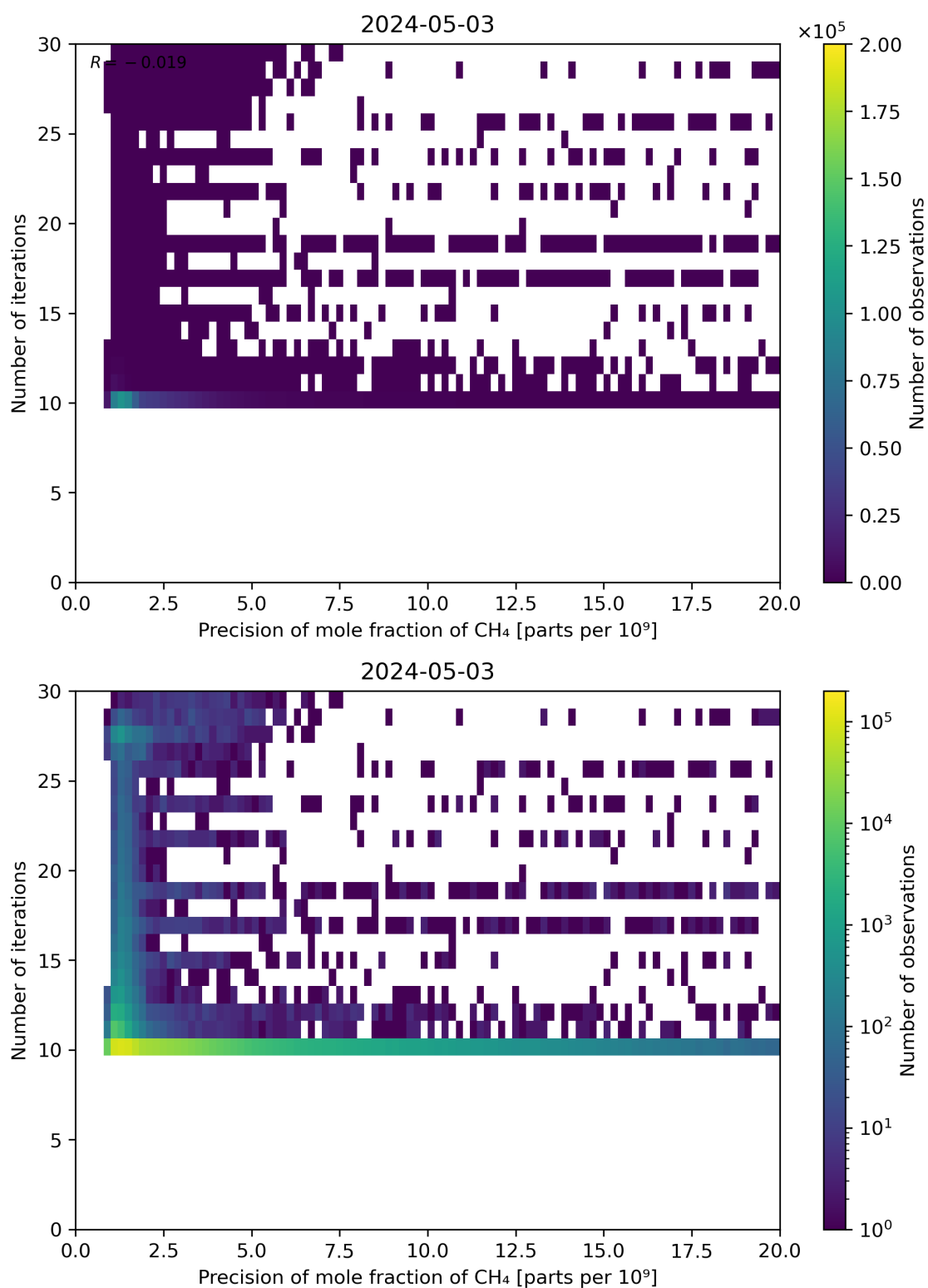
Figure 83: Scatter density plot of “Precision of mole fraction of CH 4 ” against “Number of iterations” for 2024-05-02 to 2024-05-04.
