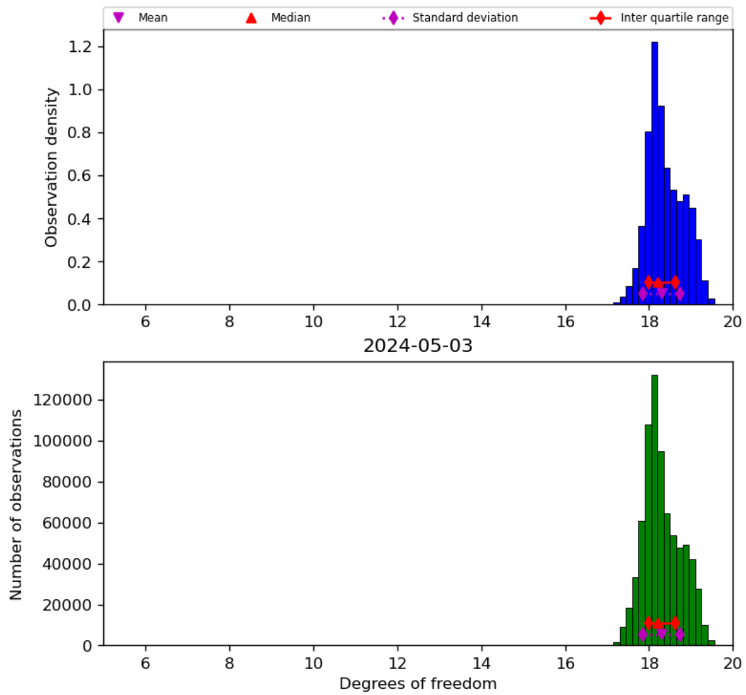
Figure 30: Histogram of “Degrees of freedom” for 2024-05-02 to 2024-05-04
