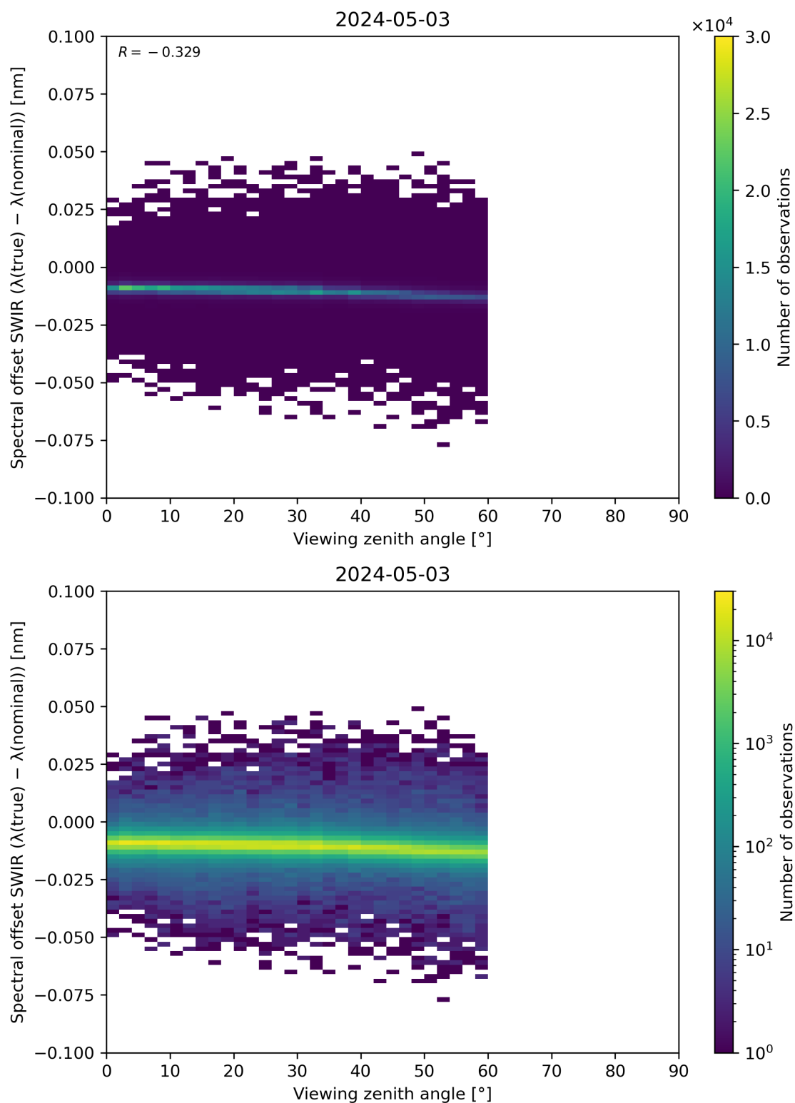
Figure 116: Scatter density plot of “Viewing zenith angle” against “Spectral offset SWIR ( \lambda(\text{true}) - \lambda(\text{nominal}) )” for 2024-05-02 to 2024-05-04.
