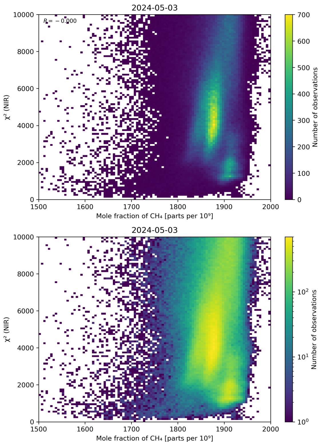
Figure 70: Scatter density plot of “Mole fraction of CH 4 ” against “ \chi^2 (NIR)” for 2024-05-02 to 2024-05-04.
