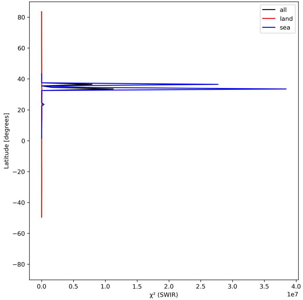
Figure 17: Zonal average of “ \chi^2 (SWIR)” for 2024-05-02 to 2024-05-04.
