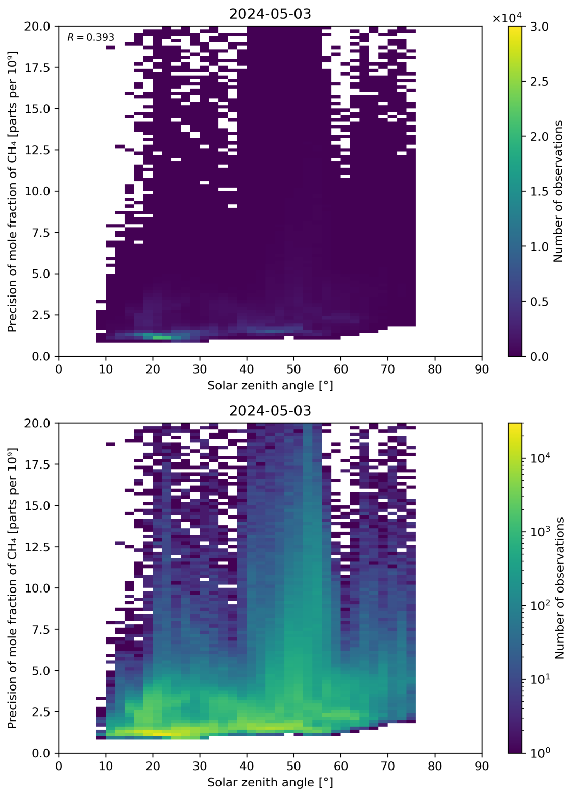
Figure 101: Scatter density plot of “Solar zenith angle” against “Precision of mole fraction of CH 4 ” for 2024-05-02 to 2024-05-04.
