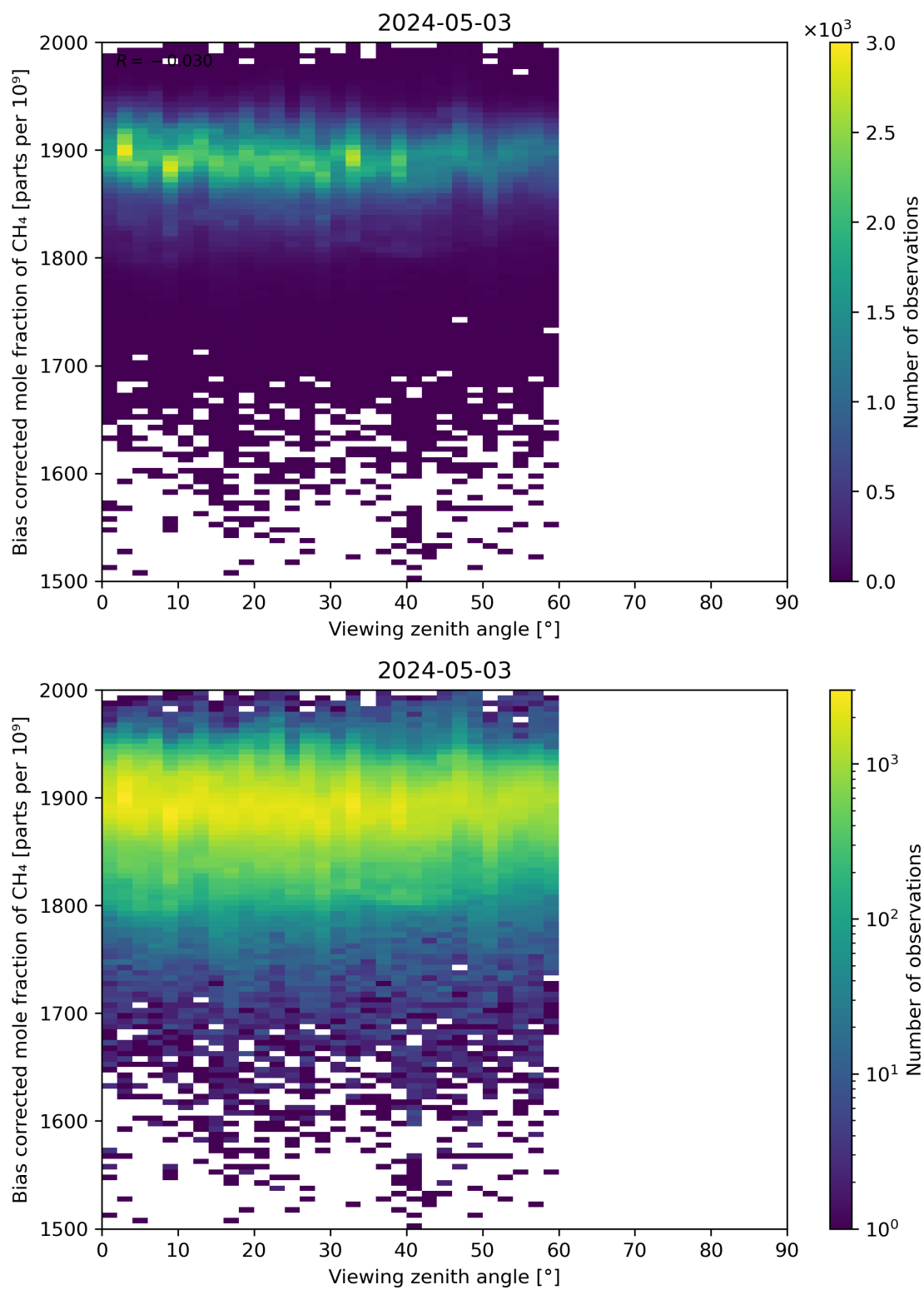
Figure 111: Scatter density plot of “Viewing zenith angle” against “Bias corrected mole fraction of CH 4 ” for 2024-05-02 to 2024-05-04.
