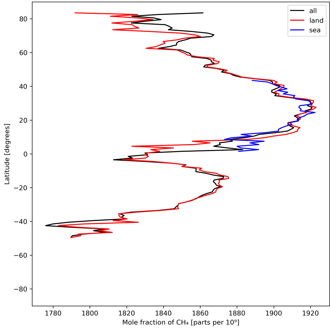
Figure 12: Zonal average of “Mole fraction of \text{CH}_4 ” for 2024-05-02 to 2024-05-04.
