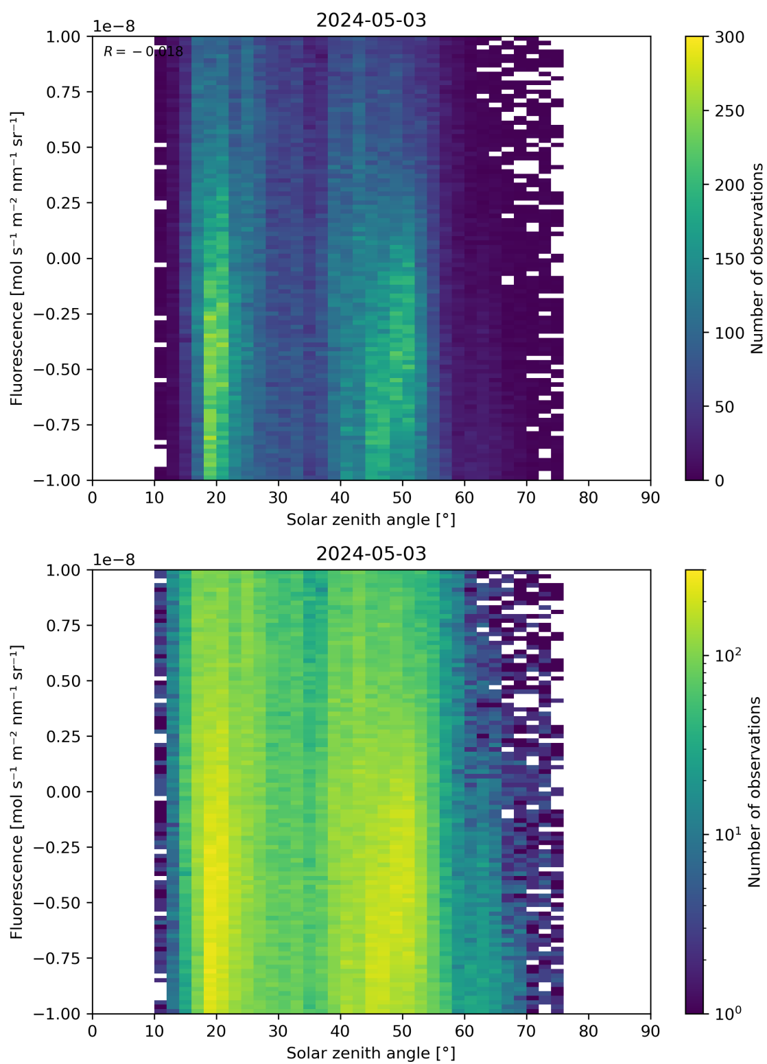
Figure 97: Scatter density plot of “Solar zenith angle” against “Fluorescence” for 2024-05-02 to 2024-05-04.
