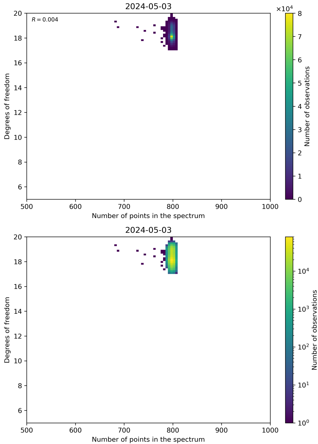
Figure 90: Scatter density plot of “Number of points in the spectrum” against “Degrees of freedom” for 2024-05-02 to 2024-05-04.
