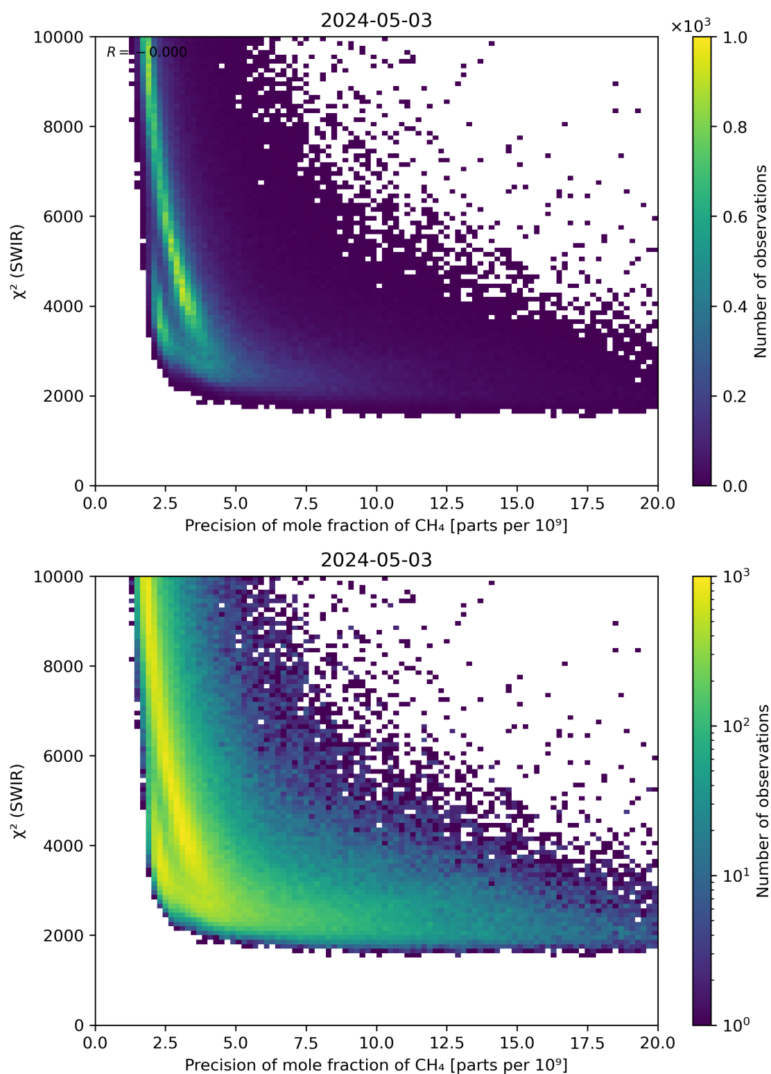
Figure 79: Scatter density plot of “Precision of mole fraction of CH 4 ” against “ \chi^2 (SWIR)” for 2024-05-02 to 2024-05-04.
