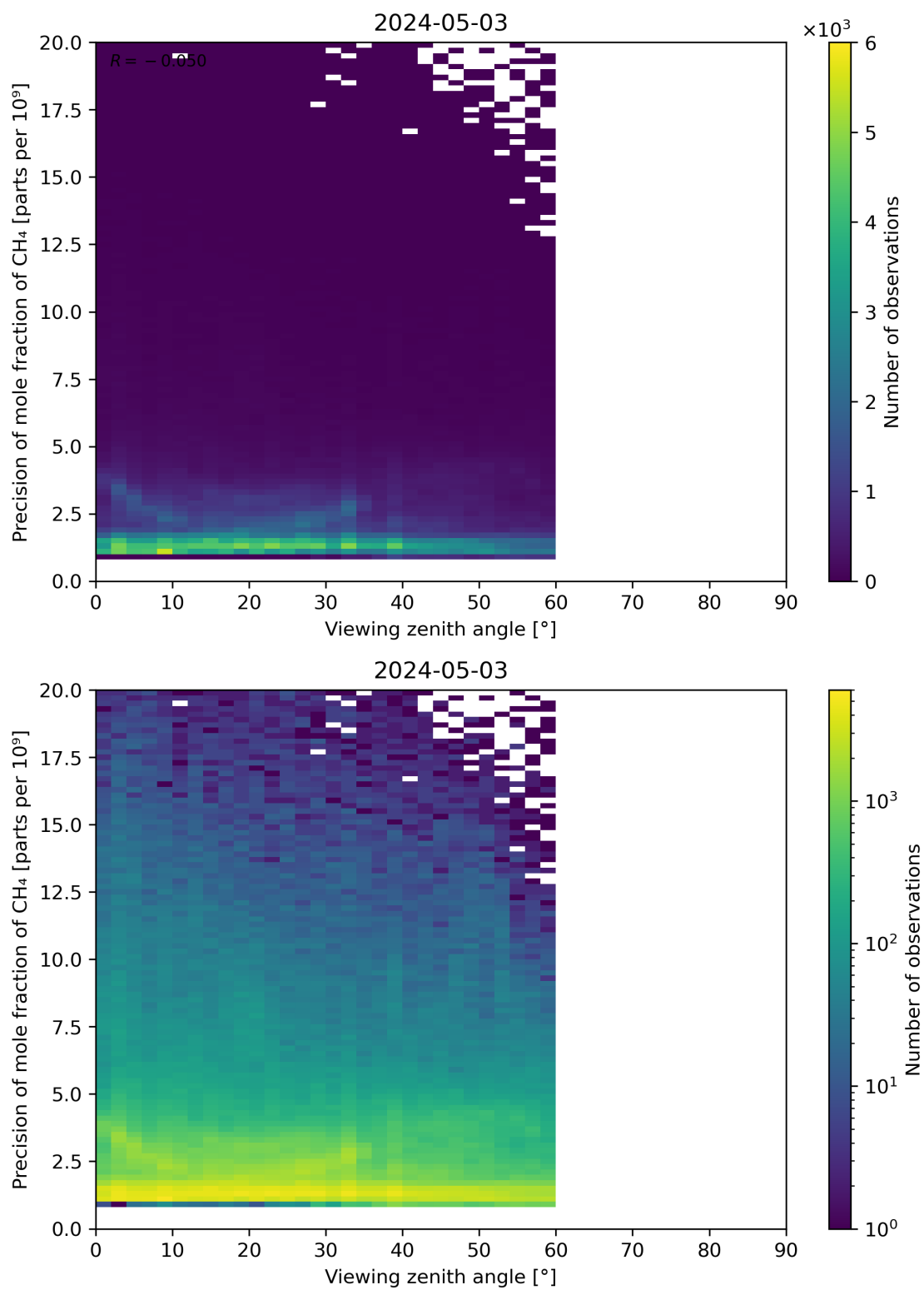
Figure 112: Scatter density plot of “Viewing zenith angle” against “Precision of mole fraction of CH 4 ” for 2024-05-02 to 2024-05-04.
