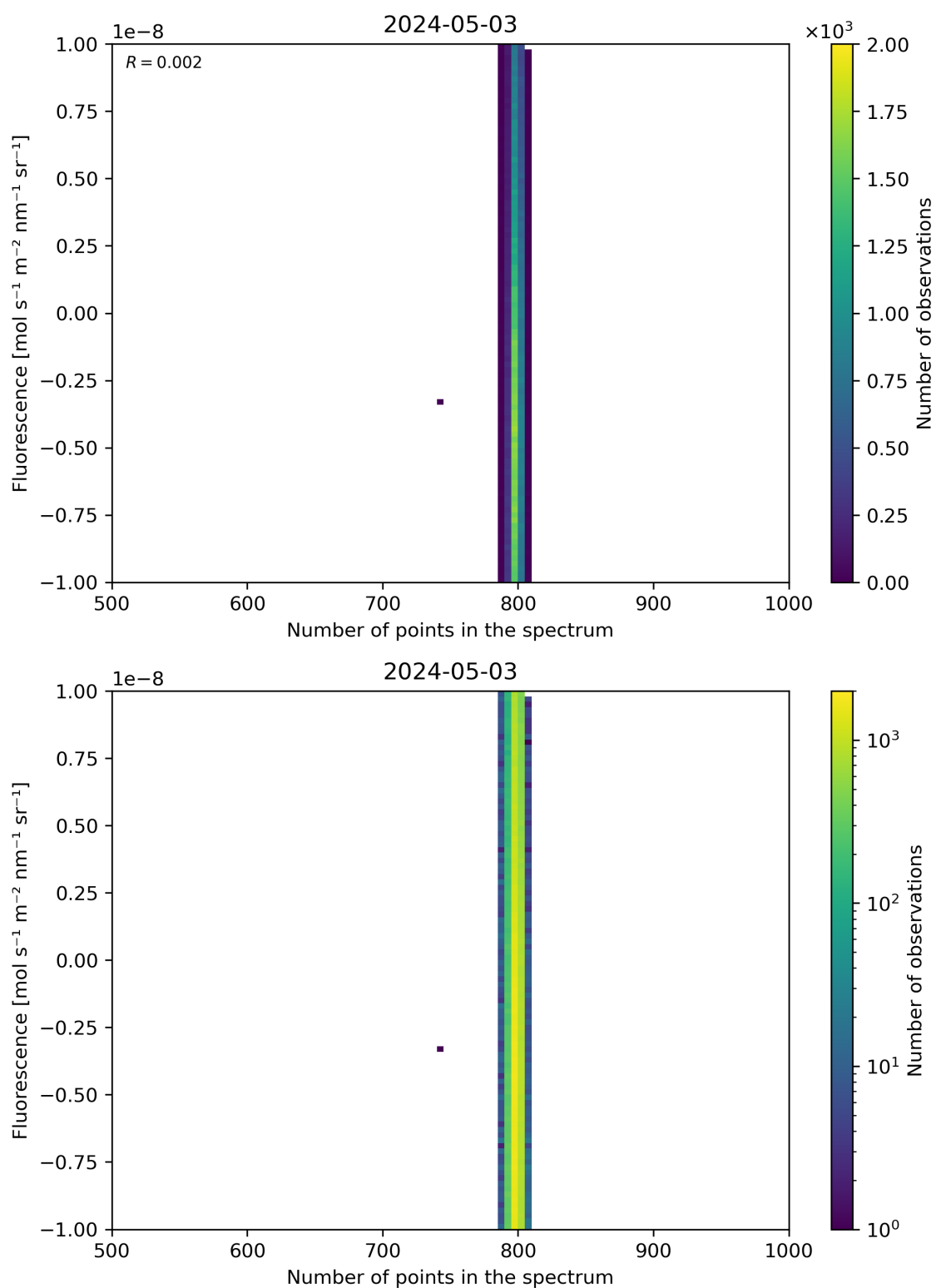
Figure 91: Scatter density plot of “Number of points in the spectrum” against “Fluorescence” for 2024-05-02 to 2024-05-04.
