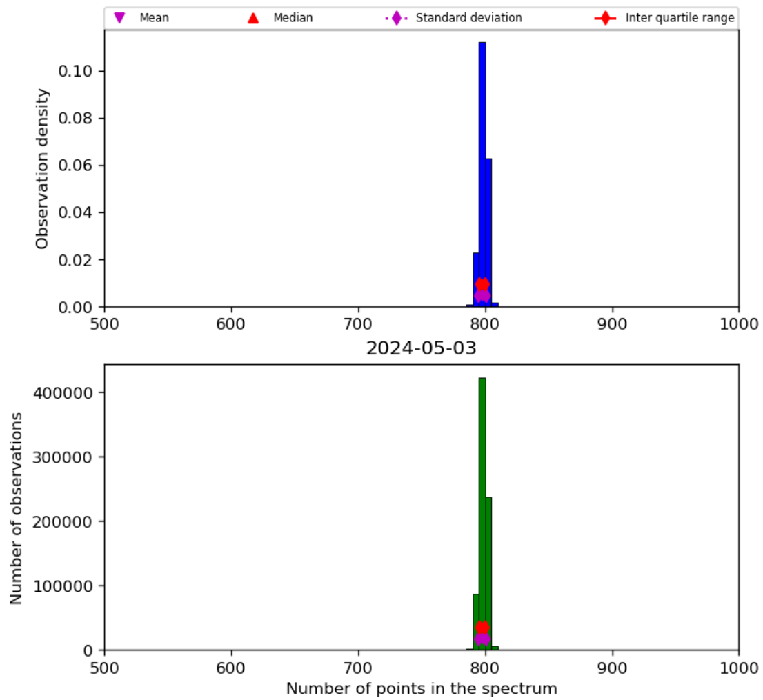
Figure 26: Histogram of “Number of points in the spectrum” for 2024-05-02 to 2024-05-04
