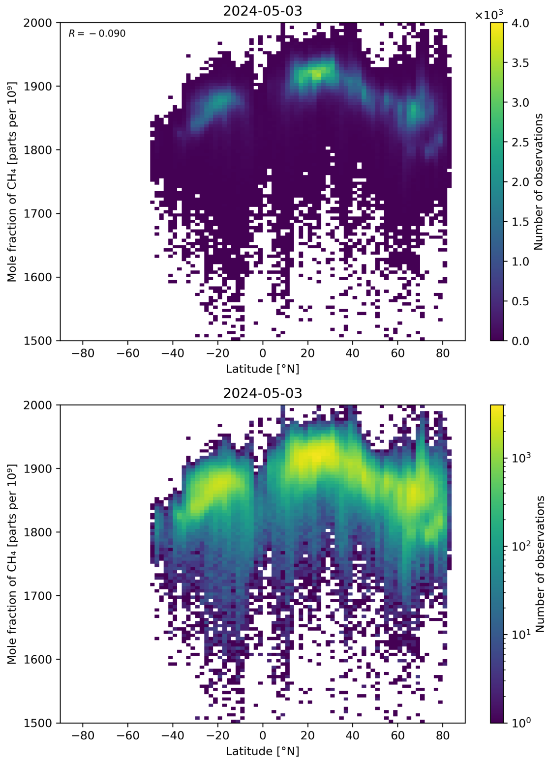
Figure 57: Scatter density plot of “Latitude” against “Mole fraction of CH 4 ” for 2024-05-02 to 2024-05-04.
