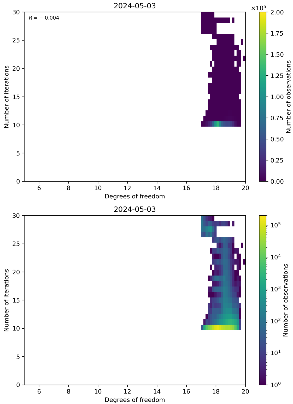
Figure 52: Scatter density plot of “Degrees of freedom” against “Number of iterations” for 2024-05-02 to 2024-05-04.
