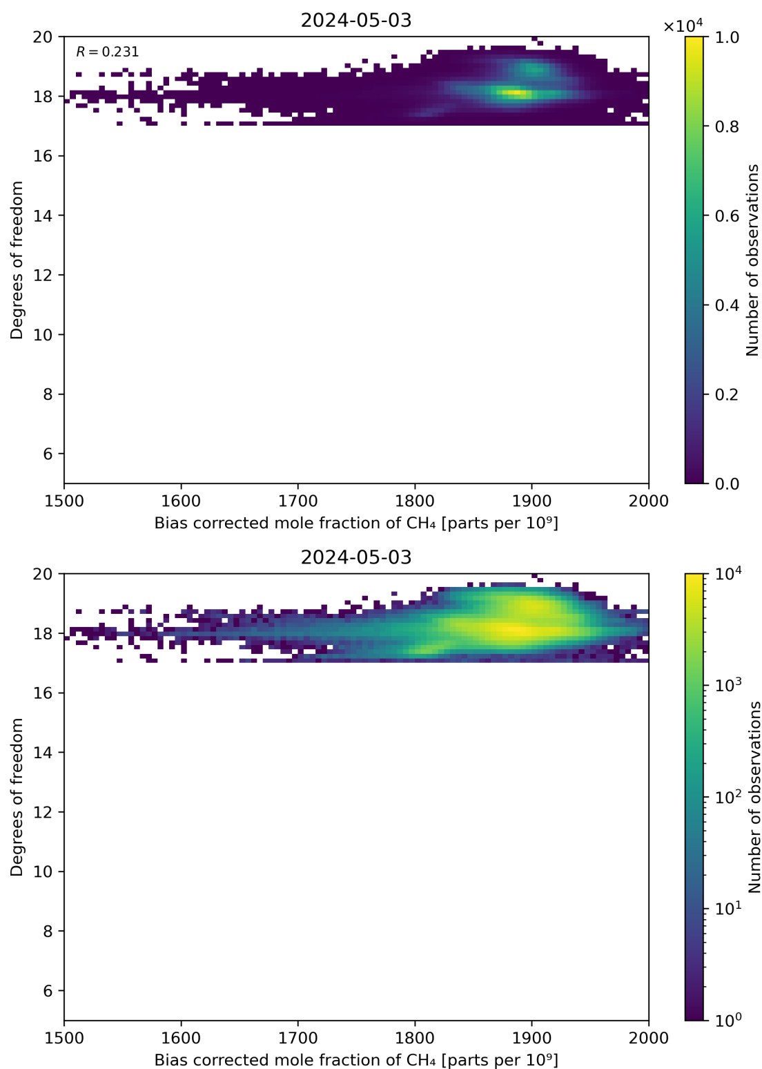
Figure 65: Scatter density plot of “Bias corrected mole fraction of CH 4 ” against “Degrees of freedom” for 2024-05-02 to 2024-05-04.
