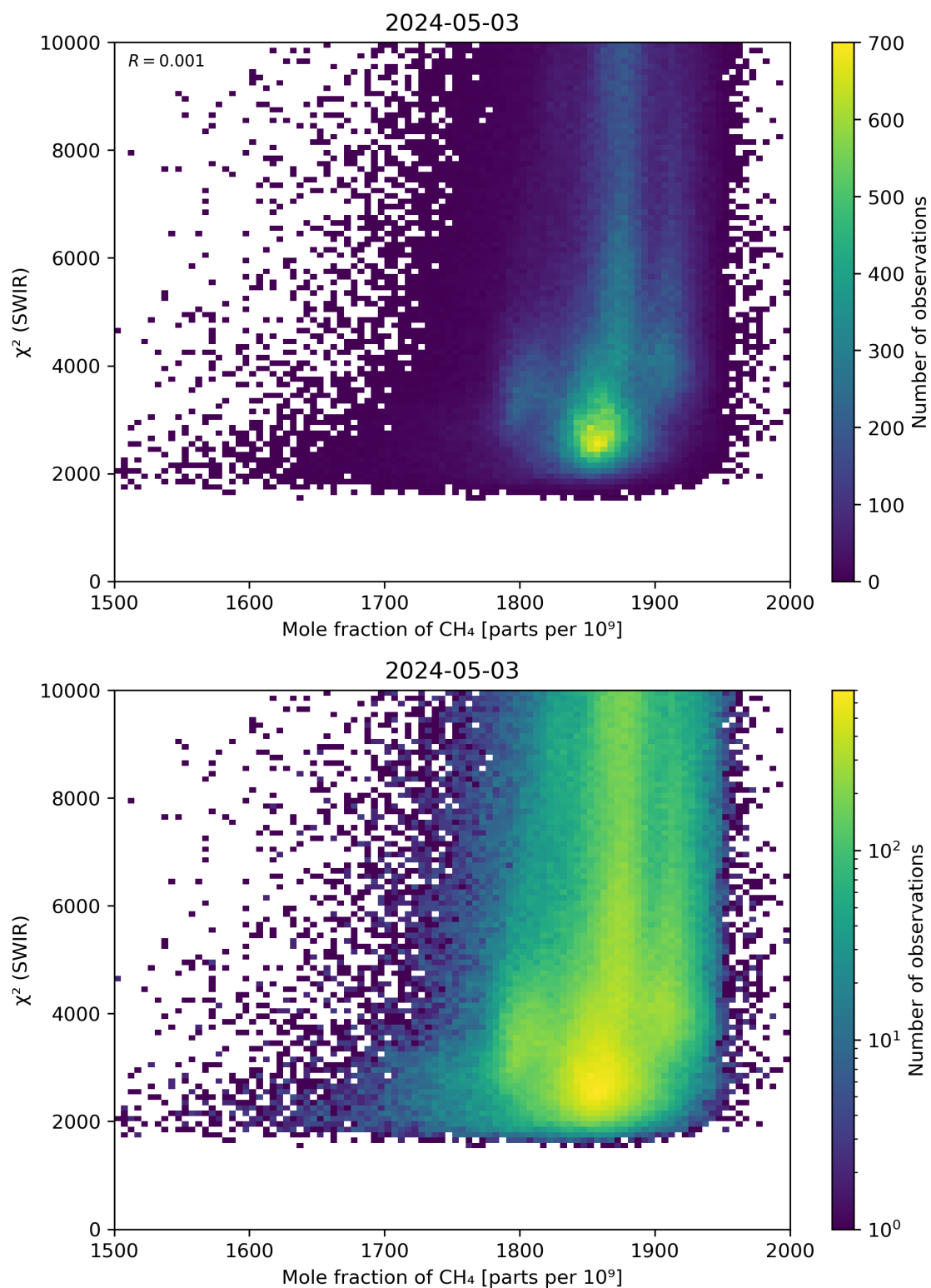
Figure 71: Scatter density plot of “Mole fraction of CH 4 ” against “ \chi^2 (SWIR)” for 2024-05-02 to 2024-05-04.
