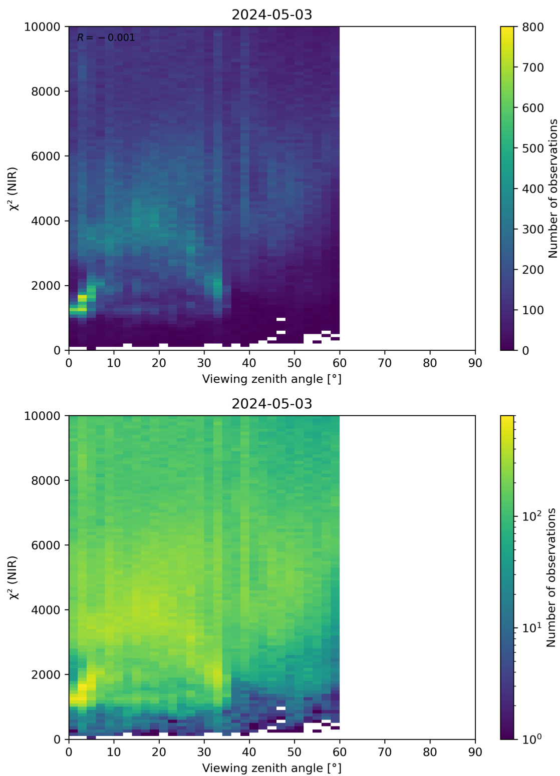
Figure 105: Scatter density plot of “Viewing zenith angle” against “ \chi^2 (NIR)” for 2024-05-02 to 2024-05-04.
