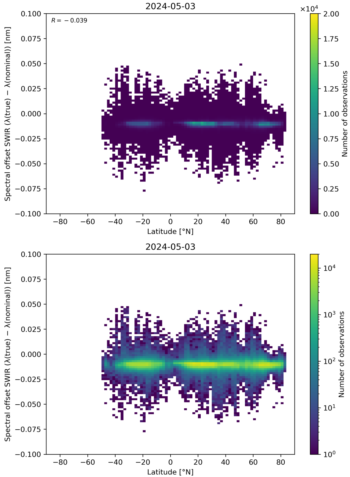
Figure 62: Scatter density plot of “Latitude” against “Spectral offset SWIR ( \lambda(\text{true}) - \lambda(\text{nominal}) )” for 2024-05-02 to 2024-05-04.
