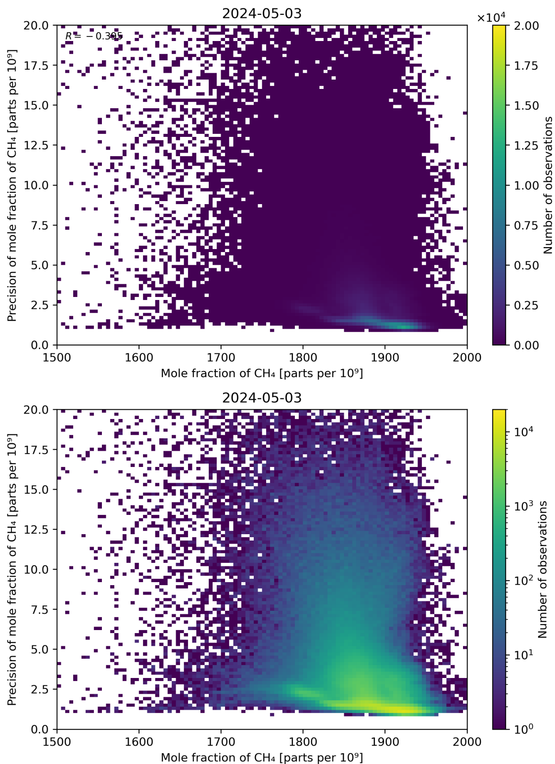
Figure 75: Scatter density plot of “Mole fraction of CH 4 ” against “Precision of mole fraction of CH 4 ” for 2024-05-02 to 2024-05-04.
