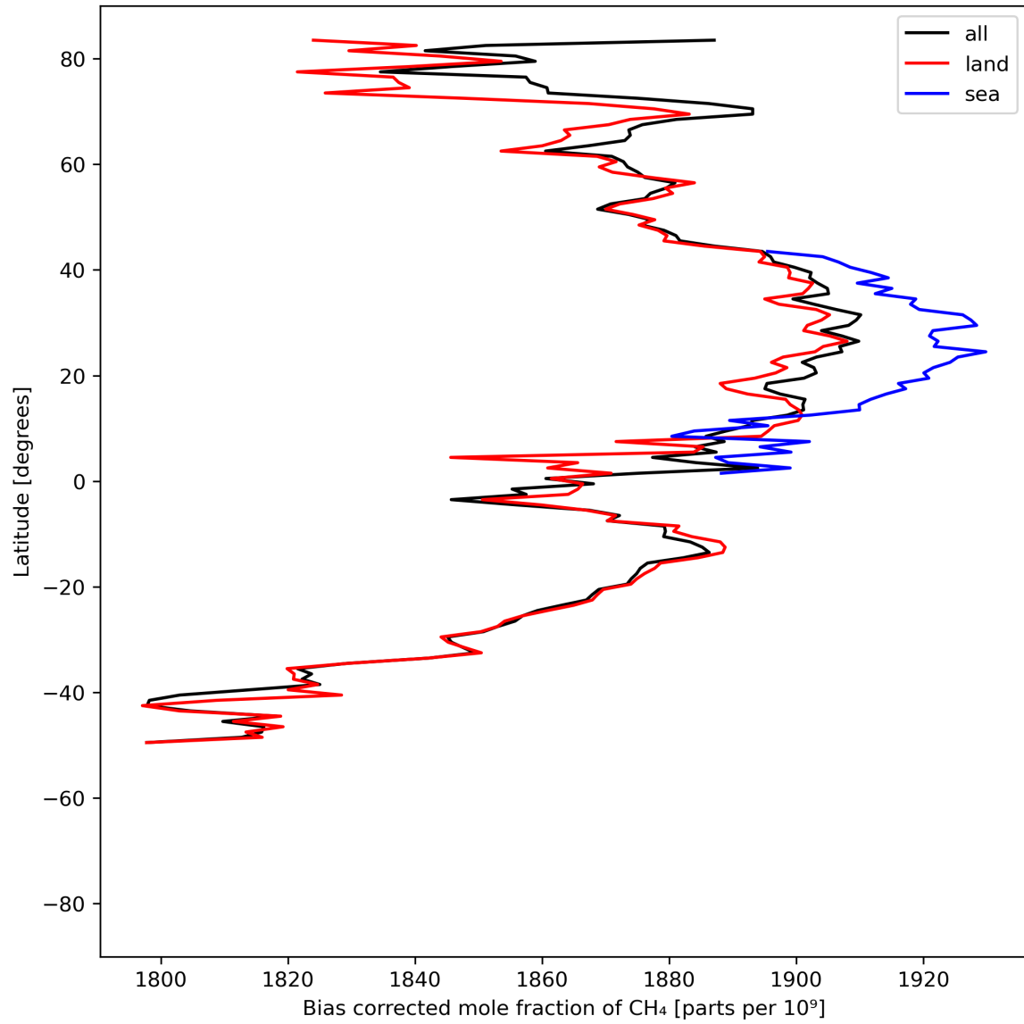
Figure 14: Zonal average of “Bias corrected mole fraction of CH 4 ” for 2024-05-02 to 2024-05-04.
