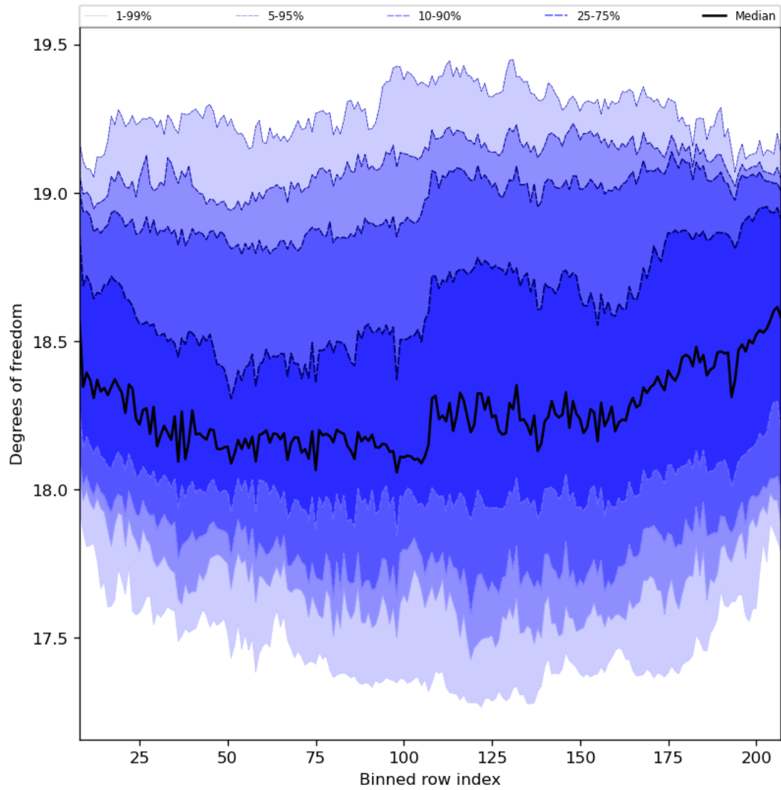
Figure 41: Along track statistics of “Degrees of freedom” for 2024-05-02 to 2024-05-04
