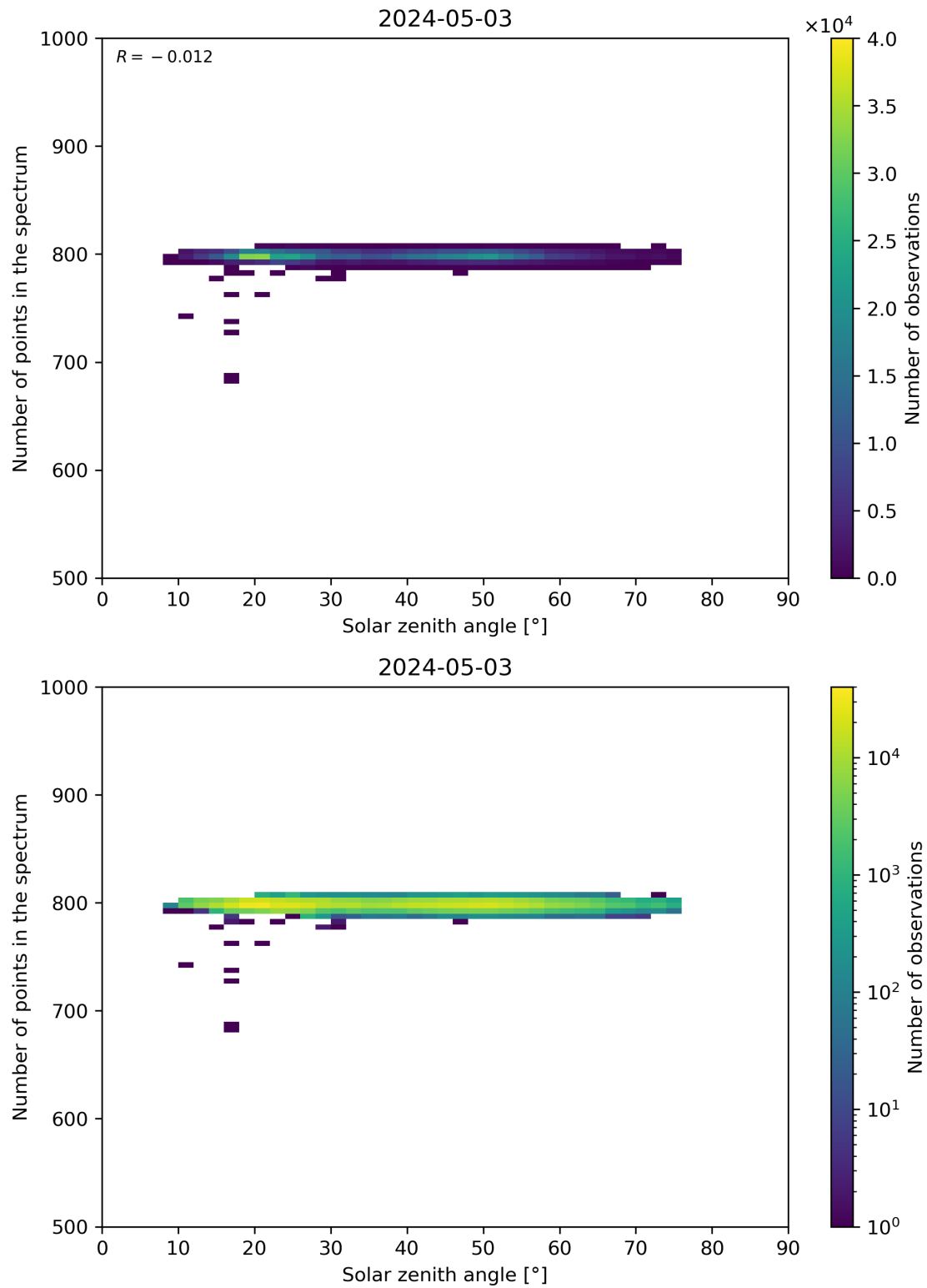
Figure 103: Scatter density plot of “Solar zenith angle” against “Number of points in the spectrum” for 2024-05-02 to 2024-05-04.
