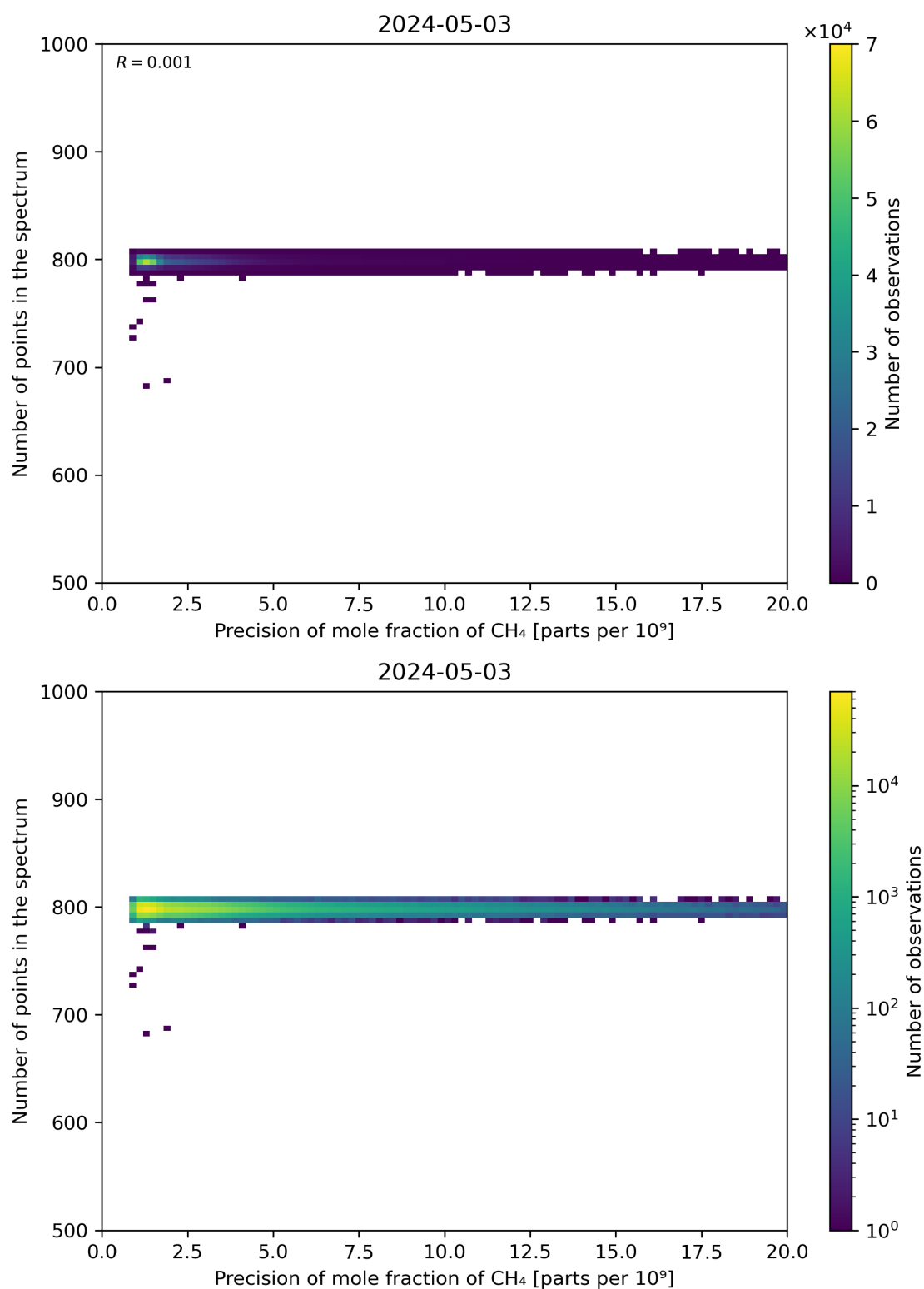
Figure 84: Scatter density plot of “Precision of mole fraction of CH 4 ” against “Number of points in the spectrum” for 2024-05-02 to 2024-05-04.
