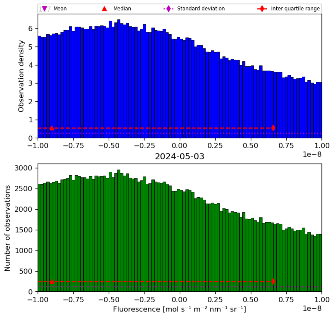
Figure 32: Histogram of “Fluorescence” for 2024-05-02 to 2024-05-04
