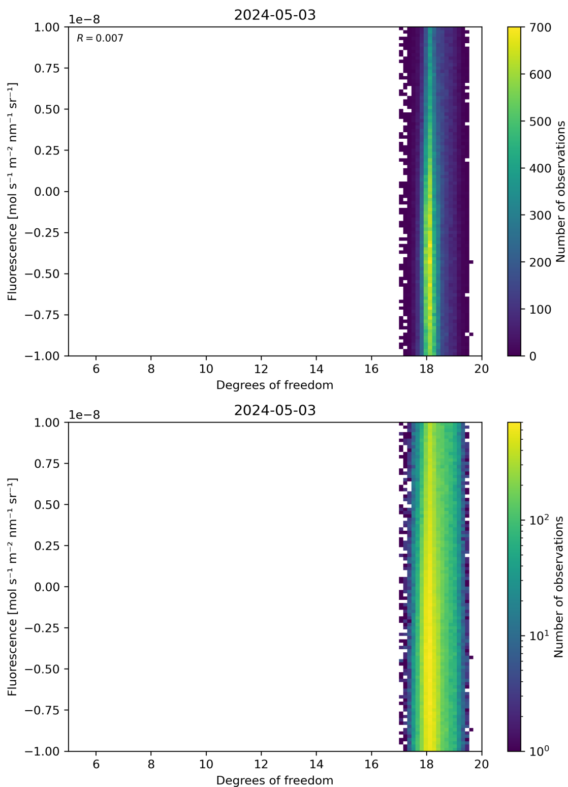
Figure 51: Scatter density plot of “Degrees of freedom” against “Fluorescence” for 2024-05-02 to 2024-05-04.
