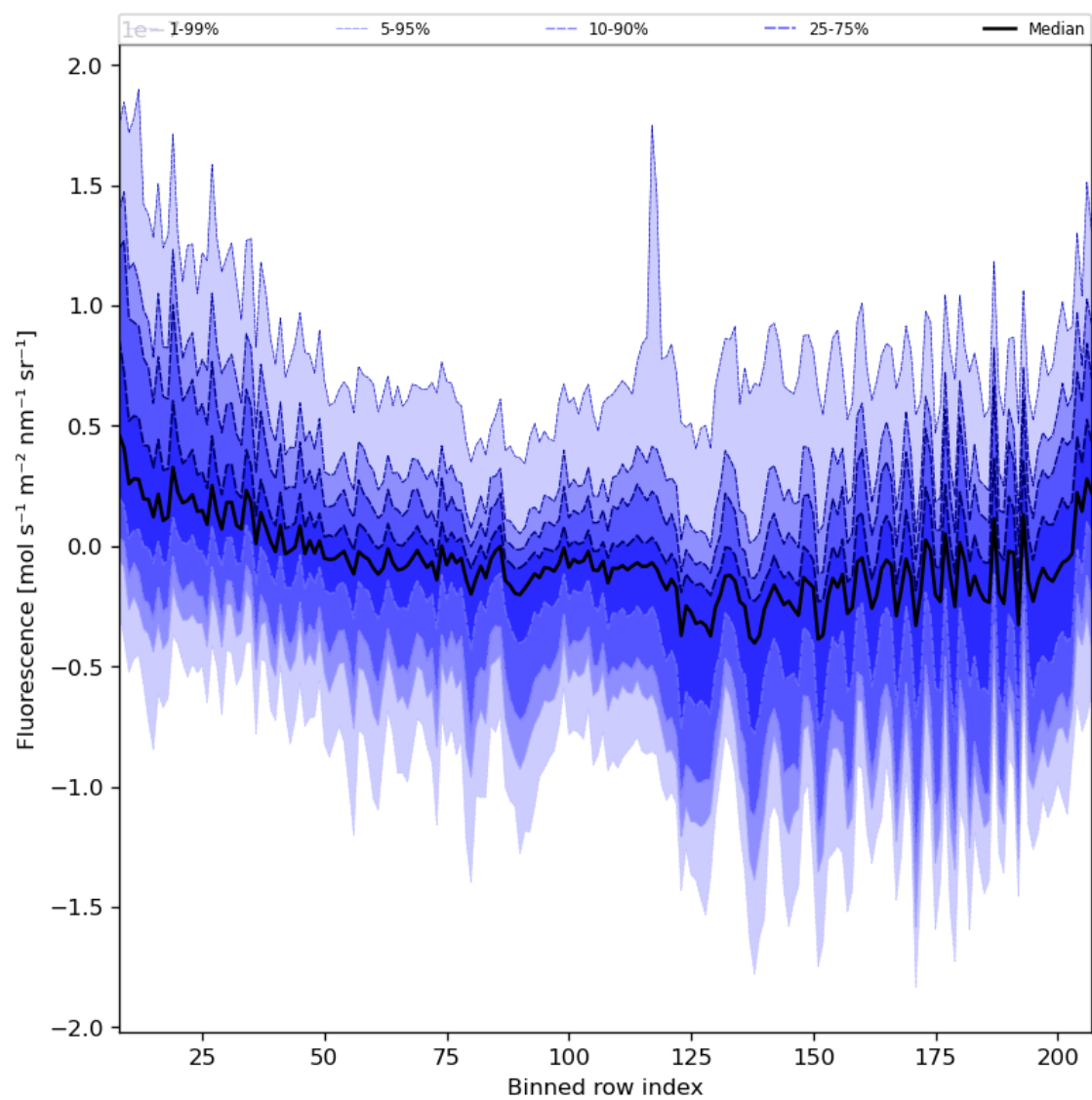
Figure 43: Along track statistics of “Fluorescence” for 2024-05-02 to 2024-05-04
