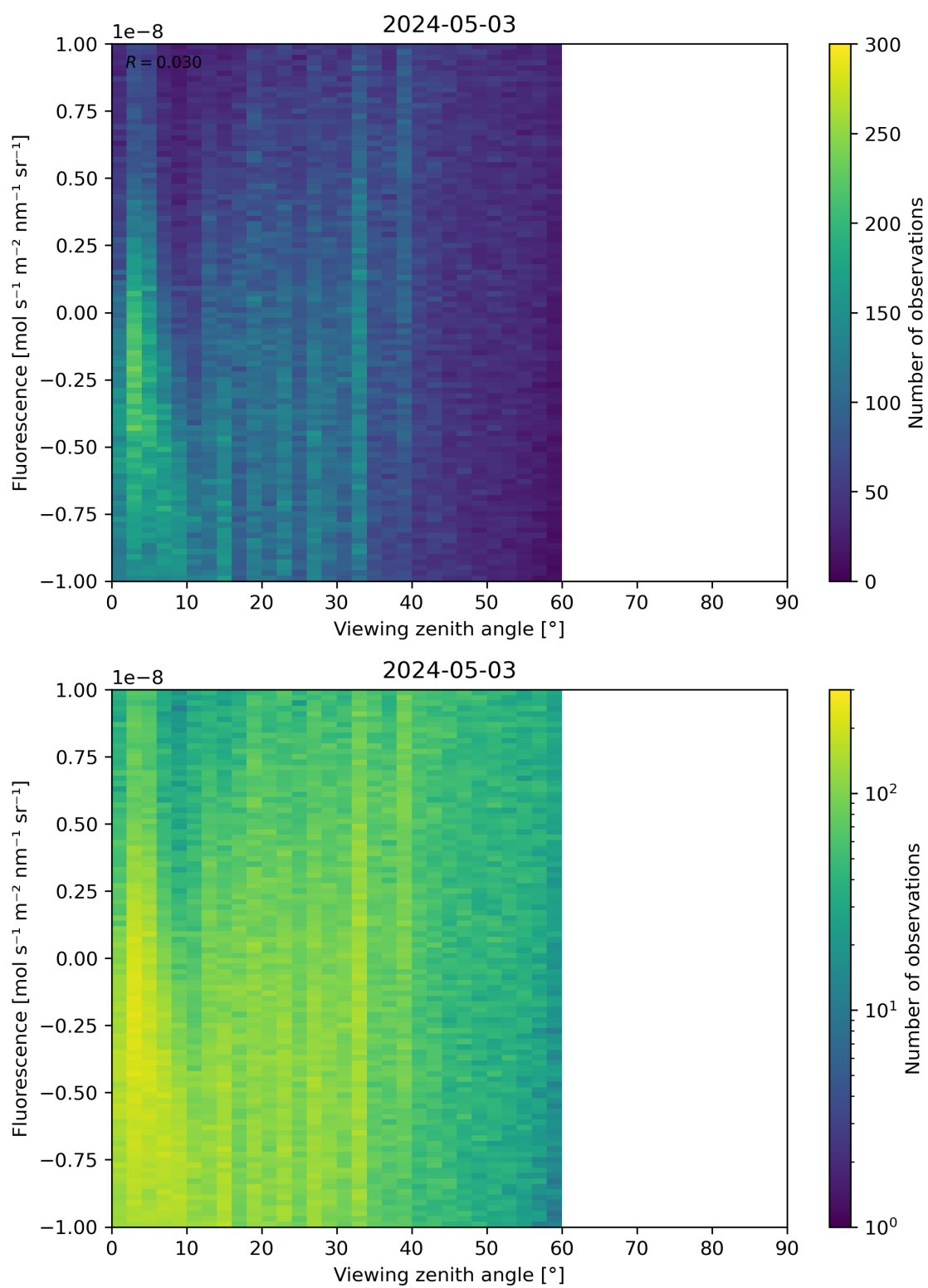
Figure 108: Scatter density plot of “Viewing zenith angle” against “Fluorescence” for 2024-05-02 to 2024-05-04.
