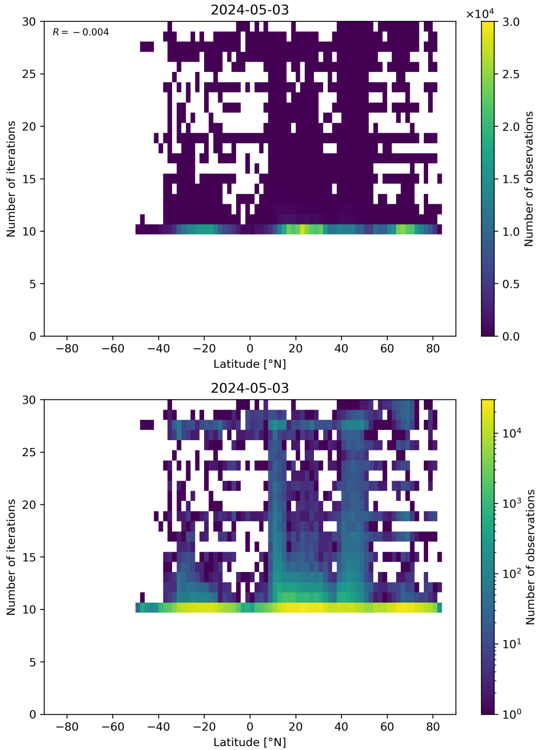
Figure 60: Scatter density plot of “Latitude” against “Number of iterations” for 2024-05-02 to 2024-05-04.
