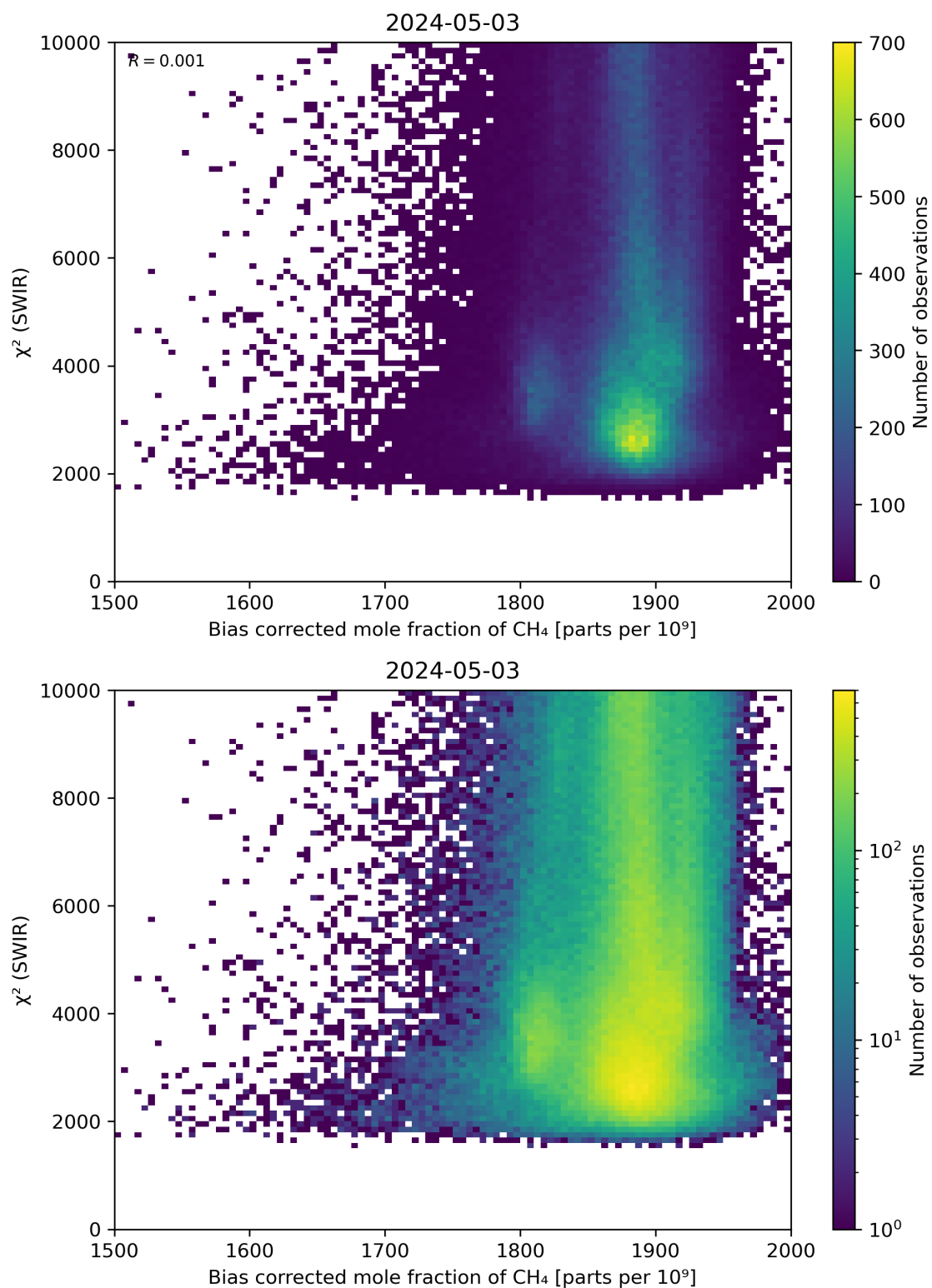
Figure 64: Scatter density plot of “Bias corrected mole fraction of \text{CH}_4 ” against “ \chi^2 (SWIR)” for 2024-05-02 to 2024-05-04.
