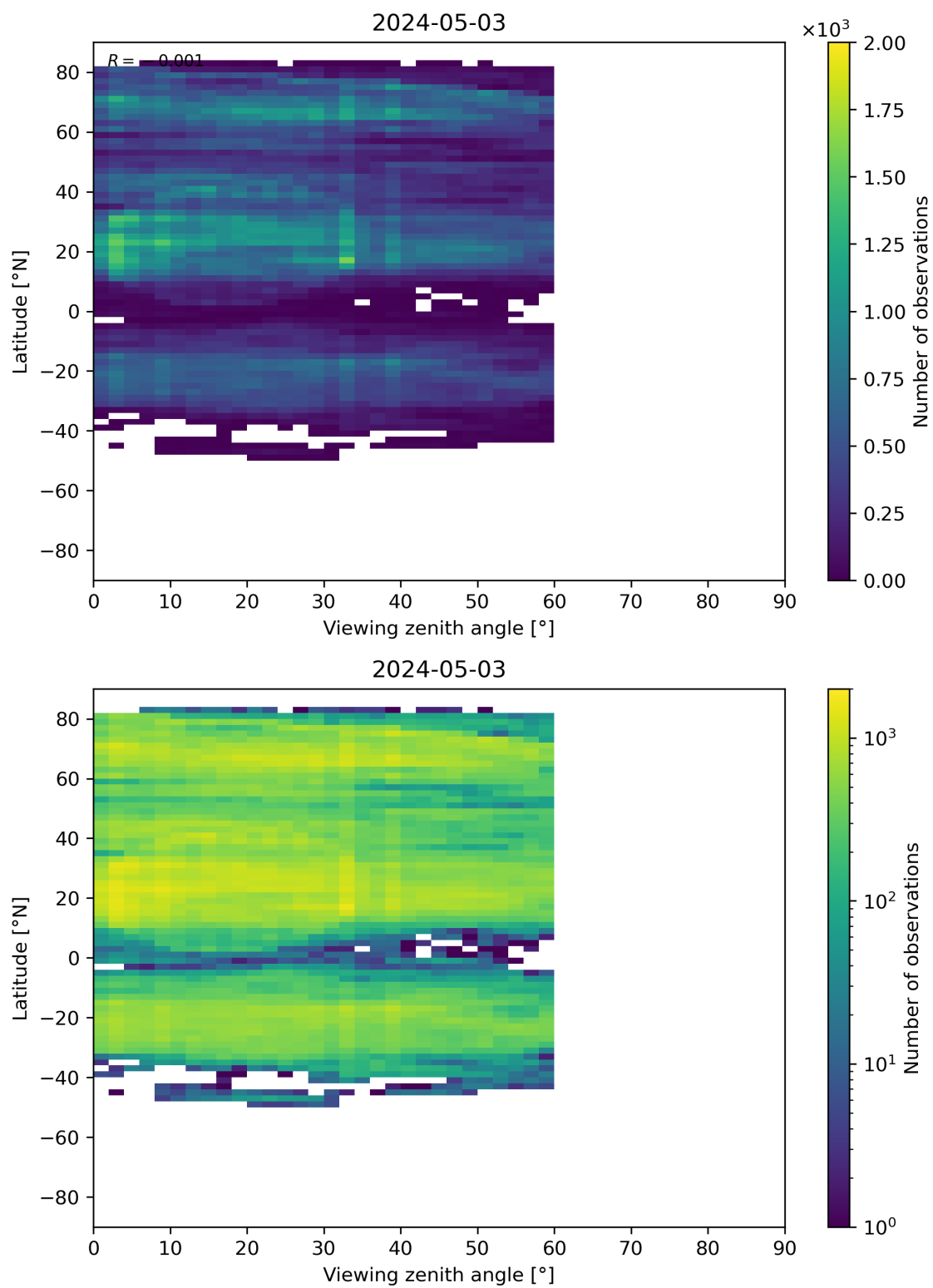
Figure 109: Scatter density plot of “Viewing zenith angle” against “Latitude” for 2024-05-02 to 2024-05-04.
