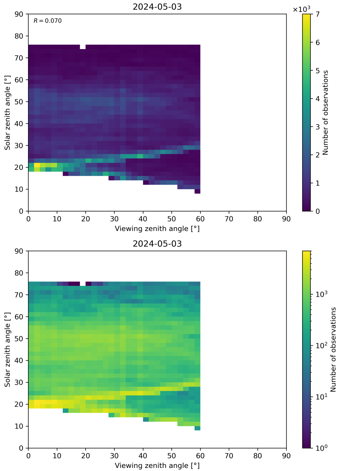
Figure 115: Scatter density plot of “Viewing zenith angle” against “Solar zenith angle” for 2024-05-02 to 2024-05-04.
