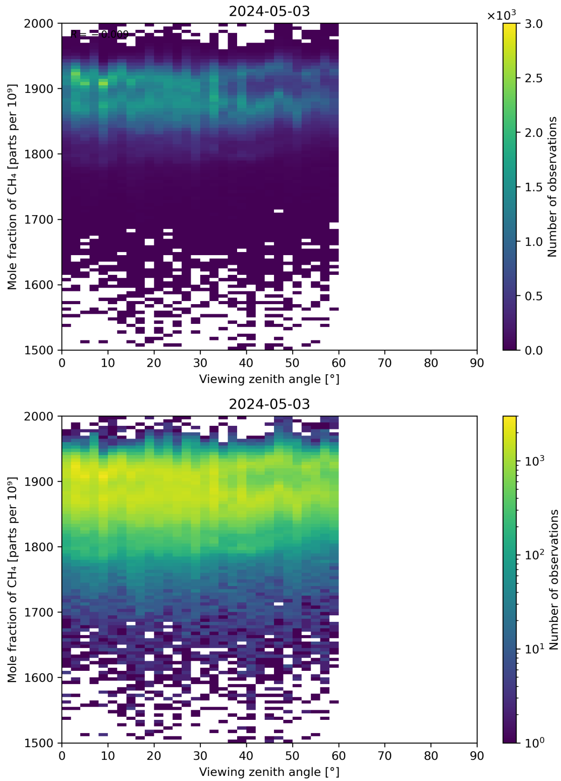
Figure 110: Scatter density plot of “Viewing zenith angle” against “Mole fraction of CH 4 ” for 2024-05-02 to 2024-05-04.
