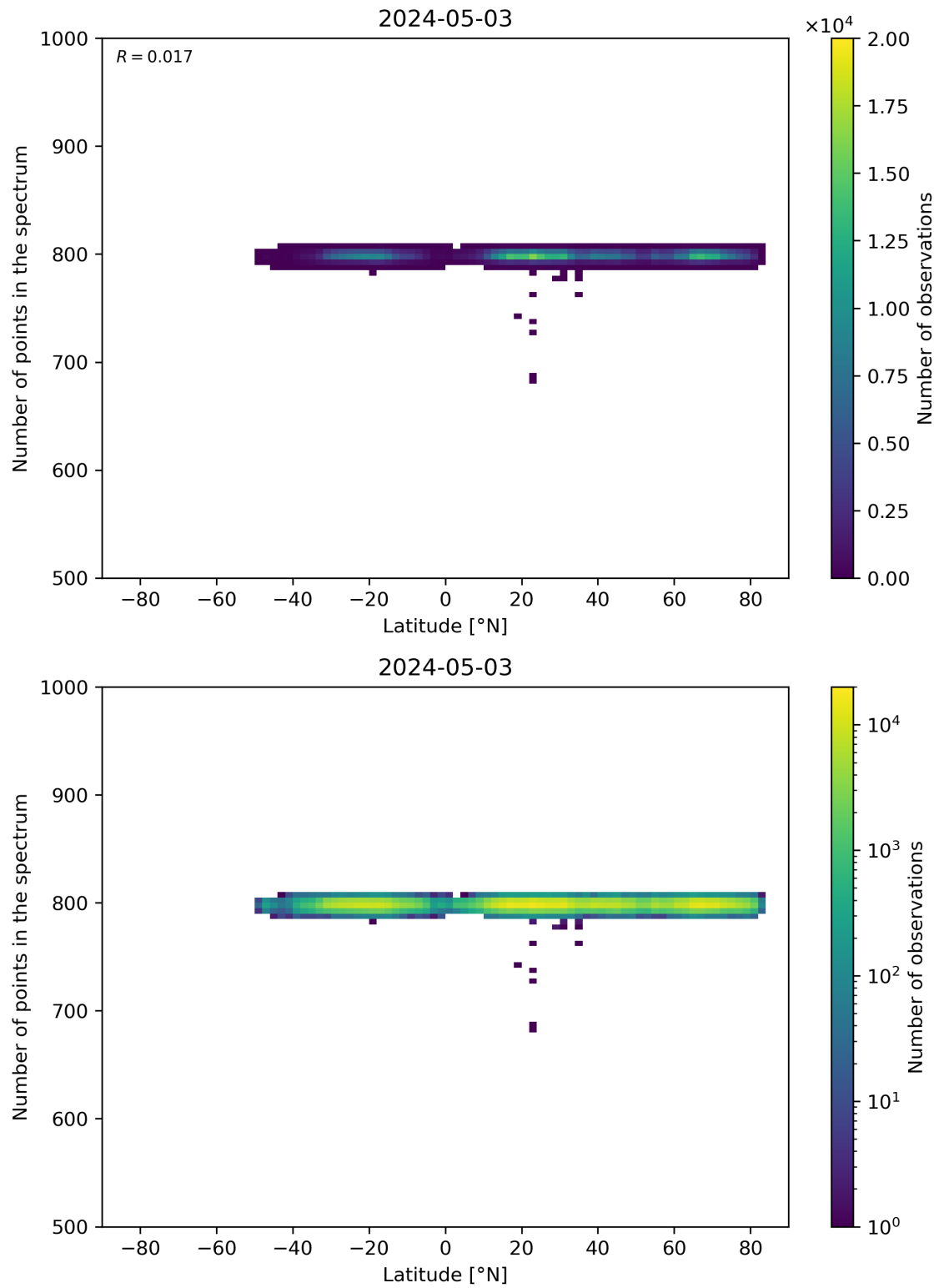
Figure 61: Scatter density plot of “Latitude” against “Number of points in the spectrum” for 2024-05-02 to 2024-05-04.
