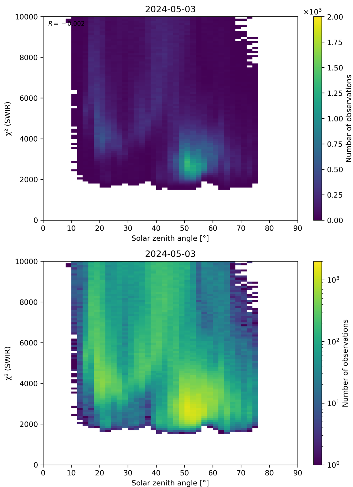
Figure 95: Scatter density plot of “Solar zenith angle” against “ \chi^2 (SWIR)” for 2024-05-02 to 2024-05-04.
