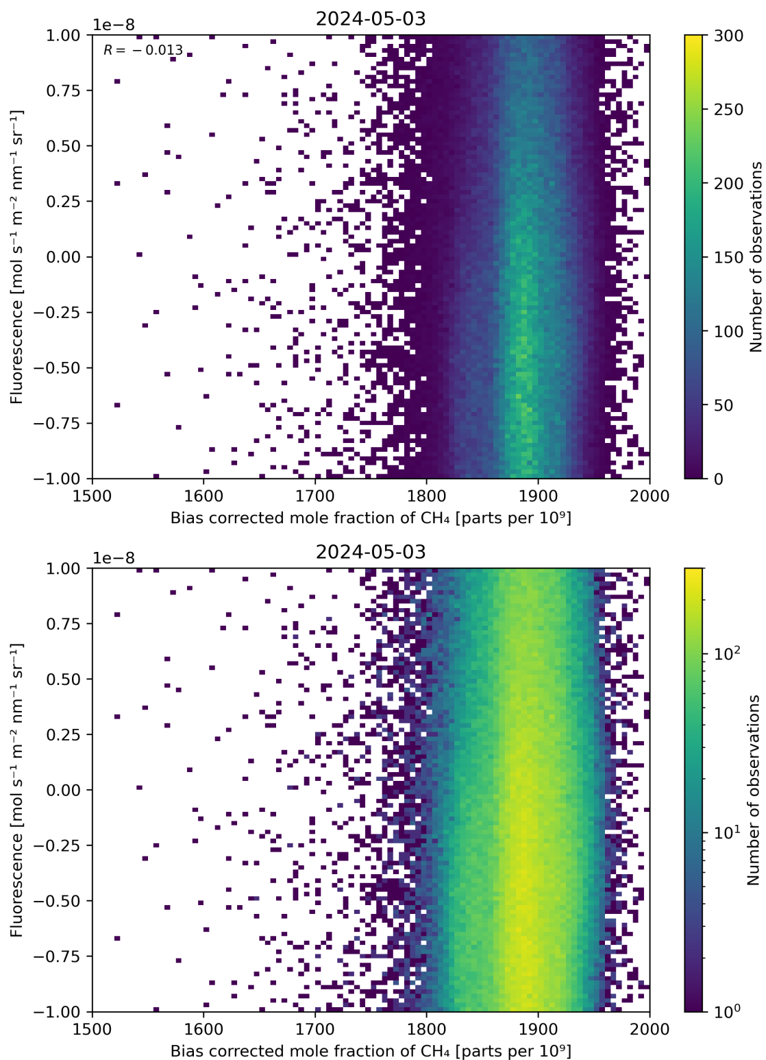
Figure 66: Scatter density plot of “Bias corrected mole fraction of \text{CH}_4 ” against “Fluorescence” for 2024-05-02 to 2024-05-04.
