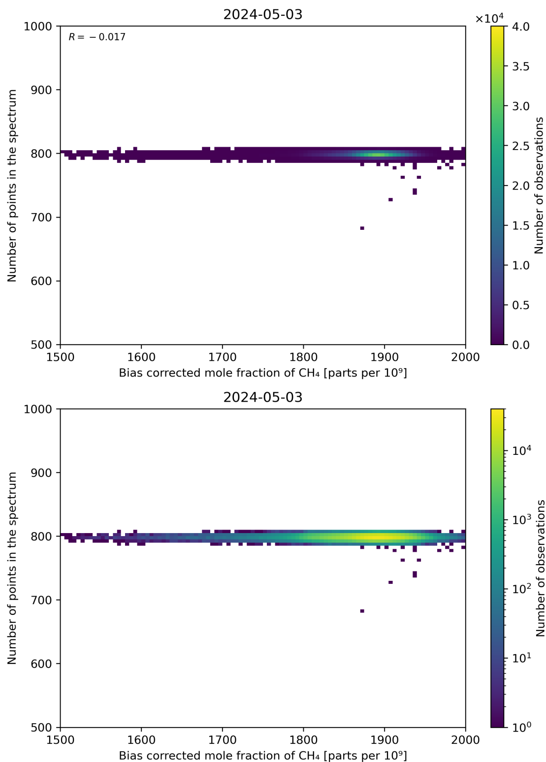
Figure 68: Scatter density plot of “Bias corrected mole fraction of CH 4 ” against “Number of points in the spectrum” for 2024-05-02 to 2024-05-04.
