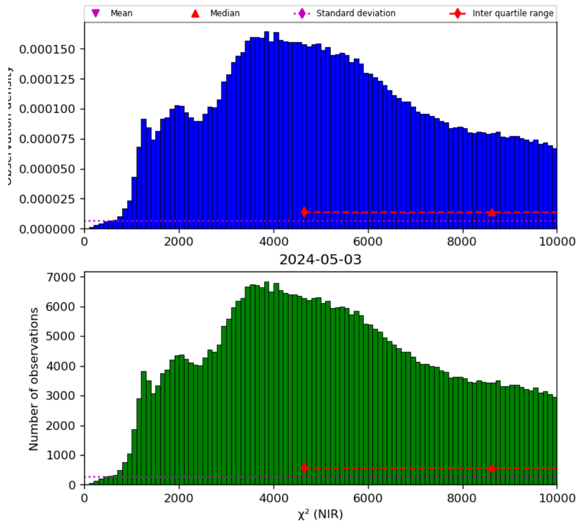
Figure 29: Histogram of “ \chi^2 (NIR)” for 2024-05-02 to 2024-05-04
