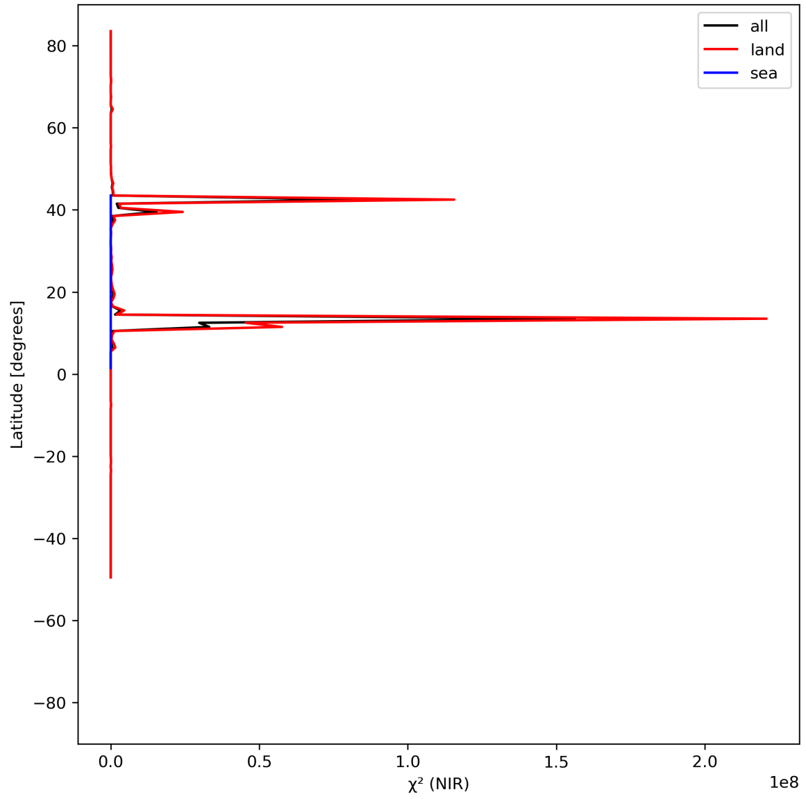
Figure 18: Zonal average of “ \chi^2 (NIR)” for 2024-05-02 to 2024-05-04.
