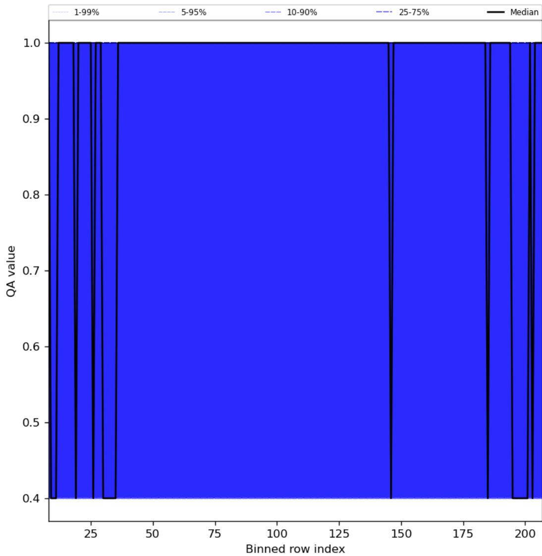
Figure 33: Along track statistics of “QA value” for 2024-05-02 to 2024-05-04
