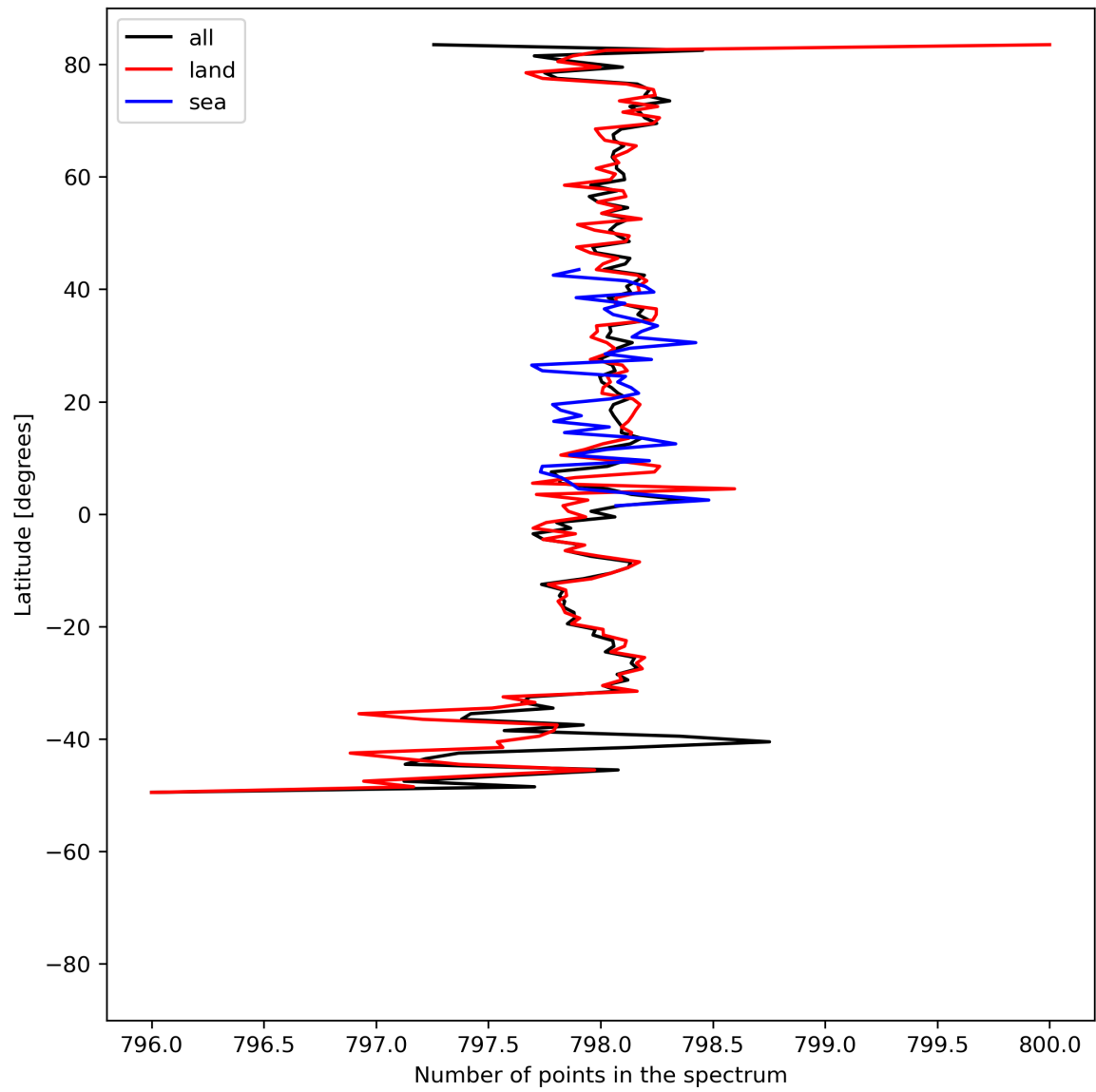
Figure 15: Zonal average of “Number of points in the spectrum” for 2024-05-02 to 2024-05-04.
