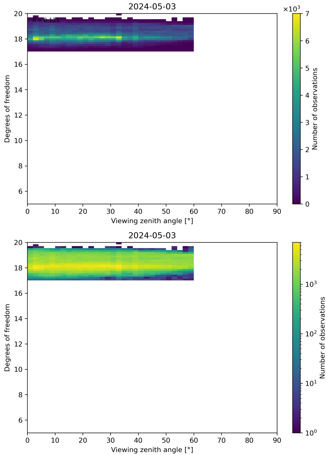
Figure 107: Scatter density plot of “Viewing zenith angle” against “Degrees of freedom” for 2024-05-02 to 2024-05-04.
