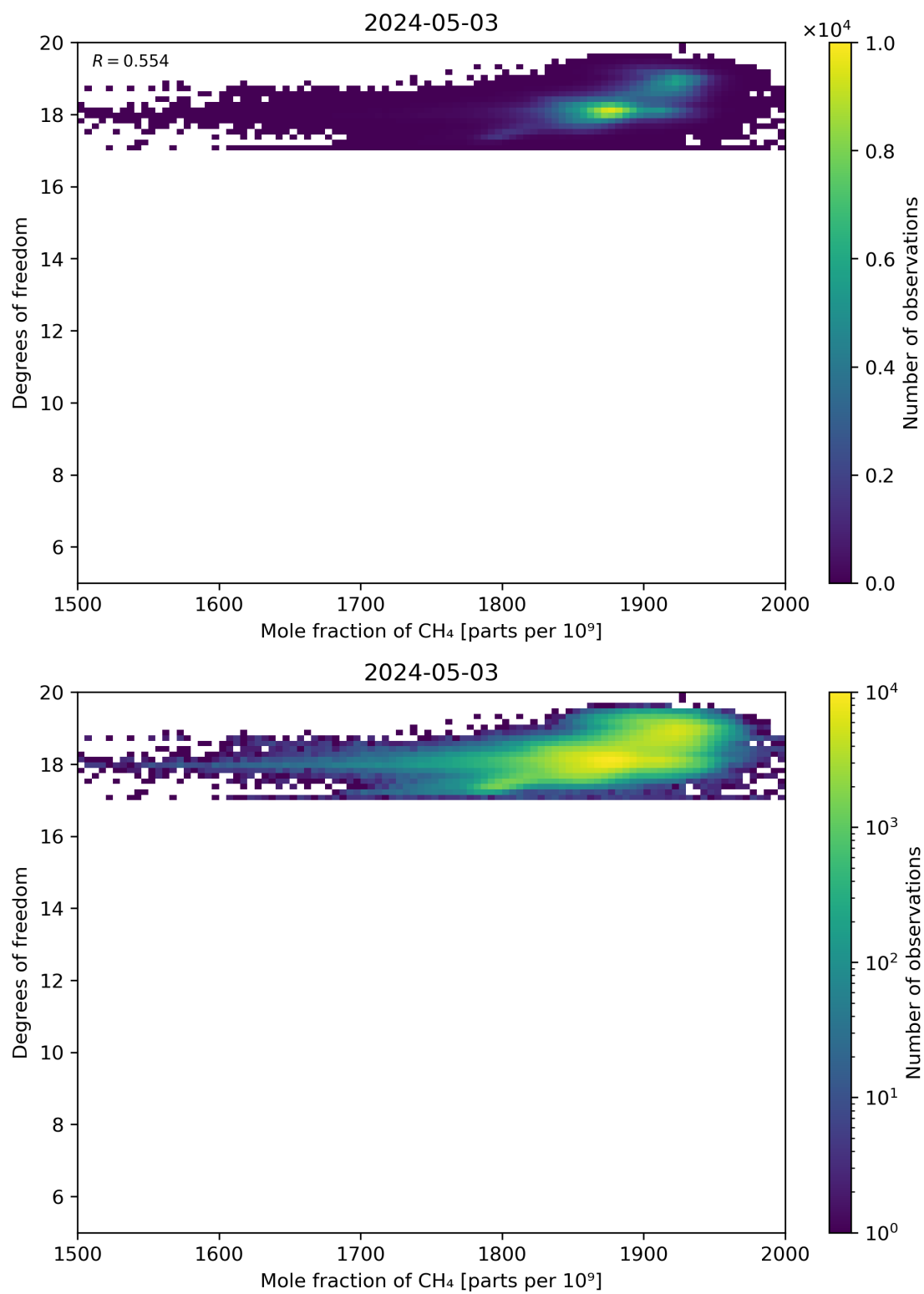
Figure 72: Scatter density plot of “Mole fraction of CH 4 ” against “Degrees of freedom” for 2024-05-02 to 2024-05-04.
