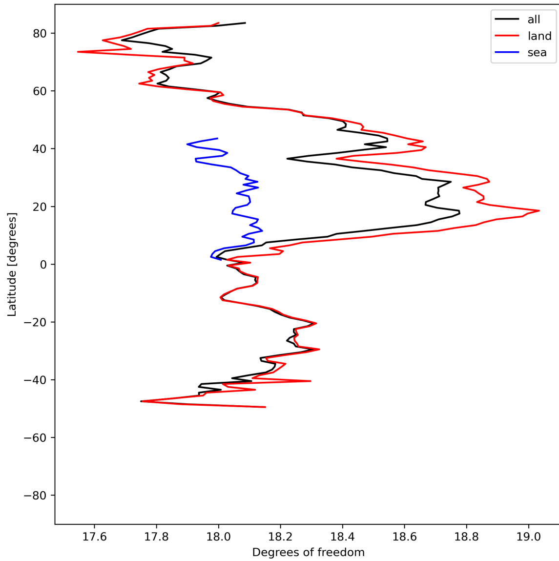
Figure 19: Zonal average of “Degrees of freedom” for 2024-05-02 to 2024-05-04.
