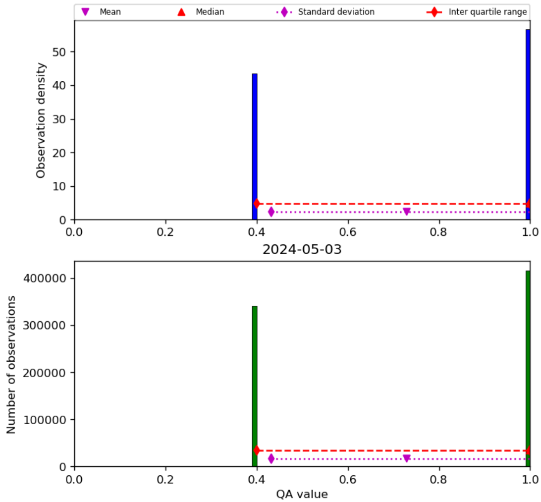
Figure 22: Histogram of “QA value” for 2024-05-02 to 2024-05-04
