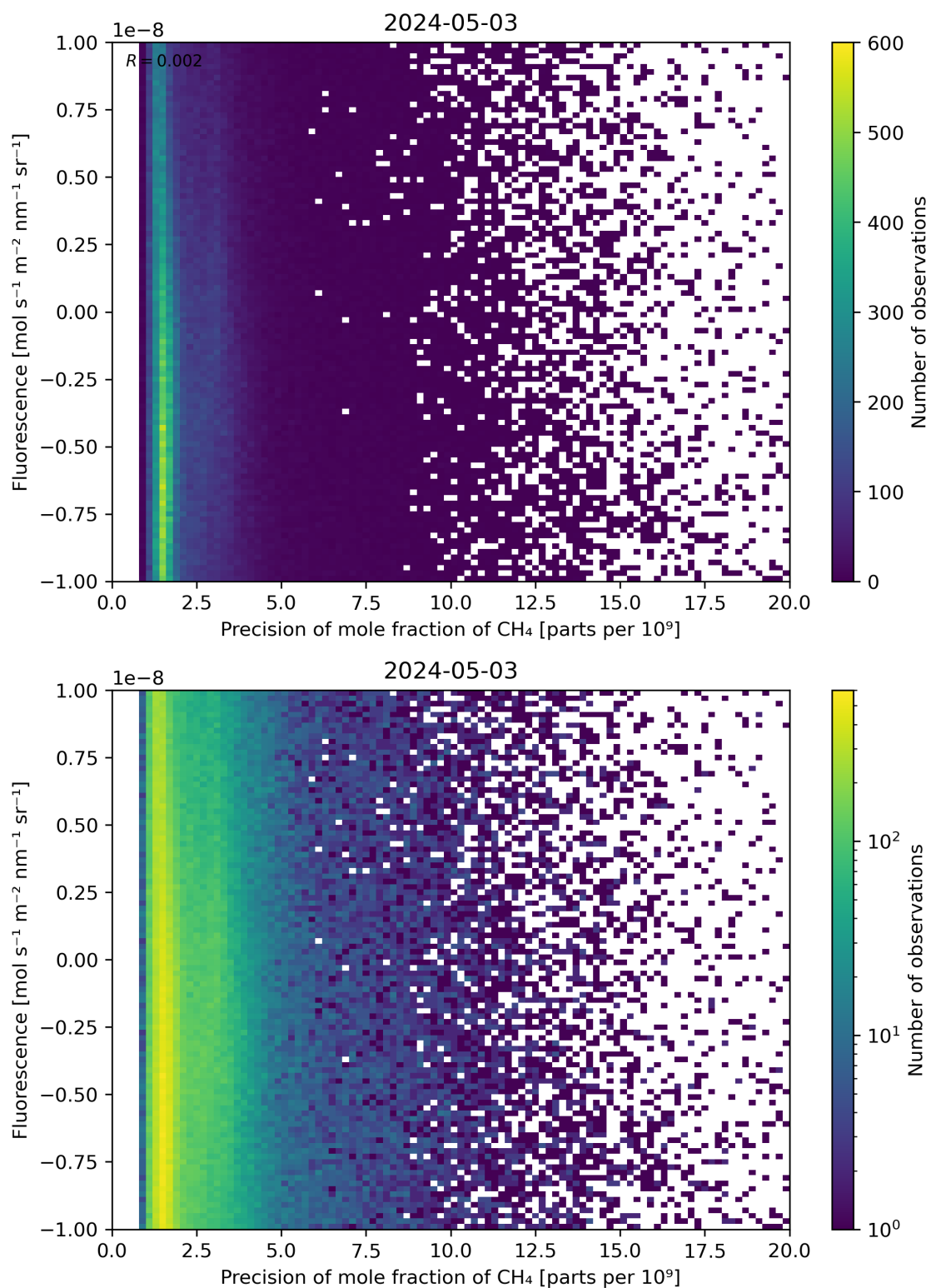
Figure 81: Scatter density plot of “Precision of mole fraction of \text{CH}_4 ” against “Fluorescence” for 2024-05-02 to 2024-05-04.
