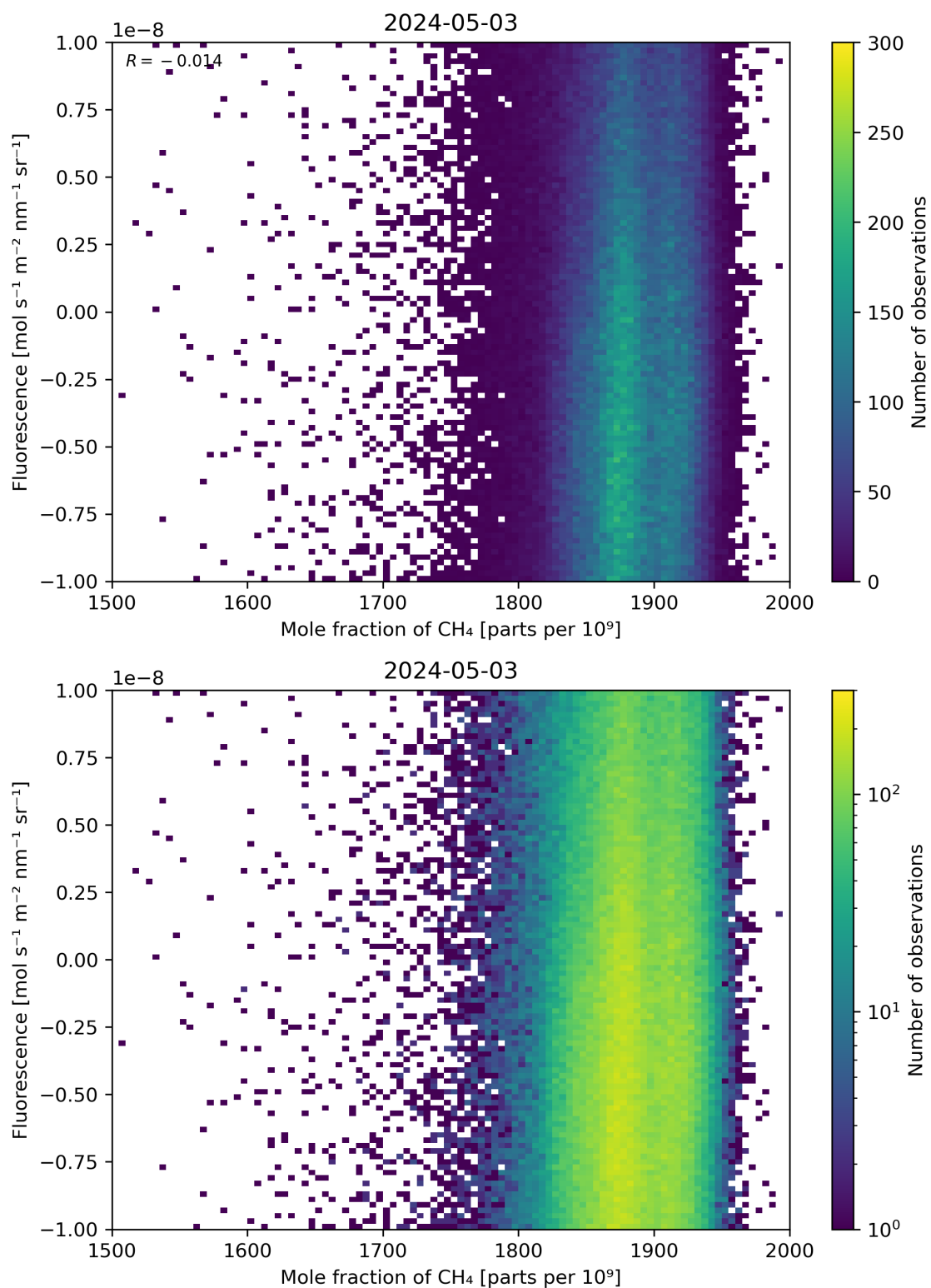
Figure 73: Scatter density plot of “Mole fraction of \text{CH}_4 ” against “Fluorescence” for 2024-05-02 to 2024-05-04.
