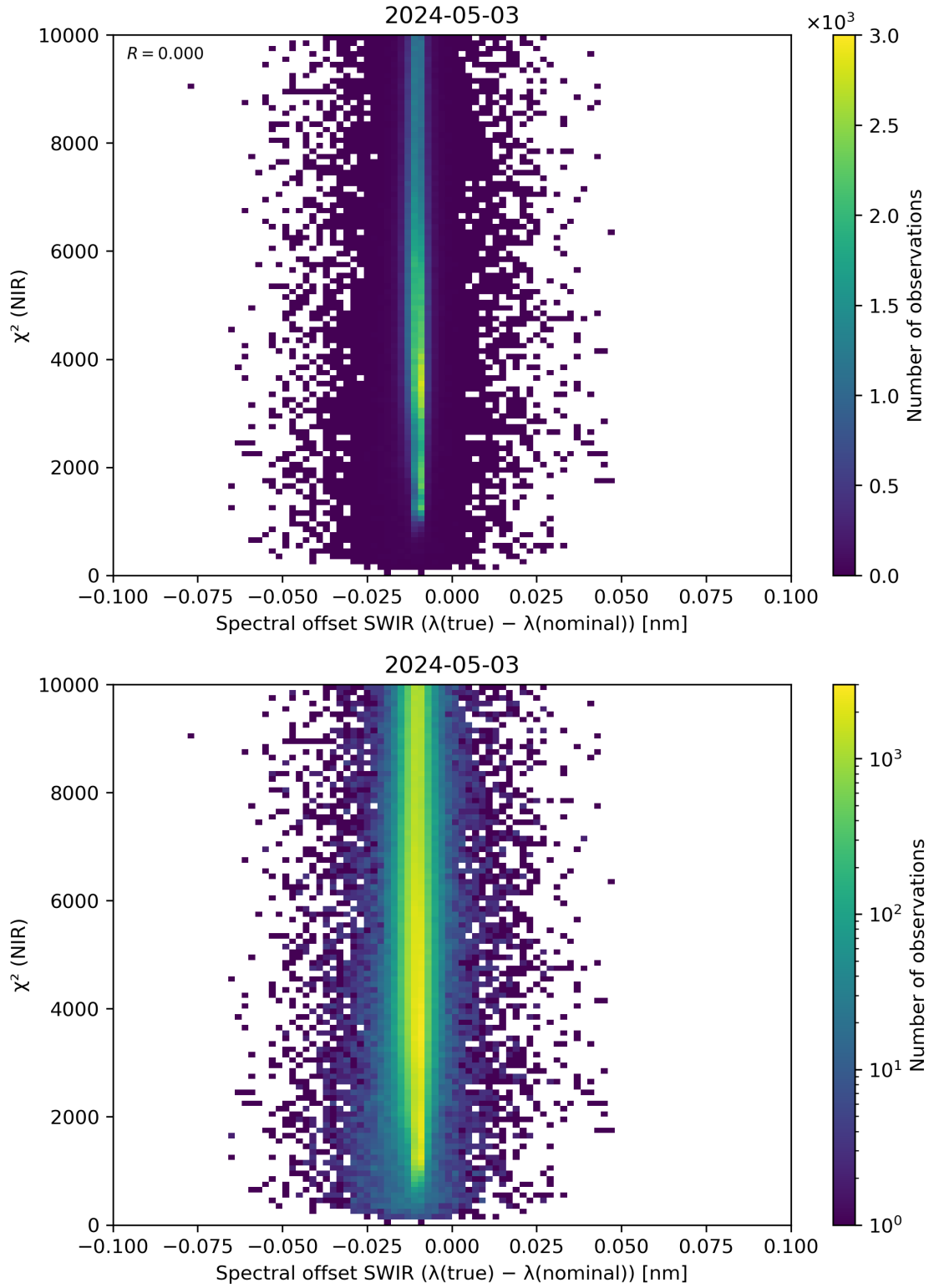
Figure 117: Scatter density plot of “Spectral offset SWIR ( \lambda(\text{true}) - \lambda(\text{nominal}) )” against “ \chi^2 (NIR)” for 2024-05-02 to 2024-05-04.
