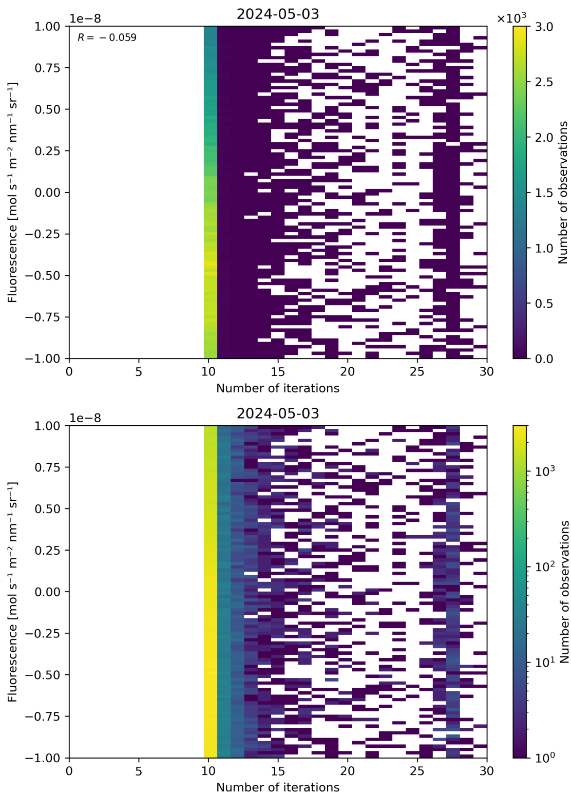
Figure 87: Scatter density plot of “Number of iterations” against “Fluorescence” for 2024-05-02 to 2024-05-04.
