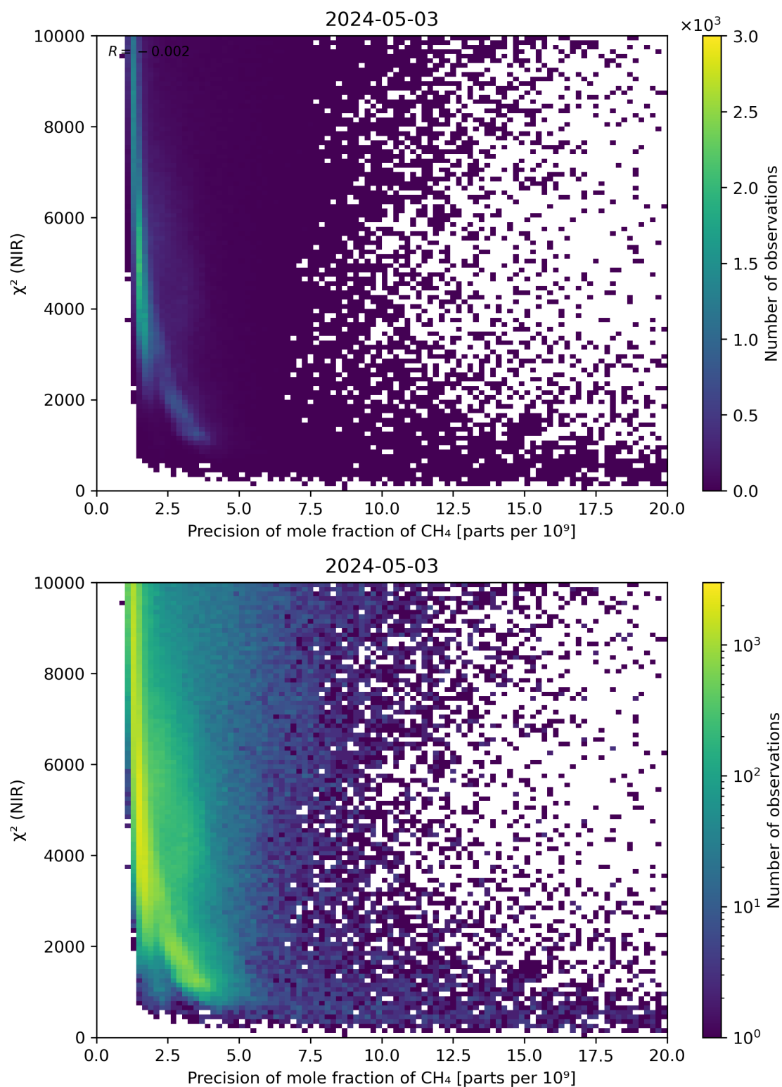
Figure 78: Scatter density plot of “Precision of mole fraction of CH 4 ” against “ \chi^2 (NIR)” for 2024-05-02 to 2024-05-04.
