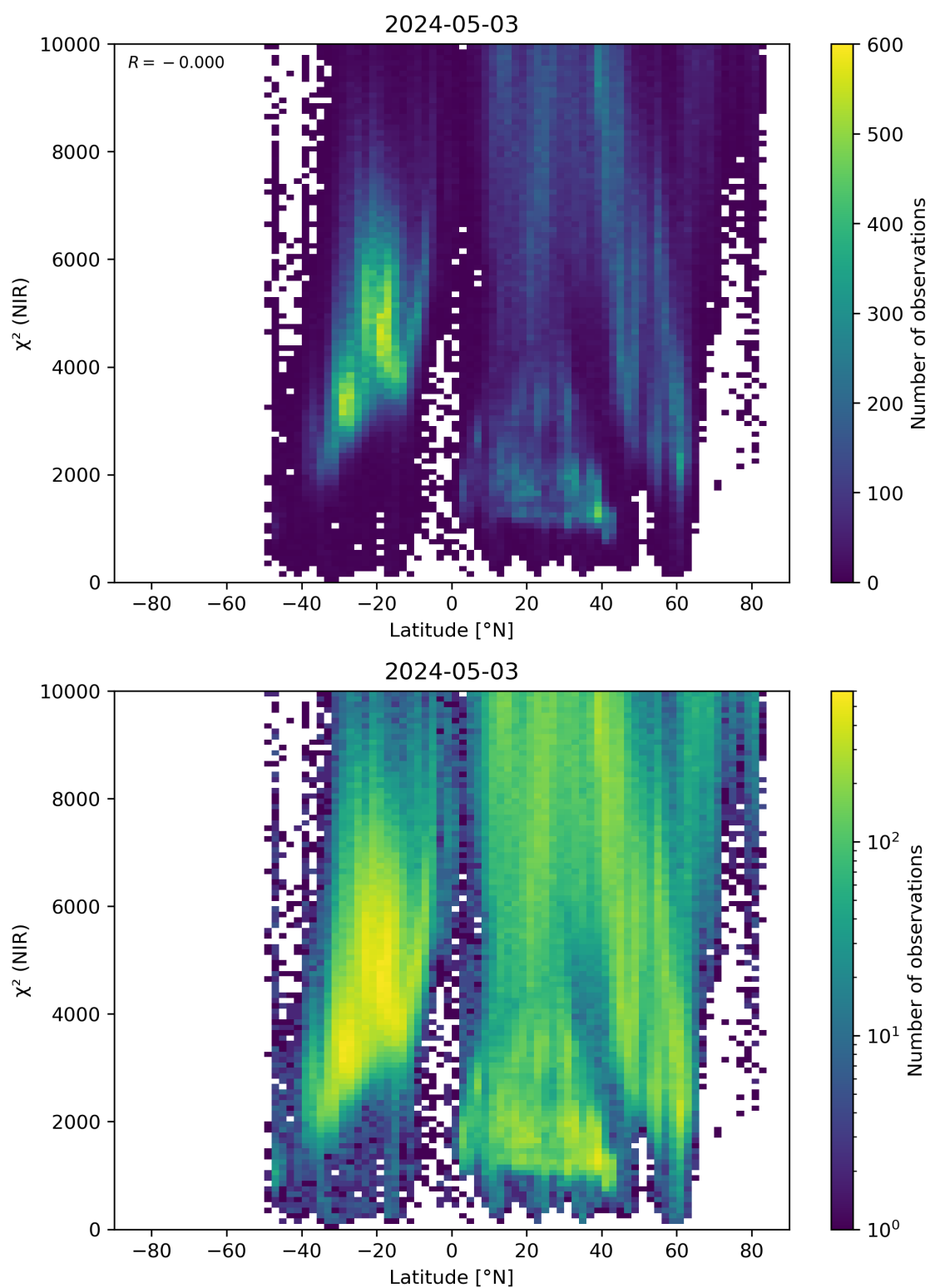
Figure 53: Scatter density plot of “Latitude” against “ \chi^2 (NIR)” for 2024-05-02 to 2024-05-04.
