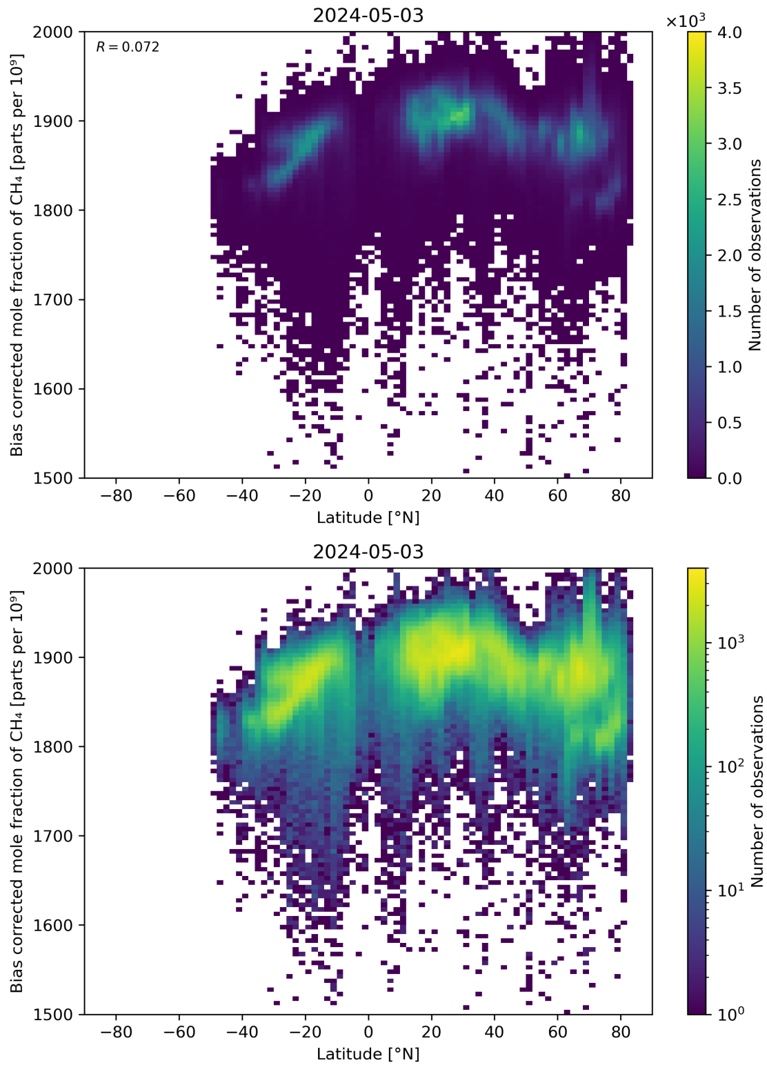
Figure 58: Scatter density plot of “Latitude” against “Bias corrected mole fraction of CH 4 ” for 2024-05-02 to 2024-05-04.
