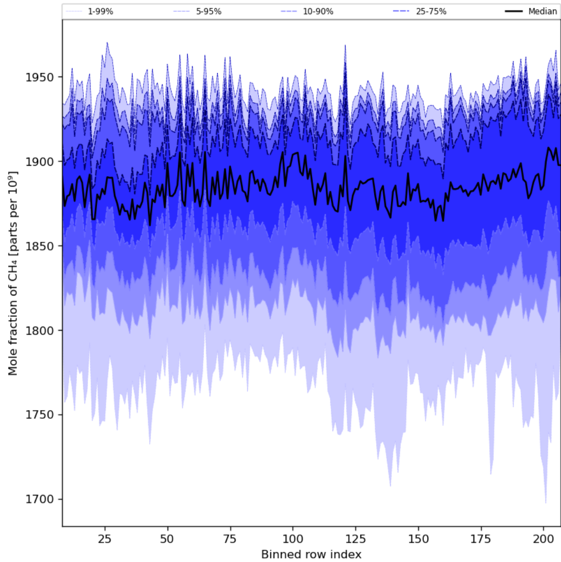
Figure 34: Along track statistics of “Mole fraction of CH 4 ” for 2024-05-02 to 2024-05-04
