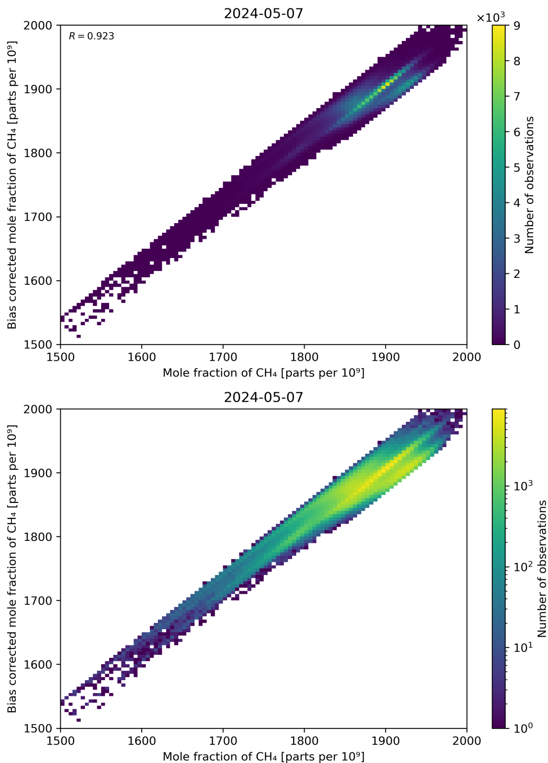
Figure 74: Scatter density plot of “Mole fraction of CH 4 ” against “Bias corrected mole fraction of CH 4 ” for 2024-05-07 to 2024-05-08.
