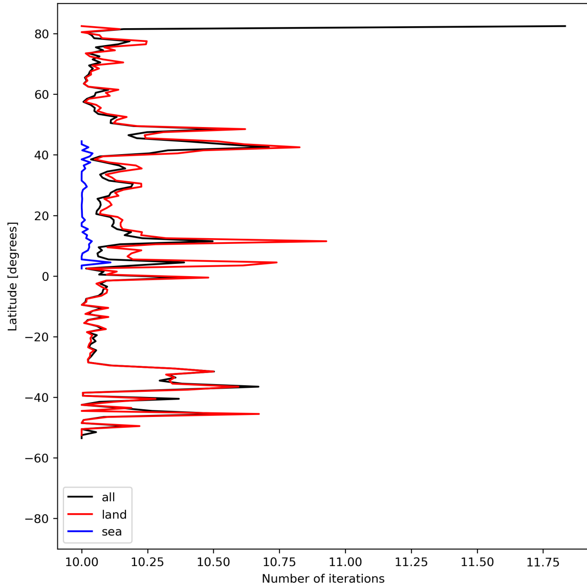
Figure 20: Zonal average of “Number of iterations” for 2024-05-07 to 2024-05-08.
