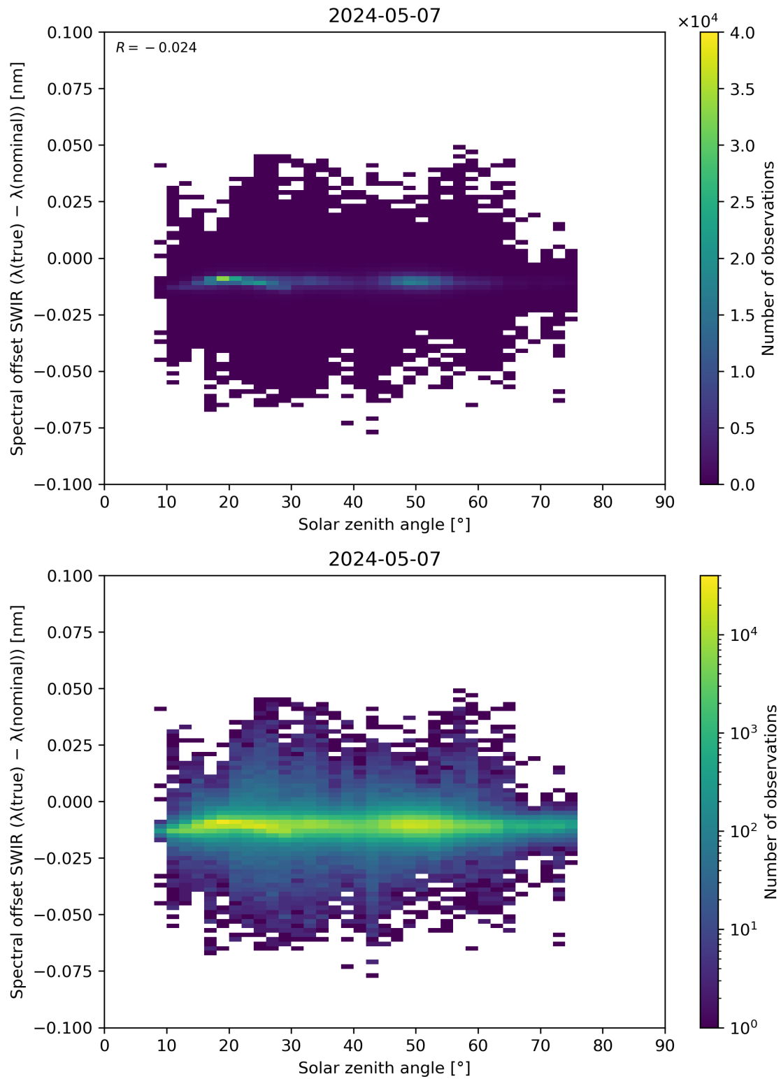
Figure 104: Scatter density plot of “Solar zenith angle” against “Spectral offset SWIR ( \lambda(\text{true}) - \lambda(\text{nominal}) )” for 2024-05-07 to 2024-05-08.
