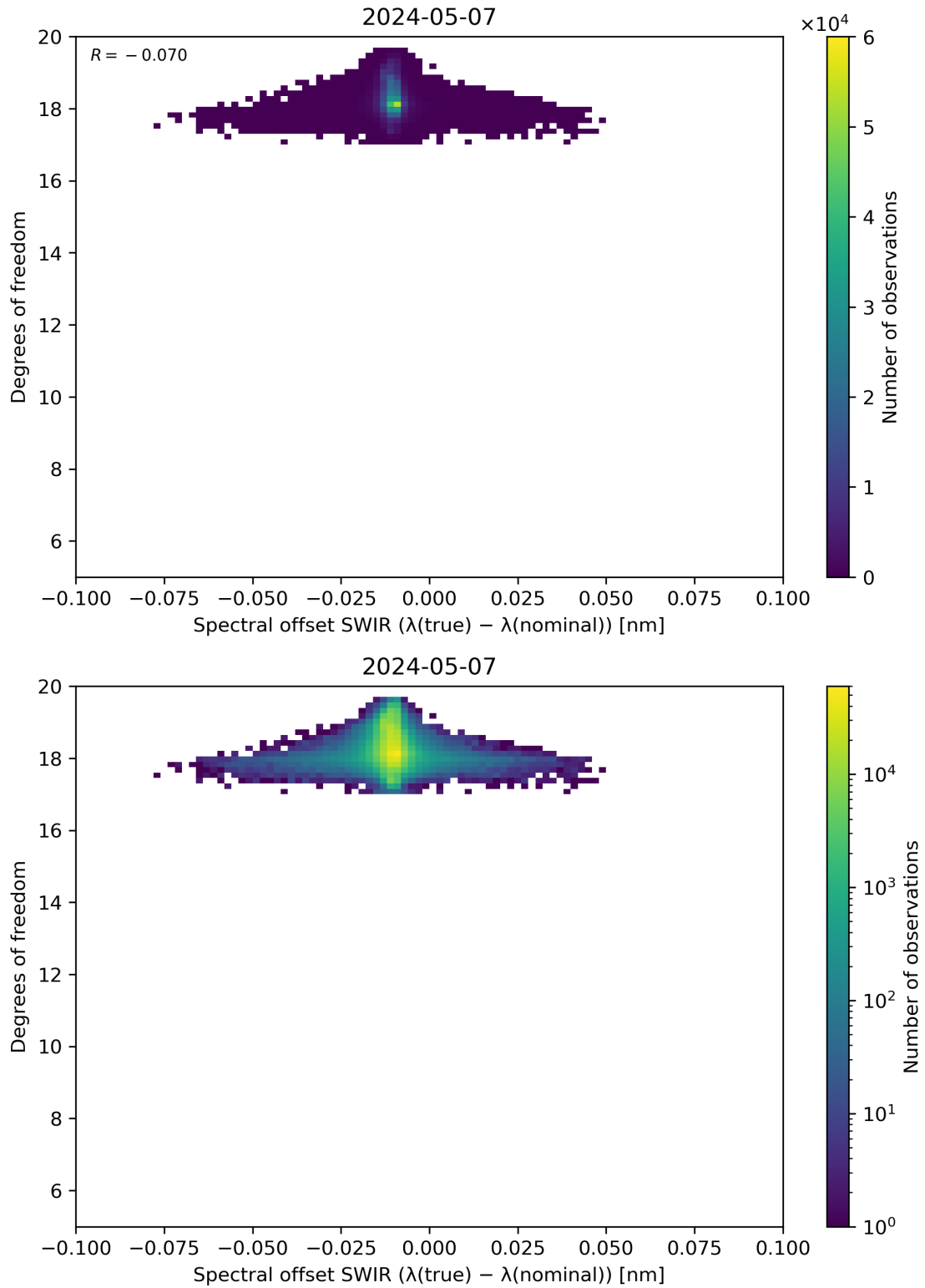
Figure 119: Scatter density plot of “Spectral offset SWIR ( \lambda(\text{true}) - \lambda(\text{nominal}) )” against “Degrees of freedom” for 2024-05-07 to 2024-05-08.
