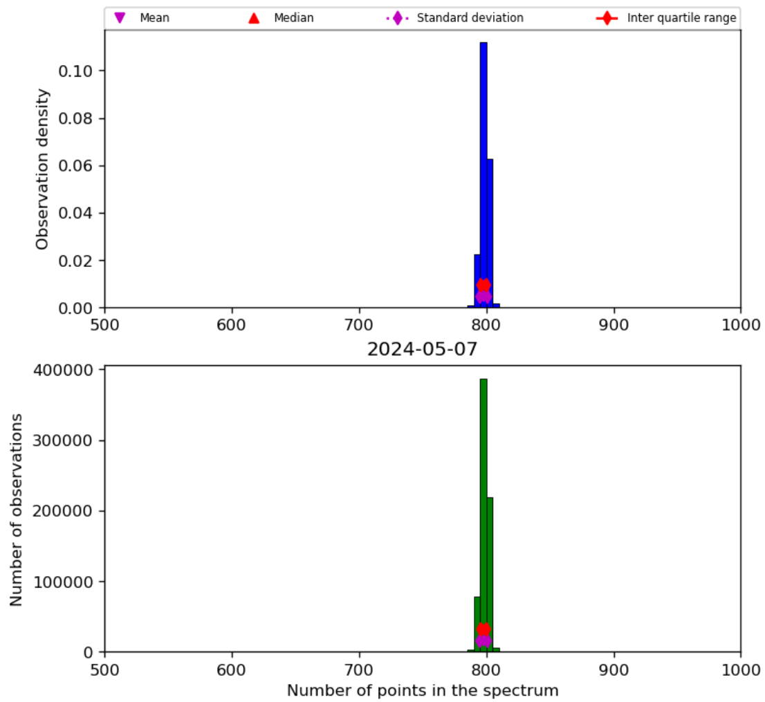
Figure 26: Histogram of “Number of points in the spectrum” for 2024-05-07 to 2024-05-08
