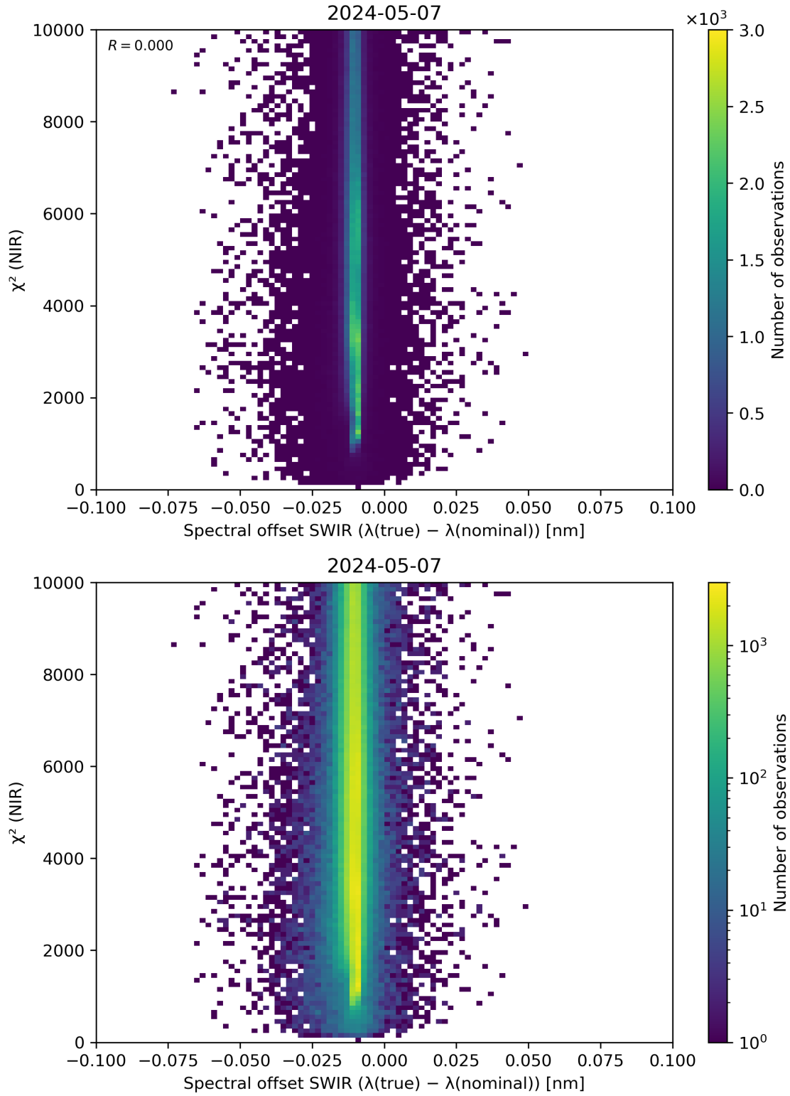
Figure 117: Scatter density plot of “Spectral offset SWIR ( \lambda(\text{true}) - \lambda(\text{nominal}) )” against “ \chi^2 (NIR)” for 2024-05-07 to 2024-05-08.
