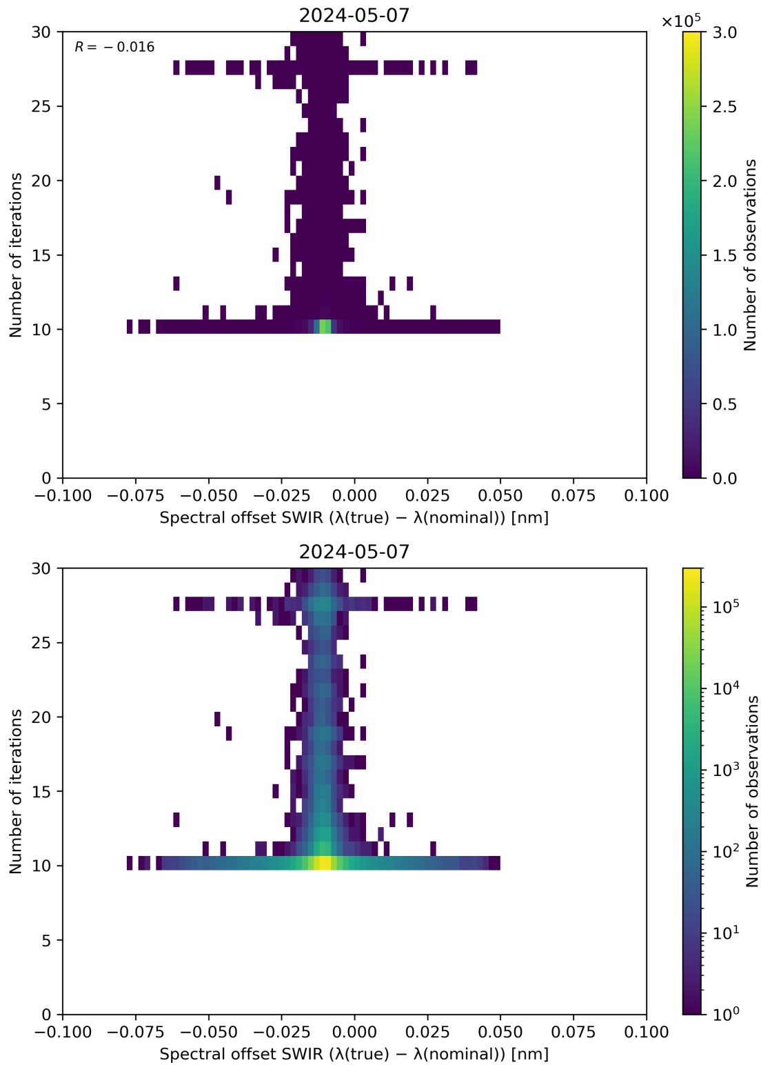
Figure 121: Scatter density plot of “Spectral offset SWIR ( \lambda(\text{true}) - \lambda(\text{nominal}) )” against “Number of iterations” for 2024-05-07 to 2024-05-08.
