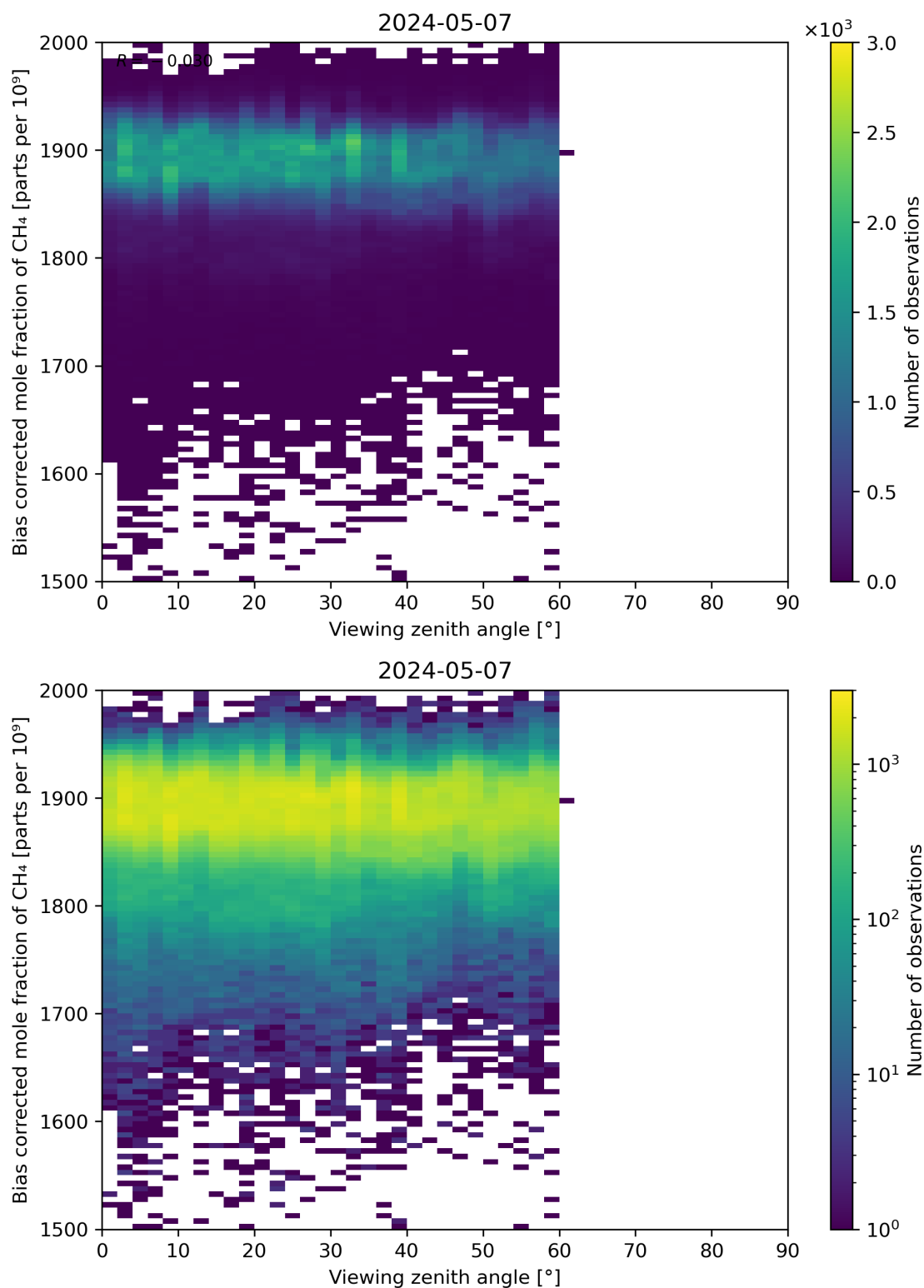
Figure 111: Scatter density plot of “Viewing zenith angle” against “Bias corrected mole fraction of CH 4 ” for 2024-05-07 to 2024-05-08.
