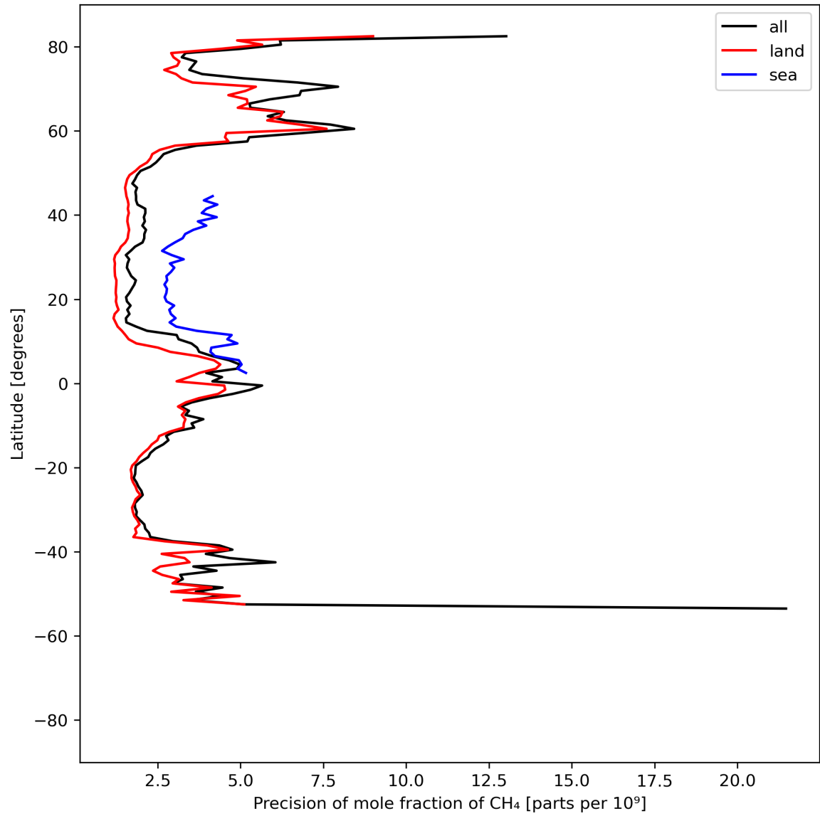
Figure 13: Zonal average of “Precision of mole fraction of CH 4 ” for 2024-05-07 to 2024-05-08.
