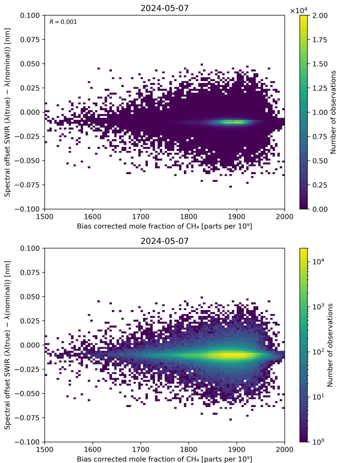
Figure 69: Scatter density plot of “Bias corrected mole fraction of \text{CH}_4 ” against “Spectral offset SWIR ( \lambda(\text{true}) - \lambda(\text{nominal}) )” for 2024-05-07 to 2024-05-08.
