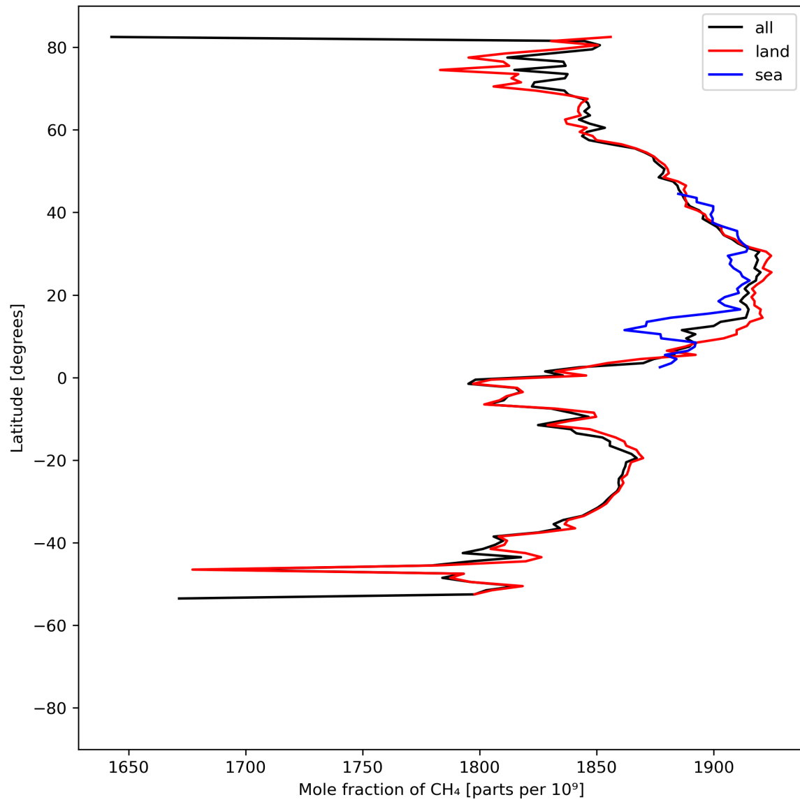
Figure 12: Zonal average of “Mole fraction of \text{CH}_4 ” for 2024-05-07 to 2024-05-08.
