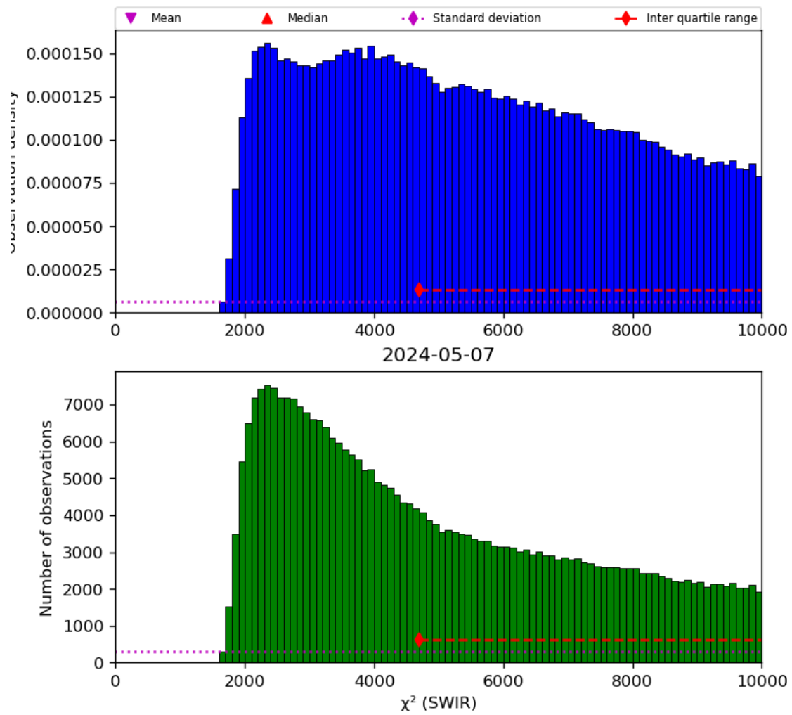
Figure 28: Histogram of “ \chi^2 (SWIR)” for 2024-05-07 to 2024-05-08
