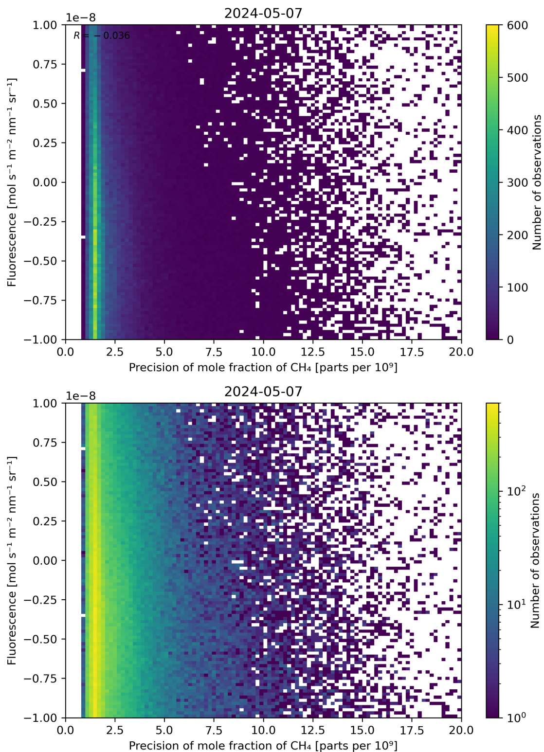
Figure 81: Scatter density plot of “Precision of mole fraction of \text{CH}_4 ” against “Fluorescence” for 2024-05-07 to 2024-05-08.
