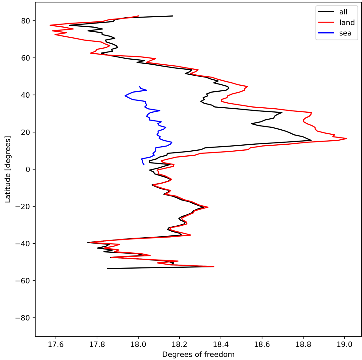
Figure 19: Zonal average of “Degrees of freedom” for 2024-05-07 to 2024-05-08.
