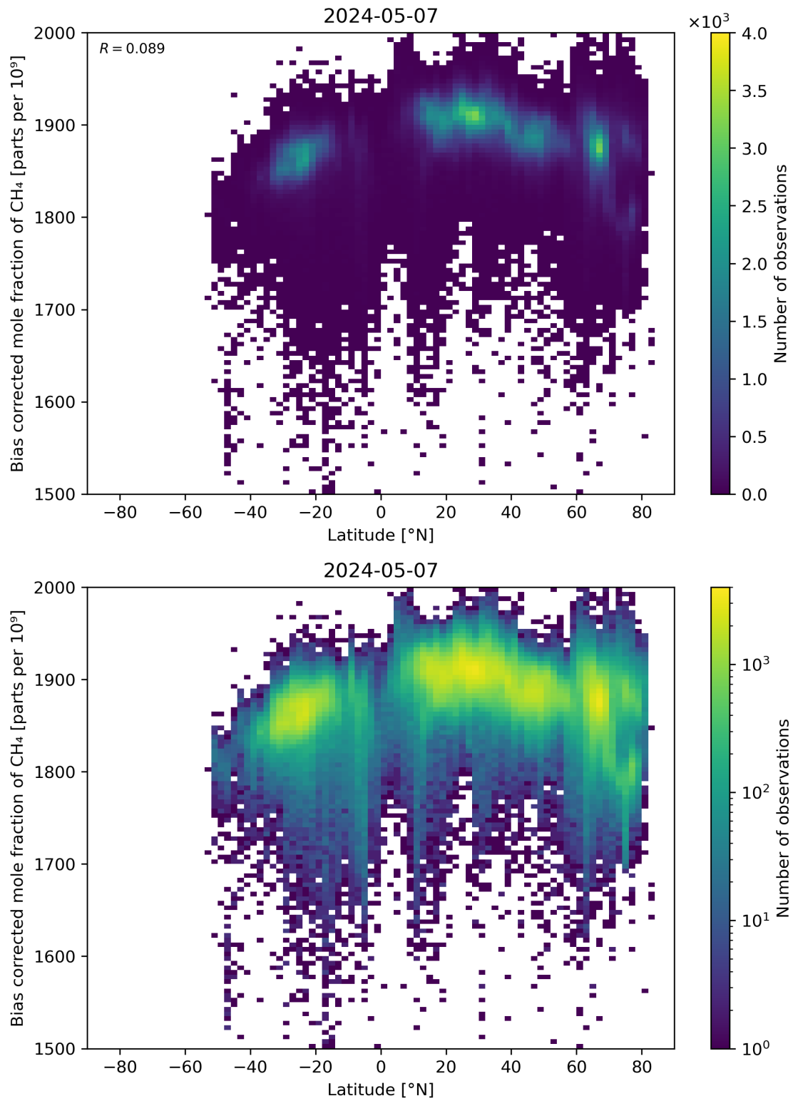
Figure 58: Scatter density plot of “Latitude” against “Bias corrected mole fraction of CH 4 ” for 2024-05-07 to 2024-05-08.
