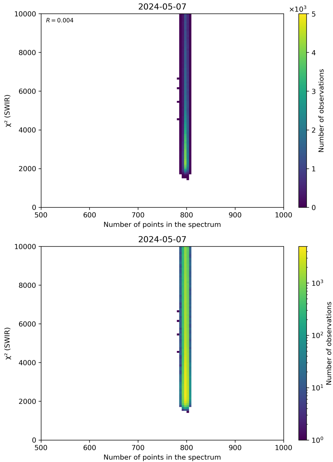
Figure 89: Scatter density plot of “Number of points in the spectrum” against “ \chi^2 (SWIR)” for 2024-05-07 to 2024-05-08.
