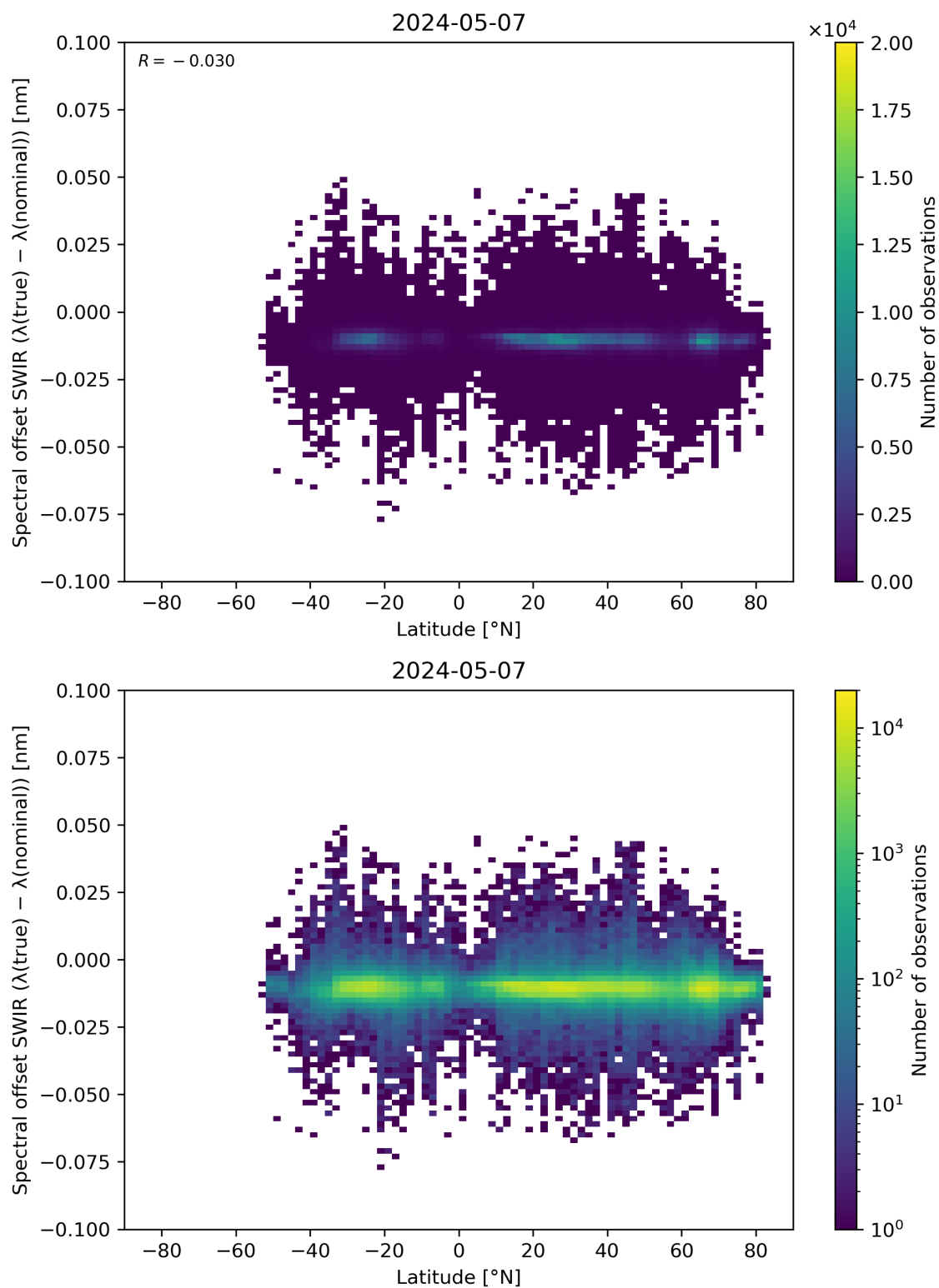
Figure 62: Scatter density plot of “Latitude” against “Spectral offset SWIR ( \lambda(\text{true}) - \lambda(\text{nominal}) )” for 2024-05-07 to 2024-05-08.
