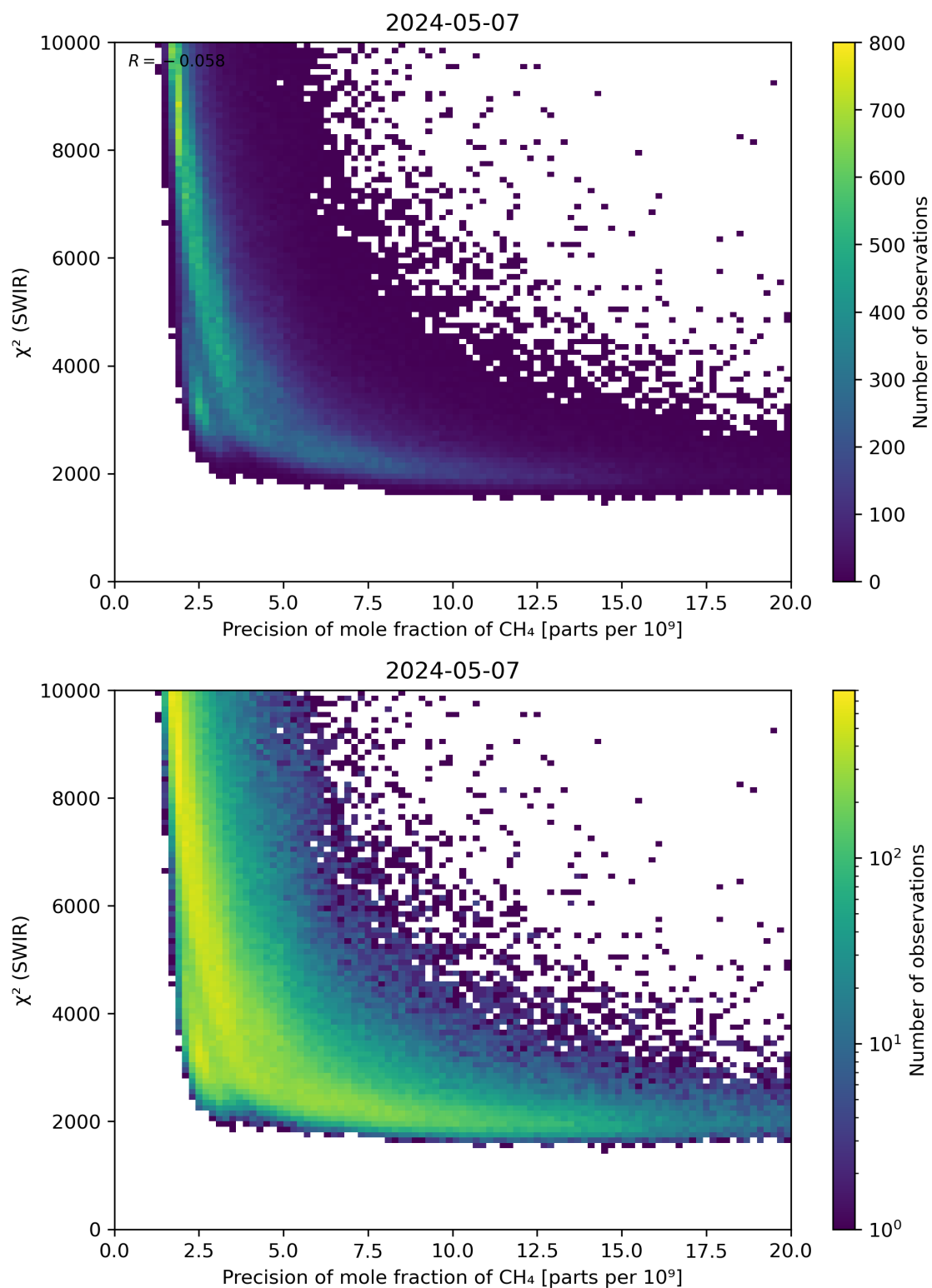
Figure 79: Scatter density plot of “Precision of mole fraction of \text{CH}_4 ” against “ \chi^2 (SWIR)” for 2024-05-07 to 2024-05-08.
