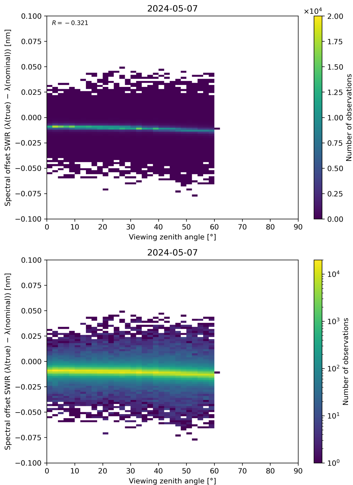
Figure 116: Scatter density plot of “Viewing zenith angle” against “Spectral offset SWIR ( \lambda(\text{true}) - \lambda(\text{nominal}) )” for 2024-05-07 to 2024-05-08.
