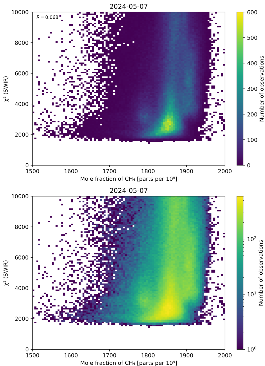
Figure 71: Scatter density plot of “Mole fraction of CH 4 ” against “ \chi^2 (SWIR)” for 2024-05-07 to 2024-05-08.
