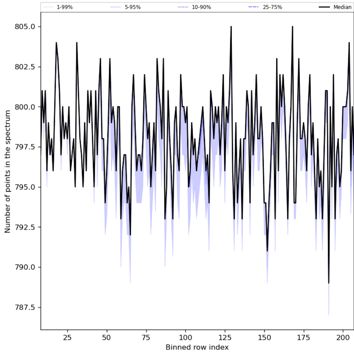
Figure 37: Along track statistics of “Number of points in the spectrum” for 2024-05-07 to 2024-05-08
