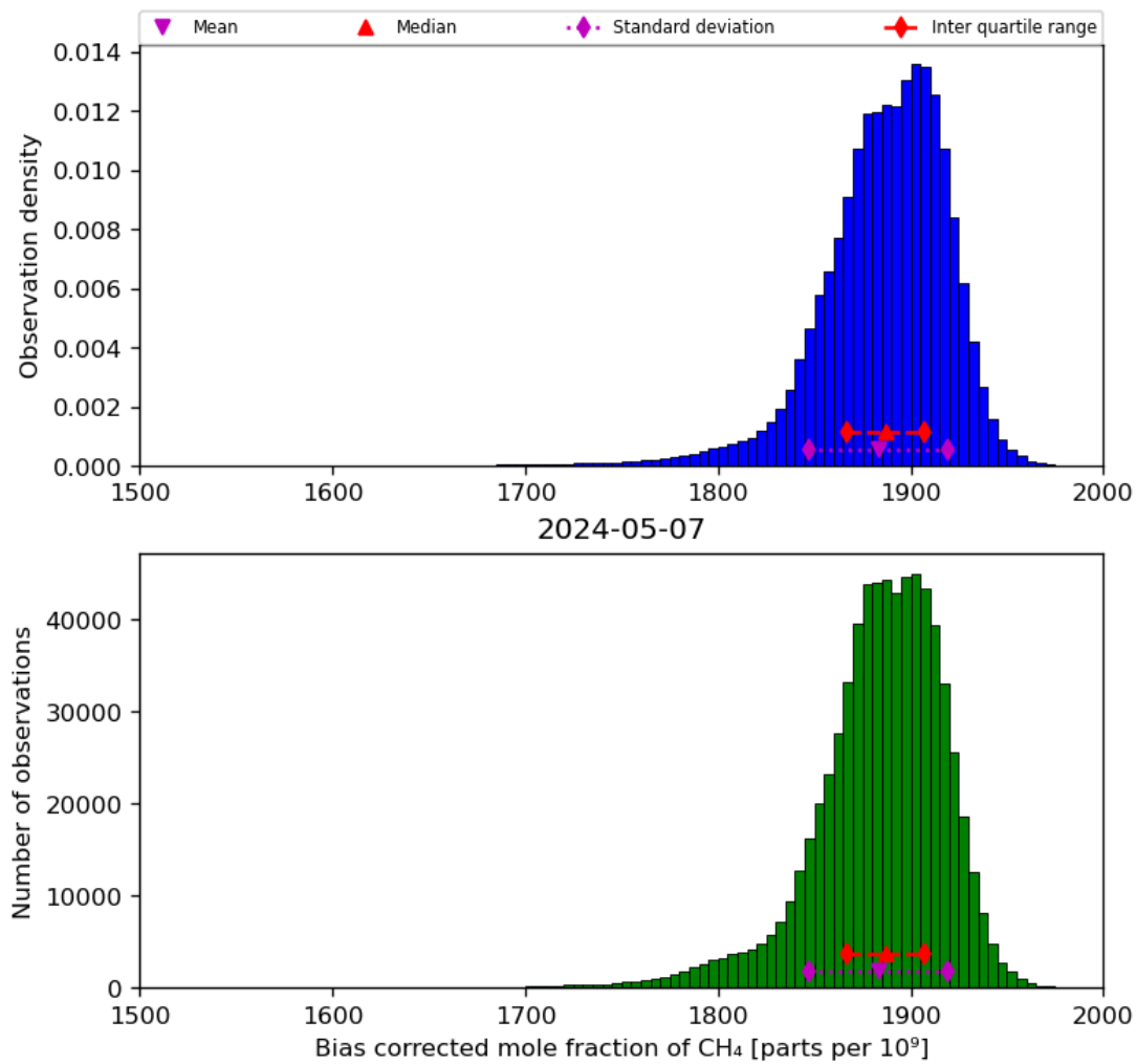
Figure 25: Histogram of “Bias corrected mole fraction of CH 4 ” for 2024-05-07 to 2024-05-08
