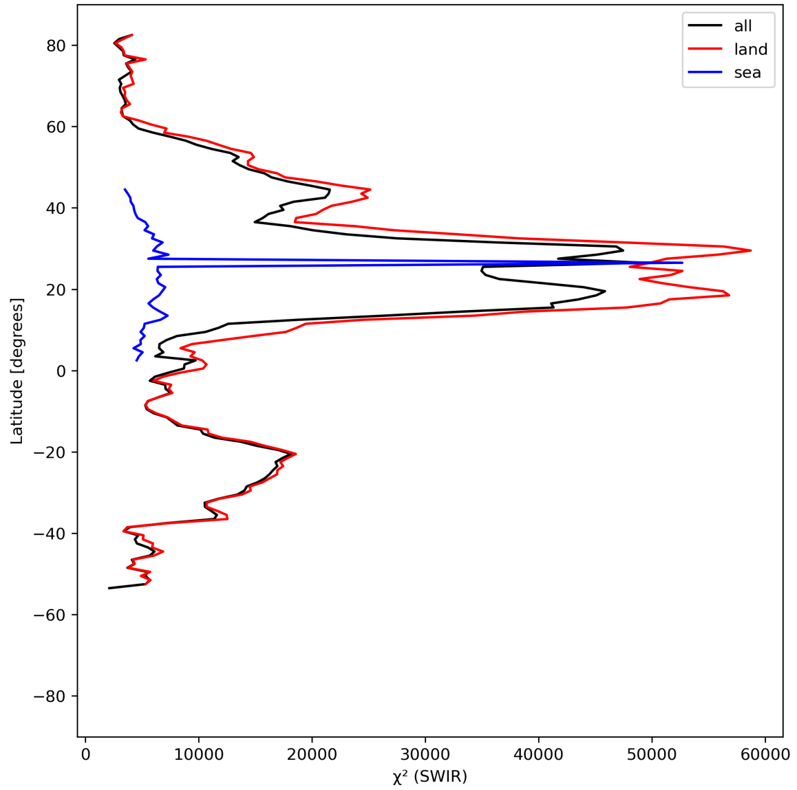
Figure 17: Zonal average of “ \chi^2 (SWIR)” for 2024-05-07 to 2024-05-08.
