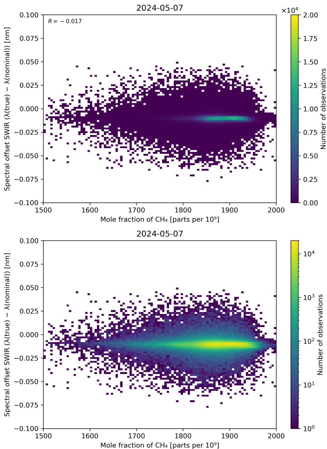
Figure 86: Scatter density plot of “Mole fraction of CH 4 ” against “Spectral offset SWIR ( \lambda(\text{true}) - \lambda(\text{nominal}) )” for 2024-05-07 to 2024-05-08.
