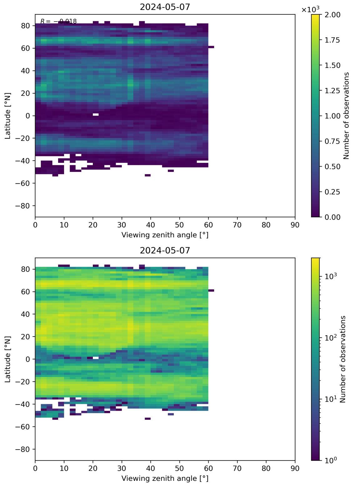
Figure 109: Scatter density plot of “Viewing zenith angle” against “Latitude” for 2024-05-07 to 2024-05-08.
