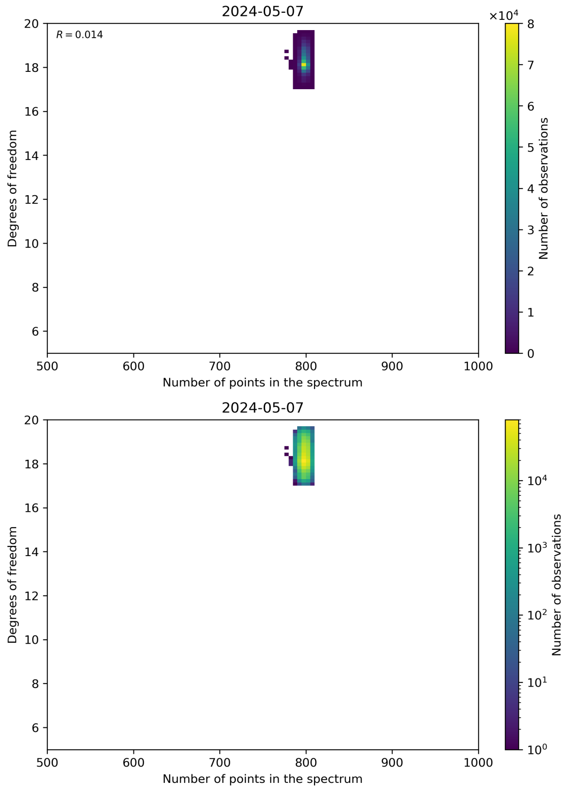
Figure 90: Scatter density plot of “Number of points in the spectrum” against “Degrees of freedom” for 2024-05-07 to 2024-05-08.
