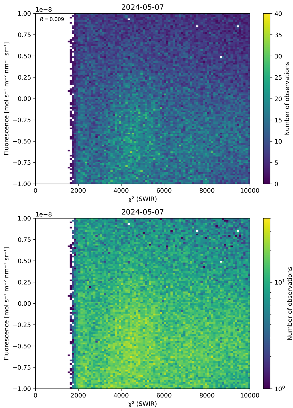
Figure 49: Scatter density plot of “ \chi^2 (SWIR)” against “Fluorescence” for 2024-05-07 to 2024-05-08.
