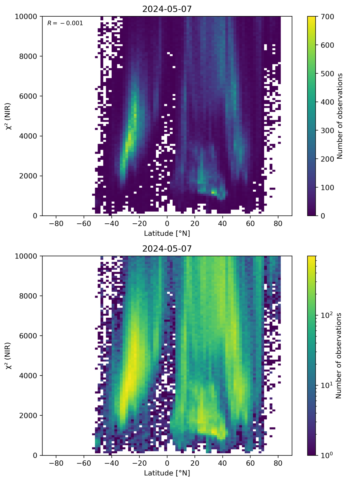
Figure 53: Scatter density plot of “Latitude” against “ \chi^2 (NIR)” for 2024-05-07 to 2024-05-08.
