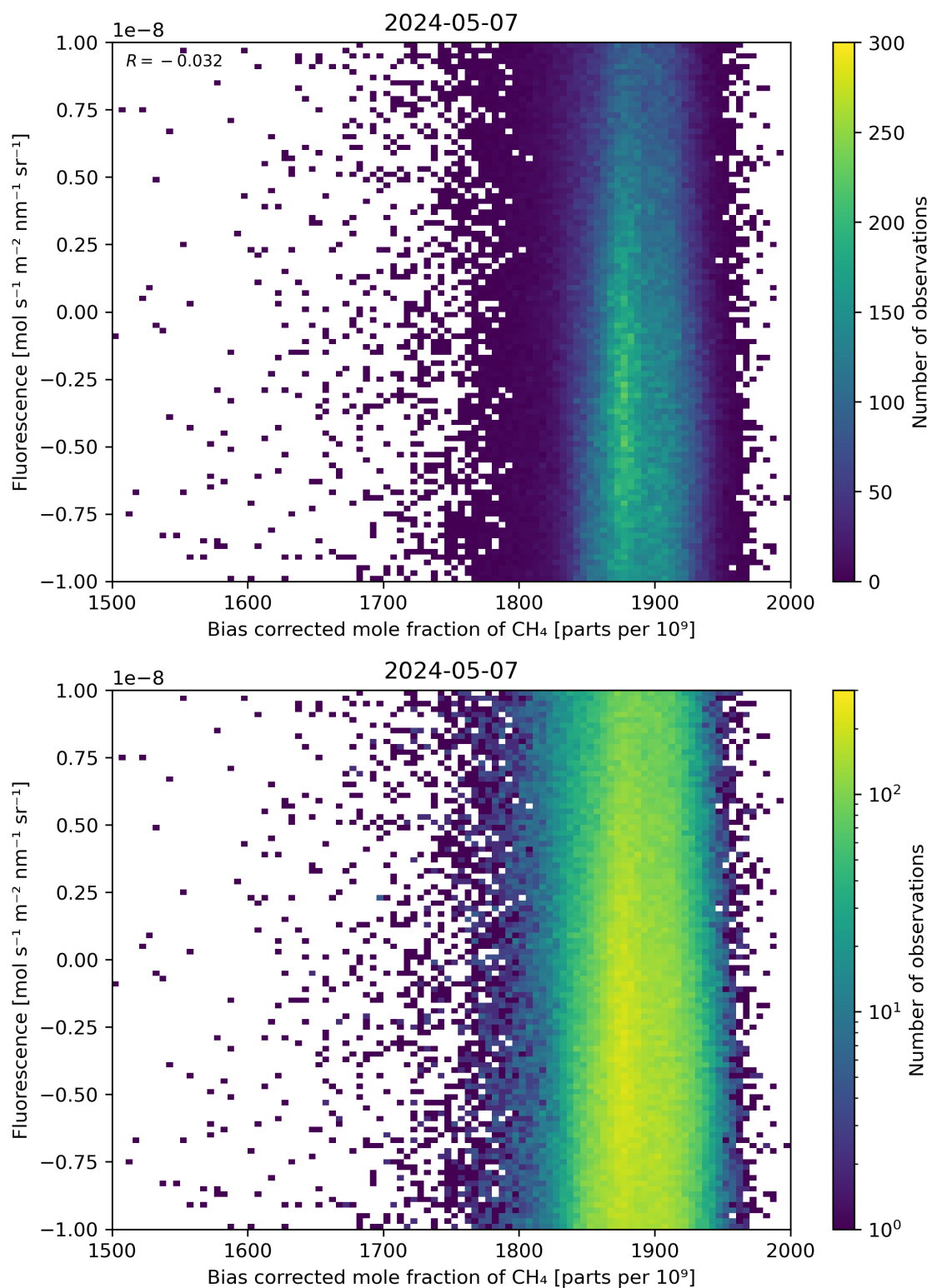
Figure 66: Scatter density plot of “Bias corrected mole fraction of \text{CH}_4 ” against “Fluorescence” for 2024-05-07 to 2024-05-08.
