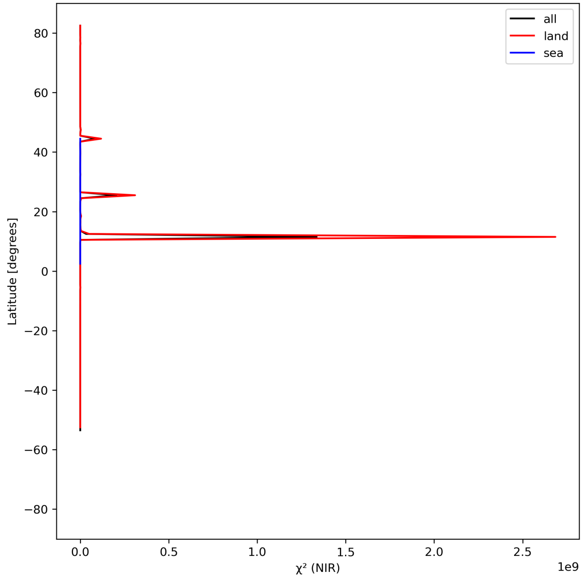
Figure 18: Zonal average of “ \chi^2 (NIR)” for 2024-05-07 to 2024-05-08.
