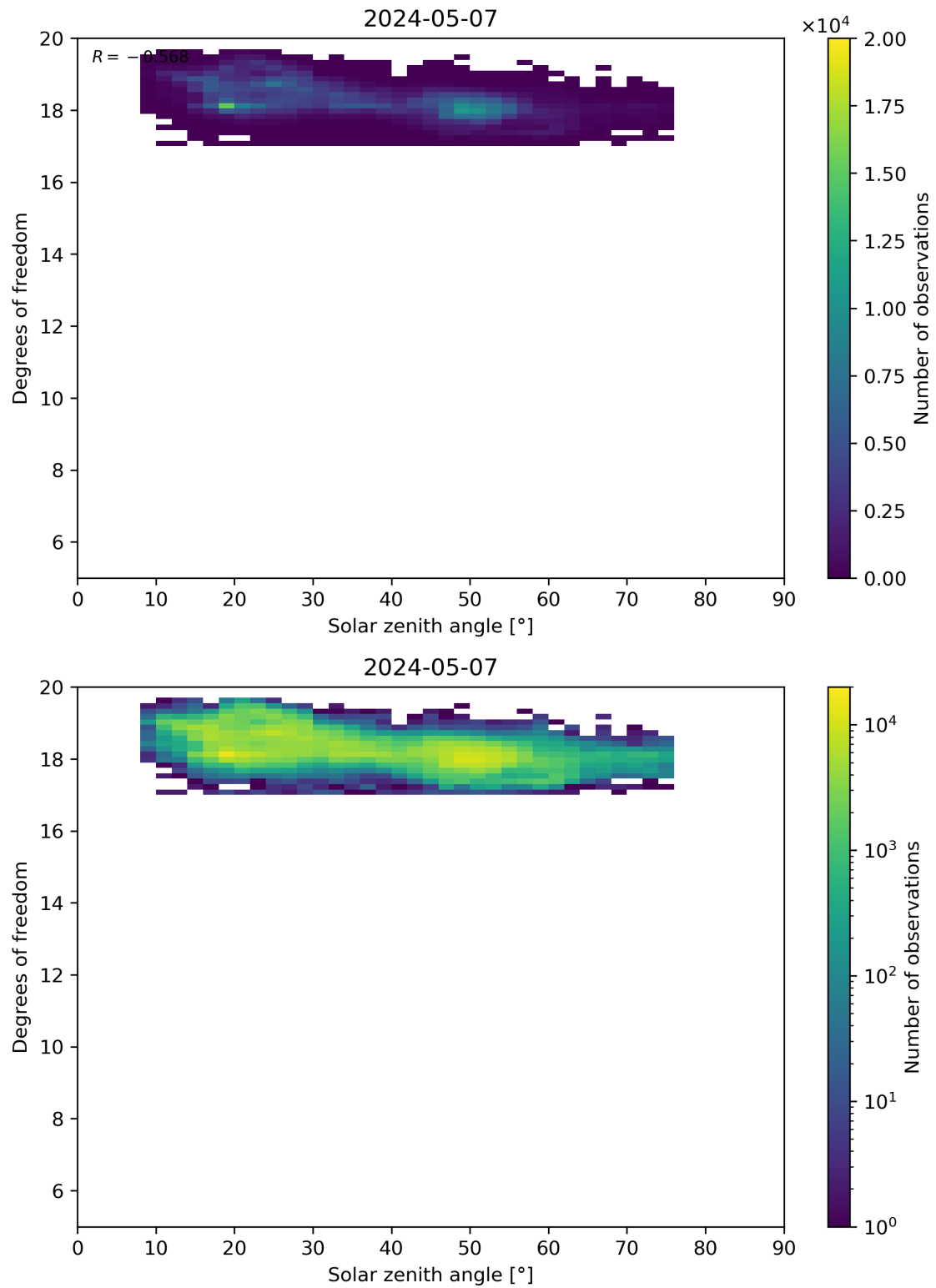
Figure 96: Scatter density plot of “Solar zenith angle” against “Degrees of freedom” for 2024-05-07 to 2024-05-08.
