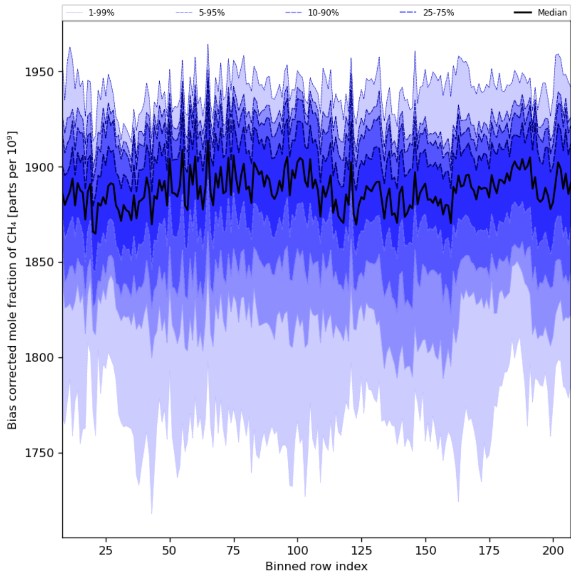
Figure 36: Along track statistics of “Bias corrected mole fraction of CH 4 ” for 2024-05-07 to 2024-05-08
