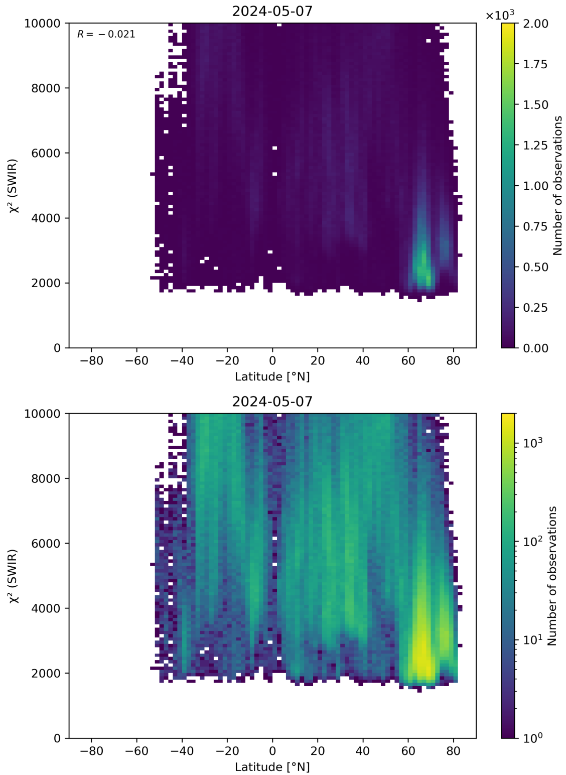
Figure 54: Scatter density plot of “Latitude” against “ \chi^2 (SWIR)” for 2024-05-07 to 2024-05-08.
