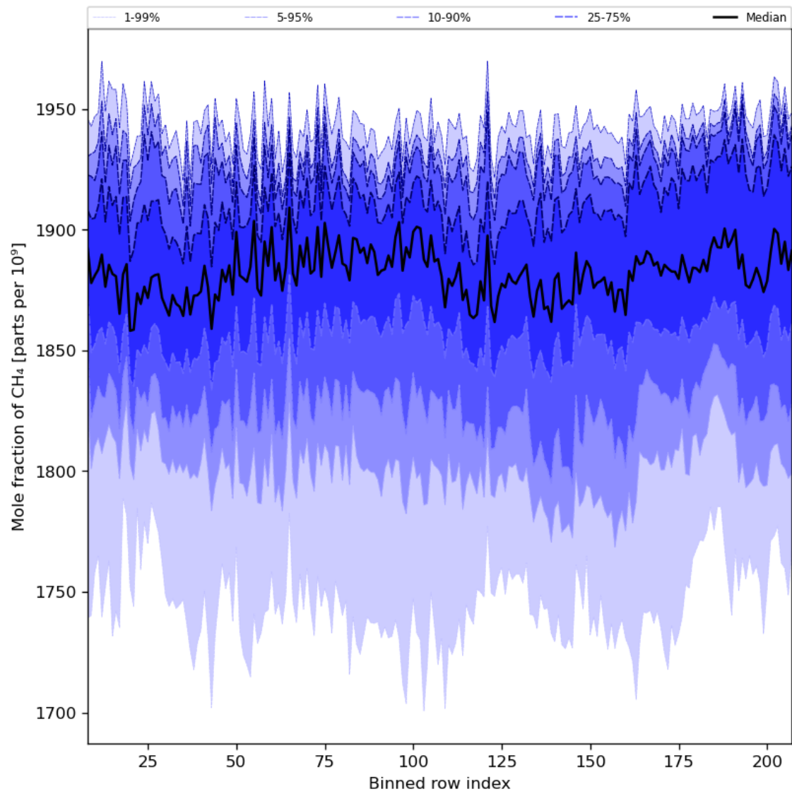
Figure 34: Along track statistics of “Mole fraction of CH 4 ” for 2024-05-07 to 2024-05-08
