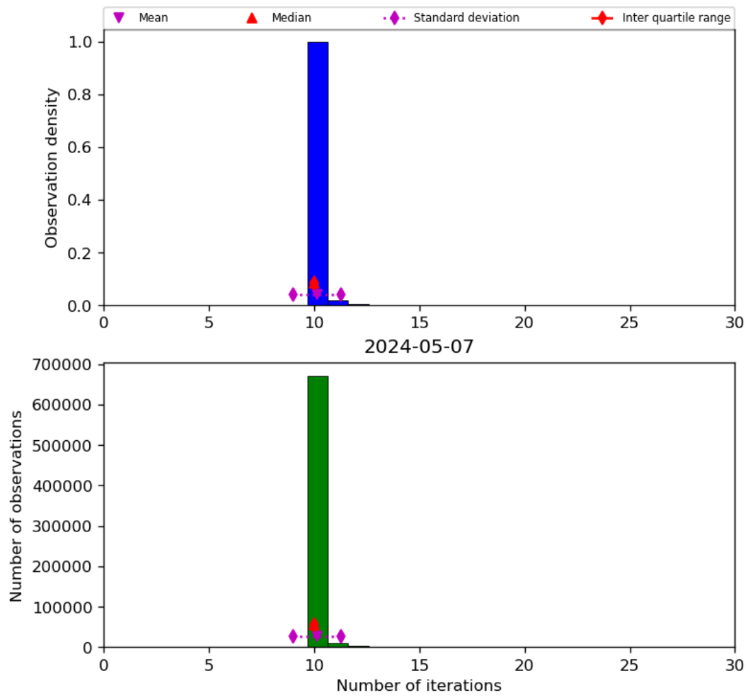
Figure 31: Histogram of “Number of iterations” for 2024-05-07 to 2024-05-08
