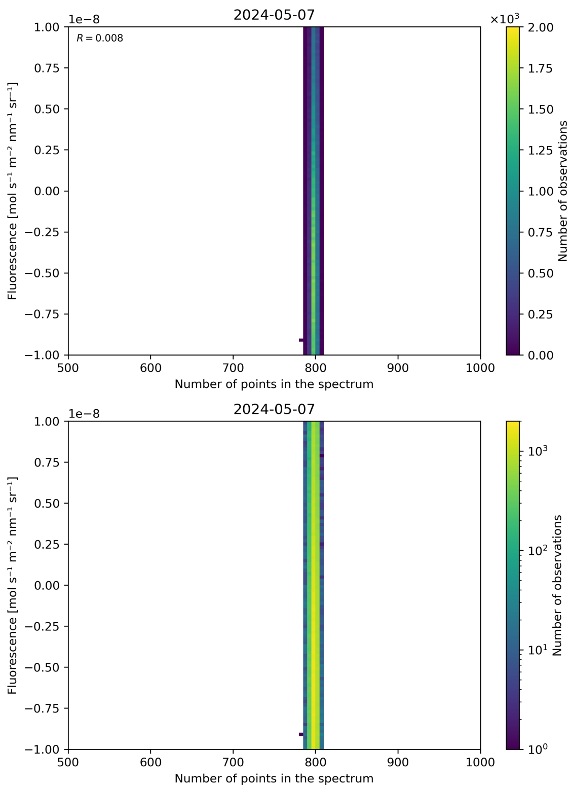
Figure 91: Scatter density plot of “Number of points in the spectrum” against “Fluorescence” for 2024-05-07 to 2024-05-08.
