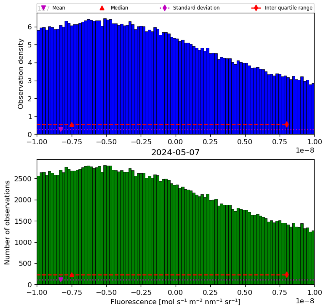
Figure 32: Histogram of “Fluorescence” for 2024-05-07 to 2024-05-08
