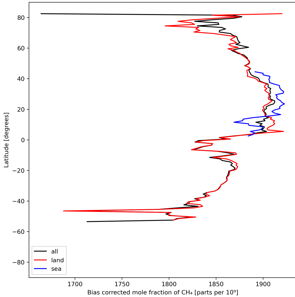
Figure 14: Zonal average of “Bias corrected mole fraction of \text{CH}_4 ” for 2024-05-07 to 2024-05-08.
