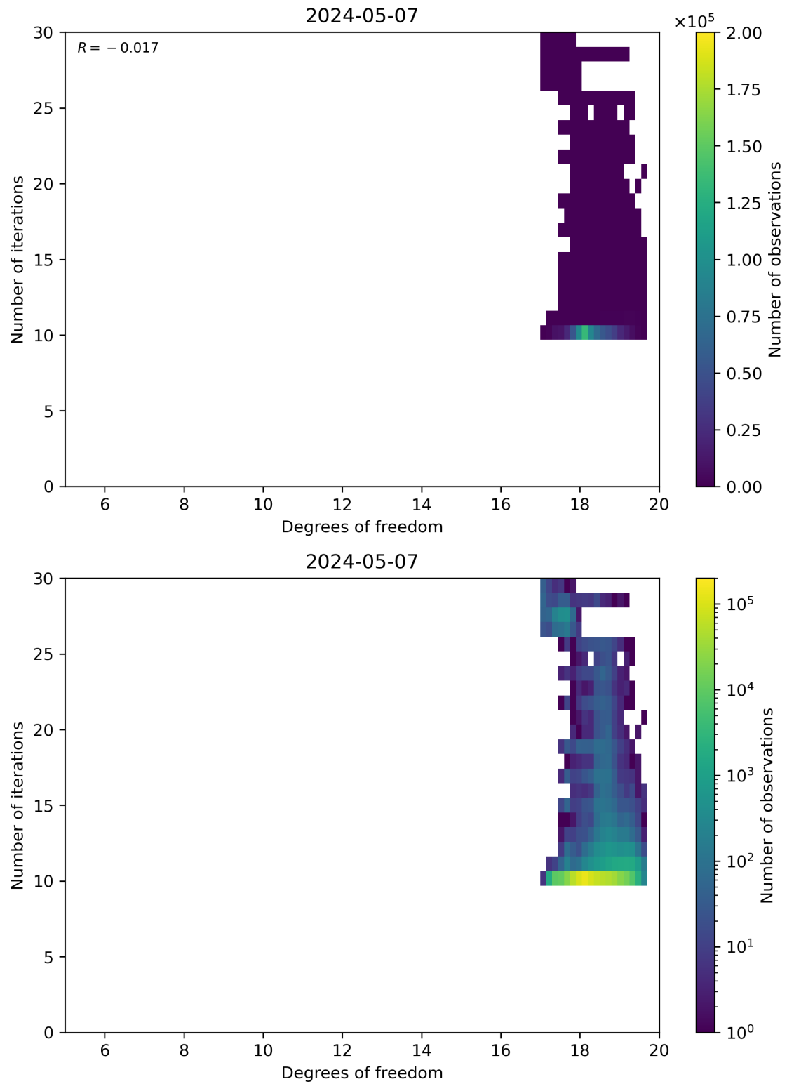
Figure 52: Scatter density plot of “Degrees of freedom” against “Number of iterations” for 2024-05-07 to 2024-05-08.
