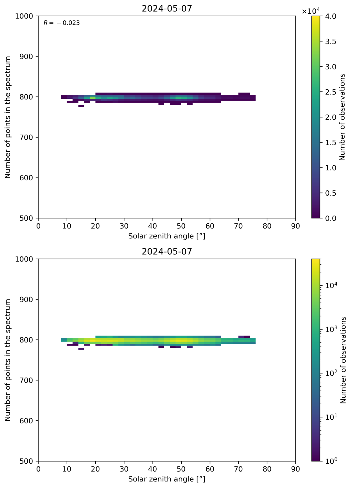
Figure 103: Scatter density plot of “Solar zenith angle” against “Number of points in the spectrum” for 2024-05-07 to 2024-05-08.
