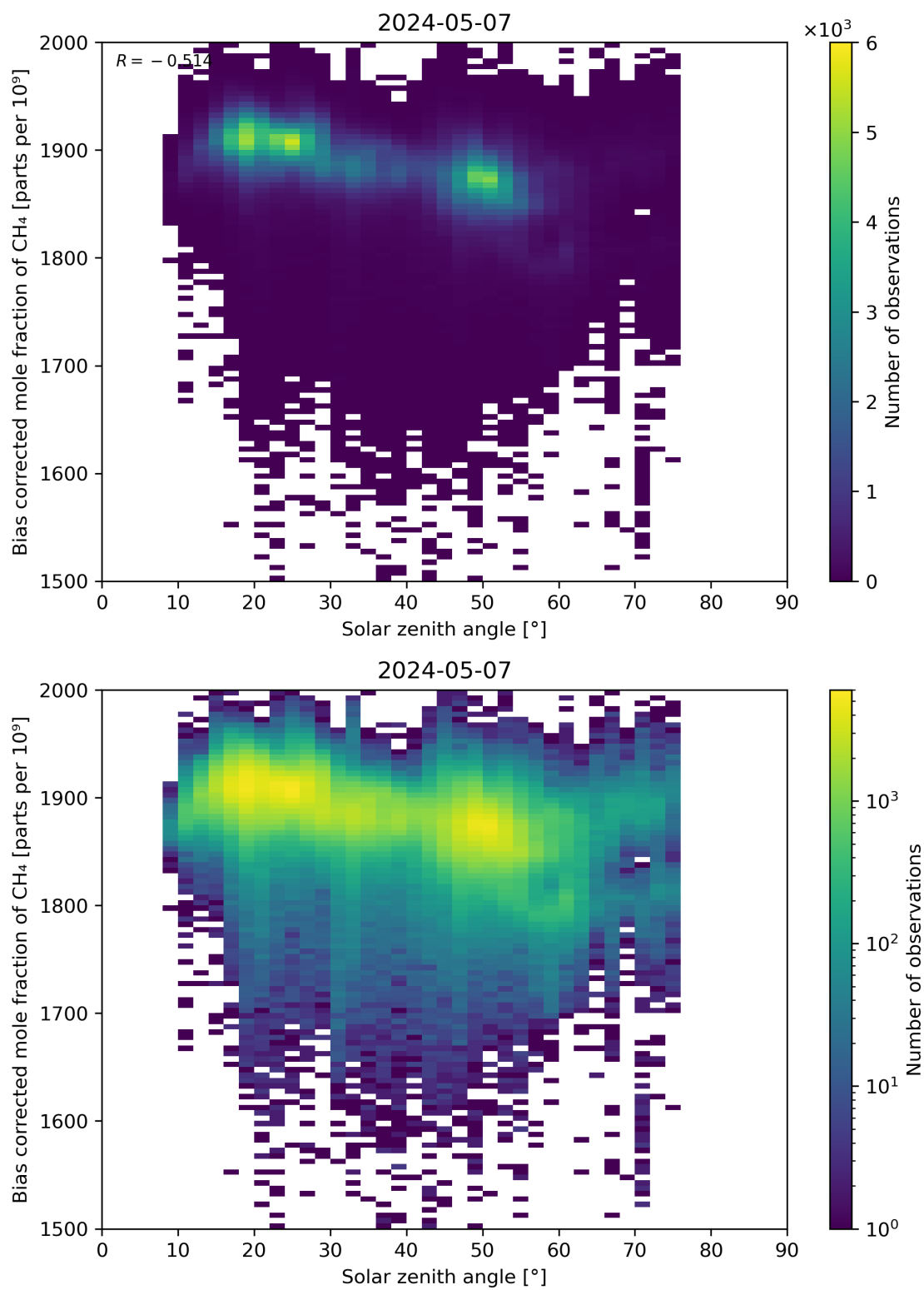
Figure 100: Scatter density plot of “Solar zenith angle” against “Bias corrected mole fraction of CH 4 ” for 2024-05-07 to 2024-05-08.
