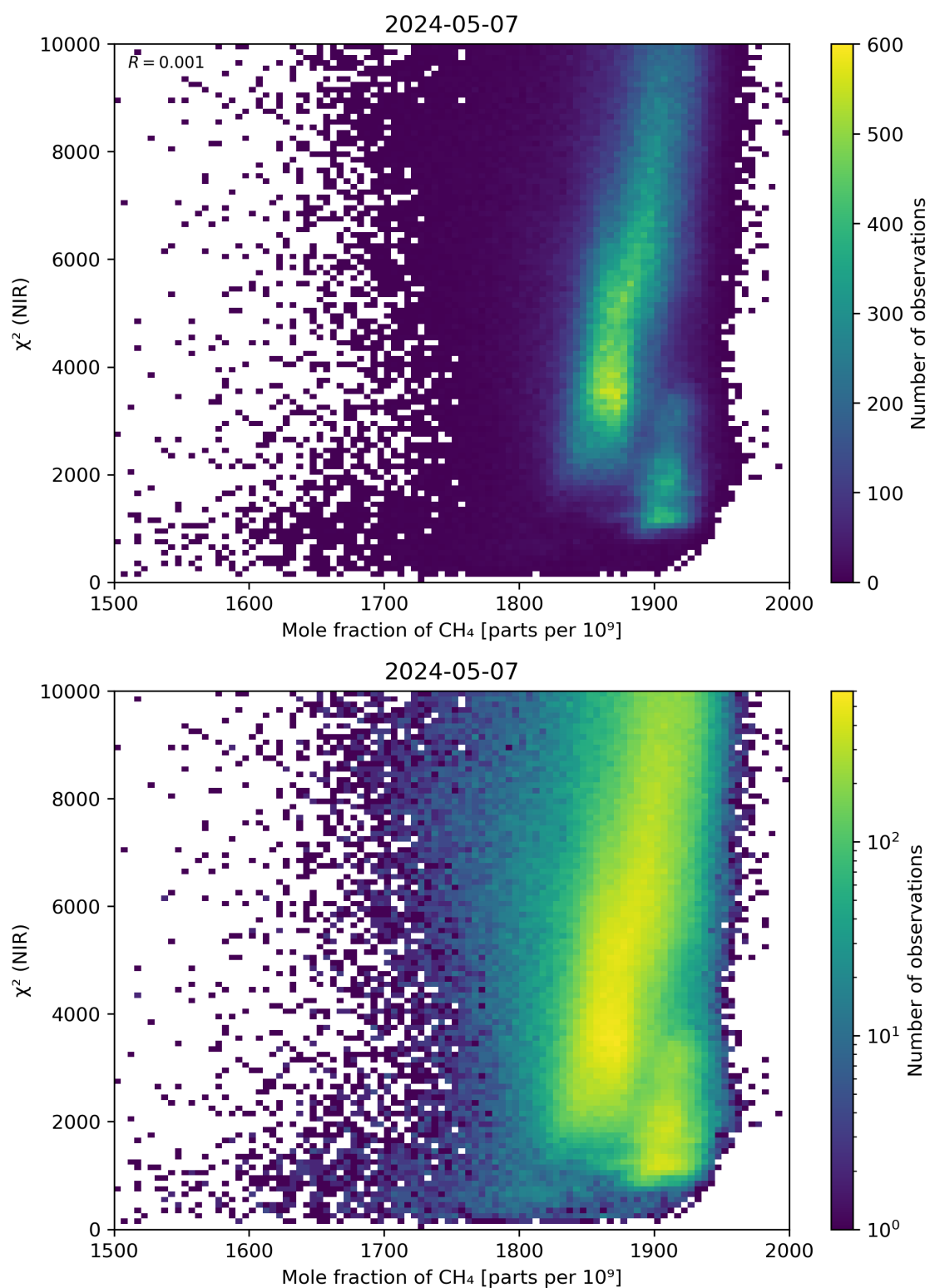
Figure 70: Scatter density plot of “Mole fraction of CH 4 ” against “ \chi^2 (NIR)” for 2024-05-07 to 2024-05-08.
