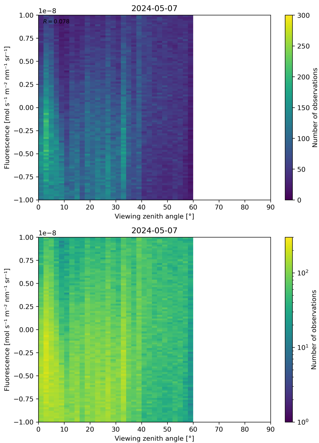
Figure 108: Scatter density plot of “Viewing zenith angle” against “Fluorescence” for 2024-05-07 to 2024-05-08.
