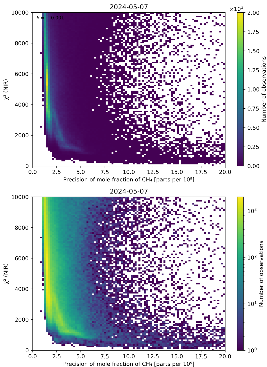
Figure 78: Scatter density plot of “Precision of mole fraction of CH 4 ” against “ \chi^2 (NIR)” for 2024-05-07 to 2024-05-08.
