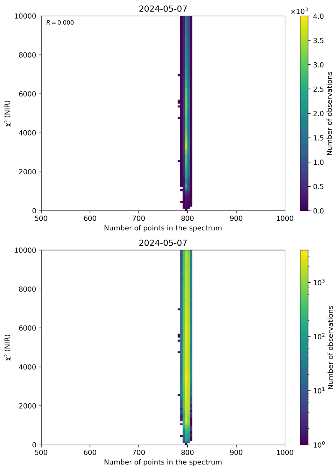
Figure 88: Scatter density plot of “Number of points in the spectrum” against “ \chi^2 (NIR)” for 2024-05-07 to 2024-05-08.
