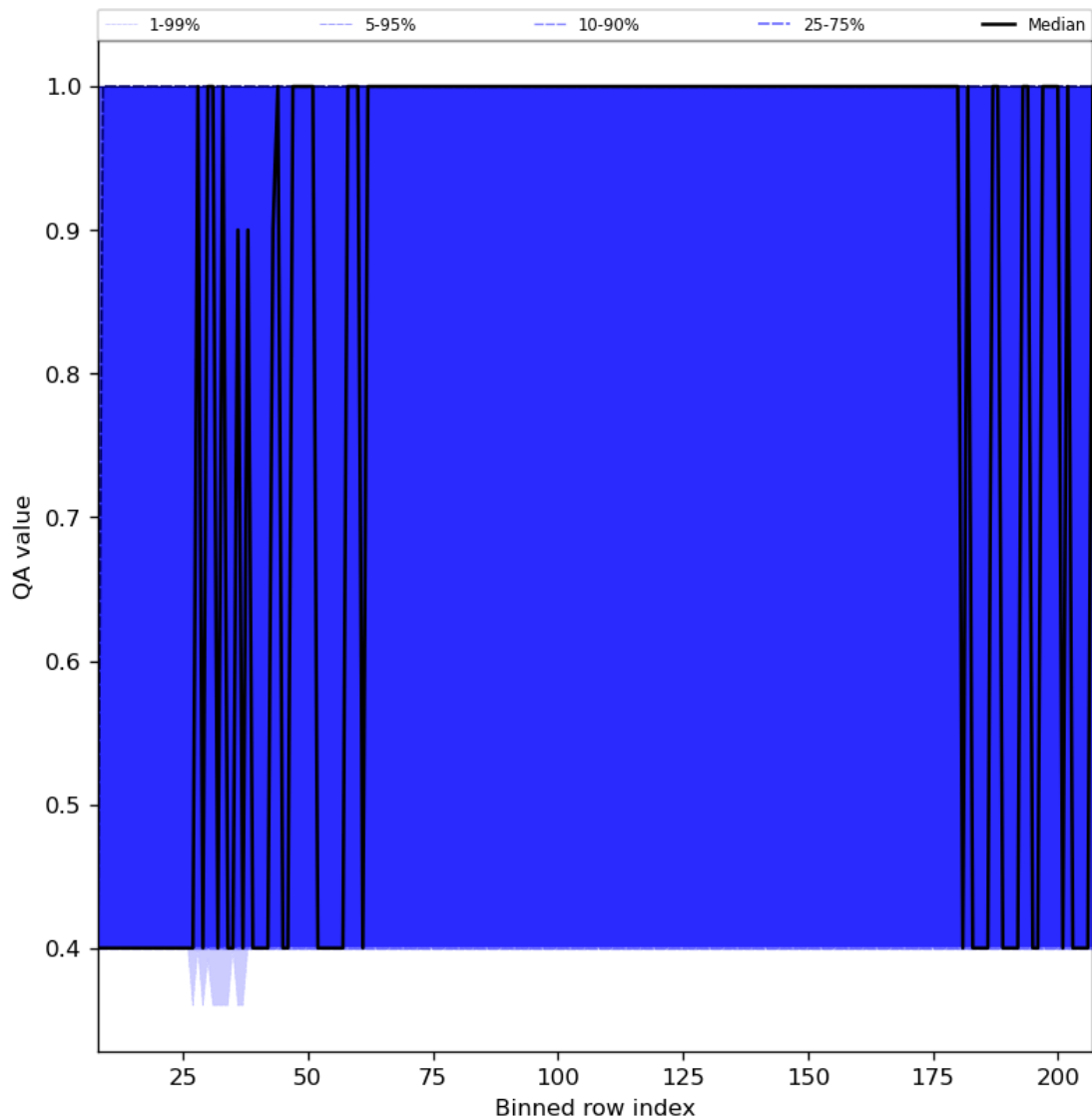
Figure 33: Along track statistics of “QA value” for 2024-05-07 to 2024-05-08
