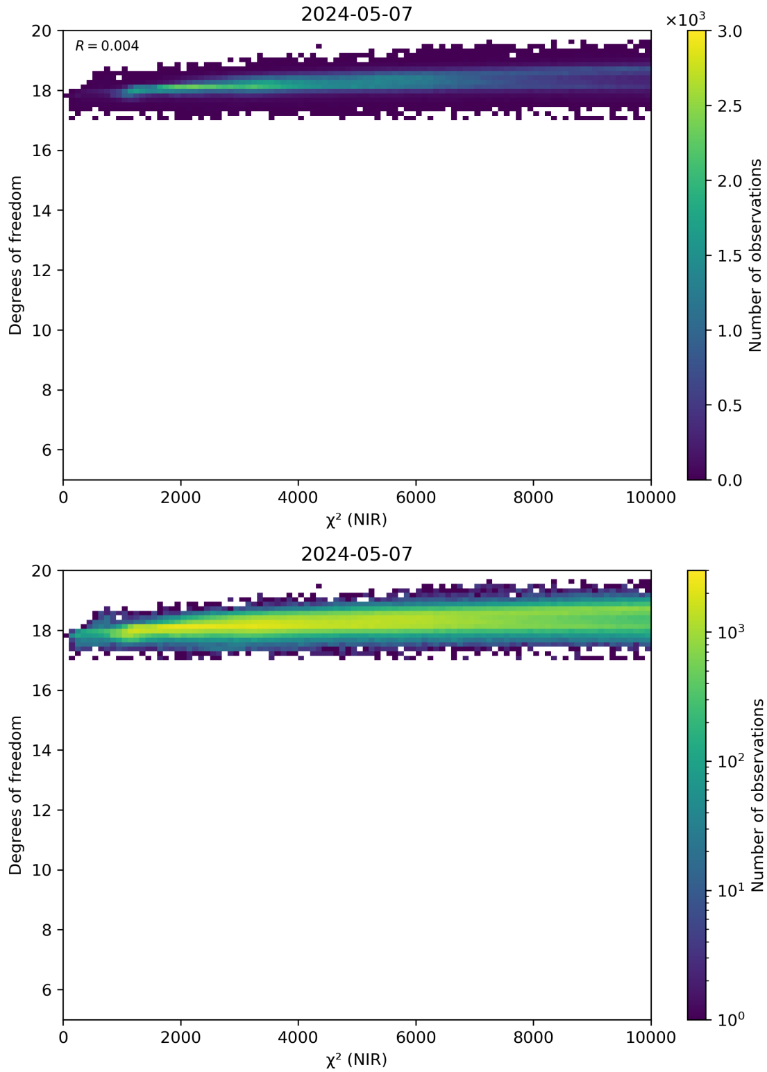
Figure 44: Scatter density plot of “ \chi^2 (NIR)” against “Degrees of freedom” for 2024-05-07 to 2024-05-08.
