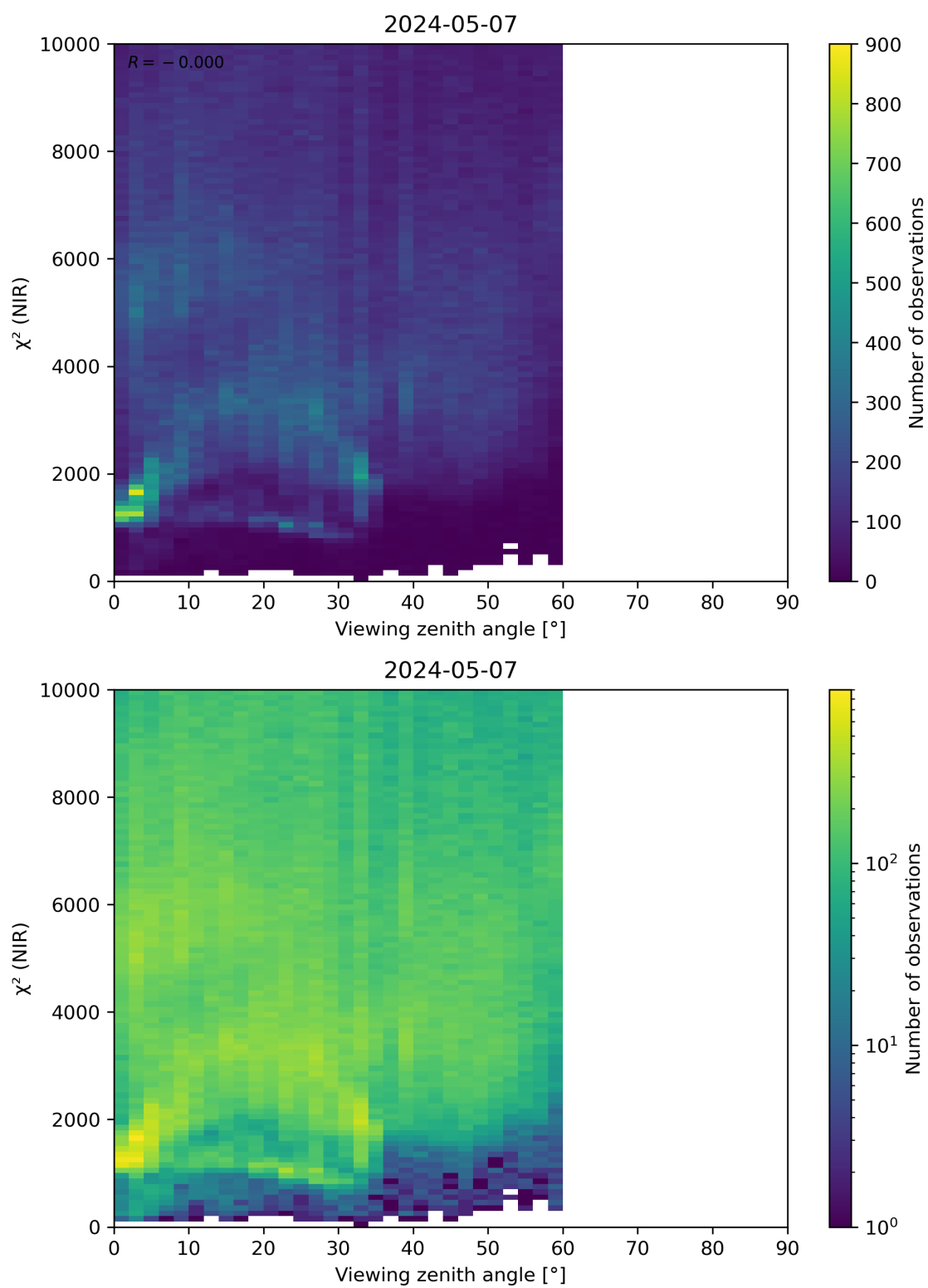
Figure 105: Scatter density plot of “Viewing zenith angle” against “ \chi^2 (NIR)” for 2024-05-07 to 2024-05-08.
