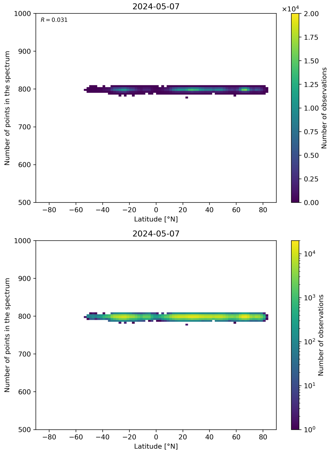
Figure 61: Scatter density plot of “Latitude” against “Number of points in the spectrum” for 2024-05-07 to 2024-05-08.
