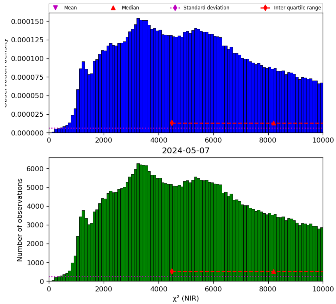
Figure 29: Histogram of “ \chi^2 (NIR)” for 2024-05-07 to 2024-05-08
