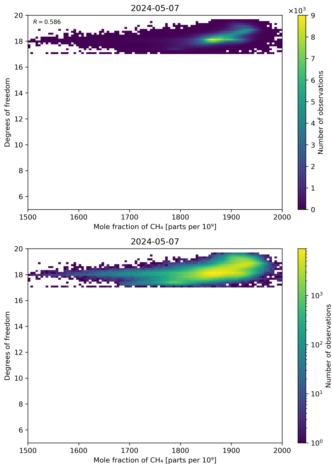
Figure 72: Scatter density plot of “Mole fraction of CH 4 ” against “Degrees of freedom” for 2024-05-07 to 2024-05-08.
