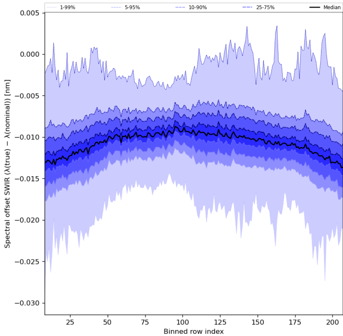
Figure 38: Along track statistics of “Spectral offset SWIR ( \lambda(\text{true}) - \lambda(\text{nominal}) )” for 2024-05-07 to 2024-05-08
