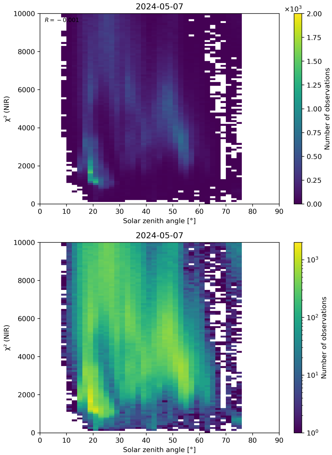
Figure 94: Scatter density plot of “Solar zenith angle” against “ \chi^2 (NIR)” for 2024-05-07 to 2024-05-08.
