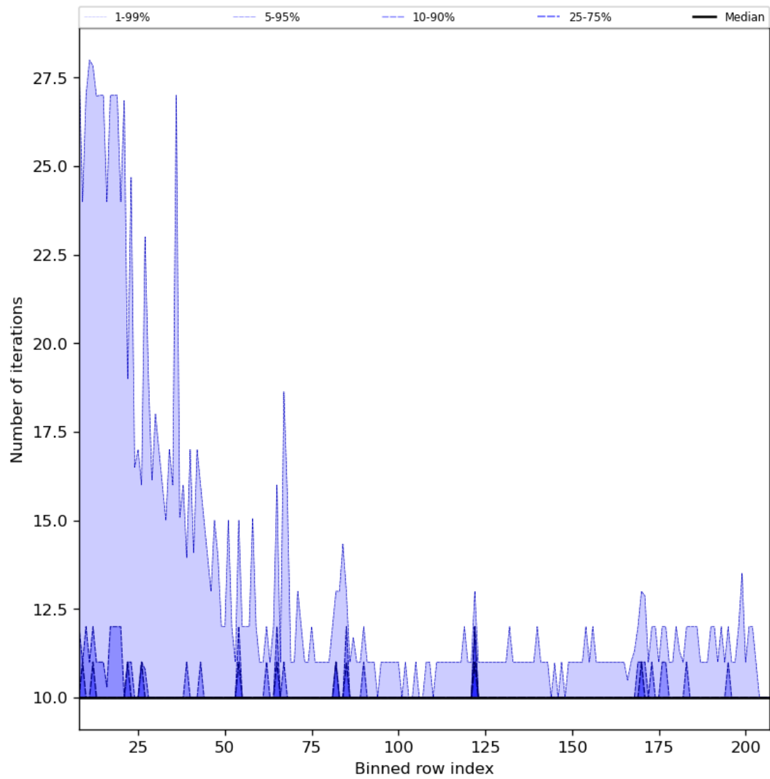
Figure 42: Along track statistics of “Number of iterations” for 2024-05-07 to 2024-05-08
