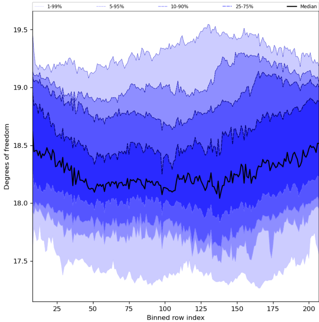
Figure 41: Along track statistics of “Degrees of freedom” for 2024-05-07 to 2024-05-08
