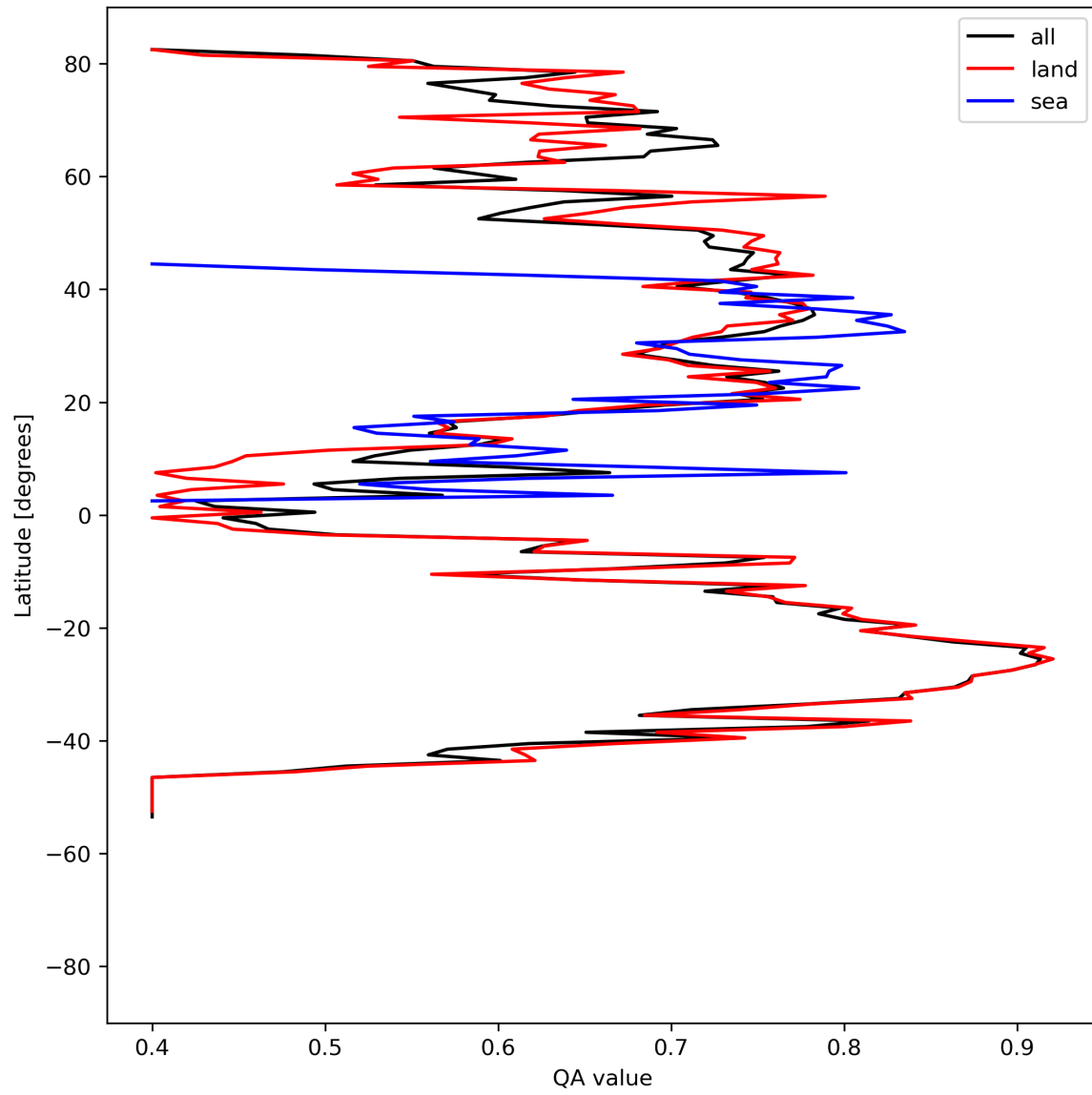
Figure 11: Zonal average of “QA value” for 2024-05-07 to 2024-05-08.
