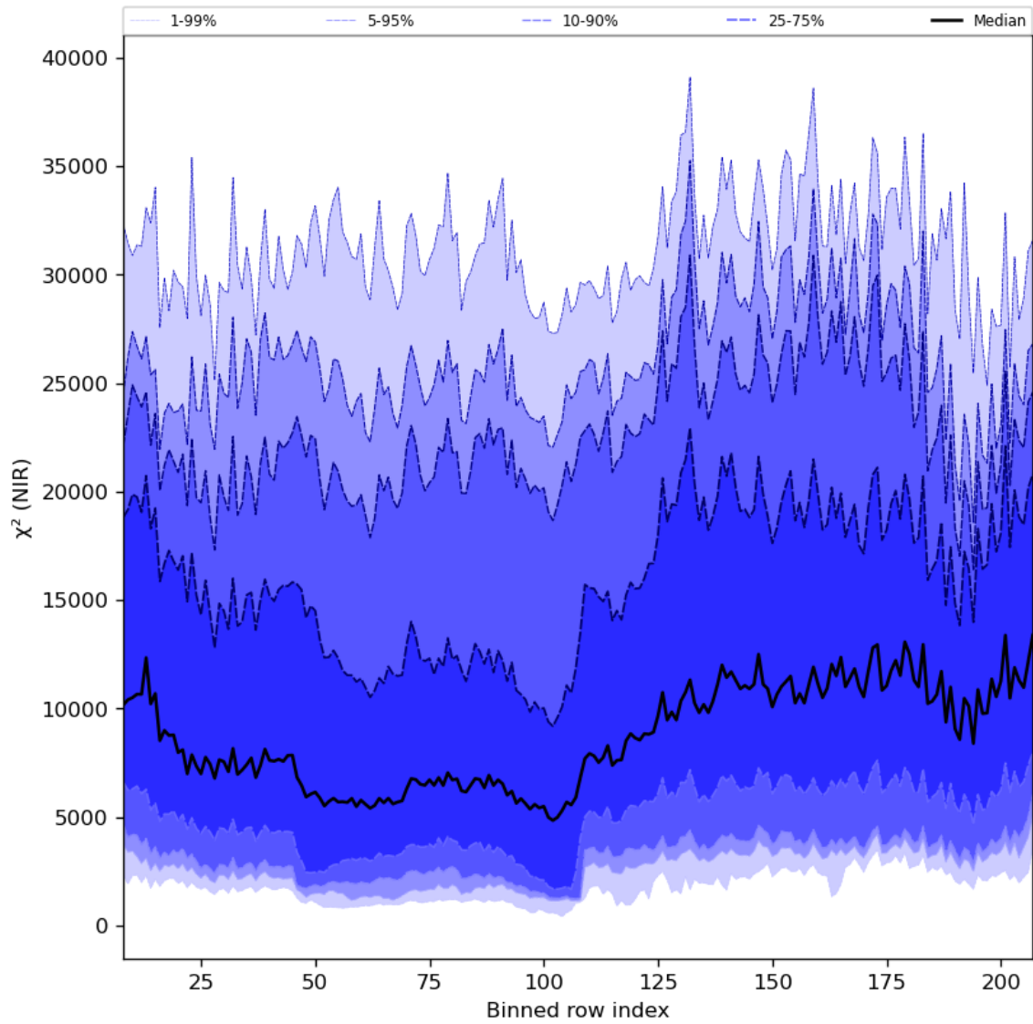
Figure 40: Along track statistics of “ \chi^2 (NIR)” for 2024-05-07 to 2024-05-08
