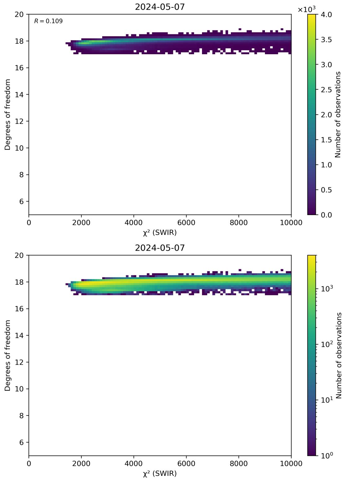
Figure 48: Scatter density plot of “ \chi^2 (SWIR)” against “Degrees of freedom” for 2024-05-07 to 2024-05-08.
