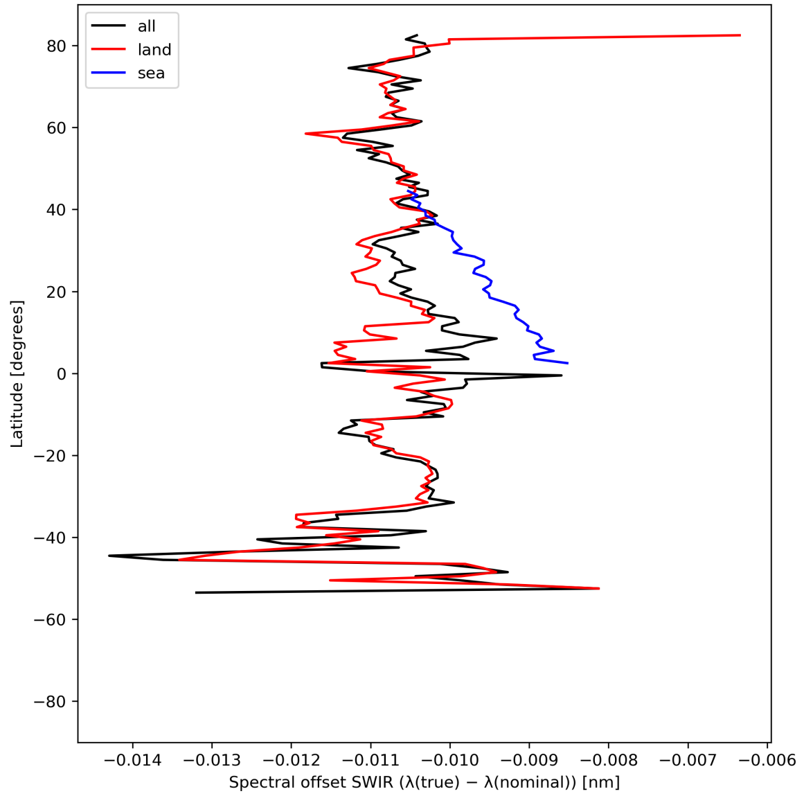
Figure 16: Zonal average of “Spectral offset SWIR ( \lambda(\text{true}) - \lambda(\text{nominal}) )” for 2024-05-07 to 2024-05-08.
