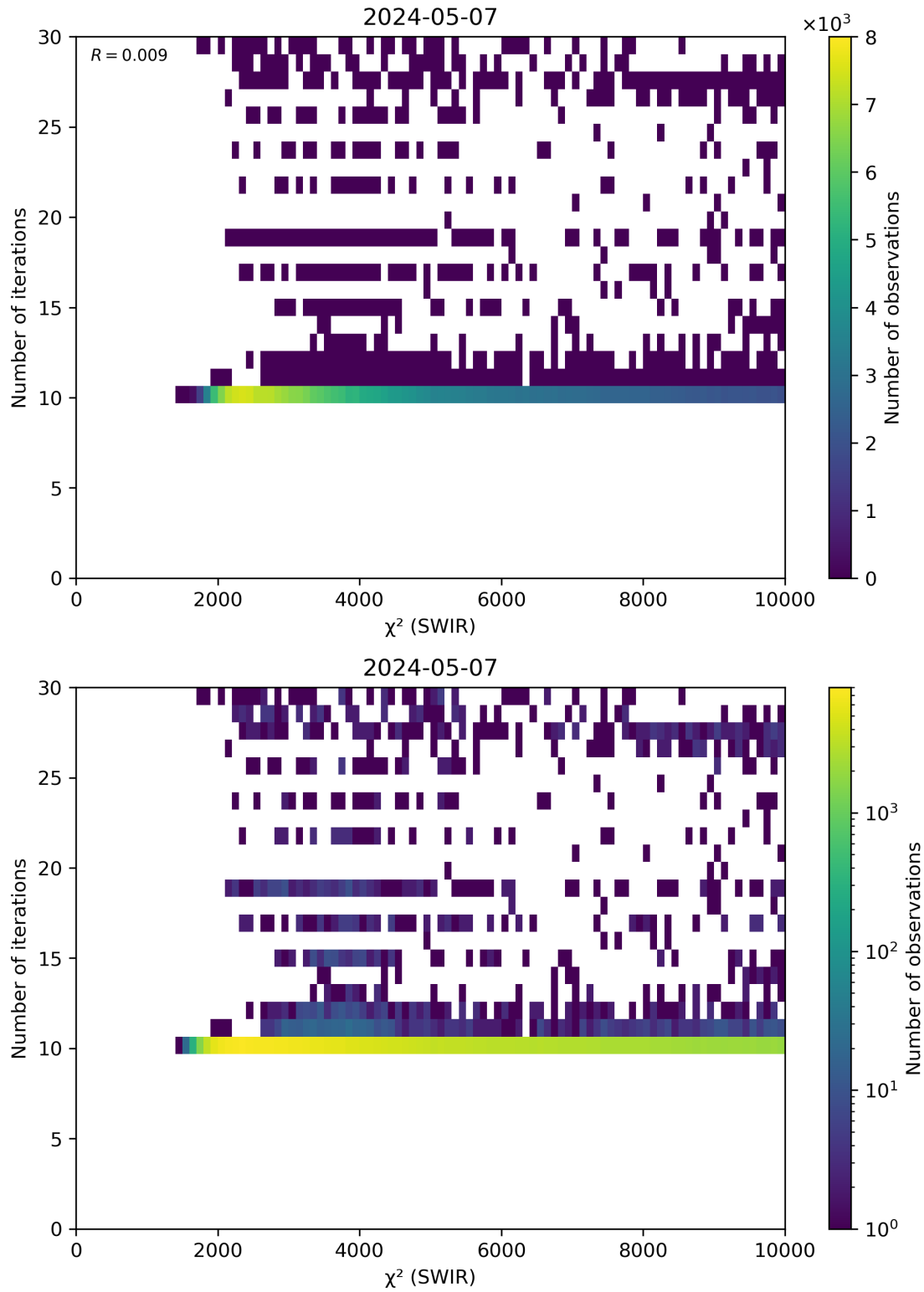
Figure 50: Scatter density plot of “ \chi^2 (SWIR)” against “Number of iterations” for 2024-05-07 to 2024-05-08.
