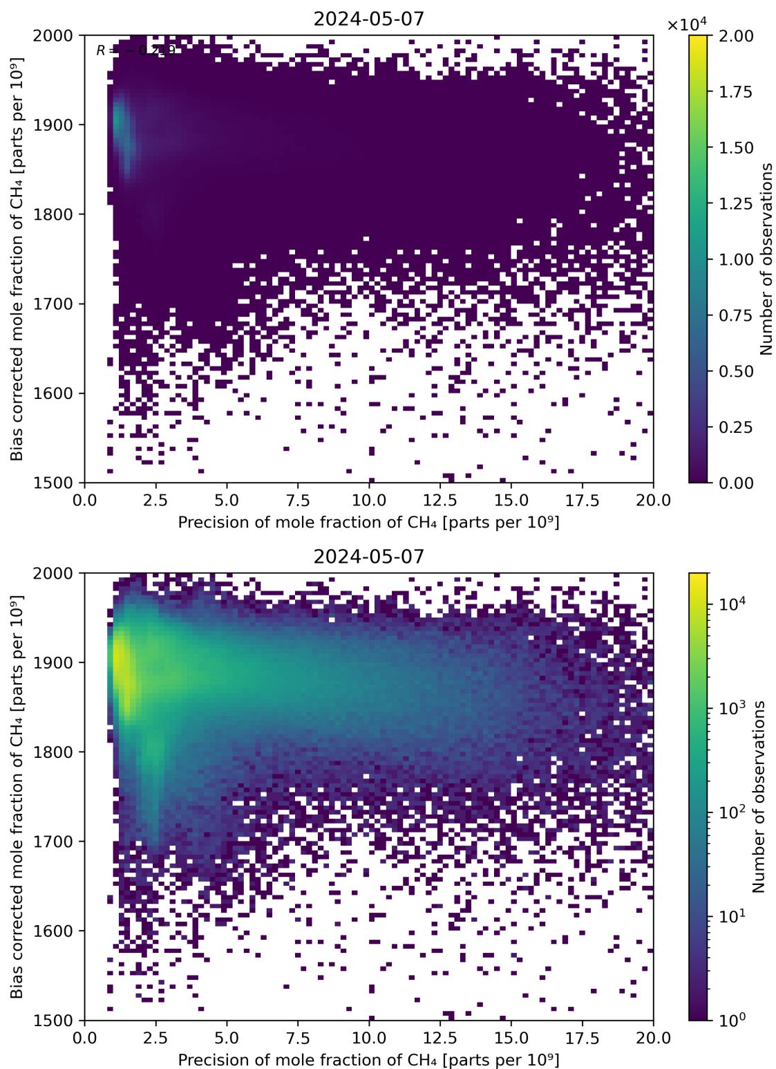
Figure 82: Scatter density plot of “Precision of mole fraction of \text{CH}_4 ” against “Bias corrected mole fraction of \text{CH}_4 ” for 2024-05-07 to 2024-05-08.
