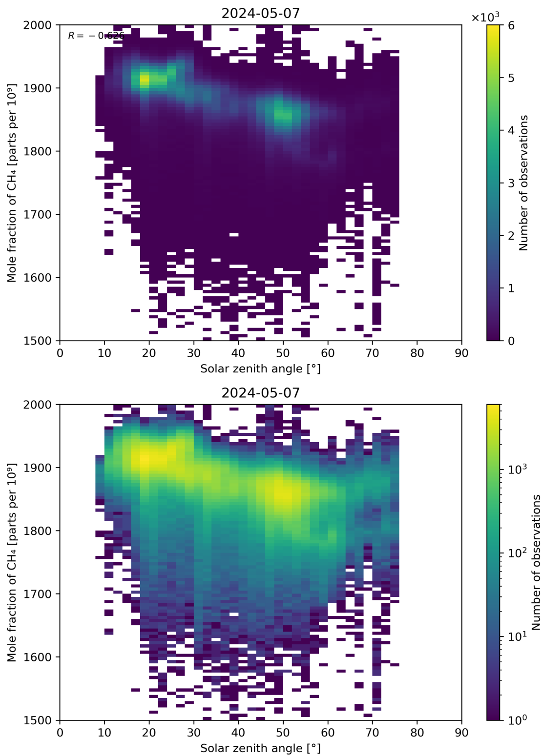
Figure 99: Scatter density plot of “Solar zenith angle” against “Mole fraction of CH 4 ” for 2024-05-07 to 2024-05-08.
