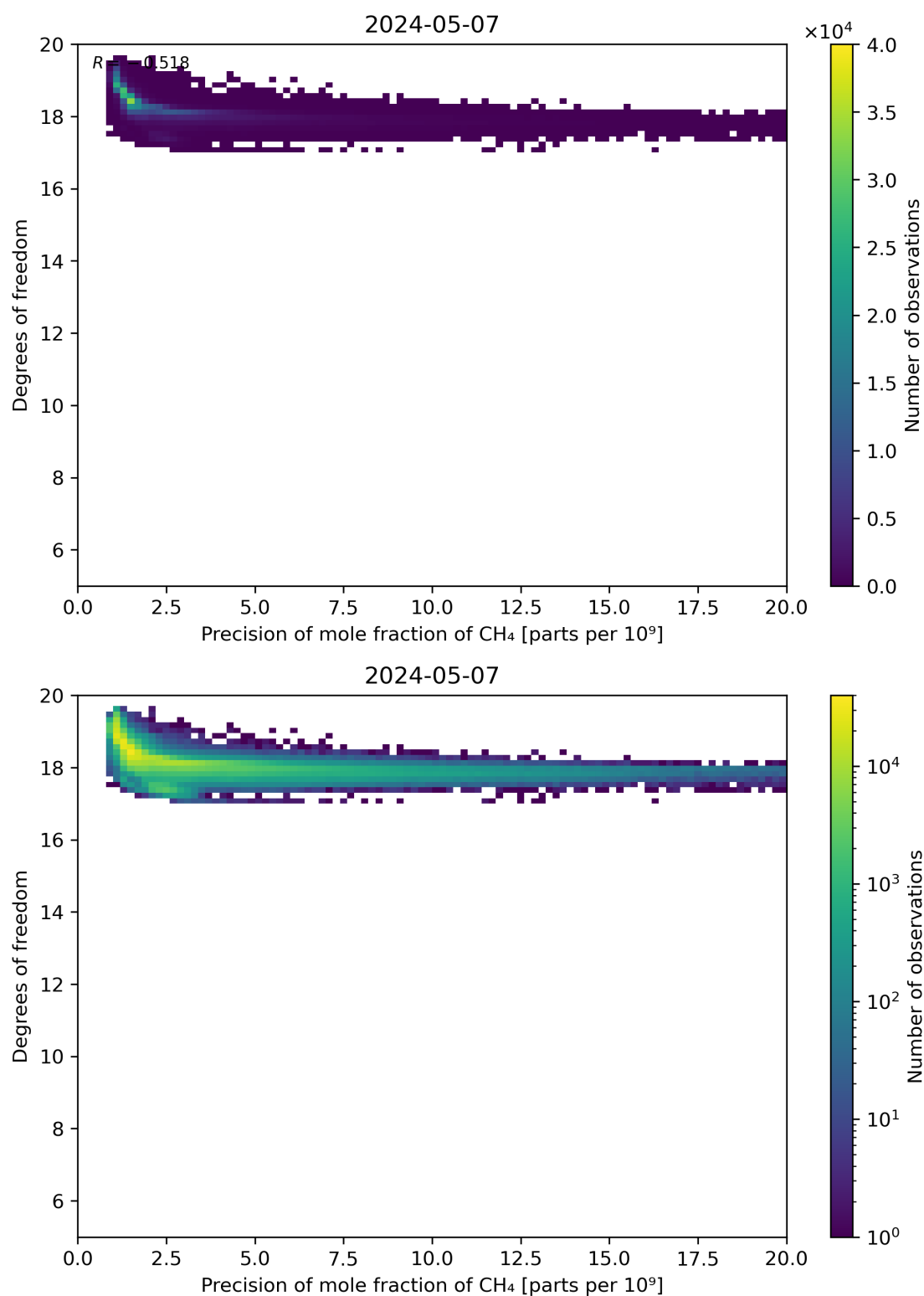
Figure 80: Scatter density plot of “Precision of mole fraction of CH 4 ” against “Degrees of freedom” for 2024-05-07 to 2024-05-08.
