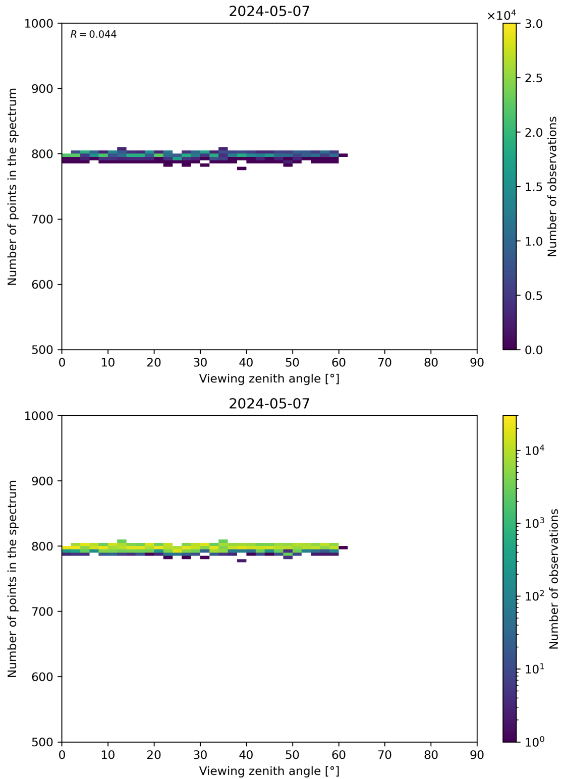
Figure 114: Scatter density plot of “Viewing zenith angle” against “Number of points in the spectrum” for 2024-05-07 to 2024-05-08.
