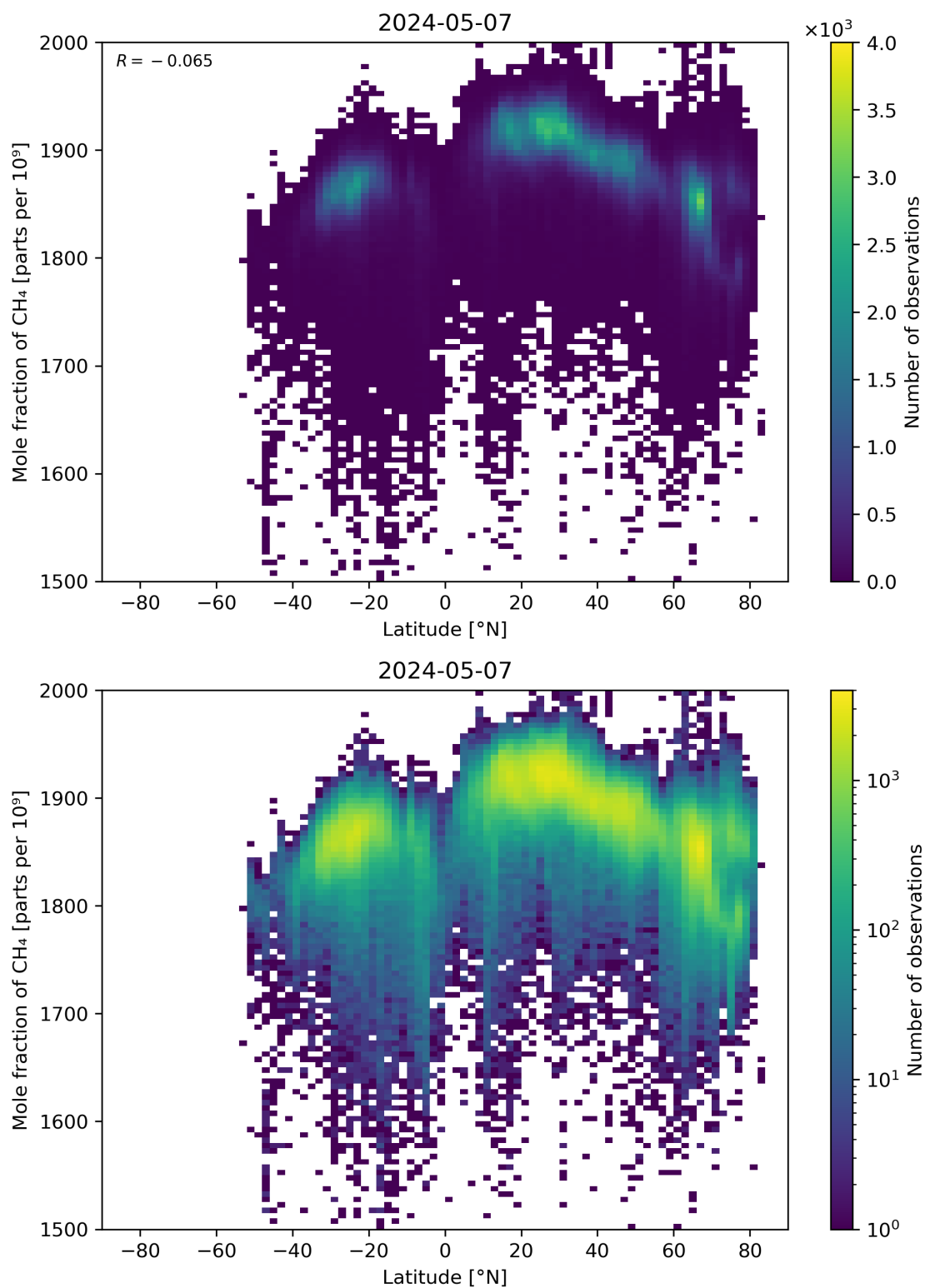
Figure 57: Scatter density plot of “Latitude” against “Mole fraction of \text{CH}_4 ” for 2024-05-07 to 2024-05-08.
