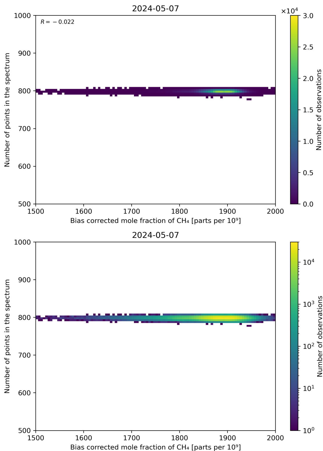
Figure 68: Scatter density plot of “Bias corrected mole fraction of CH 4 ” against “Number of points in the spectrum” for 2024-05-07 to 2024-05-08.
