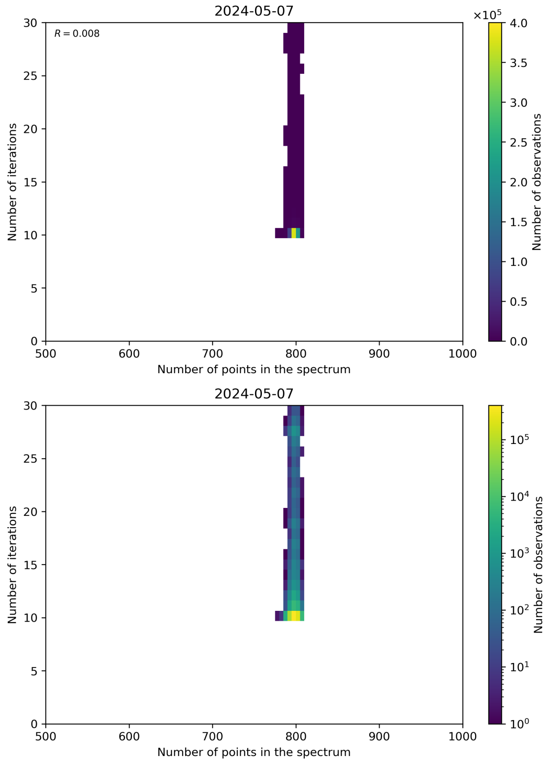
Figure 92: Scatter density plot of “Number of points in the spectrum” against “Number of iterations” for 2024-05-07 to 2024-05-08.
