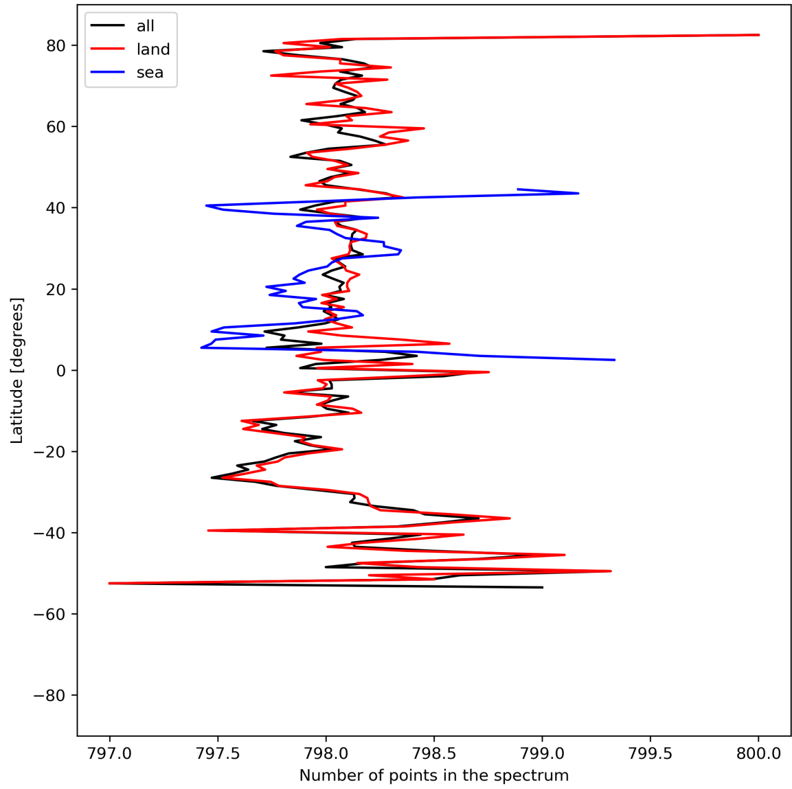
Figure 15: Zonal average of “Number of points in the spectrum” for 2024-05-07 to 2024-05-08.
