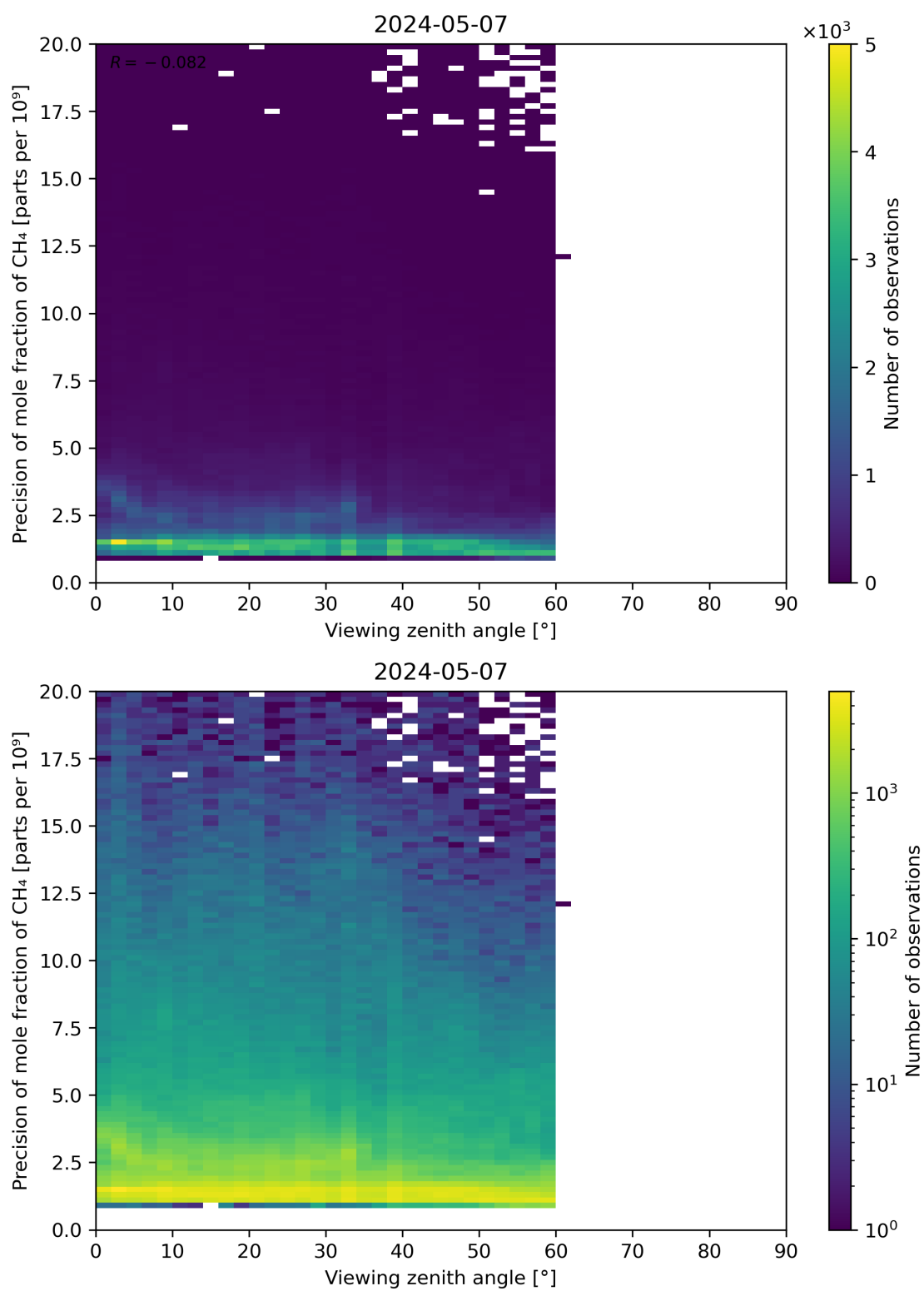
Figure 112: Scatter density plot of “Viewing zenith angle” against “Precision of mole fraction of CH 4 ” for 2024-05-07 to 2024-05-08.
