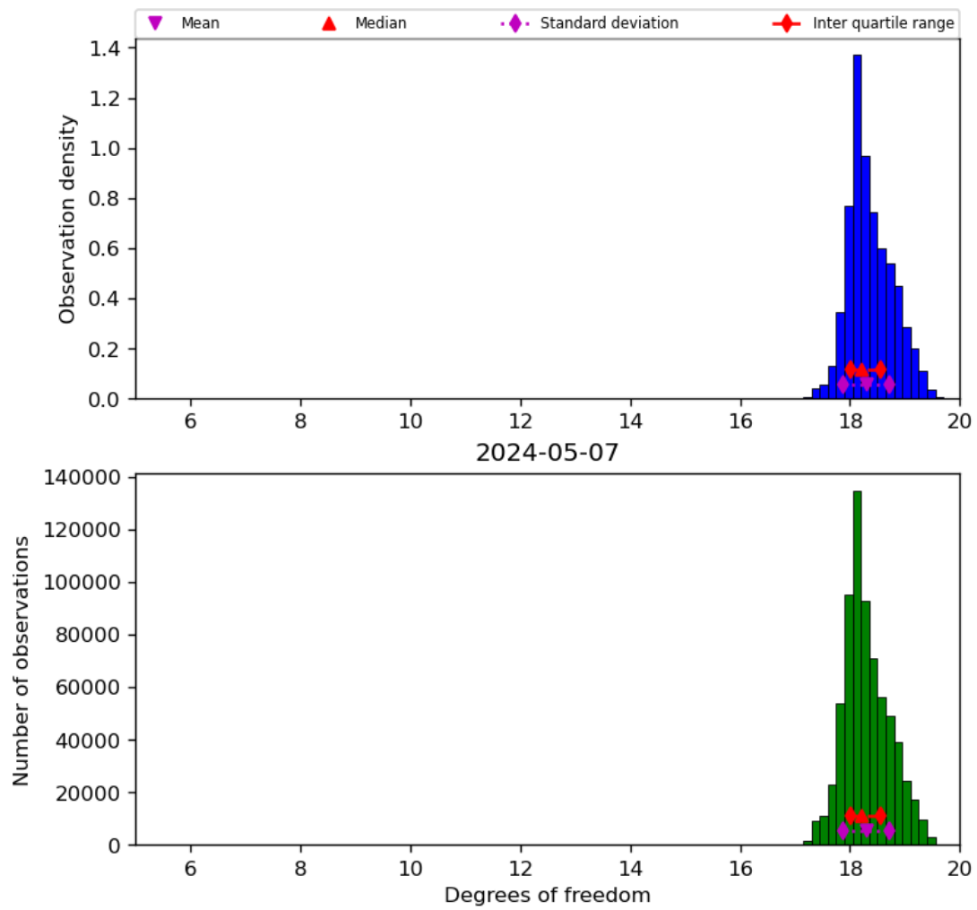
Figure 30: Histogram of “Degrees of freedom” for 2024-05-07 to 2024-05-08
