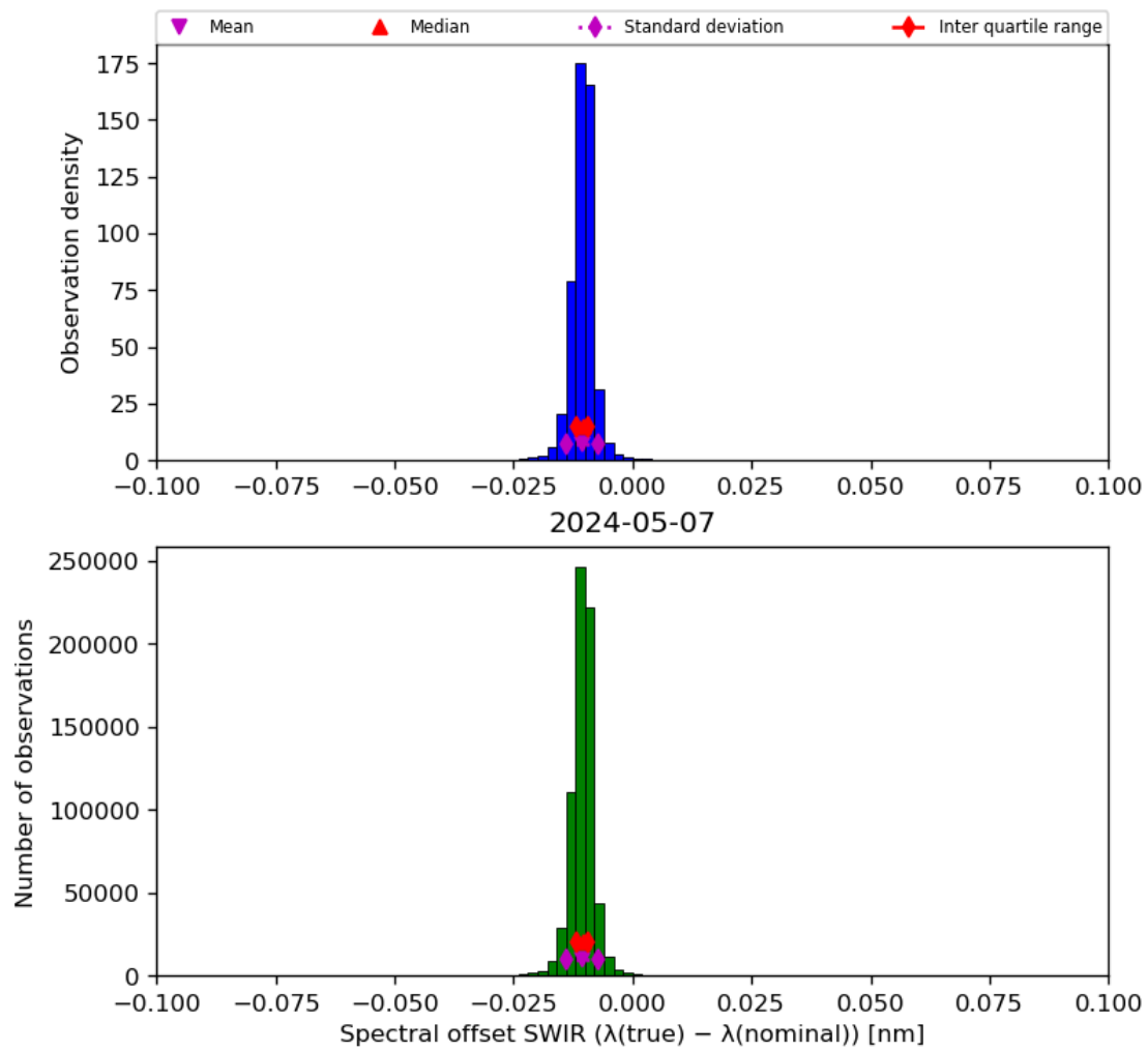
Figure 27: Histogram of “Spectral offset SWIR ( \lambda(\text{true}) - \lambda(\text{nominal}) )” for 2024-05-07 to 2024-05-08
