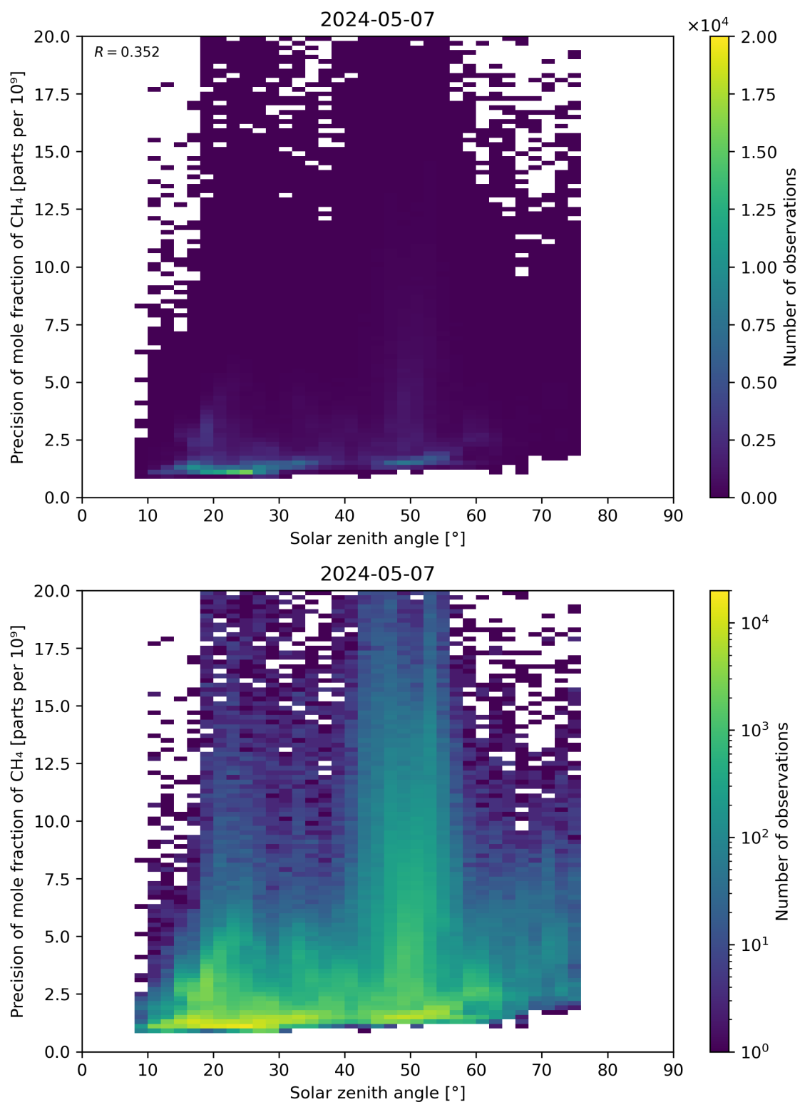
Figure 101: Scatter density plot of “Solar zenith angle” against “Precision of mole fraction of CH 4 ” for 2024-05-07 to 2024-05-08.
