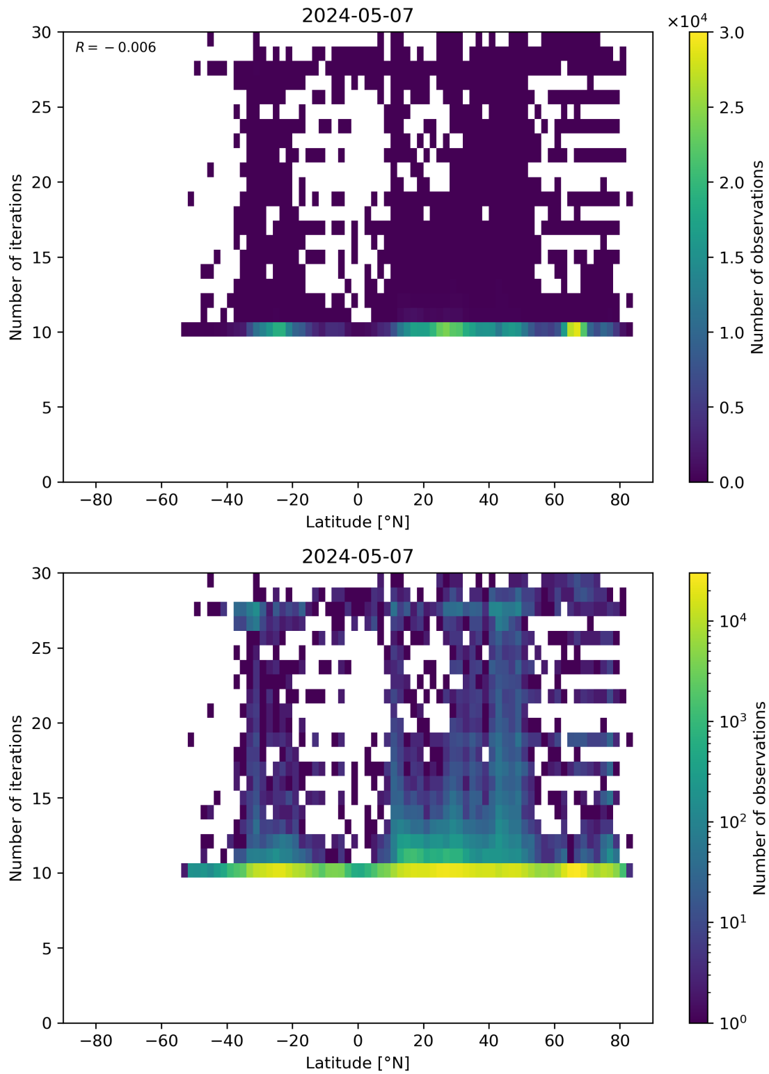
Figure 60: Scatter density plot of “Latitude” against “Number of iterations” for 2024-05-07 to 2024-05-08.
