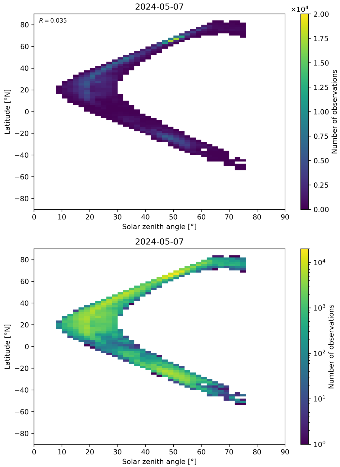
Figure 98: Scatter density plot of “Solar zenith angle” against “Latitude” for 2024-05-07 to 2024-05-08.
