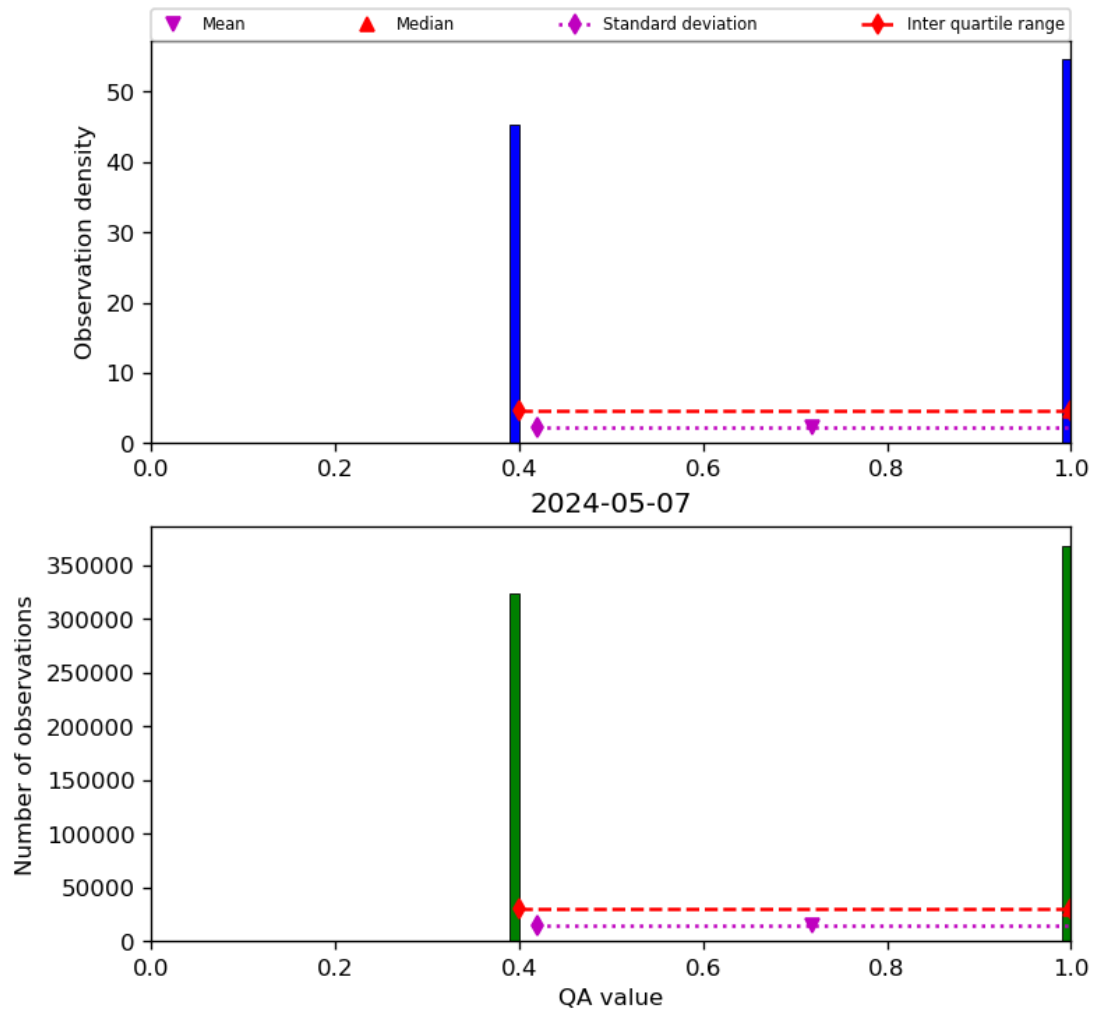
Figure 22: Histogram of “QA value” for 2024-05-07 to 2024-05-08
