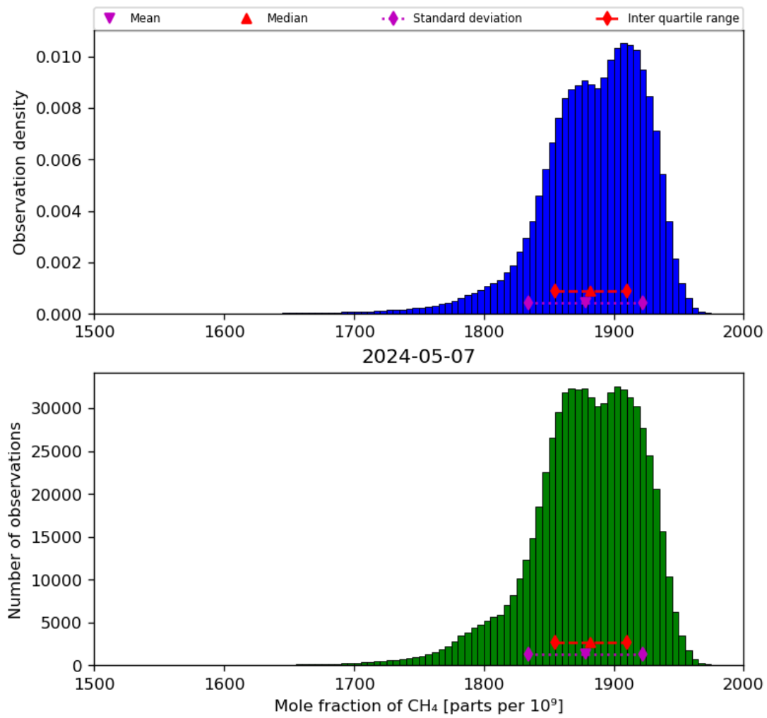
Figure 23: Histogram of “Mole fraction of CH 4 ” for 2024-05-07 to 2024-05-08
