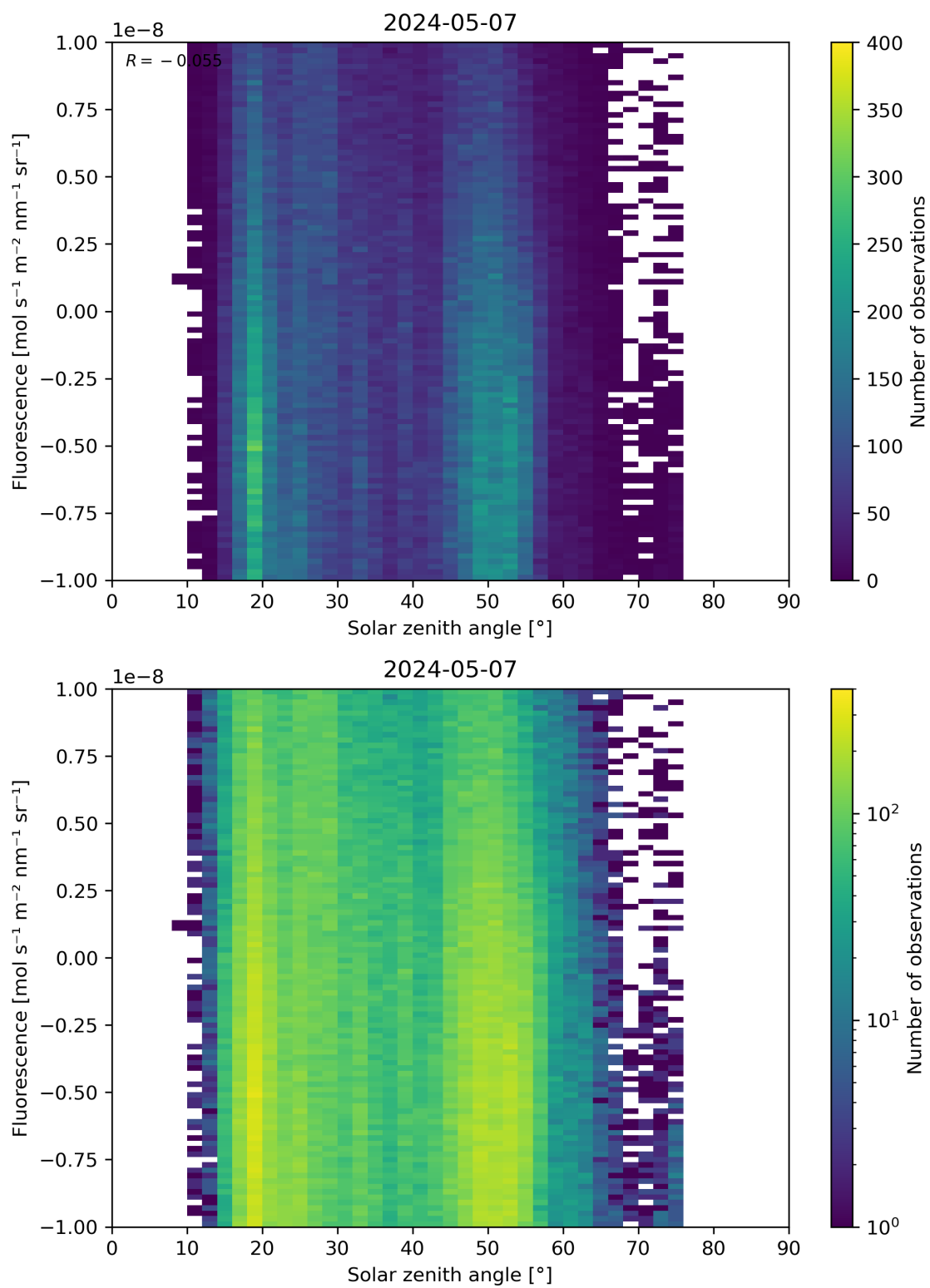
Figure 97: Scatter density plot of “Solar zenith angle” against “Fluorescence” for 2024-05-07 to 2024-05-08.
