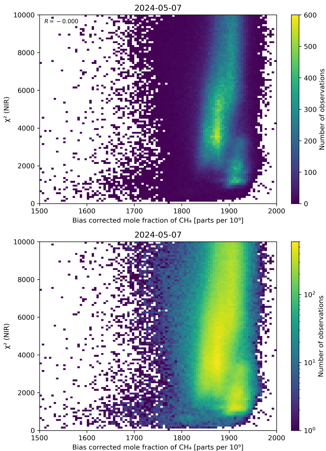
Figure 63: Scatter density plot of “Bias corrected mole fraction of CH 4 ” against “ \chi^2 (NIR)” for 2024-05-07 to 2024-05-08.
