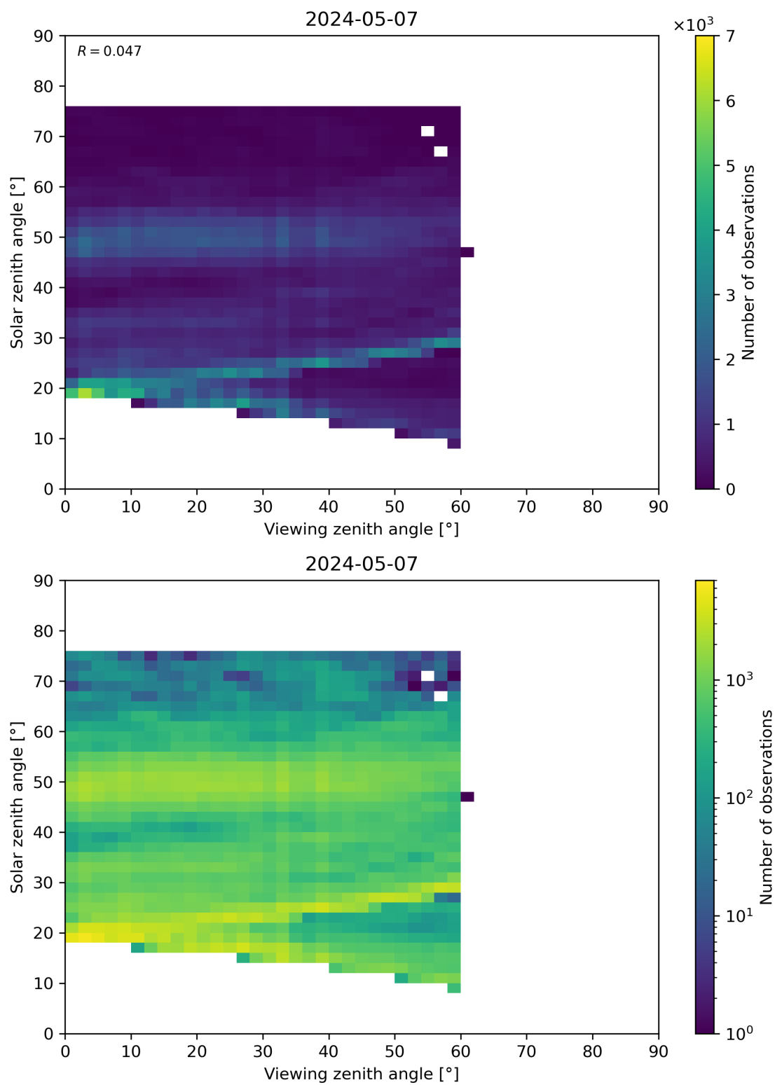
Figure 115: Scatter density plot of “Viewing zenith angle” against “Solar zenith angle” for 2024-05-07 to 2024-05-08.
