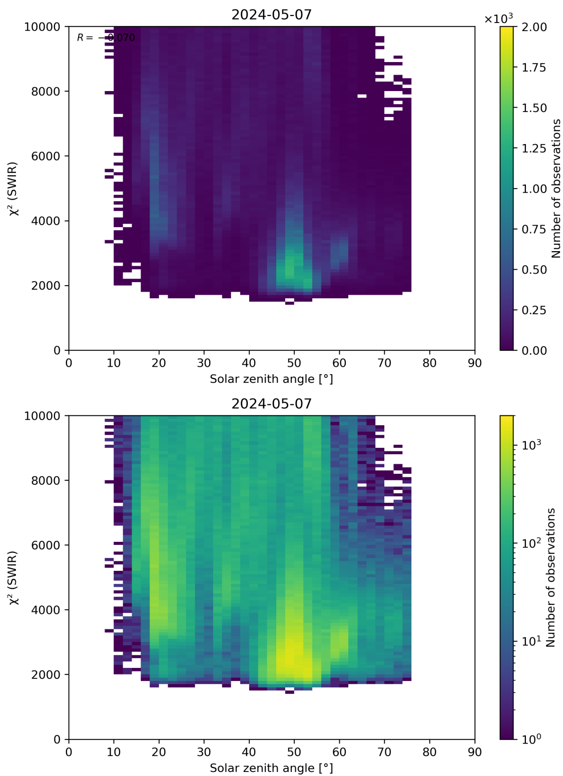
Figure 95: Scatter density plot of “Solar zenith angle” against “ \chi^2 (SWIR)” for 2024-05-07 to 2024-05-08.
