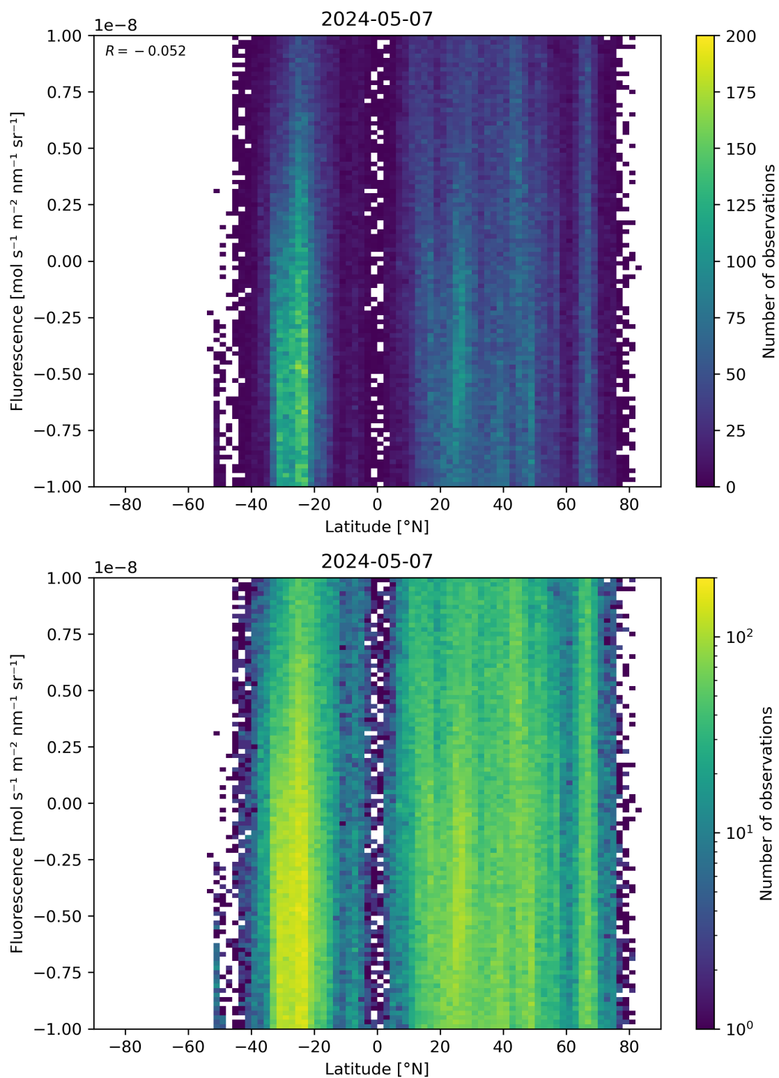
Figure 56: Scatter density plot of “Latitude” against “Fluorescence” for 2024-05-07 to 2024-05-08.
