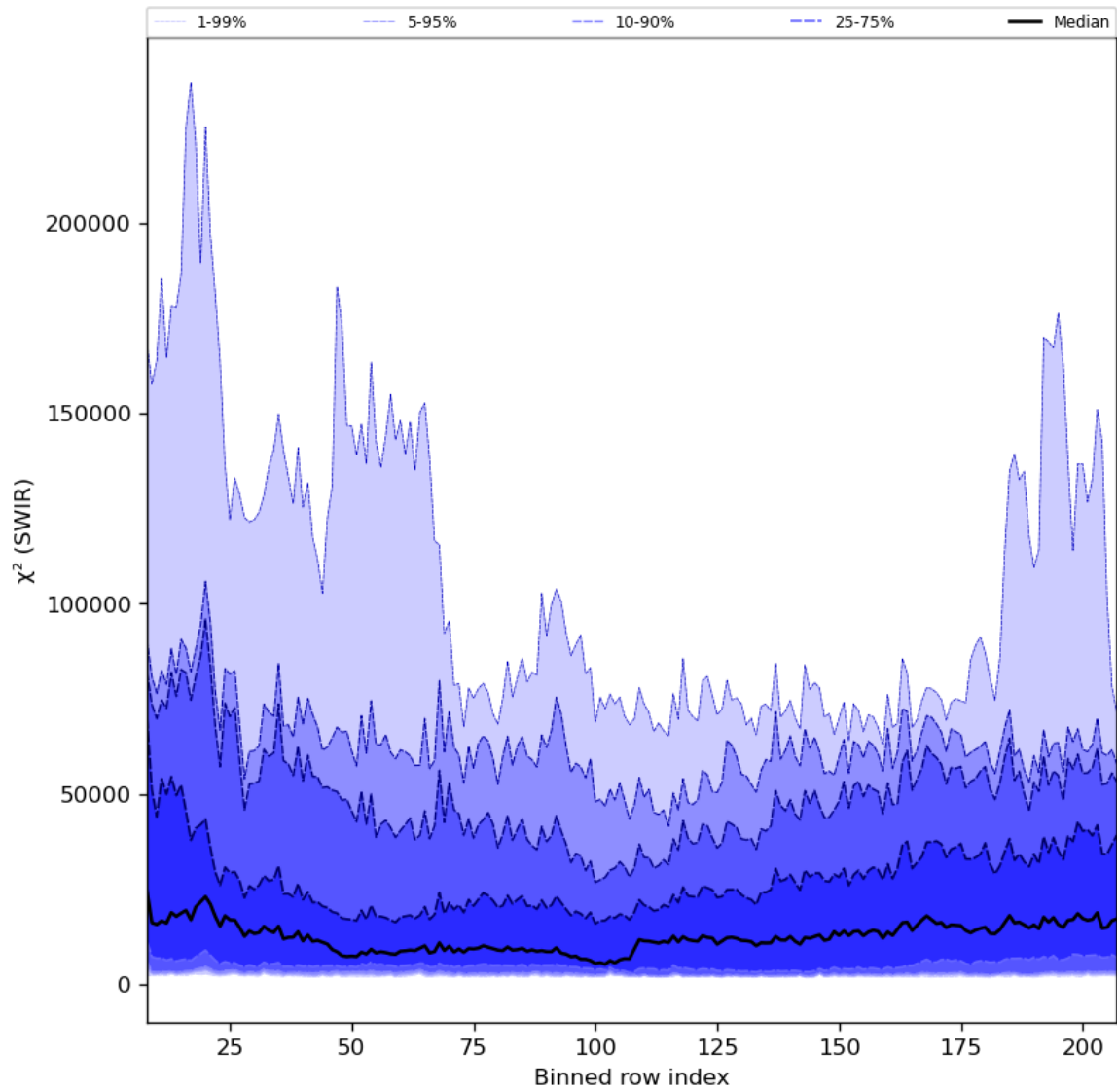
Figure 39: Along track statistics of “ \chi^2 (SWIR)” for 2024-05-07 to 2024-05-08
