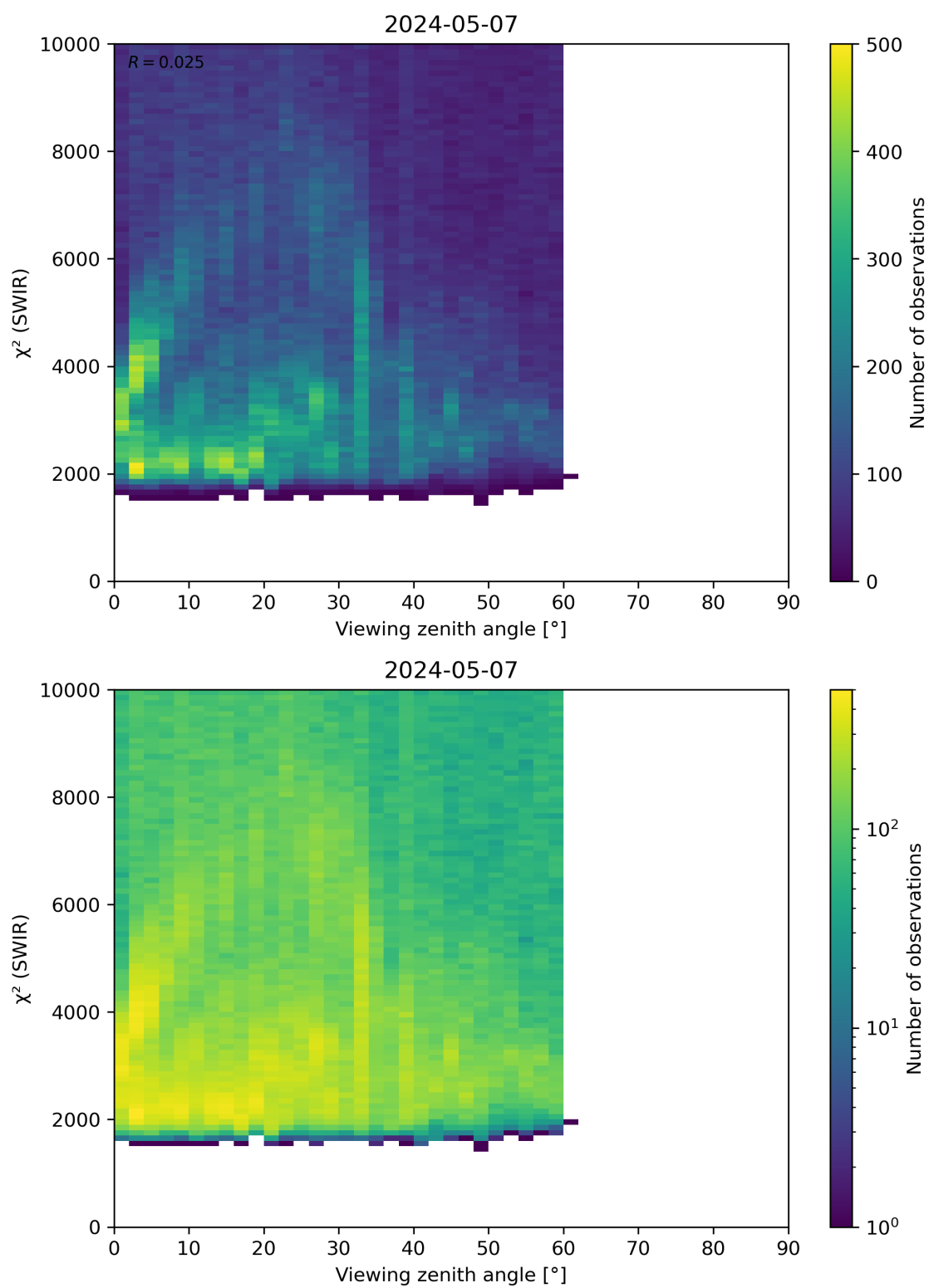
Figure 106: Scatter density plot of “Viewing zenith angle” against “ \chi^2 (SWIR)” for 2024-05-07 to 2024-05-08.
