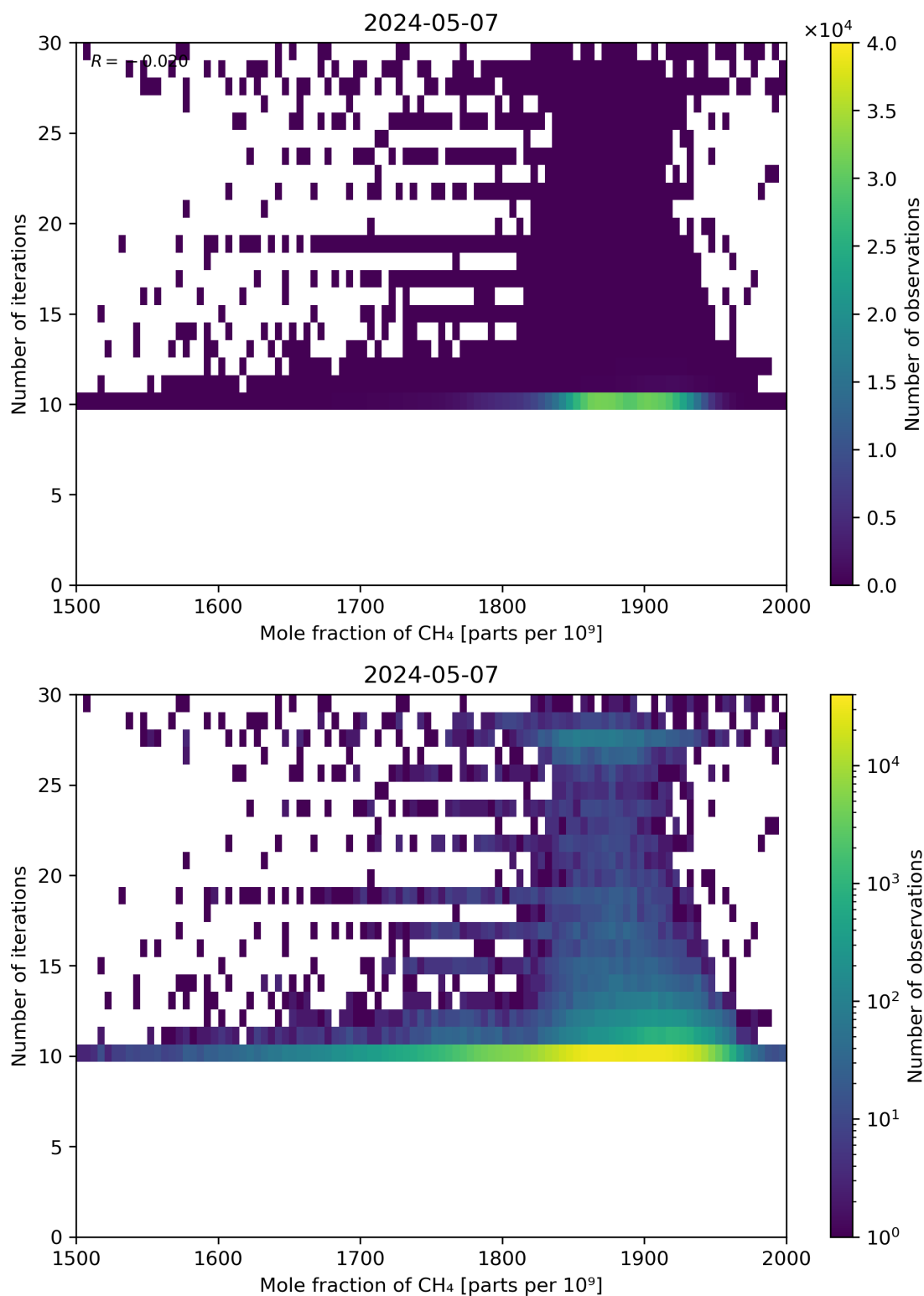
Figure 76: Scatter density plot of “Mole fraction of CH 4 ” against “Number of iterations” for 2024-05-07 to 2024-05-08.
