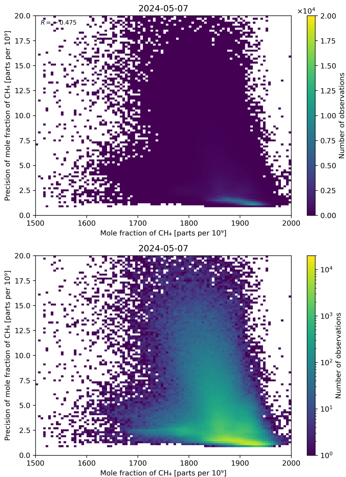
Figure 75: Scatter density plot of “Mole fraction of CH 4 ” against “Precision of mole fraction of CH 4 ” for 2024-05-07 to 2024-05-08.
