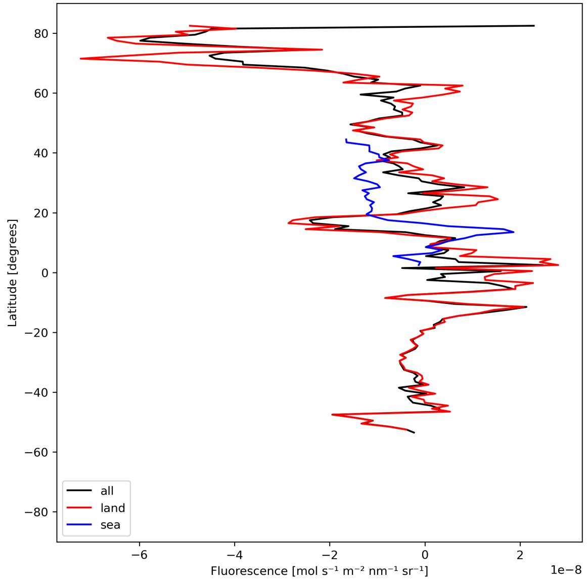
Figure 21: Zonal average of “Fluorescence” for 2024-05-07 to 2024-05-08.
