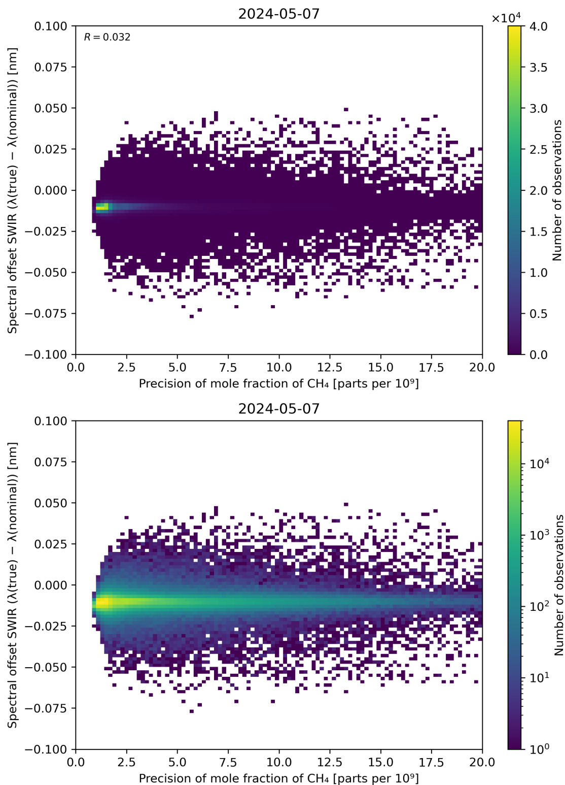
Figure 85: Scatter density plot of “Precision of mole fraction of \text{CH}_4 ” against “Spectral offset SWIR ( \lambda(\text{true}) - \lambda(\text{nominal}) )” for 2024-05-07 to 2024-05-08.
