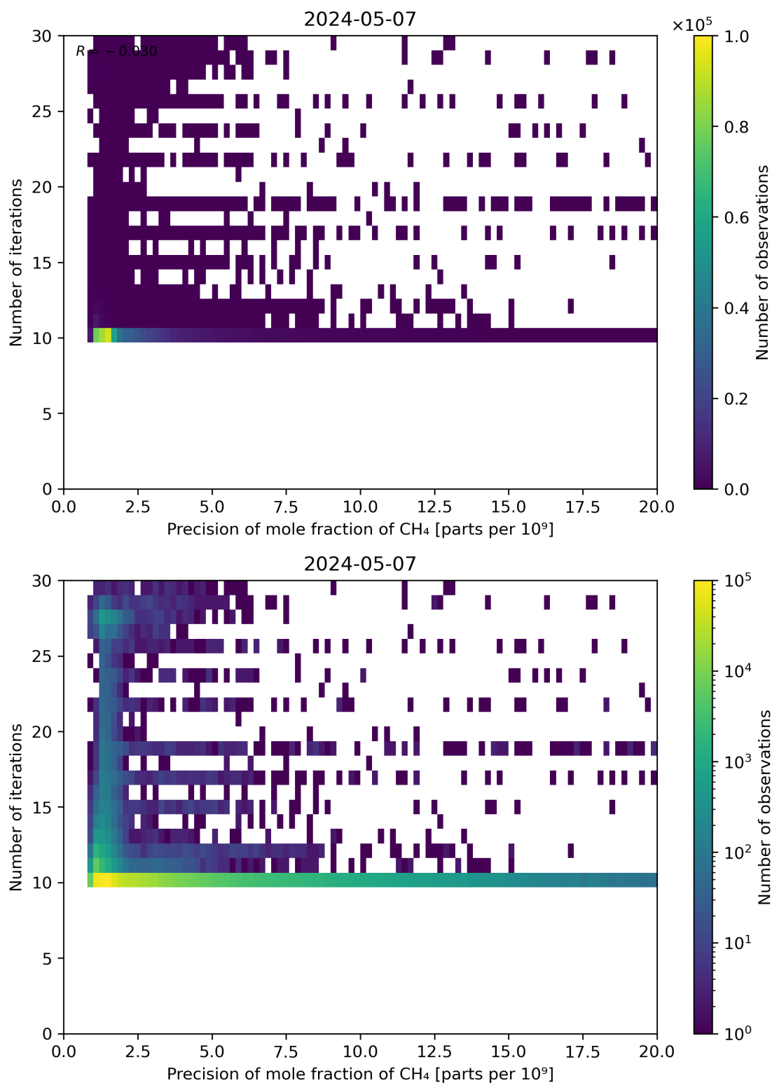
Figure 83: Scatter density plot of “Precision of mole fraction of CH 4 ” against “Number of iterations” for 2024-05-07 to 2024-05-08.
