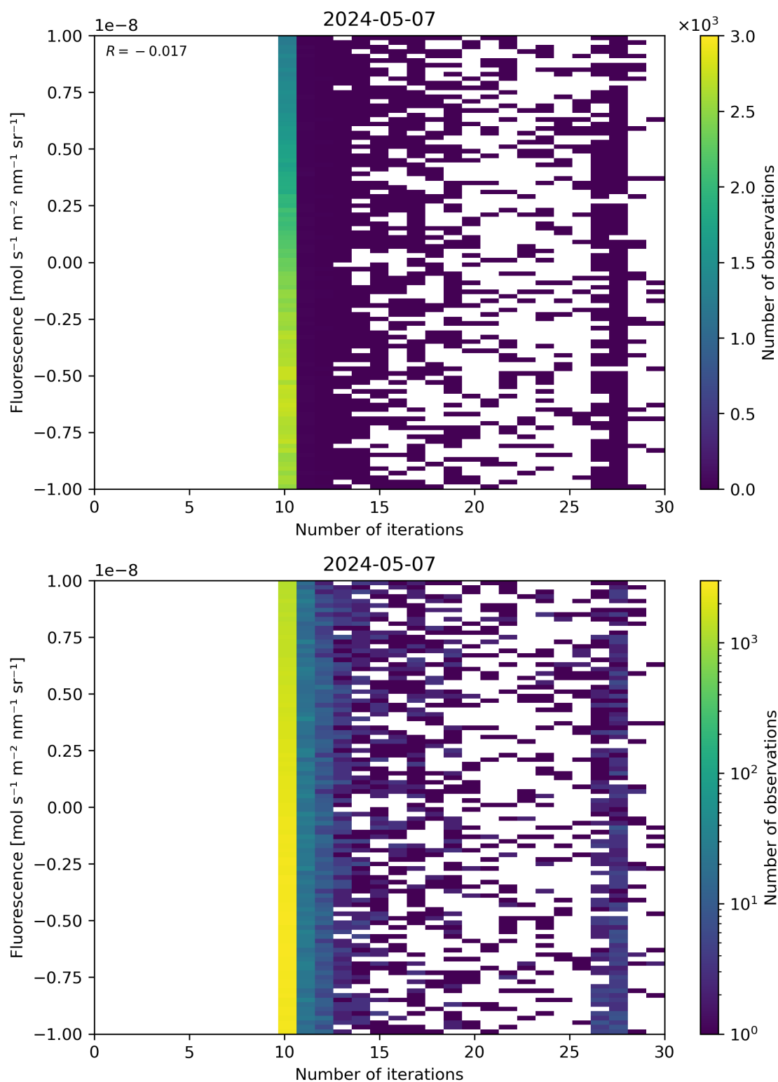
Figure 87: Scatter density plot of “Number of iterations” against “Fluorescence” for 2024-05-07 to 2024-05-08.
