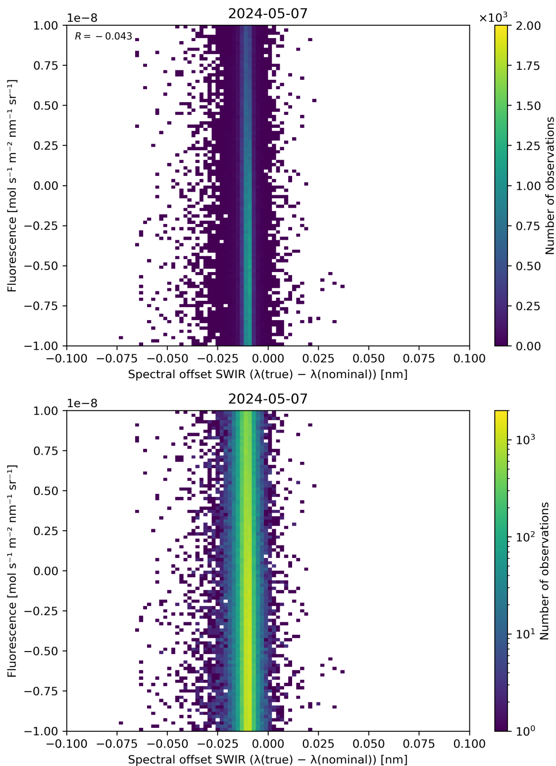
Figure 120: Scatter density plot of “Spectral offset SWIR ( \lambda(\text{true}) - \lambda(\text{nominal}) )” against “Fluorescence” for 2024-05-07 to 2024-05-08.
