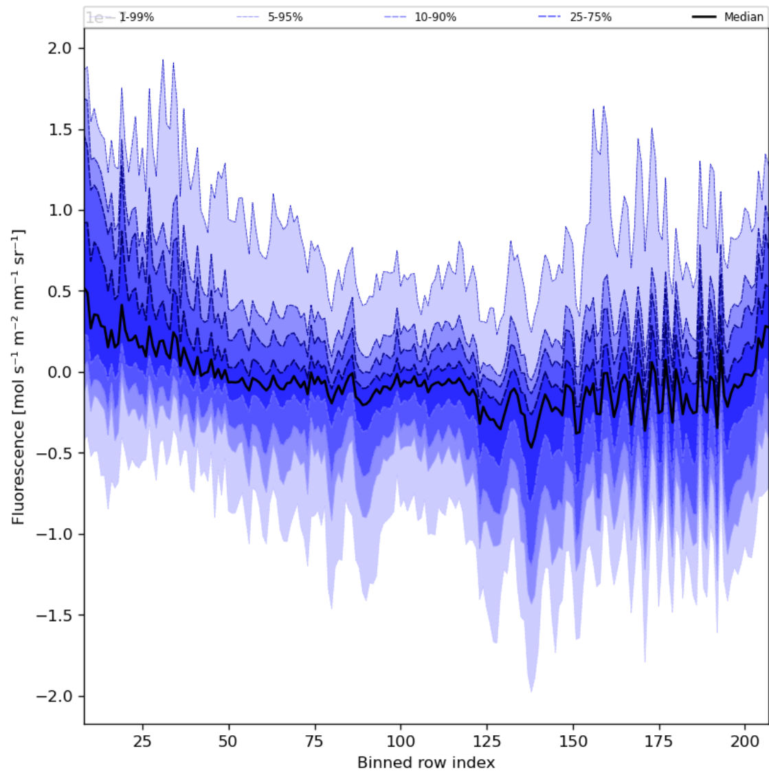
Figure 43: Along track statistics of “Fluorescence” for 2024-05-07 to 2024-05-08
