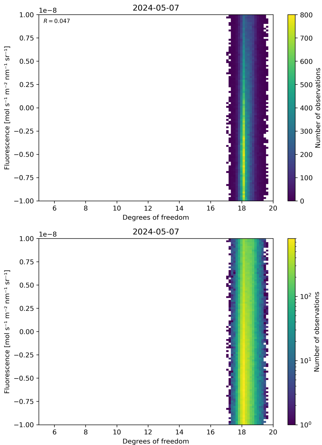
Figure 51: Scatter density plot of “Degrees of freedom” against “Fluorescence” for 2024-05-07 to 2024-05-08.
