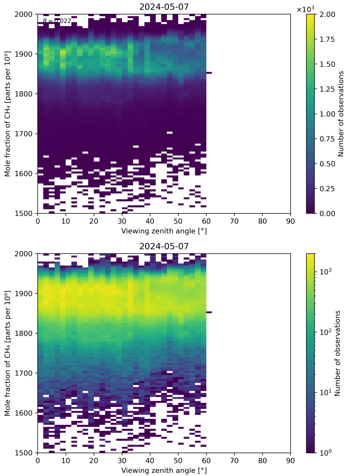
Figure 110: Scatter density plot of “Viewing zenith angle” against “Mole fraction of CH 4 ” for 2024-05-07 to 2024-05-08.
