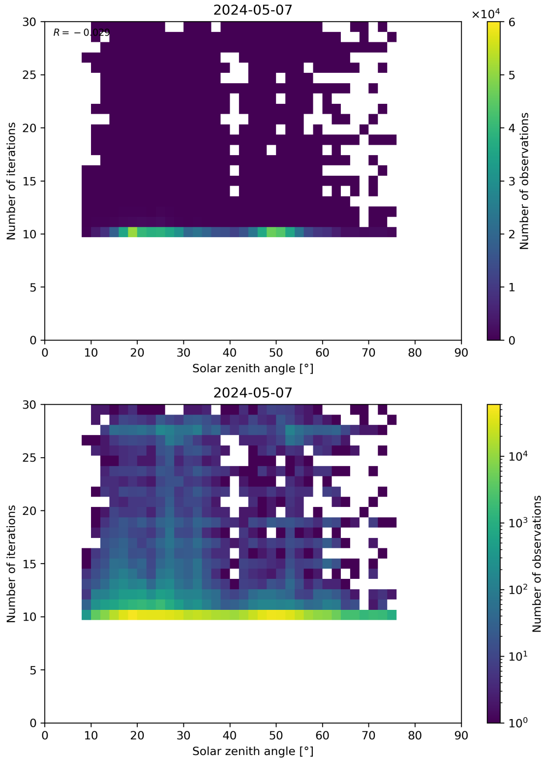
Figure 102: Scatter density plot of “Solar zenith angle” against “Number of iterations” for 2024-05-07 to 2024-05-08.
