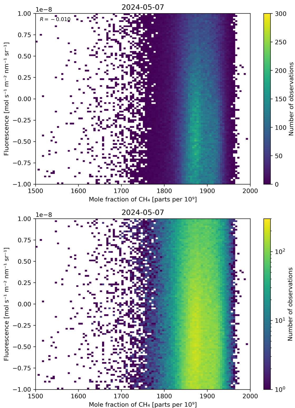
Figure 73: Scatter density plot of “Mole fraction of \text{CH}_4 ” against “Fluorescence” for 2024-05-07 to 2024-05-08.
