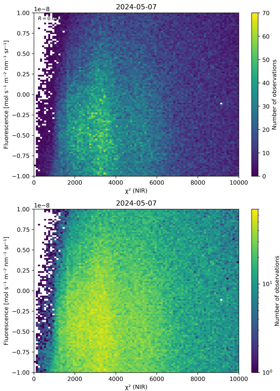
Figure 45: Scatter density plot of “ \chi^2 (NIR)” against “Fluorescence” for 2024-05-07 to 2024-05-08.
