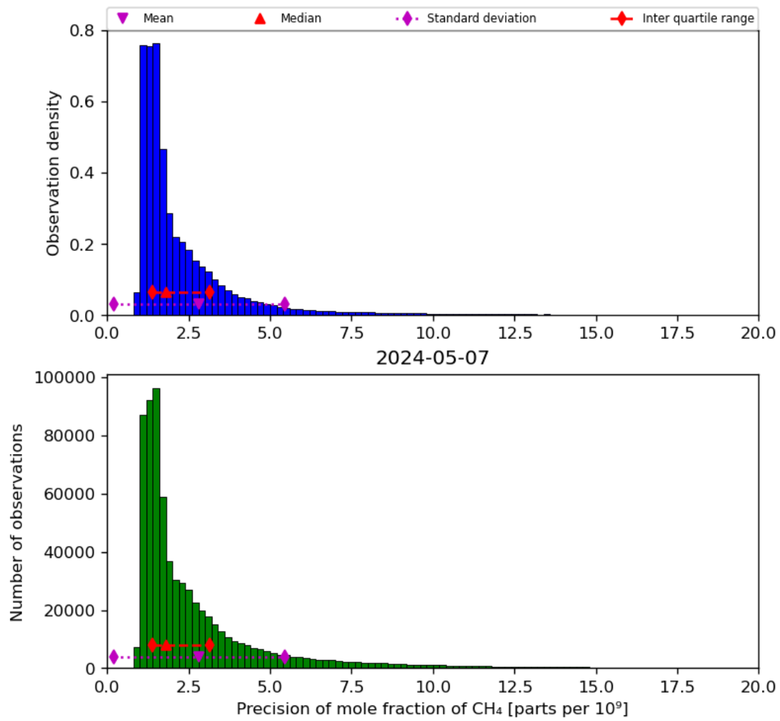
Figure 24: Histogram of “Precision of mole fraction of CH 4 ” for 2024-05-07 to 2024-05-08
