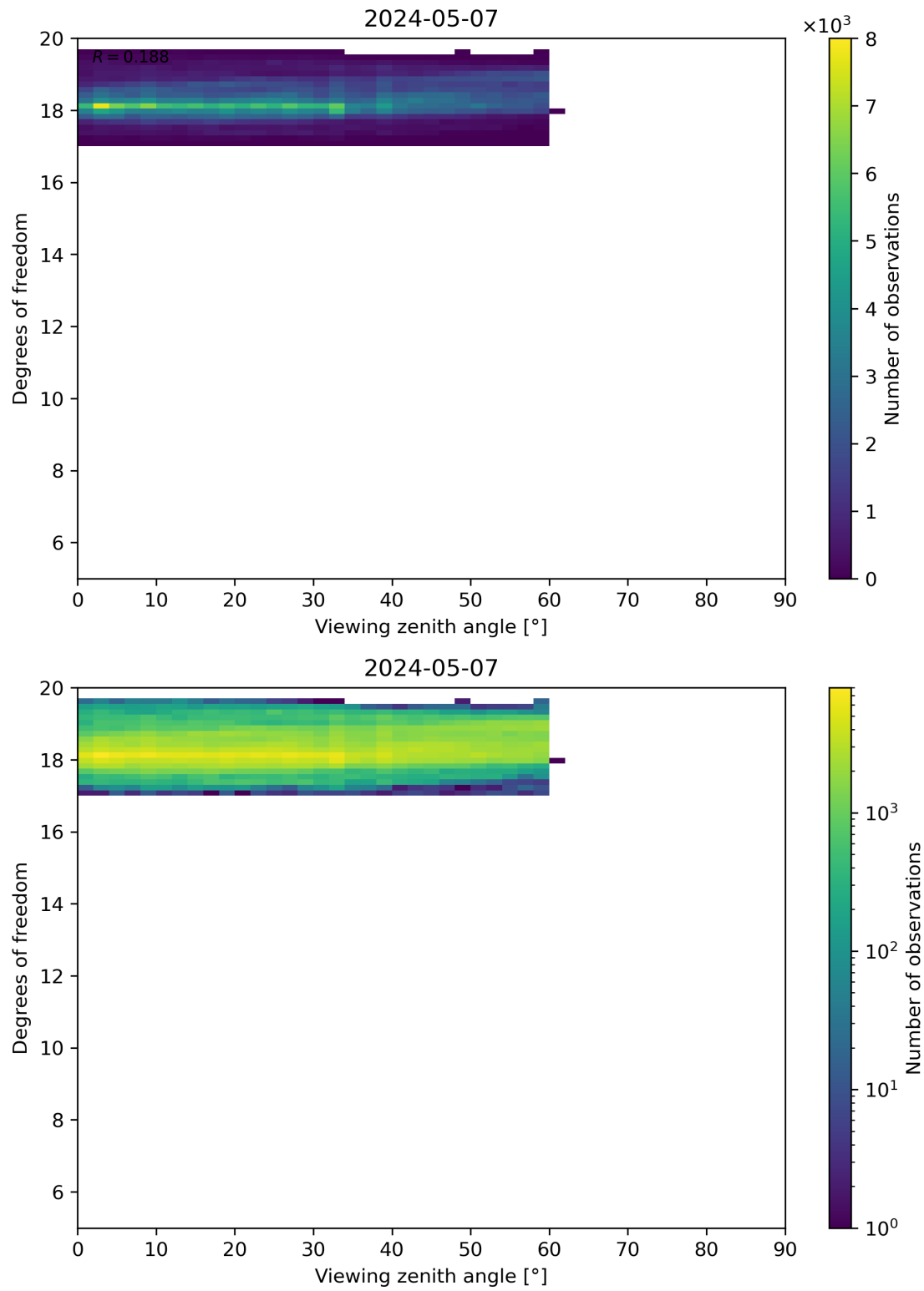
Figure 107: Scatter density plot of “Viewing zenith angle” against “Degrees of freedom” for 2024-05-07 to 2024-05-08.
