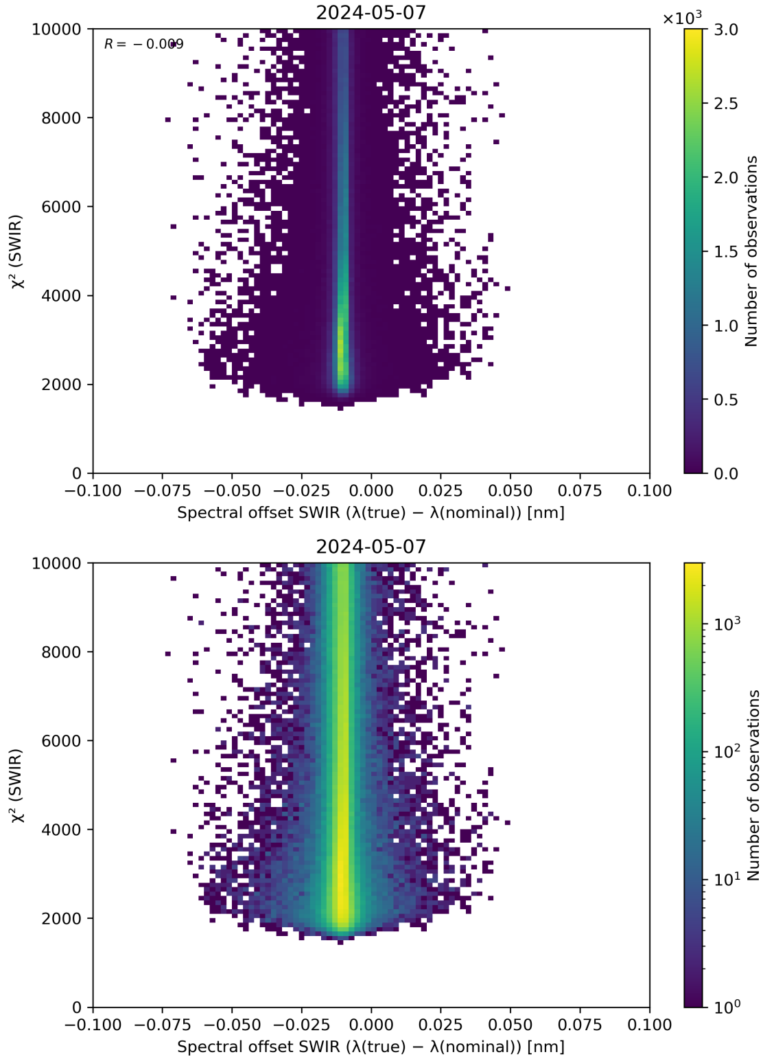
Figure 118: Scatter density plot of “Spectral offset SWIR ( \lambda(\text{true}) - \lambda(\text{nominal}) )” against “ \chi^2 (SWIR)” for 2024-05-07 to 2024-05-08.
