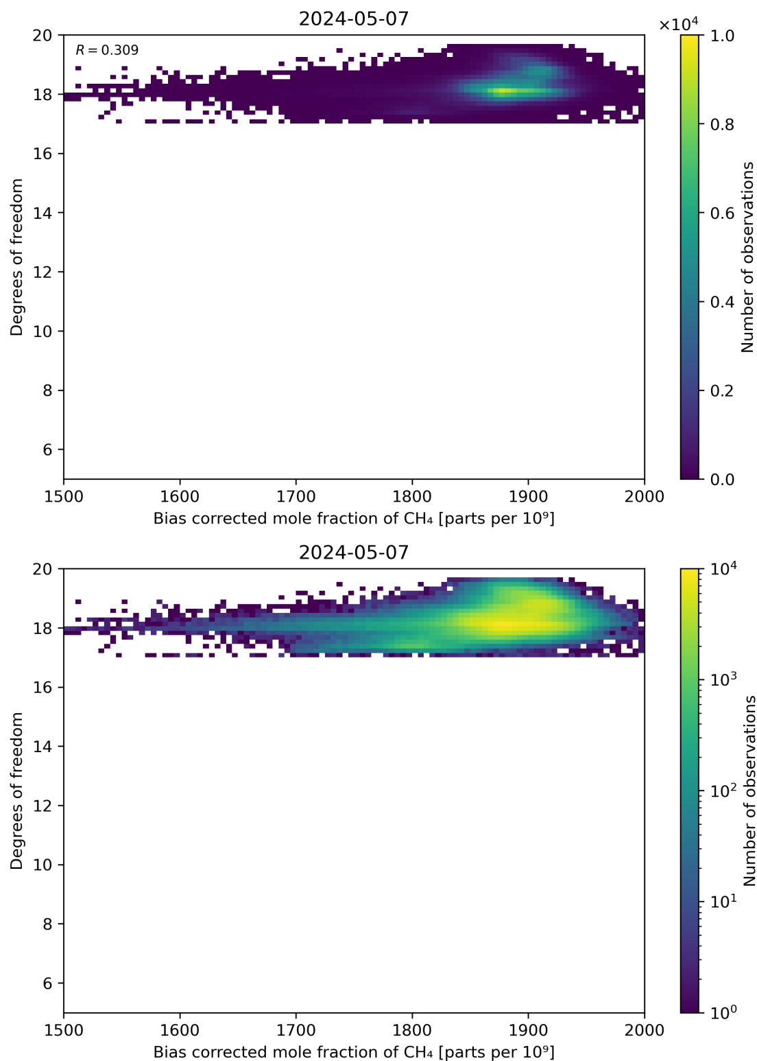
Figure 65: Scatter density plot of “Bias corrected mole fraction of CH 4 ” against “Degrees of freedom” for 2024-05-07 to 2024-05-08.
