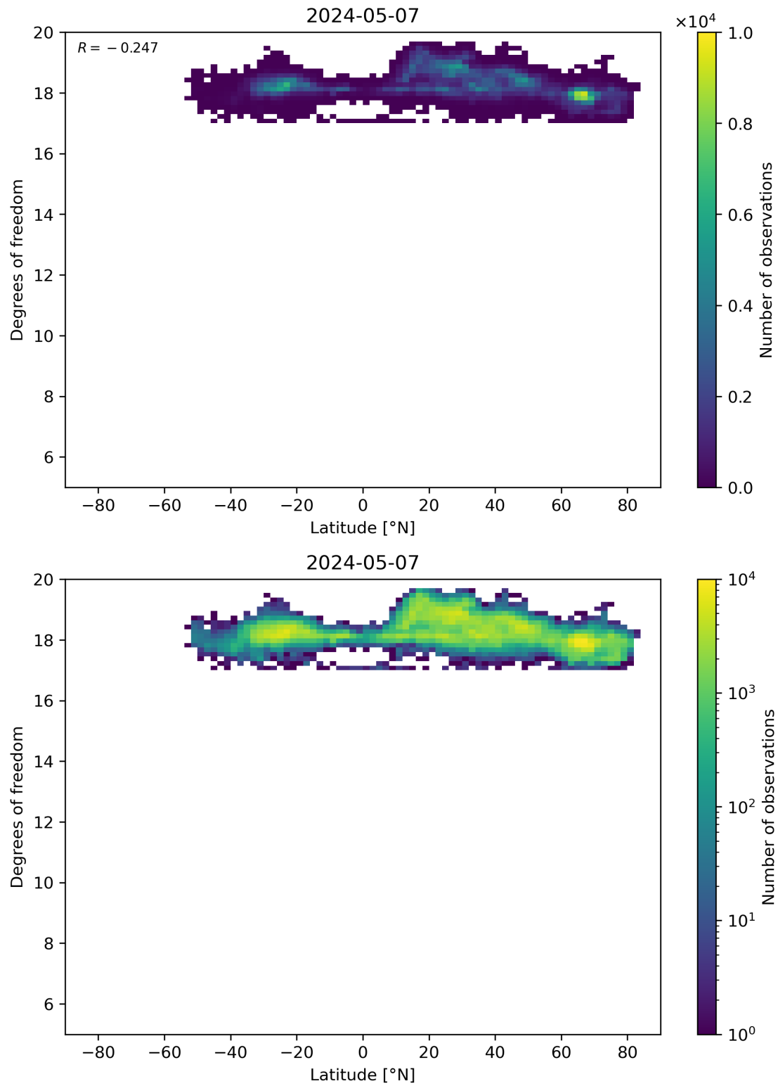
Figure 55: Scatter density plot of “Latitude” against “Degrees of freedom” for 2024-05-07 to 2024-05-08.
