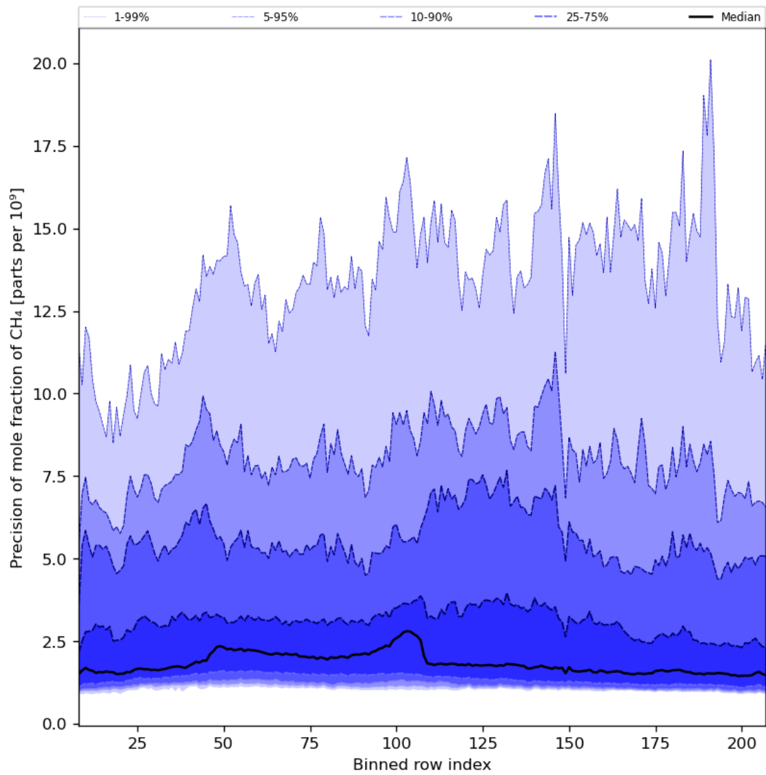
Figure 35: Along track statistics of “Precision of mole fraction of CH 4 ” for 2024-05-07 to 2024-05-08
