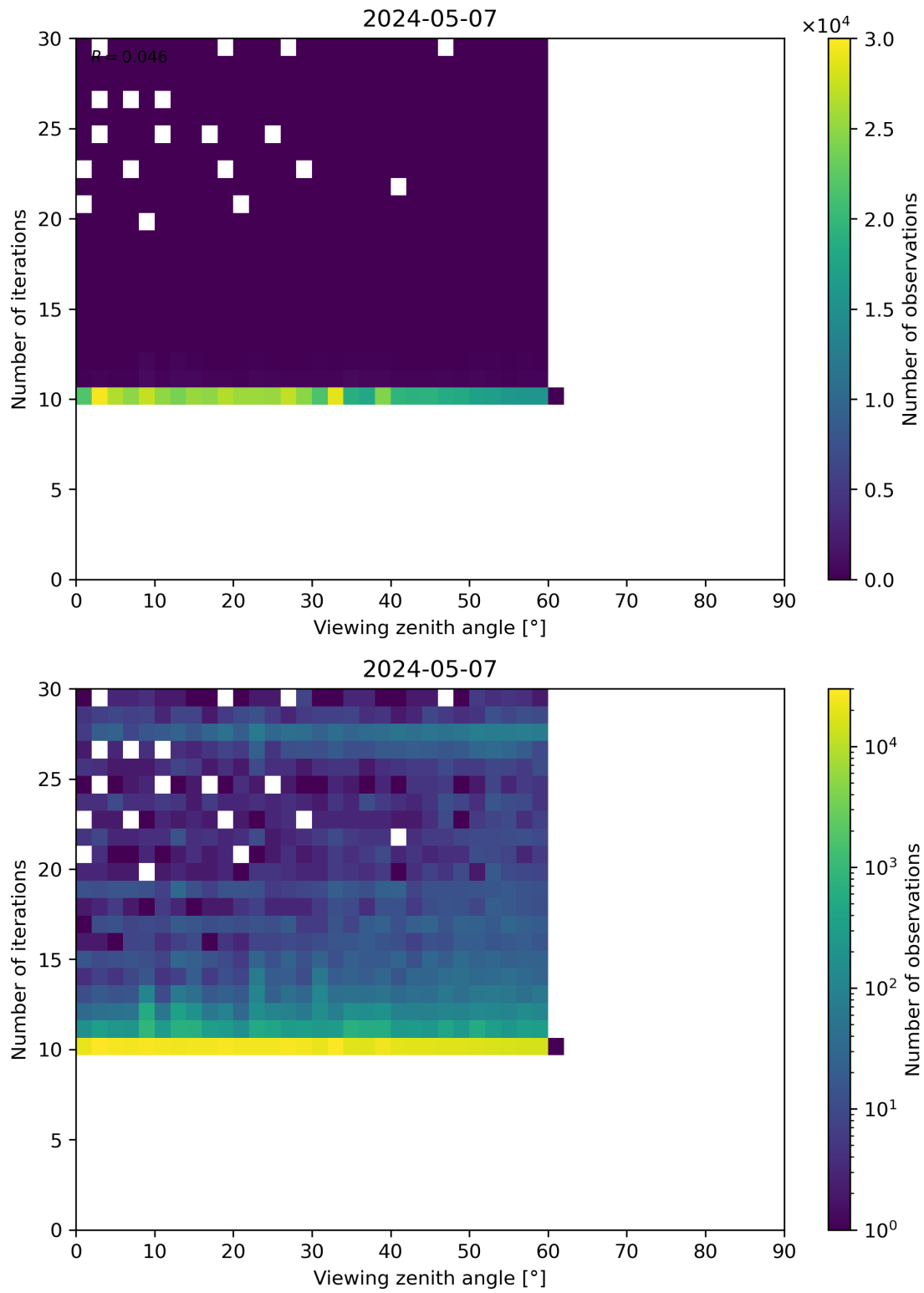
Figure 113: Scatter density plot of “Viewing zenith angle” against “Number of iterations” for 2024-05-07 to 2024-05-08.
