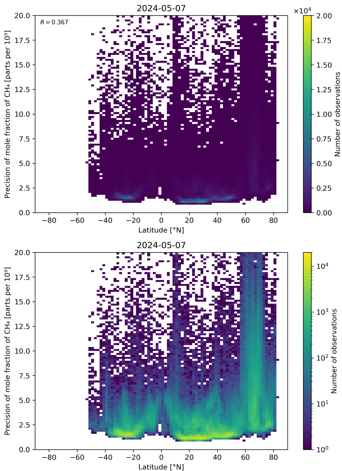
Figure 59: Scatter density plot of “Latitude” against “Precision of mole fraction of CH 4 ” for 2024-05-07 to 2024-05-08.
