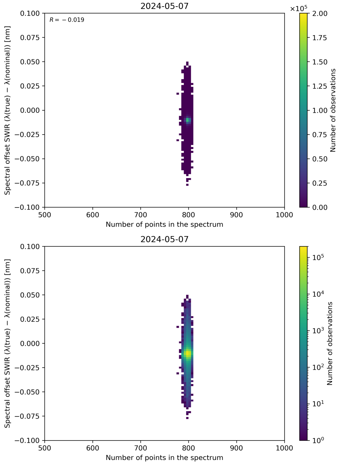
Figure 93: Scatter density plot of “Number of points in the spectrum” against “Spectral offset SWIR ( \lambda(\text{true}) - \lambda(\text{nominal}) )” for 2024-05-07 to 2024-05-08.
