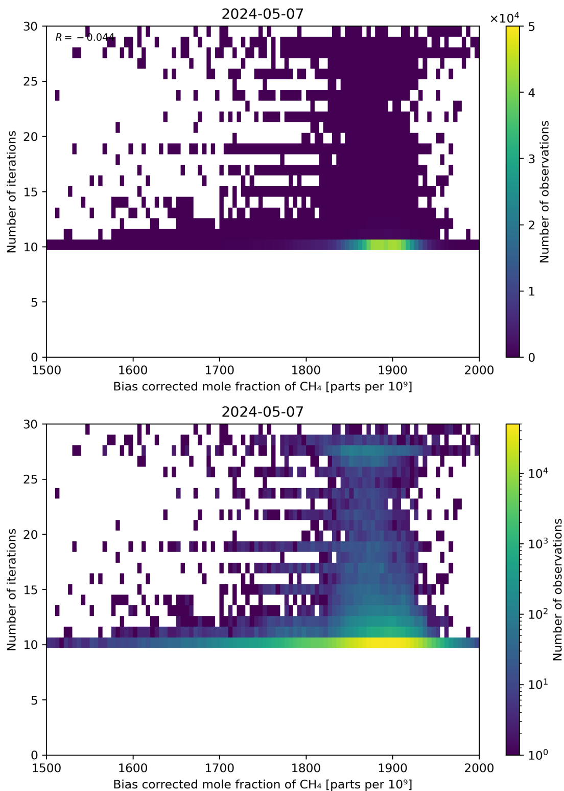
Figure 67: Scatter density plot of “Bias corrected mole fraction of CH 4 ” against “Number of iterations” for 2024-05-07 to 2024-05-08.
