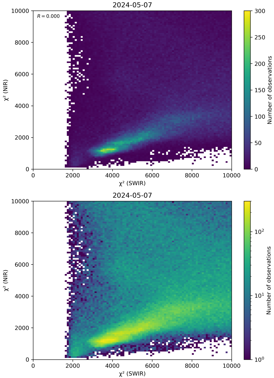
Figure 47: Scatter density plot of “ \chi^2 (SWIR)” against “ \chi^2 (NIR)” for 2024-05-07 to 2024-05-08.
