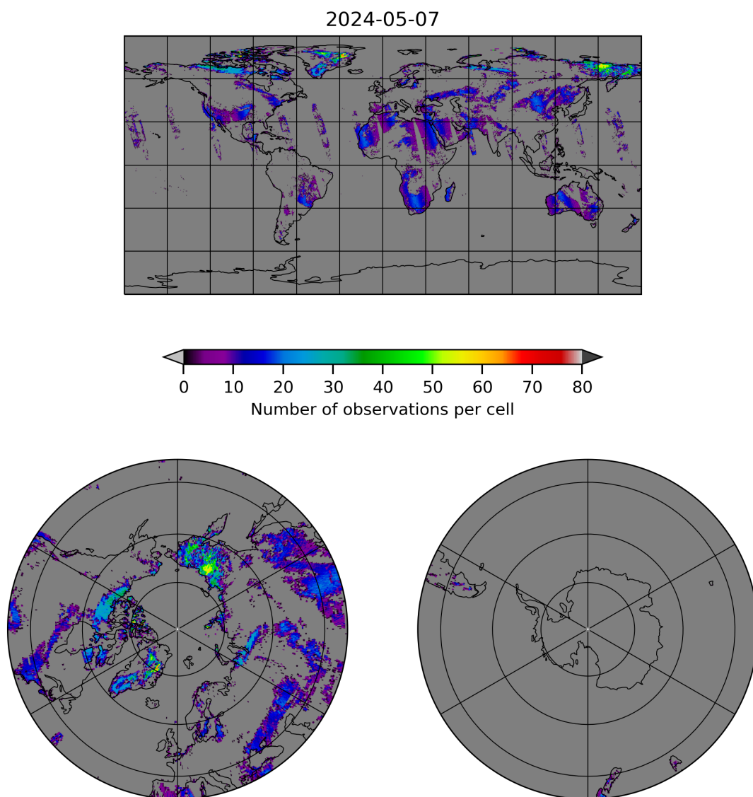
Figure 10: Map of the number of observations for 2024-05-07 to 2024-05-08
