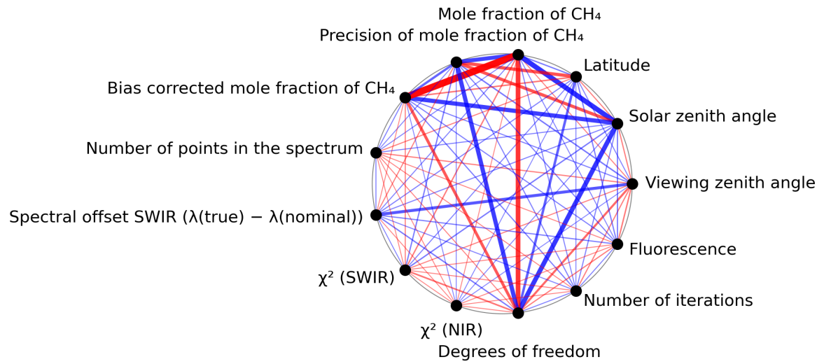
Figure 1: Map of correlation graph for 2024-05-07 to 2024-05-08.
