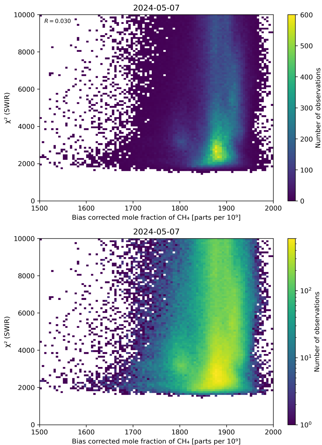
Figure 64: Scatter density plot of “Bias corrected mole fraction of \text{CH}_4 ” against “ \chi^2 (SWIR)” for 2024-05-07 to 2024-05-08.
