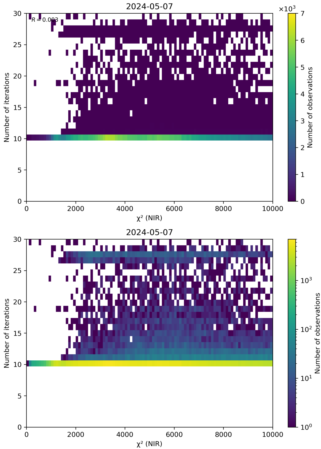
Figure 46: Scatter density plot of “ \chi^2 (NIR)” against “Number of iterations” for 2024-05-07 to 2024-05-08.
