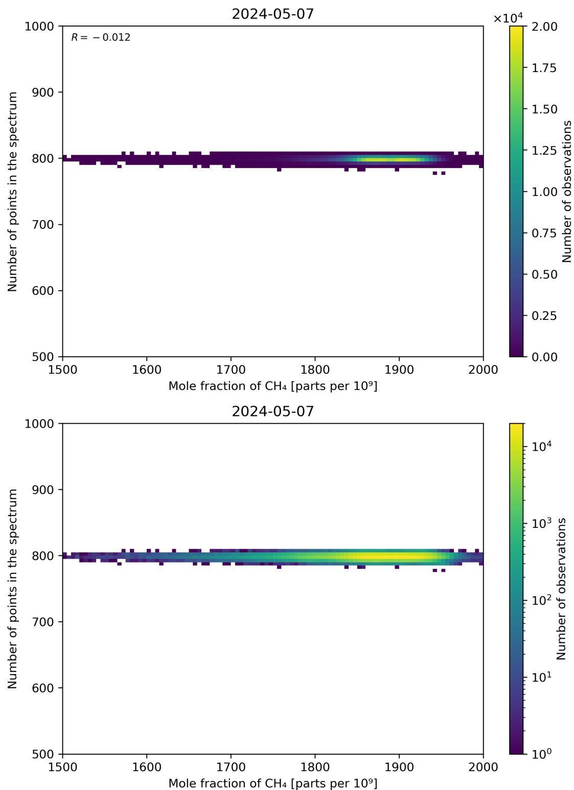
Figure 77: Scatter density plot of “Mole fraction of CH 4 ” against “Number of points in the spectrum” for 2024-05-07 to 2024-05-08.
