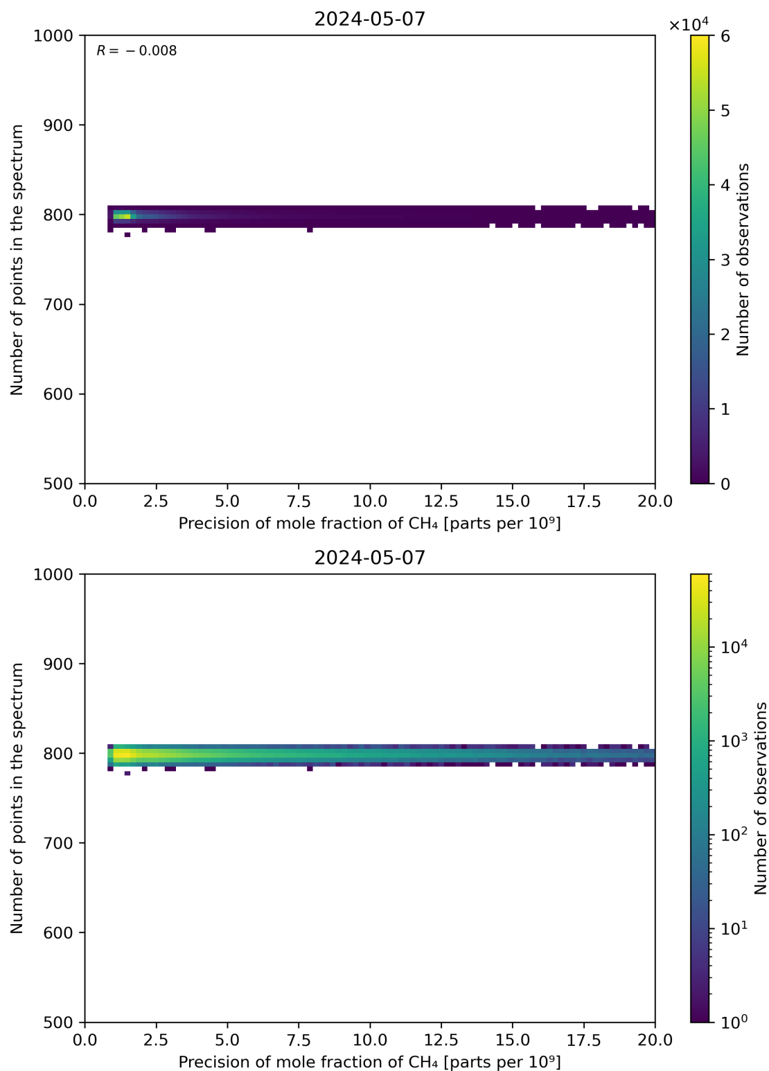
Figure 84: Scatter density plot of “Precision of mole fraction of CH 4 ” against “Number of points in the spectrum” for 2024-05-07 to 2024-05-08.
