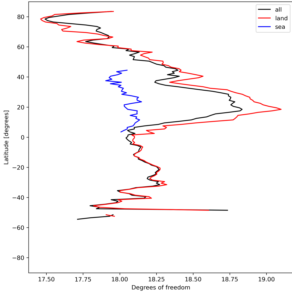
Figure 19: Zonal average of “Degrees of freedom” for 2024-05-08 to 2024-05-10.
