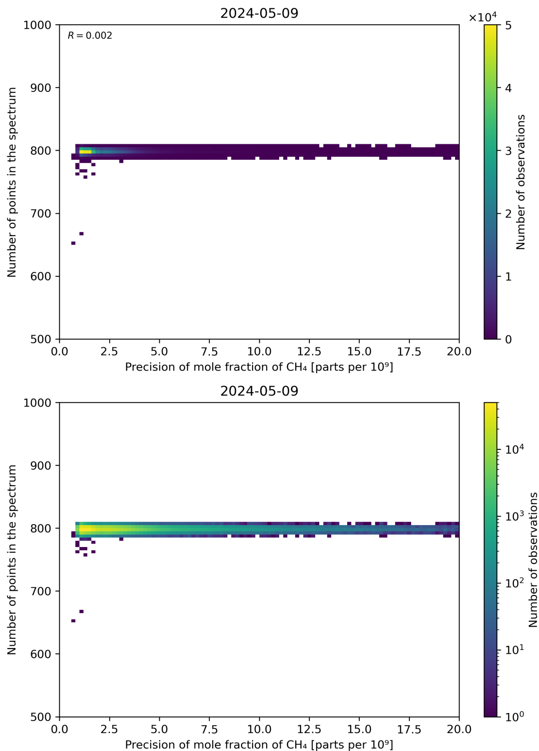
Figure 84: Scatter density plot of “Precision of mole fraction of CH 4 ” against “Number of points in the spectrum” for 2024-05-08 to 2024-05-10.
