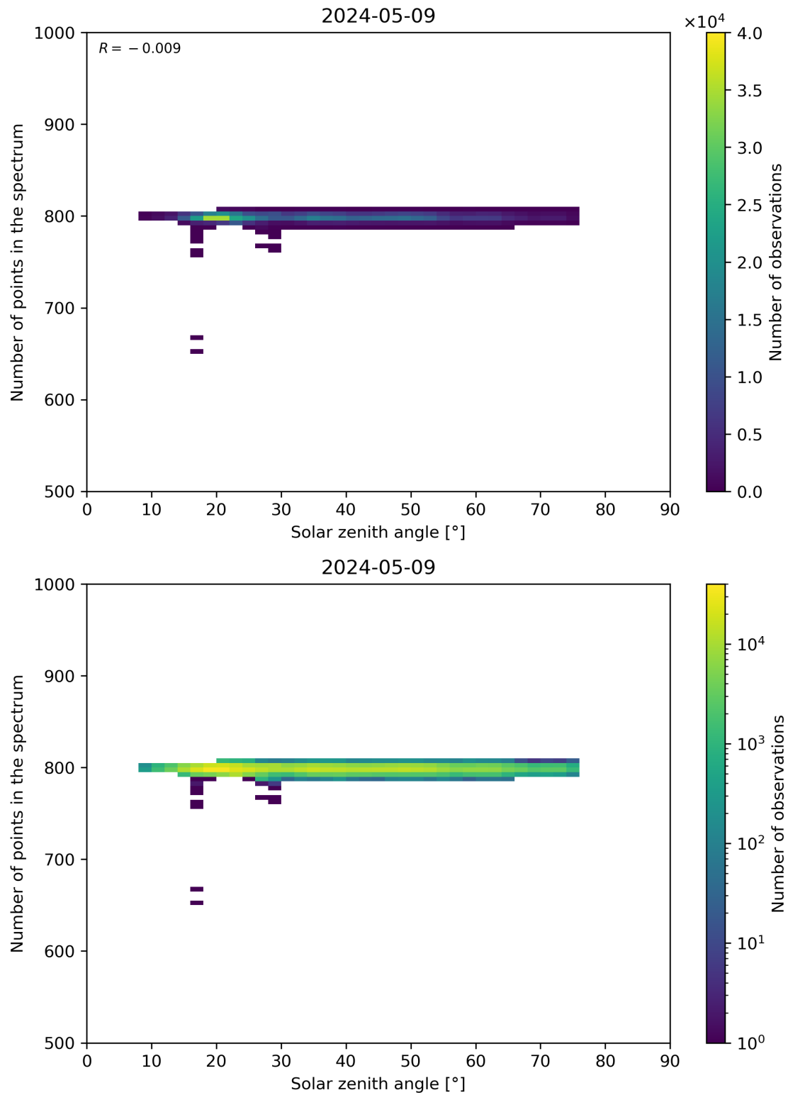
Figure 103: Scatter density plot of “Solar zenith angle” against “Number of points in the spectrum” for 2024-05-08 to 2024-05-10.
