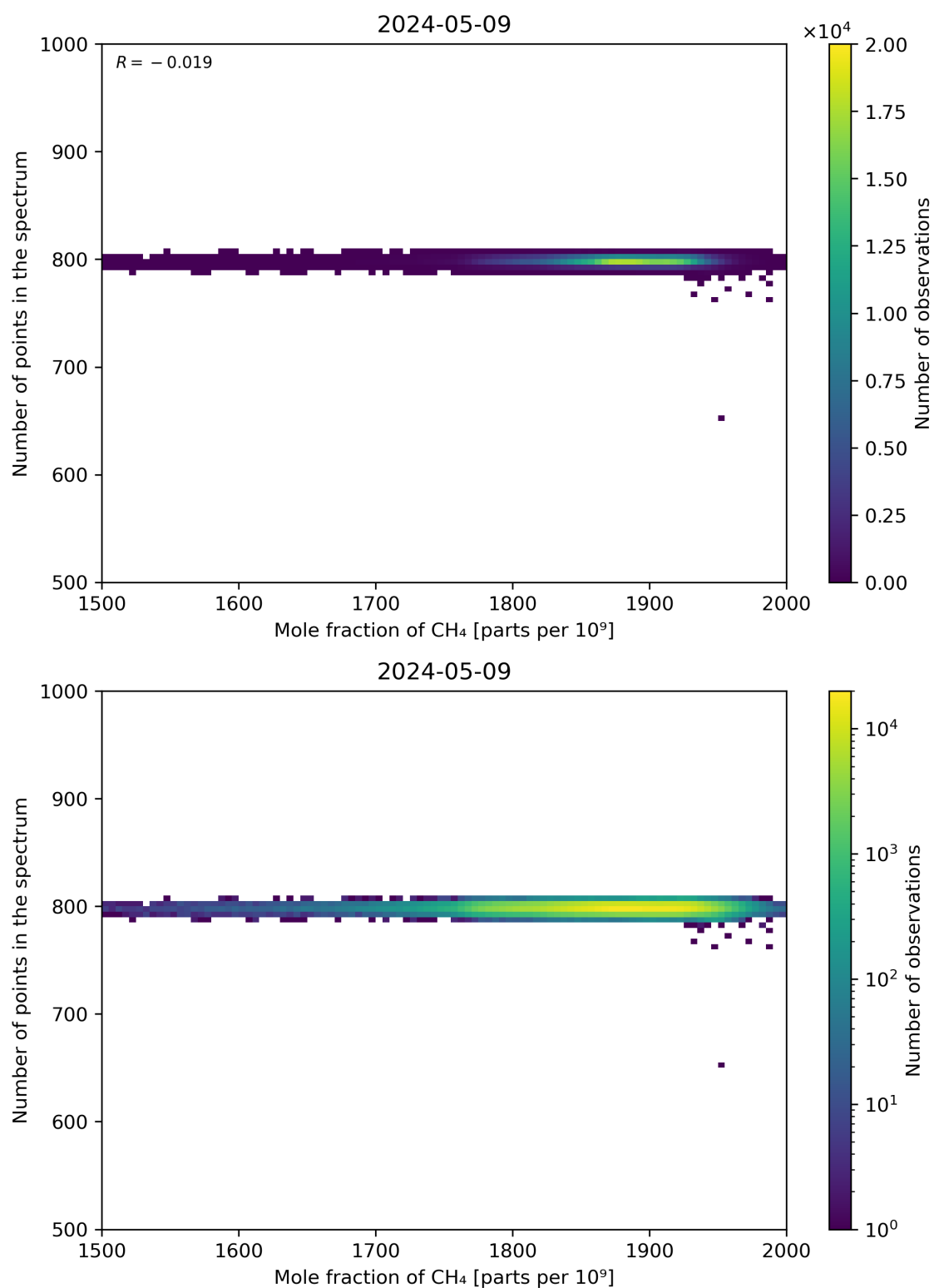
Figure 77: Scatter density plot of “Mole fraction of CH 4 ” against “Number of points in the spectrum” for 2024-05-08 to 2024-05-10.
