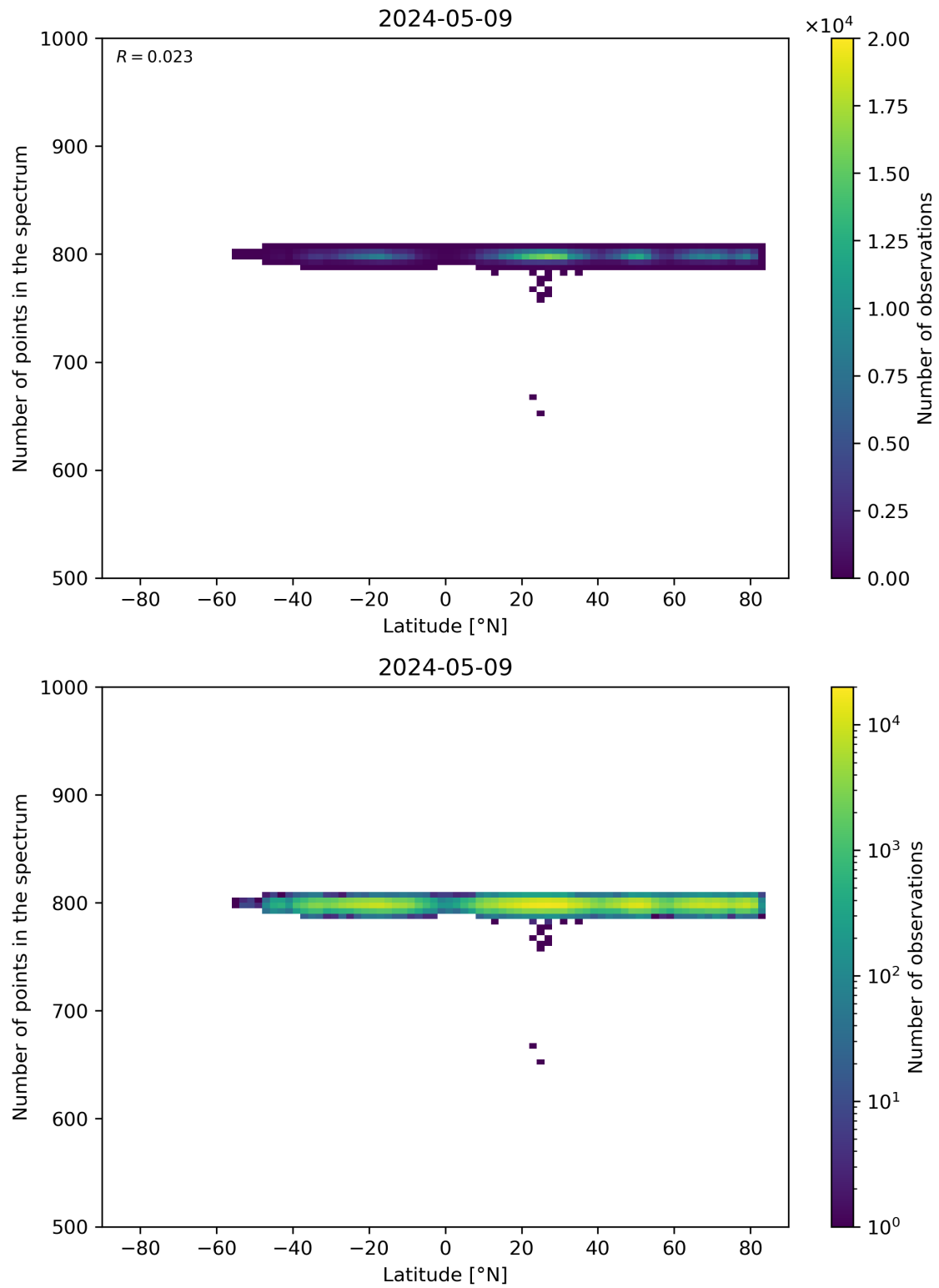
Figure 61: Scatter density plot of “Latitude” against “Number of points in the spectrum” for 2024-05-08 to 2024-05-10.
