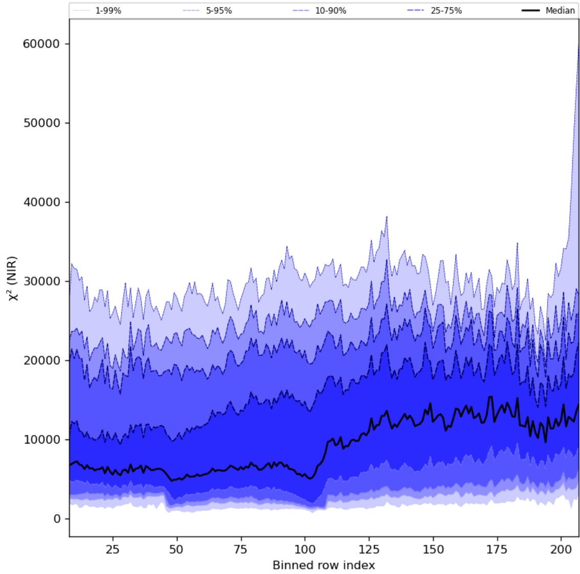
Figure 40: Along track statistics of “ \chi^2 (NIR)” for 2024-05-08 to 2024-05-10
