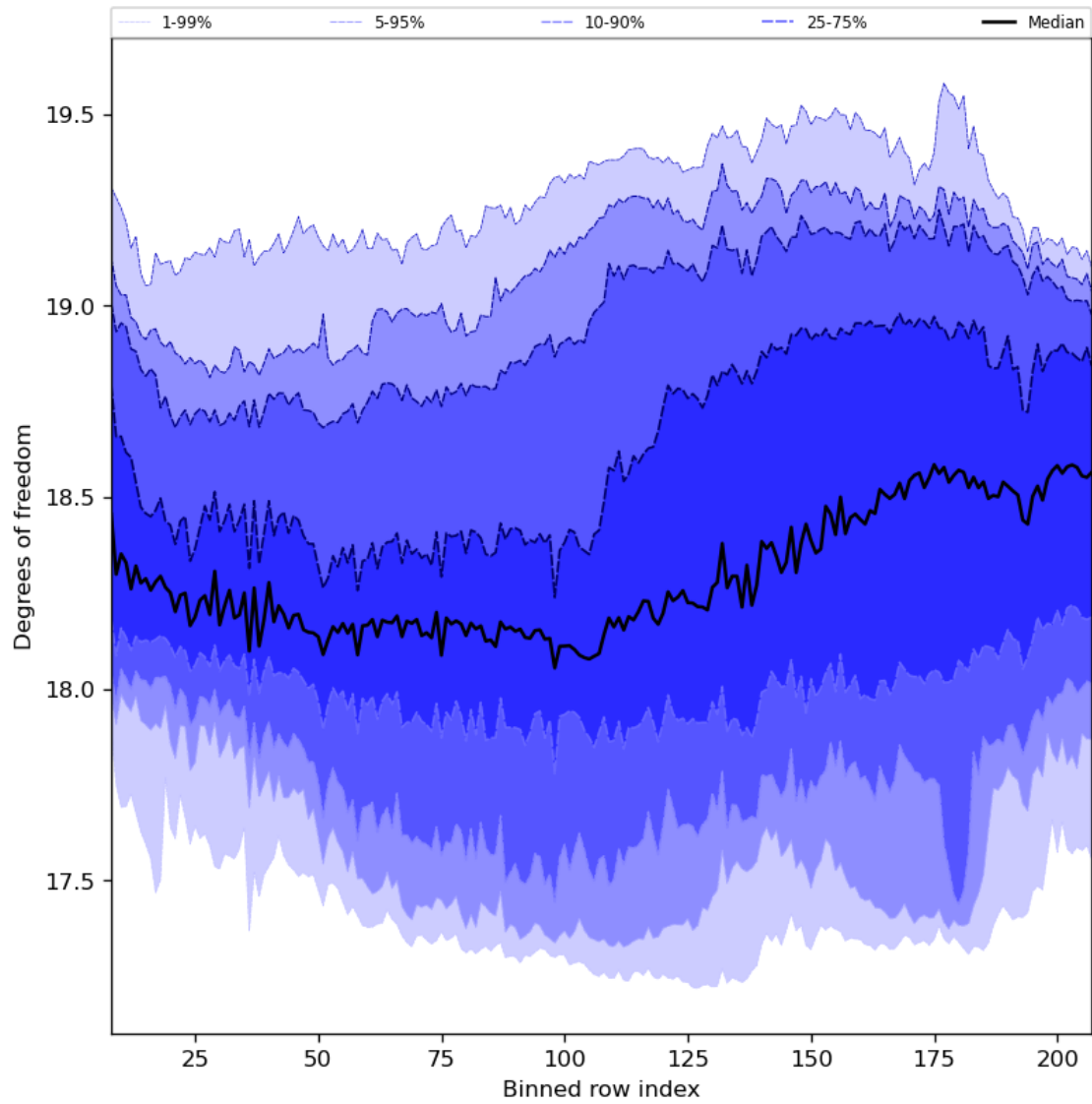
Figure 41: Along track statistics of “Degrees of freedom” for 2024-05-08 to 2024-05-10
