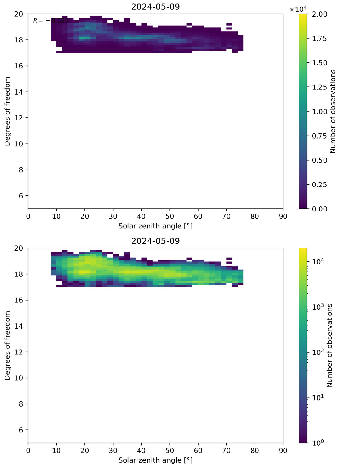
Figure 96: Scatter density plot of “Solar zenith angle” against “Degrees of freedom” for 2024-05-08 to 2024-05-10.
