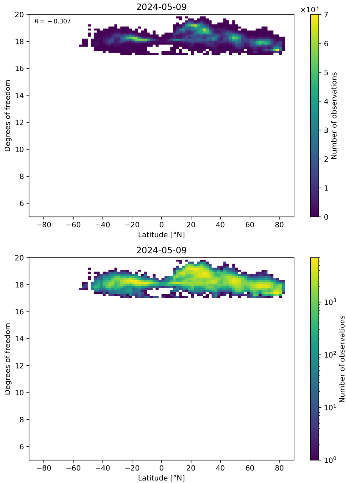
Figure 55: Scatter density plot of “Latitude” against “Degrees of freedom” for 2024-05-08 to 2024-05-10.
