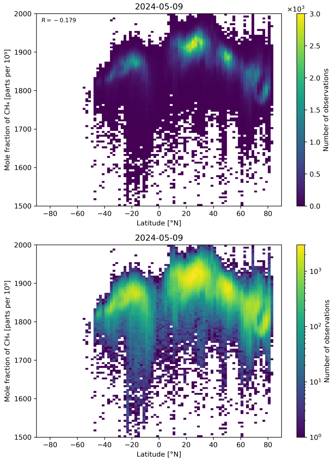
Figure 57: Scatter density plot of “Latitude” against “Mole fraction of CH 4 ” for 2024-05-08 to 2024-05-10.
