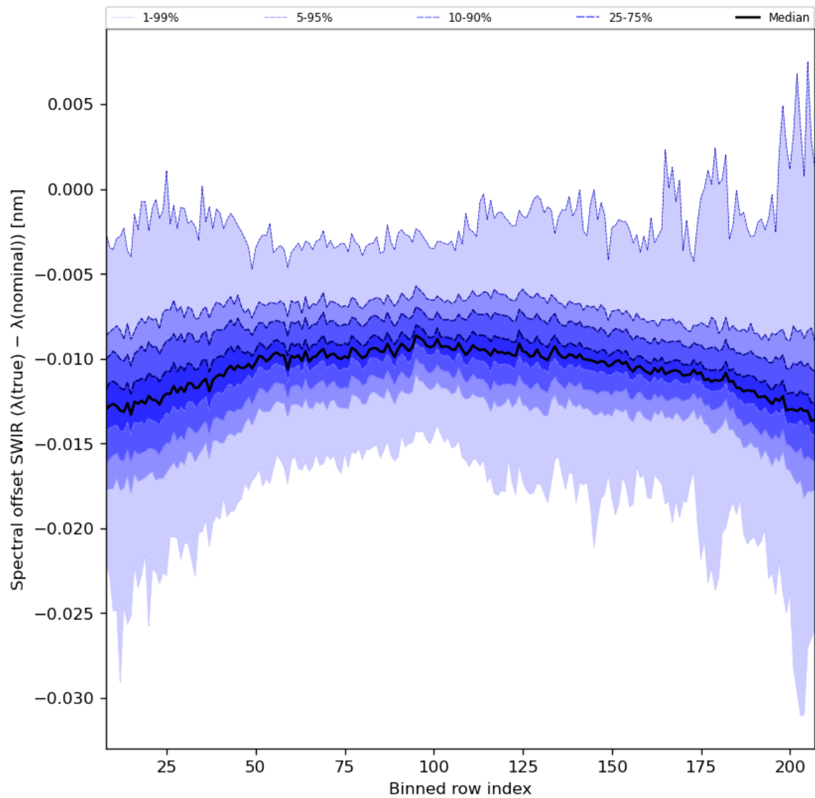
Figure 38: Along track statistics of “Spectral offset SWIR ( \lambda(\text{true}) - \lambda(\text{nominal}) )” for 2024-05-08 to 2024-05-10
