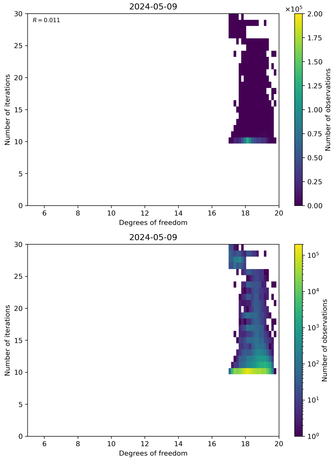
Figure 52: Scatter density plot of “Degrees of freedom” against “Number of iterations” for 2024-05-08 to 2024-05-10.
