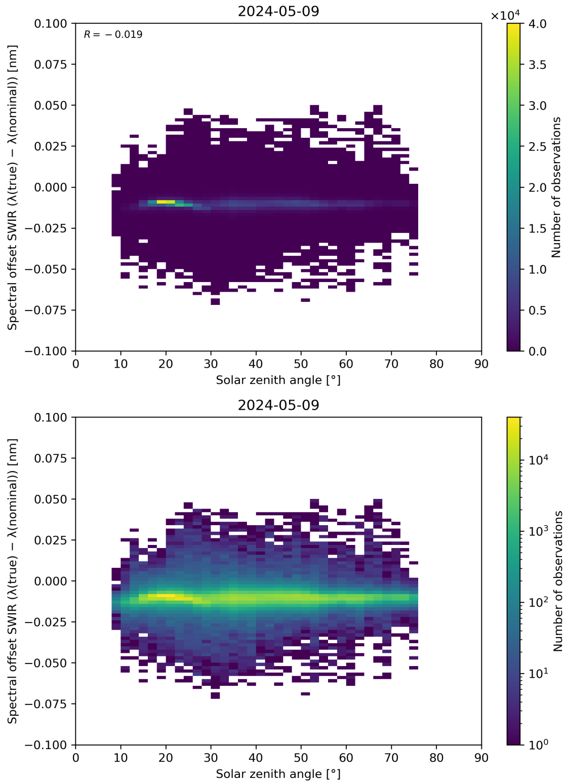
Figure 104: Scatter density plot of “Solar zenith angle” against “Spectral offset SWIR ( \lambda(\text{true}) - \lambda(\text{nominal}) )” for 2024-05-08 to 2024-05-10.
