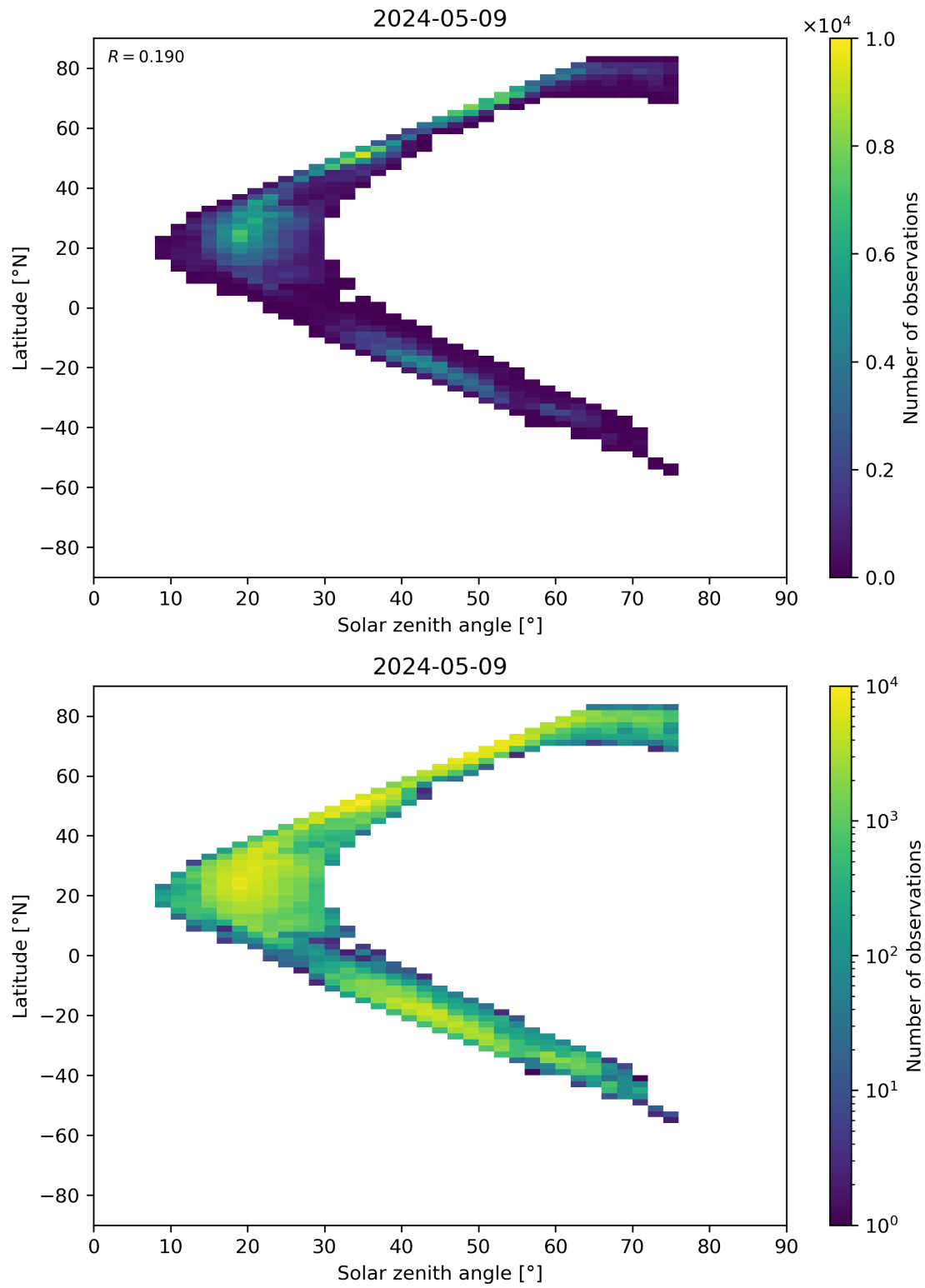
Figure 98: Scatter density plot of “Solar zenith angle” against “Latitude” for 2024-05-08 to 2024-05-10.
