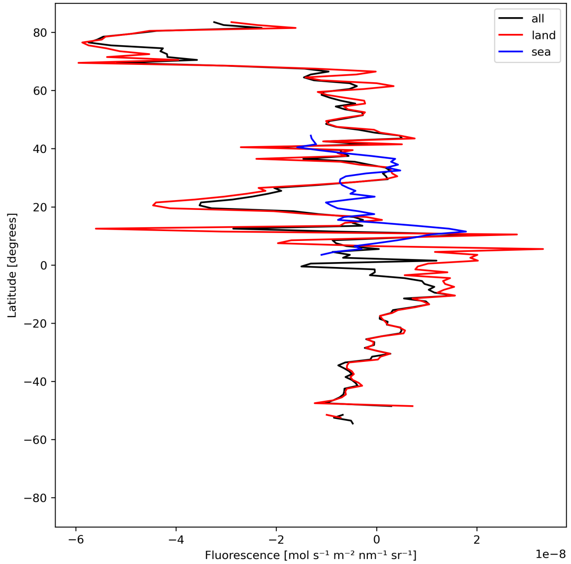
Figure 21: Zonal average of “Fluorescence” for 2024-05-08 to 2024-05-10.
