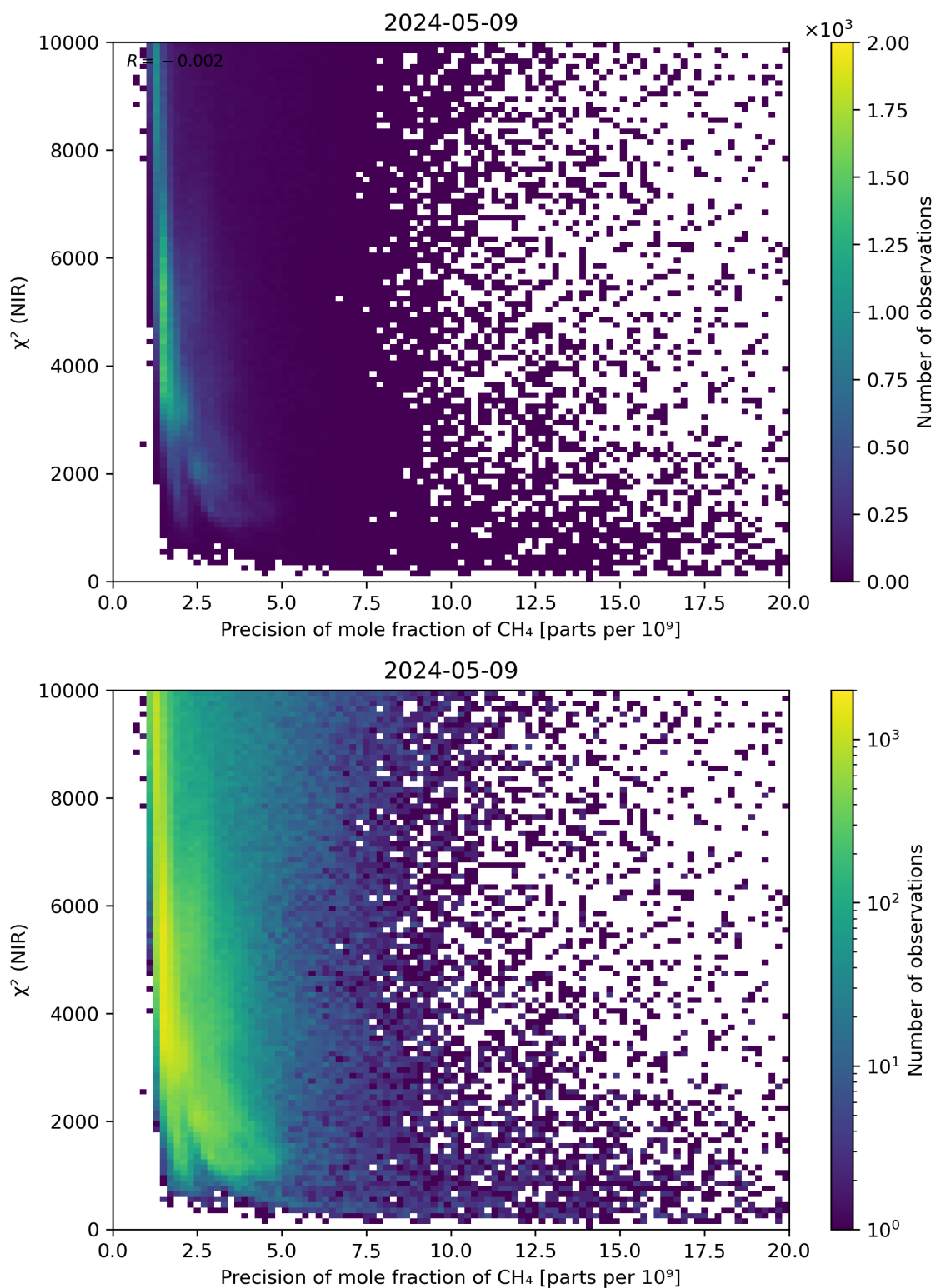
Figure 78: Scatter density plot of “Precision of mole fraction of CH 4 ” against “ \chi^2 (NIR)” for 2024-05-08 to 2024-05-10.
