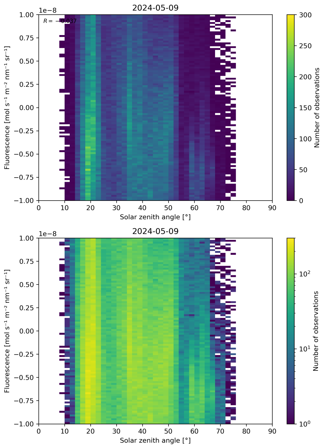
Figure 97: Scatter density plot of “Solar zenith angle” against “Fluorescence” for 2024-05-08 to 2024-05-10.
