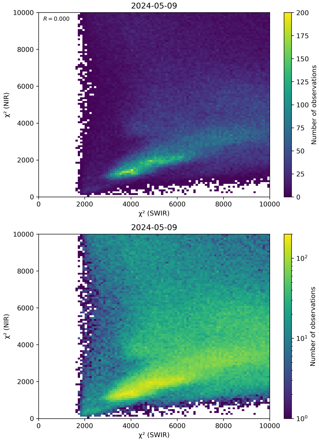
Figure 47: Scatter density plot of “ \chi^2 (SWIR)” against “ \chi^2 (NIR)” for 2024-05-08 to 2024-05-10.
