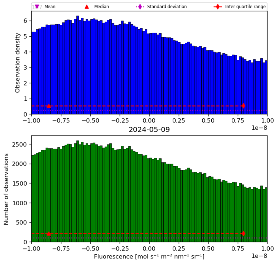
Figure 32: Histogram of “Fluorescence” for 2024-05-08 to 2024-05-10
