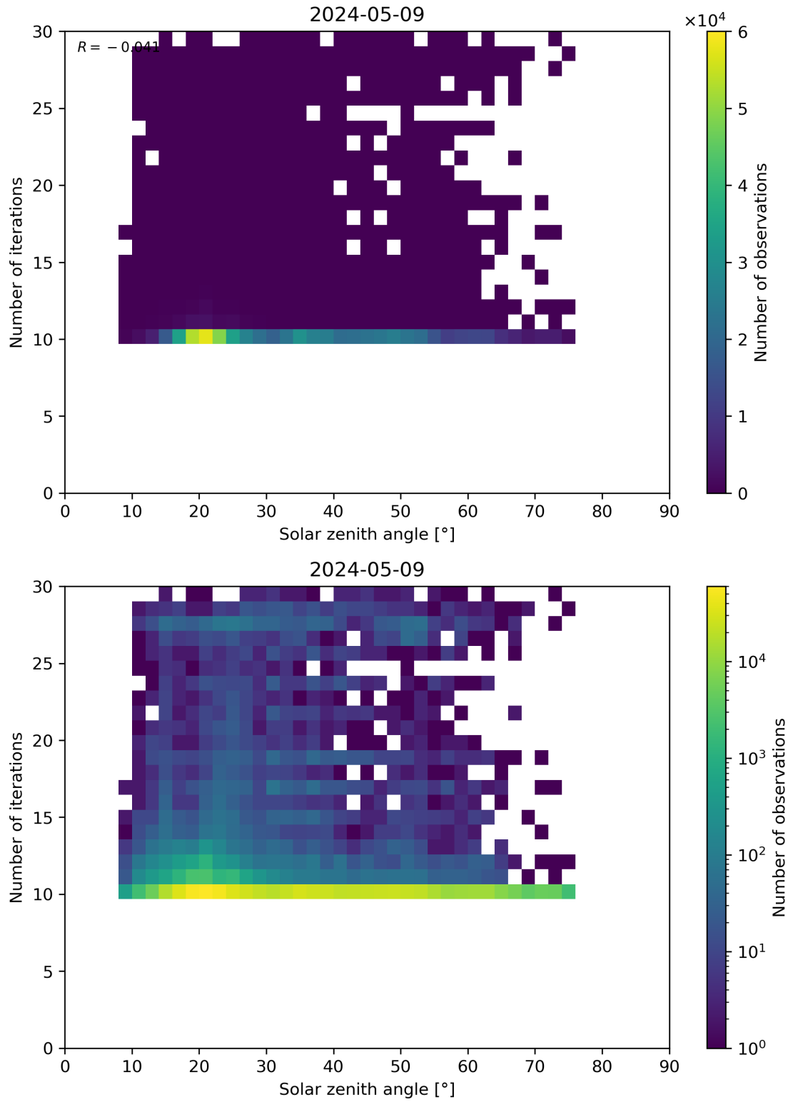
Figure 102: Scatter density plot of “Solar zenith angle” against “Number of iterations” for 2024-05-08 to 2024-05-10.
