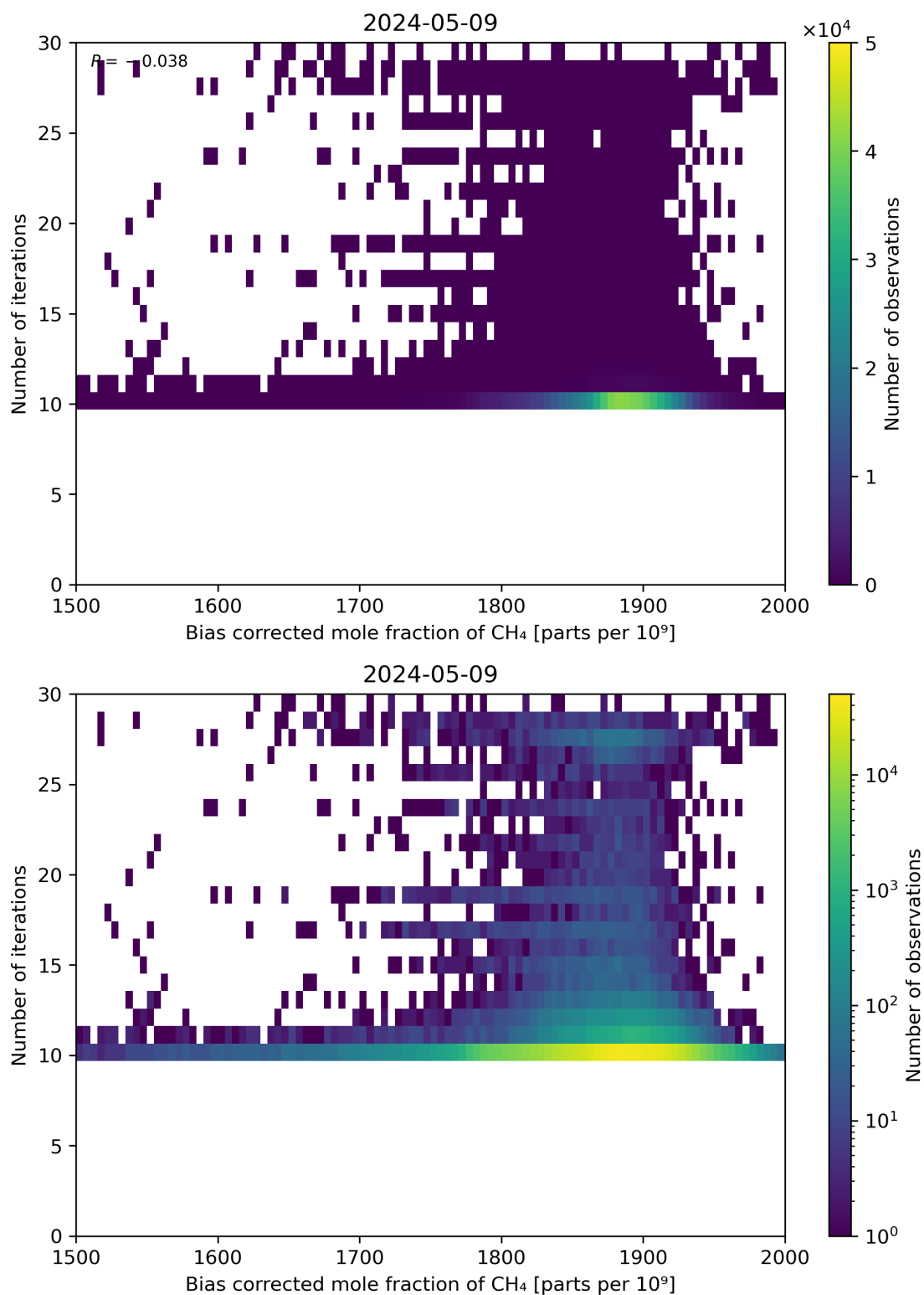
Figure 67: Scatter density plot of “Bias corrected mole fraction of CH 4 ” against “Number of iterations” for 2024-05-08 to 2024-05-10.
