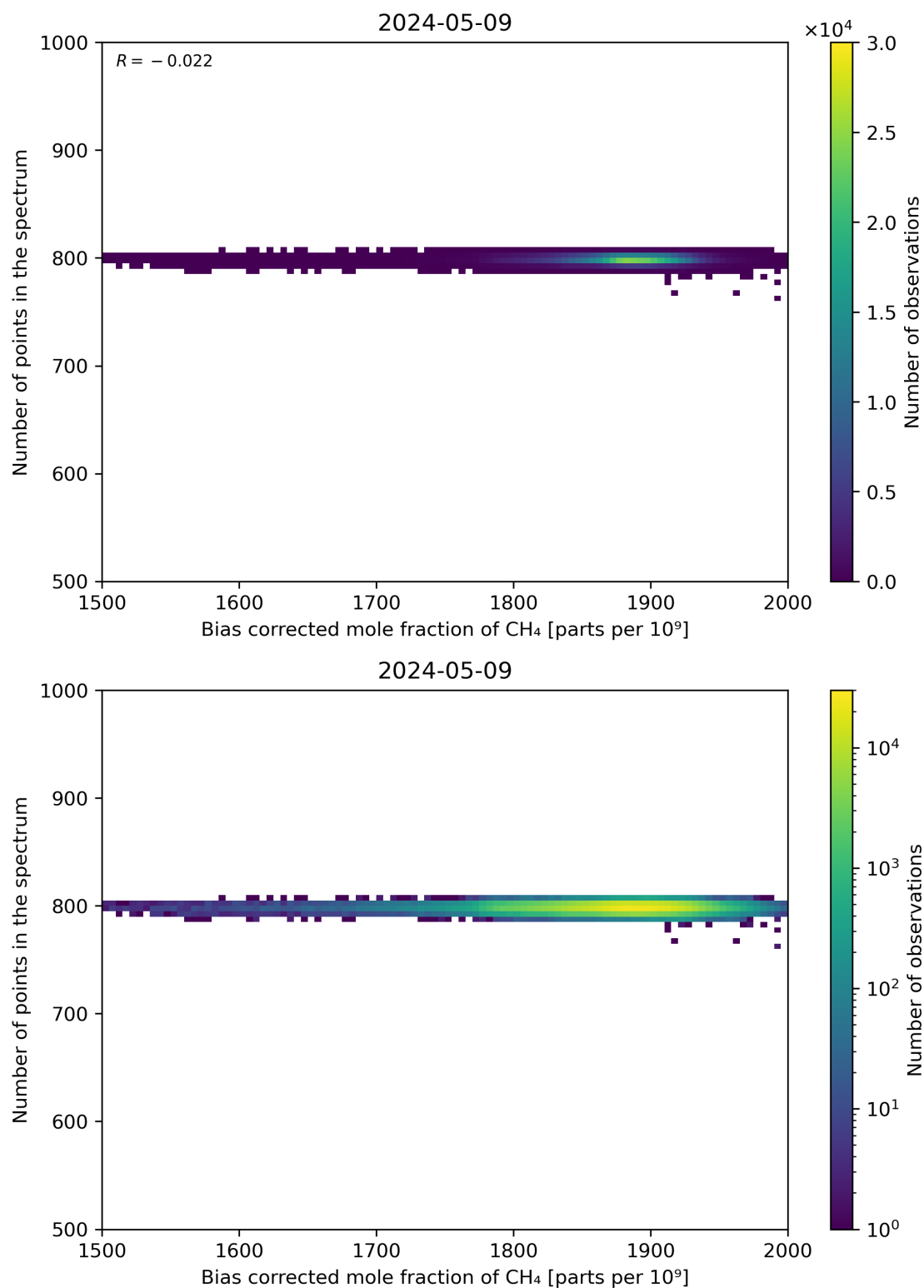
Figure 68: Scatter density plot of “Bias corrected mole fraction of CH 4 ” against “Number of points in the spectrum” for 2024-05-08 to 2024-05-10.
