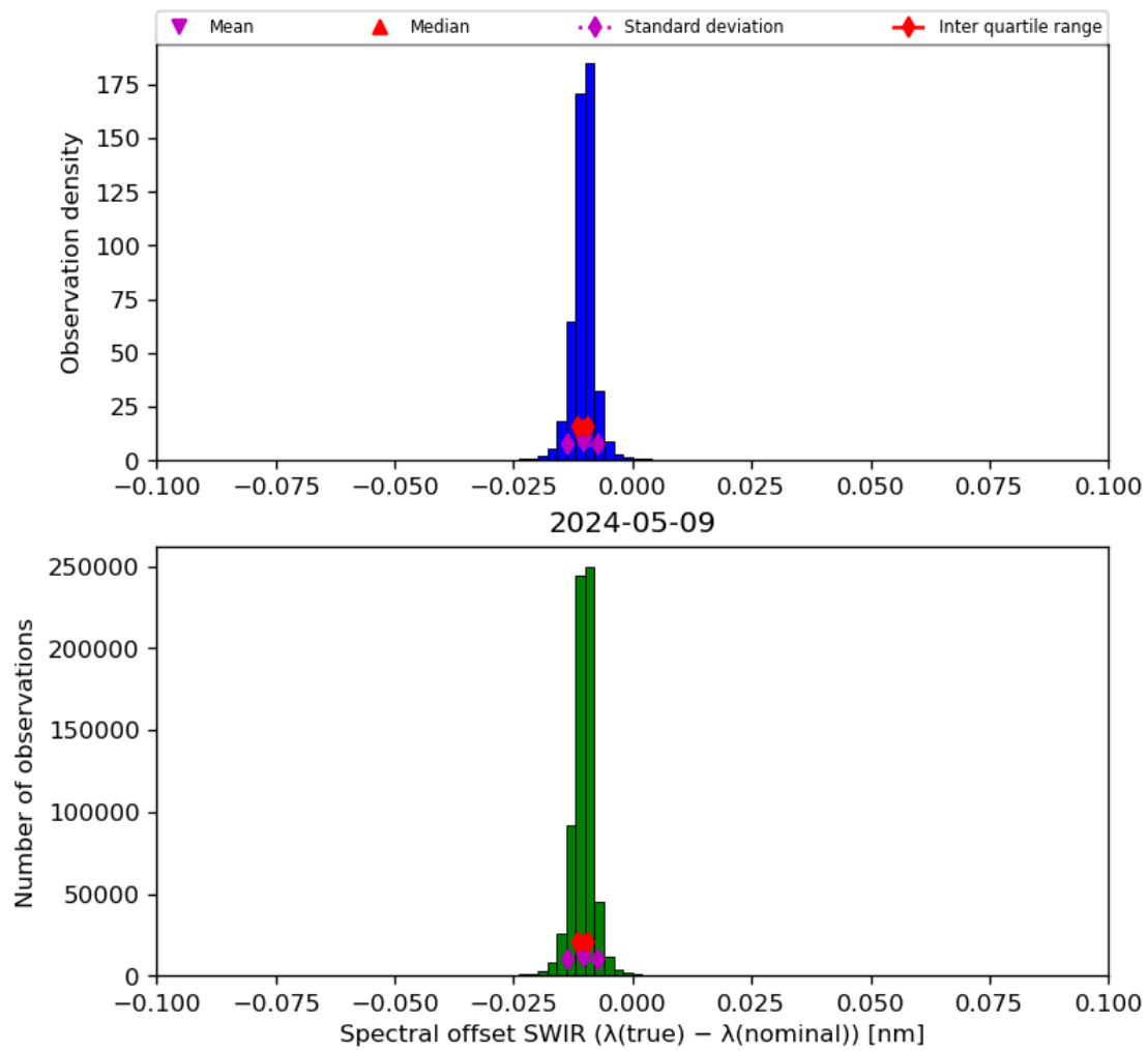
Figure 27: Histogram of “Spectral offset SWIR ( \lambda(\text{true}) - \lambda(\text{nominal}) )” for 2024-05-08 to 2024-05-10
