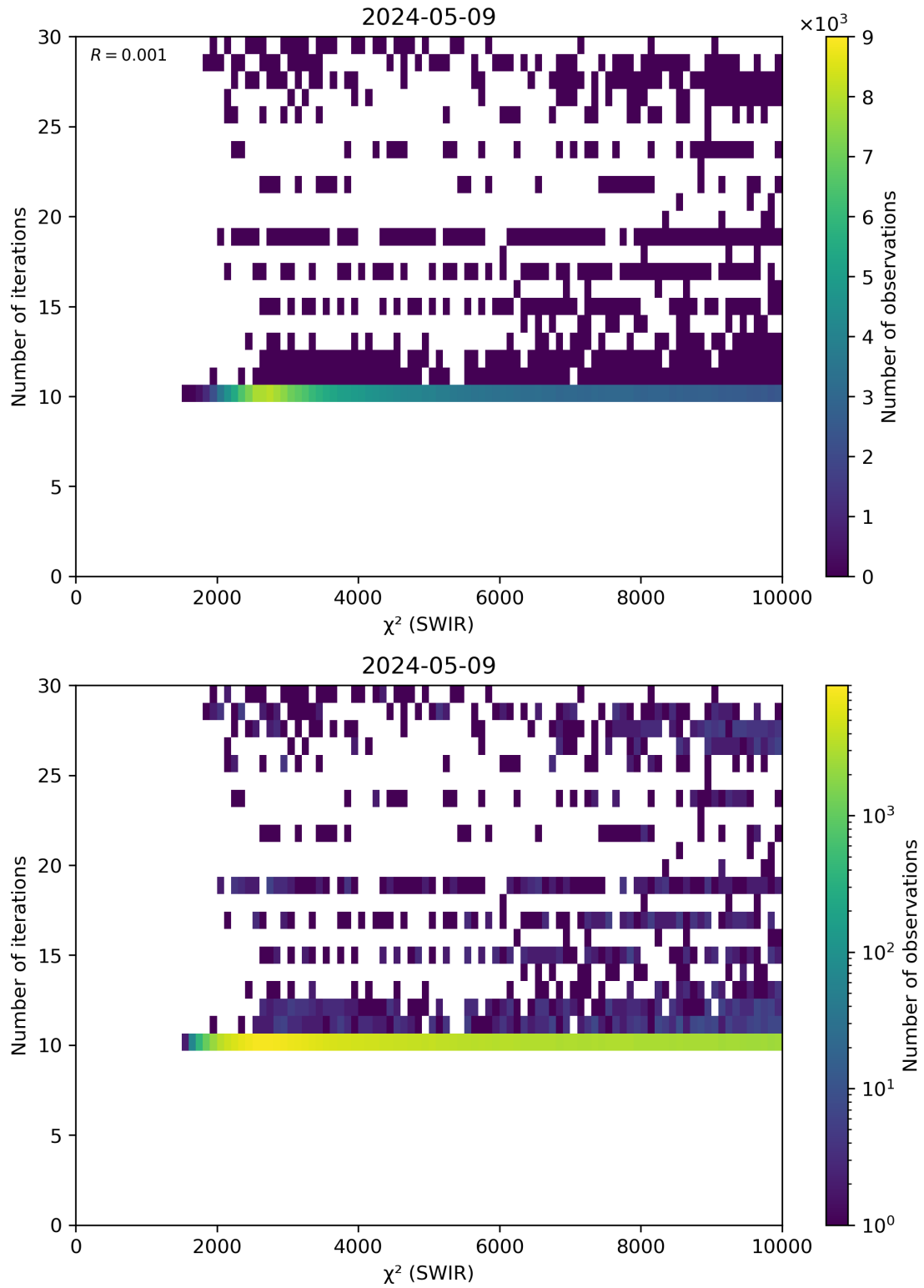
Figure 50: Scatter density plot of “ \chi^2 (SWIR)” against “Number of iterations” for 2024-05-08 to 2024-05-10.
