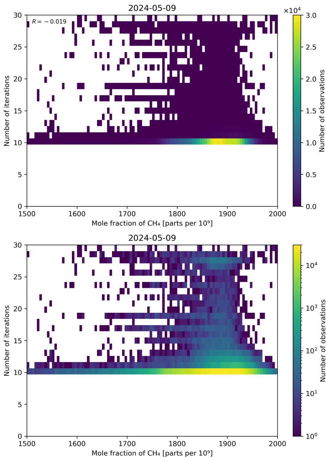
Figure 76: Scatter density plot of “Mole fraction of CH 4 ” against “Number of iterations” for 2024-05-08 to 2024-05-10.
