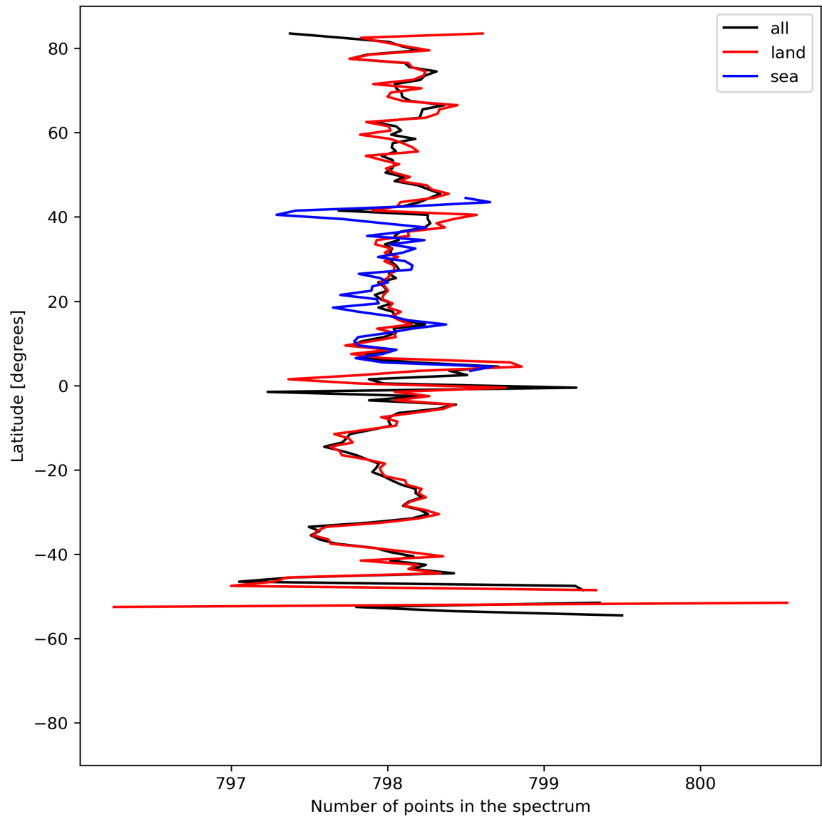
Figure 15: Zonal average of “Number of points in the spectrum” for 2024-05-08 to 2024-05-10.
