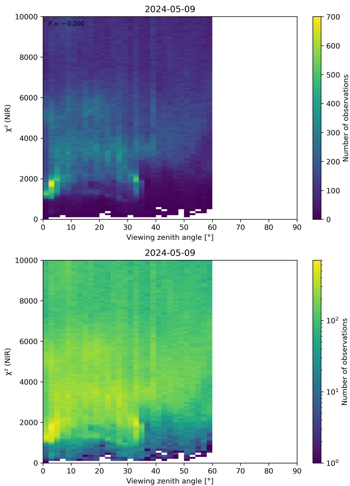
Figure 105: Scatter density plot of “Viewing zenith angle” against “ \chi^2 (NIR)” for 2024-05-08 to 2024-05-10.
