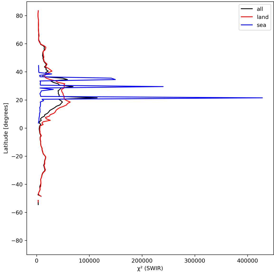
Figure 17: Zonal average of “ \chi^2 (SWIR)” for 2024-05-08 to 2024-05-10.
