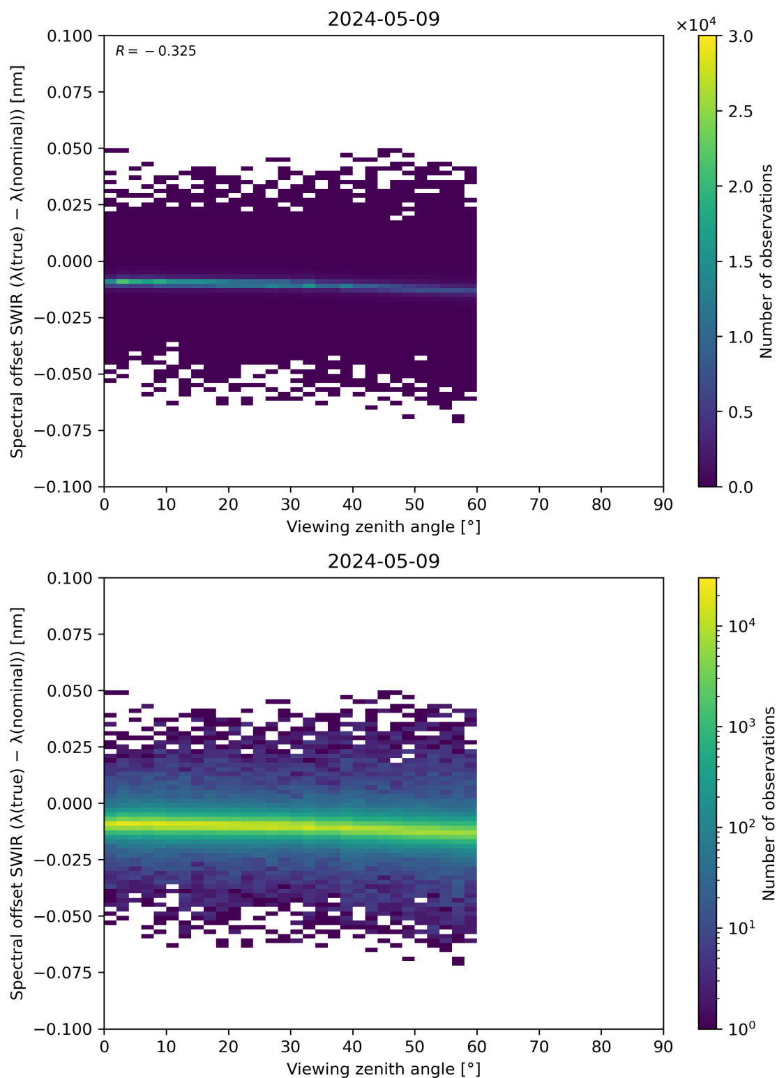
Figure 116: Scatter density plot of “Viewing zenith angle” against “Spectral offset SWIR ( \lambda(\text{true}) - \lambda(\text{nominal}) )” for 2024-05-08 to 2024-05-10.
