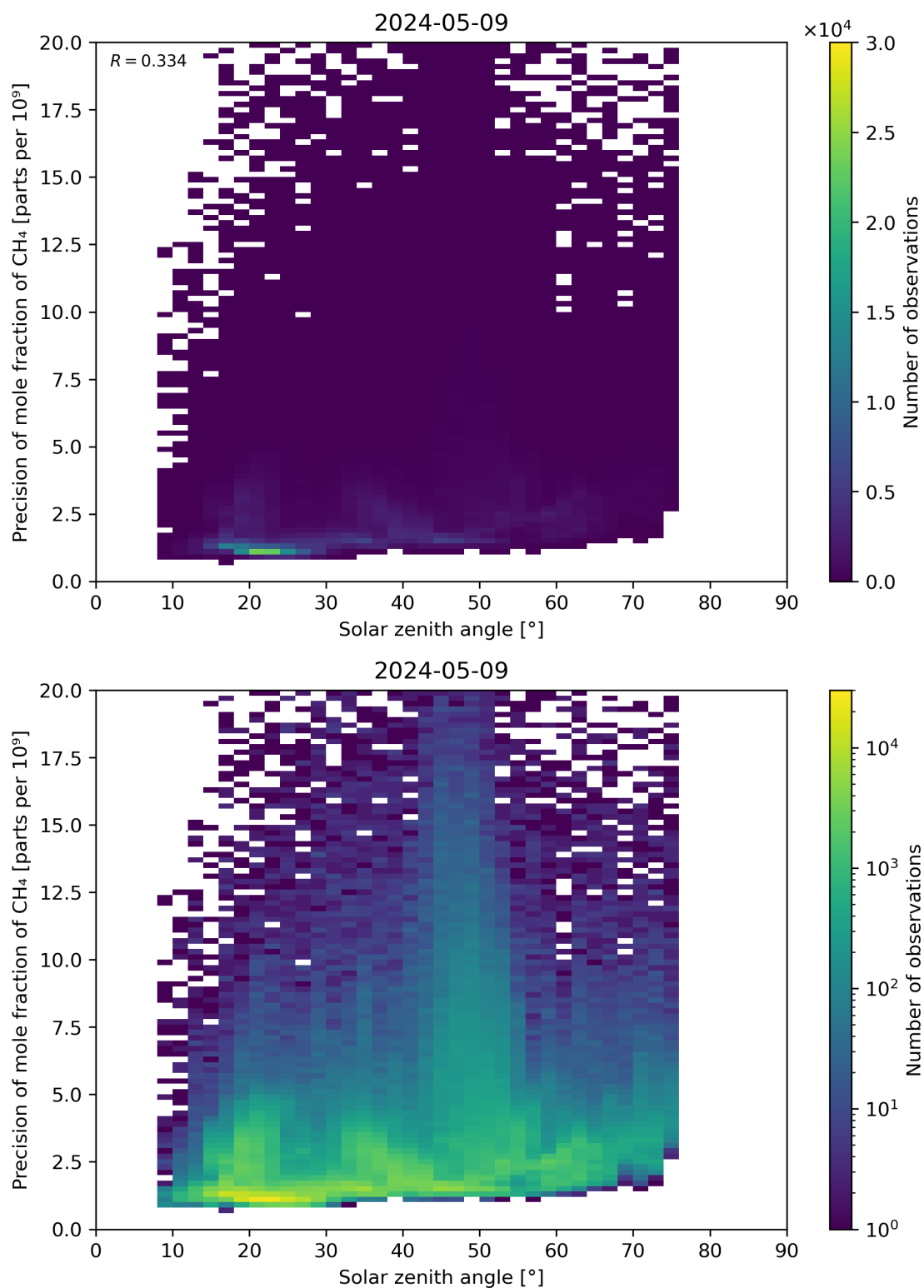
Figure 101: Scatter density plot of “Solar zenith angle” against “Precision of mole fraction of CH 4 ” for 2024-05-08 to 2024-05-10.
