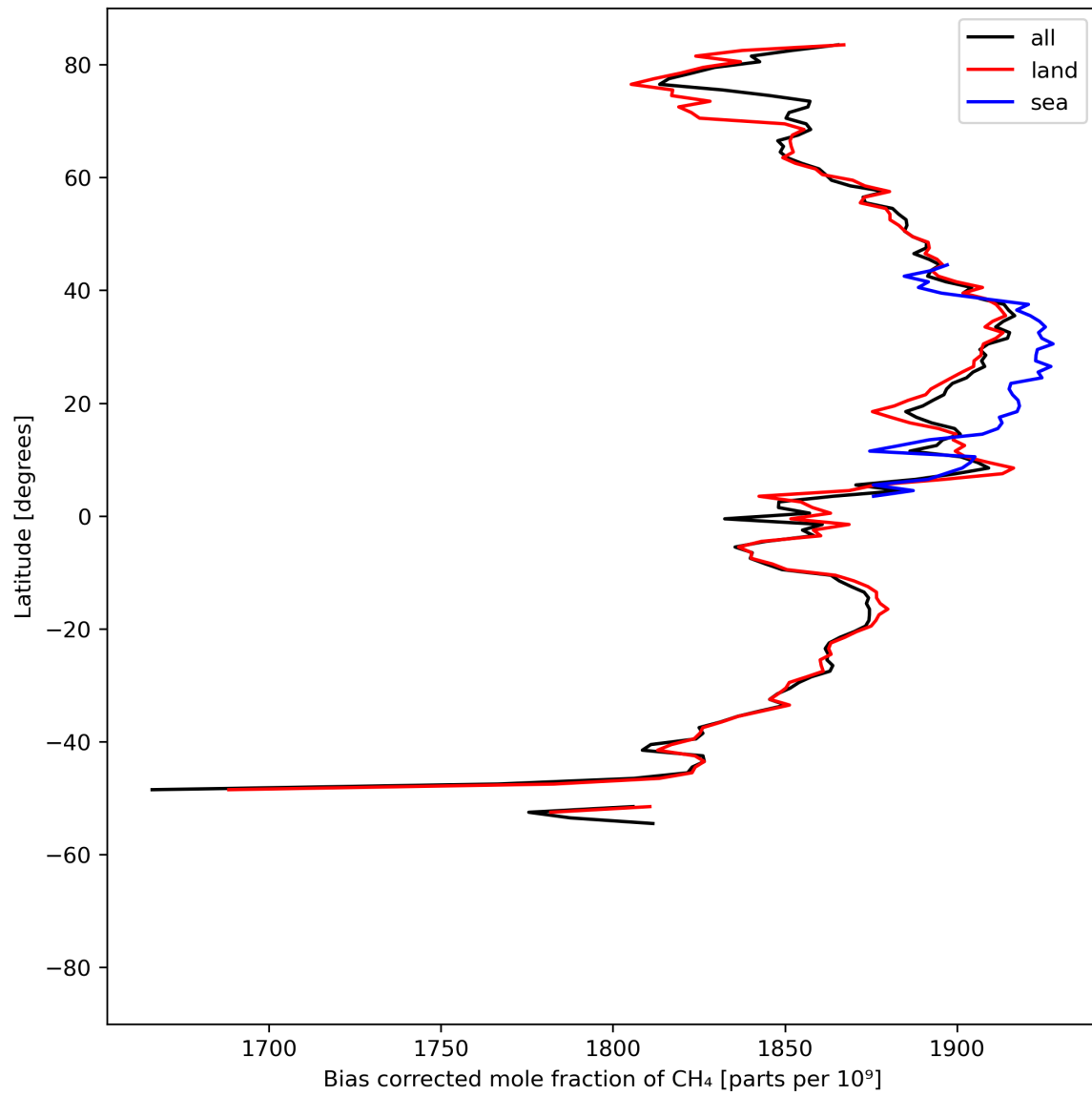
Figure 14: Zonal average of “Bias corrected mole fraction of CH 4 ” for 2024-05-08 to 2024-05-10.
