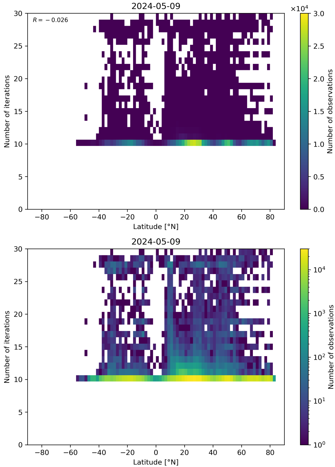
Figure 60: Scatter density plot of “Latitude” against “Number of iterations” for 2024-05-08 to 2024-05-10.
