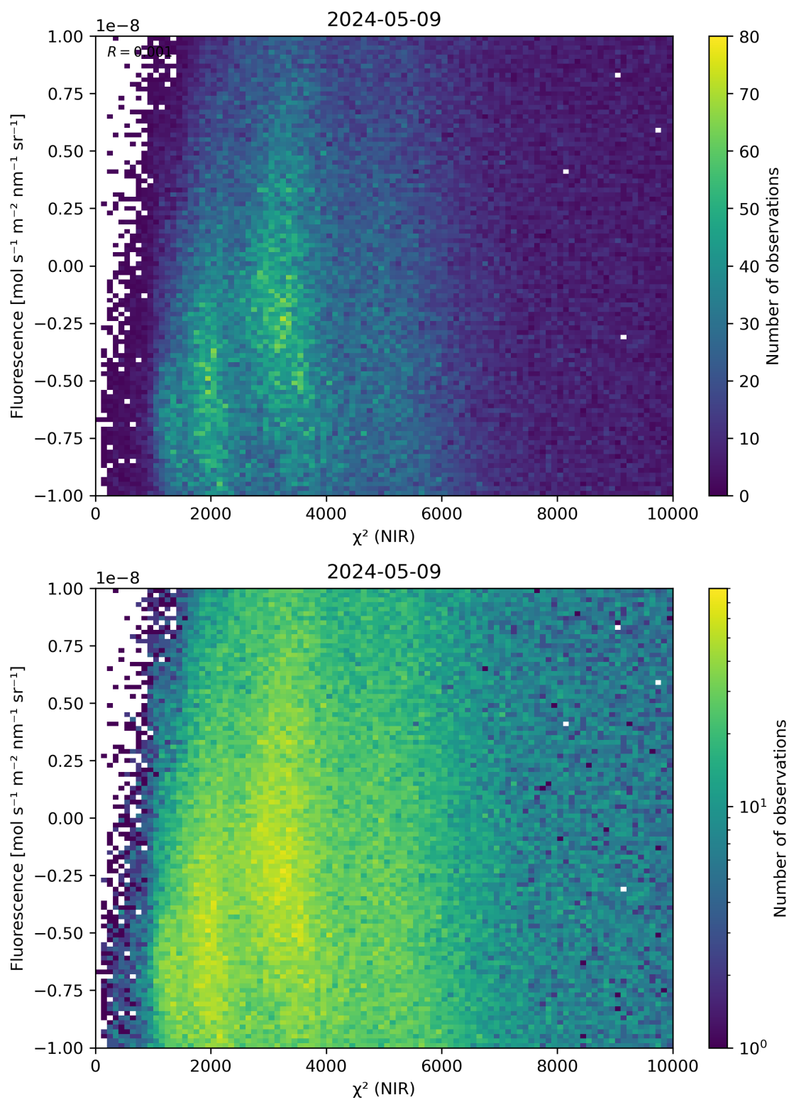
Figure 45: Scatter density plot of “ \chi^2 (NIR)” against “Fluorescence” for 2024-05-08 to 2024-05-10.
