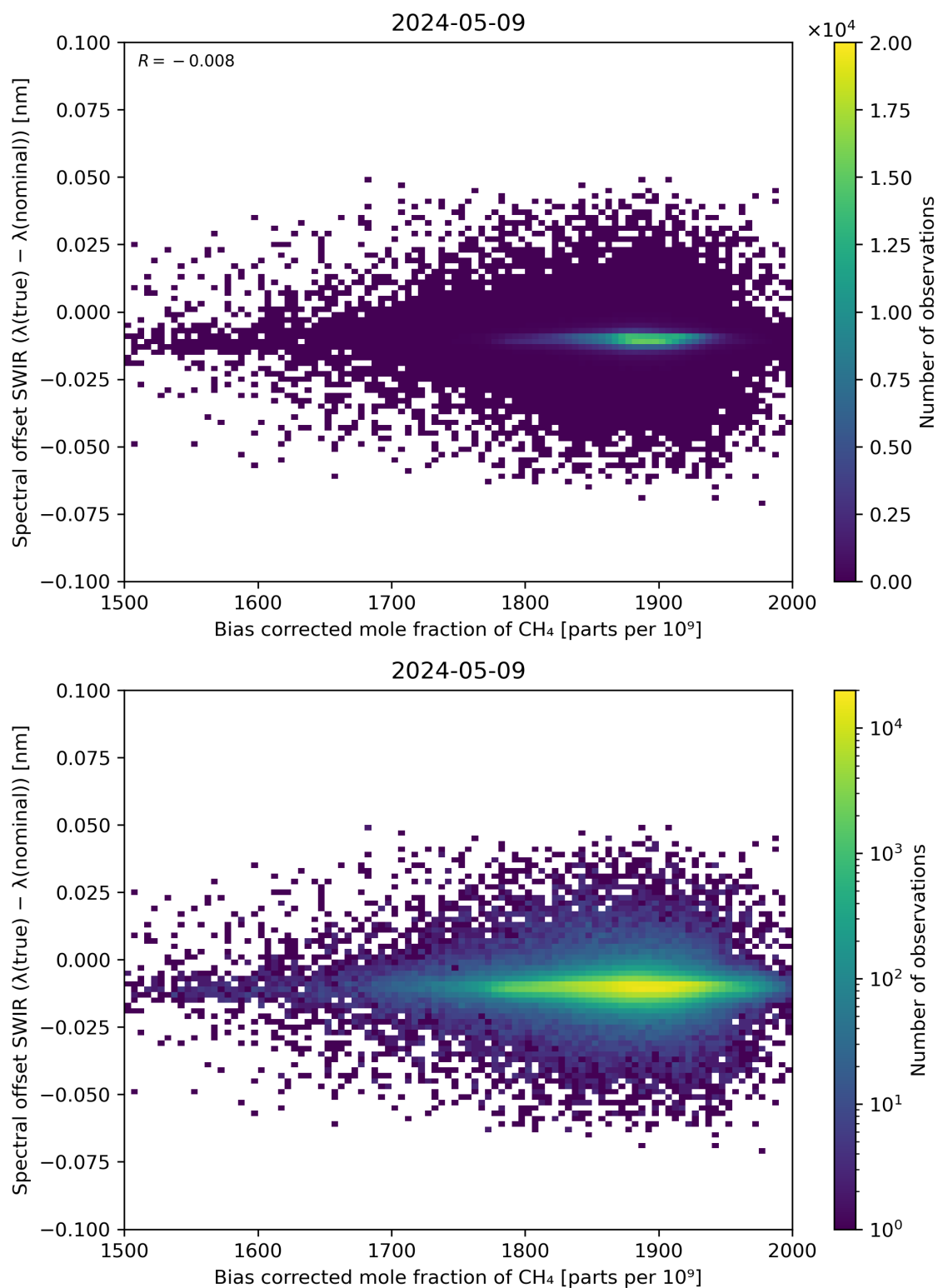
Figure 69: Scatter density plot of “Bias corrected mole fraction of \text{CH}_4 ” against “Spectral offset SWIR ( \lambda(\text{true}) - \lambda(\text{nominal}) )” for 2024-05-08 to 2024-05-10.
