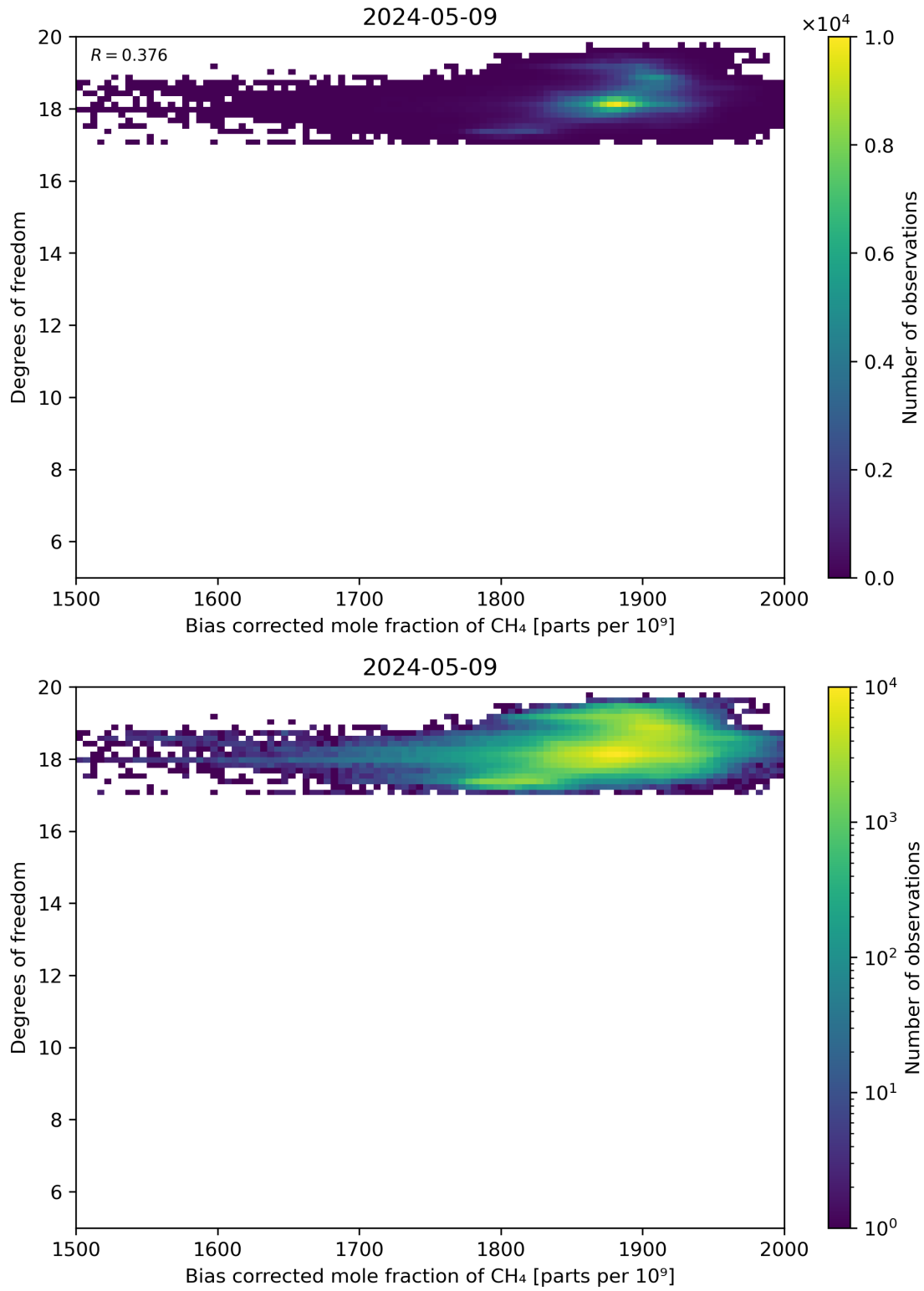
Figure 65: Scatter density plot of “Bias corrected mole fraction of CH 4 ” against “Degrees of freedom” for 2024-05-08 to 2024-05-10.
