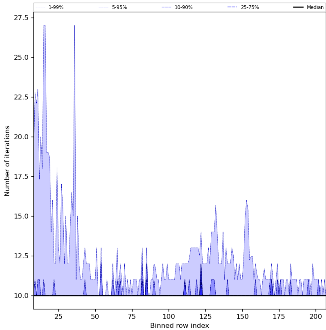
Figure 42: Along track statistics of “Number of iterations” for 2024-05-08 to 2024-05-10
