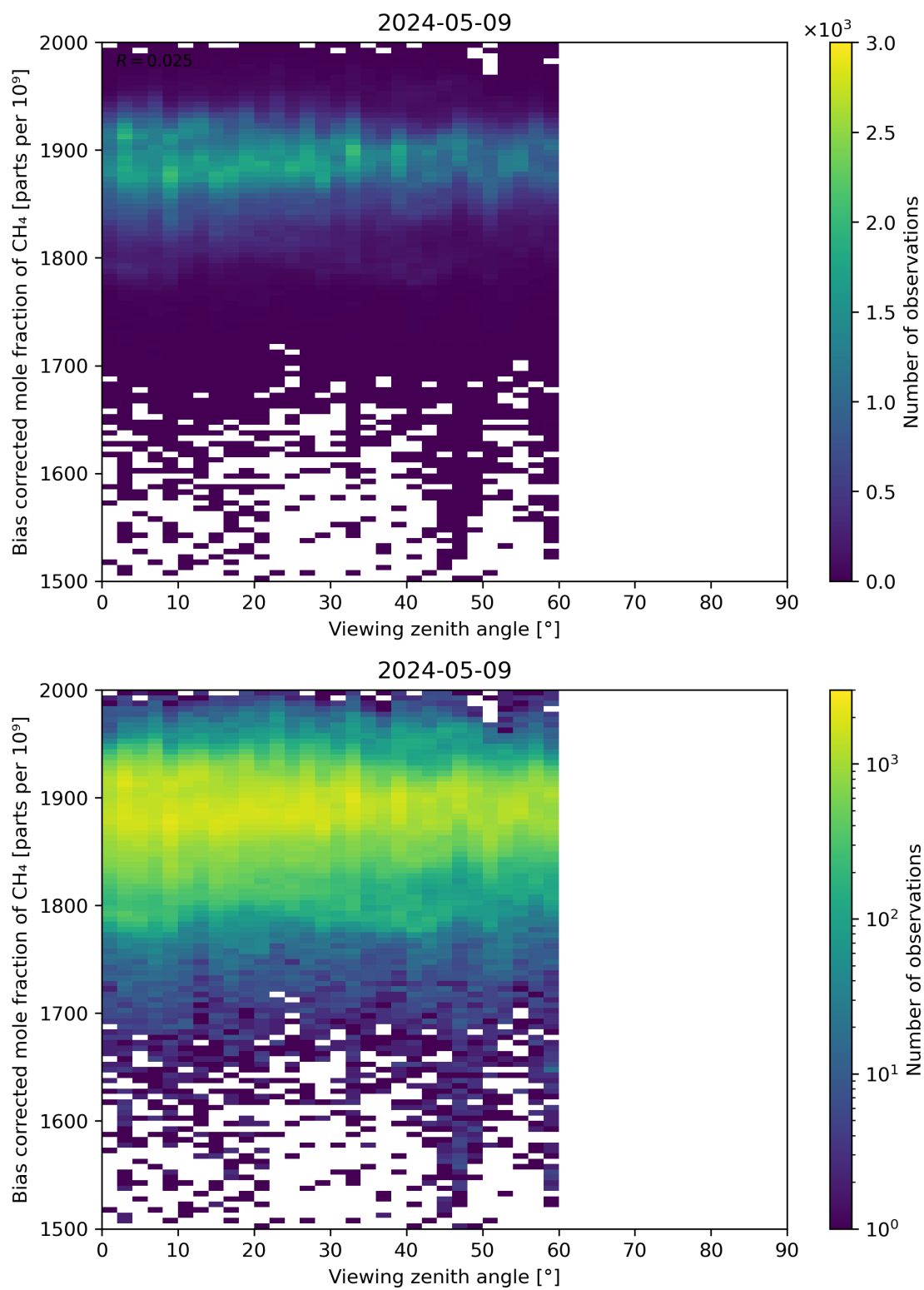
Figure 111: Scatter density plot of “Viewing zenith angle” against “Bias corrected mole fraction of CH 4 ” for 2024-05-08 to 2024-05-10.
