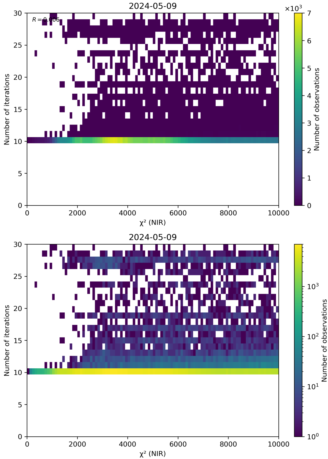
Figure 46: Scatter density plot of “ \chi^2 (NIR)” against “Number of iterations” for 2024-05-08 to 2024-05-10.
