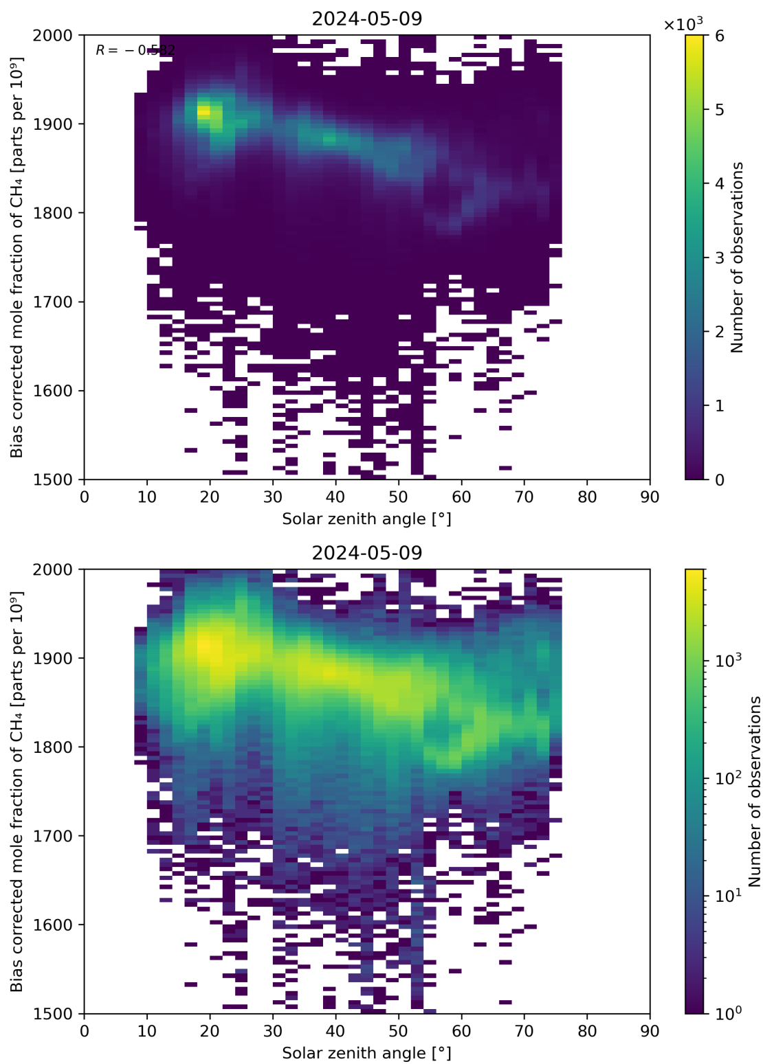
Figure 100: Scatter density plot of “Solar zenith angle” against “Bias corrected mole fraction of CH 4 ” for 2024-05-08 to 2024-05-10.
