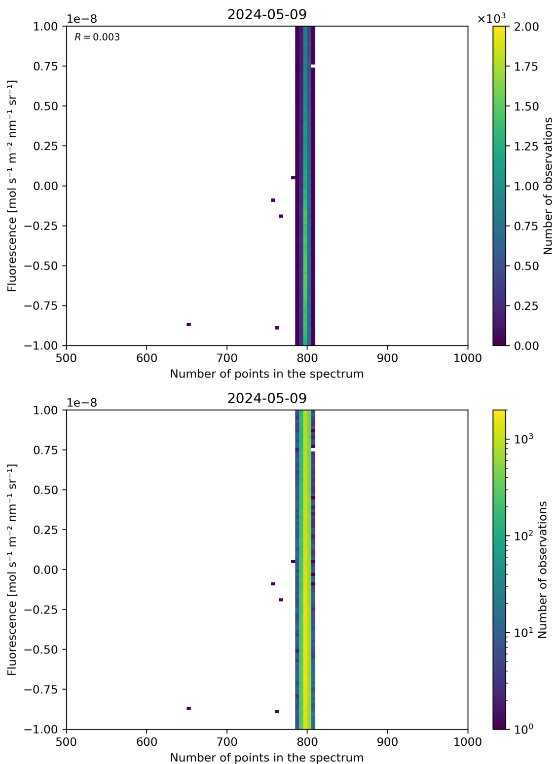
Figure 91: Scatter density plot of “Number of points in the spectrum” against “Fluorescence” for 2024-05-08 to 2024-05-10.
