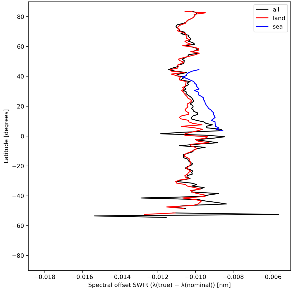
Figure 16: Zonal average of “Spectral offset SWIR ( \lambda(\text{true}) - \lambda(\text{nominal}) )” for 2024-05-08 to 2024-05-10.
