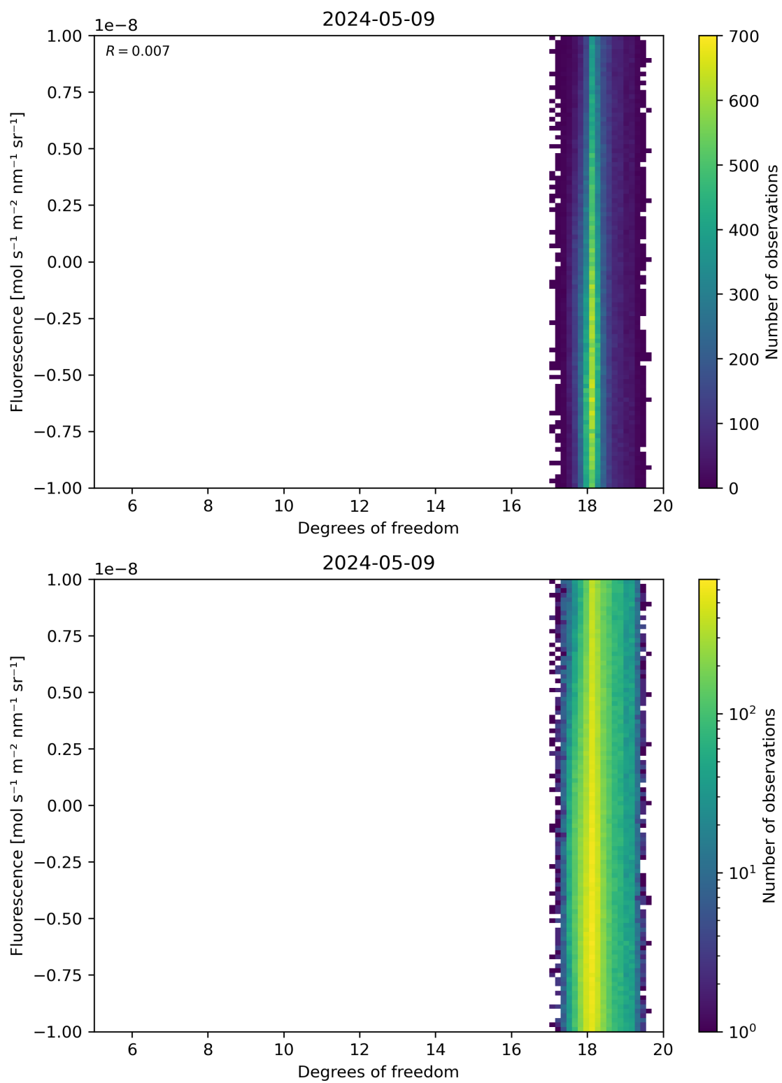
Figure 51: Scatter density plot of “Degrees of freedom” against “Fluorescence” for 2024-05-08 to 2024-05-10.
