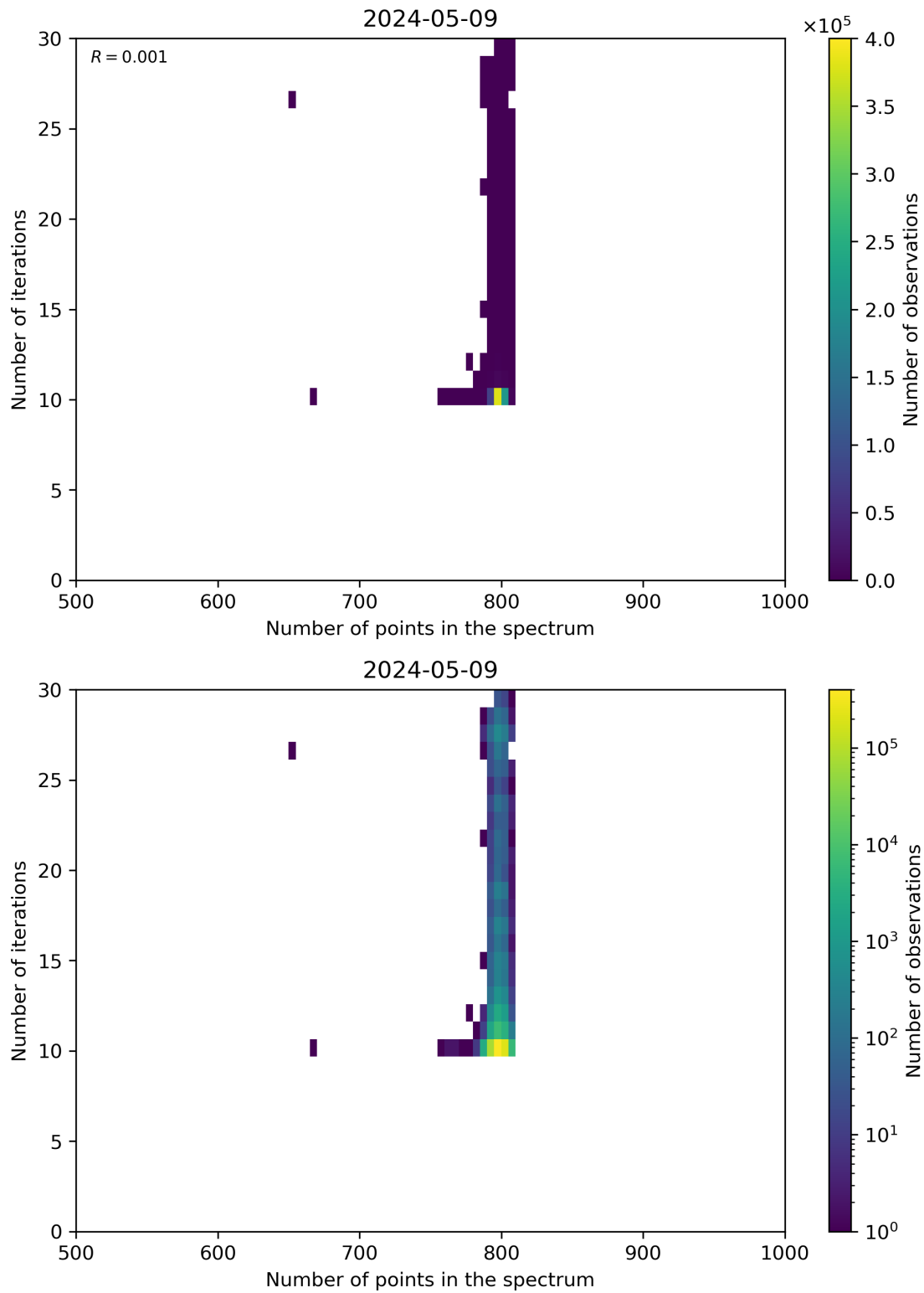
Figure 92: Scatter density plot of “Number of points in the spectrum” against “Number of iterations” for 2024-05-08 to 2024-05-10.
