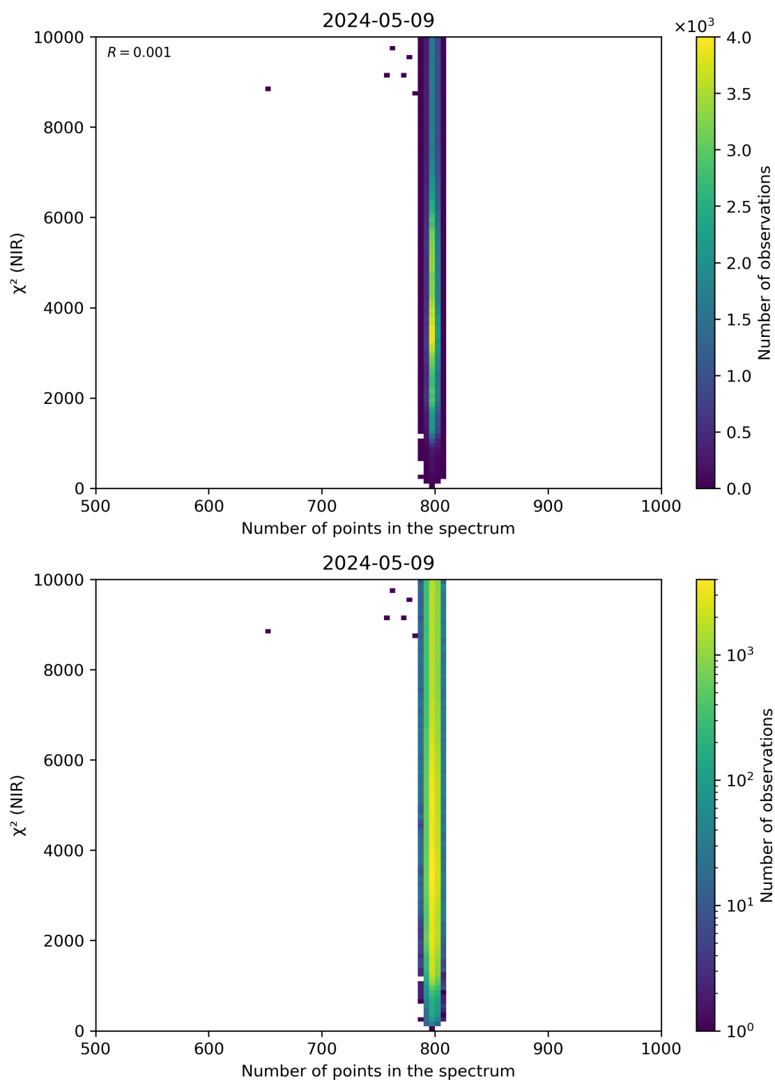
Figure 88: Scatter density plot of “Number of points in the spectrum” against “ \chi^2 (NIR)” for 2024-05-08 to 2024-05-10.
