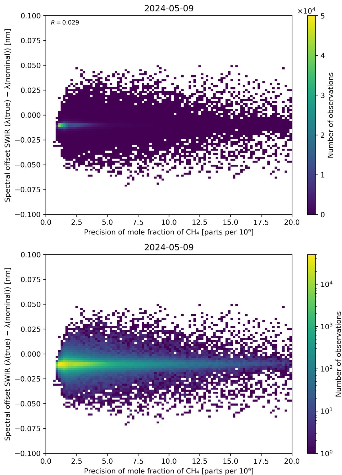
Figure 85: Scatter density plot of “Precision of mole fraction of CH 4 ” against “Spectral offset SWIR ( \lambda(\text{true}) - \lambda(\text{nominal}) )” for 2024-05-08 to 2024-05-10.
