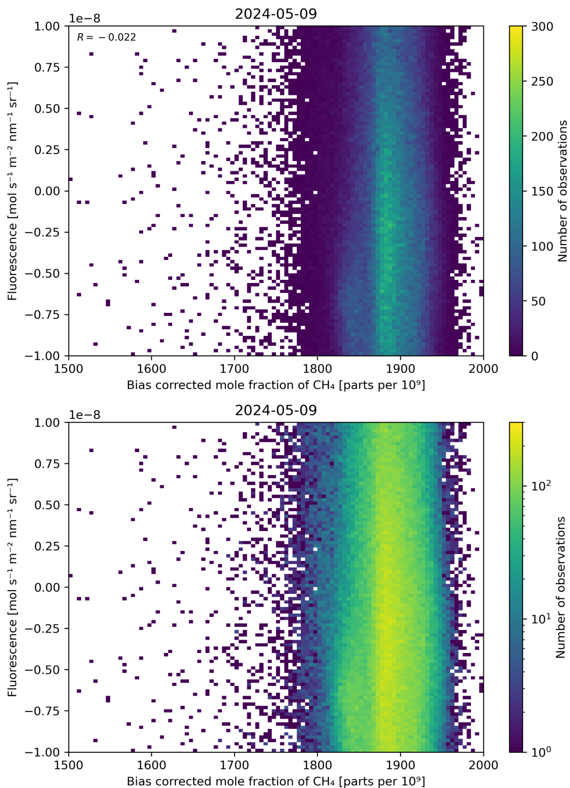
Figure 66: Scatter density plot of “Bias corrected mole fraction of \text{CH}_4 ” against “Fluorescence” for 2024-05-08 to 2024-05-10.
