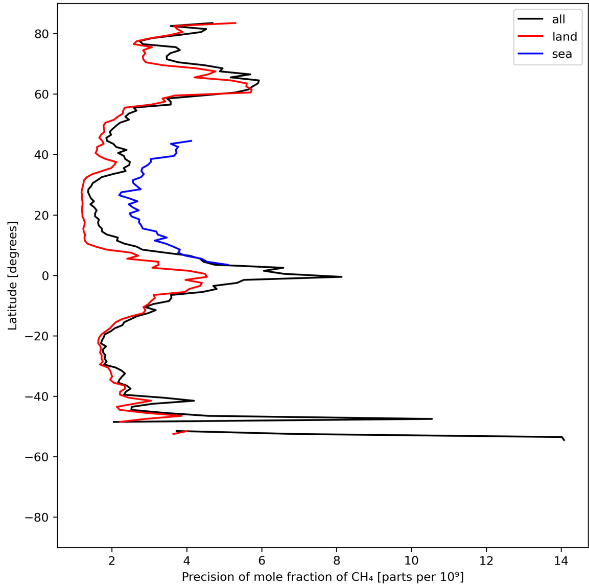
Figure 13: Zonal average of “Precision of mole fraction of CH 4 ” for 2024-05-08 to 2024-05-10.
