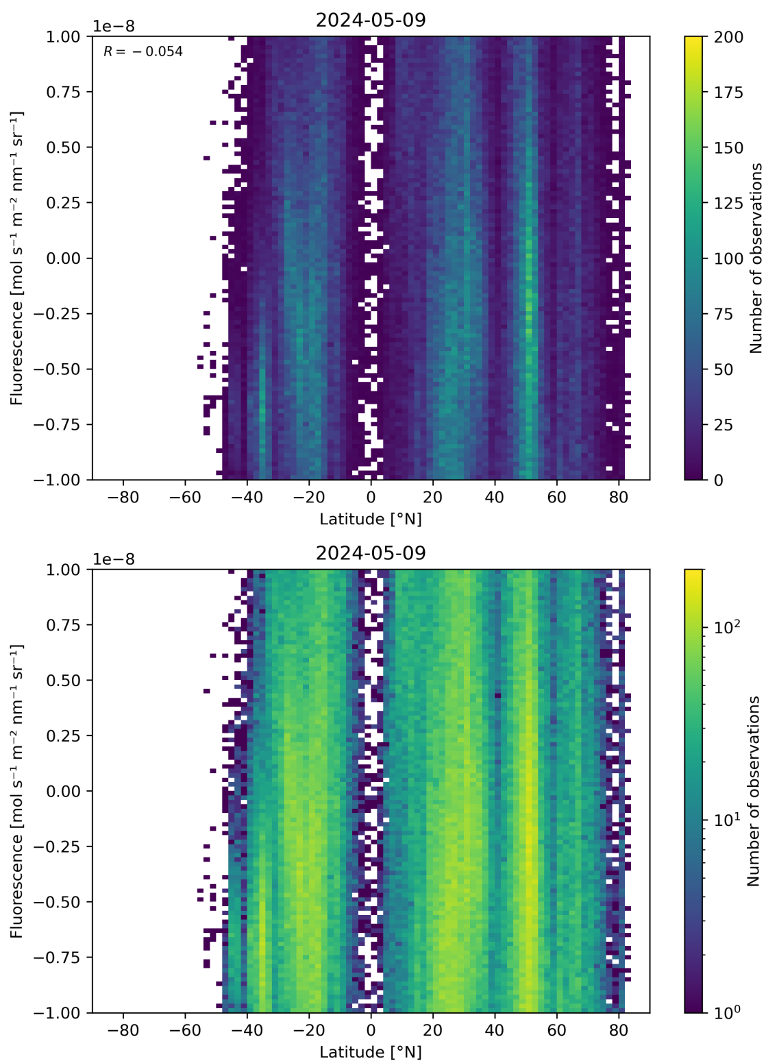
Figure 56: Scatter density plot of “Latitude” against “Fluorescence” for 2024-05-08 to 2024-05-10.
