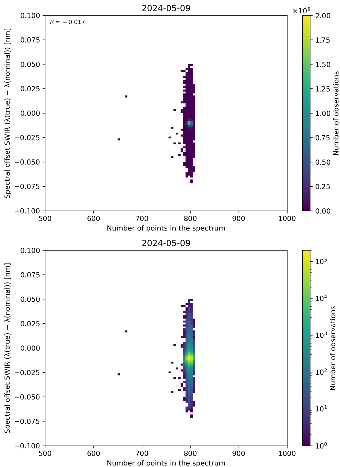
Figure 93: Scatter density plot of “Number of points in the spectrum” against “Spectral offset SWIR ( \lambda(\text{true}) - \lambda(\text{nominal}) )” for 2024-05-08 to 2024-05-10.
