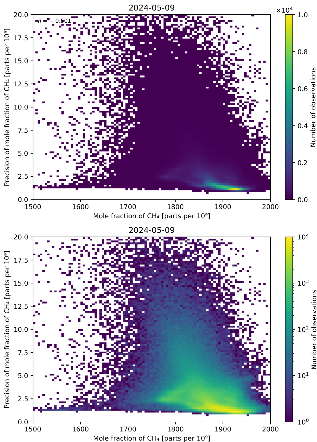
Figure 75: Scatter density plot of “Mole fraction of CH 4 ” against “Precision of mole fraction of CH 4 ” for 2024-05-08 to 2024-05-10.
