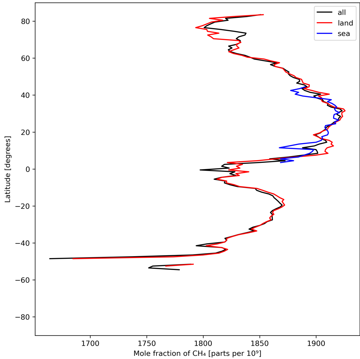
Figure 12: Zonal average of “Mole fraction of \text{CH}_4 ” for 2024-05-08 to 2024-05-10.
