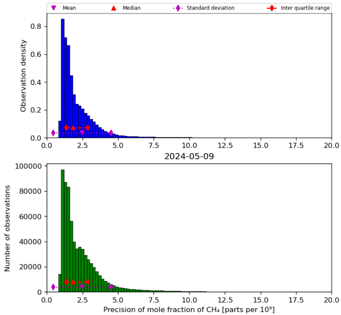
Figure 24: Histogram of “Precision of mole fraction of CH 4 ” for 2024-05-08 to 2024-05-10
