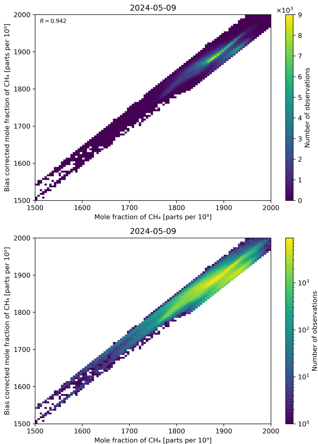
Figure 74: Scatter density plot of “Mole fraction of CH 4 ” against “Bias corrected mole fraction of CH 4 ” for 2024-05-08 to 2024-05-10.
