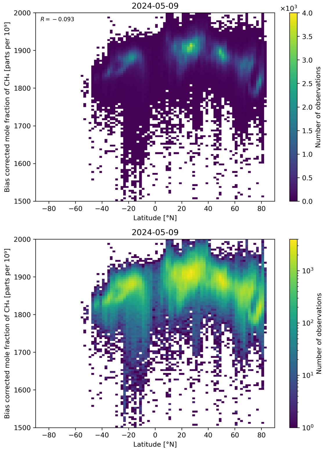
Figure 58: Scatter density plot of “Latitude” against “Bias corrected mole fraction of \text{CH}_4 ” for 2024-05-08 to 2024-05-10.
