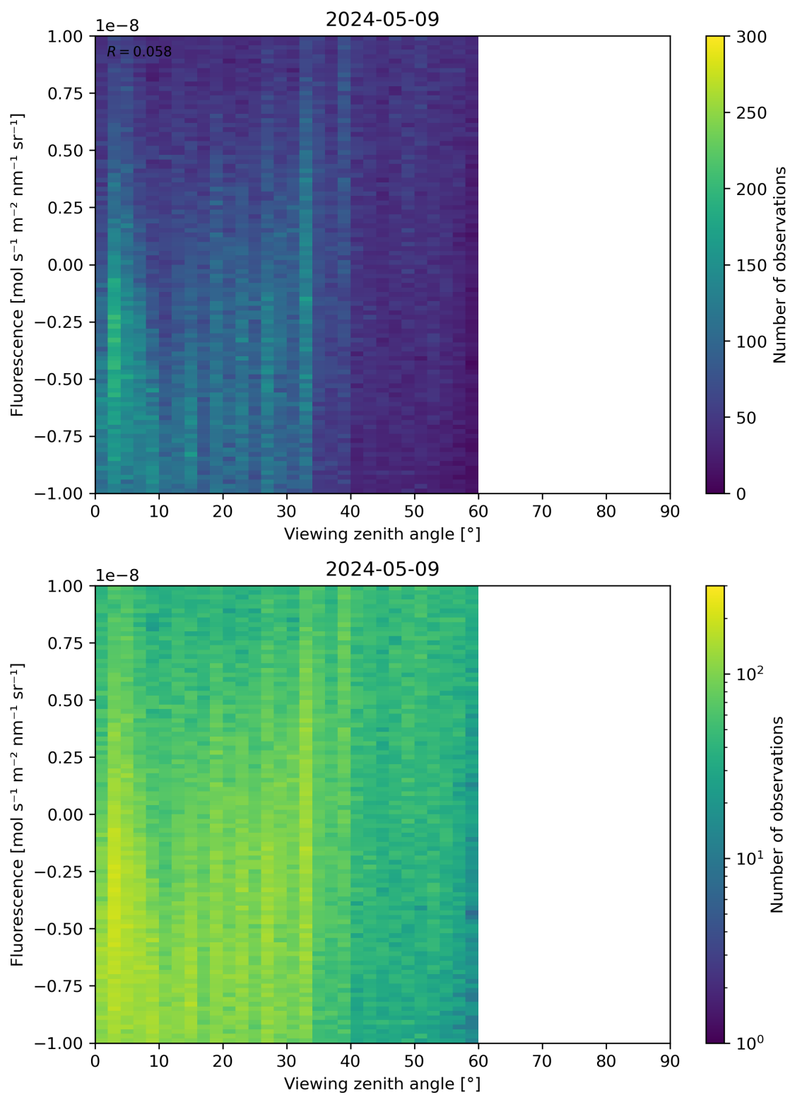
Figure 108: Scatter density plot of “Viewing zenith angle” against “Fluorescence” for 2024-05-08 to 2024-05-10.
