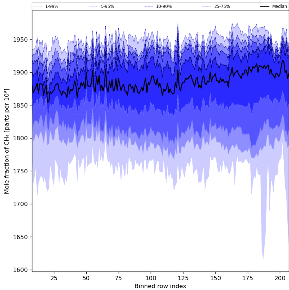
Figure 34: Along track statistics of “Mole fraction of CH 4 ” for 2024-05-08 to 2024-05-10
