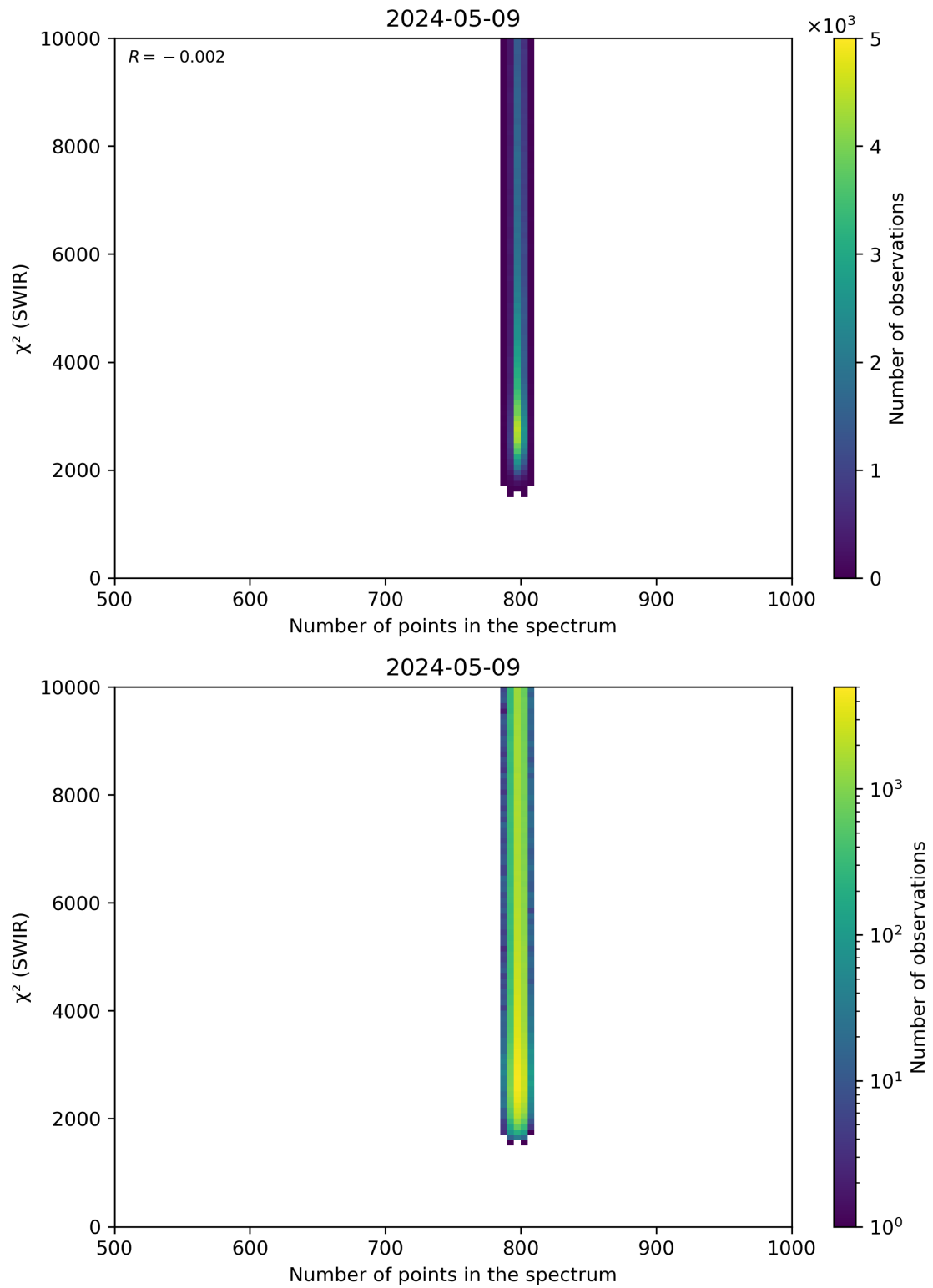
Figure 89: Scatter density plot of “Number of points in the spectrum” against “ \chi^2 (SWIR)” for 2024-05-08 to 2024-05-10.
