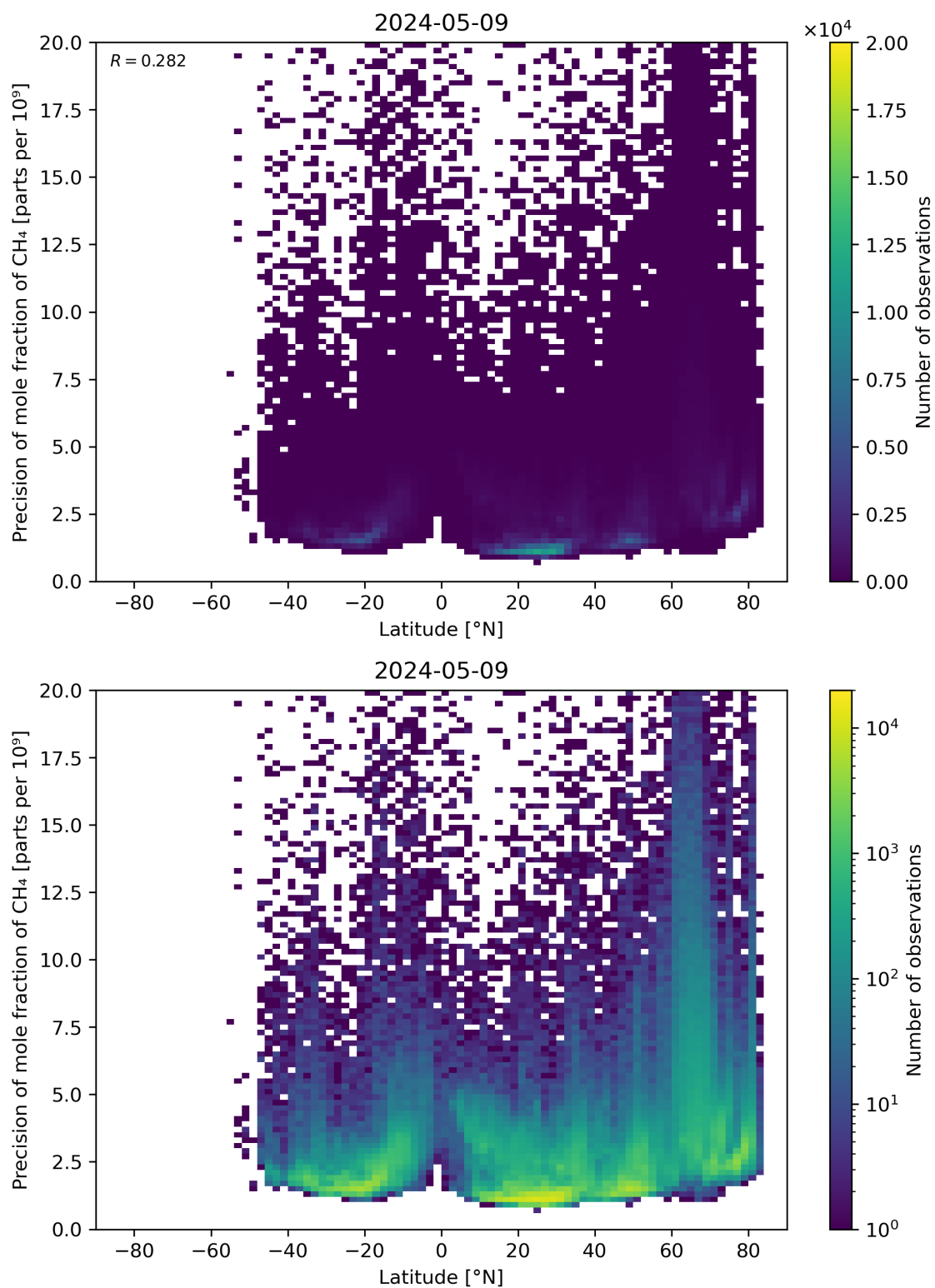
Figure 59: Scatter density plot of “Latitude” against “Precision of mole fraction of \text{CH}_4 ” for 2024-05-08 to 2024-05-10.
