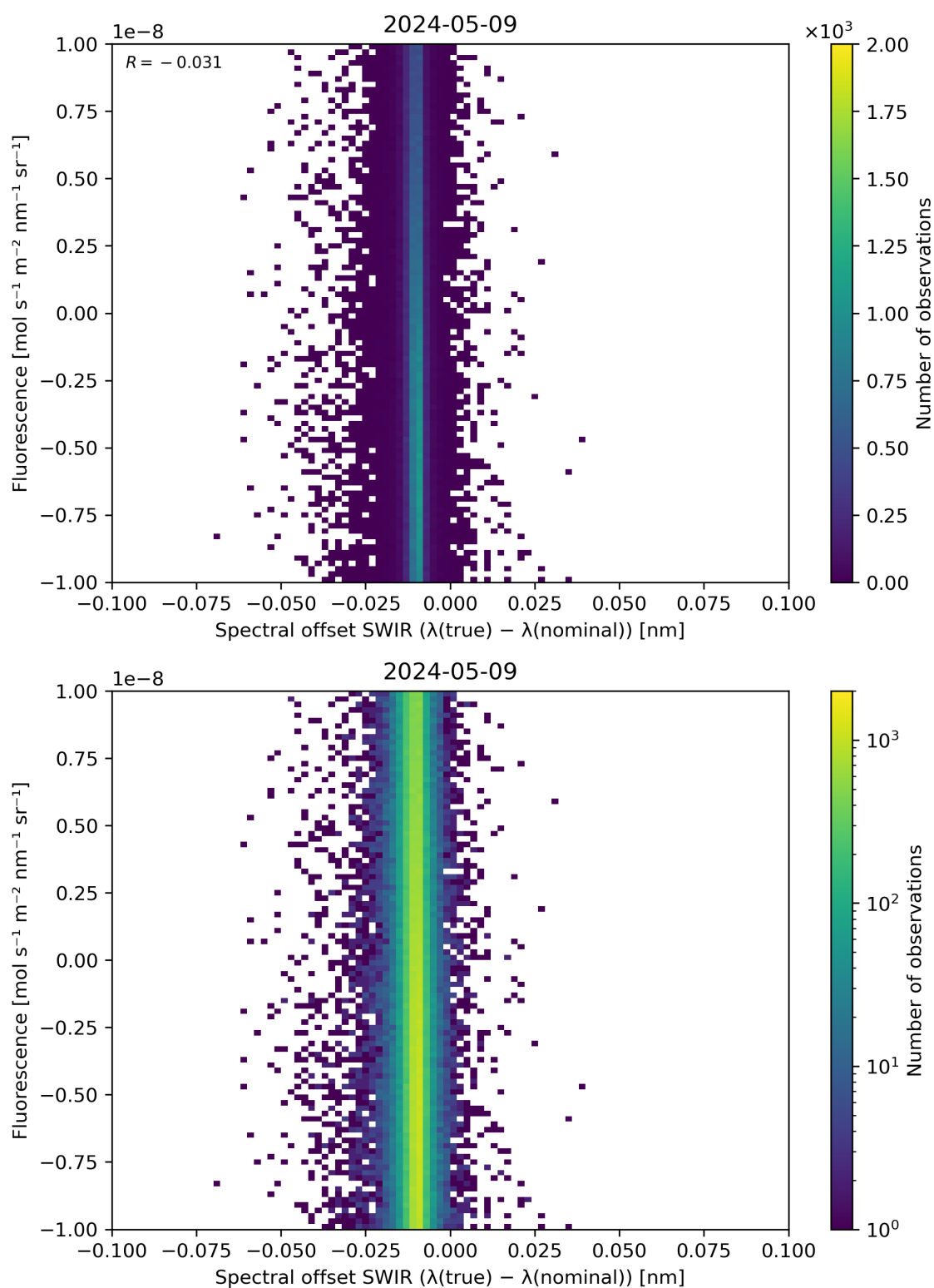
Figure 120: Scatter density plot of “Spectral offset SWIR ( \lambda(\text{true}) - \lambda(\text{nominal}) )” against “Fluorescence” for 2024-05-08 to 2024-05-10.
