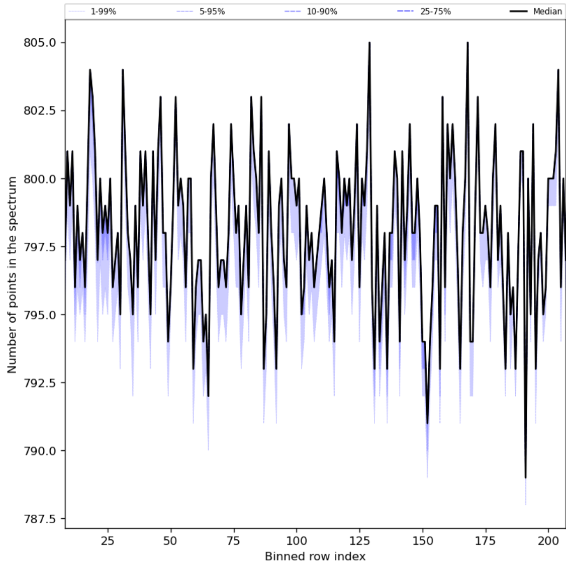
Figure 37: Along track statistics of “Number of points in the spectrum” for 2024-05-08 to 2024-05-10
