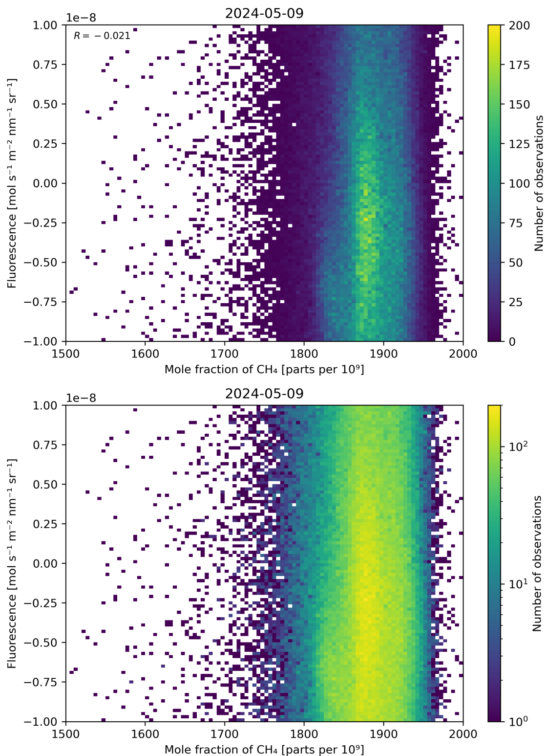
Figure 73: Scatter density plot of “Mole fraction of \text{CH}_4 ” against “Fluorescence” for 2024-05-08 to 2024-05-10.
