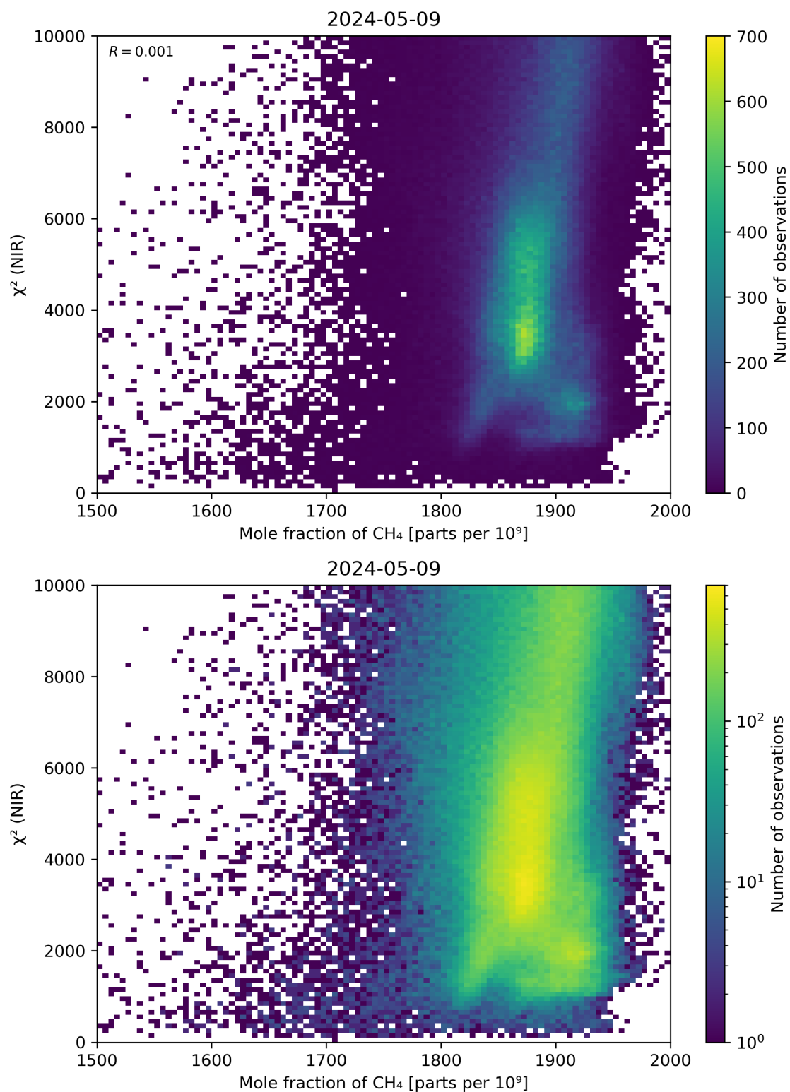
Figure 70: Scatter density plot of “Mole fraction of CH 4 ” against “ \chi^2 (NIR)” for 2024-05-08 to 2024-05-10.
