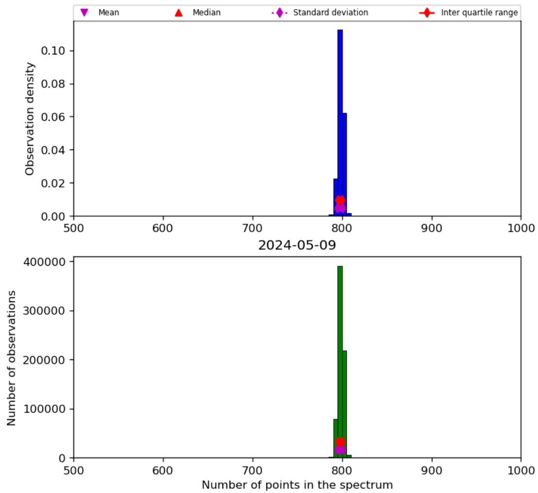
Figure 26: Histogram of “Number of points in the spectrum” for 2024-05-08 to 2024-05-10
