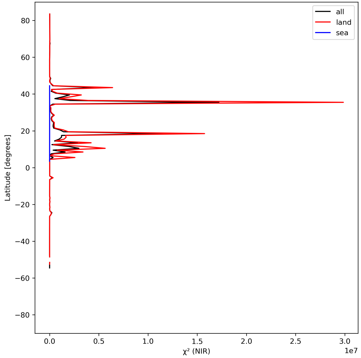
Figure 18: Zonal average of “ \chi^2 (NIR)” for 2024-05-08 to 2024-05-10.
