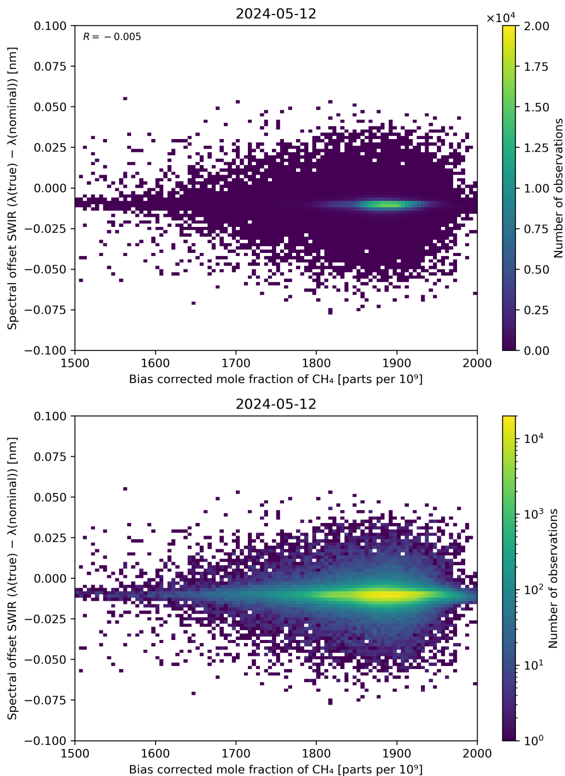
Figure 69: Scatter density plot of “Bias corrected mole fraction of \text{CH}_4 ” against “Spectral offset SWIR ( \lambda(\text{true}) - \lambda(\text{nominal}) )” for 2024-05-12 to 2024-05-13.
