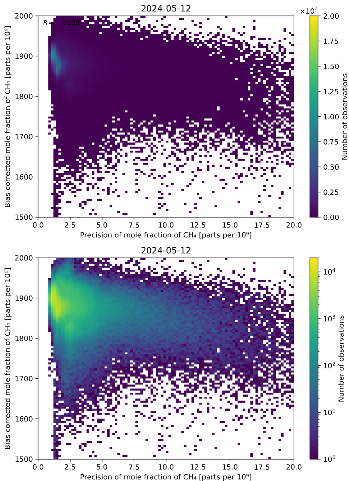
Figure 82: Scatter density plot of “Precision of mole fraction of CH 4 ” against “Bias corrected mole fraction of CH 4 ” for 2024-05-12 to 2024-05-13.
