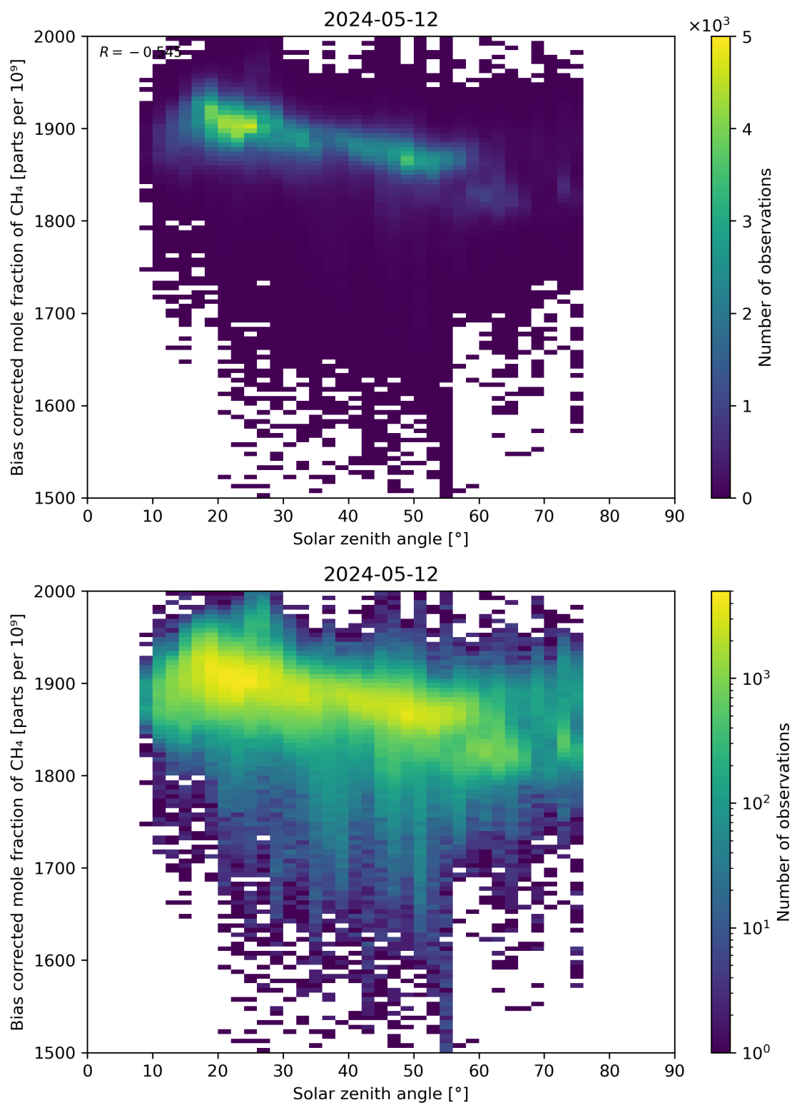
Figure 100: Scatter density plot of “Solar zenith angle” against “Bias corrected mole fraction of CH 4 ” for 2024-05-12 to 2024-05-13.
