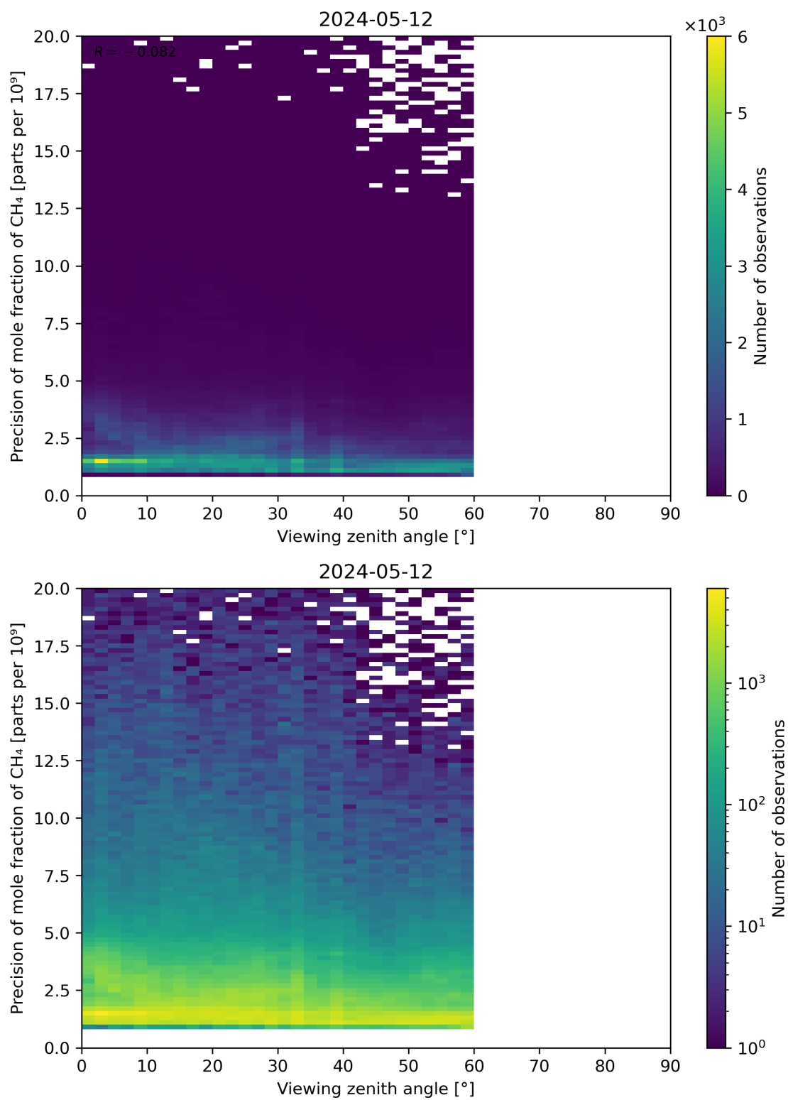
Figure 112: Scatter density plot of “Viewing zenith angle” against “Precision of mole fraction of CH 4 ” for 2024-05-12 to 2024-05-13.
