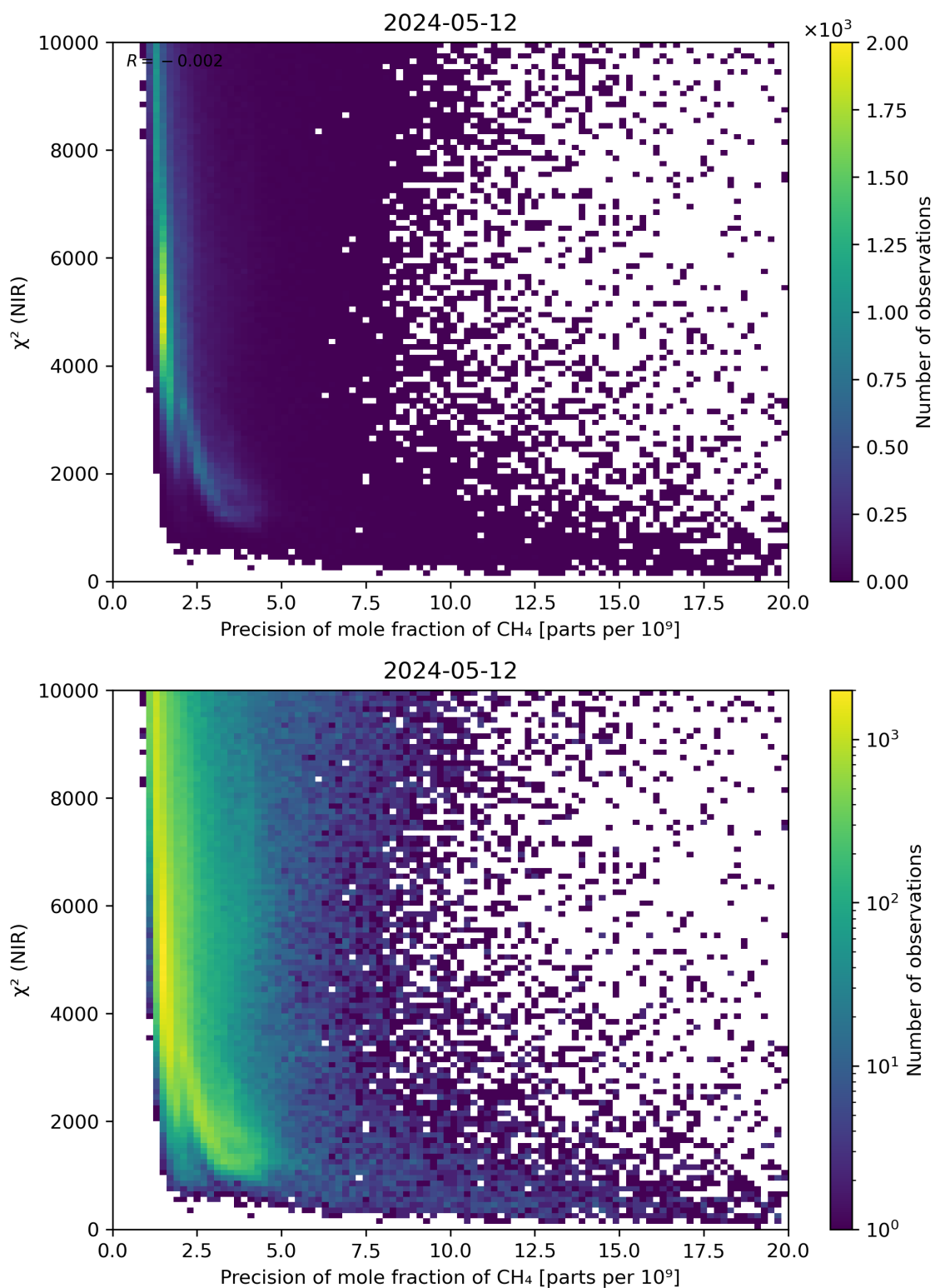
Figure 78: Scatter density plot of “Precision of mole fraction of CH 4 ” against “ \chi^2 (NIR)” for 2024-05-12 to 2024-05-13.
