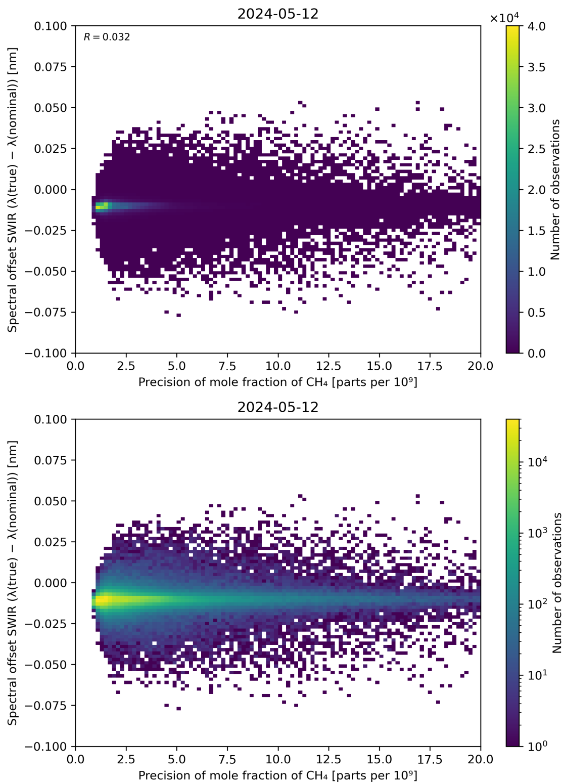
Figure 85: Scatter density plot of “Precision of mole fraction of \text{CH}_4 ” against “Spectral offset SWIR ( \lambda(\text{true}) - \lambda(\text{nominal}) )” for 2024-05-12 to 2024-05-13.
