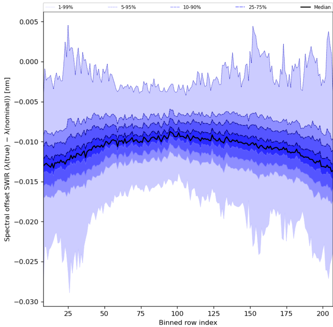
Figure 38: Along track statistics of “Spectral offset SWIR ( \lambda(\text{true}) - \lambda(\text{nominal}) )” for 2024-05-12 to 2024-05-13
