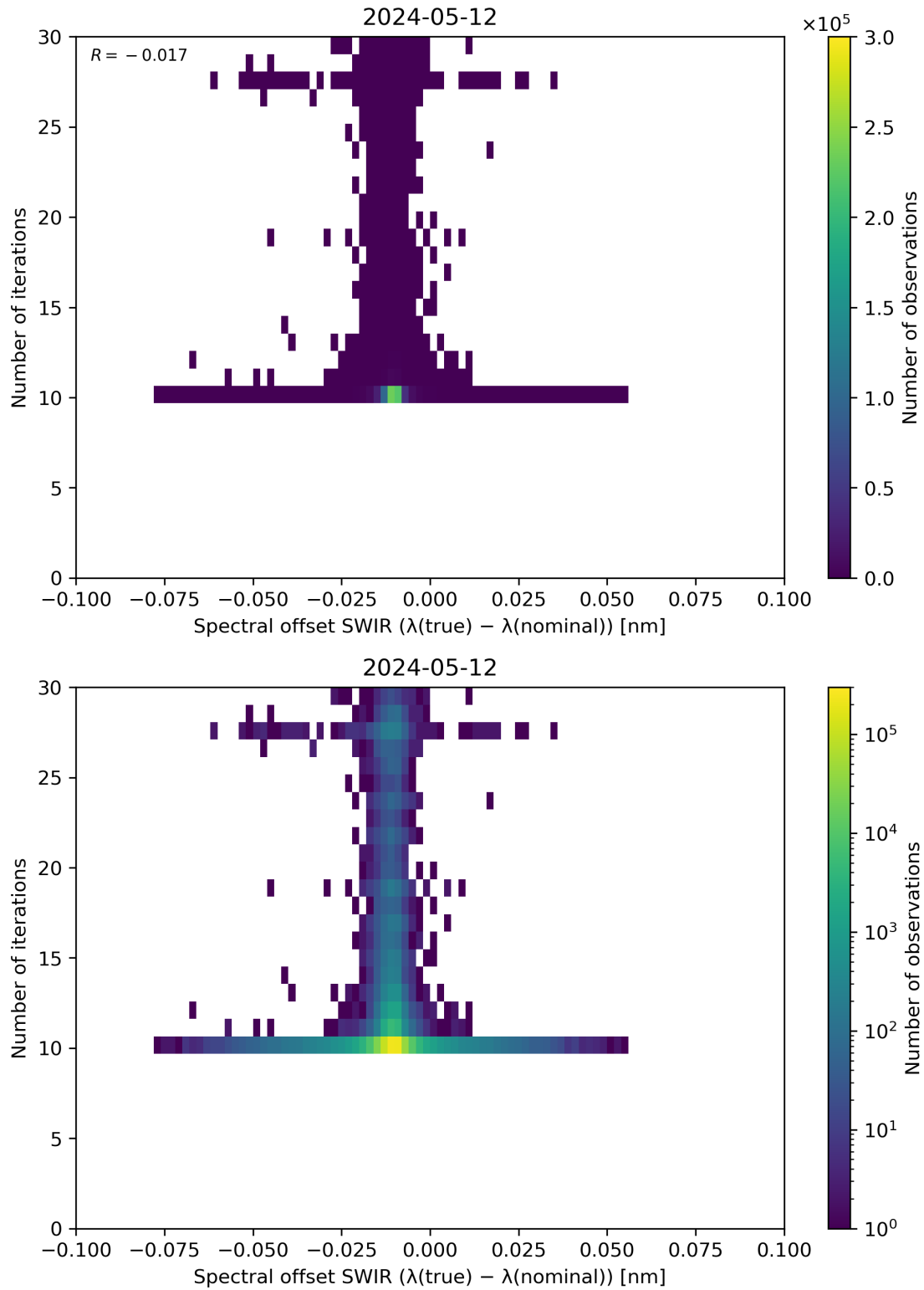
Figure 121: Scatter density plot of “Spectral offset SWIR ( \lambda(\text{true}) - \lambda(\text{nominal}) )” against “Number of iterations” for 2024-05-12 to 2024-05-13.
