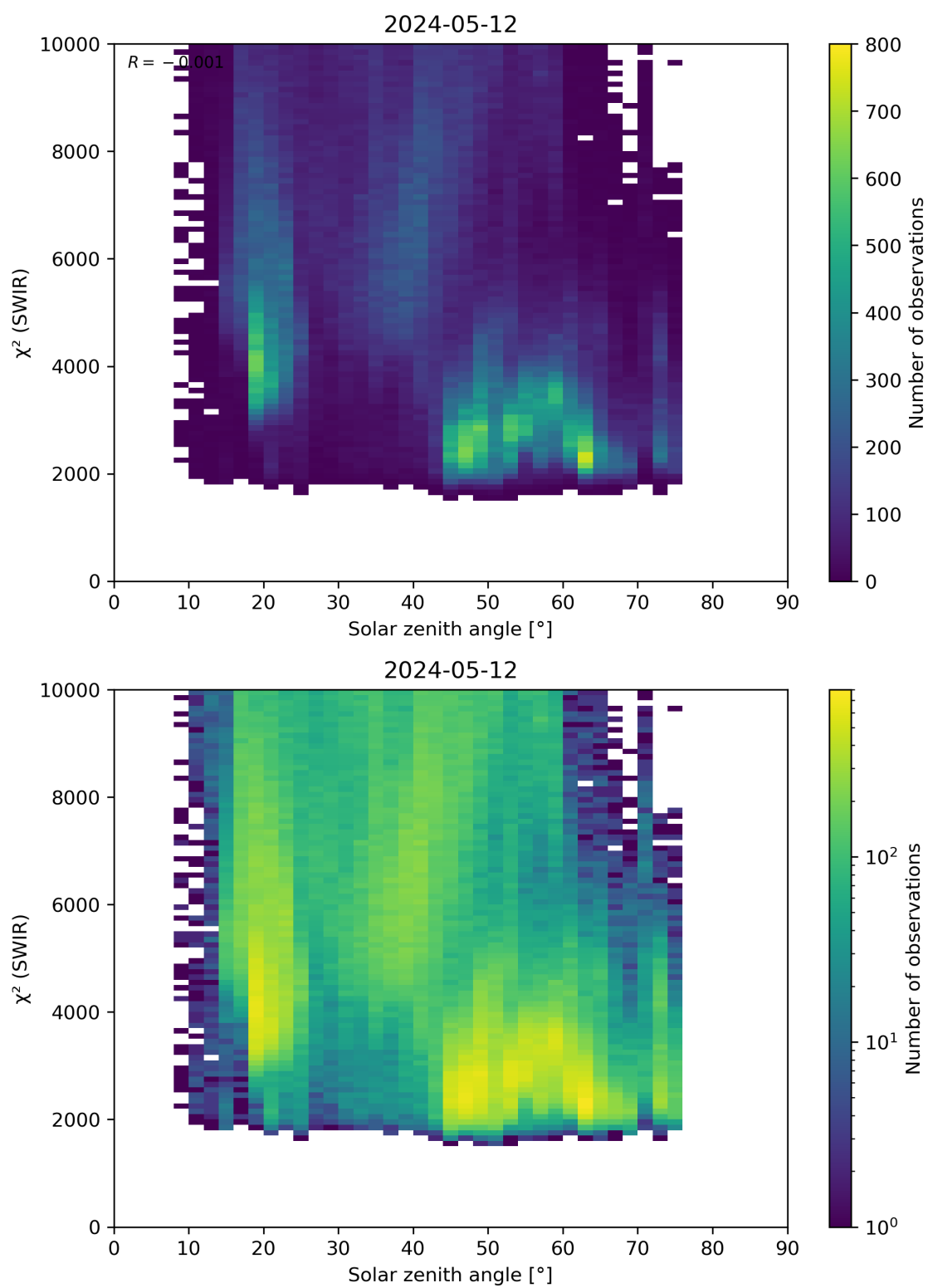
Figure 95: Scatter density plot of “Solar zenith angle” against “ \chi^2 (SWIR)” for 2024-05-12 to 2024-05-13.
