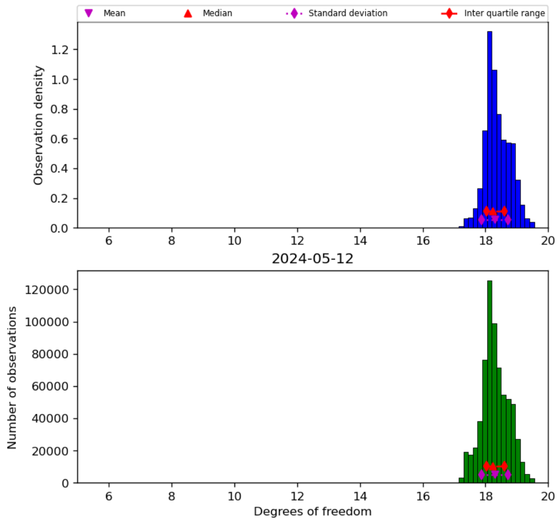
Figure 30: Histogram of “Degrees of freedom” for 2024-05-12 to 2024-05-13
