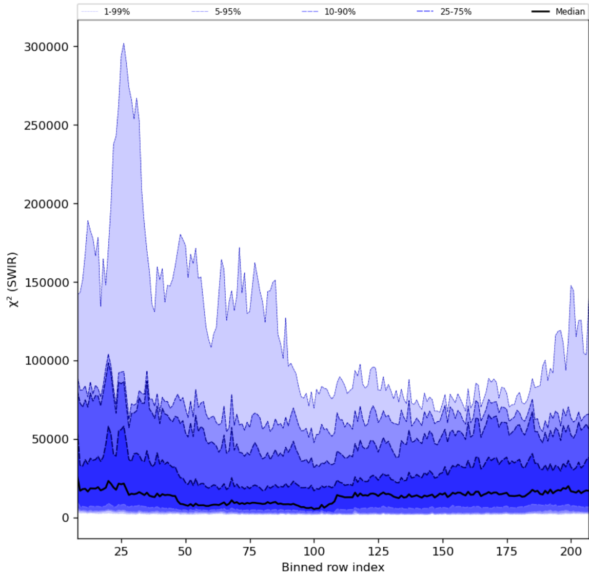
Figure 39: Along track statistics of " \chi^2 (SWIR)" for 2024-05-12 to 2024-05-13
