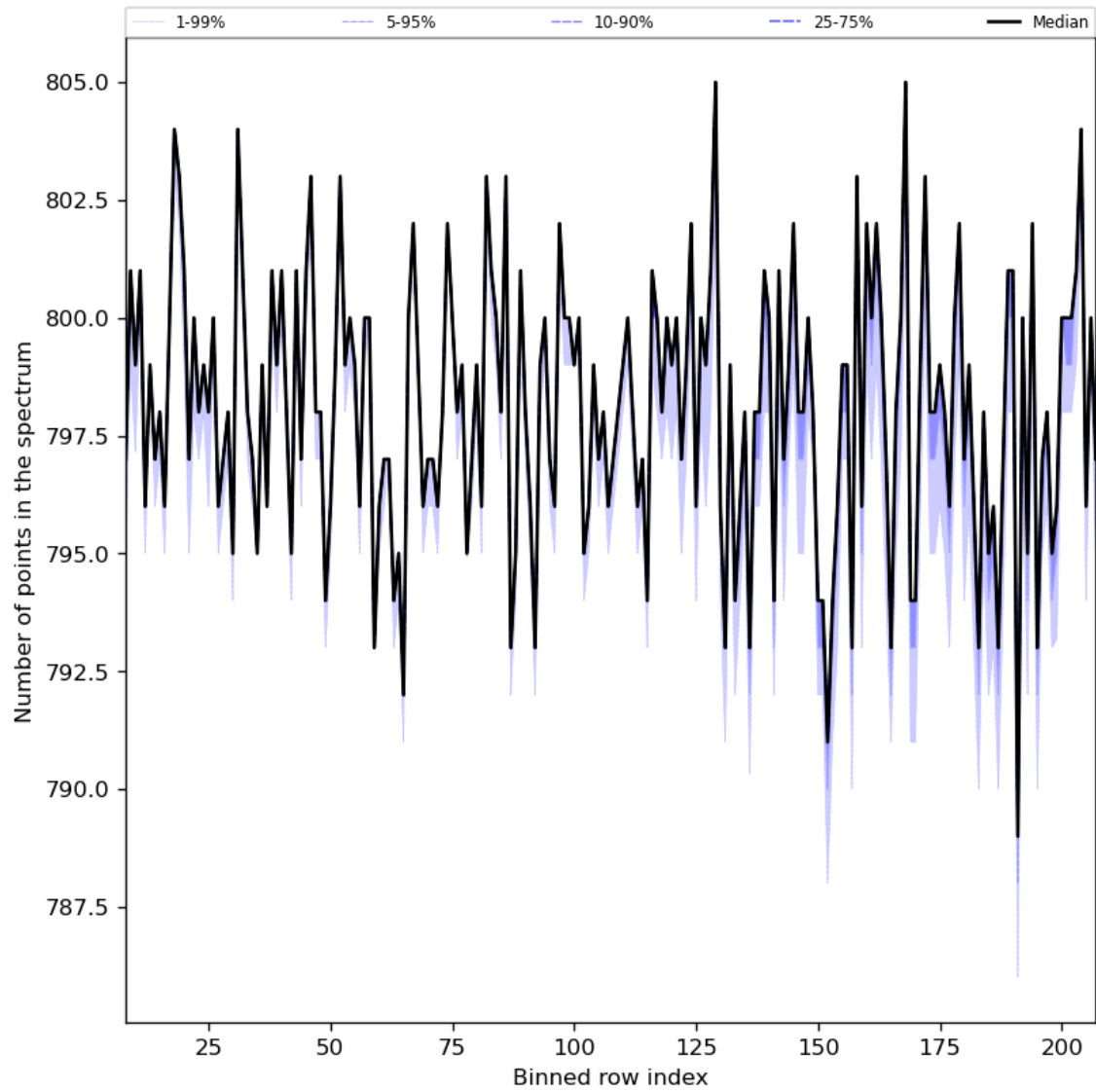
Figure 37: Along track statistics of “Number of points in the spectrum” for 2024-05-12 to 2024-05-13
