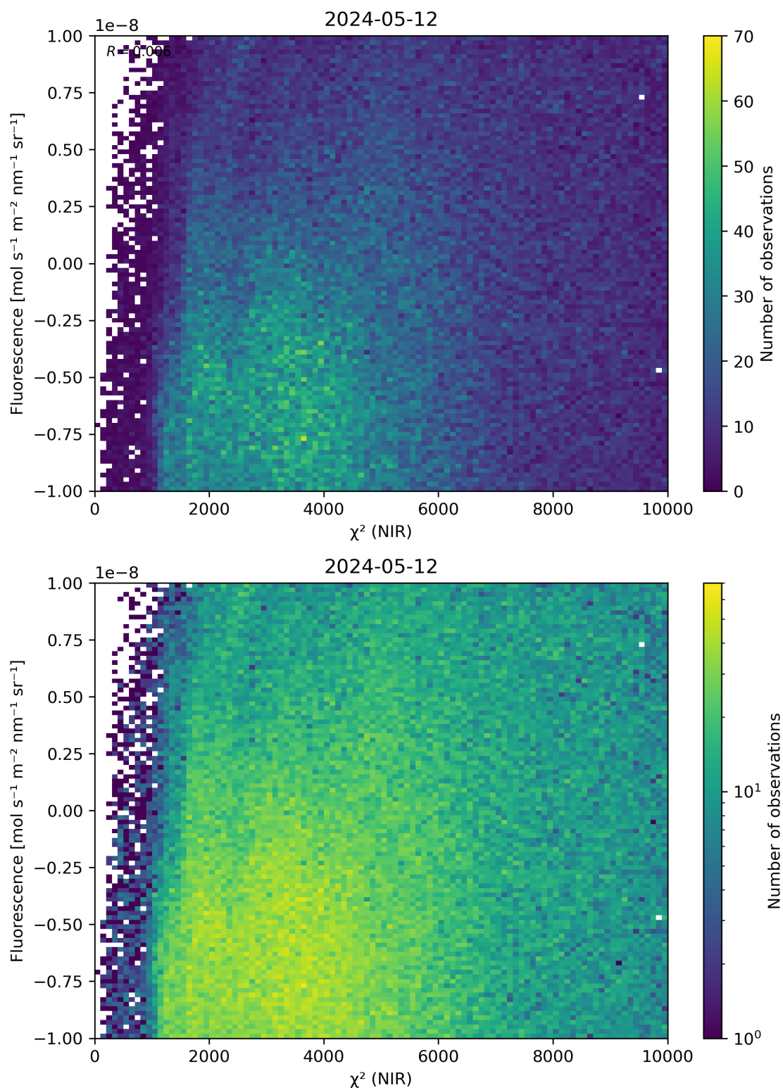
Figure 45: Scatter density plot of “ \chi^2 (NIR)” against “Fluorescence” for 2024-05-12 to 2024-05-13.
