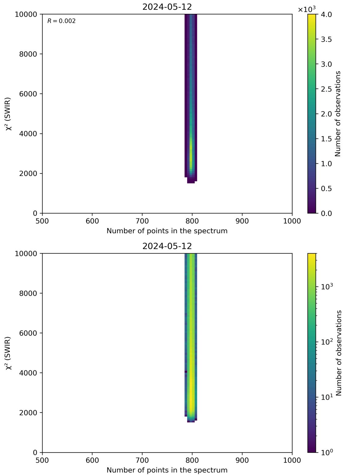
Figure 89: Scatter density plot of “Number of points in the spectrum” against “ \chi^2 (SWIR)” for 2024-05-12 to 2024-05-13.
