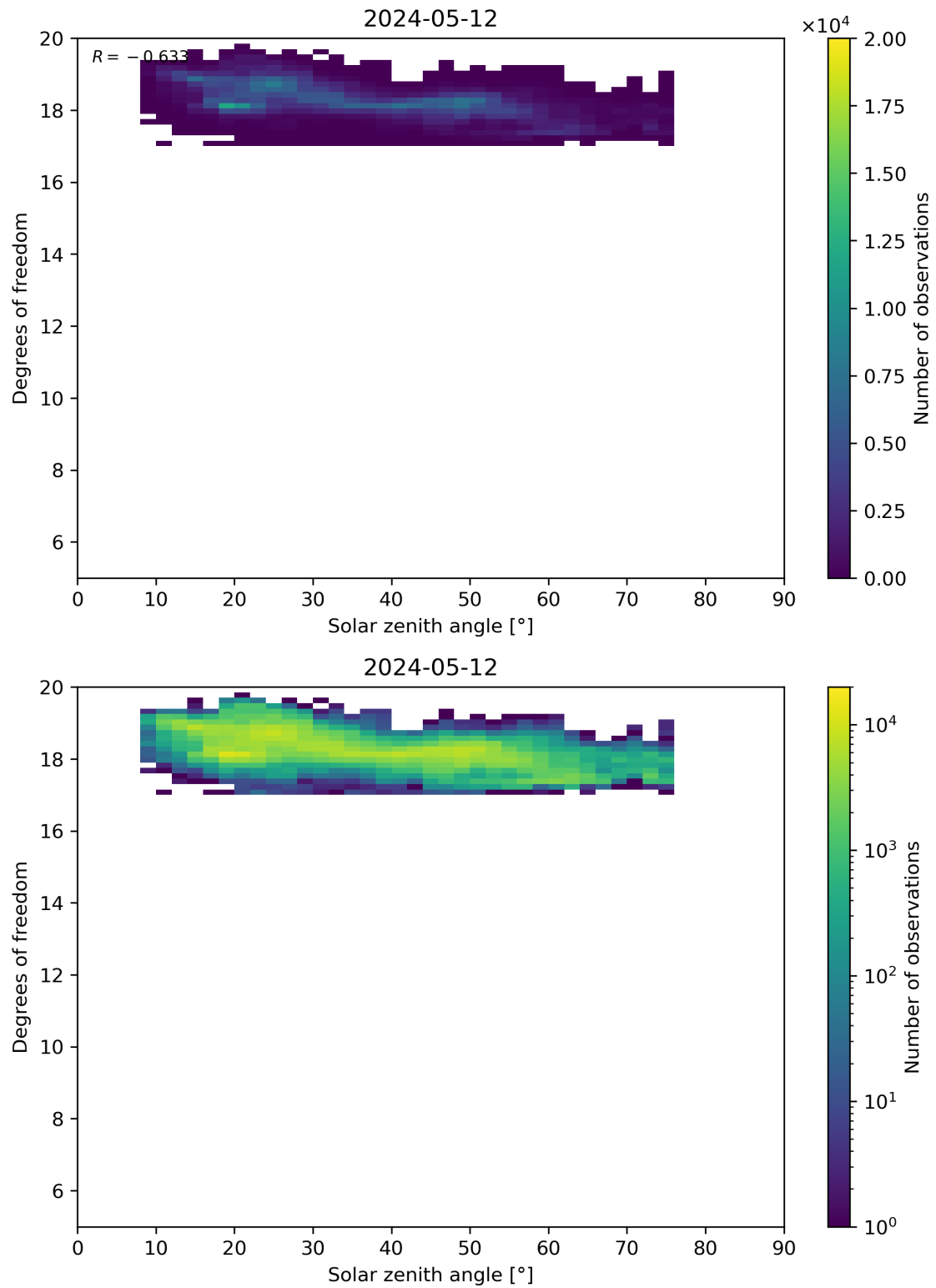
Figure 96: Scatter density plot of “Solar zenith angle” against “Degrees of freedom” for 2024-05-12 to 2024-05-13.
