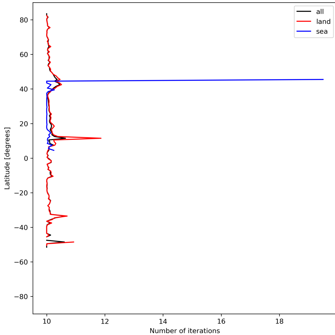
Figure 20: Zonal average of “Number of iterations” for 2024-05-12 to 2024-05-13.
