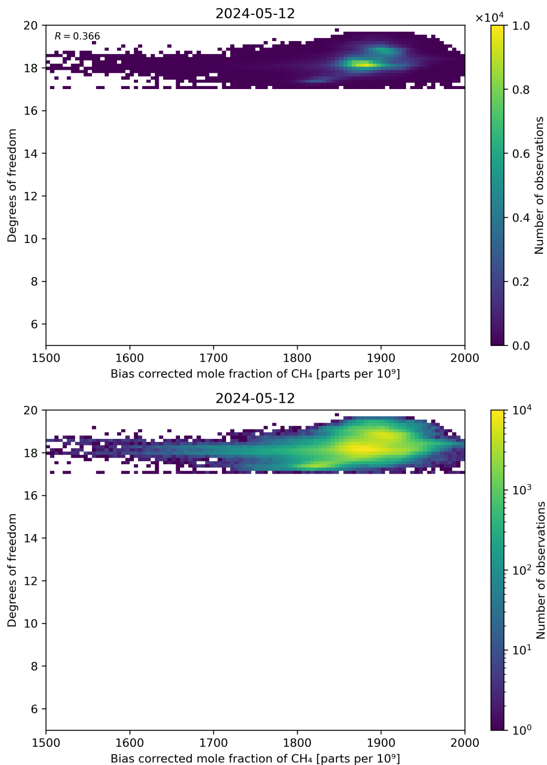
Figure 65: Scatter density plot of “Bias corrected mole fraction of CH 4 ” against “Degrees of freedom” for 2024-05-12 to 2024-05-13.
