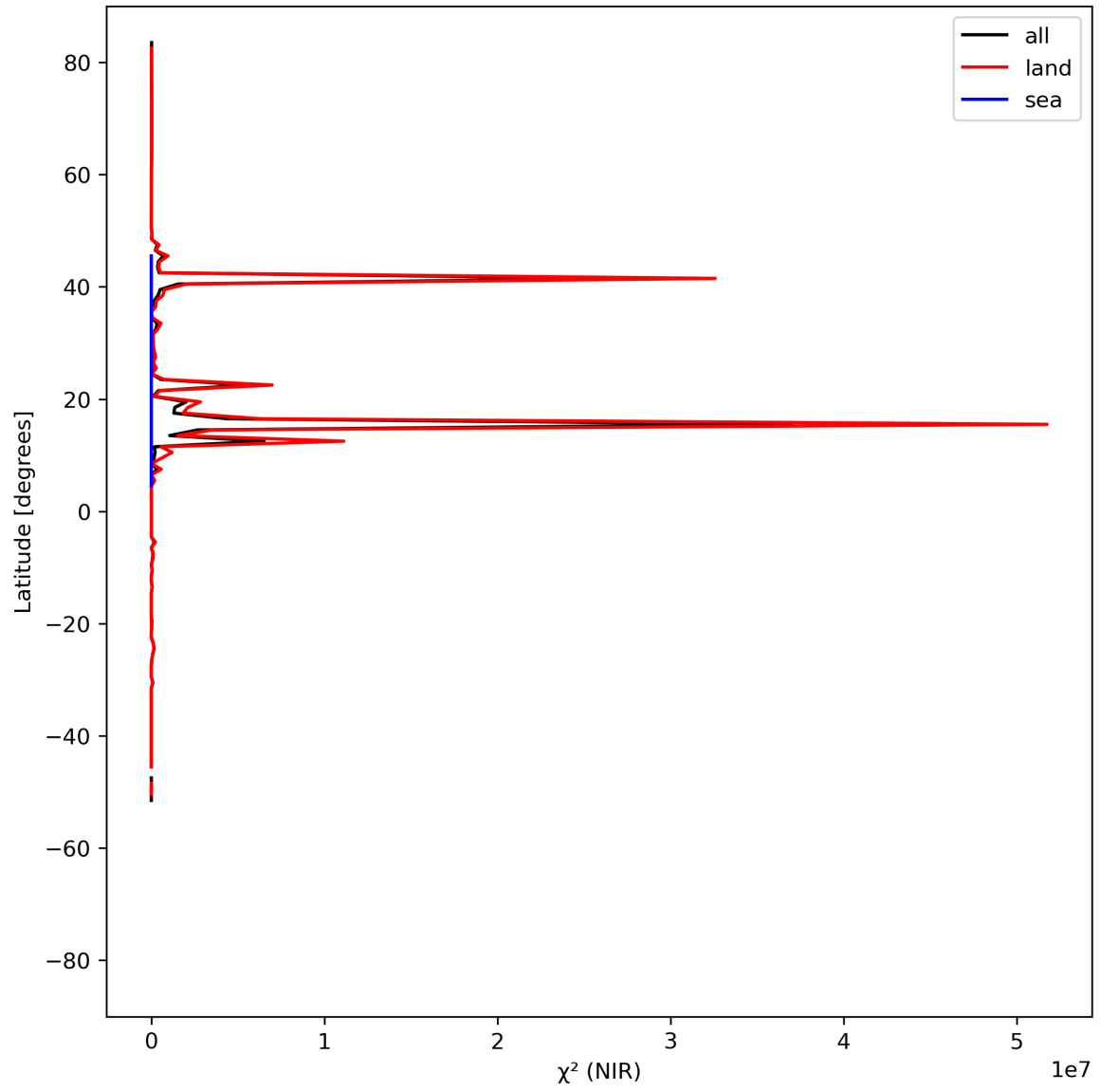
Figure 18: Zonal average of “ \chi^2 (NIR)” for 2024-05-12 to 2024-05-13.
