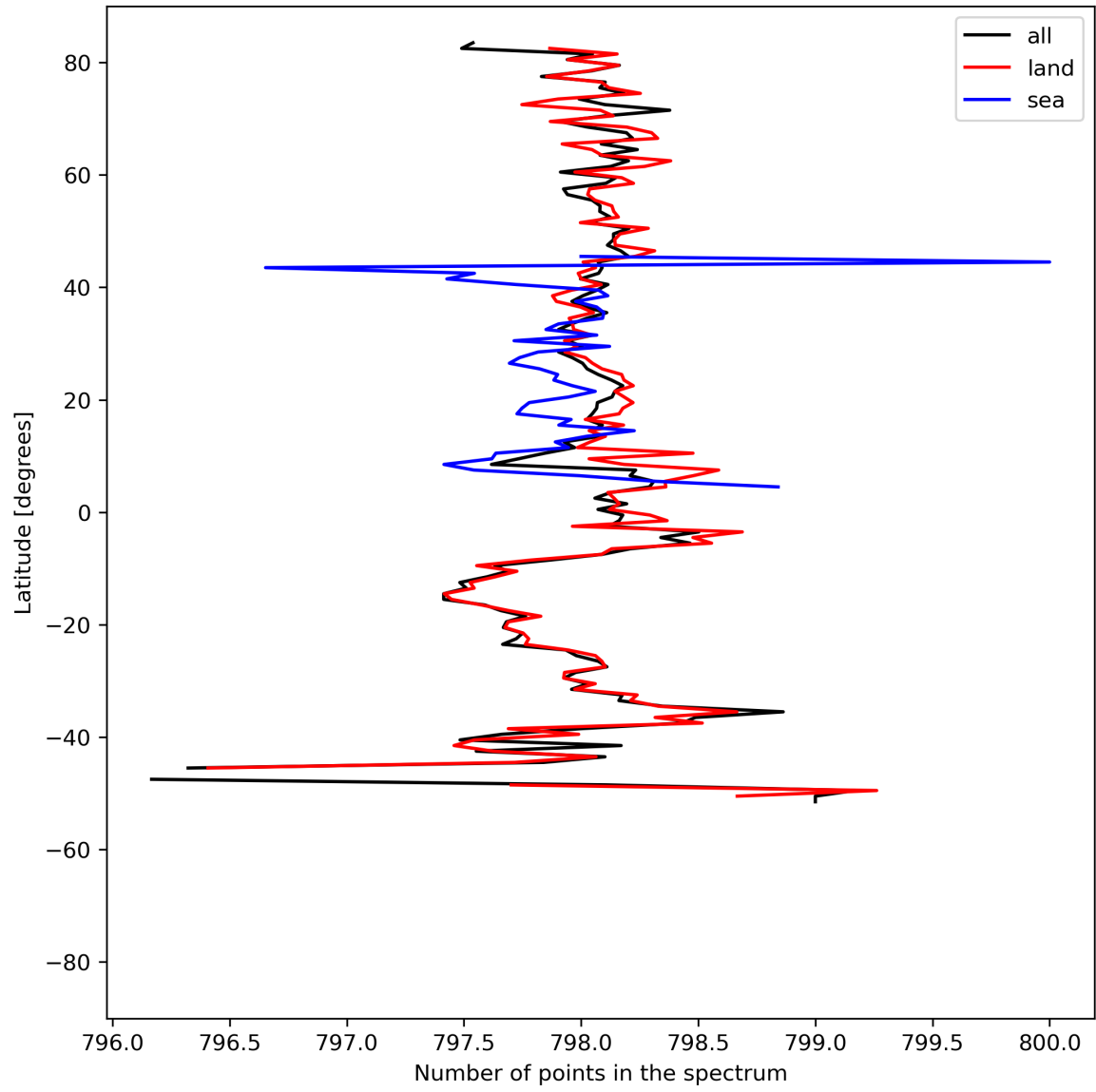
Figure 15: Zonal average of “Number of points in the spectrum” for 2024-05-12 to 2024-05-13.
