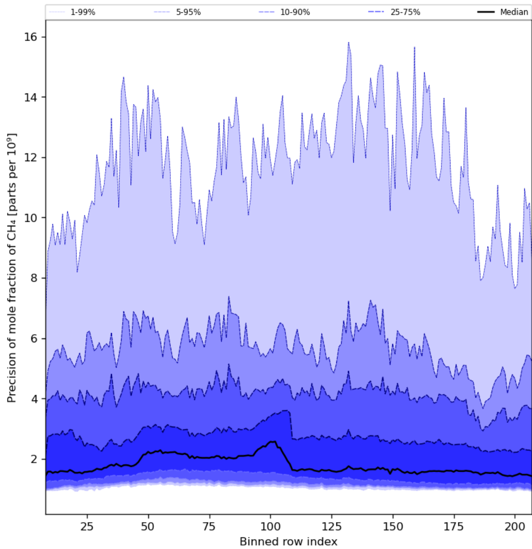
Figure 35: Along track statistics of “Precision of mole fraction of CH 4 ” for 2024-05-12 to 2024-05-13
