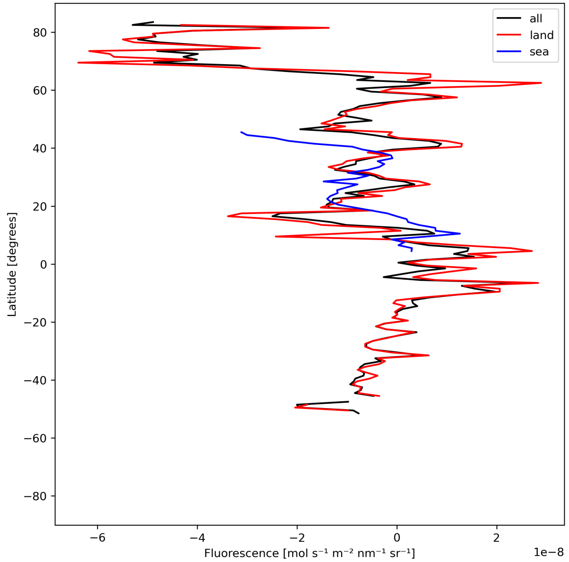
Figure 21: Zonal average of “Fluorescence” for 2024-05-12 to 2024-05-13.
