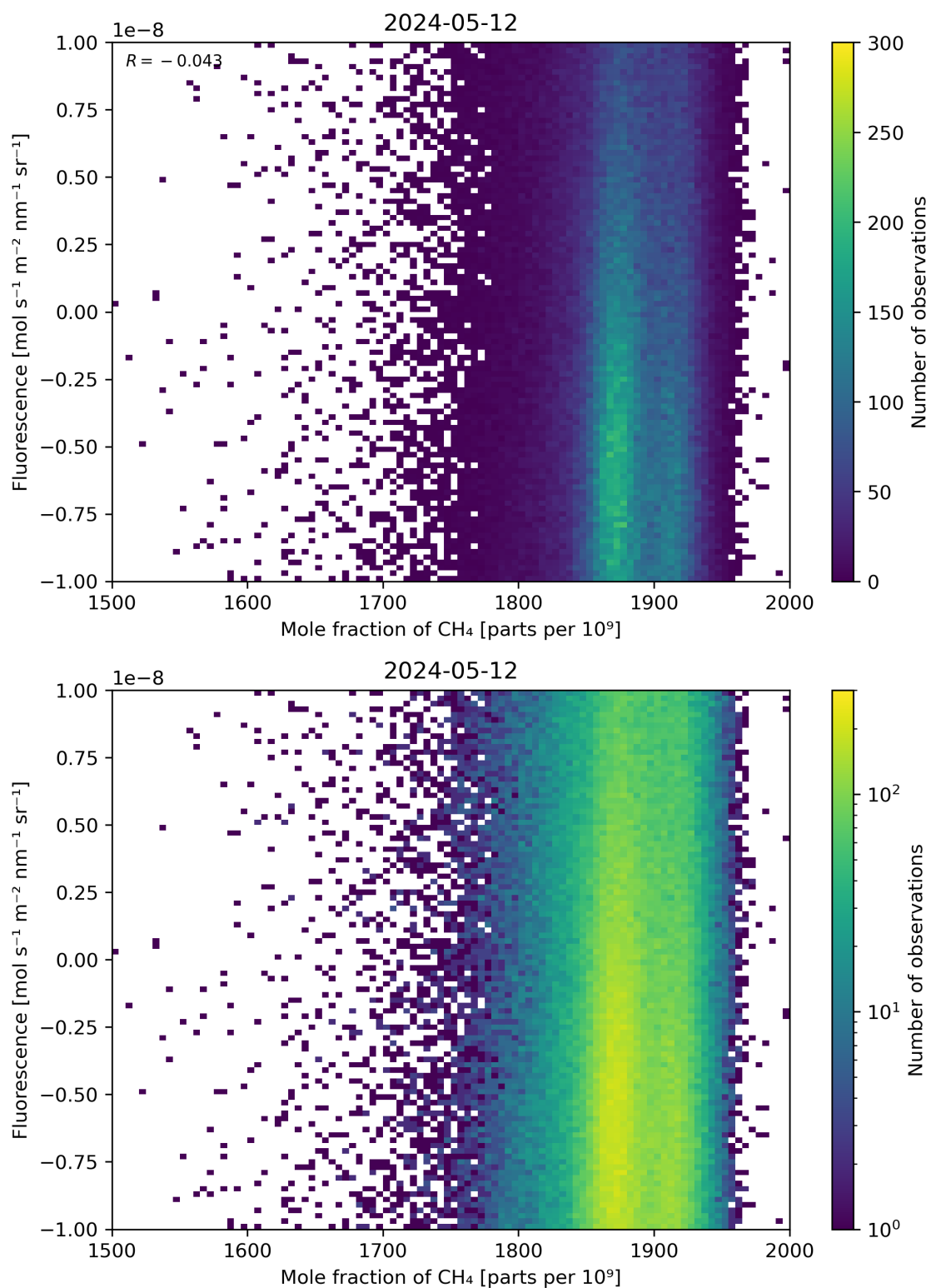
Figure 73: Scatter density plot of “Mole fraction of \text{CH}_4 ” against “Fluorescence” for 2024-05-12 to 2024-05-13.
