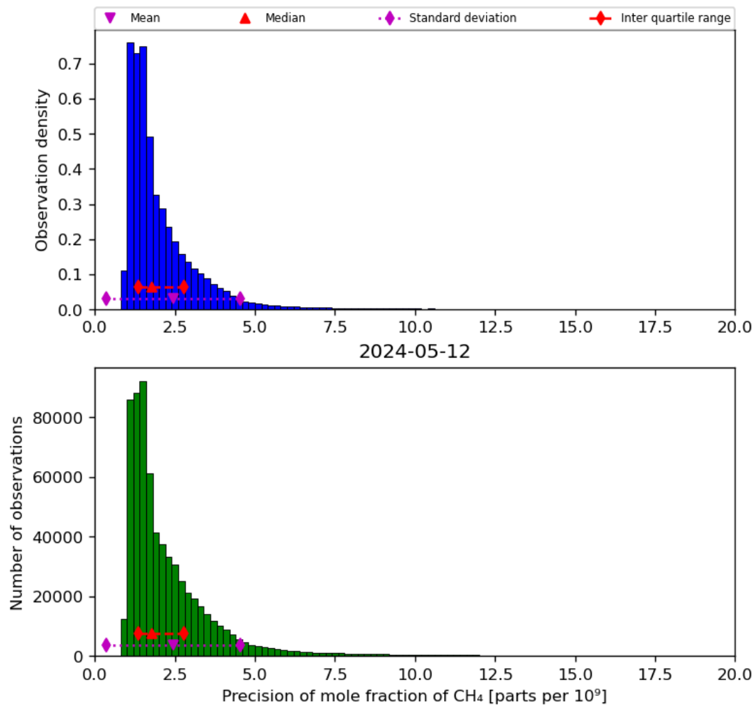
Figure 24: Histogram of “Precision of mole fraction of CH 4 ” for 2024-05-12 to 2024-05-13
