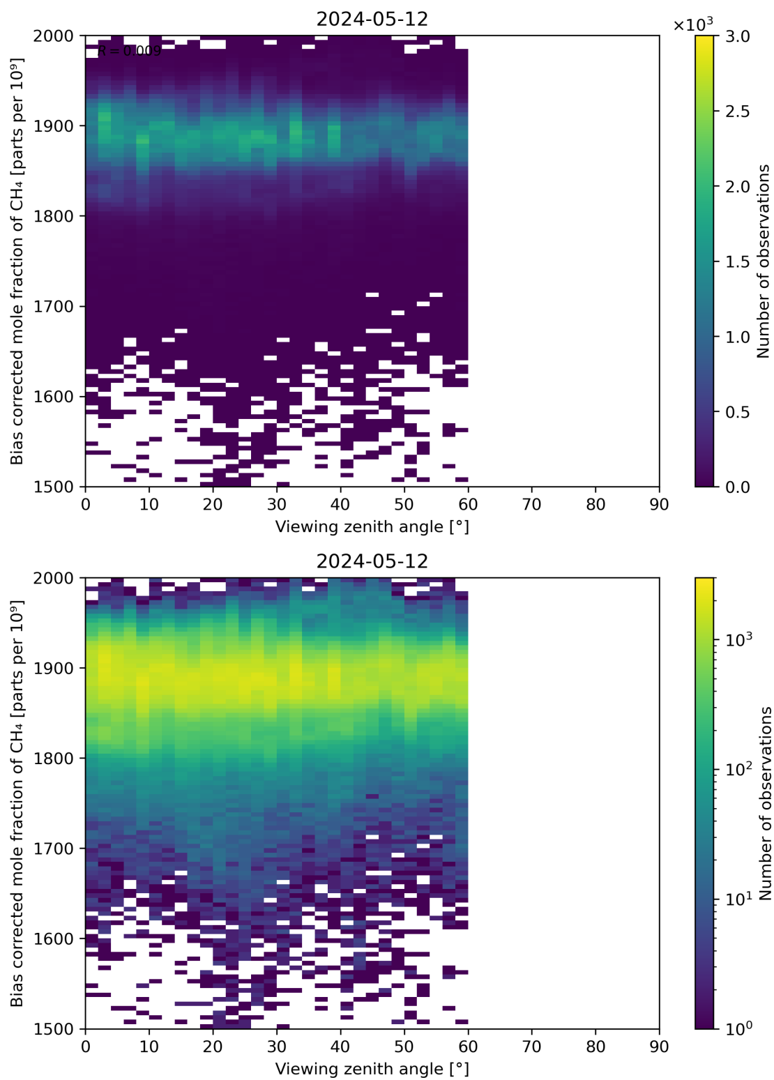
Figure 111: Scatter density plot of “Viewing zenith angle” against “Bias corrected mole fraction of CH 4 ” for 2024-05-12 to 2024-05-13.
