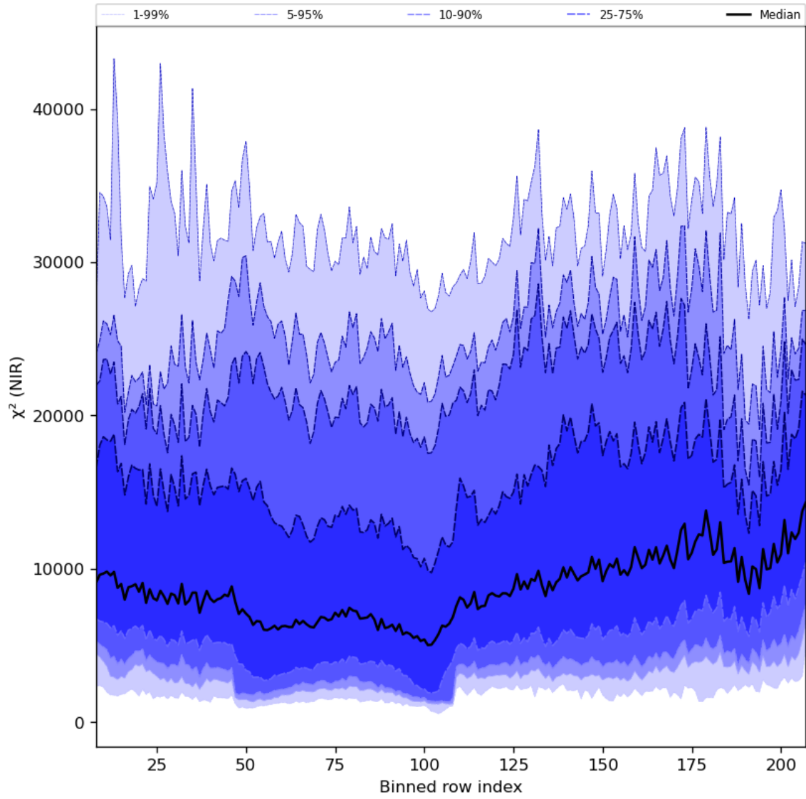
Figure 40: Along track statistics of “ \chi^2 (NIR)” for 2024-05-12 to 2024-05-13
