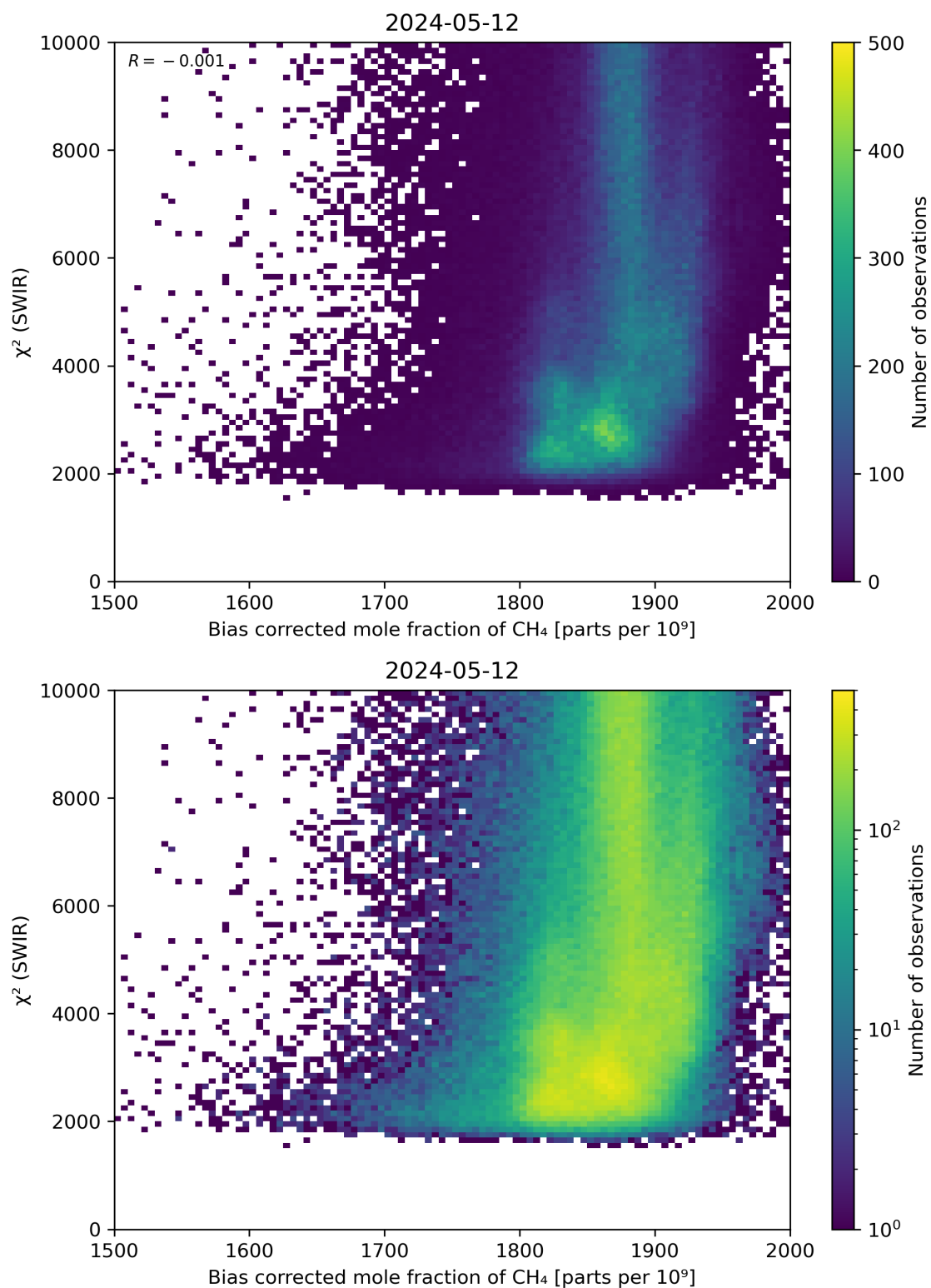
Figure 64: Scatter density plot of “Bias corrected mole fraction of CH 4 ” against “ \chi^2 (SWIR)” for 2024-05-12 to 2024-05-13.
