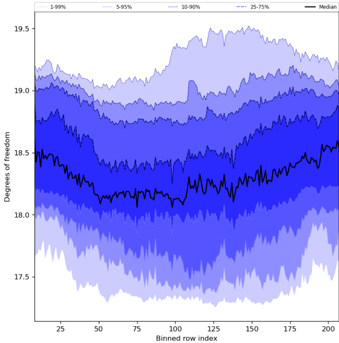
Figure 41: Along track statistics of “Degrees of freedom” for 2024-05-12 to 2024-05-13
