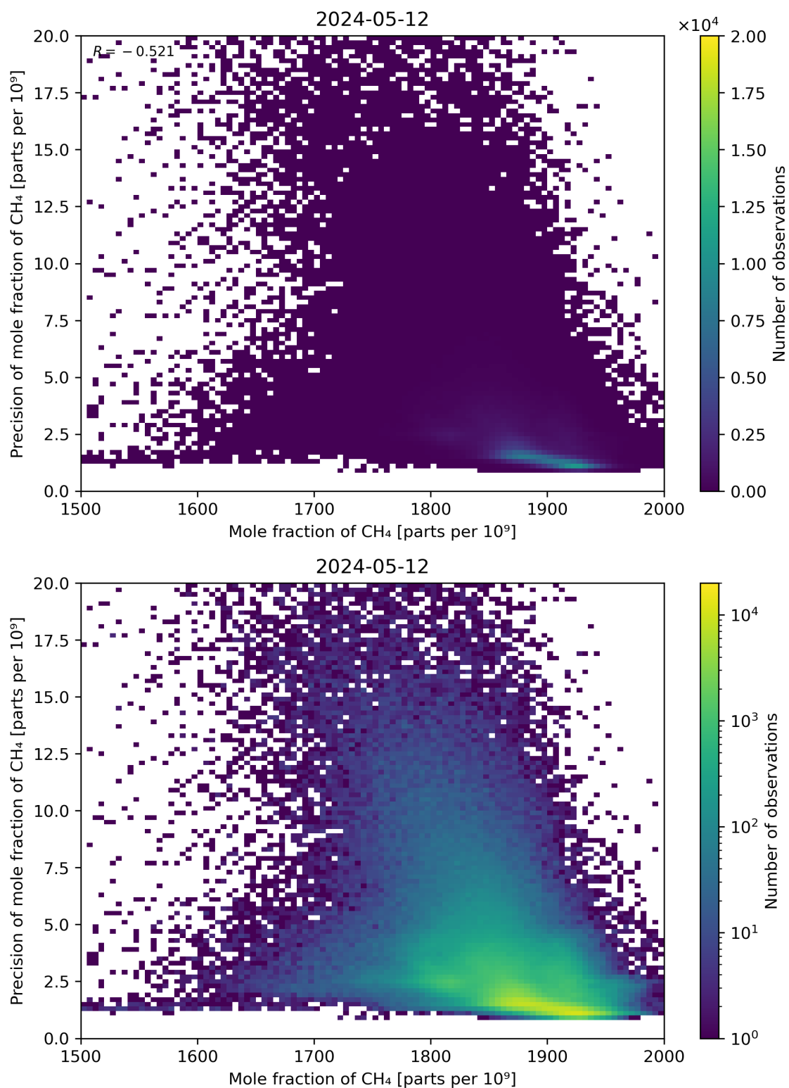
Figure 75: Scatter density plot of “Mole fraction of CH 4 ” against “Precision of mole fraction of CH 4 ” for 2024-05-12 to 2024-05-13.
