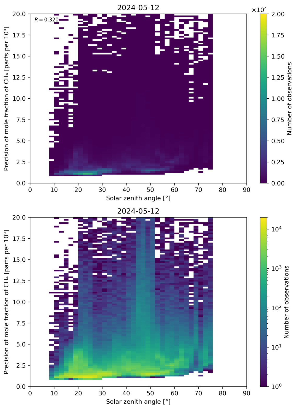
Figure 101: Scatter density plot of “Solar zenith angle” against “Precision of mole fraction of CH 4 ” for 2024-05-12 to 2024-05-13.
