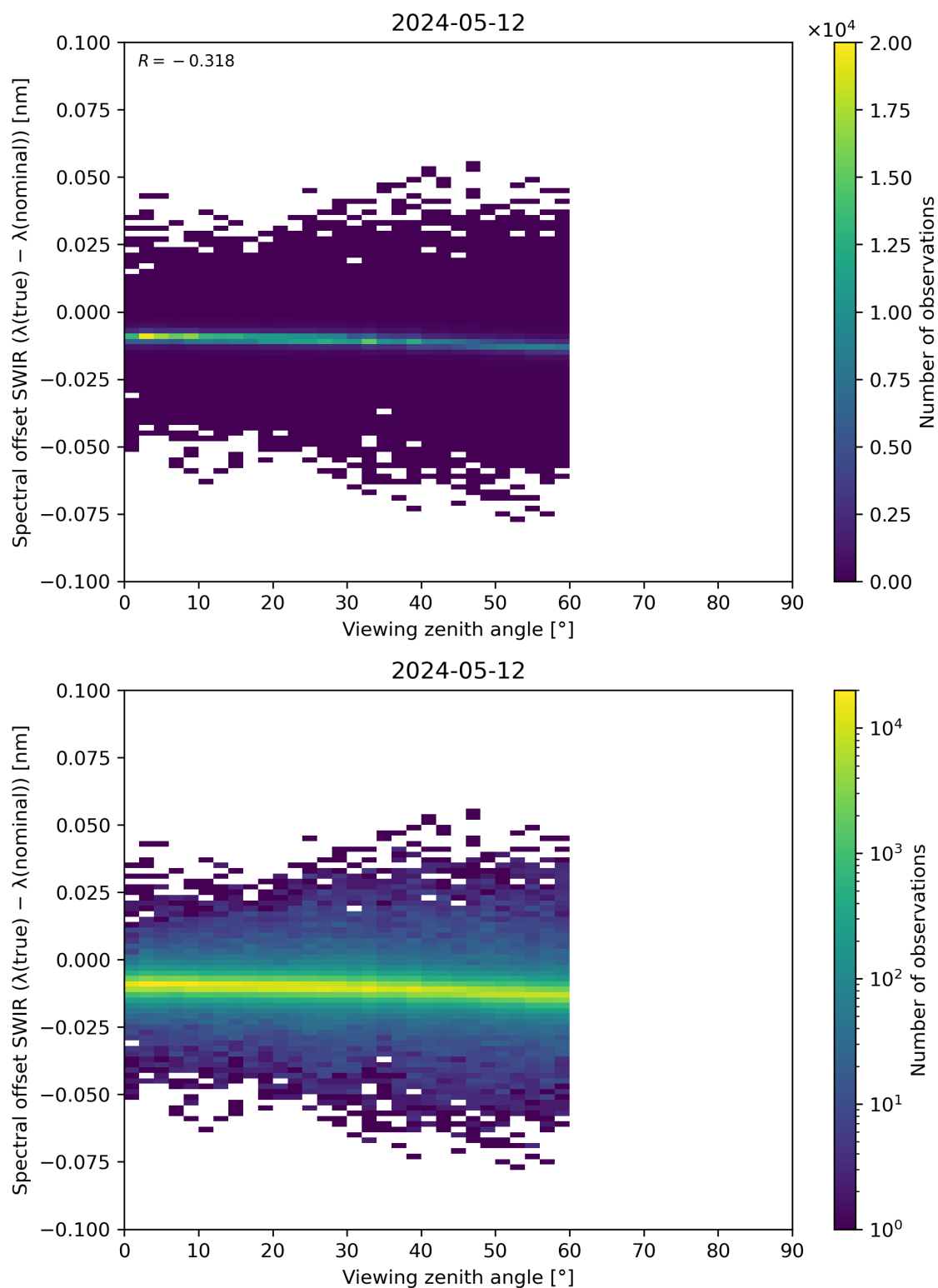
Figure 116: Scatter density plot of “Viewing zenith angle” against “Spectral offset SWIR ( \lambda(\text{true}) - \lambda(\text{nominal}) )” for 2024-05-12 to 2024-05-13.
