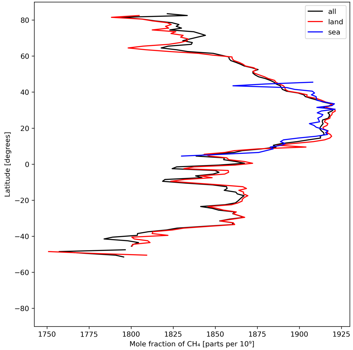
Figure 12: Zonal average of “Mole fraction of CH 4 ” for 2024-05-12 to 2024-05-13.
