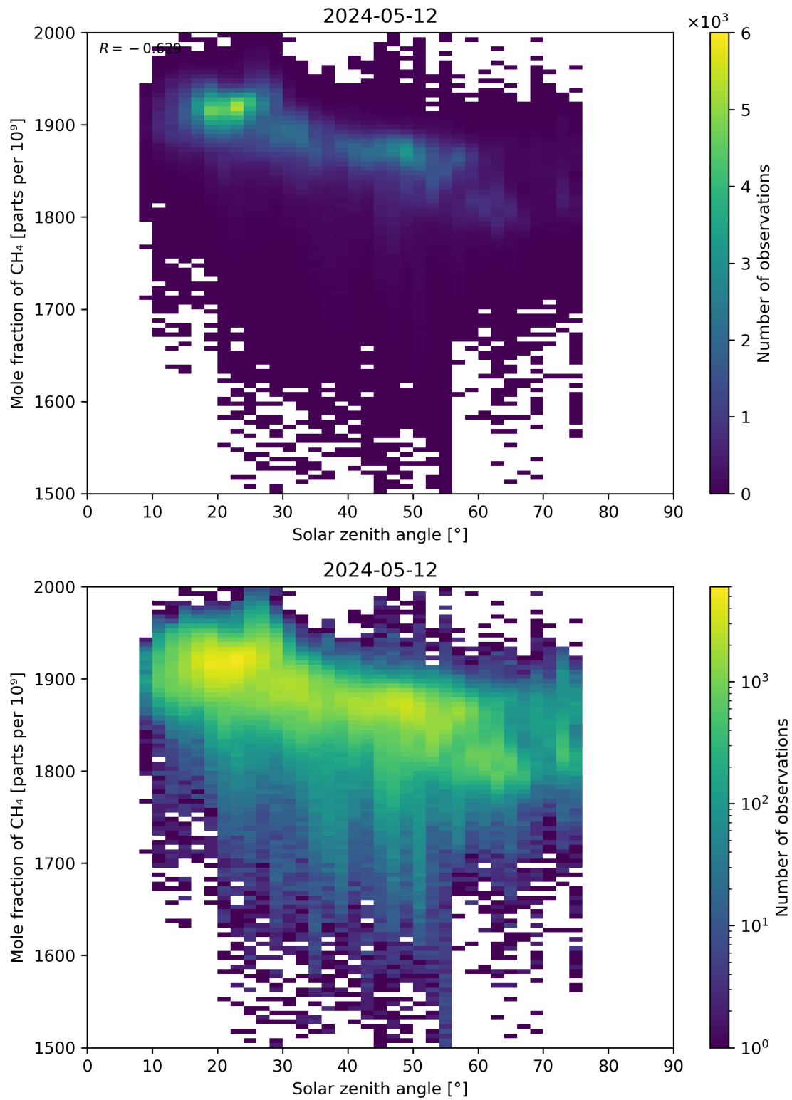
Figure 99: Scatter density plot of “Solar zenith angle” against “Mole fraction of CH 4 ” for 2024-05-12 to 2024-05-13.
