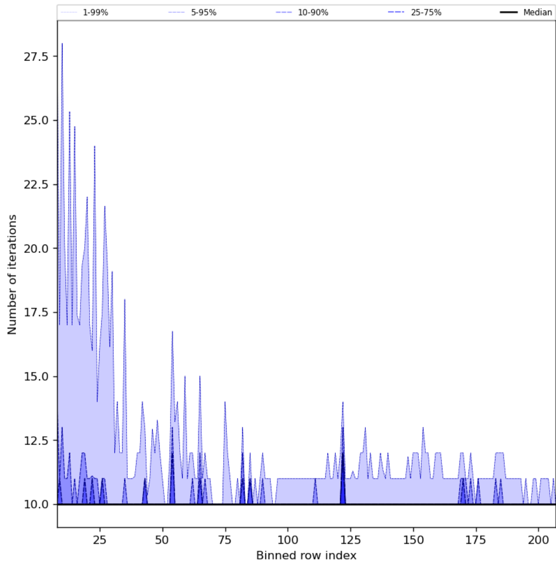
Figure 42: Along track statistics of “Number of iterations” for 2024-05-12 to 2024-05-13
