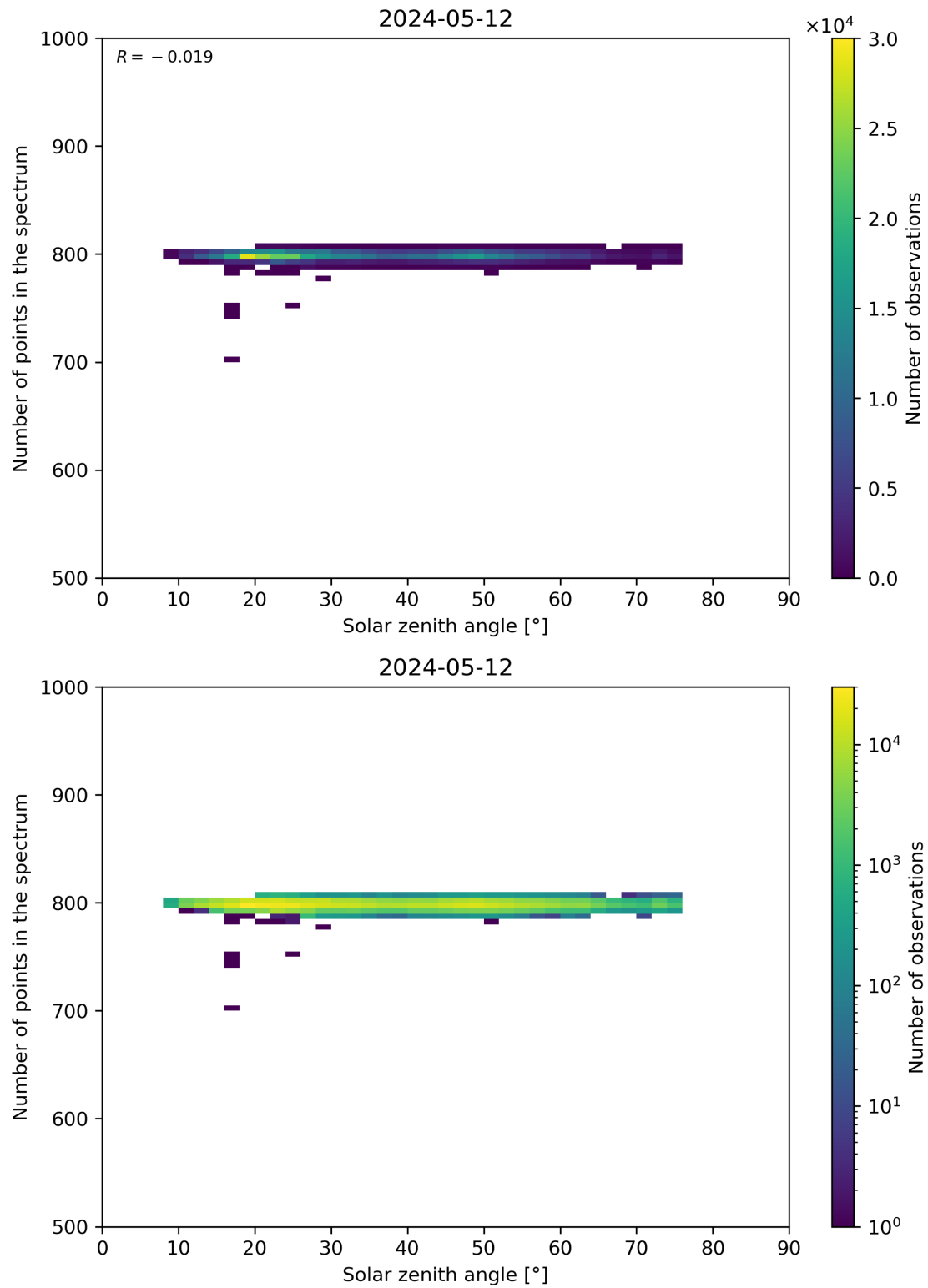
Figure 103: Scatter density plot of “Solar zenith angle” against “Number of points in the spectrum” for 2024-05-12 to 2024-05-13.
