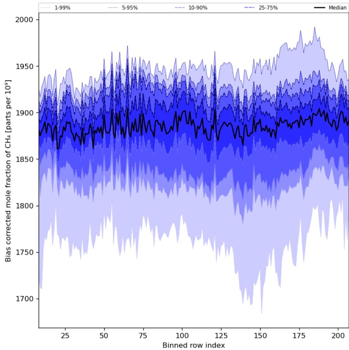
Figure 36: Along track statistics of “Bias corrected mole fraction of CH 4 ” for 2024-05-12 to 2024-05-13
