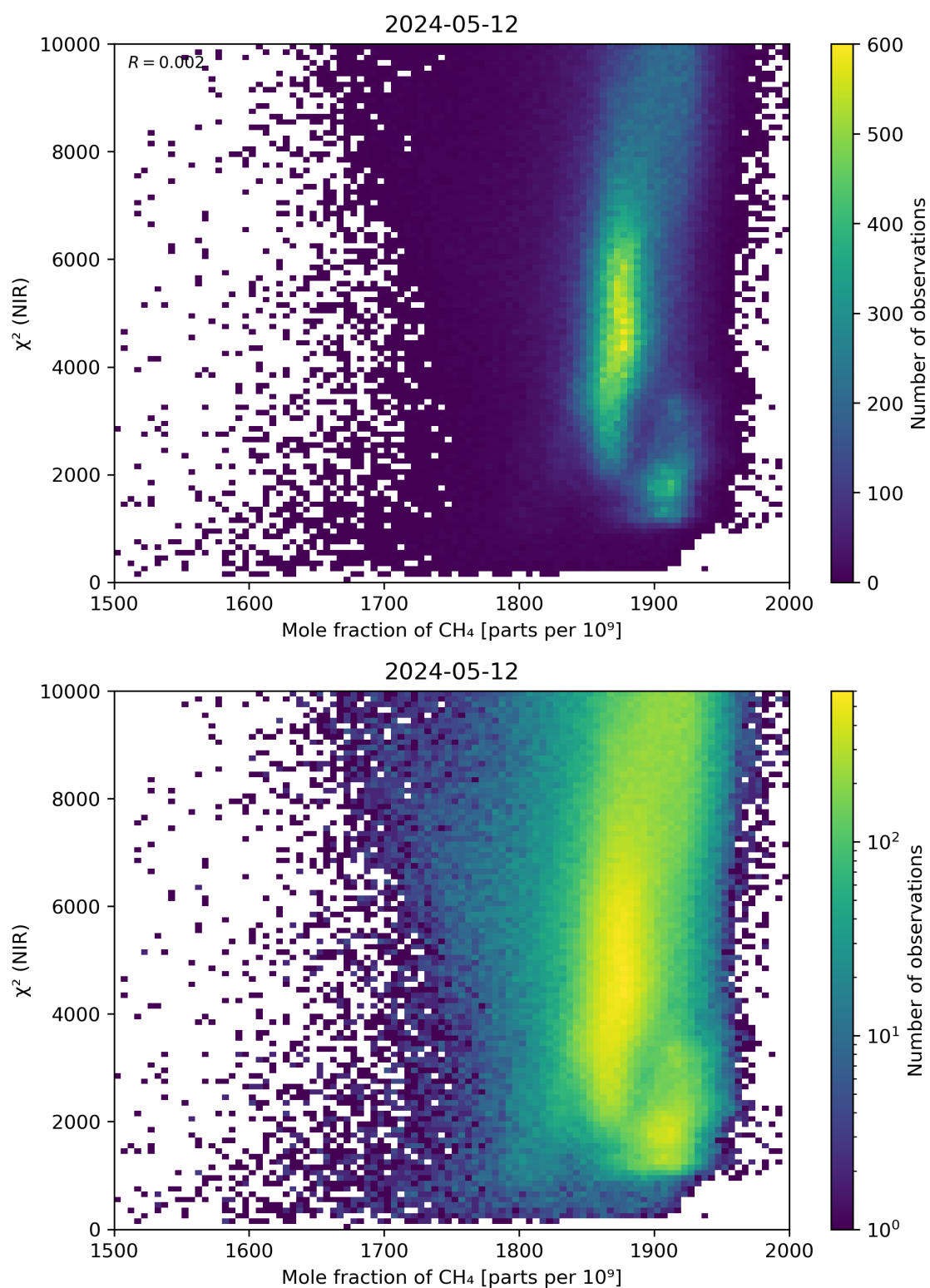
Figure 70: Scatter density plot of “Mole fraction of \text{CH}_4 ” against “ \chi^2 (NIR)” for 2024-05-12 to 2024-05-13.
