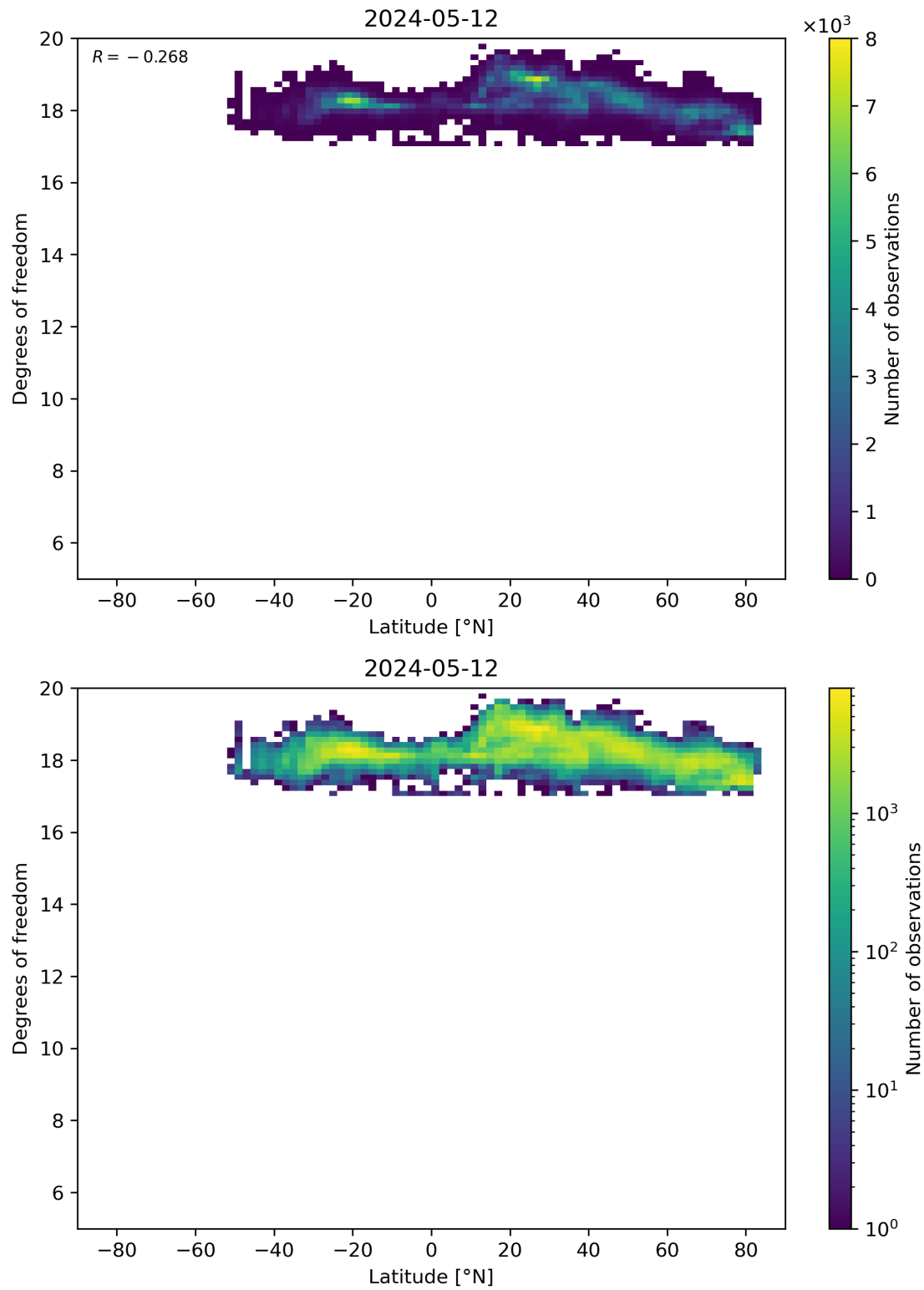
Figure 55: Scatter density plot of “Latitude” against “Degrees of freedom” for 2024-05-12 to 2024-05-13.
