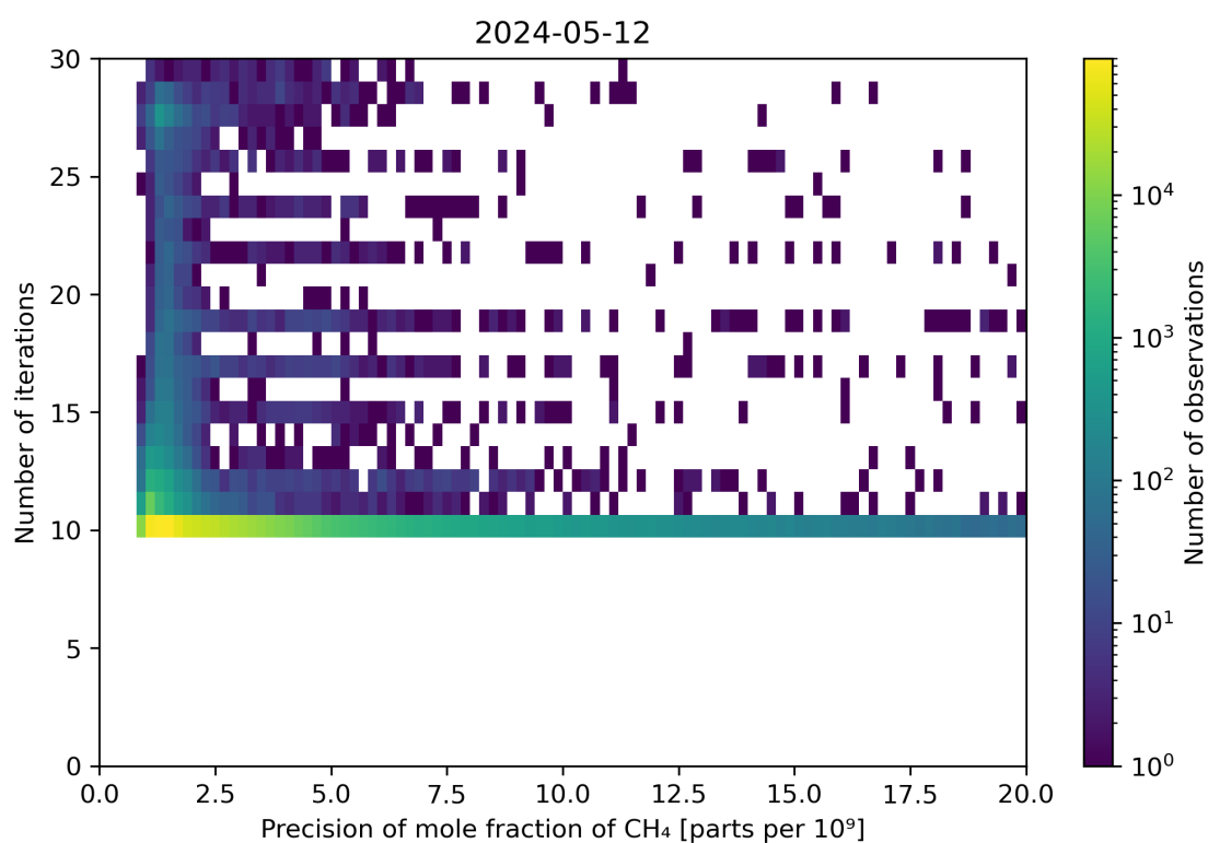
Figure 83: Scatter density plot of “Precision of mole fraction of CH 4 ” against “Number of iterations” for 2024-05-12 to 2024-05-13.
