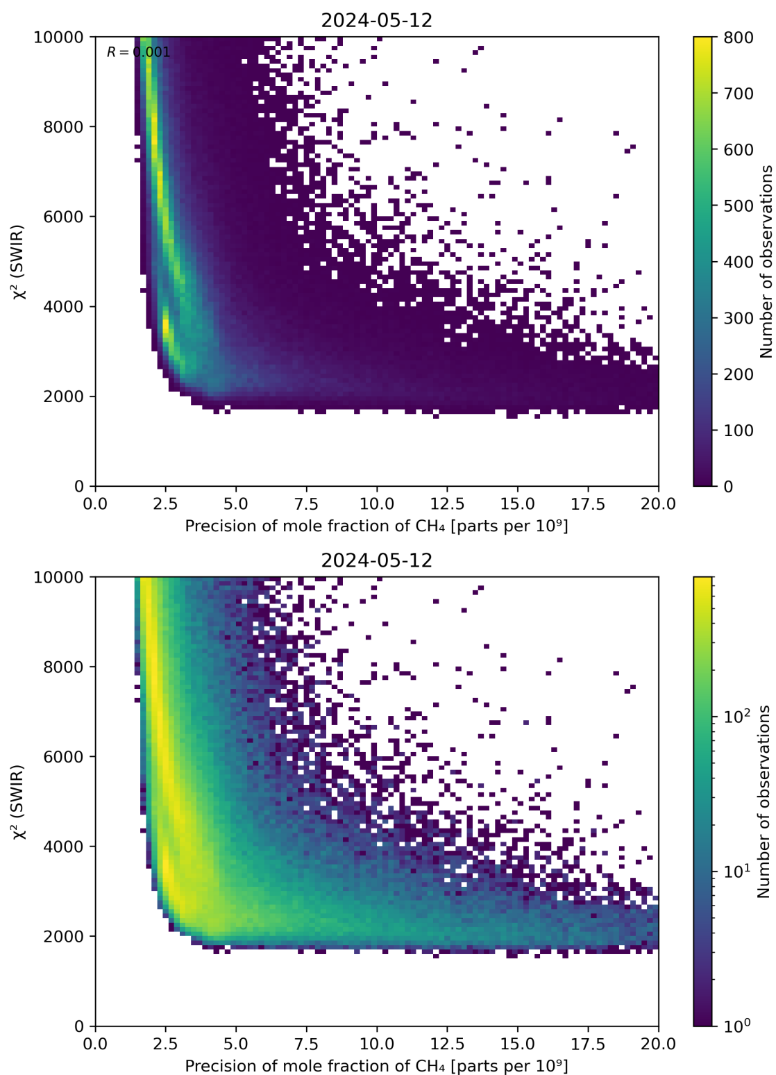
Figure 79: Scatter density plot of “Precision of mole fraction of CH 4 ” against “ \chi^2 (SWIR)” for 2024-05-12 to 2024-05-13.
