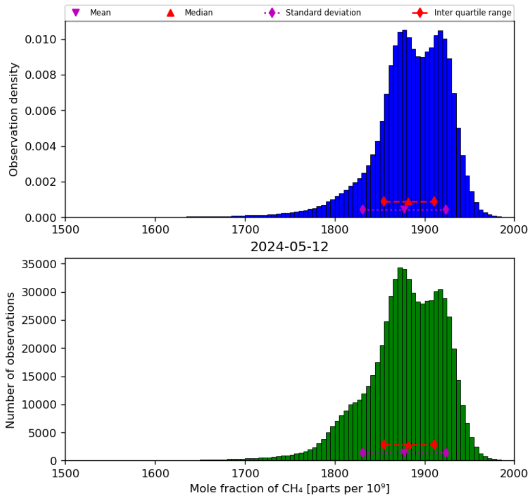
Figure 23: Histogram of “Mole fraction of CH 4 ” for 2024-05-12 to 2024-05-13
