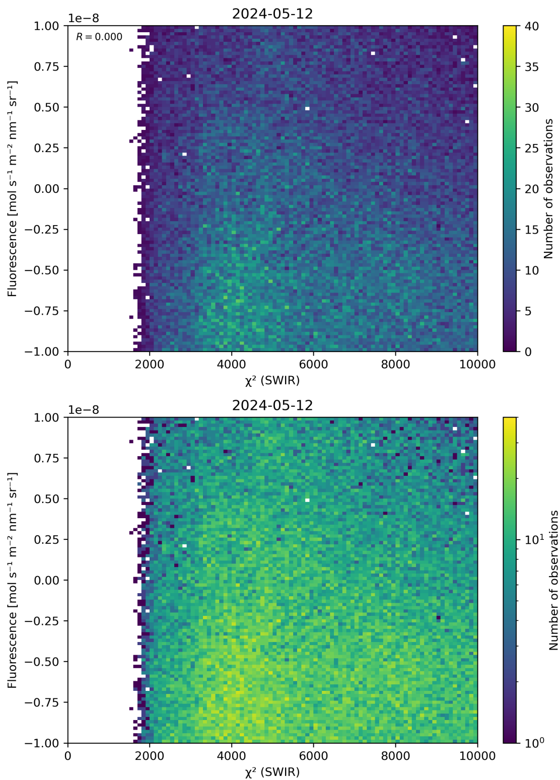
Figure 49: Scatter density plot of “ \chi^2 (SWIR)” against “Fluorescence” for 2024-05-12 to 2024-05-13.
