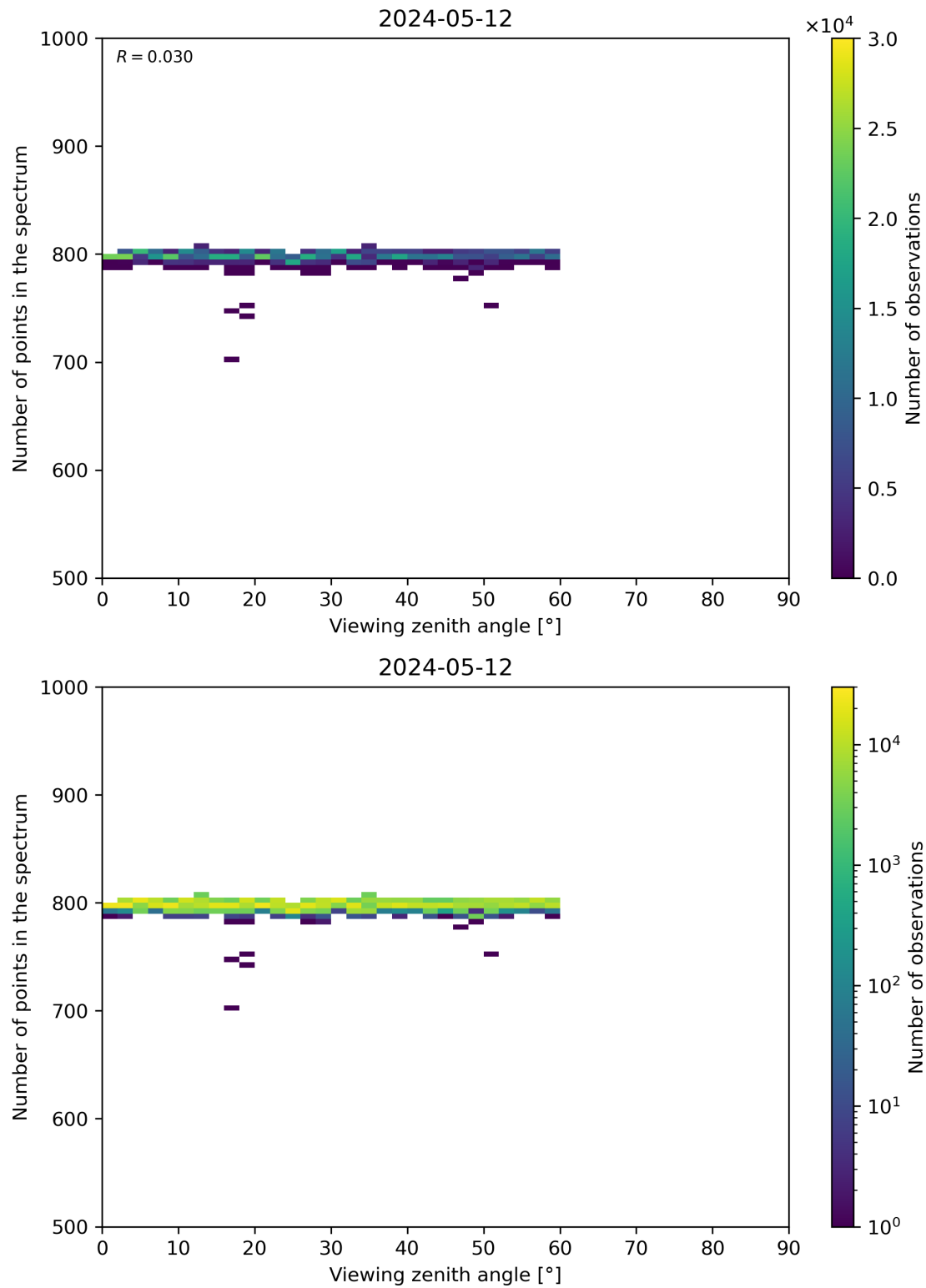
Figure 114: Scatter density plot of “Viewing zenith angle” against “Number of points in the spectrum” for 2024-05-12 to 2024-05-13.
