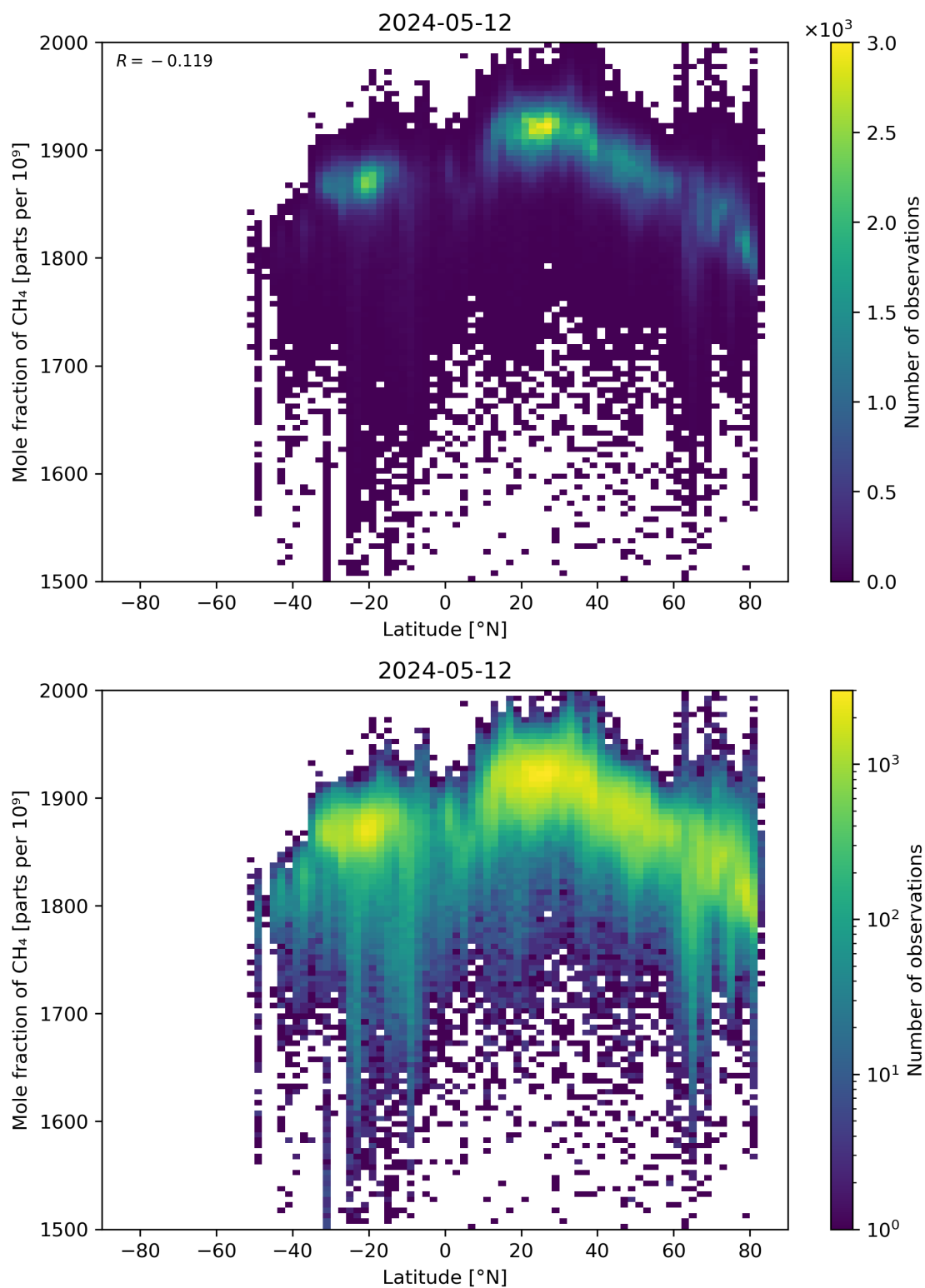
Figure 57: Scatter density plot of “Latitude” against “Mole fraction of CH 4 ” for 2024-05-12 to 2024-05-13.
