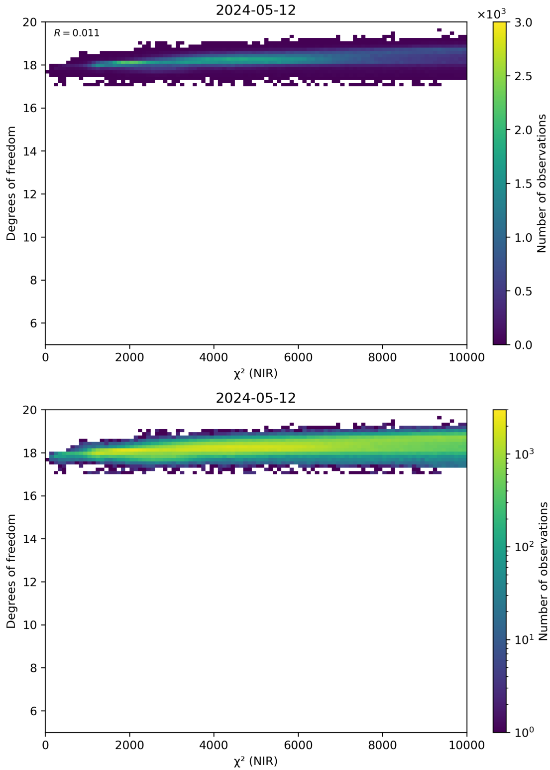
Figure 44: Scatter density plot of “ \chi^2 (NIR)” against “Degrees of freedom” for 2024-05-12 to 2024-05-13.
