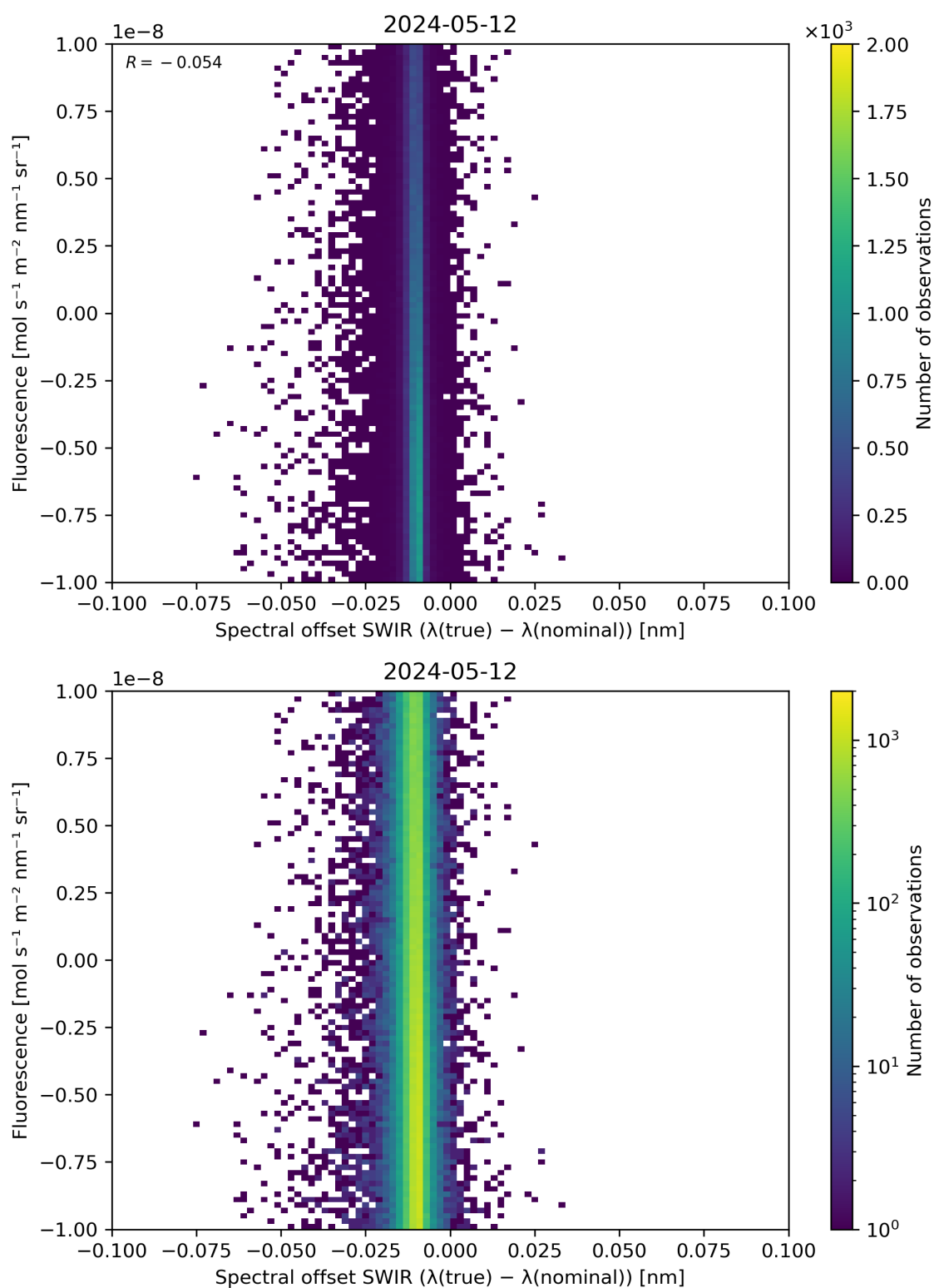
Figure 120: Scatter density plot of “Spectral offset SWIR ( \lambda(\text{true}) - \lambda(\text{nominal}) )” against “Fluorescence” for 2024-05-12 to 2024-05-13.
