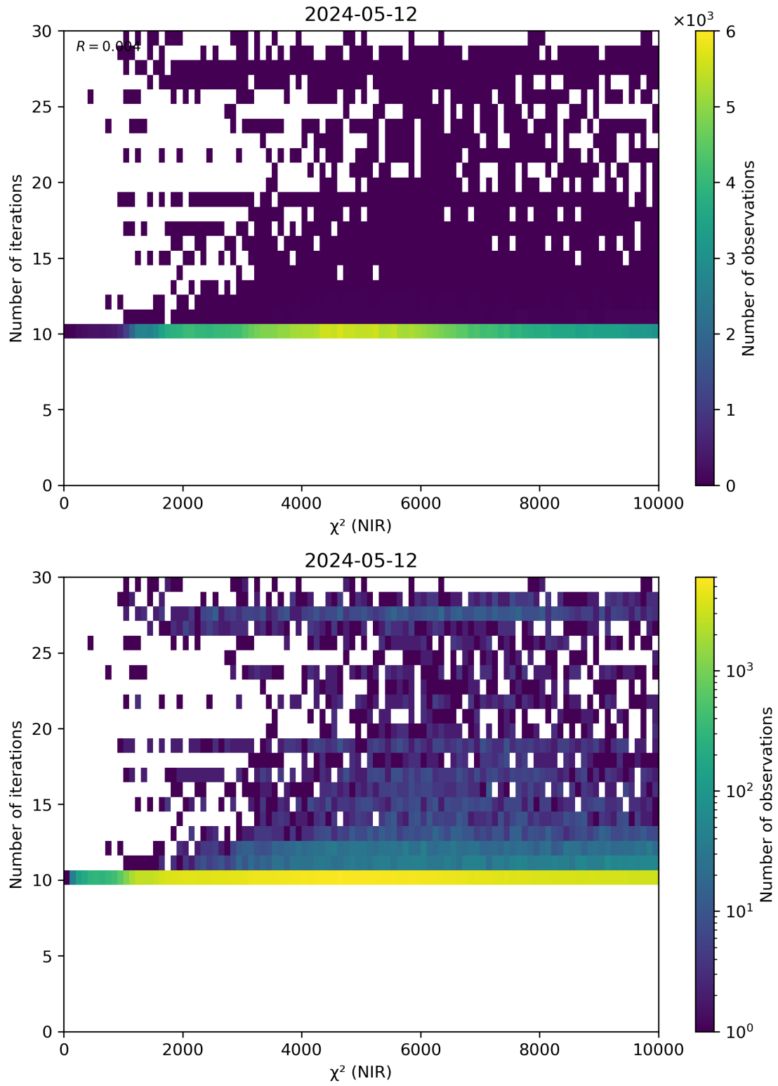
Figure 46: Scatter density plot of “ \chi^2 (NIR)” against “Number of iterations” for 2024-05-12 to 2024-05-13.
