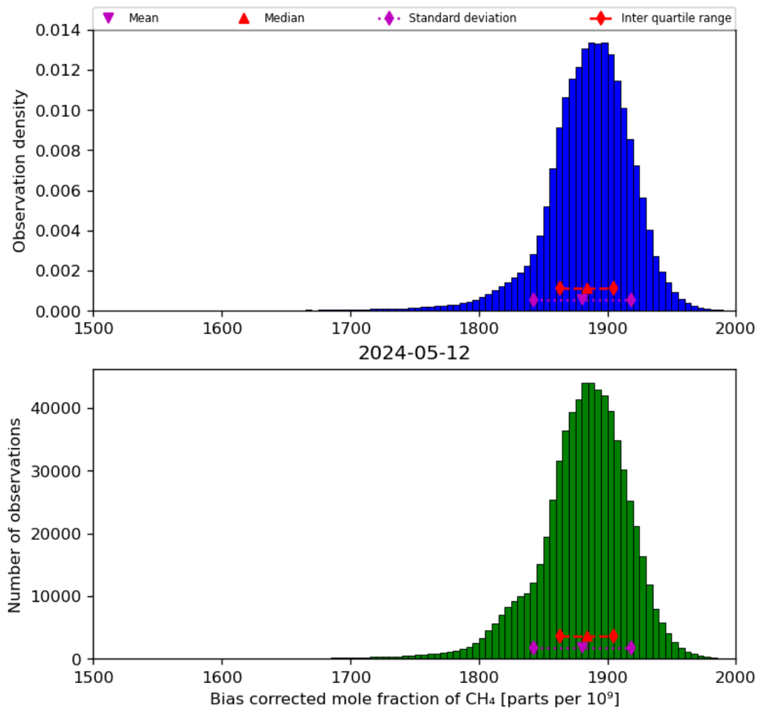
Figure 25: Histogram of “Bias corrected mole fraction of CH 4 ” for 2024-05-12 to 2024-05-13
