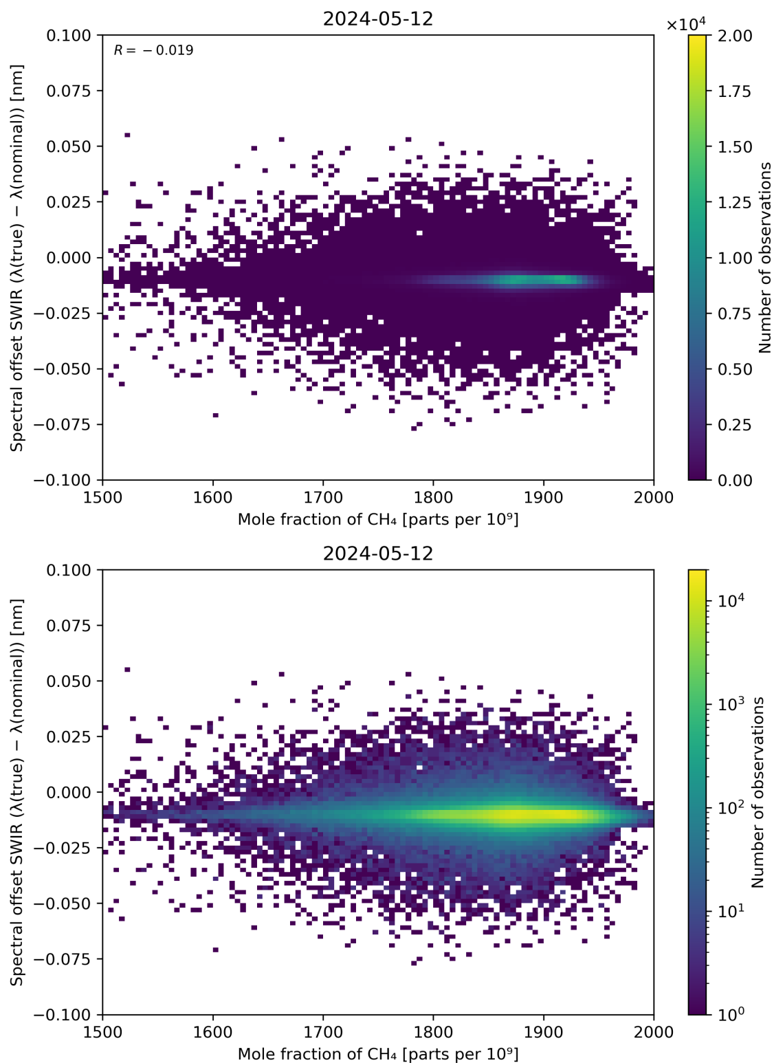
Figure 86: Scatter density plot of “Mole fraction of CH 4 ” against “Spectral offset SWIR ( \lambda(\text{true}) - \lambda(\text{nominal}) )” for 2024-05-12 to 2024-05-13.
