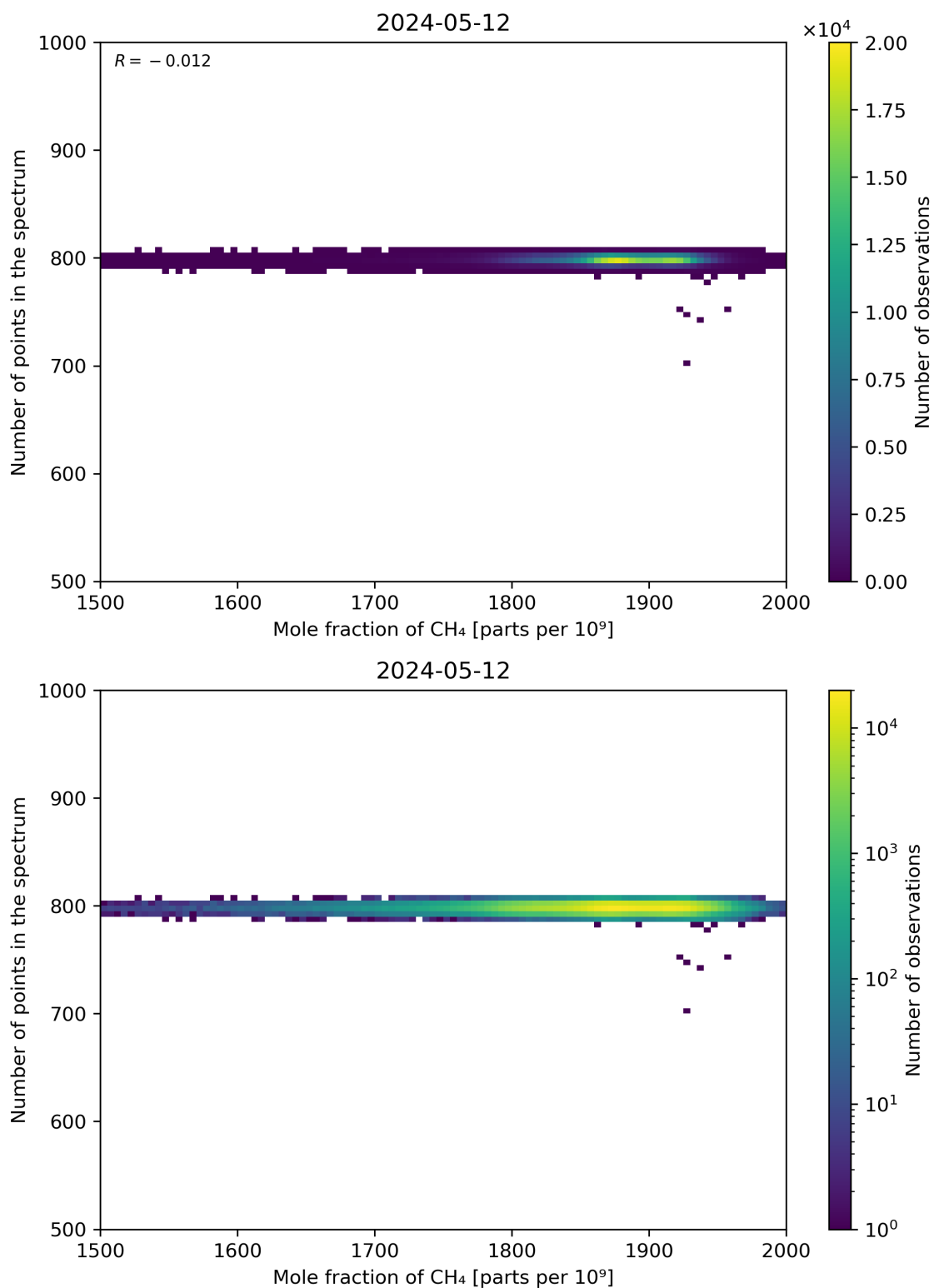
Figure 77: Scatter density plot of “Mole fraction of CH 4 ” against “Number of points in the spectrum” for 2024-05-12 to 2024-05-13.
