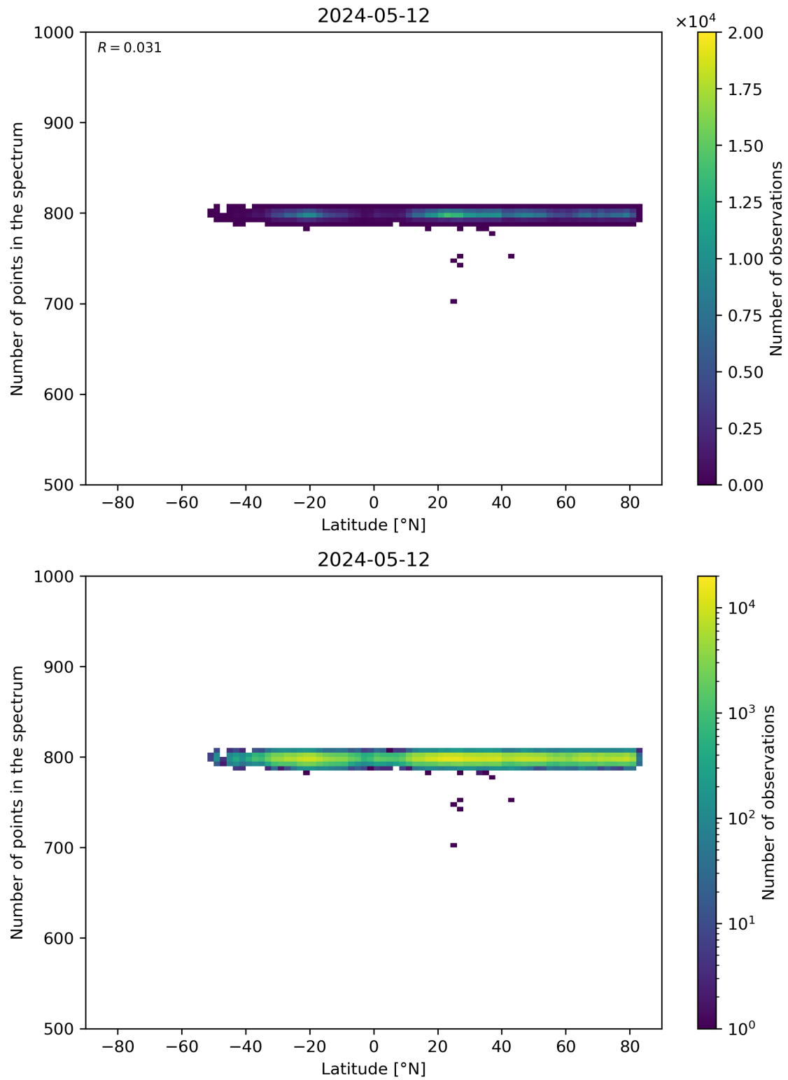
Figure 61: Scatter density plot of “Latitude” against “Number of points in the spectrum” for 2024-05-12 to 2024-05-13.
