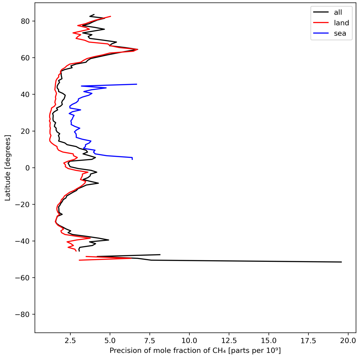
Figure 13: Zonal average of “Precision of mole fraction of CH 4 ” for 2024-05-12 to 2024-05-13.
