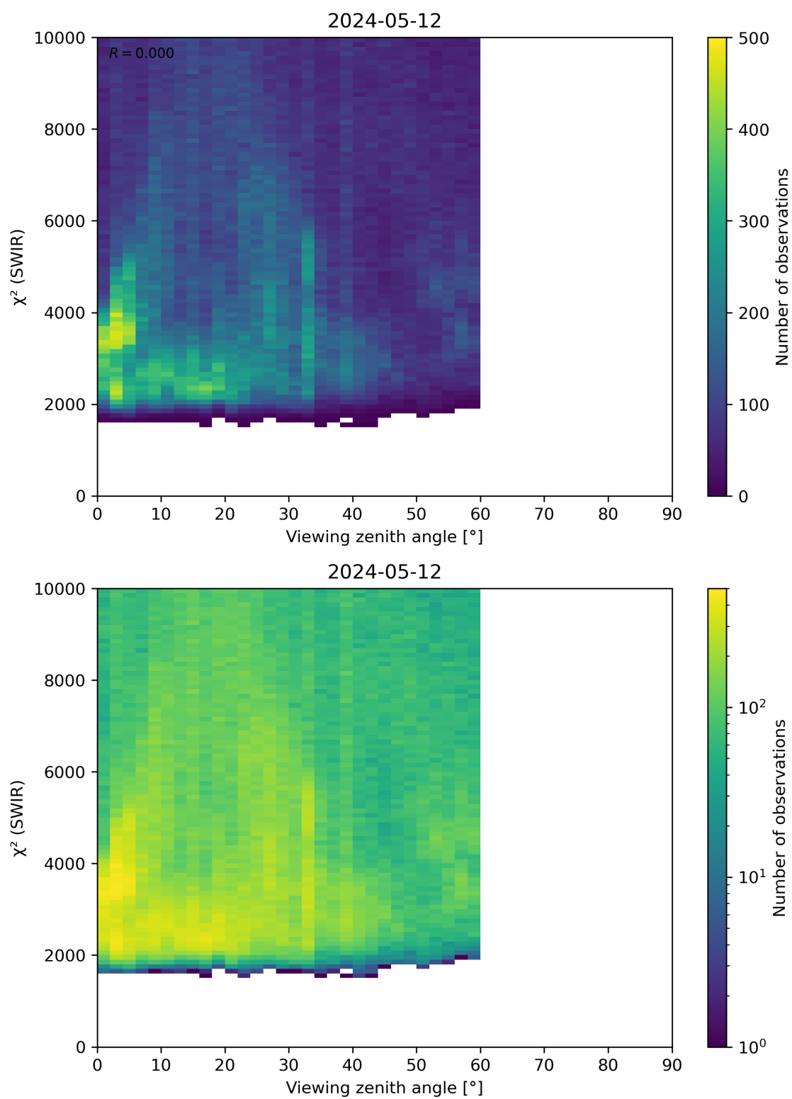
Figure 106: Scatter density plot of “Viewing zenith angle” against “ \chi^2 (SWIR)” for 2024-05-12 to 2024-05-13.
