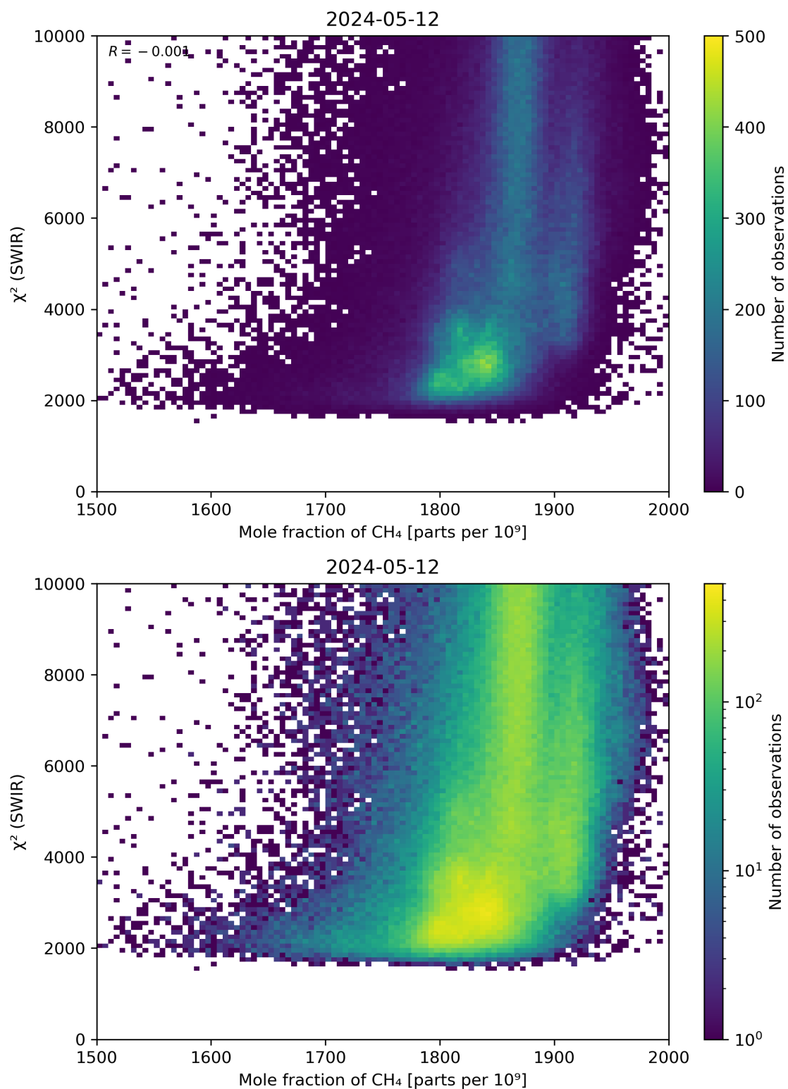
Figure 71: Scatter density plot of “Mole fraction of \text{CH}_4 ” against “ \chi^2 (SWIR)” for 2024-05-12 to 2024-05-13.
