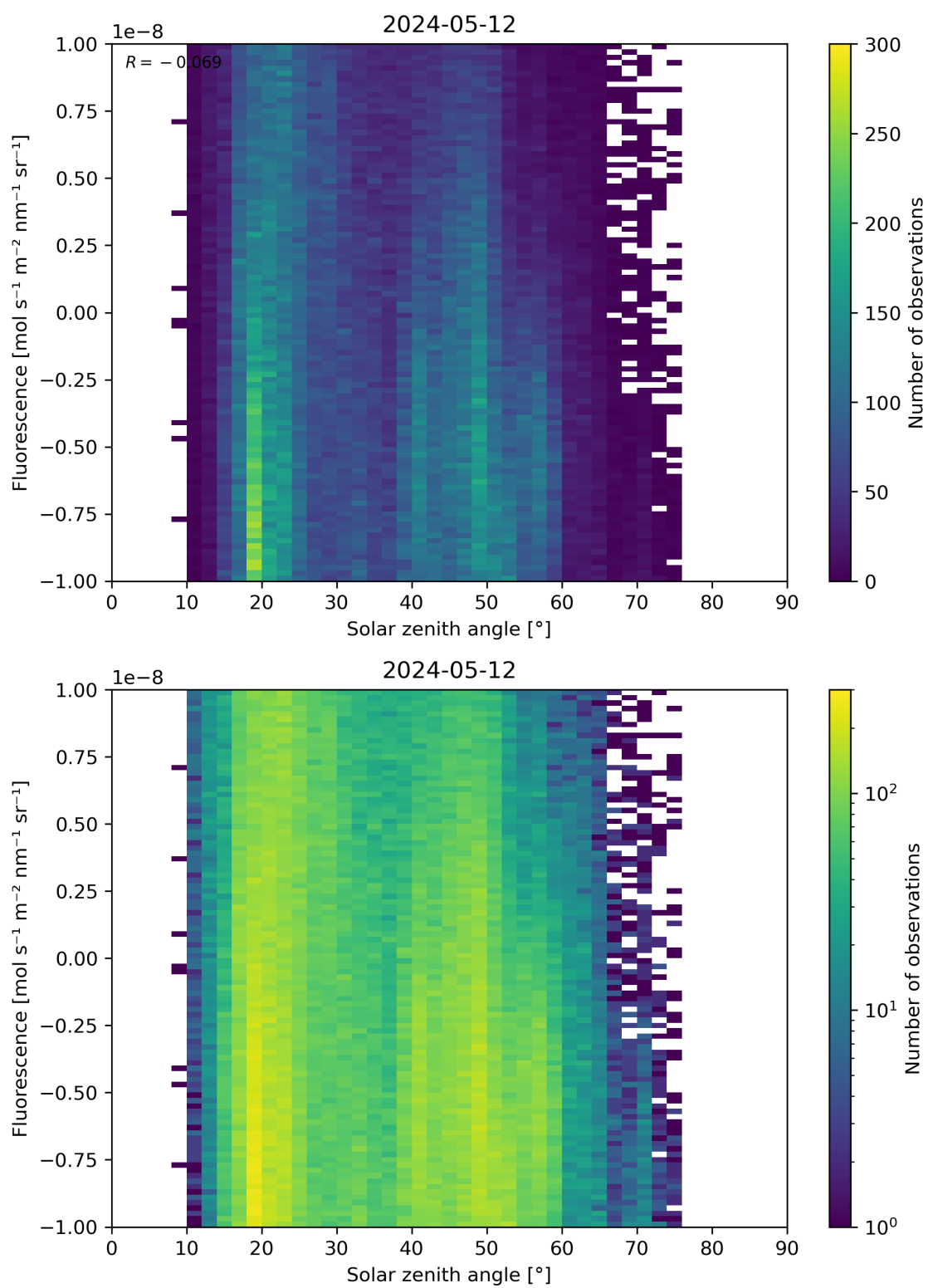
Figure 97: Scatter density plot of “Solar zenith angle” against “Fluorescence” for 2024-05-12 to 2024-05-13.
