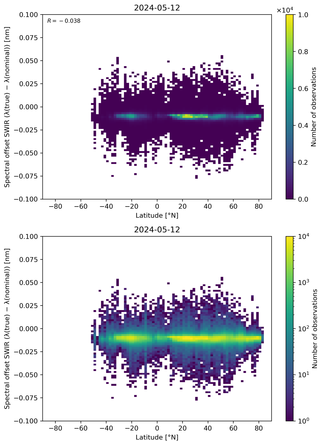
Figure 62: Scatter density plot of “Latitude” against “Spectral offset SWIR ( \lambda(\text{true}) - \lambda(\text{nominal}) )” for 2024-05-12 to 2024-05-13.
