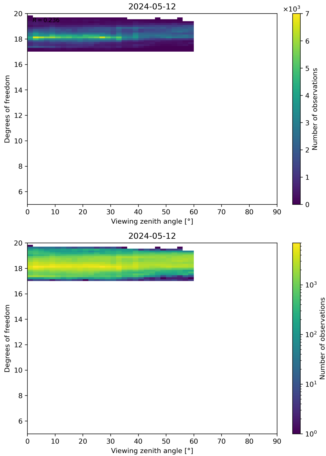
Figure 107: Scatter density plot of “Viewing zenith angle” against “Degrees of freedom” for 2024-05-12 to 2024-05-13.
