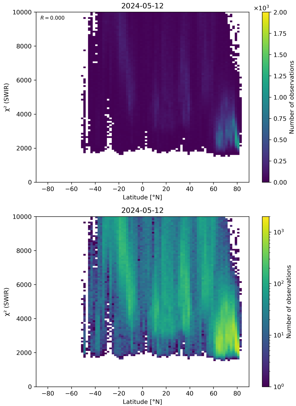
Figure 54: Scatter density plot of “Latitude” against “ \chi^2 (SWIR)” for 2024-05-12 to 2024-05-13.
