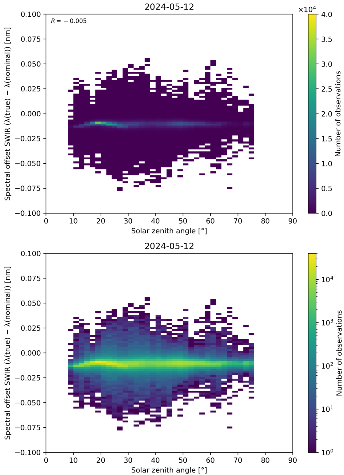
Figure 104: Scatter density plot of “Solar zenith angle” against “Spectral offset SWIR ( \lambda(\text{true}) - \lambda(\text{nominal}) )” for 2024-05-12 to 2024-05-13.
