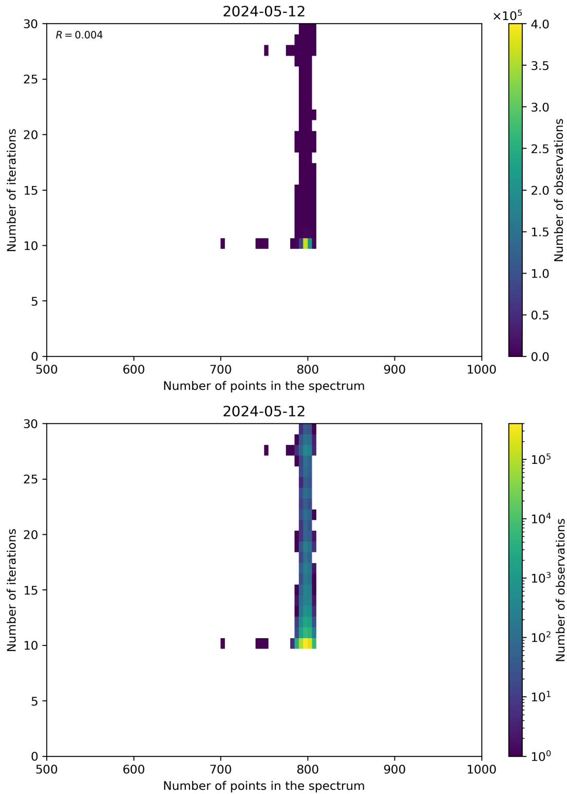
Figure 92: Scatter density plot of “Number of points in the spectrum” against “Number of iterations” for 2024-05-12 to 2024-05-13.
