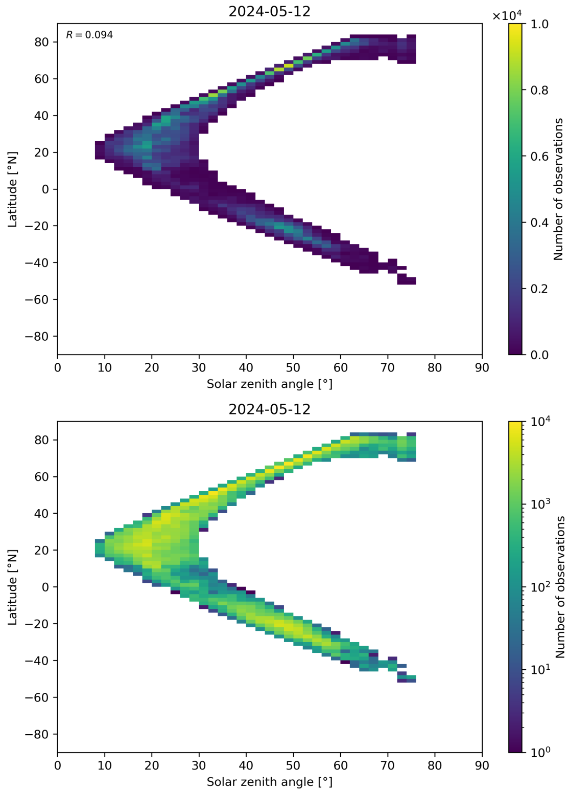
Figure 98: Scatter density plot of “Solar zenith angle” against “Latitude” for 2024-05-12 to 2024-05-13.
