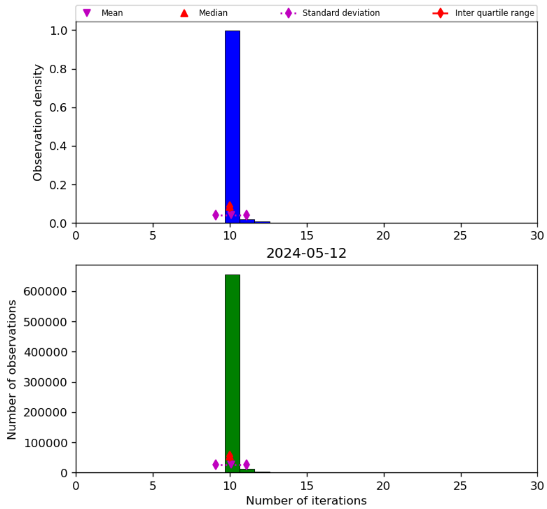
Figure 31: Histogram of “Number of iterations” for 2024-05-12 to 2024-05-13
