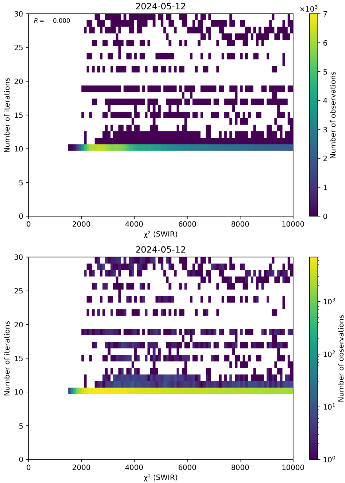
Figure 50: Scatter density plot of “ \chi^2 (SWIR)” against “Number of iterations” for 2024-05-12 to 2024-05-13.
