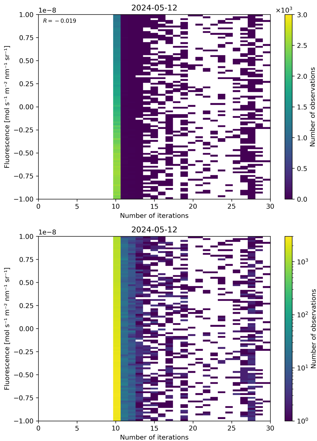
Figure 87: Scatter density plot of “Number of iterations” against “Fluorescence” for 2024-05-12 to 2024-05-13.
