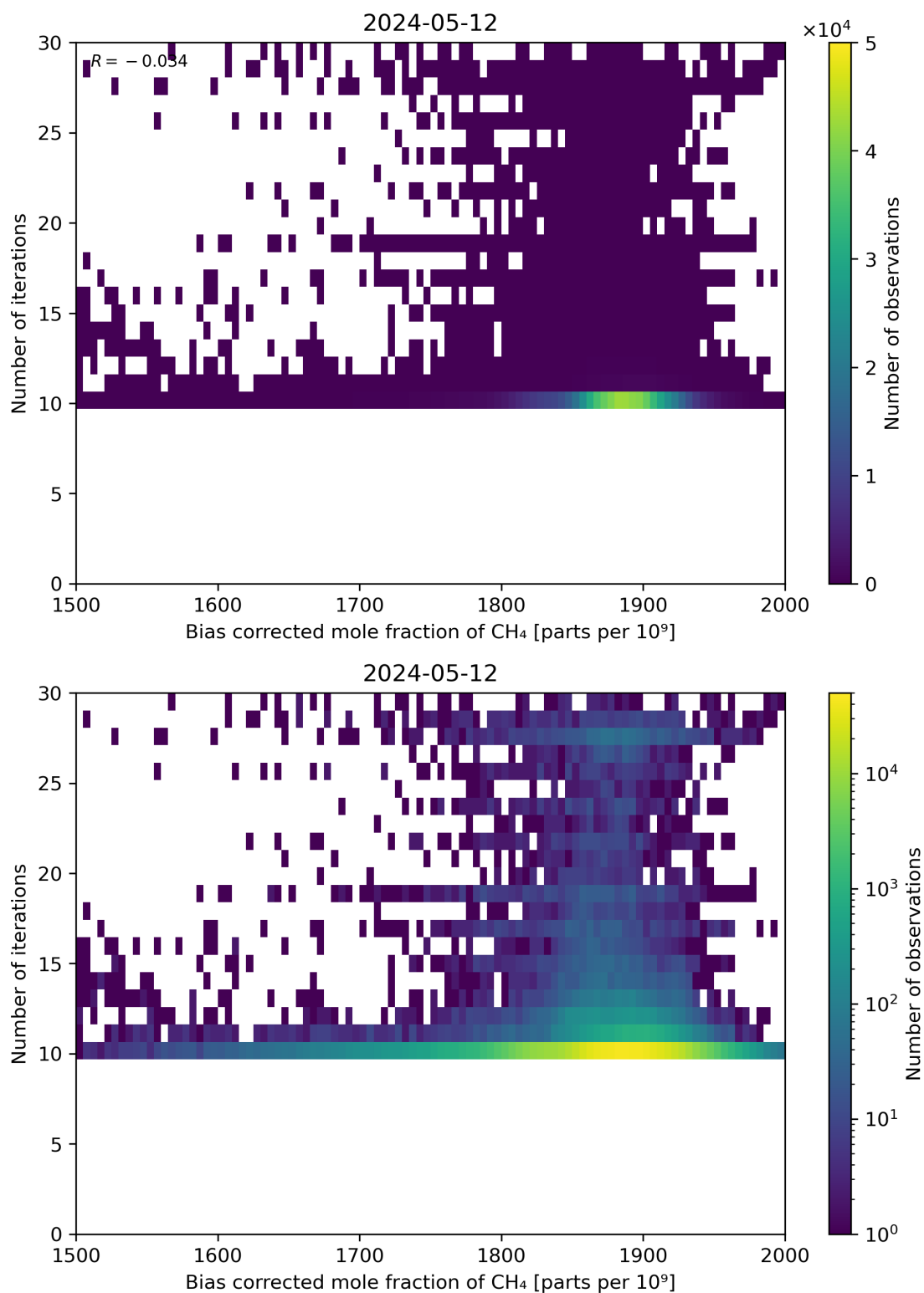
Figure 67: Scatter density plot of “Bias corrected mole fraction of CH 4 ” against “Number of iterations” for 2024-05-12 to 2024-05-13.
