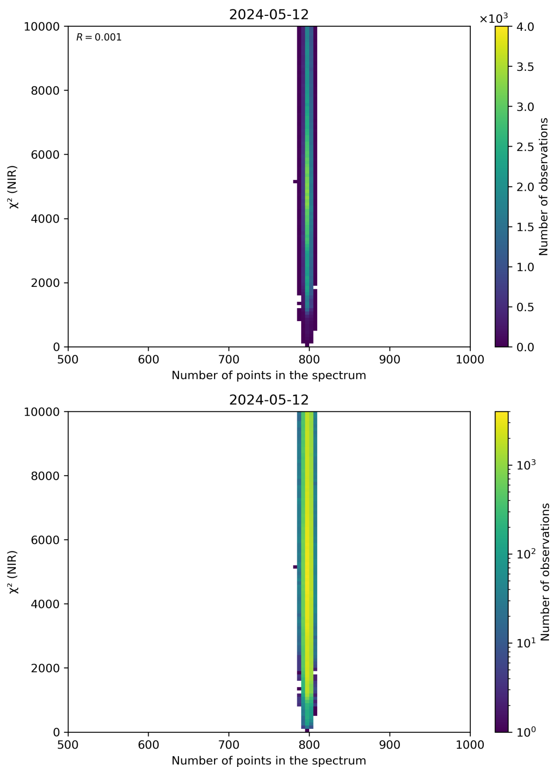
Figure 88: Scatter density plot of “Number of points in the spectrum” against “ \chi^2 (NIR)” for 2024-05-12 to 2024-05-13.
