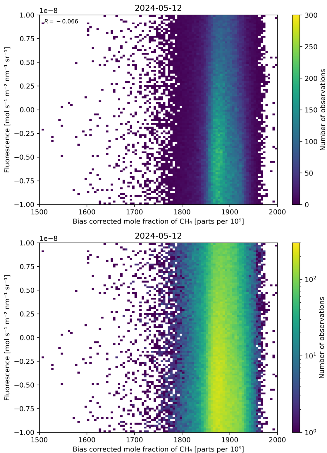
Figure 66: Scatter density plot of “Bias corrected mole fraction of \text{CH}_4 ” against “Fluorescence” for 2024-05-12 to 2024-05-13.
