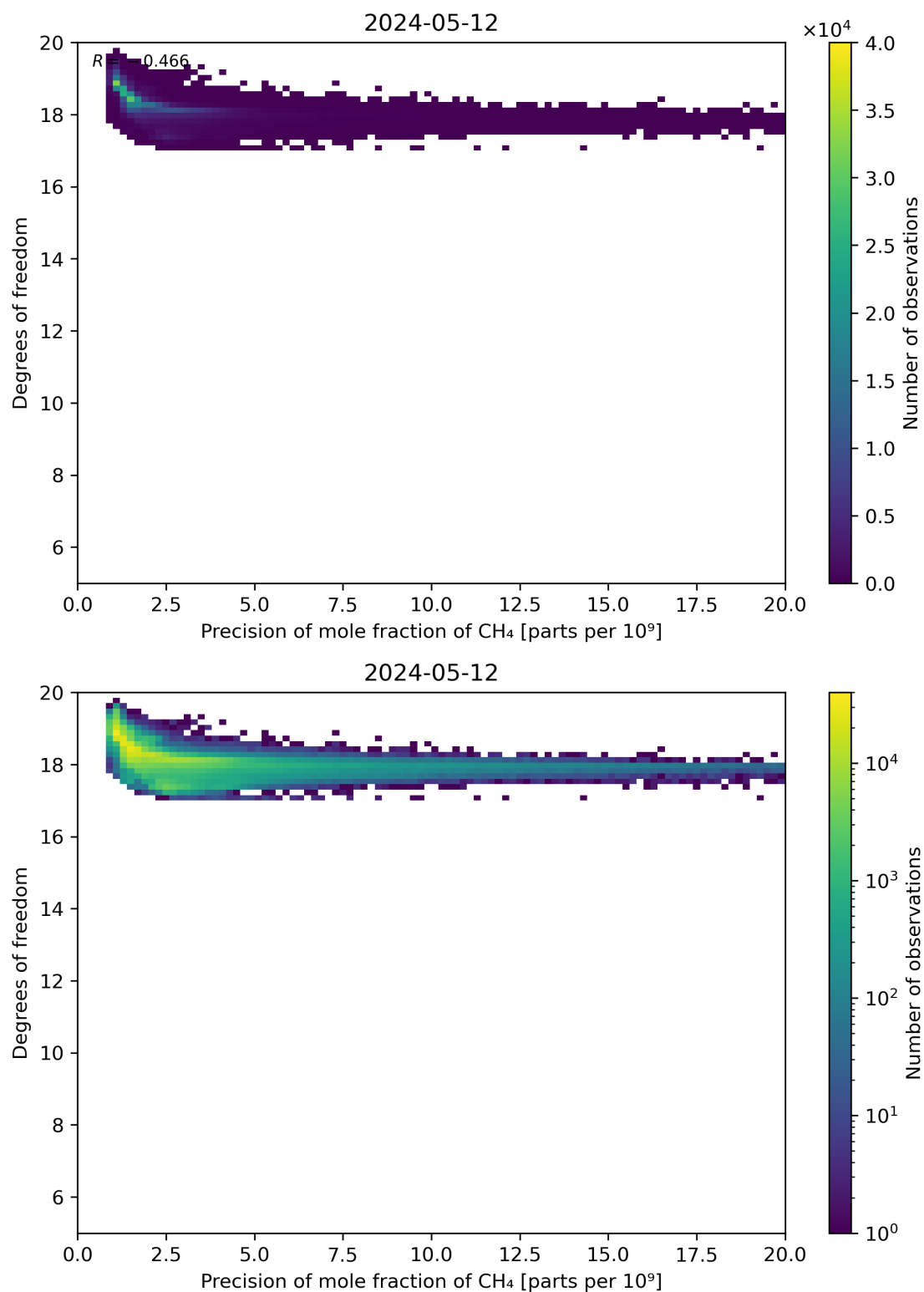
Figure 80: Scatter density plot of “Precision of mole fraction of CH 4 ” against “Degrees of freedom” for 2024-05-12 to 2024-05-13.
