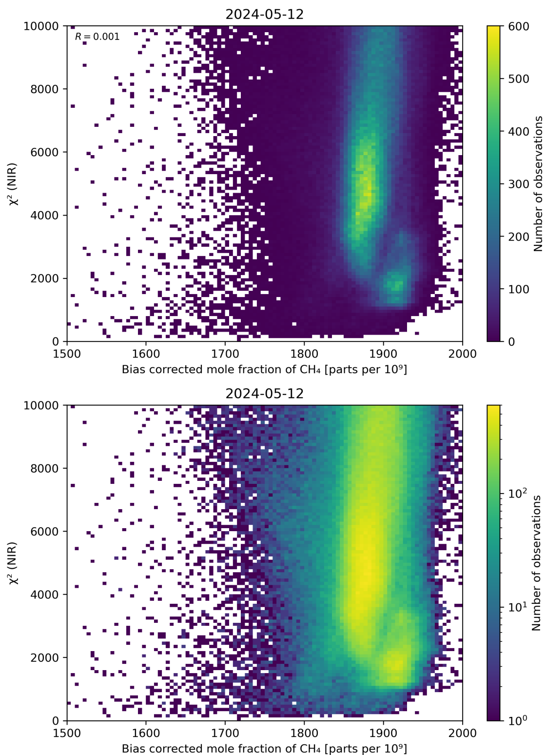
Figure 63: Scatter density plot of “Bias corrected mole fraction of CH 4 ” against “ \chi^2 (NIR)” for 2024-05-12 to 2024-05-13.
