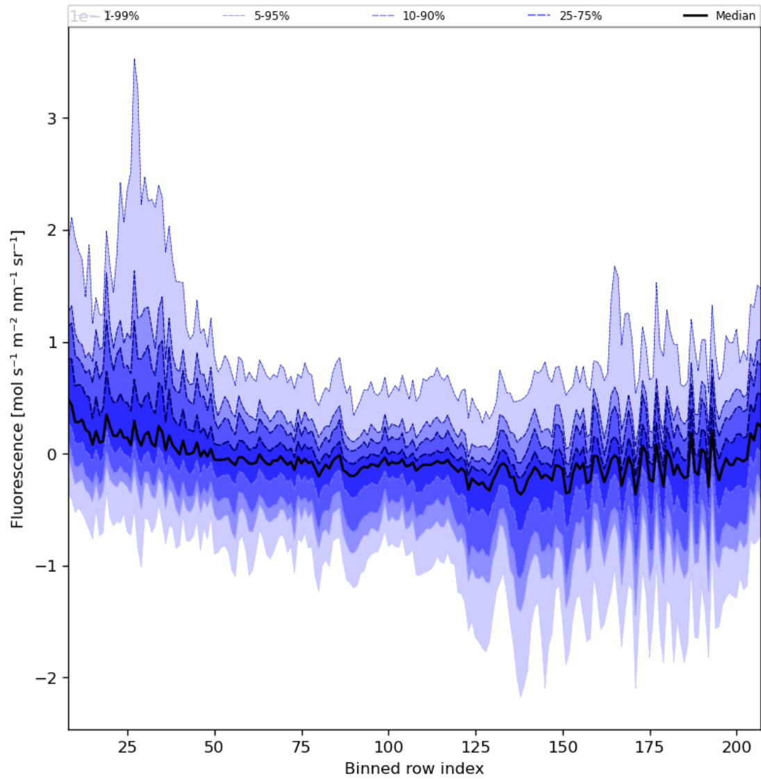
Figure 43: Along track statistics of “Fluorescence” for 2024-05-12 to 2024-05-13
