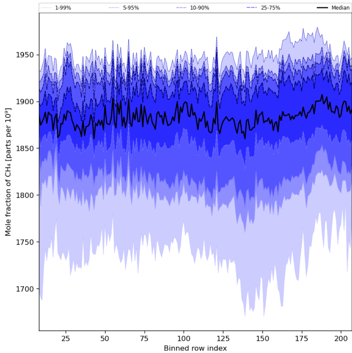
Figure 34: Along track statistics of “Mole fraction of CH 4 ” for 2024-05-12 to 2024-05-13
