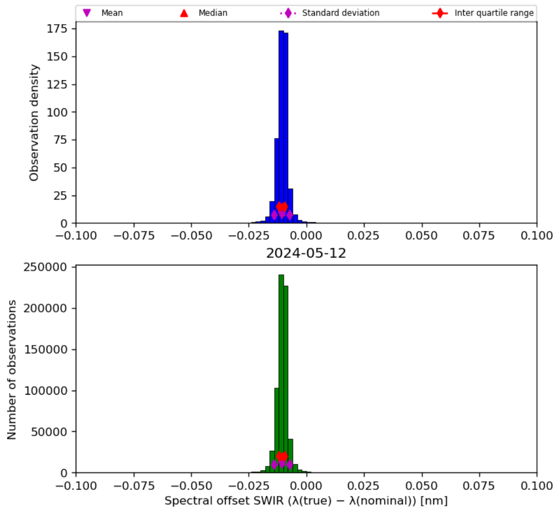
Figure 27: Histogram of “Spectral offset SWIR ( \lambda(\text{true}) - \lambda(\text{nominal}) )” for 2024-05-12 to 2024-05-13
