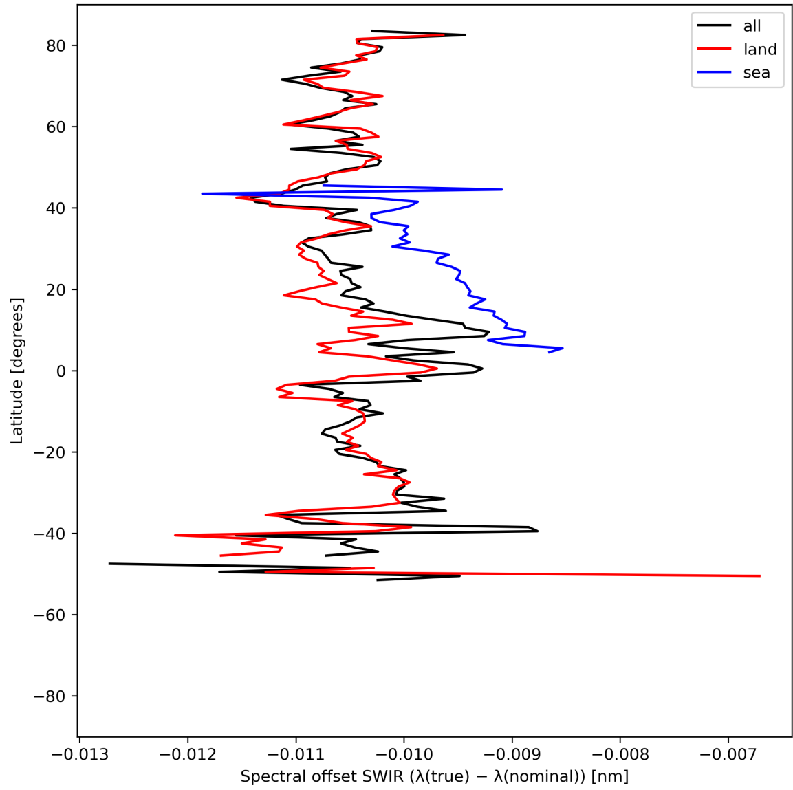
Figure 16: Zonal average of “Spectral offset SWIR ( \lambda(\text{true}) - \lambda(\text{nominal}) )” for 2024-05-12 to 2024-05-13.
