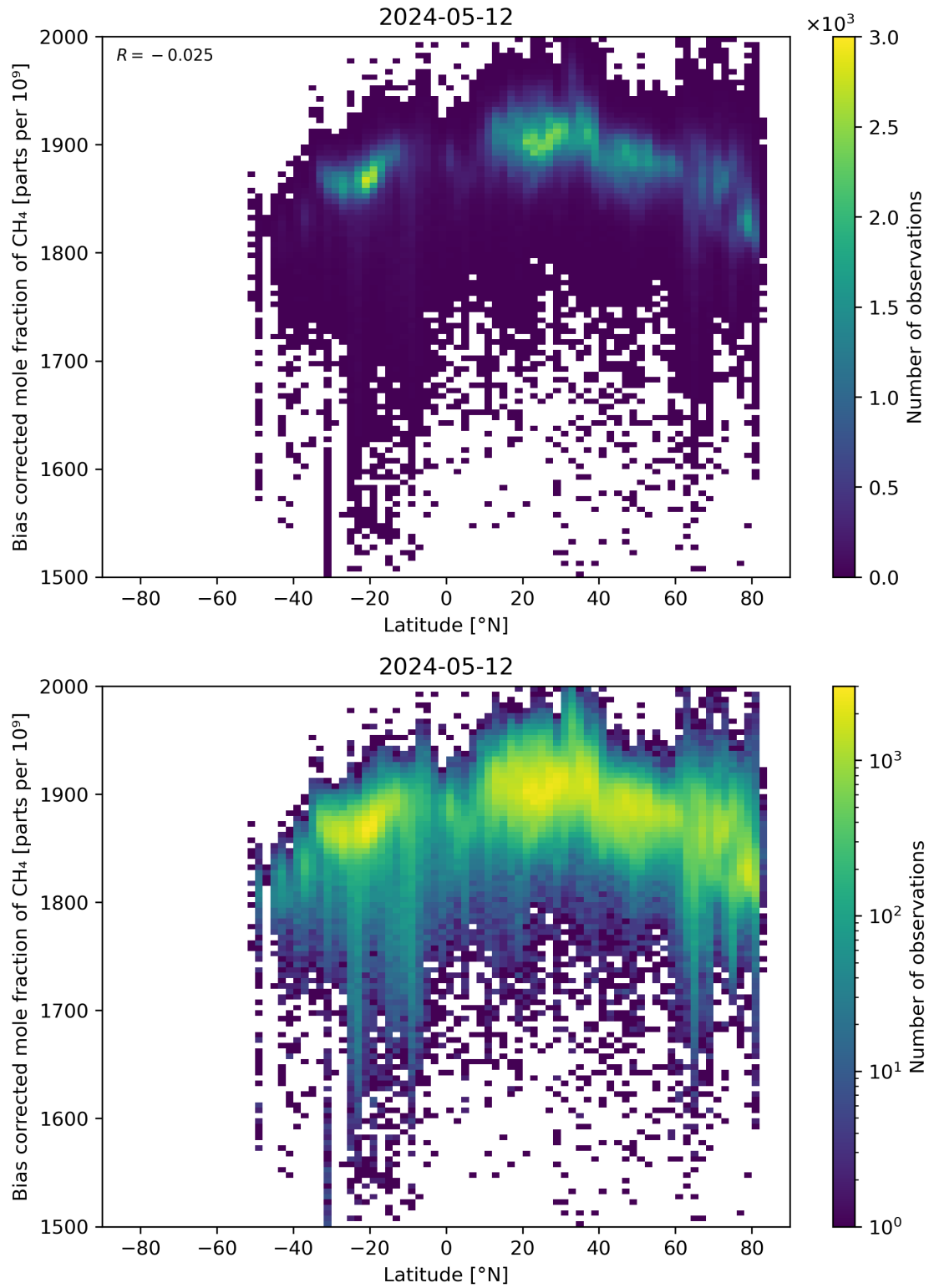
Figure 58: Scatter density plot of “Latitude” against “Bias corrected mole fraction of CH 4 ” for 2024-05-12 to 2024-05-13.
