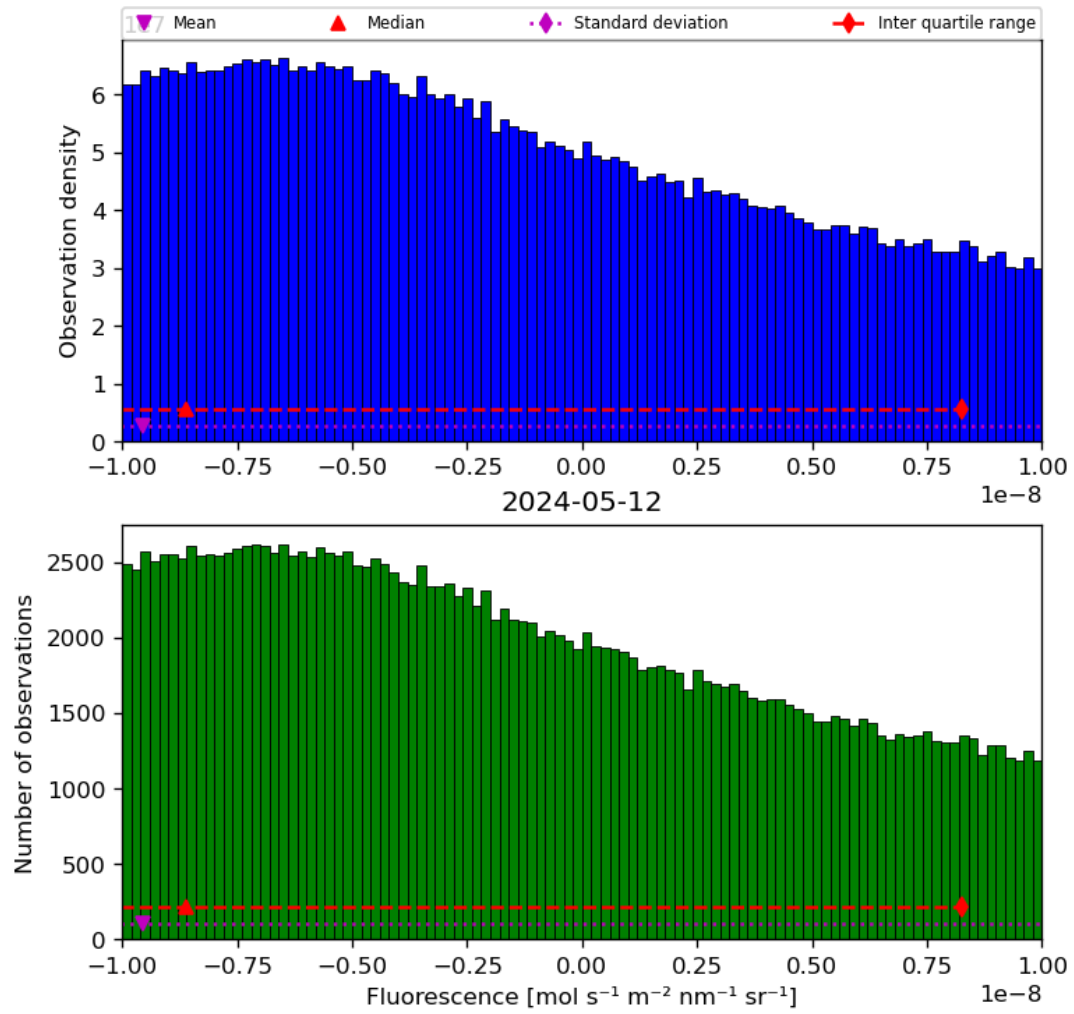
Figure 32: Histogram of “Fluorescence” for 2024-05-12 to 2024-05-13
