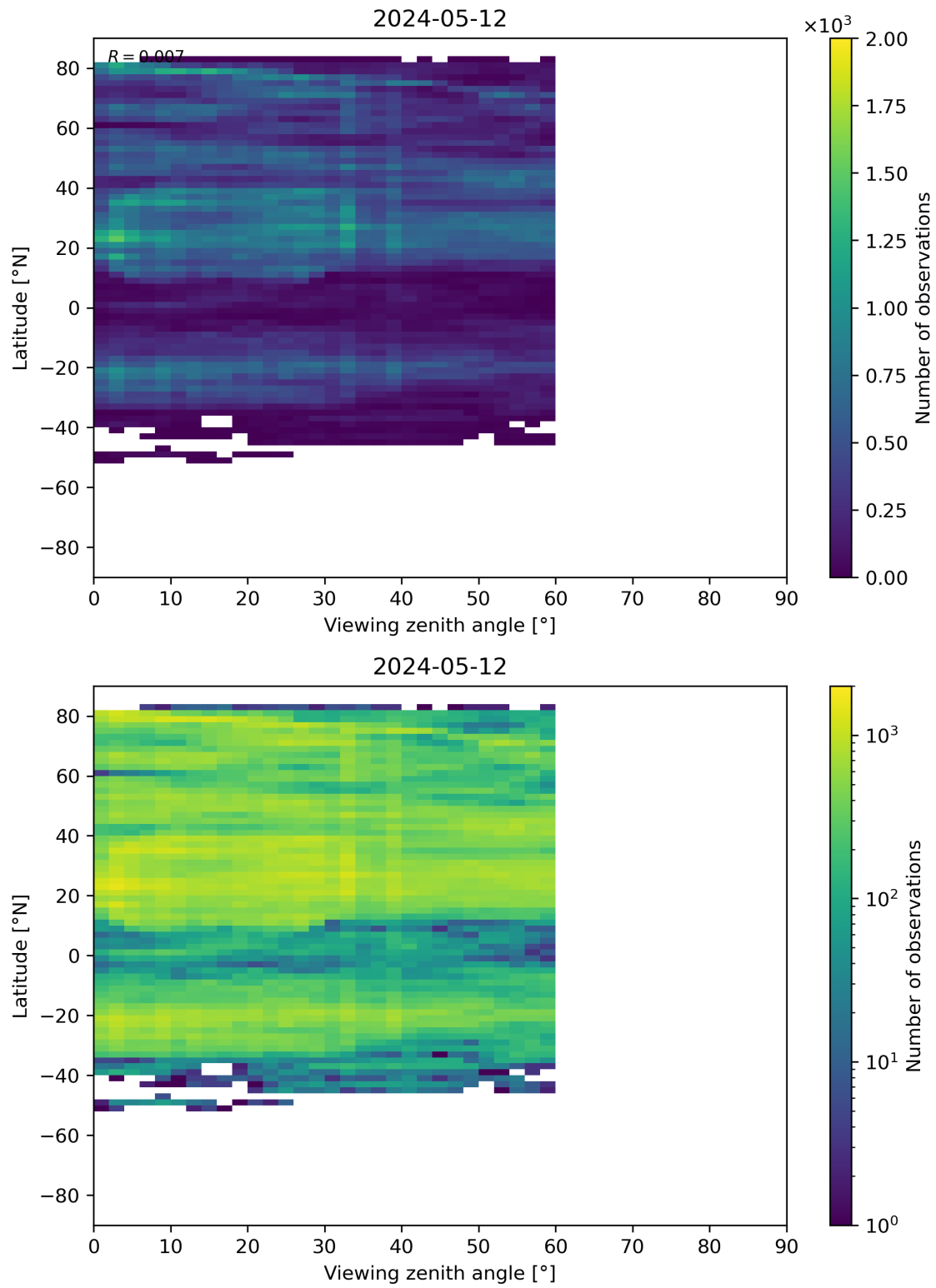
Figure 109: Scatter density plot of “Viewing zenith angle” against “Latitude” for 2024-05-12 to 2024-05-13.
