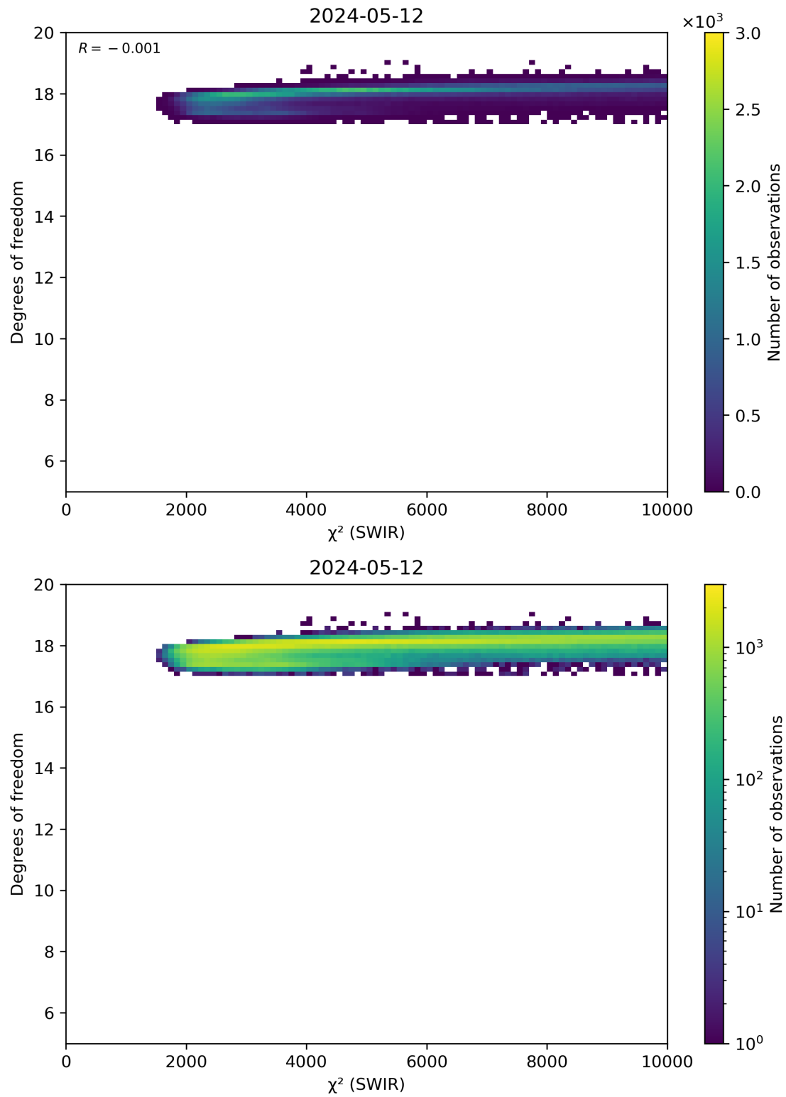
Figure 48: Scatter density plot of “ \chi^2 (SWIR)” against “Degrees of freedom” for 2024-05-12 to 2024-05-13.
