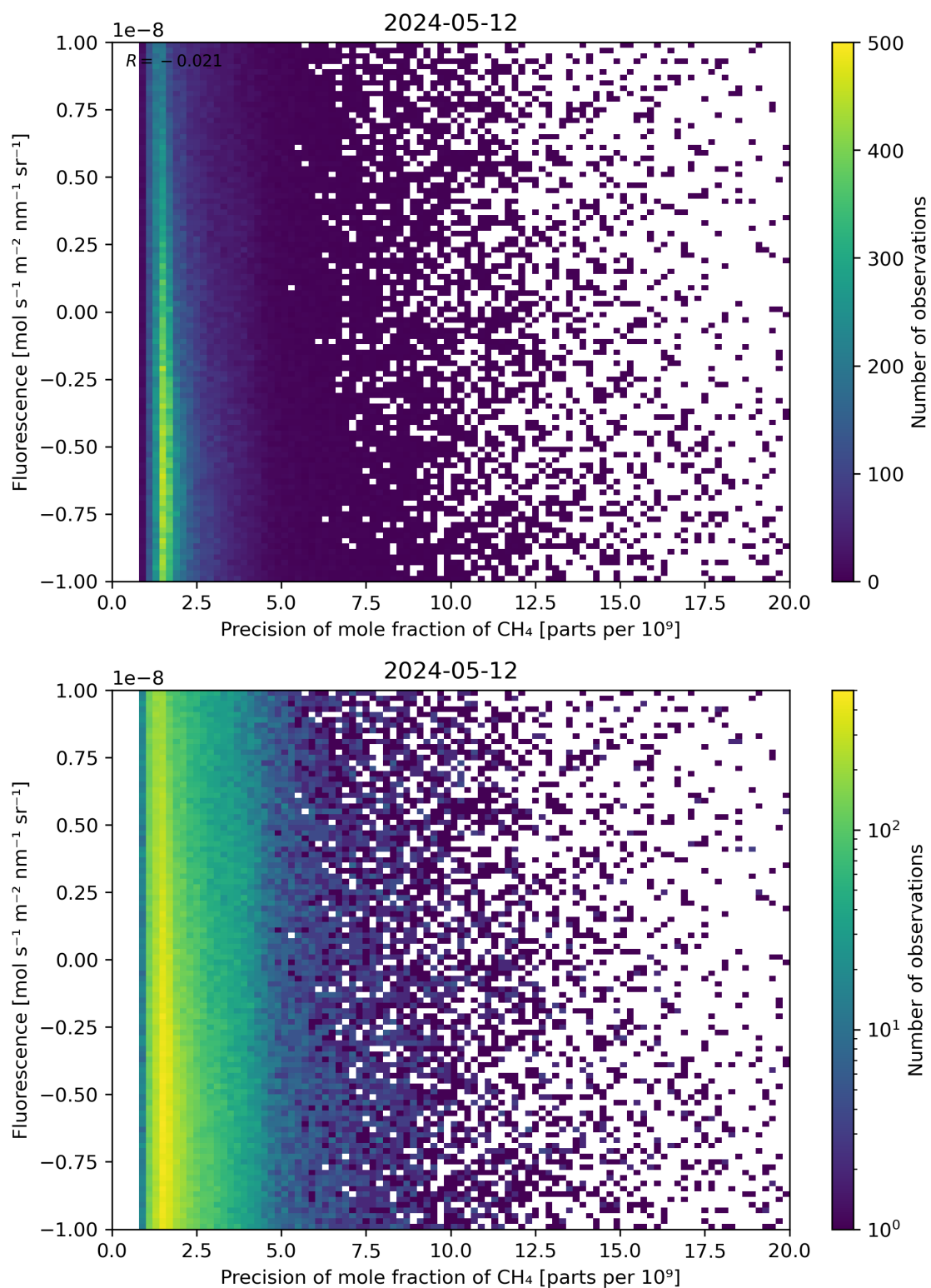
Figure 81: Scatter density plot of “Precision of mole fraction of CH 4 ” against “Fluorescence” for 2024-05-12 to 2024-05-13.
