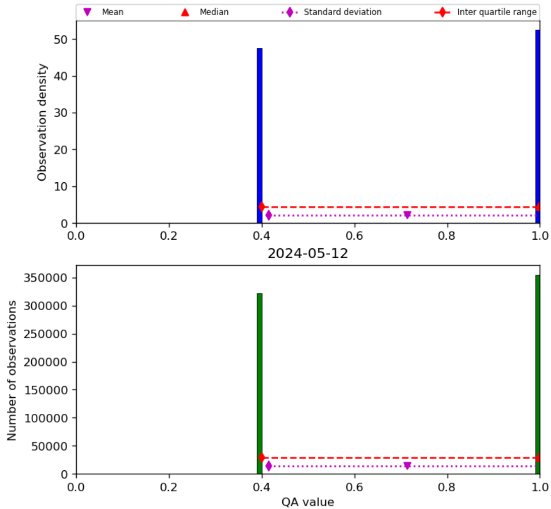
Figure 22: Histogram of “QA value” for 2024-05-12 to 2024-05-13
