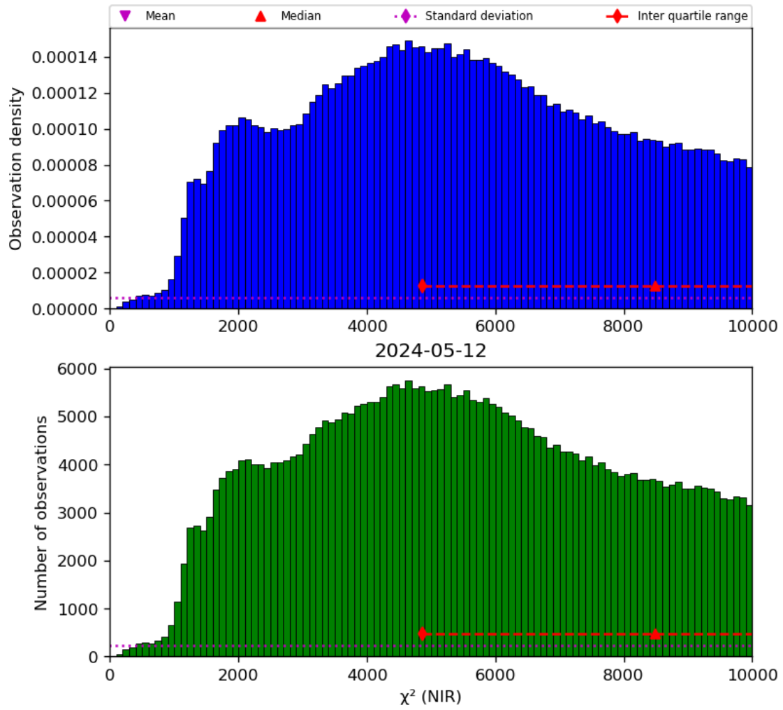
Figure 29: Histogram of “ \chi^2 (NIR)” for 2024-05-12 to 2024-05-13
