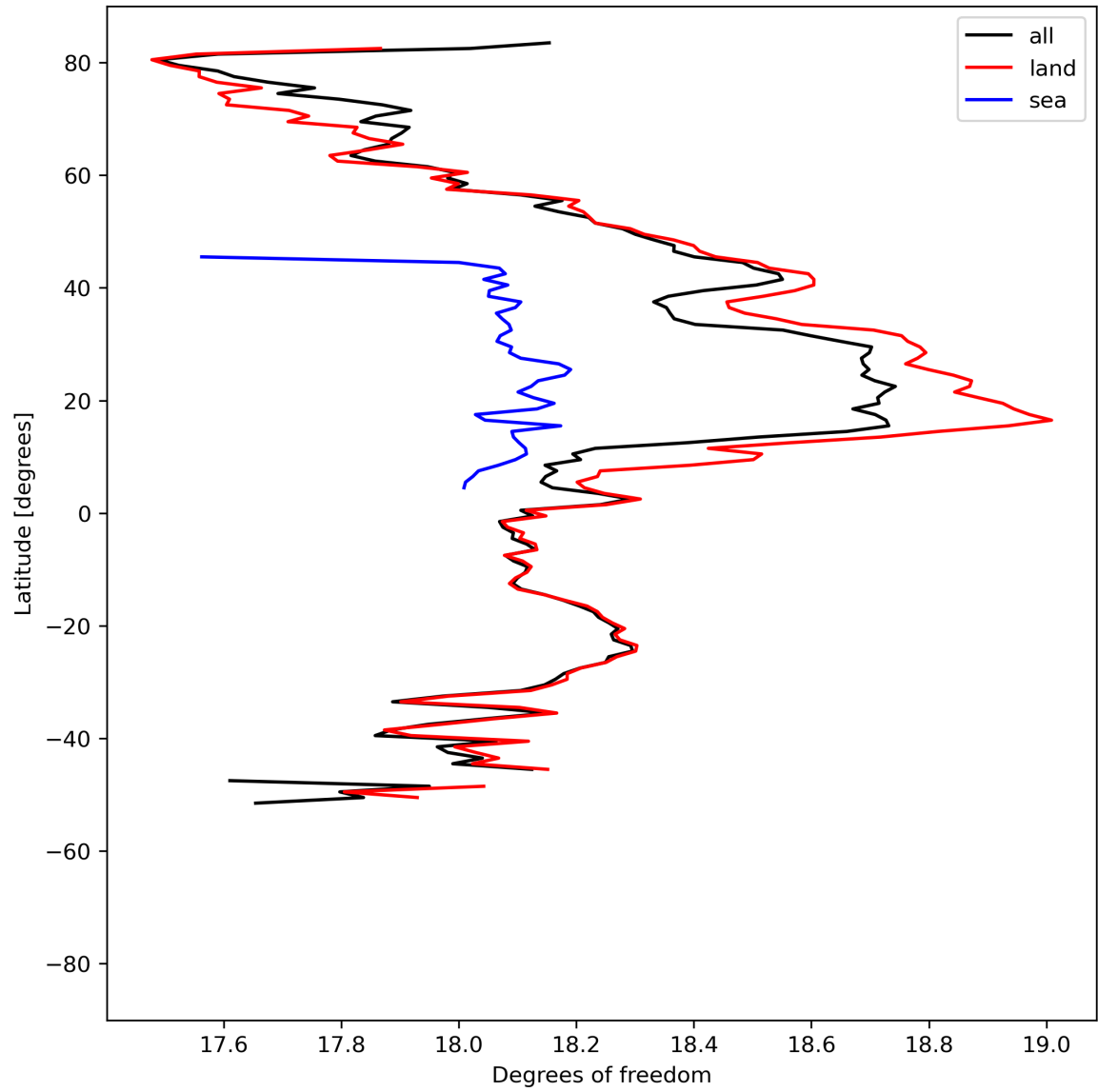
Figure 19: Zonal average of “Degrees of freedom” for 2024-05-12 to 2024-05-13.
