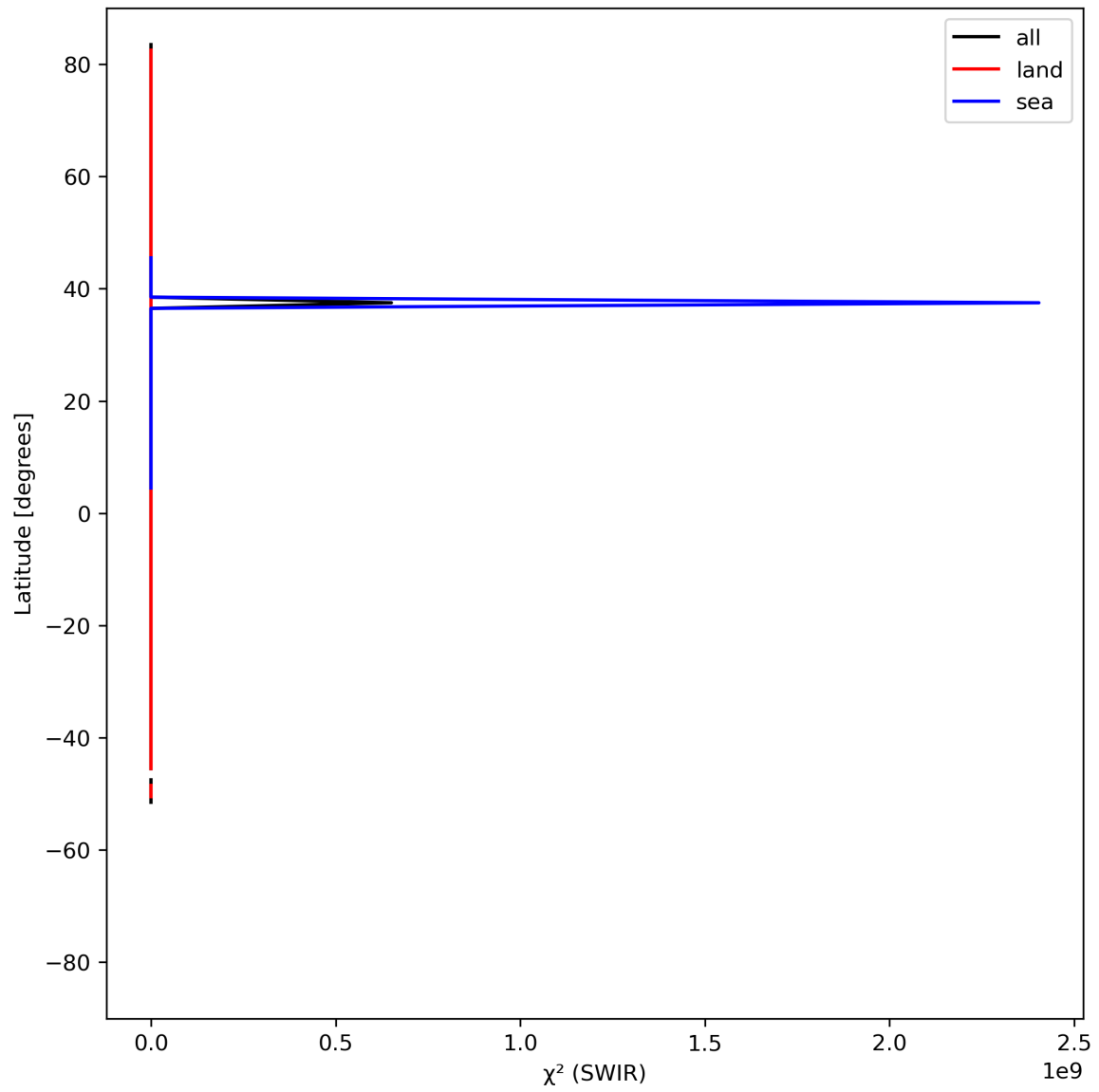
Figure 17: Zonal average of “ \chi^2 (SWIR)” for 2024-05-12 to 2024-05-13.
