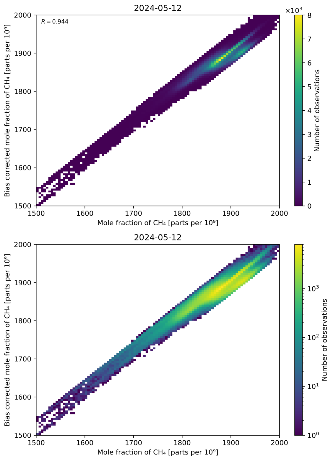
Figure 74: Scatter density plot of “Mole fraction of CH 4 ” against “Bias corrected mole fraction of CH 4 ” for 2024-05-12 to 2024-05-13.
