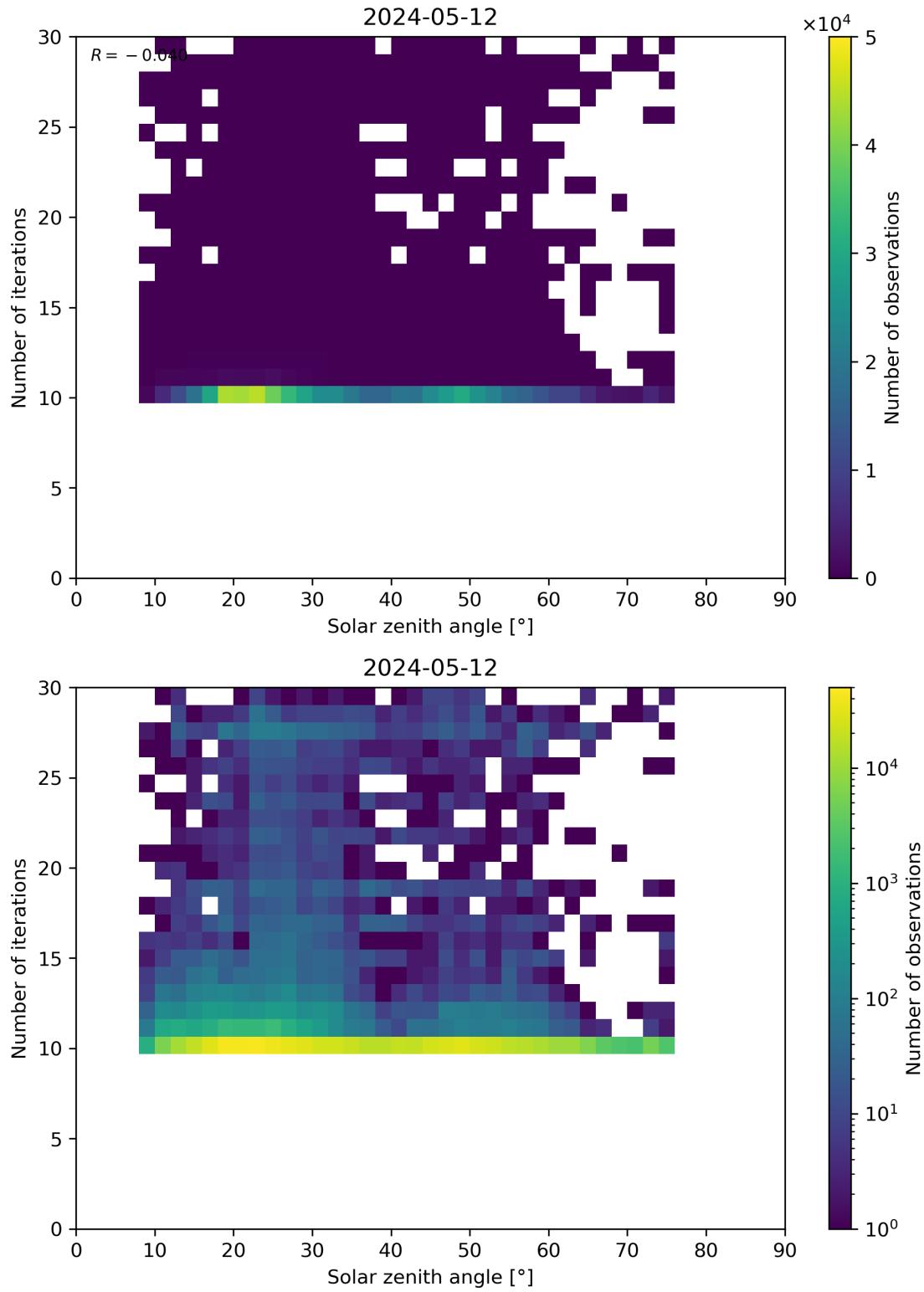
Figure 102: Scatter density plot of “Solar zenith angle” against “Number of iterations” for 2024-05-12 to 2024-05-13.
