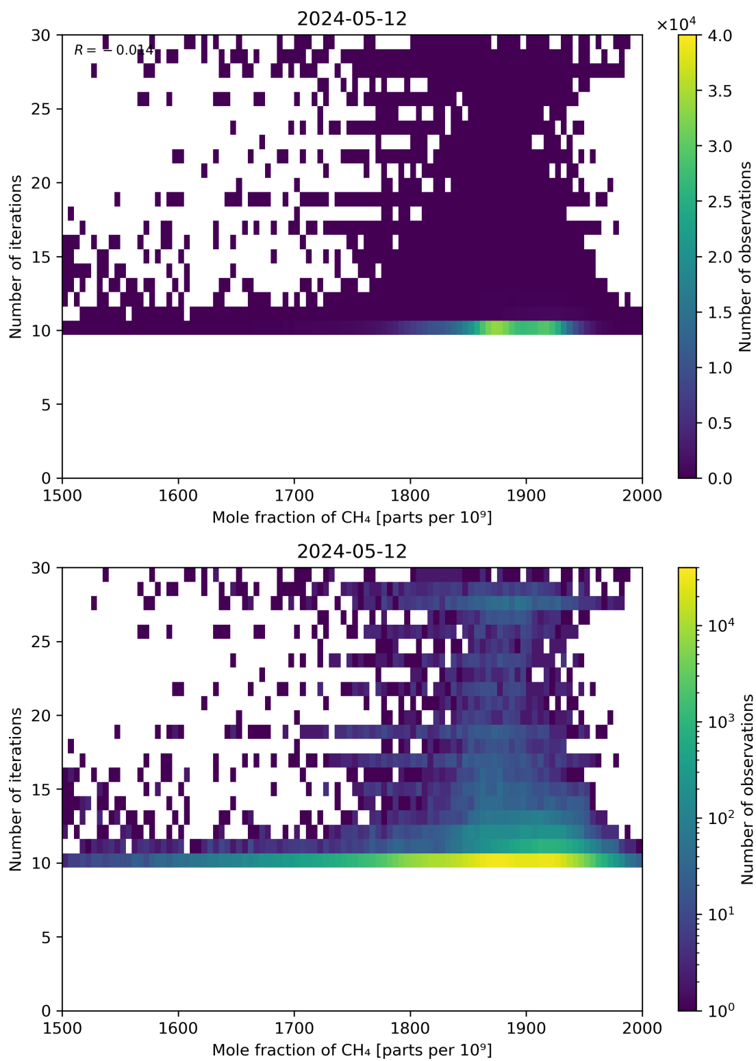
Figure 76: Scatter density plot of “Mole fraction of CH 4 ” against “Number of iterations” for 2024-05-12 to 2024-05-13.
