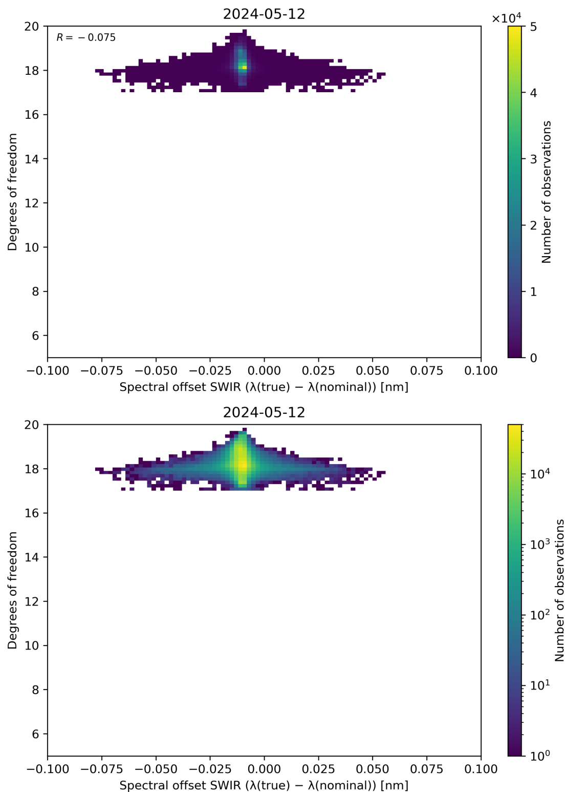
Figure 119: Scatter density plot of “Spectral offset SWIR ( \lambda(\text{true}) - \lambda(\text{nominal}) )” against “Degrees of freedom” for 2024-05-12 to 2024-05-13.
