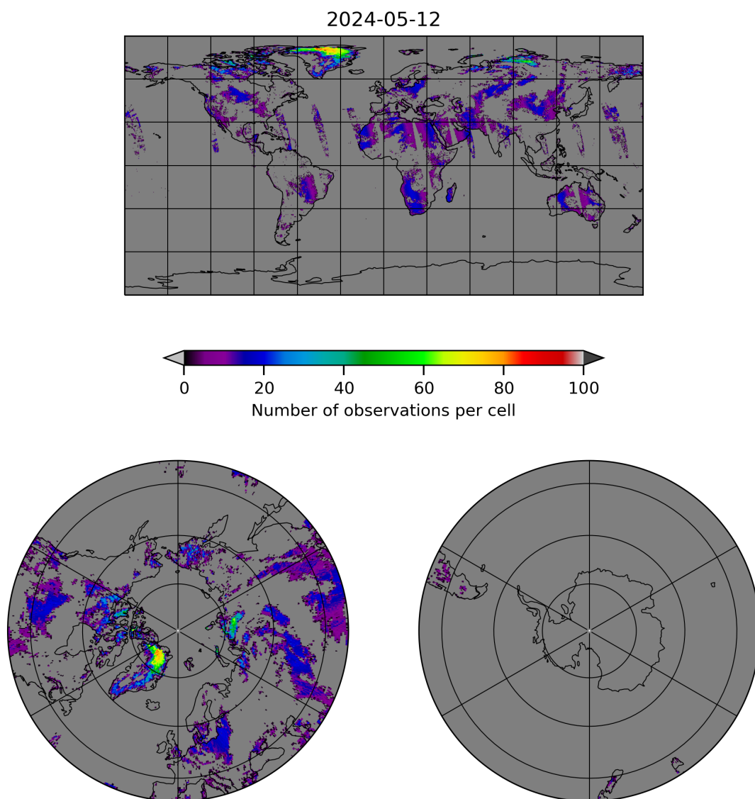
Figure 10: Map of the number of observations for 2024-05-12 to 2024-05-13
