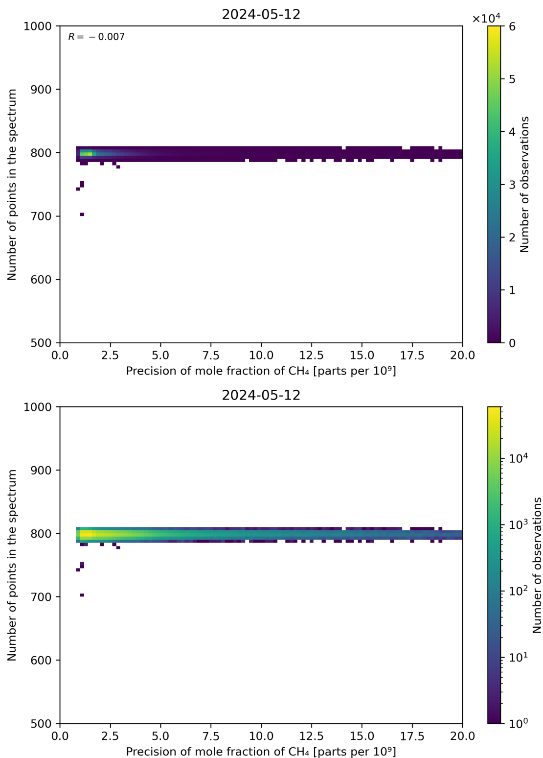
Figure 84: Scatter density plot of “Precision of mole fraction of CH 4 ” against “Number of points in the spectrum” for 2024-05-12 to 2024-05-13.
