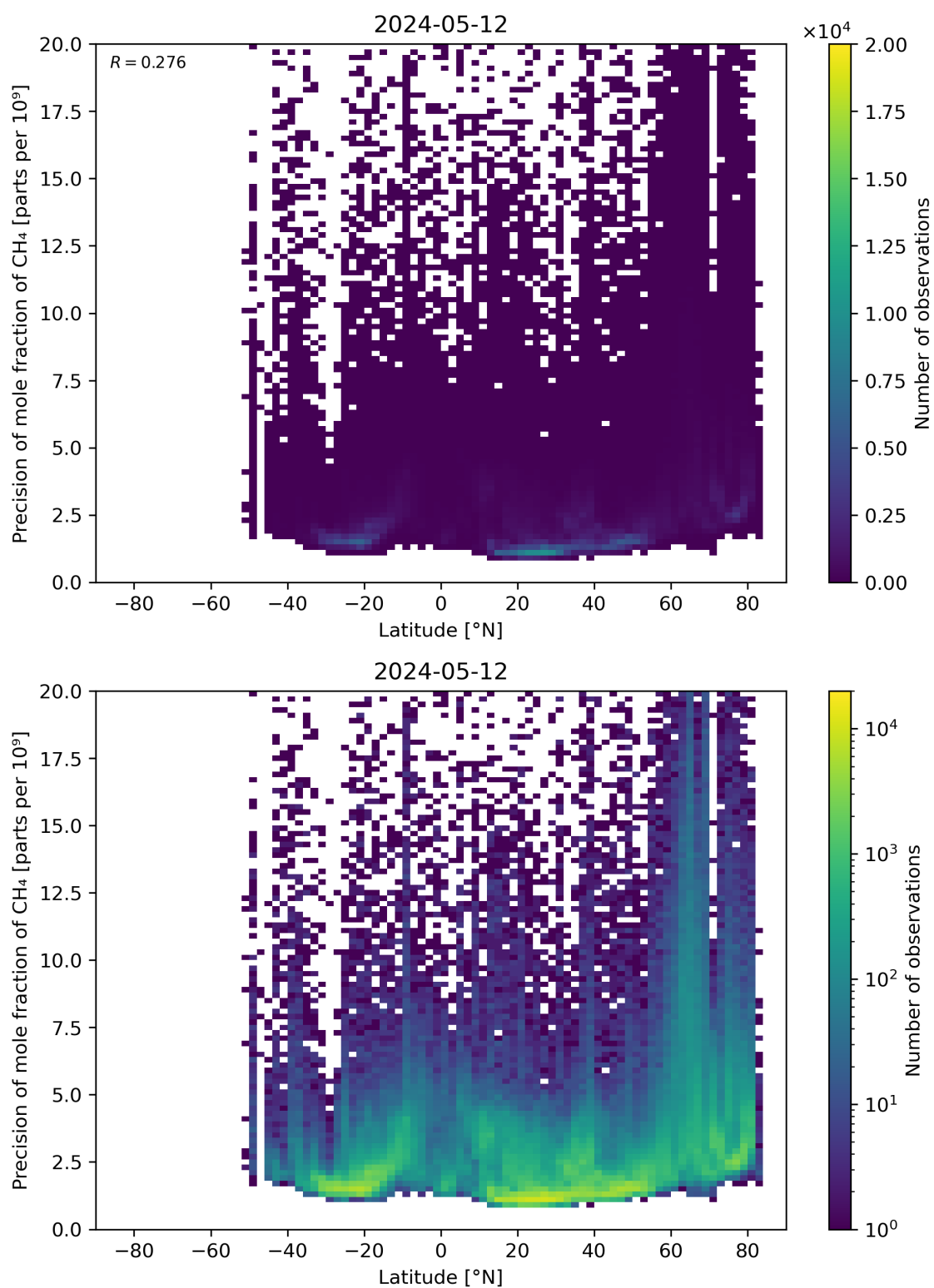
Figure 59: Scatter density plot of “Latitude” against “Precision of mole fraction of \text{CH}_4 ” for 2024-05-12 to 2024-05-13.
