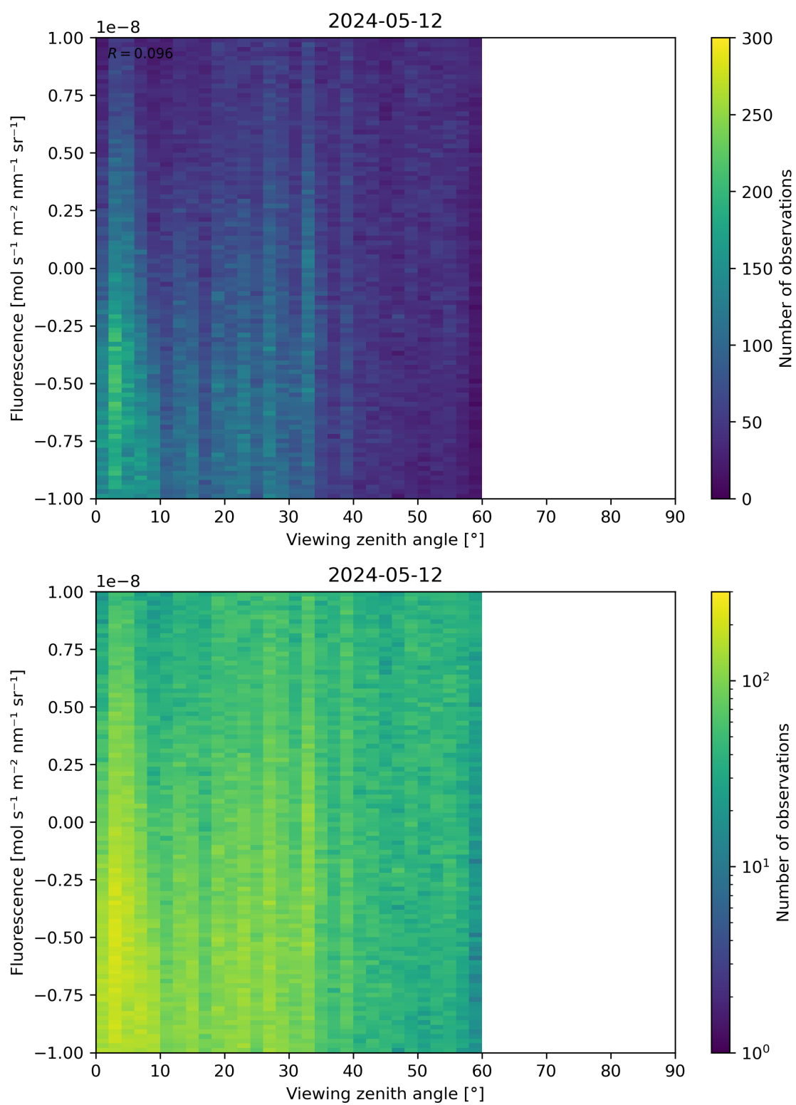
Figure 108: Scatter density plot of “Viewing zenith angle” against “Fluorescence” for 2024-05-12 to 2024-05-13.
