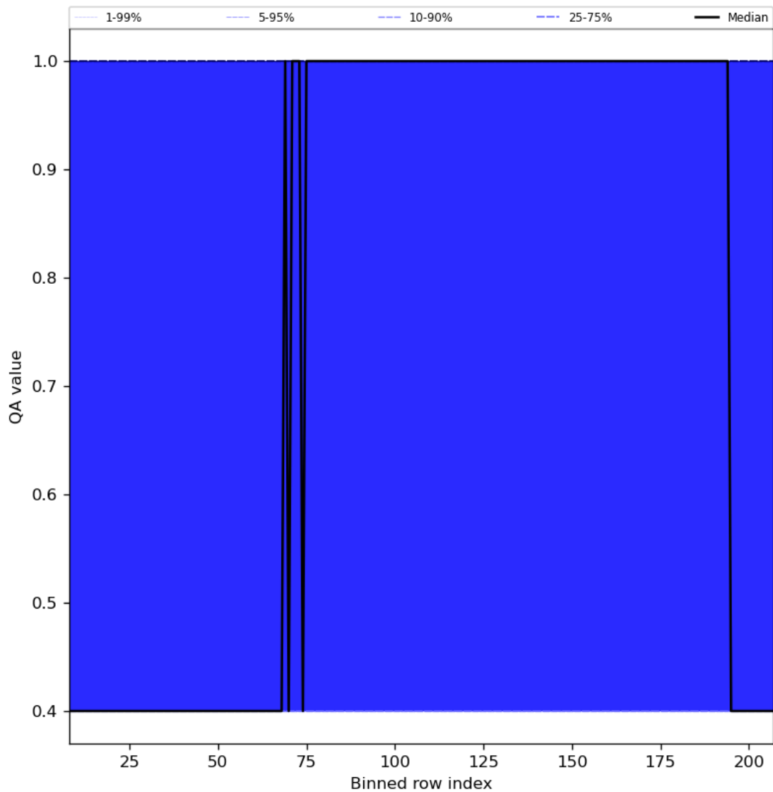
Figure 33: Along track statistics of “QA value” for 2024-05-12 to 2024-05-13
