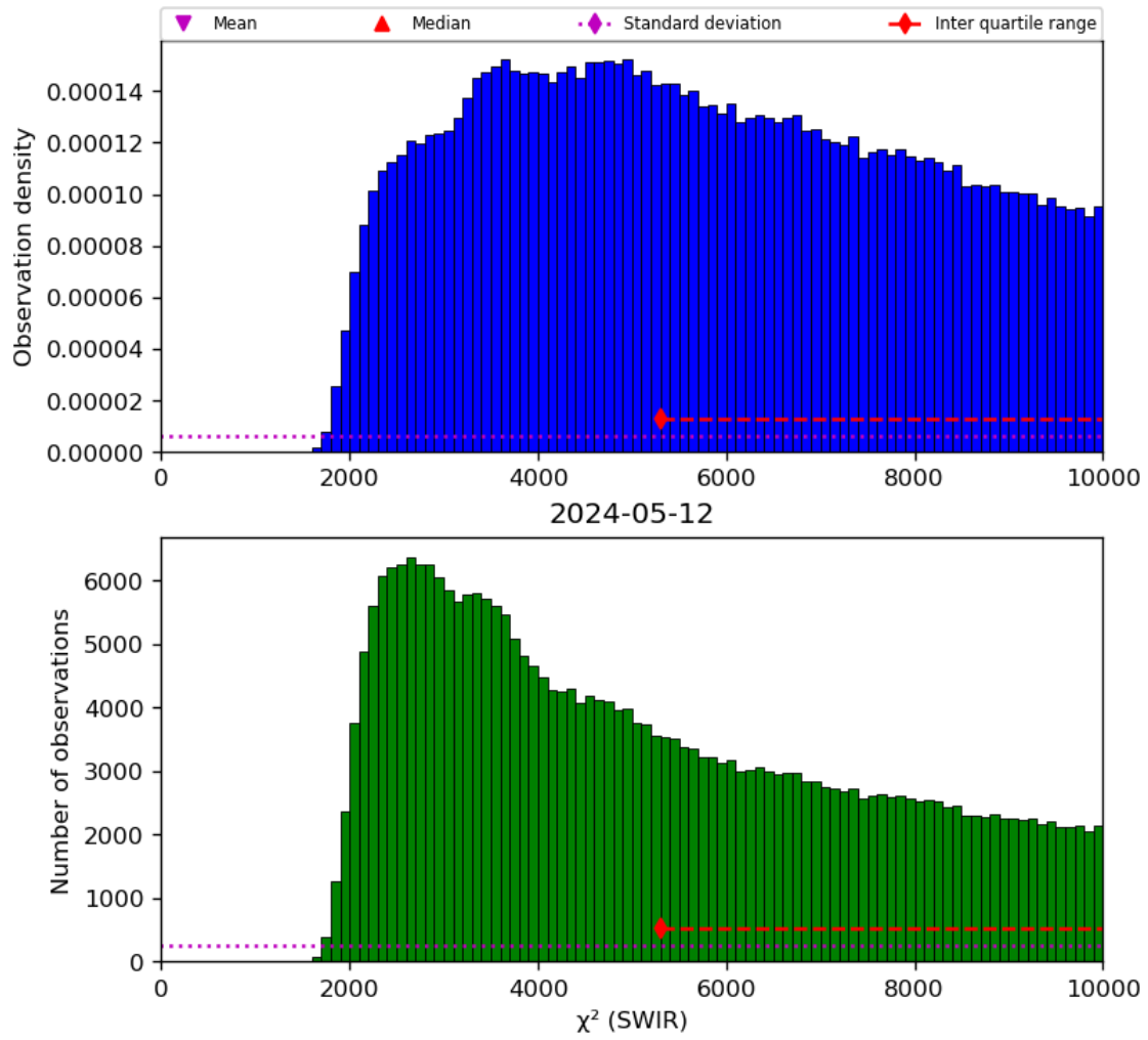
Figure 28: Histogram of “ \chi^2 (SWIR)” for 2024-05-12 to 2024-05-13
