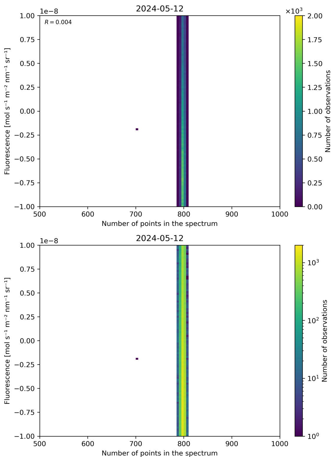
Figure 91: Scatter density plot of “Number of points in the spectrum” against “Fluorescence” for 2024-05-12 to 2024-05-13.
