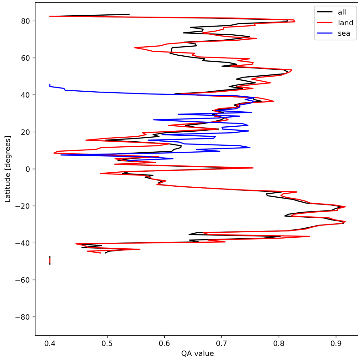
Figure 11: Zonal average of “QA value” for 2024-05-12 to 2024-05-13.
