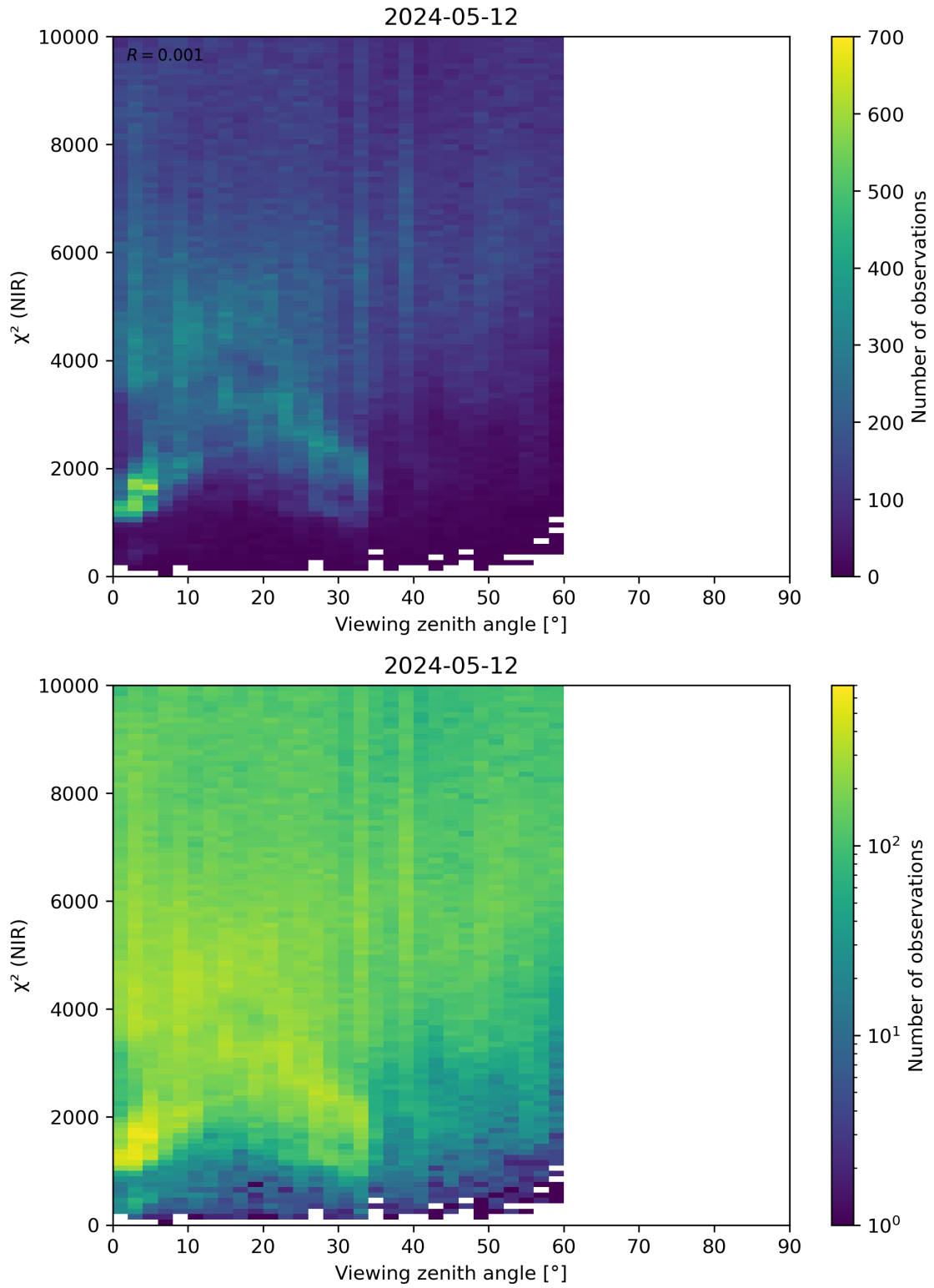
Figure 105: Scatter density plot of “Viewing zenith angle” against “ \chi^2 (NIR)” for 2024-05-12 to 2024-05-13.
