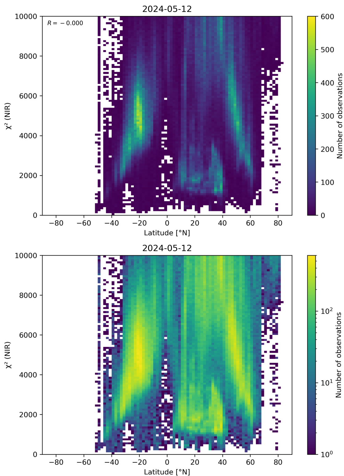
Figure 53: Scatter density plot of “Latitude” against “ \chi^2 (NIR)” for 2024-05-12 to 2024-05-13.
