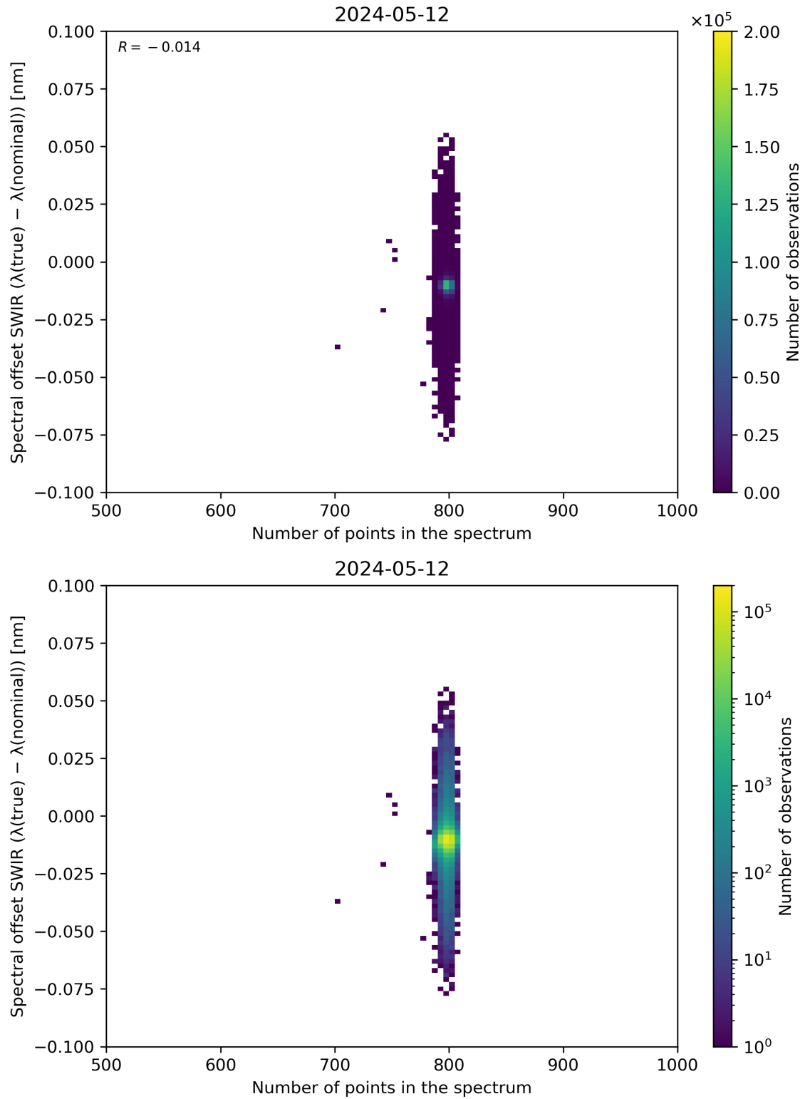
Figure 93: Scatter density plot of “Number of points in the spectrum” against “Spectral offset SWIR ( \lambda(\text{true}) - \lambda(\text{nominal}) )” for 2024-05-12 to 2024-05-13.
