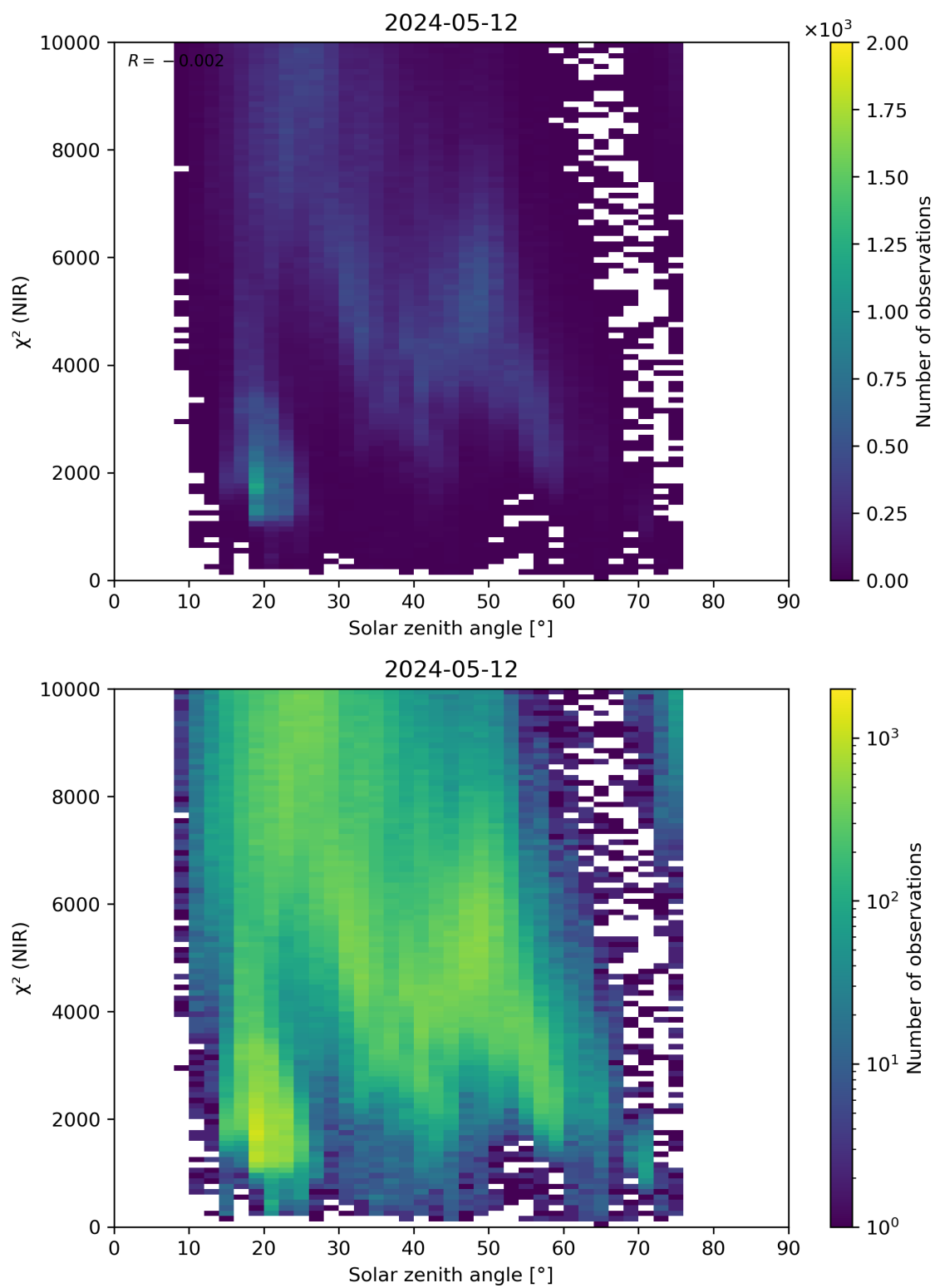
Figure 94: Scatter density plot of “Solar zenith angle” against “ \chi^2 (NIR)” for 2024-05-12 to 2024-05-13.
