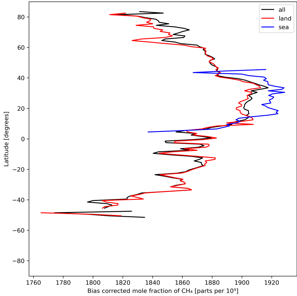
Figure 14: Zonal average of “Bias corrected mole fraction of \text{CH}_4 ” for 2024-05-12 to 2024-05-13.
