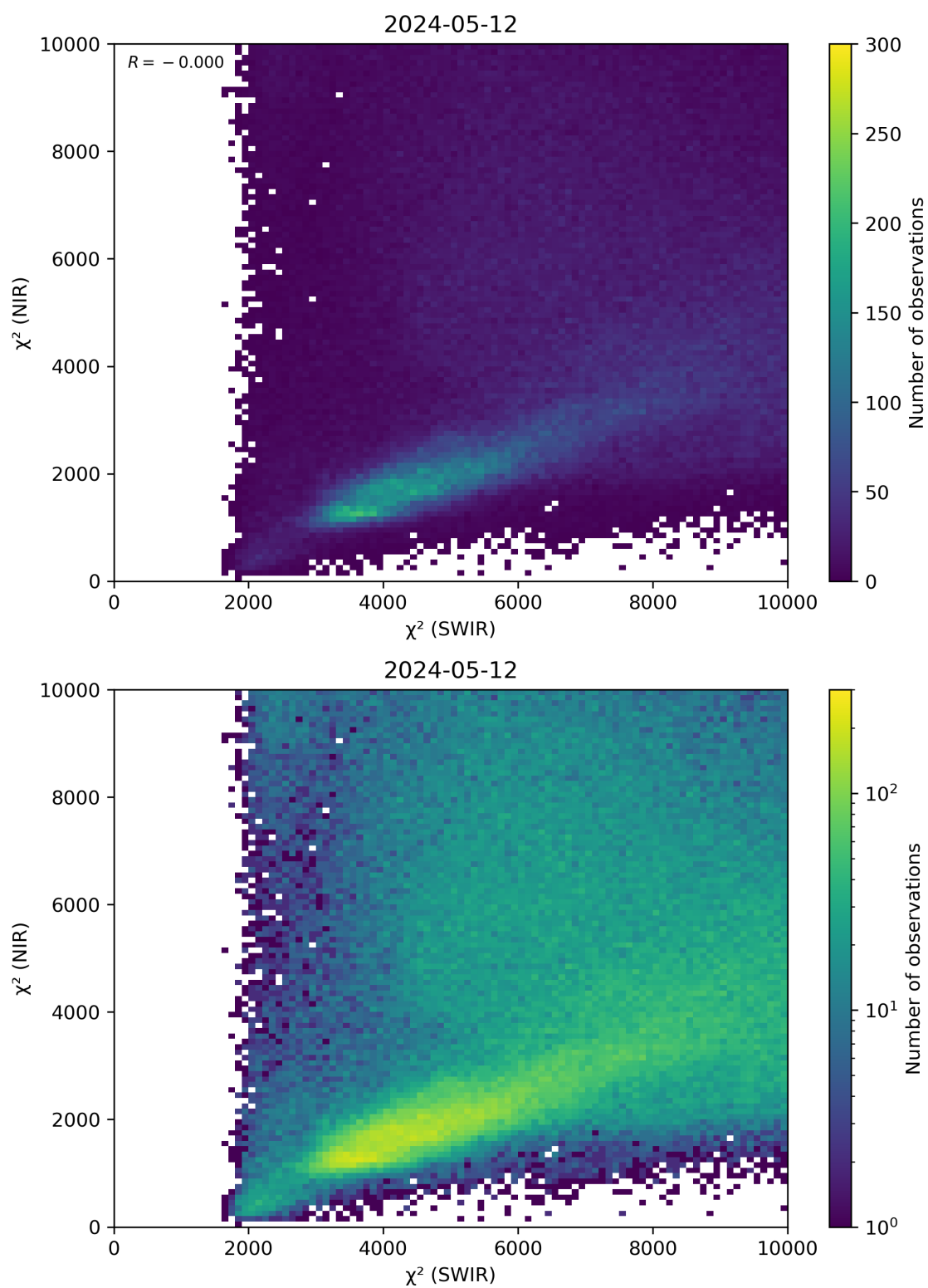
Figure 47: Scatter density plot of “ \chi^2 (SWIR)” against “ \chi^2 (NIR)” for 2024-05-12 to 2024-05-13.
