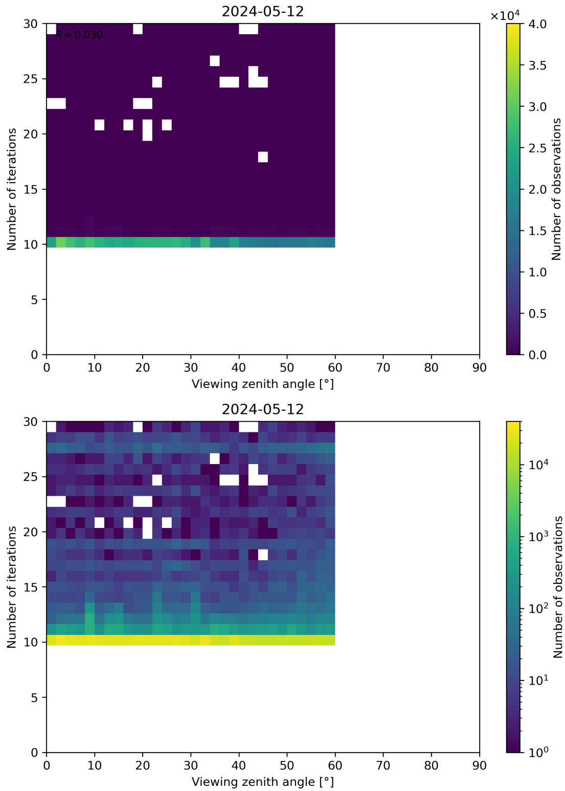
Figure 113: Scatter density plot of “Viewing zenith angle” against “Number of iterations” for 2024-05-12 to 2024-05-13.
