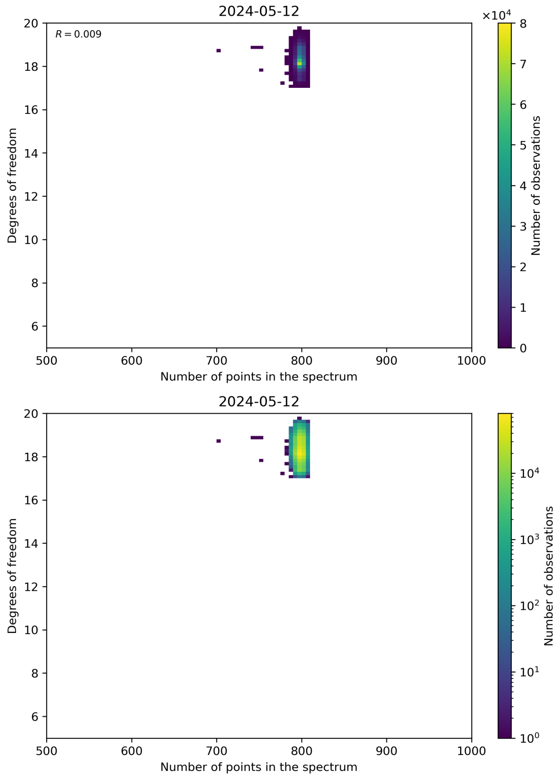
Figure 90: Scatter density plot of “Number of points in the spectrum” against “Degrees of freedom” for 2024-05-12 to 2024-05-13.
