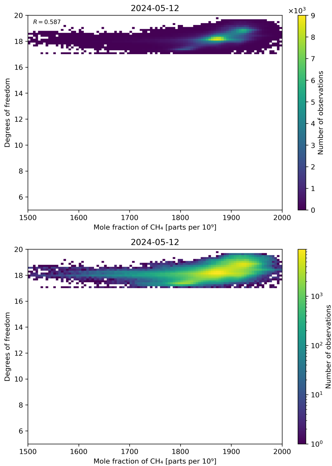
Figure 72: Scatter density plot of “Mole fraction of CH 4 ” against “Degrees of freedom” for 2024-05-12 to 2024-05-13.
