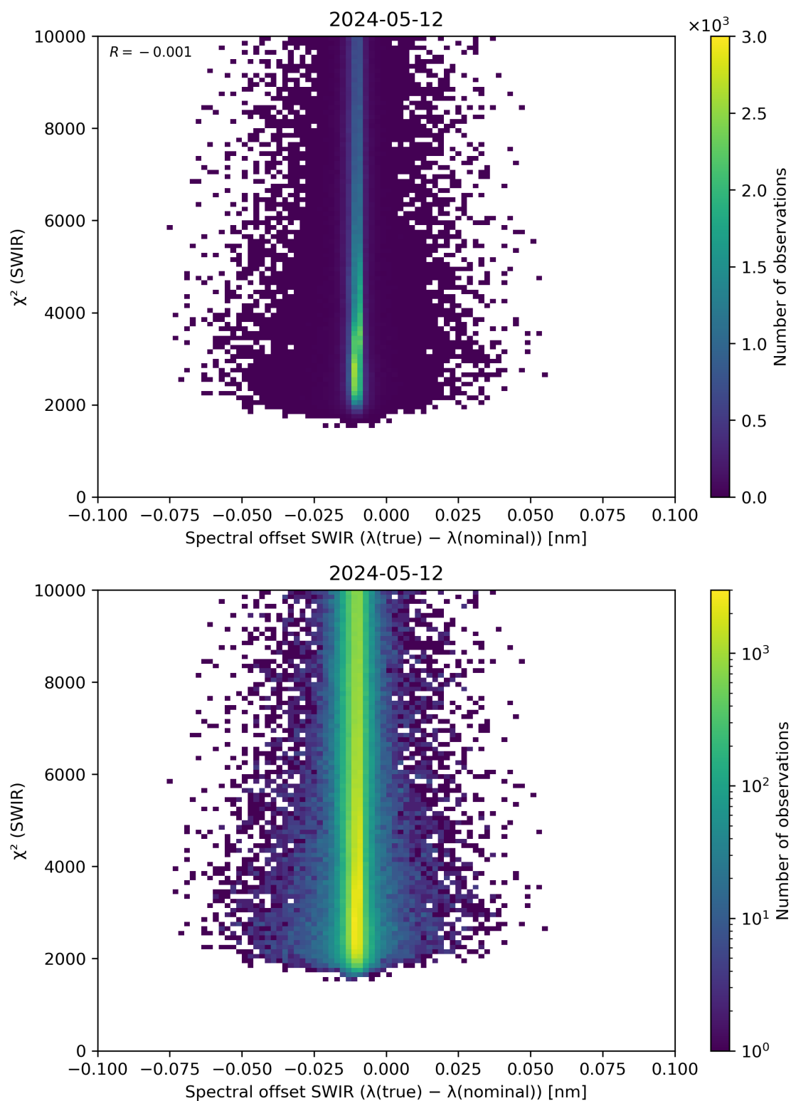
Figure 118: Scatter density plot of “Spectral offset SWIR ( \lambda(\text{true}) - \lambda(\text{nominal}) )” against “ \chi^2 (SWIR)” for 2024-05-12 to 2024-05-13.
