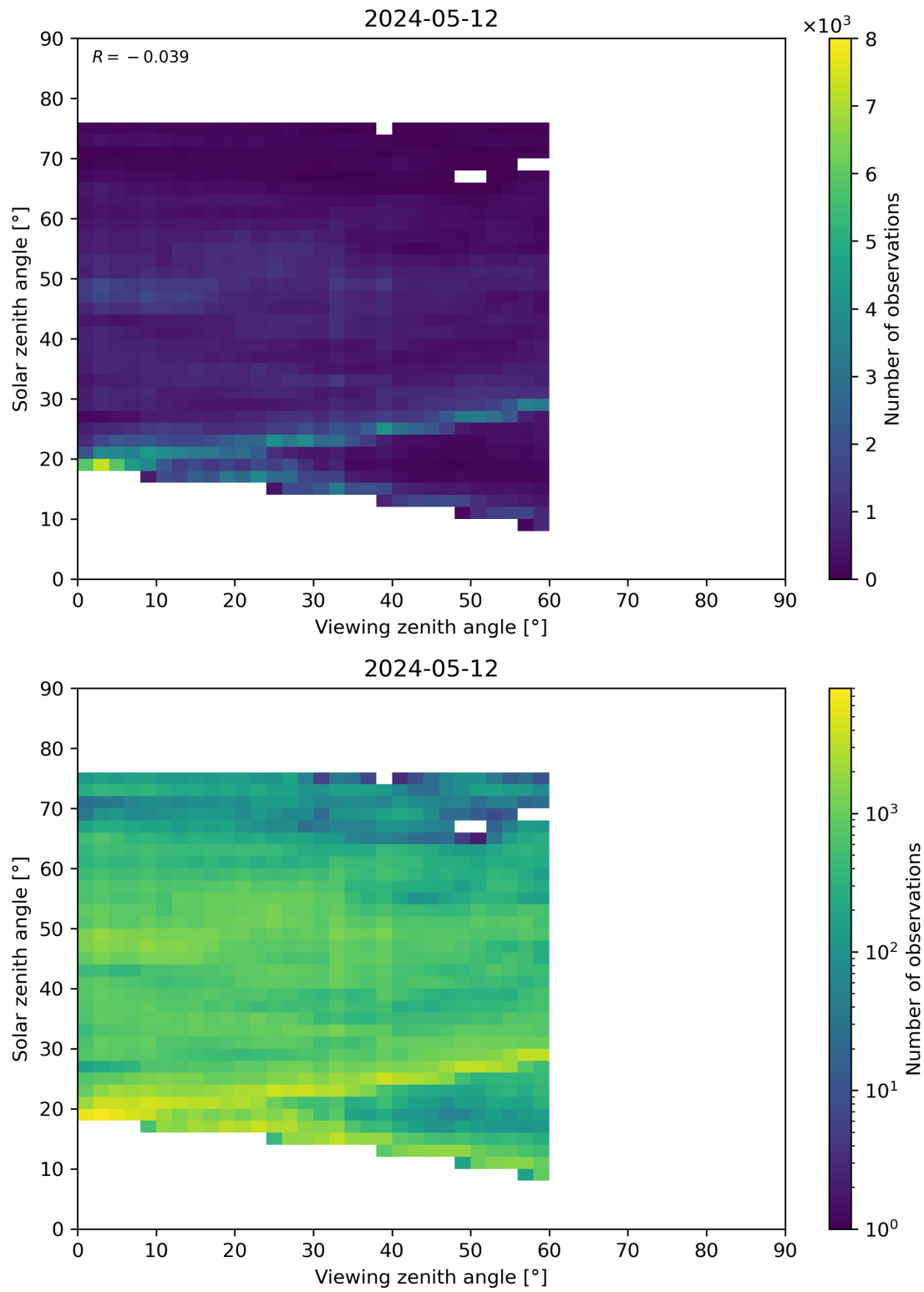
Figure 115: Scatter density plot of “Viewing zenith angle” against “Solar zenith angle” for 2024-05-12 to 2024-05-13.
