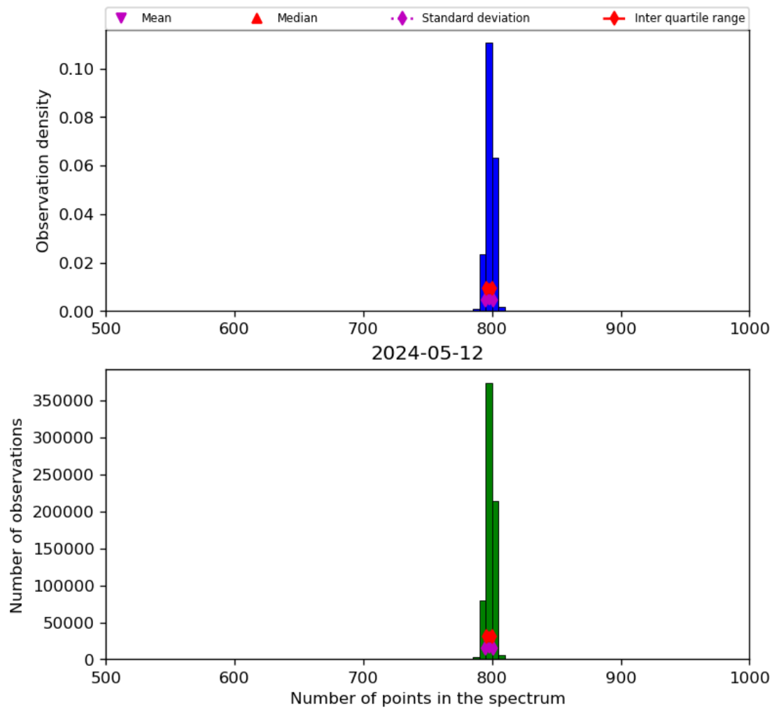
Figure 26: Histogram of “Number of points in the spectrum” for 2024-05-12 to 2024-05-13
