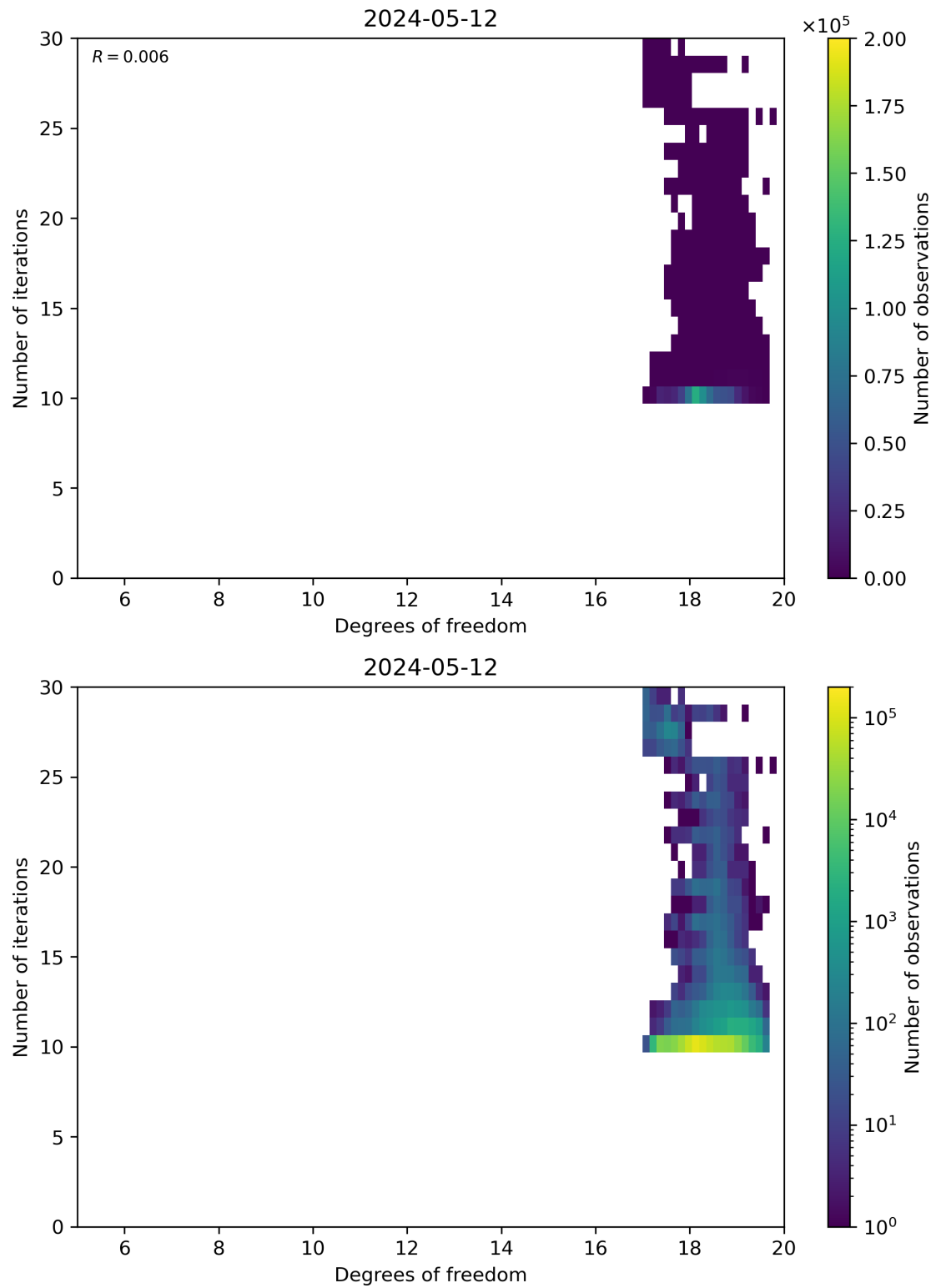
Figure 52: Scatter density plot of “Degrees of freedom” against “Number of iterations” for 2024-05-12 to 2024-05-13.
