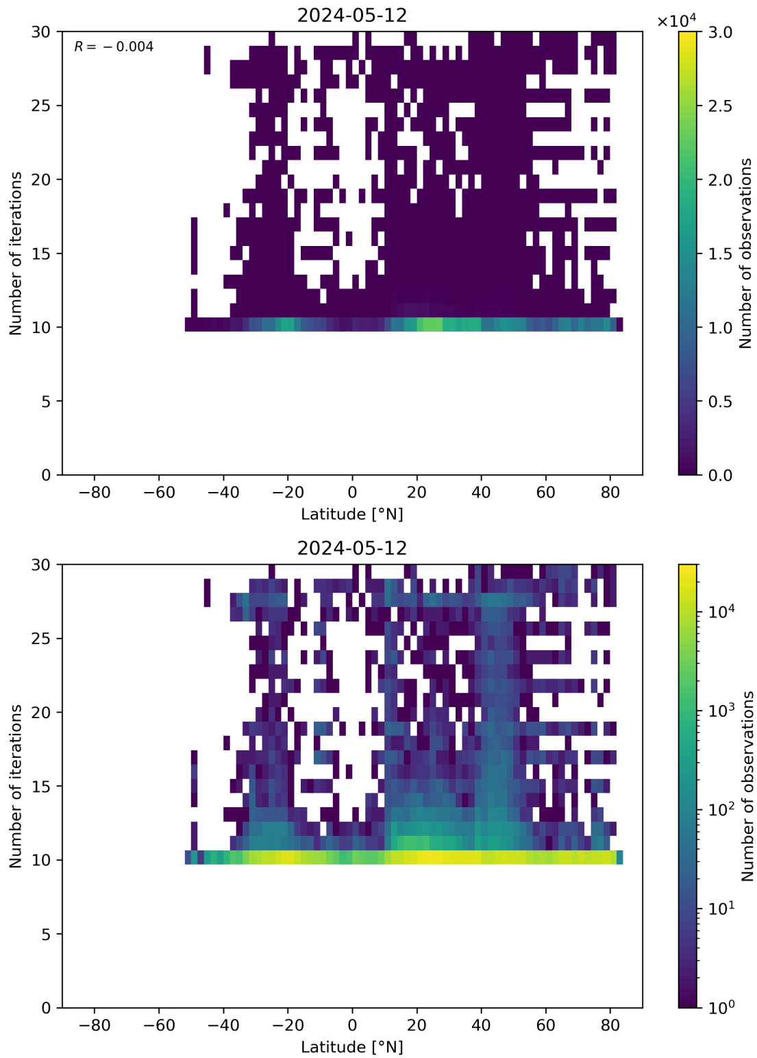
Figure 60: Scatter density plot of “Latitude” against “Number of iterations” for 2024-05-12 to 2024-05-13.
