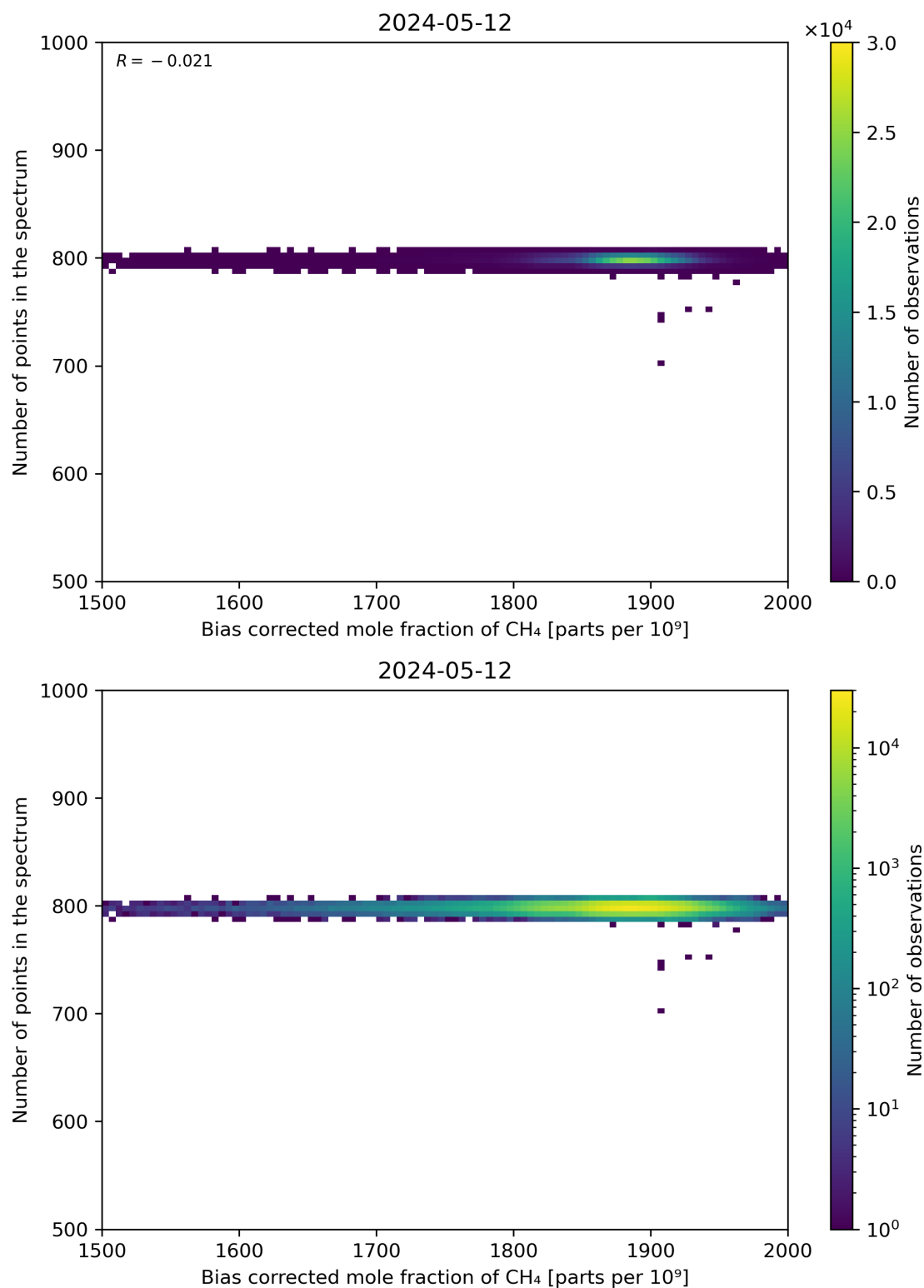
Figure 68: Scatter density plot of “Bias corrected mole fraction of CH 4 ” against “Number of points in the spectrum” for 2024-05-12 to 2024-05-13.
