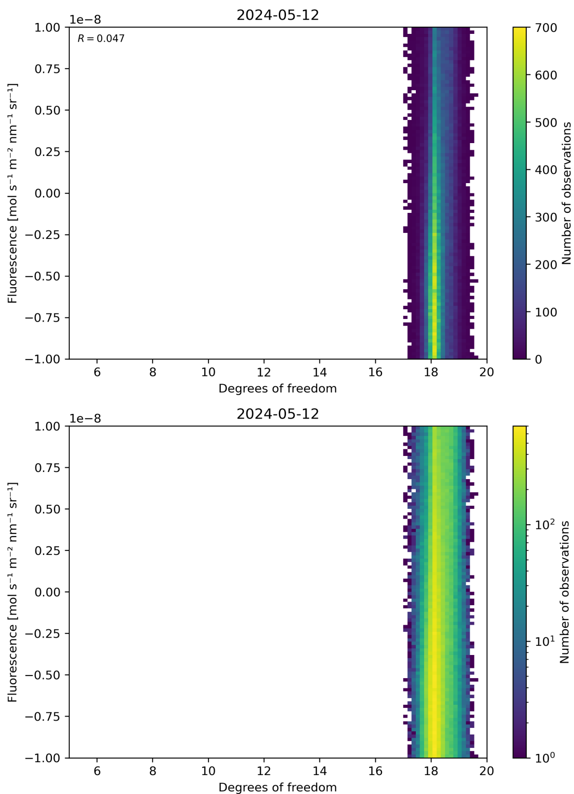
Figure 51: Scatter density plot of “Degrees of freedom” against “Fluorescence” for 2024-05-12 to 2024-05-13.
