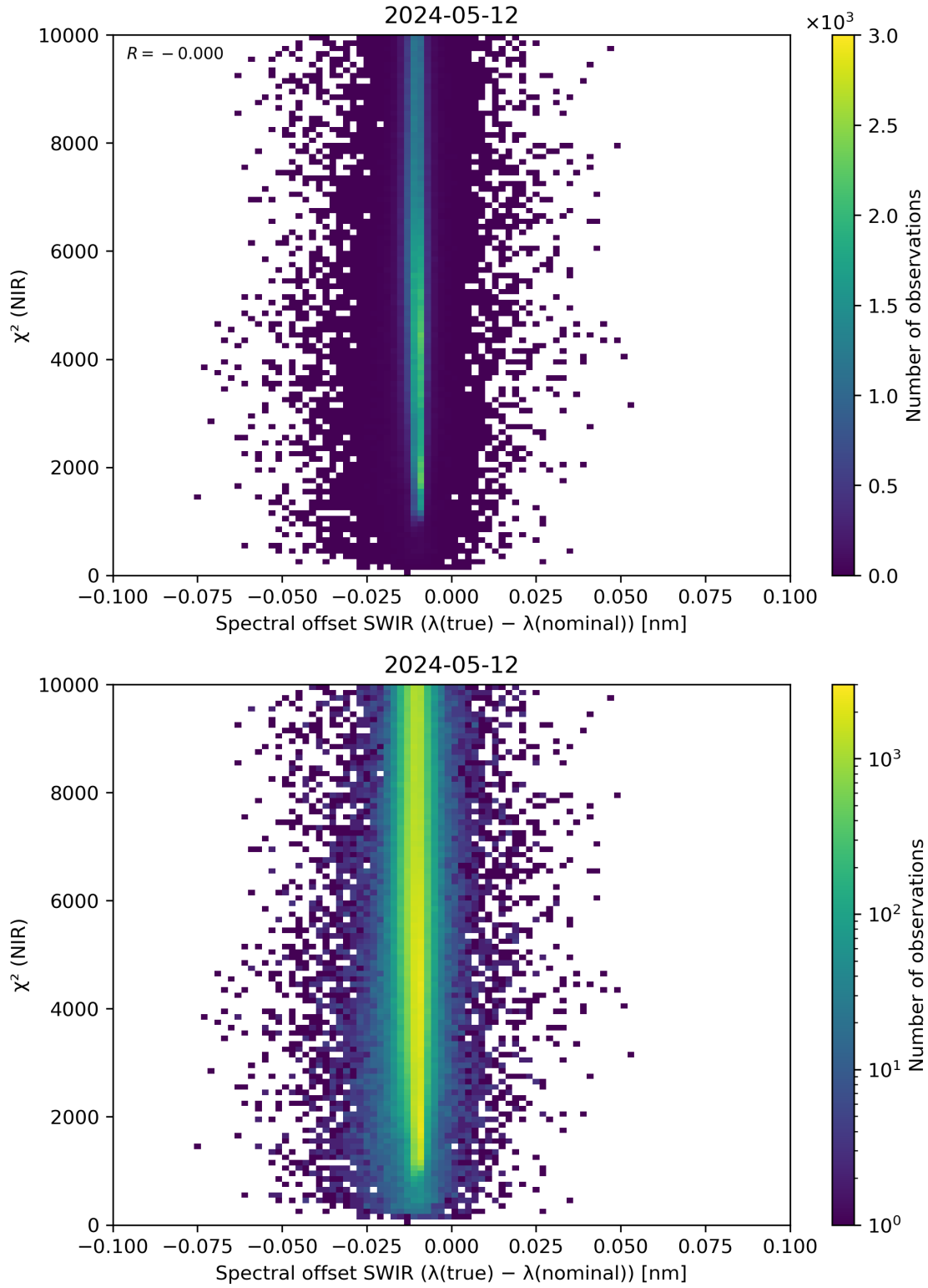
Figure 117: Scatter density plot of “Spectral offset SWIR ( \lambda(\text{true}) - \lambda(\text{nominal}) )” against “ \chi^2 (NIR)” for 2024-05-12 to 2024-05-13.
