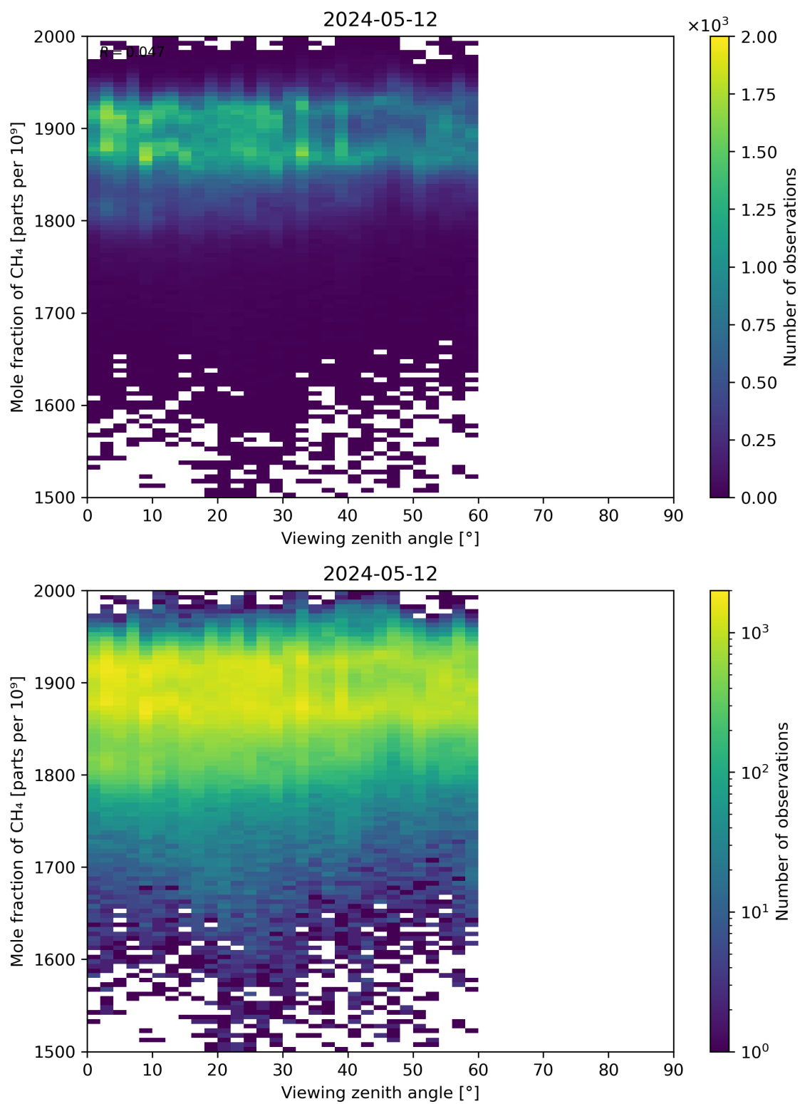
Figure 110: Scatter density plot of “Viewing zenith angle” against “Mole fraction of CH 4 ” for 2024-05-12 to 2024-05-13.
