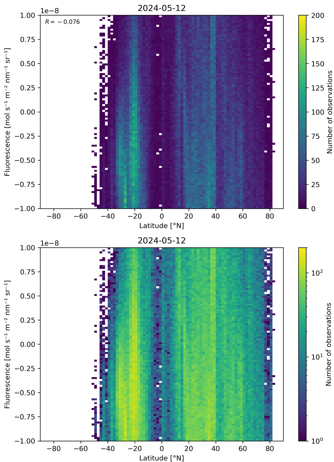
Figure 56: Scatter density plot of “Latitude” against “Fluorescence” for 2024-05-12 to 2024-05-13.
