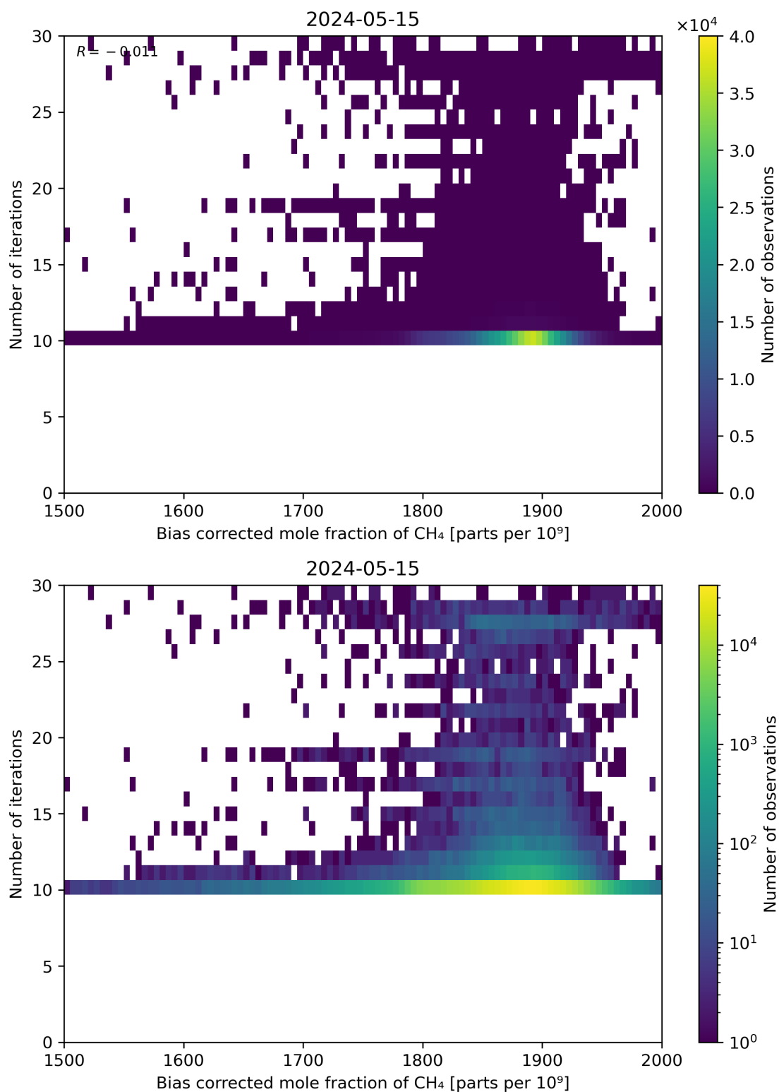
Figure 67: Scatter density plot of “Bias corrected mole fraction of CH 4 ” against “Number of iterations” for 2024-05-14 to 2024-05-16.
