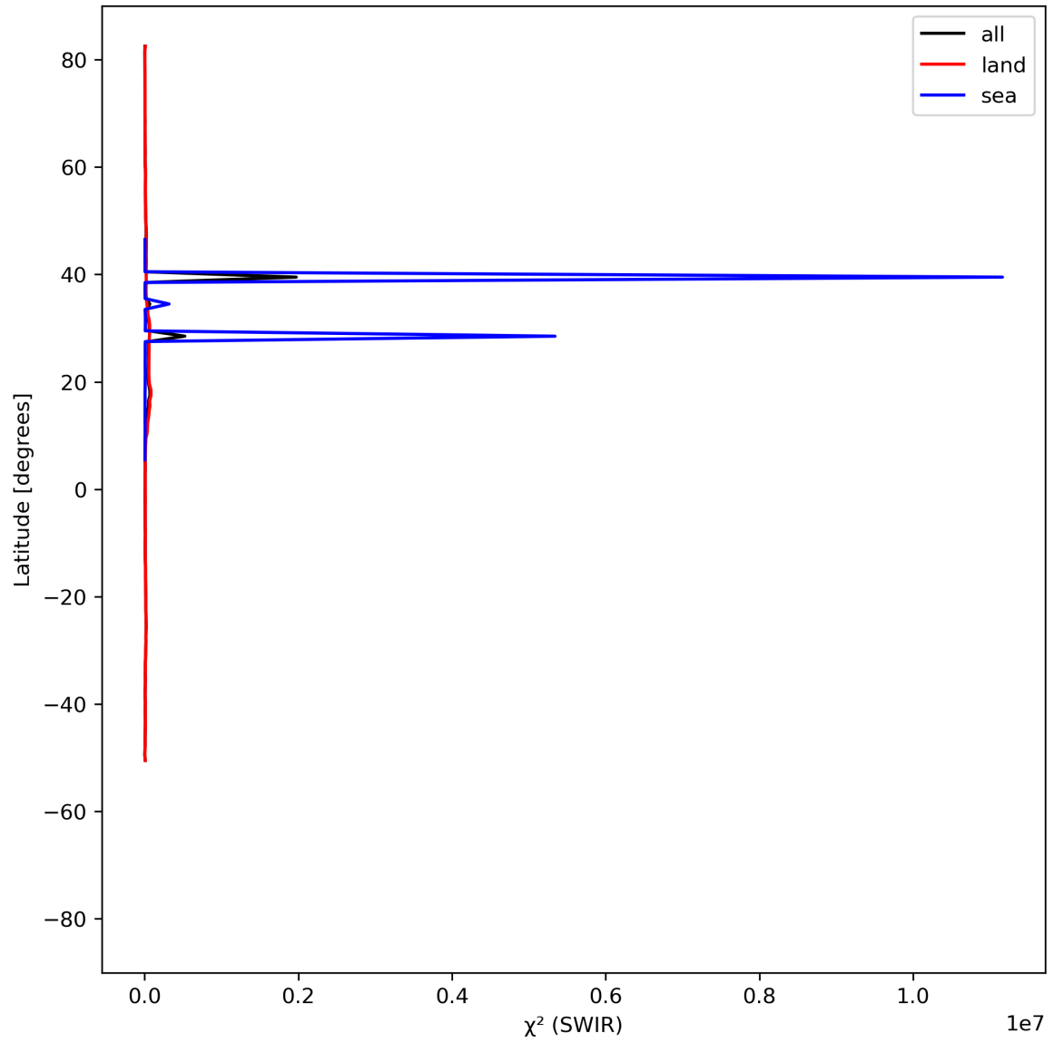
Figure 17: Zonal average of “ \chi^2 (SWIR)” for 2024-05-14 to 2024-05-16.
