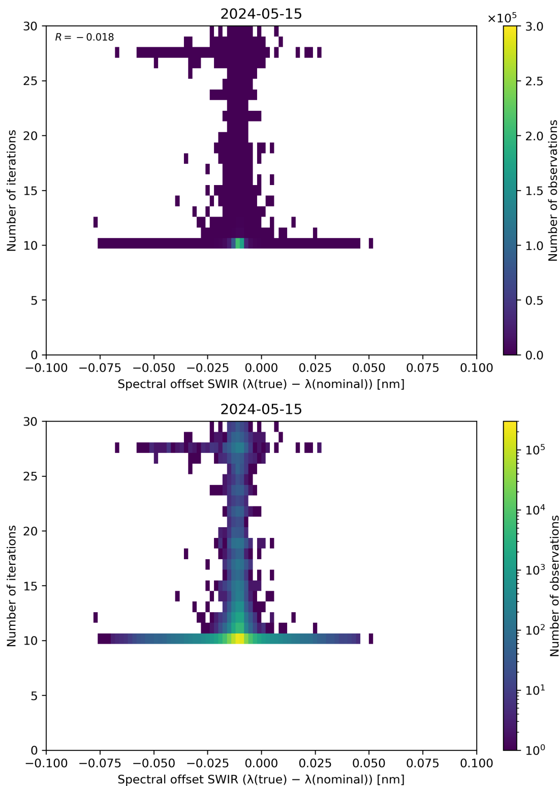
Figure 121: Scatter density plot of “Spectral offset SWIR ( \lambda(\text{true}) - \lambda(\text{nominal}) )” against “Number of iterations” for 2024-05-14 to 2024-05-16.
