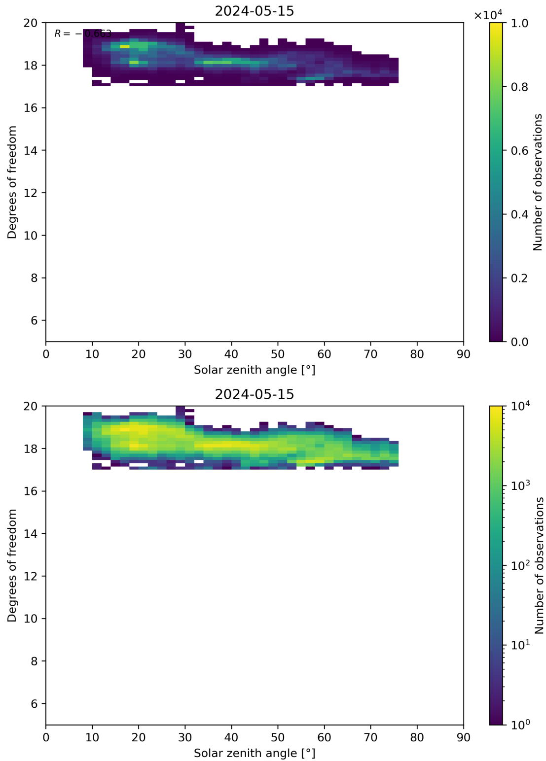
Figure 96: Scatter density plot of “Solar zenith angle” against “Degrees of freedom” for 2024-05-14 to 2024-05-16.
