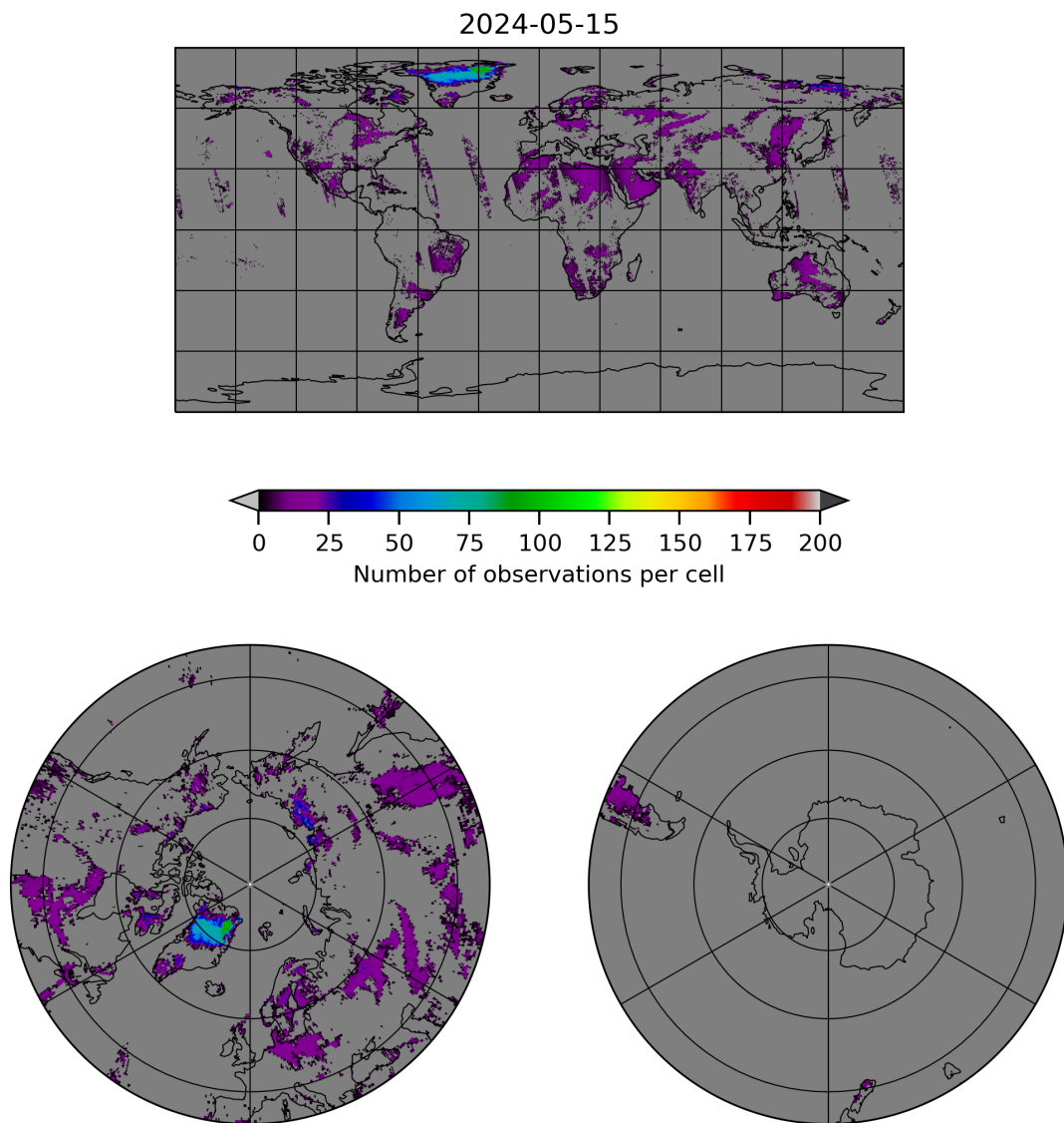
Figure 10: Map of the number of observations for 2024-05-14 to 2024-05-16
