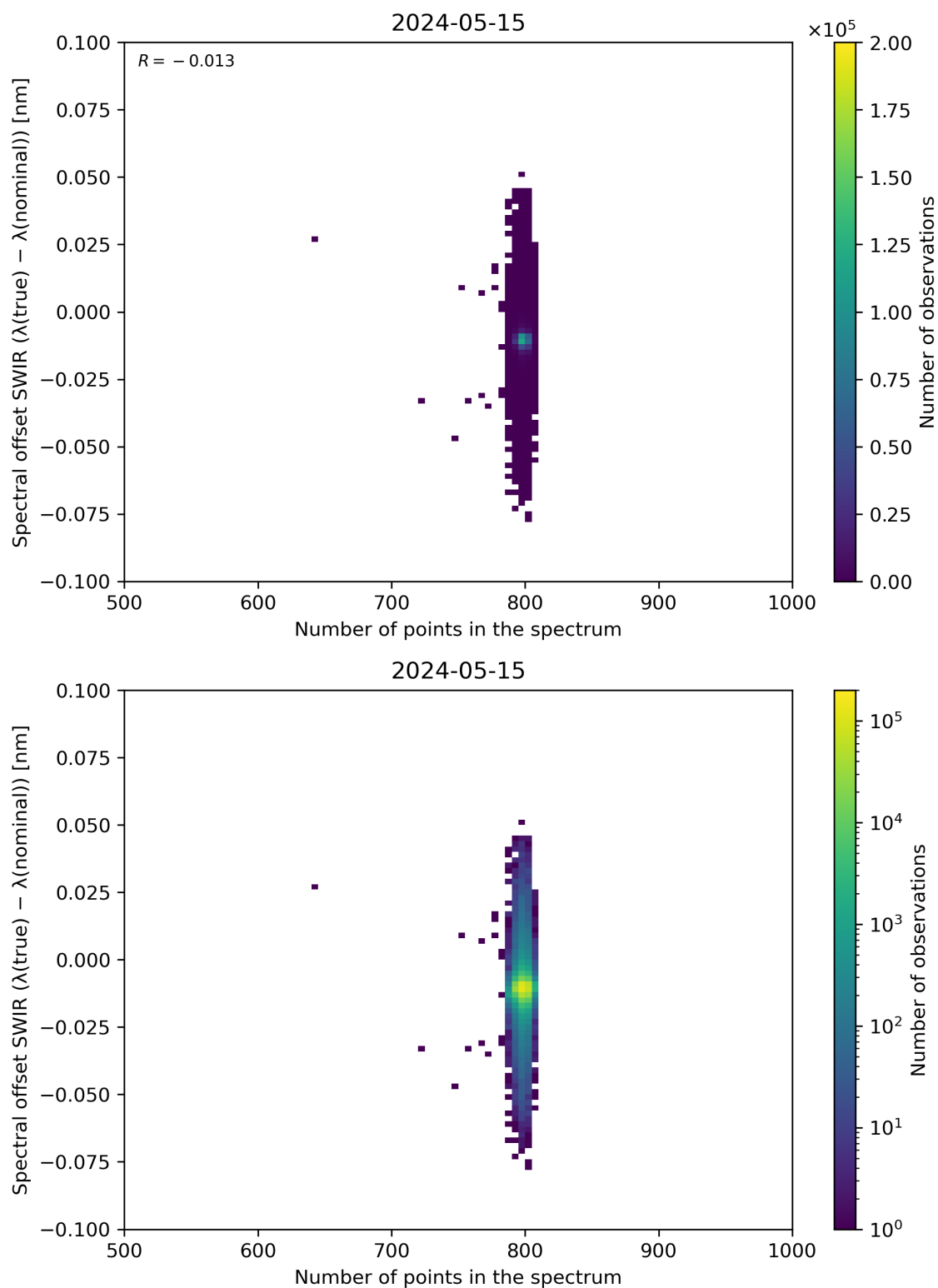
Figure 93: Scatter density plot of “Number of points in the spectrum” against “Spectral offset SWIR ( \lambda(\text{true}) - \lambda(\text{nominal}) )” for 2024-05-14 to 2024-05-16.
