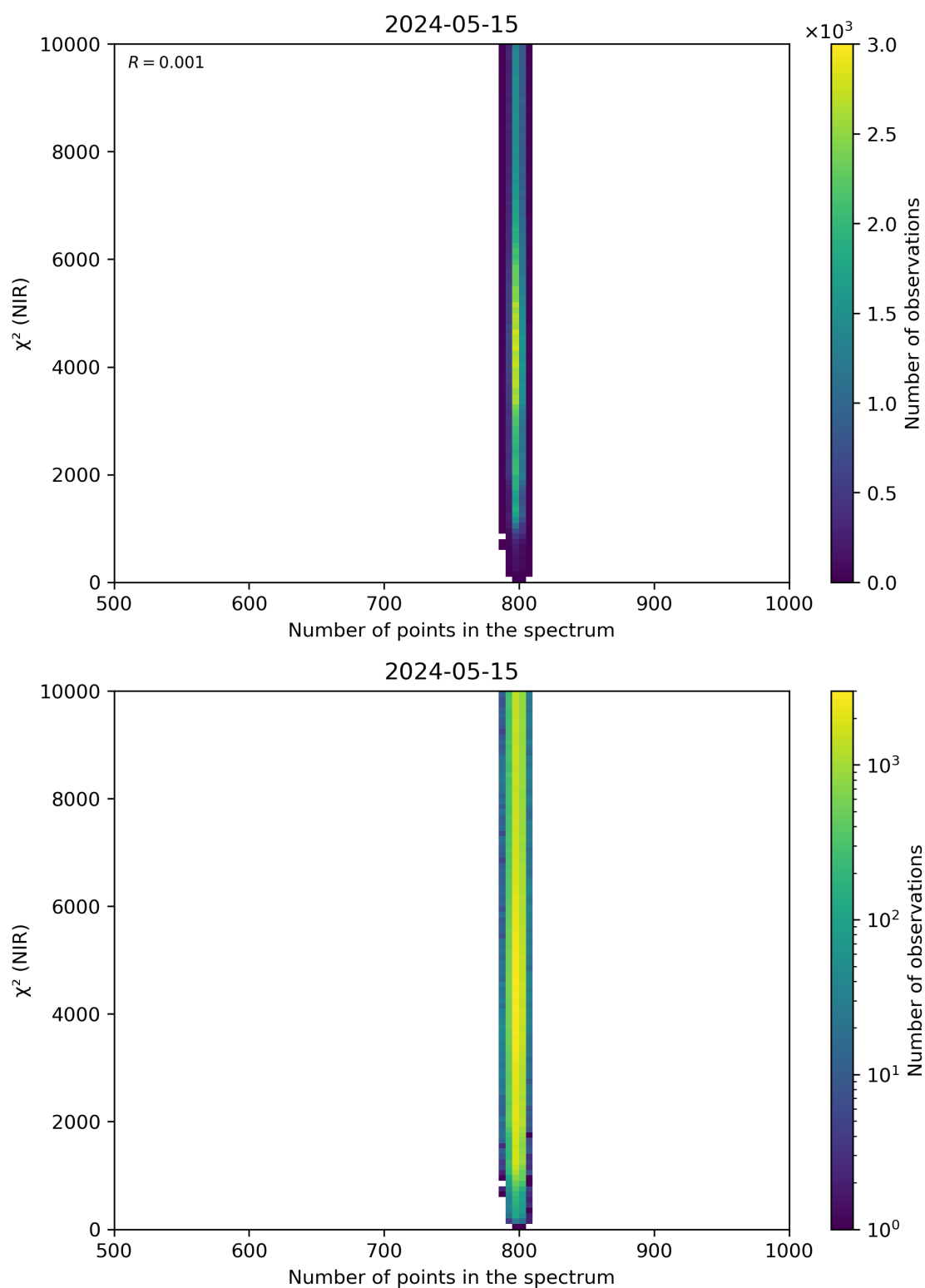
Figure 88: Scatter density plot of “Number of points in the spectrum” against “ \chi^2 (NIR)” for 2024-05-14 to 2024-05-16.
