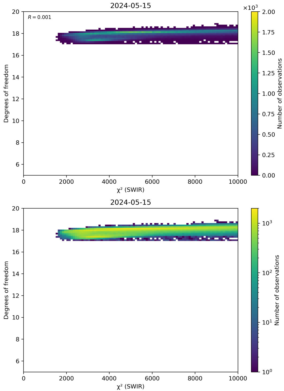
Figure 48: Scatter density plot of “ \chi^2 (SWIR)” against “Degrees of freedom” for 2024-05-14 to 2024-05-16.
