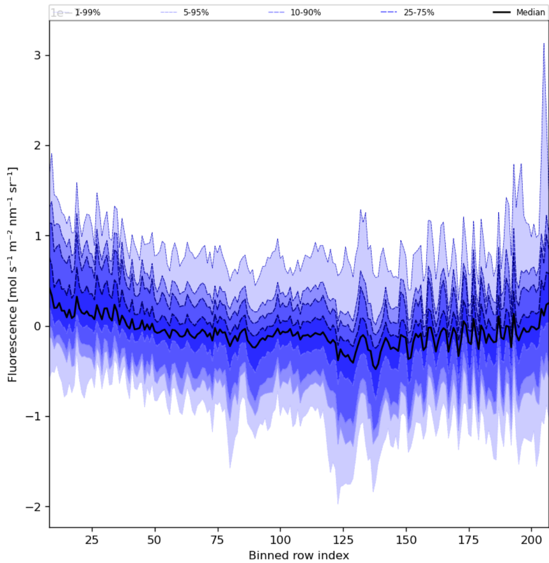
Figure 43: Along track statistics of “Fluorescence” for 2024-05-14 to 2024-05-16
