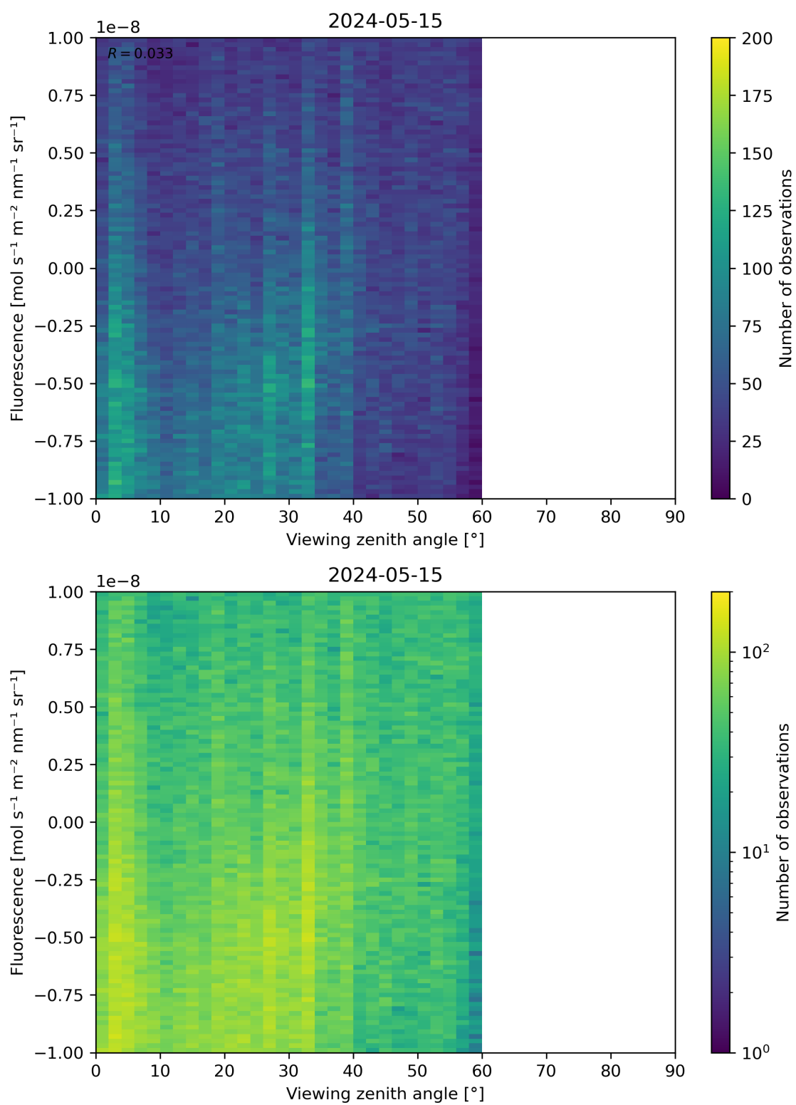
Figure 108: Scatter density plot of “Viewing zenith angle” against “Fluorescence” for 2024-05-14 to 2024-05-16.
