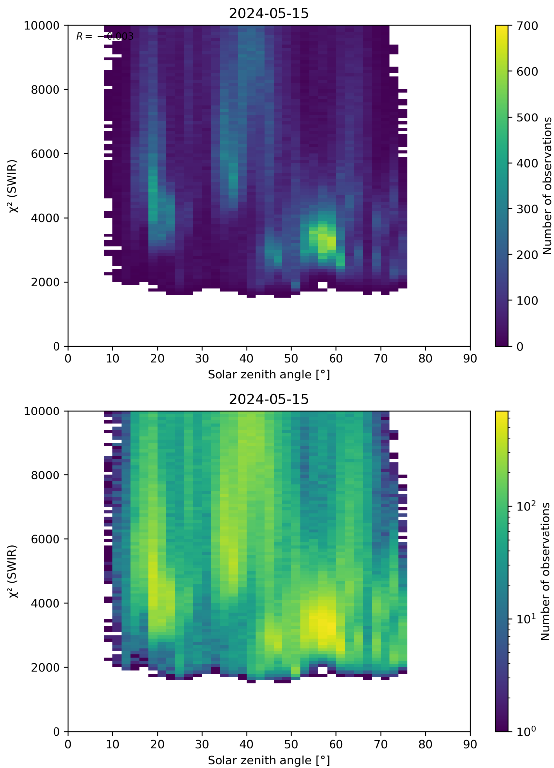
Figure 95: Scatter density plot of “Solar zenith angle” against “ \chi^2 (SWIR)” for 2024-05-14 to 2024-05-16.
