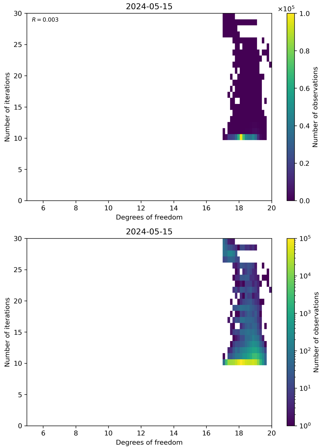
Figure 52: Scatter density plot of “Degrees of freedom” against “Number of iterations” for 2024-05-14 to 2024-05-16.
