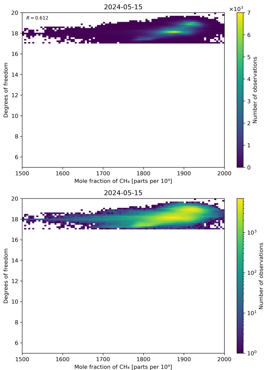
Figure 72: Scatter density plot of “Mole fraction of CH 4 ” against “Degrees of freedom” for 2024-05-14 to 2024-05-16.
