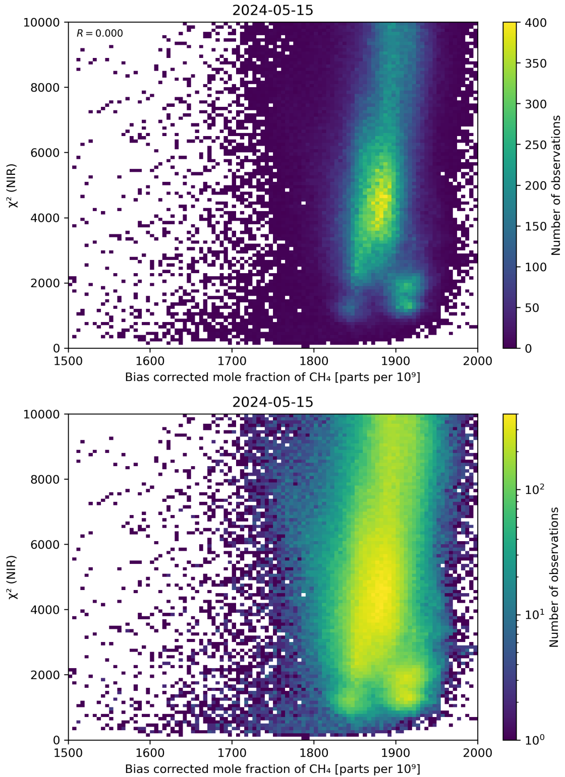
Figure 63: Scatter density plot of “Bias corrected mole fraction of CH 4 ” against “ \chi^2 (NIR)” for 2024-05-14 to 2024-05-16.
