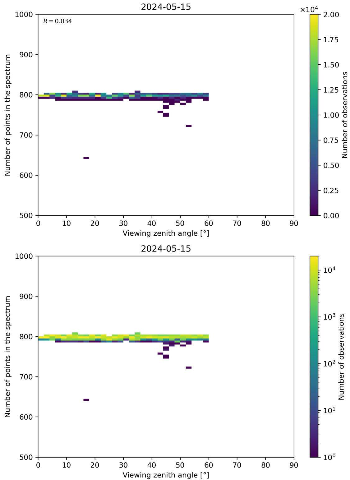
Figure 114: Scatter density plot of “Viewing zenith angle” against “Number of points in the spectrum” for 2024-05-14 to 2024-05-16.
