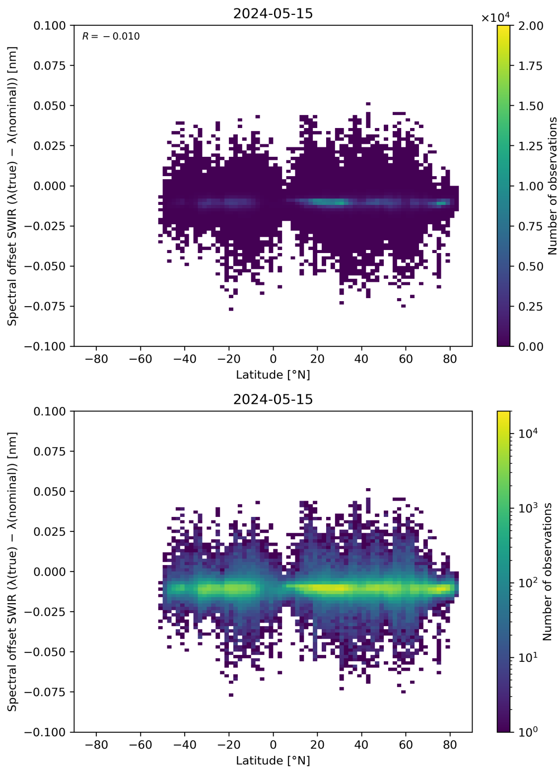
Figure 62: Scatter density plot of “Latitude” against “Spectral offset SWIR ( \lambda(\text{true}) - \lambda(\text{nominal}) )” for 2024-05-14 to 2024-05-16.
