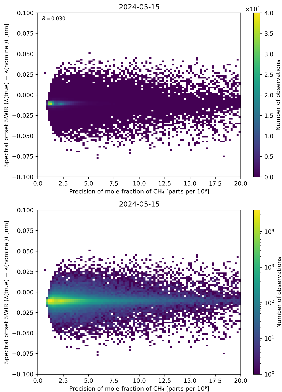
Figure 85: Scatter density plot of “Precision of mole fraction of CH 4 ” against “Spectral offset SWIR ( \lambda(\text{true}) - \lambda(\text{nominal}) )” for 2024-05-14 to 2024-05-16.
