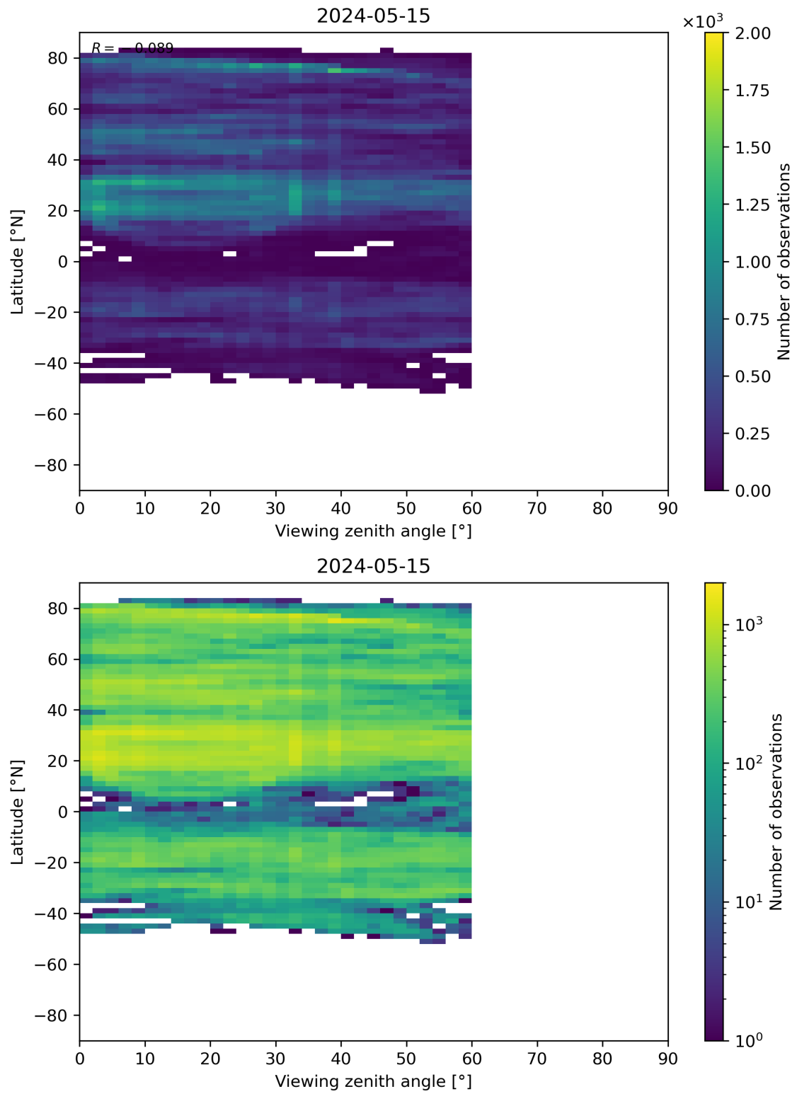
Figure 109: Scatter density plot of “Viewing zenith angle” against “Latitude” for 2024-05-14 to 2024-05-16.
