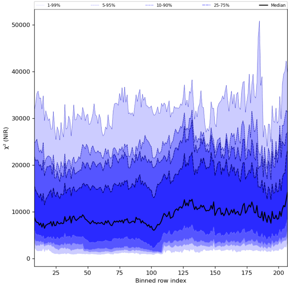
Figure 40: Along track statistics of “ \chi^2 (NIR)” for 2024-05-14 to 2024-05-16
