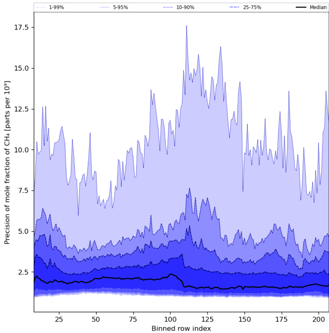
Figure 35: Along track statistics of “Precision of mole fraction of CH 4 ” for 2024-05-14 to 2024-05-16
