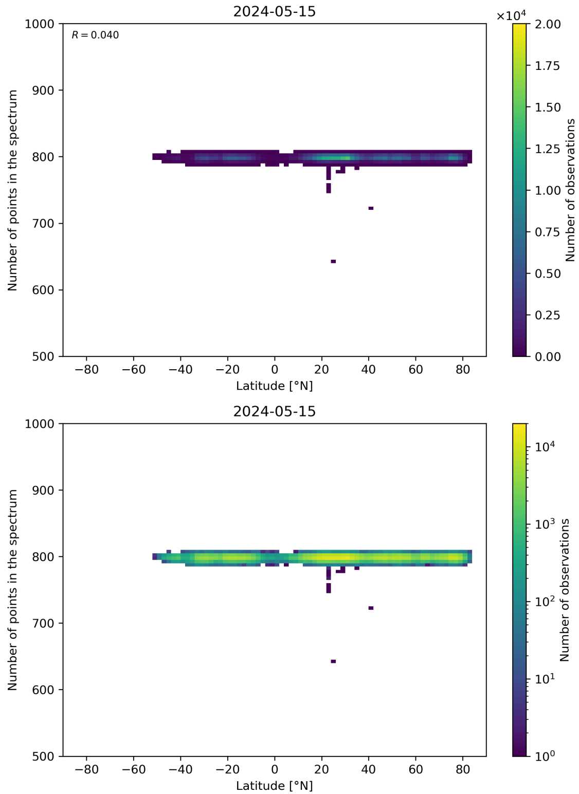
Figure 61: Scatter density plot of “Latitude” against “Number of points in the spectrum” for 2024-05-14 to 2024-05-16.
