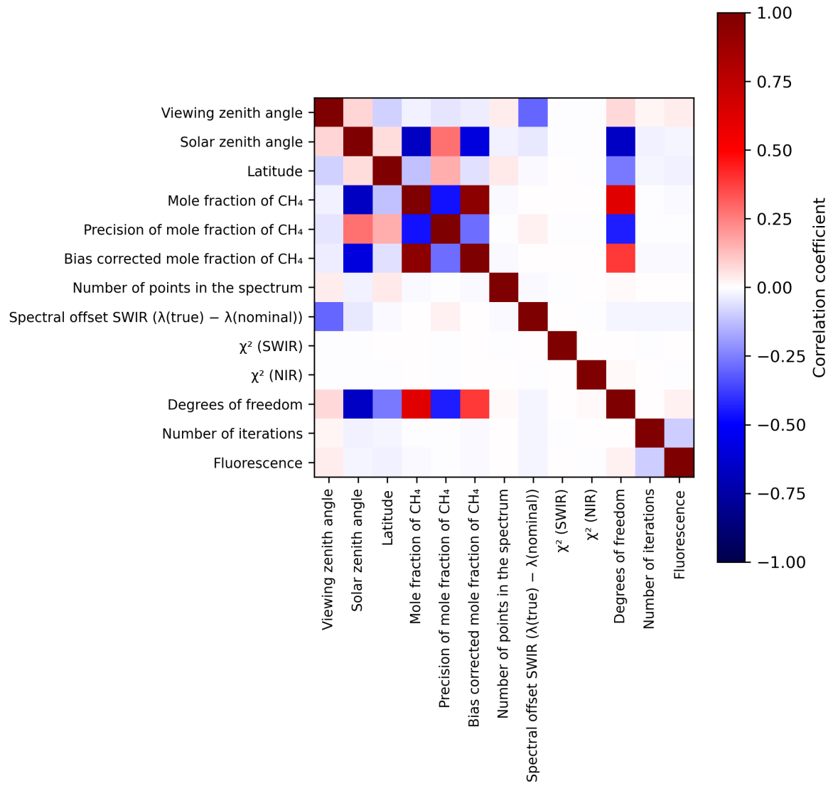
Figure 2: Map of correlation matrix for 2024-05-14 to 2024-05-16.
