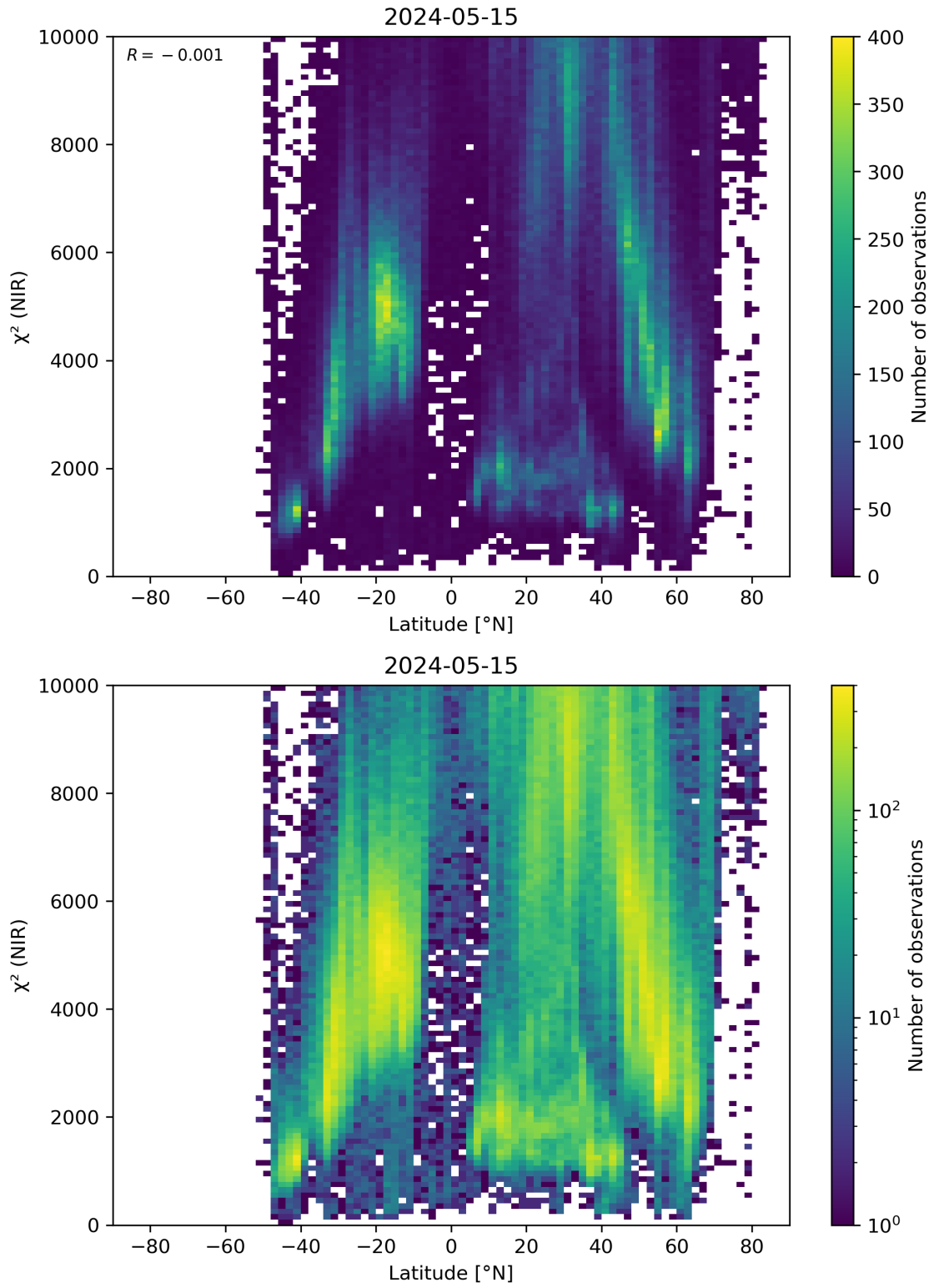
Figure 53: Scatter density plot of “Latitude” against “ \chi^2 (NIR)” for 2024-05-14 to 2024-05-16.
