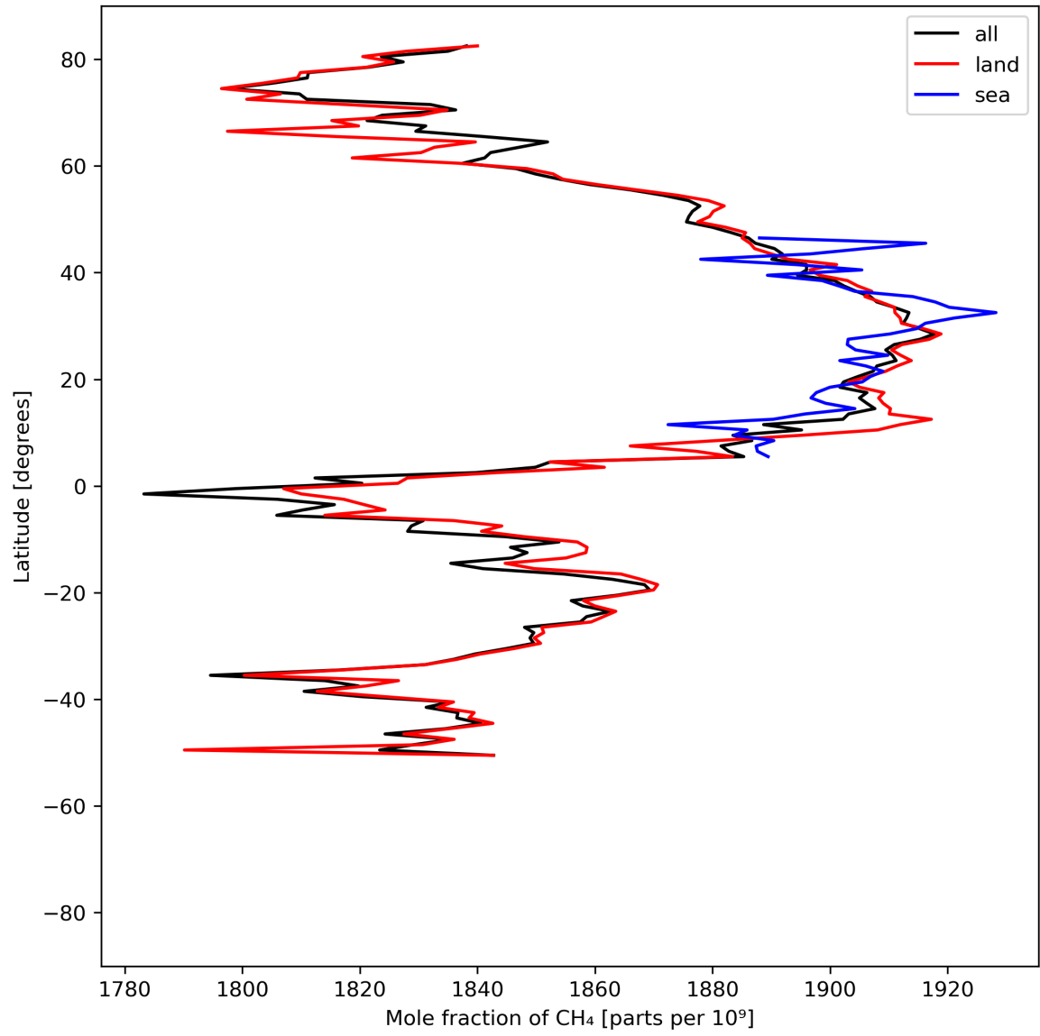
Figure 12: Zonal average of “Mole fraction of \text{CH}_4 ” for 2024-05-14 to 2024-05-16.
