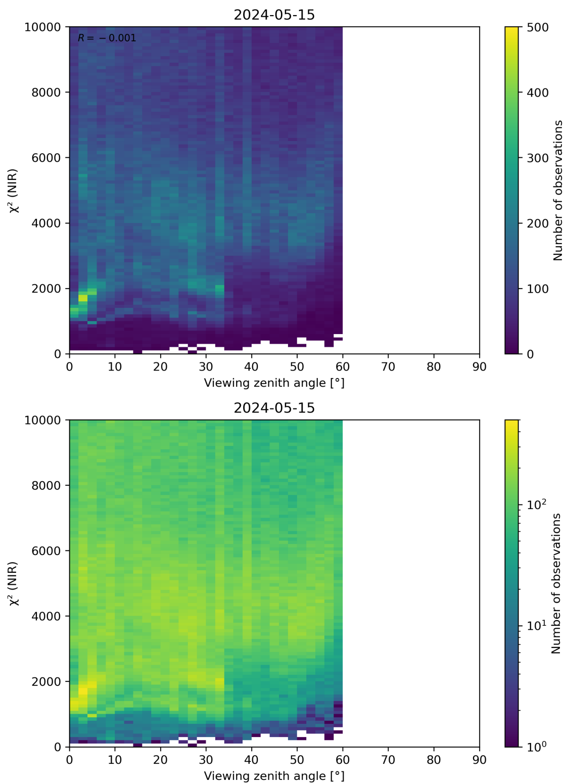
Figure 105: Scatter density plot of “Viewing zenith angle” against “ \chi^2 (NIR)” for 2024-05-14 to 2024-05-16.
