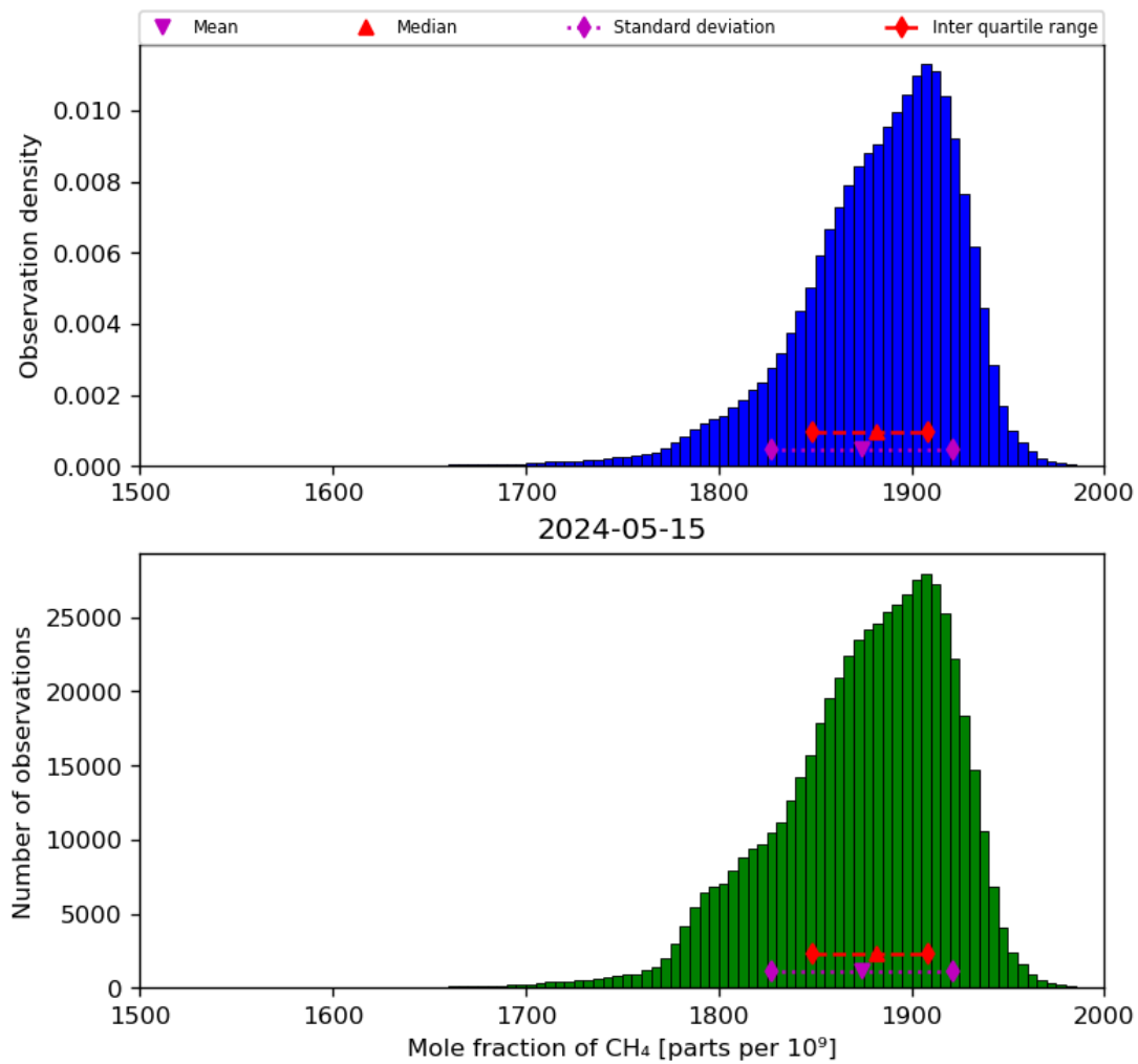
Figure 23: Histogram of “Mole fraction of CH 4 ” for 2024-05-14 to 2024-05-16
