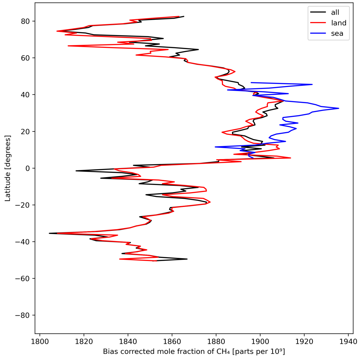
Figure 14: Zonal average of “Bias corrected mole fraction of \text{CH}_4 ” for 2024-05-14 to 2024-05-16.
