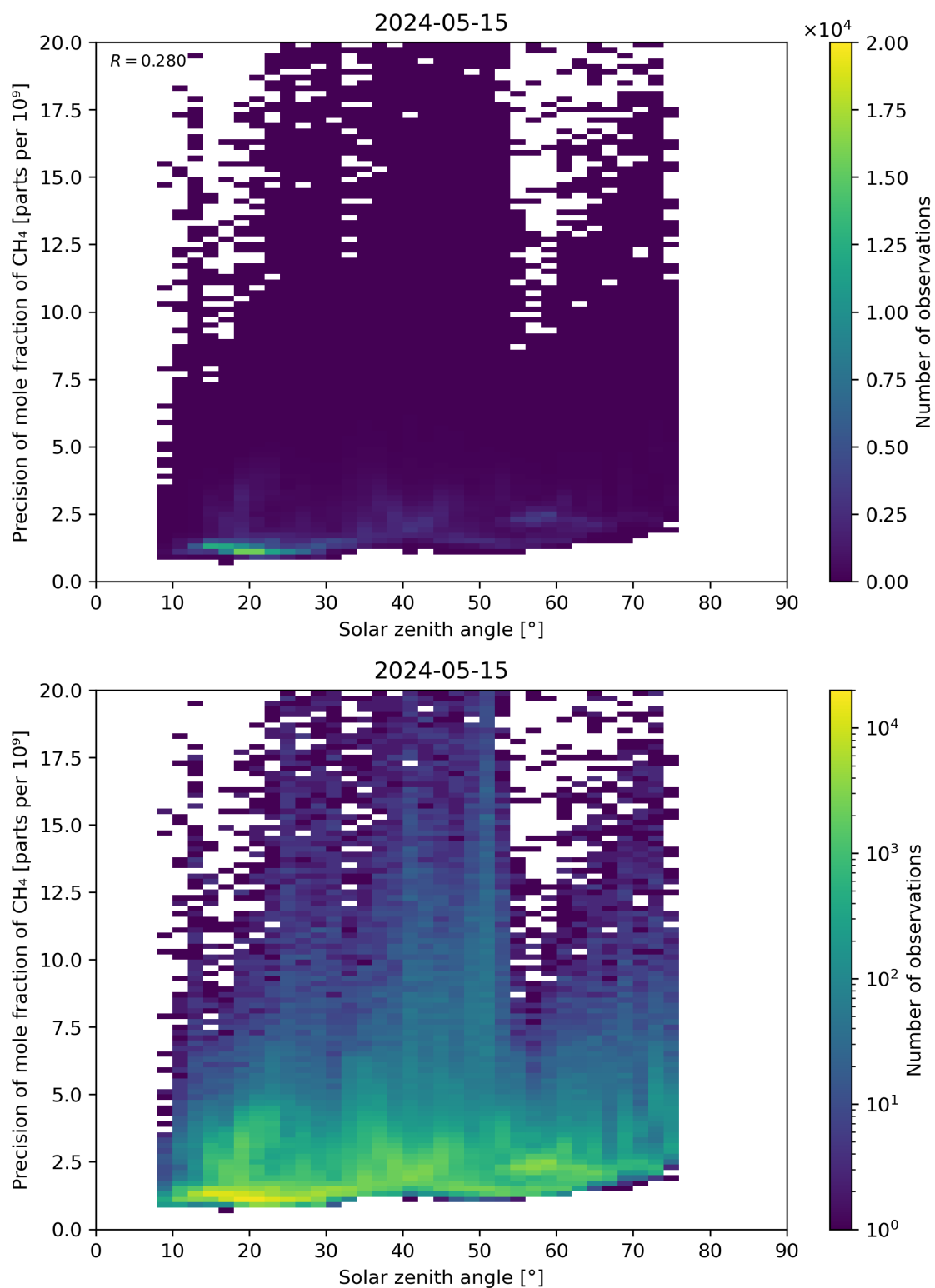
Figure 101: Scatter density plot of “Solar zenith angle” against “Precision of mole fraction of \text{CH}_4 ” for 2024-05-14 to 2024-05-16.
