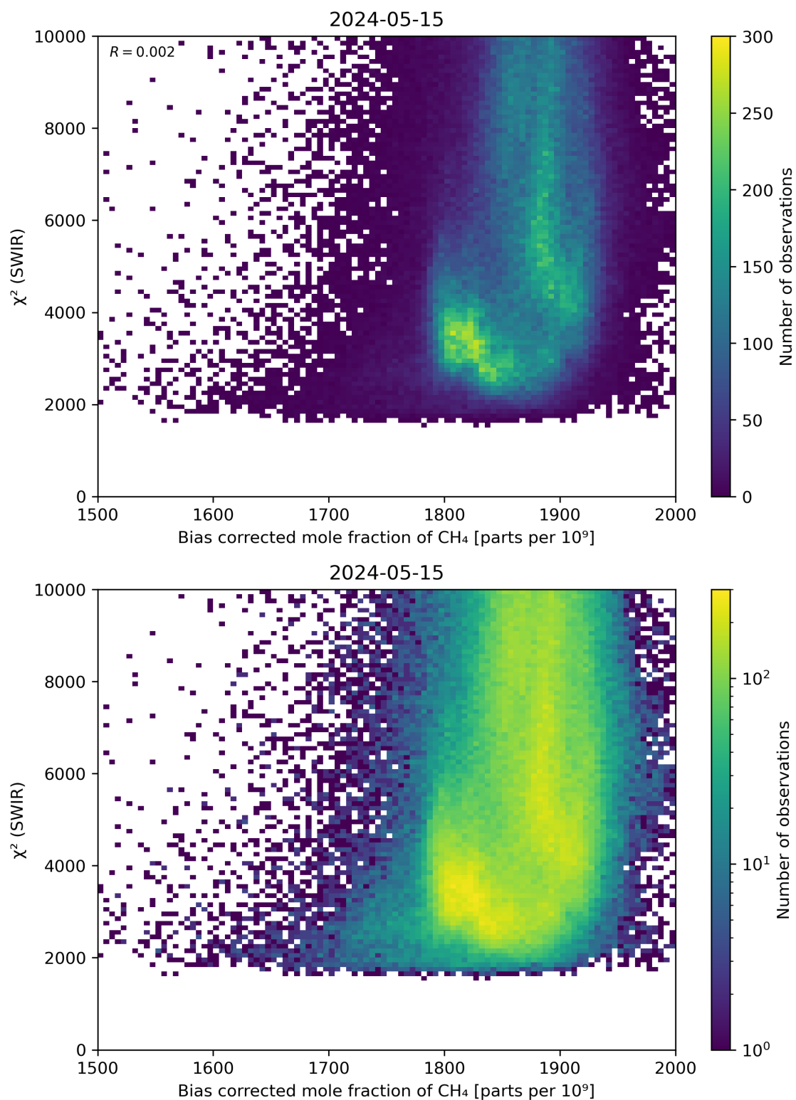
Figure 64: Scatter density plot of “Bias corrected mole fraction of \text{CH}_4 ” against “ \chi^2 (SWIR)” for 2024-05-14 to 2024-05-16.
