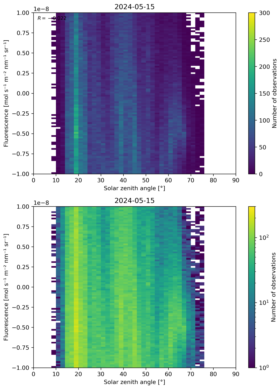
Figure 97: Scatter density plot of “Solar zenith angle” against “Fluorescence” for 2024-05-14 to 2024-05-16.
