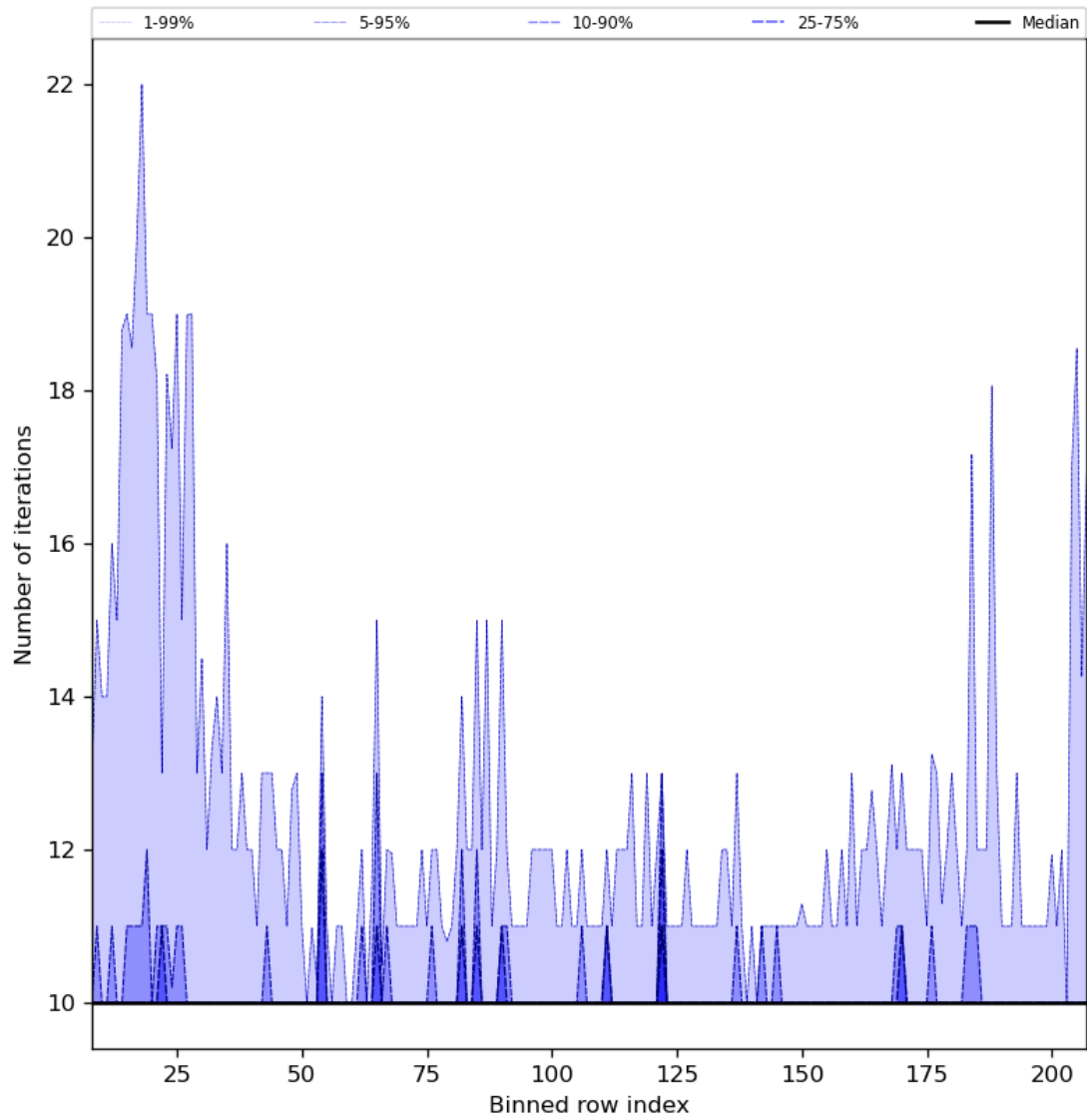
Figure 42: Along track statistics of “Number of iterations” for 2024-05-14 to 2024-05-16
