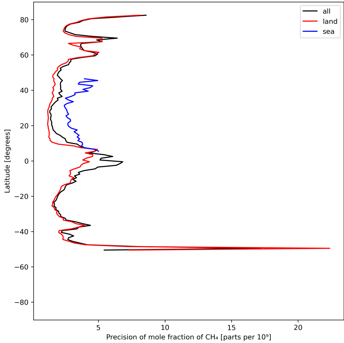
Figure 13: Zonal average of “Precision of mole fraction of CH 4 ” for 2024-05-14 to 2024-05-16.
