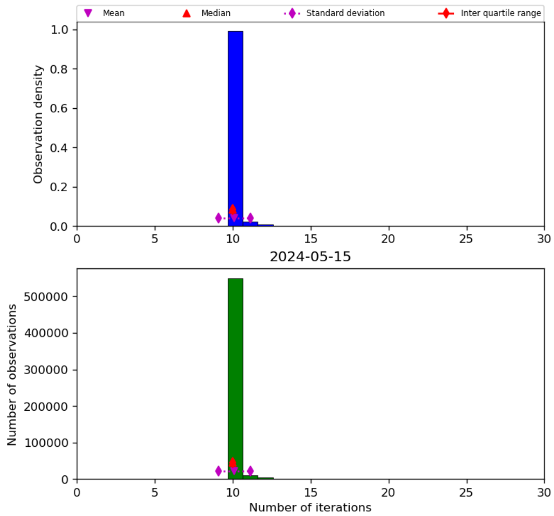
Figure 31: Histogram of “Number of iterations” for 2024-05-14 to 2024-05-16
