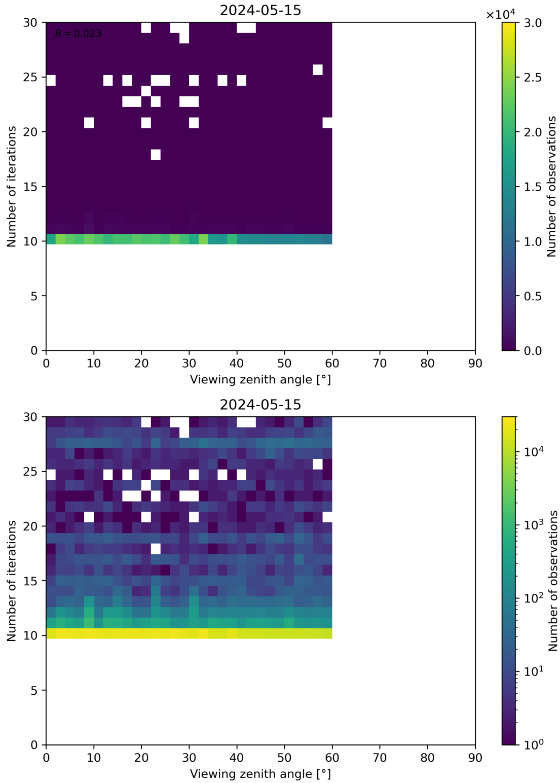
Figure 113: Scatter density plot of “Viewing zenith angle” against “Number of iterations” for 2024-05-14 to 2024-05-16.
