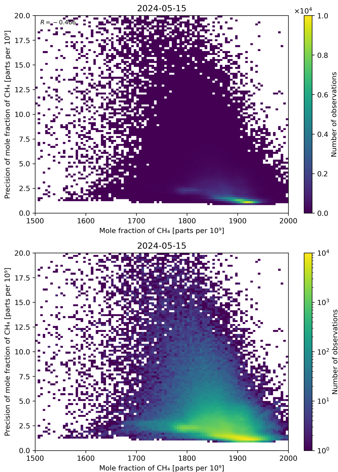
Figure 75: Scatter density plot of “Mole fraction of CH 4 ” against “Precision of mole fraction of CH 4 ” for 2024-05-14 to 2024-05-16.
