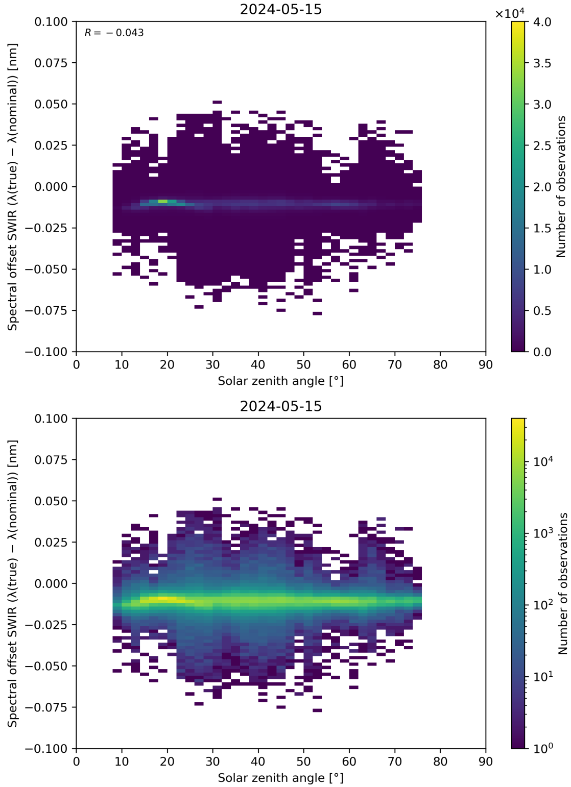
Figure 104: Scatter density plot of “Solar zenith angle” against “Spectral offset SWIR ( \lambda(\text{true}) - \lambda(\text{nominal}) )” for 2024-05-14 to 2024-05-16.
