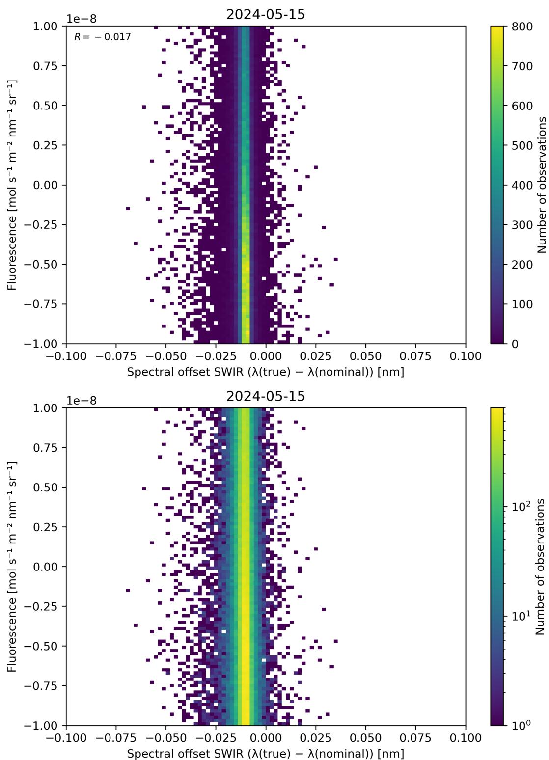
Figure 120: Scatter density plot of “Spectral offset SWIR ( \lambda(\text{true}) - \lambda(\text{nominal}) )” against “Fluorescence” for 2024-05-14 to 2024-05-16.
