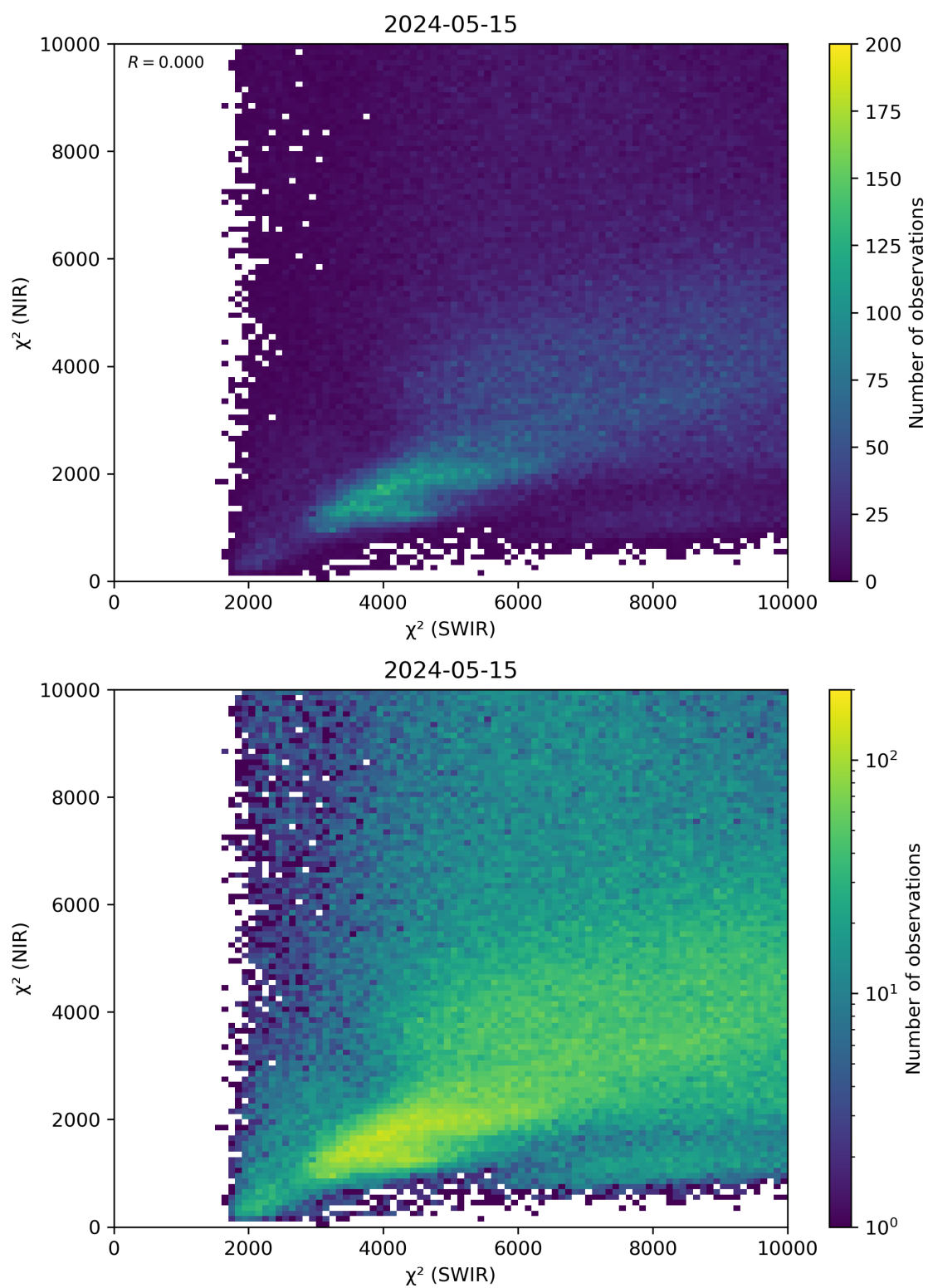
Figure 47: Scatter density plot of “ \chi^2 (SWIR)” against “ \chi^2 (NIR)” for 2024-05-14 to 2024-05-16.
