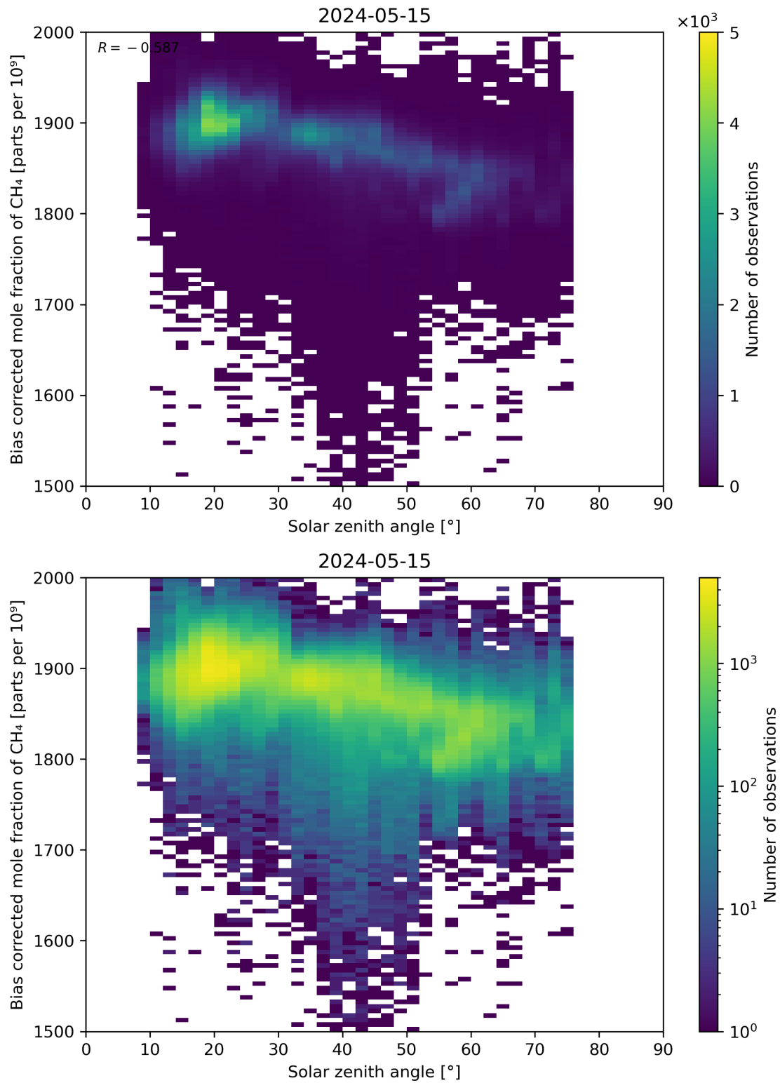
Figure 100: Scatter density plot of “Solar zenith angle” against “Bias corrected mole fraction of \text{CH}_4 ” for 2024-05-14 to 2024-05-16.
