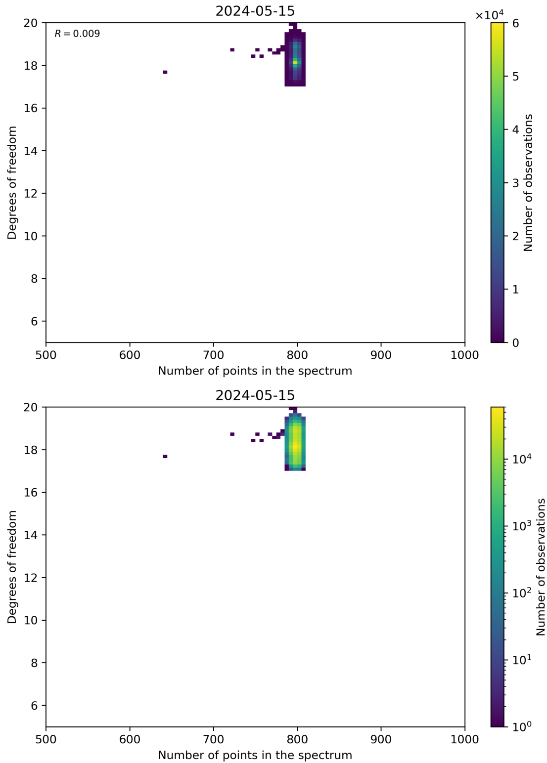
Figure 90: Scatter density plot of “Number of points in the spectrum” against “Degrees of freedom” for 2024-05-14 to 2024-05-16.
