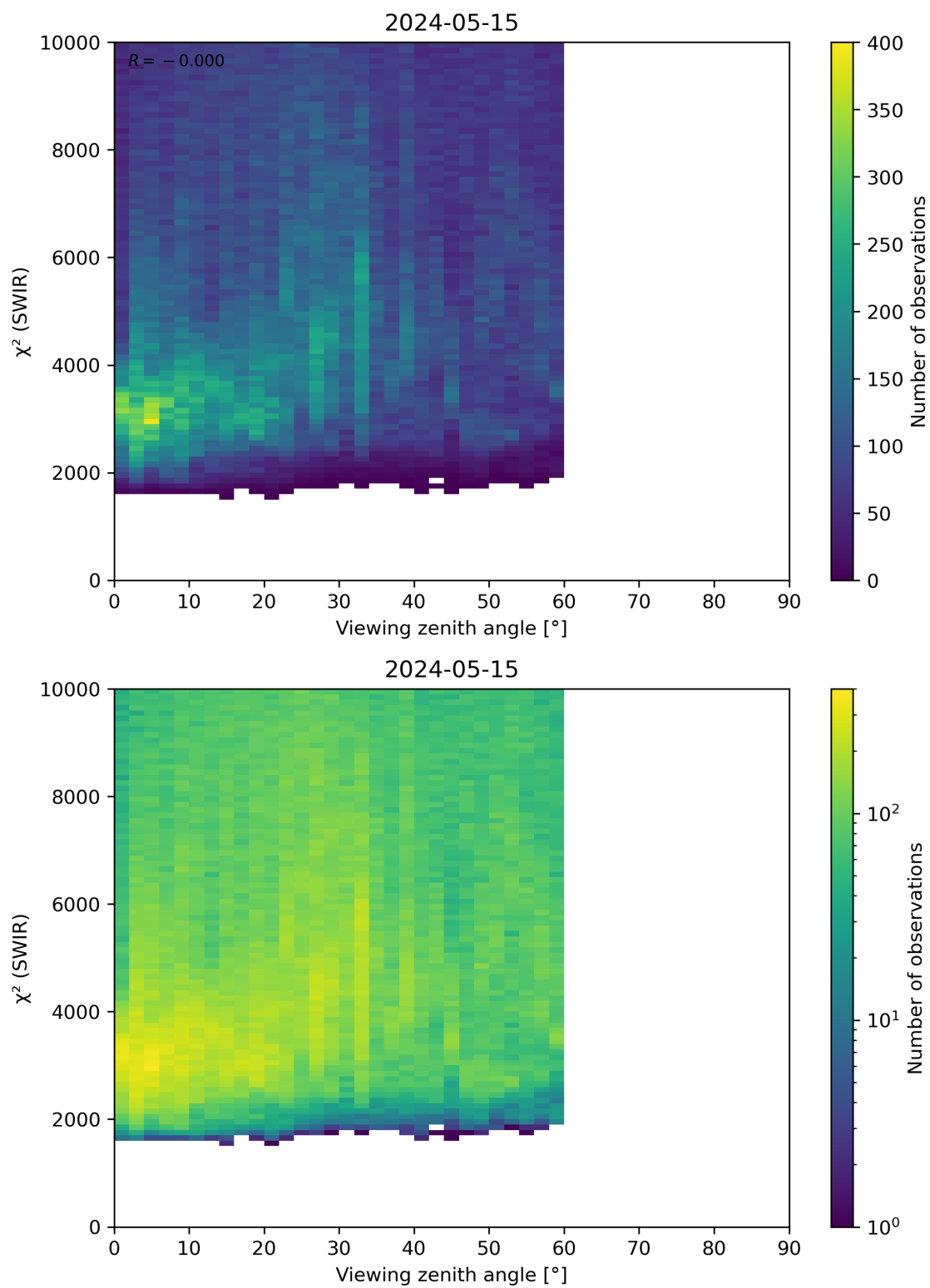
Figure 106: Scatter density plot of “Viewing zenith angle” against “ \chi^2 (SWIR)” for 2024-05-14 to 2024-05-16.
