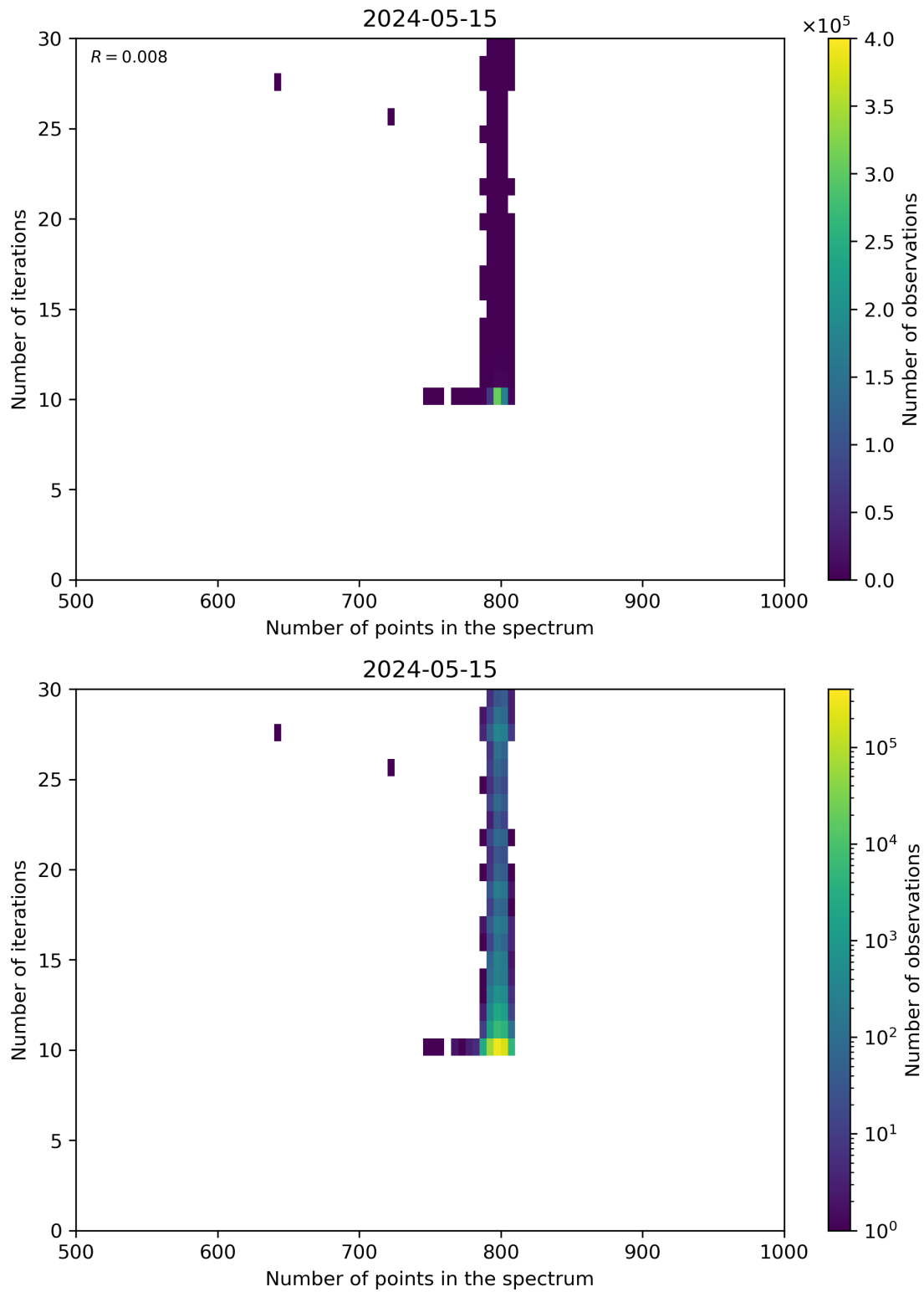
Figure 92: Scatter density plot of “Number of points in the spectrum” against “Number of iterations” for 2024-05-14 to 2024-05-16.
