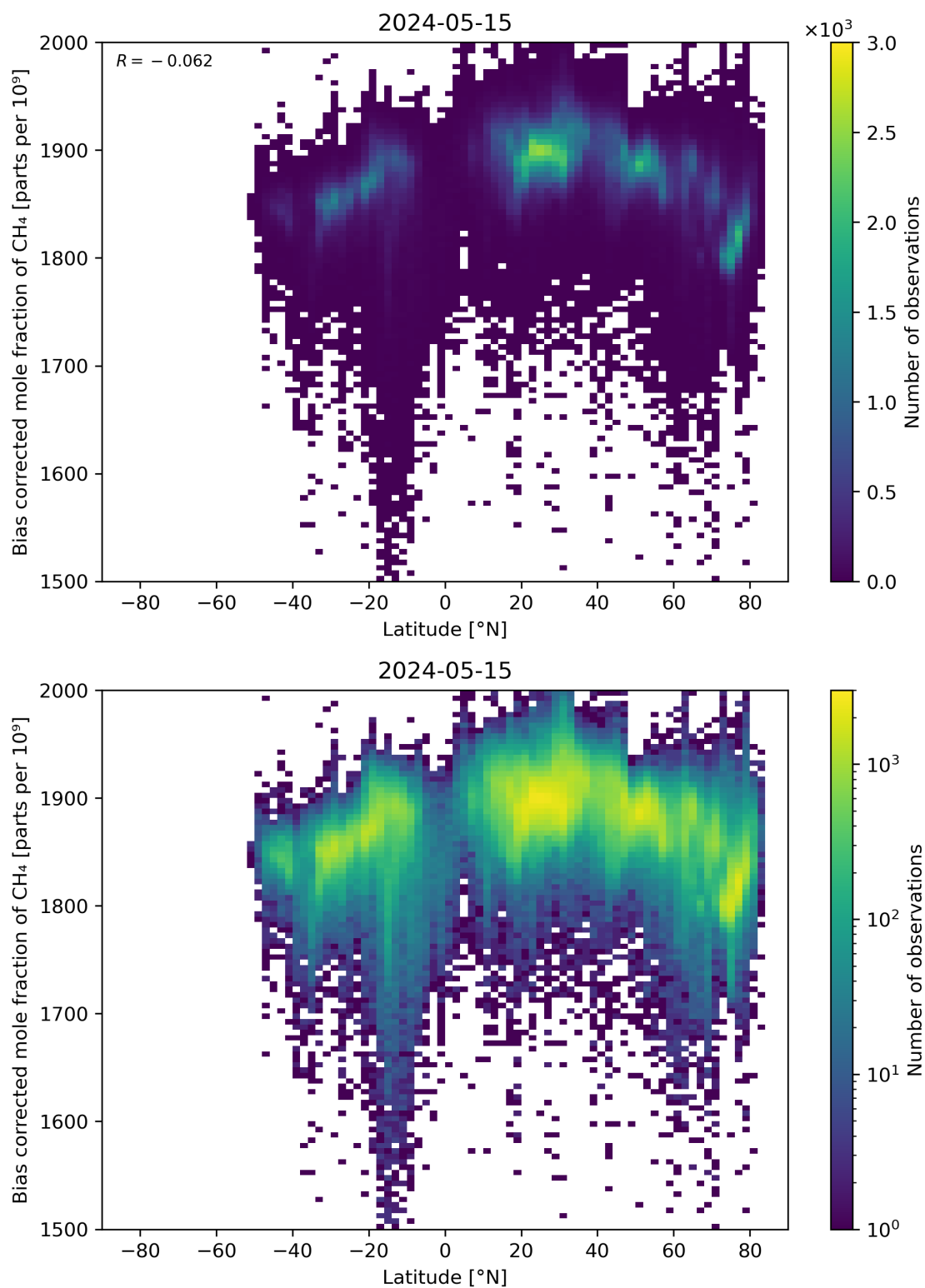
Figure 58: Scatter density plot of “Latitude” against “Bias corrected mole fraction of \text{CH}_4 ” for 2024-05-14 to 2024-05-16.
