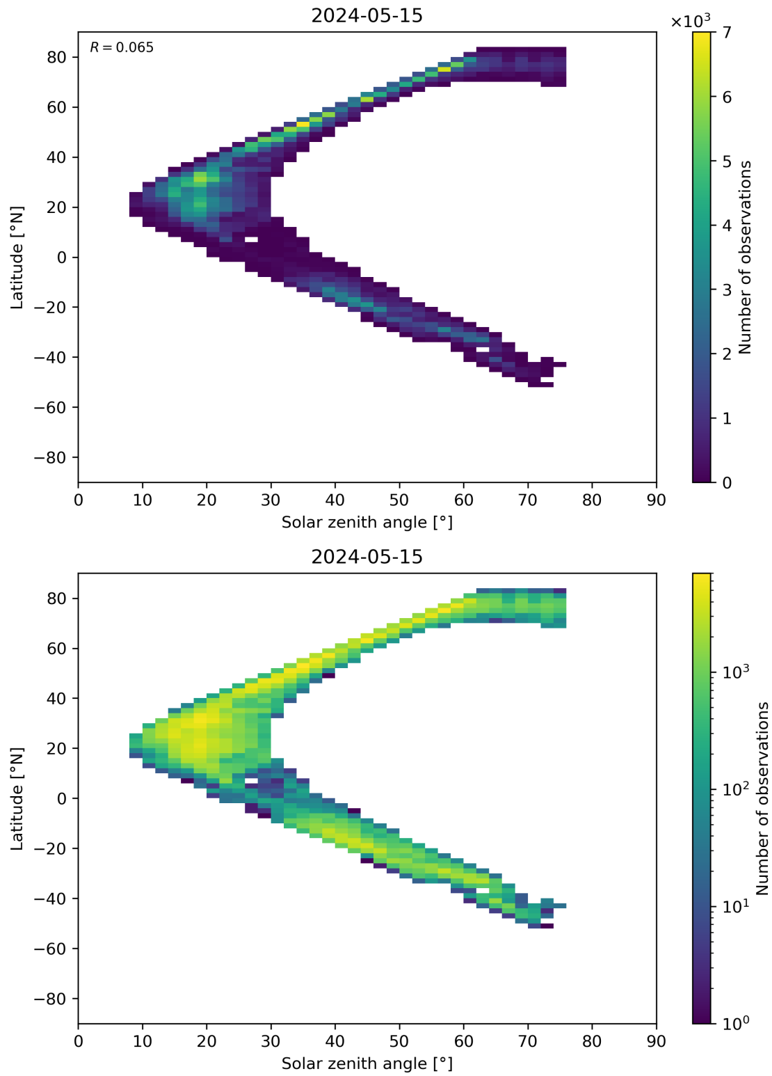
Figure 98: Scatter density plot of “Solar zenith angle” against “Latitude” for 2024-05-14 to 2024-05-16.
