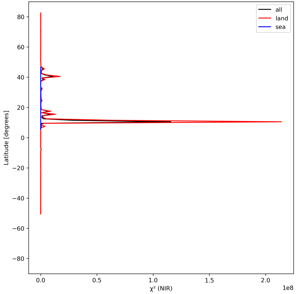
Figure 18: Zonal average of “ \chi^2 (NIR)” for 2024-05-14 to 2024-05-16.
