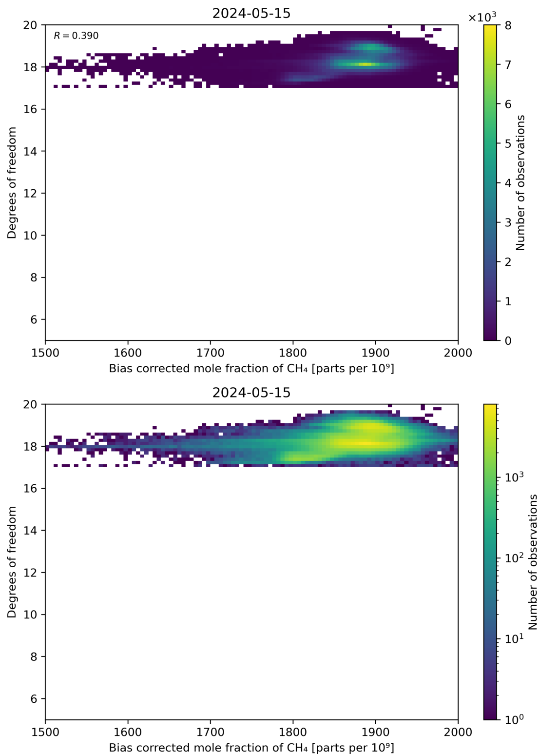
Figure 65: Scatter density plot of “Bias corrected mole fraction of CH 4 ” against “Degrees of freedom” for 2024-05-14 to 2024-05-16.
