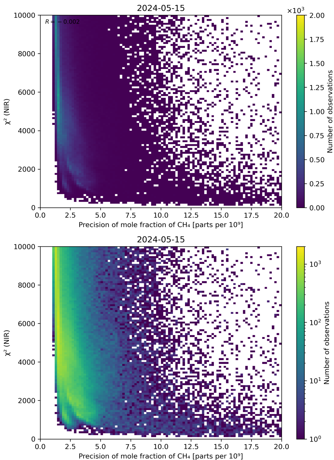
Figure 78: Scatter density plot of “Precision of mole fraction of CH 4 ” against “ \chi^2 (NIR)” for 2024-05-14 to 2024-05-16.
