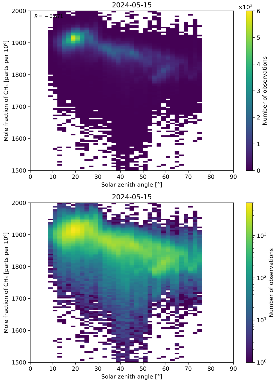
Figure 99: Scatter density plot of “Solar zenith angle” against “Mole fraction of CH 4 ” for 2024-05-14 to 2024-05-16.
