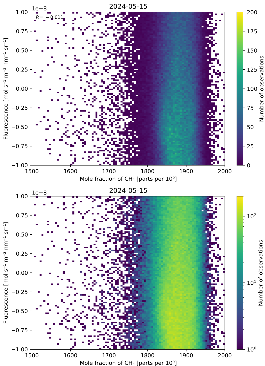
Figure 73: Scatter density plot of “Mole fraction of \text{CH}_4 ” against “Fluorescence” for 2024-05-14 to 2024-05-16.
