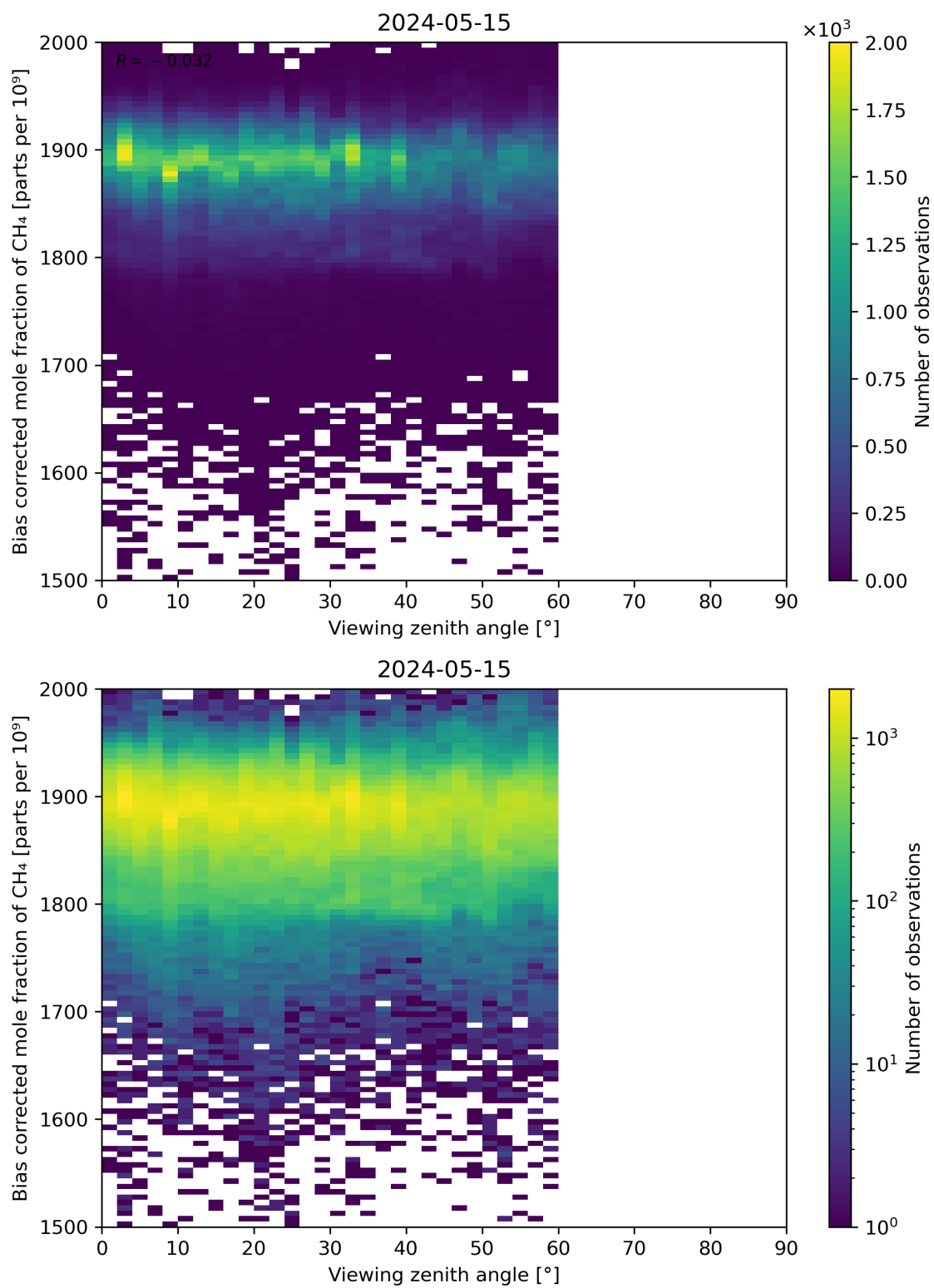
Figure 111: Scatter density plot of “Viewing zenith angle” against “Bias corrected mole fraction of CH 4 ” for 2024-05-14 to 2024-05-16.
