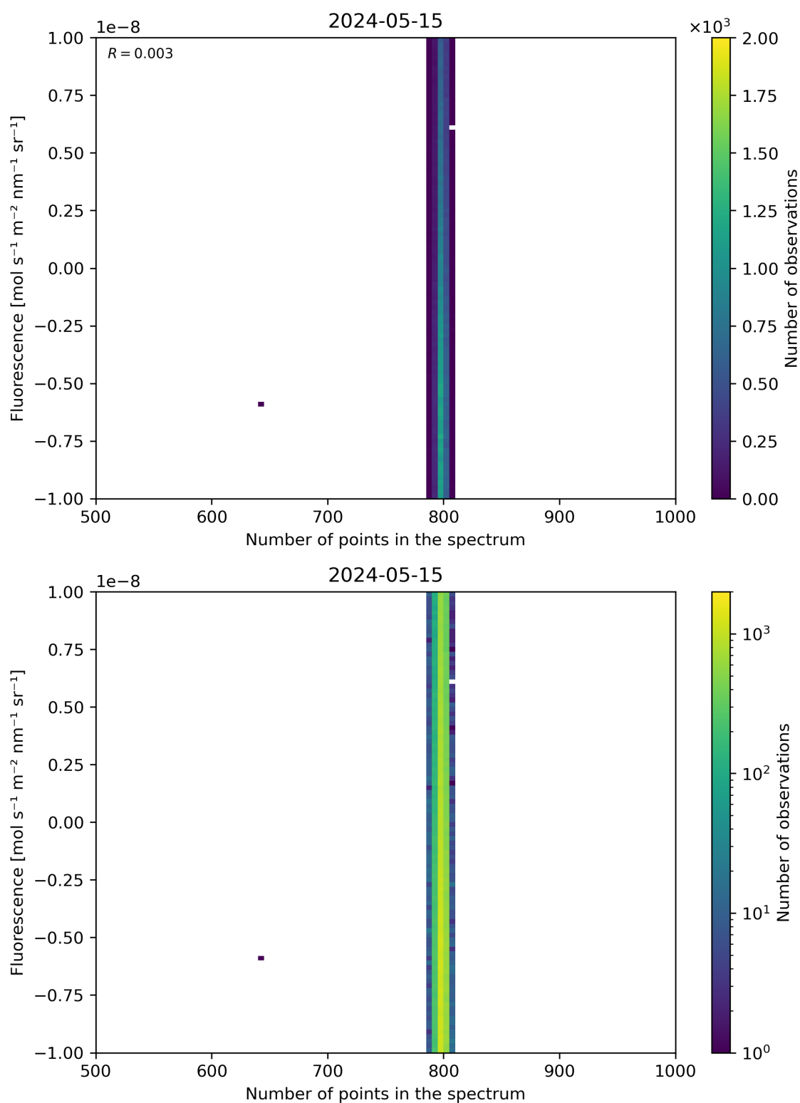
Figure 91: Scatter density plot of “Number of points in the spectrum” against “Fluorescence” for 2024-05-14 to 2024-05-16.
