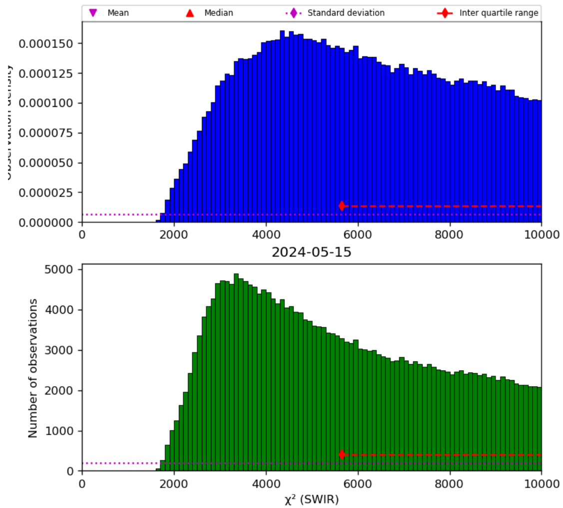
Figure 28: Histogram of “ \chi^2 (SWIR)” for 2024-05-14 to 2024-05-16
