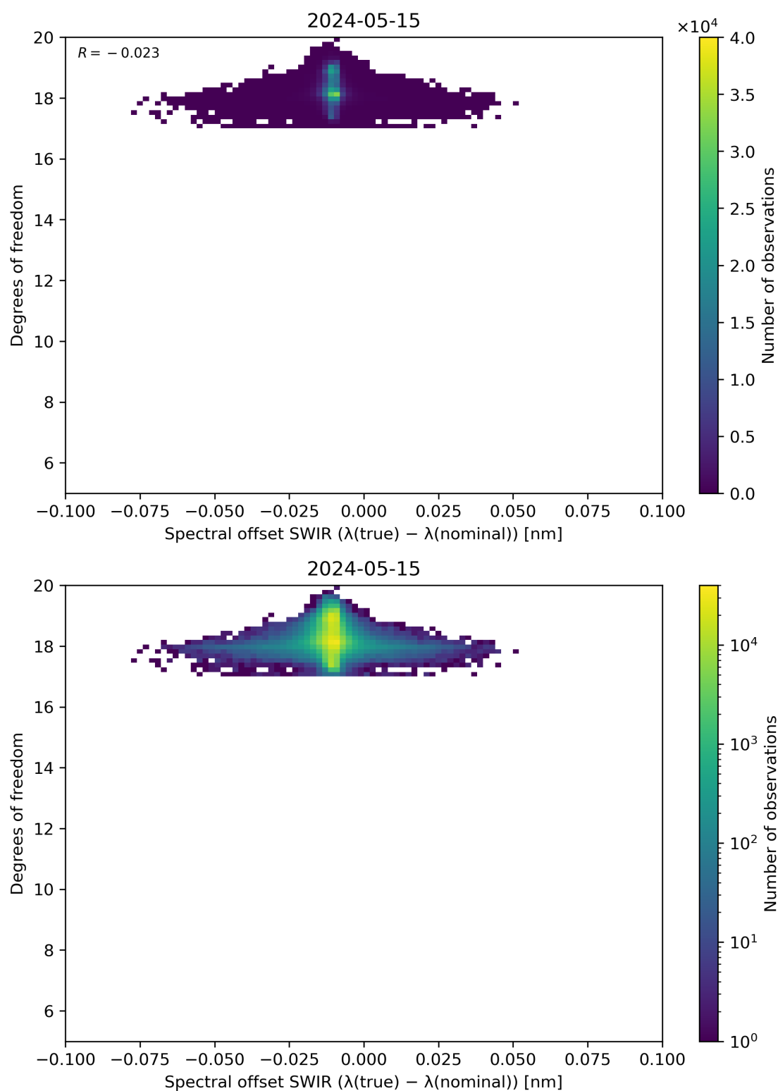
Figure 119: Scatter density plot of “Spectral offset SWIR ( \lambda(\text{true}) - \lambda(\text{nominal}) )” against “Degrees of freedom” for 2024-05-14 to 2024-05-16.
