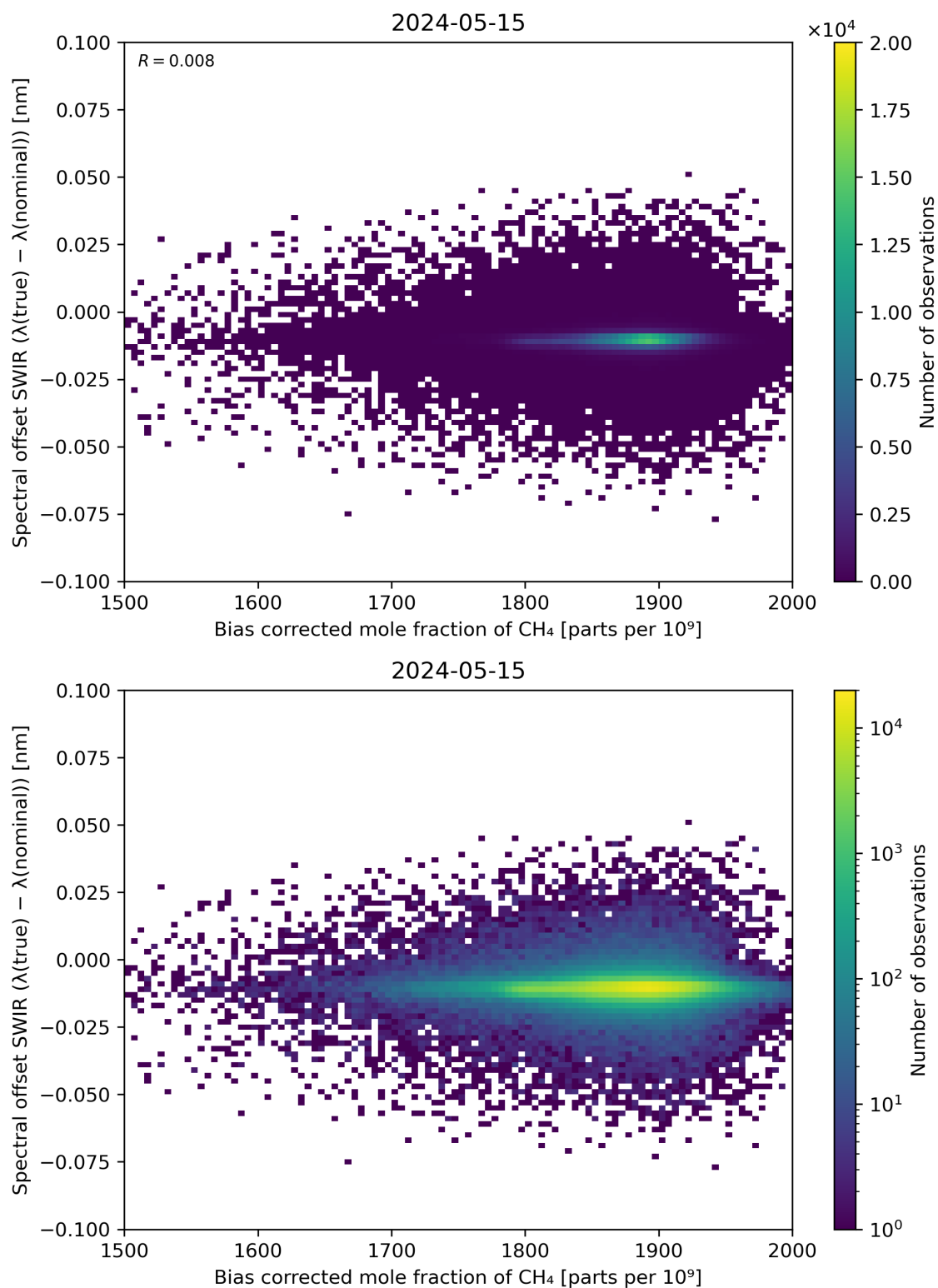
Figure 69: Scatter density plot of “Bias corrected mole fraction of \text{CH}_4 ” against “Spectral offset SWIR ( \lambda(\text{true}) - \lambda(\text{nominal}) )” for 2024-05-14 to 2024-05-16.
