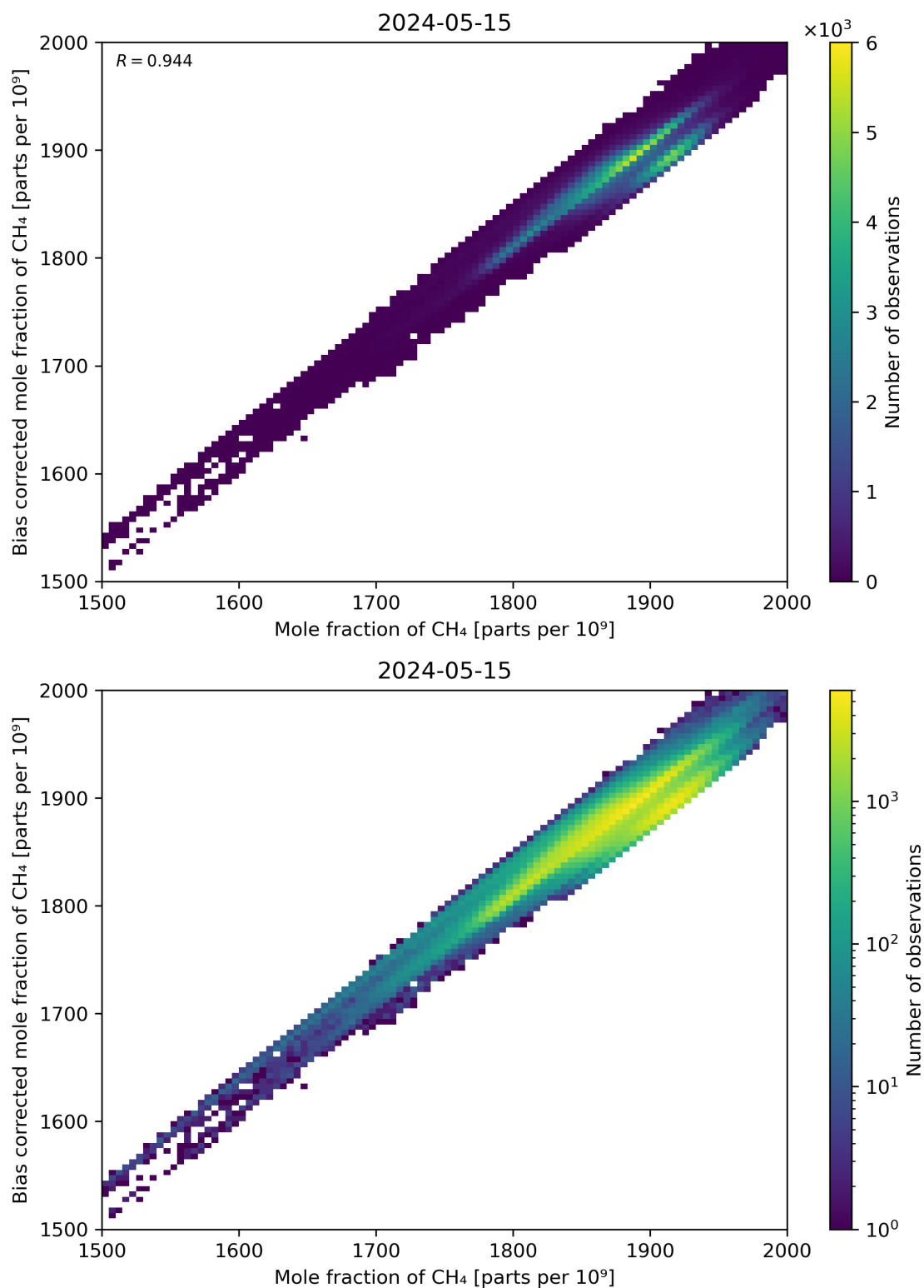
Figure 74: Scatter density plot of “Mole fraction of CH 4 ” against “Bias corrected mole fraction of CH 4 ” for 2024-05-14 to 2024-05-16.
