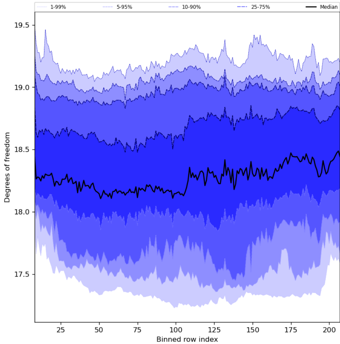
Figure 41: Along track statistics of “Degrees of freedom” for 2024-05-14 to 2024-05-16
