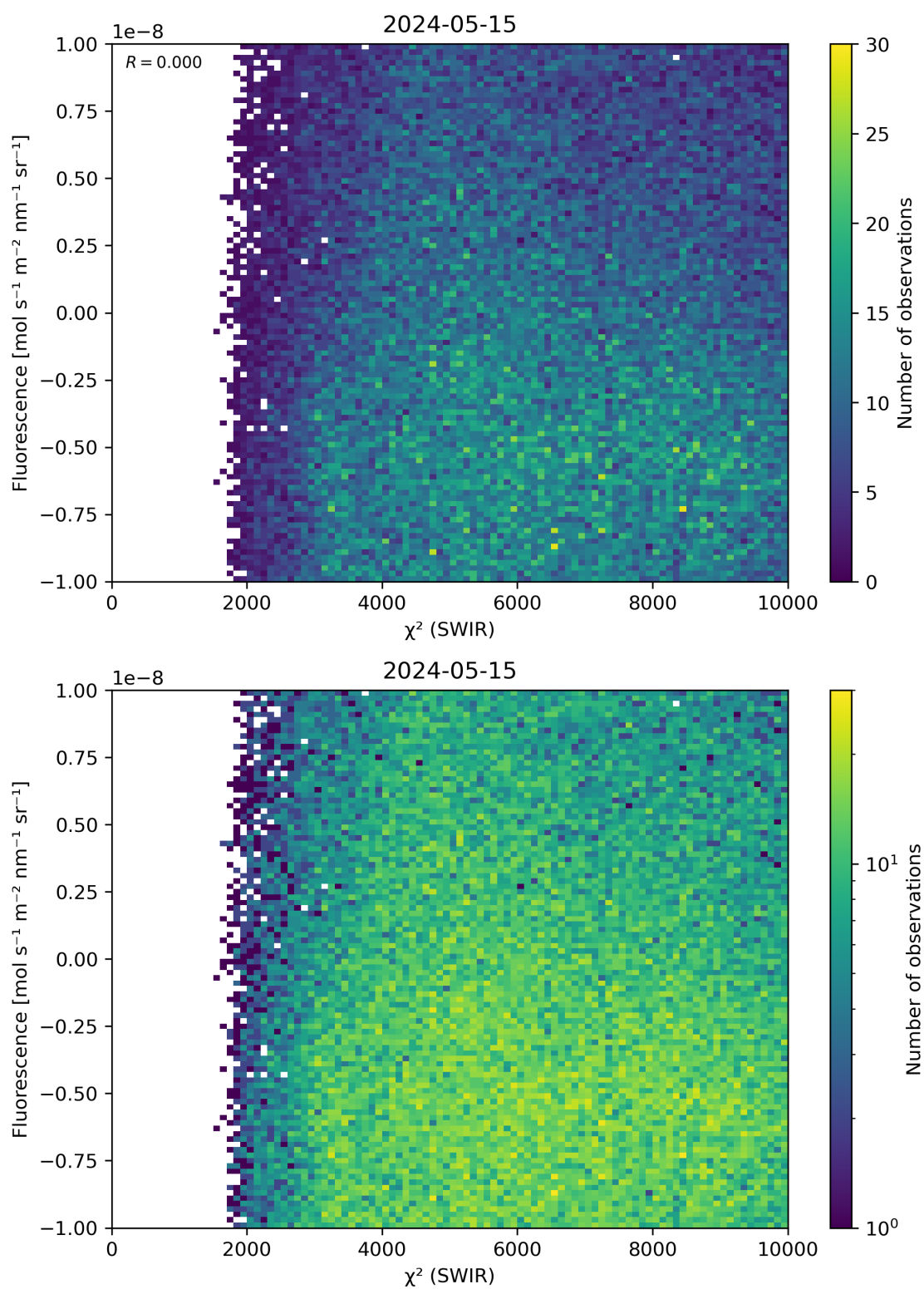
Figure 49: Scatter density plot of “ \chi^2 (SWIR)” against “Fluorescence” for 2024-05-14 to 2024-05-16.
