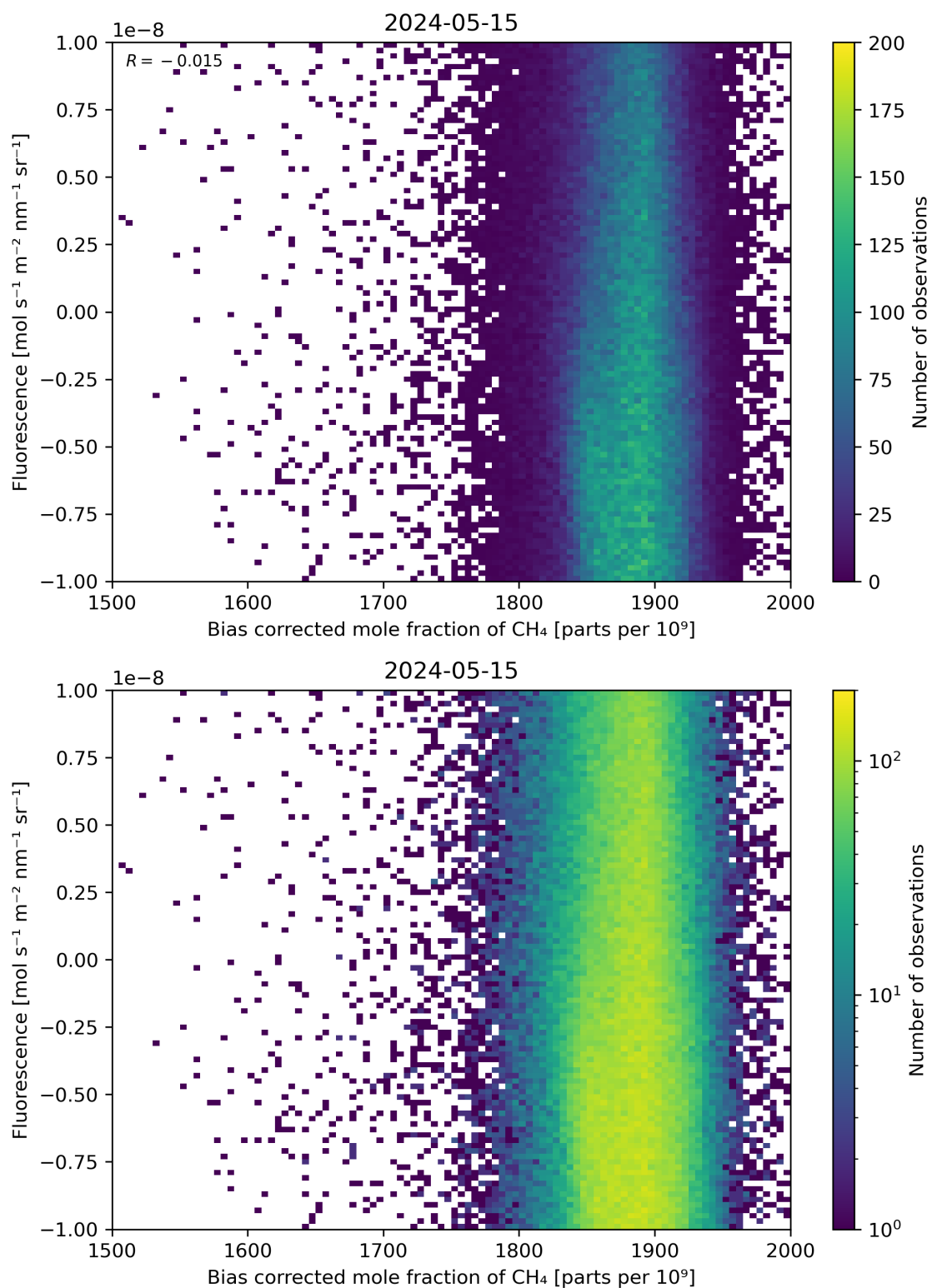
Figure 66: Scatter density plot of “Bias corrected mole fraction of \text{CH}_4 ” against “Fluorescence” for 2024-05-14 to 2024-05-16.
