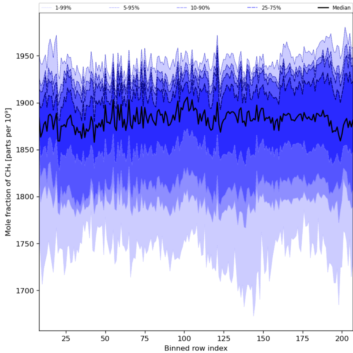
Figure 34: Along track statistics of “Mole fraction of CH 4 ” for 2024-05-14 to 2024-05-16
