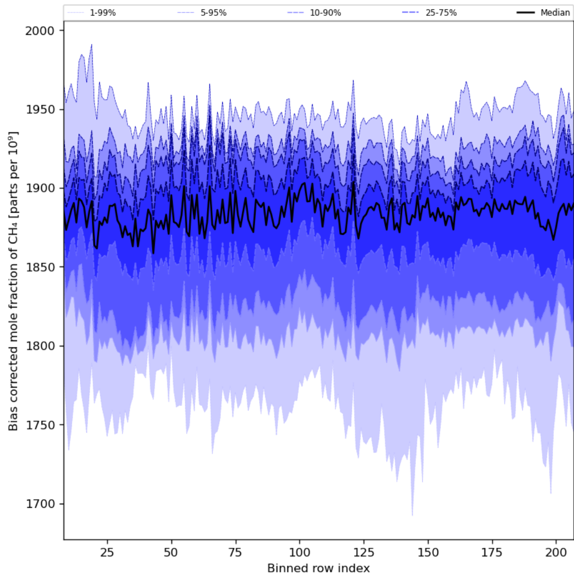
Figure 36: Along track statistics of “Bias corrected mole fraction of CH 4 ” for 2024-05-14 to 2024-05-16
