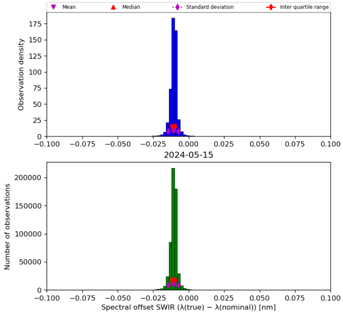
Figure 27: Histogram of “Spectral offset SWIR ( \lambda(\text{true}) - \lambda(\text{nominal}) )” for 2024-05-14 to 2024-05-16
