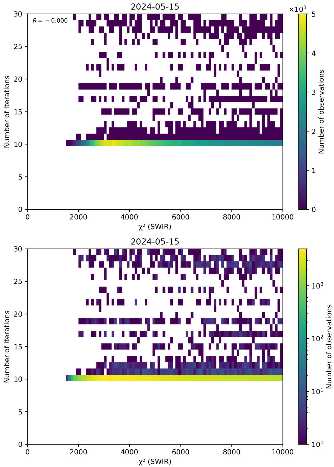
Figure 50: Scatter density plot of “ \chi^2 (SWIR)” against “Number of iterations” for 2024-05-14 to 2024-05-16.
