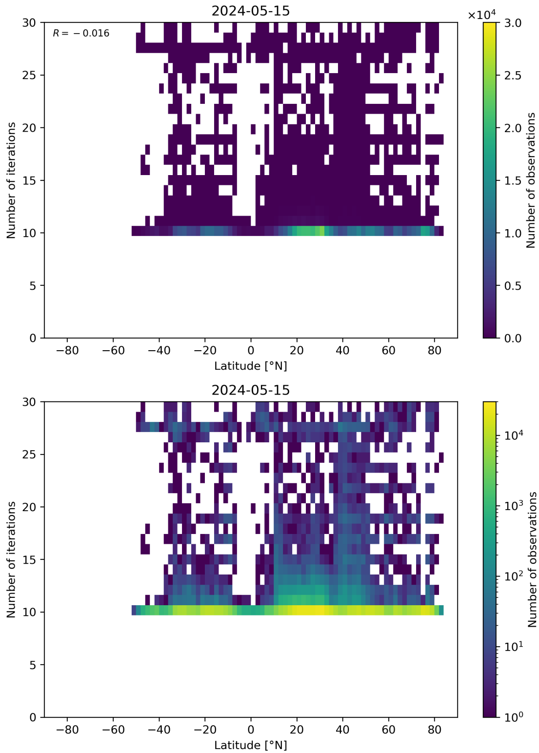
Figure 60: Scatter density plot of “Latitude” against “Number of iterations” for 2024-05-14 to 2024-05-16.
