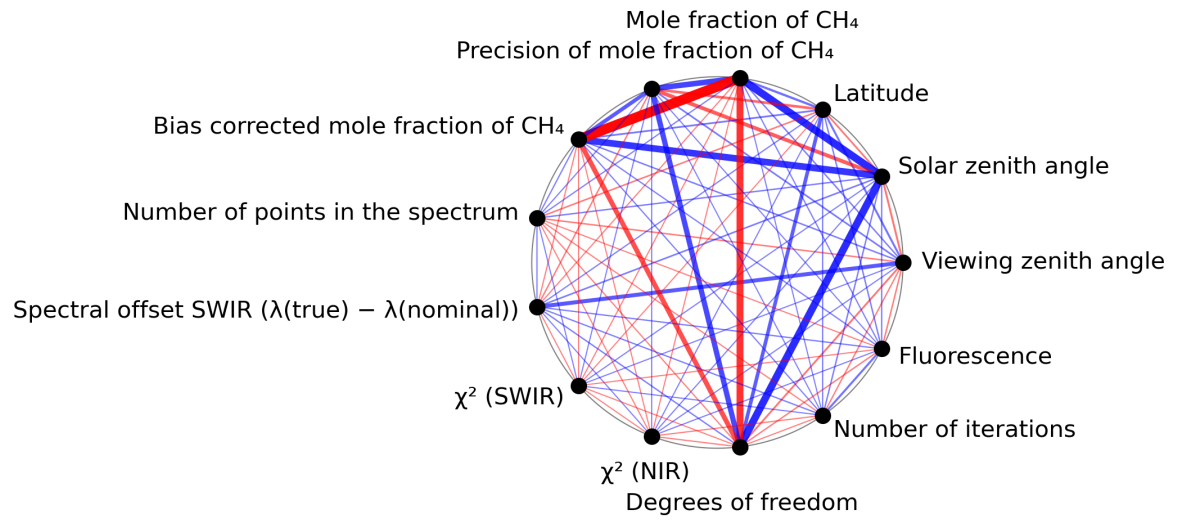
Figure 1: Map of correlation graph for 2024-05-14 to 2024-05-16.
