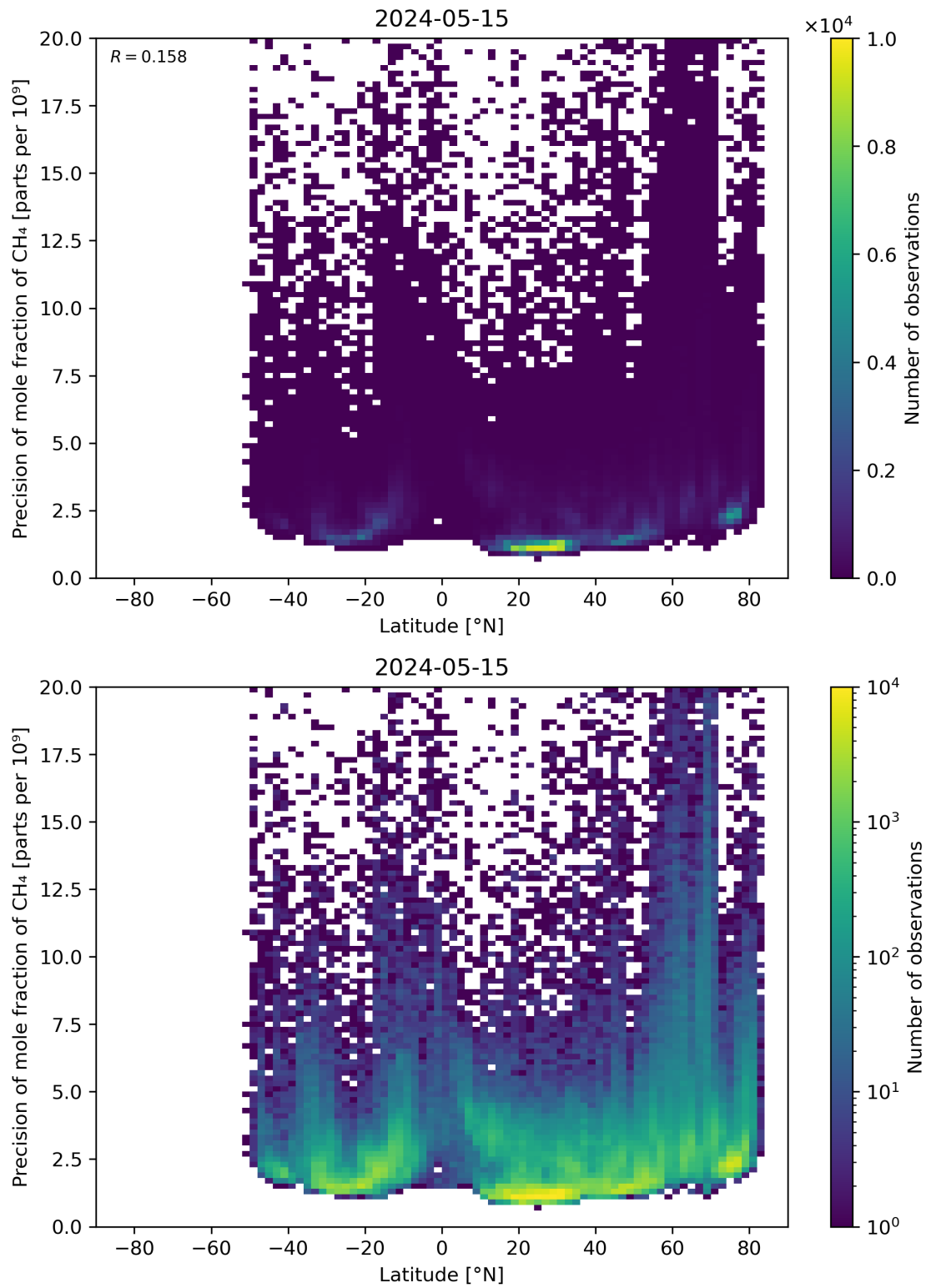
Figure 59: Scatter density plot of “Latitude” against “Precision of mole fraction of \text{CH}_4 ” for 2024-05-14 to 2024-05-16.
