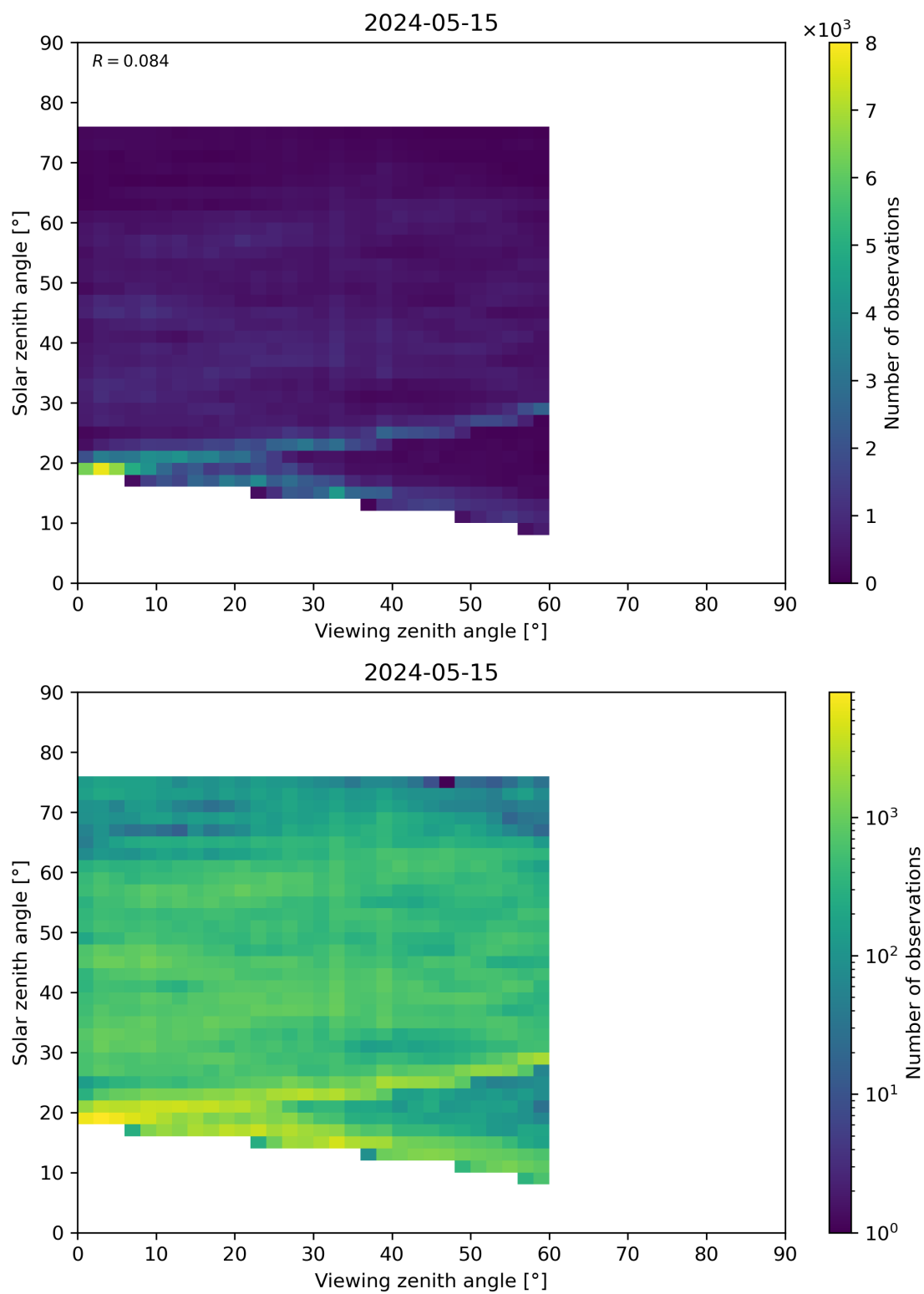
Figure 115: Scatter density plot of “Viewing zenith angle” against “Solar zenith angle” for 2024-05-14 to 2024-05-16.
