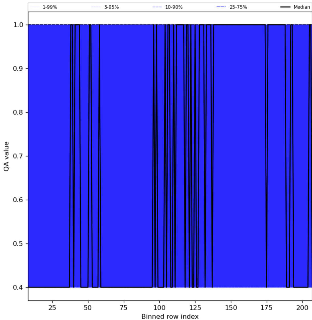
Figure 33: Along track statistics of “QA value” for 2024-05-14 to 2024-05-16
