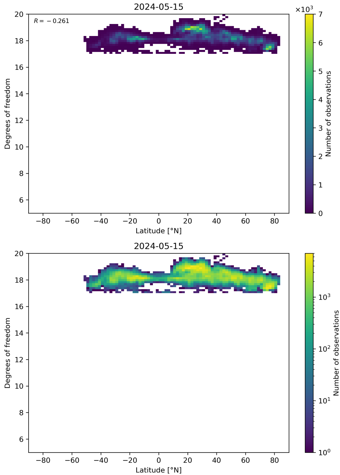
Figure 55: Scatter density plot of “Latitude” against “Degrees of freedom” for 2024-05-14 to 2024-05-16.
