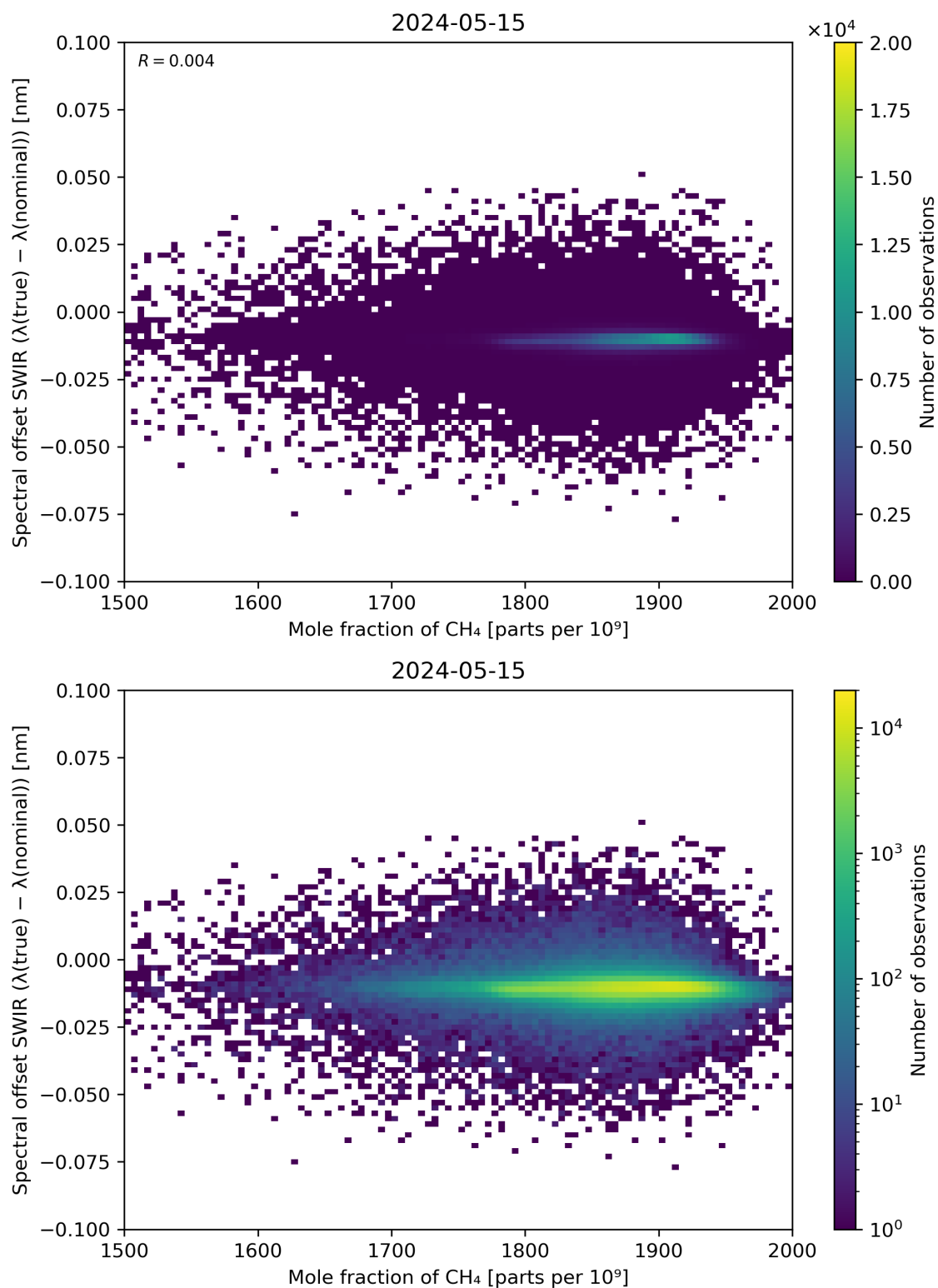
Figure 86: Scatter density plot of “Mole fraction of CH 4 ” against “Spectral offset SWIR ( \lambda(\text{true}) - \lambda(\text{nominal}) )” for 2024-05-14 to 2024-05-16.
