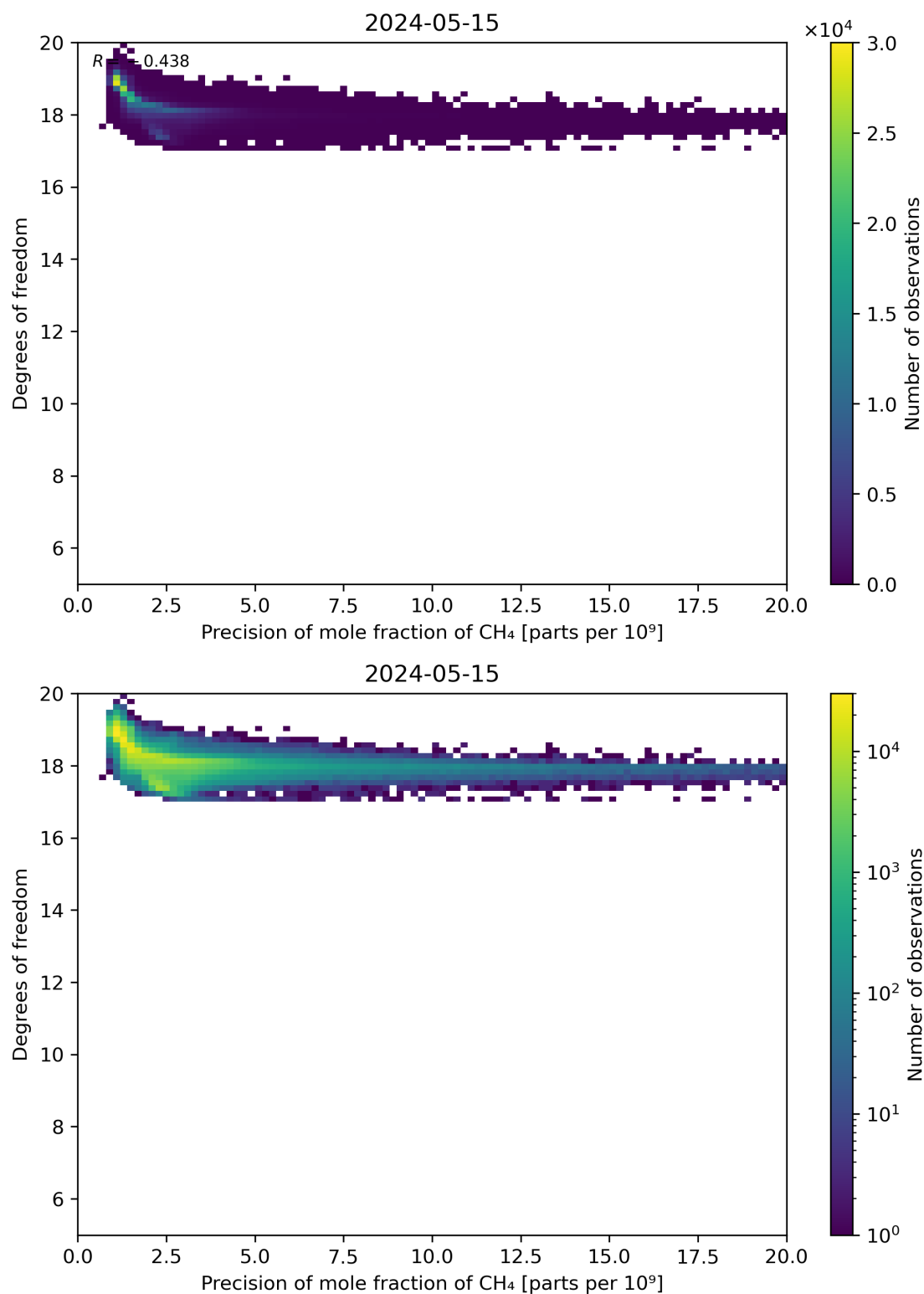
Figure 80: Scatter density plot of “Precision of mole fraction of CH 4 ” against “Degrees of freedom” for 2024-05-14 to 2024-05-16.
