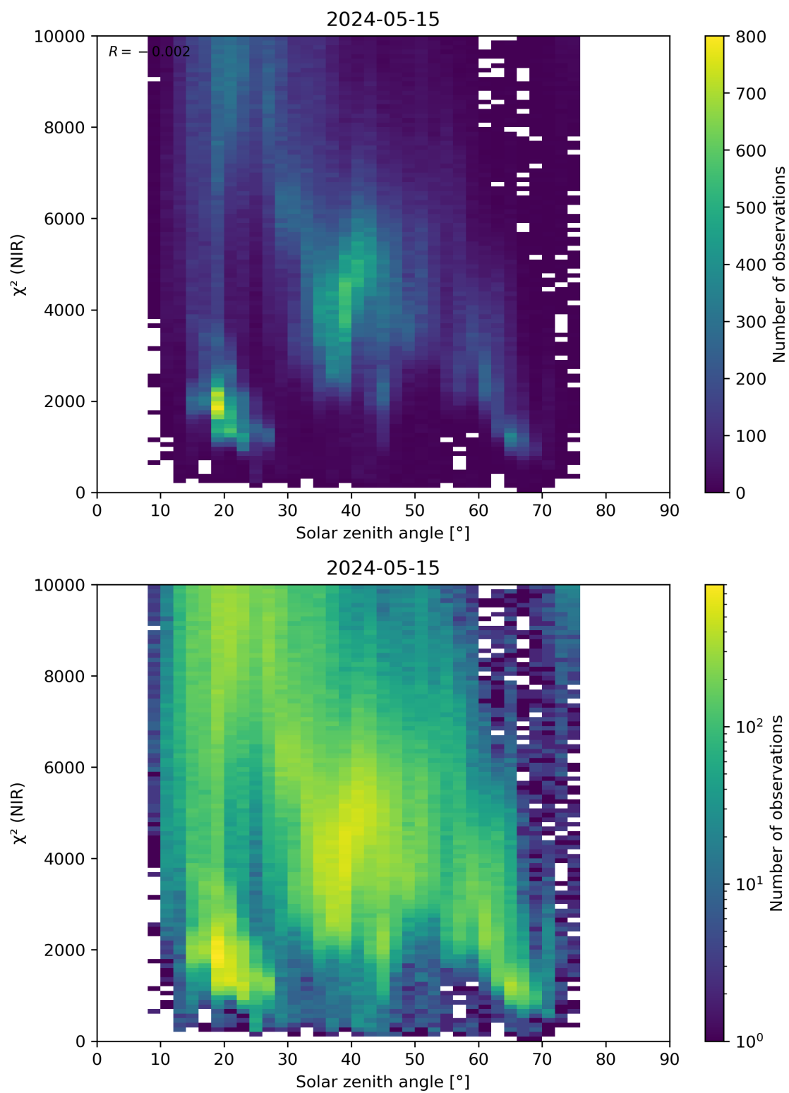
Figure 94: Scatter density plot of “Solar zenith angle” against “ \chi^2 (NIR)” for 2024-05-14 to 2024-05-16.
