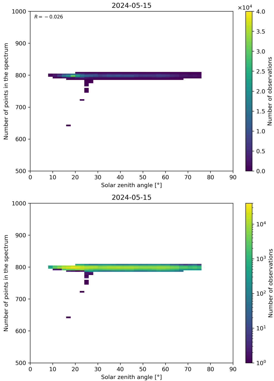
Figure 103: Scatter density plot of “Solar zenith angle” against “Number of points in the spectrum” for 2024-05-14 to 2024-05-16.
