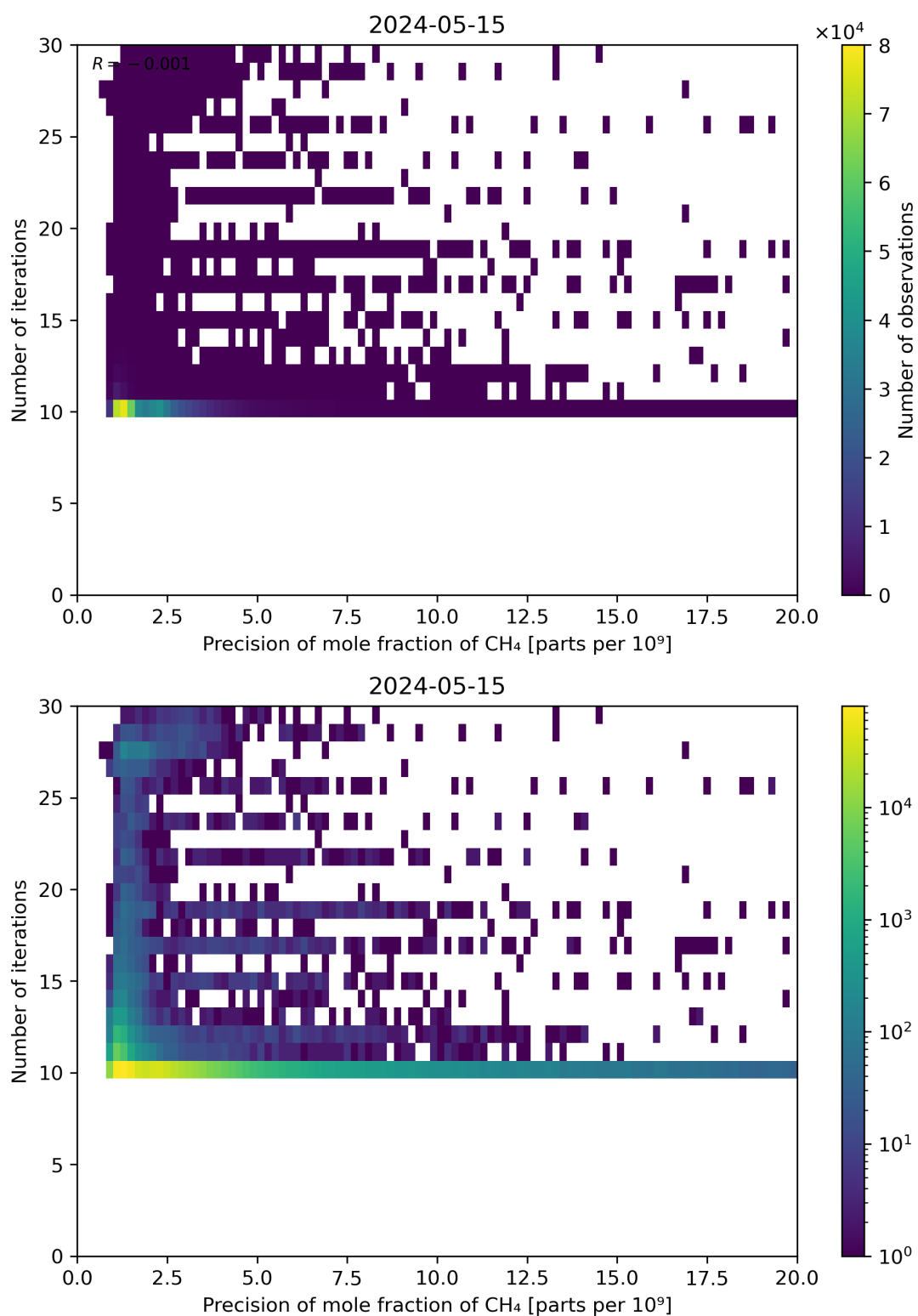
Figure 83: Scatter density plot of “Precision of mole fraction of CH 4 ” against “Number of iterations” for 2024-05-14 to 2024-05-16.
