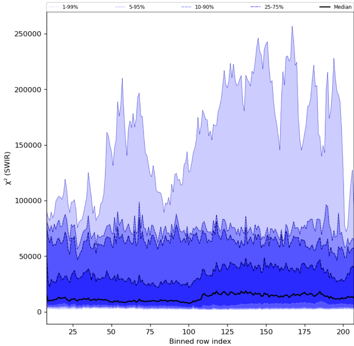
Figure 39: Along track statistics of “ \chi^2 (SWIR)” for 2024-05-14 to 2024-05-16
