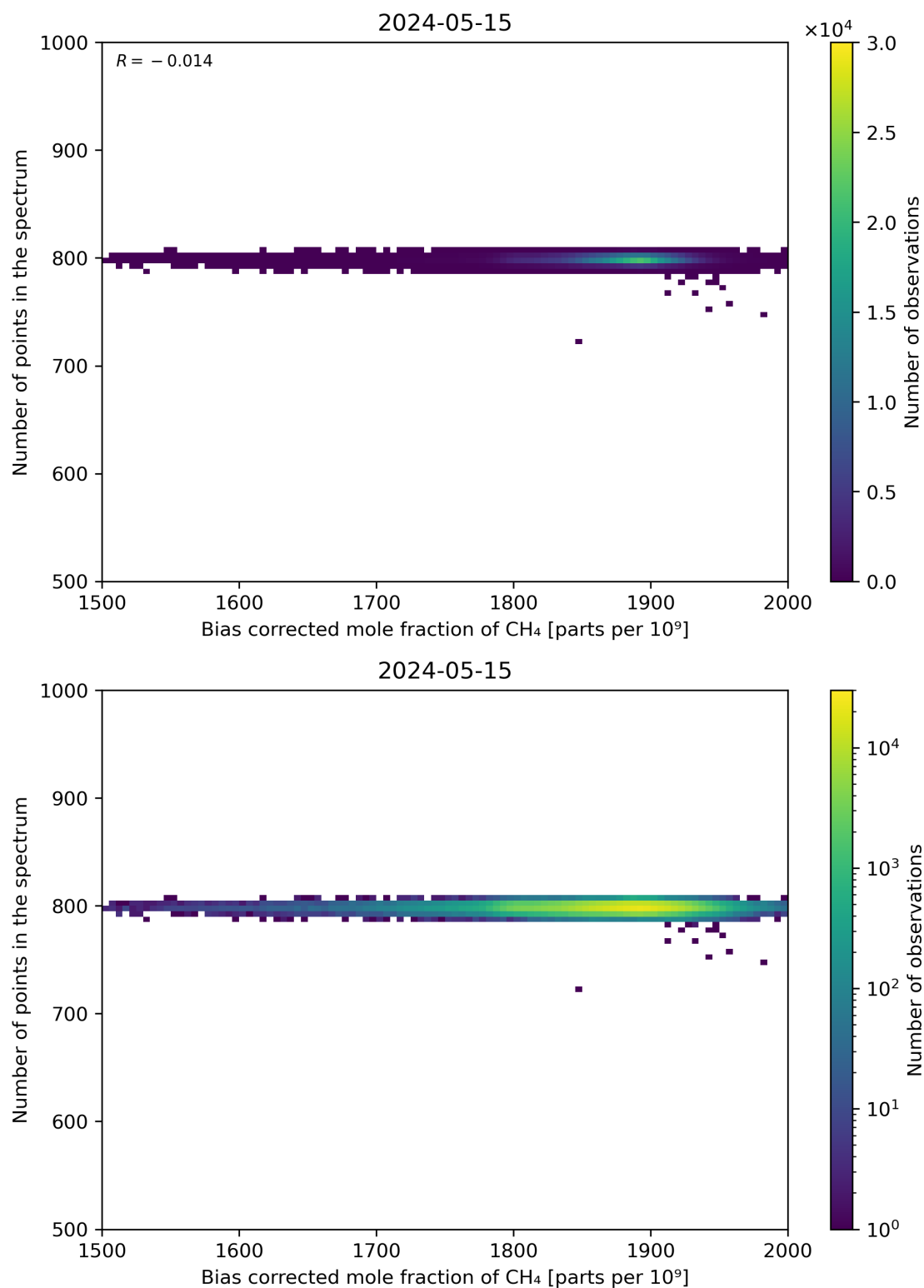
Figure 68: Scatter density plot of “Bias corrected mole fraction of CH 4 ” against “Number of points in the spectrum” for 2024-05-14 to 2024-05-16.
