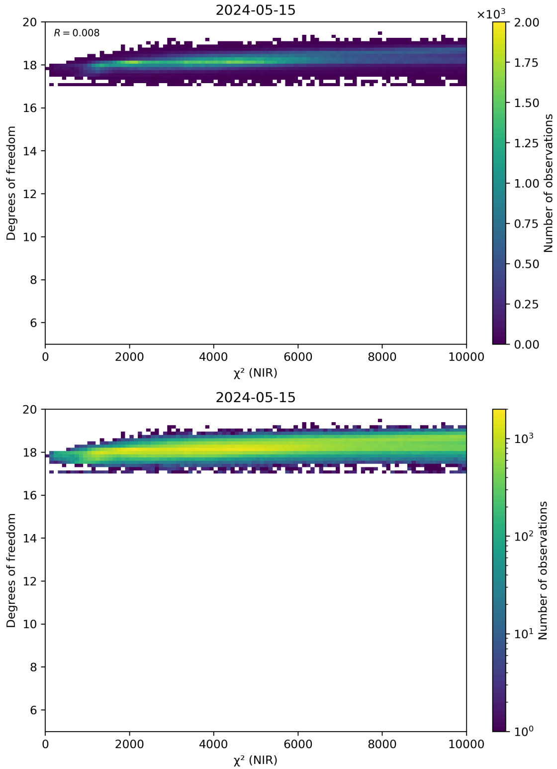
Figure 44: Scatter density plot of “ \chi^2 (NIR)” against “Degrees of freedom” for 2024-05-14 to 2024-05-16.
