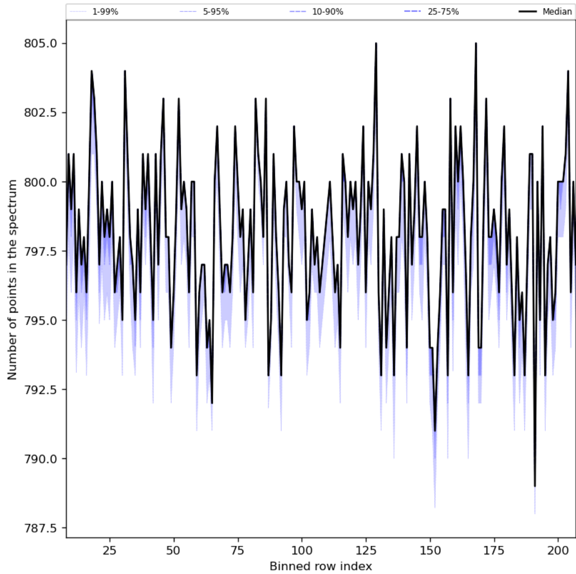
Figure 37: Along track statistics of “Number of points in the spectrum” for 2024-05-14 to 2024-05-16
