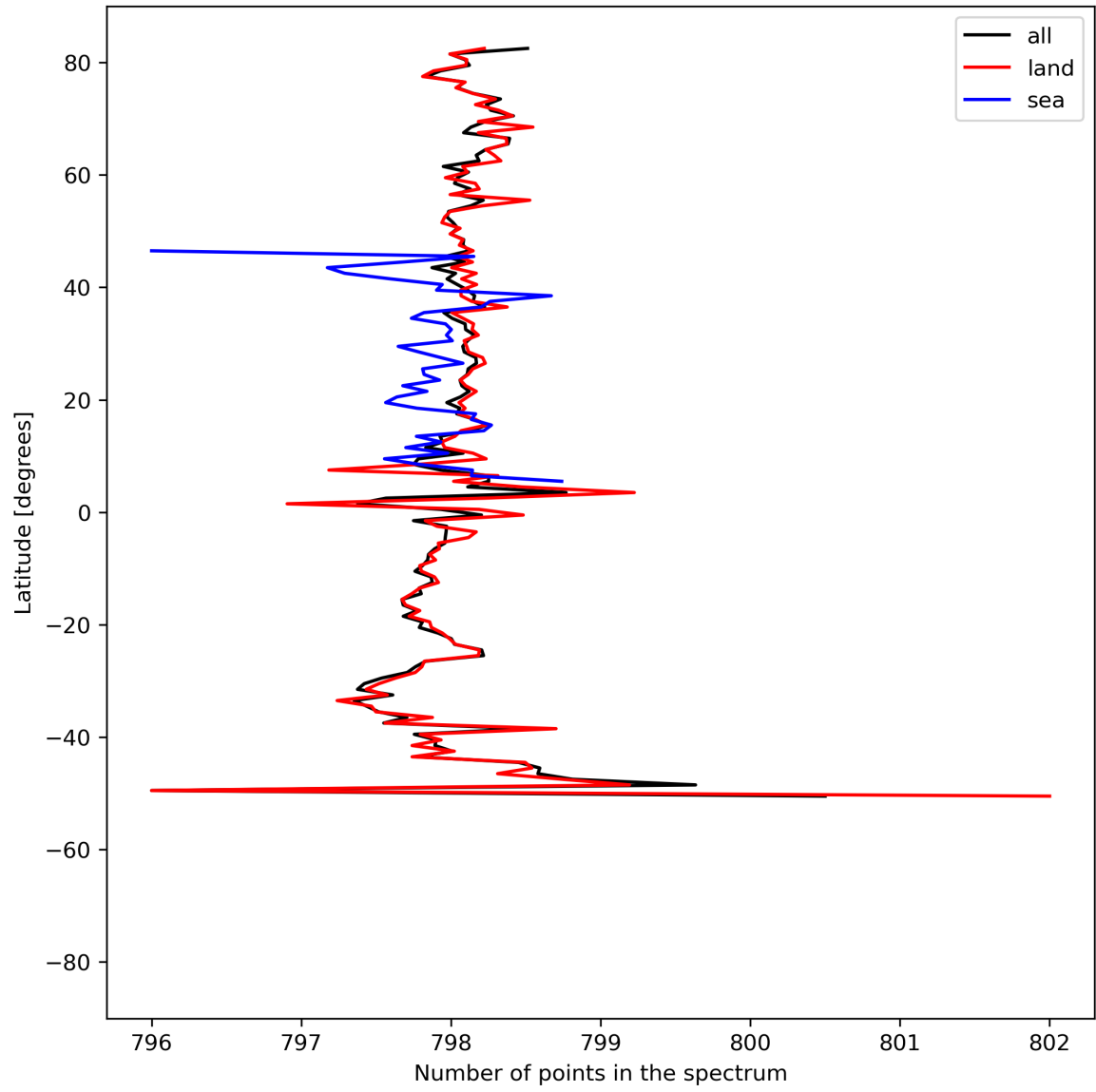
Figure 15: Zonal average of “Number of points in the spectrum” for 2024-05-14 to 2024-05-16.
