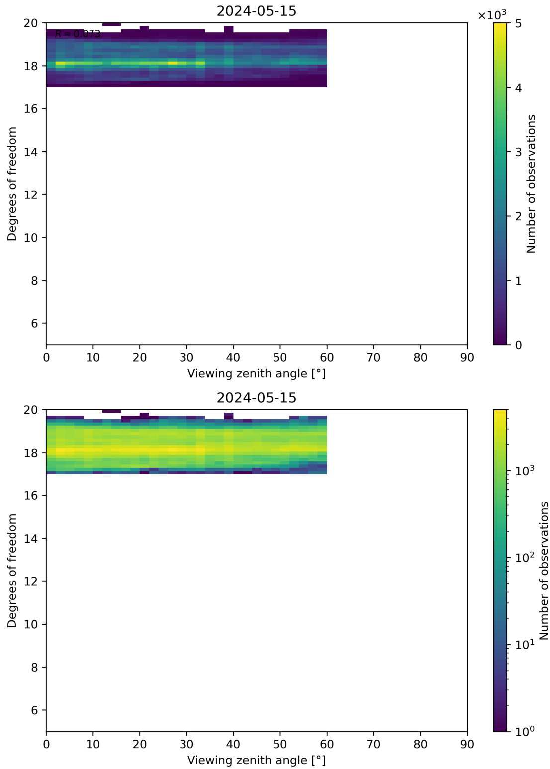
Figure 107: Scatter density plot of “Viewing zenith angle” against “Degrees of freedom” for 2024-05-14 to 2024-05-16.
