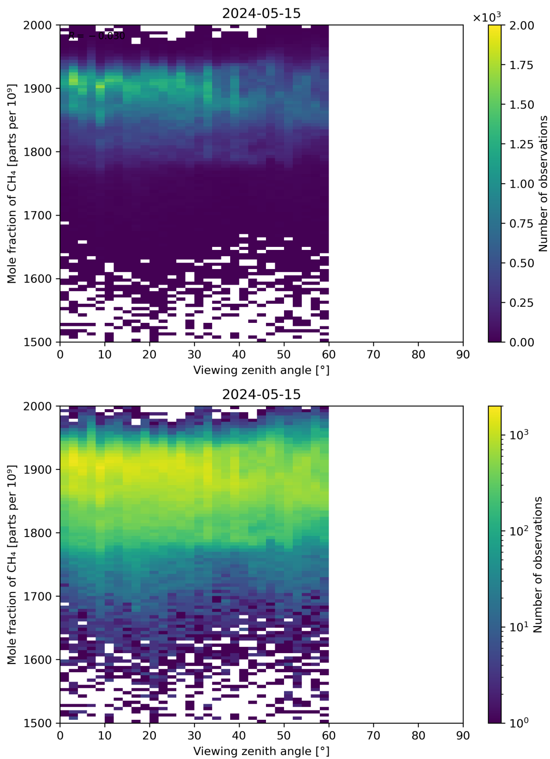
Figure 110: Scatter density plot of “Viewing zenith angle” against “Mole fraction of CH 4 ” for 2024-05-14 to 2024-05-16.
