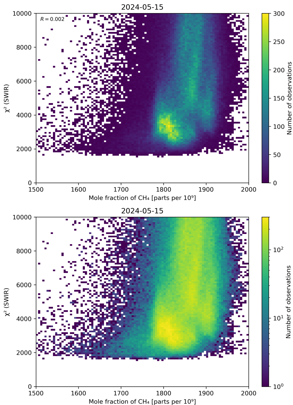
Figure 71: Scatter density plot of “Mole fraction of \text{CH}_4 ” against “ \chi^2 (SWIR)” for 2024-05-14 to 2024-05-16.
