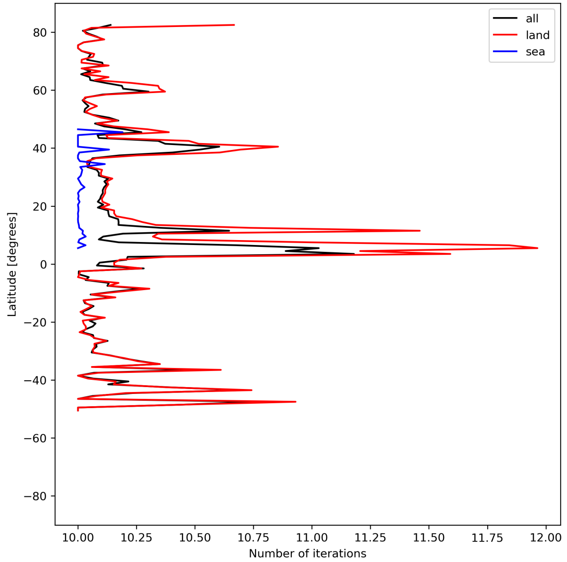
Figure 20: Zonal average of “Number of iterations” for 2024-05-14 to 2024-05-16.
