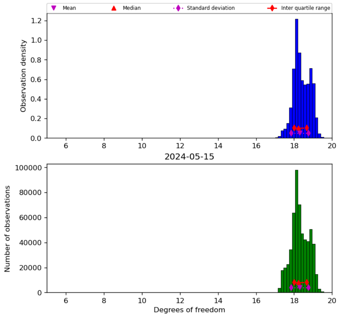
Figure 30: Histogram of “Degrees of freedom” for 2024-05-14 to 2024-05-16
