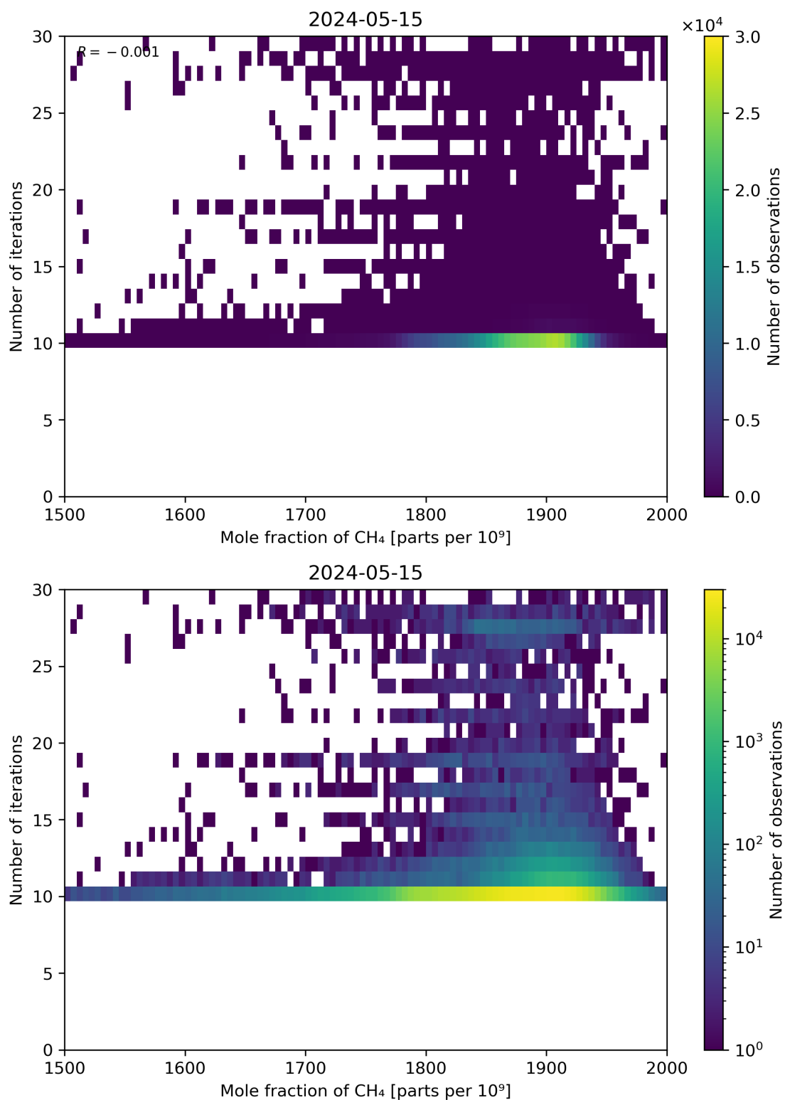
Figure 76: Scatter density plot of “Mole fraction of CH 4 ” against “Number of iterations” for 2024-05-14 to 2024-05-16.
