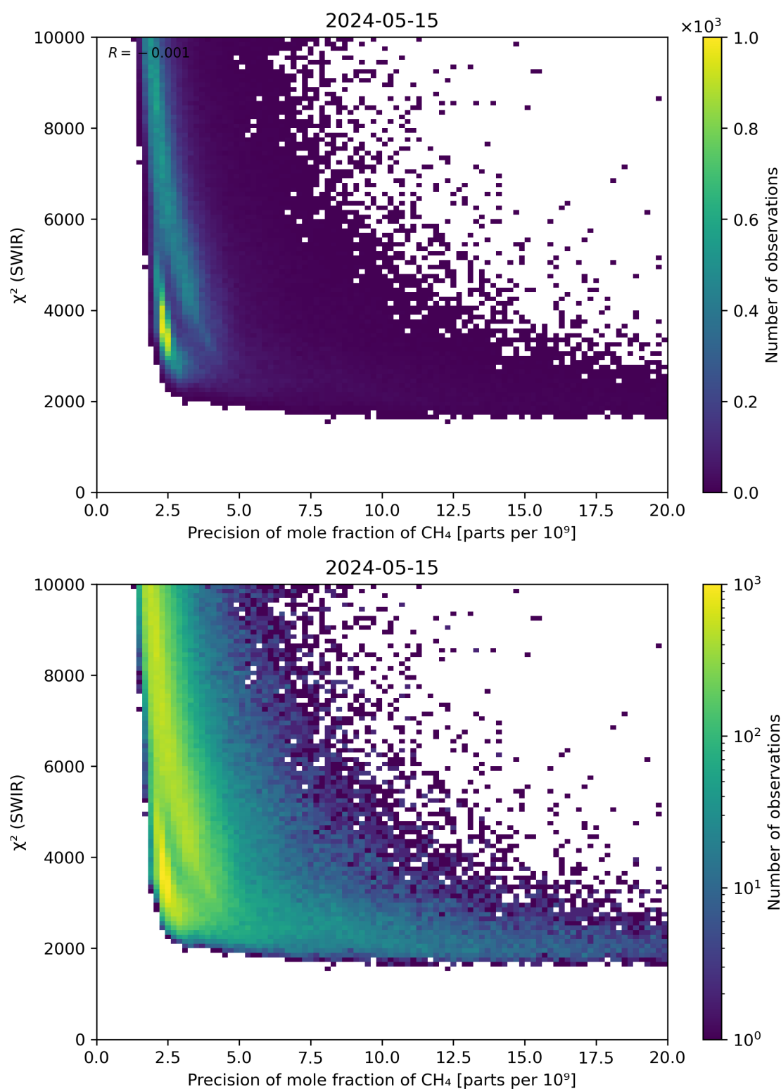
Figure 79: Scatter density plot of “Precision of mole fraction of CH 4 ” against “ \chi^2 (SWIR)” for 2024-05-14 to 2024-05-16.
