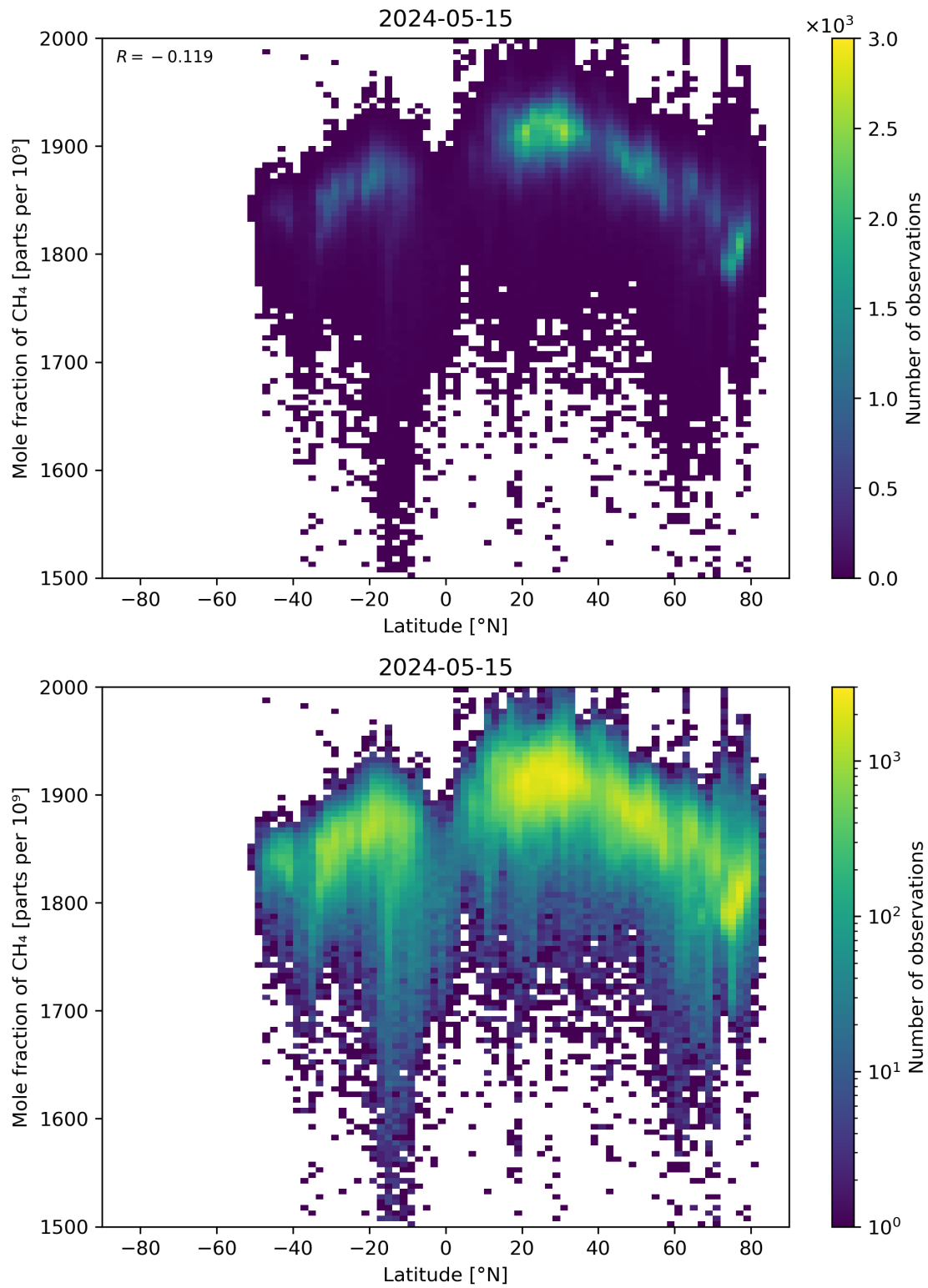
Figure 57: Scatter density plot of “Latitude” against “Mole fraction of CH 4 ” for 2024-05-14 to 2024-05-16.
