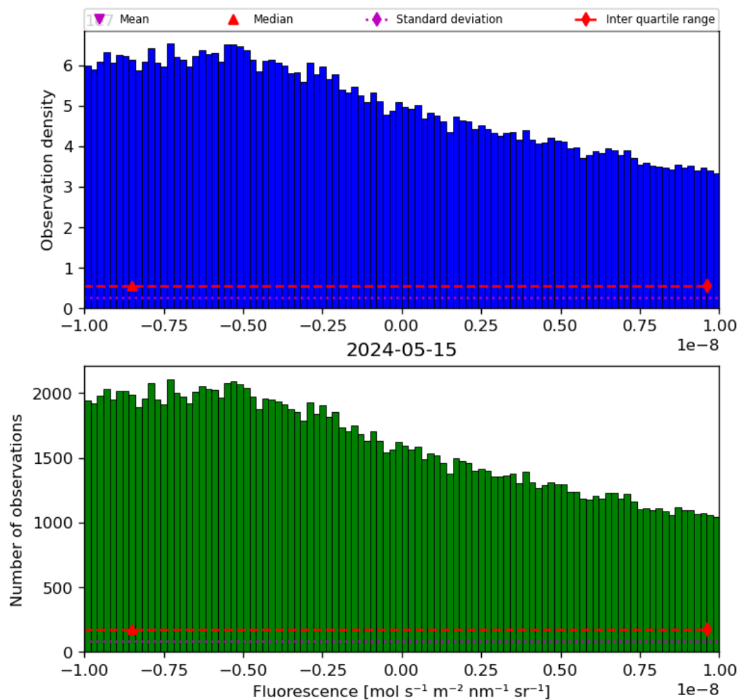
Figure 32: Histogram of “Fluorescence” for 2024-05-14 to 2024-05-16
