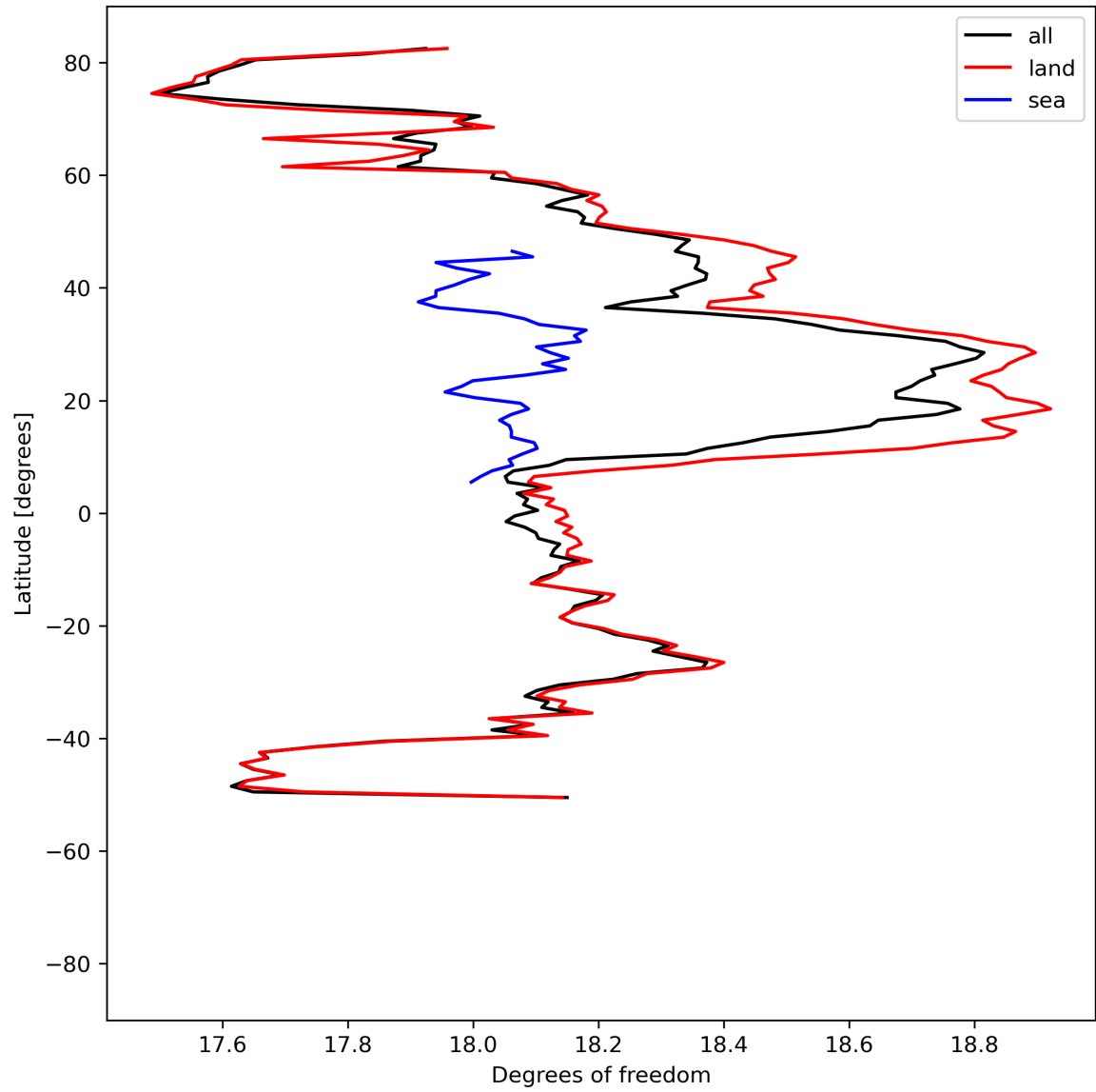
Figure 19: Zonal average of “Degrees of freedom” for 2024-05-14 to 2024-05-16.
