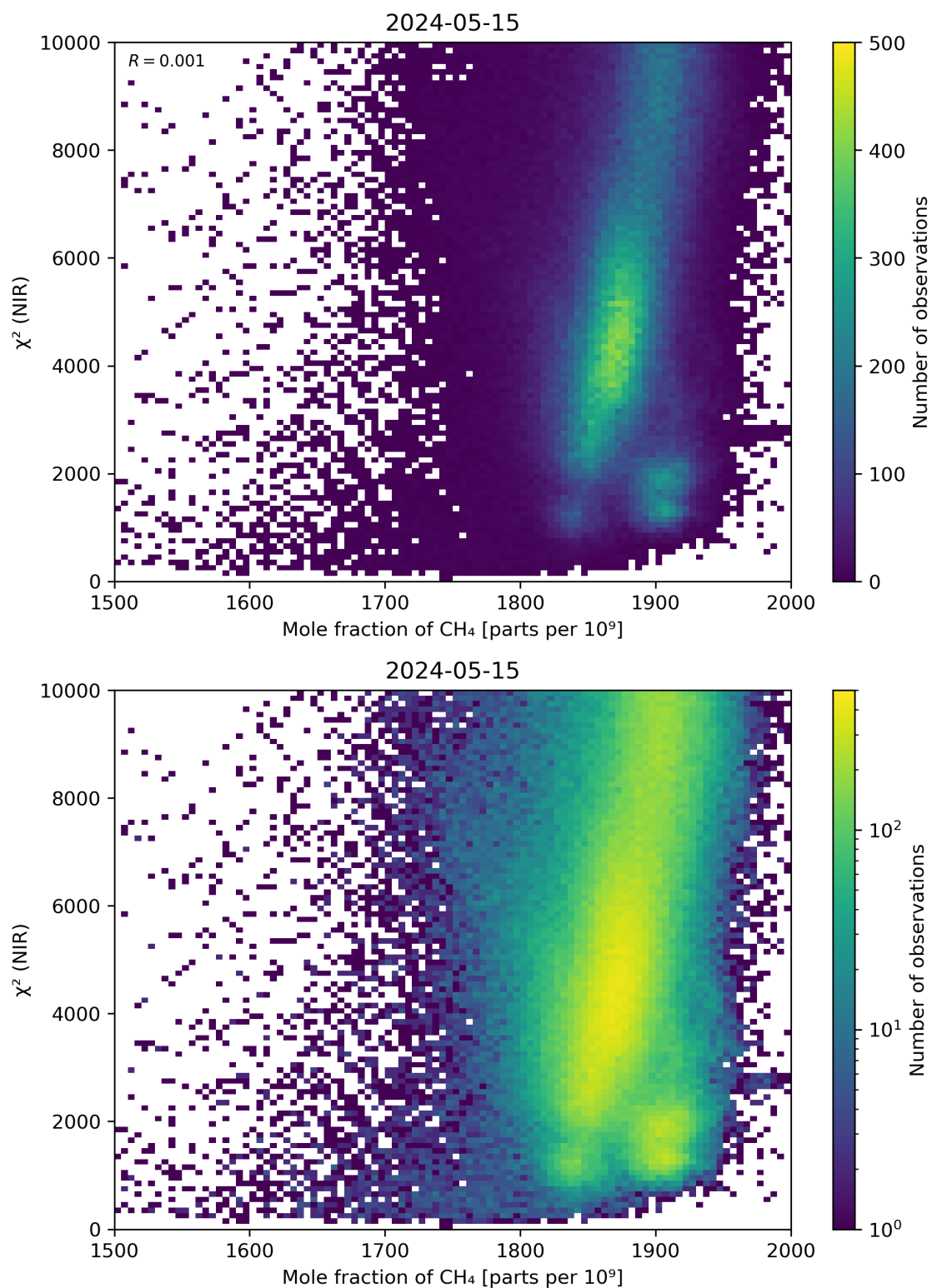
Figure 70: Scatter density plot of “Mole fraction of CH 4 ” against “ \chi^2 (NIR)” for 2024-05-14 to 2024-05-16.
