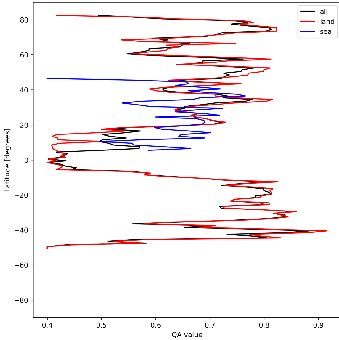
Figure 11: Zonal average of “QA value” for 2024-05-14 to 2024-05-16.
