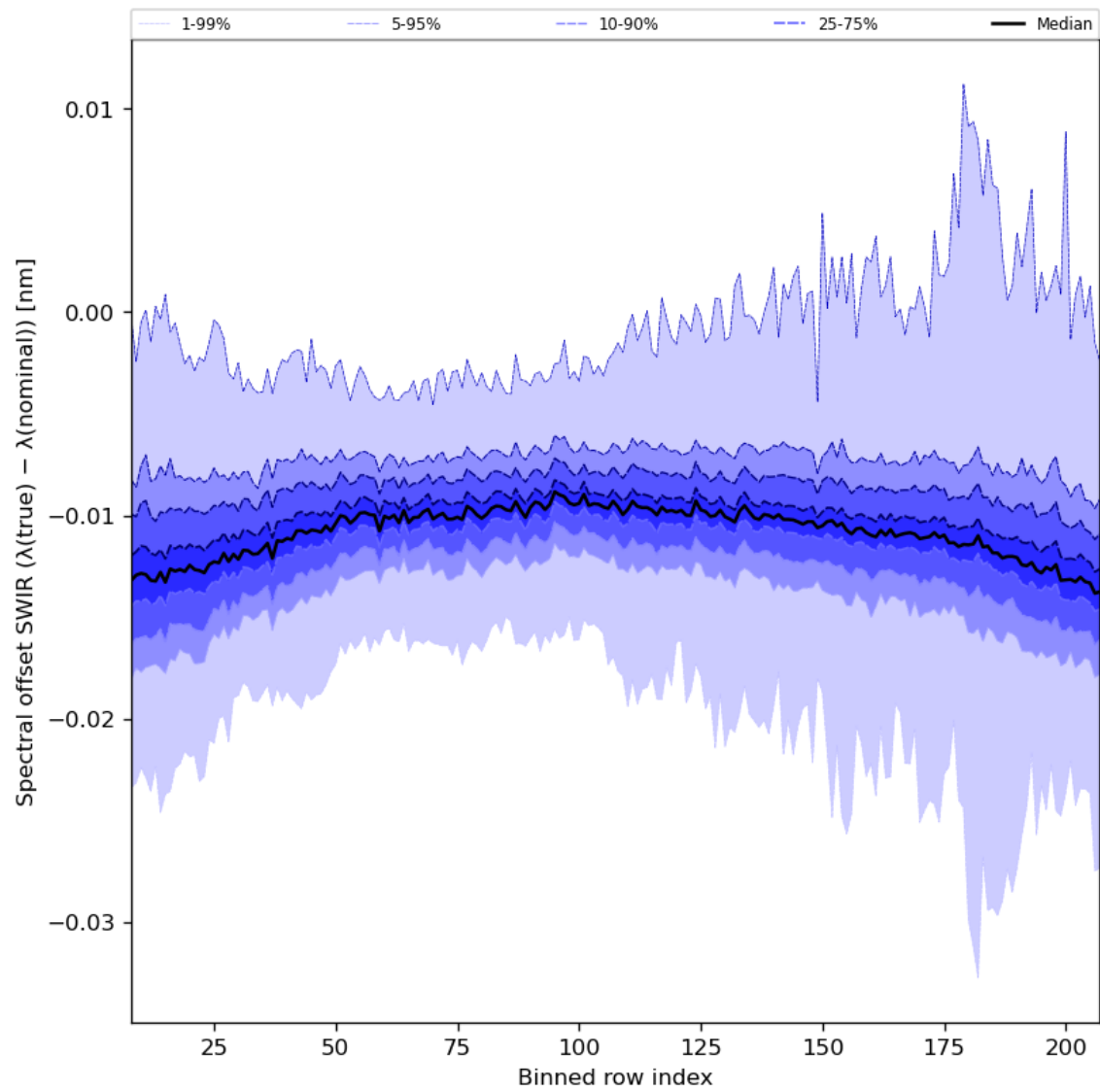
Figure 38: Along track statistics of “Spectral offset SWIR ( \lambda(\text{true}) - \lambda(\text{nominal}) )” for 2024-05-14 to 2024-05-16
