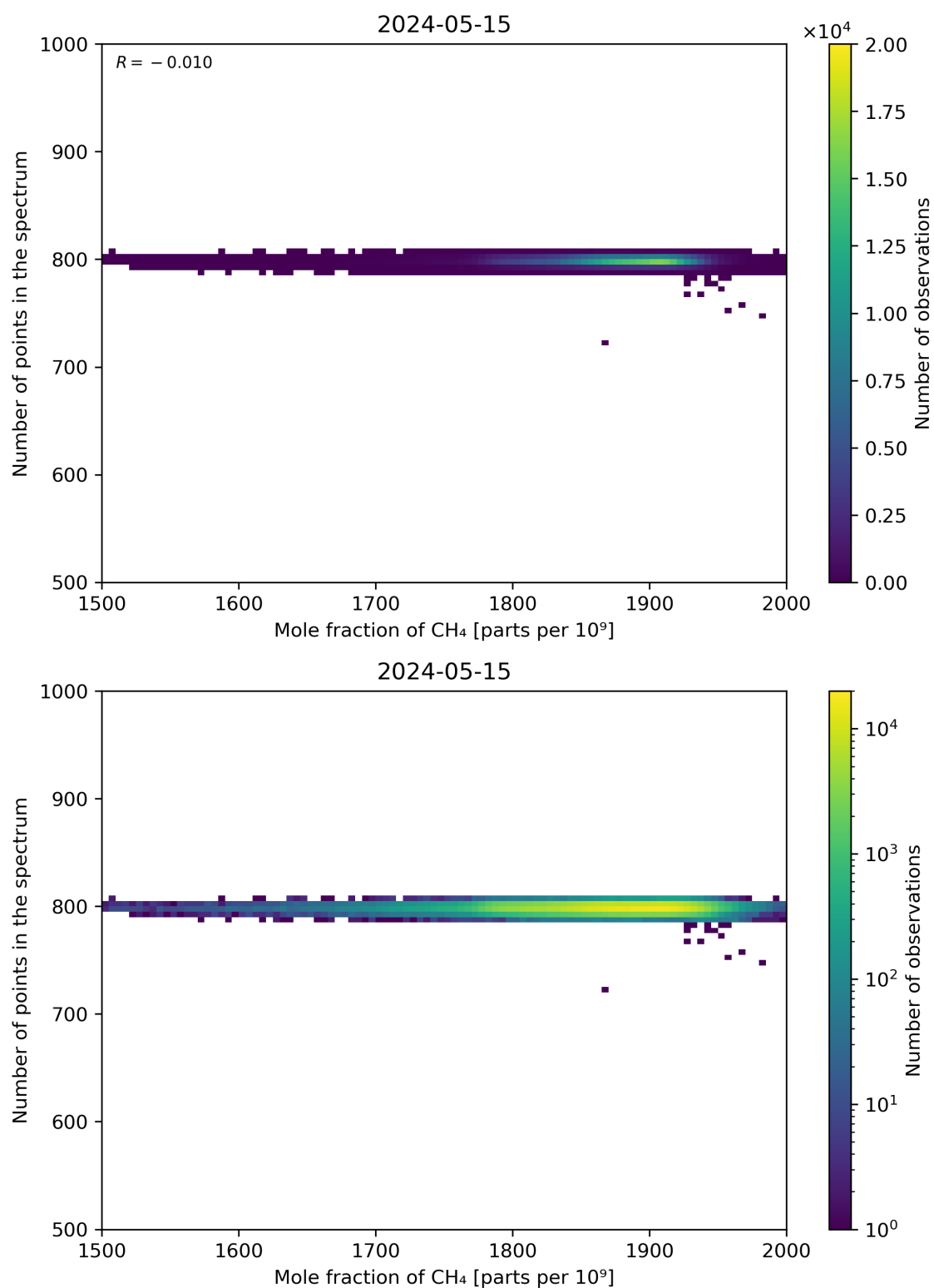
Figure 77: Scatter density plot of “Mole fraction of CH 4 ” against “Number of points in the spectrum” for 2024-05-14 to 2024-05-16.
