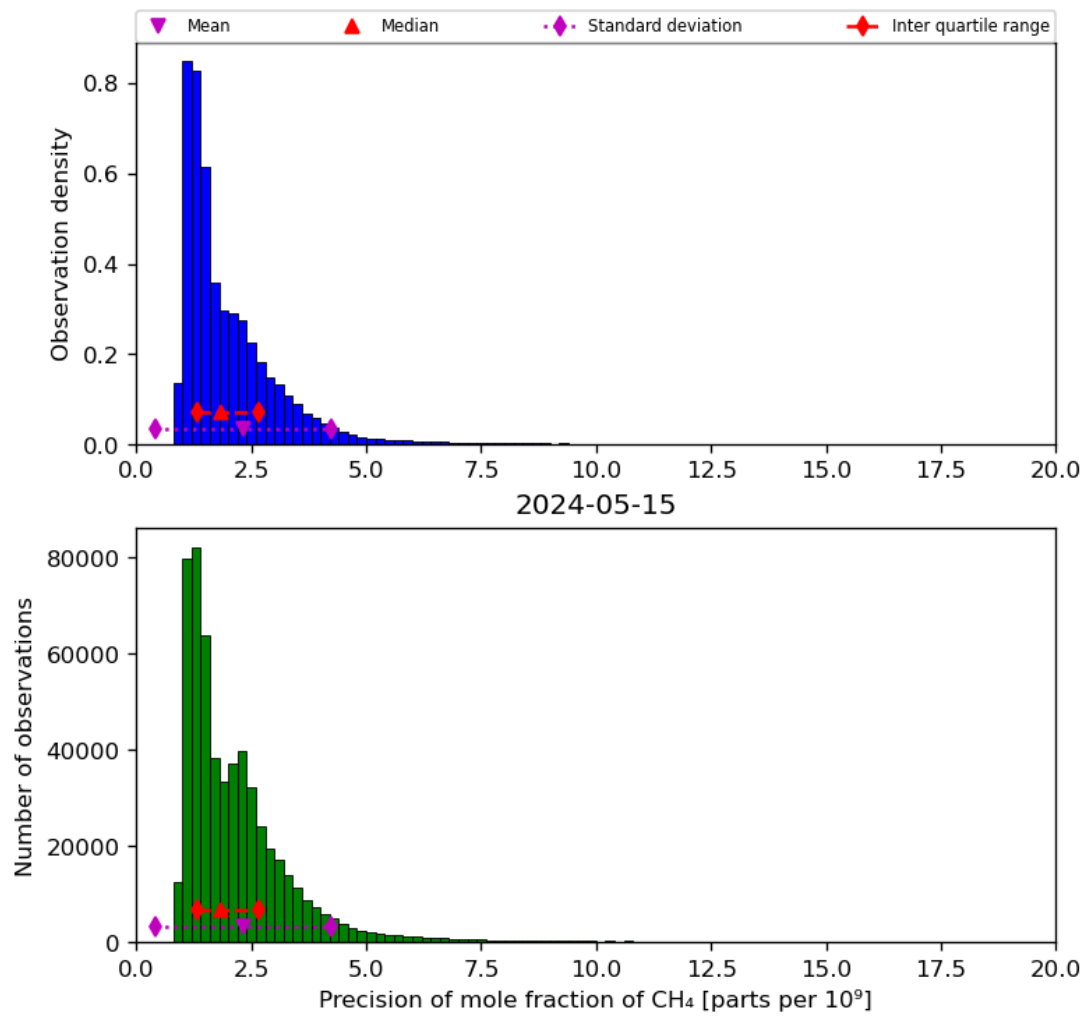
Figure 24: Histogram of “Precision of mole fraction of CH 4 ” for 2024-05-14 to 2024-05-16
