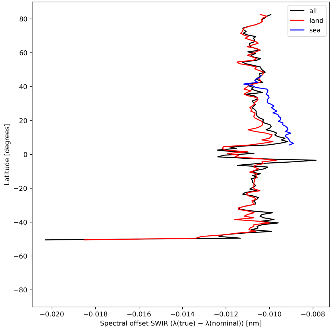
Figure 16: Zonal average of “Spectral offset SWIR ( \lambda(\text{true}) - \lambda(\text{nominal}) )” for 2024-05-14 to 2024-05-16.
