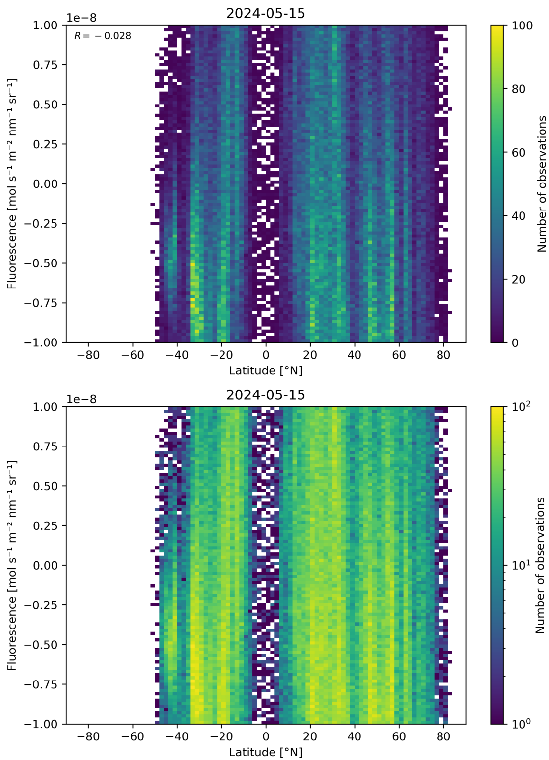
Figure 56: Scatter density plot of “Latitude” against “Fluorescence” for 2024-05-14 to 2024-05-16.
