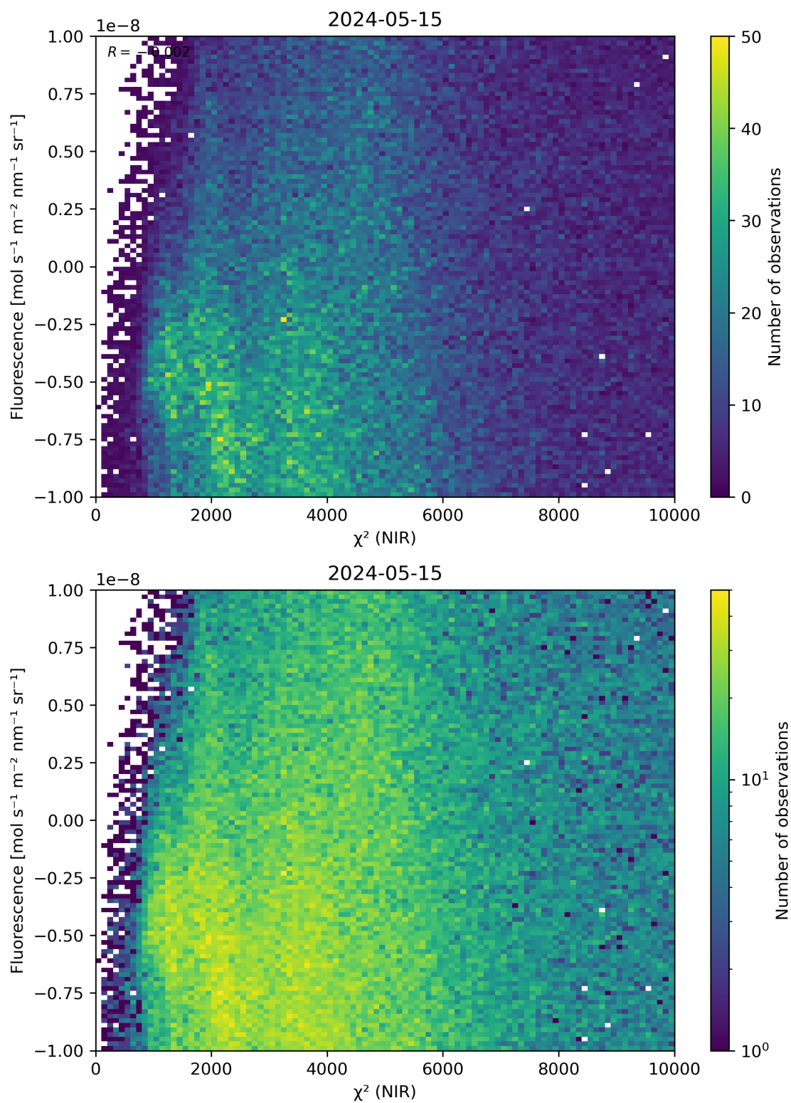
Figure 45: Scatter density plot of “ \chi^2 (NIR)” against “Fluorescence” for 2024-05-14 to 2024-05-16.
