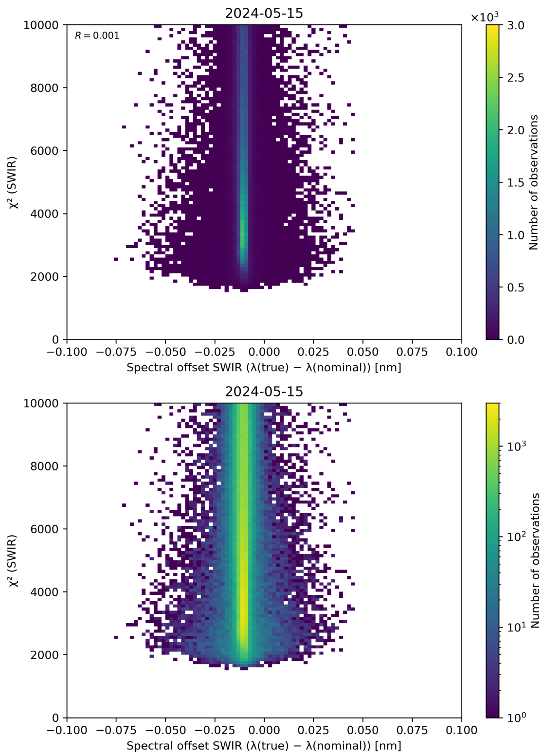
Figure 118: Scatter density plot of “Spectral offset SWIR ( \lambda(\text{true}) - \lambda(\text{nominal}) )” against “ \chi^2 (SWIR)” for 2024-05-14 to 2024-05-16.
