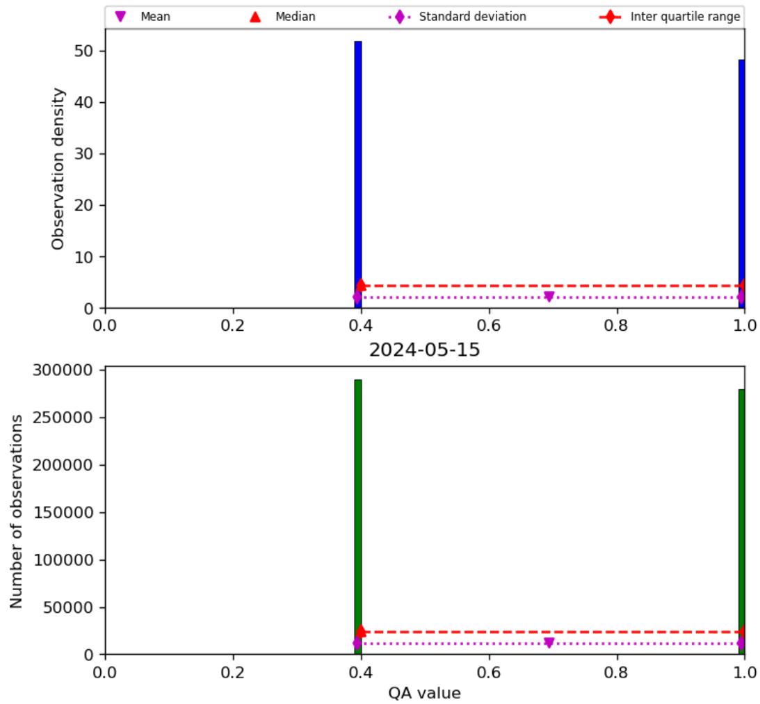
Figure 22: Histogram of “QA value” for 2024-05-14 to 2024-05-16
