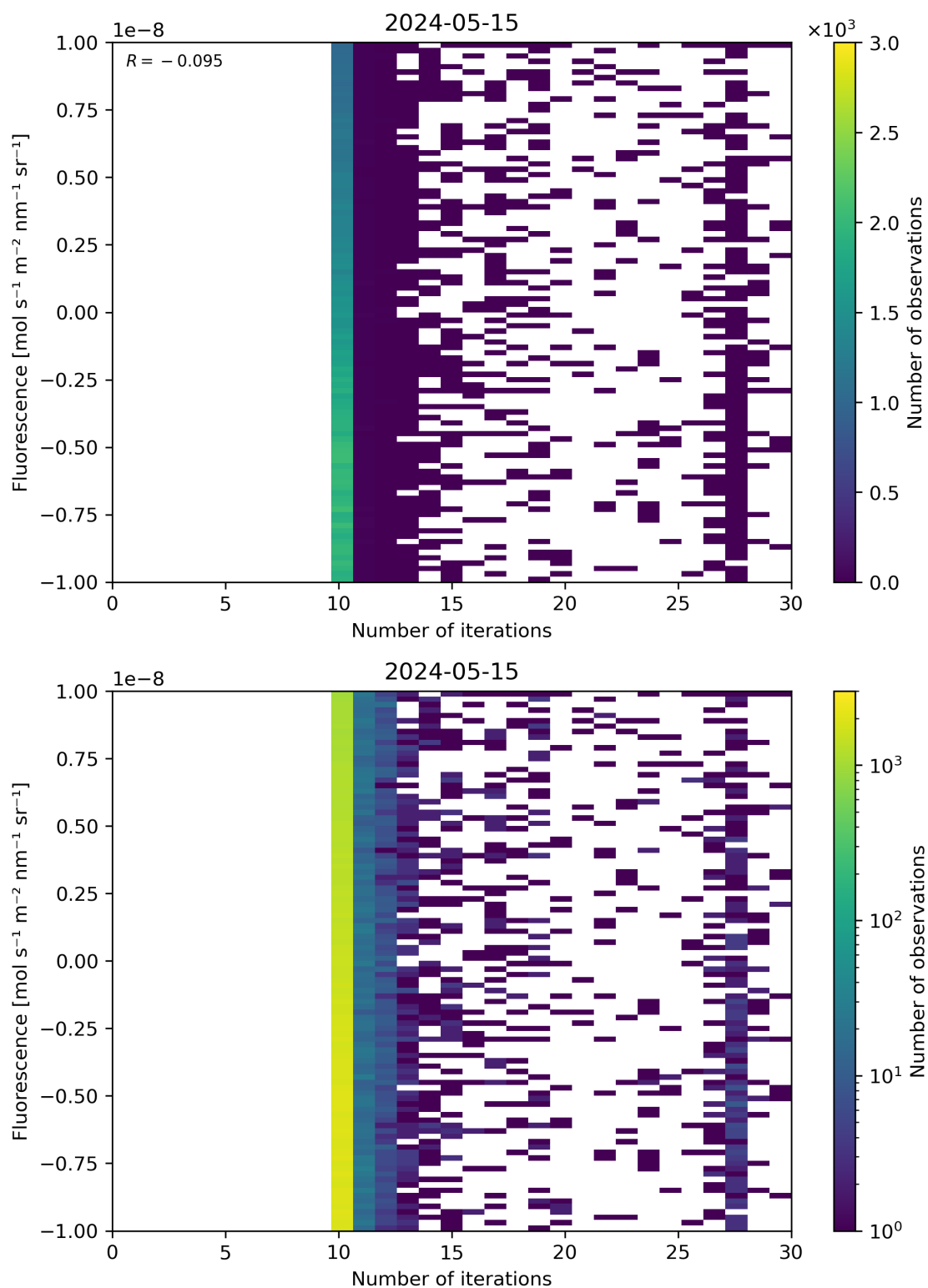
Figure 87: Scatter density plot of “Number of iterations” against “Fluorescence” for 2024-05-14 to 2024-05-16.
