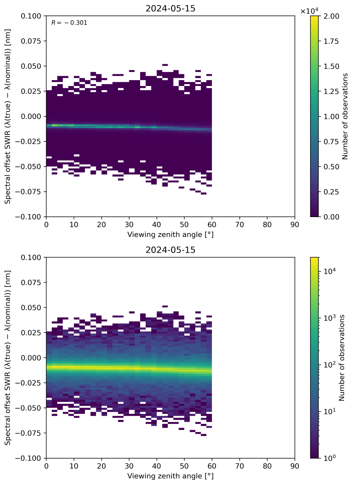
Figure 116: Scatter density plot of “Viewing zenith angle” against “Spectral offset SWIR ( \lambda(\text{true}) - \lambda(\text{nominal}) )” for 2024-05-14 to 2024-05-16.
