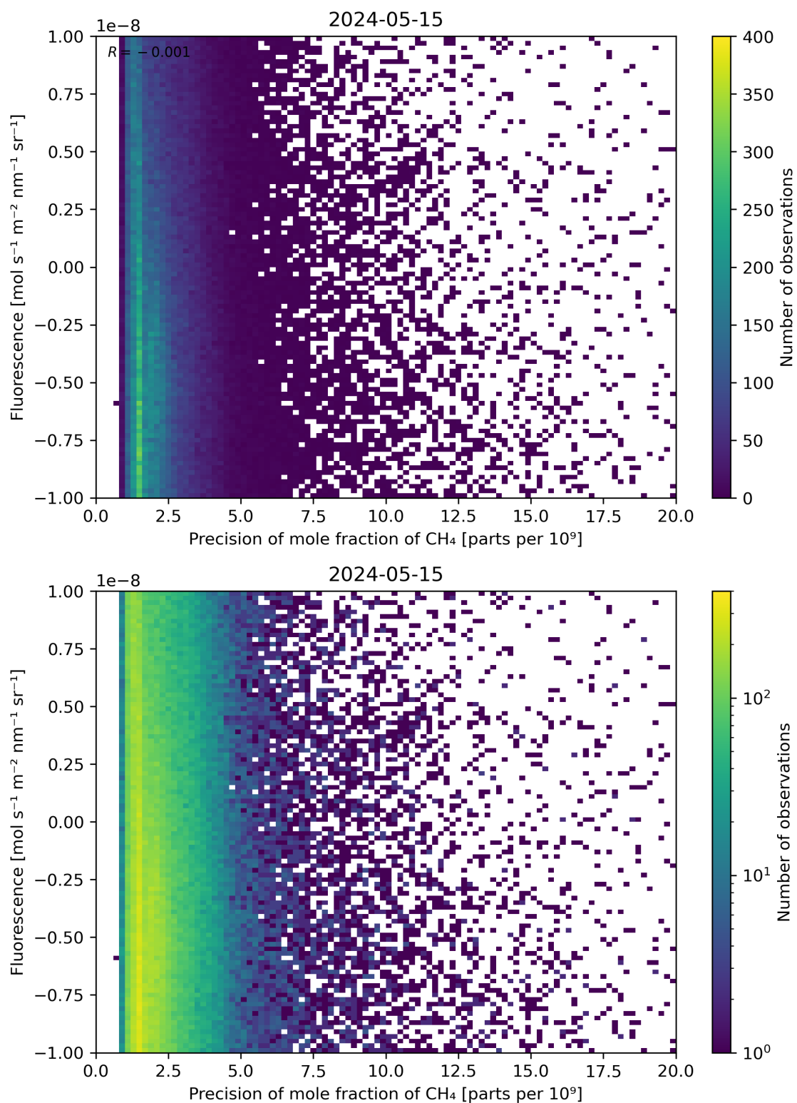
Figure 81: Scatter density plot of “Precision of mole fraction of \text{CH}_4 ” against “Fluorescence” for 2024-05-14 to 2024-05-16.
