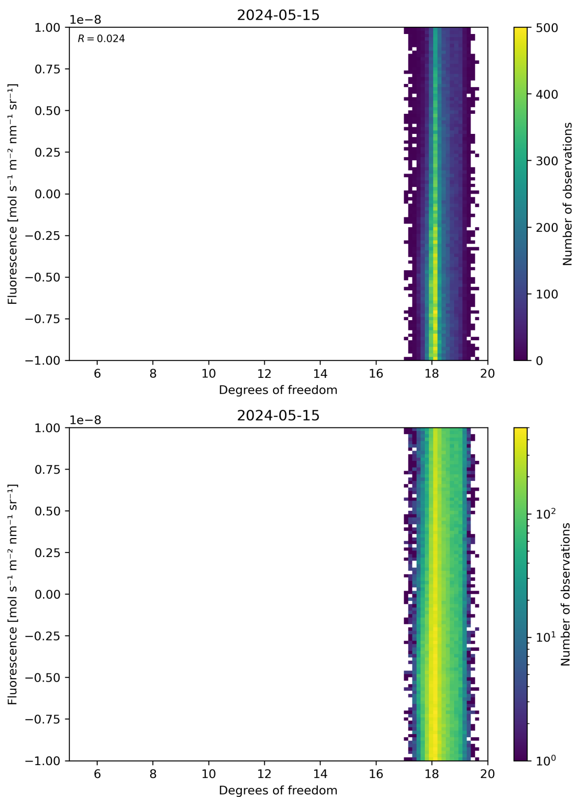
Figure 51: Scatter density plot of “Degrees of freedom” against “Fluorescence” for 2024-05-14 to 2024-05-16.
