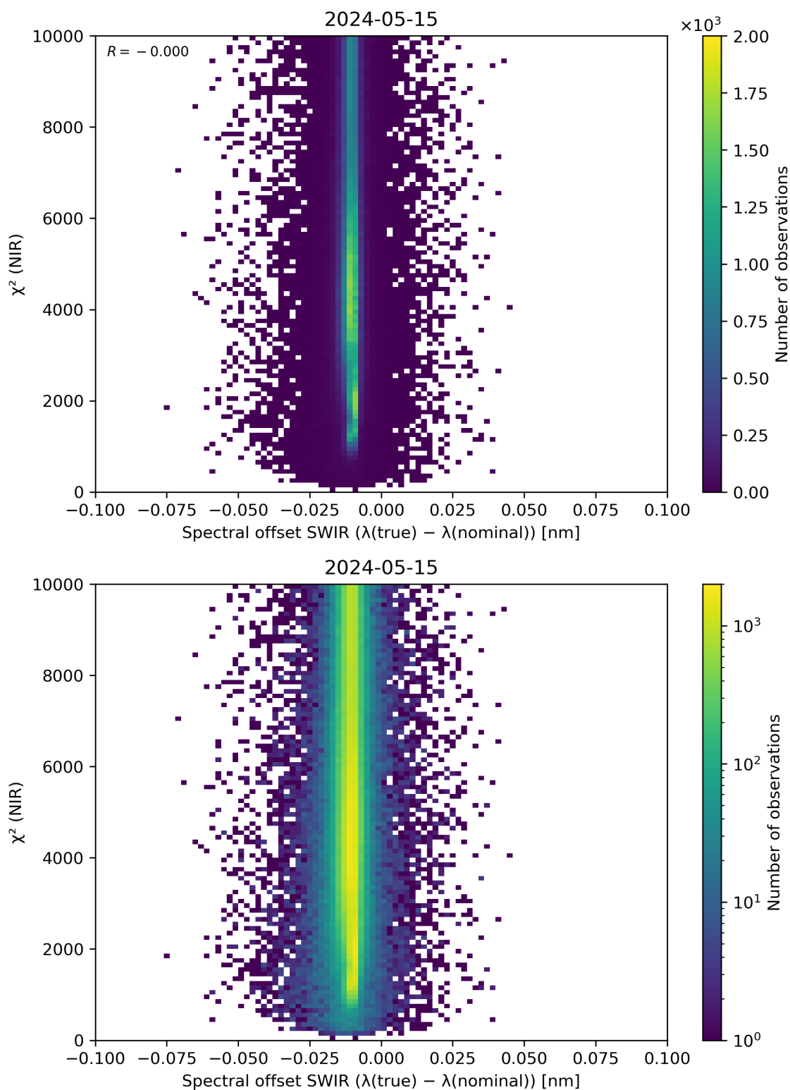
Figure 117: Scatter density plot of “Spectral offset SWIR ( \lambda(\text{true}) - \lambda(\text{nominal}) )” against “ \chi^2 (NIR)” for 2024-05-14 to 2024-05-16.
