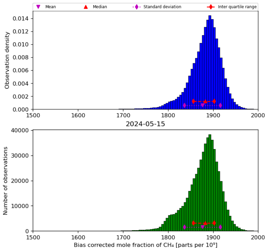
Figure 25: Histogram of “Bias corrected mole fraction of CH 4 ” for 2024-05-14 to 2024-05-16
