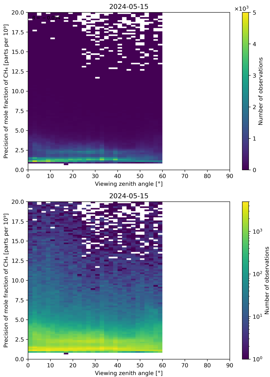
Figure 112: Scatter density plot of “Viewing zenith angle” against “Precision of mole fraction of CH 4 ” for 2024-05-14 to 2024-05-16.
