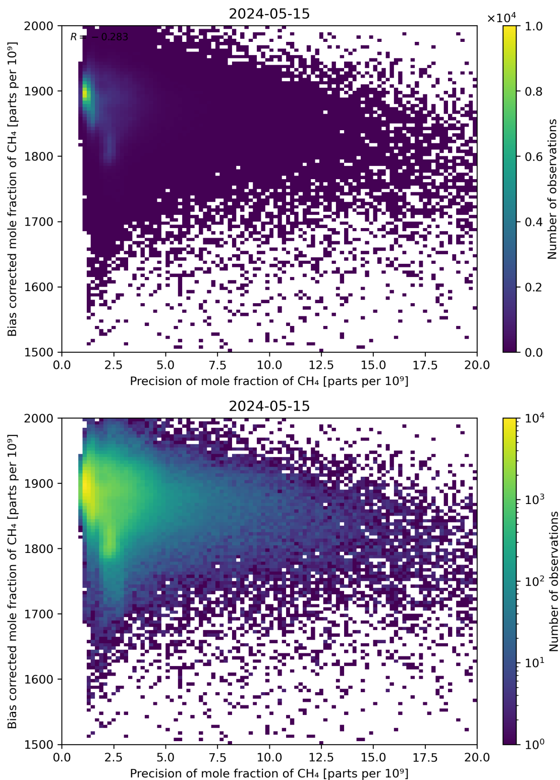
Figure 82: Scatter density plot of “Precision of mole fraction of \text{CH}_4 ” against “Bias corrected mole fraction of \text{CH}_4 ” for 2024-05-14 to 2024-05-16.
