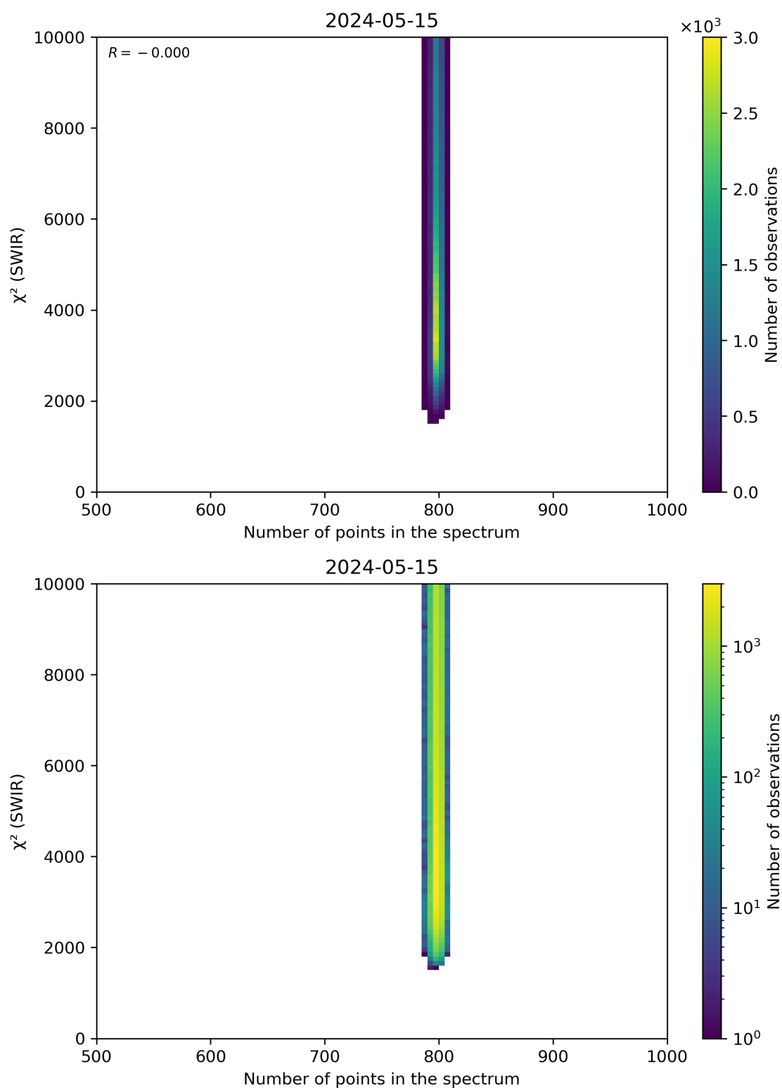
Figure 89: Scatter density plot of “Number of points in the spectrum” against “ \chi^2 (SWIR)” for 2024-05-14 to 2024-05-16.
