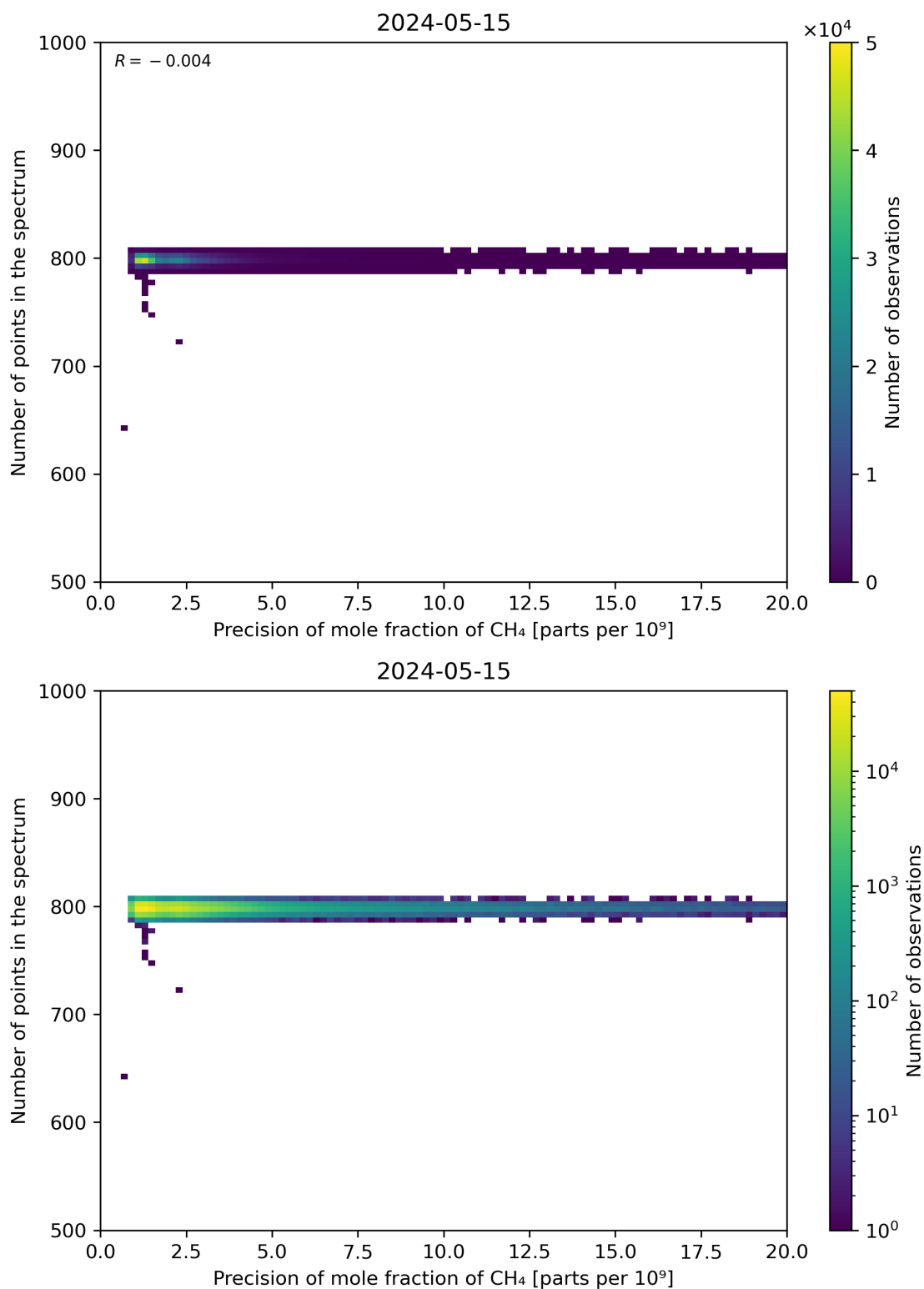
Figure 84: Scatter density plot of “Precision of mole fraction of CH 4 ” against “Number of points in the spectrum” for 2024-05-14 to 2024-05-16.
