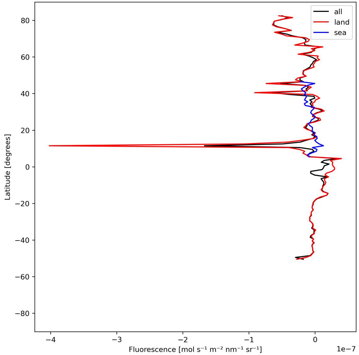
Figure 21: Zonal average of “Fluorescence” for 2024-05-14 to 2024-05-16.
