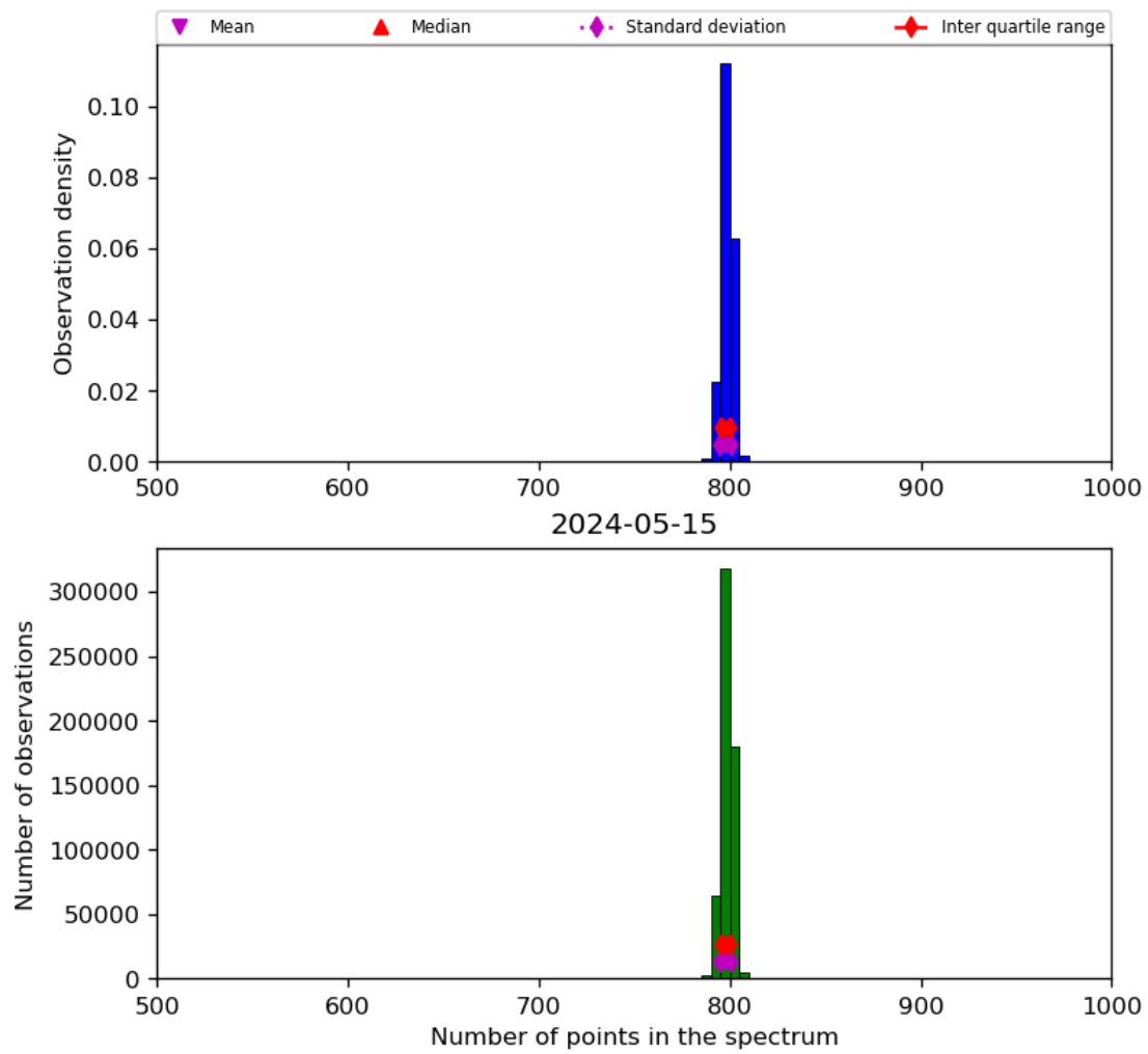
Figure 26: Histogram of “Number of points in the spectrum” for 2024-05-14 to 2024-05-16
