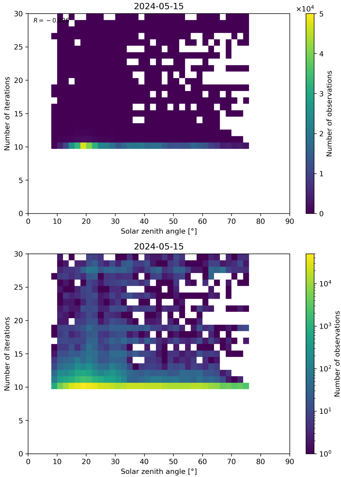
Figure 102: Scatter density plot of “Solar zenith angle” against “Number of iterations” for 2024-05-14 to 2024-05-16.
