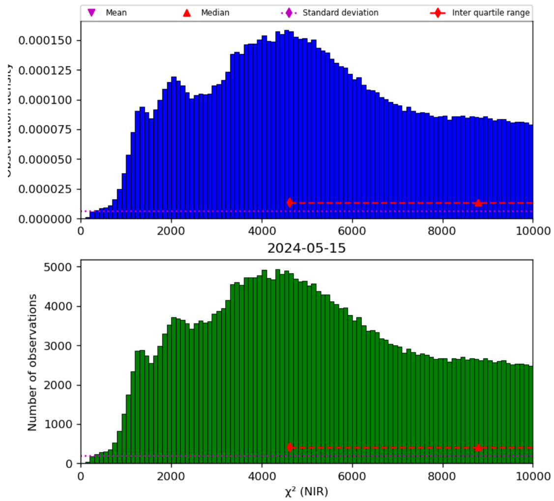
Figure 29: Histogram of “ \chi^2 (NIR)” for 2024-05-14 to 2024-05-16
