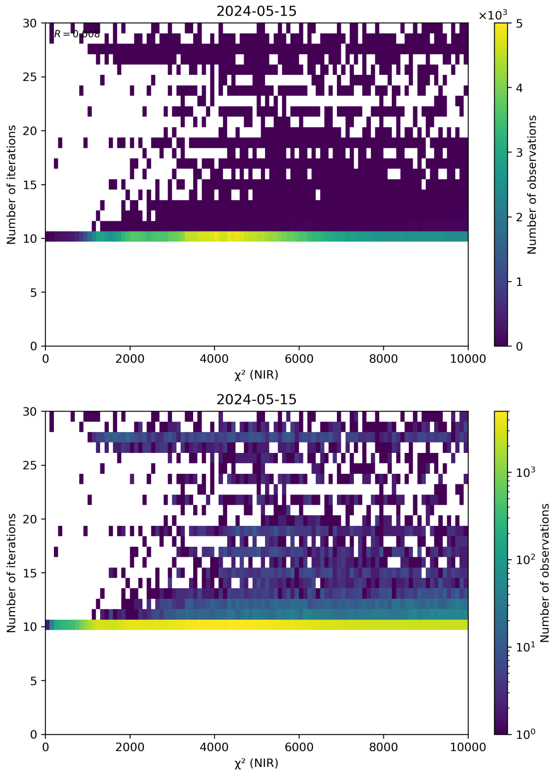
Figure 46: Scatter density plot of “ \chi^2 (NIR)” against “Number of iterations” for 2024-05-14 to 2024-05-16.
