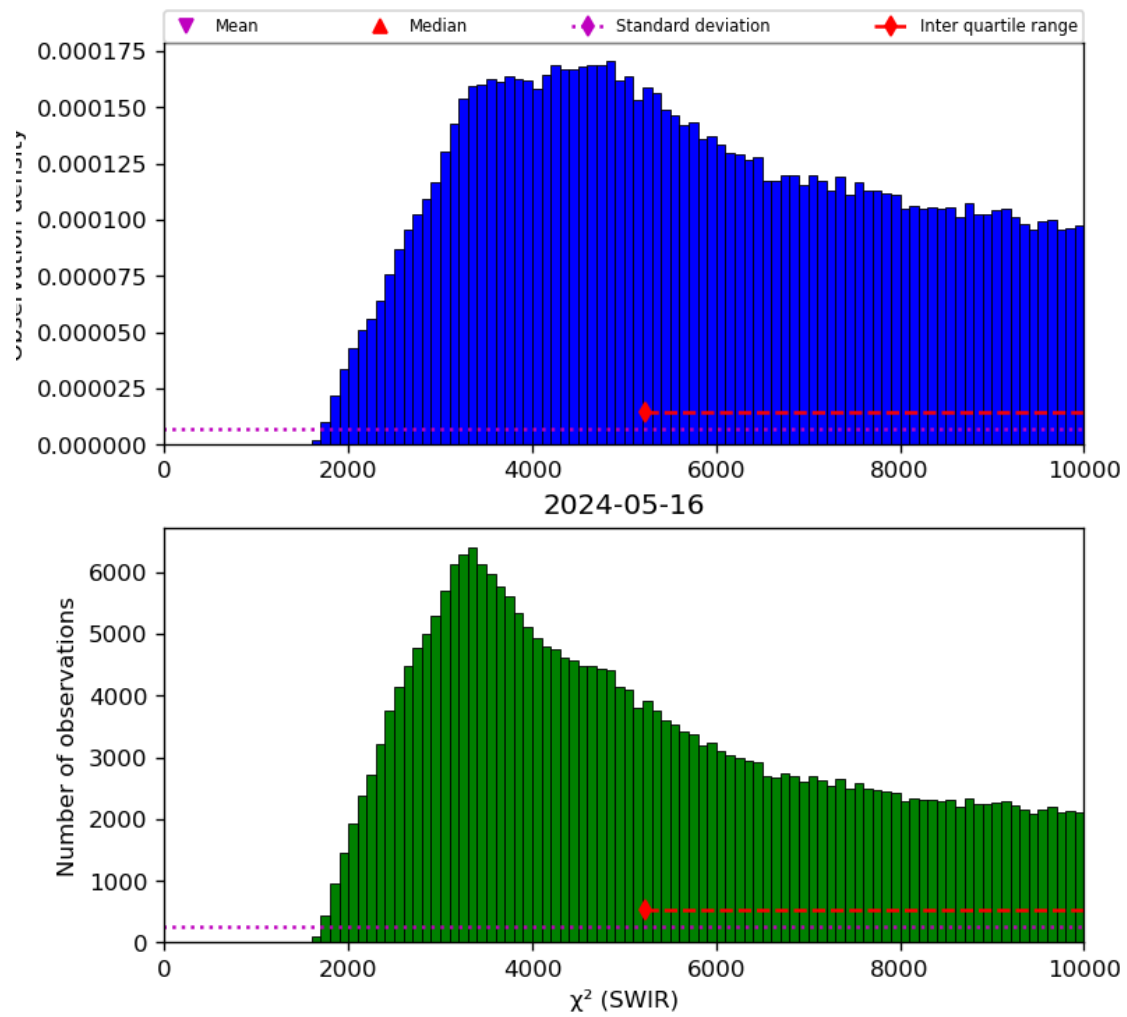
Figure 28: Histogram of “ \chi^2 (SWIR)” for 2024-05-15 to 2024-05-17
