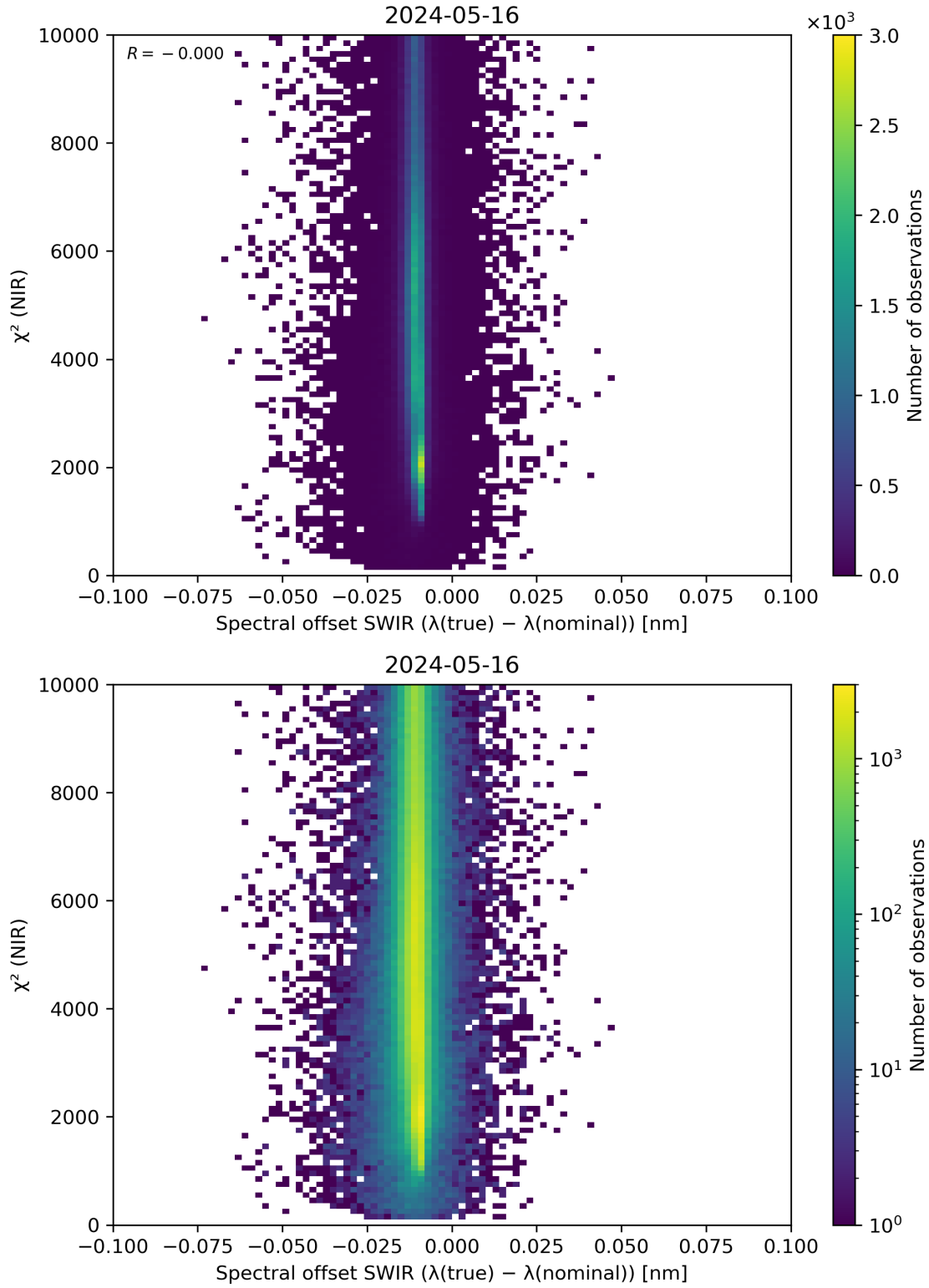
Figure 117: Scatter density plot of “Spectral offset SWIR ( \lambda(\text{true}) - \lambda(\text{nominal}) )” against “ \chi^2 (NIR)” for 2024-05-15 to 2024-05-17.
