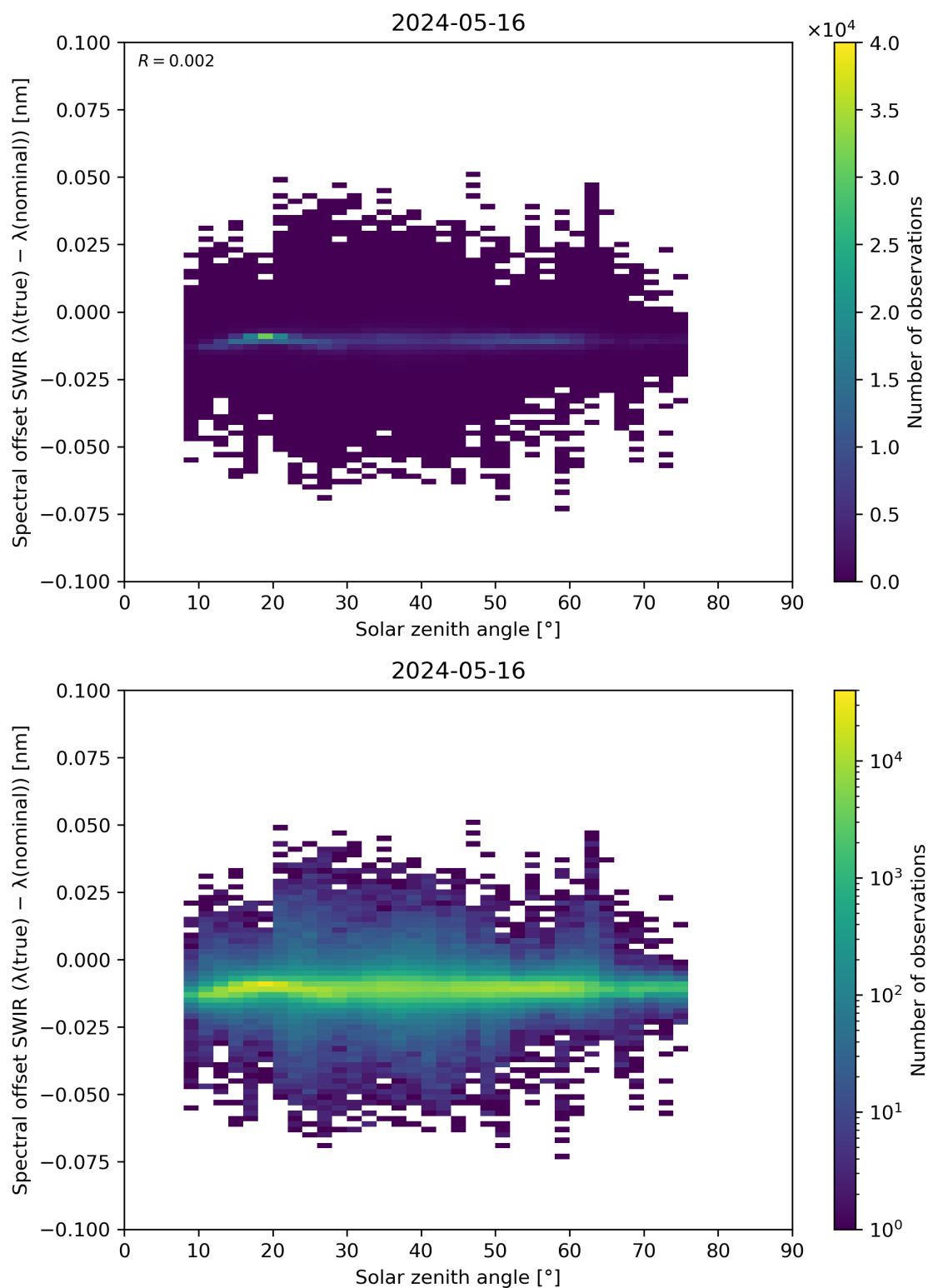
Figure 104: Scatter density plot of “Solar zenith angle” against “Spectral offset SWIR ( \lambda(\text{true}) - \lambda(\text{nominal}) )” for 2024-05-15 to 2024-05-17.
