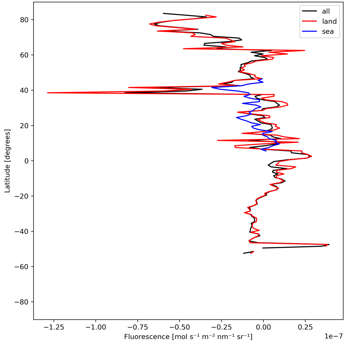
Figure 21: Zonal average of “Fluorescence” for 2024-05-15 to 2024-05-17.
