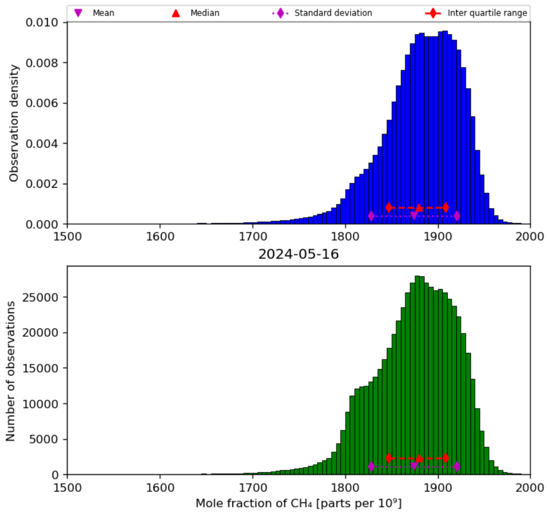
Figure 23: Histogram of “Mole fraction of CH 4 ” for 2024-05-15 to 2024-05-17
