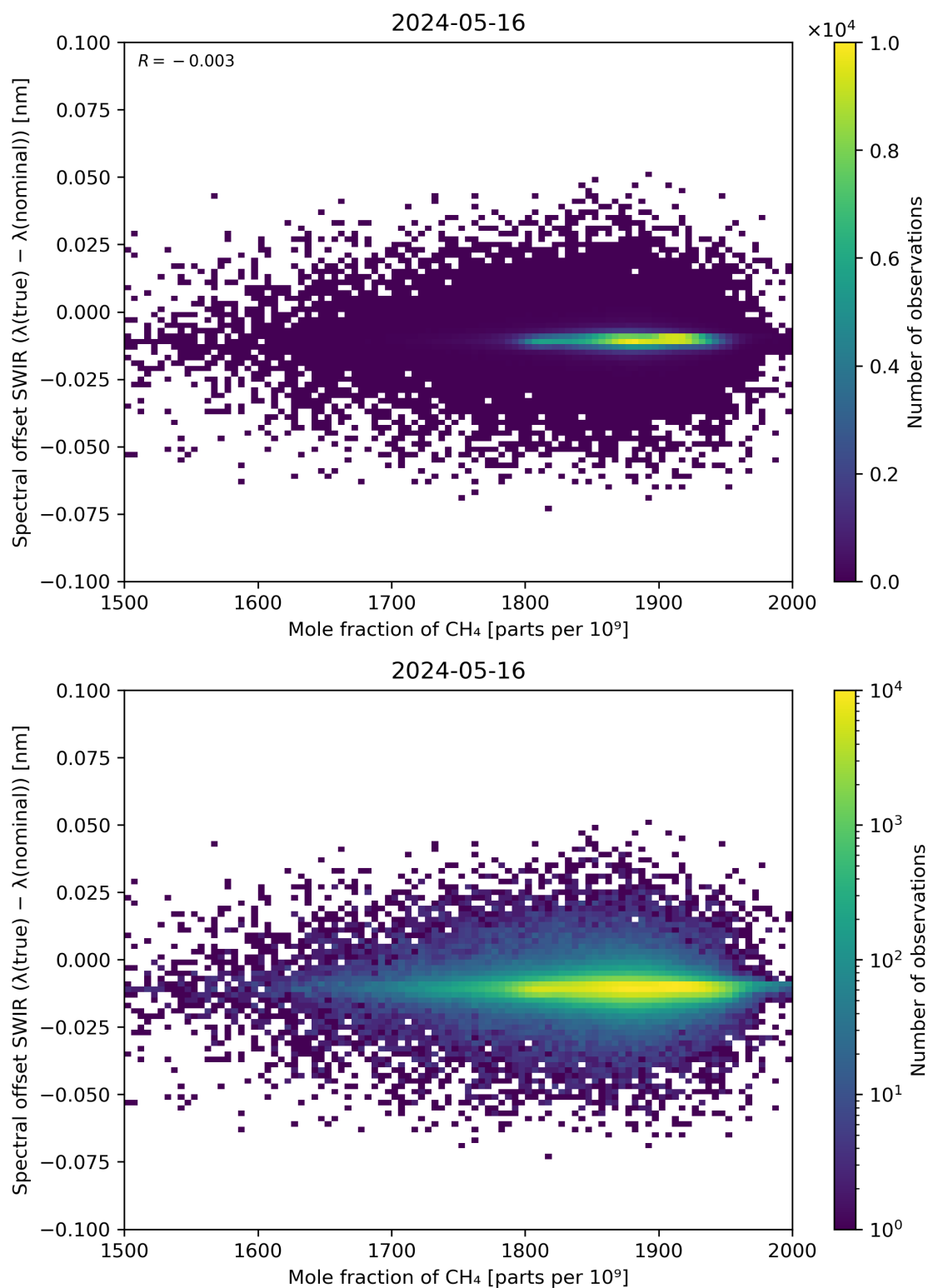
Figure 86: Scatter density plot of “Mole fraction of CH 4 ” against “Spectral offset SWIR ( \lambda(\text{true}) - \lambda(\text{nominal}) )” for 2024-05-15 to 2024-05-17.
