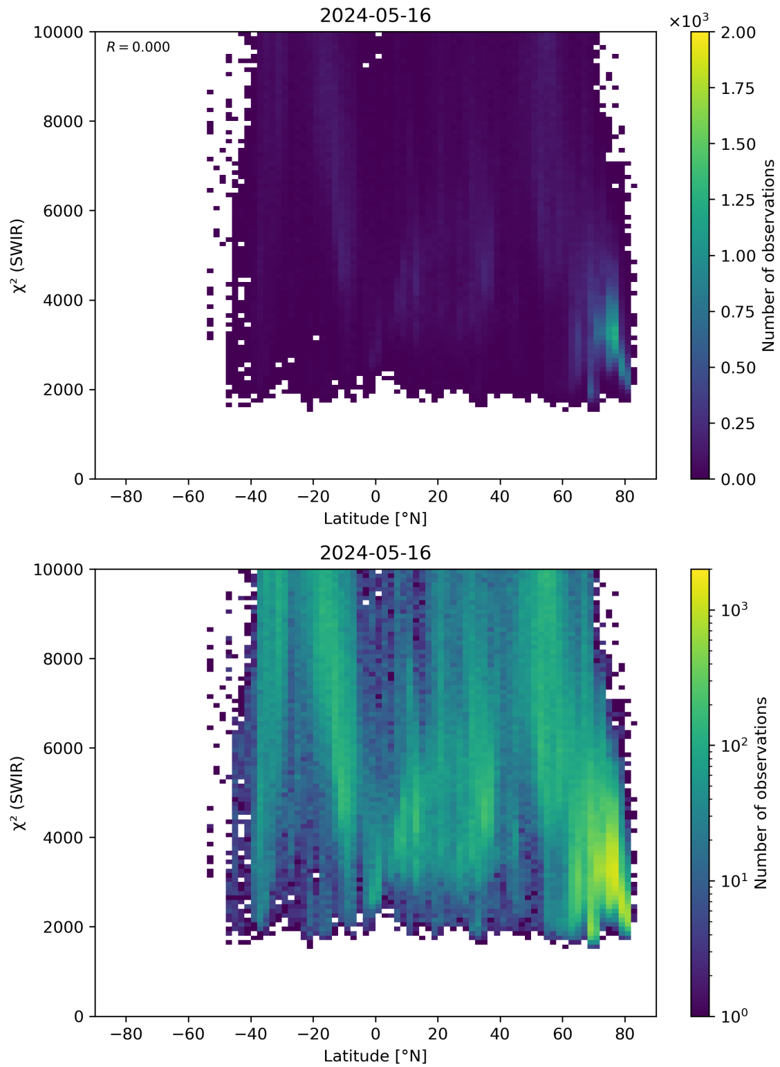
Figure 54: Scatter density plot of “Latitude” against “ \chi^2 (SWIR)” for 2024-05-15 to 2024-05-17.
