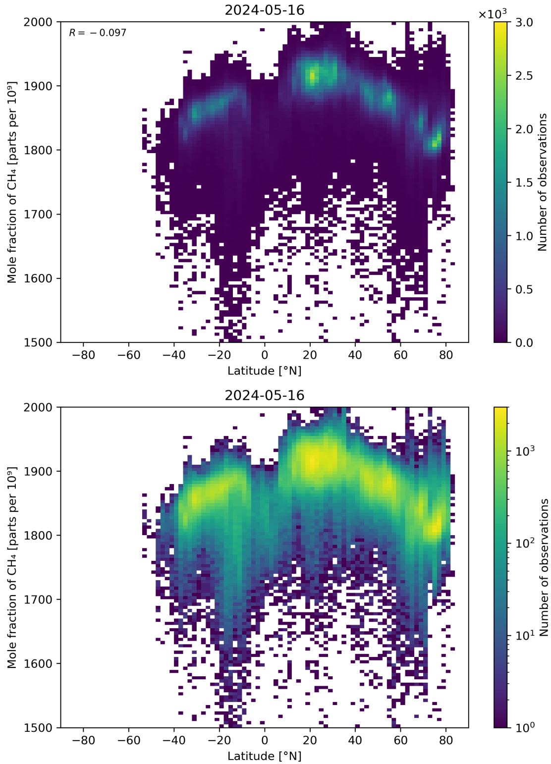
Figure 57: Scatter density plot of “Latitude” against “Mole fraction of CH 4 ” for 2024-05-15 to 2024-05-17.
