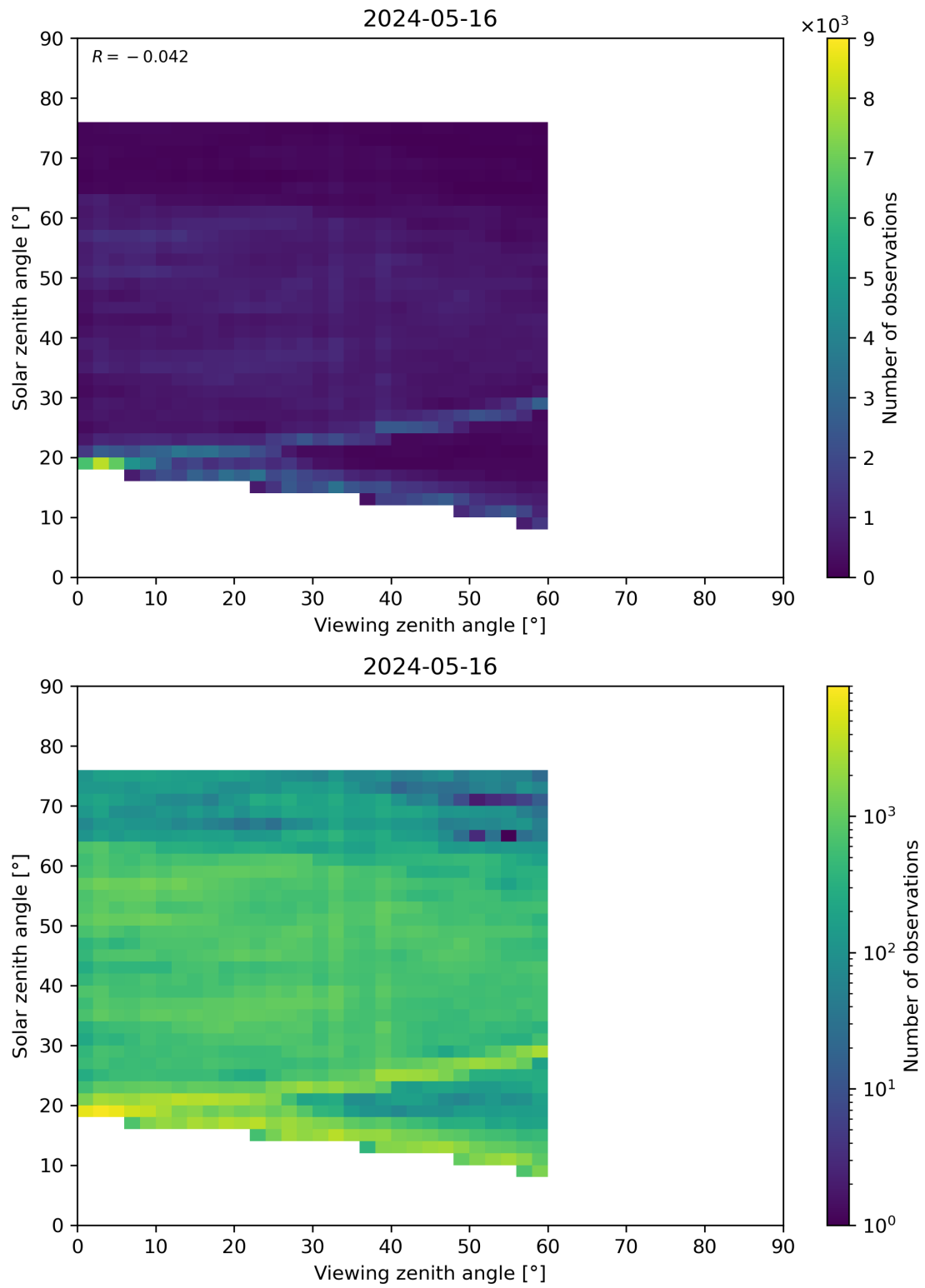
Figure 115: Scatter density plot of “Viewing zenith angle” against “Solar zenith angle” for 2024-05-15 to 2024-05-17.
