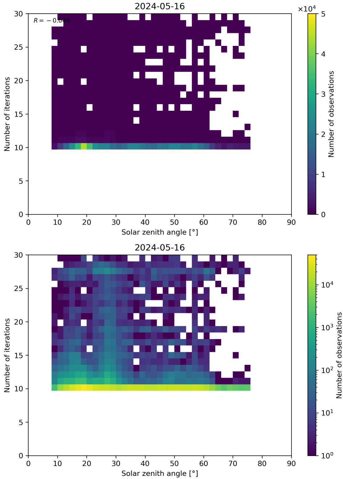
Figure 102: Scatter density plot of “Solar zenith angle” against “Number of iterations” for 2024-05-15 to 2024-05-17.
