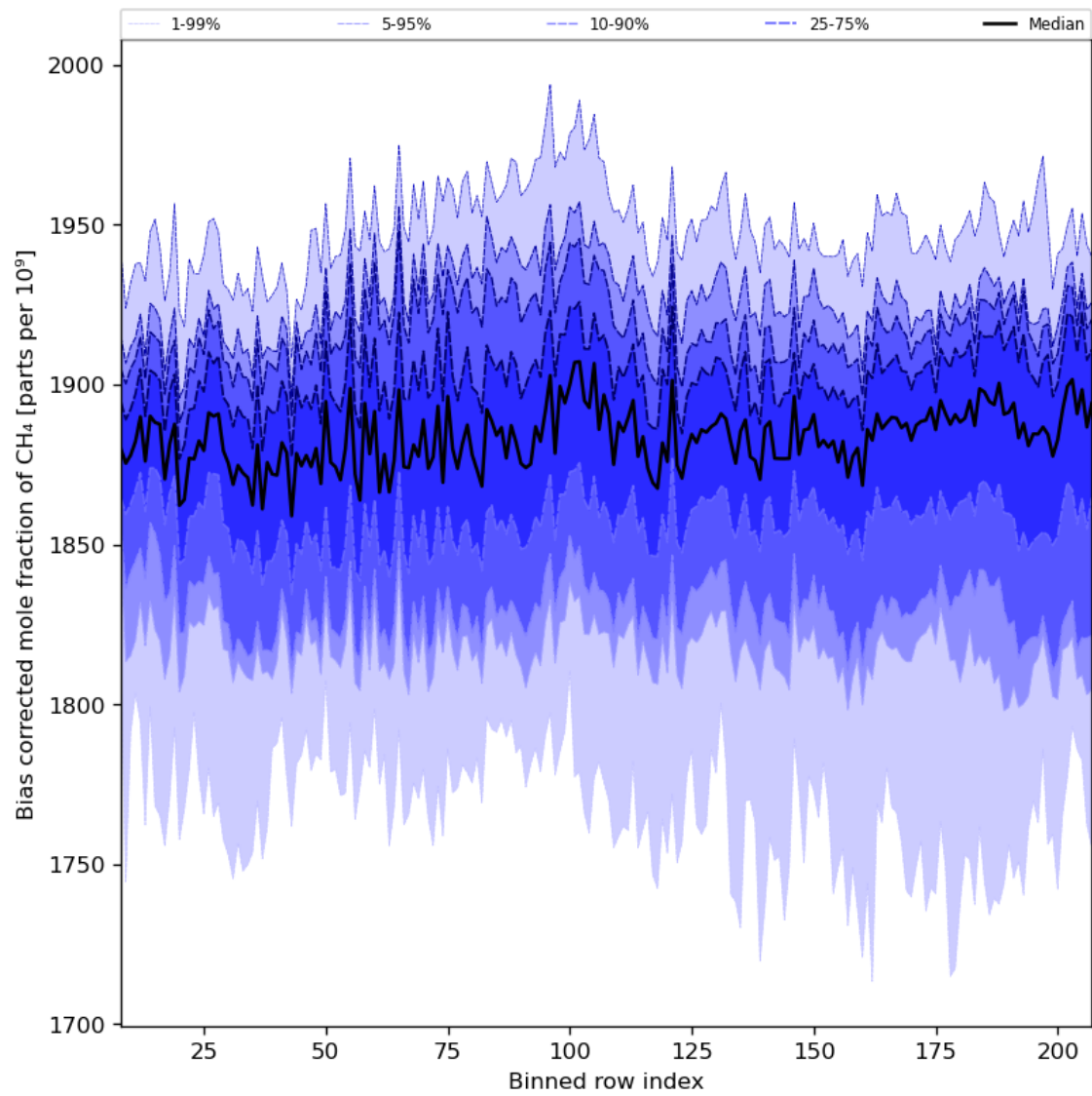
Figure 36: Along track statistics of “Bias corrected mole fraction of CH 4 ” for 2024-05-15 to 2024-05-17
