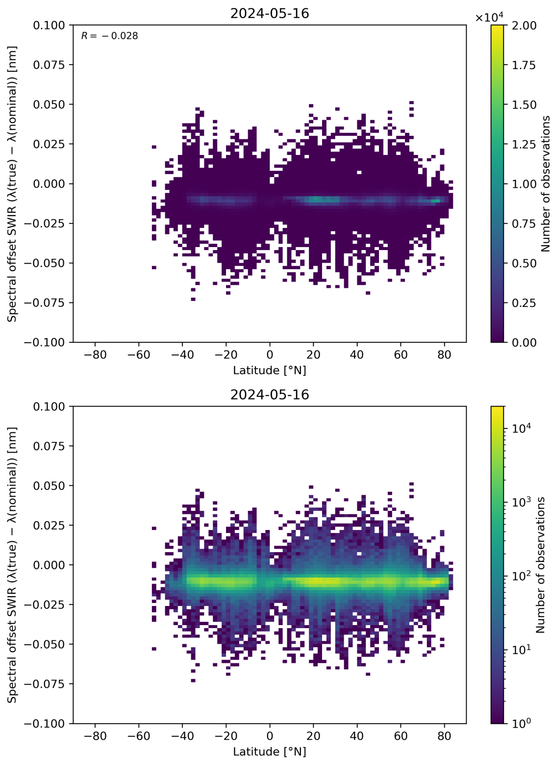
Figure 62: Scatter density plot of “Latitude” against “Spectral offset SWIR ( \lambda(\text{true}) - \lambda(\text{nominal}) )” for 2024-05-15 to 2024-05-17.
