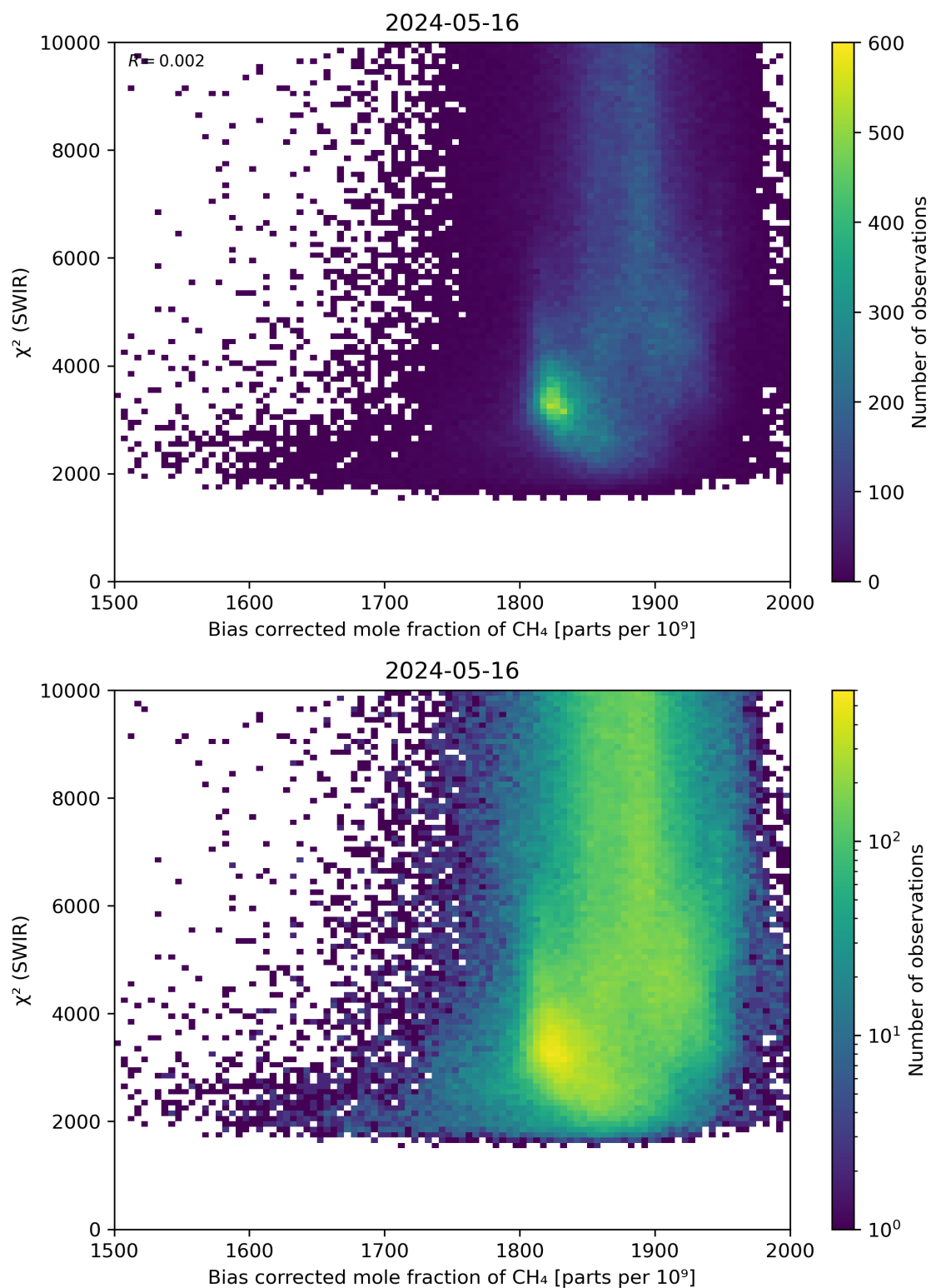
Figure 64: Scatter density plot of “Bias corrected mole fraction of CH 4 ” against “ \chi^2 (SWIR)” for 2024-05-15 to 2024-05-17.
