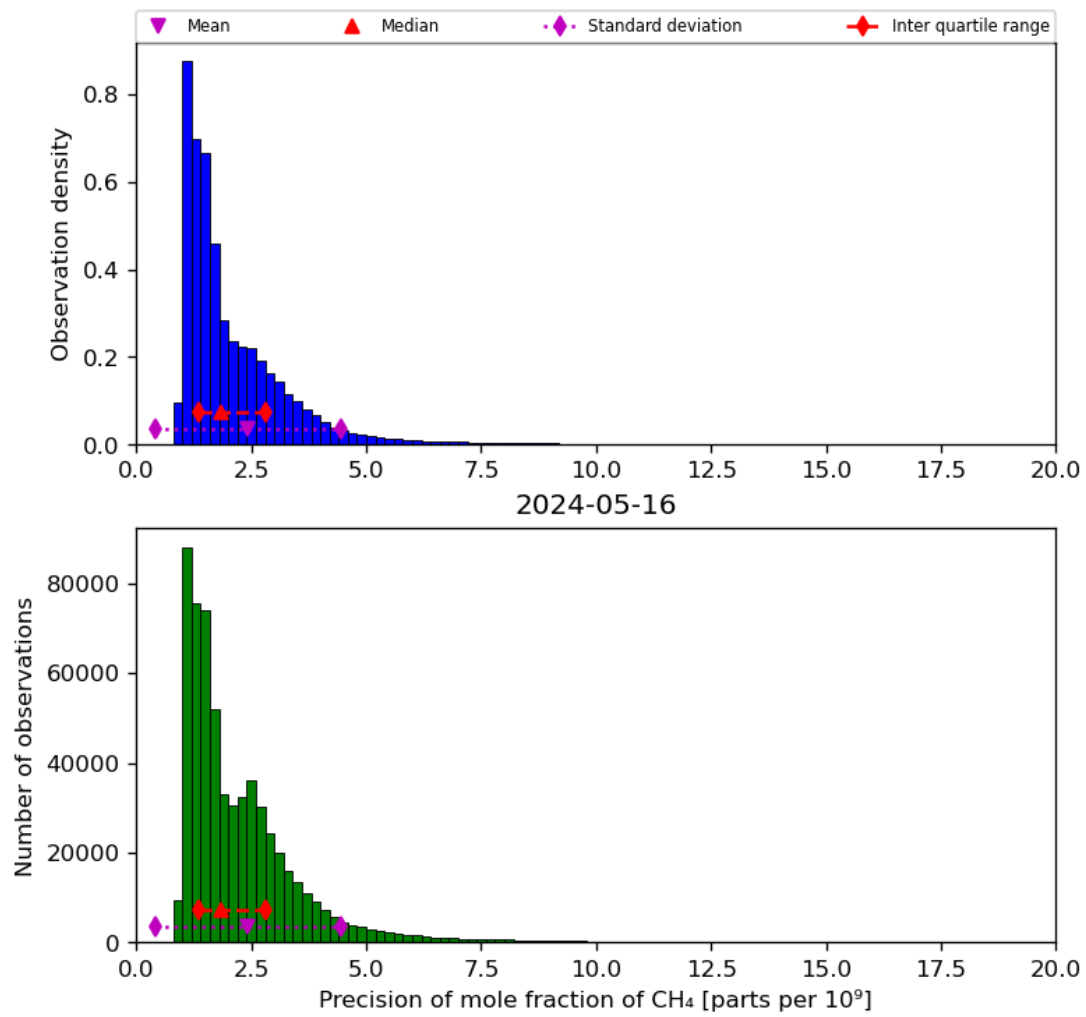
Figure 24: Histogram of “Precision of mole fraction of CH 4 ” for 2024-05-15 to 2024-05-17
