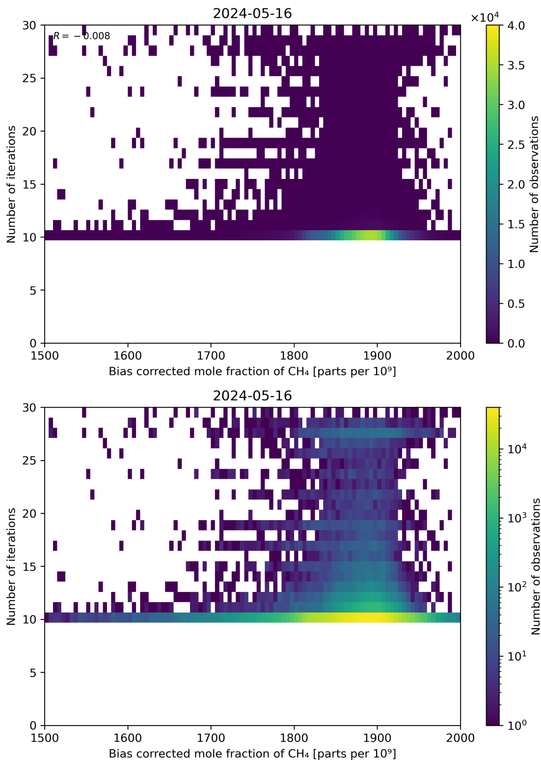
Figure 67: Scatter density plot of “Bias corrected mole fraction of CH 4 ” against “Number of iterations” for 2024-05-15 to 2024-05-17.
