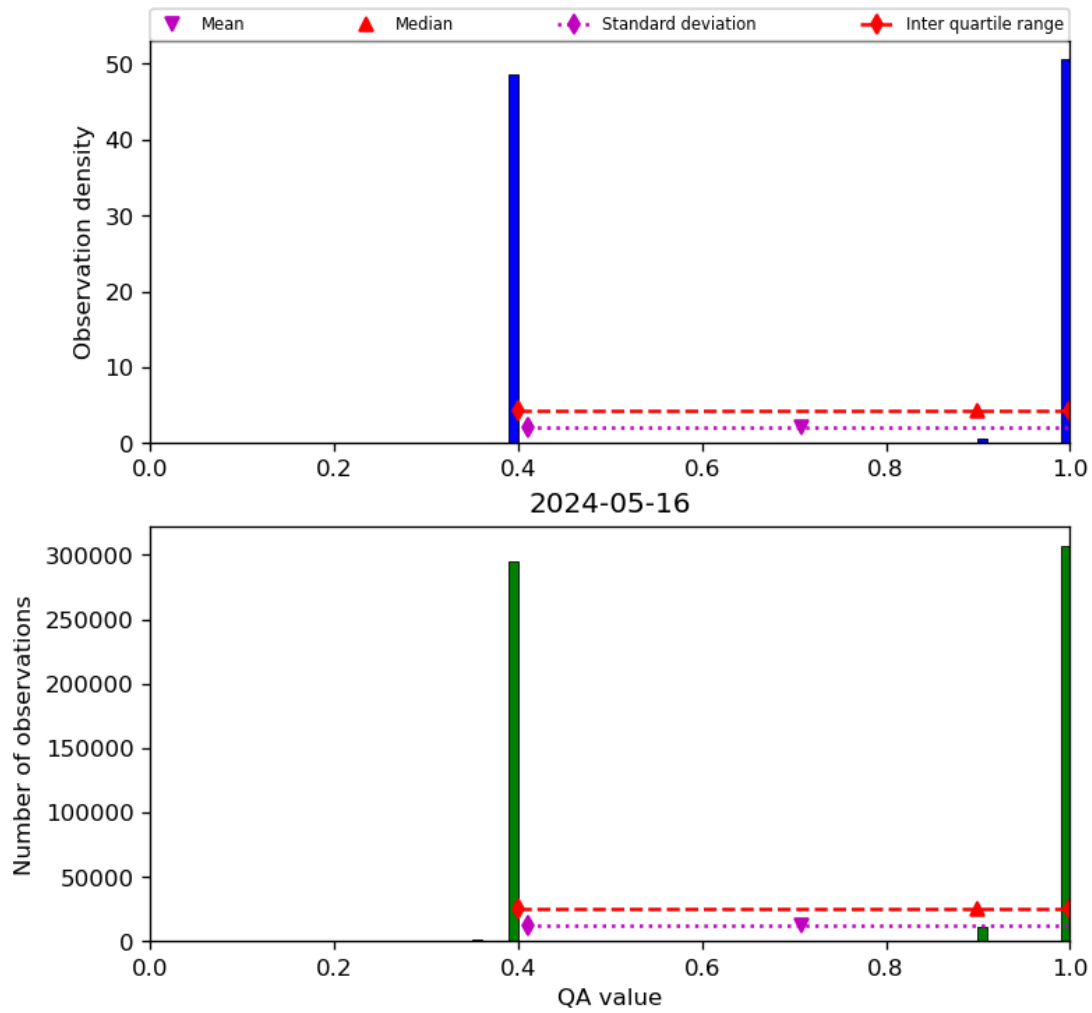
Figure 22: Histogram of “QA value” for 2024-05-15 to 2024-05-17
