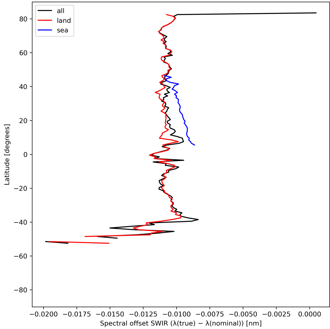
Figure 16: Zonal average of “Spectral offset SWIR ( \lambda(\text{true}) - \lambda(\text{nominal}) )” for 2024-05-15 to 2024-05-17.
