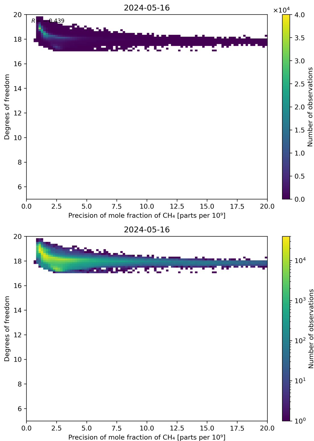
Figure 80: Scatter density plot of “Precision of mole fraction of CH 4 ” against “Degrees of freedom” for 2024-05-15 to 2024-05-17.
