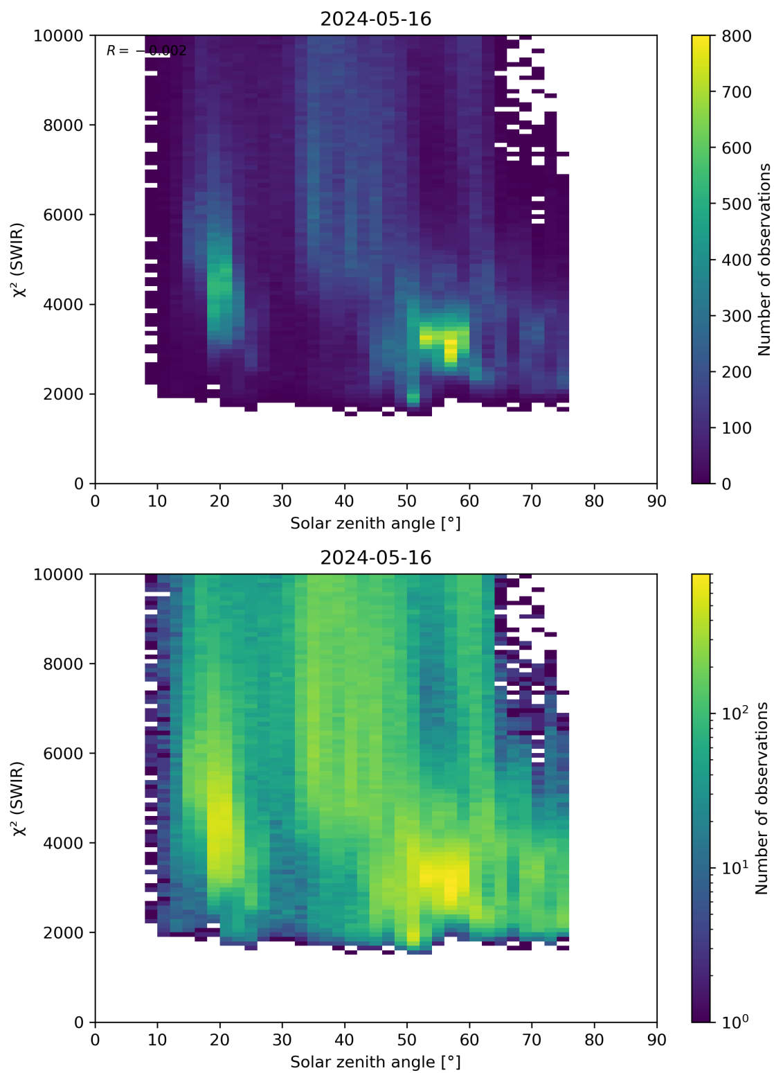
Figure 95: Scatter density plot of “Solar zenith angle” against “ \chi^2 (SWIR)” for 2024-05-15 to 2024-05-17.
