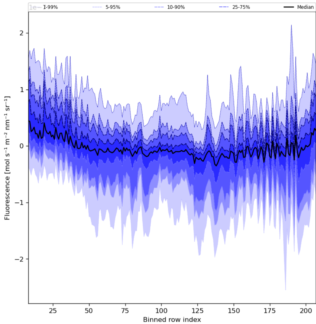
Figure 43: Along track statistics of “Fluorescence” for 2024-05-15 to 2024-05-17
