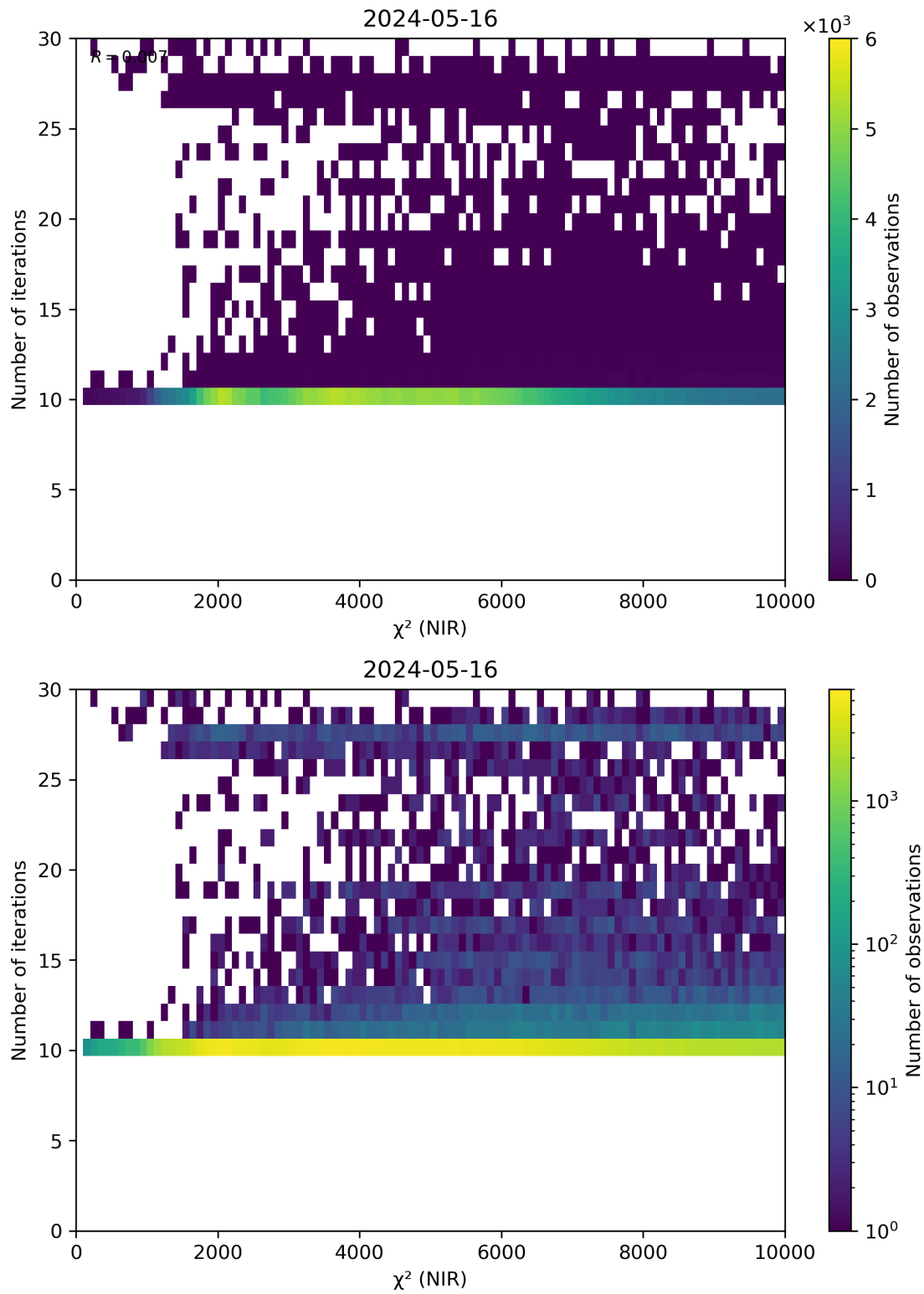
Figure 46: Scatter density plot of “ \chi^2 (NIR)” against “Number of iterations” for 2024-05-15 to 2024-05-17.
