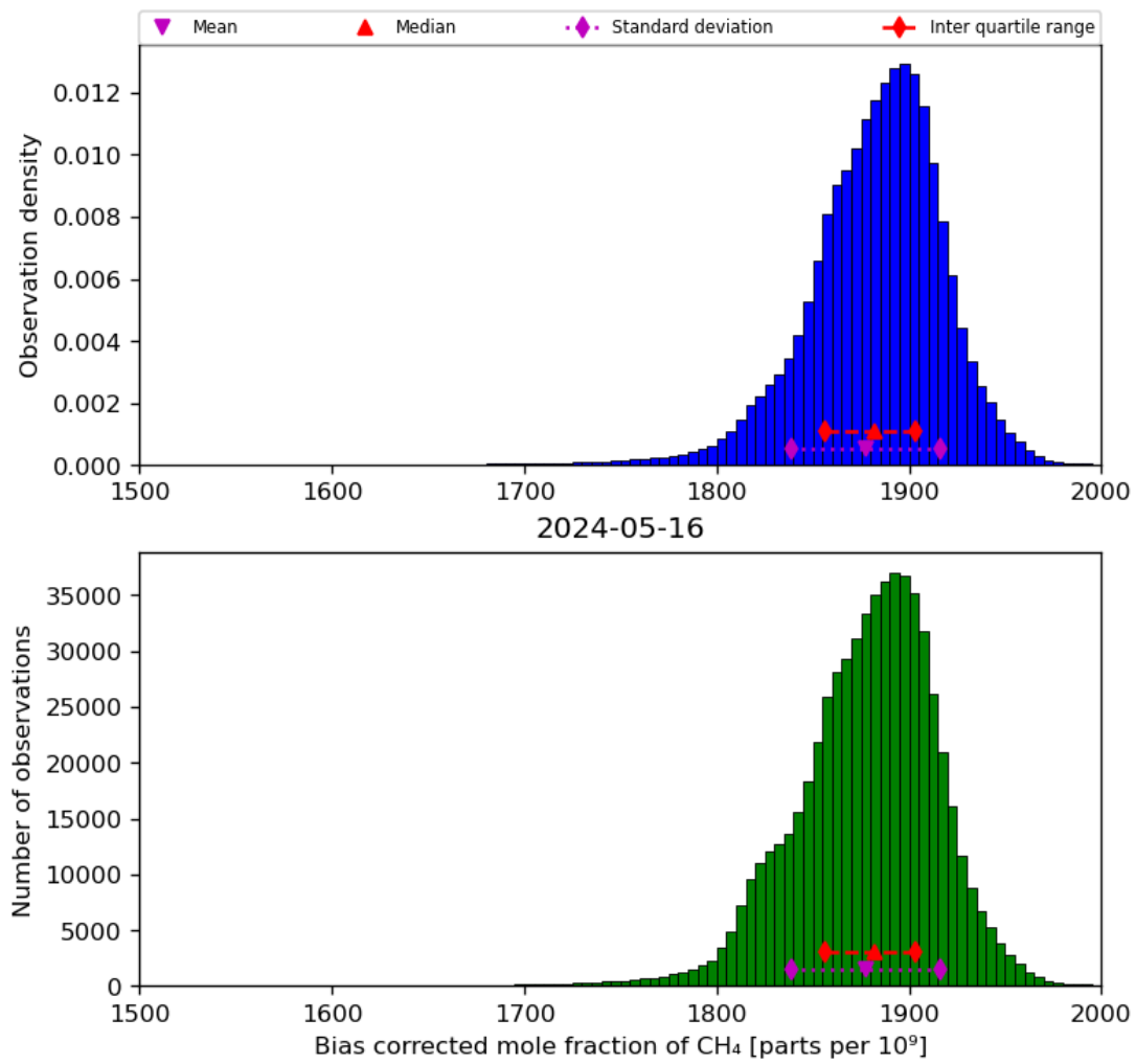
Figure 25: Histogram of “Bias corrected mole fraction of CH 4 ” for 2024-05-15 to 2024-05-17
