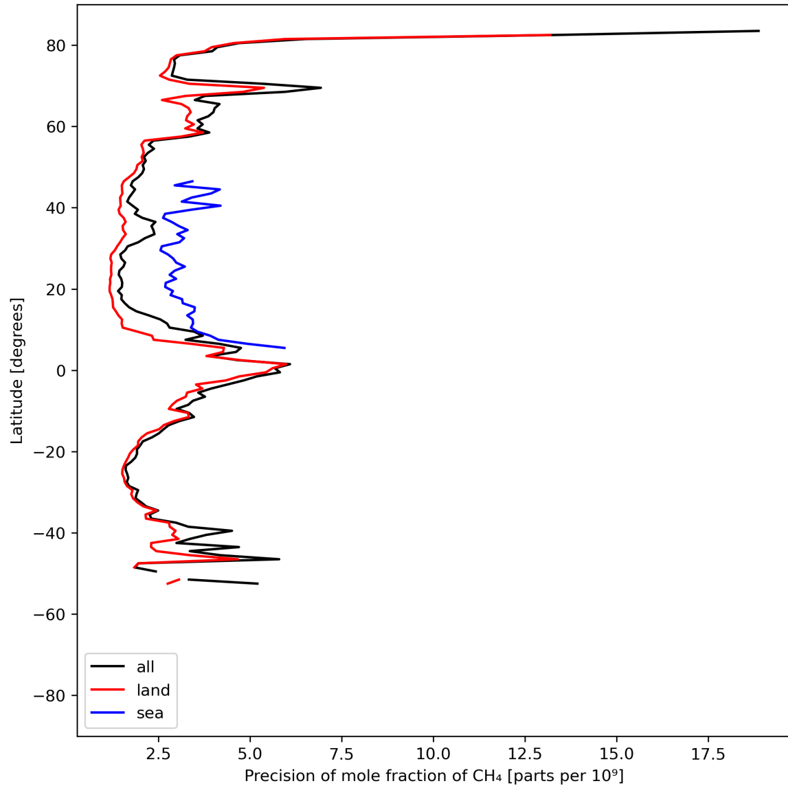
Figure 13: Zonal average of “Precision of mole fraction of CH 4 ” for 2024-05-15 to 2024-05-17.
