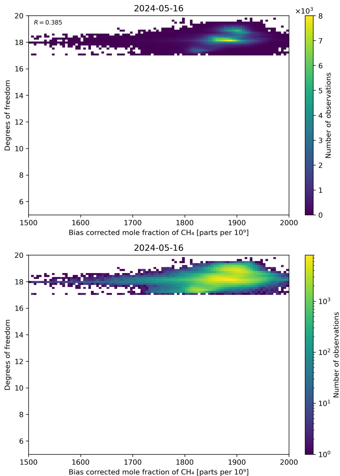
Figure 65: Scatter density plot of “Bias corrected mole fraction of CH 4 ” against “Degrees of freedom” for 2024-05-15 to 2024-05-17.
