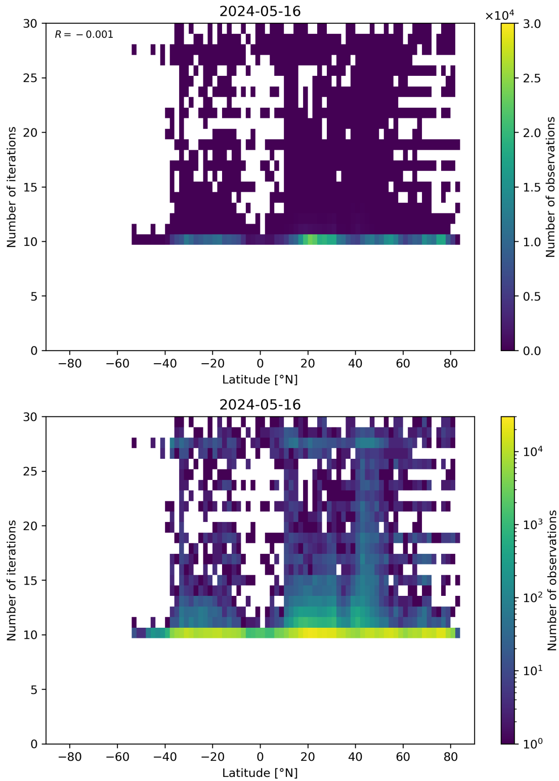
Figure 60: Scatter density plot of “Latitude” against “Number of iterations” for 2024-05-15 to 2024-05-17.
