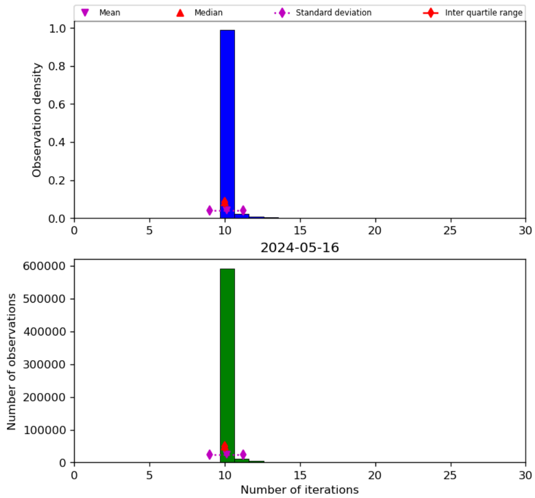
Figure 31: Histogram of “Number of iterations” for 2024-05-15 to 2024-05-17
