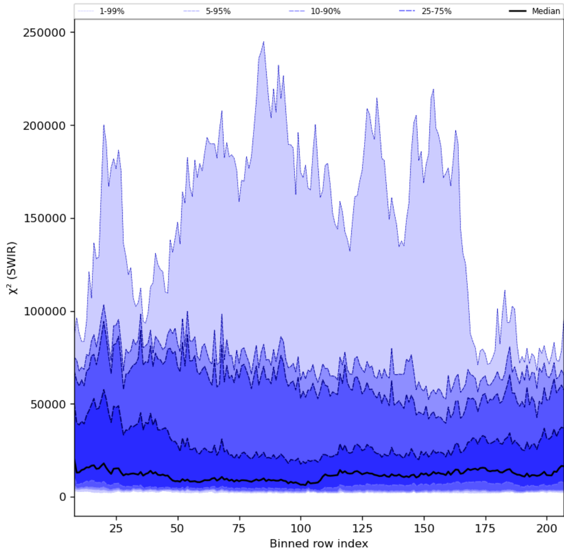
Figure 39: Along track statistics of “ \chi^2 (SWIR)” for 2024-05-15 to 2024-05-17
