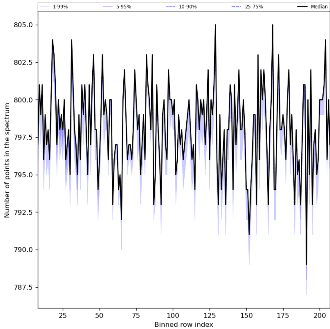
Figure 37: Along track statistics of “Number of points in the spectrum” for 2024-05-15 to 2024-05-17
