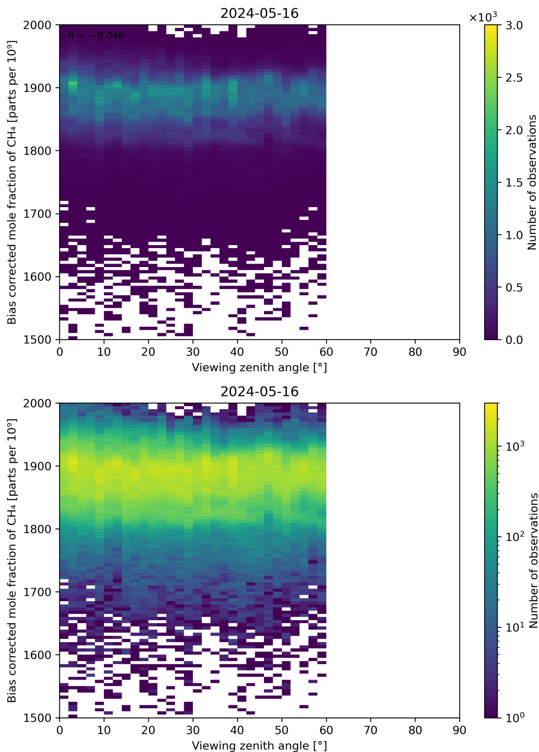
Figure 111: Scatter density plot of “Viewing zenith angle” against “Bias corrected mole fraction of CH 4 ” for 2024-05-15 to 2024-05-17.
