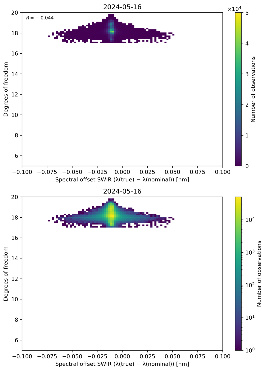
Figure 119: Scatter density plot of “Spectral offset SWIR ( \lambda(\text{true}) - \lambda(\text{nominal}) )” against “Degrees of freedom” for 2024-05-15 to 2024-05-17.
