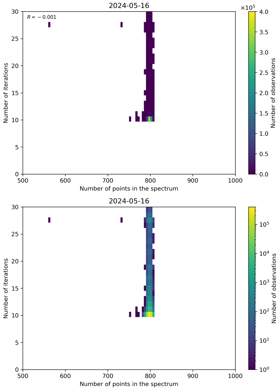
Figure 92: Scatter density plot of “Number of points in the spectrum” against “Number of iterations” for 2024-05-15 to 2024-05-17.
