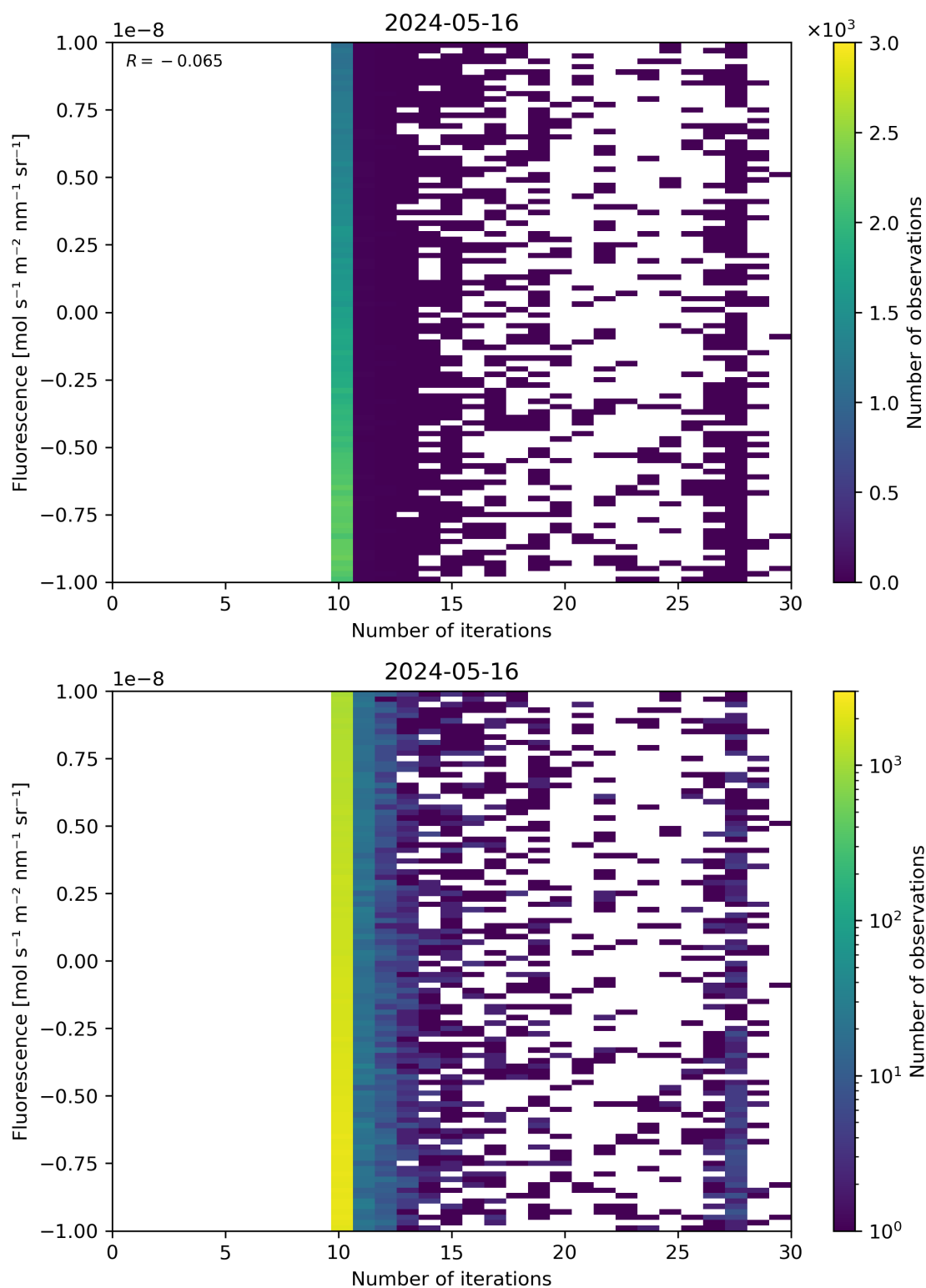
Figure 87: Scatter density plot of “Number of iterations” against “Fluorescence” for 2024-05-15 to 2024-05-17.
