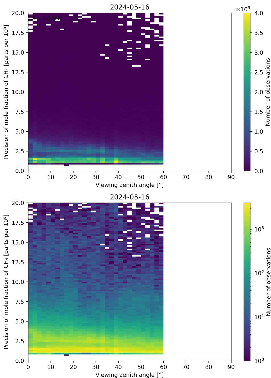
Figure 112: Scatter density plot of “Viewing zenith angle” against “Precision of mole fraction of CH 4 ” for 2024-05-15 to 2024-05-17.
