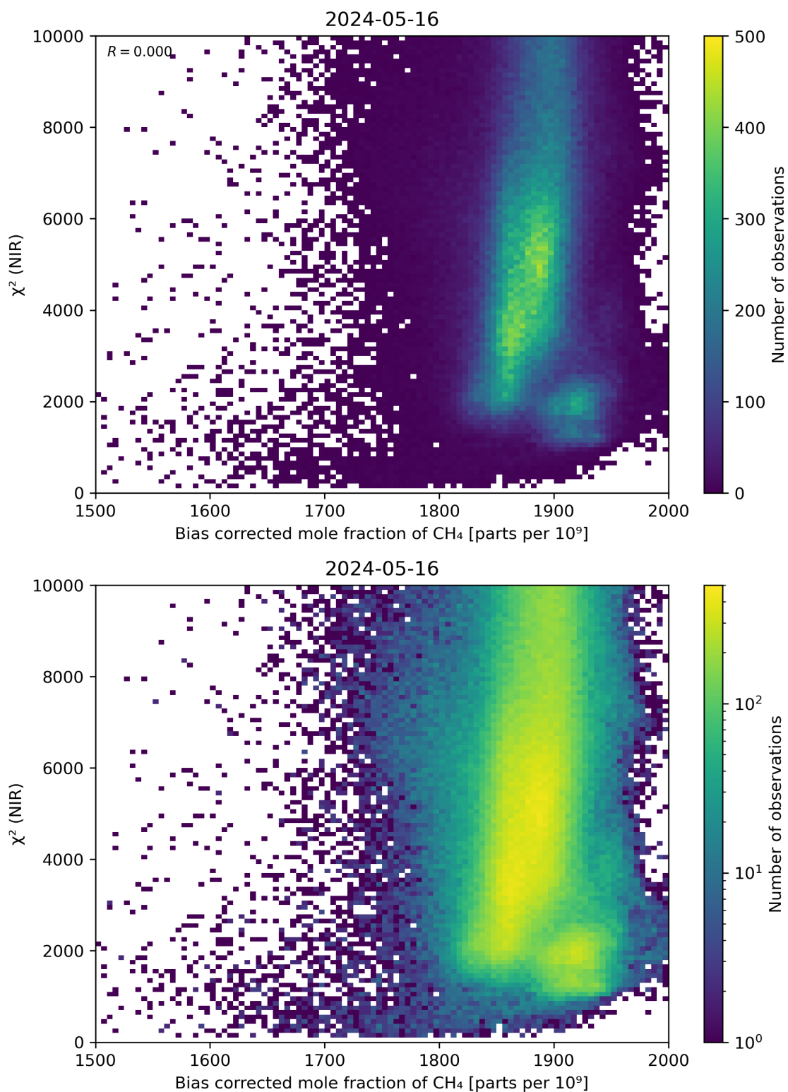
Figure 63: Scatter density plot of “Bias corrected mole fraction of CH 4 ” against “ \chi^2 (NIR)” for 2024-05-15 to 2024-05-17.
