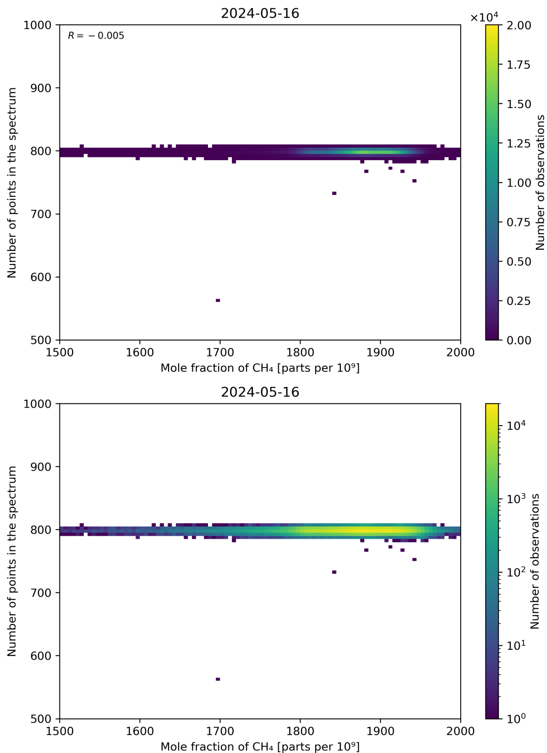
Figure 77: Scatter density plot of “Mole fraction of CH 4 ” against “Number of points in the spectrum” for 2024-05-15 to 2024-05-17.
