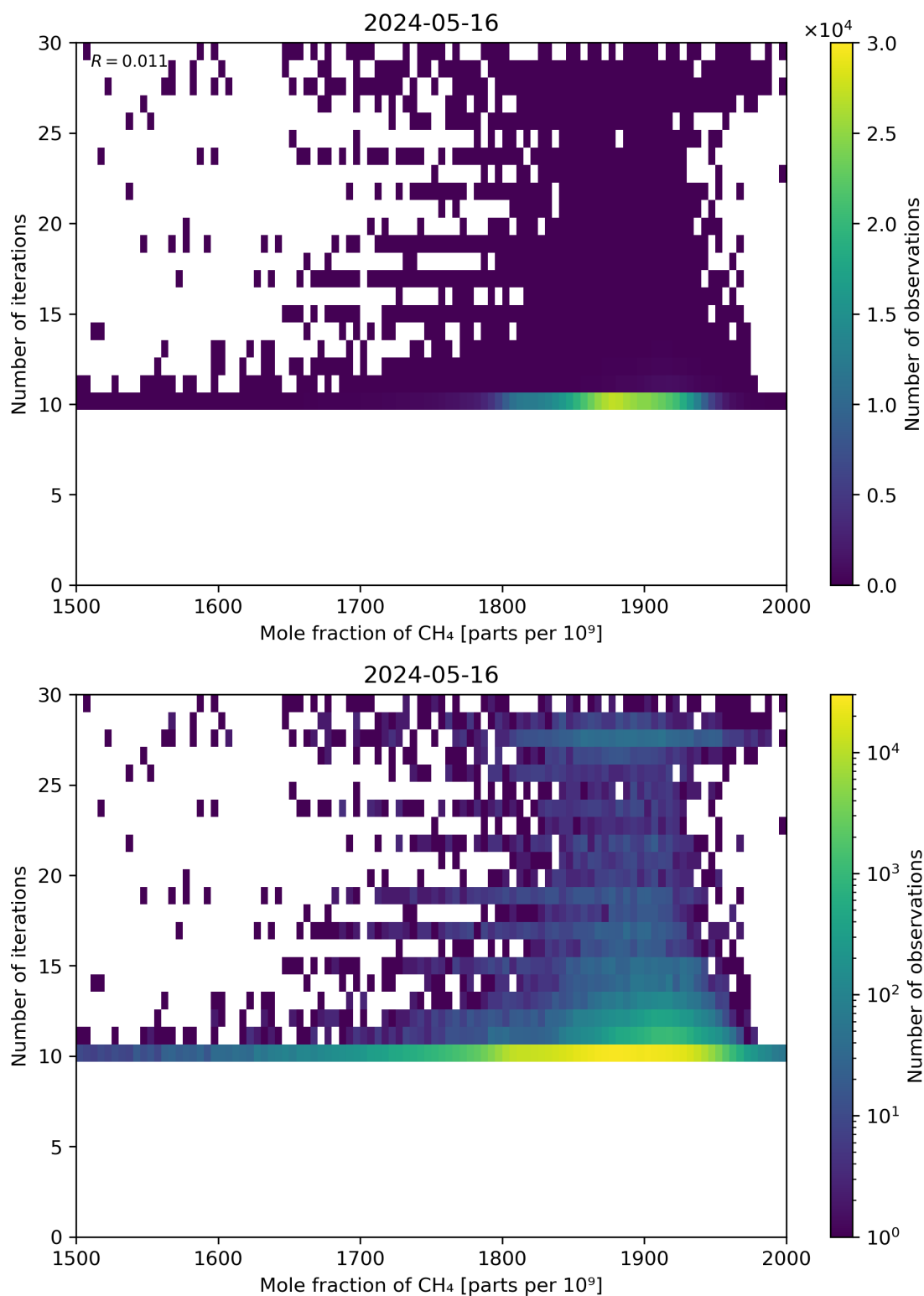
Figure 76: Scatter density plot of “Mole fraction of CH 4 ” against “Number of iterations” for 2024-05-15 to 2024-05-17.
