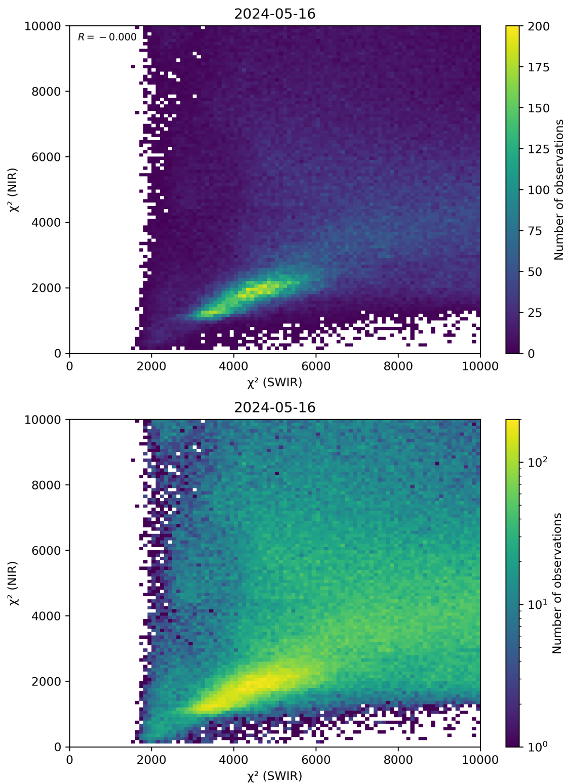
Figure 47: Scatter density plot of “ \chi^2 (SWIR)” against “ \chi^2 (NIR)” for 2024-05-15 to 2024-05-17.
