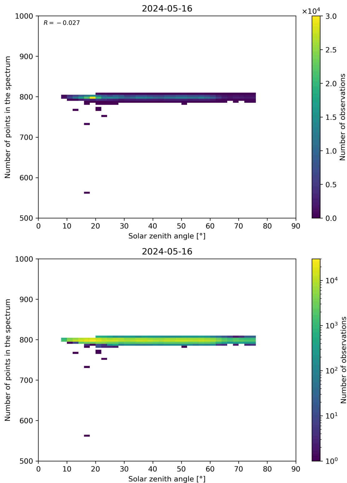
Figure 103: Scatter density plot of “Solar zenith angle” against “Number of points in the spectrum” for 2024-05-15 to 2024-05-17.
