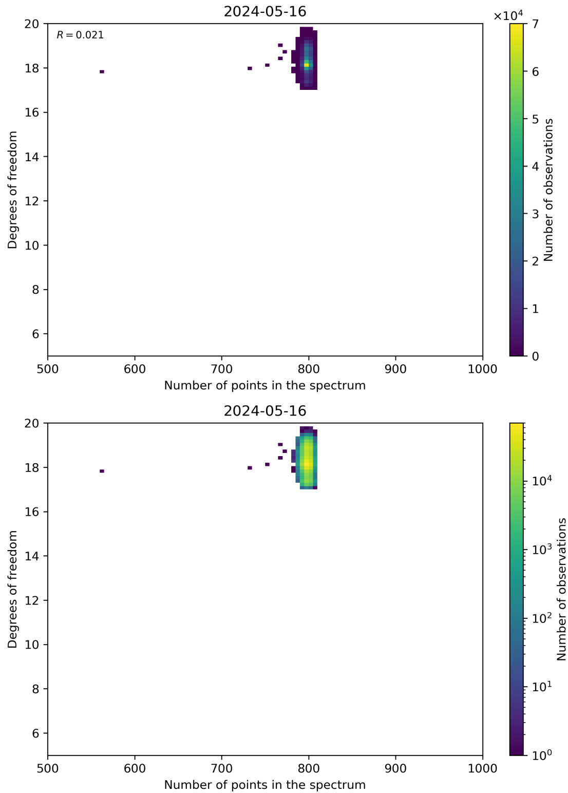
Figure 90: Scatter density plot of “Number of points in the spectrum” against “Degrees of freedom” for 2024-05-15 to 2024-05-17.
