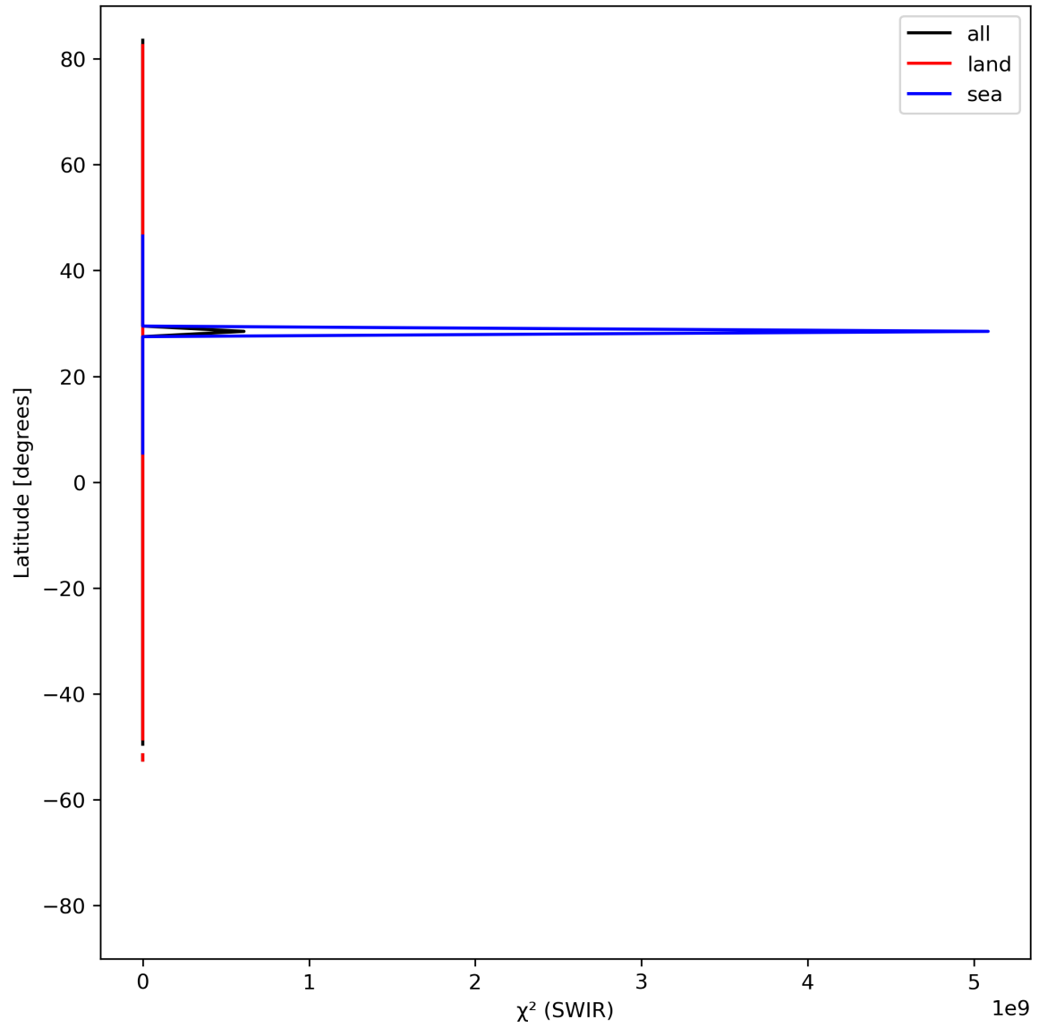
Figure 17: Zonal average of “ \chi^2 (SWIR)” for 2024-05-15 to 2024-05-17.
