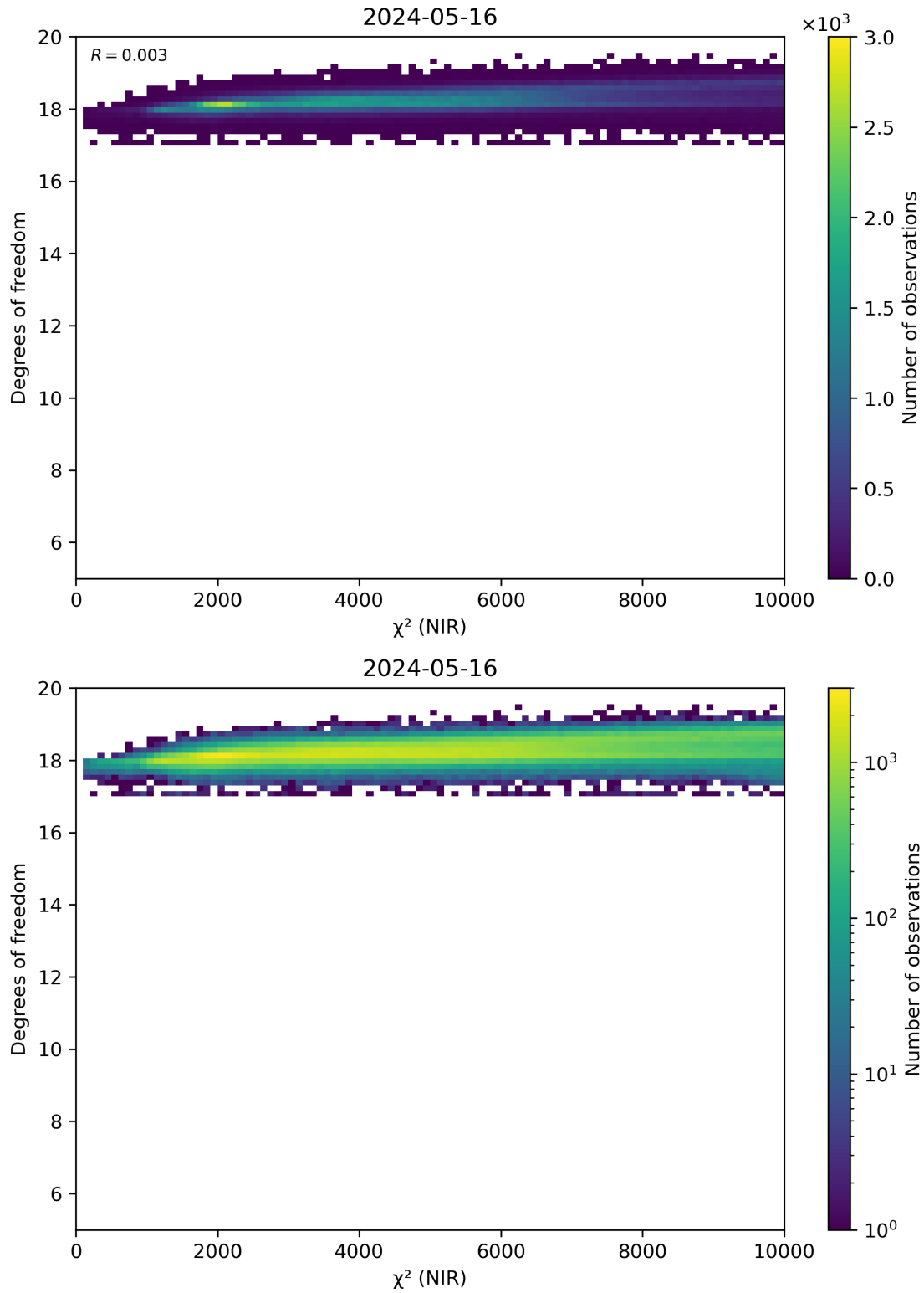
Figure 44: Scatter density plot of “ \chi^2 (NIR)” against “Degrees of freedom” for 2024-05-15 to 2024-05-17.
