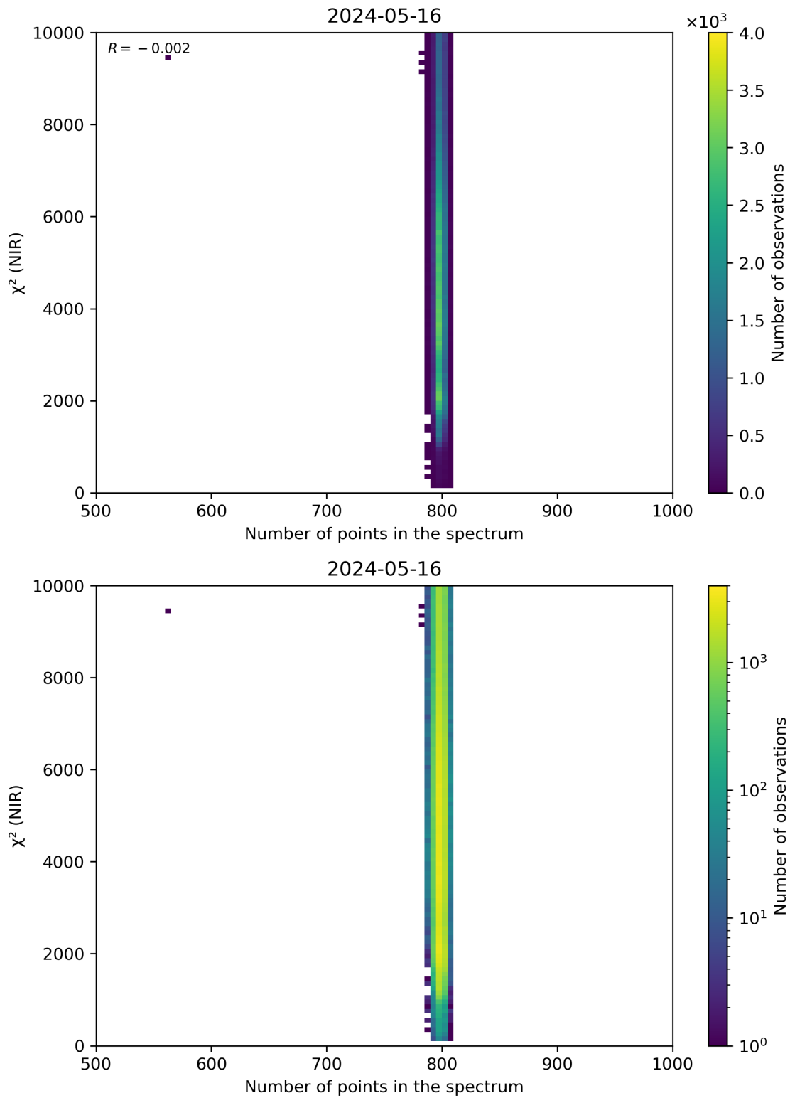
Figure 88: Scatter density plot of “Number of points in the spectrum” against “ \chi^2 (NIR)” for 2024-05-15 to 2024-05-17.
