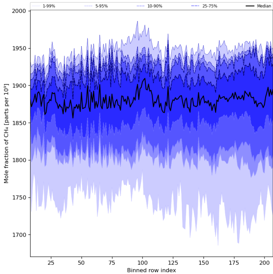
Figure 34: Along track statistics of “Mole fraction of CH 4 ” for 2024-05-15 to 2024-05-17
