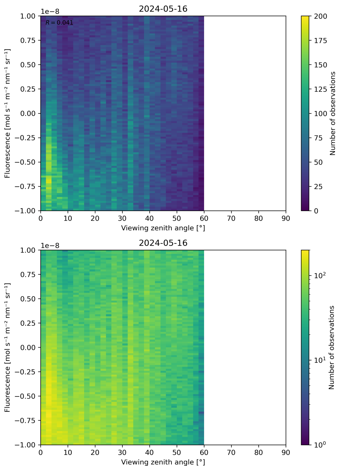
Figure 108: Scatter density plot of “Viewing zenith angle” against “Fluorescence” for 2024-05-15 to 2024-05-17.
