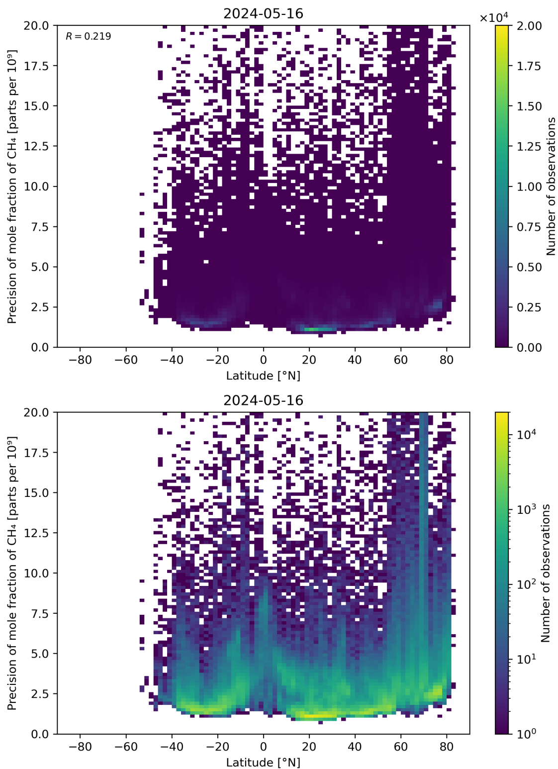
Figure 59: Scatter density plot of “Latitude” against “Precision of mole fraction of \text{CH}_4 ” for 2024-05-15 to 2024-05-17.
