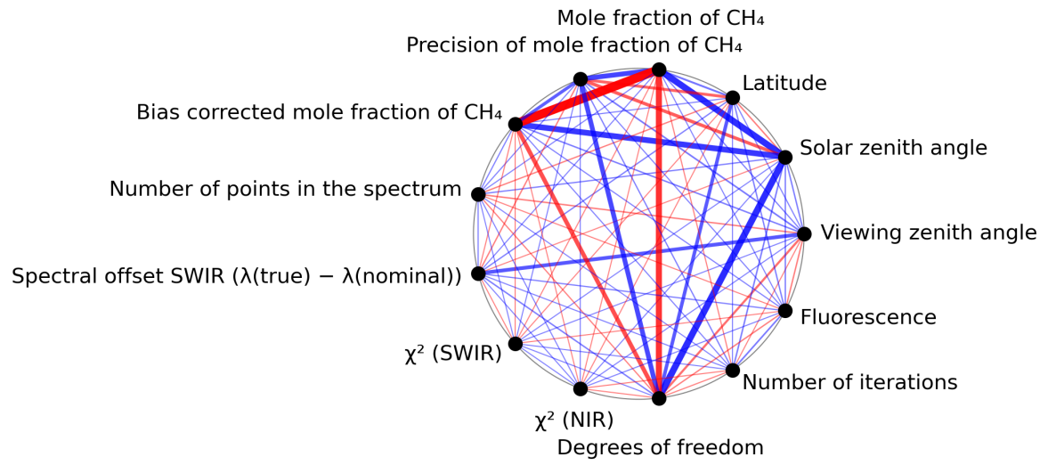
Figure 1: Map of correlation graph for 2024-05-15 to 2024-05-17.
