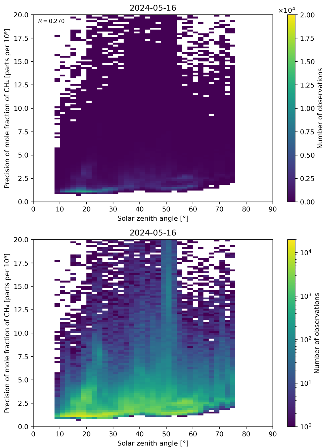
Figure 101: Scatter density plot of “Solar zenith angle” against “Precision of mole fraction of CH 4 ” for 2024-05-15 to 2024-05-17.
