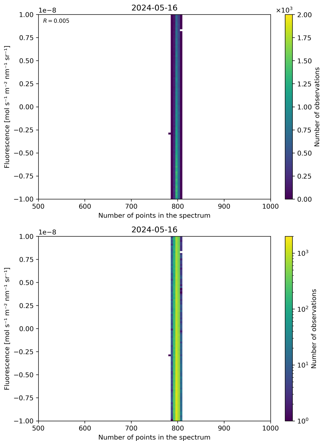
Figure 91: Scatter density plot of “Number of points in the spectrum” against “Fluorescence” for 2024-05-15 to 2024-05-17.
