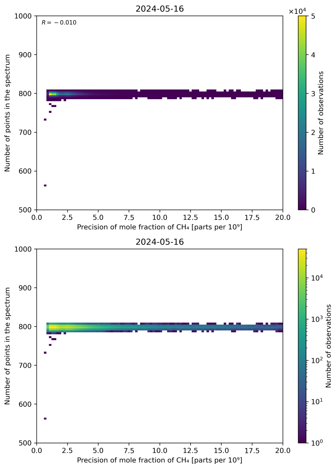
Figure 84: Scatter density plot of “Precision of mole fraction of CH 4 ” against “Number of points in the spectrum” for 2024-05-15 to 2024-05-17.
