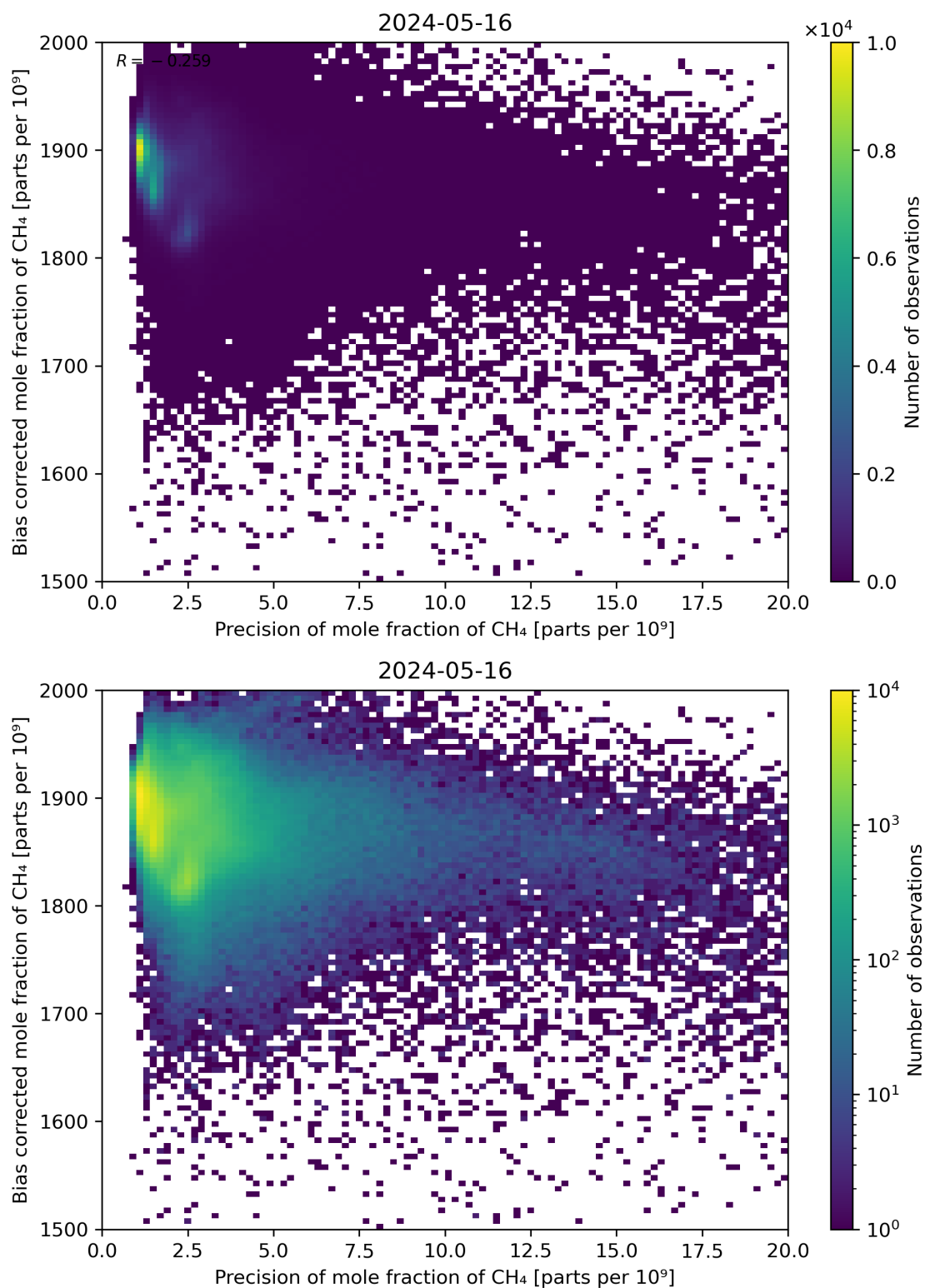
Figure 82: Scatter density plot of “Precision of mole fraction of CH 4 ” against “Bias corrected mole fraction of CH 4 ” for 2024-05-15 to 2024-05-17.
