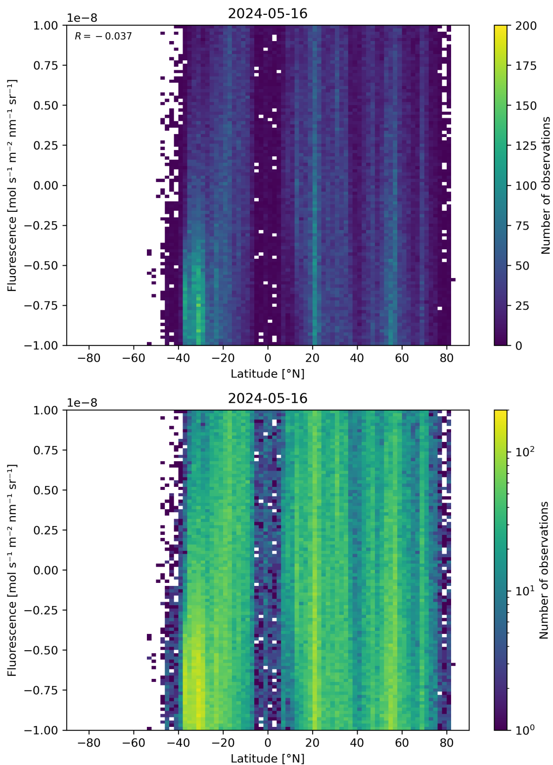
Figure 56: Scatter density plot of “Latitude” against “Fluorescence” for 2024-05-15 to 2024-05-17.
