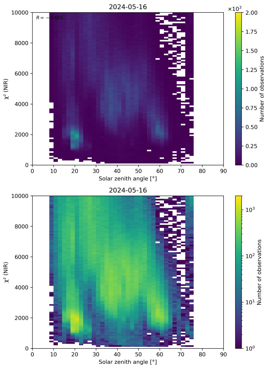
Figure 94: Scatter density plot of “Solar zenith angle” against “ \chi^2 (NIR)” for 2024-05-15 to 2024-05-17.
