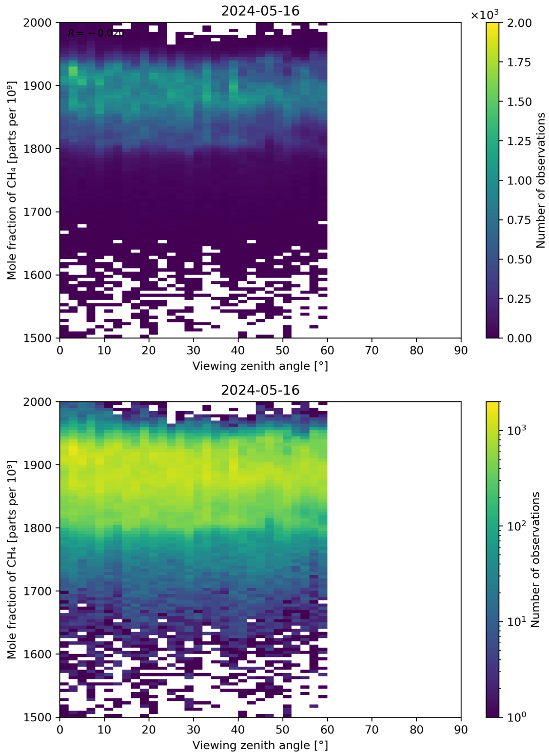
Figure 110: Scatter density plot of “Viewing zenith angle” against “Mole fraction of CH 4 ” for 2024-05-15 to 2024-05-17.
