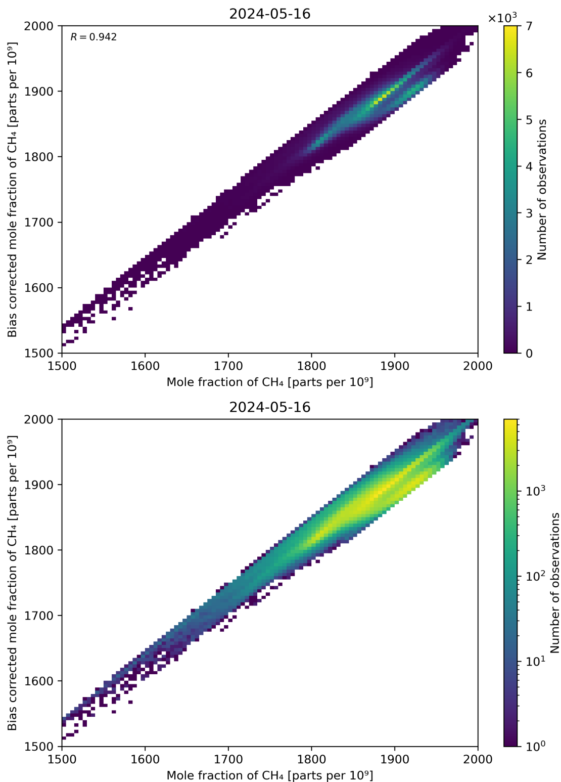
Figure 74: Scatter density plot of “Mole fraction of CH 4 ” against “Bias corrected mole fraction of CH 4 ” for 2024-05-15 to 2024-05-17.
