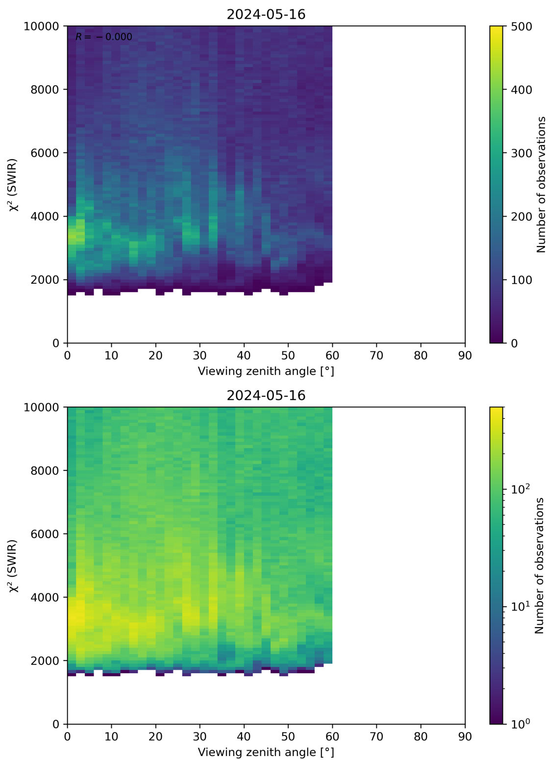
Figure 106: Scatter density plot of “Viewing zenith angle” against “ \chi^2 (SWIR)” for 2024-05-15 to 2024-05-17.
