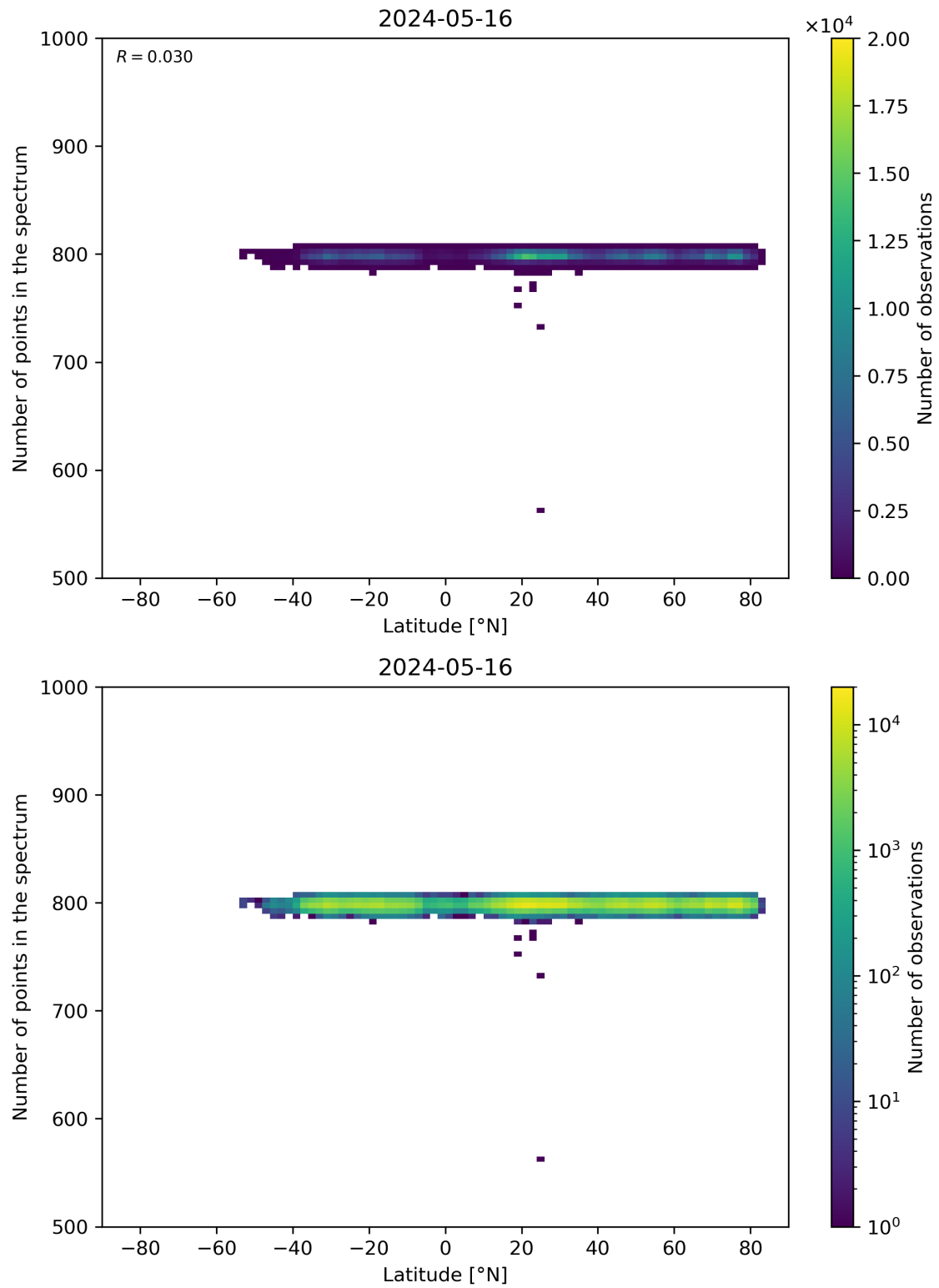
Figure 61: Scatter density plot of “Latitude” against “Number of points in the spectrum” for 2024-05-15 to 2024-05-17.
