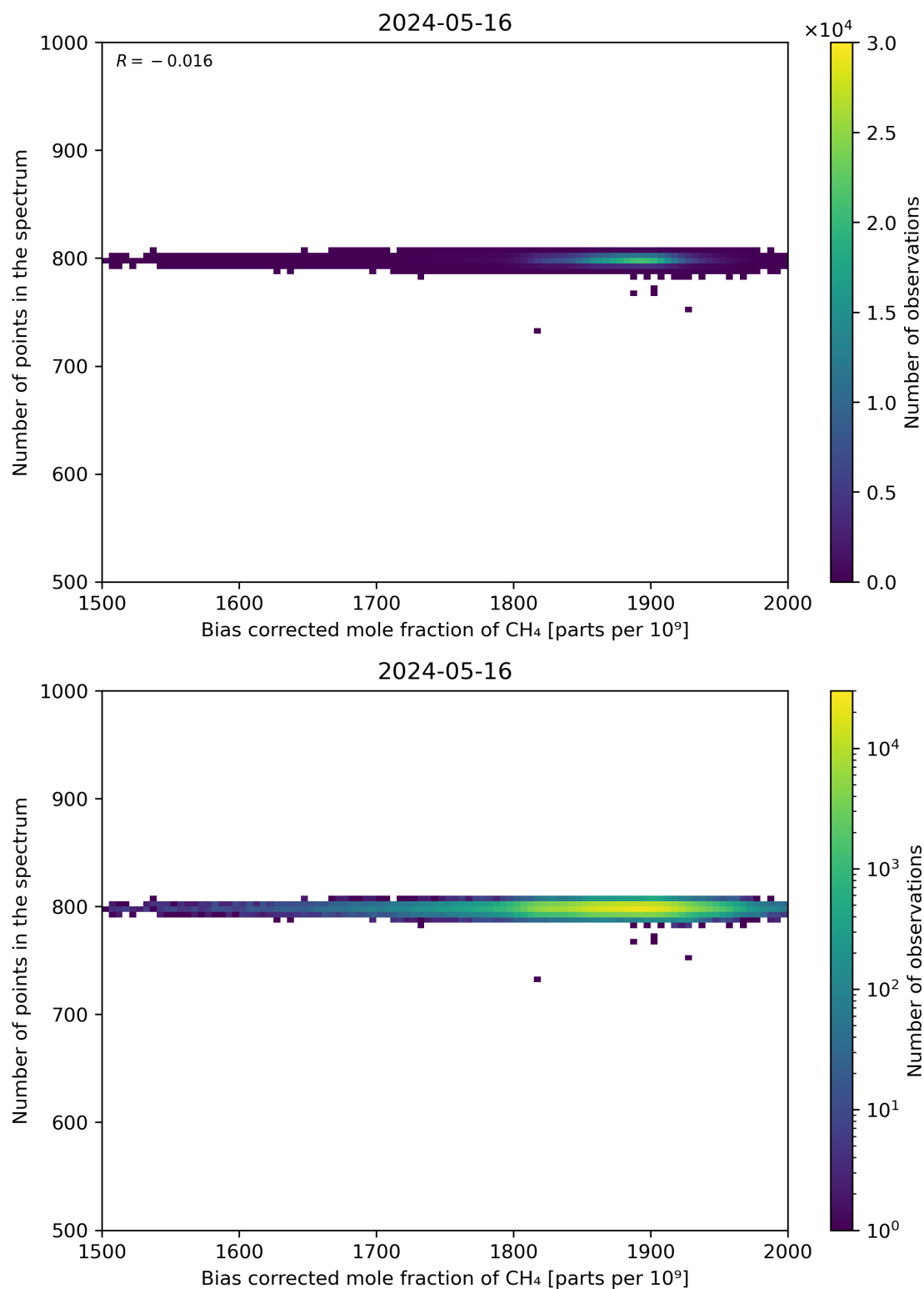
Figure 68: Scatter density plot of “Bias corrected mole fraction of CH 4 ” against “Number of points in the spectrum” for 2024-05-15 to 2024-05-17.
