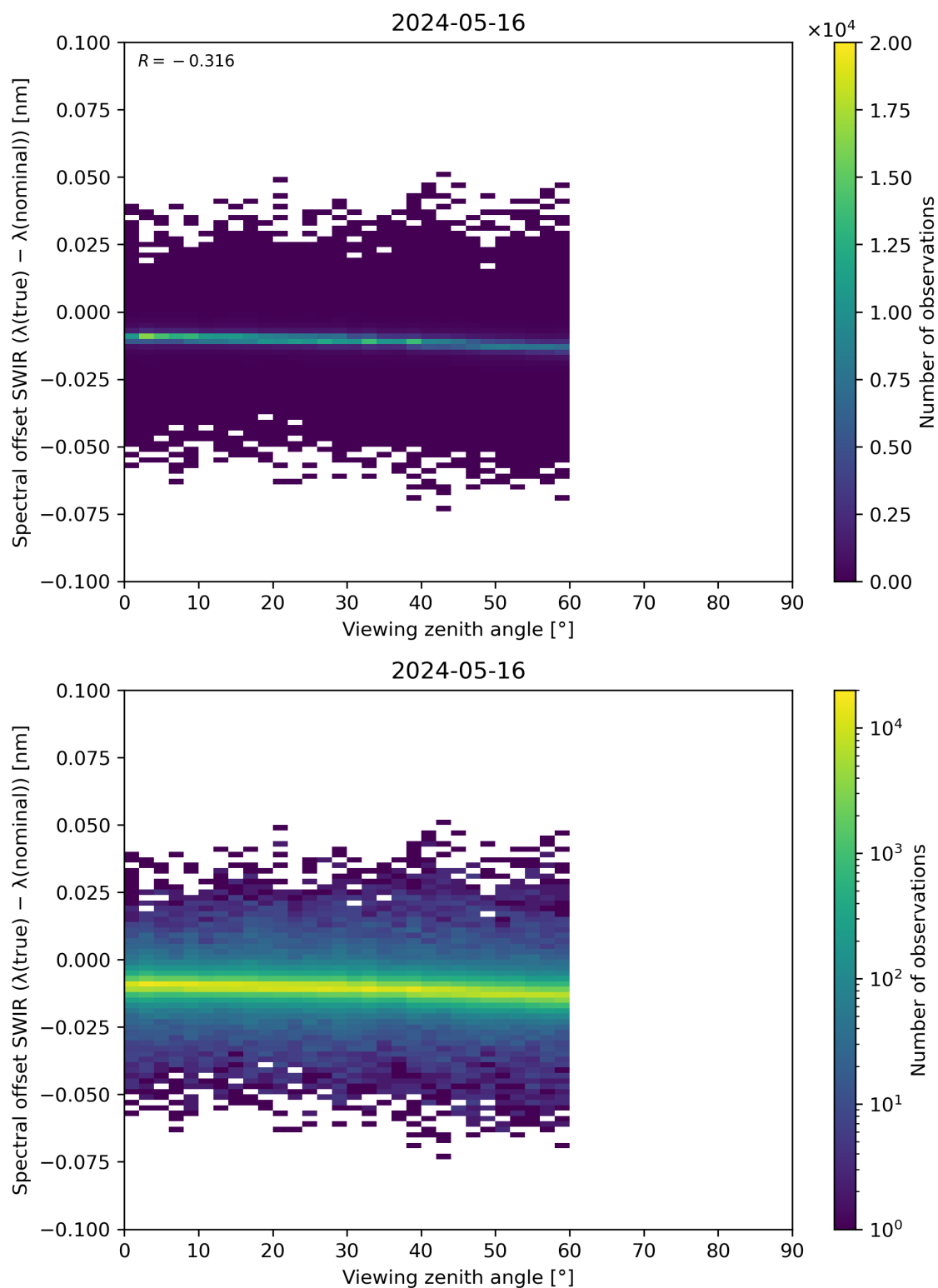
Figure 116: Scatter density plot of “Viewing zenith angle” against “Spectral offset SWIR ( \lambda(\text{true}) - \lambda(\text{nominal}) )” for 2024-05-15 to 2024-05-17.
