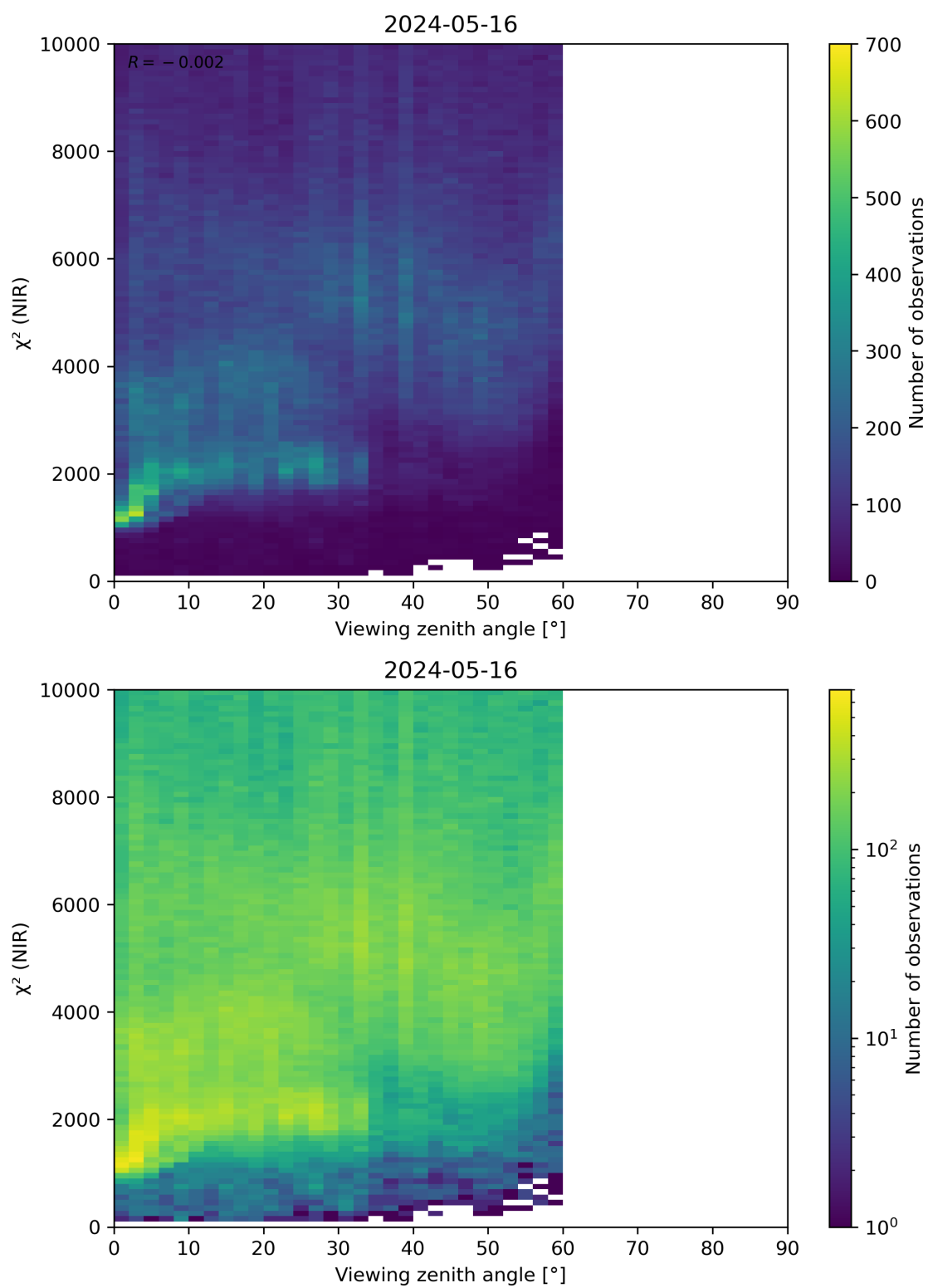
Figure 105: Scatter density plot of “Viewing zenith angle” against “ \chi^2 (NIR)” for 2024-05-15 to 2024-05-17.
