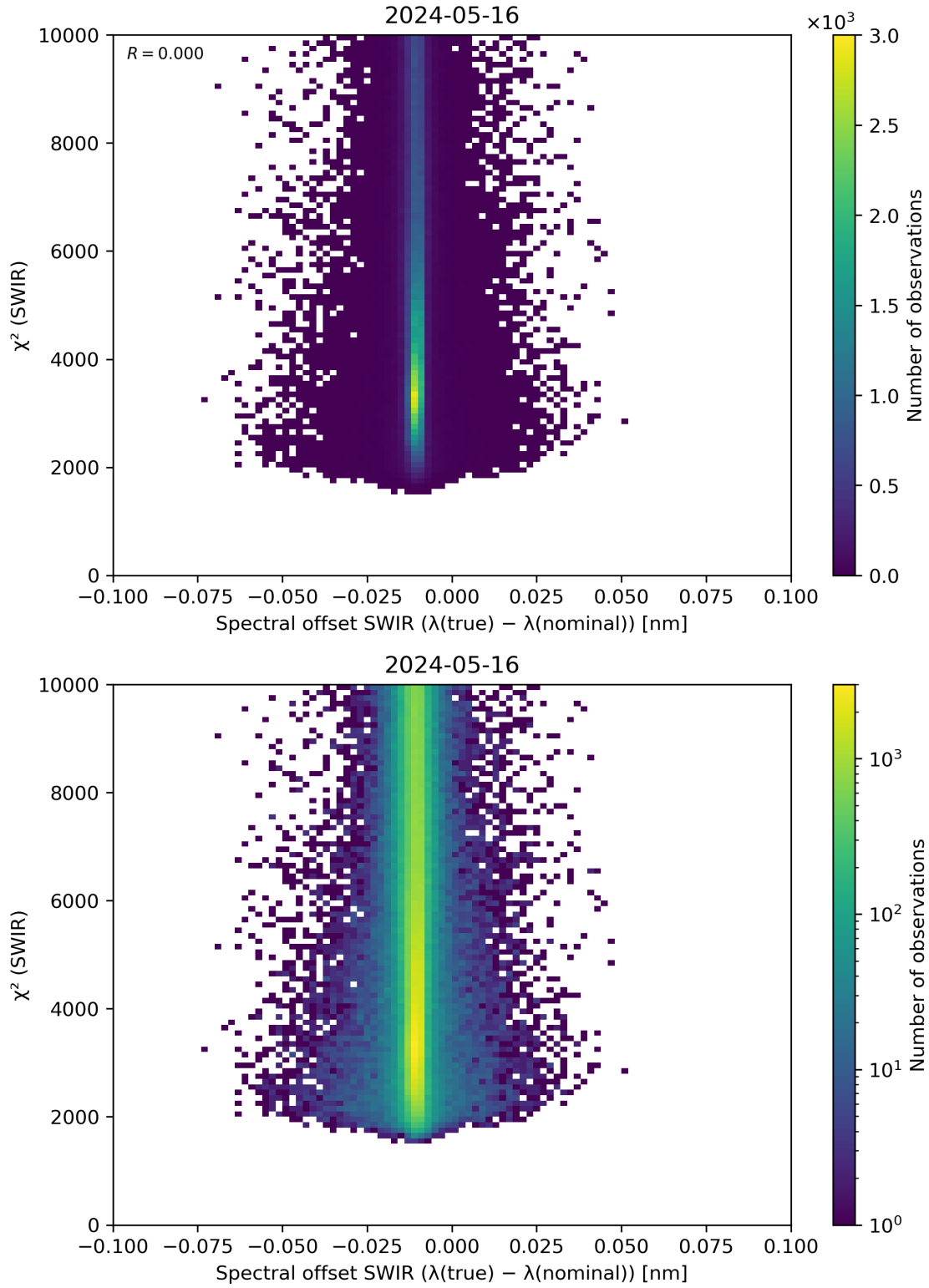
Figure 118: Scatter density plot of “Spectral offset SWIR ( \lambda(\text{true}) - \lambda(\text{nominal}) )” against “ \chi^2 (SWIR)” for 2024-05-15 to 2024-05-17.
