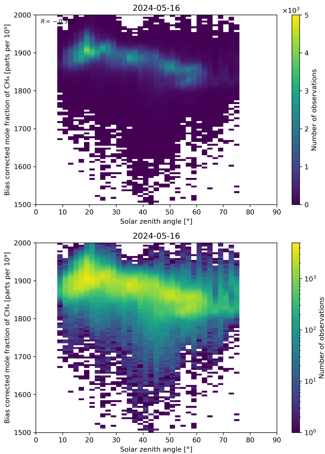
Figure 100: Scatter density plot of “Solar zenith angle” against “Bias corrected mole fraction of \text{CH}_4 ” for 2024-05-15 to 2024-05-17.
