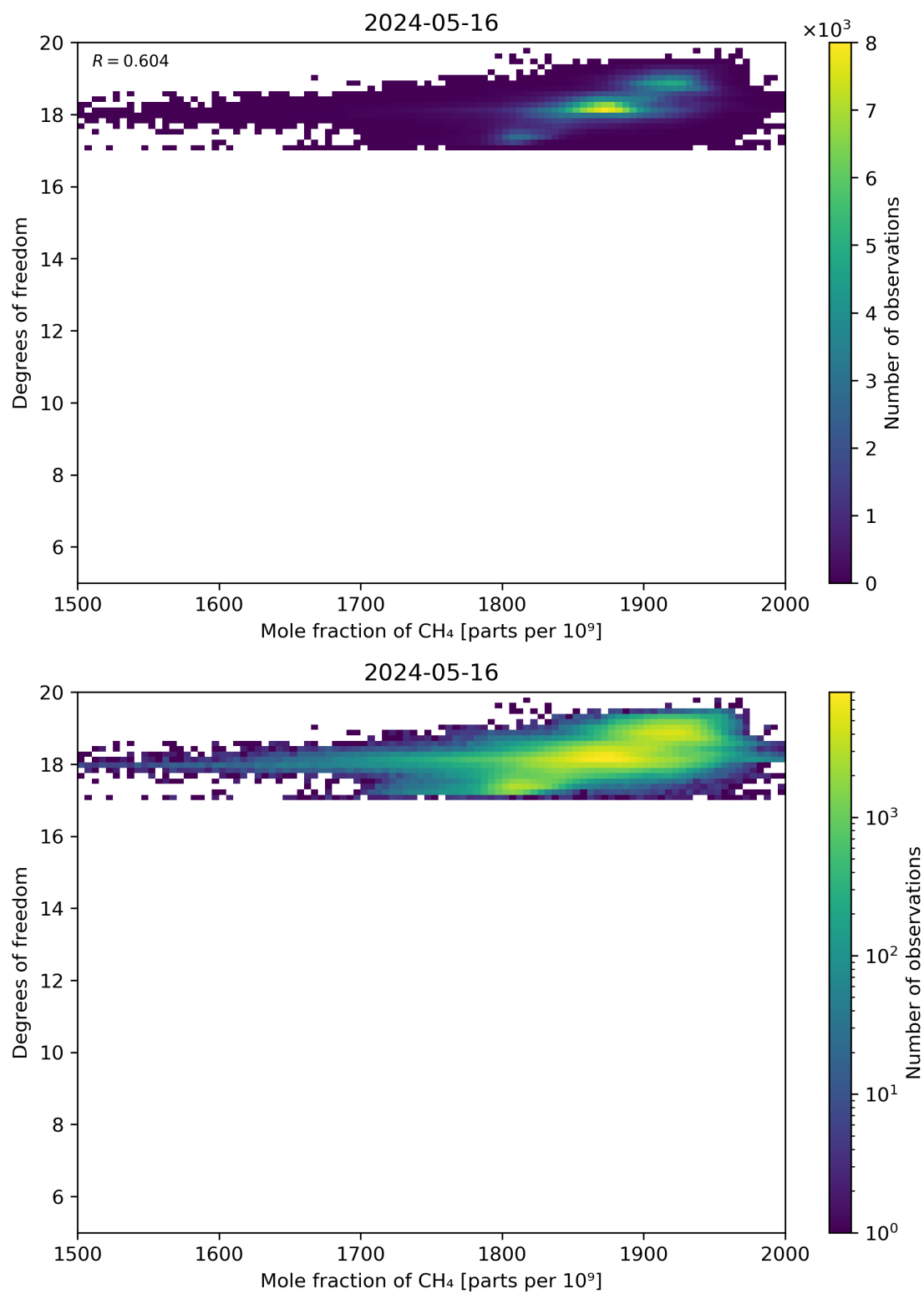
Figure 72: Scatter density plot of “Mole fraction of CH 4 ” against “Degrees of freedom” for 2024-05-15 to 2024-05-17.
