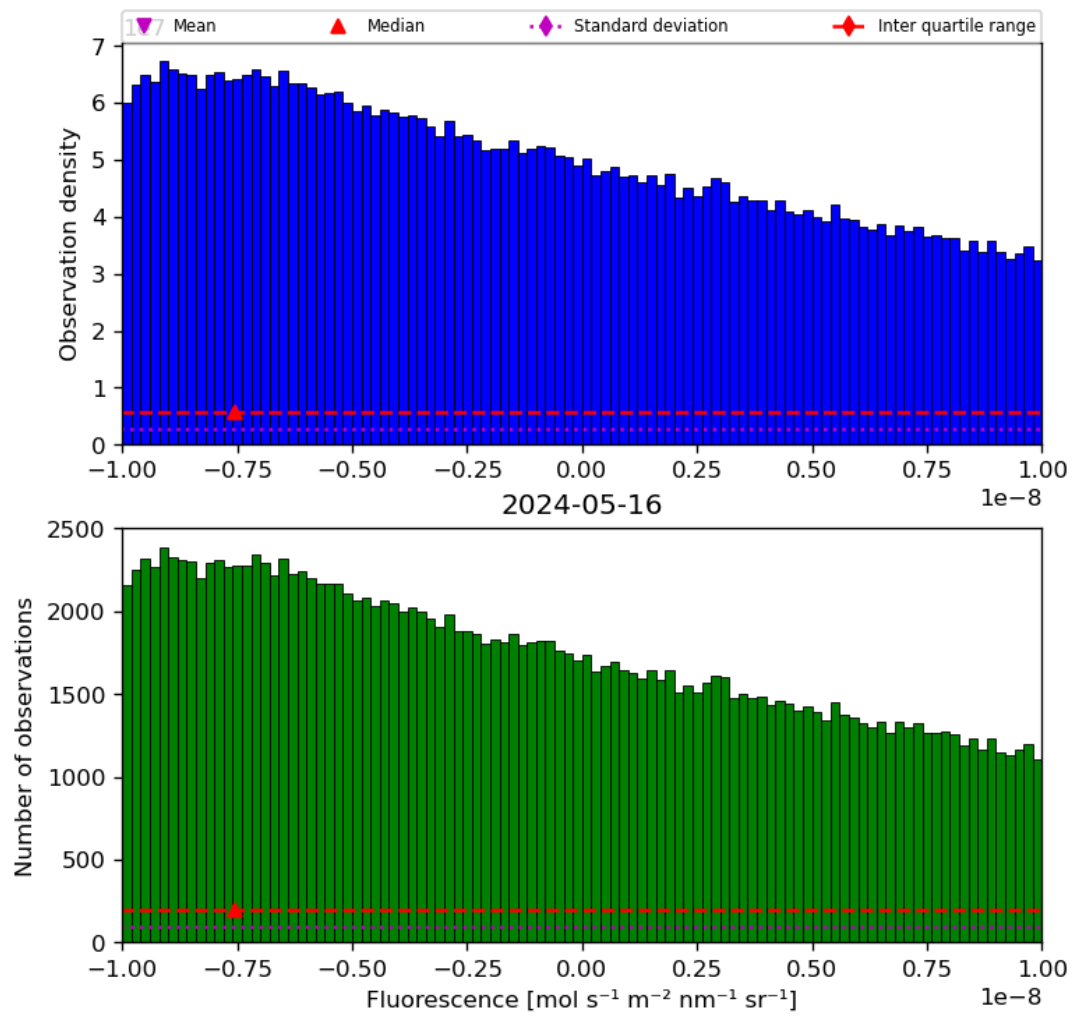
Figure 32: Histogram of “Fluorescence” for 2024-05-15 to 2024-05-17
