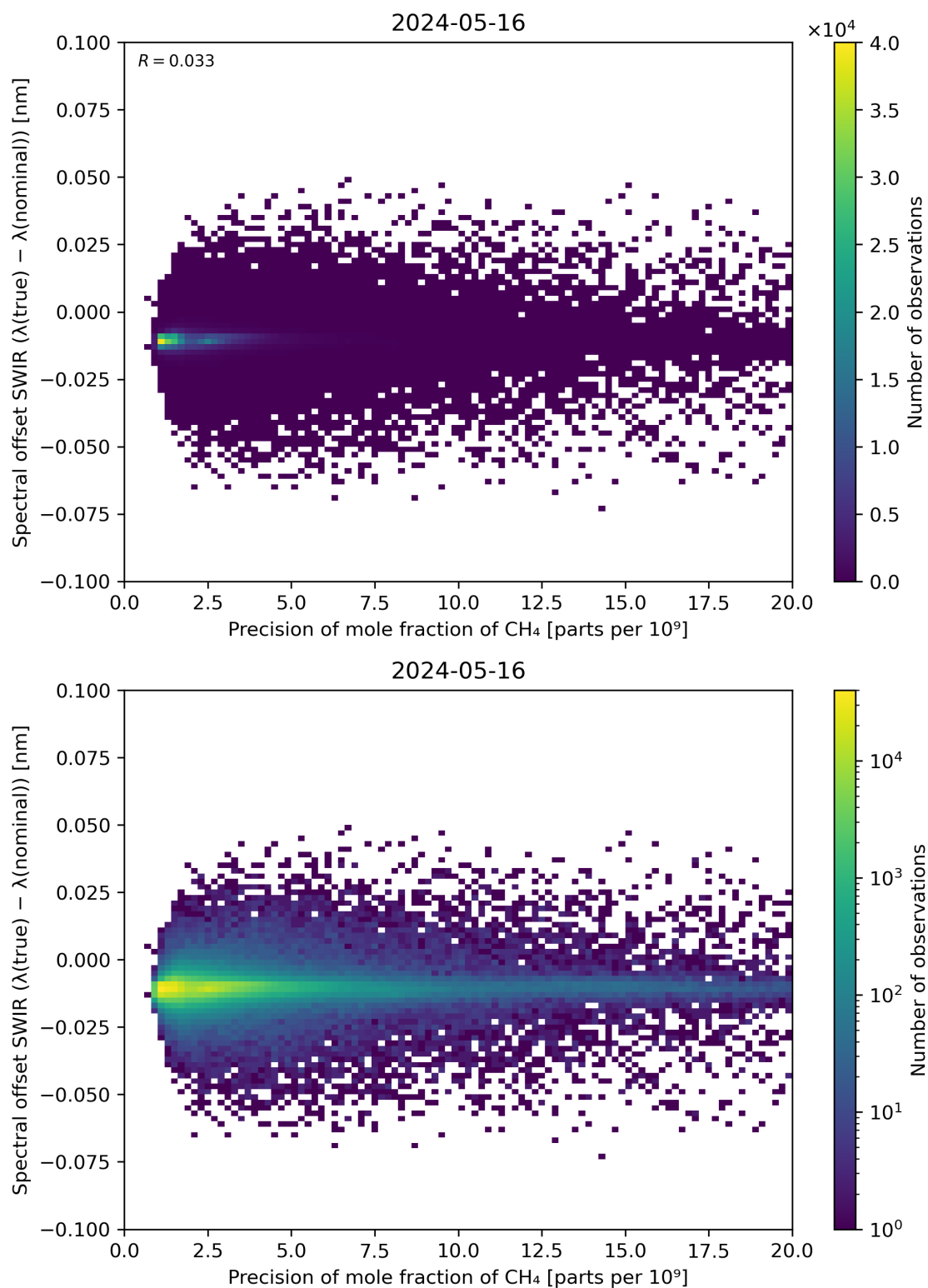
Figure 85: Scatter density plot of “Precision of mole fraction of \text{CH}_4 ” against “Spectral offset SWIR ( \lambda(\text{true}) - \lambda(\text{nominal}) )” for 2024-05-15 to 2024-05-17.
