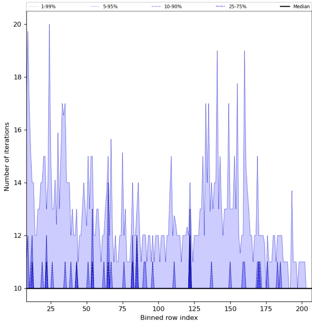
Figure 42: Along track statistics of “Number of iterations” for 2024-05-15 to 2024-05-17
