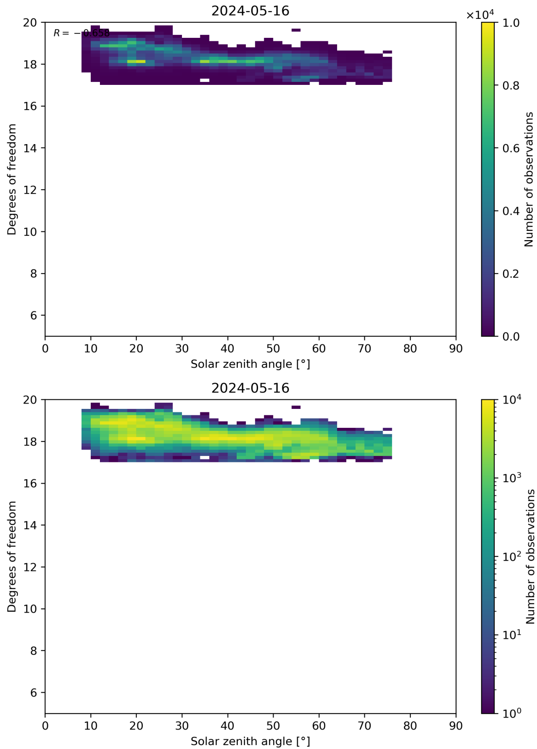
Figure 96: Scatter density plot of “Solar zenith angle” against “Degrees of freedom” for 2024-05-15 to 2024-05-17.
