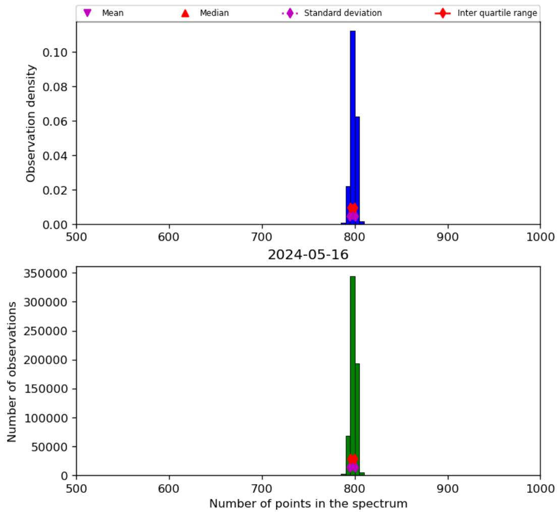
Figure 26: Histogram of “Number of points in the spectrum” for 2024-05-15 to 2024-05-17
