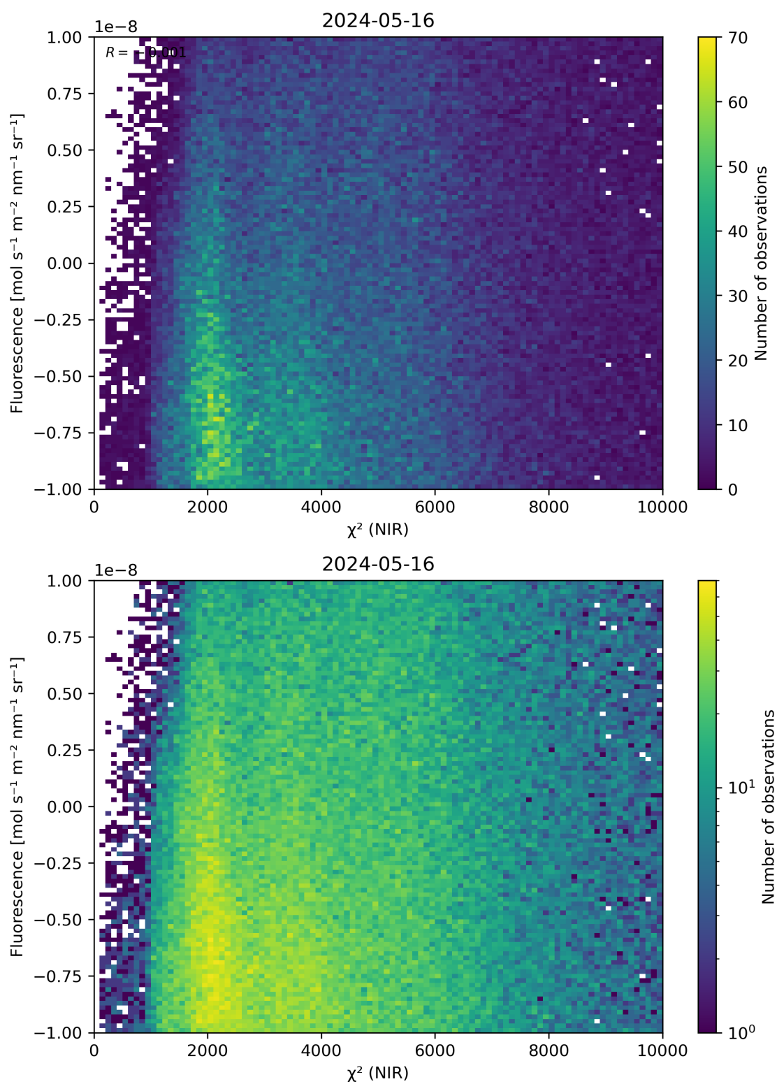
Figure 45: Scatter density plot of “ \chi^2 (NIR)” against “Fluorescence” for 2024-05-15 to 2024-05-17.
