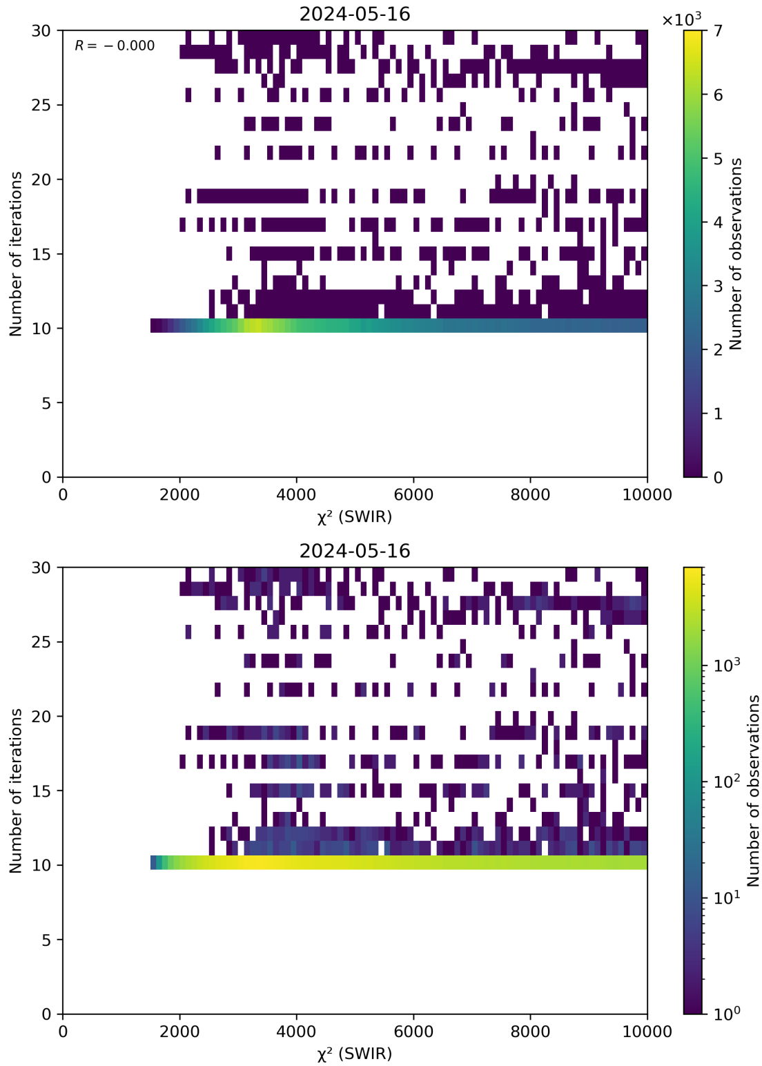
Figure 50: Scatter density plot of “ \chi^2 (SWIR)” against “Number of iterations” for 2024-05-15 to 2024-05-17.
