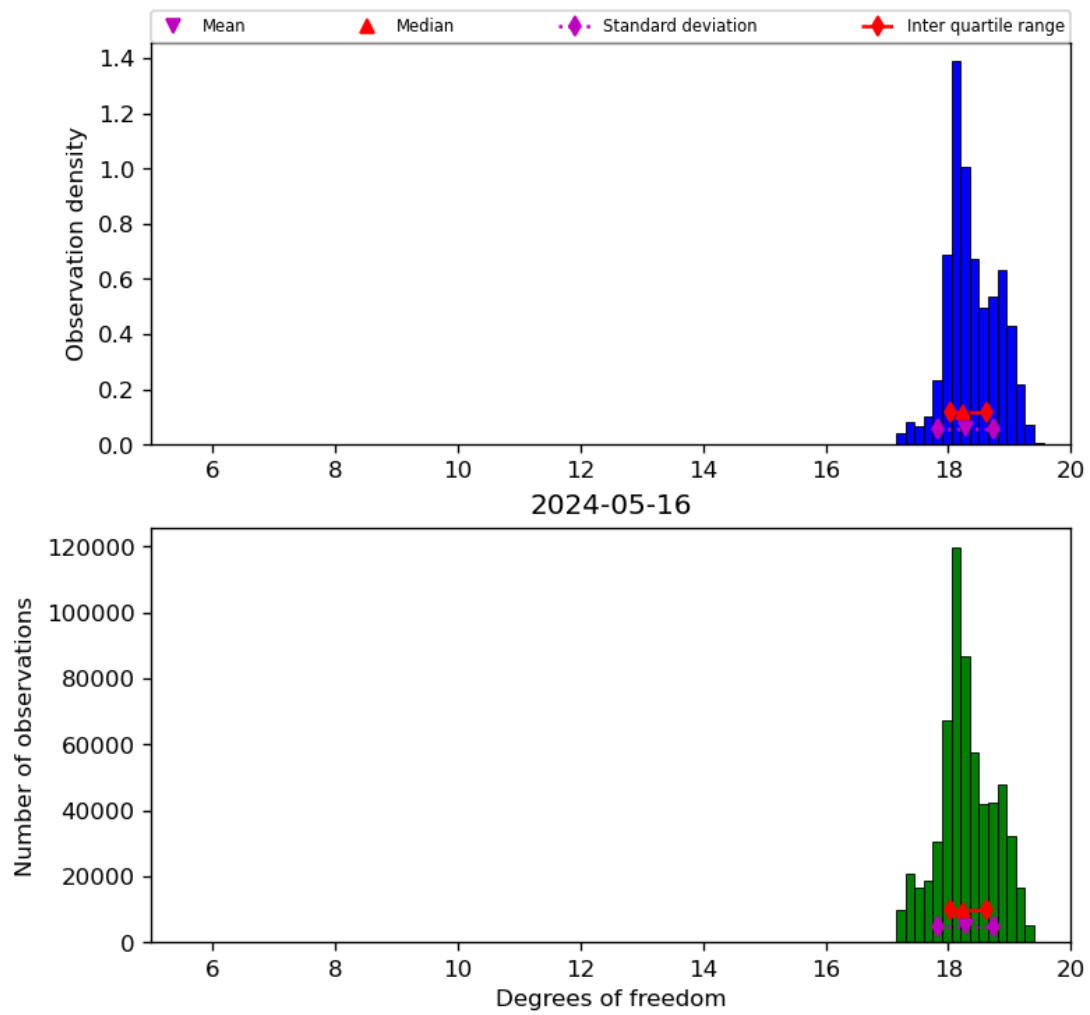
Figure 30: Histogram of “Degrees of freedom” for 2024-05-15 to 2024-05-17
