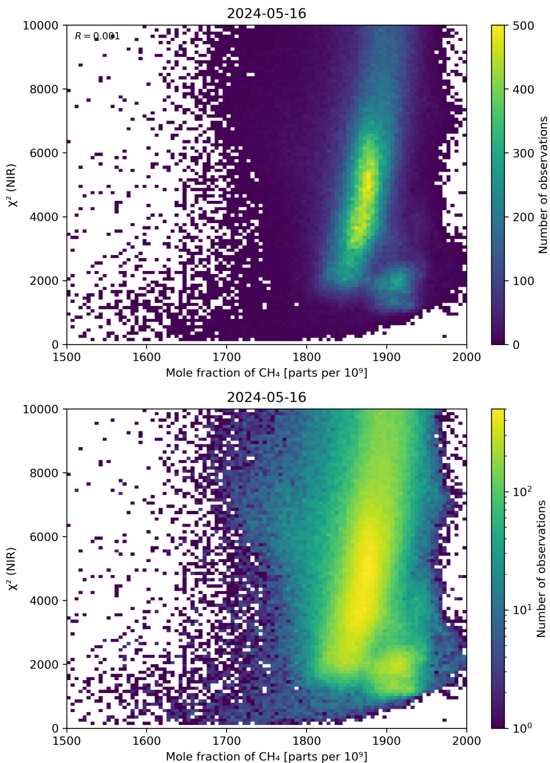
Figure 70: Scatter density plot of “Mole fraction of CH 4 ” against “ \chi^2 (NIR)” for 2024-05-15 to 2024-05-17.
