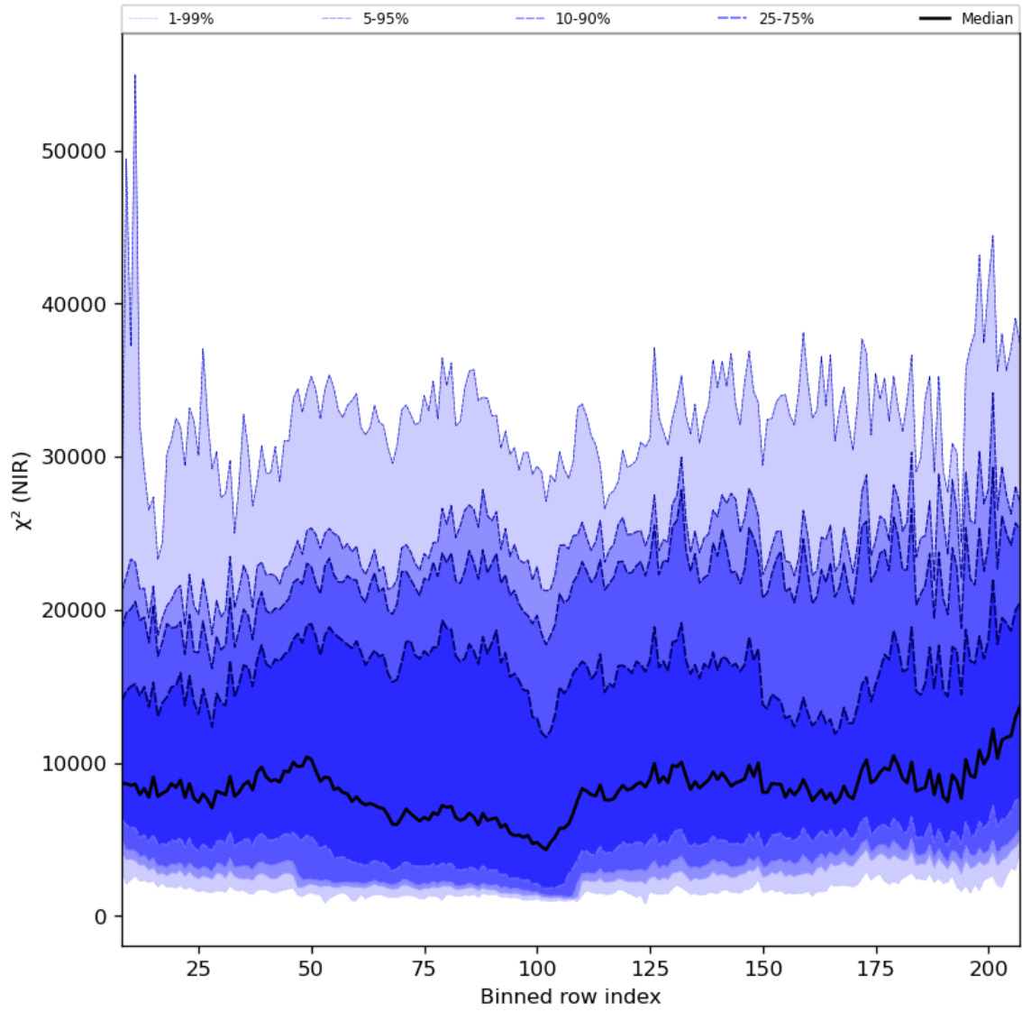
Figure 40: Along track statistics of “ \chi^2 (NIR)” for 2024-05-15 to 2024-05-17
