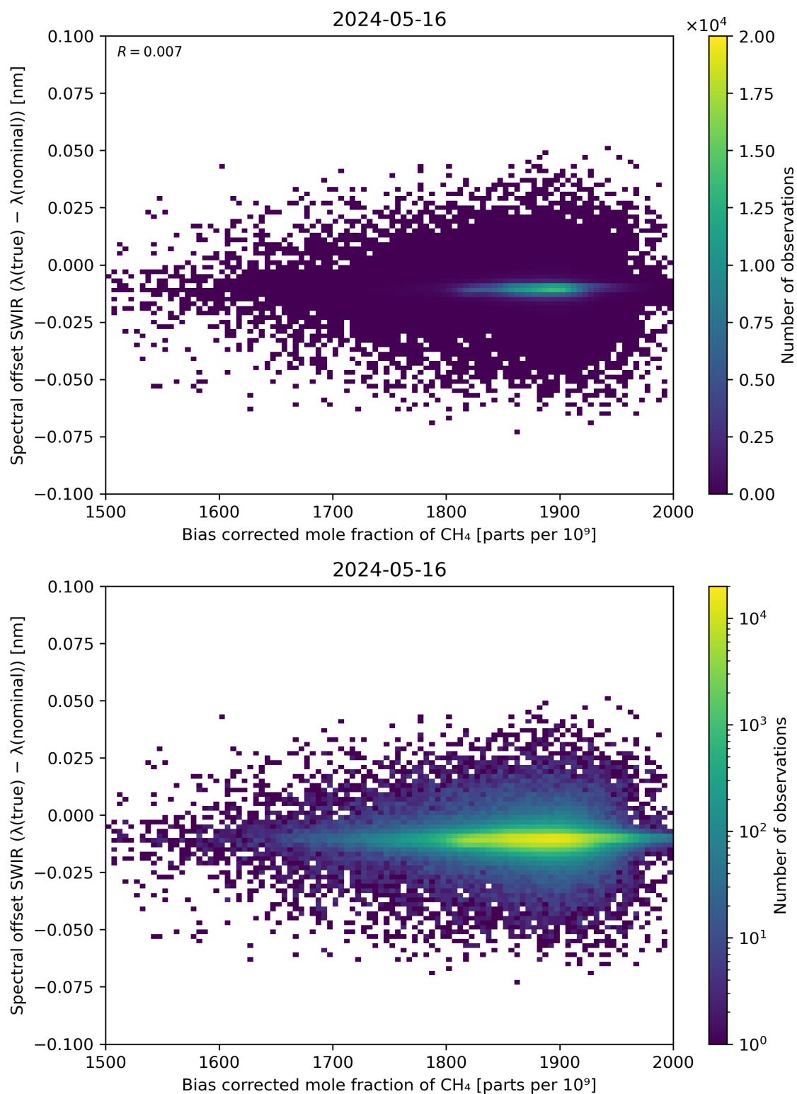
Figure 69: Scatter density plot of “Bias corrected mole fraction of \text{CH}_4 ” against “Spectral offset SWIR ( \lambda(\text{true}) - \lambda(\text{nominal}) )” for 2024-05-15 to 2024-05-17.
