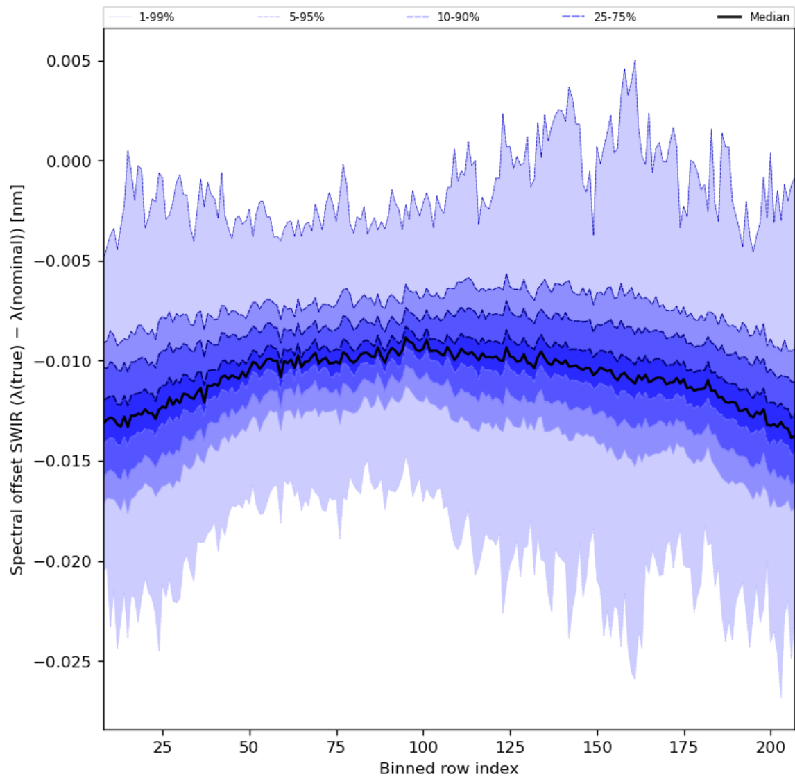
Figure 38: Along track statistics of “Spectral offset SWIR ( \lambda(\text{true}) - \lambda(\text{nominal}) )” for 2024-05-15 to 2024-05-17
