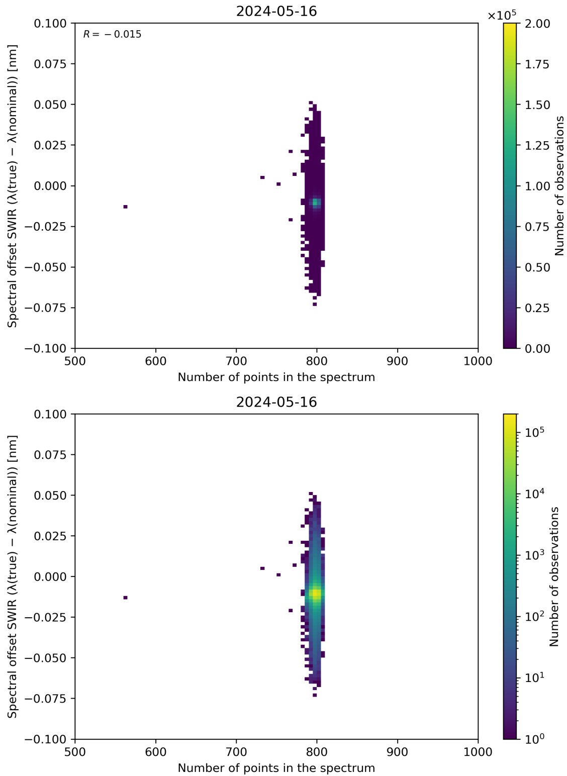
Figure 93: Scatter density plot of “Number of points in the spectrum” against “Spectral offset SWIR ( \lambda(\text{true}) - \lambda(\text{nominal}) )” for 2024-05-15 to 2024-05-17.
