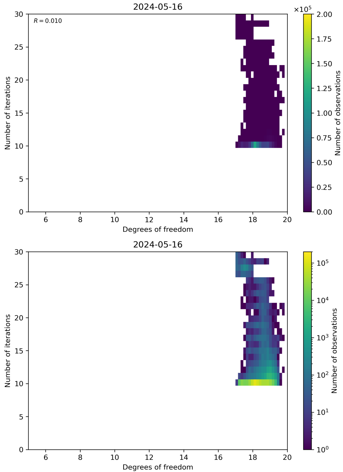
Figure 52: Scatter density plot of “Degrees of freedom” against “Number of iterations” for 2024-05-15 to 2024-05-17.
