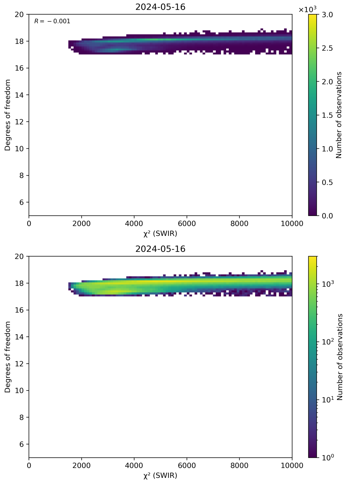
Figure 48: Scatter density plot of “ \chi^2 (SWIR)” against “Degrees of freedom” for 2024-05-15 to 2024-05-17.
