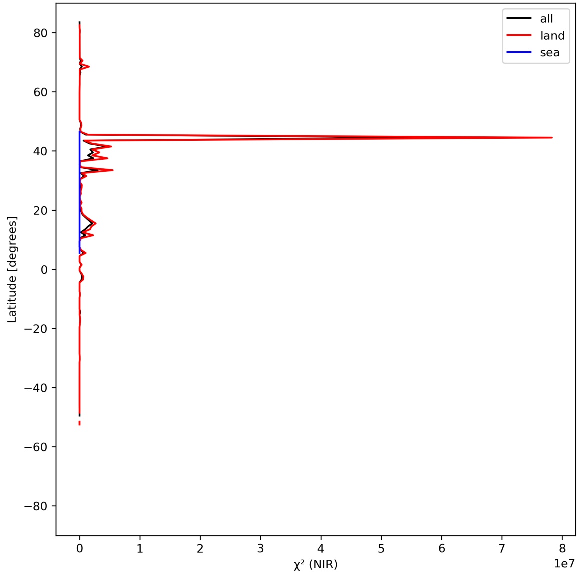
Figure 18: Zonal average of “ \chi^2 (NIR)” for 2024-05-15 to 2024-05-17.
