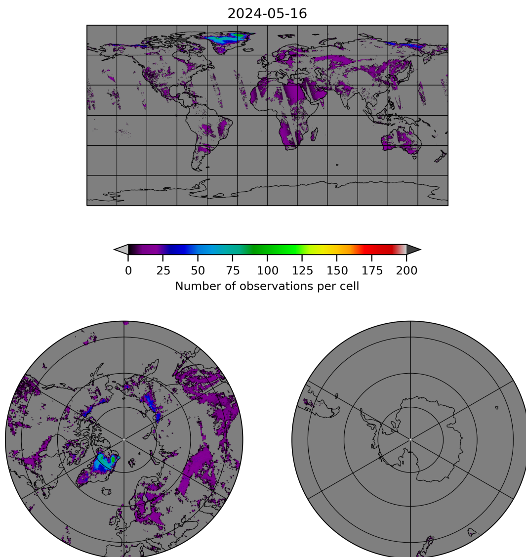
Figure 10: Map of the number of observations for 2024-05-15 to 2024-05-17
