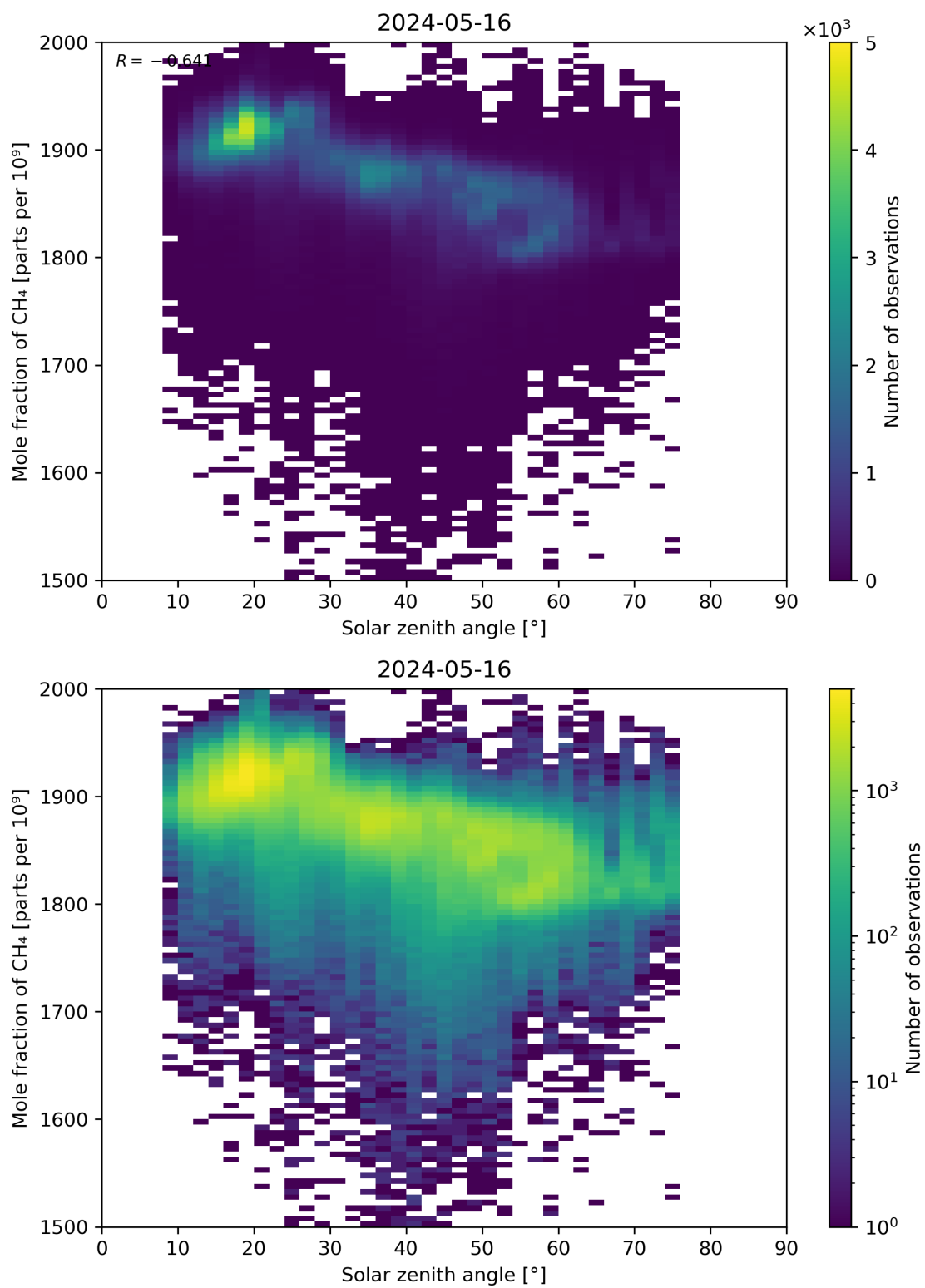
Figure 99: Scatter density plot of “Solar zenith angle” against “Mole fraction of CH 4 ” for 2024-05-15 to 2024-05-17.
