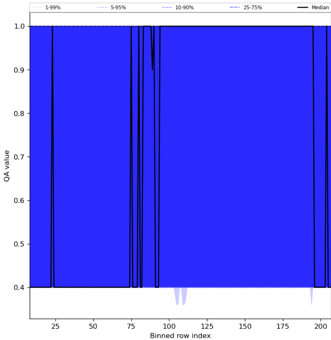
Figure 33: Along track statistics of “QA value” for 2024-05-15 to 2024-05-17
