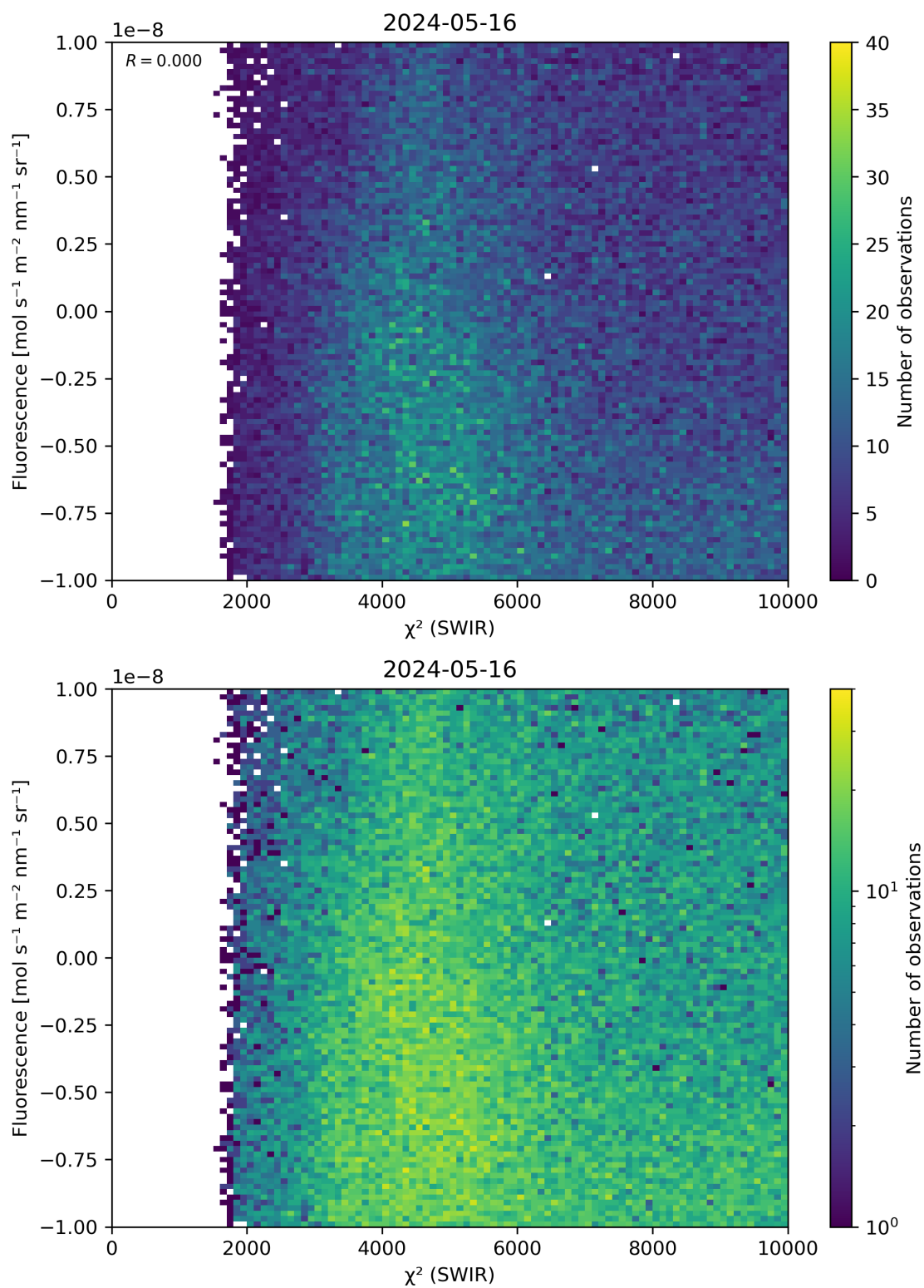
Figure 49: Scatter density plot of “ \chi^2 (SWIR)” against “Fluorescence” for 2024-05-15 to 2024-05-17.
