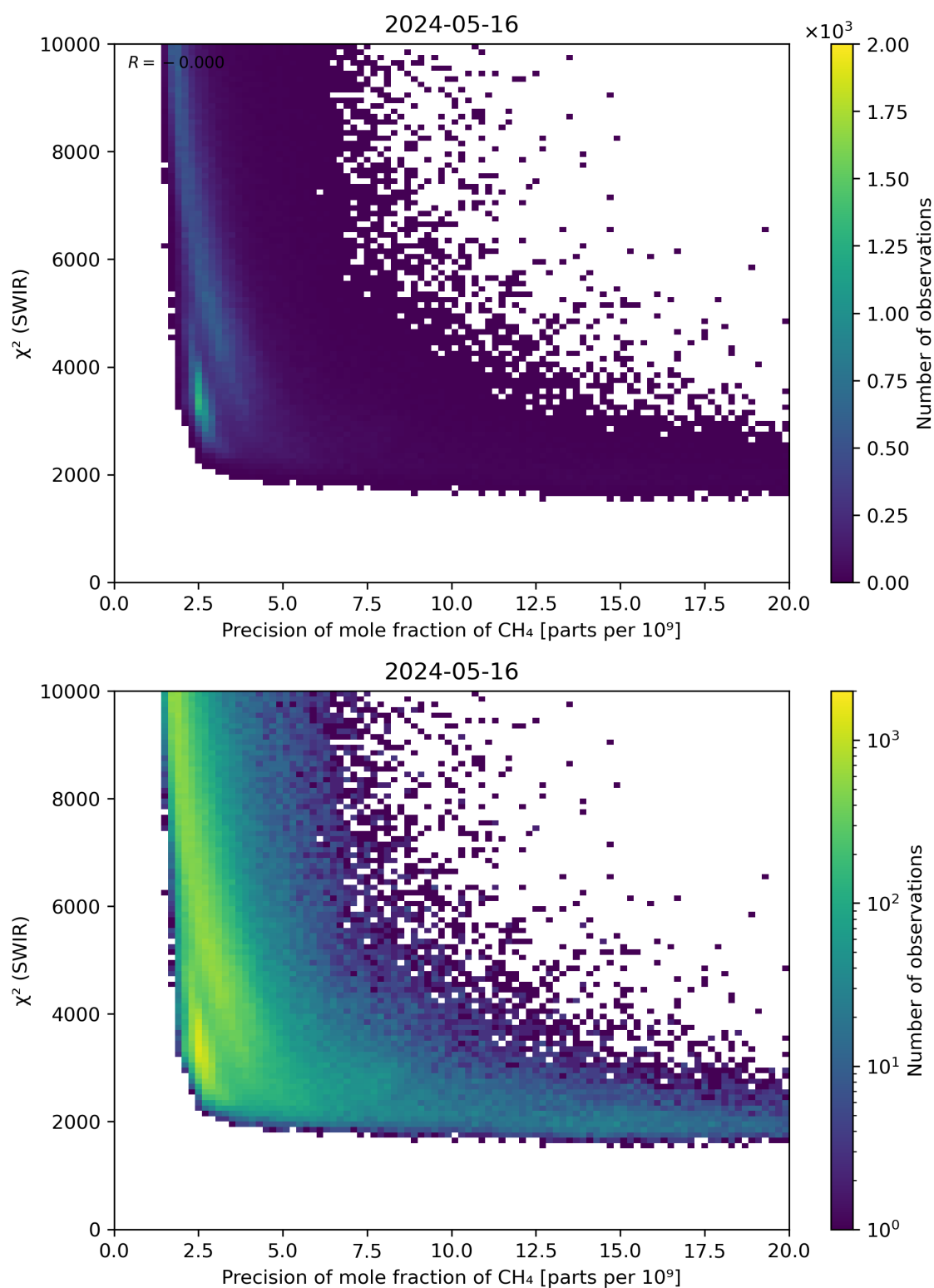
Figure 79: Scatter density plot of “Precision of mole fraction of \text{CH}_4 ” against “ \chi^2 (SWIR)” for 2024-05-15 to 2024-05-17.
