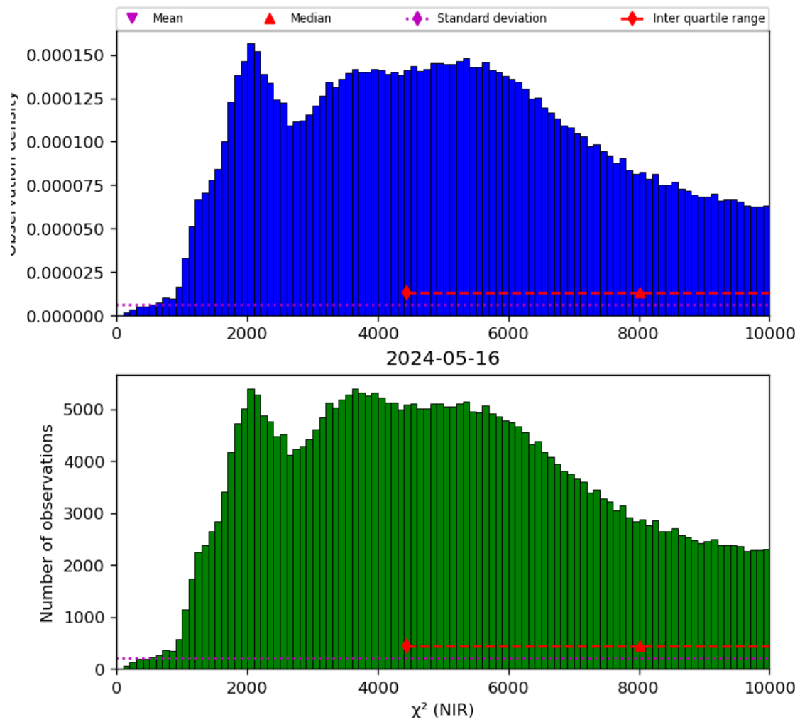
Figure 29: Histogram of " \chi^2 (NIR)" for 2024-05-15 to 2024-05-17
