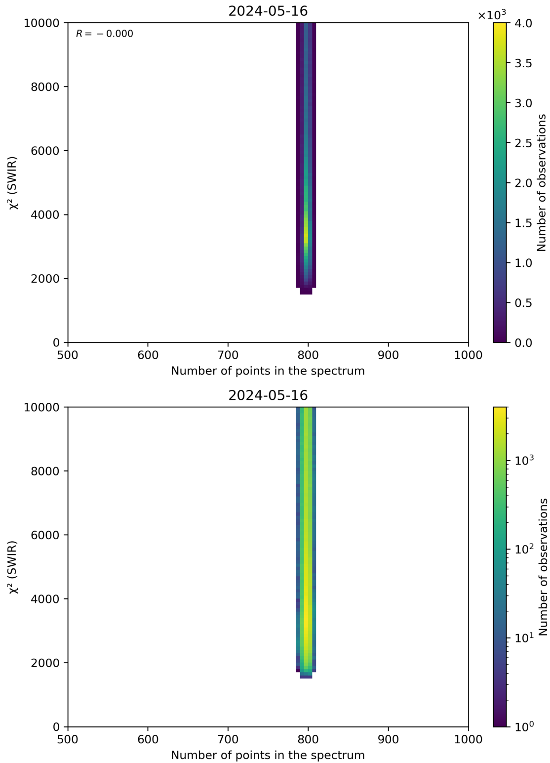
Figure 89: Scatter density plot of “Number of points in the spectrum” against “ \chi^2 (SWIR)” for 2024-05-15 to 2024-05-17.
