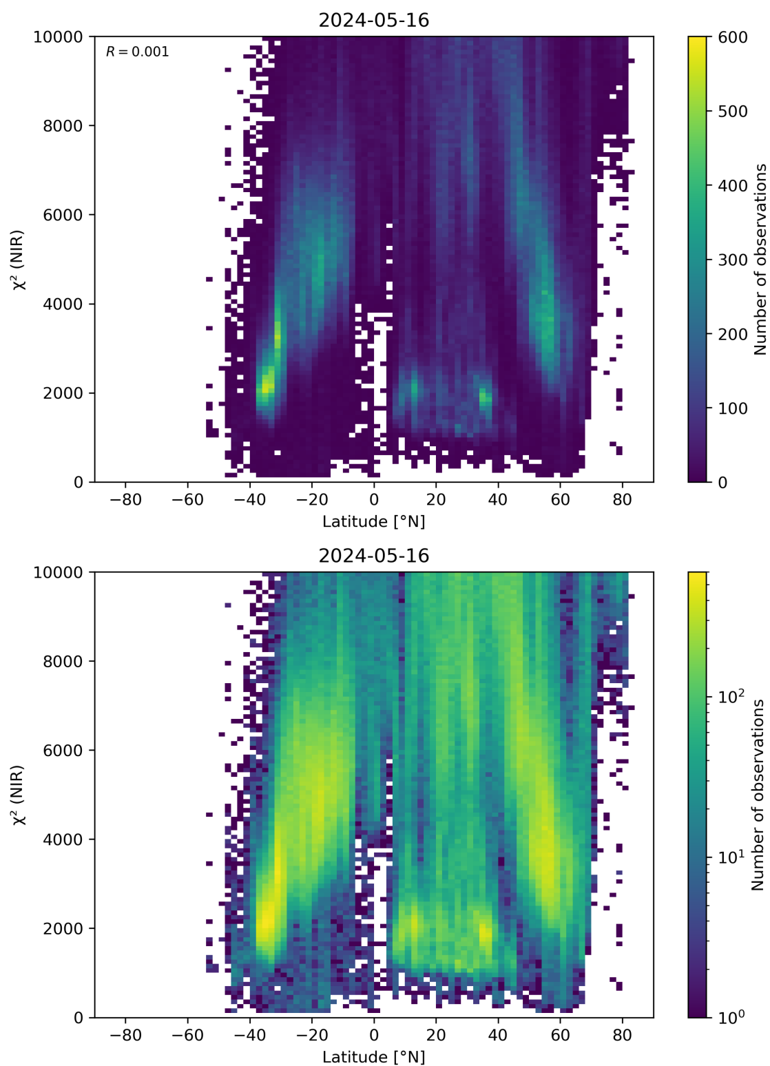
Figure 53: Scatter density plot of “Latitude” against “ \chi^2 (NIR)” for 2024-05-15 to 2024-05-17.
