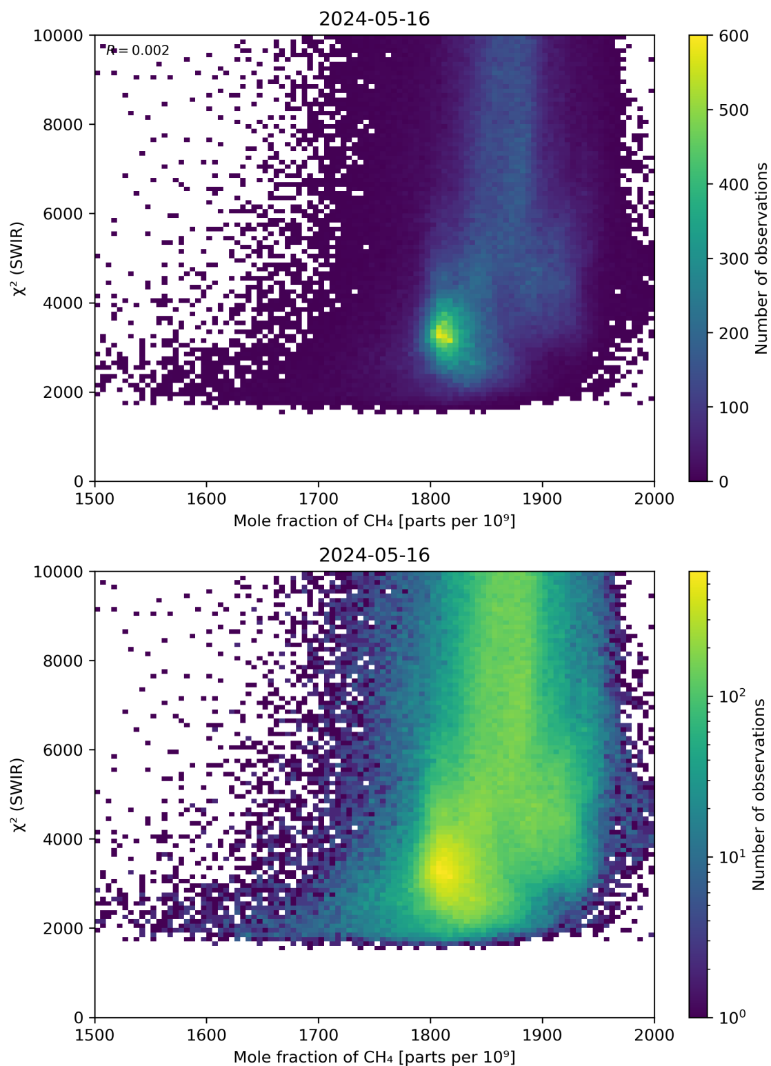
Figure 71: Scatter density plot of “Mole fraction of CH 4 ” against “ \chi^2 (SWIR)” for 2024-05-15 to 2024-05-17.
