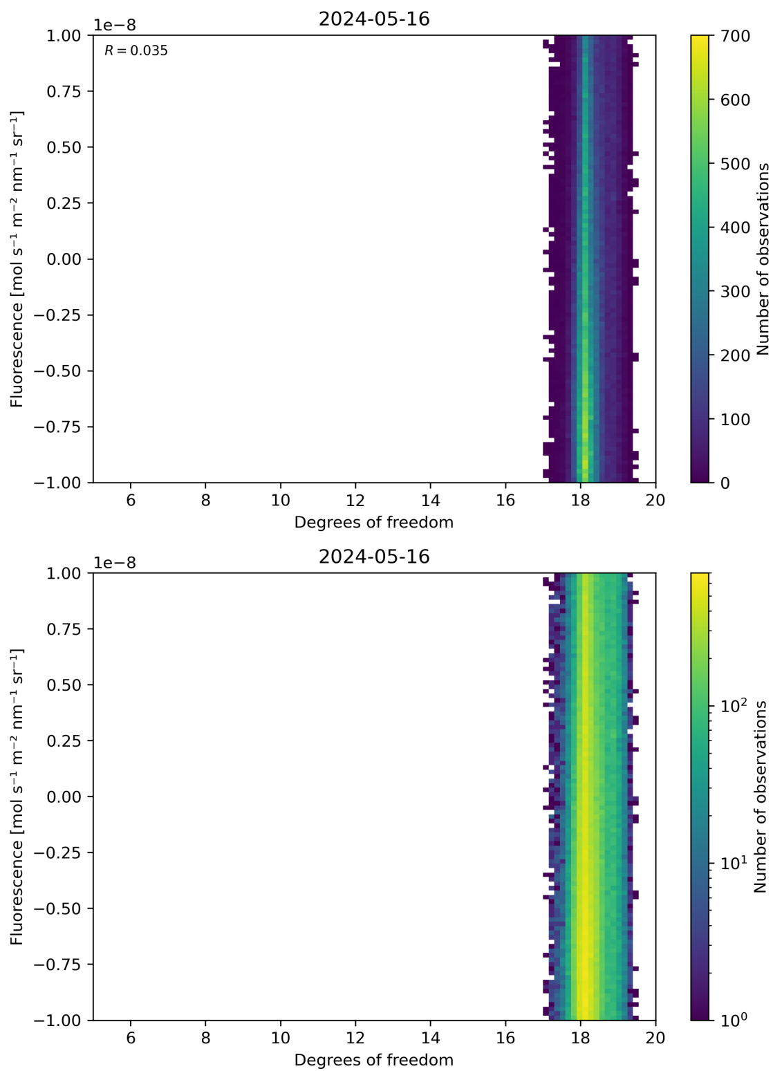
Figure 51: Scatter density plot of “Degrees of freedom” against “Fluorescence” for 2024-05-15 to 2024-05-17.
