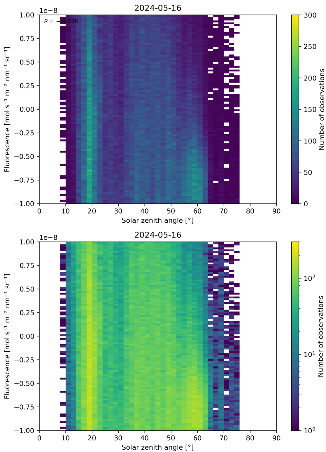
Figure 97: Scatter density plot of “Solar zenith angle” against “Fluorescence” for 2024-05-15 to 2024-05-17.
