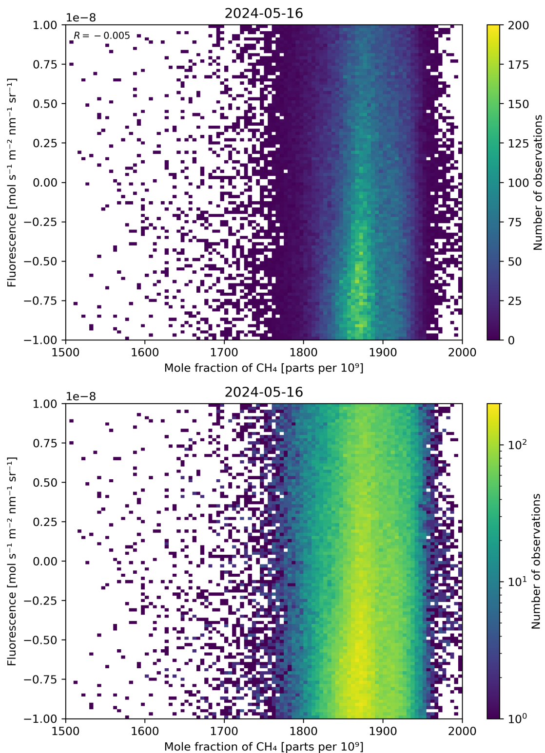
Figure 73: Scatter density plot of “Mole fraction of \text{CH}_4 ” against “Fluorescence” for 2024-05-15 to 2024-05-17.
