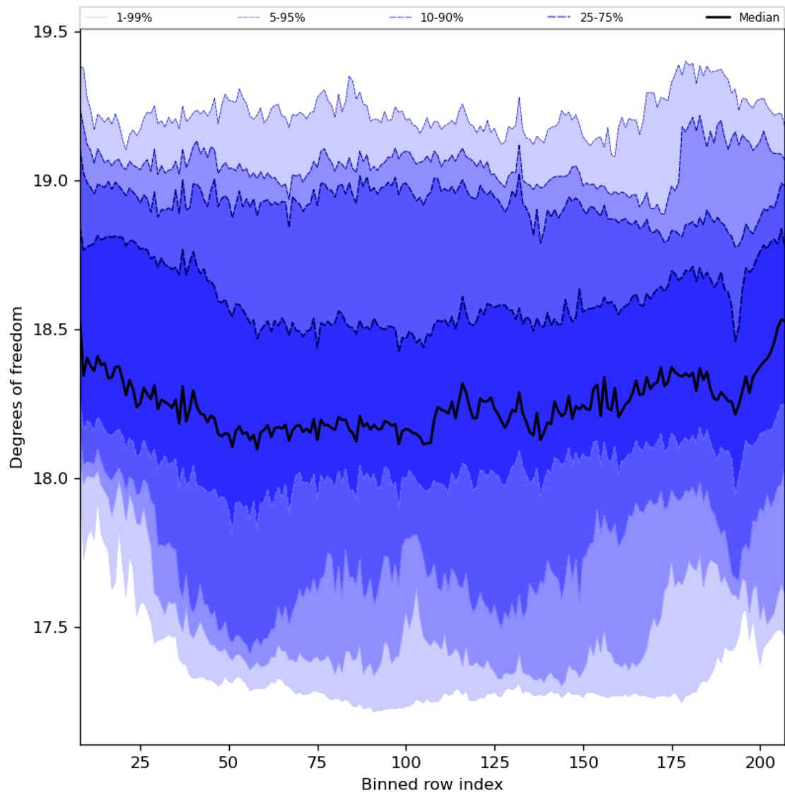
Figure 41: Along track statistics of “Degrees of freedom” for 2024-05-15 to 2024-05-17
