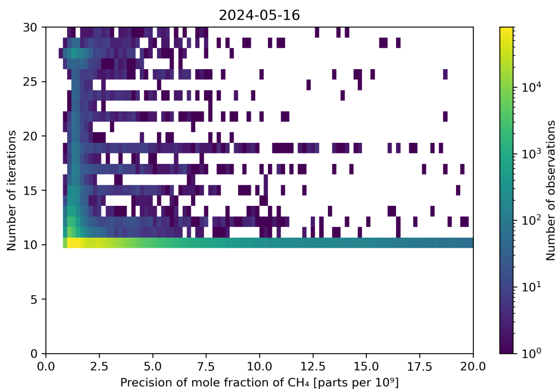
Figure 83: Scatter density plot of “Precision of mole fraction of \text{CH}_4 ” against “Number of iterations” for 2024-05-15 to 2024-05-17.
