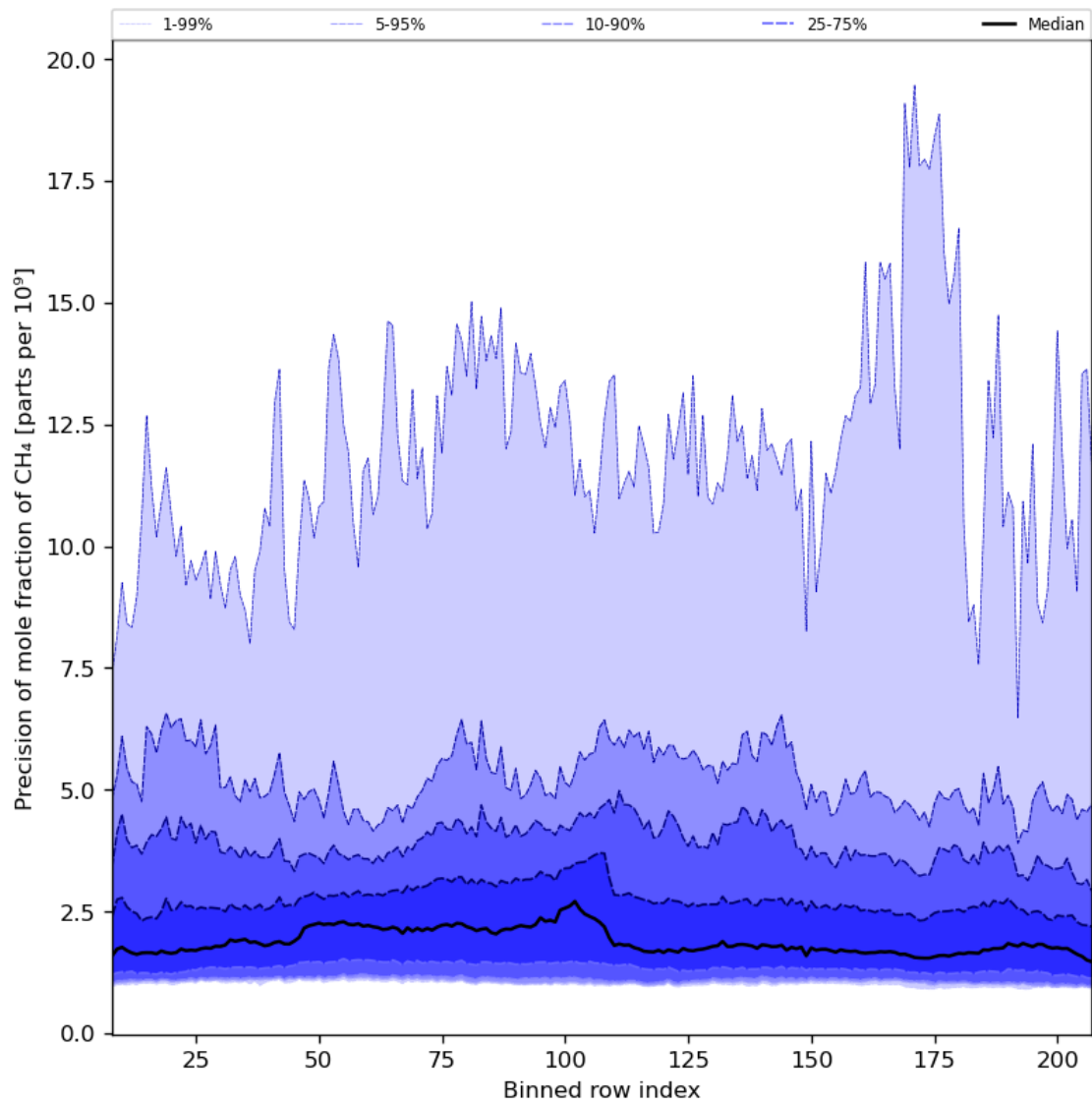
Figure 35: Along track statistics of “Precision of mole fraction of CH 4 ” for 2024-05-15 to 2024-05-17
