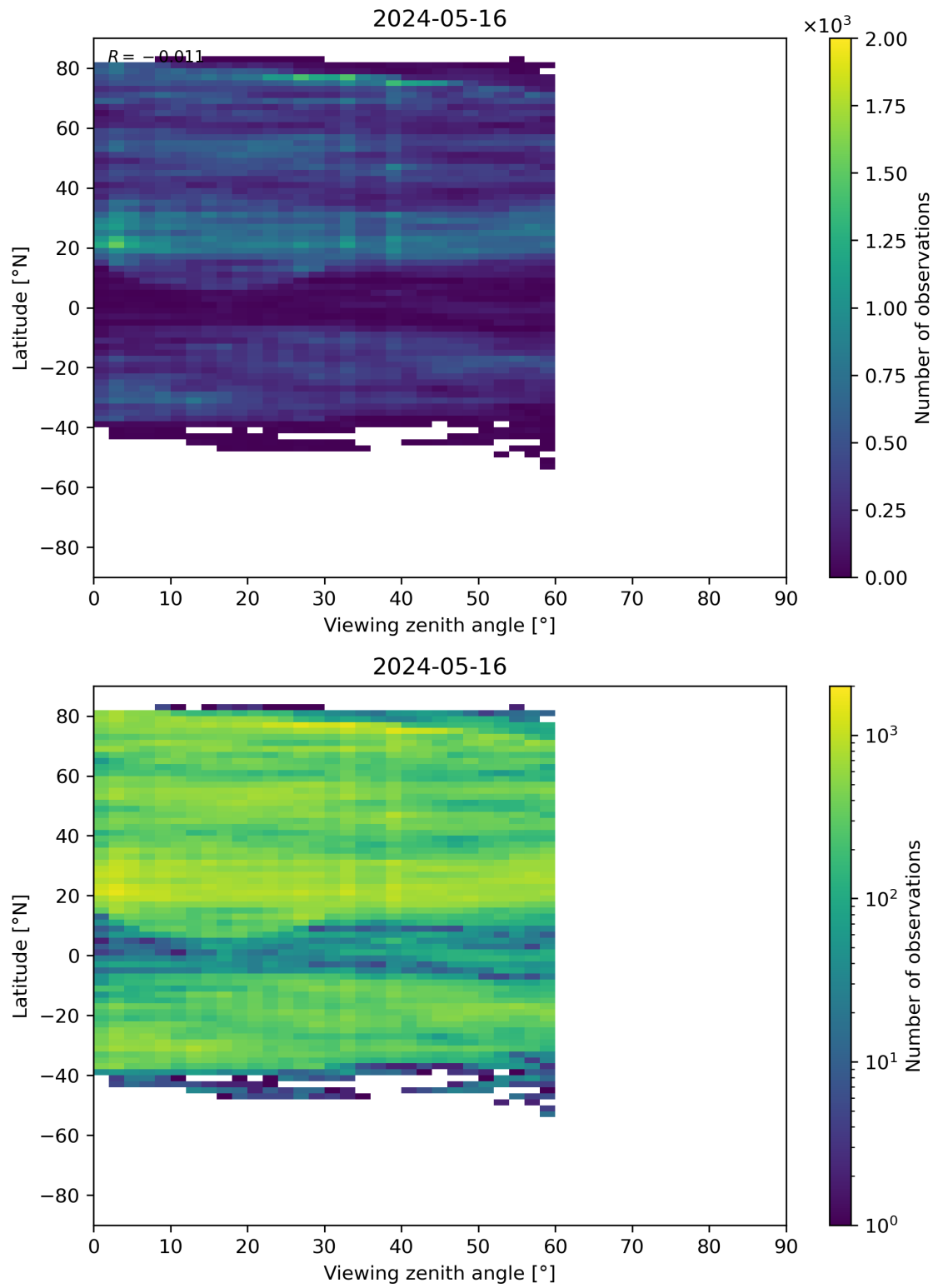
Figure 109: Scatter density plot of “Viewing zenith angle” against “Latitude” for 2024-05-15 to 2024-05-17.
