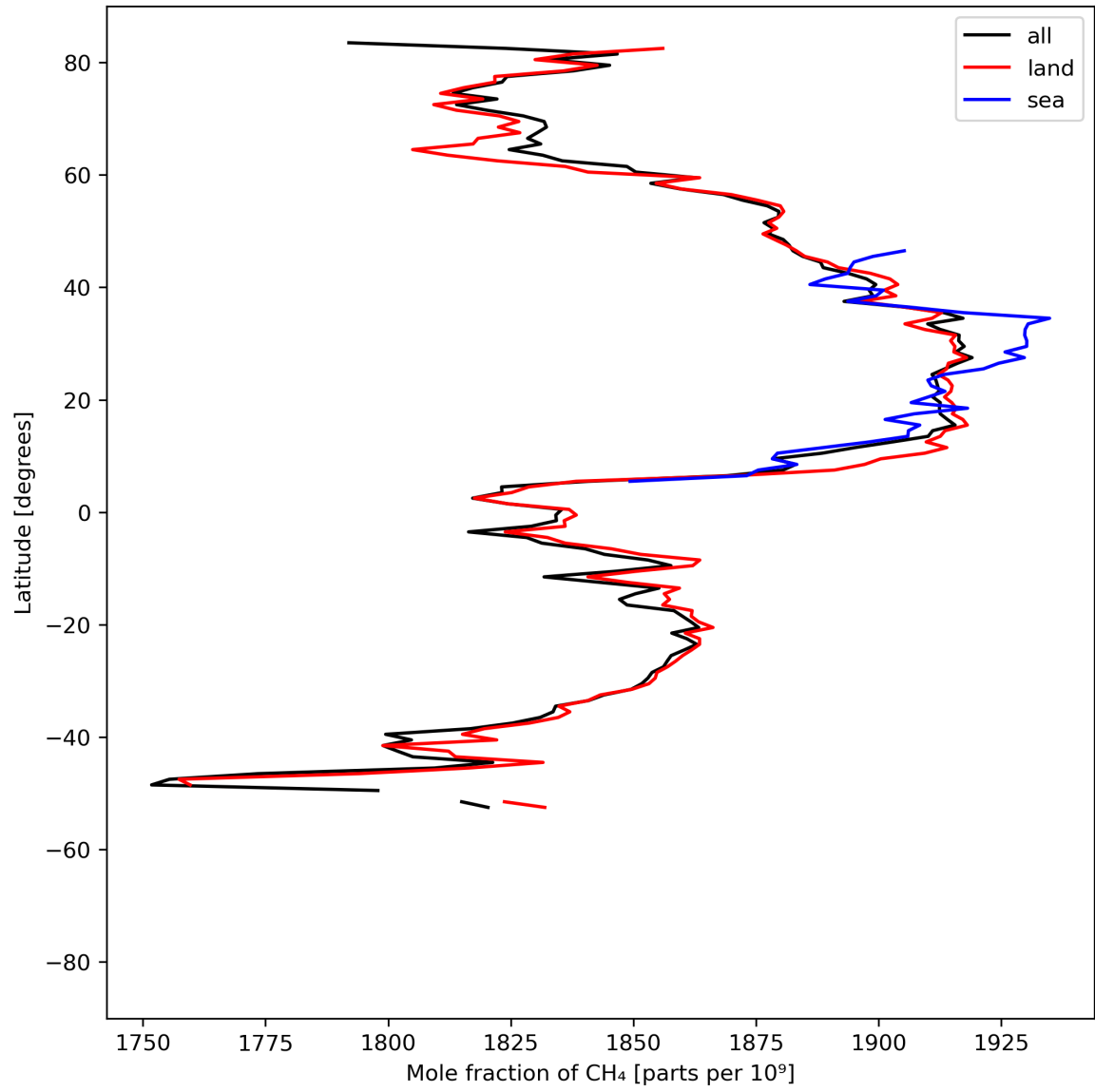
Figure 12: Zonal average of “Mole fraction of \text{CH}_4 ” for 2024-05-15 to 2024-05-17.
