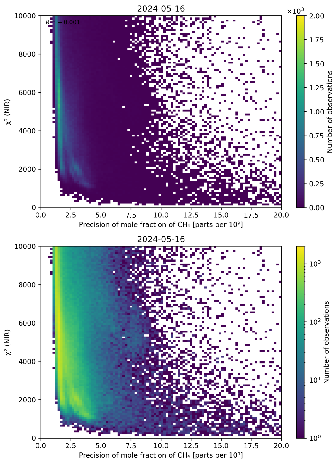
Figure 78: Scatter density plot of “Precision of mole fraction of CH 4 ” against “ \chi^2 (NIR)” for 2024-05-15 to 2024-05-17.
