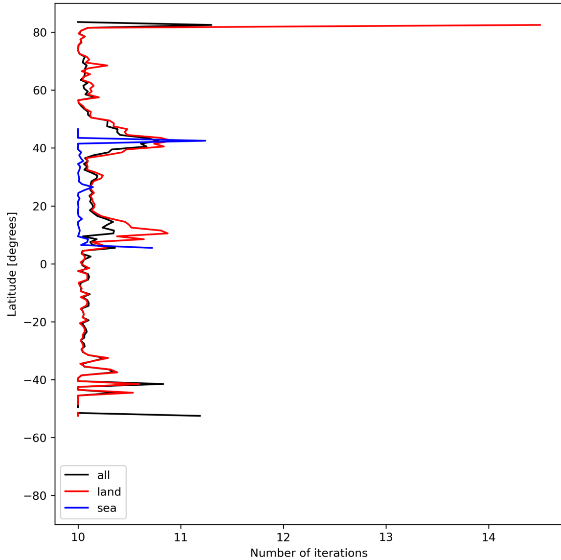
Figure 20: Zonal average of “Number of iterations” for 2024-05-15 to 2024-05-17.
