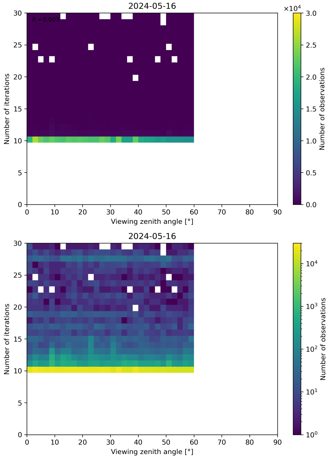
Figure 113: Scatter density plot of “Viewing zenith angle” against “Number of iterations” for 2024-05-15 to 2024-05-17.
