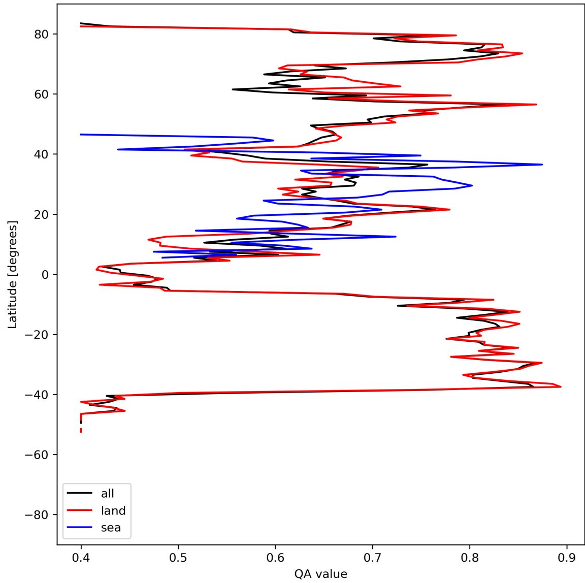
Figure 11: Zonal average of “QA value” for 2024-05-15 to 2024-05-17.
