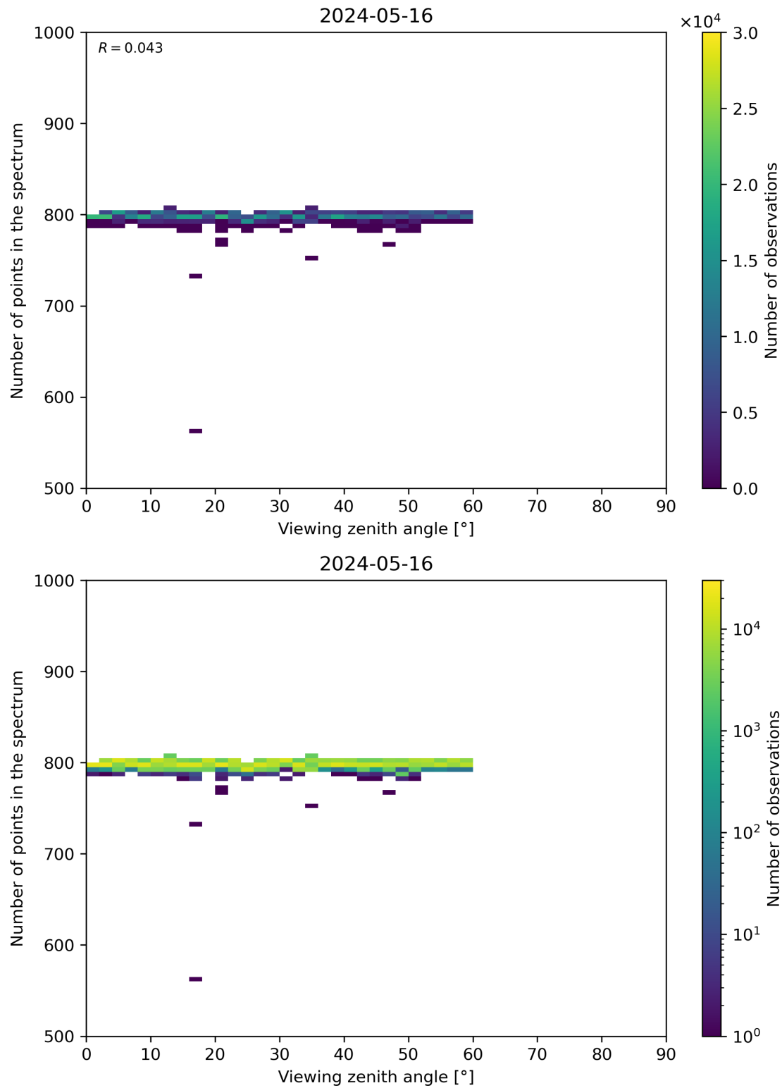
Figure 114: Scatter density plot of “Viewing zenith angle” against “Number of points in the spectrum” for 2024-05-15 to 2024-05-17.
