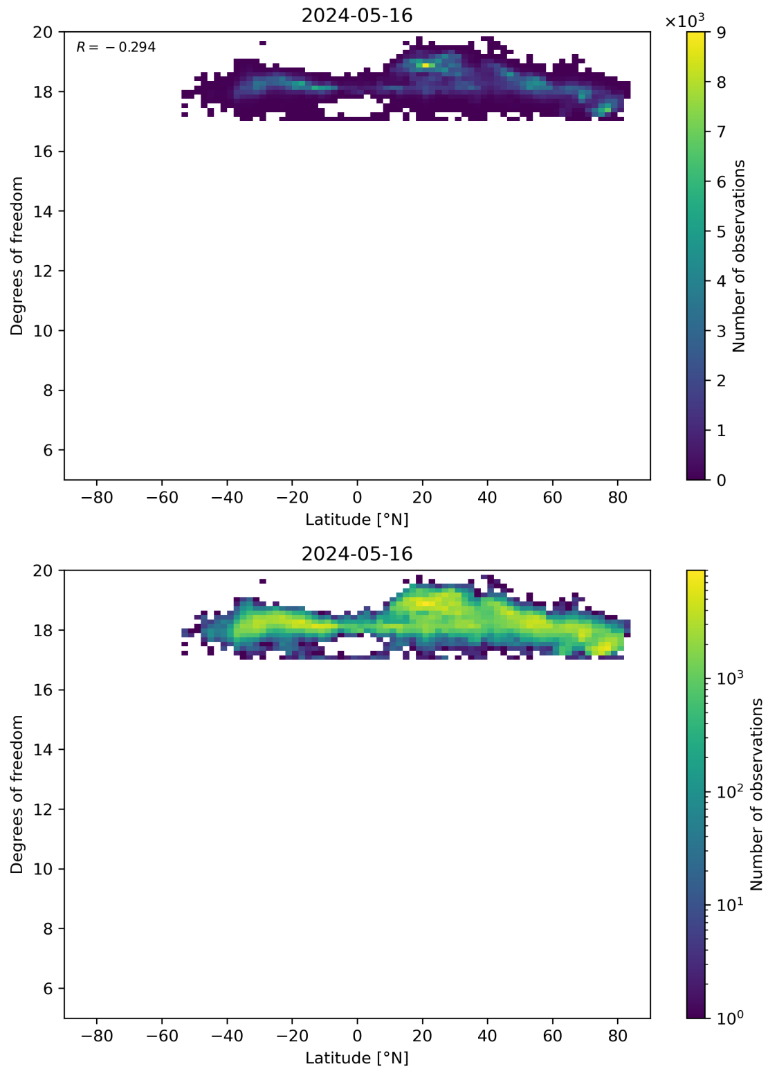
Figure 55: Scatter density plot of “Latitude” against “Degrees of freedom” for 2024-05-15 to 2024-05-17.
