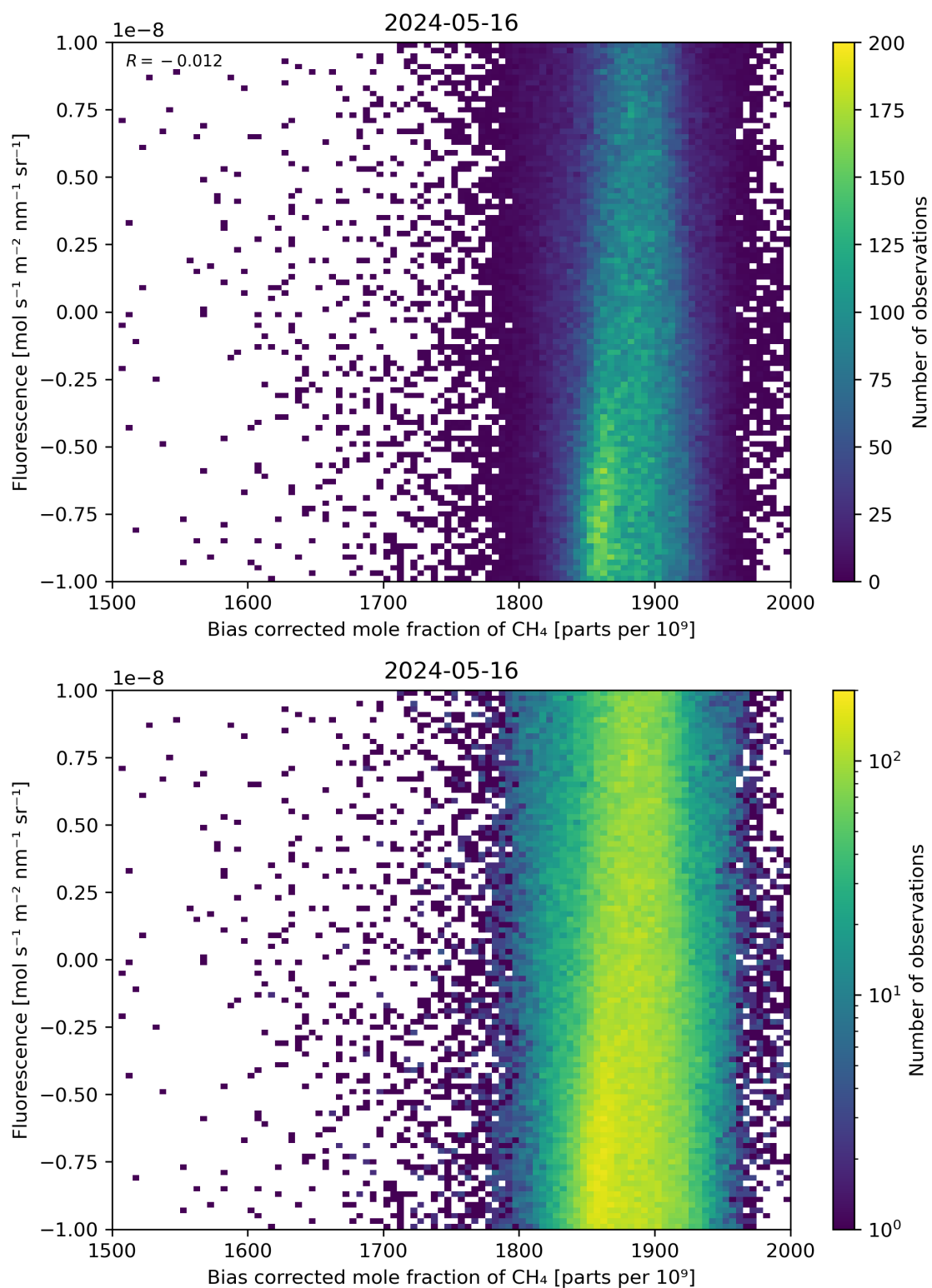
Figure 66: Scatter density plot of “Bias corrected mole fraction of \text{CH}_4 ” against “Fluorescence” for 2024-05-15 to 2024-05-17.
