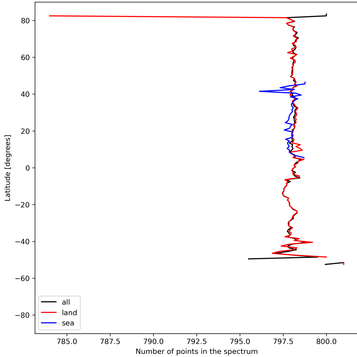
Figure 15: Zonal average of “Number of points in the spectrum” for 2024-05-15 to 2024-05-17.
