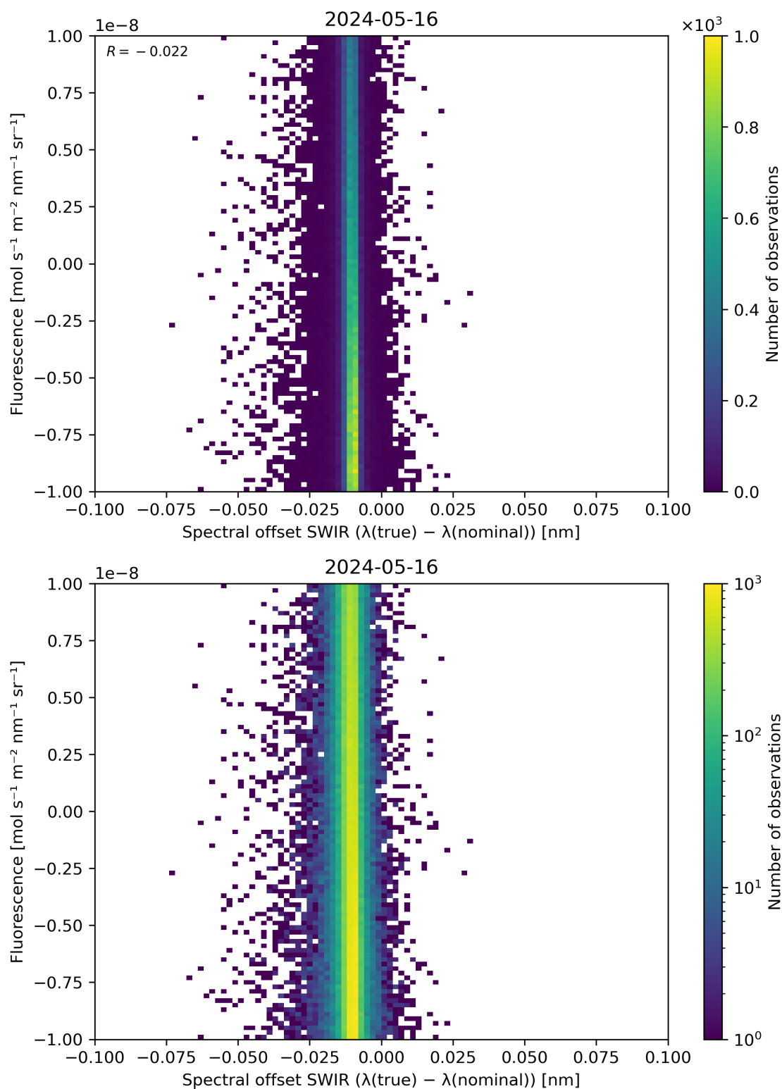
Figure 120: Scatter density plot of “Spectral offset SWIR ( \lambda(\text{true}) - \lambda(\text{nominal}) )” against “Fluorescence” for 2024-05-15 to 2024-05-17.
