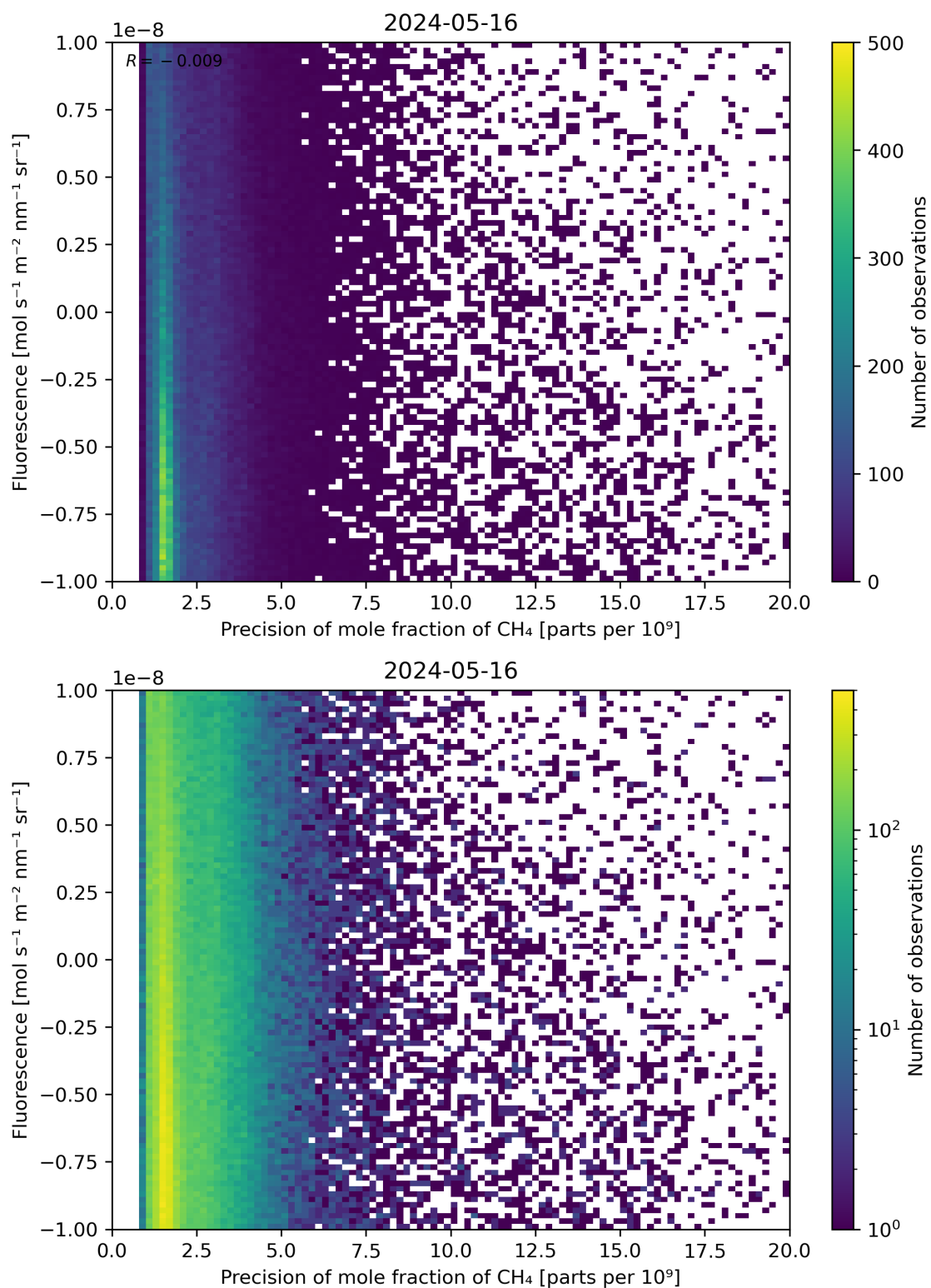
Figure 81: Scatter density plot of “Precision of mole fraction of \text{CH}_4 ” against “Fluorescence” for 2024-05-15 to 2024-05-17.
