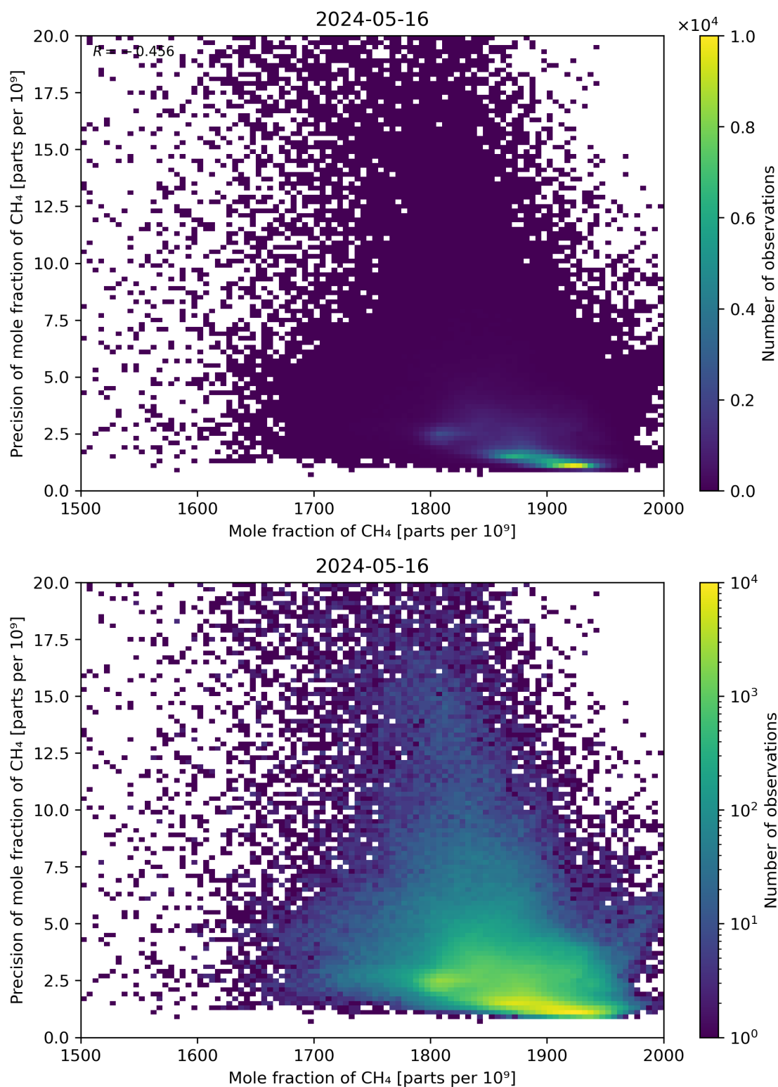
Figure 75: Scatter density plot of “Mole fraction of CH 4 ” against “Precision of mole fraction of CH 4 ” for 2024-05-15 to 2024-05-17.
