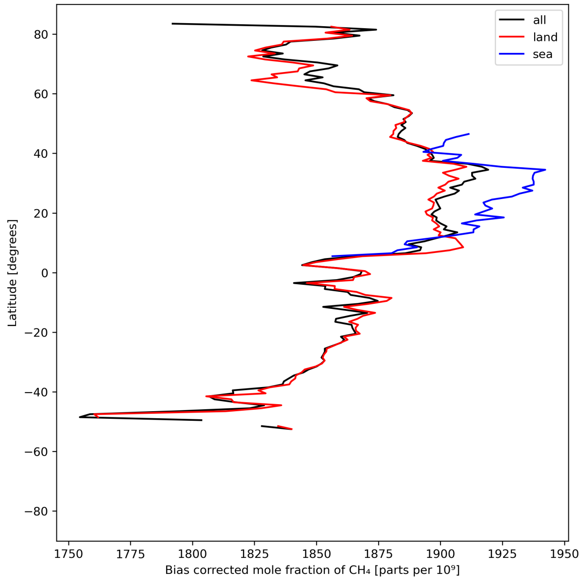
Figure 14: Zonal average of “Bias corrected mole fraction of \text{CH}_4 ” for 2024-05-15 to 2024-05-17.
