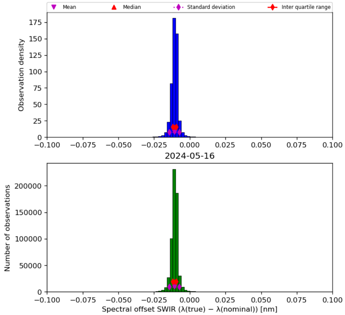
Figure 27: Histogram of “Spectral offset SWIR ( \lambda(\text{true}) - \lambda(\text{nominal}) )” for 2024-05-15 to 2024-05-17
