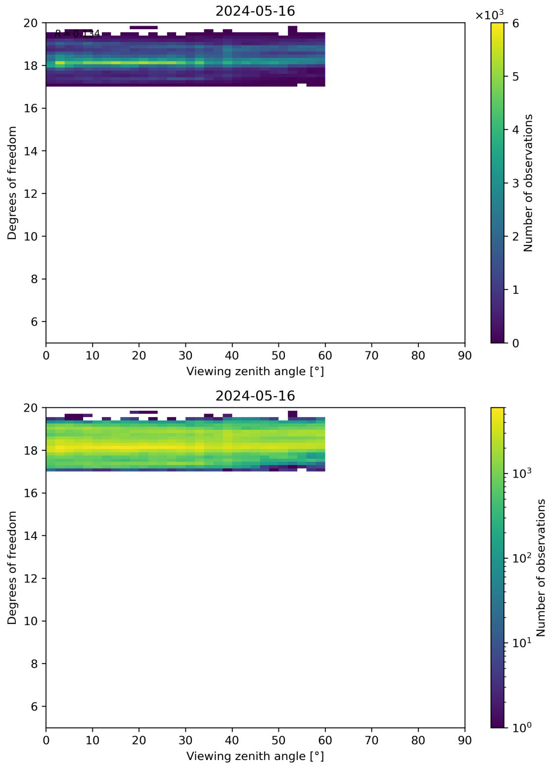
Figure 107: Scatter density plot of “Viewing zenith angle” against “Degrees of freedom” for 2024-05-15 to 2024-05-17.
