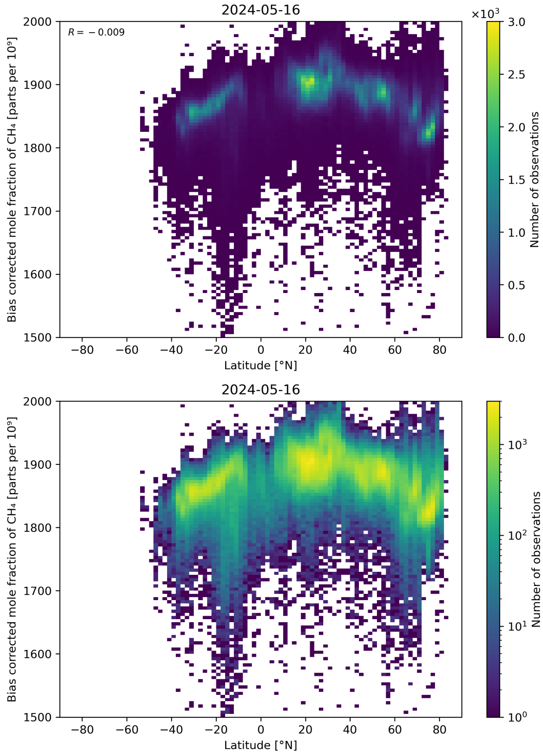
Figure 58: Scatter density plot of “Latitude” against “Bias corrected mole fraction of CH 4 ” for 2024-05-15 to 2024-05-17.
