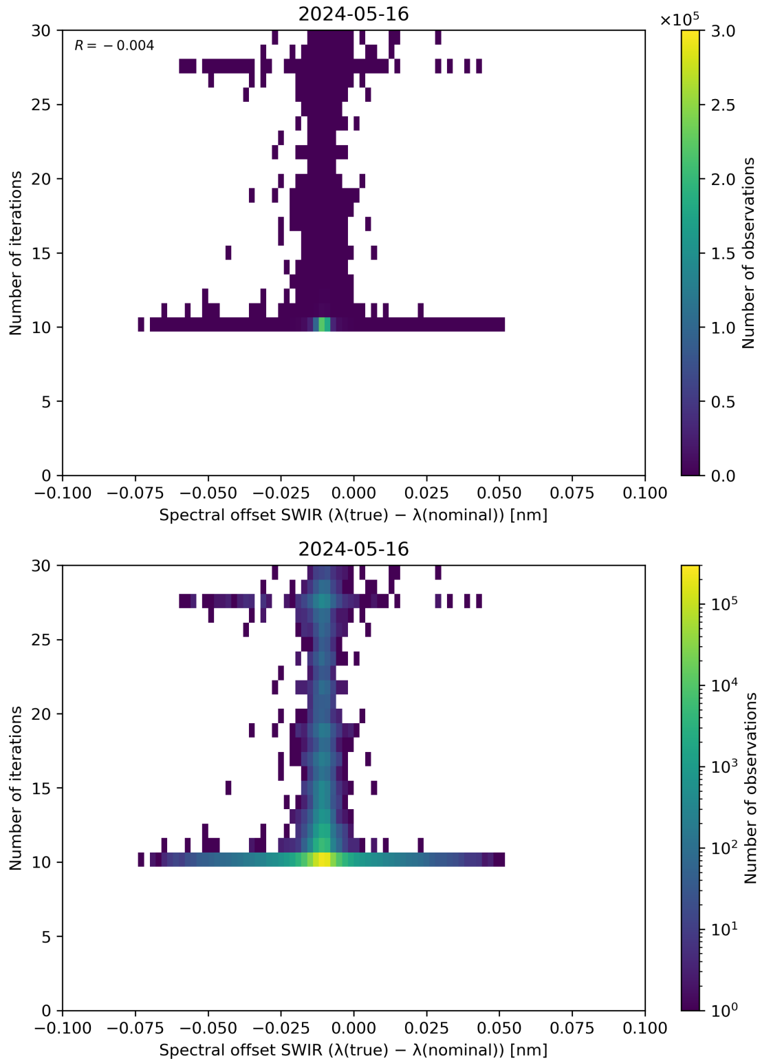
Figure 121: Scatter density plot of “Spectral offset SWIR ( \lambda(\text{true}) - \lambda(\text{nominal}) )” against “Number of iterations” for 2024-05-15 to 2024-05-17.
