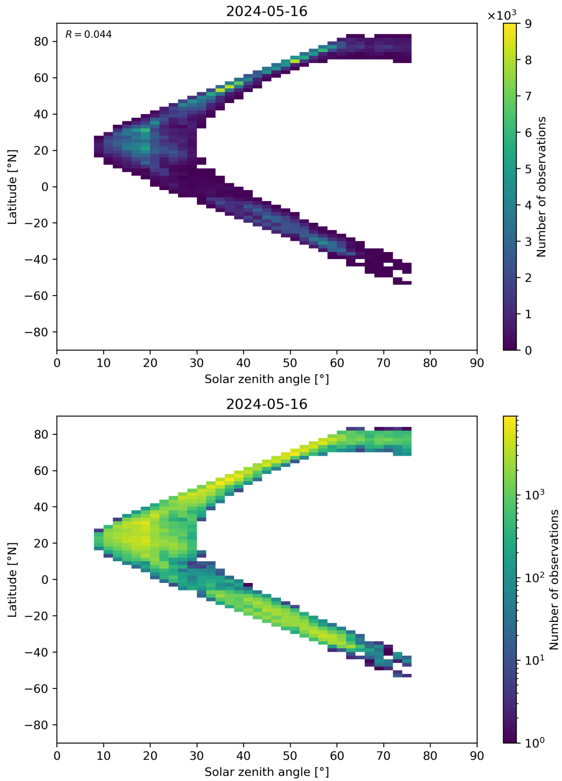
Figure 98: Scatter density plot of “Solar zenith angle” against “Latitude” for 2024-05-15 to 2024-05-17.
