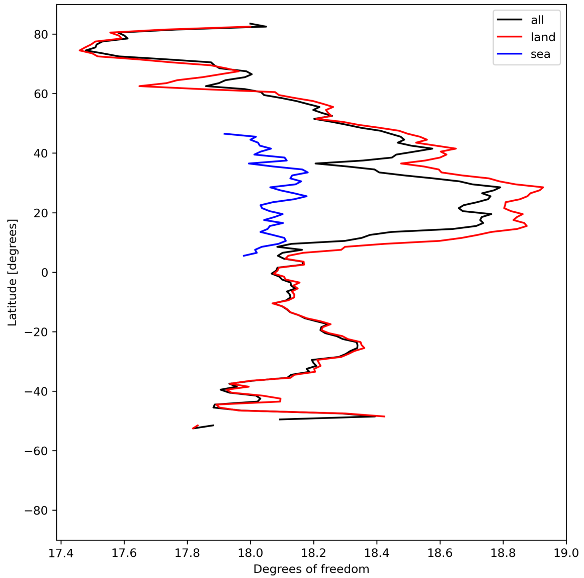
Figure 19: Zonal average of “Degrees of freedom” for 2024-05-15 to 2024-05-17.
