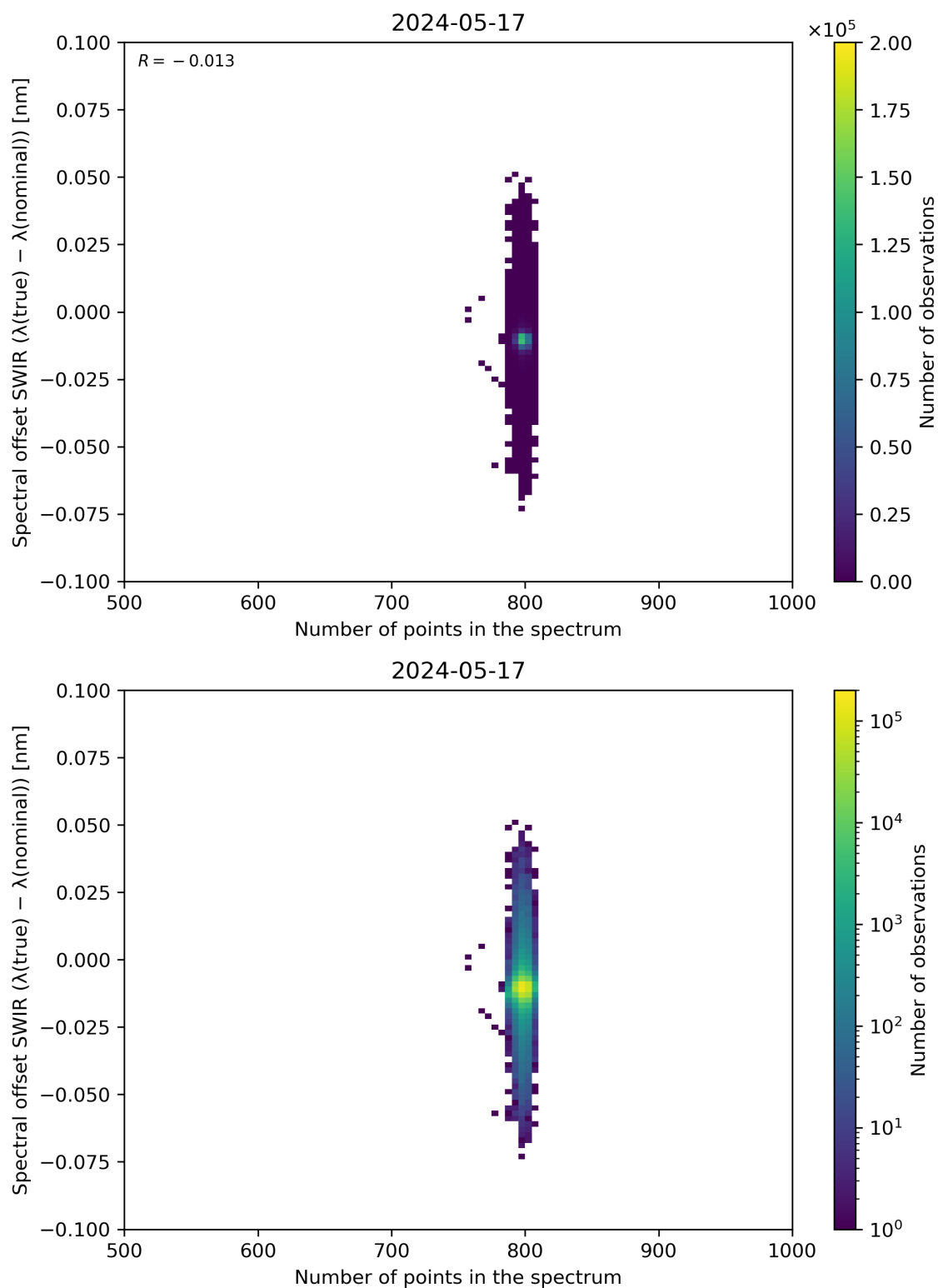
Figure 93: Scatter density plot of “Number of points in the spectrum” against “Spectral offset SWIR ( \lambda(\text{true}) - \lambda(\text{nominal}) )” for 2024-05-16 to 2024-05-18.
