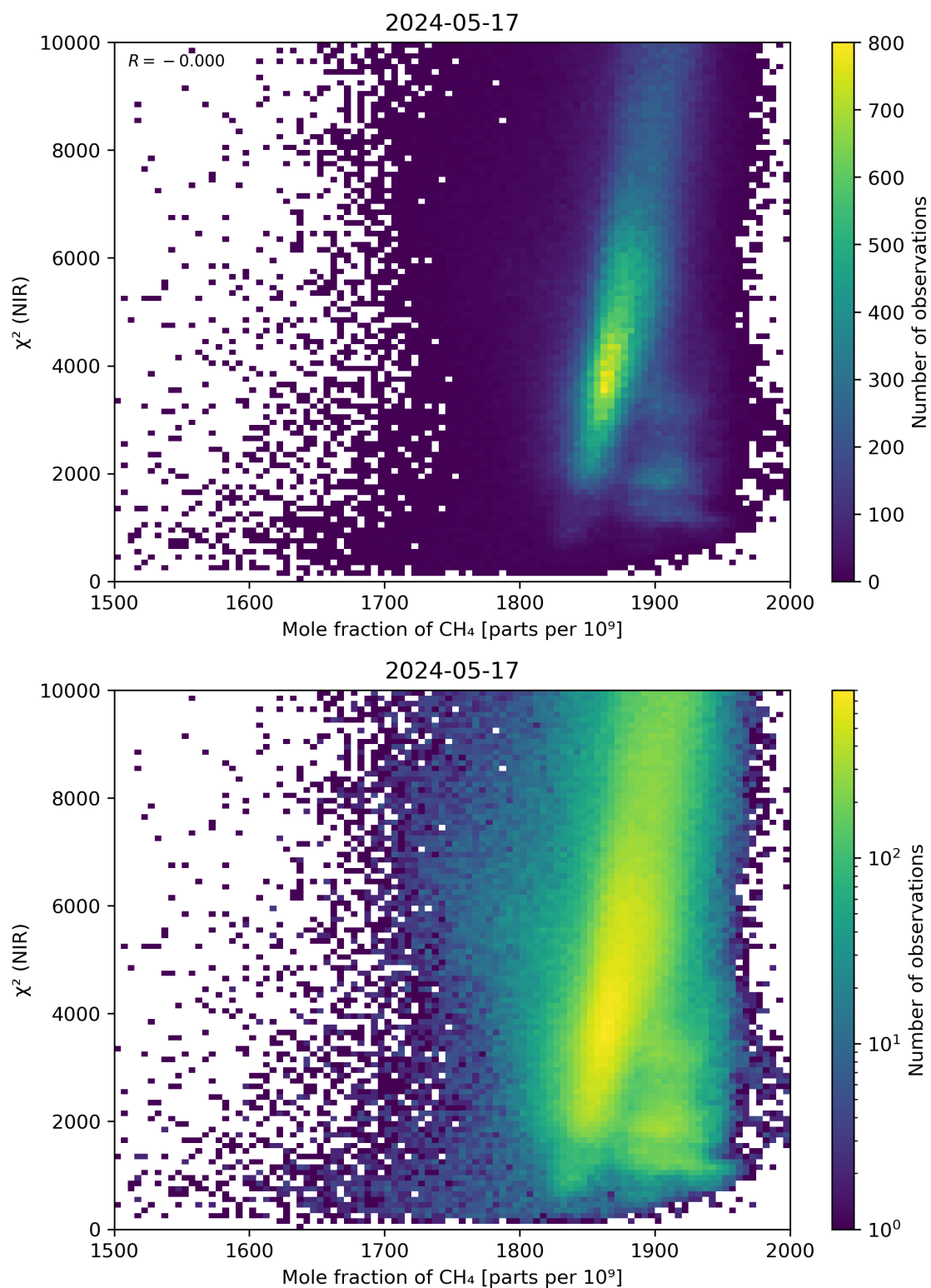
Figure 70: Scatter density plot of “Mole fraction of CH 4 ” against “ \chi^2 (NIR)” for 2024-05-16 to 2024-05-18.
