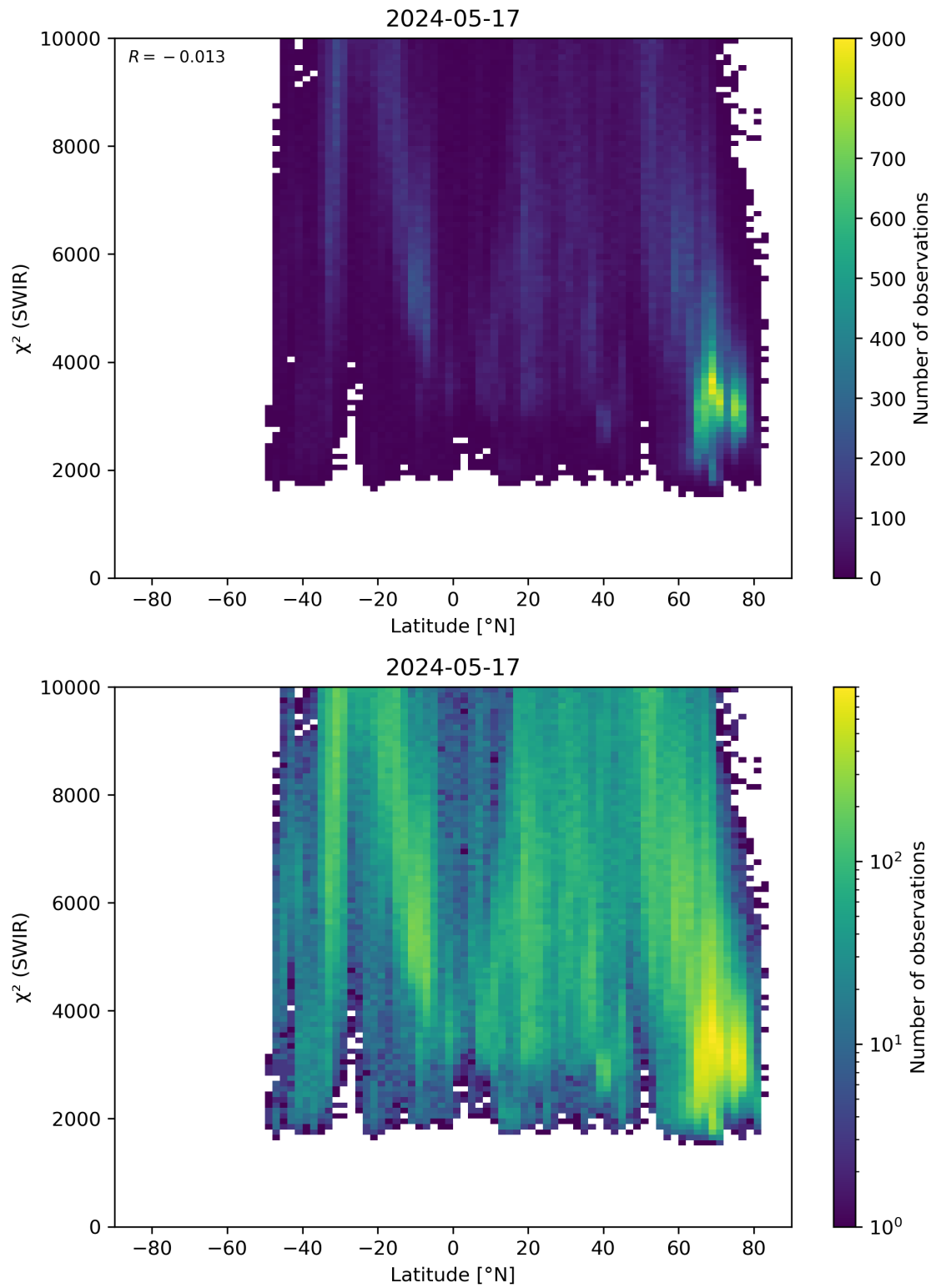
Figure 54: Scatter density plot of “Latitude” against “ \chi^2 (SWIR)” for 2024-05-16 to 2024-05-18.
