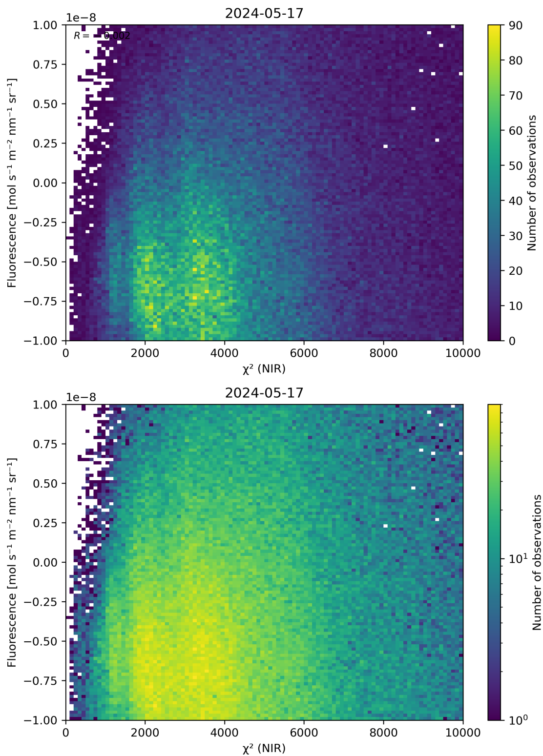
Figure 45: Scatter density plot of “ \chi^2 (NIR)” against “Fluorescence” for 2024-05-16 to 2024-05-18.
