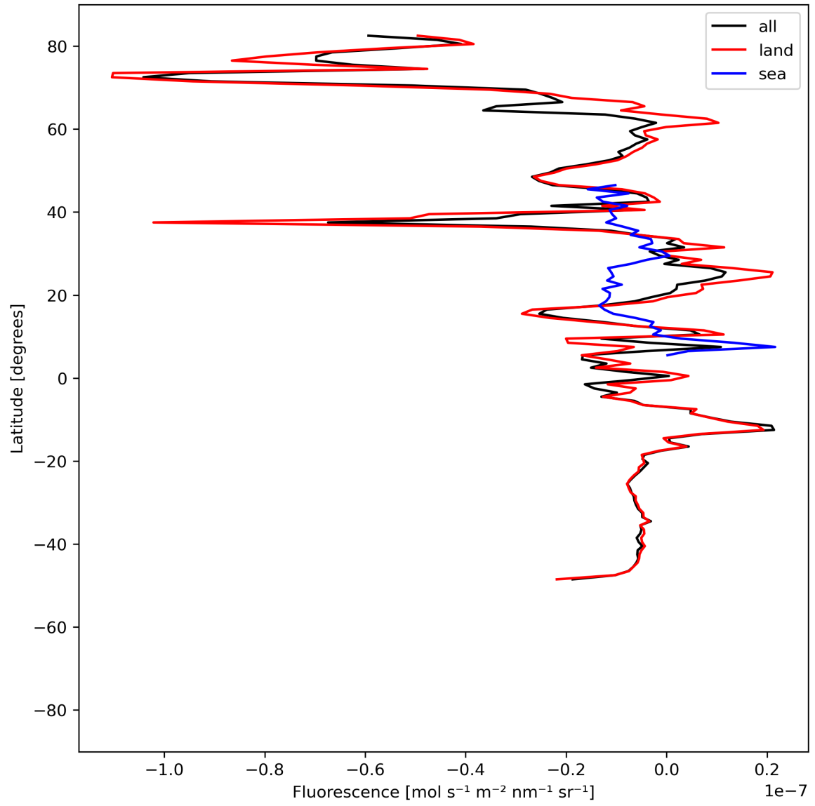
Figure 21: Zonal average of “Fluorescence” for 2024-05-16 to 2024-05-18.
