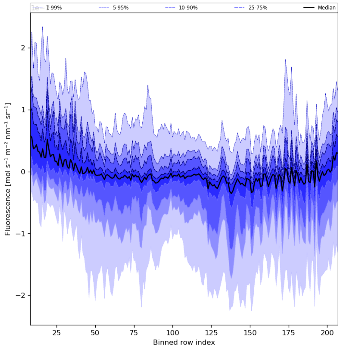
Figure 43: Along track statistics of “Fluorescence” for 2024-05-16 to 2024-05-18
