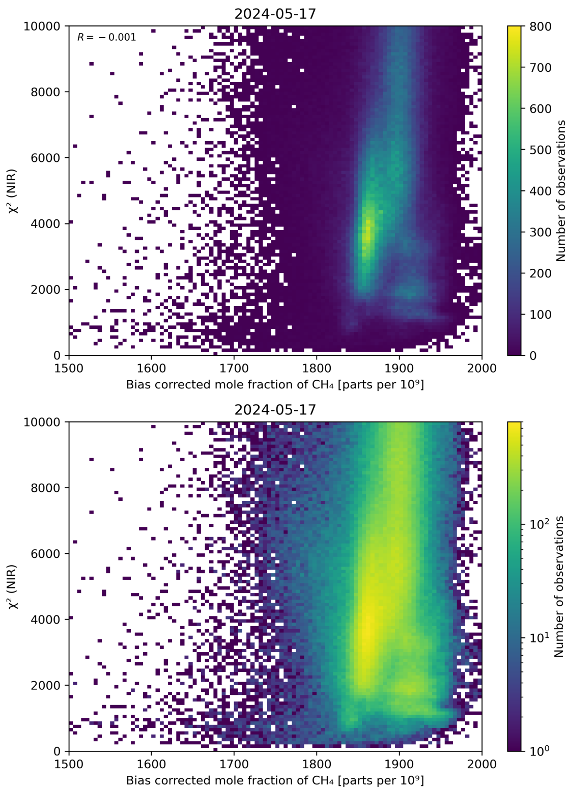
Figure 63: Scatter density plot of “Bias corrected mole fraction of CH 4 ” against “ \chi^2 (NIR)” for 2024-05-16 to 2024-05-18.
