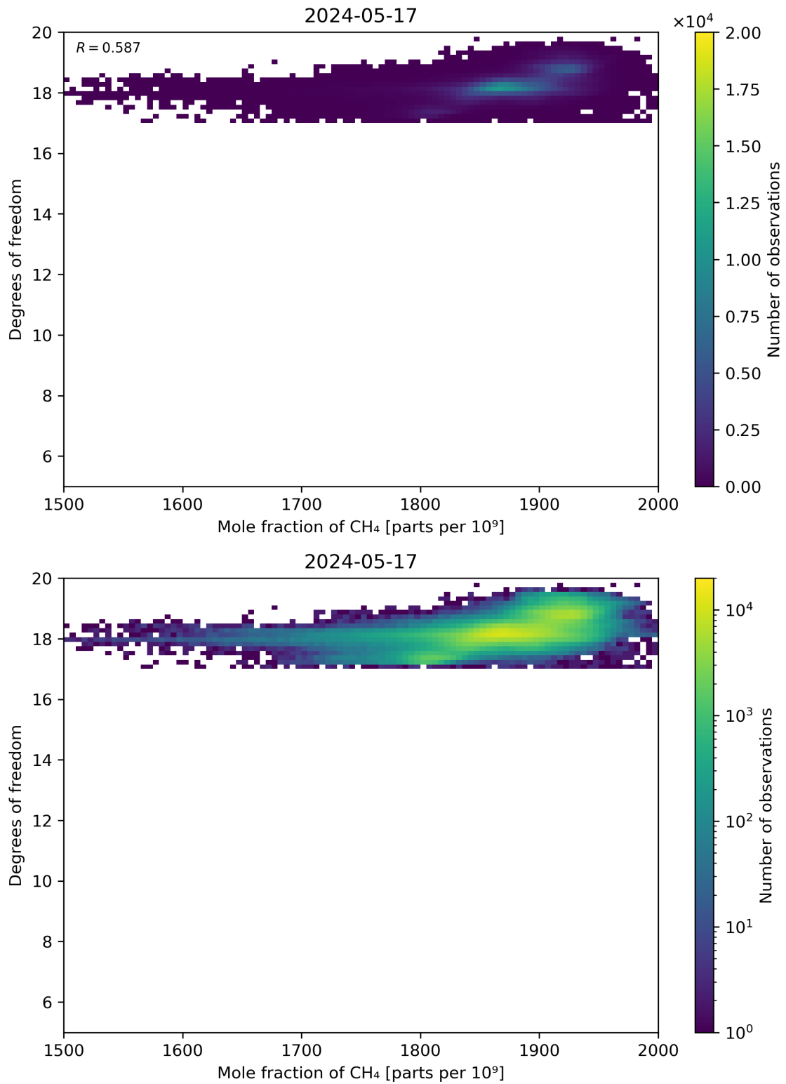
Figure 72: Scatter density plot of “Mole fraction of CH 4 ” against “Degrees of freedom” for 2024-05-16 to 2024-05-18.
