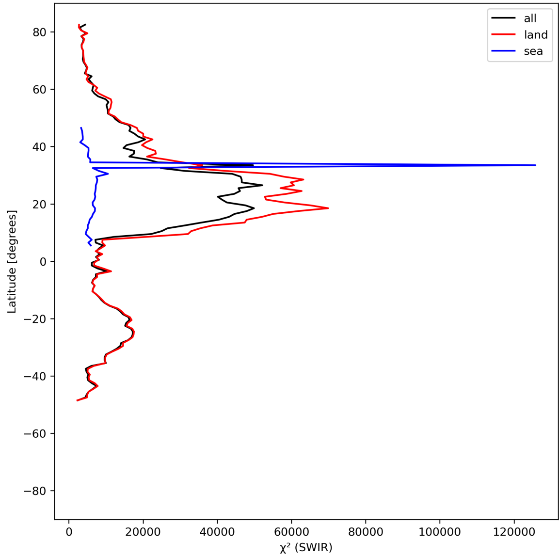
Figure 17: Zonal average of “ \chi^2 (SWIR)” for 2024-05-16 to 2024-05-18.
