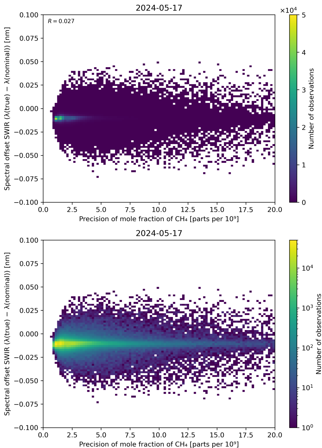
Figure 85: Scatter density plot of “Precision of mole fraction of CH 4 ” against “Spectral offset SWIR ( \lambda(\text{true}) - \lambda(\text{nominal}) )” for 2024-05-16 to 2024-05-18.
