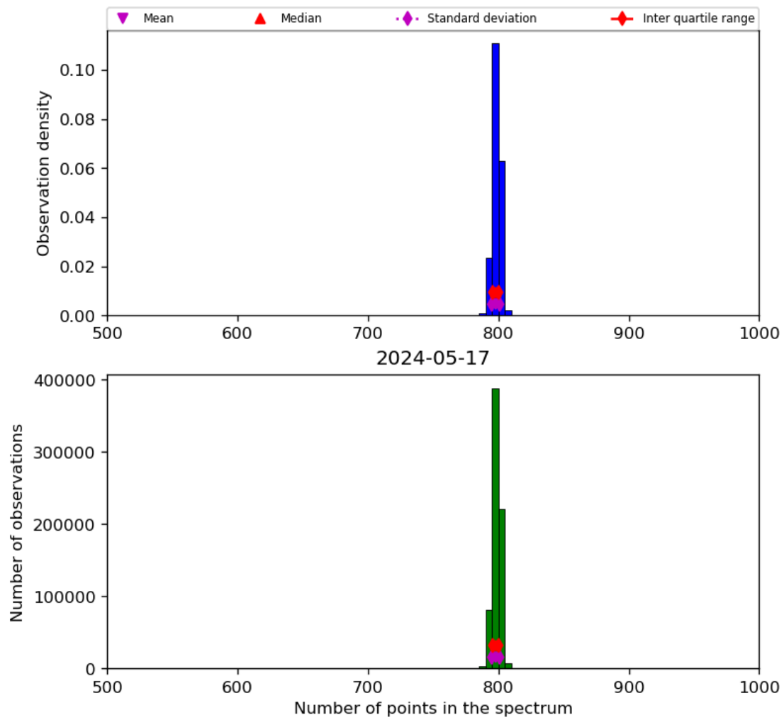
Figure 26: Histogram of “Number of points in the spectrum” for 2024-05-16 to 2024-05-18
