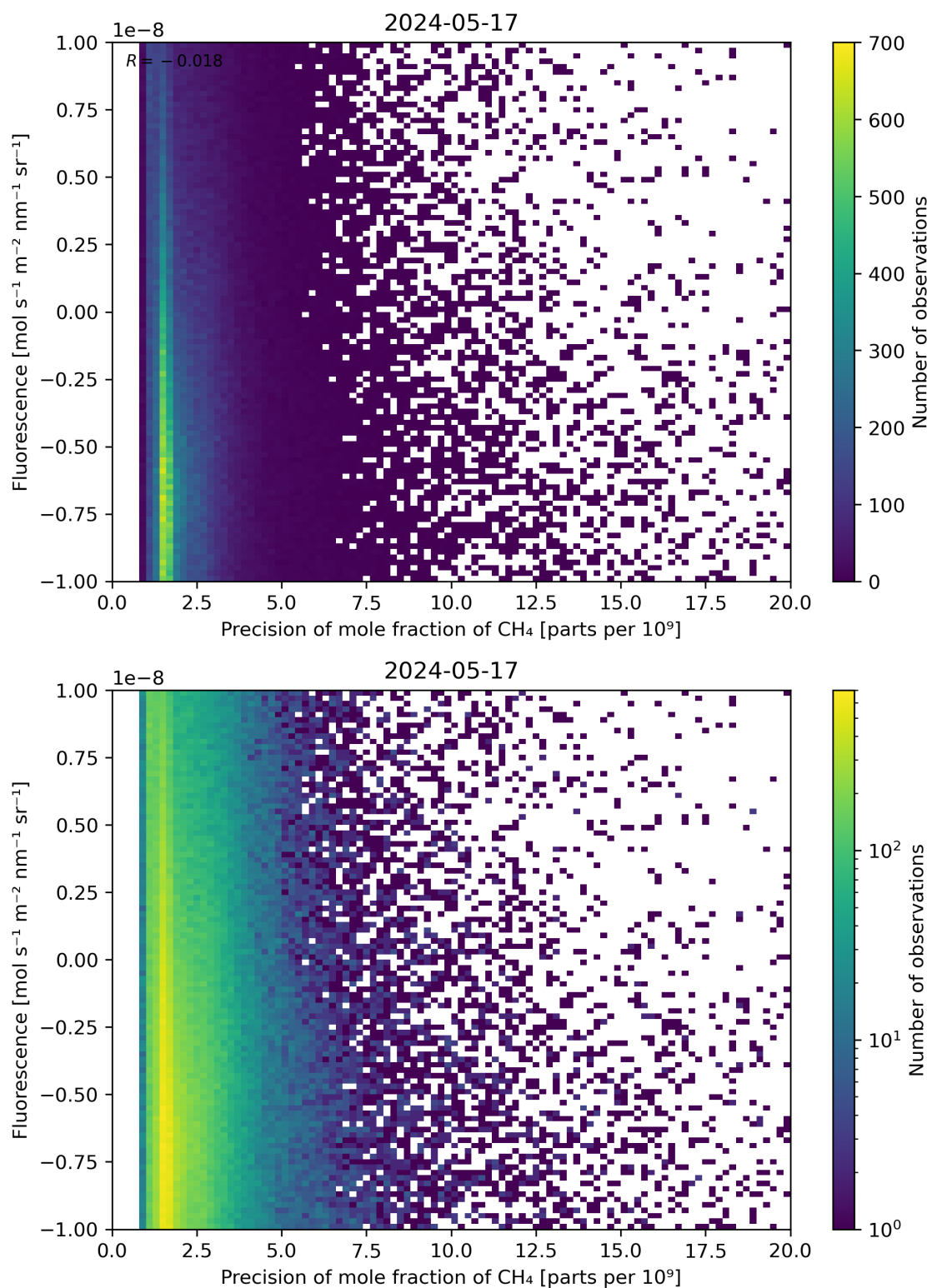
Figure 81: Scatter density plot of “Precision of mole fraction of CH 4 ” against “Fluorescence” for 2024-05-16 to 2024-05-18.
