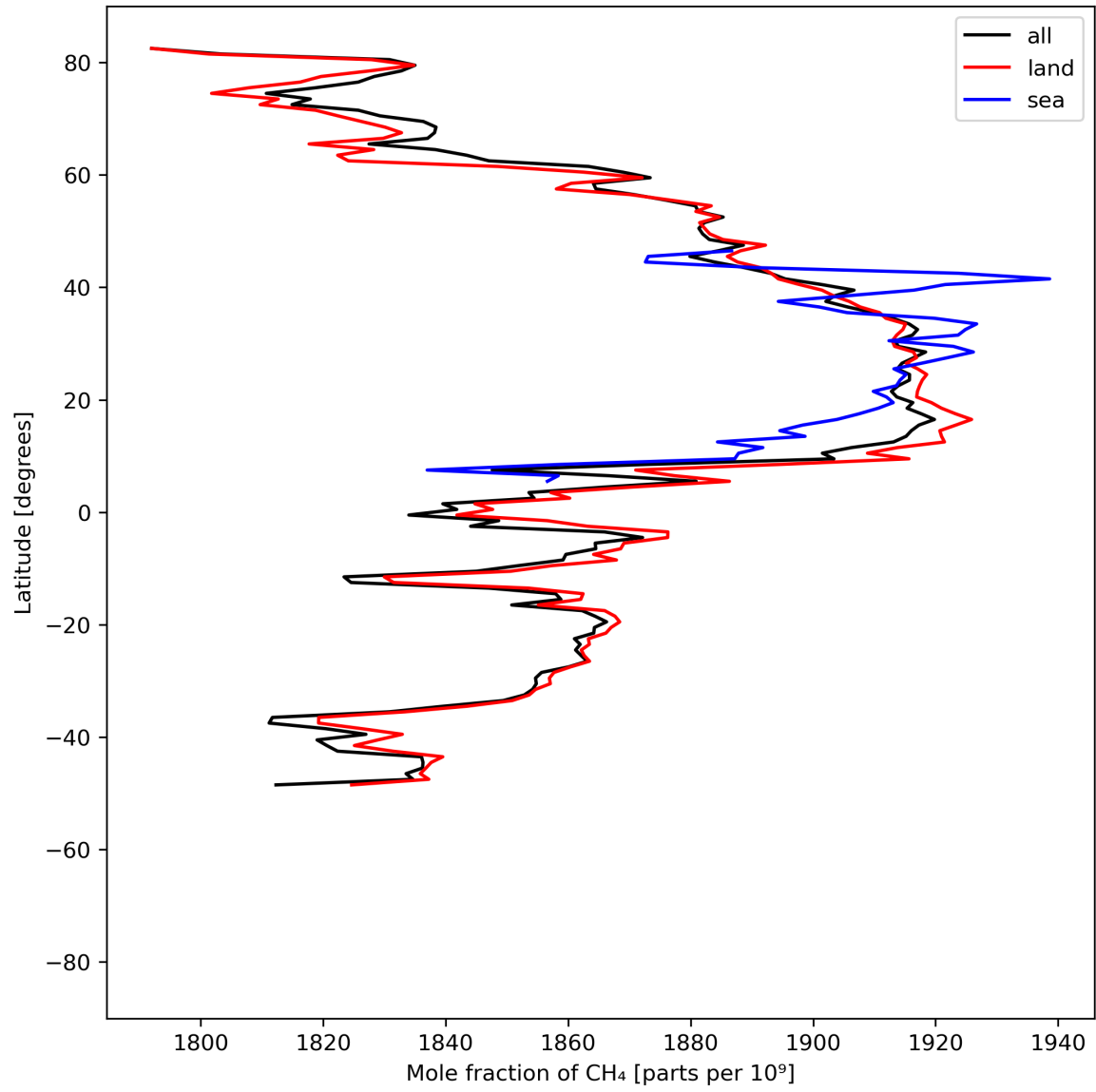
Figure 12: Zonal average of “Mole fraction of \text{CH}_4 ” for 2024-05-16 to 2024-05-18.
