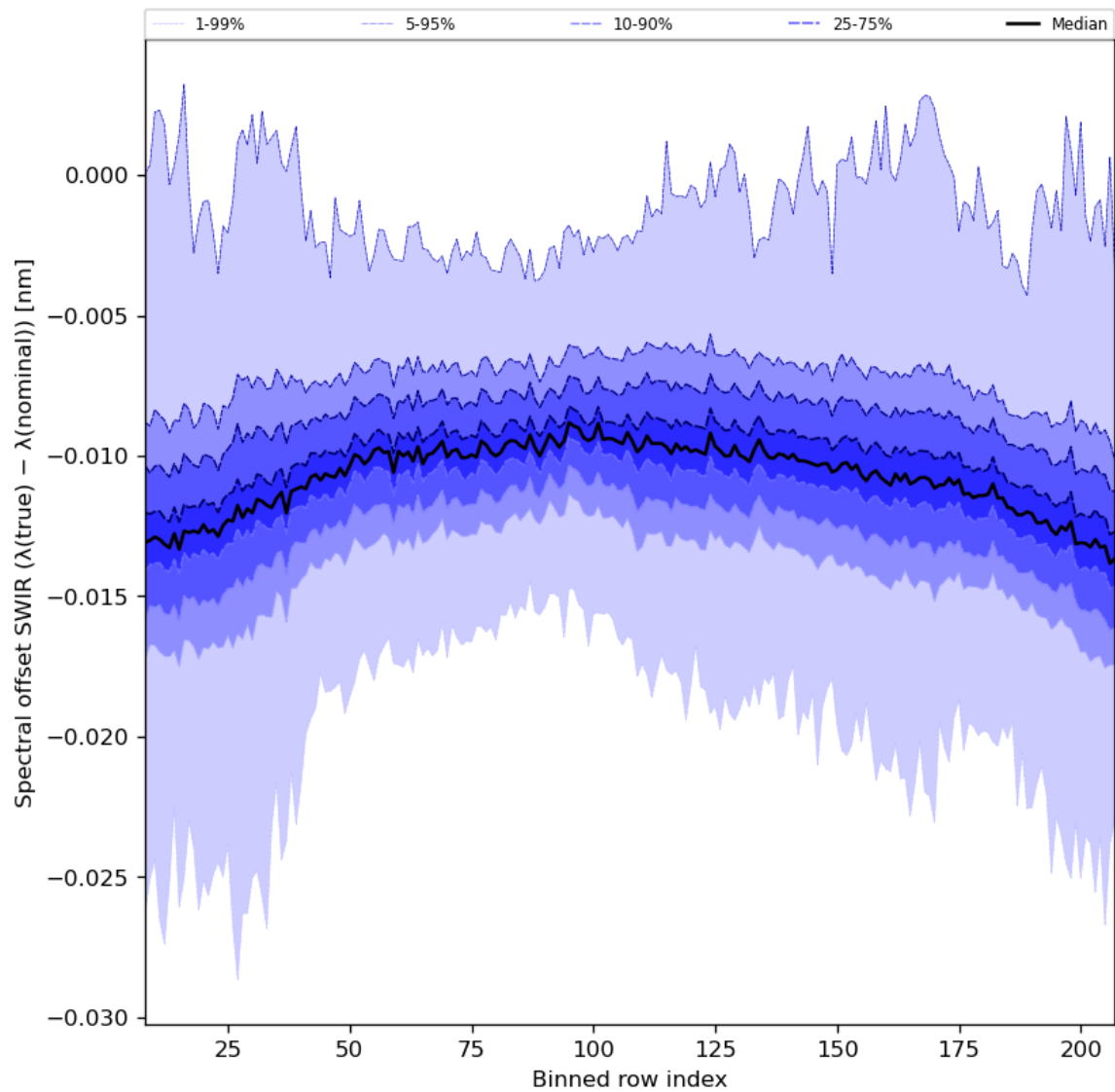
Figure 38: Along track statistics of “Spectral offset SWIR ( \lambda(\text{true}) - \lambda(\text{nominal}) )” for 2024-05-16 to 2024-05-18
