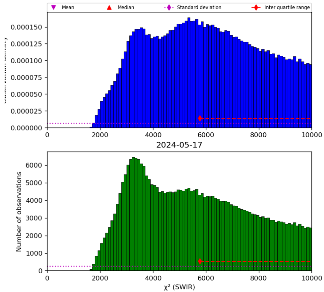
Figure 28: Histogram of " \chi^2 (SWIR)" for 2024-05-16 to 2024-05-18
