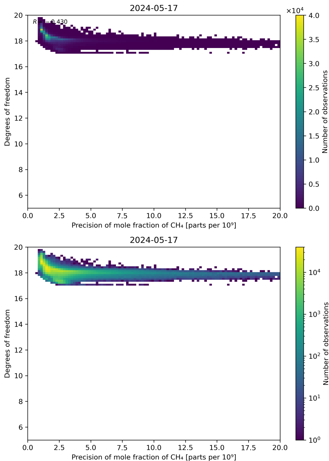
Figure 80: Scatter density plot of “Precision of mole fraction of CH 4 ” against “Degrees of freedom” for 2024-05-16 to 2024-05-18.
