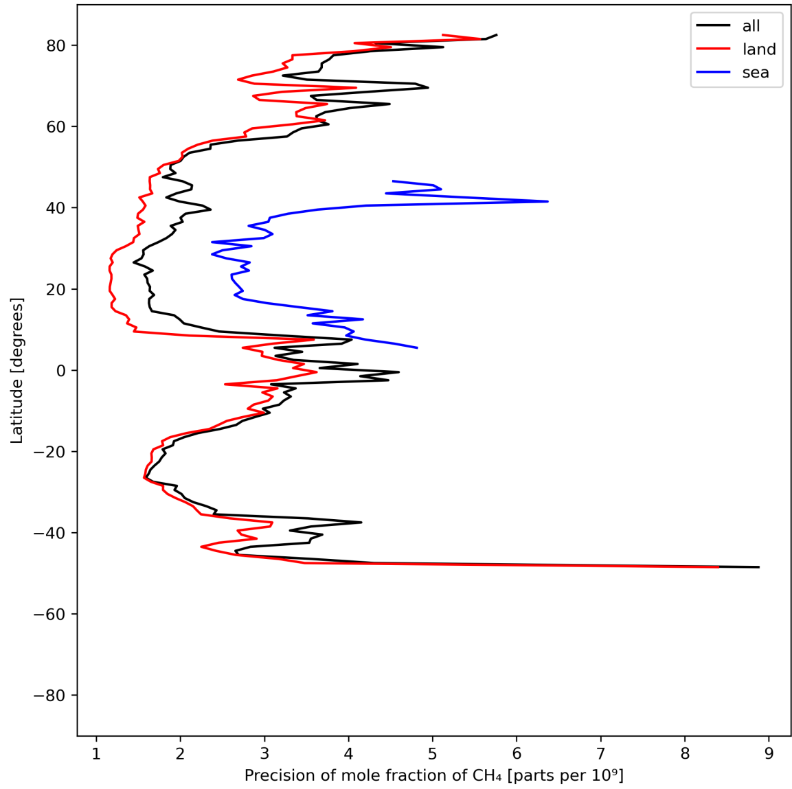
Figure 13: Zonal average of “Precision of mole fraction of CH 4 ” for 2024-05-16 to 2024-05-18.
