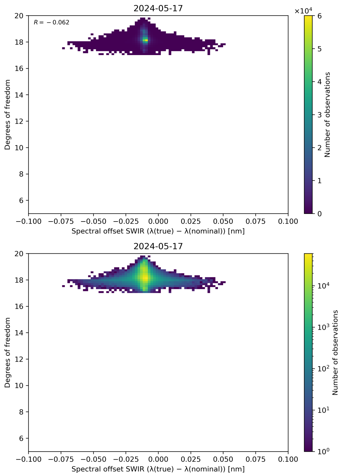
Figure 119: Scatter density plot of “Spectral offset SWIR ( \lambda(\text{true}) - \lambda(\text{nominal}) )” against “Degrees of freedom” for 2024-05-16 to 2024-05-18.
