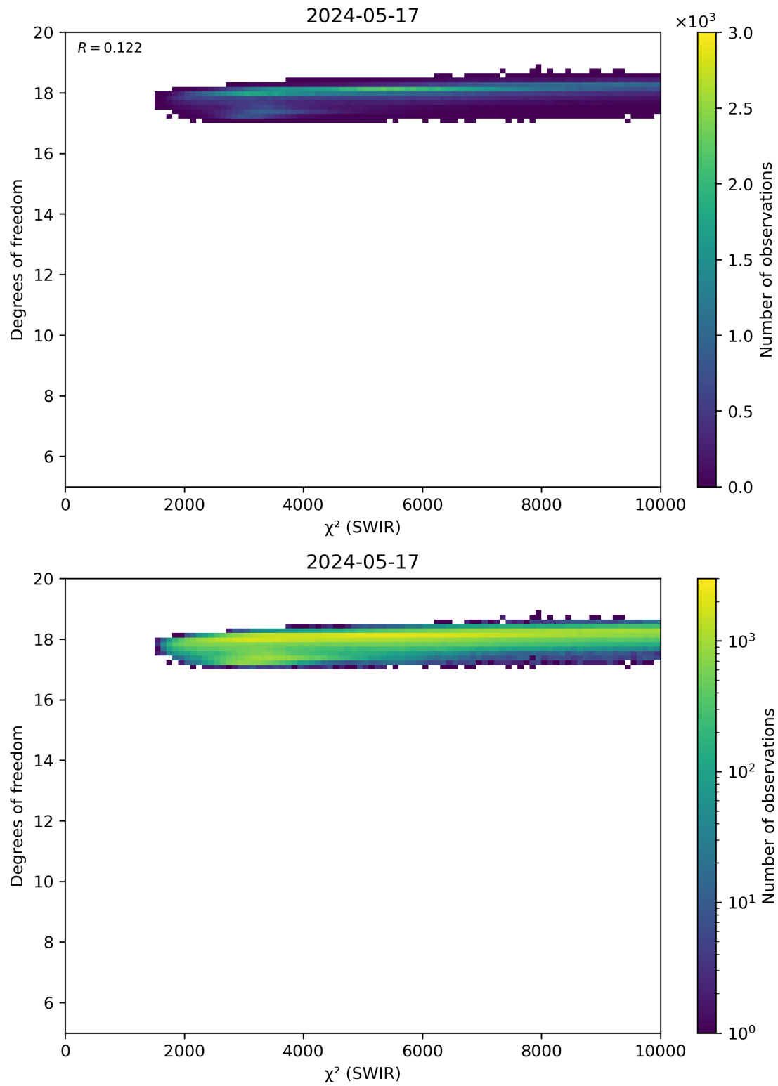
Figure 48: Scatter density plot of “ \chi^2 (SWIR)” against “Degrees of freedom” for 2024-05-16 to 2024-05-18.
