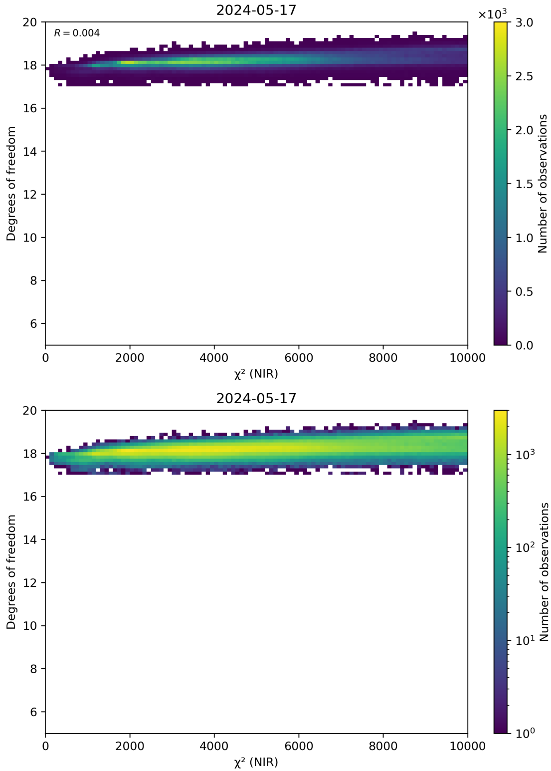
Figure 44: Scatter density plot of “ \chi^2 (NIR)” against “Degrees of freedom” for 2024-05-16 to 2024-05-18.
