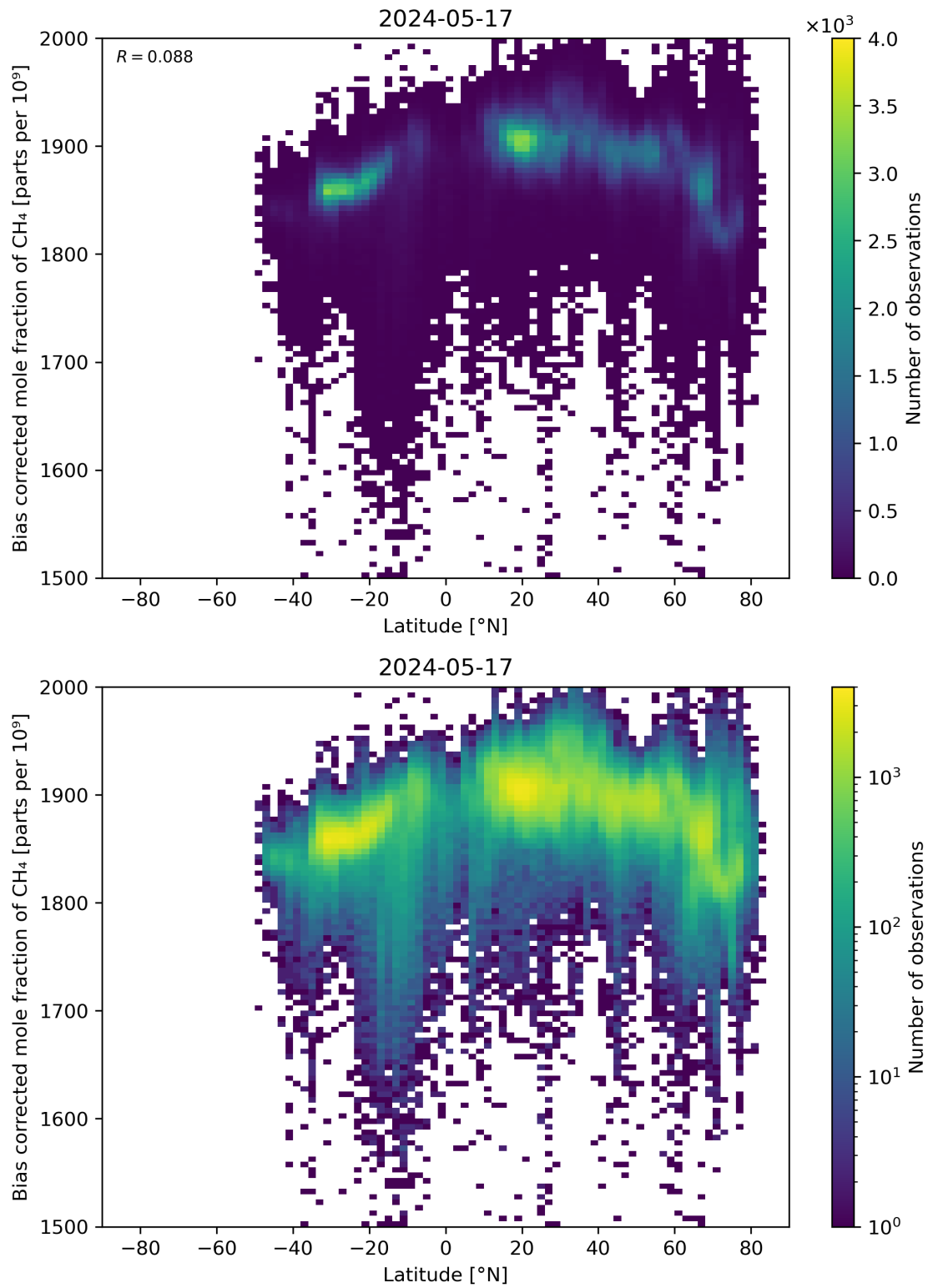
Figure 58: Scatter density plot of “Latitude” against “Bias corrected mole fraction of CH 4 ” for 2024-05-16 to 2024-05-18.
