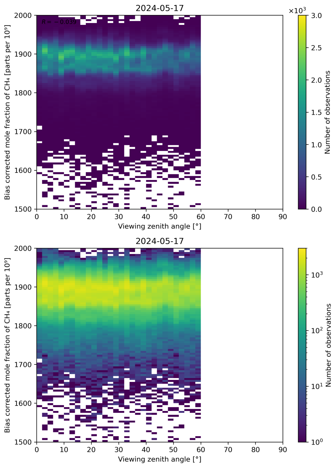
Figure 111: Scatter density plot of “Viewing zenith angle” against “Bias corrected mole fraction of CH 4 ” for 2024-05-16 to 2024-05-18.
