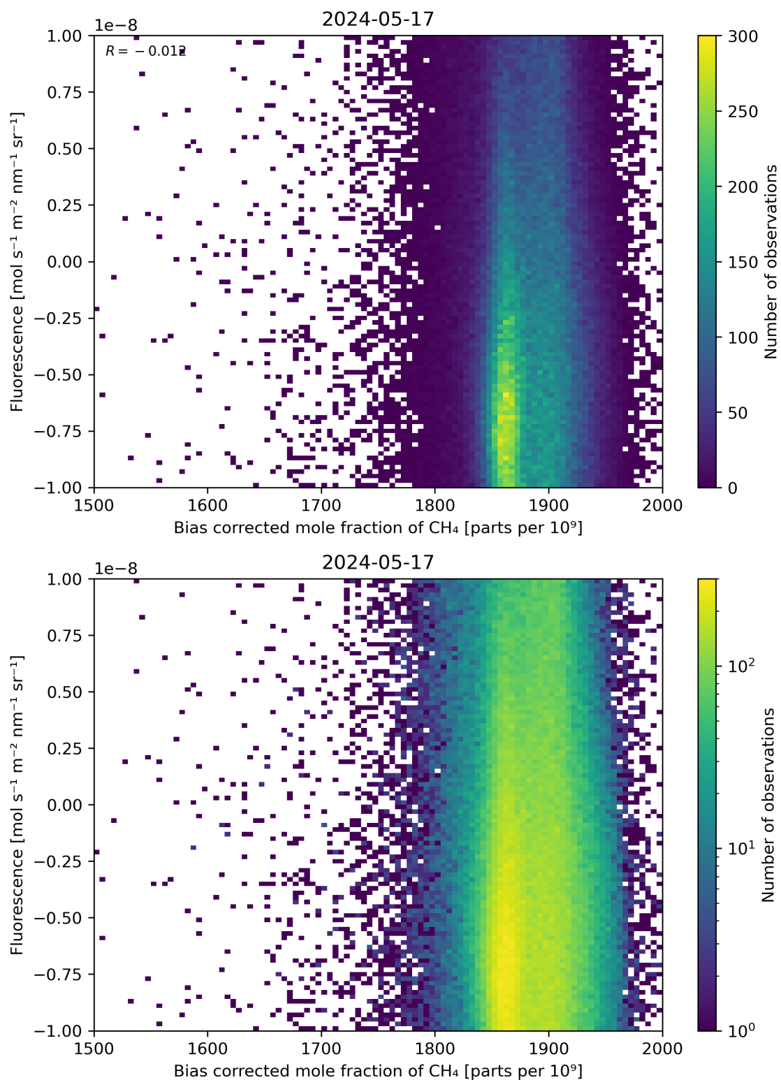
Figure 66: Scatter density plot of “Bias corrected mole fraction of \text{CH}_4 ” against “Fluorescence” for 2024-05-16 to 2024-05-18.
