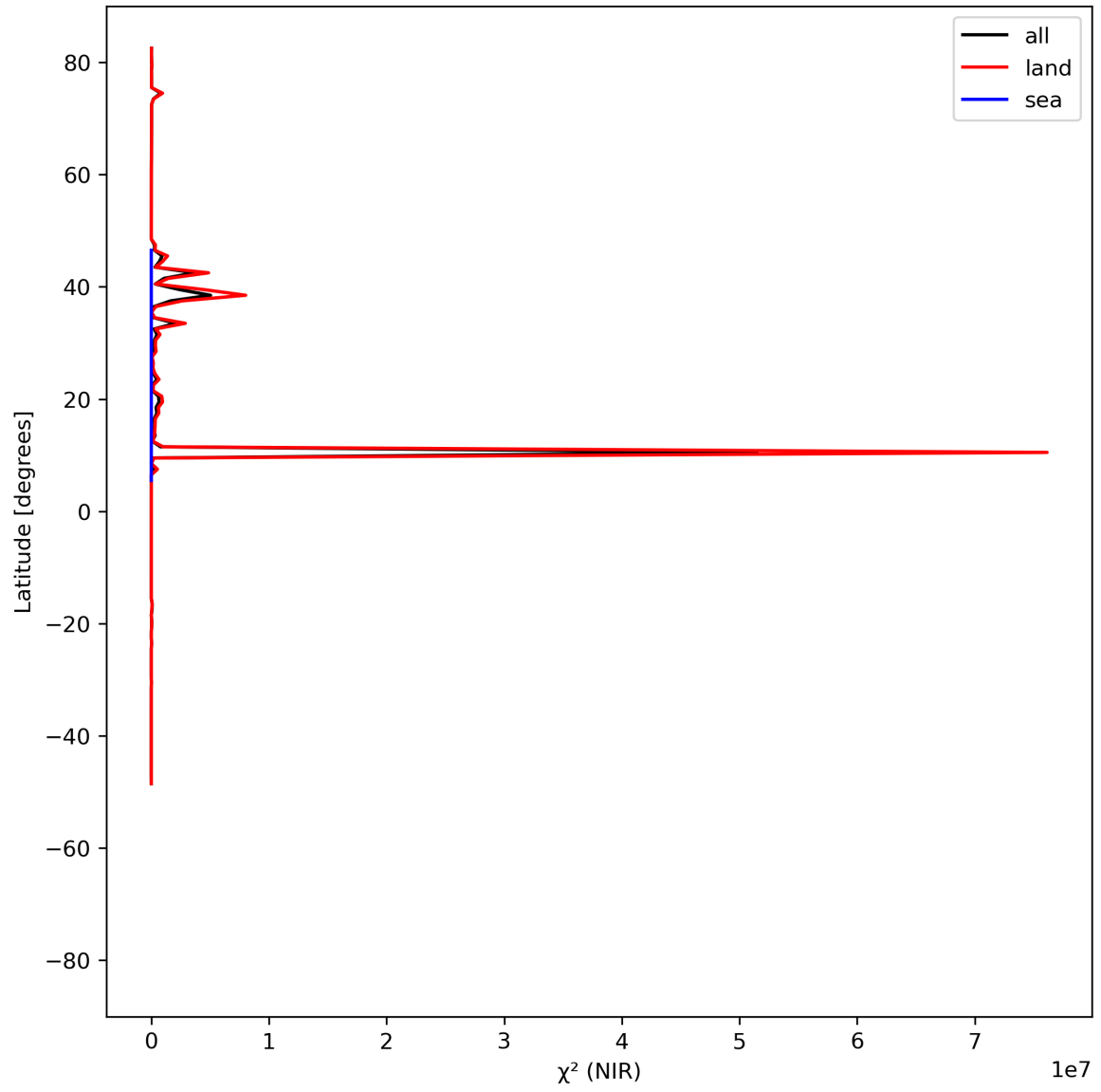
Figure 18: Zonal average of “ \chi^2 (NIR)” for 2024-05-16 to 2024-05-18.
