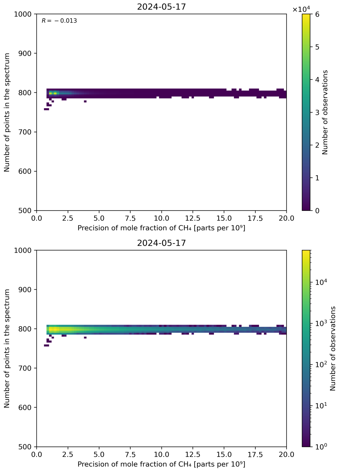
Figure 84: Scatter density plot of “Precision of mole fraction of CH 4 ” against “Number of points in the spectrum” for 2024-05-16 to 2024-05-18.
