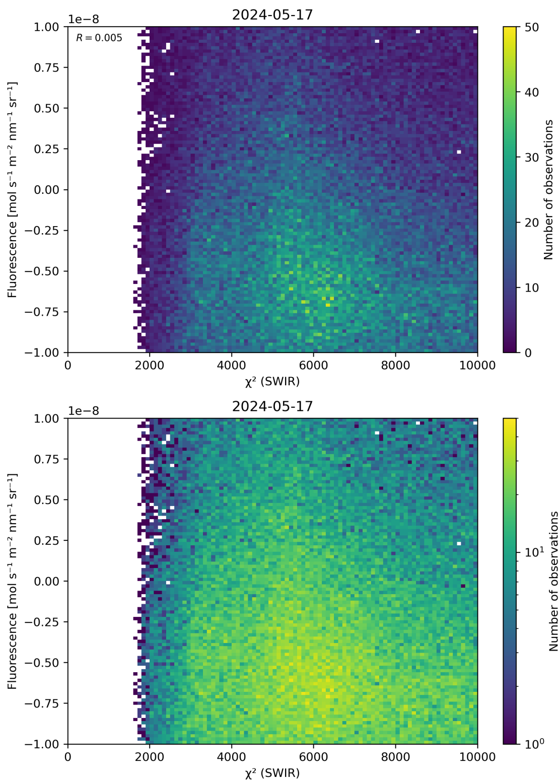
Figure 49: Scatter density plot of “ \chi^2 (SWIR)” against “Fluorescence” for 2024-05-16 to 2024-05-18.
