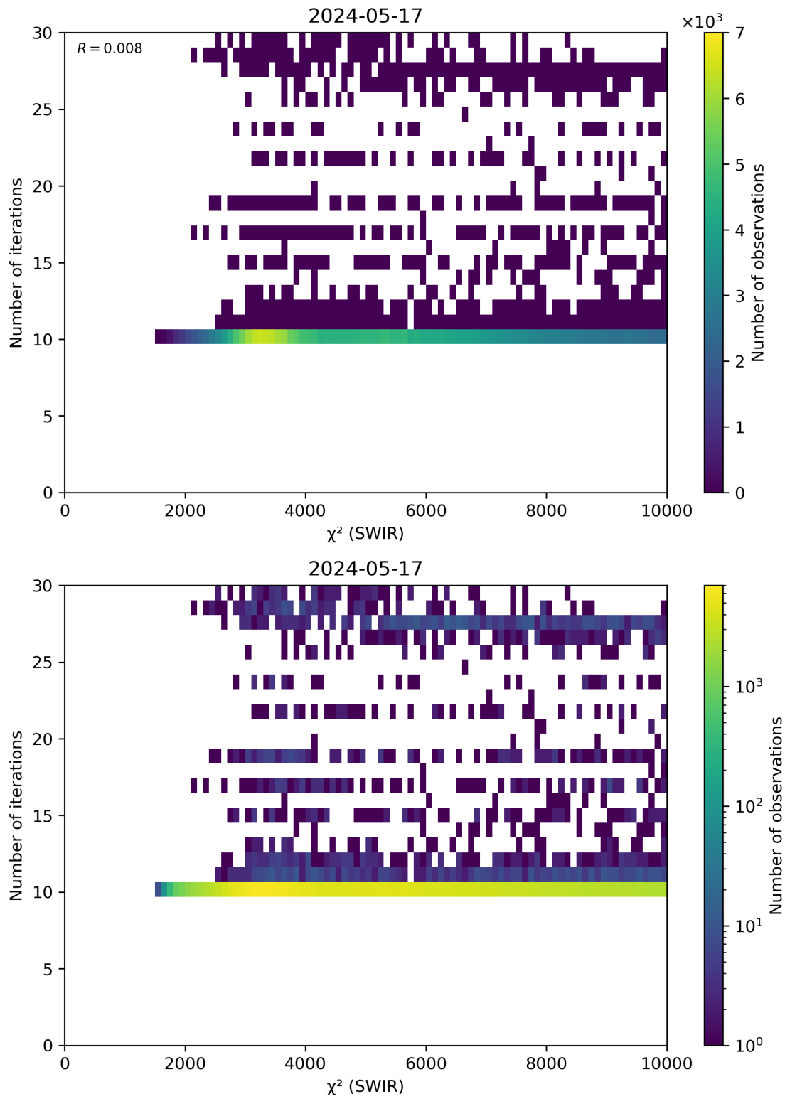
Figure 50: Scatter density plot of “ \chi^2 (SWIR)” against “Number of iterations” for 2024-05-16 to 2024-05-18.
