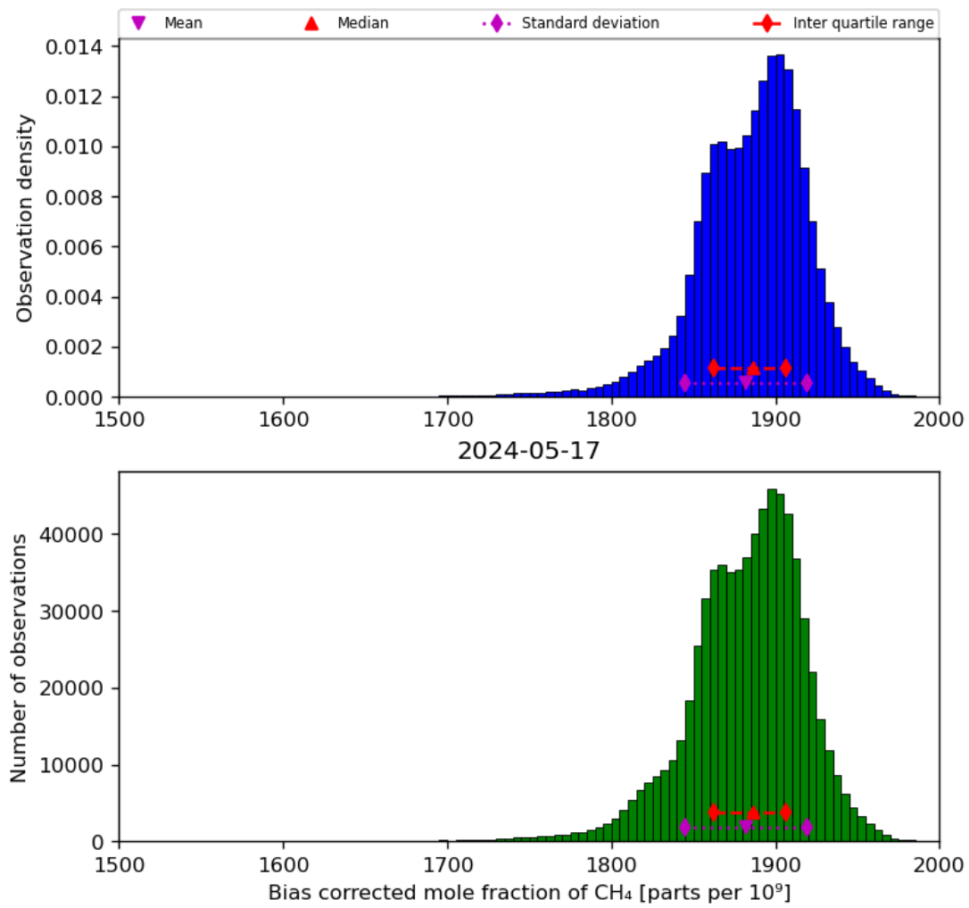
Figure 25: Histogram of “Bias corrected mole fraction of CH 4 ” for 2024-05-16 to 2024-05-18
