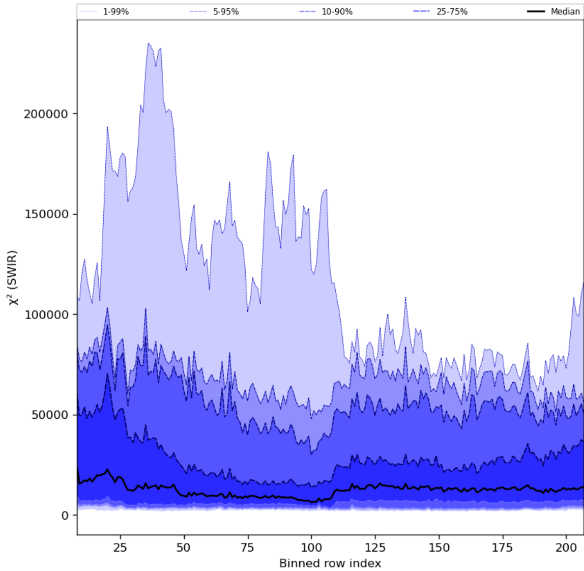
Figure 39: Along track statistics of “ \chi^2 (SWIR)” for 2024-05-16 to 2024-05-18
