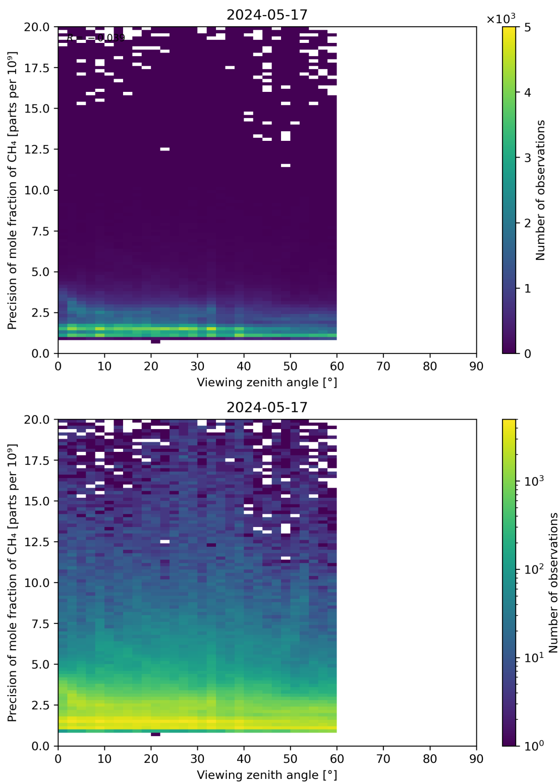
Figure 112: Scatter density plot of “Viewing zenith angle” against “Precision of mole fraction of CH 4 ” for 2024-05-16 to 2024-05-18.
