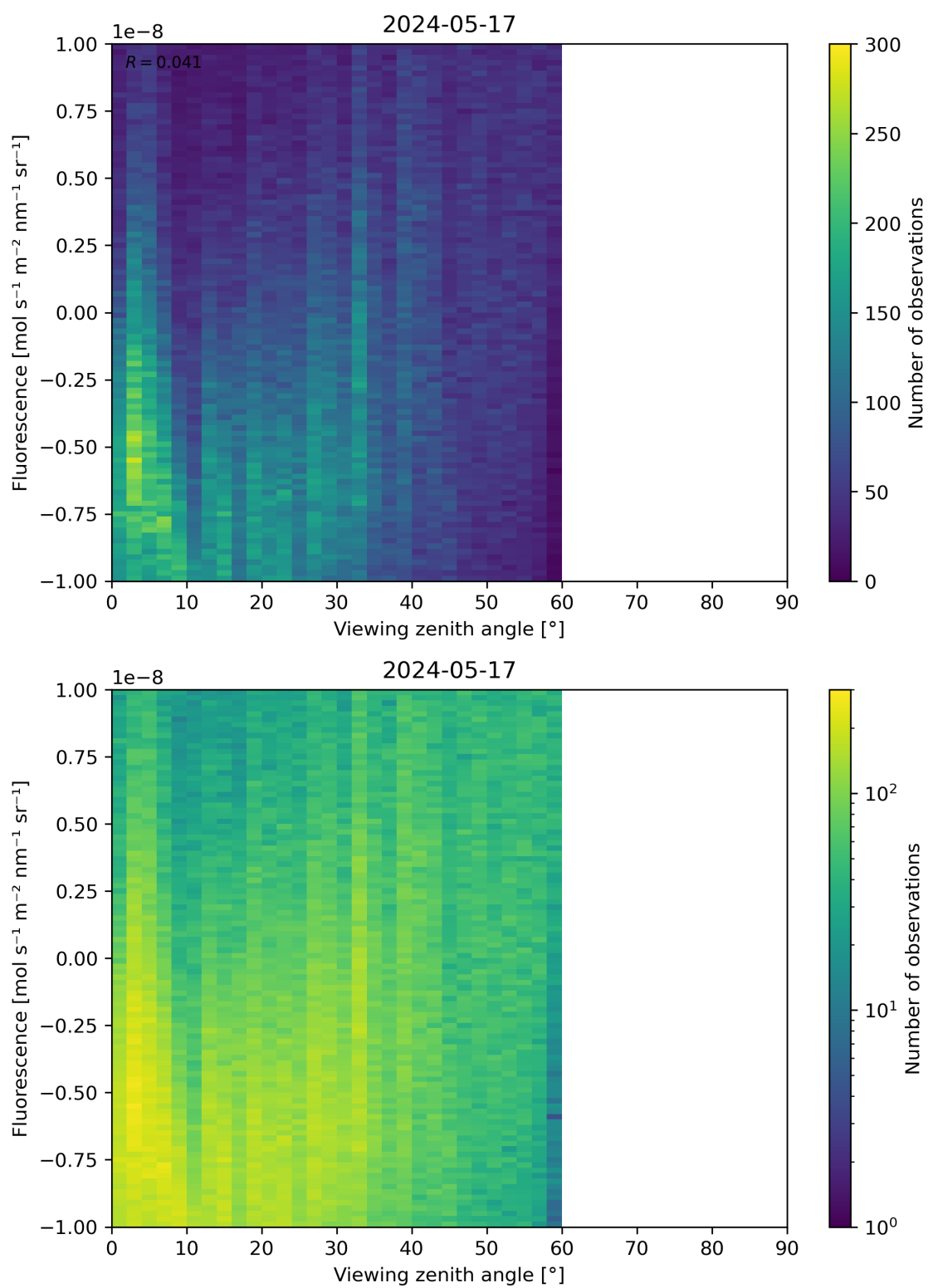
Figure 108: Scatter density plot of “Viewing zenith angle” against “Fluorescence” for 2024-05-16 to 2024-05-18.
