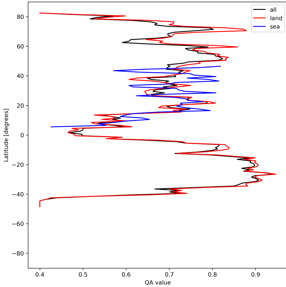
Figure 11: Zonal average of “QA value” for 2024-05-16 to 2024-05-18.
