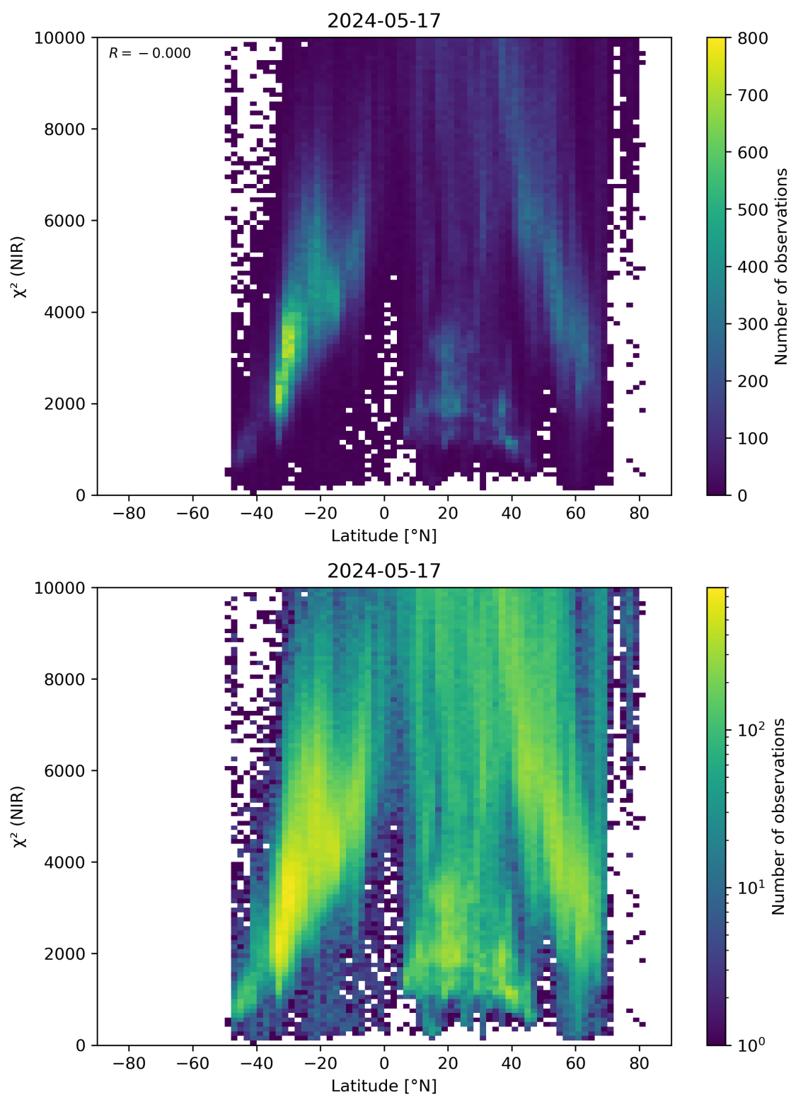
Figure 53: Scatter density plot of “Latitude” against “ \chi^2 (NIR)” for 2024-05-16 to 2024-05-18.
