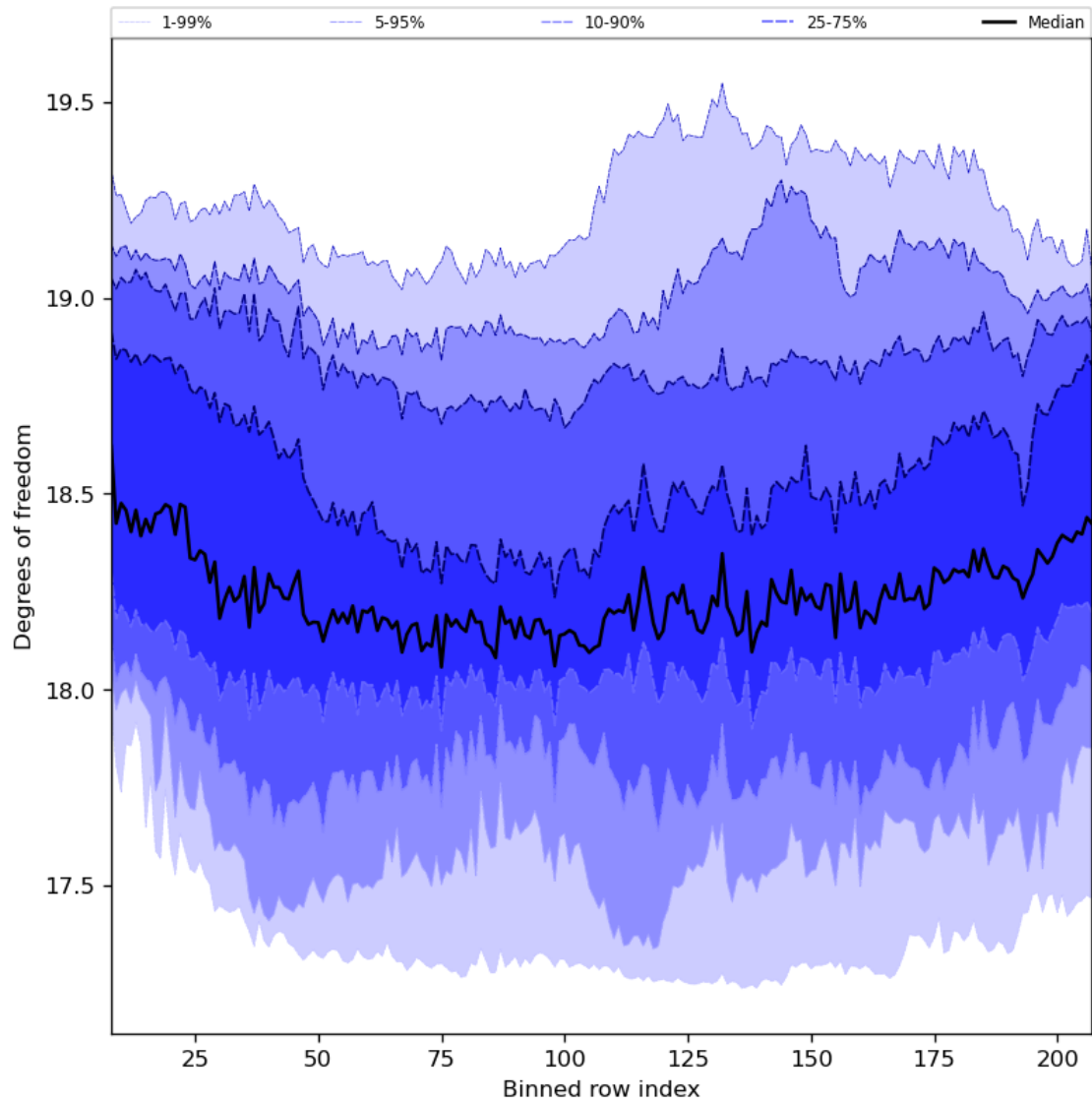
Figure 41: Along track statistics of “Degrees of freedom” for 2024-05-16 to 2024-05-18
