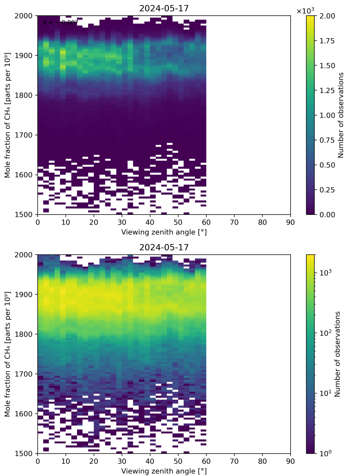
Figure 110: Scatter density plot of “Viewing zenith angle” against “Mole fraction of CH 4 ” for 2024-05-16 to 2024-05-18.
