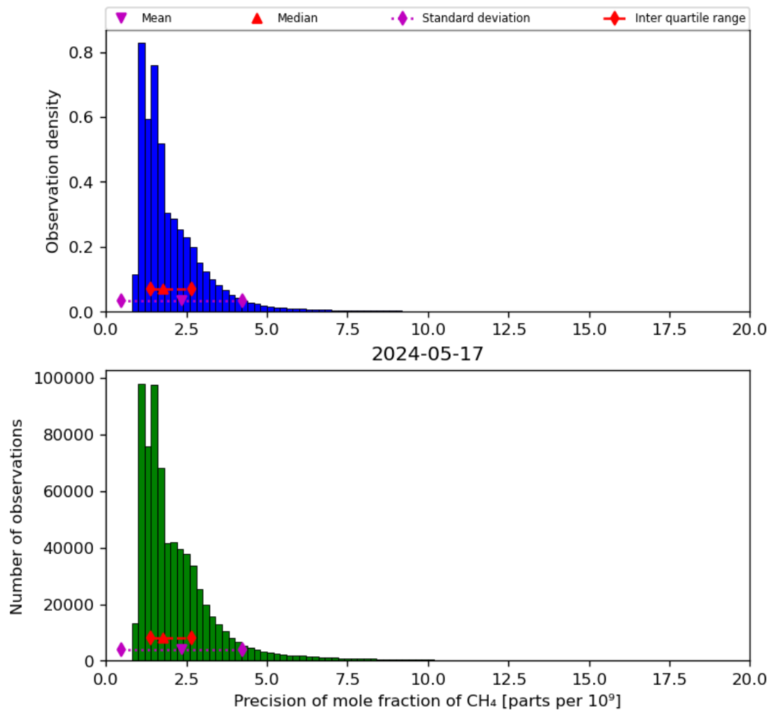
Figure 24: Histogram of “Precision of mole fraction of CH 4 ” for 2024-05-16 to 2024-05-18
