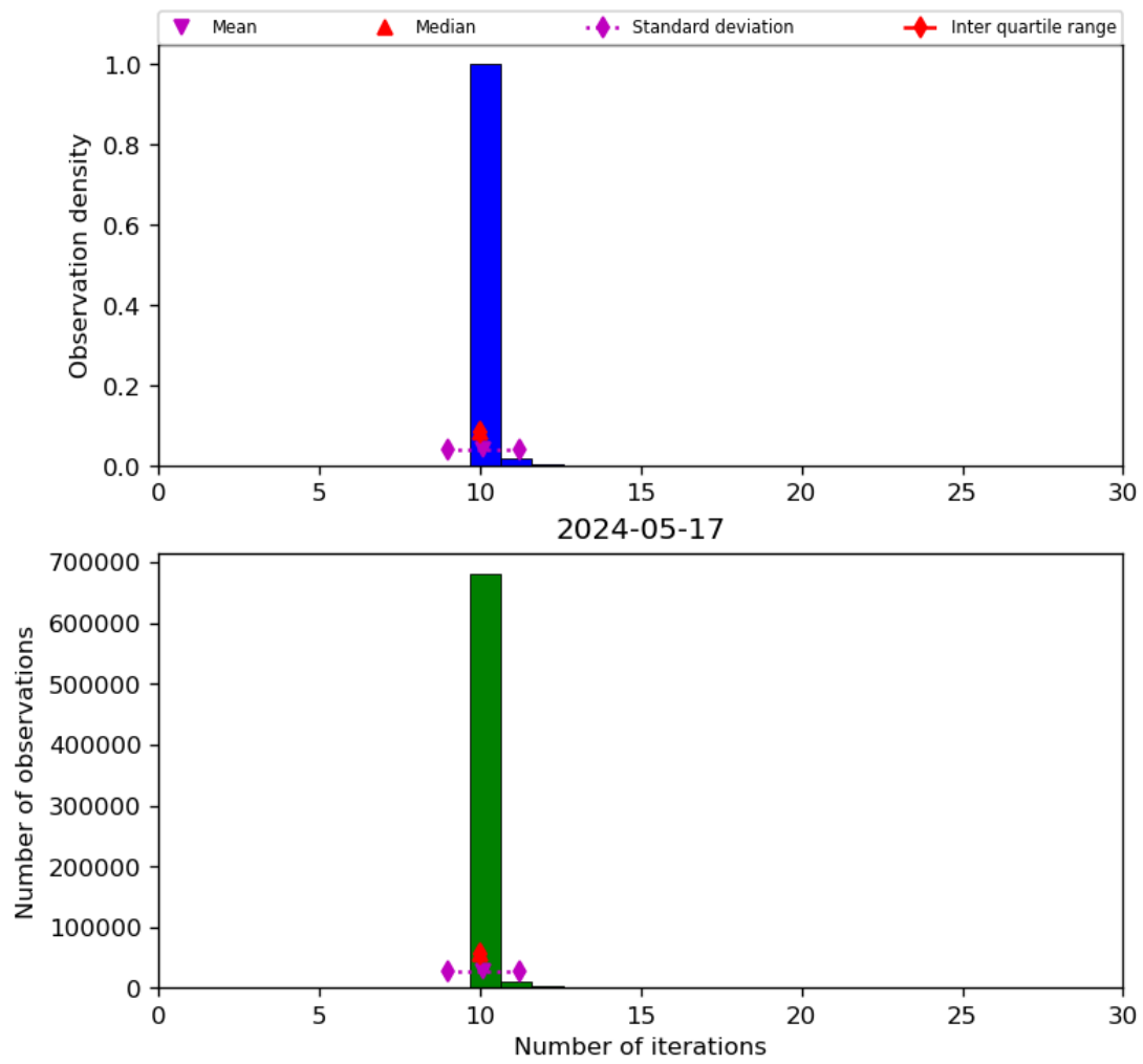
Figure 31: Histogram of “Number of iterations” for 2024-05-16 to 2024-05-18
