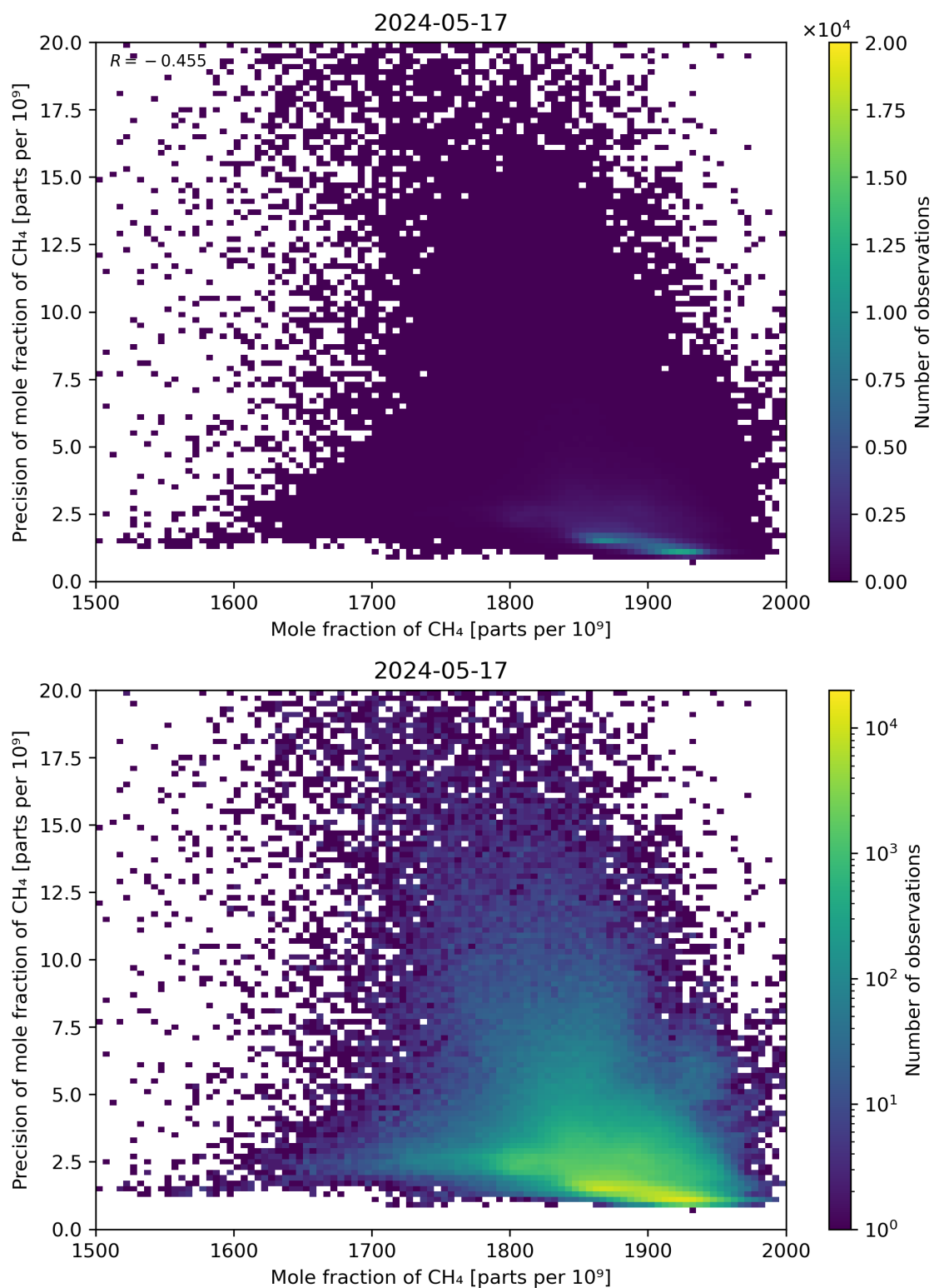
Figure 75: Scatter density plot of “Mole fraction of CH 4 ” against “Precision of mole fraction of CH 4 ” for 2024-05-16 to 2024-05-18.
