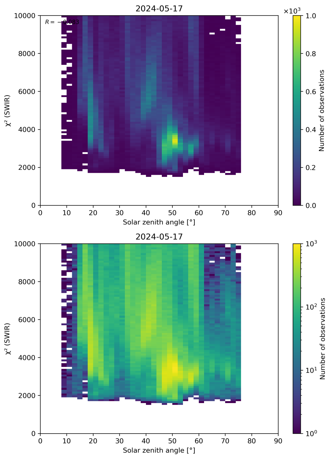
Figure 95: Scatter density plot of “Solar zenith angle” against “ \chi^2 (SWIR)” for 2024-05-16 to 2024-05-18.
