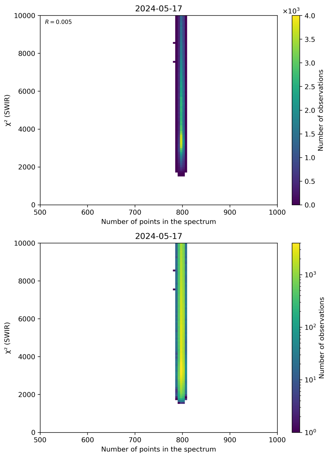
Figure 89: Scatter density plot of “Number of points in the spectrum” against “ \chi^2 (SWIR)” for 2024-05-16 to 2024-05-18.
