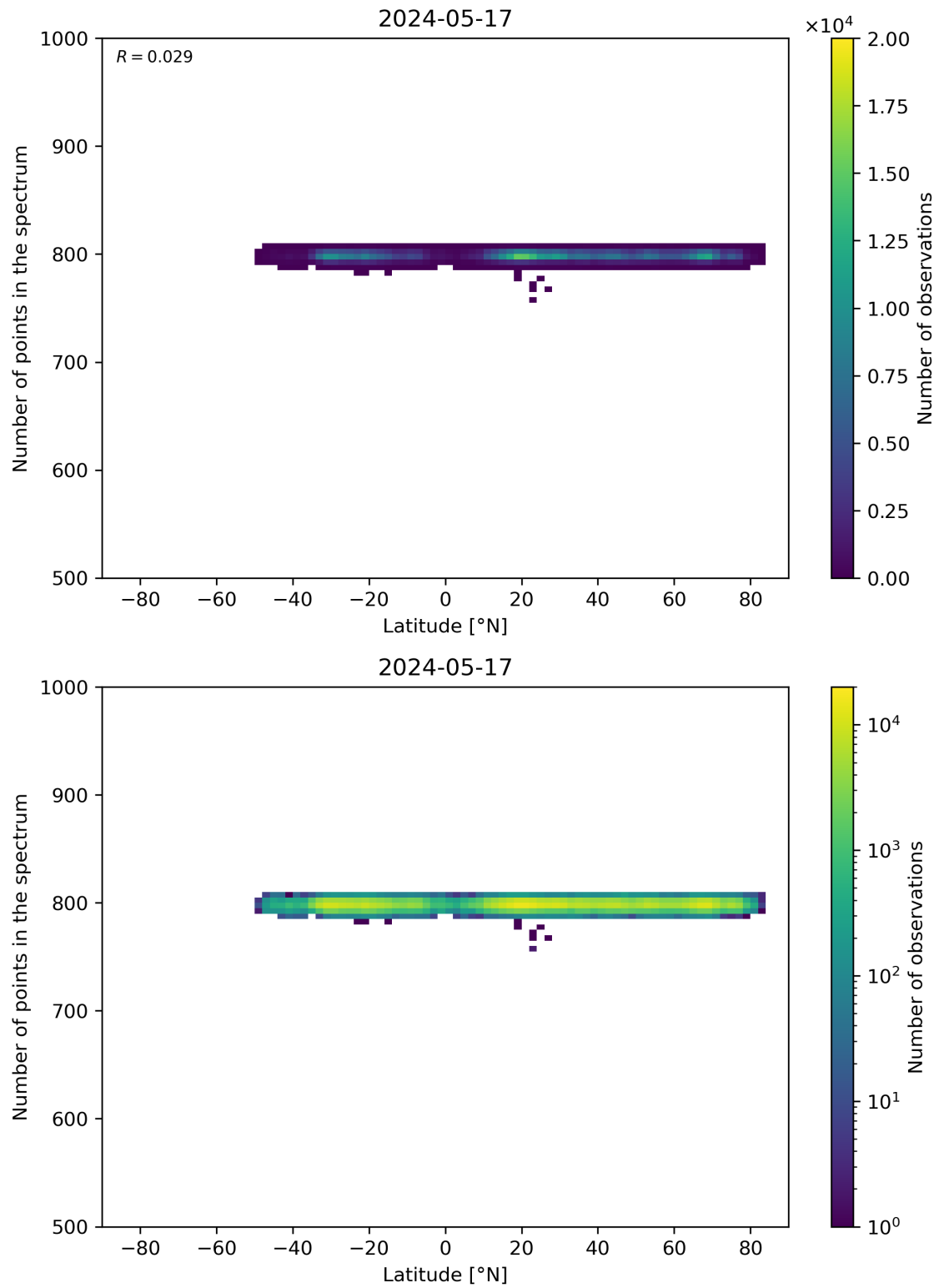
Figure 61: Scatter density plot of “Latitude” against “Number of points in the spectrum” for 2024-05-16 to 2024-05-18.
