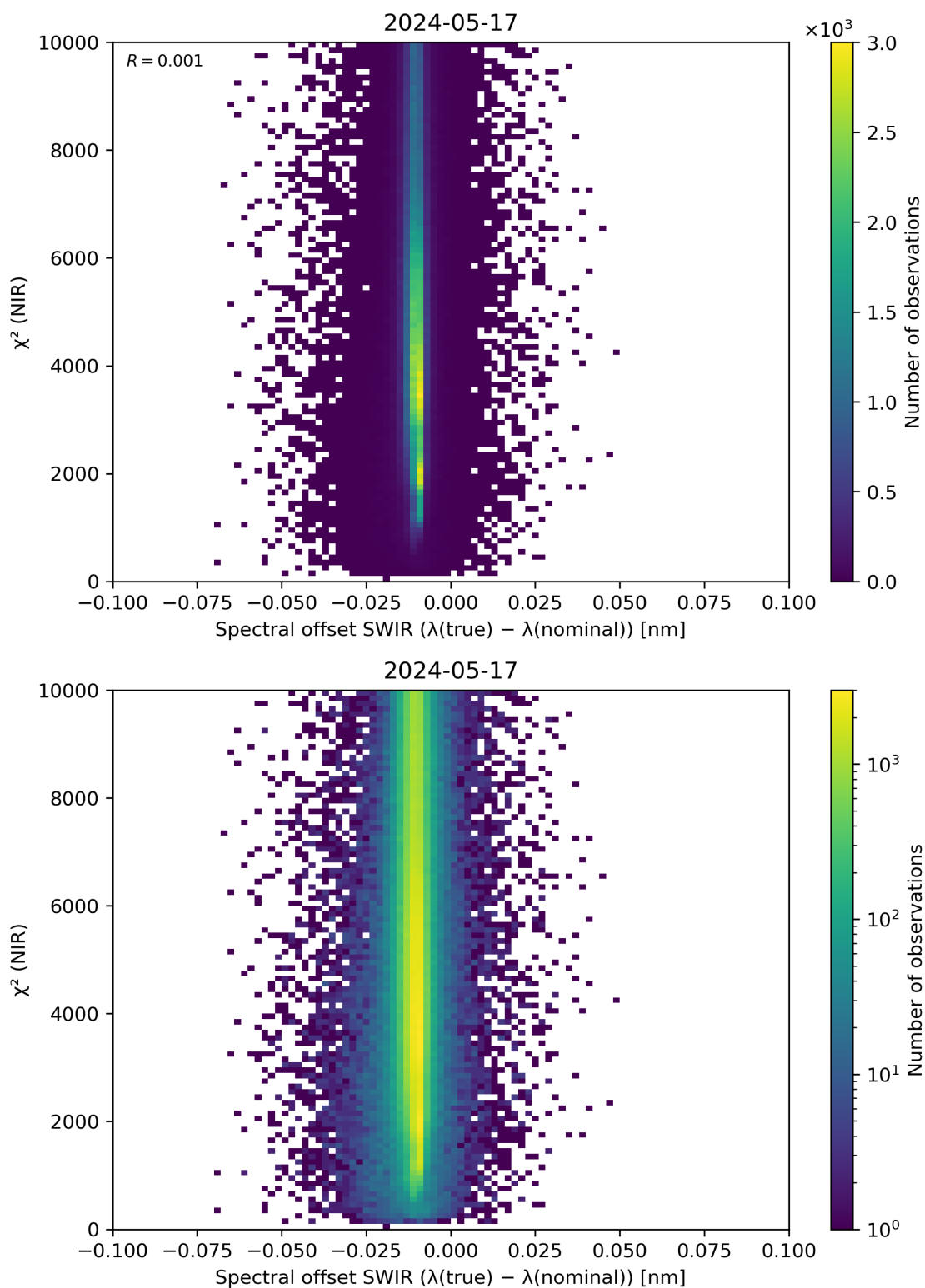
Figure 117: Scatter density plot of “Spectral offset SWIR ( \lambda(\text{true}) - \lambda(\text{nominal}) )” against “ \chi^2 (NIR)” for 2024-05-16 to 2024-05-18.
