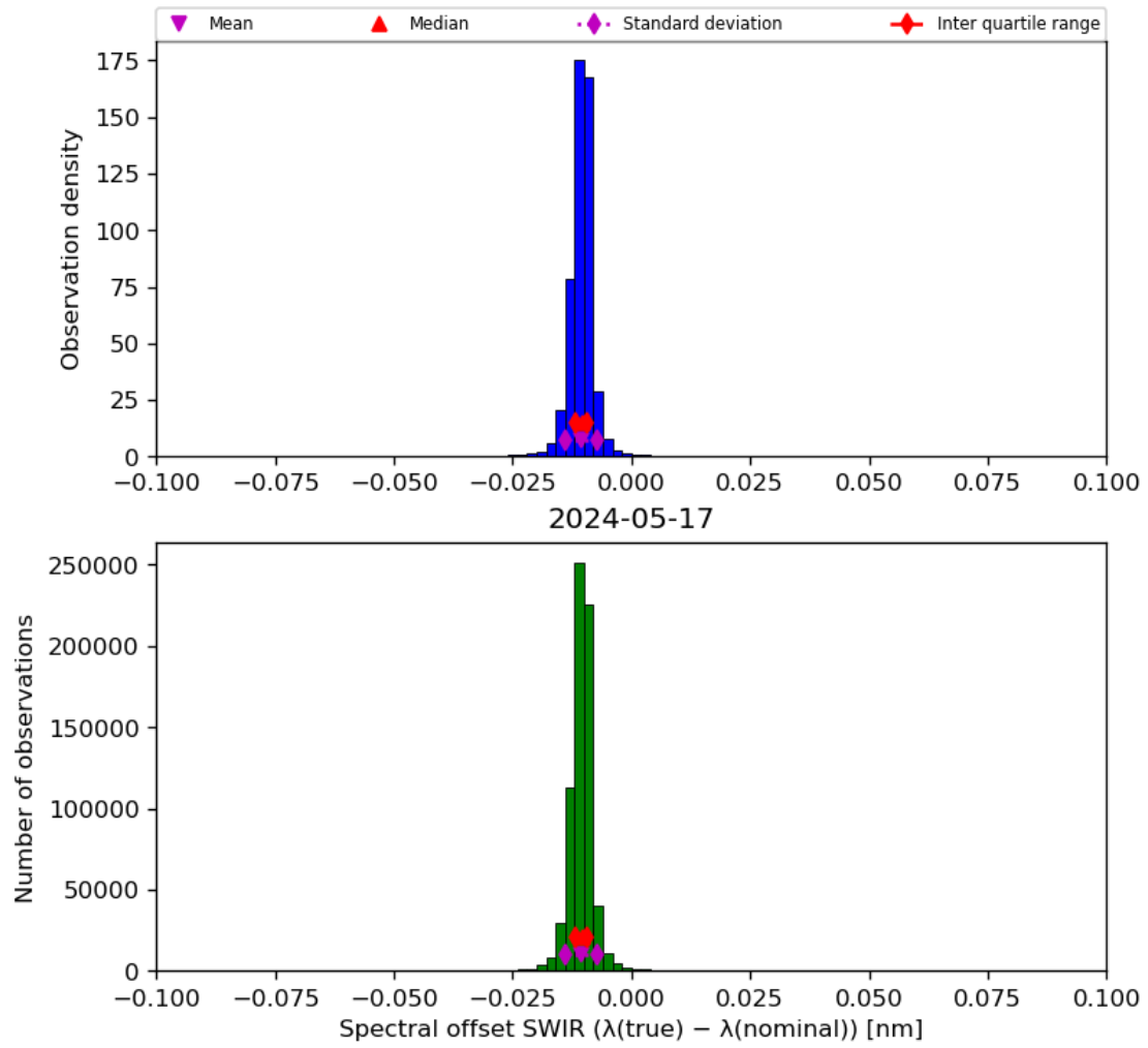
Figure 27: Histogram of “Spectral offset SWIR ( \lambda(\text{true}) - \lambda(\text{nominal}) )” for 2024-05-16 to 2024-05-18
