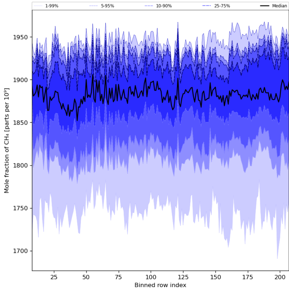
Figure 34: Along track statistics of “Mole fraction of CH 4 ” for 2024-05-16 to 2024-05-18
