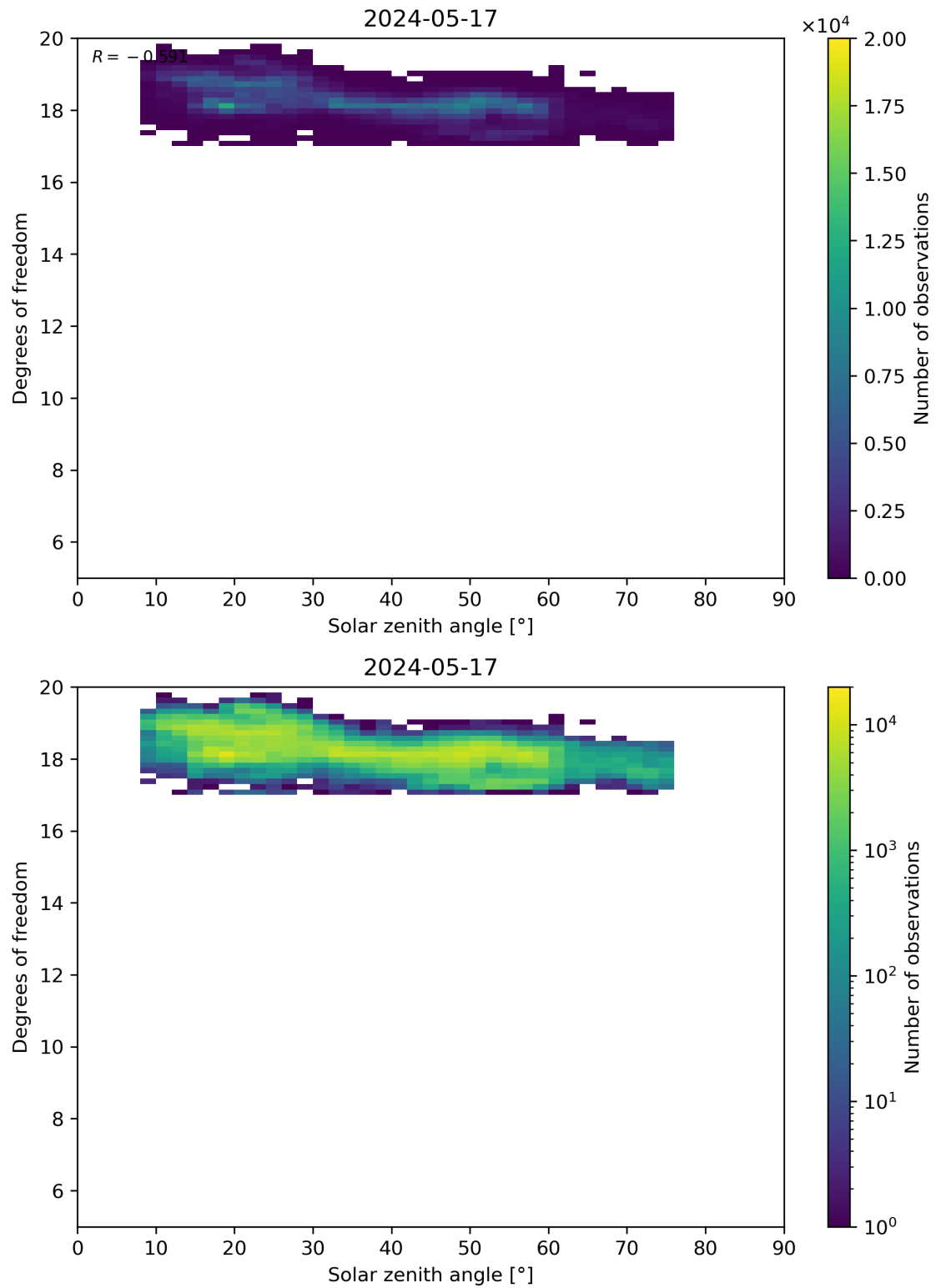
Figure 96: Scatter density plot of “Solar zenith angle” against “Degrees of freedom” for 2024-05-16 to 2024-05-18.
