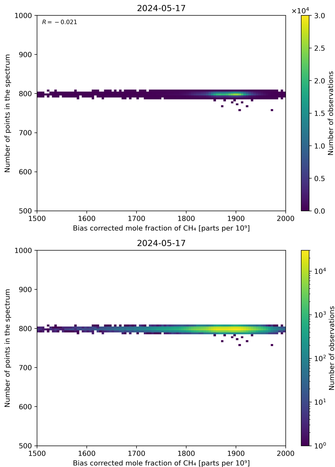
Figure 68: Scatter density plot of “Bias corrected mole fraction of CH 4 ” against “Number of points in the spectrum” for 2024-05-16 to 2024-05-18.
