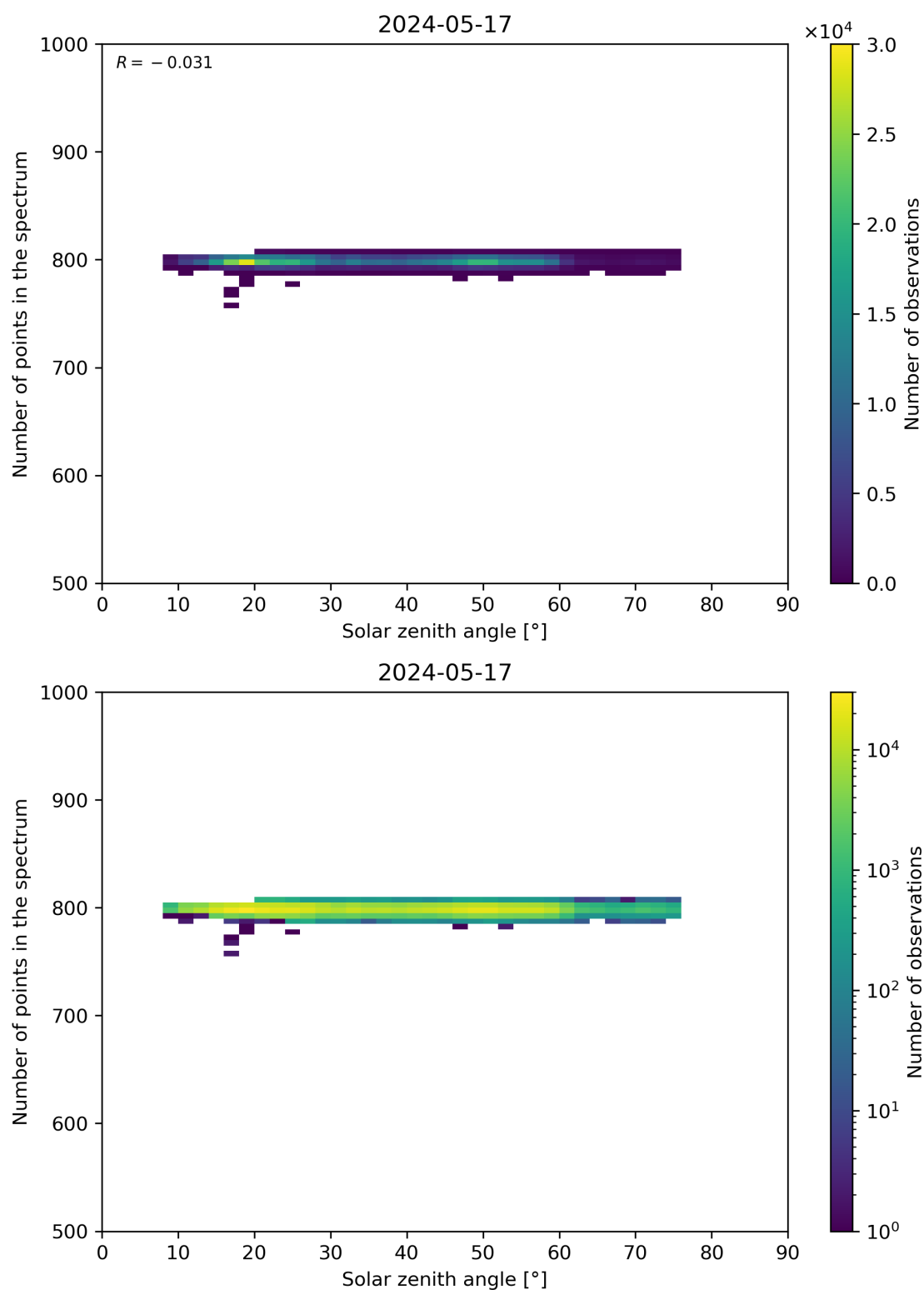
Figure 103: Scatter density plot of “Solar zenith angle” against “Number of points in the spectrum” for 2024-05-16 to 2024-05-18.
