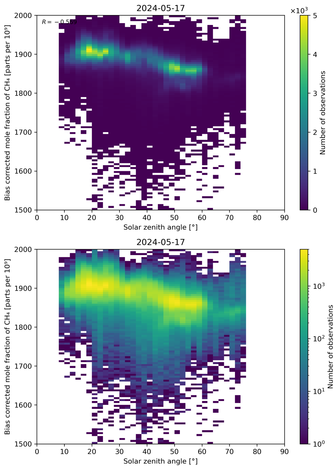
Figure 100: Scatter density plot of “Solar zenith angle” against “Bias corrected mole fraction of CH 4 ” for 2024-05-16 to 2024-05-18.
