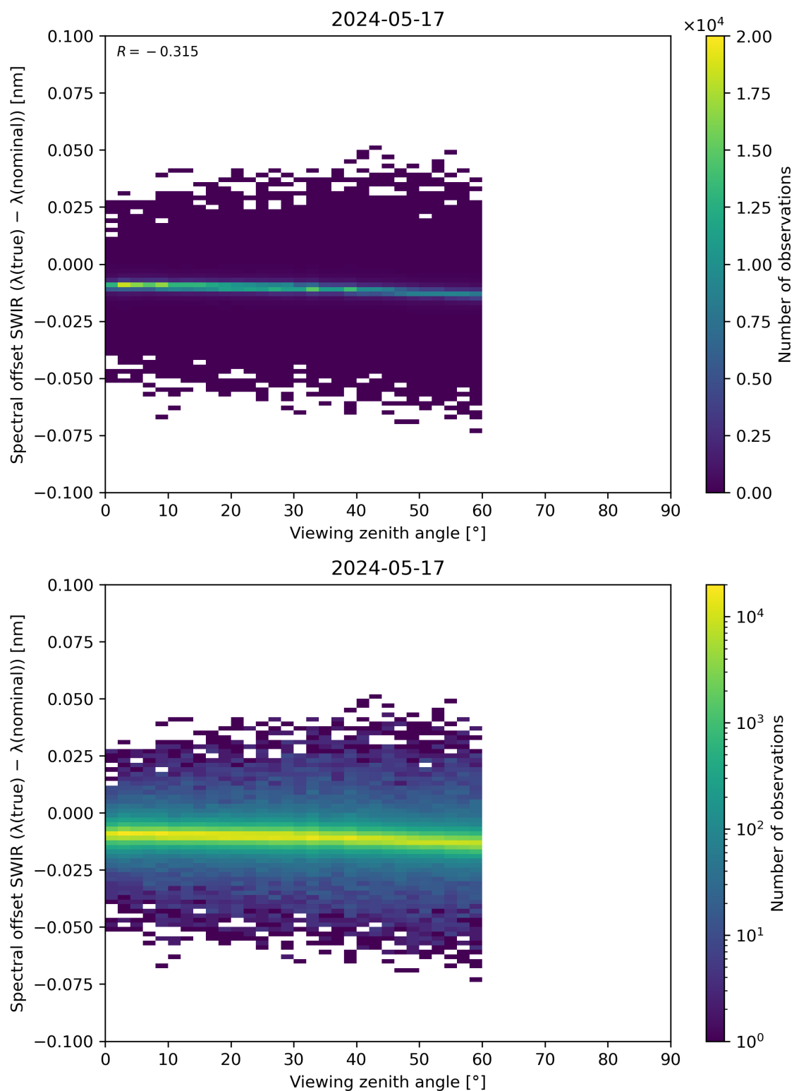
Figure 116: Scatter density plot of “Viewing zenith angle” against “Spectral offset SWIR ( \lambda(\text{true}) - \lambda(\text{nominal}) )” for 2024-05-16 to 2024-05-18.
