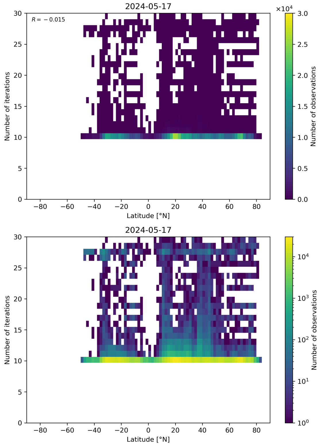
Figure 60: Scatter density plot of “Latitude” against “Number of iterations” for 2024-05-16 to 2024-05-18.
