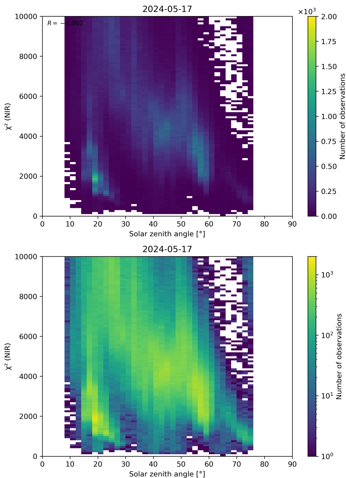
Figure 94: Scatter density plot of “Solar zenith angle” against “ \chi^2 (NIR)” for 2024-05-16 to 2024-05-18.
