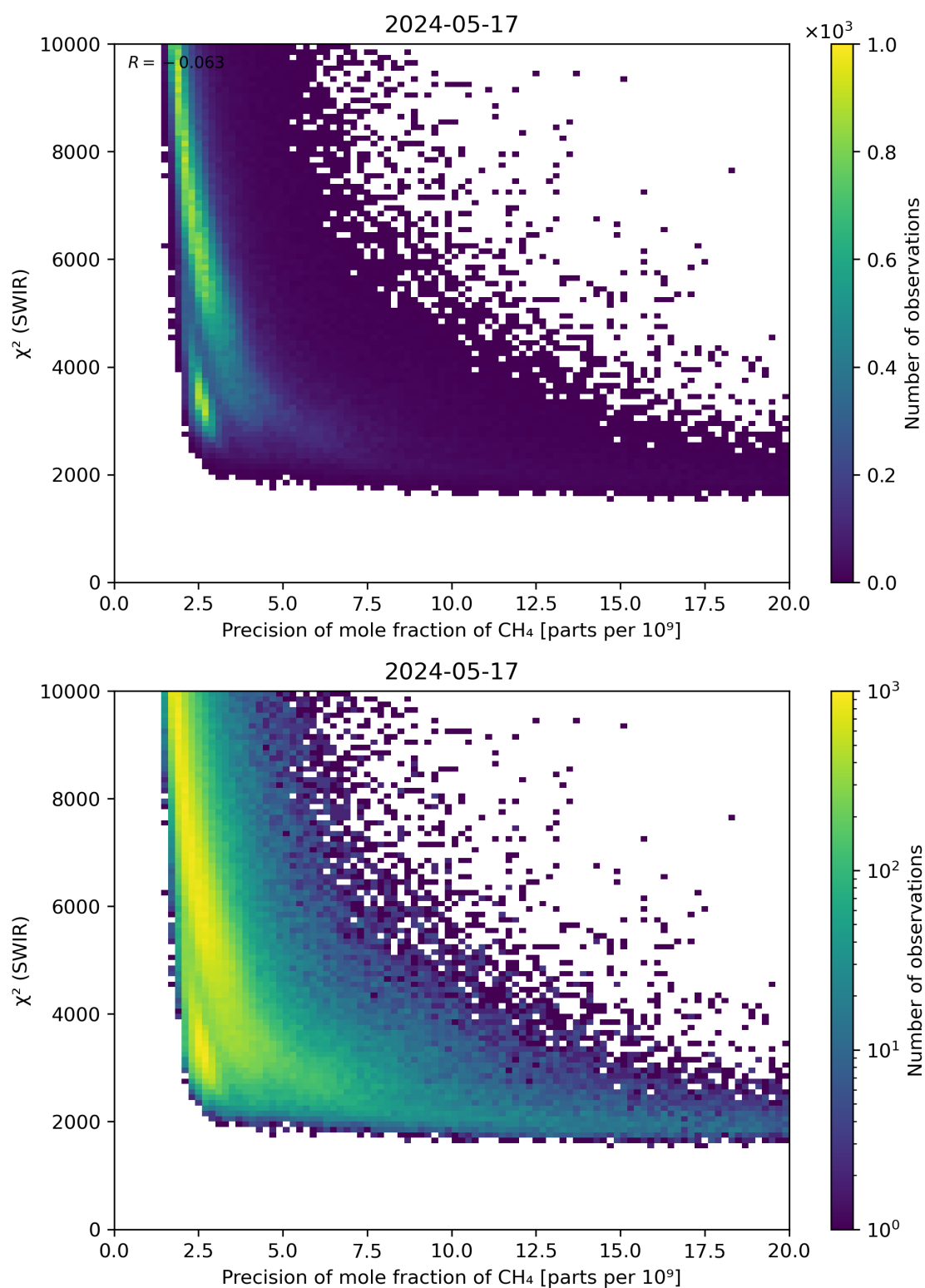
Figure 79: Scatter density plot of “Precision of mole fraction of \text{CH}_4 ” against “ \chi^2 (SWIR)” for 2024-05-16 to 2024-05-18.
