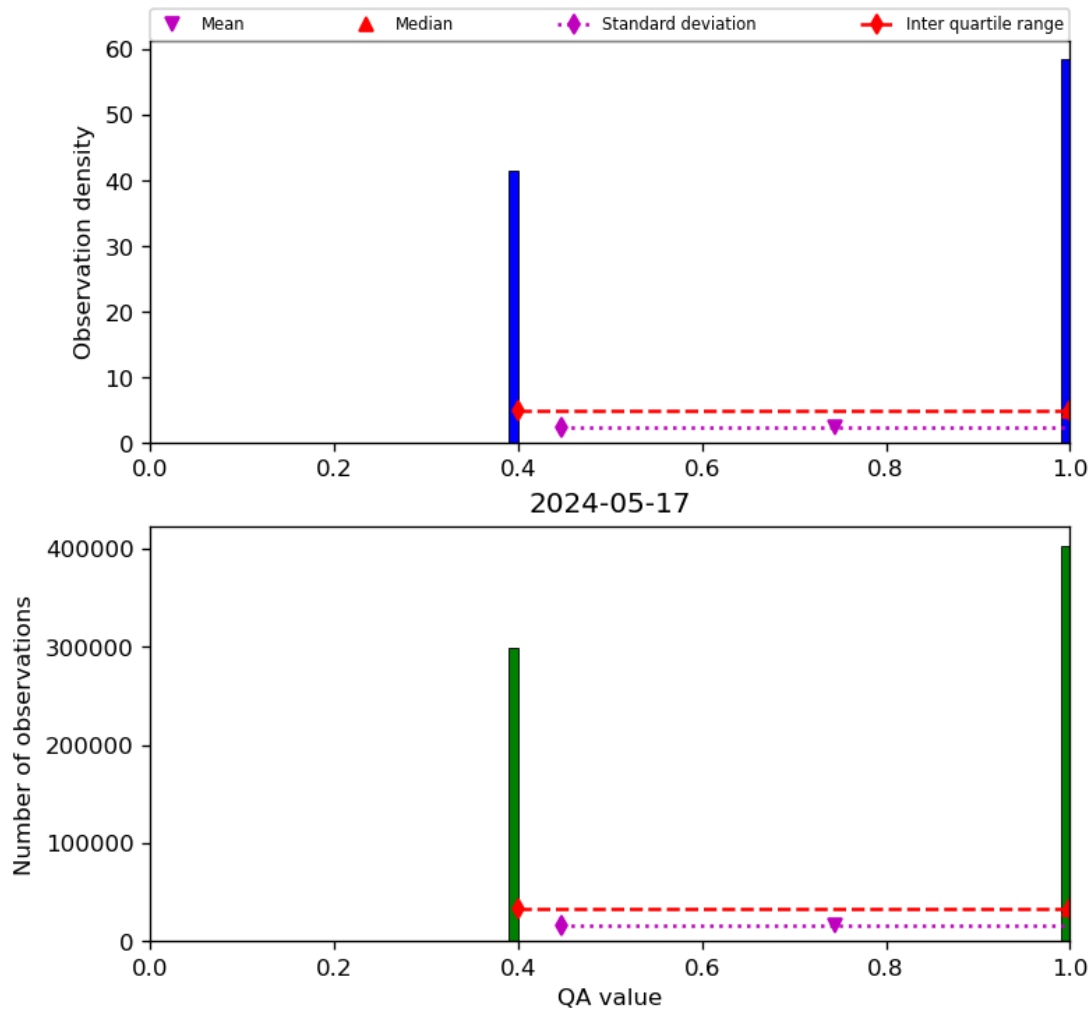
Figure 22: Histogram of “QA value” for 2024-05-16 to 2024-05-18
