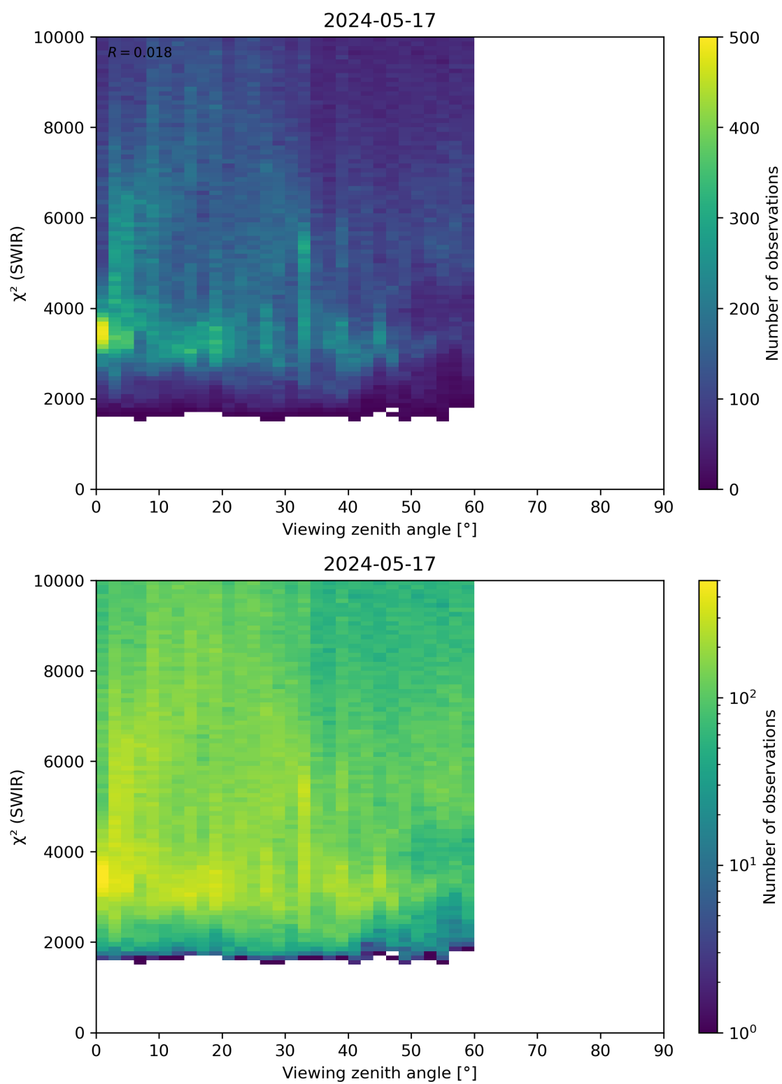
Figure 106: Scatter density plot of “Viewing zenith angle” against “ \chi^2 (SWIR)” for 2024-05-16 to 2024-05-18.
