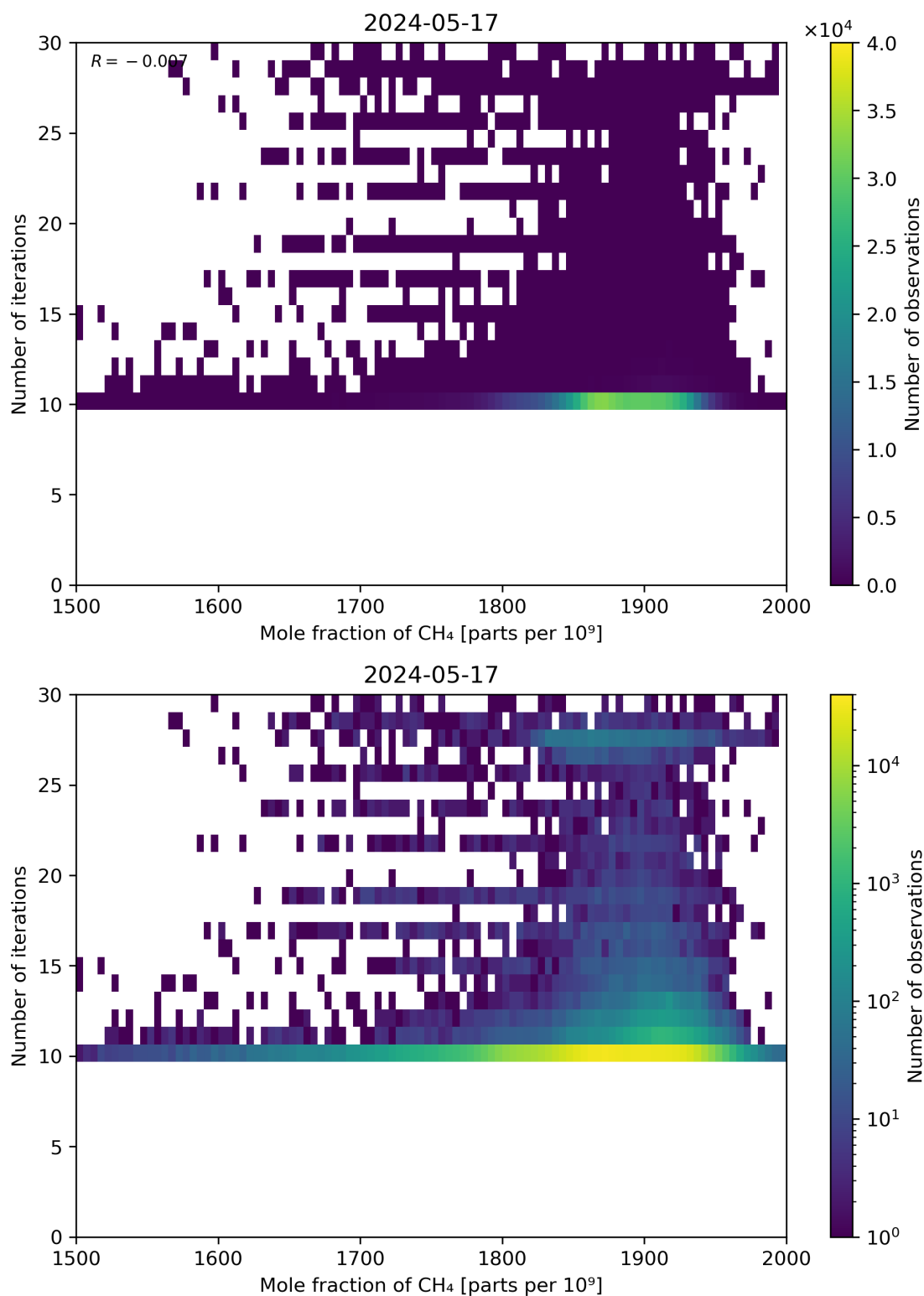
Figure 76: Scatter density plot of “Mole fraction of CH 4 ” against “Number of iterations” for 2024-05-16 to 2024-05-18.
