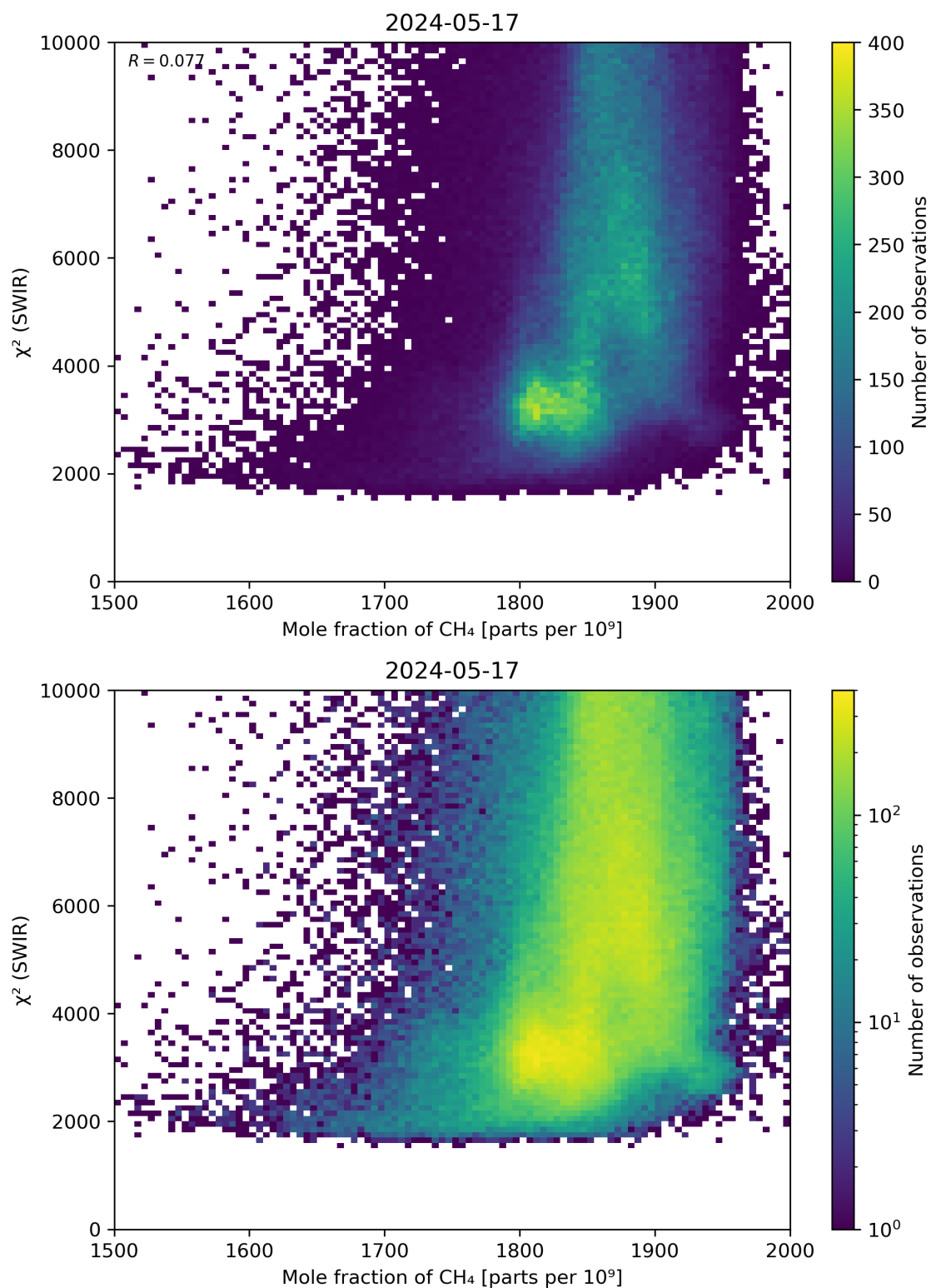
Figure 71: Scatter density plot of “Mole fraction of \text{CH}_4 ” against “ \chi^2 (SWIR)” for 2024-05-16 to 2024-05-18.
