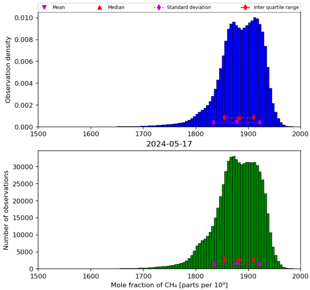
Figure 23: Histogram of “Mole fraction of CH 4 ” for 2024-05-16 to 2024-05-18
