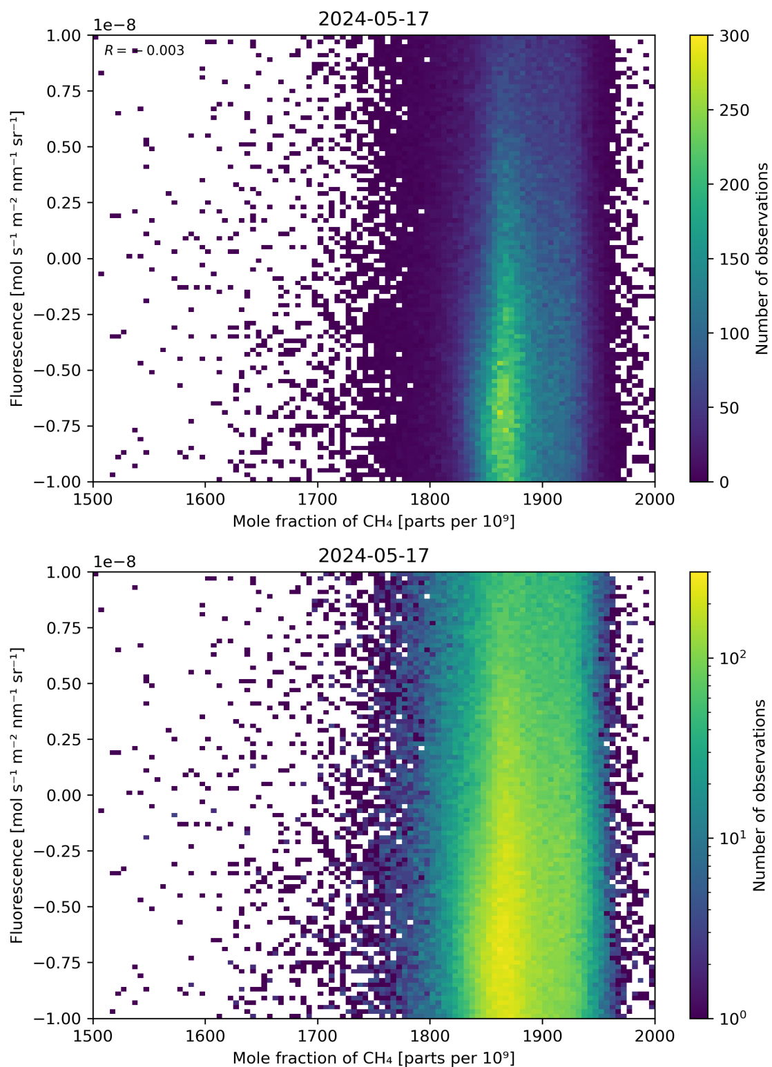
Figure 73: Scatter density plot of “Mole fraction of \text{CH}_4 ” against “Fluorescence” for 2024-05-16 to 2024-05-18.
