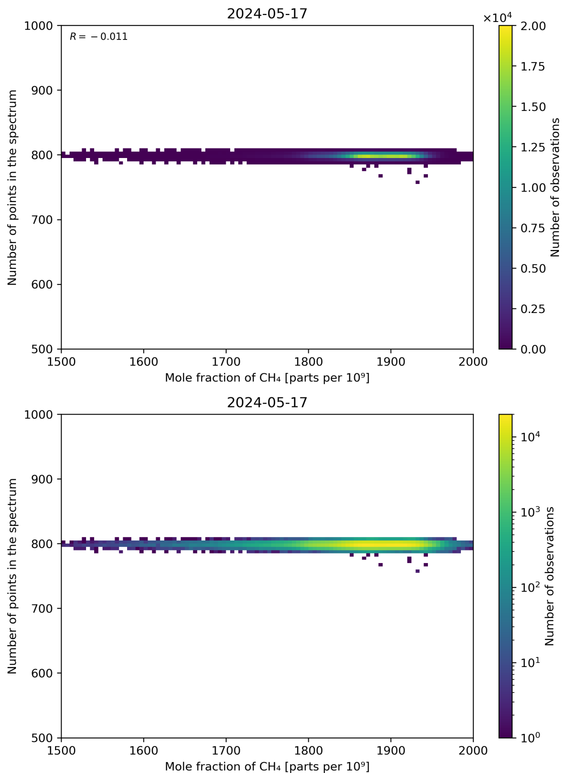
Figure 77: Scatter density plot of “Mole fraction of CH 4 ” against “Number of points in the spectrum” for 2024-05-16 to 2024-05-18.
