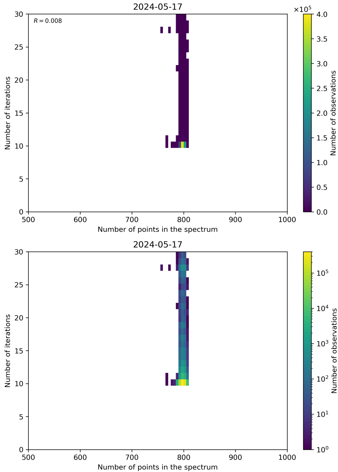
Figure 92: Scatter density plot of “Number of points in the spectrum” against “Number of iterations” for 2024-05-16 to 2024-05-18.
