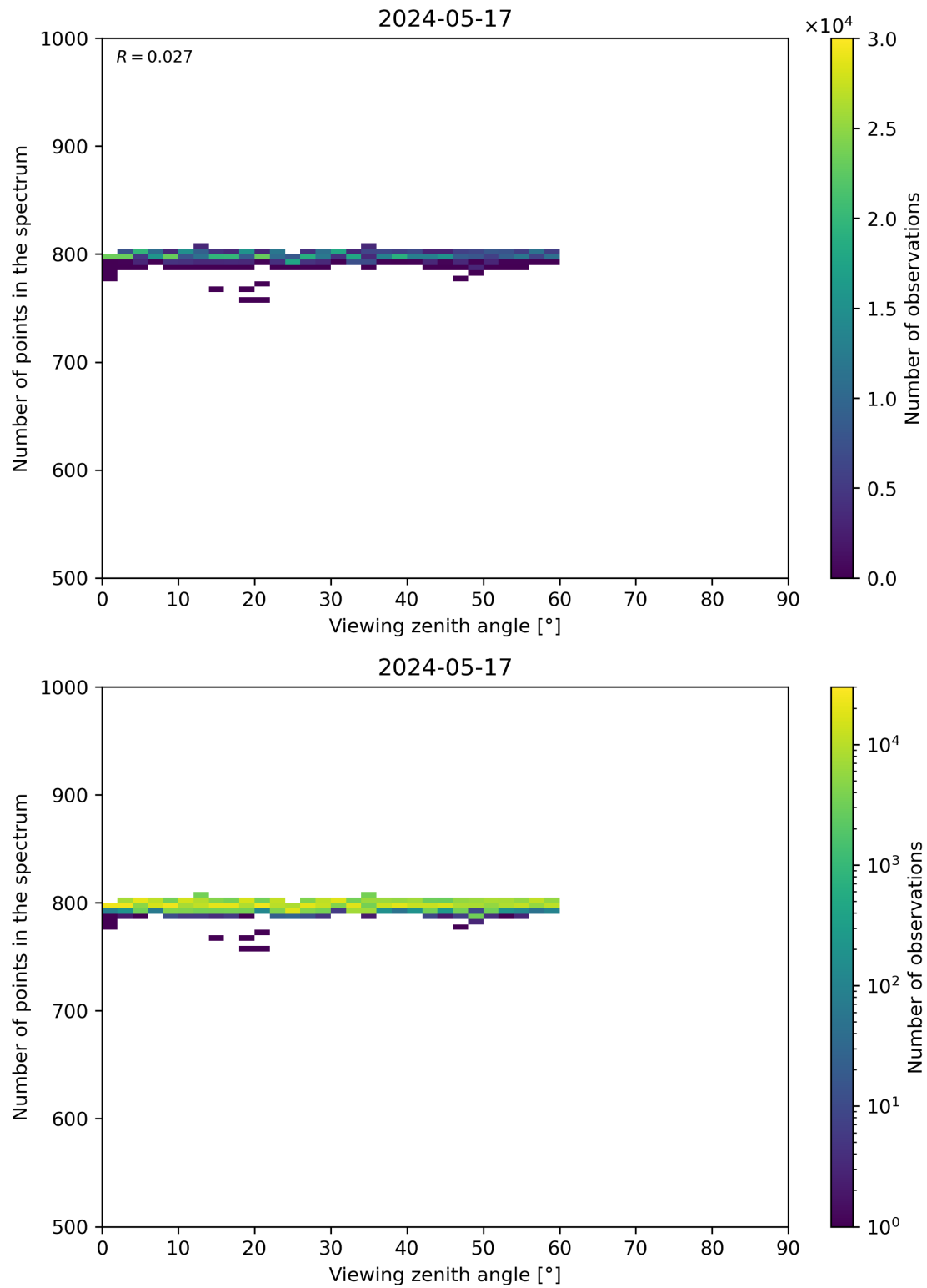
Figure 114: Scatter density plot of “Viewing zenith angle” against “Number of points in the spectrum” for 2024-05-16 to 2024-05-18.
