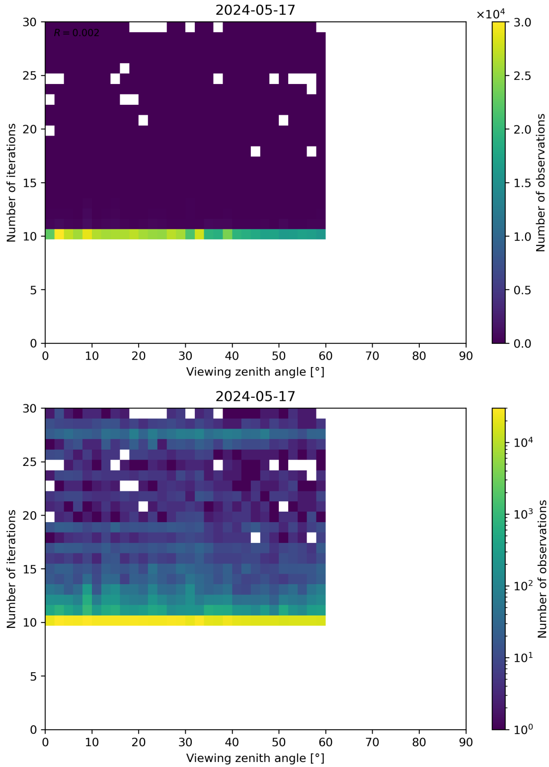
Figure 113: Scatter density plot of “Viewing zenith angle” against “Number of iterations” for 2024-05-16 to 2024-05-18.
