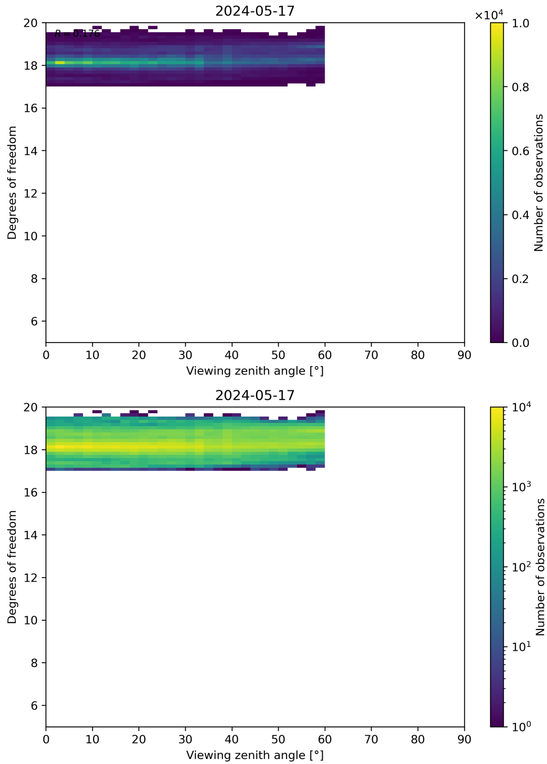
Figure 107: Scatter density plot of “Viewing zenith angle” against “Degrees of freedom” for 2024-05-16 to 2024-05-18.
