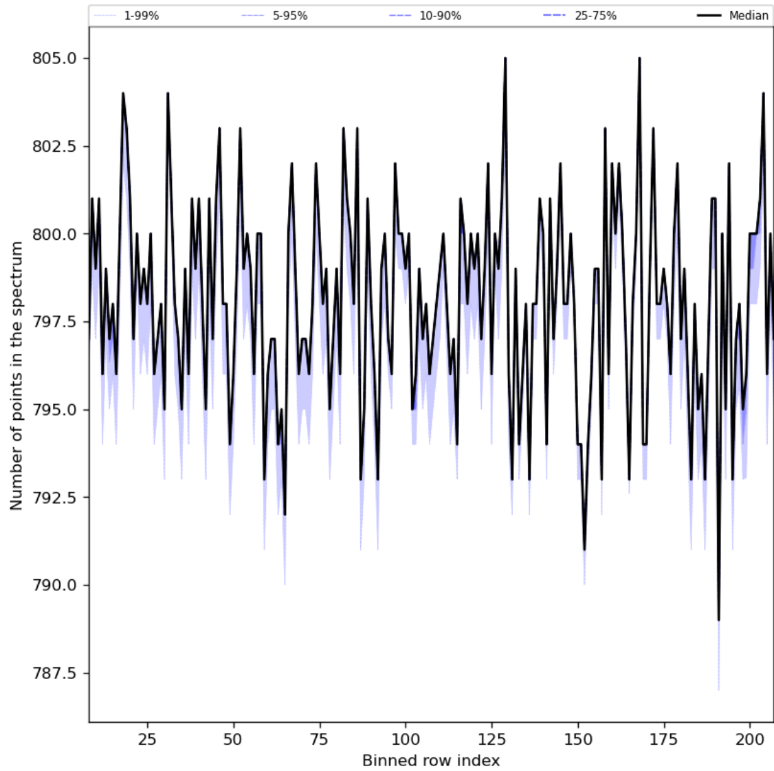
Figure 37: Along track statistics of “Number of points in the spectrum” for 2024-05-16 to 2024-05-18
