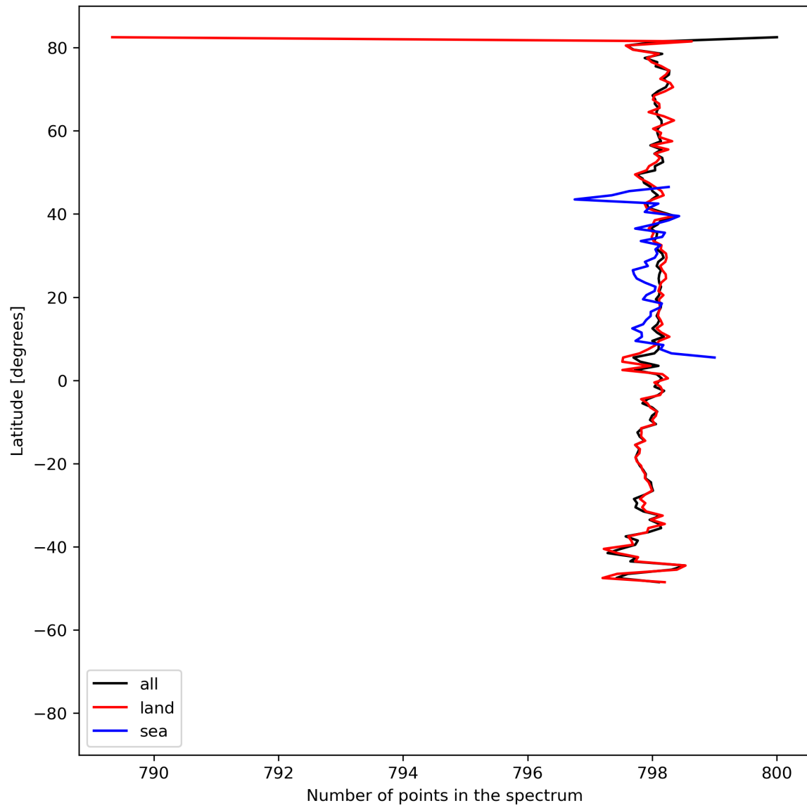
Figure 15: Zonal average of “Number of points in the spectrum” for 2024-05-16 to 2024-05-18.
