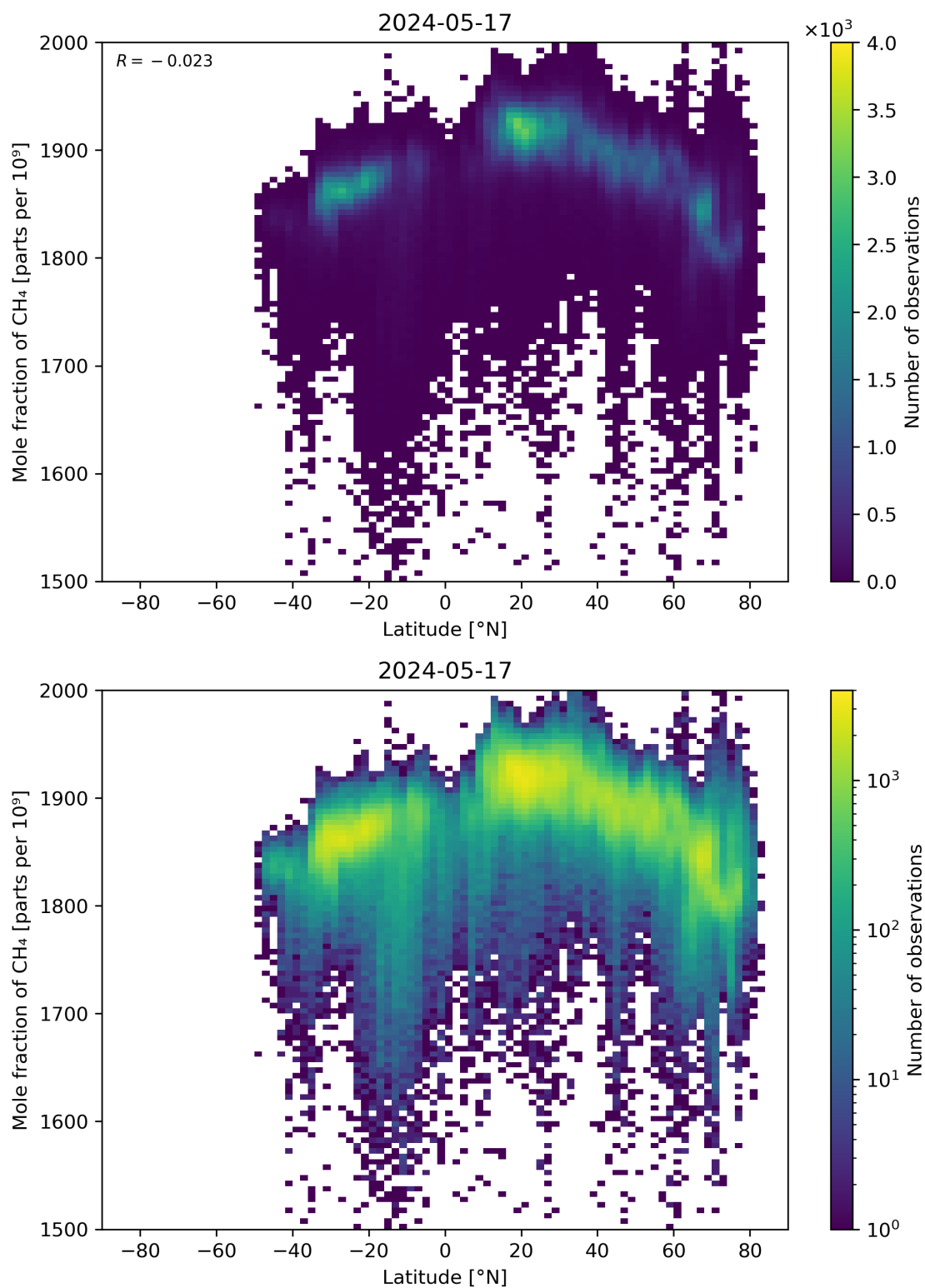
Figure 57: Scatter density plot of “Latitude” against “Mole fraction of \text{CH}_4 ” for 2024-05-16 to 2024-05-18.
