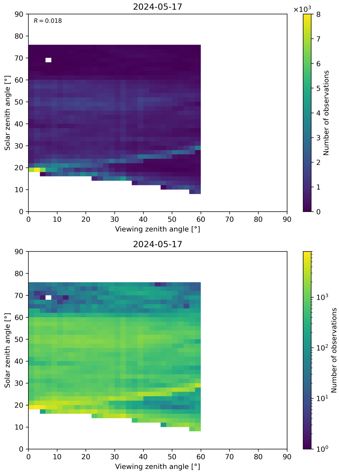
Figure 115: Scatter density plot of “Viewing zenith angle” against “Solar zenith angle” for 2024-05-16 to 2024-05-18.
