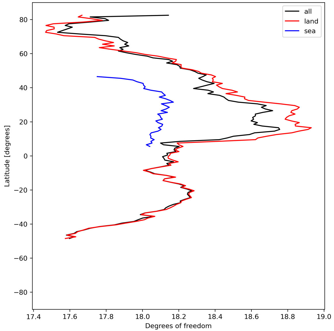
Figure 19: Zonal average of “Degrees of freedom” for 2024-05-16 to 2024-05-18.
