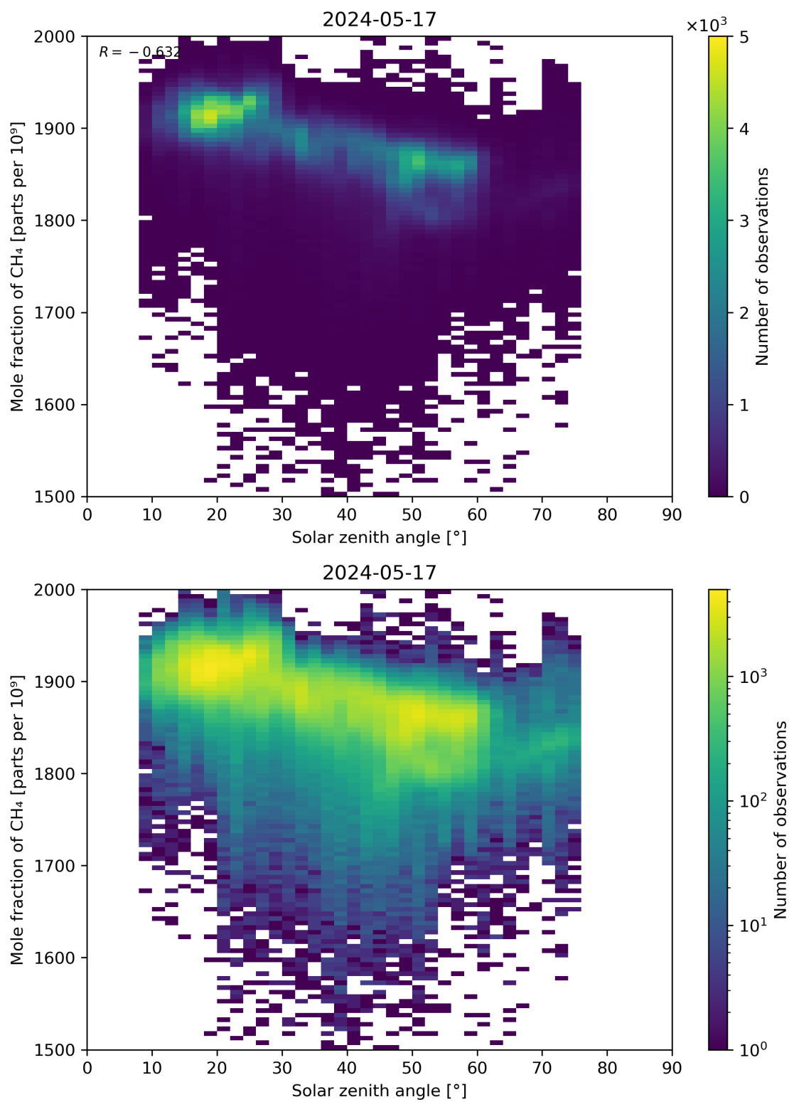
Figure 99: Scatter density plot of “Solar zenith angle” against “Mole fraction of CH 4 ” for 2024-05-16 to 2024-05-18.
