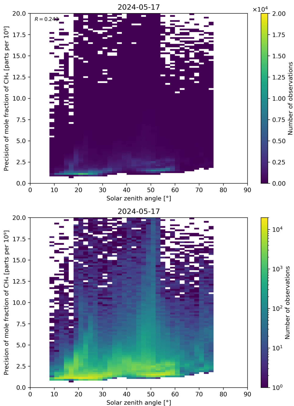
Figure 101: Scatter density plot of “Solar zenith angle” against “Precision of mole fraction of CH 4 ” for 2024-05-16 to 2024-05-18.
