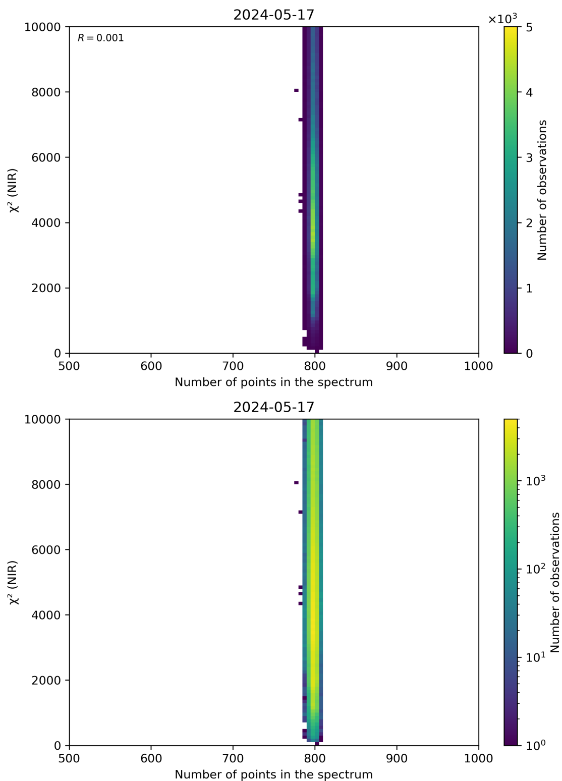
Figure 88: Scatter density plot of “Number of points in the spectrum” against “ \chi^2 (NIR)” for 2024-05-16 to 2024-05-18.
