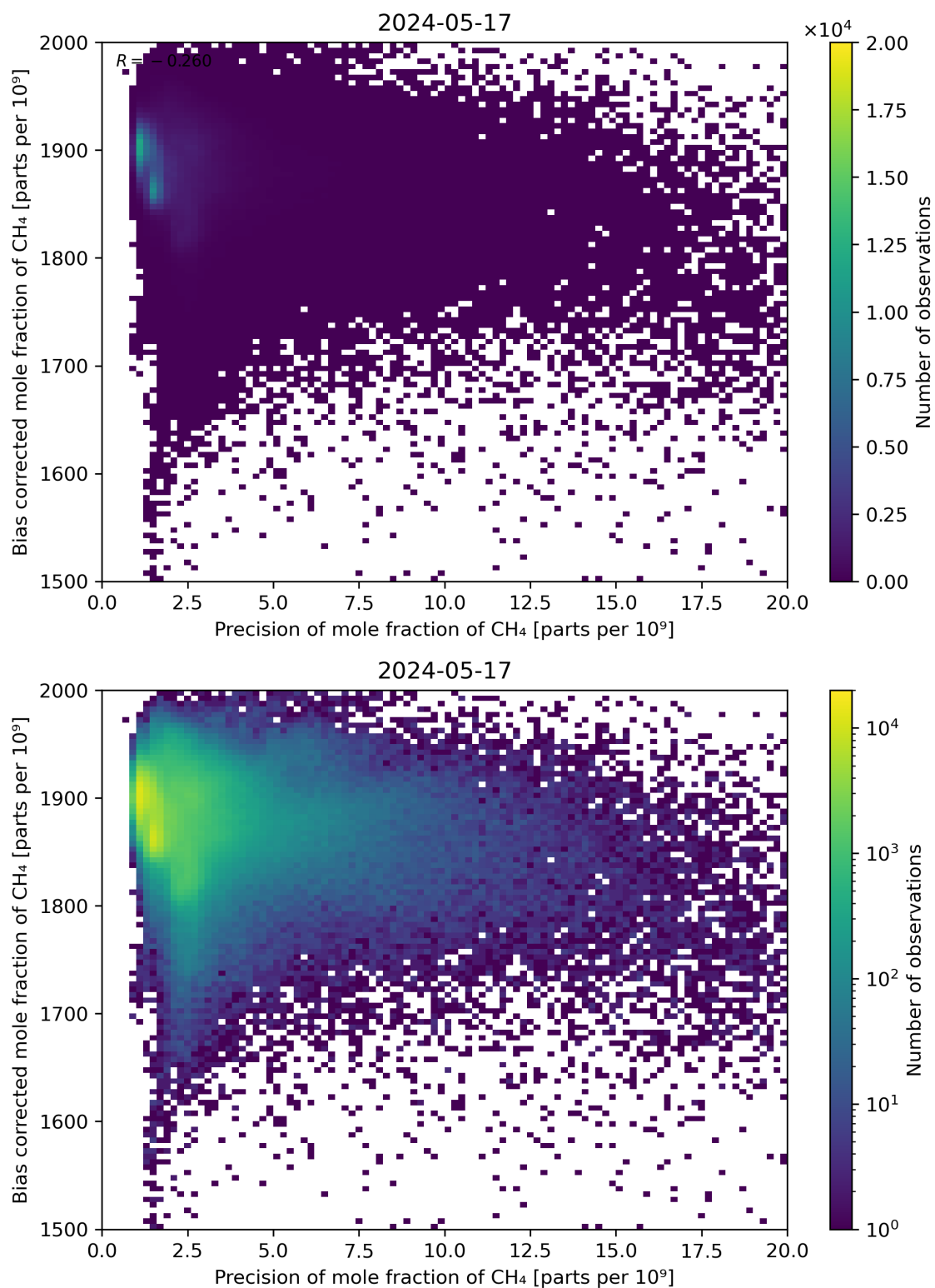
Figure 82: Scatter density plot of “Precision of mole fraction of CH 4 ” against “Bias corrected mole fraction of CH 4 ” for 2024-05-16 to 2024-05-18.
