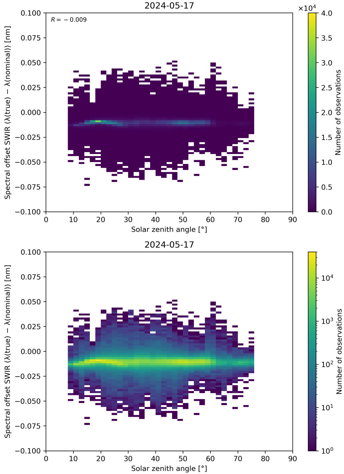
Figure 104: Scatter density plot of “Solar zenith angle” against “Spectral offset SWIR ( \lambda(\text{true}) - \lambda(\text{nominal}) )” for 2024-05-16 to 2024-05-18.
