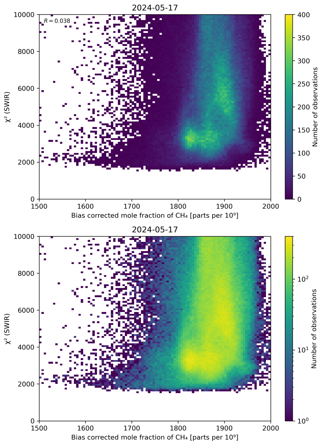
Figure 64: Scatter density plot of “Bias corrected mole fraction of CH 4 ” against “ \chi^2 (SWIR)” for 2024-05-16 to 2024-05-18.
