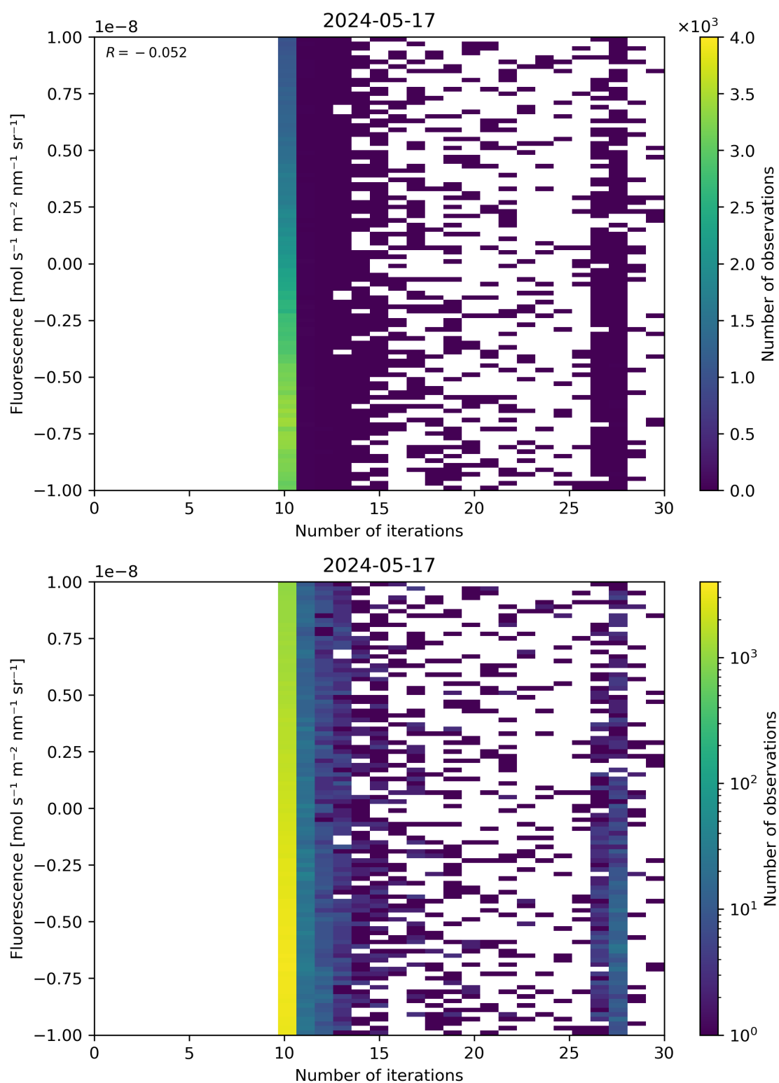
Figure 87: Scatter density plot of “Number of iterations” against “Fluorescence” for 2024-05-16 to 2024-05-18.
