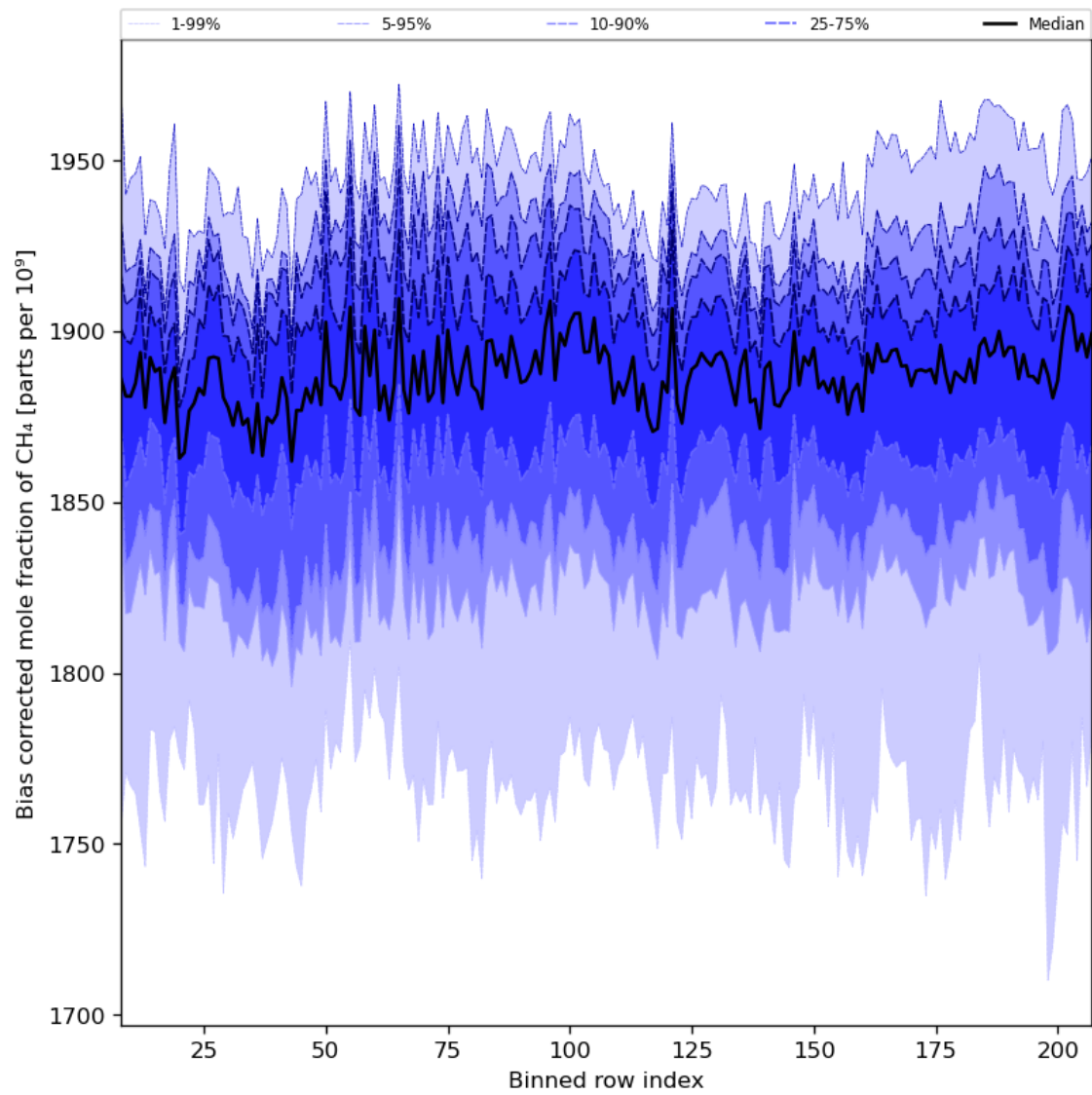
Figure 36: Along track statistics of “Bias corrected mole fraction of CH 4 ” for 2024-05-16 to 2024-05-18
