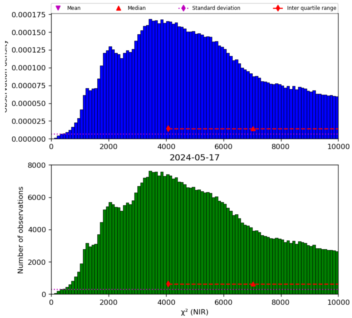
Figure 29: Histogram of “ \chi^2 (NIR)” for 2024-05-16 to 2024-05-18
