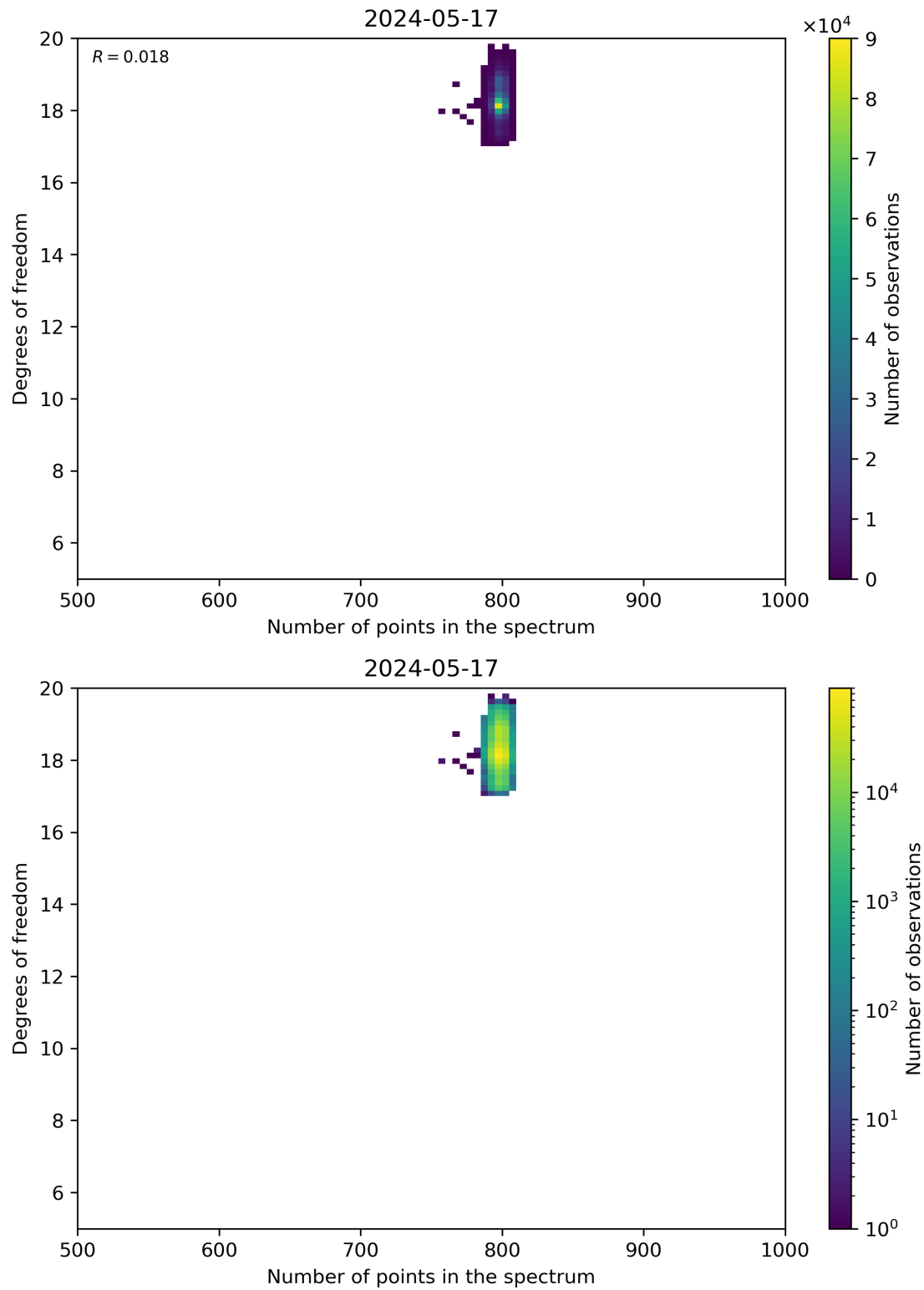
Figure 90: Scatter density plot of “Number of points in the spectrum” against “Degrees of freedom” for 2024-05-16 to 2024-05-18.
