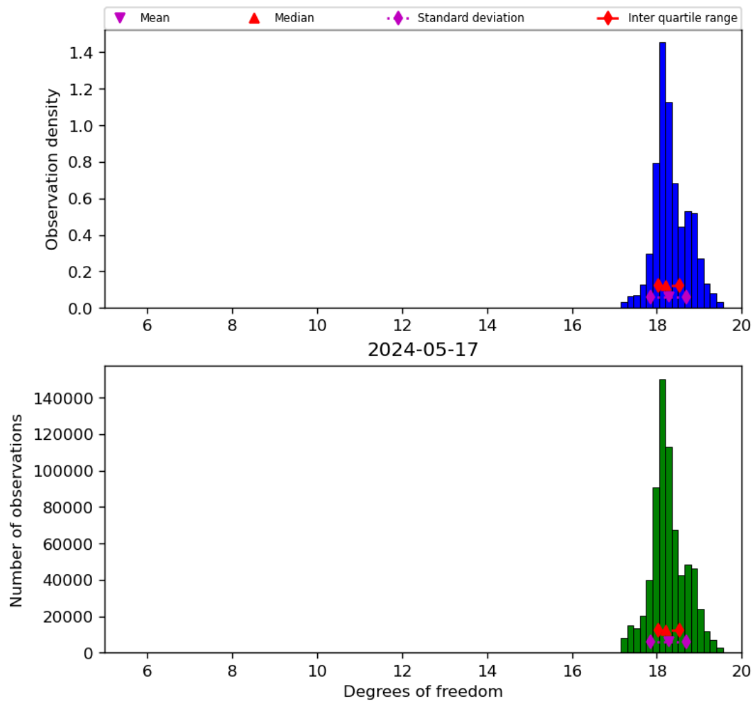
Figure 30: Histogram of “Degrees of freedom” for 2024-05-16 to 2024-05-18
