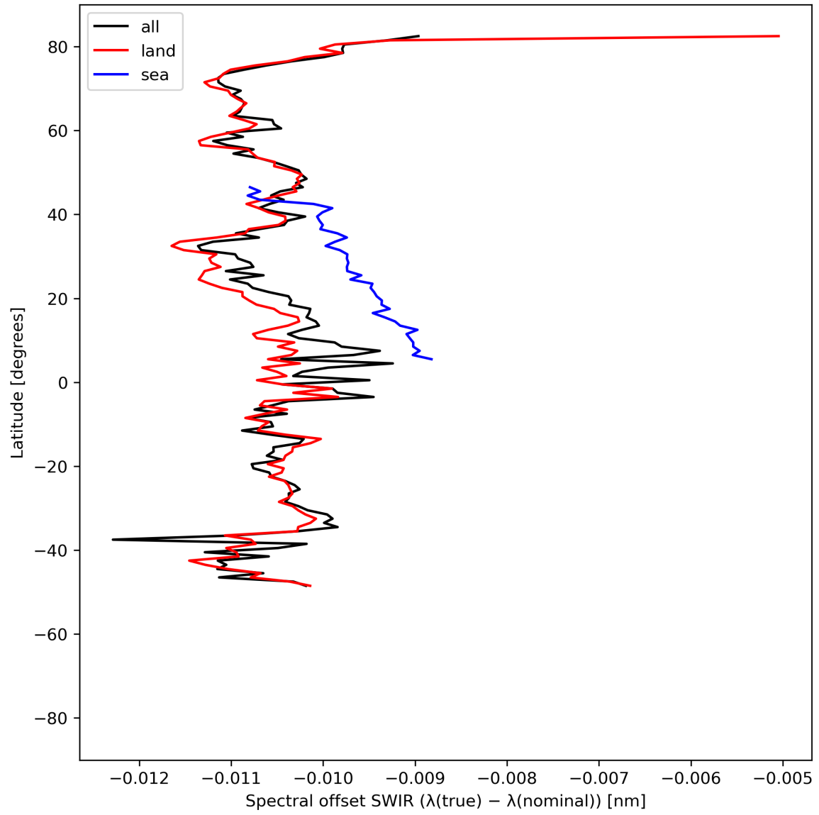
Figure 16: Zonal average of “Spectral offset SWIR ( \lambda(\text{true}) - \lambda(\text{nominal}) )” for 2024-05-16 to 2024-05-18.
