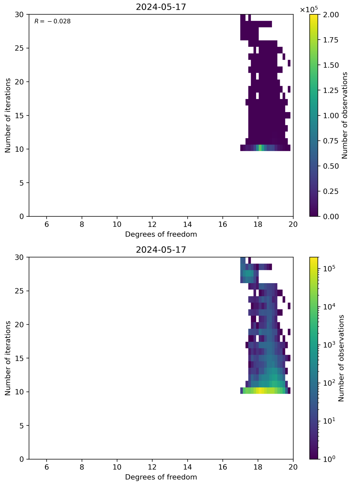
Figure 52: Scatter density plot of “Degrees of freedom” against “Number of iterations” for 2024-05-16 to 2024-05-18.
