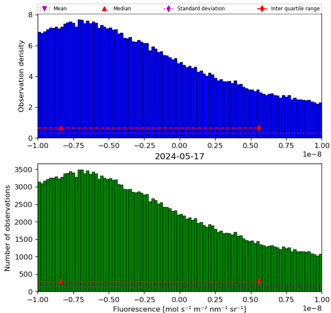
Figure 32: Histogram of “Fluorescence” for 2024-05-16 to 2024-05-18
