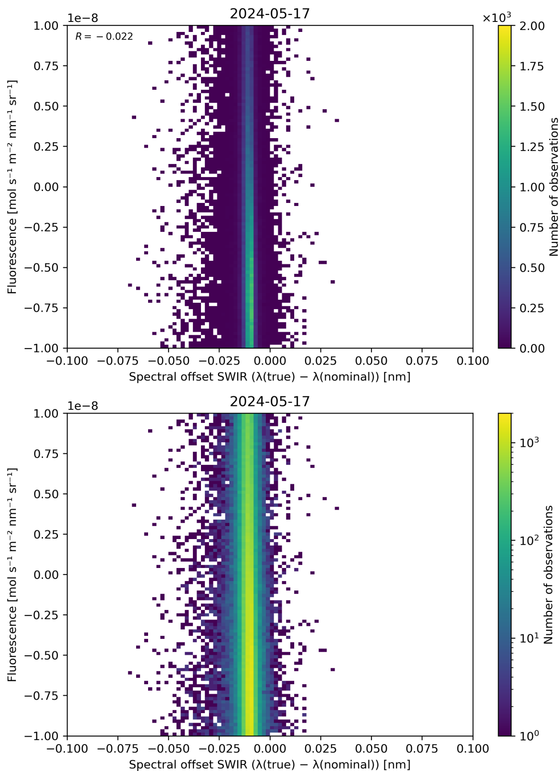
Figure 120: Scatter density plot of “Spectral offset SWIR ( \lambda(\text{true}) - \lambda(\text{nominal}) )” against “Fluorescence” for 2024-05-16 to 2024-05-18.
