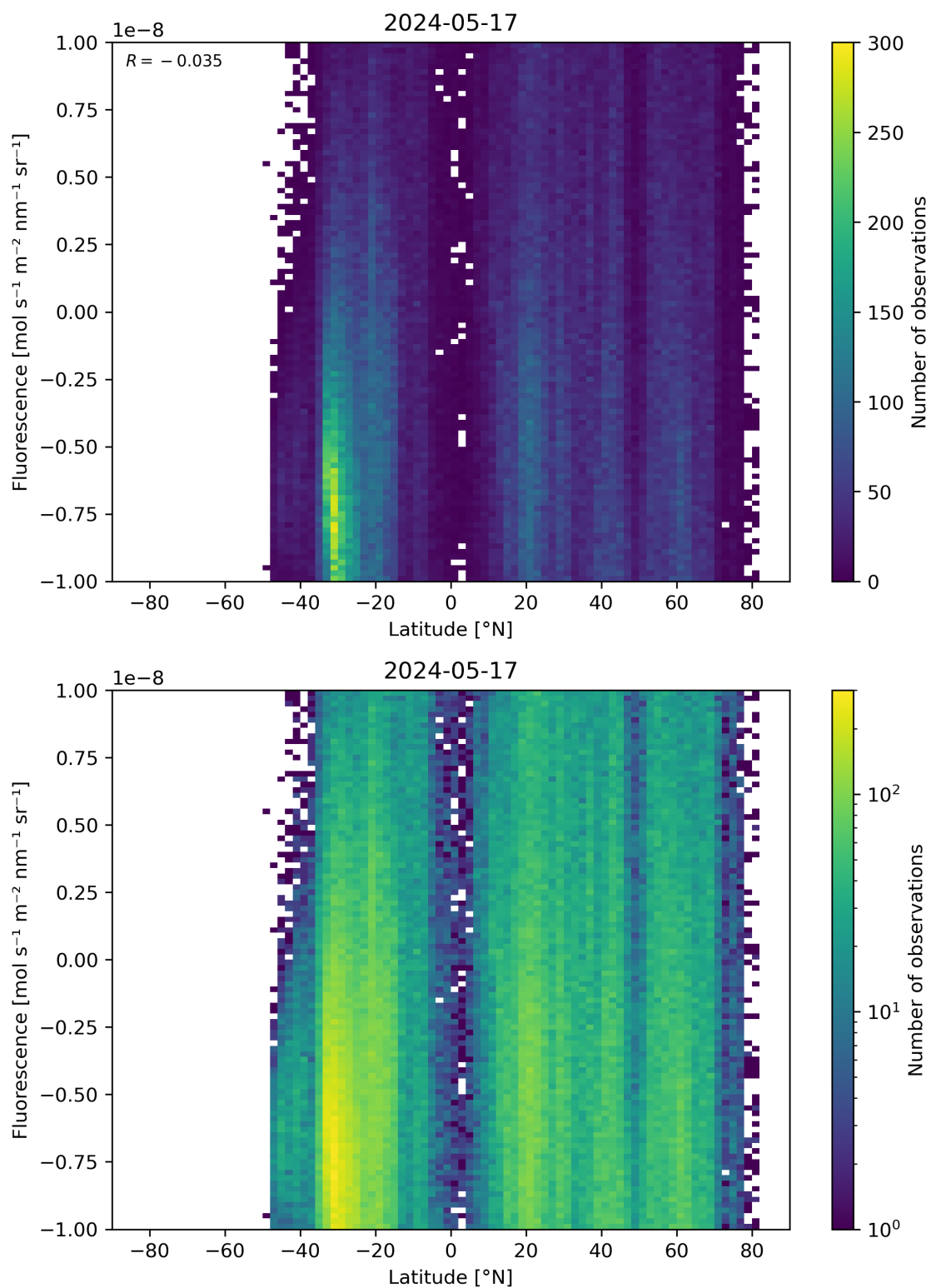
Figure 56: Scatter density plot of “Latitude” against “Fluorescence” for 2024-05-16 to 2024-05-18.
