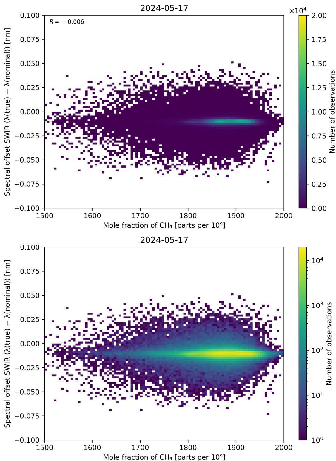
Figure 86: Scatter density plot of “Mole fraction of CH 4 ” against “Spectral offset SWIR ( \lambda(\text{true}) - \lambda(\text{nominal}) )” for 2024-05-16 to 2024-05-18.
