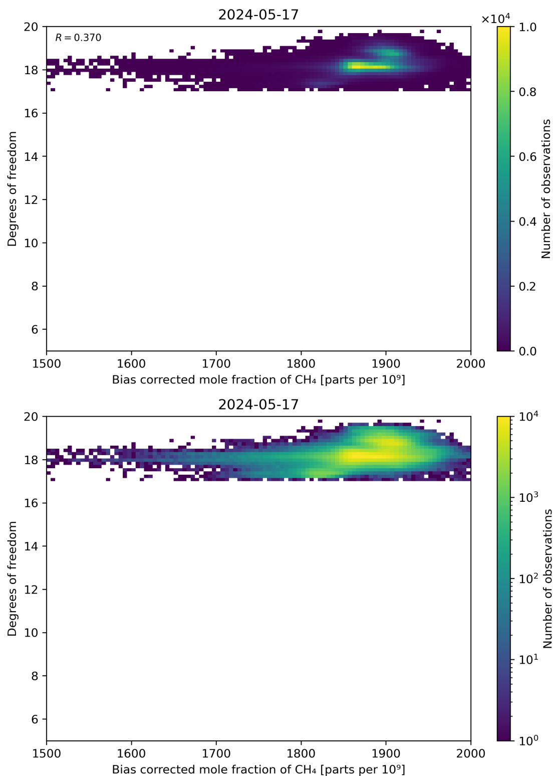
Figure 65: Scatter density plot of “Bias corrected mole fraction of CH 4 ” against “Degrees of freedom” for 2024-05-16 to 2024-05-18.
