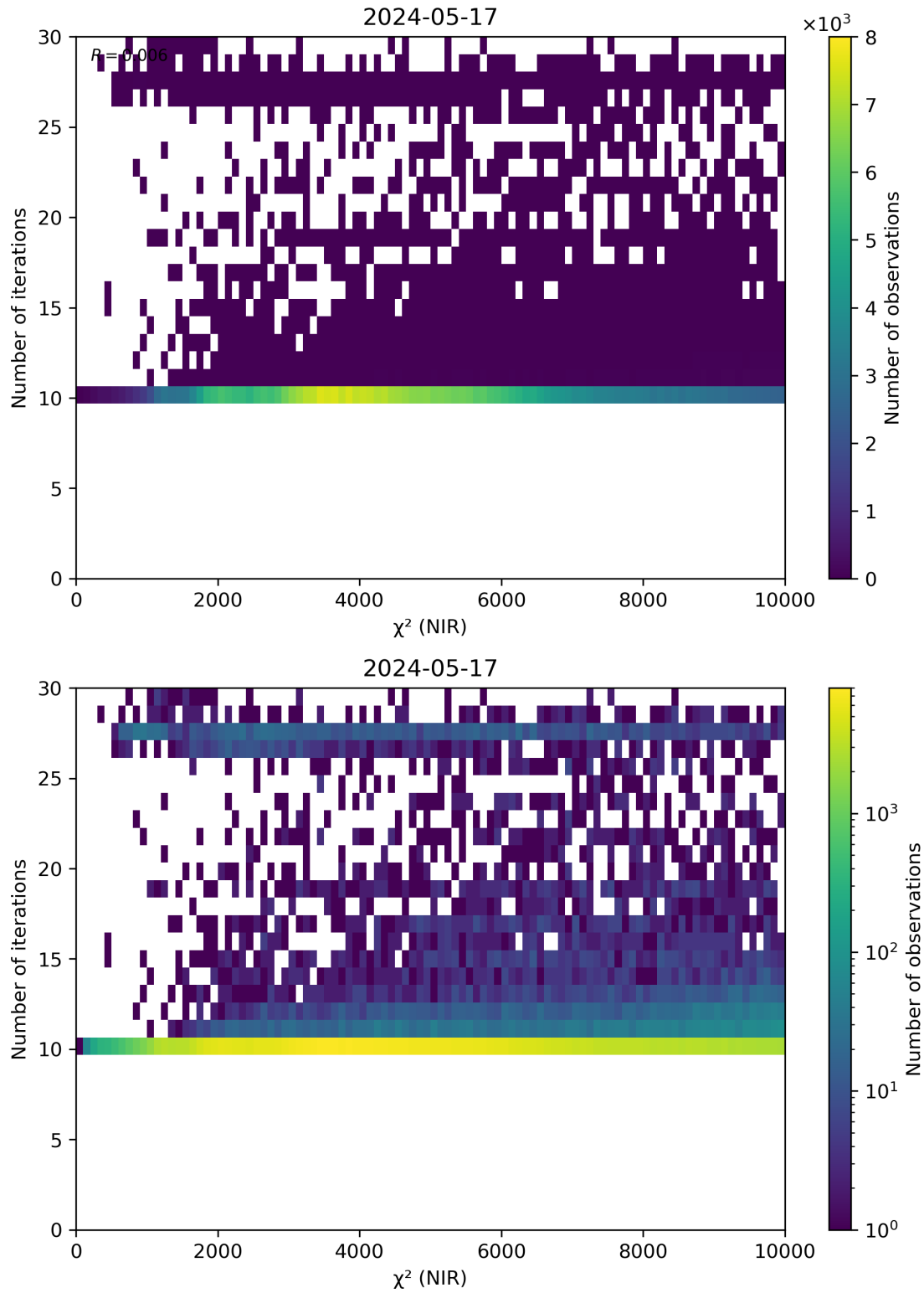
Figure 46: Scatter density plot of “ \chi^2 (NIR)” against “Number of iterations” for 2024-05-16 to 2024-05-18.
