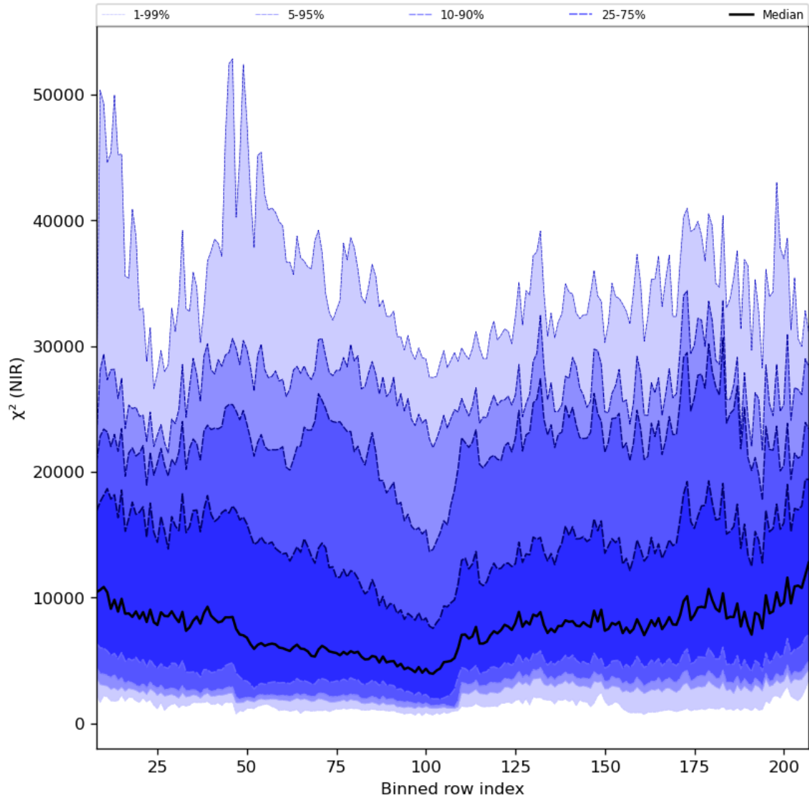
Figure 40: Along track statistics of “ \chi^2 (NIR)” for 2024-05-16 to 2024-05-18
