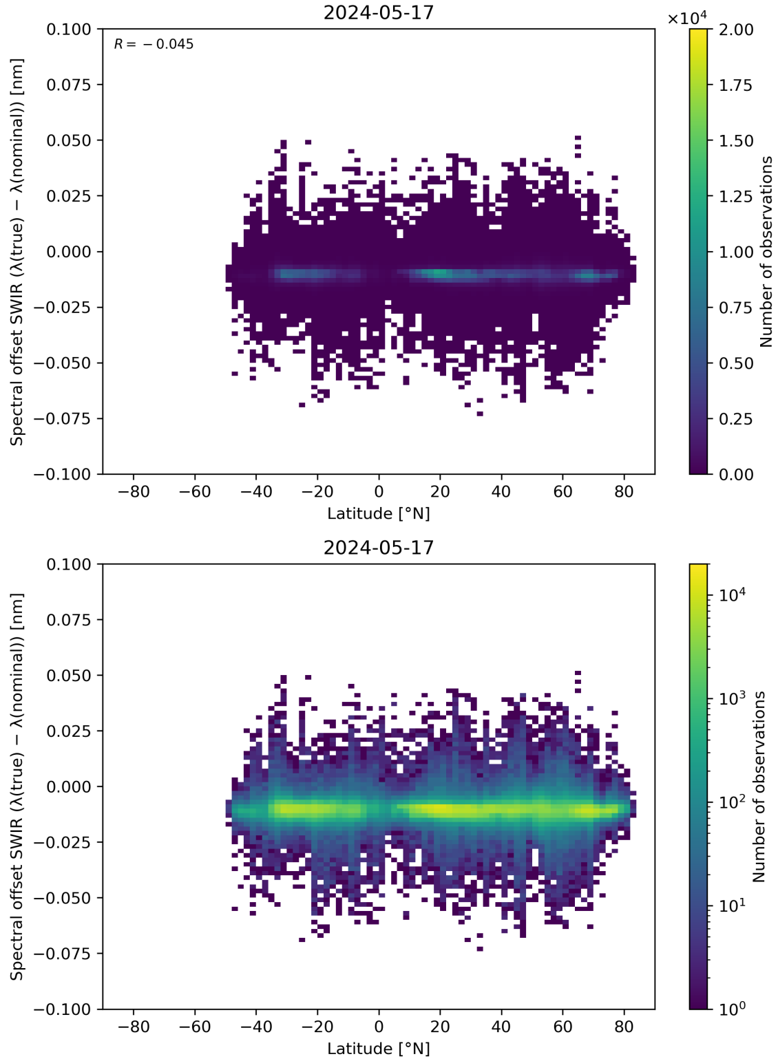
Figure 62: Scatter density plot of “Latitude” against “Spectral offset SWIR ( \lambda(\text{true}) - \lambda(\text{nominal}) )” for 2024-05-16 to 2024-05-18.
