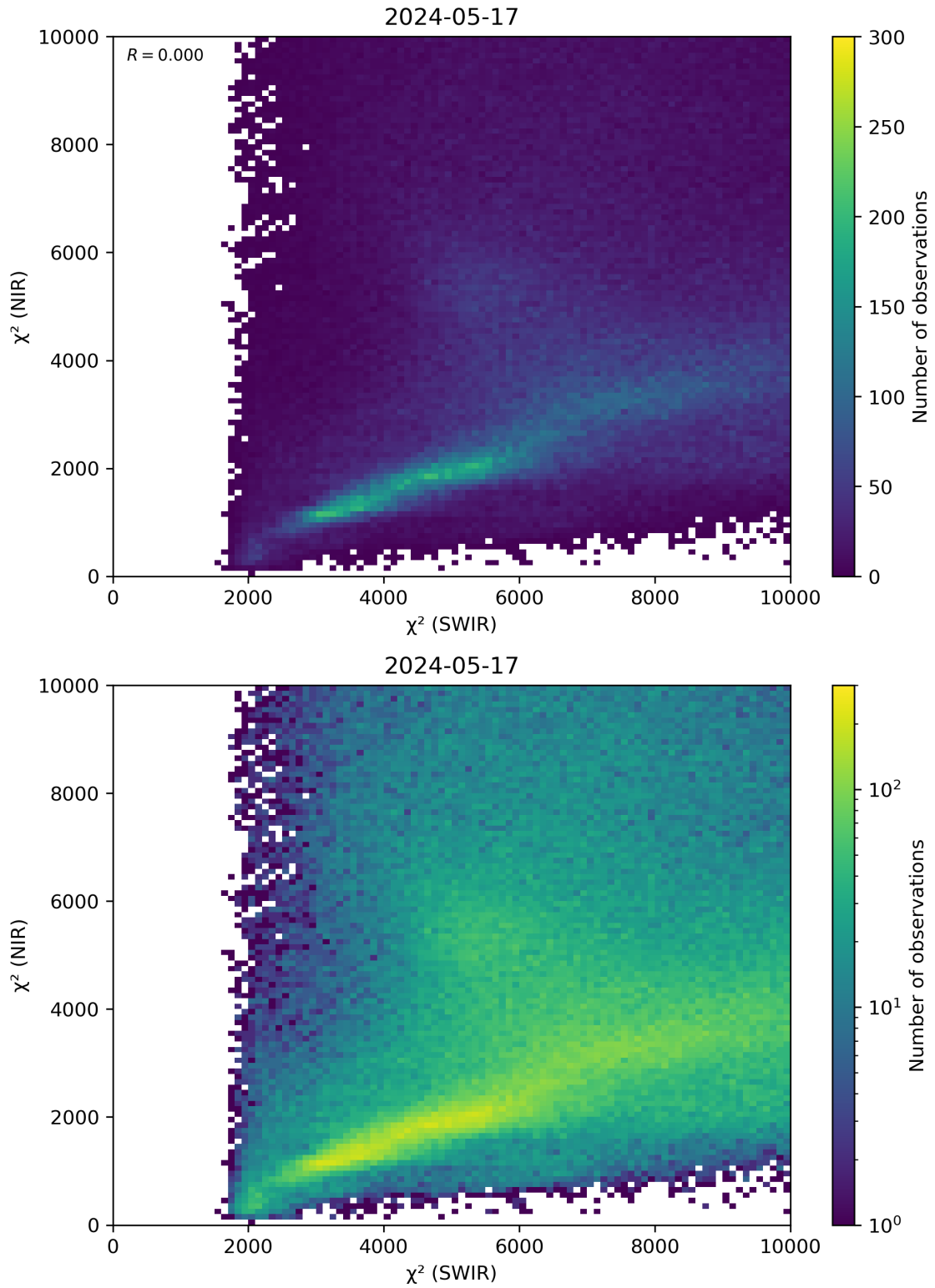
Figure 47: Scatter density plot of “ \chi^2 (SWIR)” against “ \chi^2 (NIR)” for 2024-05-16 to 2024-05-18.
