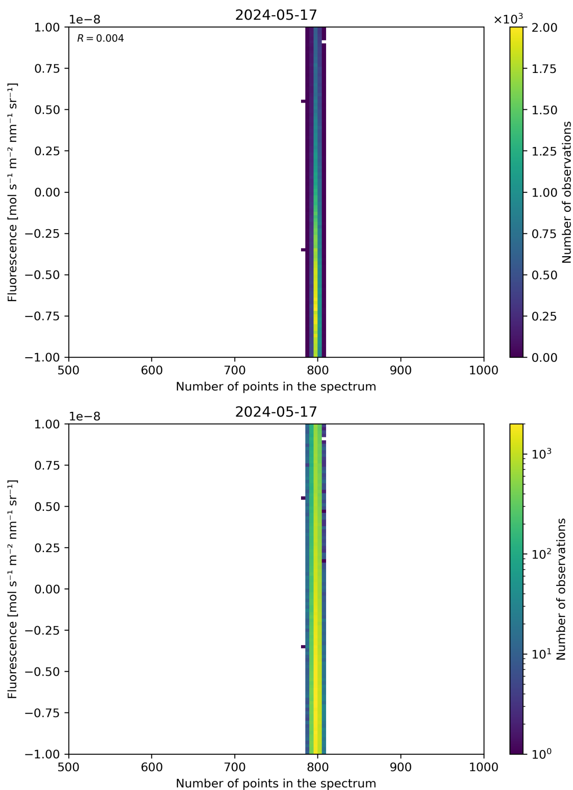
Figure 91: Scatter density plot of “Number of points in the spectrum” against “Fluorescence” for 2024-05-16 to 2024-05-18.
