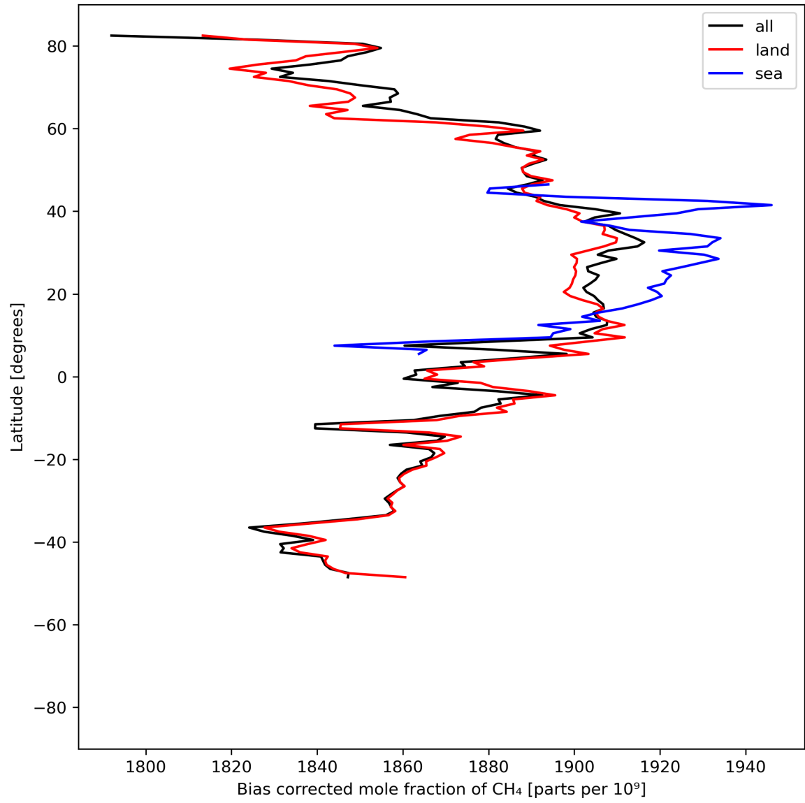
Figure 14: Zonal average of “Bias corrected mole fraction of CH 4 ” for 2024-05-16 to 2024-05-18.
