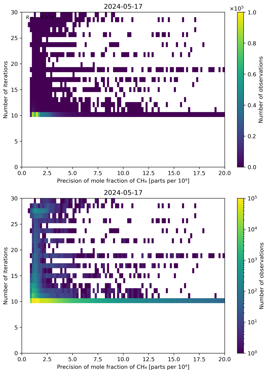
Figure 83: Scatter density plot of “Precision of mole fraction of CH 4 ” against “Number of iterations” for 2024-05-16 to 2024-05-18.
