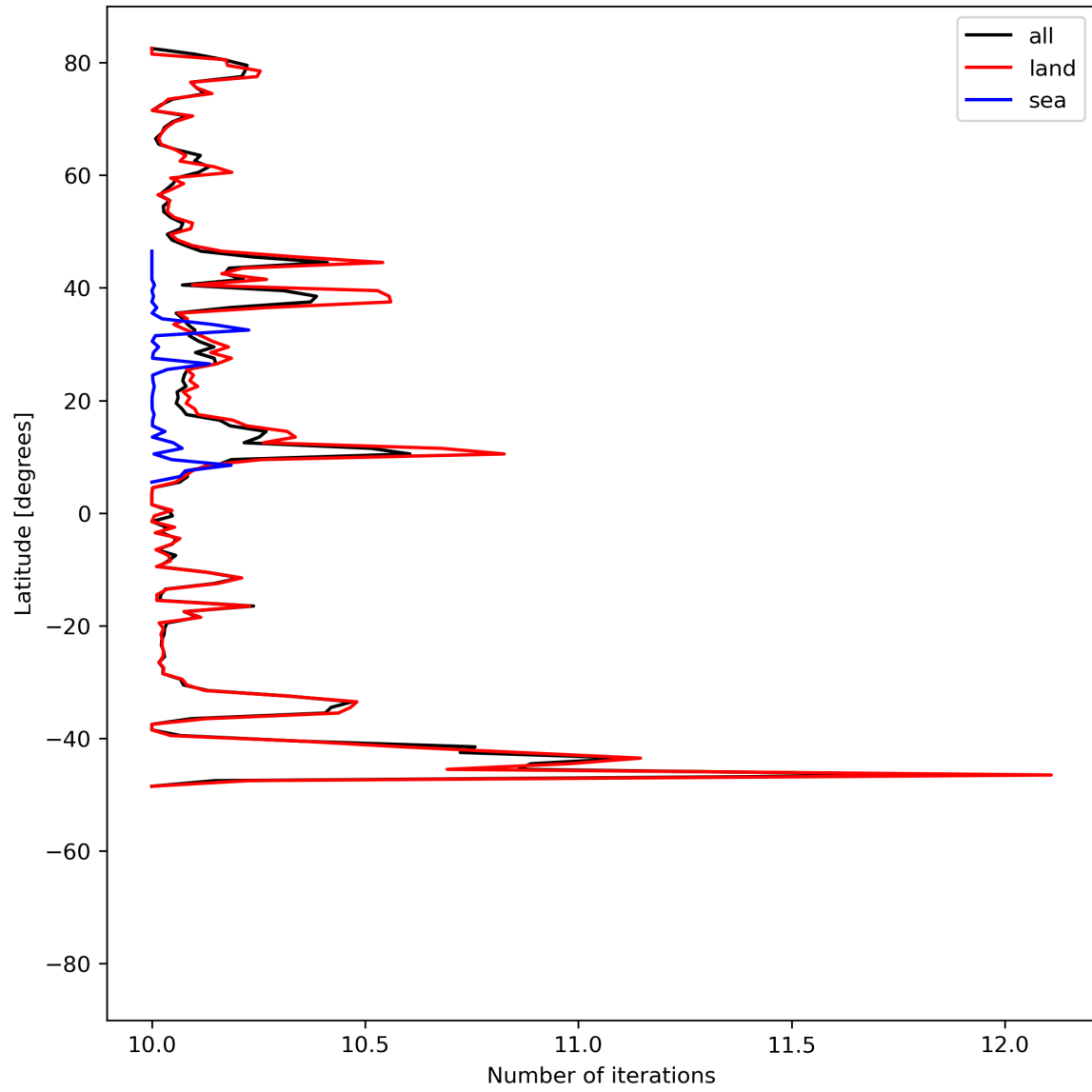
Figure 20: Zonal average of “Number of iterations” for 2024-05-16 to 2024-05-18.
