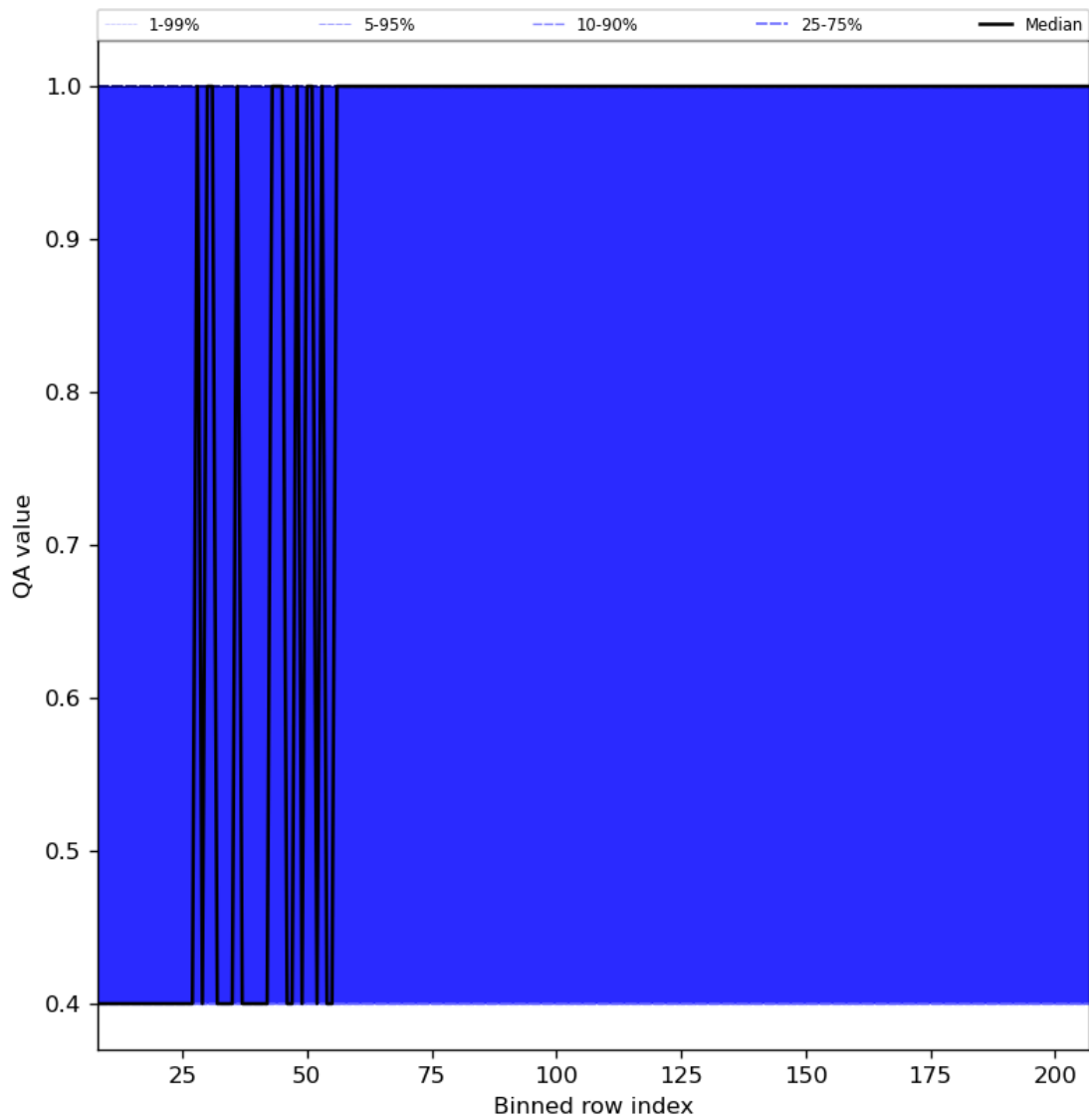
Figure 33: Along track statistics of “QA value” for 2024-05-16 to 2024-05-18
