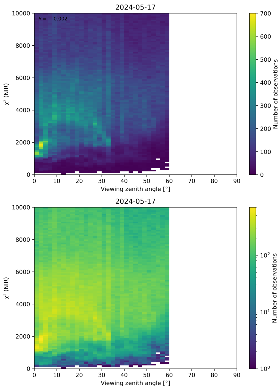
Figure 105: Scatter density plot of “Viewing zenith angle” against “ \chi^2 (NIR)” for 2024-05-16 to 2024-05-18.
