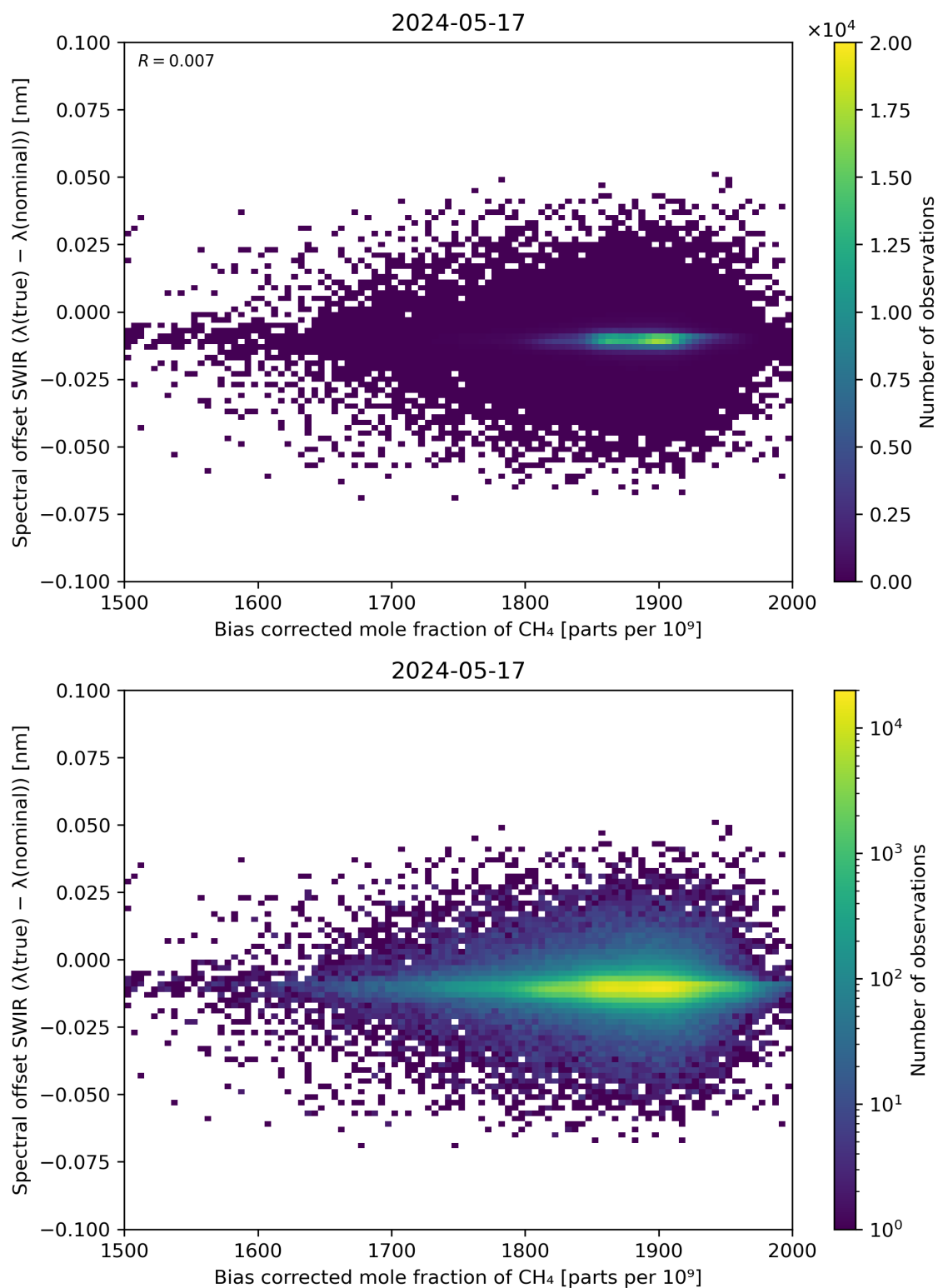
Figure 69: Scatter density plot of “Bias corrected mole fraction of \text{CH}_4 ” against “Spectral offset SWIR ( \lambda(\text{true}) - \lambda(\text{nominal}) )” for 2024-05-16 to 2024-05-18.
