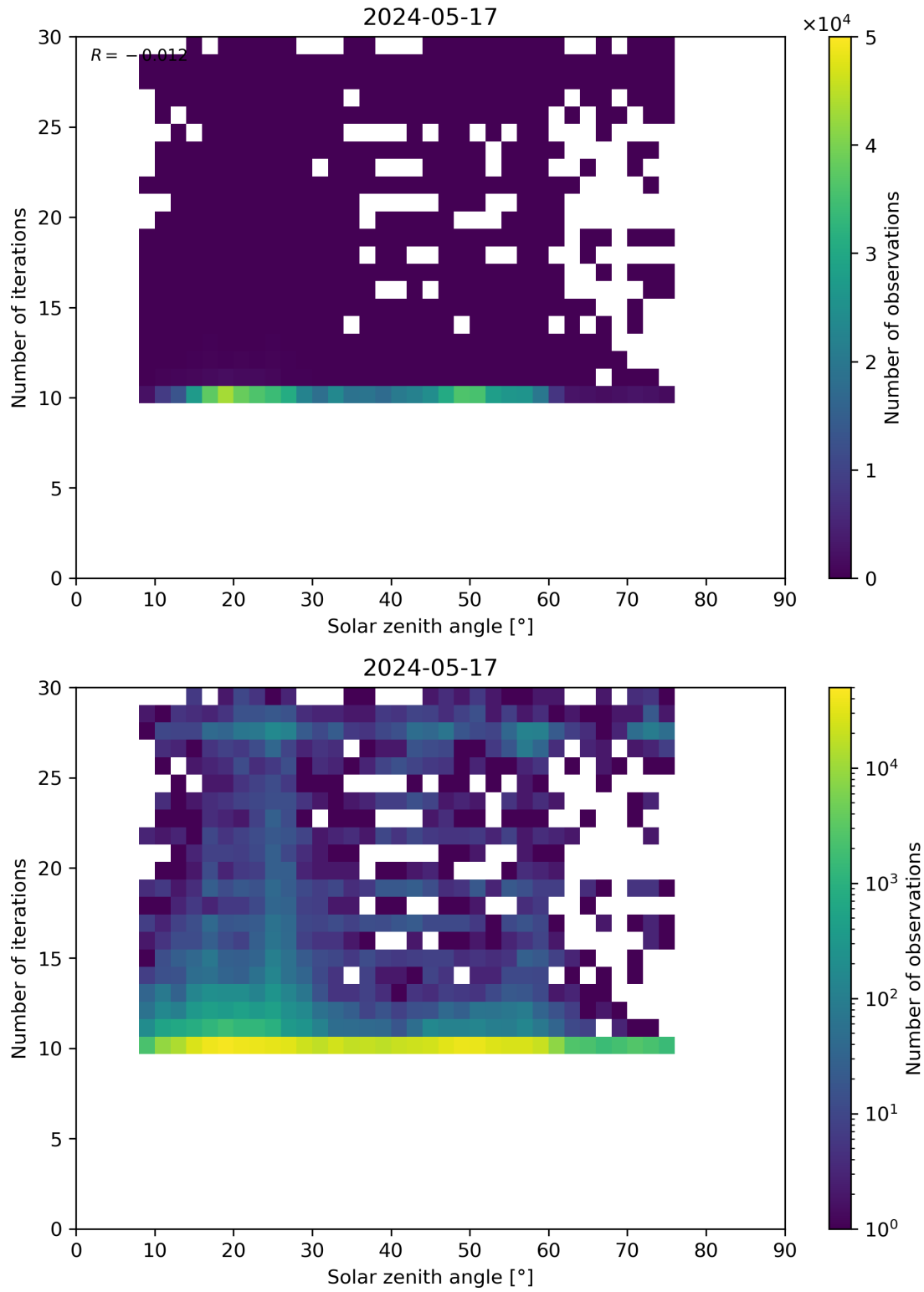
Figure 102: Scatter density plot of “Solar zenith angle” against “Number of iterations” for 2024-05-16 to 2024-05-18.
