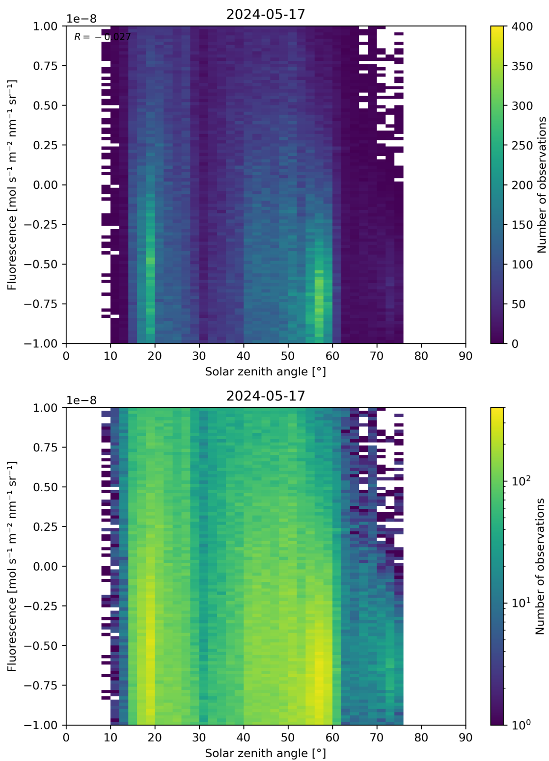
Figure 97: Scatter density plot of “Solar zenith angle” against “Fluorescence” for 2024-05-16 to 2024-05-18.
