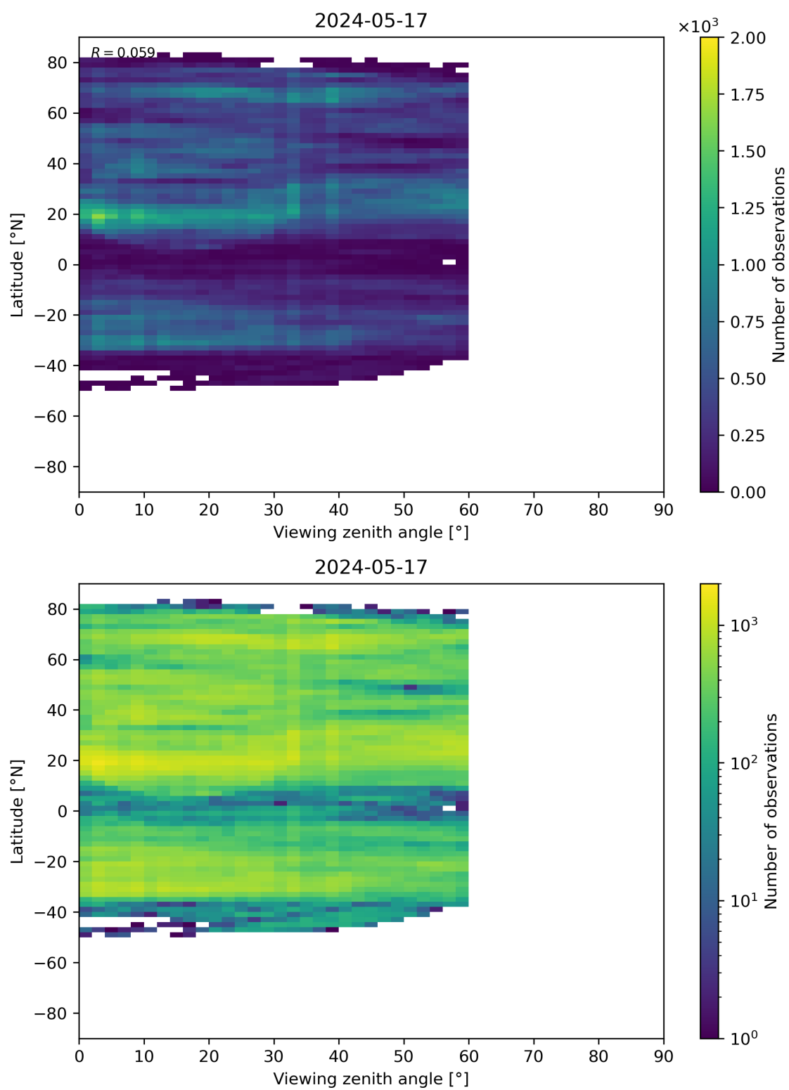
Figure 109: Scatter density plot of “Viewing zenith angle” against “Latitude” for 2024-05-16 to 2024-05-18.
