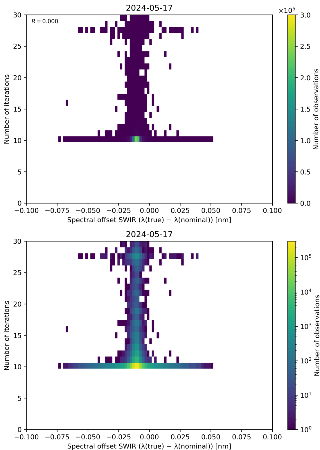
Figure 121: Scatter density plot of “Spectral offset SWIR ( \lambda(\text{true}) - \lambda(\text{nominal}) )” against “Number of iterations” for 2024-05-16 to 2024-05-18.
