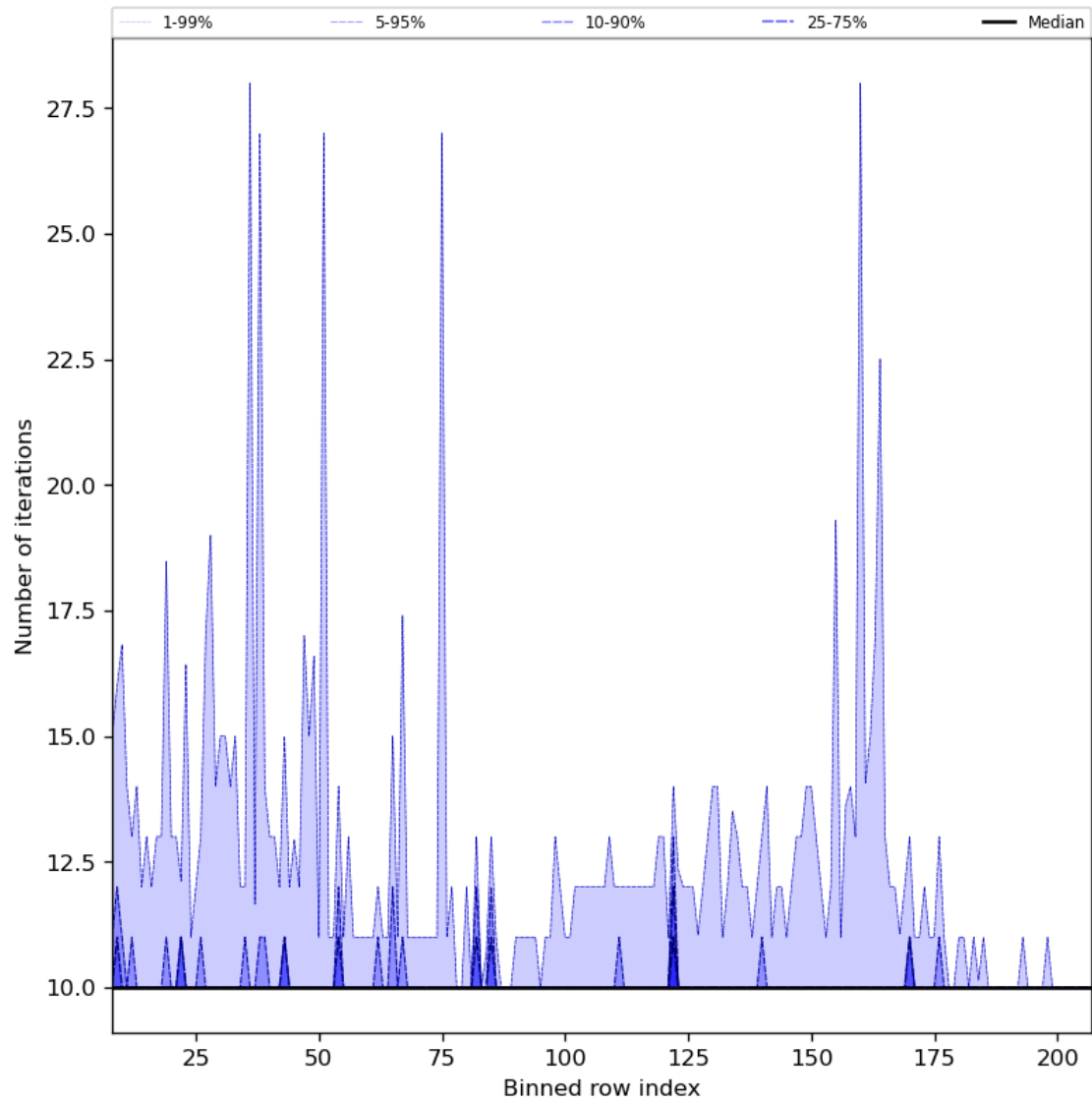
Figure 42: Along track statistics of “Number of iterations” for 2024-05-16 to 2024-05-18
