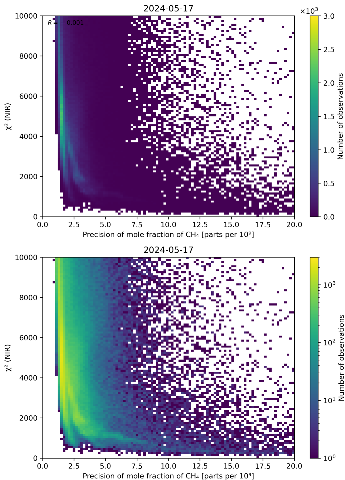
Figure 78: Scatter density plot of “Precision of mole fraction of CH 4 ” against “ \chi^2 (NIR)” for 2024-05-16 to 2024-05-18.
