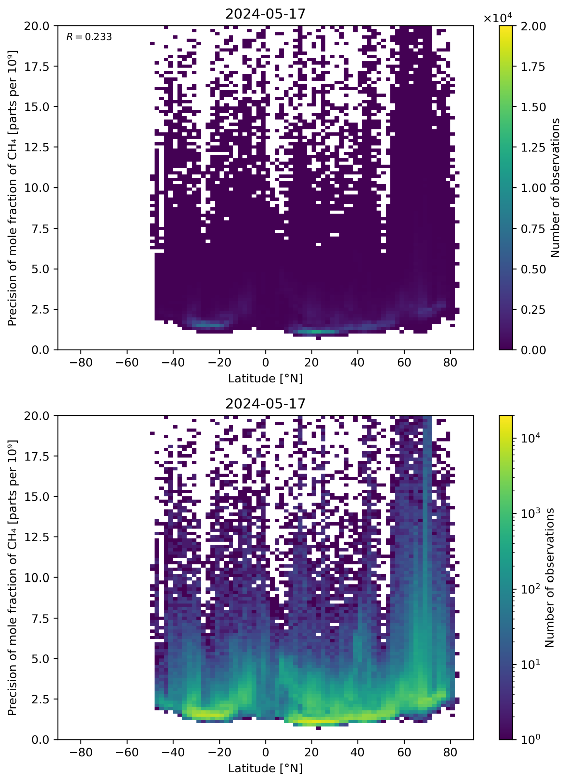
Figure 59: Scatter density plot of “Latitude” against “Precision of mole fraction of \text{CH}_4 ” for 2024-05-16 to 2024-05-18.
