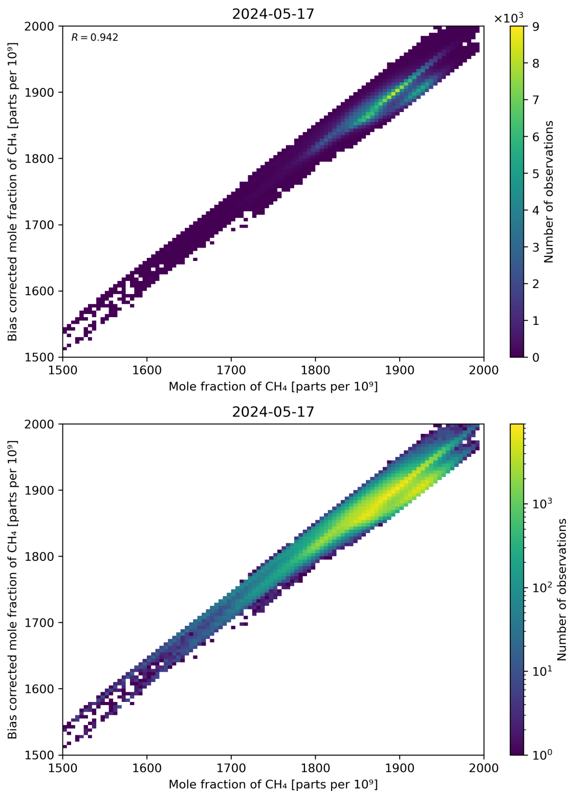
Figure 74: Scatter density plot of “Mole fraction of CH 4 ” against “Bias corrected mole fraction of CH 4 ” for 2024-05-16 to 2024-05-18.
