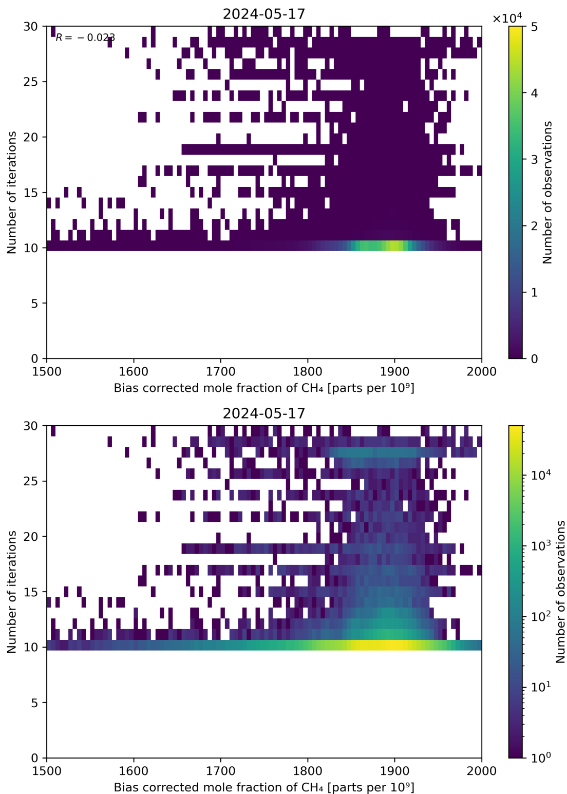
Figure 67: Scatter density plot of “Bias corrected mole fraction of CH 4 ” against “Number of iterations” for 2024-05-16 to 2024-05-18.
