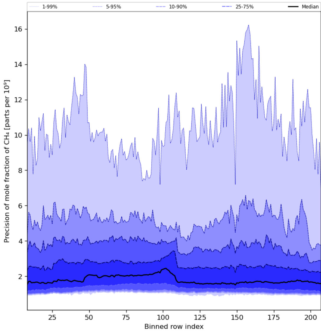
Figure 35: Along track statistics of “Precision of mole fraction of CH 4 ” for 2024-05-16 to 2024-05-18
