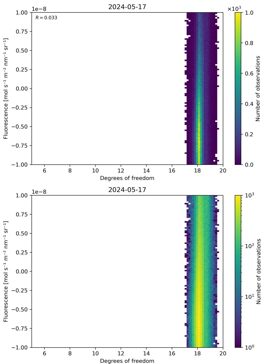
Figure 51: Scatter density plot of “Degrees of freedom” against “Fluorescence” for 2024-05-16 to 2024-05-18.
