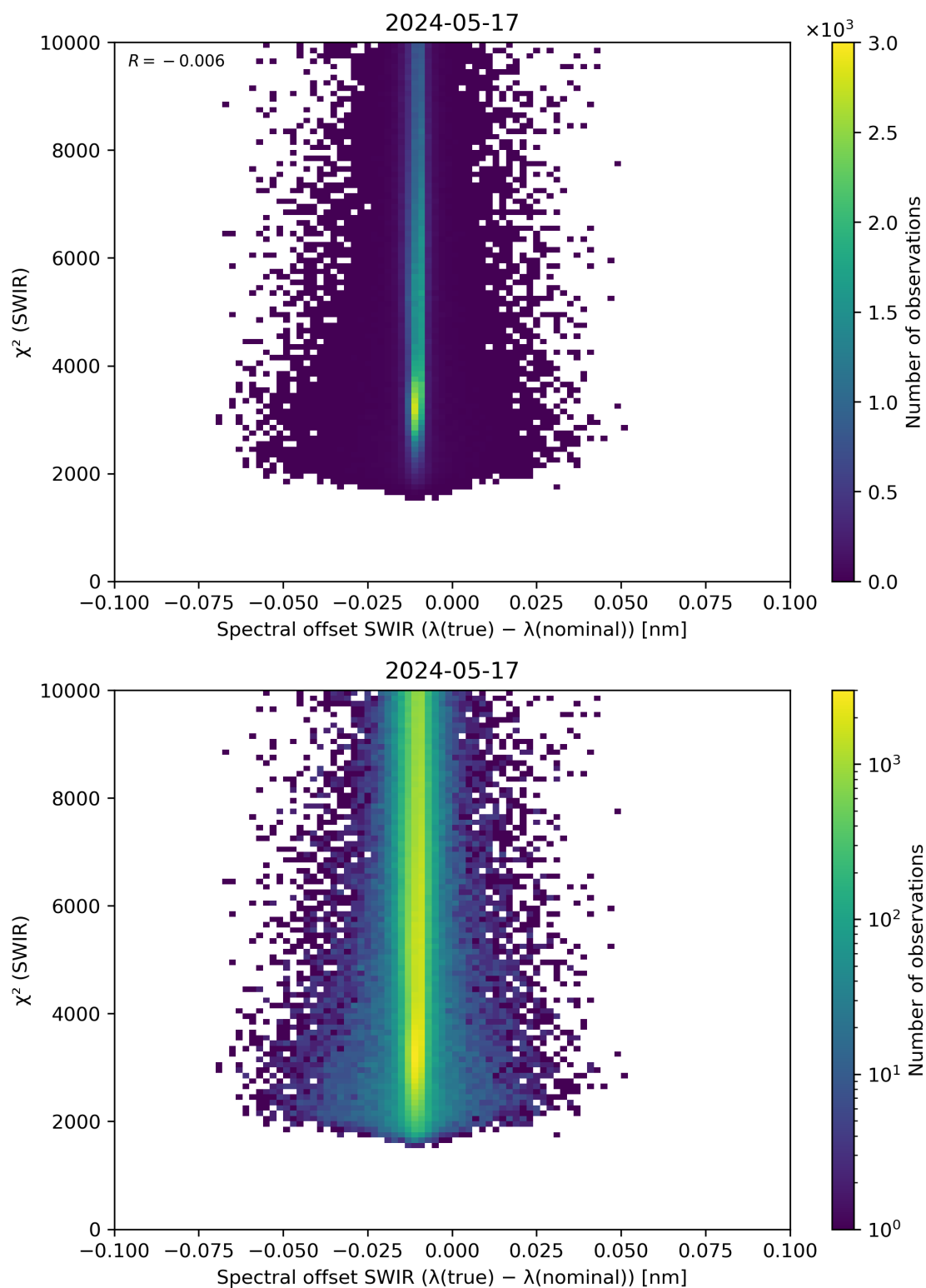
Figure 118: Scatter density plot of “Spectral offset SWIR ( \lambda(\text{true}) - \lambda(\text{nominal}) )” against “ \chi^2 (SWIR)” for 2024-05-16 to 2024-05-18.
