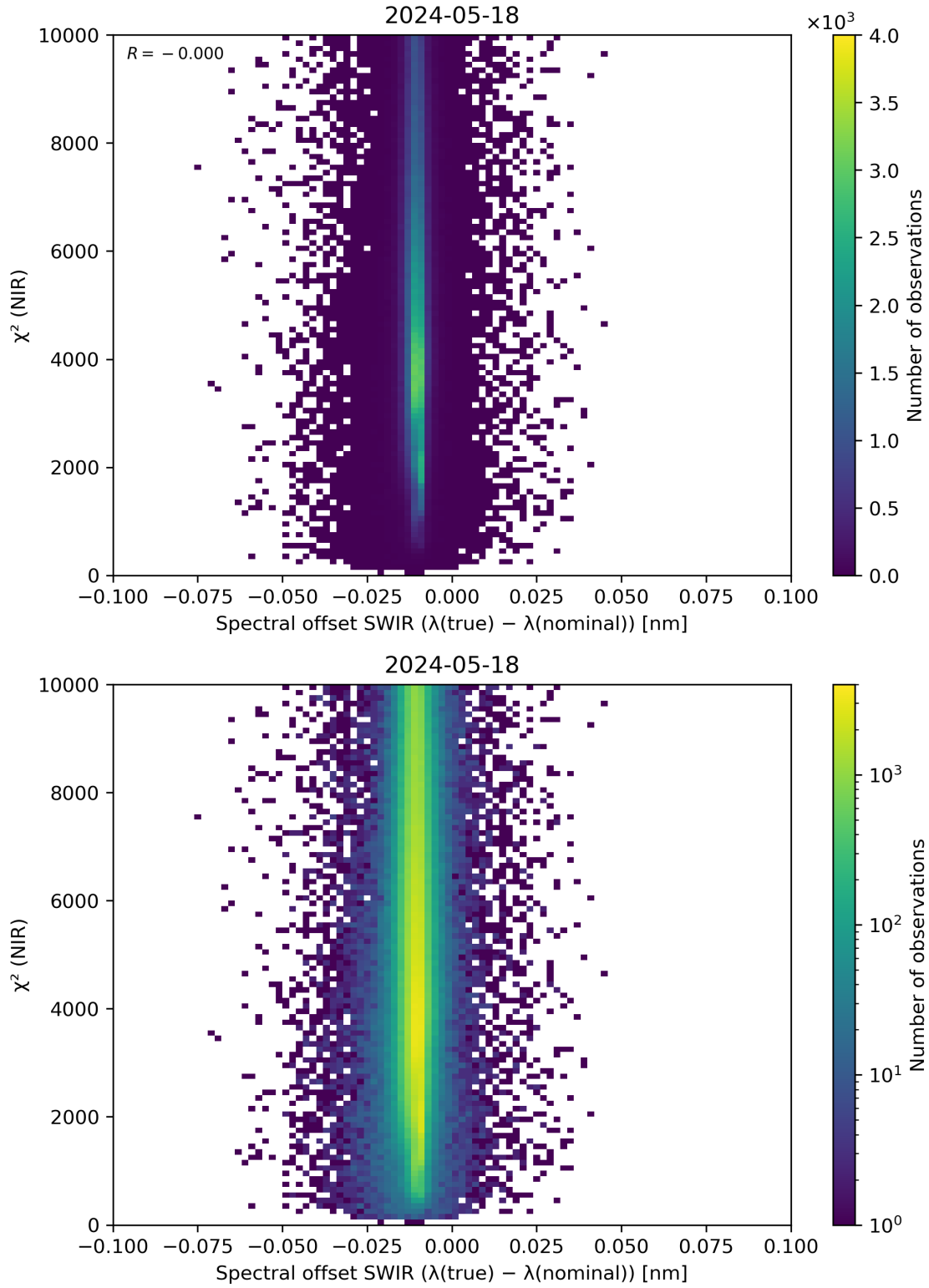
Figure 117: Scatter density plot of “Spectral offset SWIR ( \lambda(\text{true}) - \lambda(\text{nominal}) )” against “ \chi^2 (NIR)” for 2024-05-18 to 2024-05-19.
