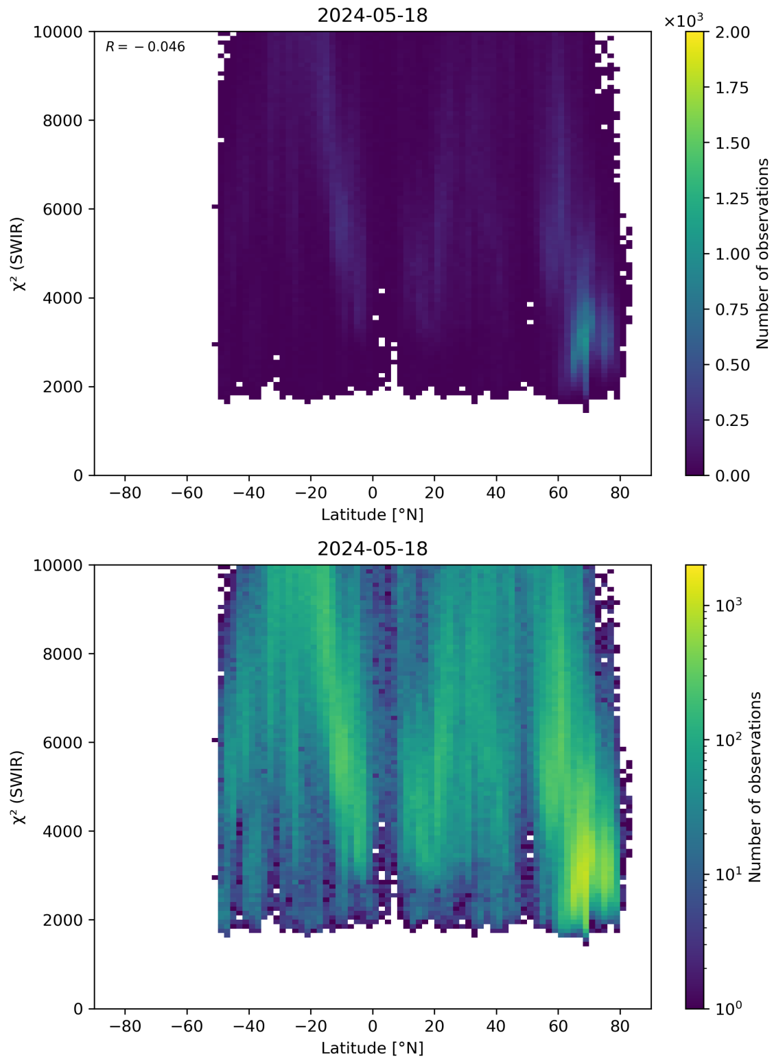
Figure 54: Scatter density plot of “Latitude” against “ \chi^2 (SWIR)” for 2024-05-18 to 2024-05-19.
