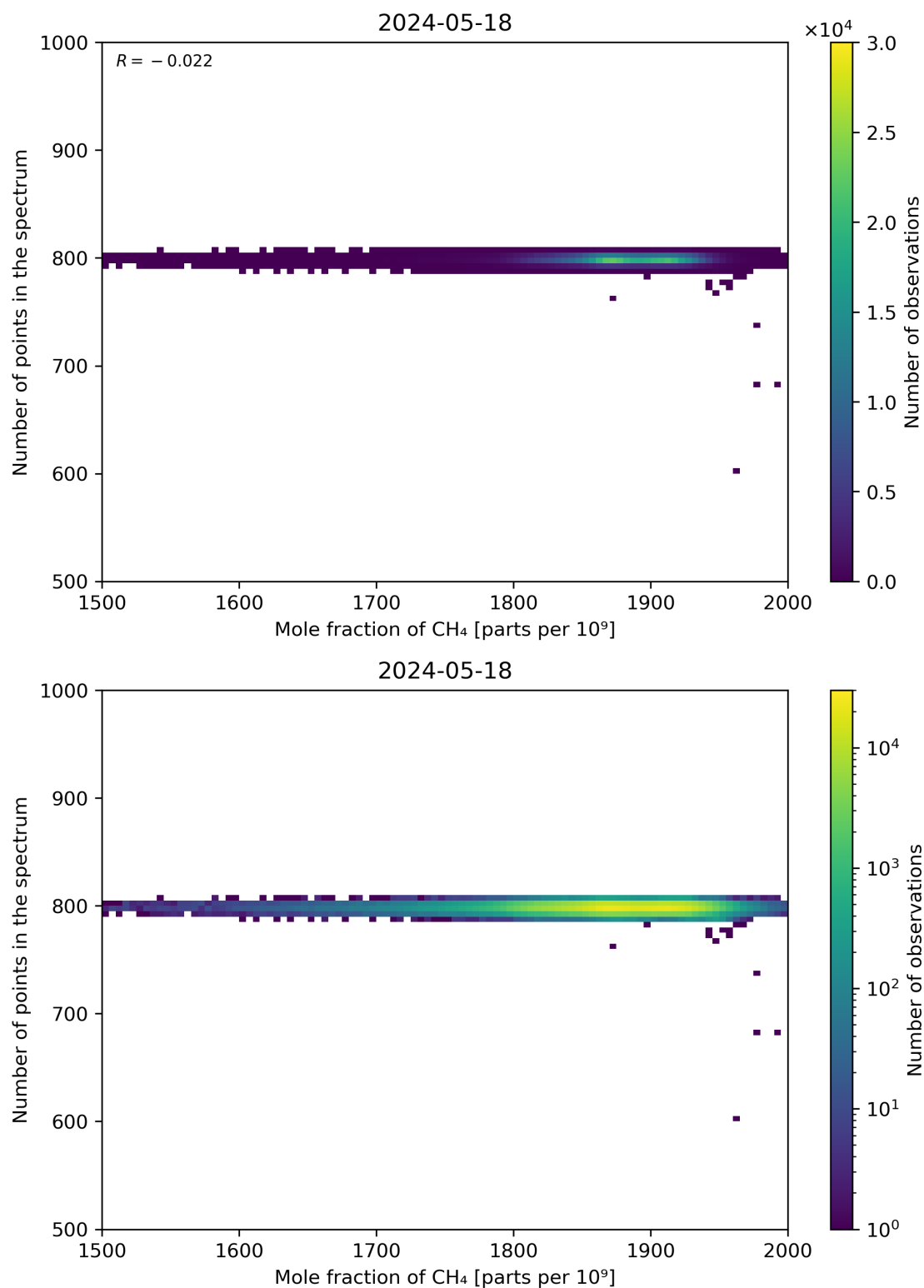
Figure 77: Scatter density plot of “Mole fraction of CH 4 ” against “Number of points in the spectrum” for 2024-05-18 to 2024-05-19.
