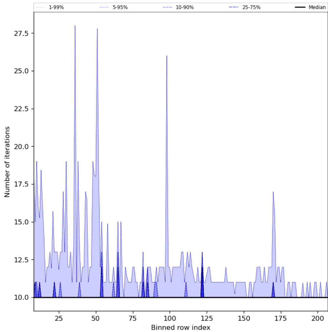
Figure 42: Along track statistics of “Number of iterations” for 2024-05-18 to 2024-05-19
