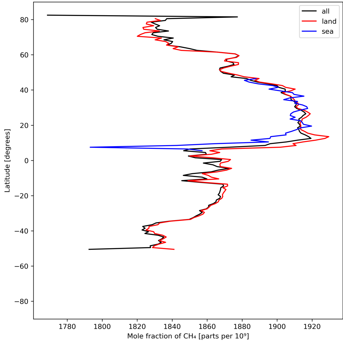
Figure 12: Zonal average of “Mole fraction of \text{CH}_4 ” for 2024-05-18 to 2024-05-19.
