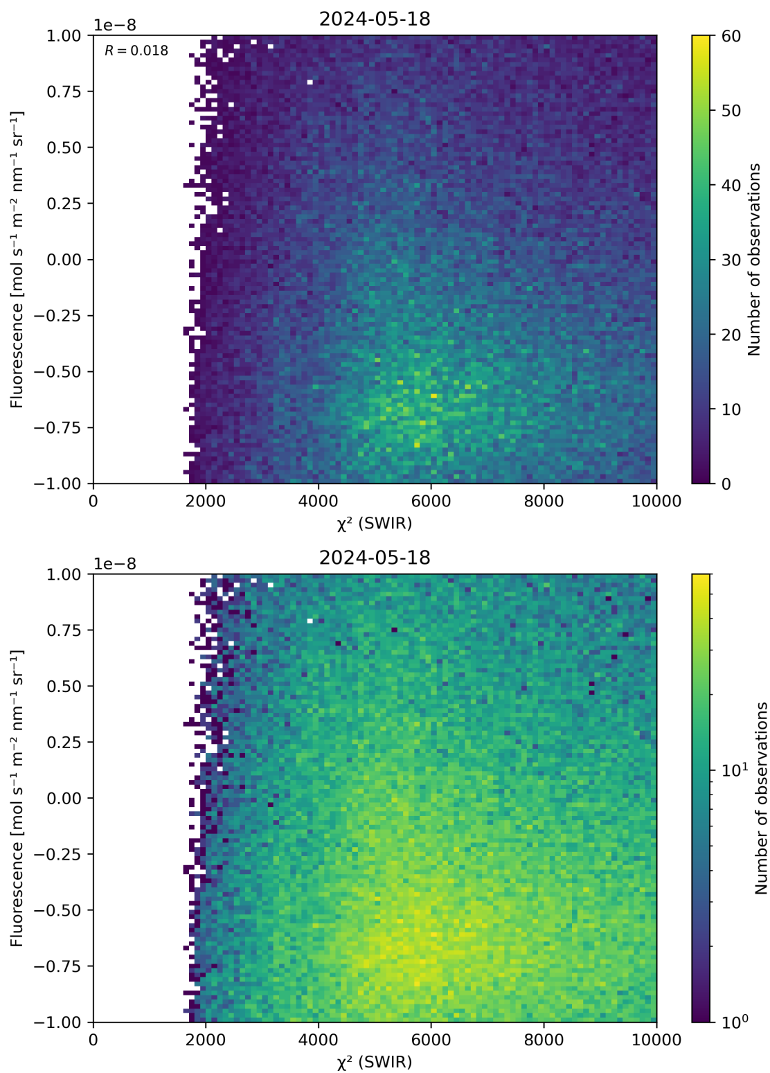
Figure 49: Scatter density plot of “ \chi^2 (SWIR)” against “Fluorescence” for 2024-05-18 to 2024-05-19.
