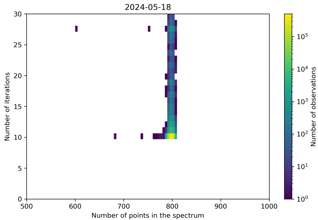
Figure 92: Scatter density plot of “Number of points in the spectrum” against “Number of iterations” for 2024-05-18 to 2024-05-19.
