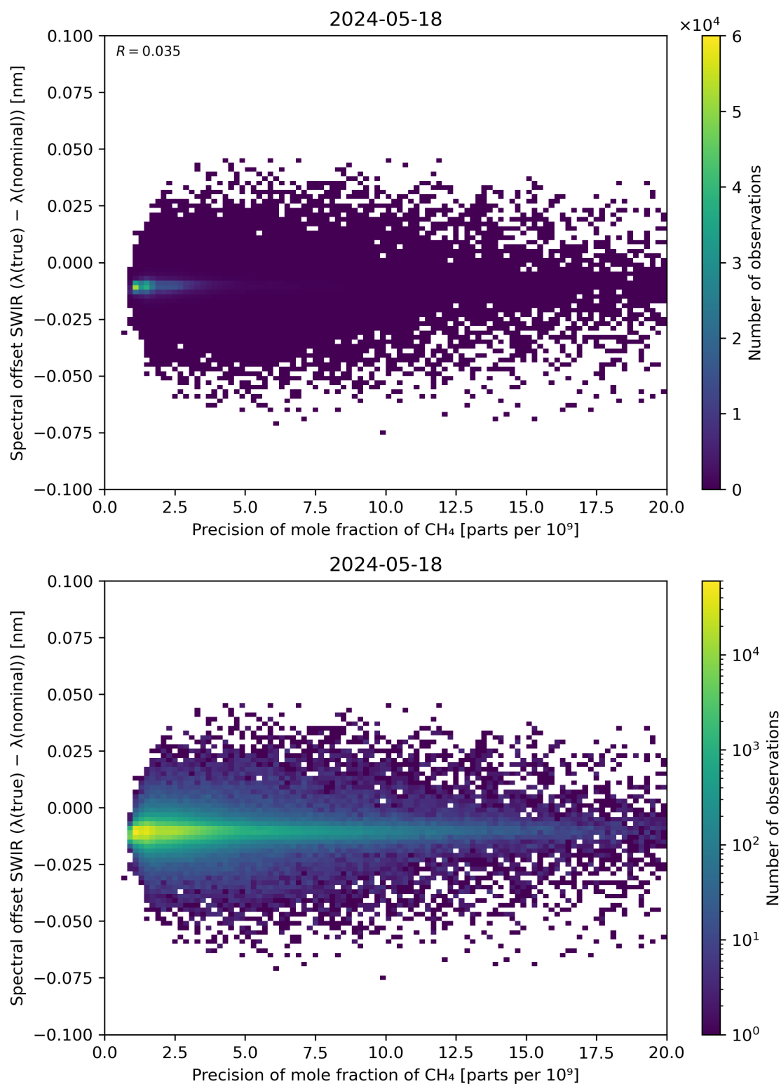
Figure 85: Scatter density plot of “Precision of mole fraction of CH 4 ” against “Spectral offset SWIR ( \lambda(\text{true}) - \lambda(\text{nominal}) )” for 2024-05-18 to 2024-05-19.
