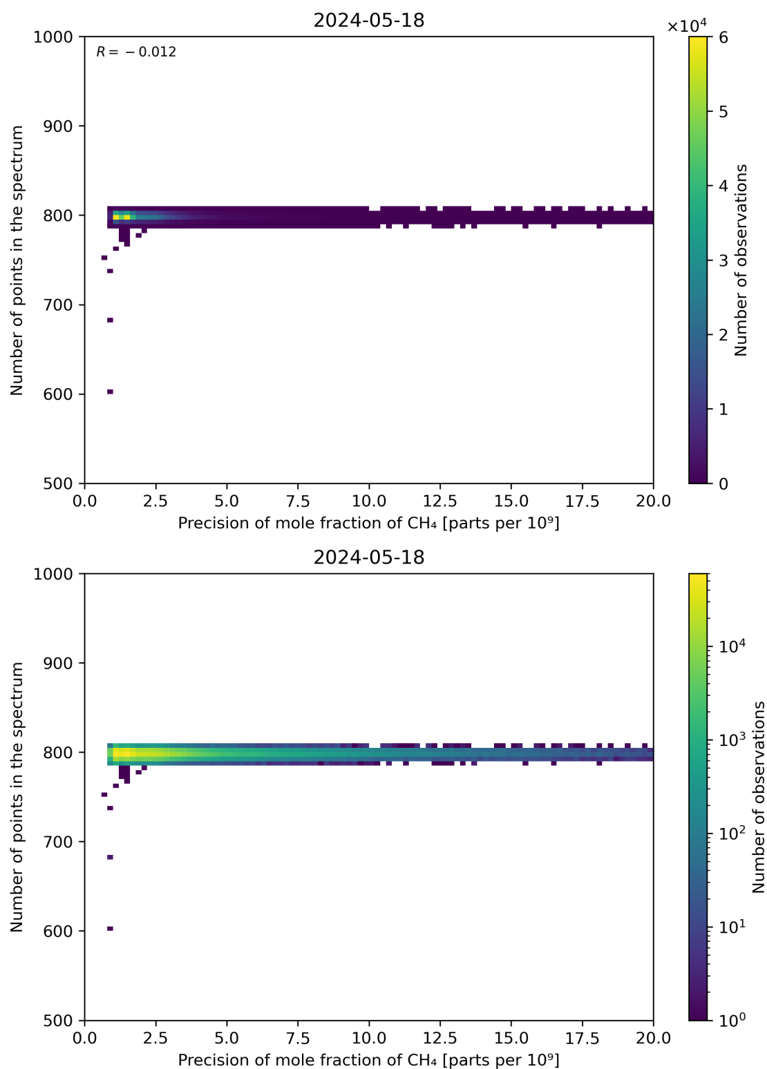
Figure 84: Scatter density plot of “Precision of mole fraction of CH 4 ” against “Number of points in the spectrum” for 2024-05-18 to 2024-05-19.
