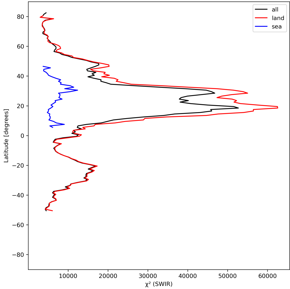
Figure 17: Zonal average of “ \chi^2 (SWIR)” for 2024-05-18 to 2024-05-19.
