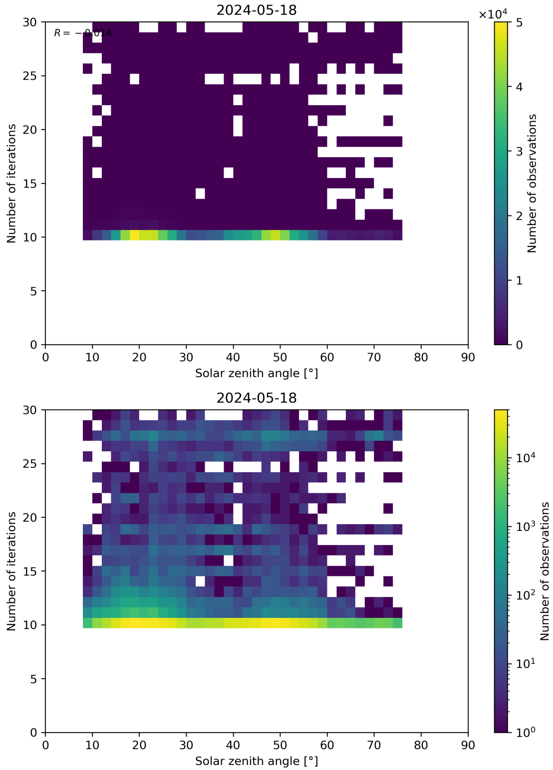
Figure 102: Scatter density plot of “Solar zenith angle” against “Number of iterations” for 2024-05-18 to 2024-05-19.
