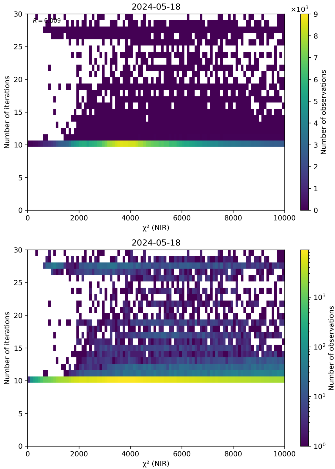
Figure 46: Scatter density plot of “ \chi^2 (NIR)” against “Number of iterations” for 2024-05-18 to 2024-05-19.
