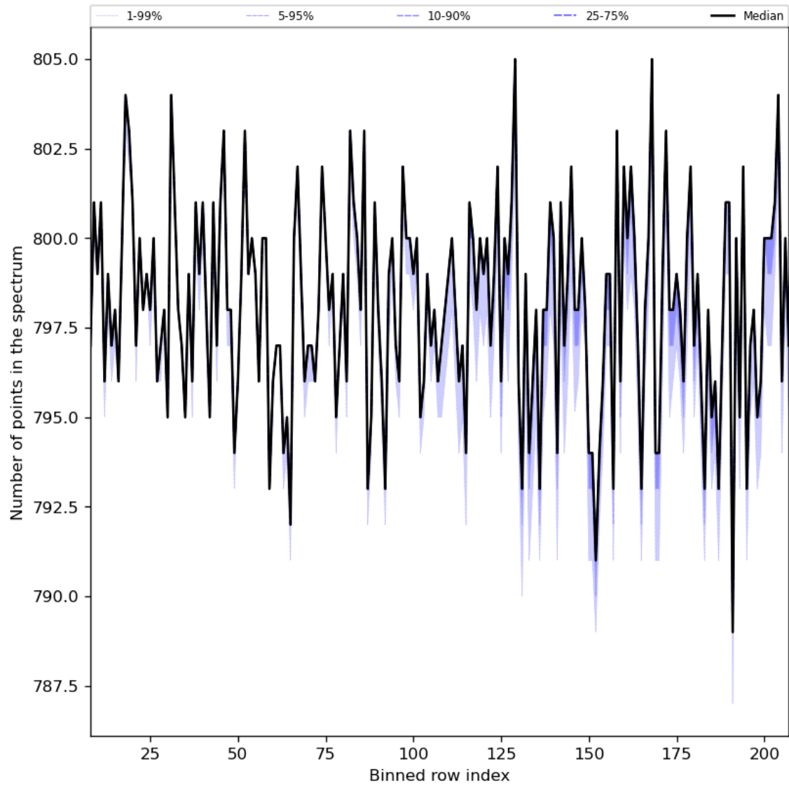
Figure 37: Along track statistics of “Number of points in the spectrum” for 2024-05-18 to 2024-05-19
