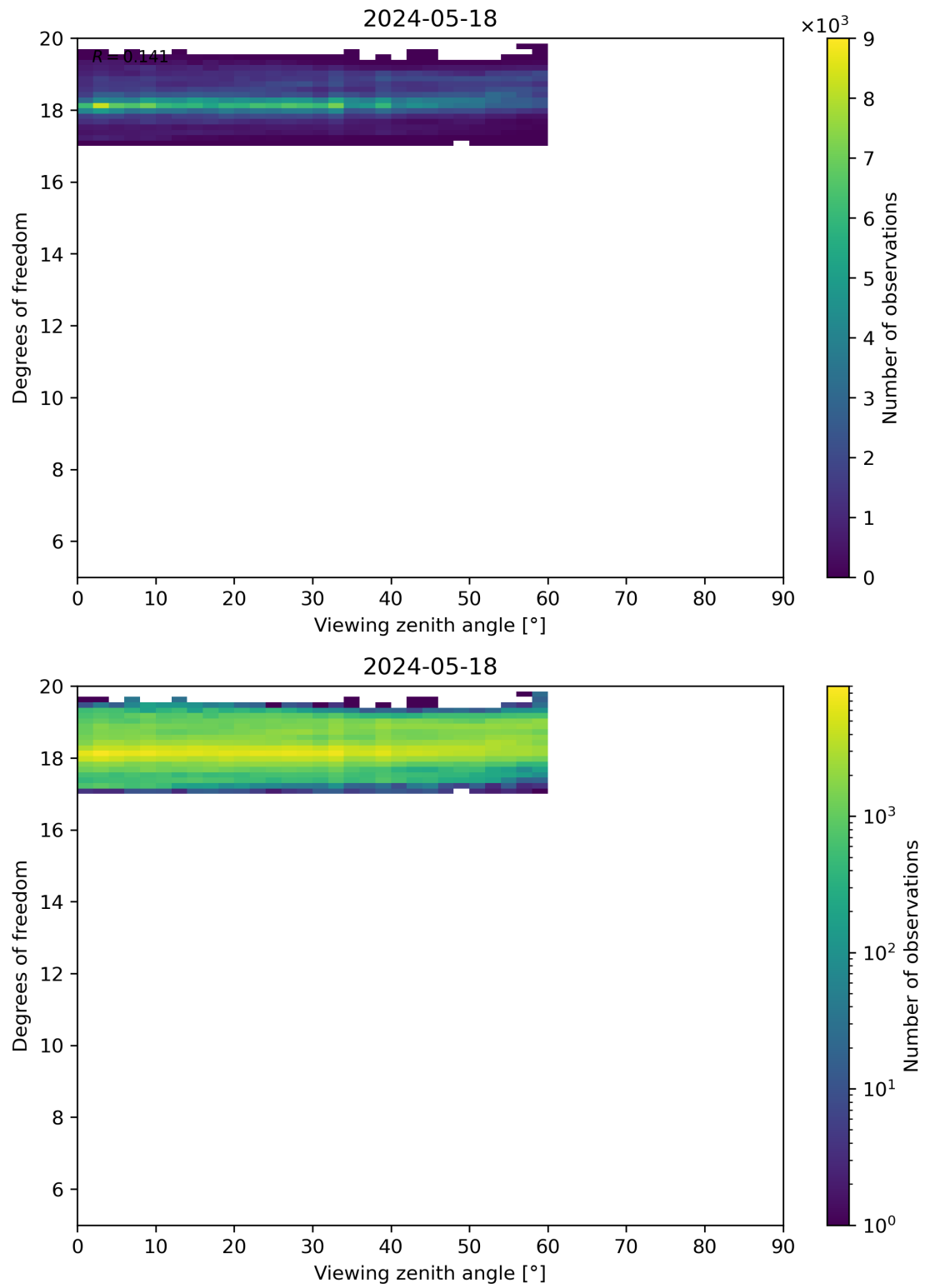
Figure 107: Scatter density plot of “Viewing zenith angle” against “Degrees of freedom” for 2024-05-18 to 2024-05-19.
