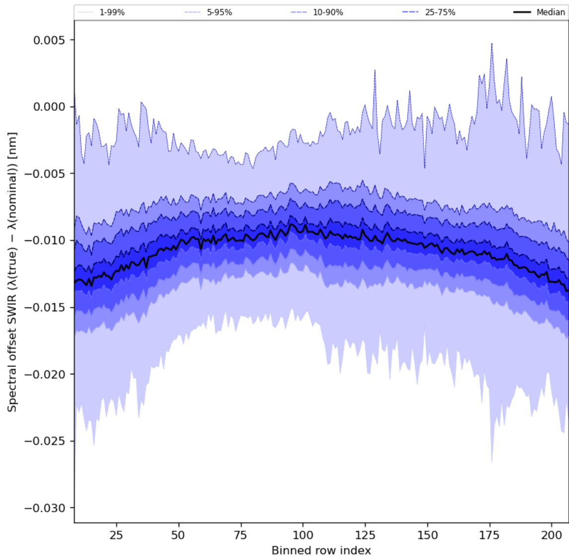
Figure 38: Along track statistics of “Spectral offset SWIR ( \lambda(\text{true}) - \lambda(\text{nominal}) )” for 2024-05-18 to 2024-05-19
