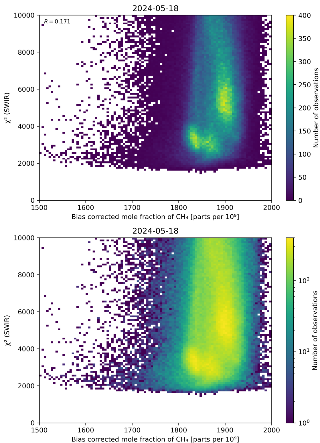
Figure 64: Scatter density plot of “Bias corrected mole fraction of CH 4 ” against “ \chi^2 (SWIR)” for 2024-05-18 to 2024-05-19.
