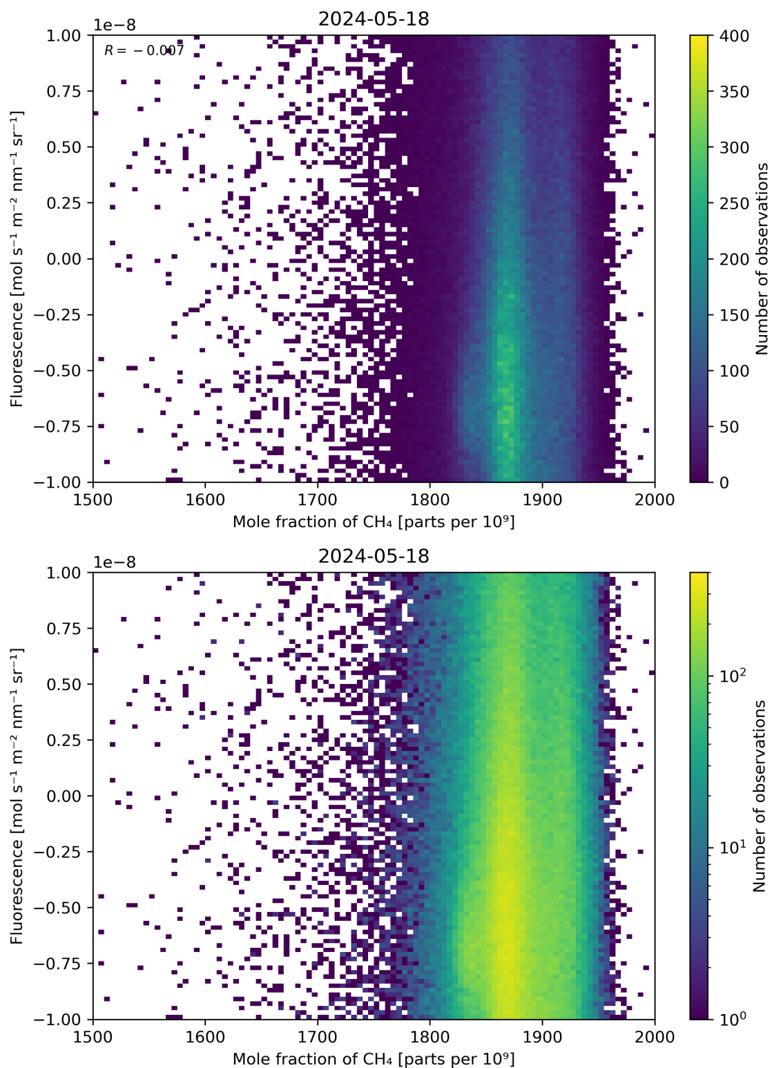
Figure 73: Scatter density plot of “Mole fraction of CH 4 ” against “Fluorescence” for 2024-05-18 to 2024-05-19.
