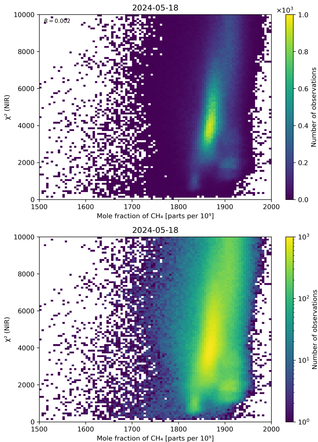
Figure 70: Scatter density plot of “Mole fraction of \text{CH}_4 ” against “ \chi^2 (NIR)” for 2024-05-18 to 2024-05-19.
