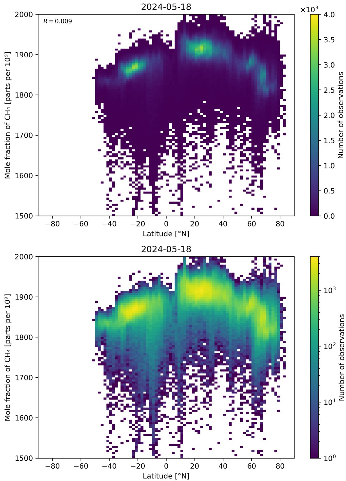
Figure 57: Scatter density plot of “Latitude” against “Mole fraction of \text{CH}_4 ” for 2024-05-18 to 2024-05-19.
