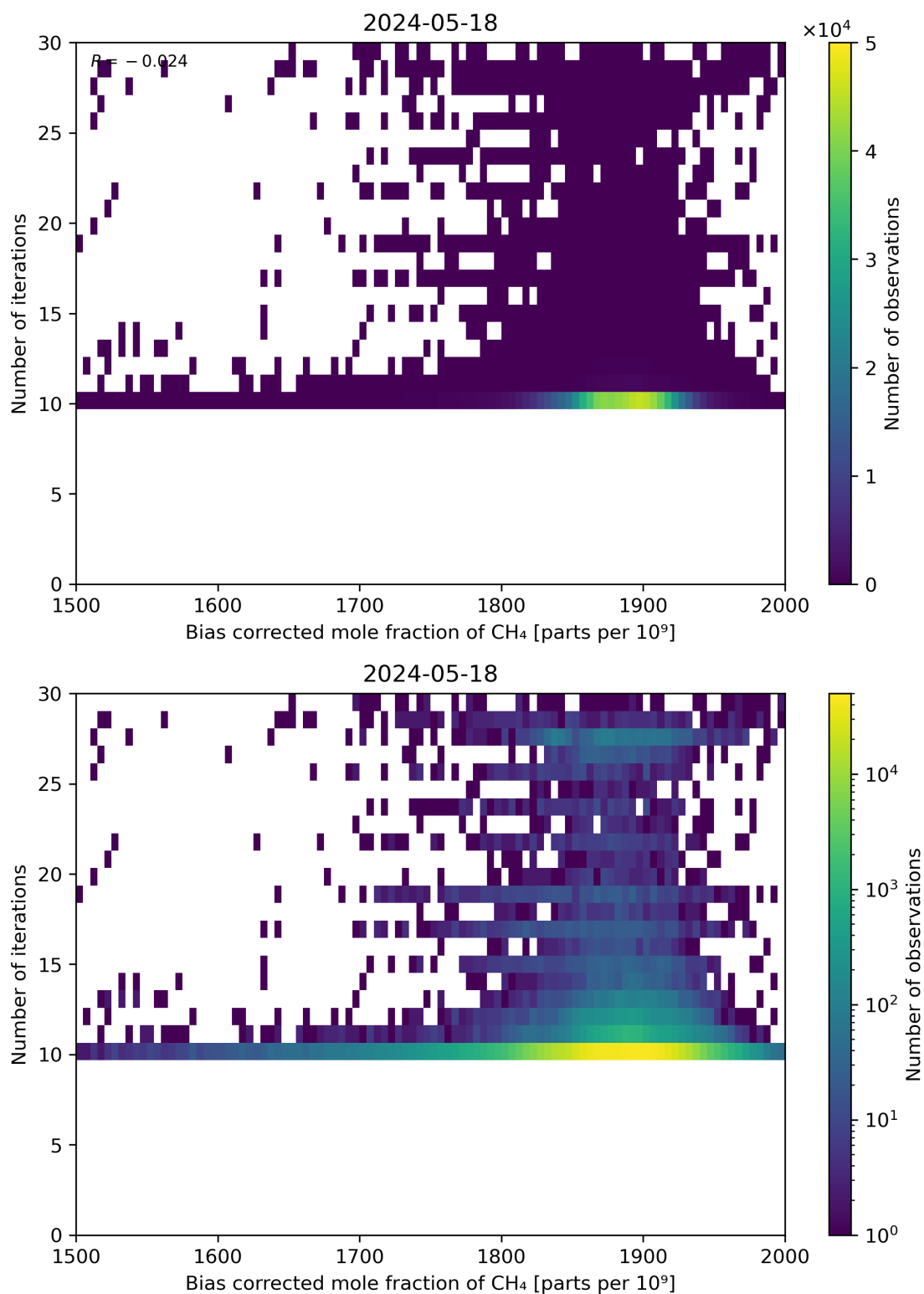
Figure 67: Scatter density plot of “Bias corrected mole fraction of CH 4 ” against “Number of iterations” for 2024-05-18 to 2024-05-19.
