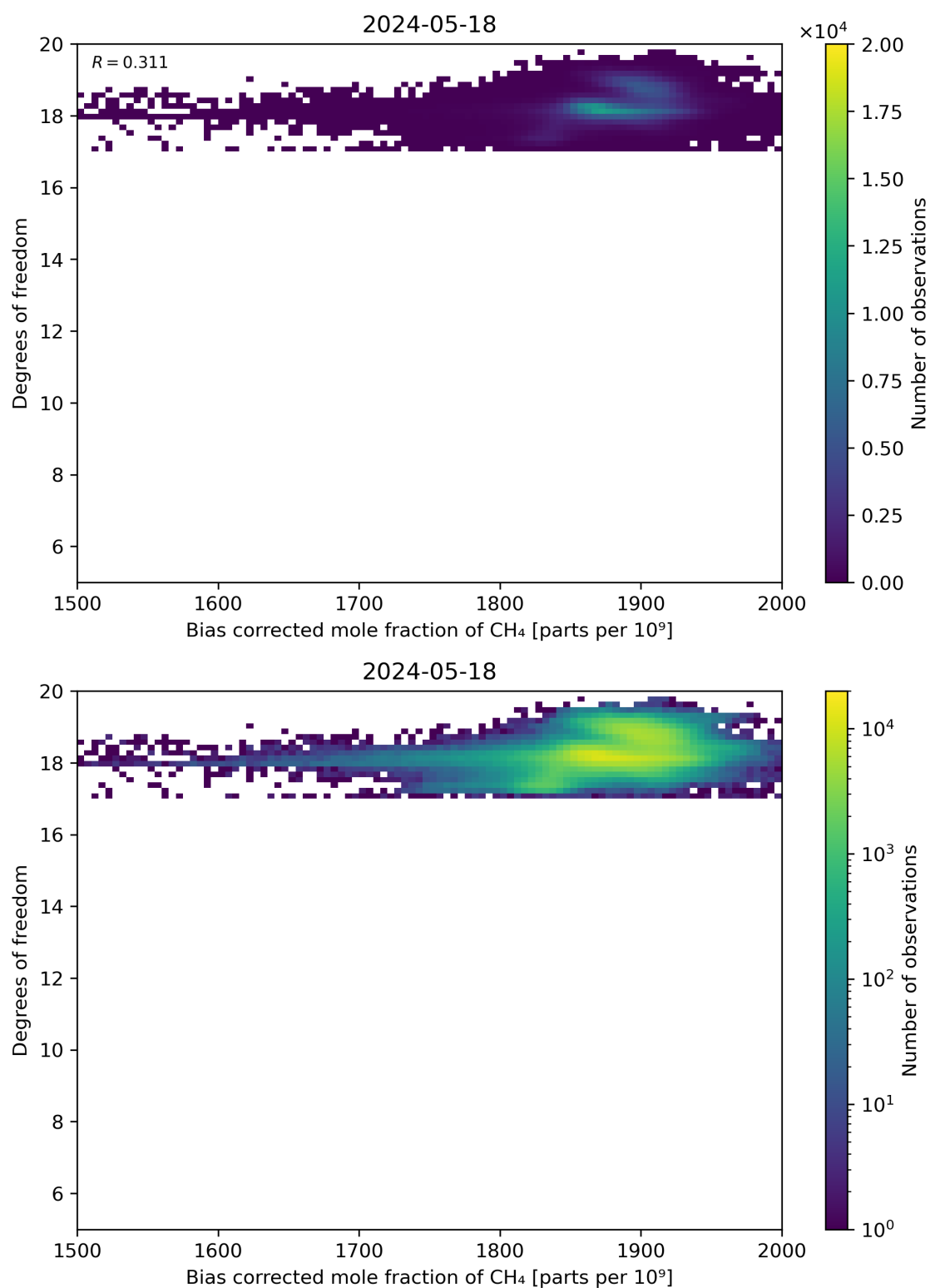
Figure 65: Scatter density plot of “Bias corrected mole fraction of CH 4 ” against “Degrees of freedom” for 2024-05-18 to 2024-05-19.
