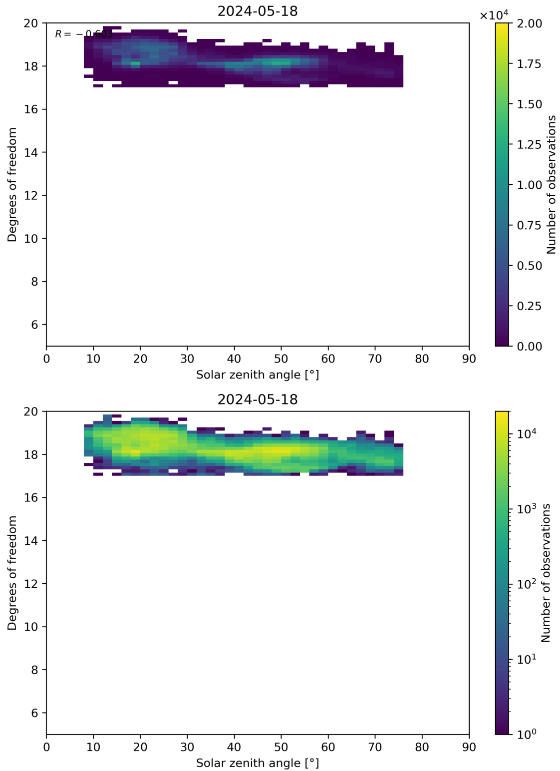
Figure 96: Scatter density plot of “Solar zenith angle” against “Degrees of freedom” for 2024-05-18 to 2024-05-19.
