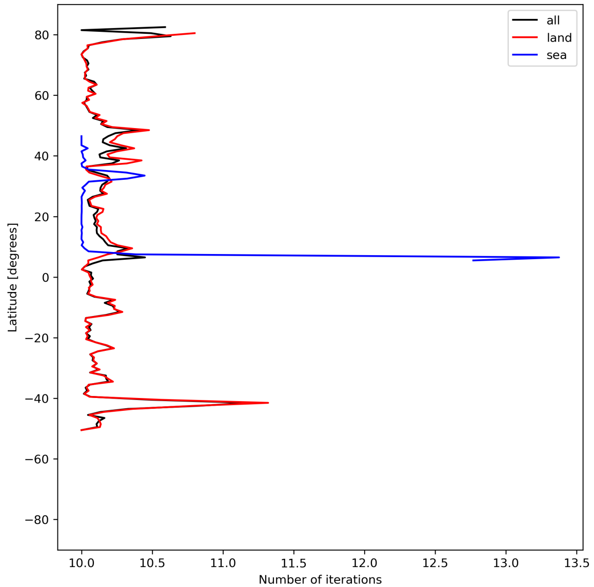
Figure 20: Zonal average of “Number of iterations” for 2024-05-18 to 2024-05-19.
