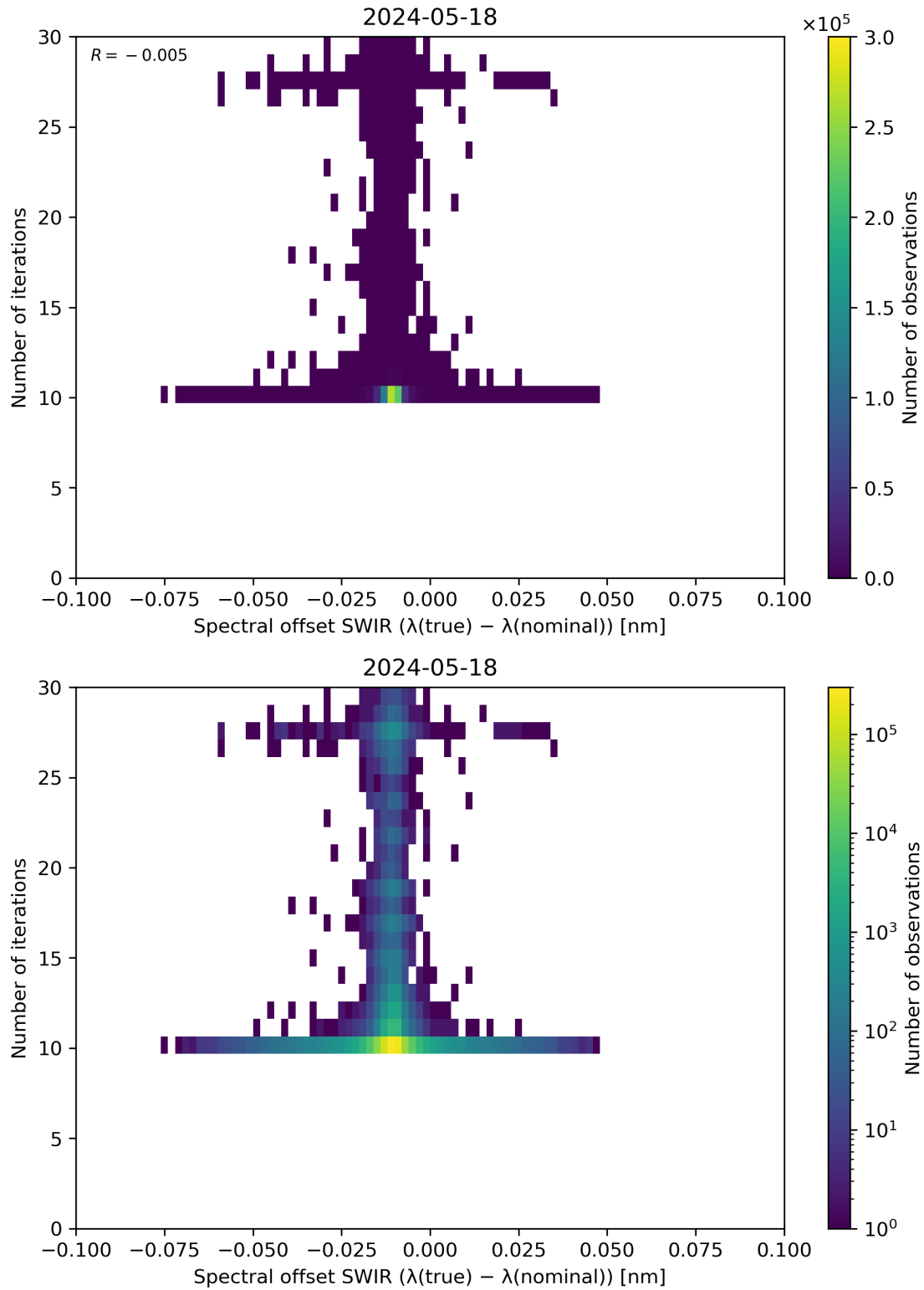
Figure 121: Scatter density plot of “Spectral offset SWIR ( \lambda(\text{true}) - \lambda(\text{nominal}) )” against “Number of iterations” for 2024-05-18 to 2024-05-19.
