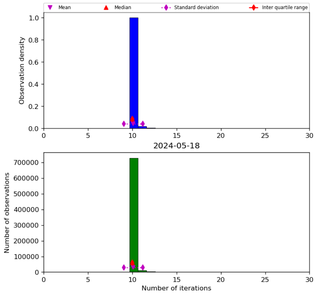
Figure 31: Histogram of “Number of iterations” for 2024-05-18 to 2024-05-19
