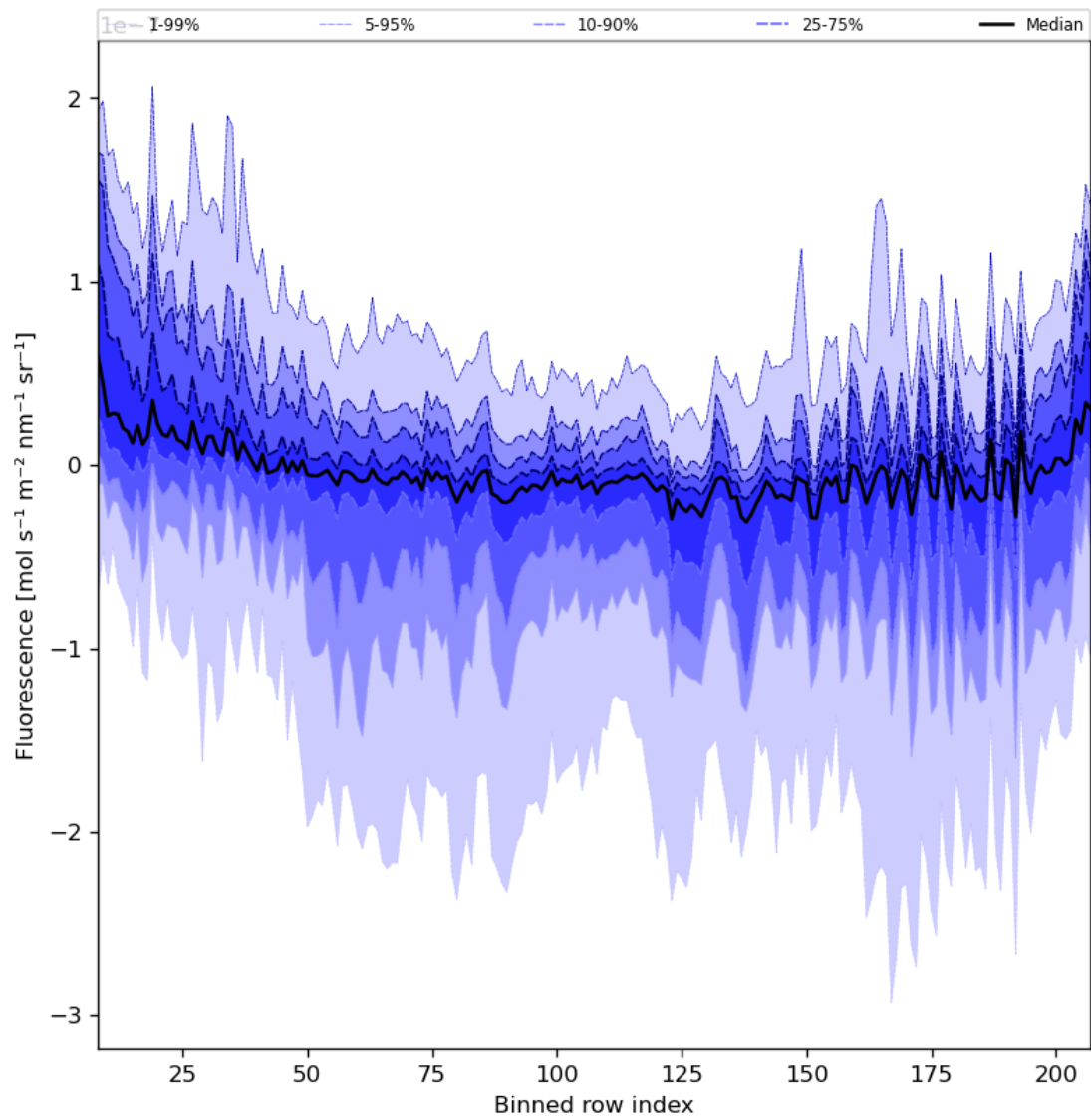
Figure 43: Along track statistics of “Fluorescence” for 2024-05-18 to 2024-05-19
