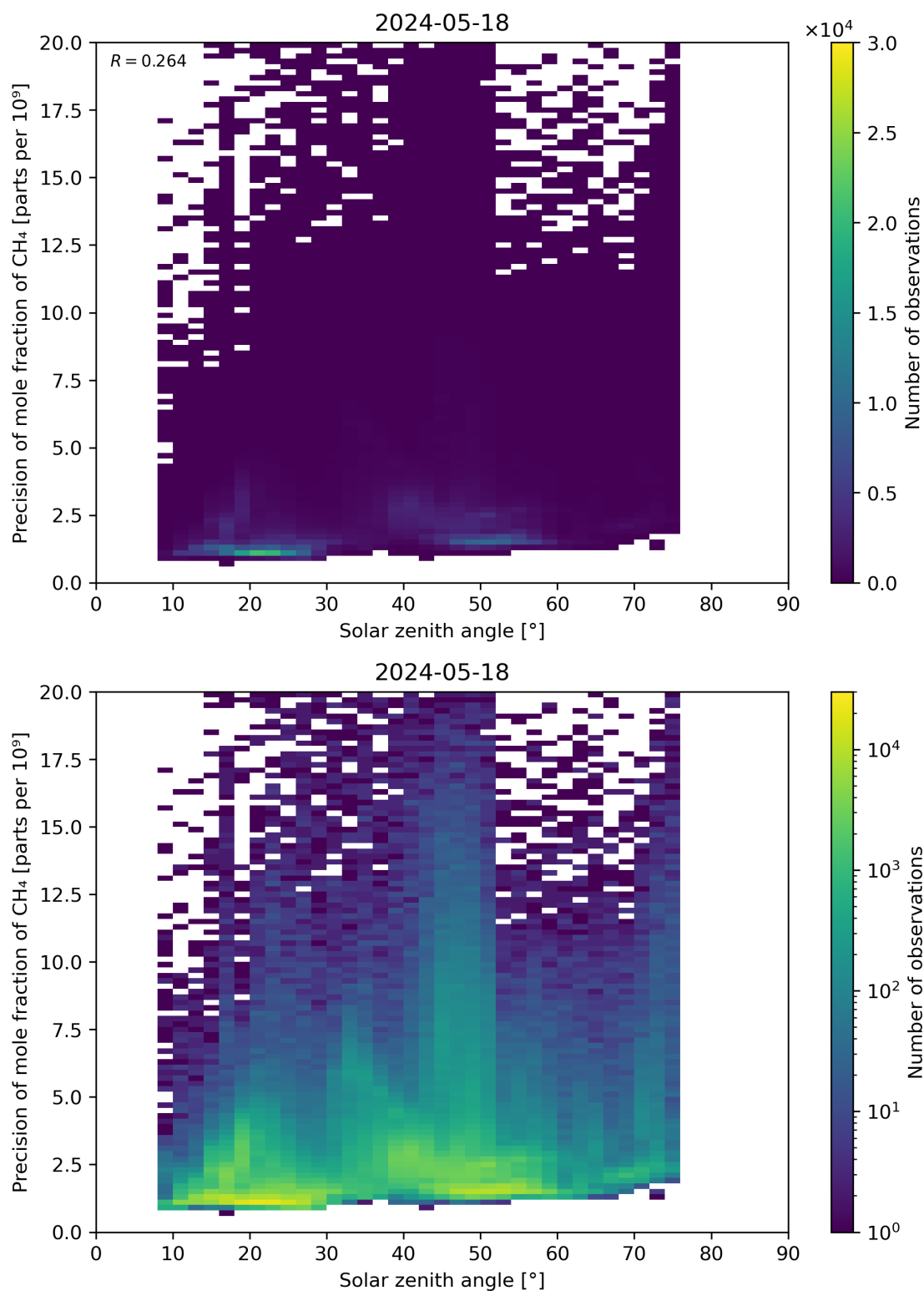
Figure 101: Scatter density plot of “Solar zenith angle” against “Precision of mole fraction of CH 4 ” for 2024-05-18 to 2024-05-19.
