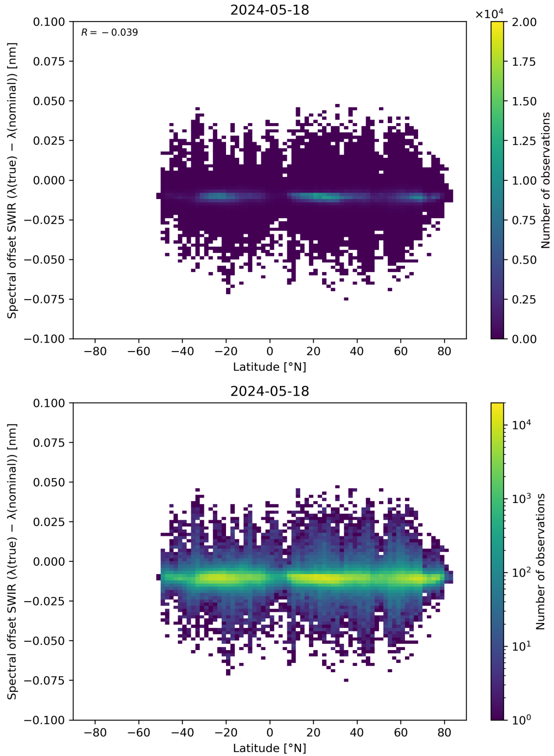
Figure 62: Scatter density plot of “Latitude” against “Spectral offset SWIR ( \lambda(\text{true}) - \lambda(\text{nominal}) )” for 2024-05-18 to 2024-05-19.
