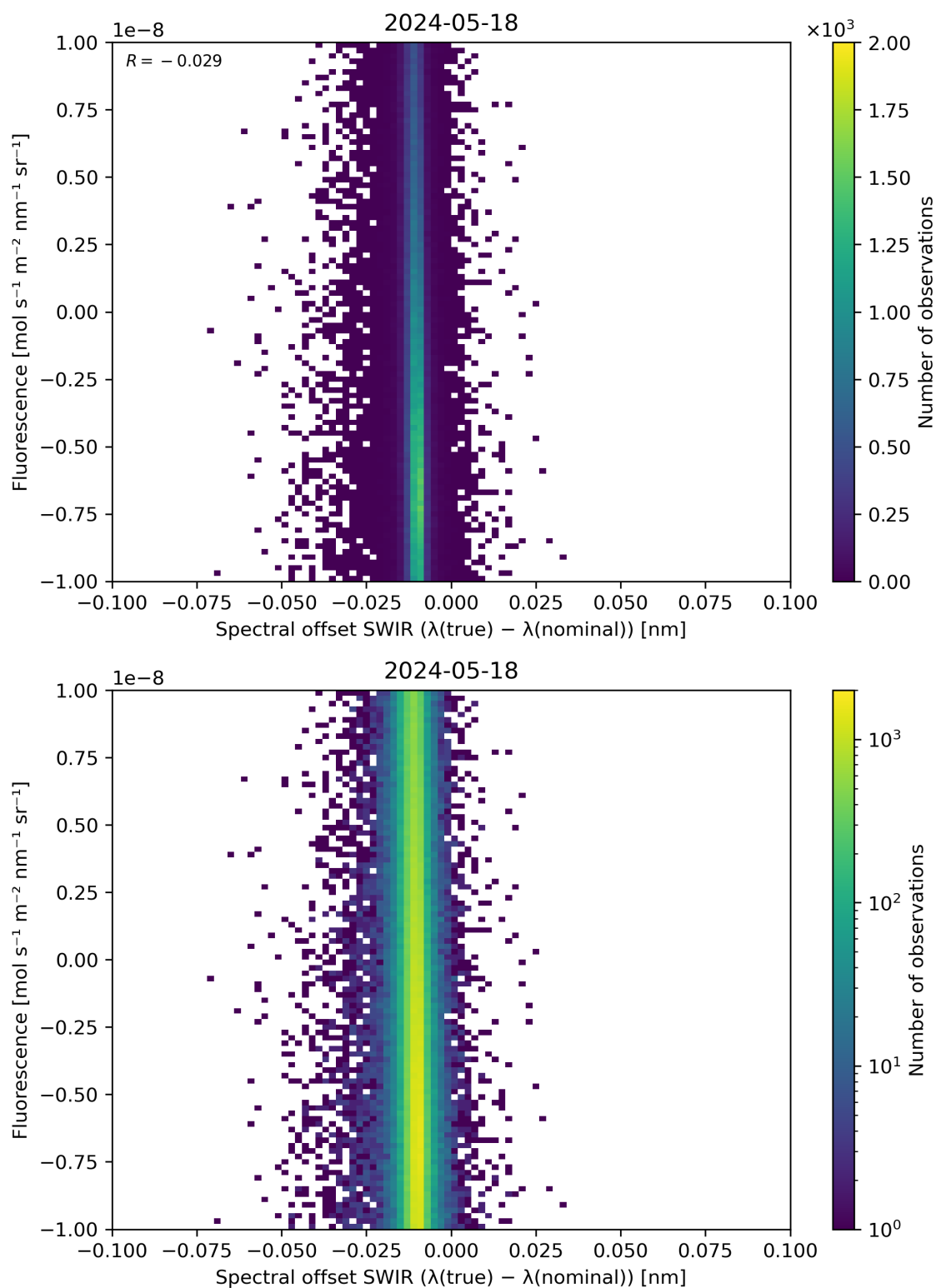
Figure 120: Scatter density plot of “Spectral offset SWIR ( \lambda(\text{true}) - \lambda(\text{nominal}) )” against “Fluorescence” for 2024-05-18 to 2024-05-19.
