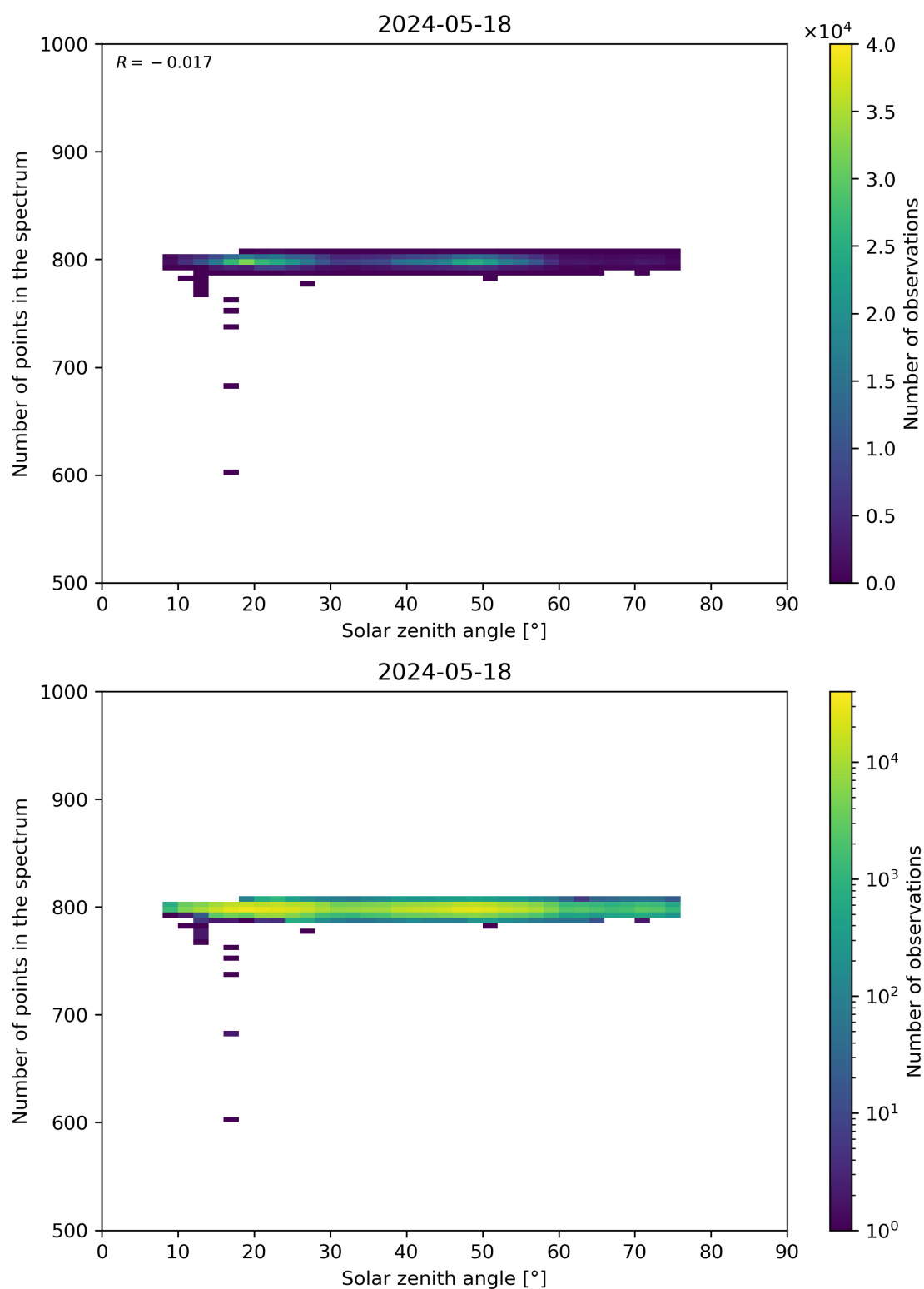
Figure 103: Scatter density plot of “Solar zenith angle” against “Number of points in the spectrum” for 2024-05-18 to 2024-05-19.
