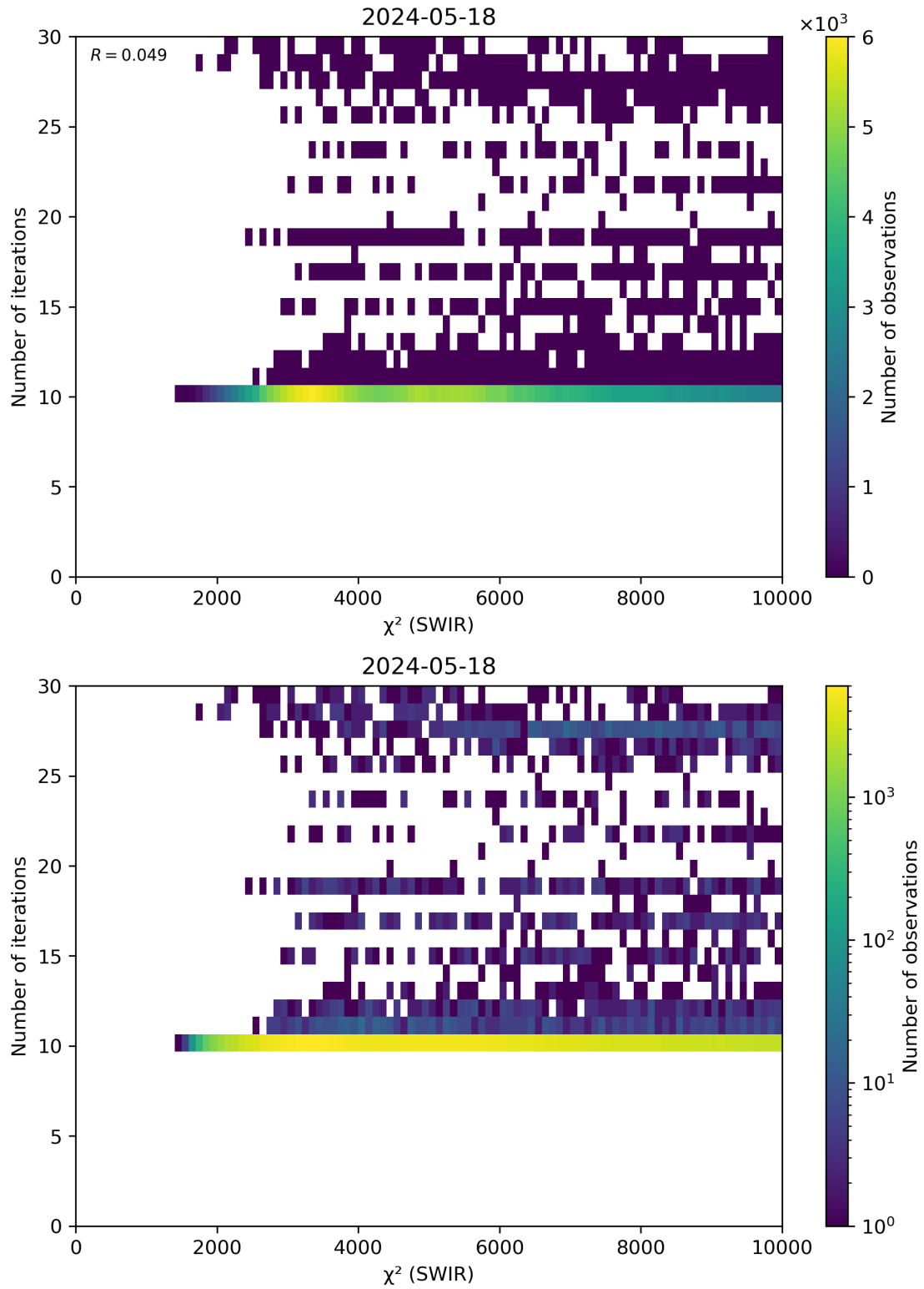
Figure 50: Scatter density plot of “ \chi^2 (SWIR)” against “Number of iterations” for 2024-05-18 to 2024-05-19.
