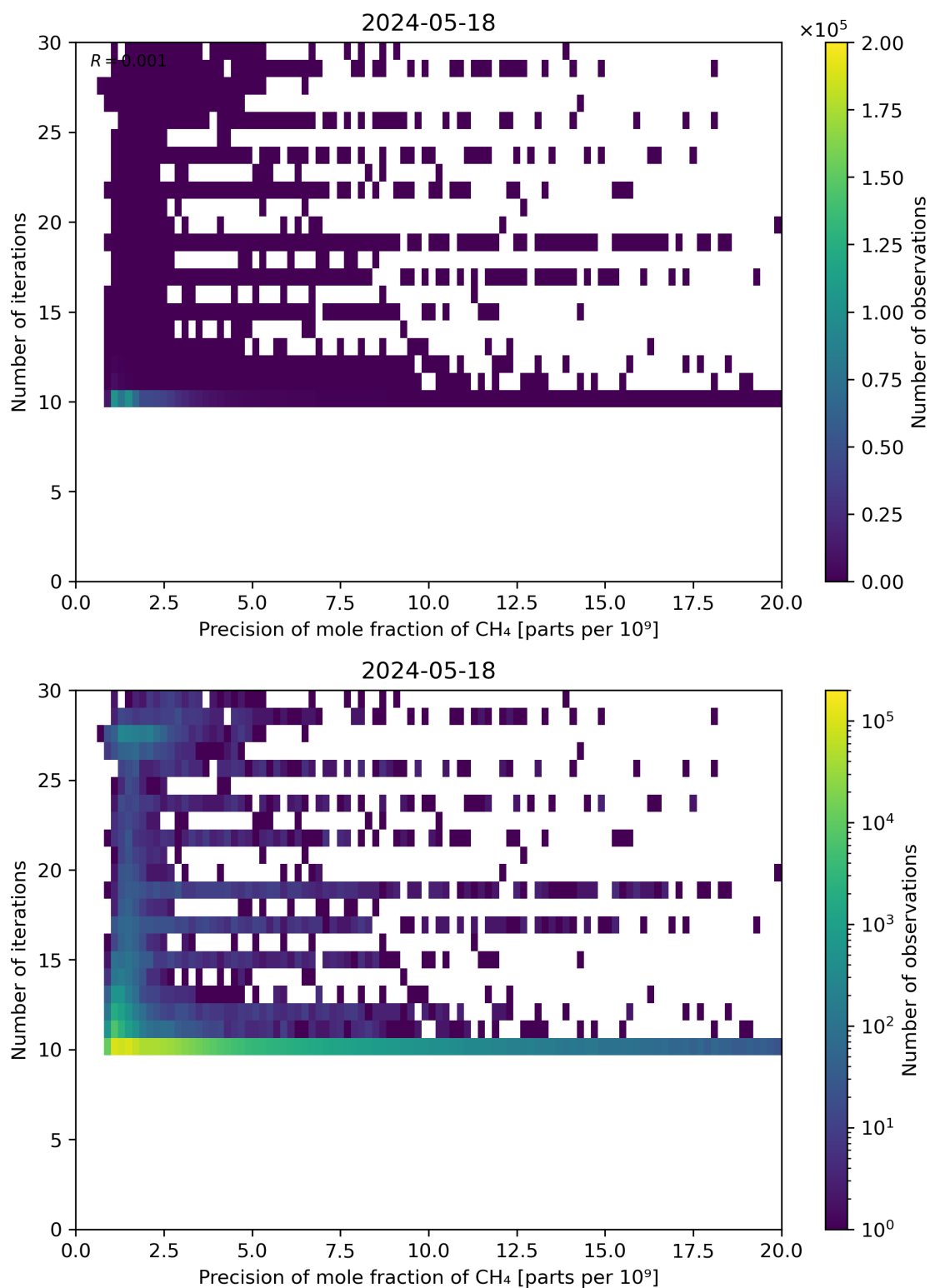
Figure 83: Scatter density plot of “Precision of mole fraction of CH 4 ” against “Number of iterations” for 2024-05-18 to 2024-05-19.
