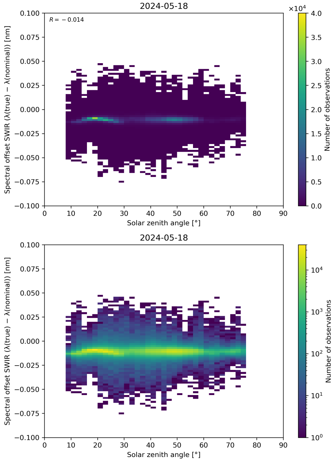
Figure 104: Scatter density plot of “Solar zenith angle” against “Spectral offset SWIR ( \lambda(\text{true}) - \lambda(\text{nominal}) )” for 2024-05-18 to 2024-05-19.
