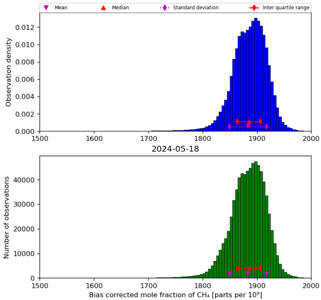
Figure 25: Histogram of “Bias corrected mole fraction of CH 4 ” for 2024-05-18 to 2024-05-19
