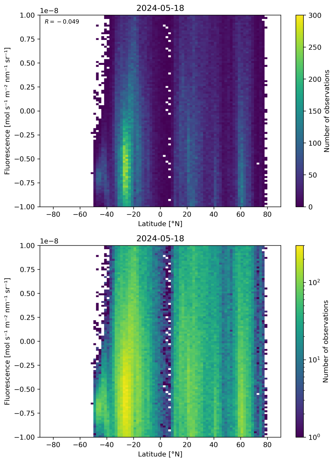
Figure 56: Scatter density plot of “Latitude” against “Fluorescence” for 2024-05-18 to 2024-05-19.
