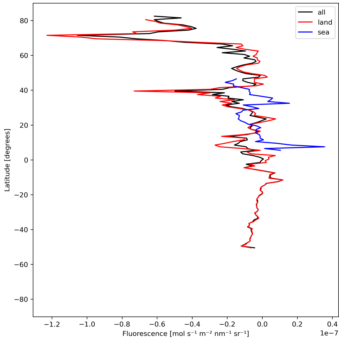
Figure 21: Zonal average of “Fluorescence” for 2024-05-18 to 2024-05-19.
