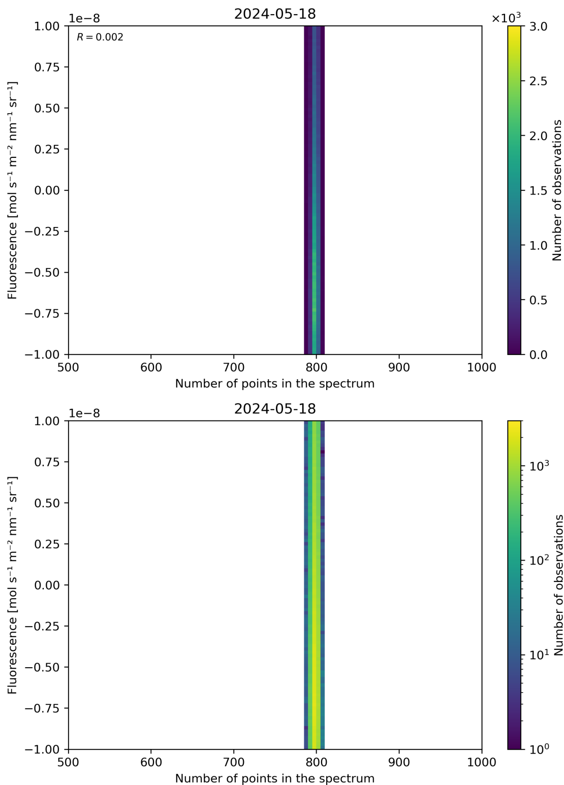
Figure 91: Scatter density plot of “Number of points in the spectrum” against “Fluorescence” for 2024-05-18 to 2024-05-19.
