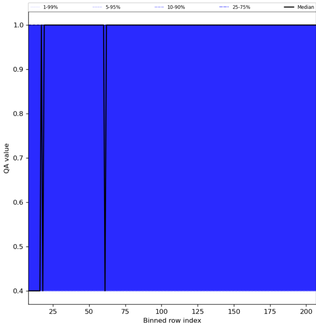
Figure 33: Along track statistics of “QA value” for 2024-05-18 to 2024-05-19
