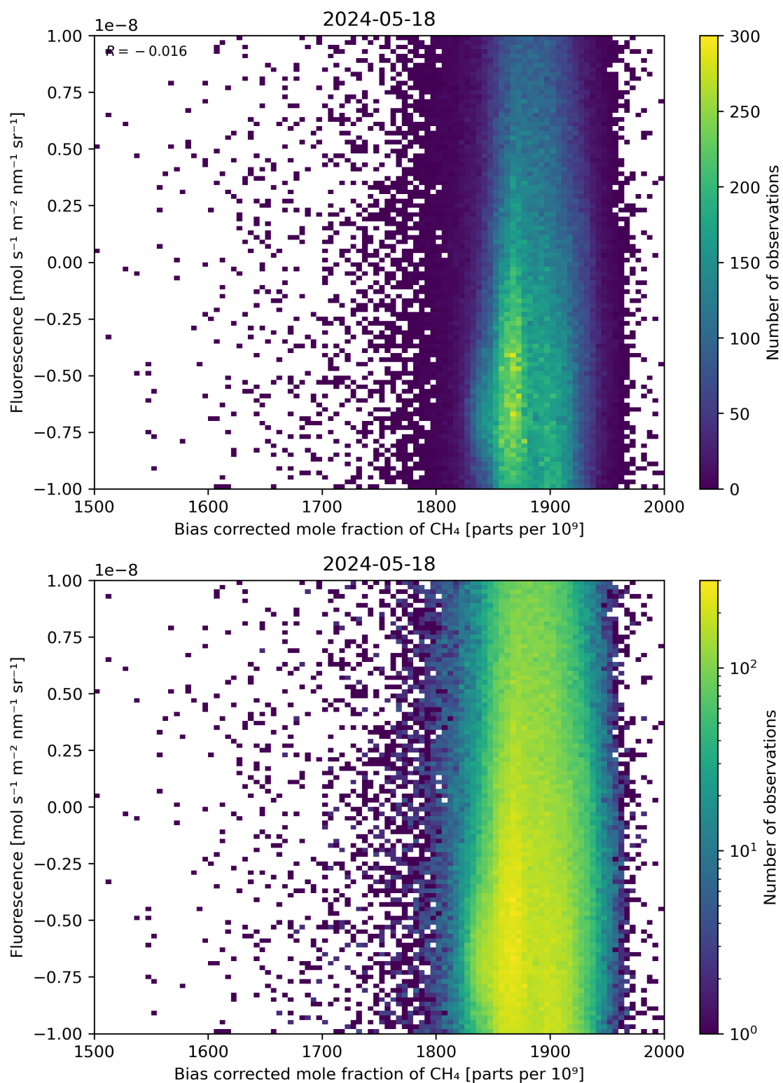
Figure 66: Scatter density plot of “Bias corrected mole fraction of \text{CH}_4 ” against “Fluorescence” for 2024-05-18 to 2024-05-19.
