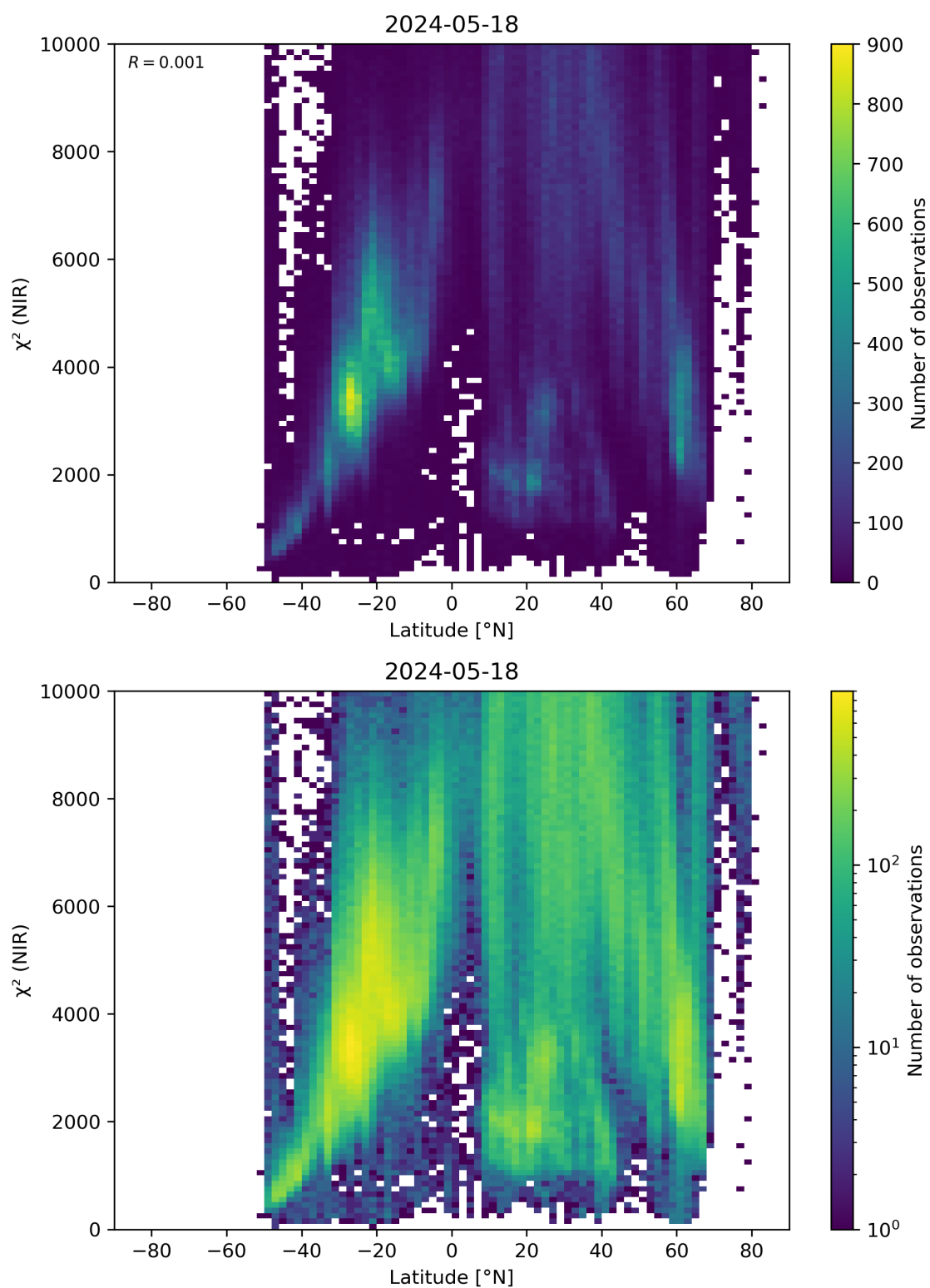
Figure 53: Scatter density plot of “Latitude” against “ \chi^2 (NIR)” for 2024-05-18 to 2024-05-19.
