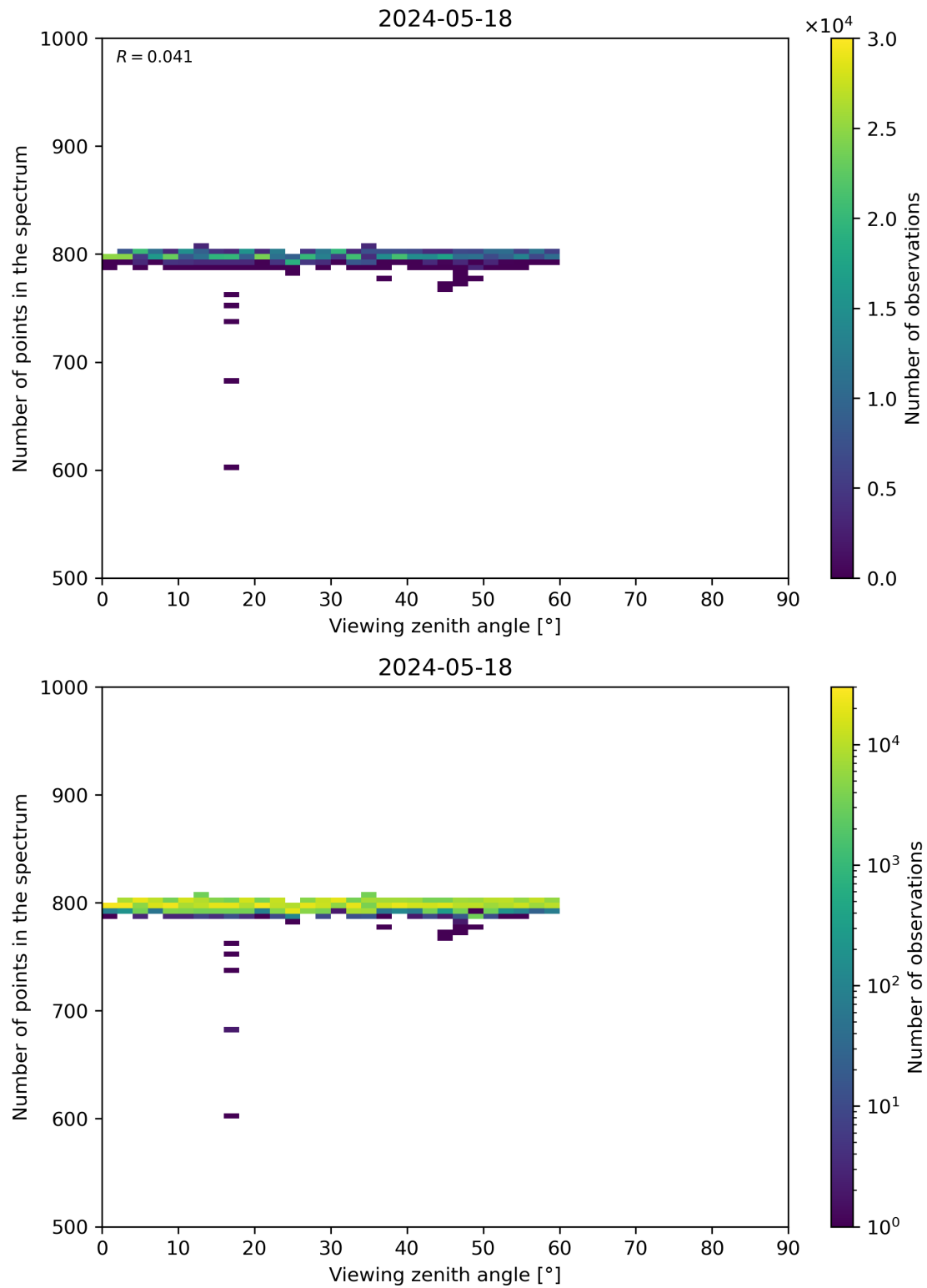
Figure 114: Scatter density plot of “Viewing zenith angle” against “Number of points in the spectrum” for 2024-05-18 to 2024-05-19.
