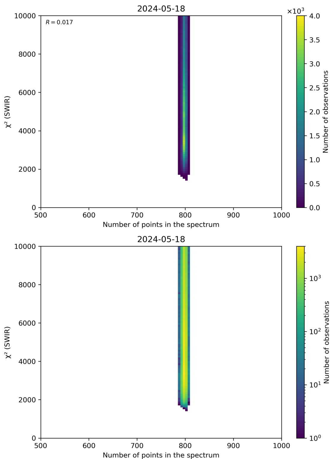
Figure 89: Scatter density plot of “Number of points in the spectrum” against “ \chi^2 (SWIR)” for 2024-05-18 to 2024-05-19.
