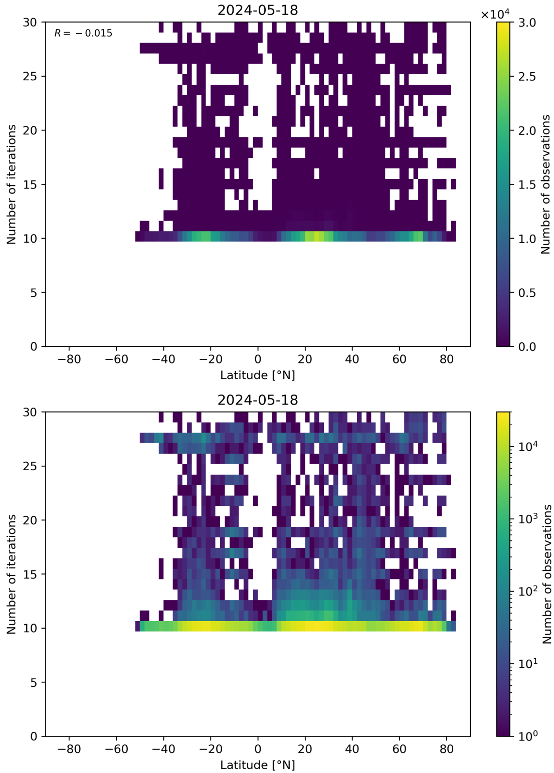
Figure 60: Scatter density plot of “Latitude” against “Number of iterations” for 2024-05-18 to 2024-05-19.
