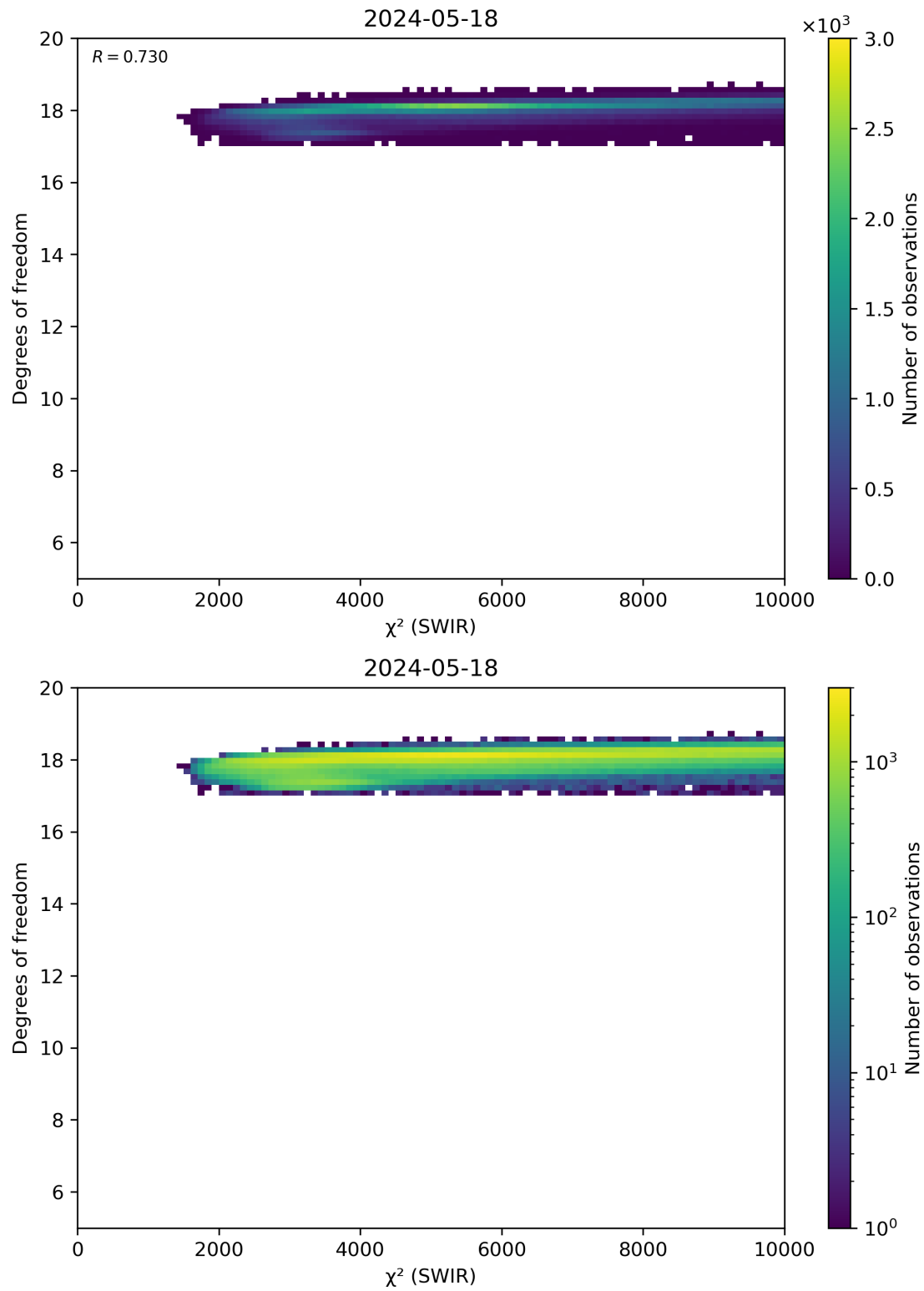
Figure 48: Scatter density plot of “ \chi^2 (SWIR)” against “Degrees of freedom” for 2024-05-18 to 2024-05-19.
