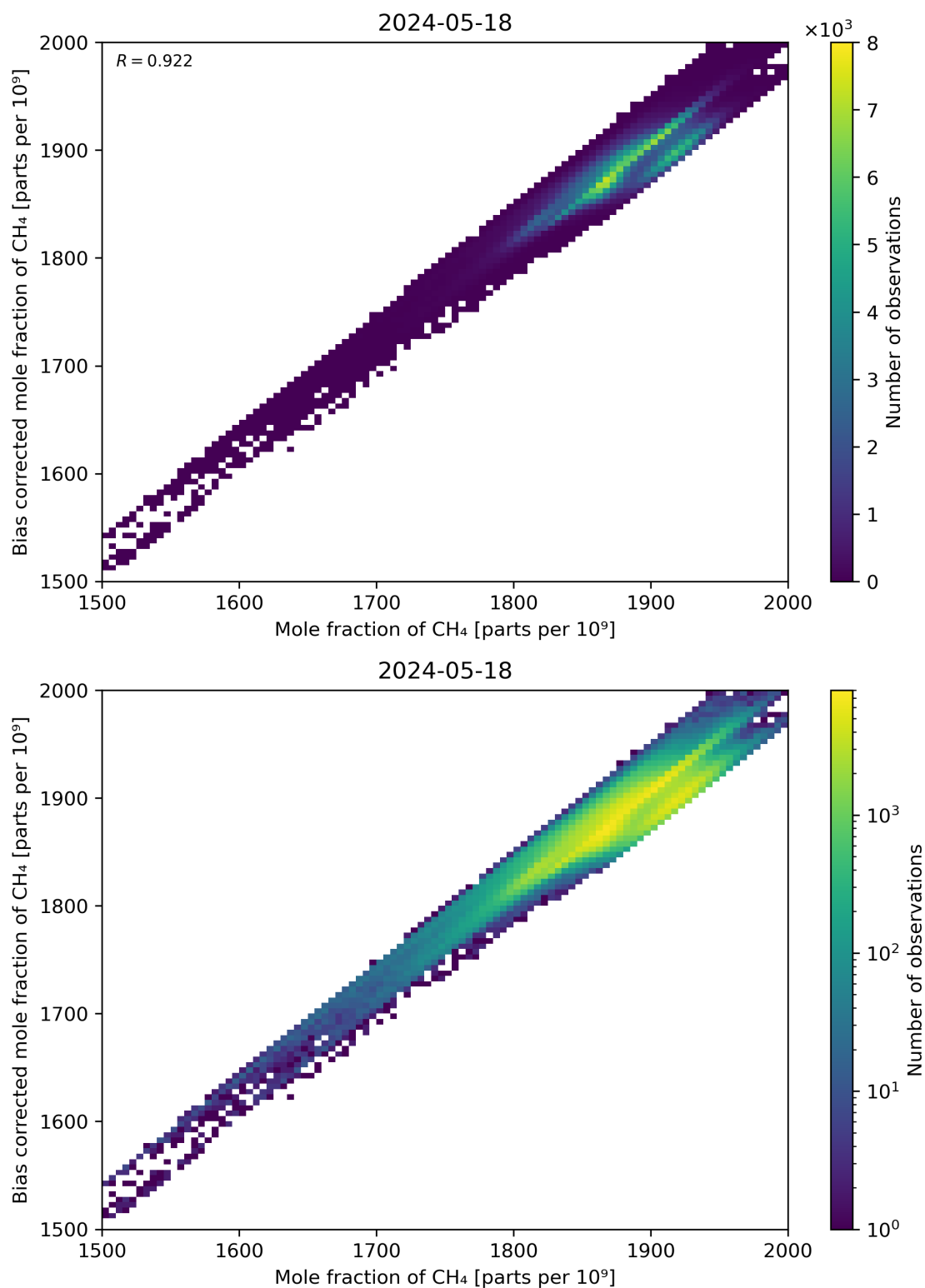
Figure 74: Scatter density plot of “Mole fraction of CH 4 ” against “Bias corrected mole fraction of CH 4 ” for 2024-05-18 to 2024-05-19.
