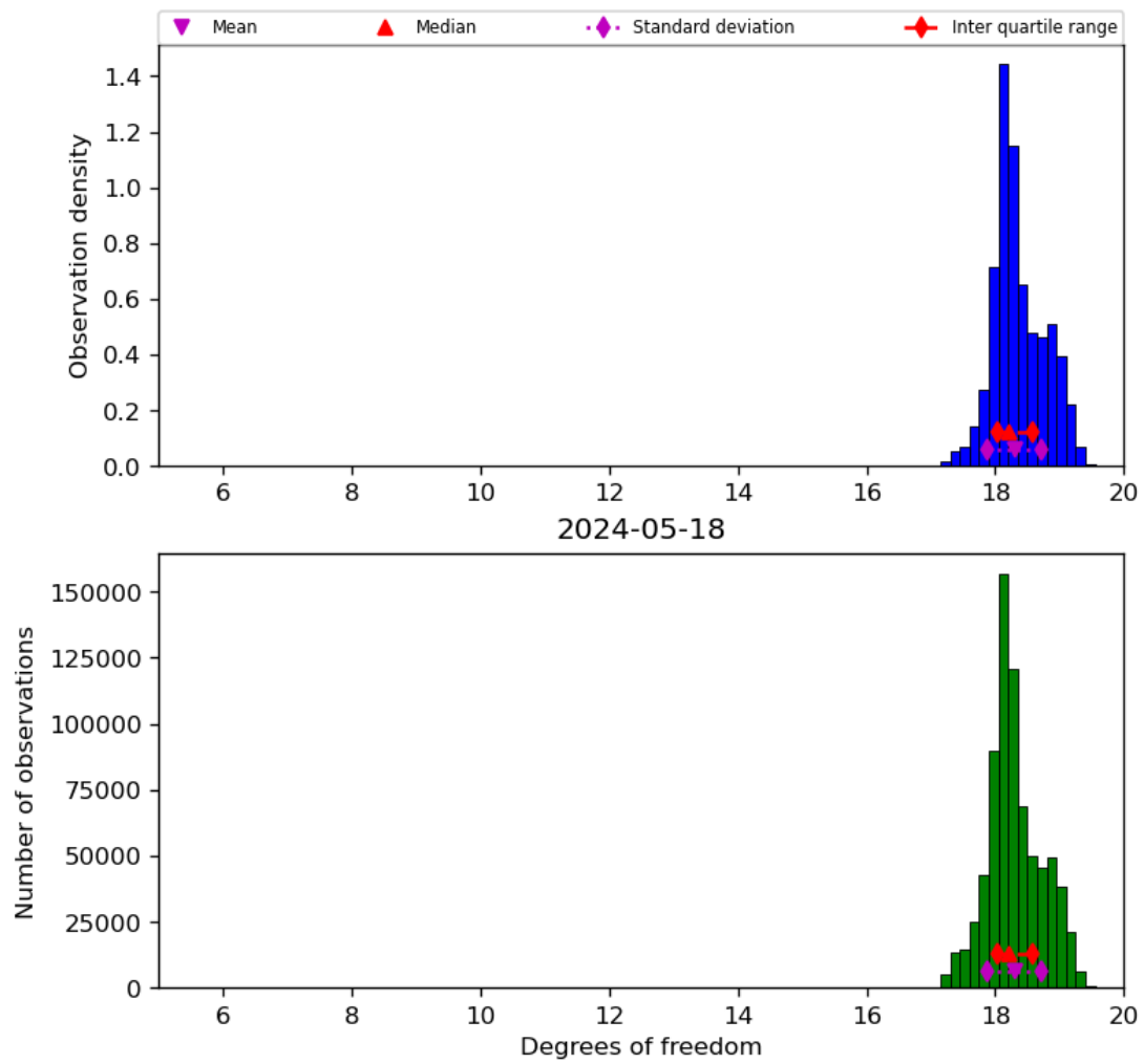
Figure 30: Histogram of “Degrees of freedom” for 2024-05-18 to 2024-05-19
