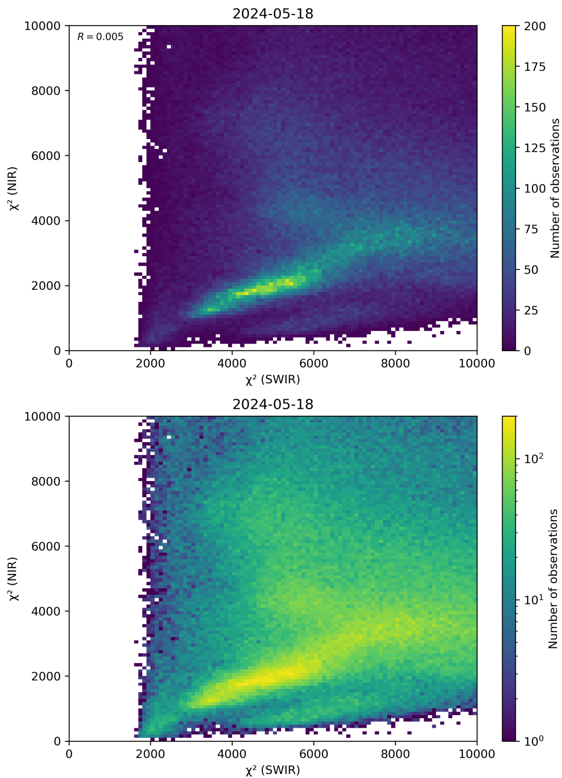
Figure 47: Scatter density plot of “ \chi^2 (SWIR)” against “ \chi^2 (NIR)” for 2024-05-18 to 2024-05-19.
