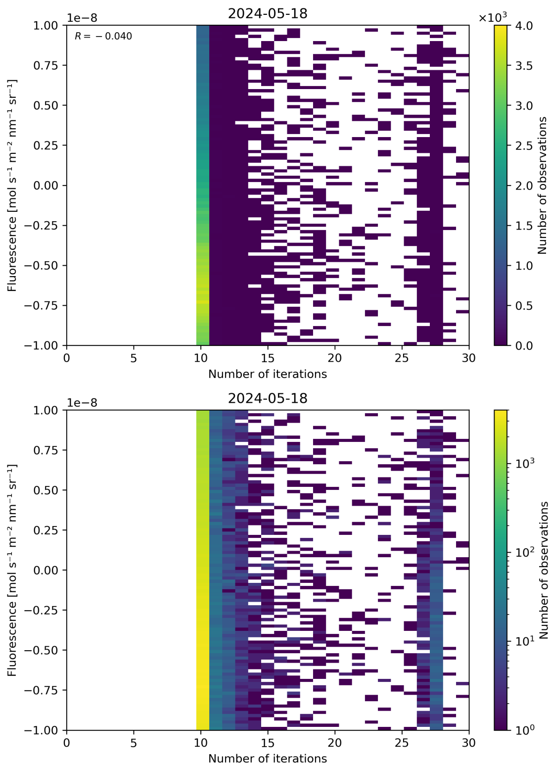
Figure 87: Scatter density plot of “Number of iterations” against “Fluorescence” for 2024-05-18 to 2024-05-19.
