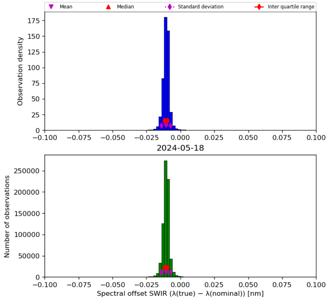
Figure 27: Histogram of “Spectral offset SWIR ( \lambda(\text{true}) - \lambda(\text{nominal}) )” for 2024-05-18 to 2024-05-19
