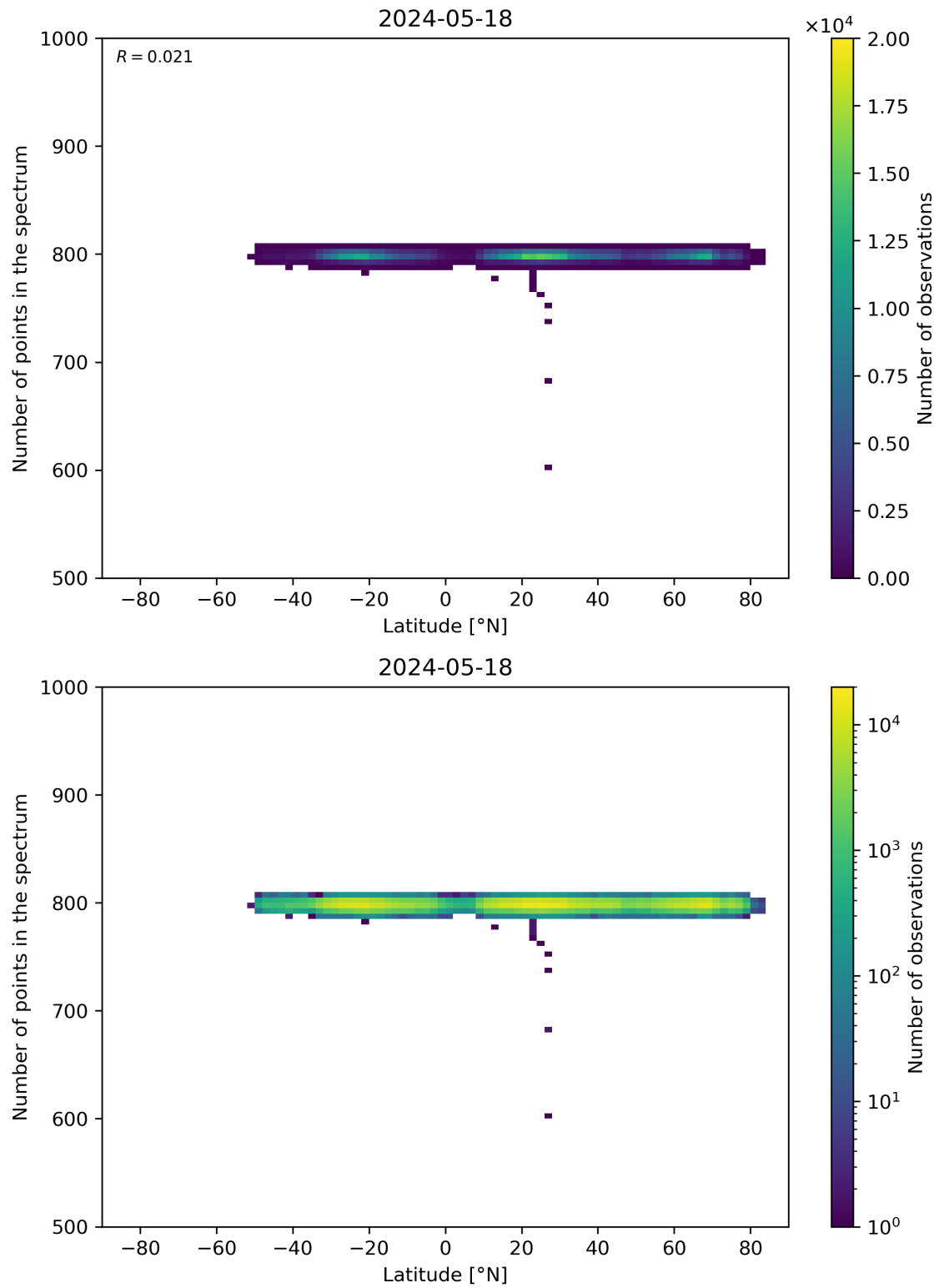
Figure 61: Scatter density plot of “Latitude” against “Number of points in the spectrum” for 2024-05-18 to 2024-05-19.
