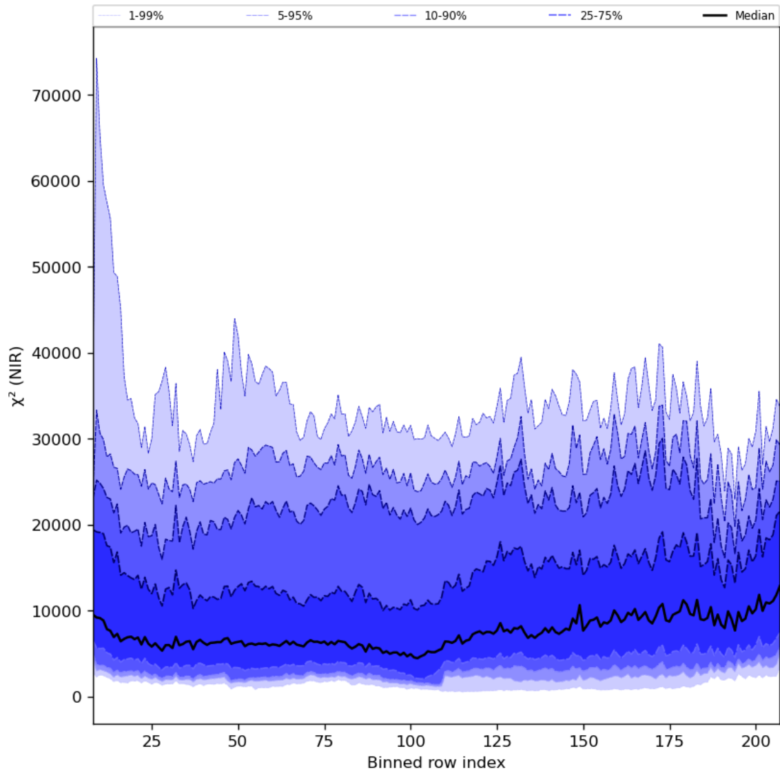
Figure 40: Along track statistics of “ \chi^2 (NIR)” for 2024-05-18 to 2024-05-19
