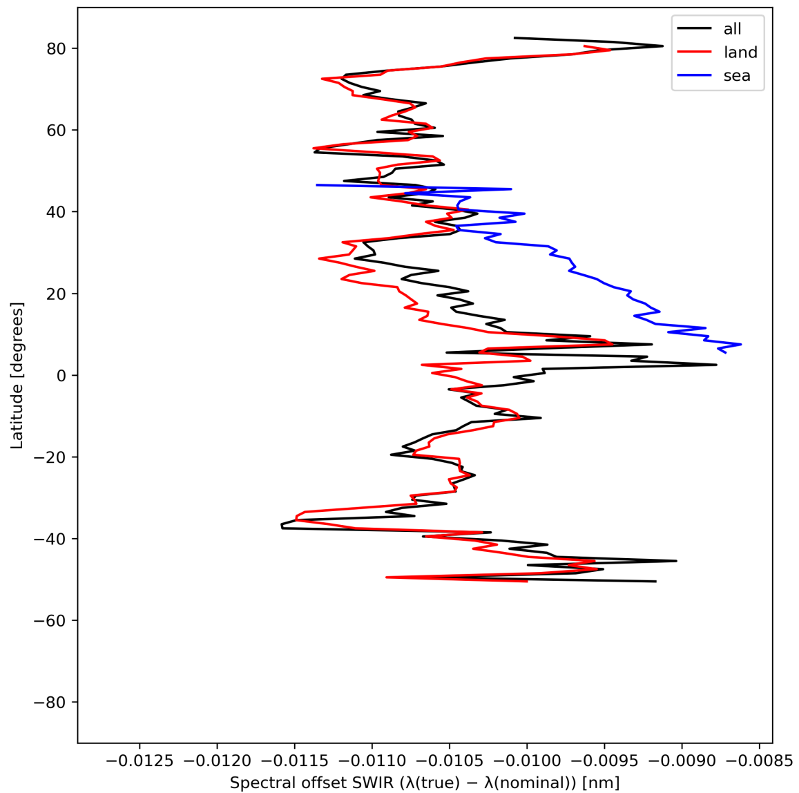
Figure 16: Zonal average of “Spectral offset SWIR ( \lambda(\text{true}) - \lambda(\text{nominal}) )” for 2024-05-18 to 2024-05-19.
