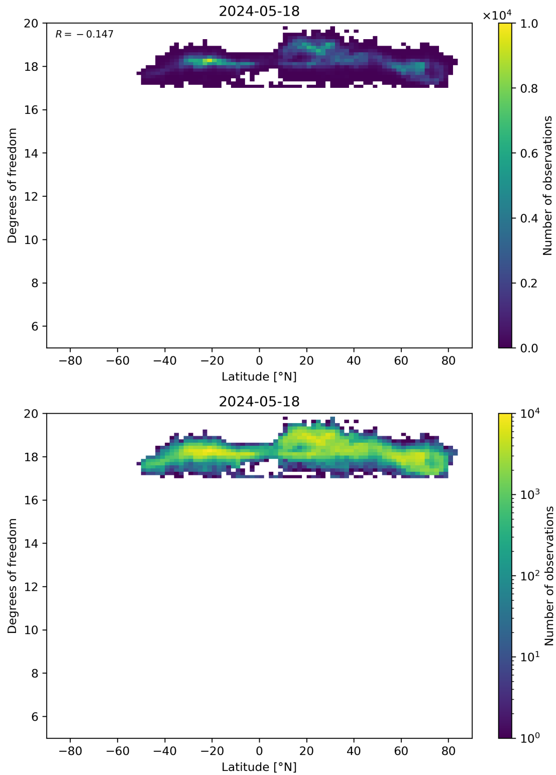
Figure 55: Scatter density plot of “Latitude” against “Degrees of freedom” for 2024-05-18 to 2024-05-19.
