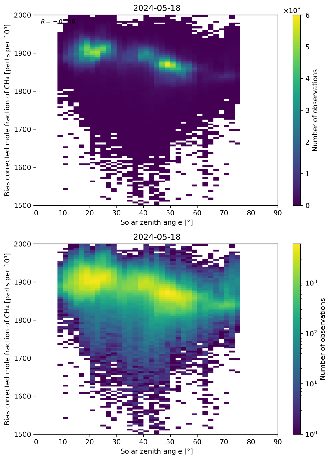
Figure 100: Scatter density plot of “Solar zenith angle” against “Bias corrected mole fraction of CH 4 ” for 2024-05-18 to 2024-05-19.
