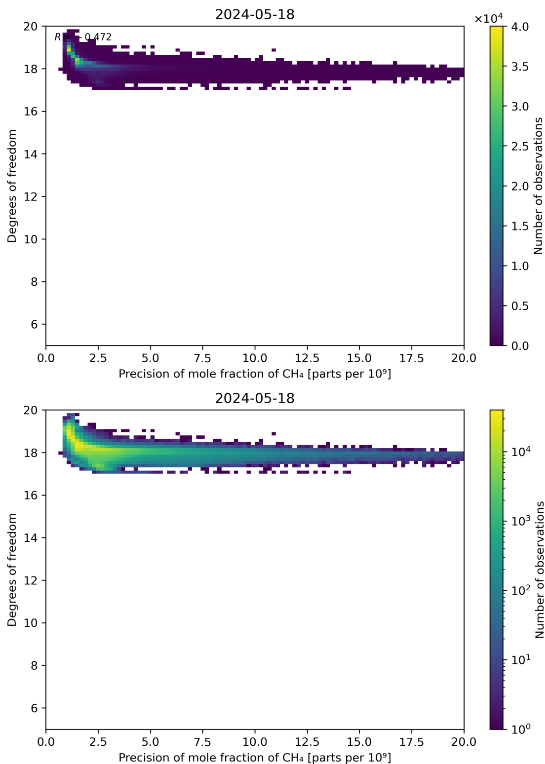
Figure 80: Scatter density plot of “Precision of mole fraction of CH 4 ” against “Degrees of freedom” for 2024-05-18 to 2024-05-19.
