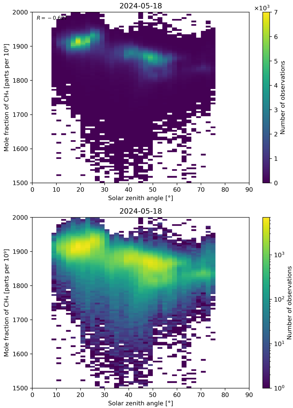
Figure 99: Scatter density plot of “Solar zenith angle” against “Mole fraction of CH 4 ” for 2024-05-18 to 2024-05-19.
