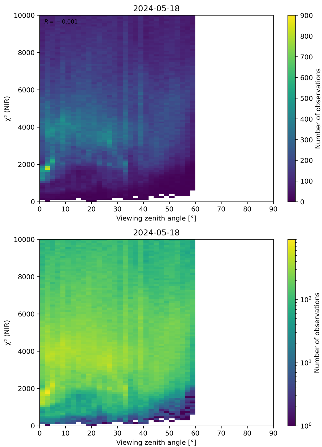
Figure 105: Scatter density plot of “Viewing zenith angle” against “ \chi^2 (NIR)” for 2024-05-18 to 2024-05-19.
