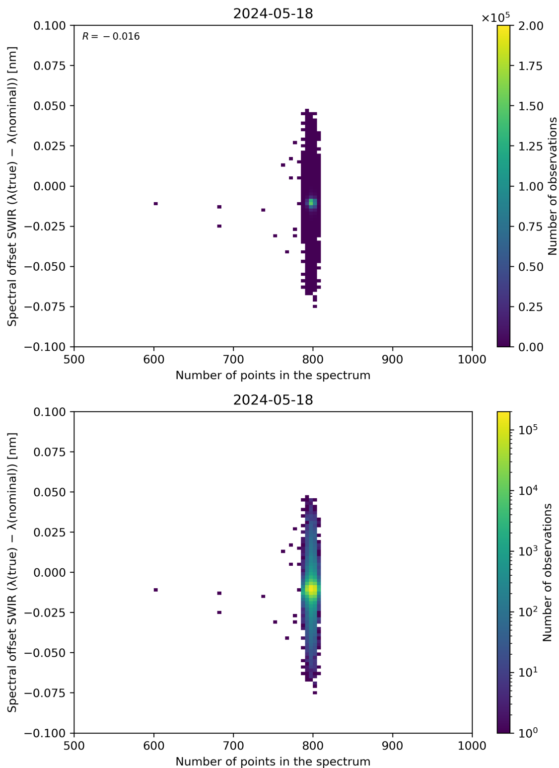
Figure 93: Scatter density plot of “Number of points in the spectrum” against “Spectral offset SWIR ( \lambda(\text{true}) - \lambda(\text{nominal}) )” for 2024-05-18 to 2024-05-19.
