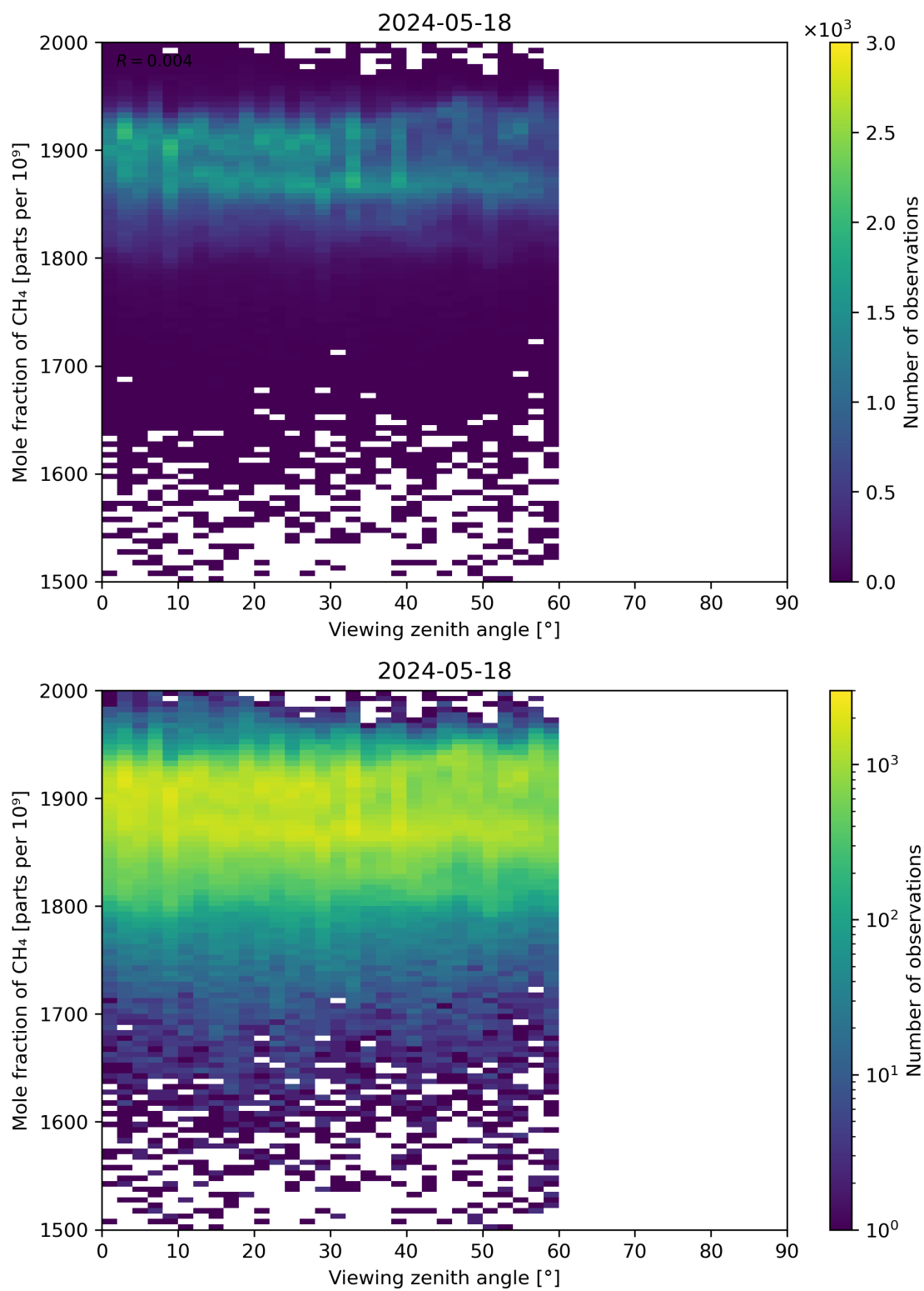
Figure 110: Scatter density plot of “Viewing zenith angle” against “Mole fraction of CH 4 ” for 2024-05-18 to 2024-05-19.
