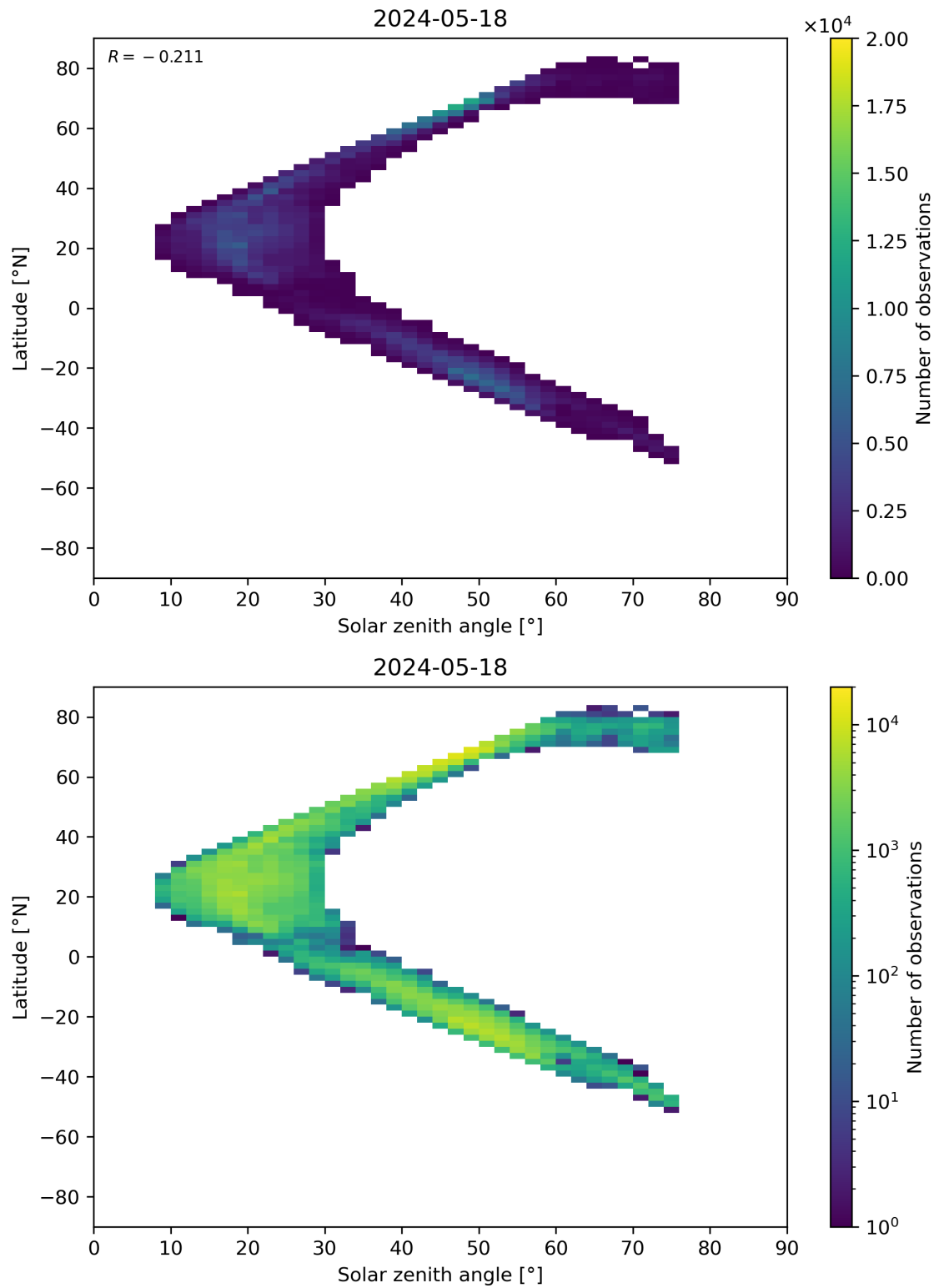
Figure 98: Scatter density plot of “Solar zenith angle” against “Latitude” for 2024-05-18 to 2024-05-19.
