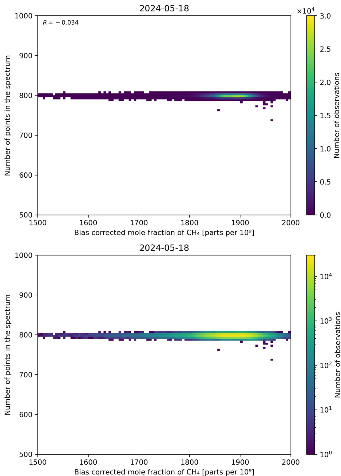
Figure 68: Scatter density plot of “Bias corrected mole fraction of CH 4 ” against “Number of points in the spectrum” for 2024-05-18 to 2024-05-19.
