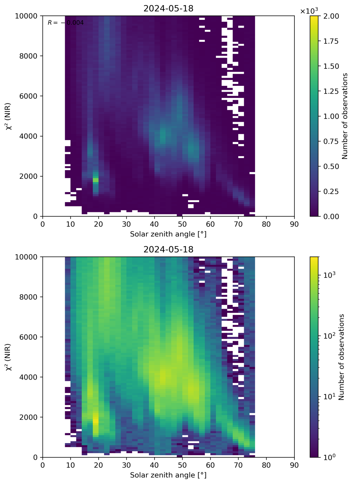
Figure 94: Scatter density plot of “Solar zenith angle” against “ \chi^2 (NIR)” for 2024-05-18 to 2024-05-19.
