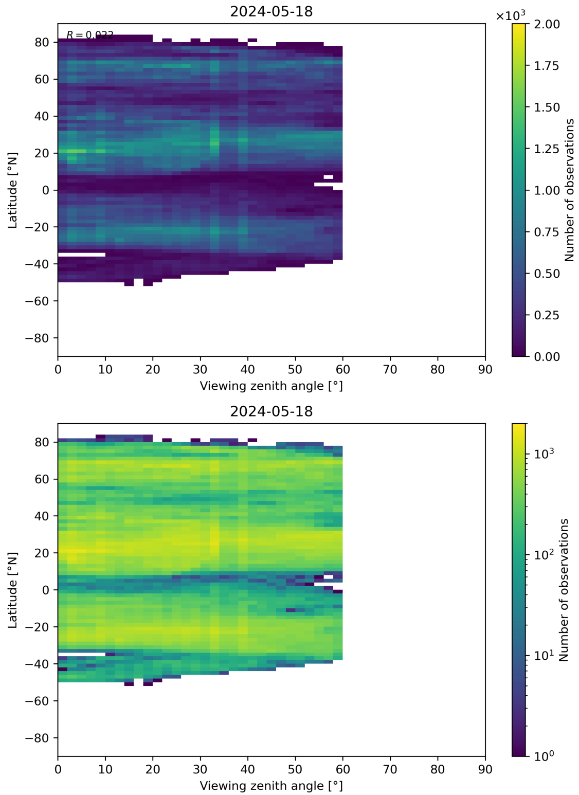
Figure 109: Scatter density plot of “Viewing zenith angle” against “Latitude” for 2024-05-18 to 2024-05-19.
