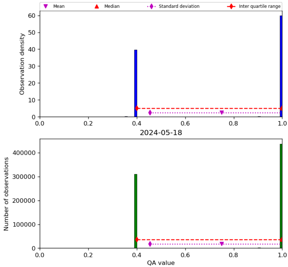
Figure 22: Histogram of “QA value” for 2024-05-18 to 2024-05-19
