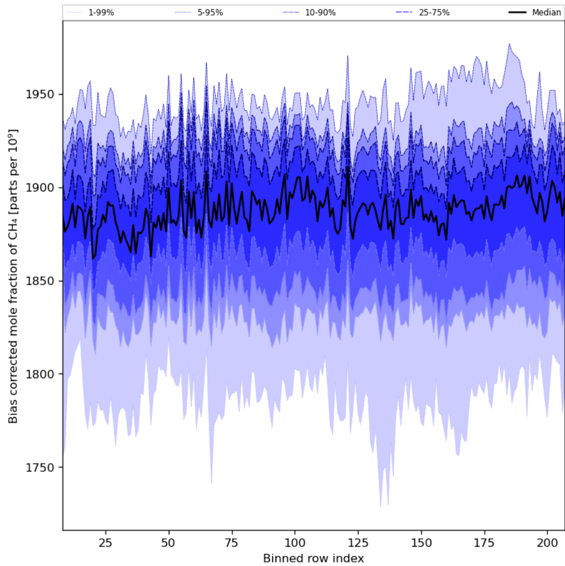
Figure 36: Along track statistics of “Bias corrected mole fraction of CH 4 ” for 2024-05-18 to 2024-05-19
