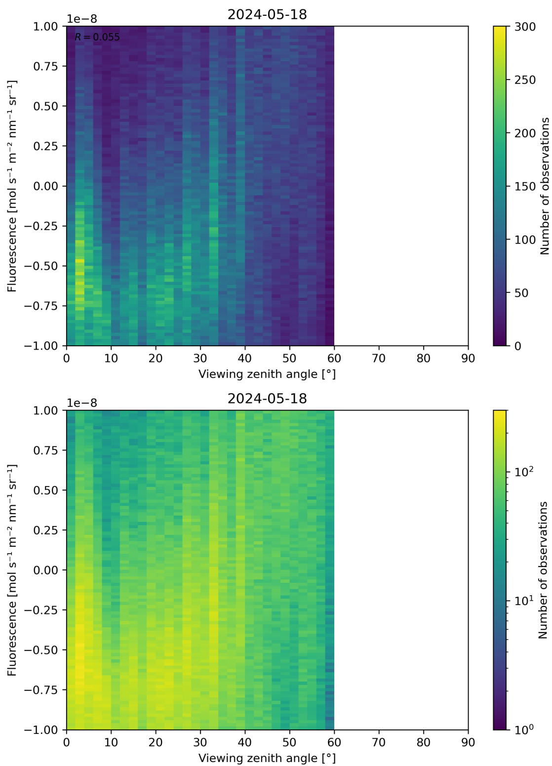
Figure 108: Scatter density plot of “Viewing zenith angle” against “Fluorescence” for 2024-05-18 to 2024-05-19.
