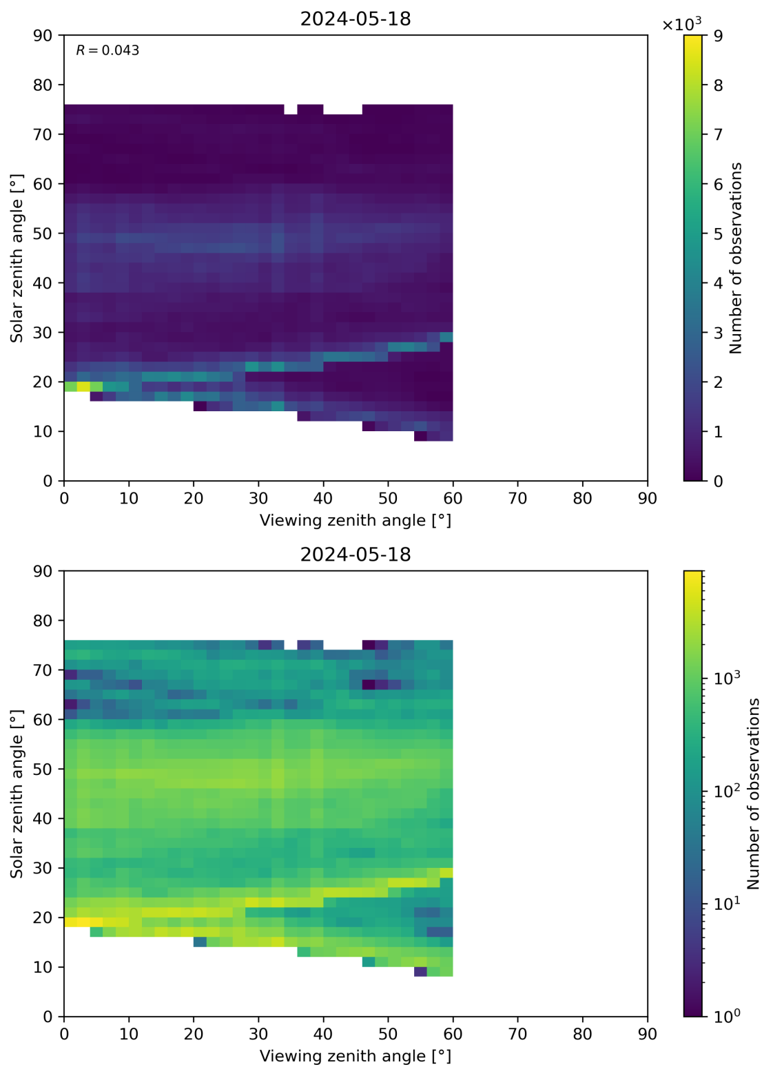
Figure 115: Scatter density plot of “Viewing zenith angle” against “Solar zenith angle” for 2024-05-18 to 2024-05-19.
