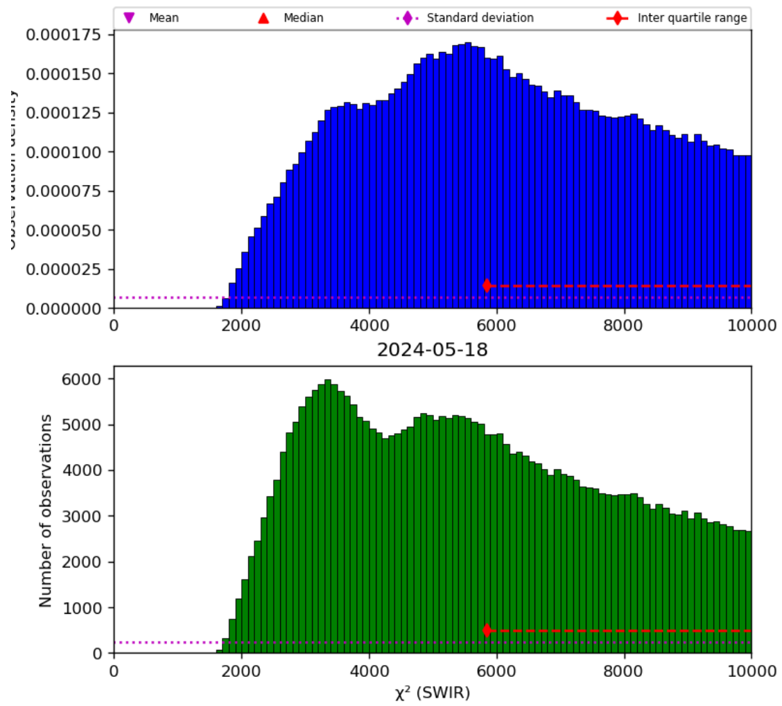
Figure 28: Histogram of “ \chi^2 (SWIR)” for 2024-05-18 to 2024-05-19
