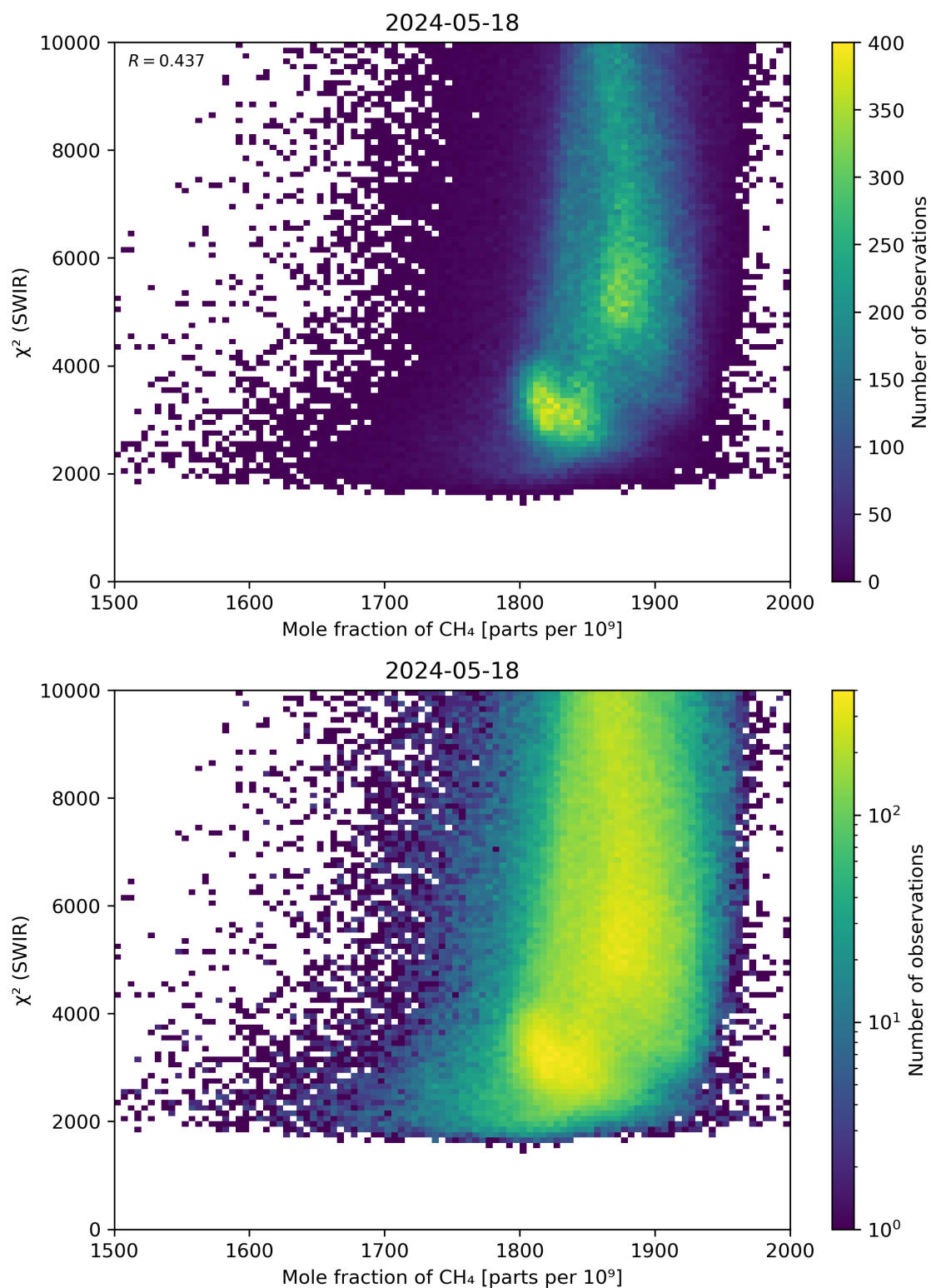
Figure 71: Scatter density plot of “Mole fraction of \text{CH}_4 ” against “ \chi^2 (SWIR)” for 2024-05-18 to 2024-05-19.
