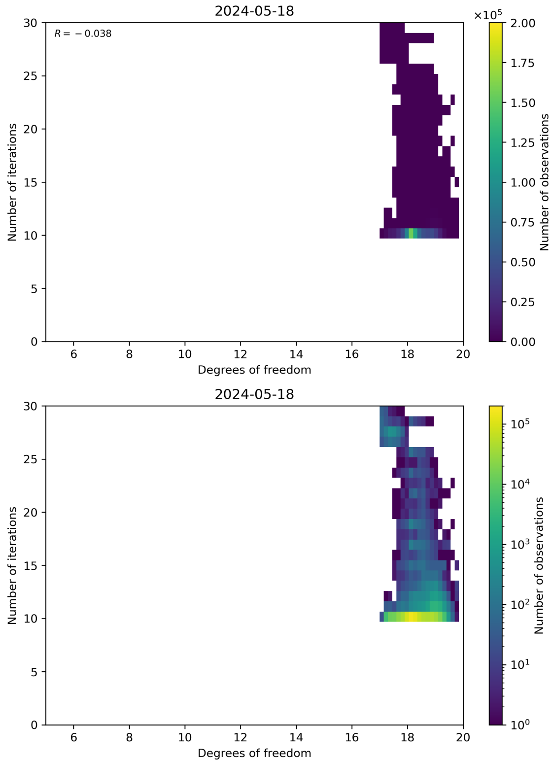
Figure 52: Scatter density plot of “Degrees of freedom” against “Number of iterations” for 2024-05-18 to 2024-05-19.
