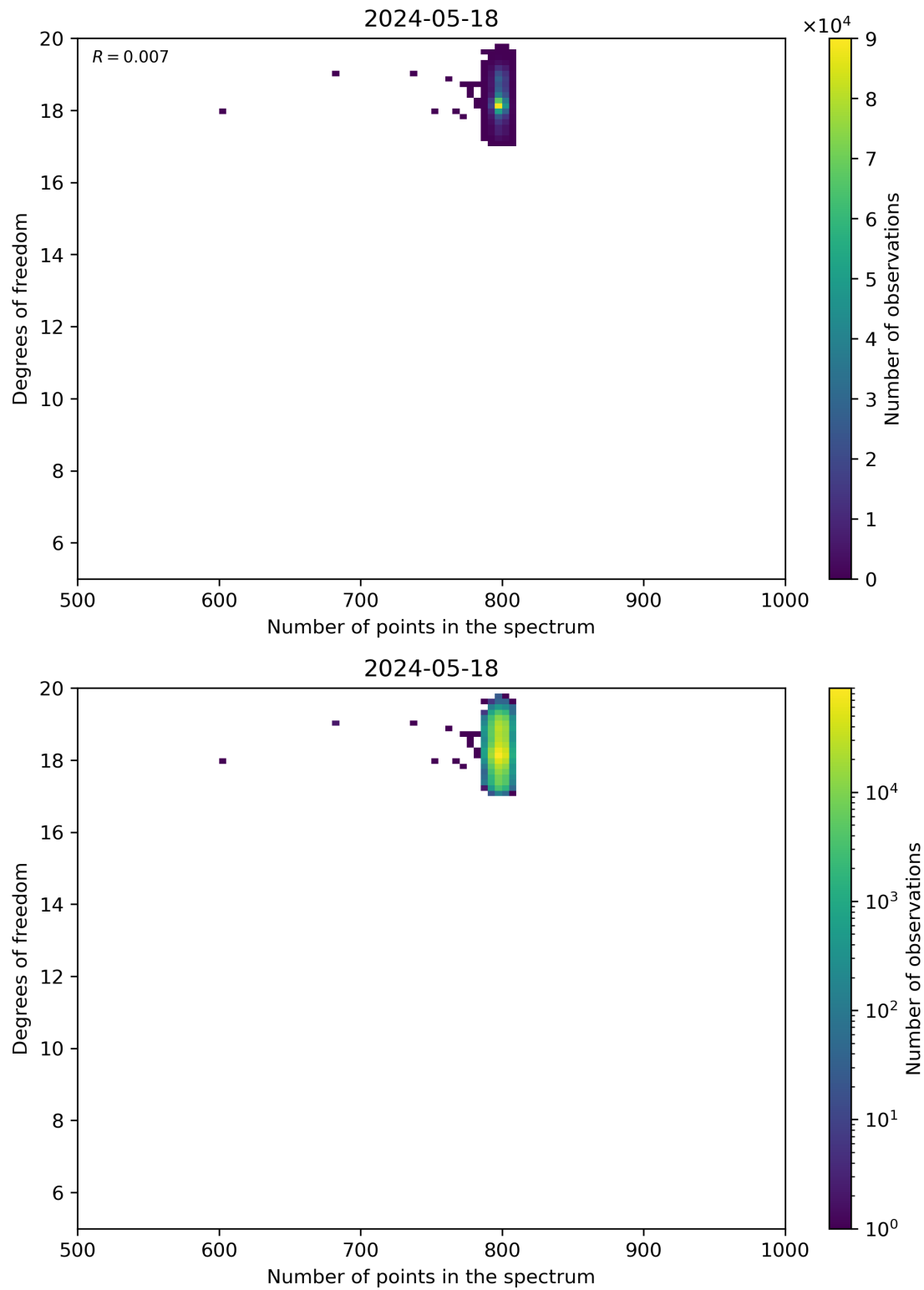
Figure 90: Scatter density plot of “Number of points in the spectrum” against “Degrees of freedom” for 2024-05-18 to 2024-05-19.
