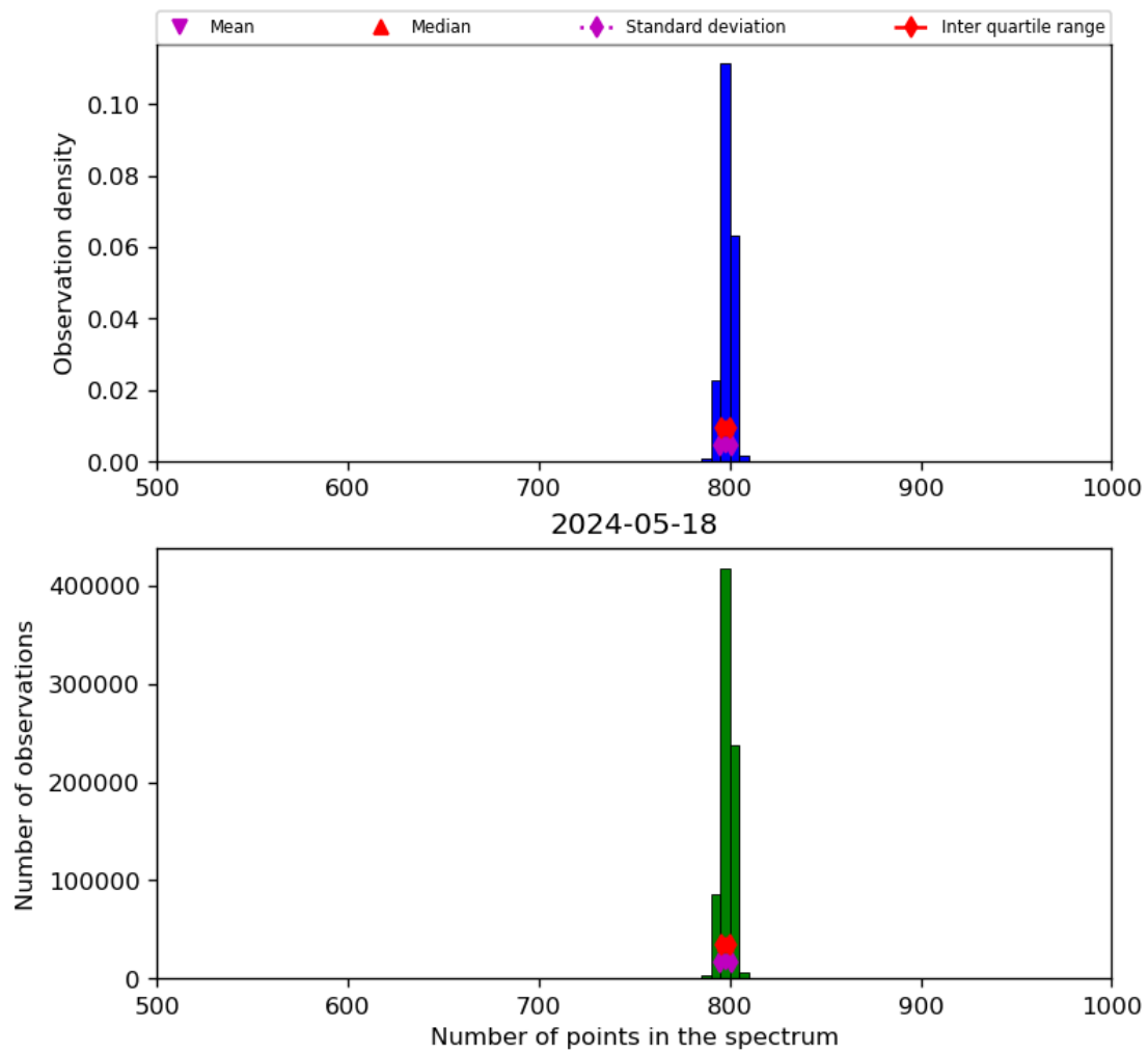
Figure 26: Histogram of “Number of points in the spectrum” for 2024-05-18 to 2024-05-19
