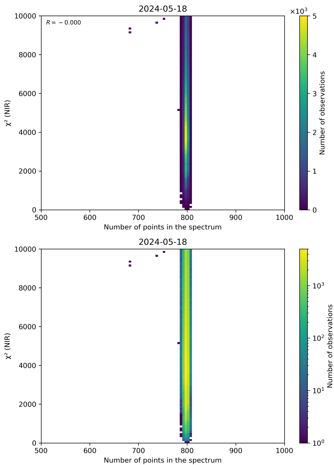
Figure 88: Scatter density plot of “Number of points in the spectrum” against “ \chi^2 (NIR)” for 2024-05-18 to 2024-05-19.
