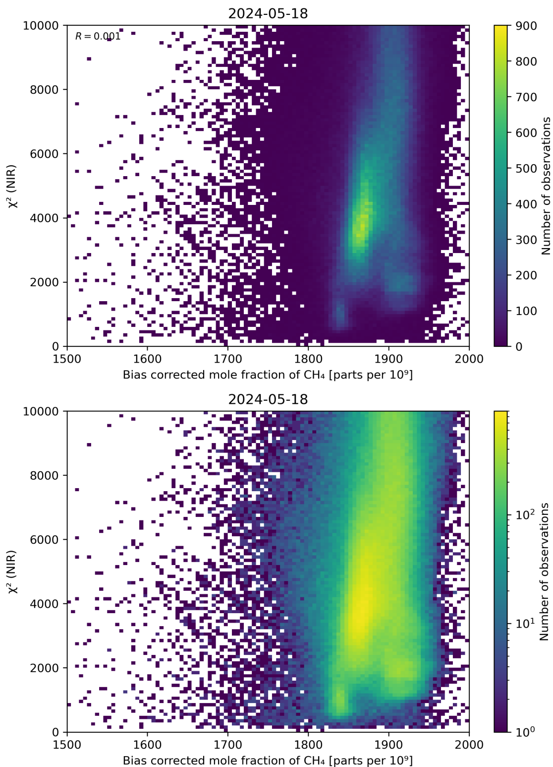
Figure 63: Scatter density plot of “Bias corrected mole fraction of CH 4 ” against “ \chi^2 (NIR)” for 2024-05-18 to 2024-05-19.
