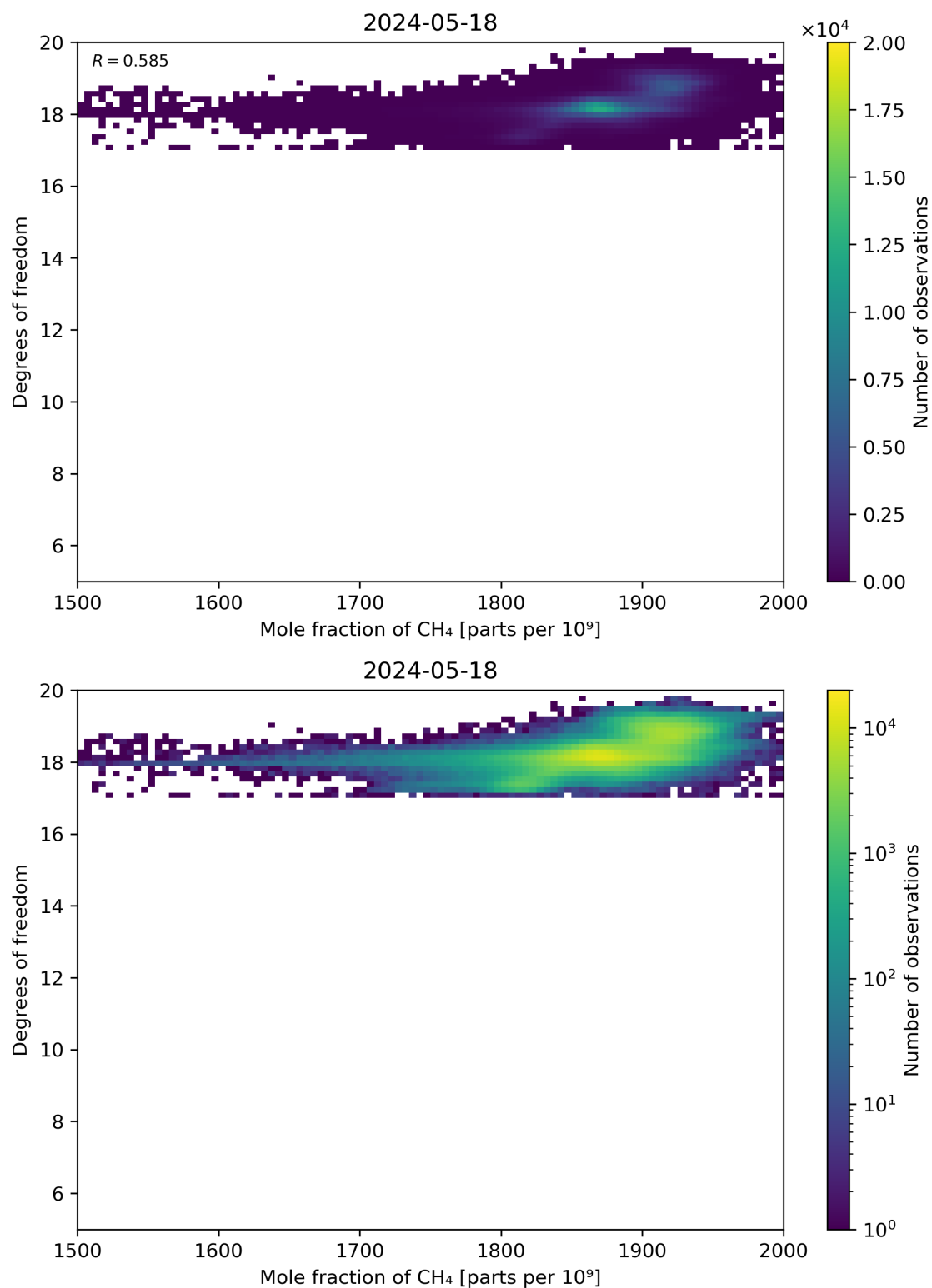
Figure 72: Scatter density plot of “Mole fraction of CH 4 ” against “Degrees of freedom” for 2024-05-18 to 2024-05-19.
