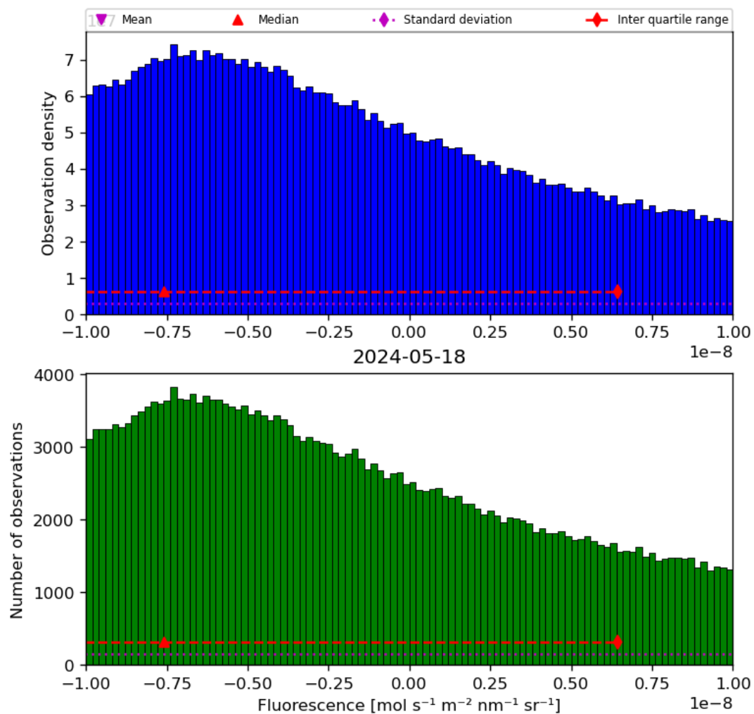
Figure 32: Histogram of “Fluorescence” for 2024-05-18 to 2024-05-19
