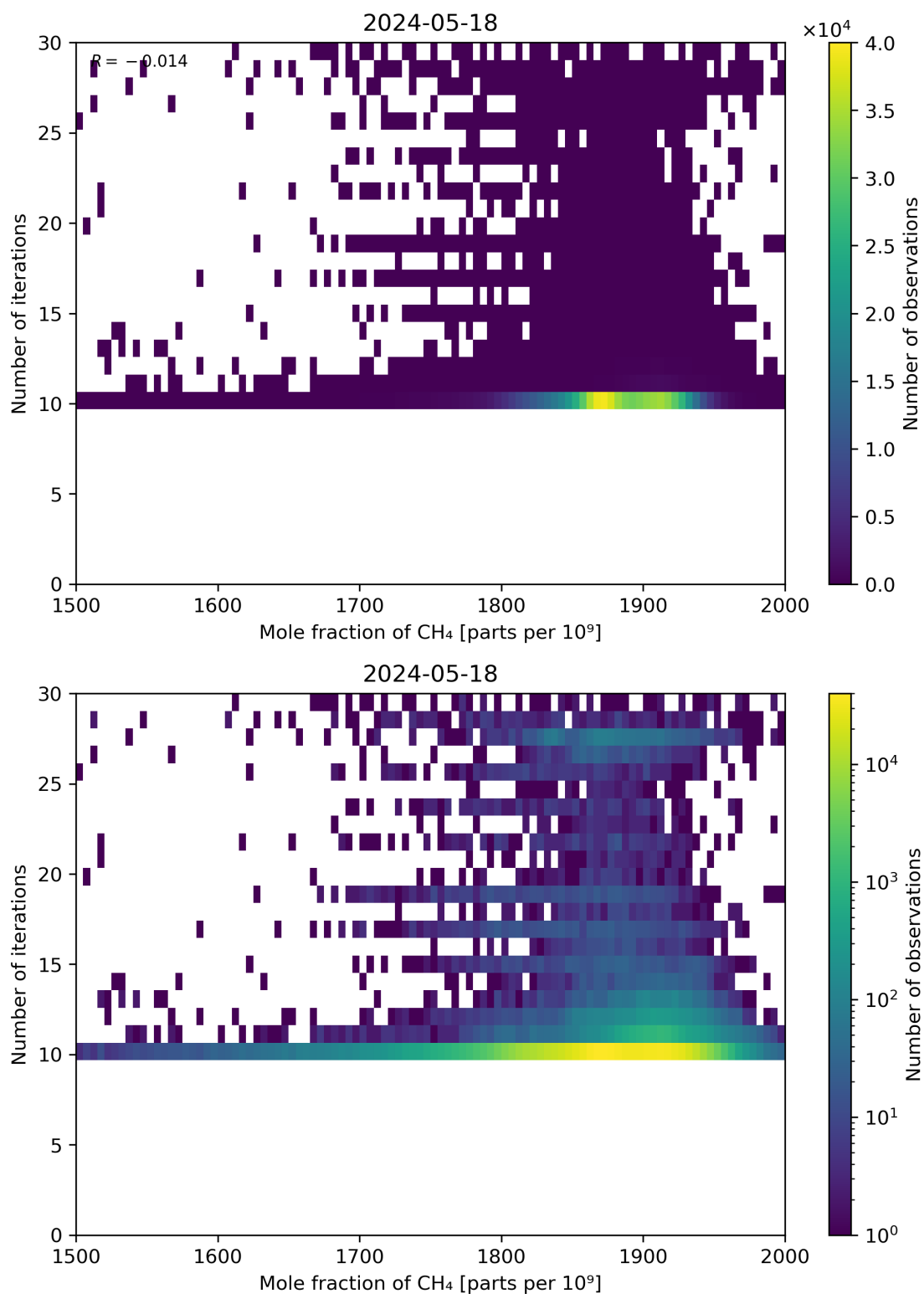
Figure 76: Scatter density plot of “Mole fraction of CH 4 ” against “Number of iterations” for 2024-05-18 to 2024-05-19.
