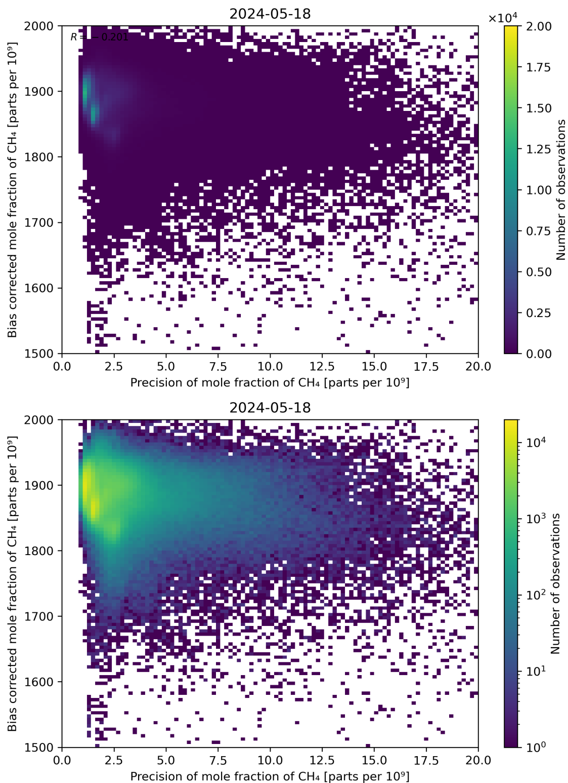
Figure 82: Scatter density plot of “Precision of mole fraction of CH 4 ” against “Bias corrected mole fraction of CH 4 ” for 2024-05-18 to 2024-05-19.
