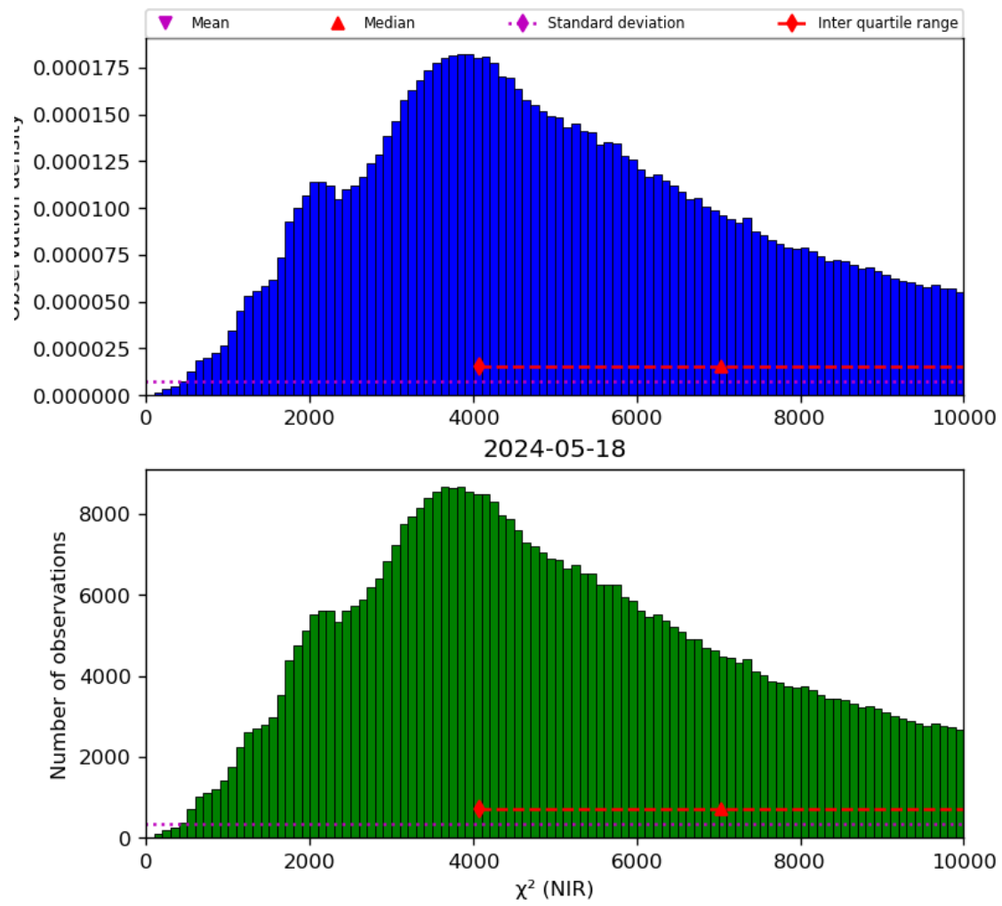
Figure 29: Histogram of “ \chi^2 (NIR)” for 2024-05-18 to 2024-05-19
