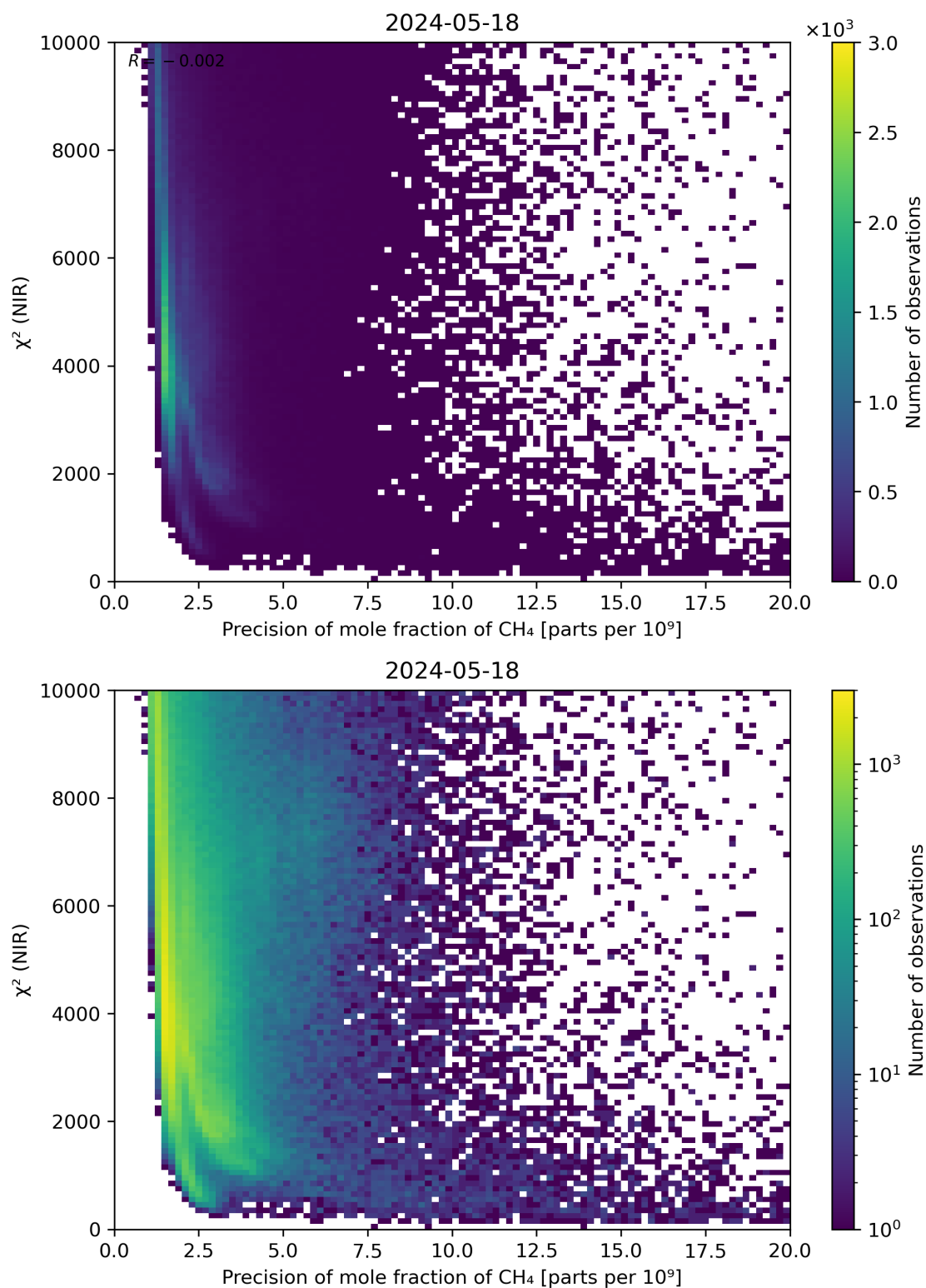
Figure 78: Scatter density plot of “Precision of mole fraction of CH 4 ” against “ \chi^2 (NIR)” for 2024-05-18 to 2024-05-19.
