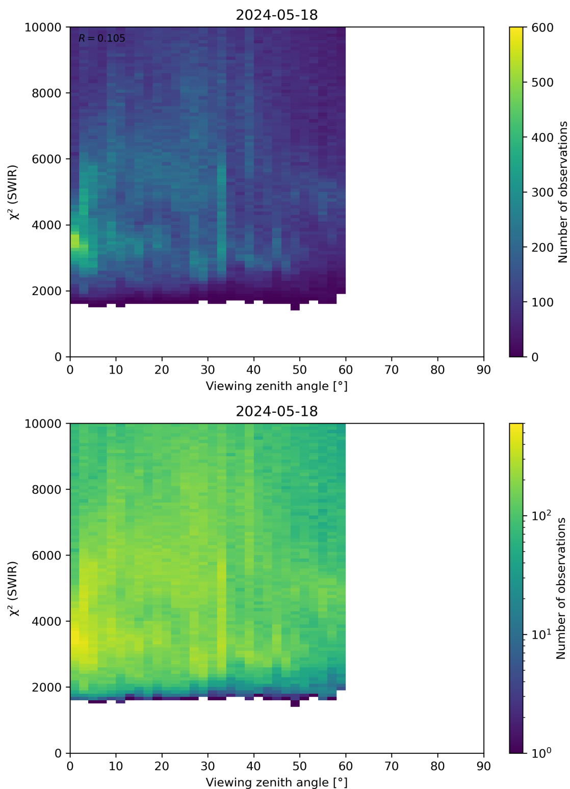
Figure 106: Scatter density plot of “Viewing zenith angle” against “ \chi^2 (SWIR)” for 2024-05-18 to 2024-05-19.
