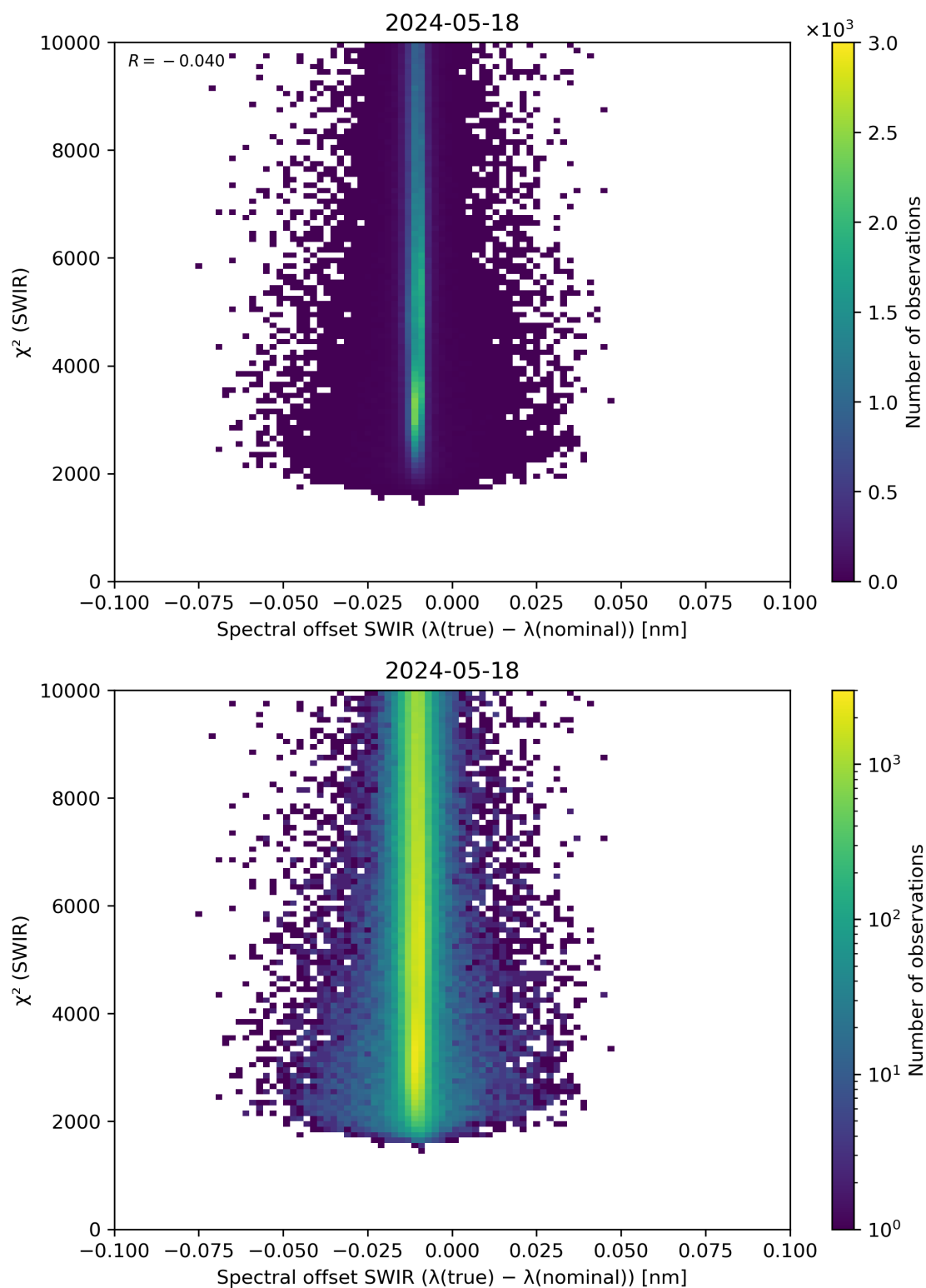
Figure 118: Scatter density plot of “Spectral offset SWIR ( \lambda(\text{true}) - \lambda(\text{nominal}) )” against “ \chi^2 (SWIR)” for 2024-05-18 to 2024-05-19.
