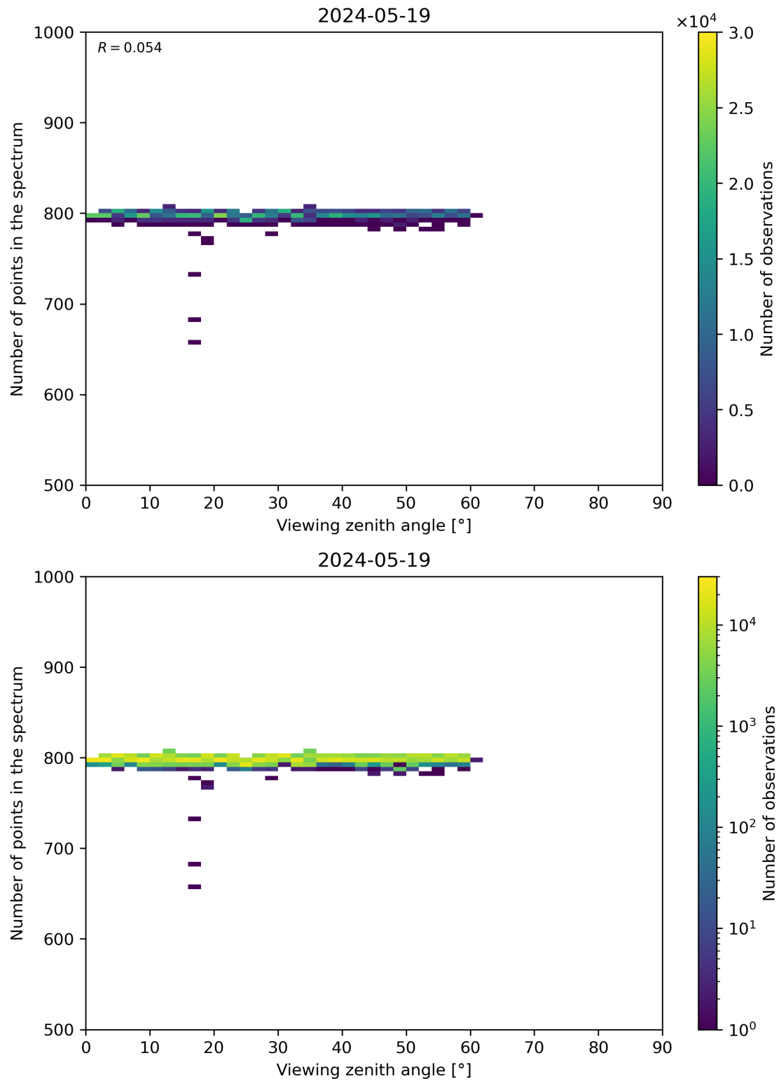
Figure 114: Scatter density plot of “Viewing zenith angle” against “Number of points in the spectrum” for 2024-05-18 to 2024-05-20.
