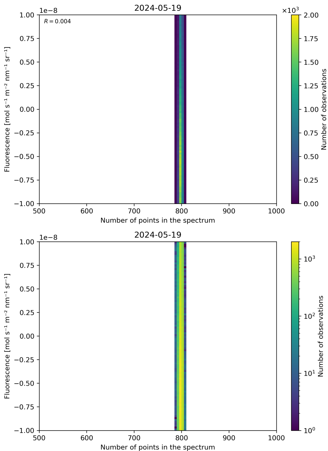
Figure 91: Scatter density plot of “Number of points in the spectrum” against “Fluorescence” for 2024-05-18 to 2024-05-20.
