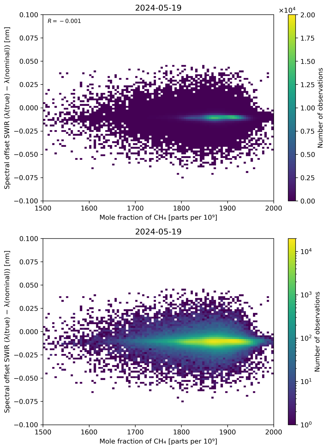
Figure 86: Scatter density plot of “Mole fraction of CH 4 ” against “Spectral offset SWIR ( \lambda(\text{true}) - \lambda(\text{nominal}) )” for 2024-05-18 to 2024-05-20.
