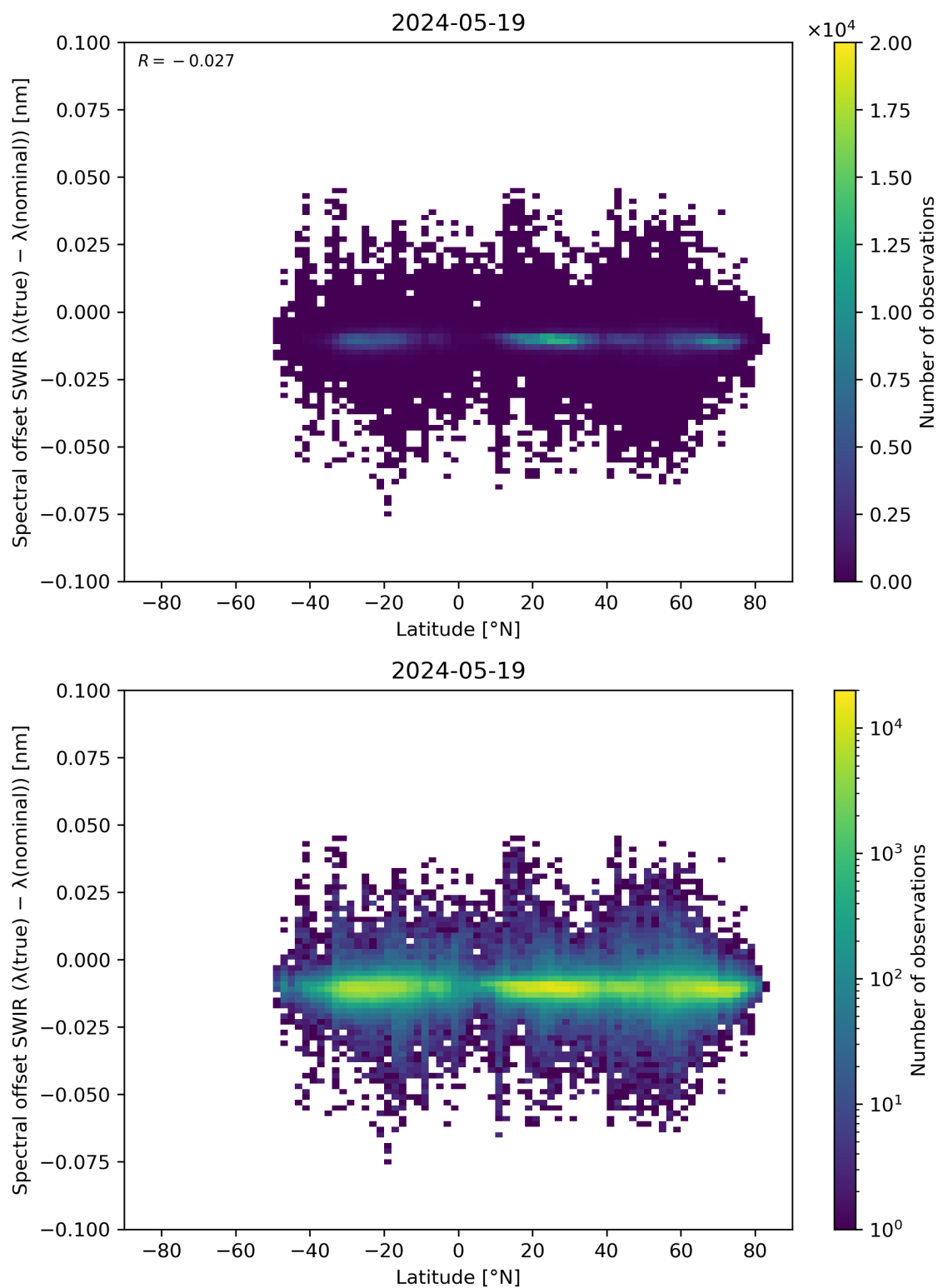
Figure 62: Scatter density plot of “Latitude” against “Spectral offset SWIR ( \lambda(\text{true}) - \lambda(\text{nominal}) )” for 2024-05-18 to 2024-05-20.
