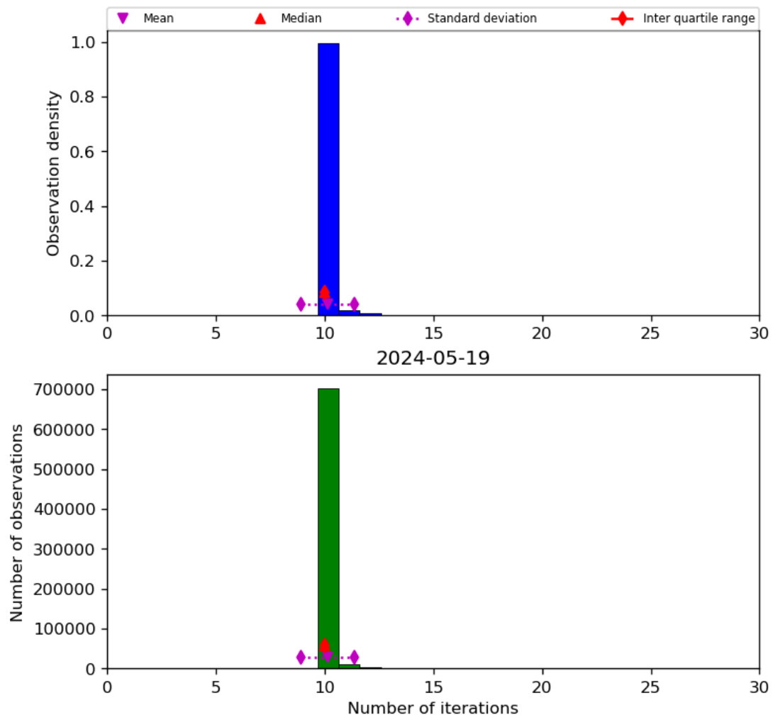
Figure 31: Histogram of “Number of iterations” for 2024-05-18 to 2024-05-20
