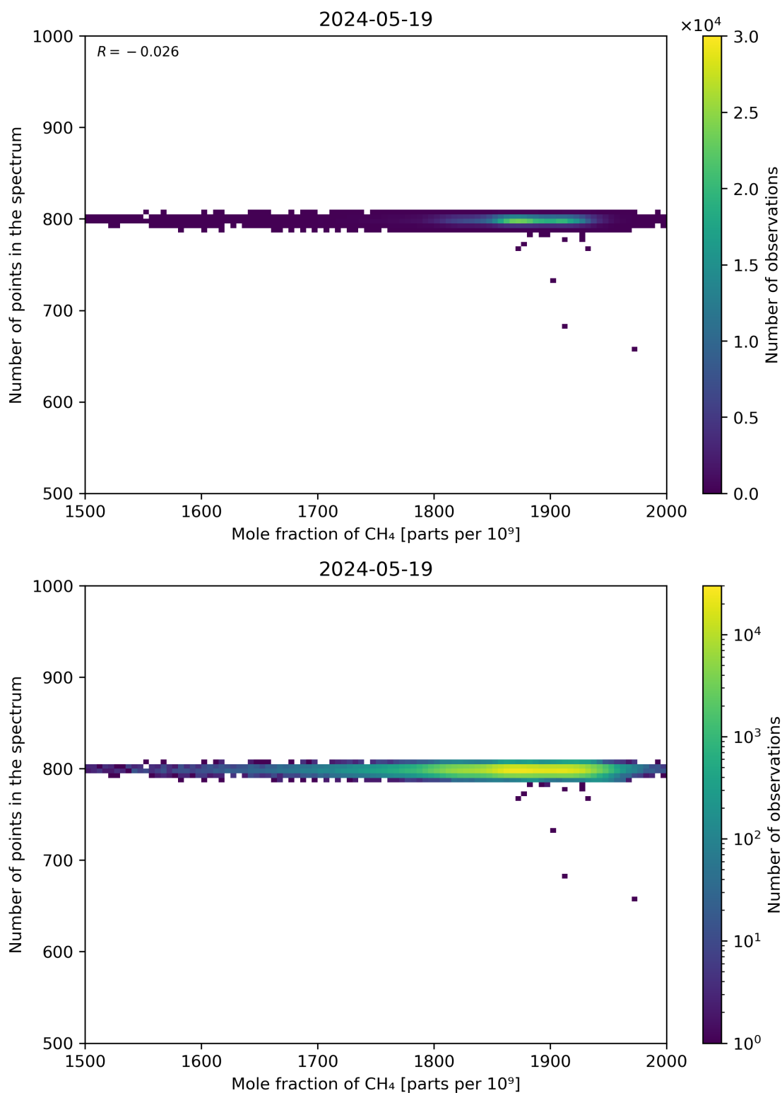
Figure 77: Scatter density plot of “Mole fraction of CH 4 ” against “Number of points in the spectrum” for 2024-05-18 to 2024-05-20.
