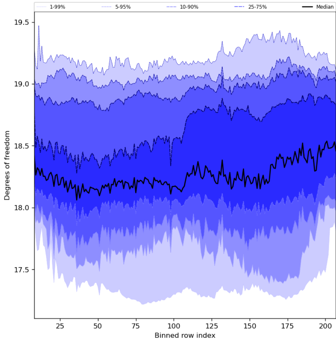
Figure 41: Along track statistics of “Degrees of freedom” for 2024-05-18 to 2024-05-20
