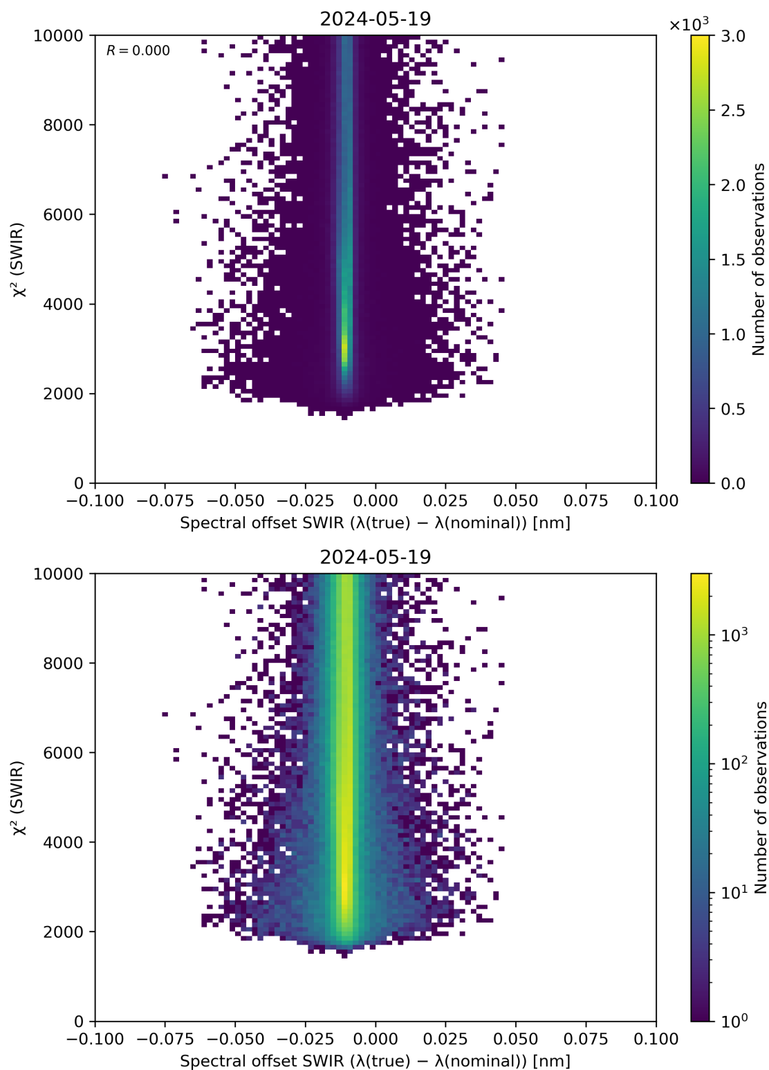
Figure 118: Scatter density plot of “Spectral offset SWIR ( \lambda(\text{true}) - \lambda(\text{nominal}) )” against “ \chi^2 (SWIR)” for 2024-05-18 to 2024-05-20.
