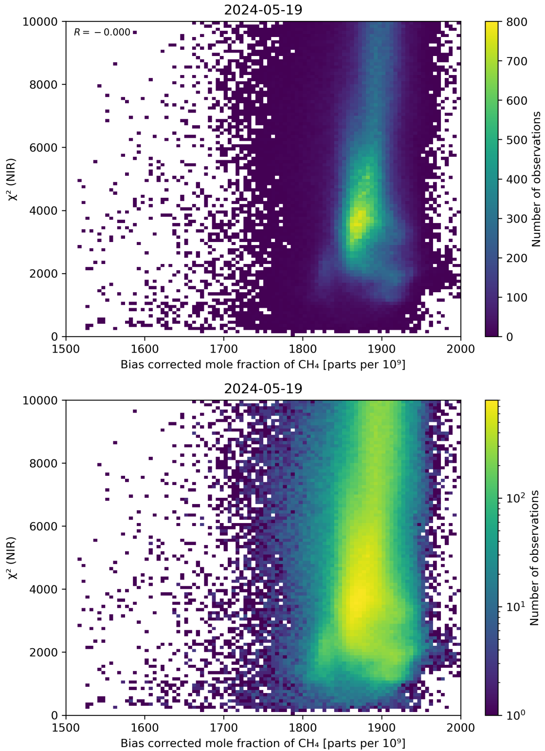
Figure 63: Scatter density plot of “Bias corrected mole fraction of \text{CH}_4 ” against “ \chi^2 (NIR)” for 2024-05-18 to 2024-05-20.
