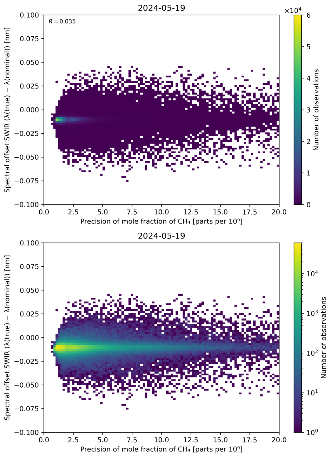
Figure 85: Scatter density plot of “Precision of mole fraction of CH 4 ” against “Spectral offset SWIR ( \lambda(\text{true}) - \lambda(\text{nominal}) )” for 2024-05-18 to 2024-05-20.
