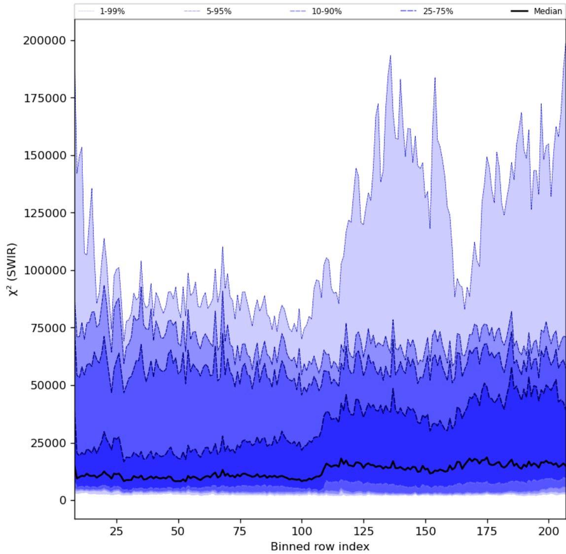
Figure 39: Along track statistics of “ \chi^2 (SWIR)” for 2024-05-18 to 2024-05-20
