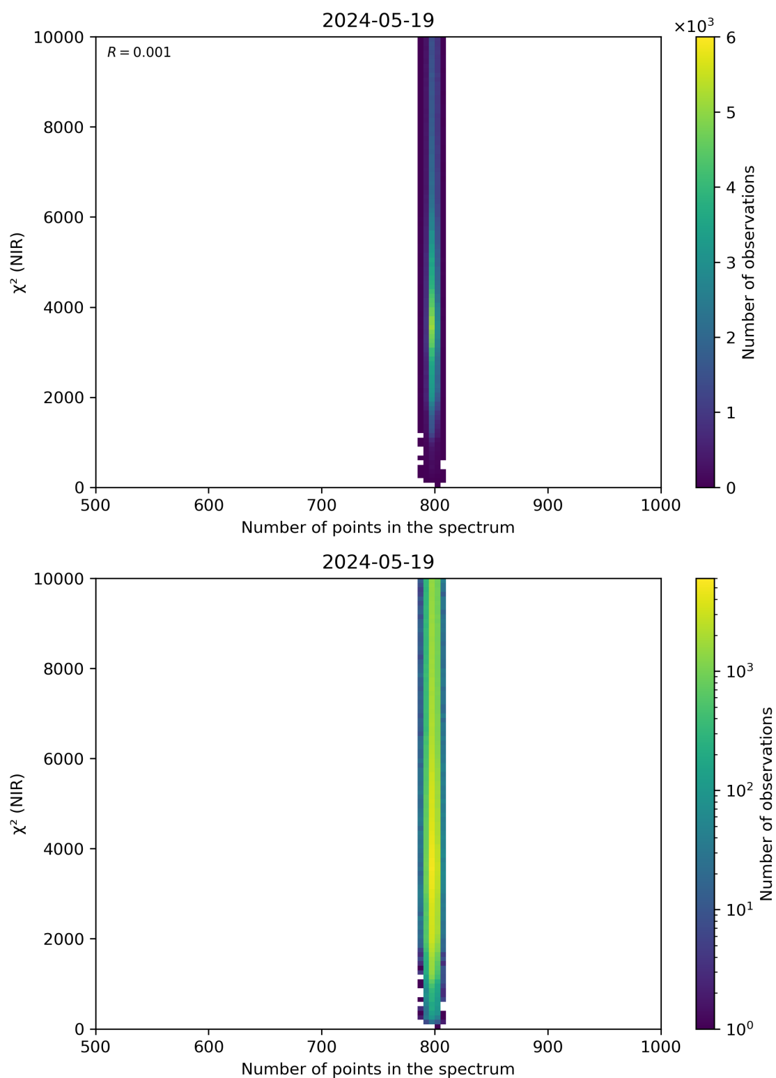
Figure 88: Scatter density plot of “Number of points in the spectrum” against “ \chi^2 (NIR)” for 2024-05-18 to 2024-05-20.
