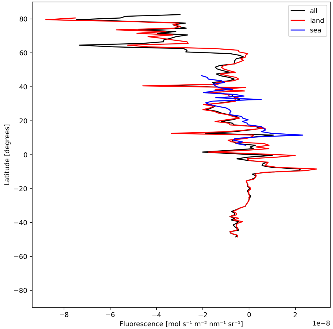
Figure 21: Zonal average of “Fluorescence” for 2024-05-18 to 2024-05-20.
