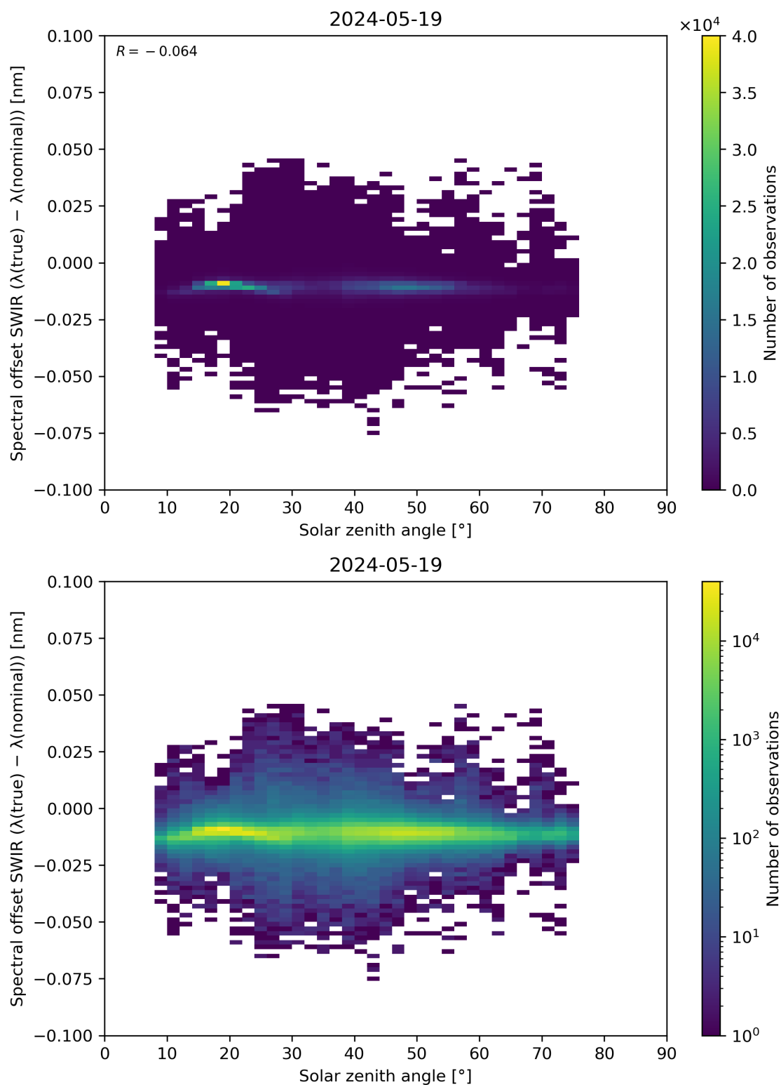
Figure 104: Scatter density plot of “Solar zenith angle” against “Spectral offset SWIR ( \lambda(\text{true}) - \lambda(\text{nominal}) )” for 2024-05-18 to 2024-05-20.
