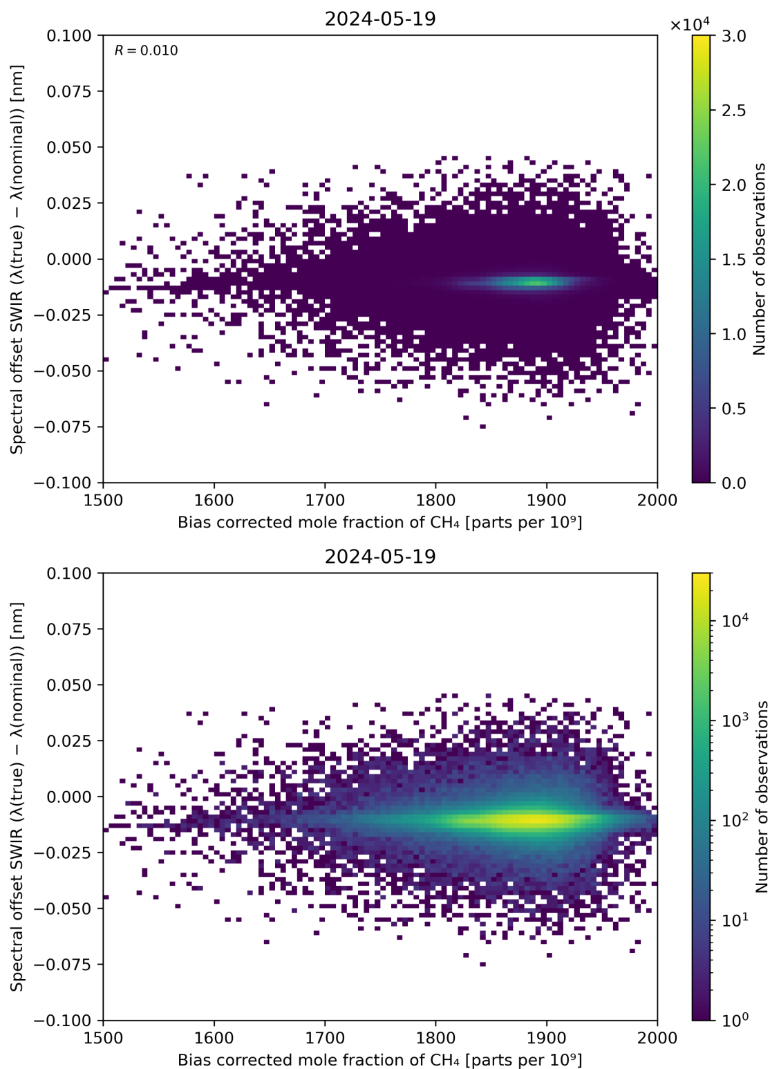
Figure 69: Scatter density plot of “Bias corrected mole fraction of \text{CH}_4 ” against “Spectral offset SWIR ( \lambda(\text{true}) - \lambda(\text{nominal}) )” for 2024-05-18 to 2024-05-20.
