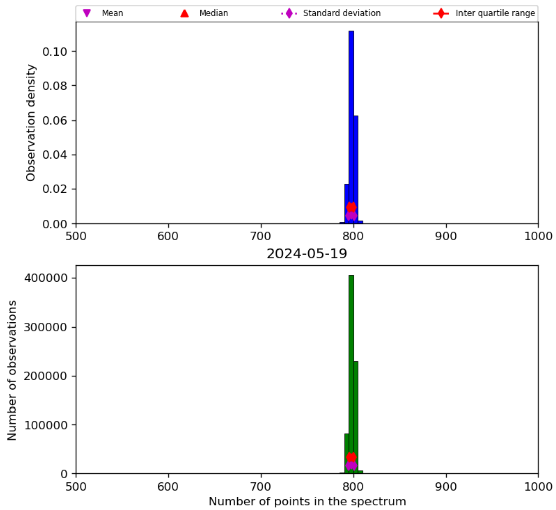
Figure 26: Histogram of “Number of points in the spectrum” for 2024-05-18 to 2024-05-20
