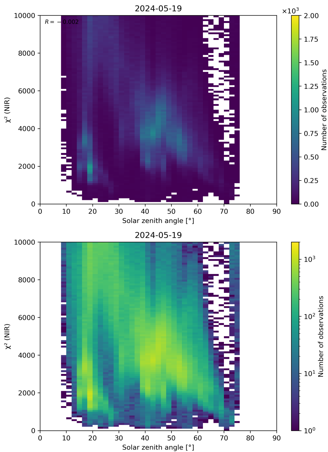
Figure 94: Scatter density plot of “Solar zenith angle” against “ \chi^2 (NIR)” for 2024-05-18 to 2024-05-20.
