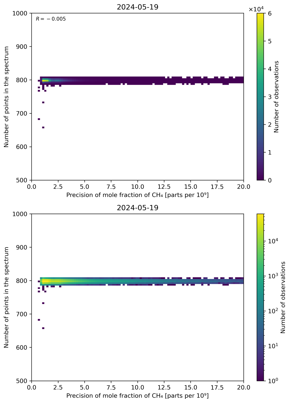
Figure 84: Scatter density plot of “Precision of mole fraction of CH 4 ” against “Number of points in the spectrum” for 2024-05-18 to 2024-05-20.
