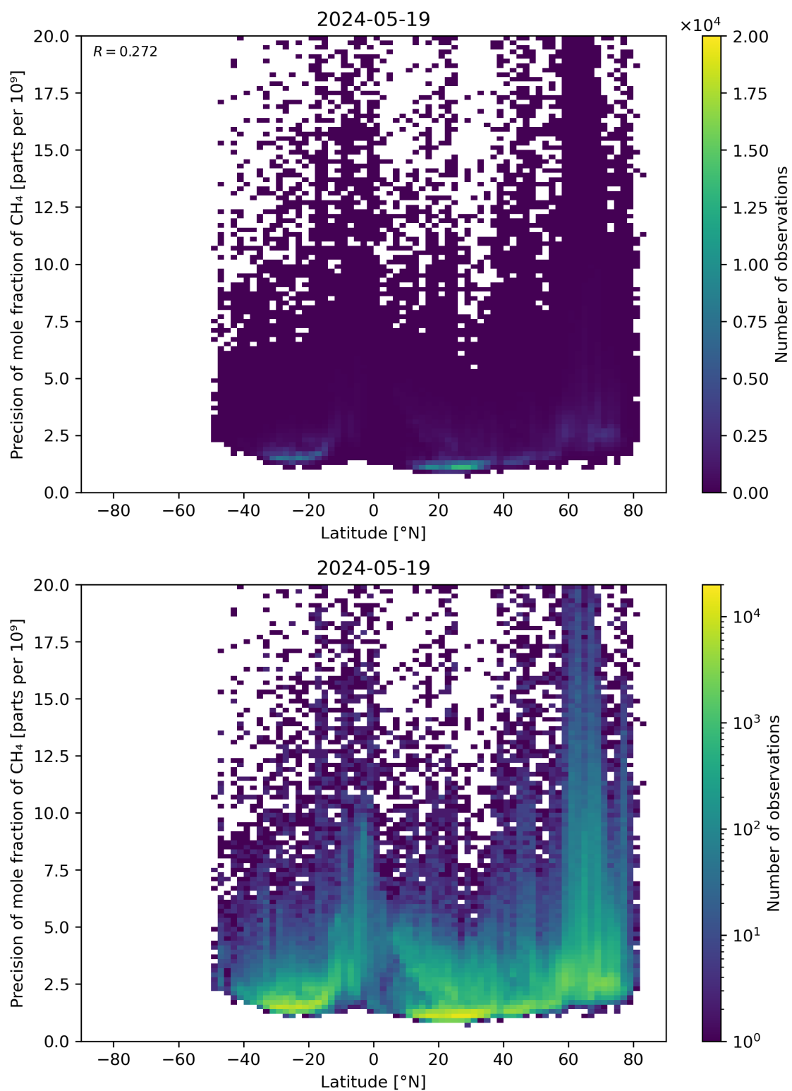
Figure 59: Scatter density plot of “Latitude” against “Precision of mole fraction of \text{CH}_4 ” for 2024-05-18 to 2024-05-20.
