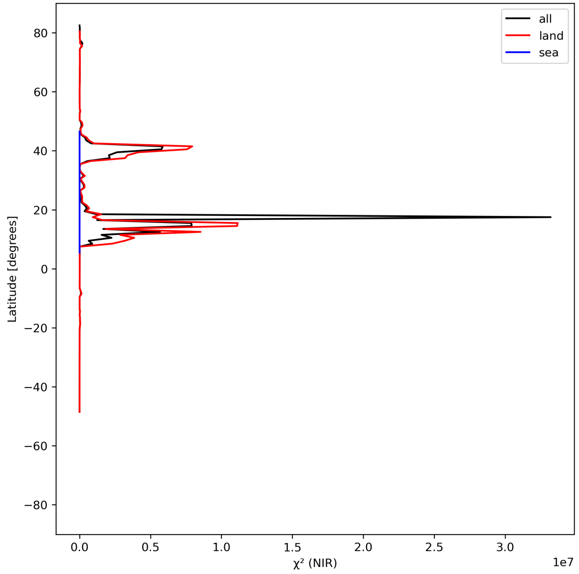
Figure 18: Zonal average of “ \chi^2 (NIR)” for 2024-05-18 to 2024-05-20.
