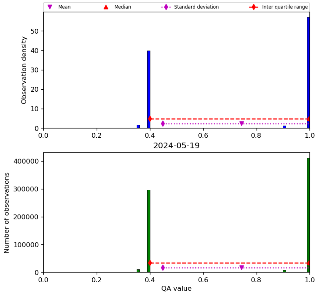
Figure 22: Histogram of “QA value” for 2024-05-18 to 2024-05-20
