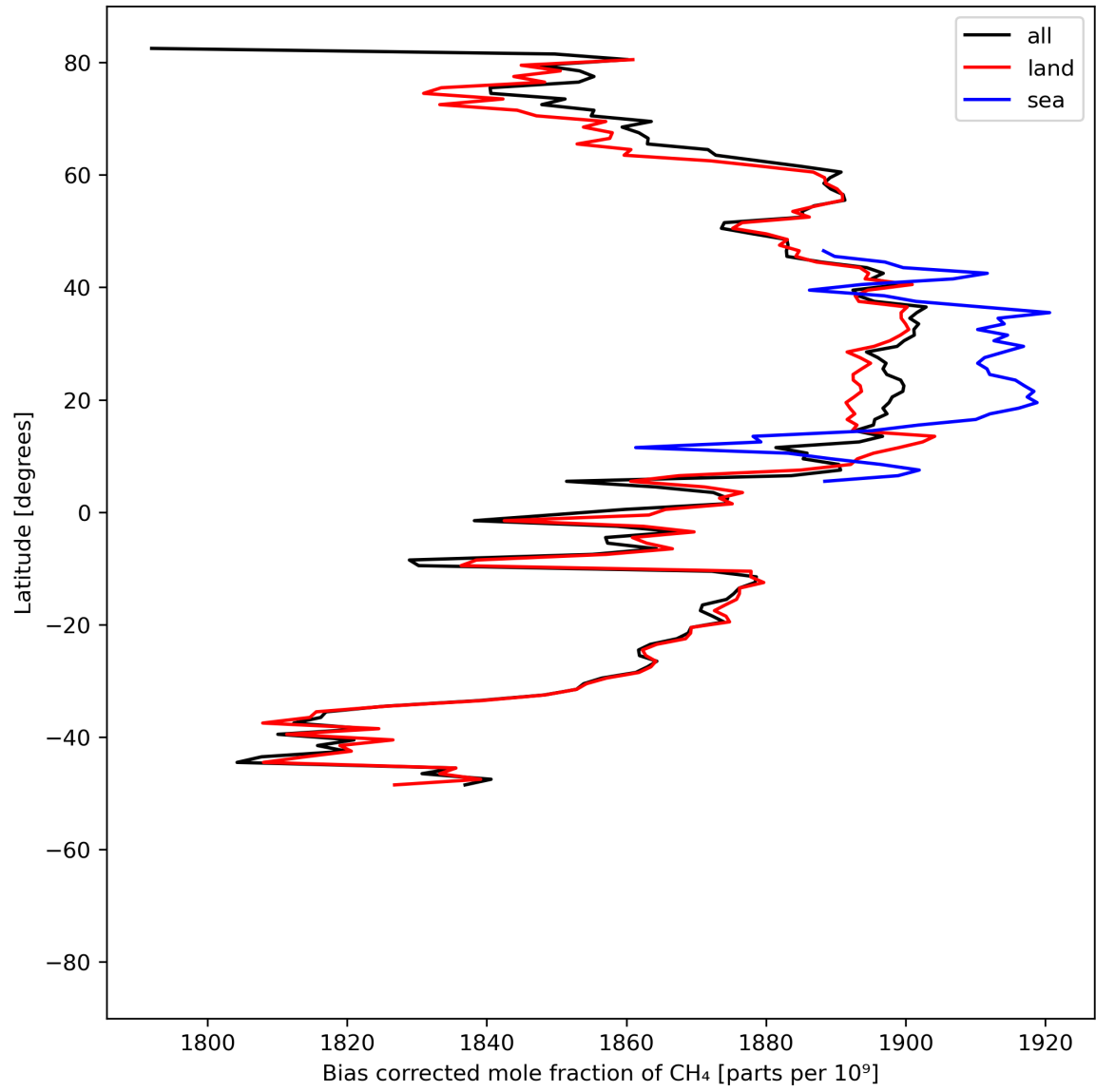
Figure 14: Zonal average of “Bias corrected mole fraction of \text{CH}_4 ” for 2024-05-18 to 2024-05-20.
