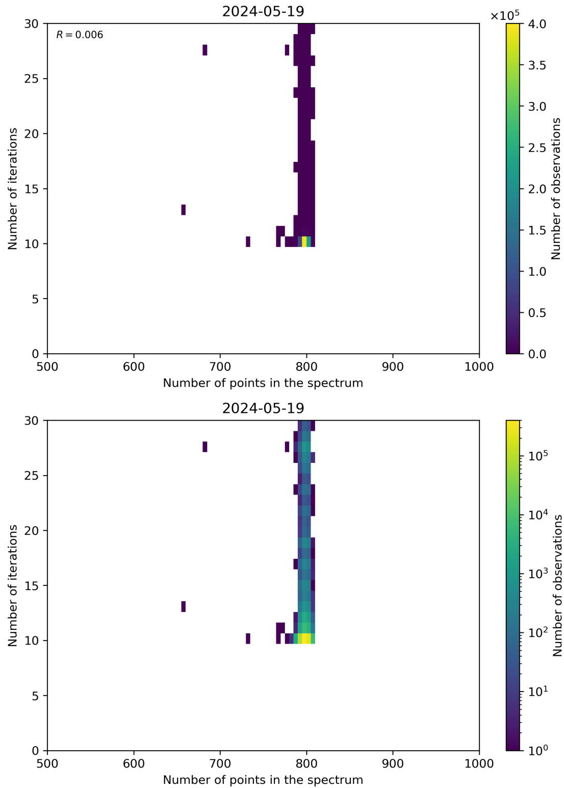
Figure 92: Scatter density plot of “Number of points in the spectrum” against “Number of iterations” for 2024-05-18 to 2024-05-20.
