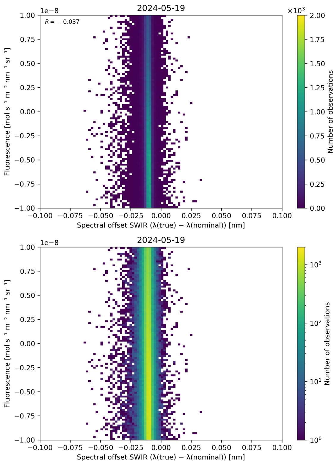
Figure 120: Scatter density plot of “Spectral offset SWIR ( \lambda(\text{true}) - \lambda(\text{nominal}) )” against “Fluorescence” for 2024-05-18 to 2024-05-20.
