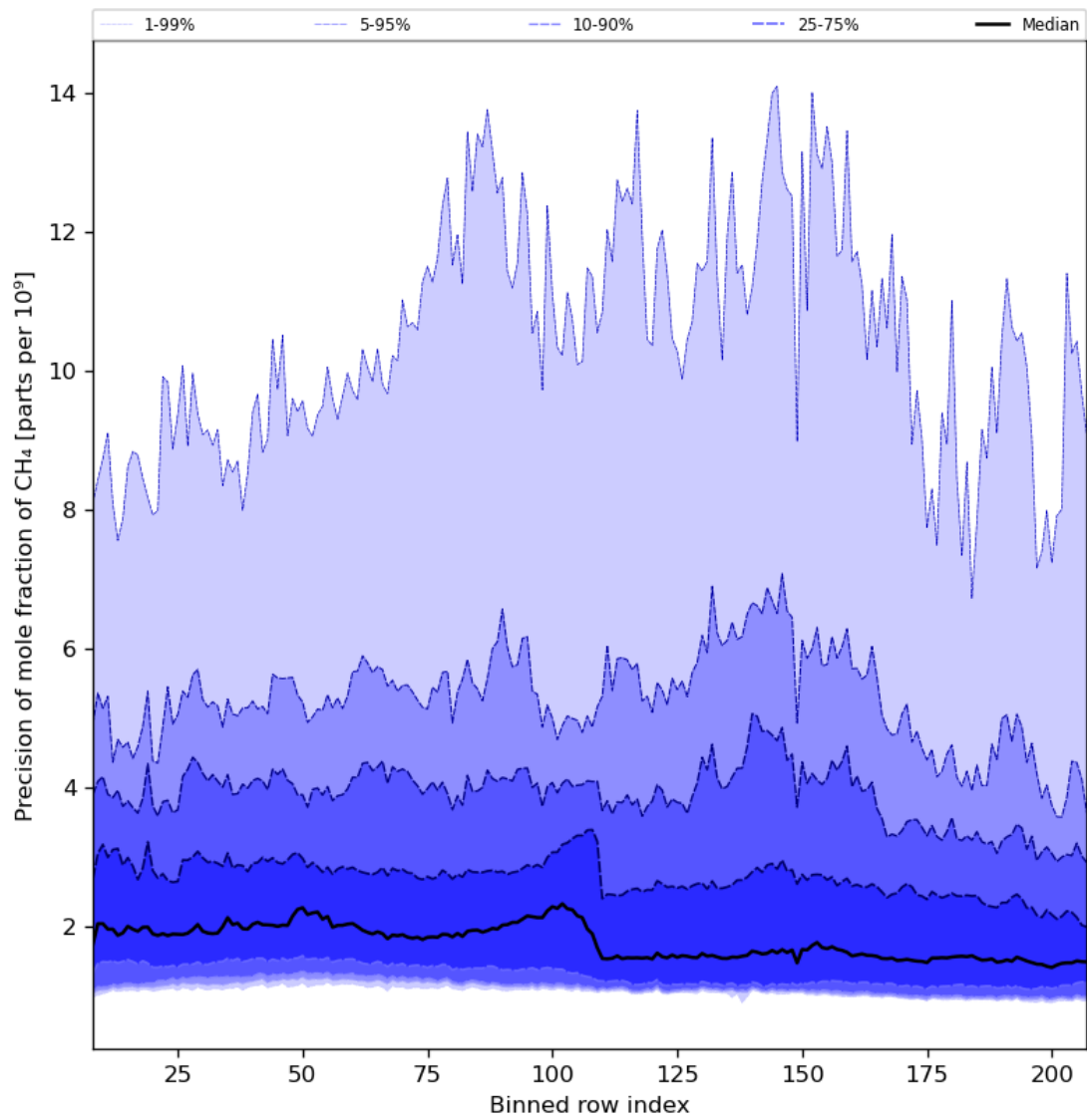
Figure 35: Along track statistics of “Precision of mole fraction of CH 4 ” for 2024-05-18 to 2024-05-20
