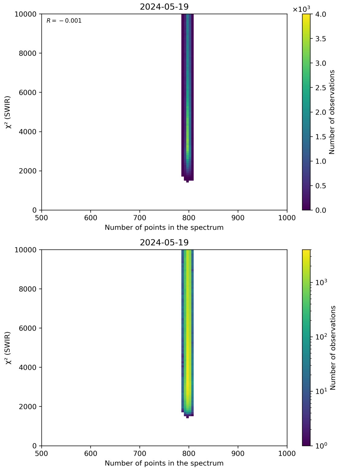
Figure 89: Scatter density plot of “Number of points in the spectrum” against “ \chi^2 (SWIR)” for 2024-05-18 to 2024-05-20.
