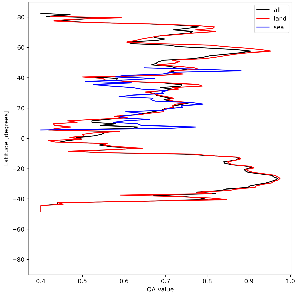
Figure 11: Zonal average of “QA value” for 2024-05-18 to 2024-05-20.
