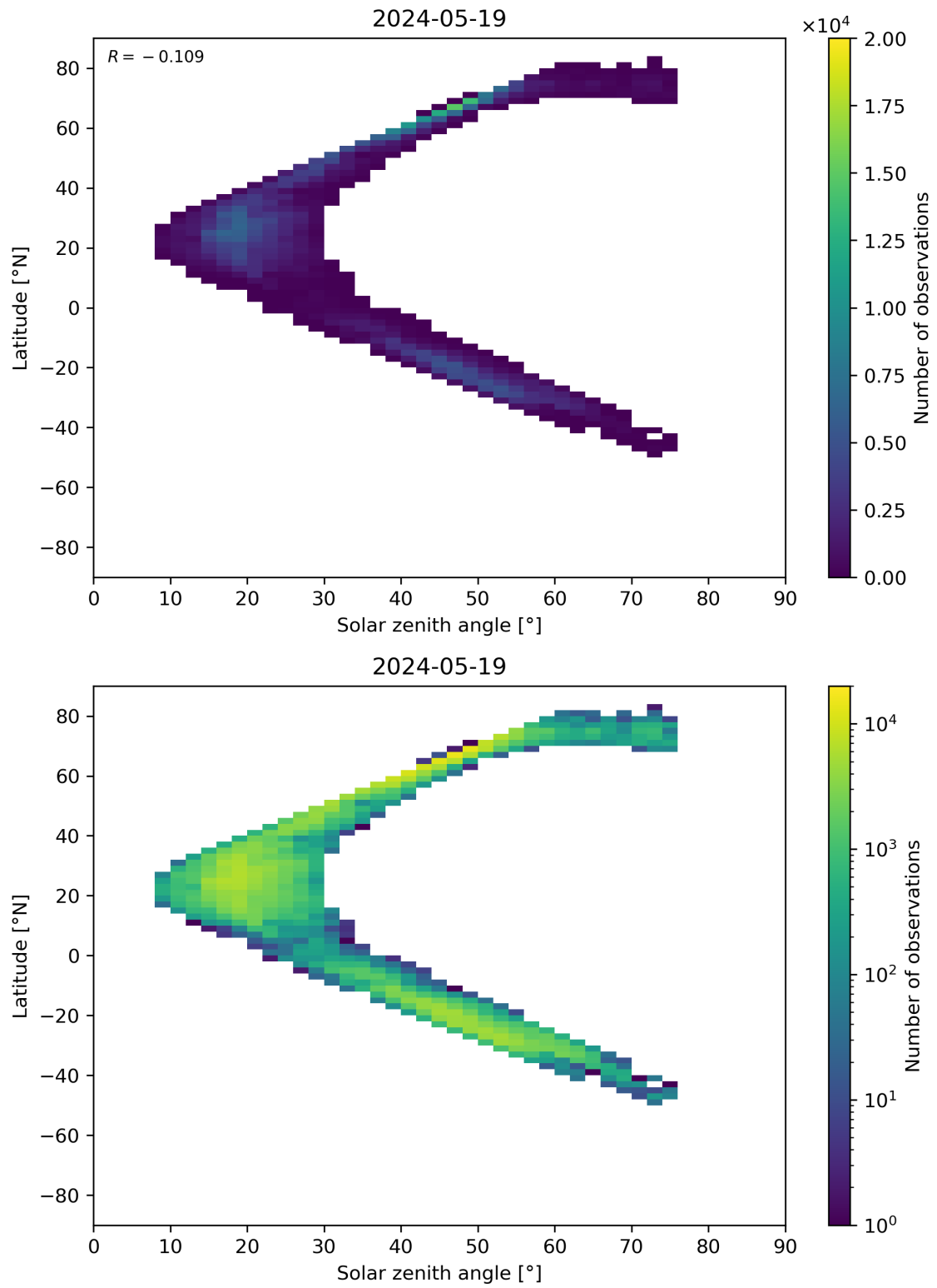
Figure 98: Scatter density plot of “Solar zenith angle” against “Latitude” for 2024-05-18 to 2024-05-20.
