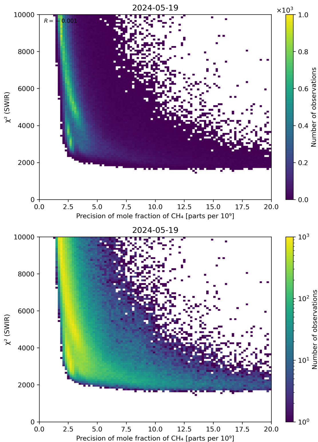
Figure 79: Scatter density plot of “Precision of mole fraction of \text{CH}_4 ” against “ \chi^2 (SWIR)” for 2024-05-18 to 2024-05-20.
