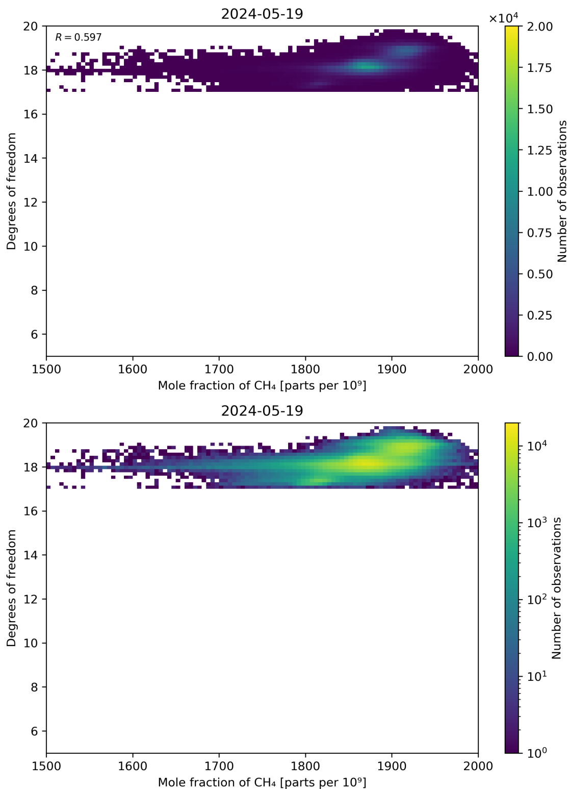
Figure 72: Scatter density plot of “Mole fraction of CH 4 ” against “Degrees of freedom” for 2024-05-18 to 2024-05-20.
