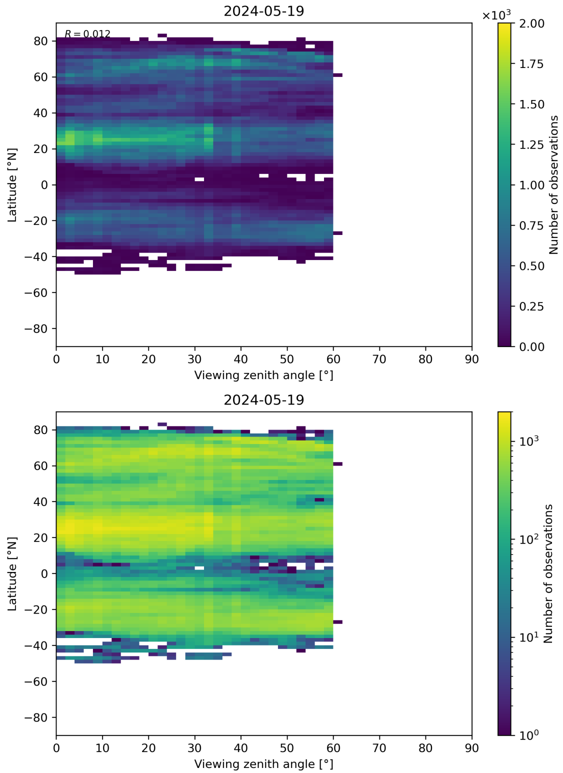
Figure 109: Scatter density plot of “Viewing zenith angle” against “Latitude” for 2024-05-18 to 2024-05-20.
