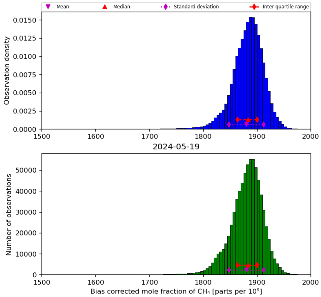
Figure 25: Histogram of “Bias corrected mole fraction of CH 4 ” for 2024-05-18 to 2024-05-20
