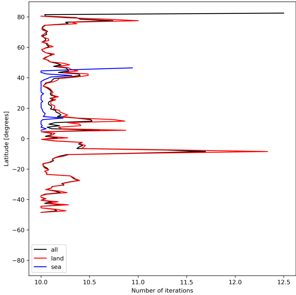
Figure 20: Zonal average of “Number of iterations” for 2024-05-18 to 2024-05-20.
