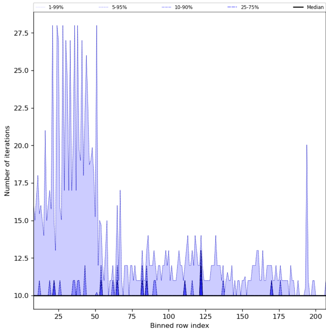
Figure 42: Along track statistics of “Number of iterations” for 2024-05-18 to 2024-05-20
