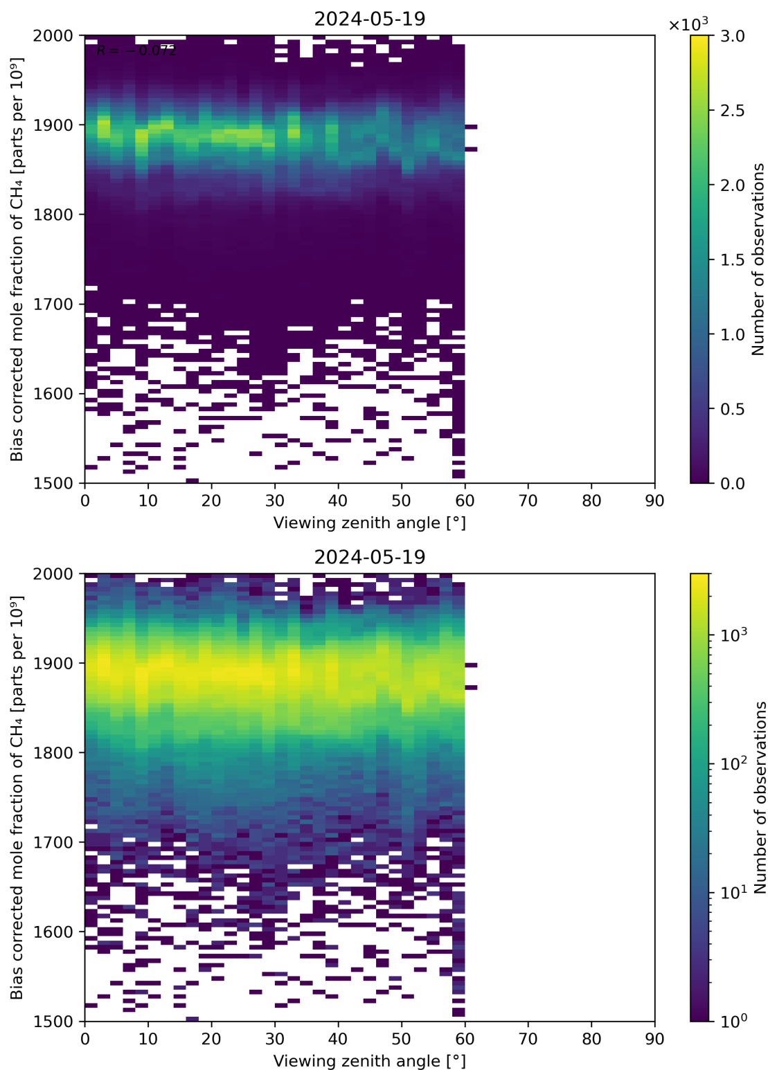
Figure 111: Scatter density plot of “Viewing zenith angle” against “Bias corrected mole fraction of CH 4 ” for 2024-05-18 to 2024-05-20.
