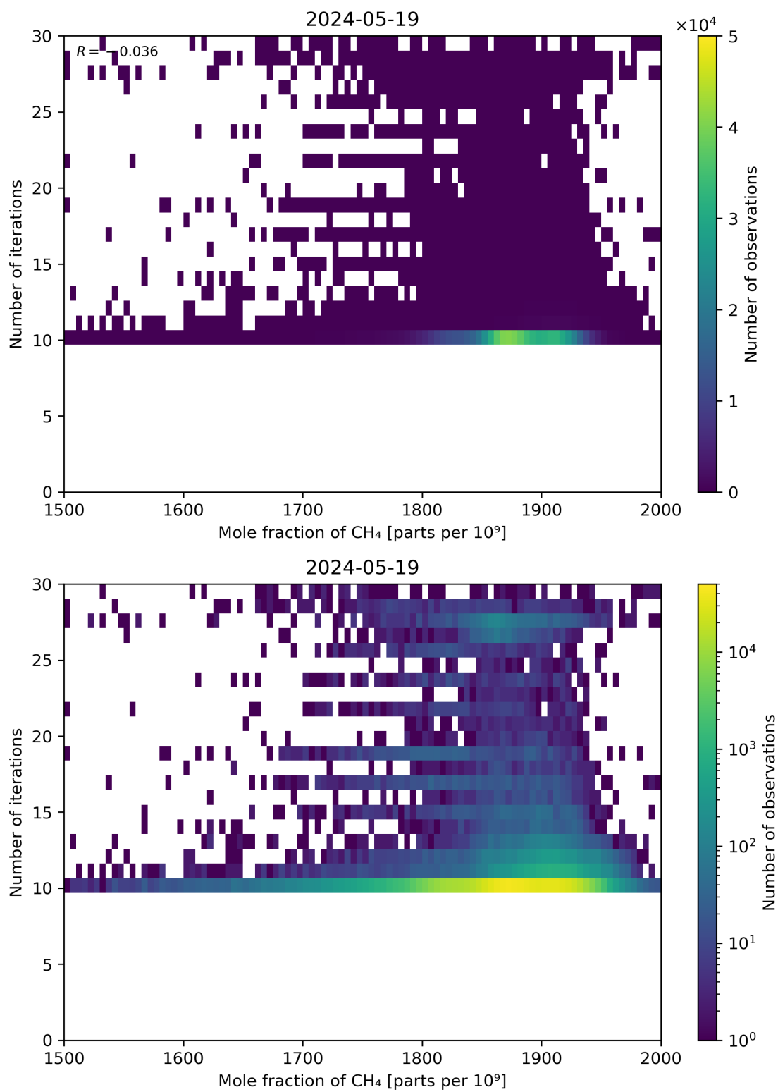
Figure 76: Scatter density plot of “Mole fraction of CH 4 ” against “Number of iterations” for 2024-05-18 to 2024-05-20.
