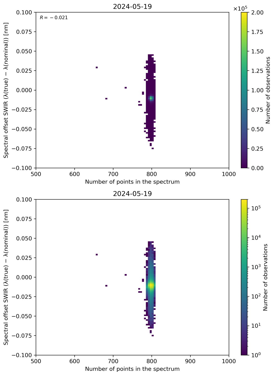
Figure 93: Scatter density plot of “Number of points in the spectrum” against “Spectral offset SWIR ( \lambda(\text{true}) - \lambda(\text{nominal}) )” for 2024-05-18 to 2024-05-20.
