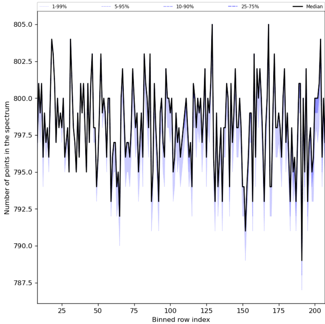
Figure 37: Along track statistics of “Number of points in the spectrum” for 2024-05-18 to 2024-05-20
