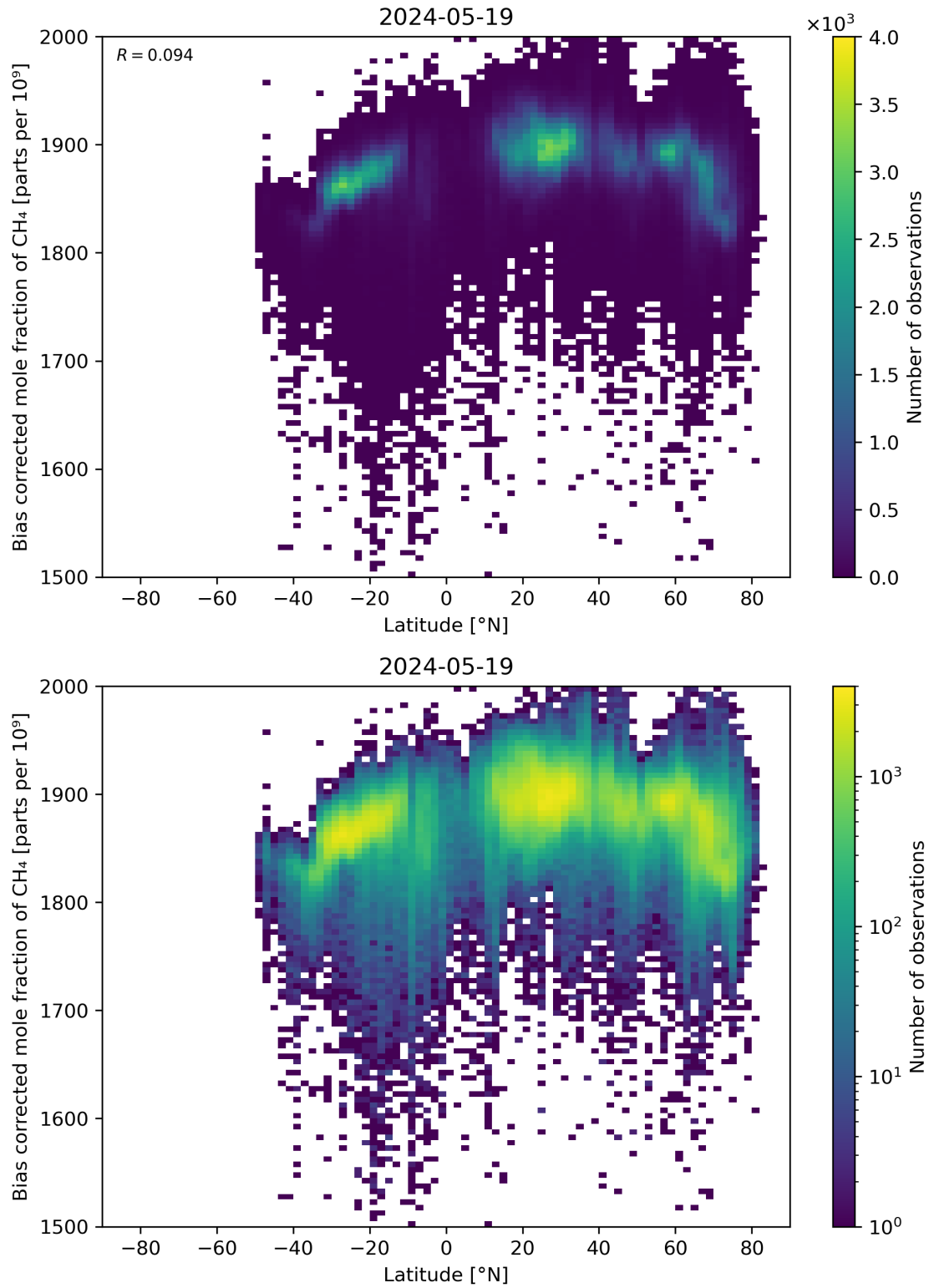
Figure 58: Scatter density plot of “Latitude” against “Bias corrected mole fraction of \text{CH}_4 ” for 2024-05-18 to 2024-05-20.
