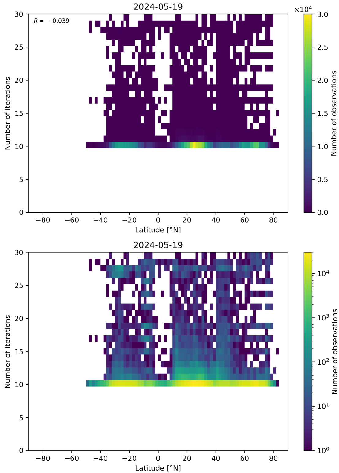
Figure 60: Scatter density plot of “Latitude” against “Number of iterations” for 2024-05-18 to 2024-05-20.
