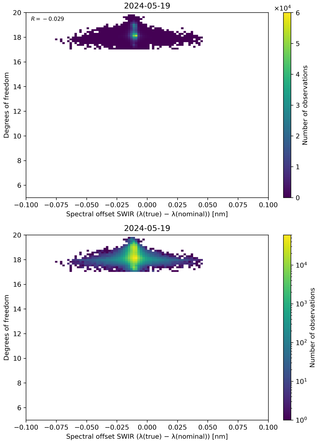
Figure 119: Scatter density plot of “Spectral offset SWIR ( \lambda(\text{true}) - \lambda(\text{nominal}) )” against “Degrees of freedom” for 2024-05-18 to 2024-05-20.
