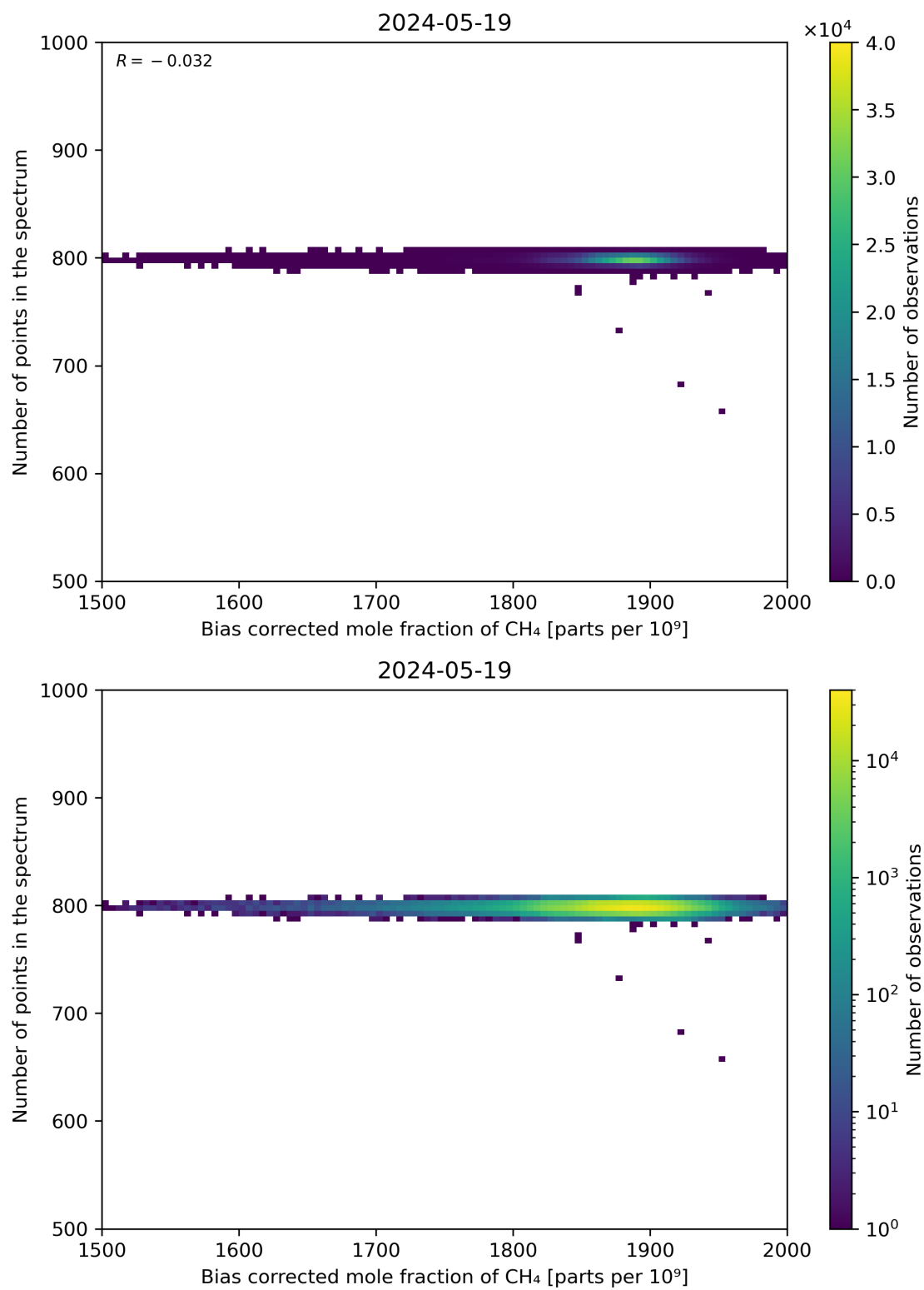
Figure 68: Scatter density plot of “Bias corrected mole fraction of CH 4 ” against “Number of points in the spectrum” for 2024-05-18 to 2024-05-20.
