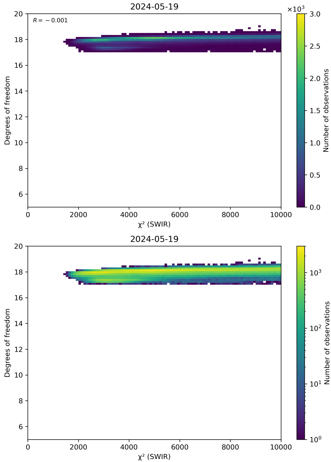
Figure 48: Scatter density plot of “ \chi^2 (SWIR)” against “Degrees of freedom” for 2024-05-18 to 2024-05-20.
