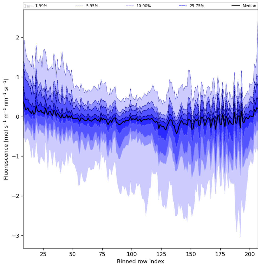
Figure 43: Along track statistics of “Fluorescence” for 2024-05-18 to 2024-05-20
