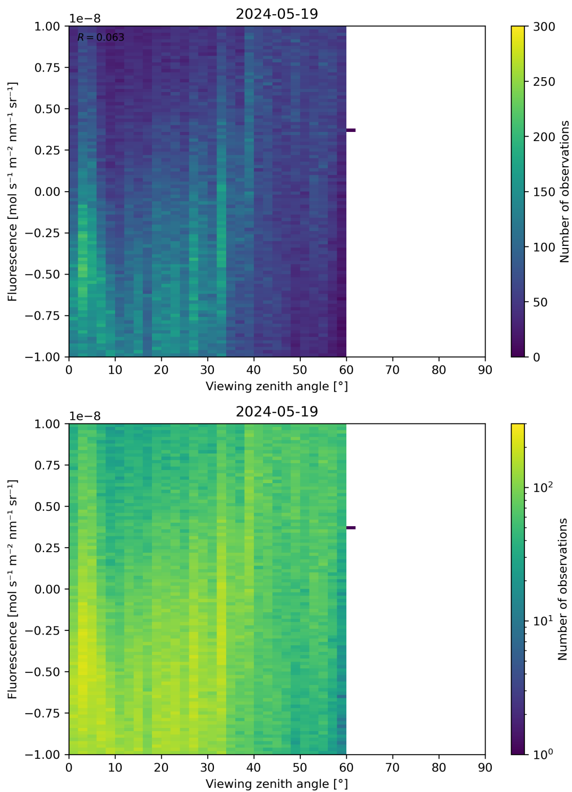
Figure 108: Scatter density plot of “Viewing zenith angle” against “Fluorescence” for 2024-05-18 to 2024-05-20.
