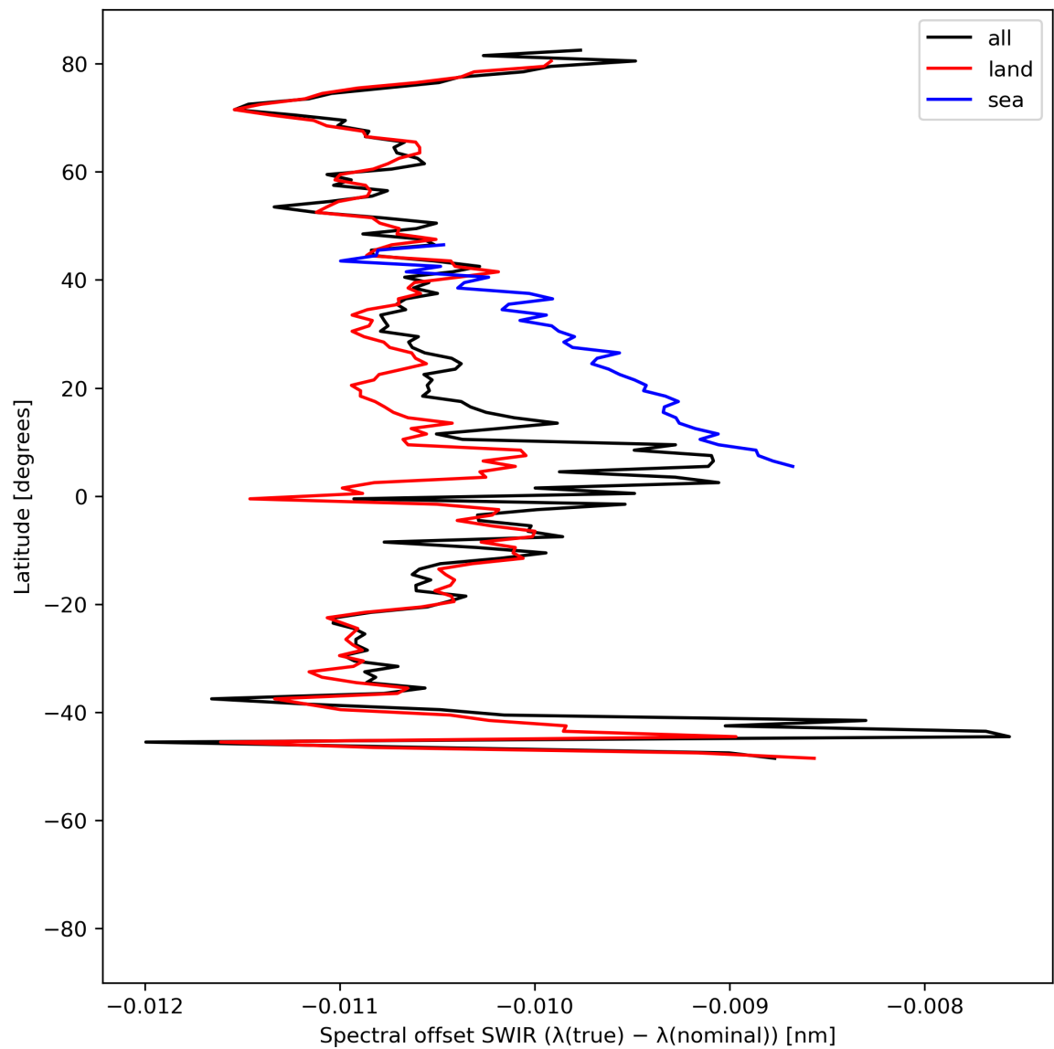
Figure 16: Zonal average of “Spectral offset SWIR ( \lambda(\text{true}) - \lambda(\text{nominal}) )” for 2024-05-18 to 2024-05-20.
