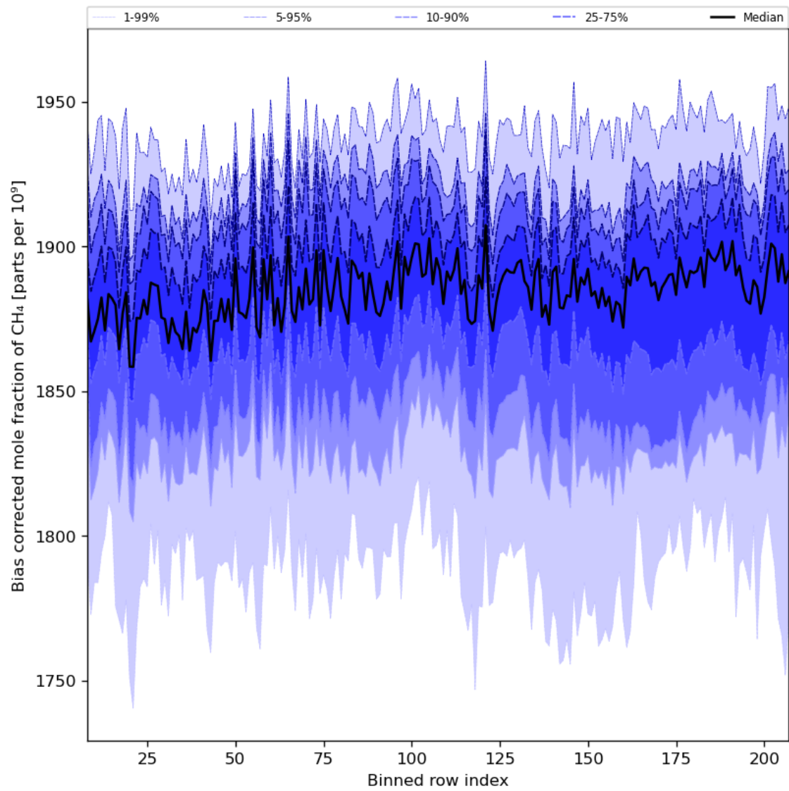
Figure 36: Along track statistics of “Bias corrected mole fraction of CH 4 ” for 2024-05-18 to 2024-05-20
