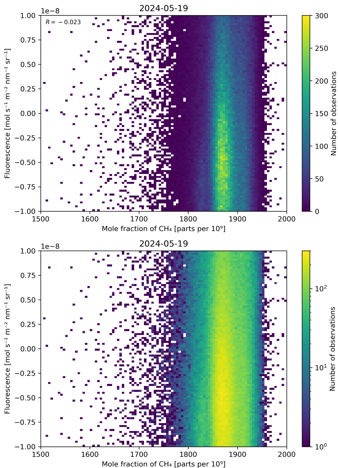
Figure 73: Scatter density plot of “Mole fraction of \text{CH}_4 ” against “Fluorescence” for 2024-05-18 to 2024-05-20.
