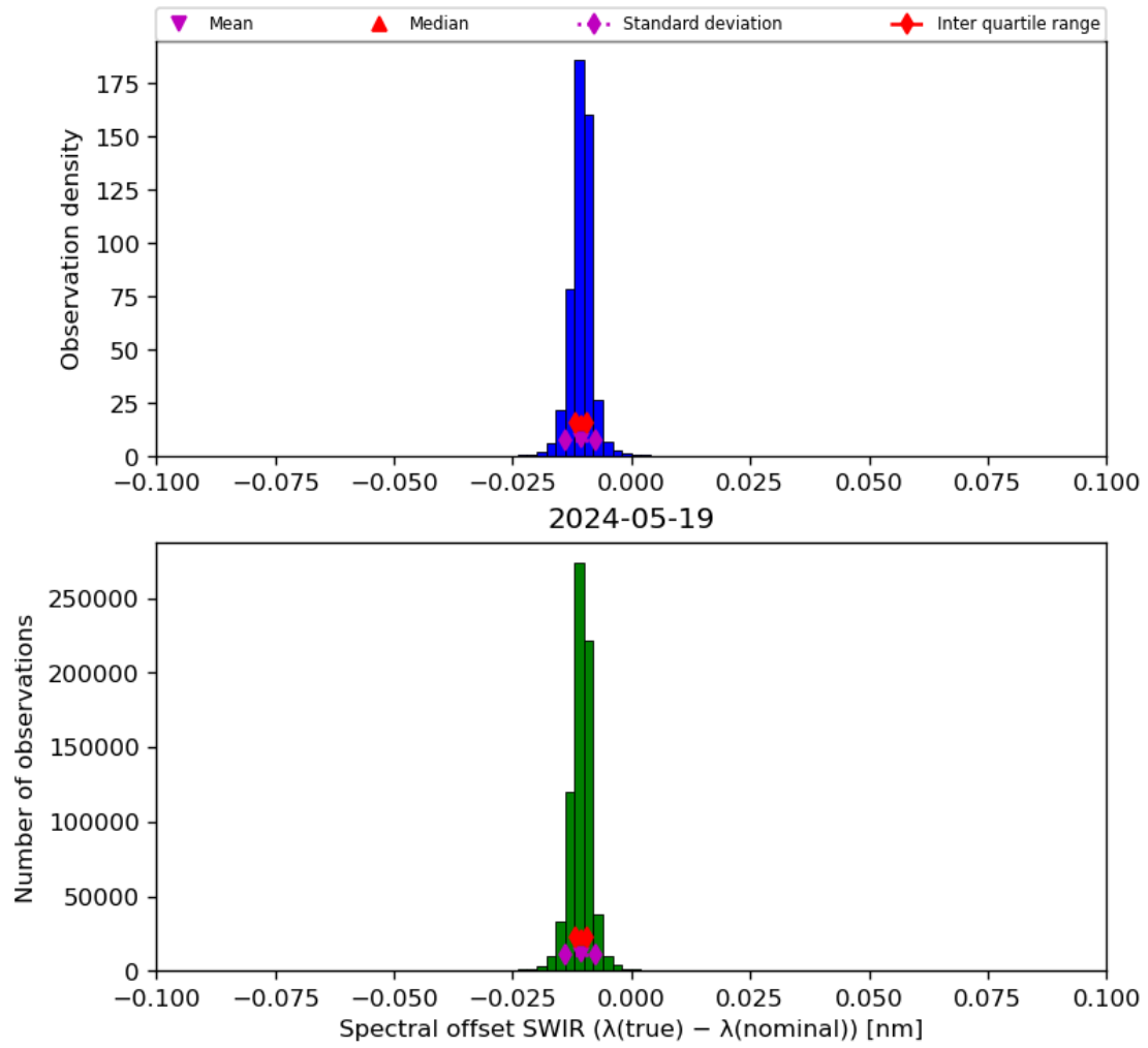
Figure 27: Histogram of “Spectral offset SWIR ( \lambda(\text{true}) - \lambda(\text{nominal}) )” for 2024-05-18 to 2024-05-20
