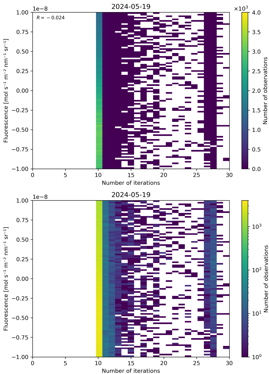
Figure 87: Scatter density plot of “Number of iterations” against “Fluorescence” for 2024-05-18 to 2024-05-20.
