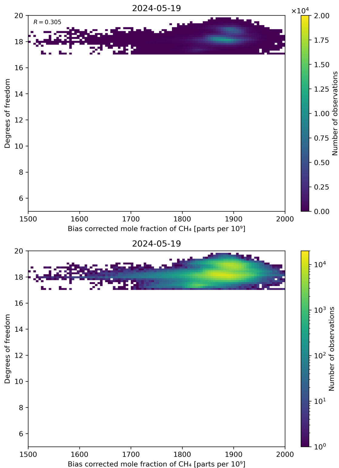
Figure 65: Scatter density plot of “Bias corrected mole fraction of CH 4 ” against “Degrees of freedom” for 2024-05-18 to 2024-05-20.
