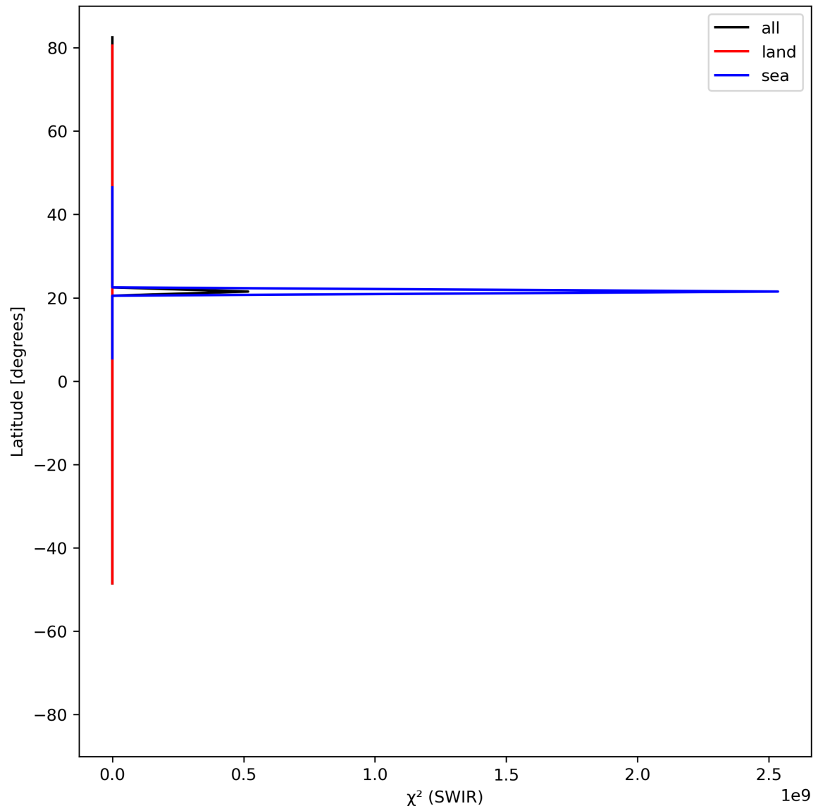
Figure 17: Zonal average of “ \chi^2 (SWIR)” for 2024-05-18 to 2024-05-20.
