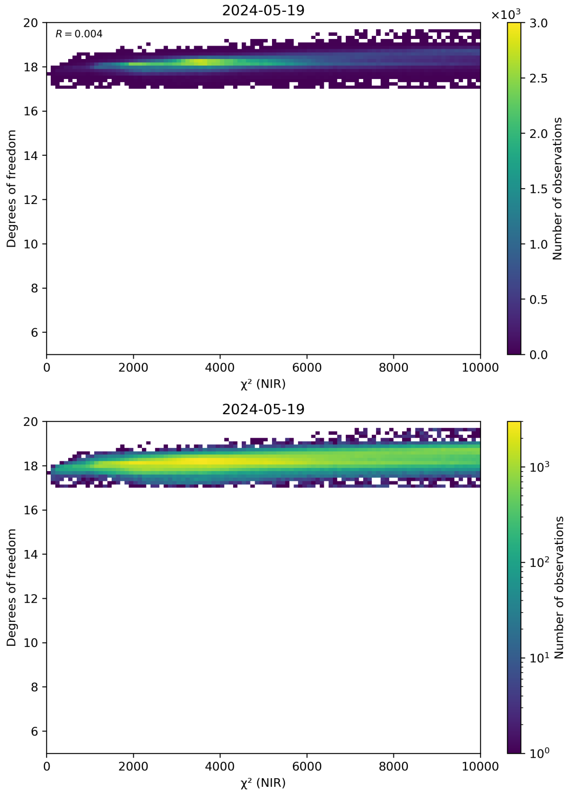
Figure 44: Scatter density plot of “ \chi^2 (NIR)” against “Degrees of freedom” for 2024-05-18 to 2024-05-20.
