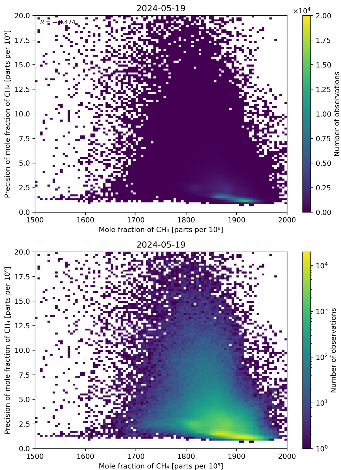
Figure 75: Scatter density plot of “Mole fraction of CH 4 ” against “Precision of mole fraction of CH 4 ” for 2024-05-18 to 2024-05-20.
