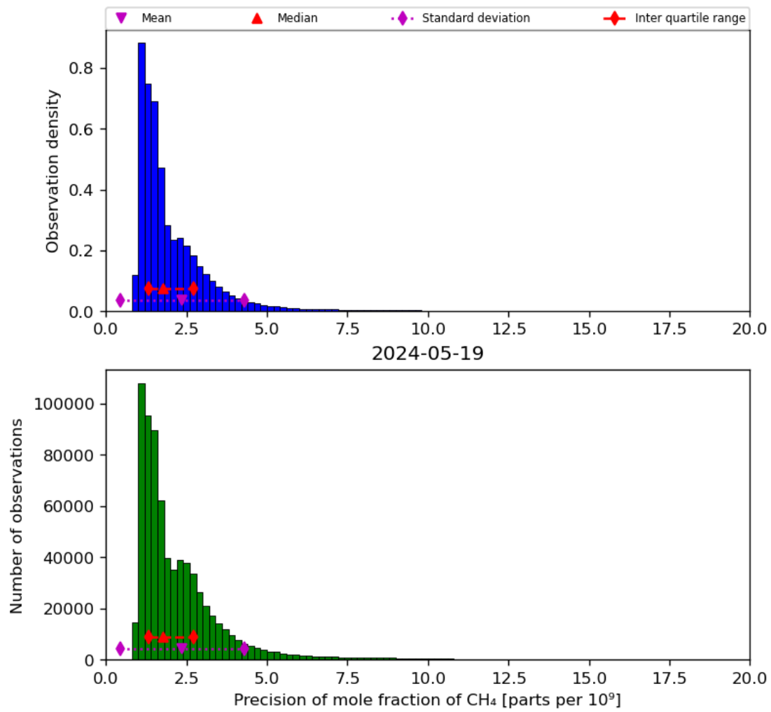
Figure 24: Histogram of “Precision of mole fraction of CH 4 ” for 2024-05-18 to 2024-05-20
