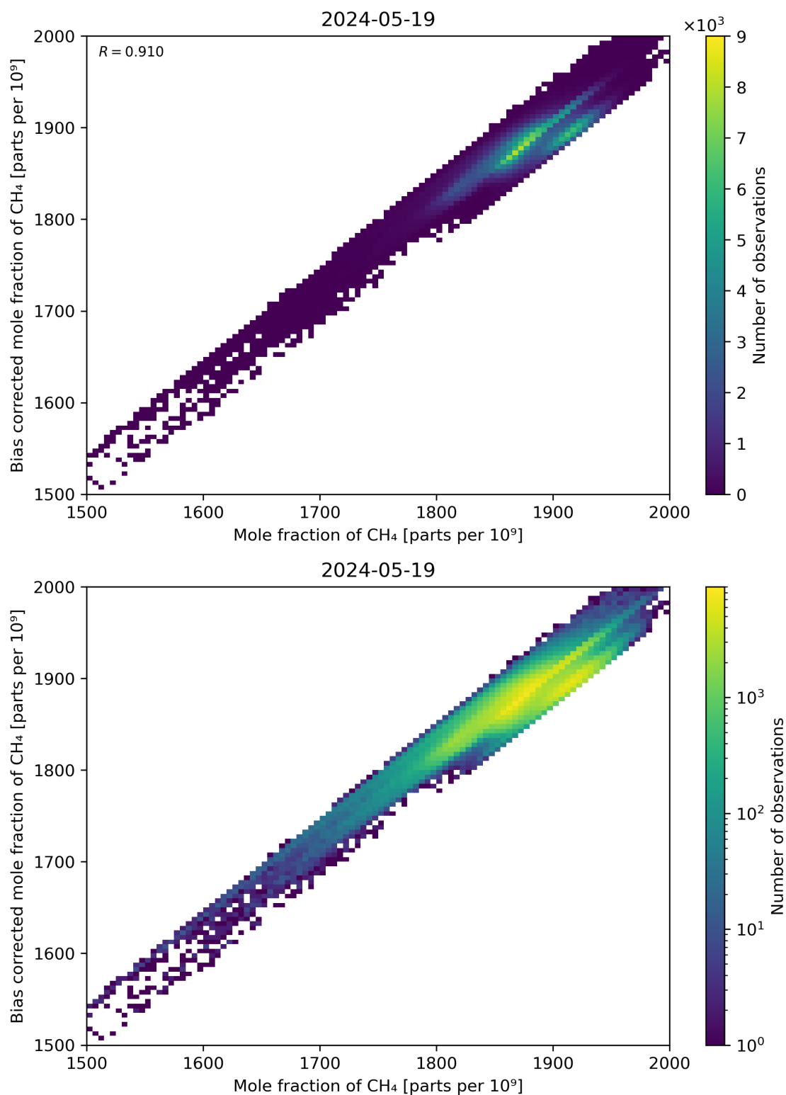
Figure 74: Scatter density plot of “Mole fraction of CH 4 ” against “Bias corrected mole fraction of CH 4 ” for 2024-05-18 to 2024-05-20.
