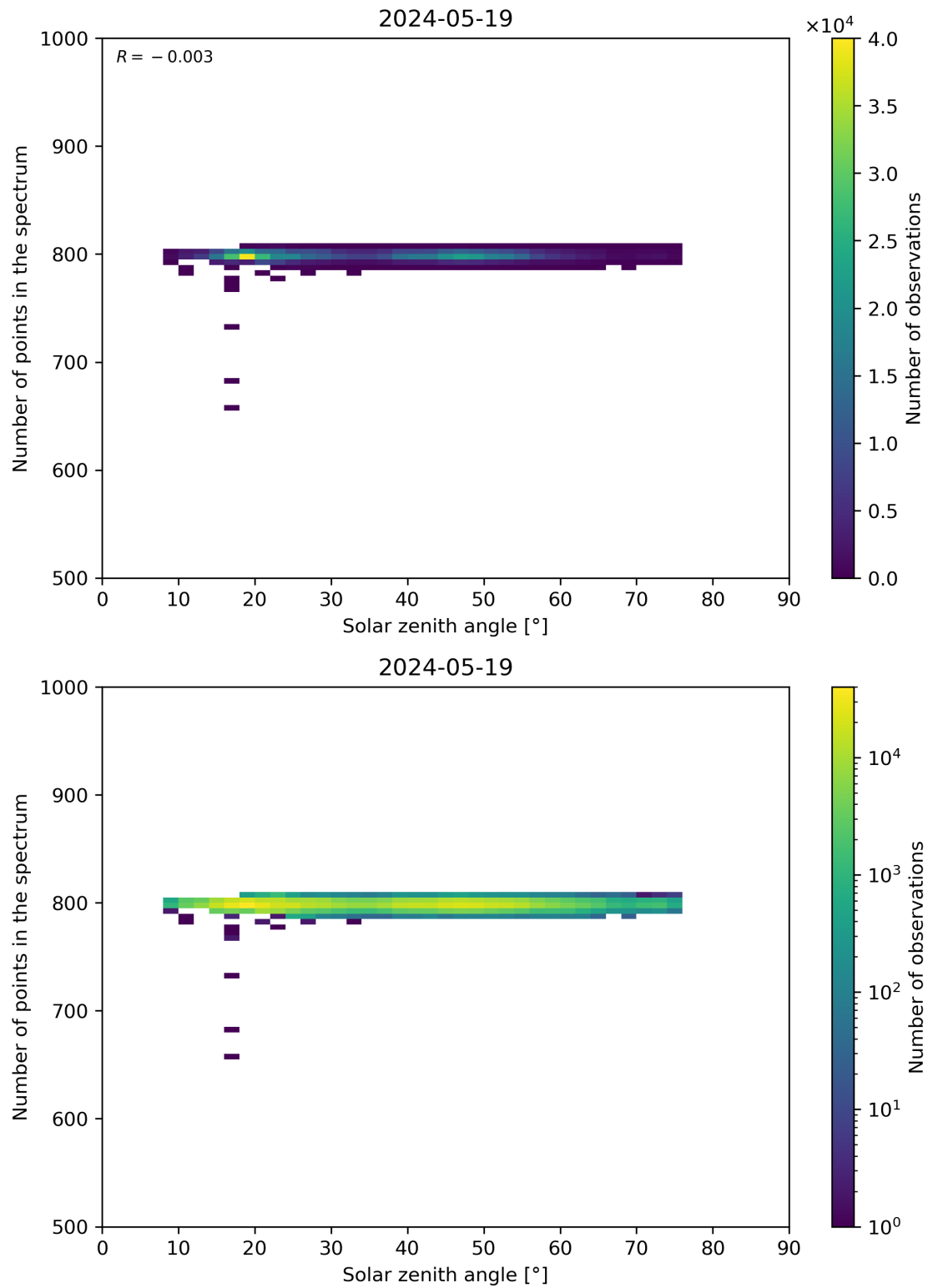
Figure 103: Scatter density plot of “Solar zenith angle” against “Number of points in the spectrum” for 2024-05-18 to 2024-05-20.
