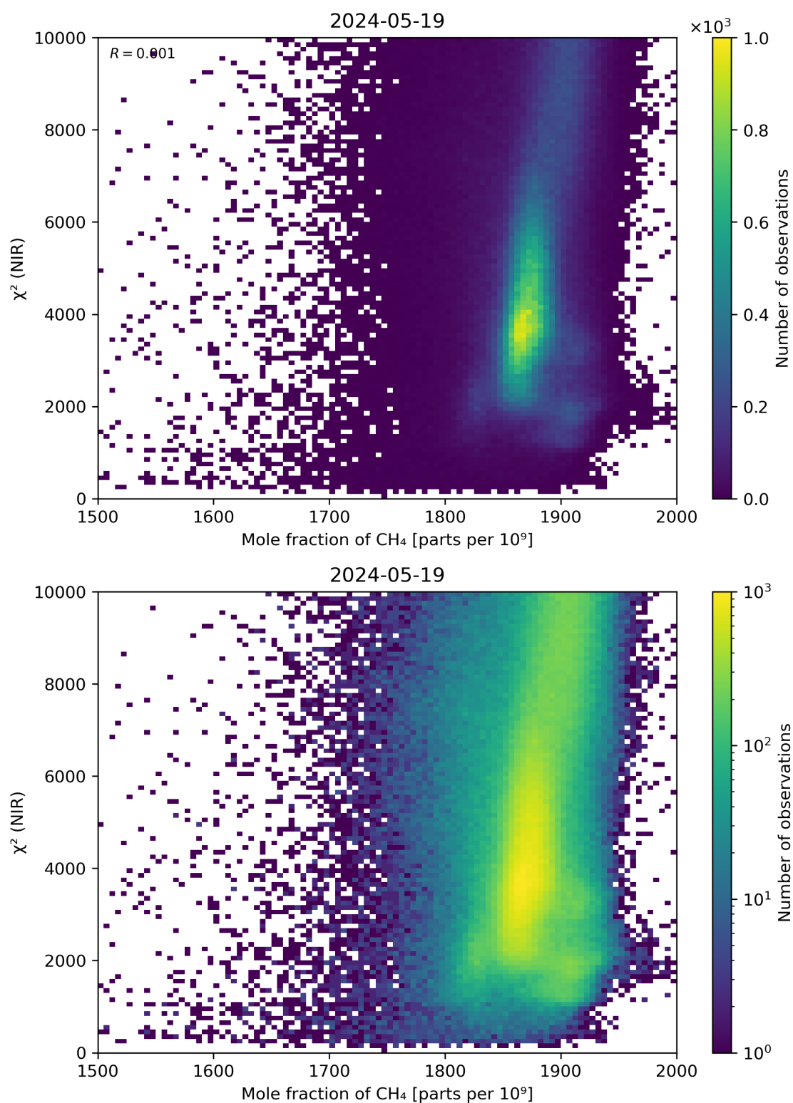
Figure 70: Scatter density plot of “Mole fraction of \text{CH}_4 ” against “ \chi^2 (NIR)” for 2024-05-18 to 2024-05-20.
