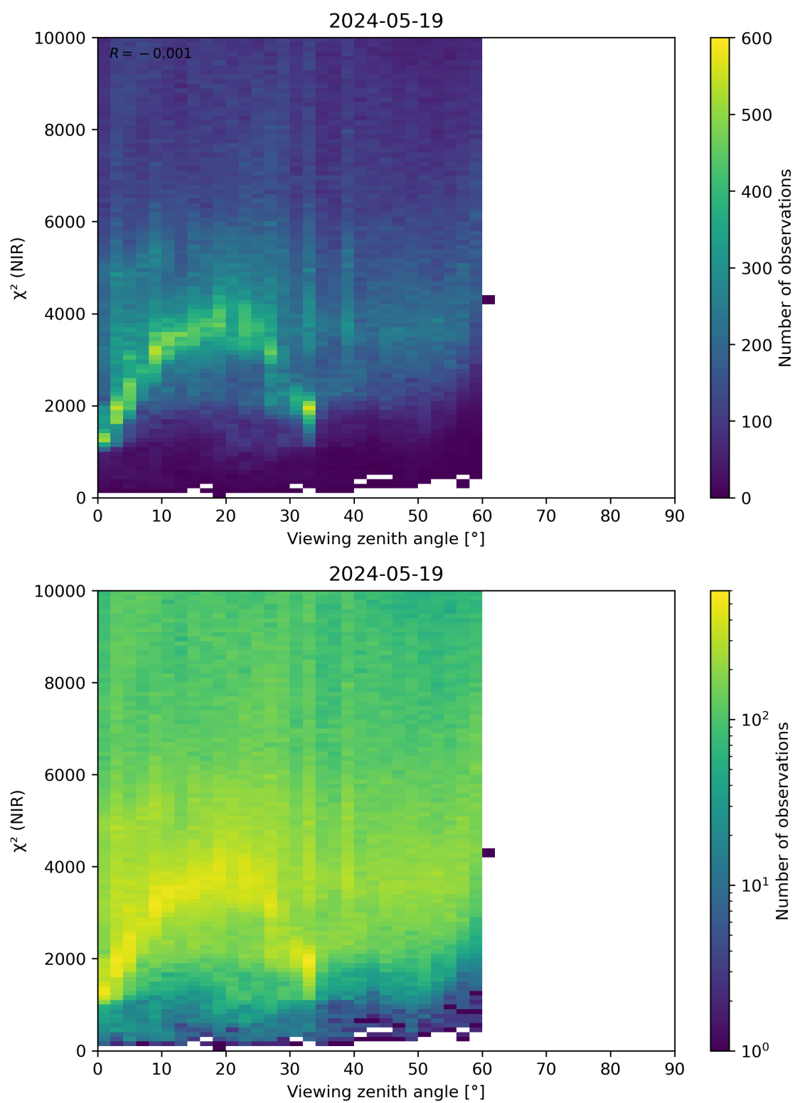
Figure 105: Scatter density plot of “Viewing zenith angle” against “ \chi^2 (NIR)” for 2024-05-18 to 2024-05-20.
