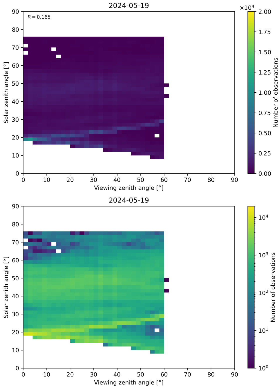
Figure 115: Scatter density plot of “Viewing zenith angle” against “Solar zenith angle” for 2024-05-18 to 2024-05-20.
