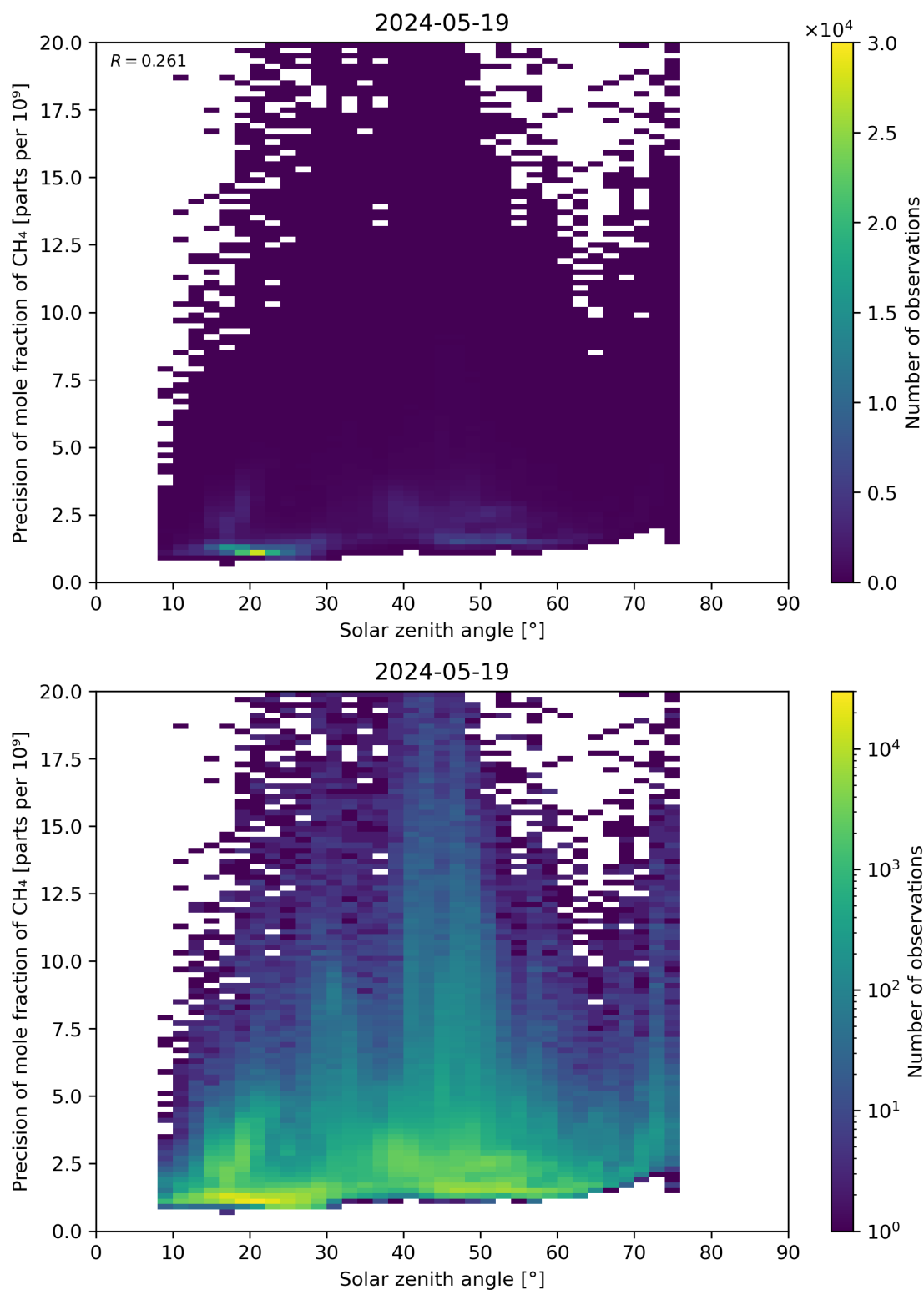
Figure 101: Scatter density plot of “Solar zenith angle” against “Precision of mole fraction of CH 4 ” for 2024-05-18 to 2024-05-20.
