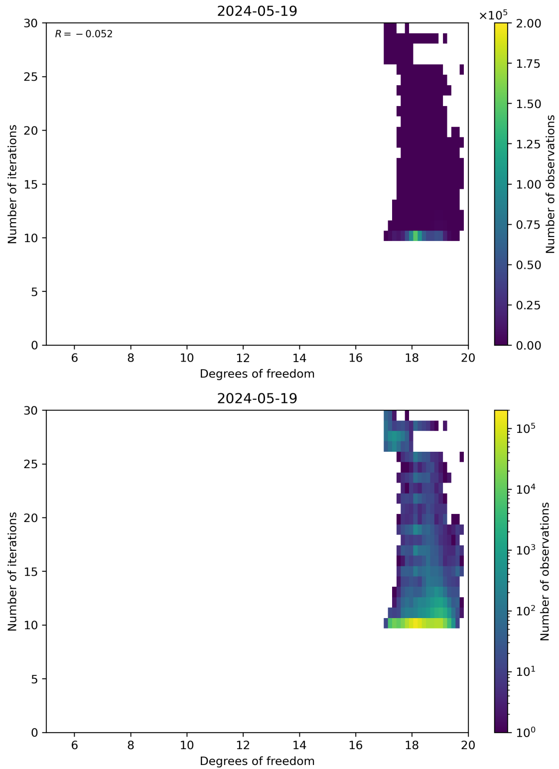
Figure 52: Scatter density plot of “Degrees of freedom” against “Number of iterations” for 2024-05-18 to 2024-05-20.
