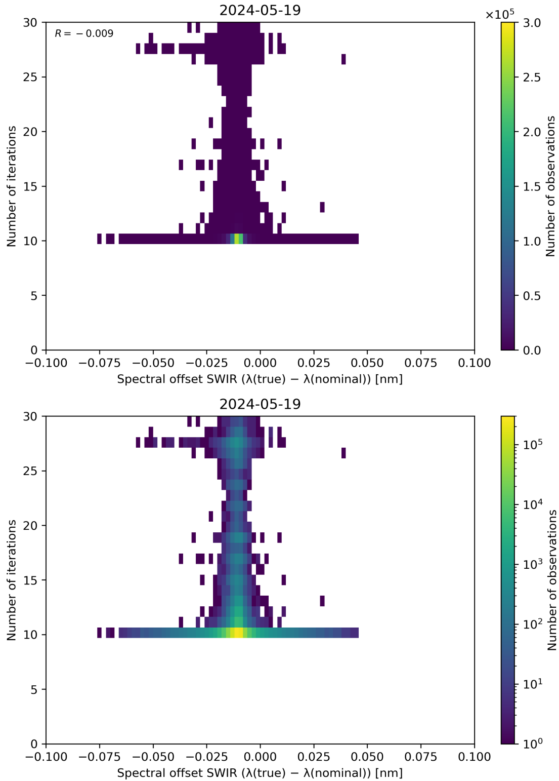
Figure 121: Scatter density plot of “Spectral offset SWIR ( \lambda(\text{true}) - \lambda(\text{nominal}) )” against “Number of iterations” for 2024-05-18 to 2024-05-20.
