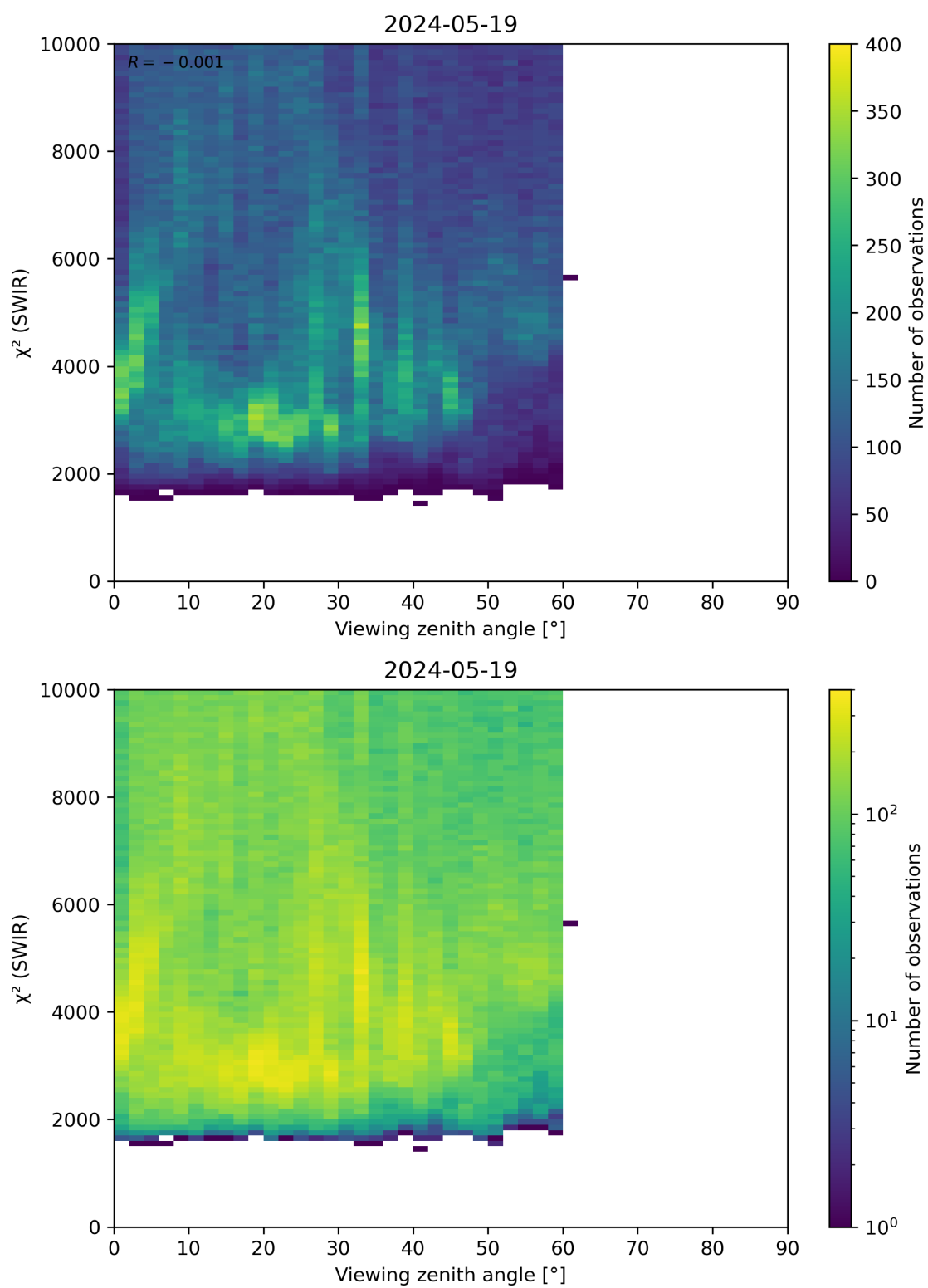
Figure 106: Scatter density plot of “Viewing zenith angle” against “ \chi^2 (SWIR)” for 2024-05-18 to 2024-05-20.
