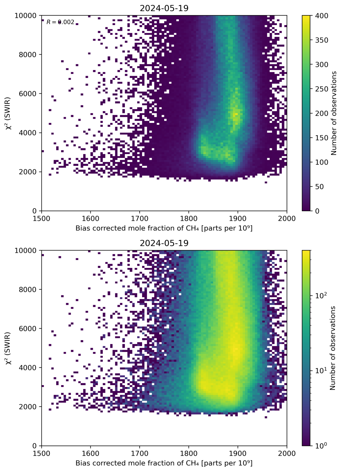
Figure 64: Scatter density plot of “Bias corrected mole fraction of \text{CH}_4 ” against “ \chi^2 (SWIR)” for 2024-05-18 to 2024-05-20.
