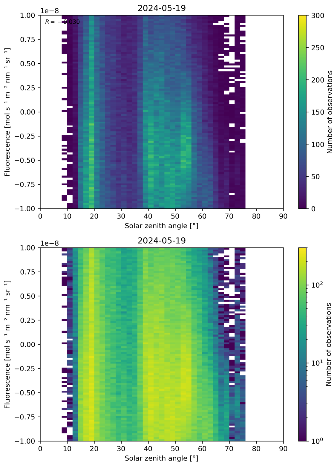
Figure 97: Scatter density plot of “Solar zenith angle” against “Fluorescence” for 2024-05-18 to 2024-05-20.
