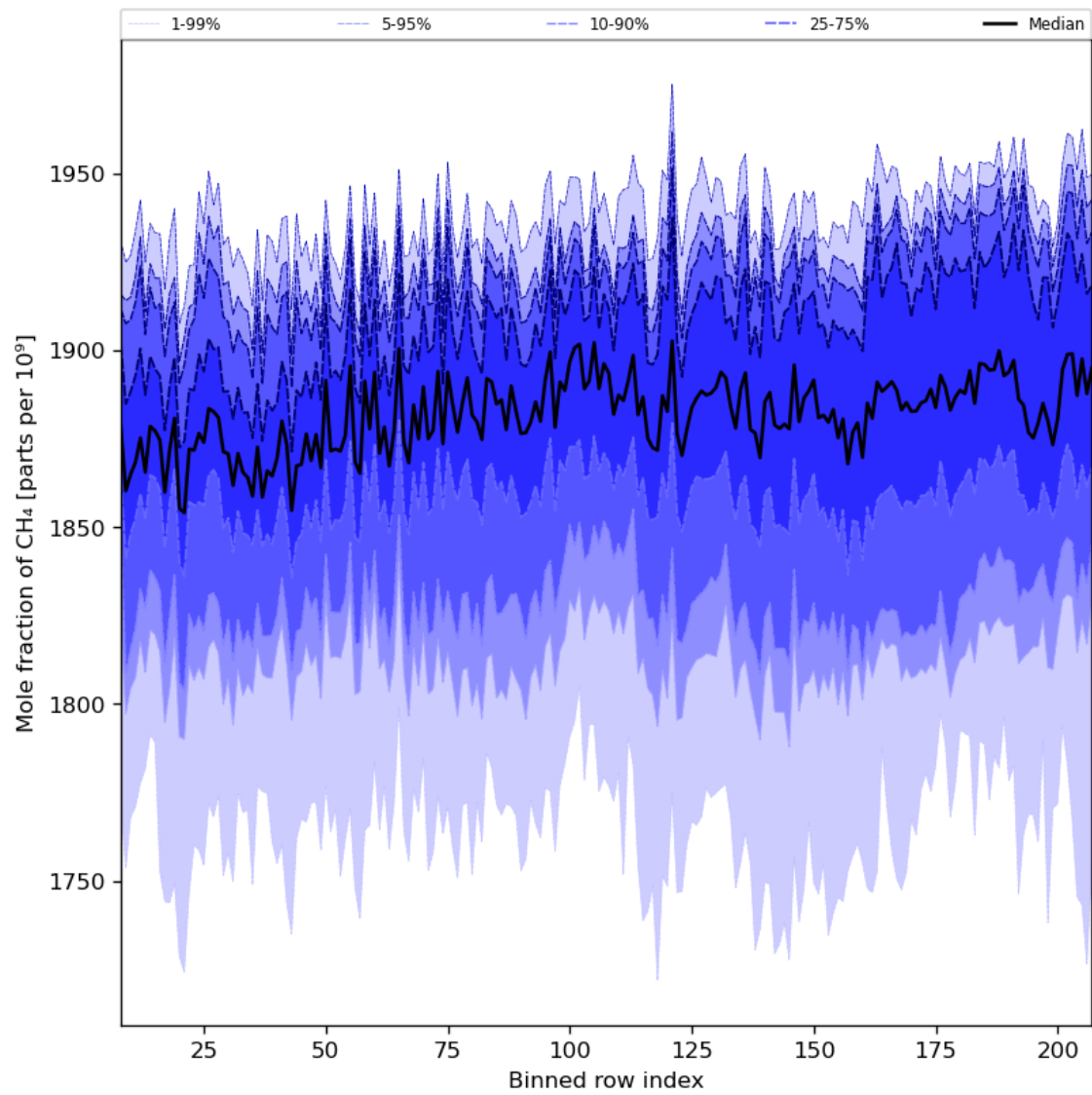
Figure 34: Along track statistics of “Mole fraction of CH 4 ” for 2024-05-18 to 2024-05-20
