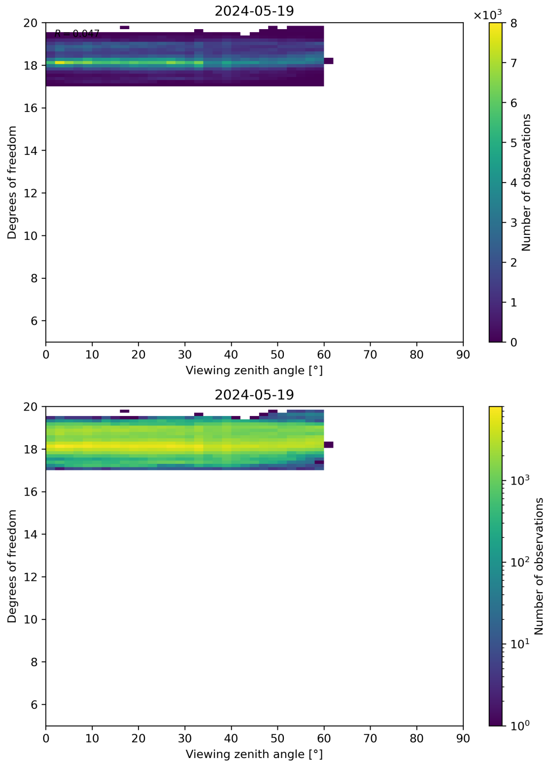
Figure 107: Scatter density plot of “Viewing zenith angle” against “Degrees of freedom” for 2024-05-18 to 2024-05-20.
