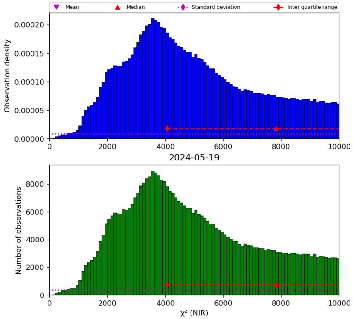
Figure 29: Histogram of “ \chi^2 (NIR)” for 2024-05-18 to 2024-05-20
