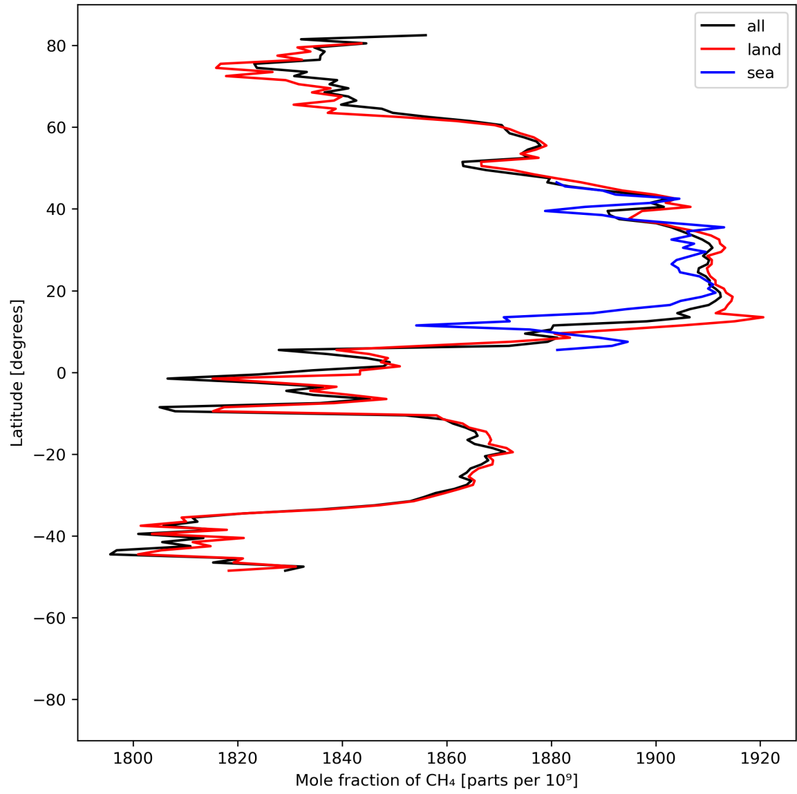
Figure 12: Zonal average of “Mole fraction of \text{CH}_4 ” for 2024-05-18 to 2024-05-20.
