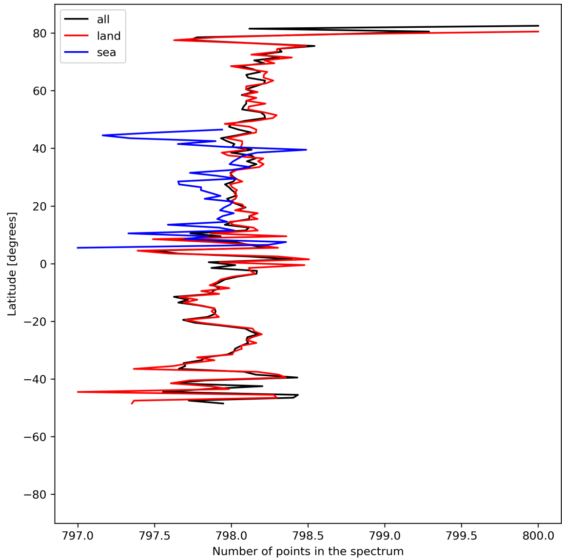
Figure 15: Zonal average of “Number of points in the spectrum” for 2024-05-18 to 2024-05-20.
