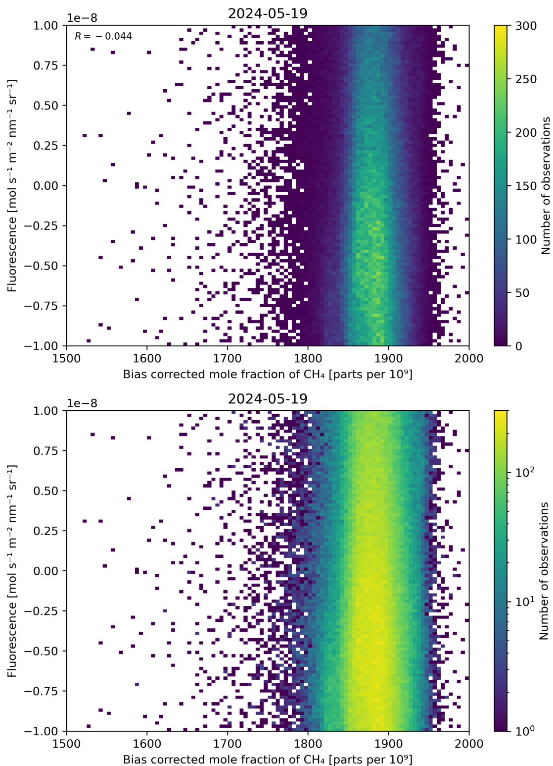
Figure 66: Scatter density plot of “Bias corrected mole fraction of \text{CH}_4 ” against “Fluorescence” for 2024-05-18 to 2024-05-20.
