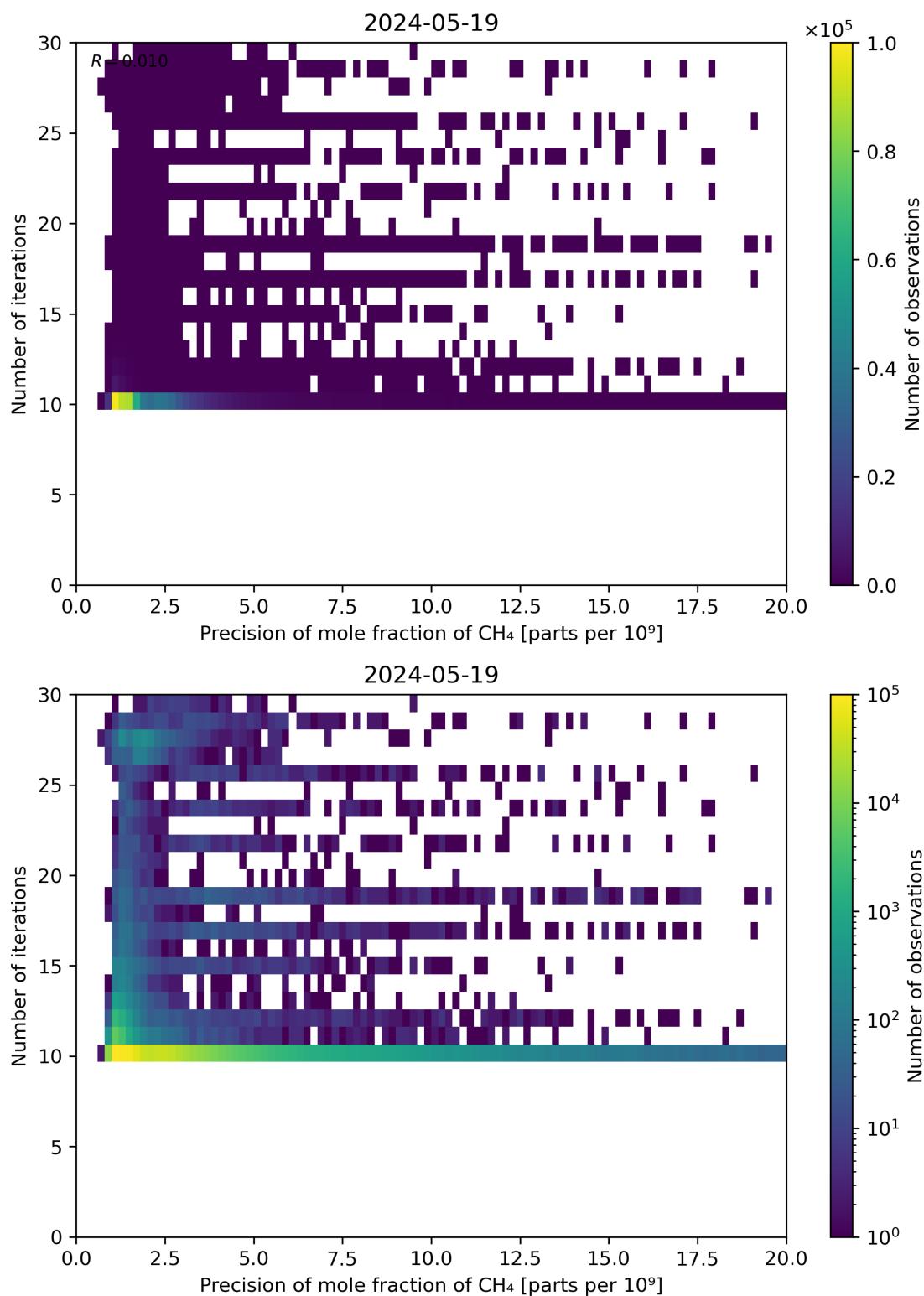
Figure 83: Scatter density plot of “Precision of mole fraction of CH 4 ” against “Number of iterations” for 2024-05-18 to 2024-05-20.
