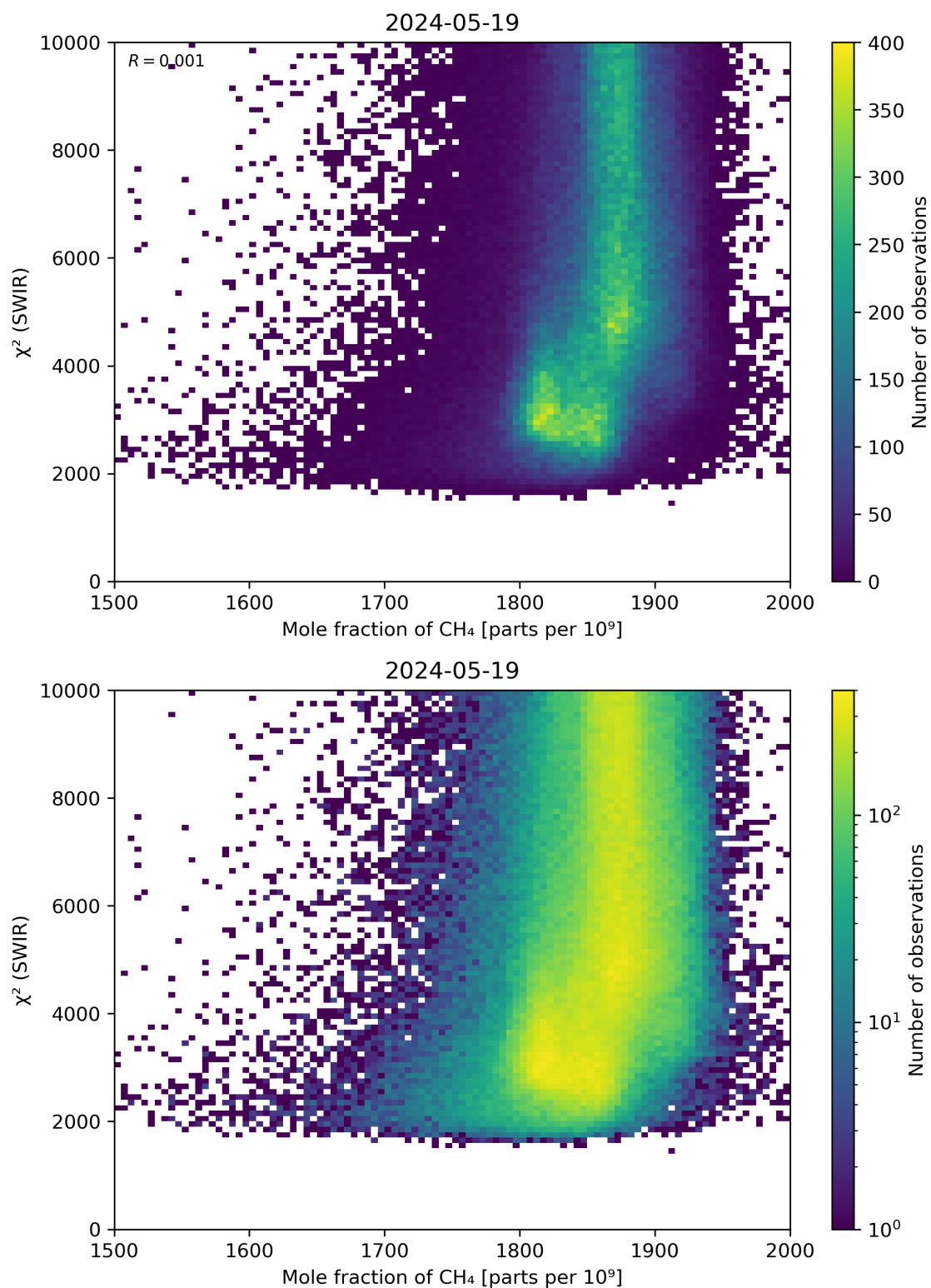
Figure 71: Scatter density plot of “Mole fraction of \text{CH}_4 ” against “ \chi^2 (SWIR)” for 2024-05-18 to 2024-05-20.
