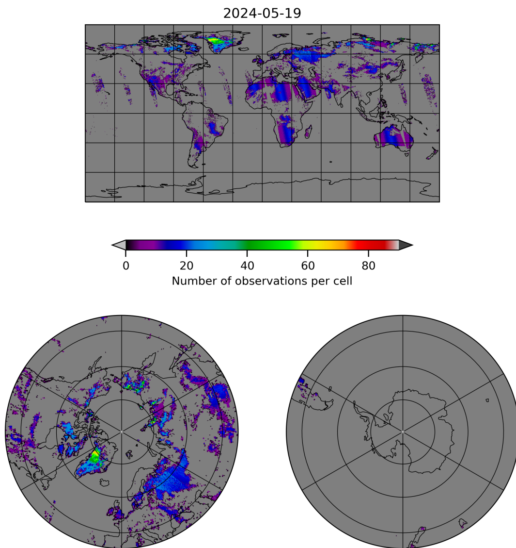
Figure 10: Map of the number of observations for 2024-05-18 to 2024-05-20
