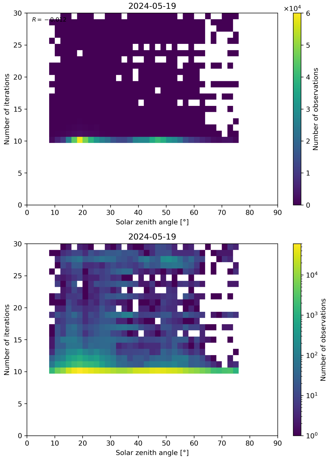
Figure 102: Scatter density plot of “Solar zenith angle” against “Number of iterations” for 2024-05-18 to 2024-05-20.
