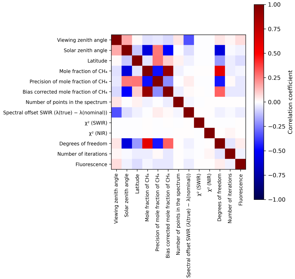
Figure 2: Map of correlation matrix for 2024-05-18 to 2024-05-20.
