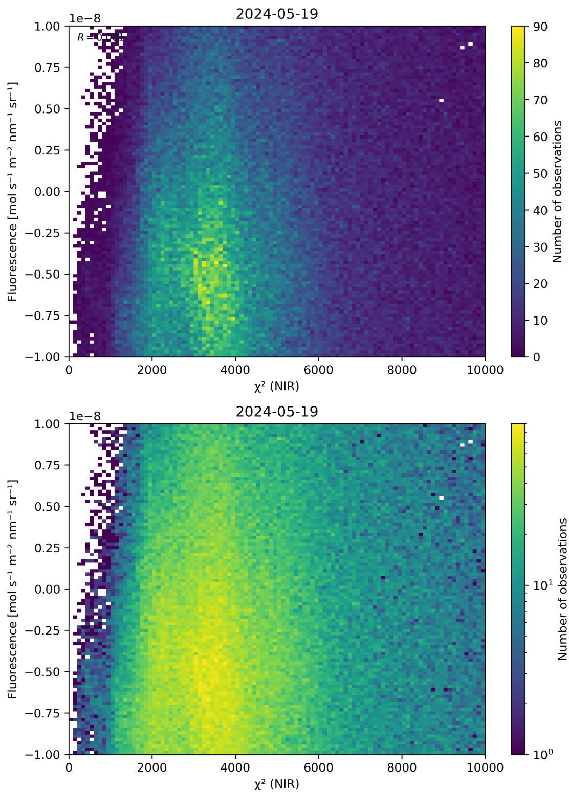
Figure 45: Scatter density plot of “ \chi^2 (NIR)” against “Fluorescence” for 2024-05-18 to 2024-05-20.
