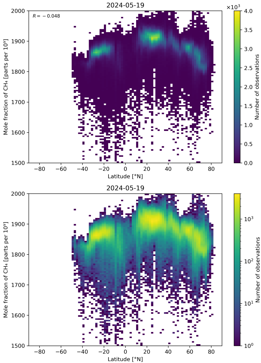
Figure 57: Scatter density plot of “Latitude” against “Mole fraction of CH 4 ” for 2024-05-18 to 2024-05-20.
