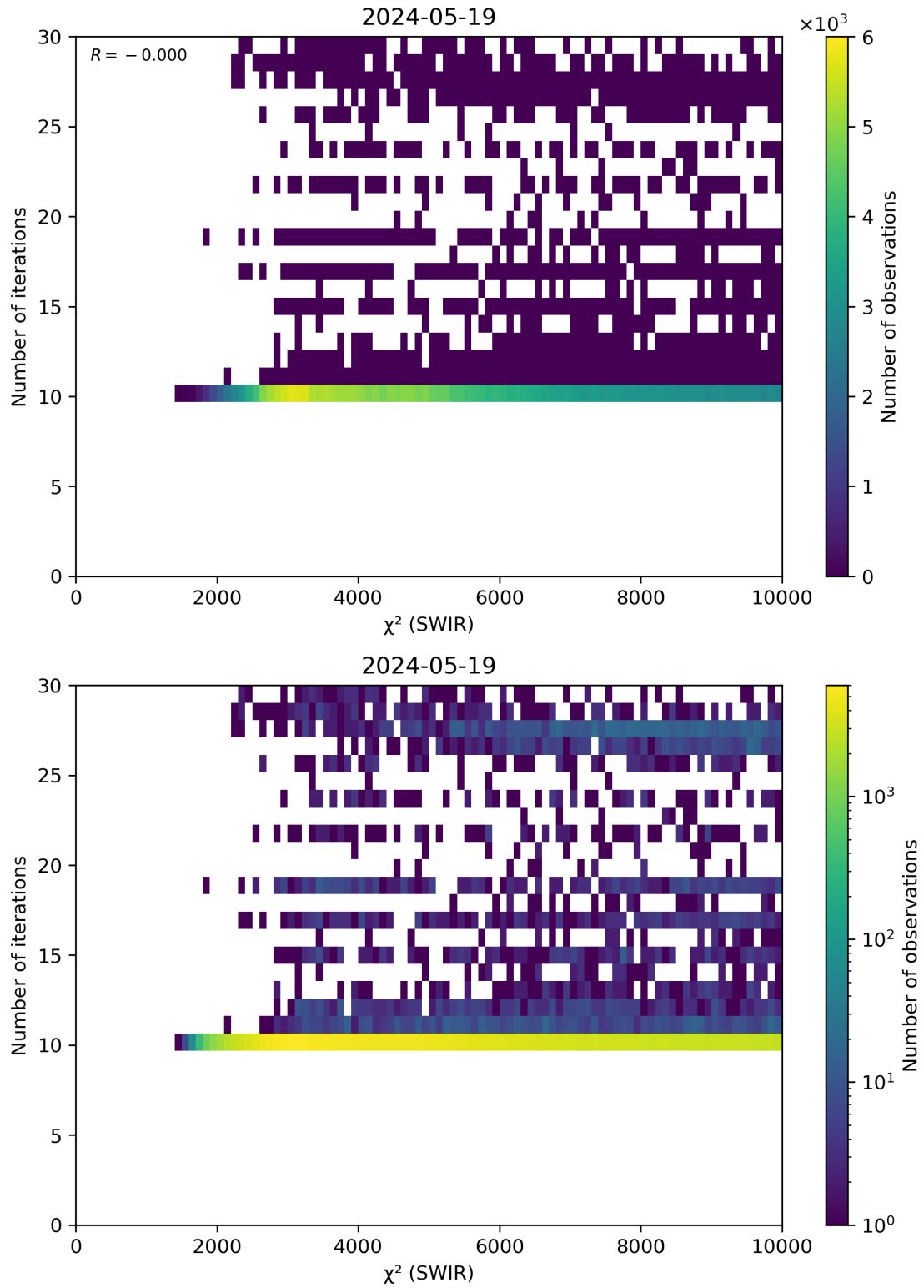
Figure 50: Scatter density plot of “ \chi^2 (SWIR)” against “Number of iterations” for 2024-05-18 to 2024-05-20.
