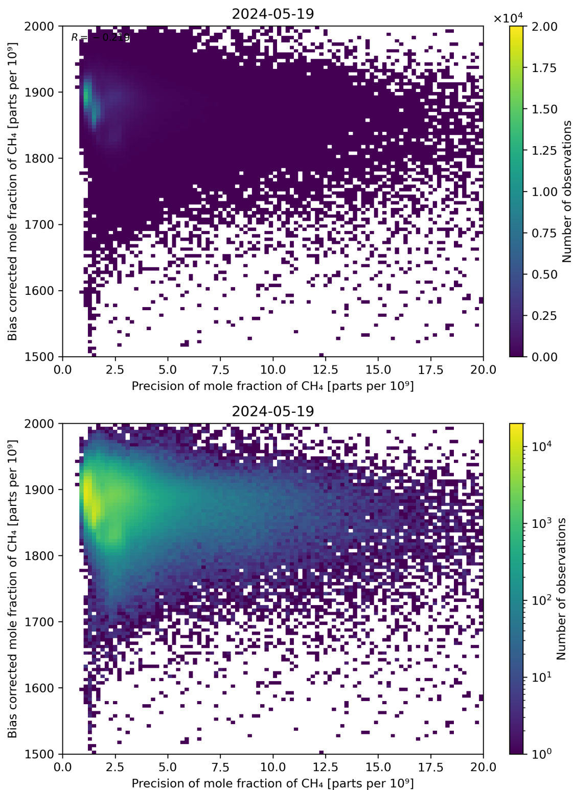
Figure 82: Scatter density plot of “Precision of mole fraction of CH 4 ” against “Bias corrected mole fraction of CH 4 ” for 2024-05-18 to 2024-05-20.
