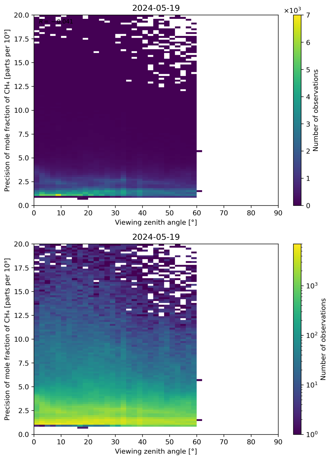
Figure 112: Scatter density plot of “Viewing zenith angle” against “Precision of mole fraction of CH 4 ” for 2024-05-18 to 2024-05-20.
