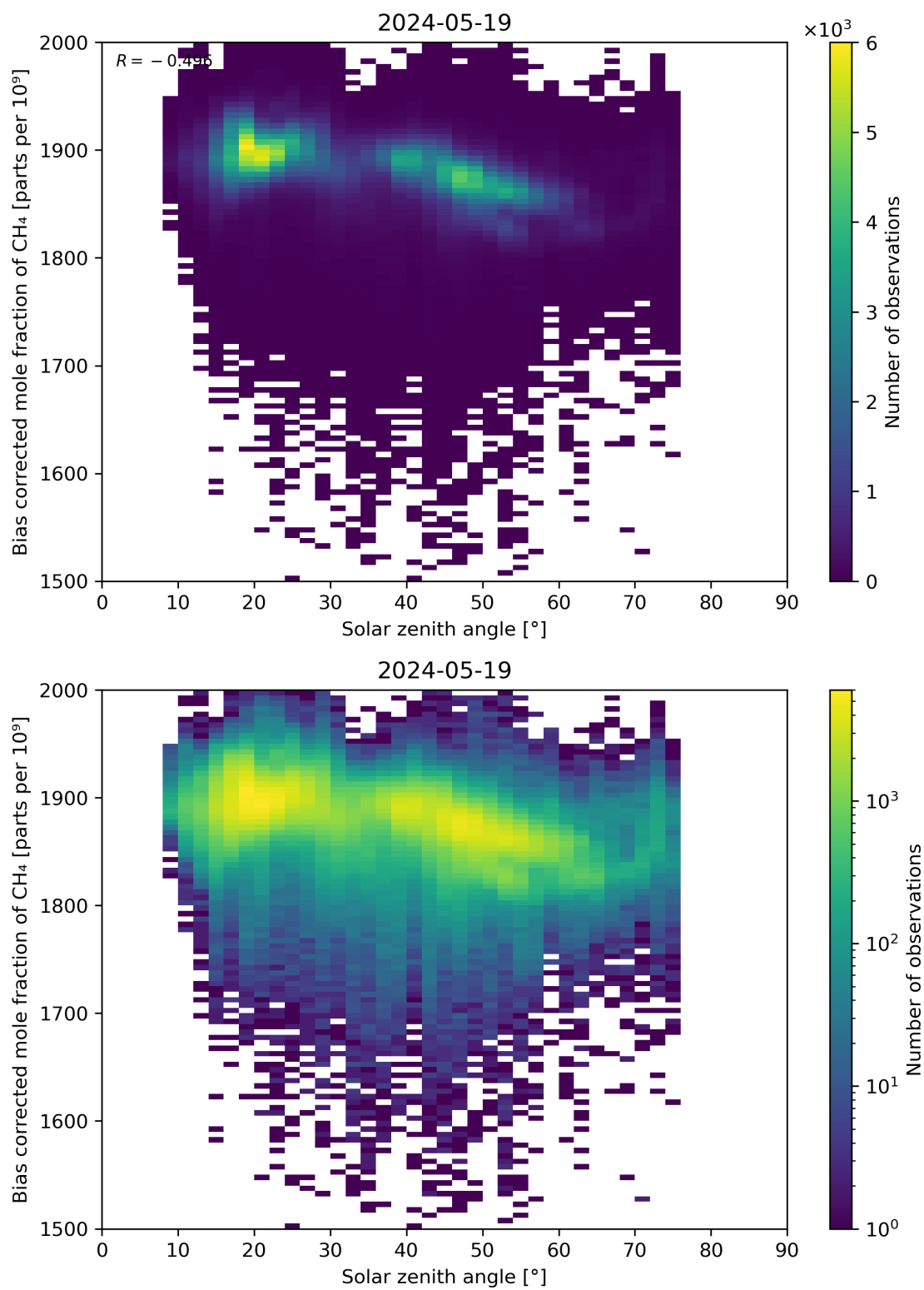
Figure 100: Scatter density plot of “Solar zenith angle” against “Bias corrected mole fraction of CH 4 ” for 2024-05-18 to 2024-05-20.
