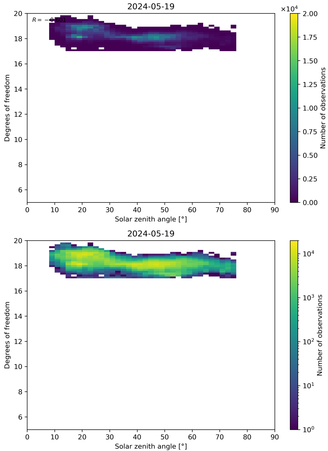
Figure 96: Scatter density plot of “Solar zenith angle” against “Degrees of freedom” for 2024-05-18 to 2024-05-20.
