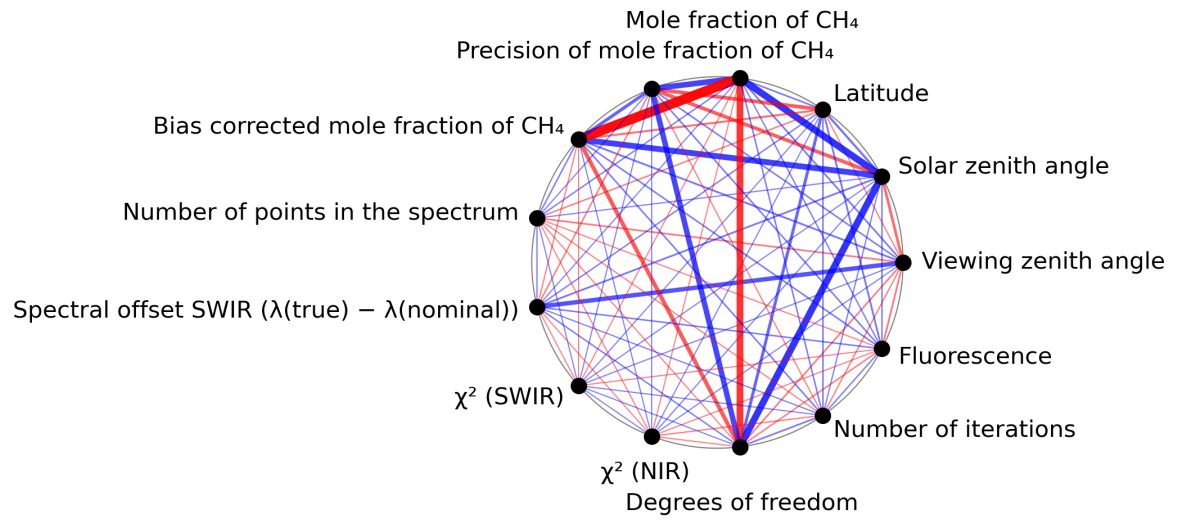
Figure 1: Map of correlation graph for 2024-05-18 to 2024-05-20.
