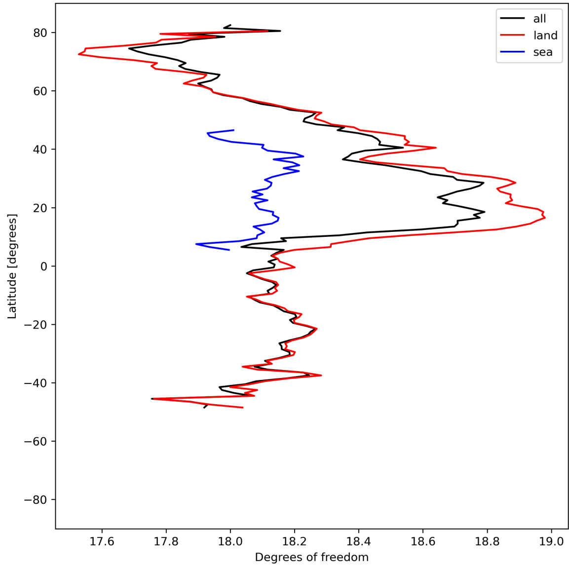
Figure 19: Zonal average of “Degrees of freedom” for 2024-05-18 to 2024-05-20.
