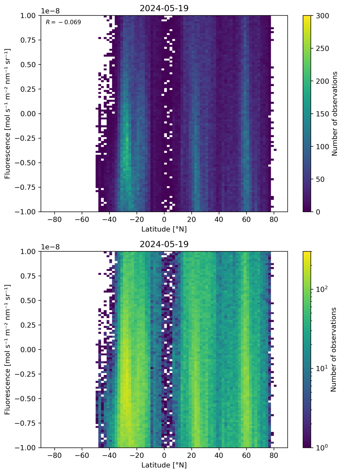
Figure 56: Scatter density plot of “Latitude” against “Fluorescence” for 2024-05-18 to 2024-05-20.
