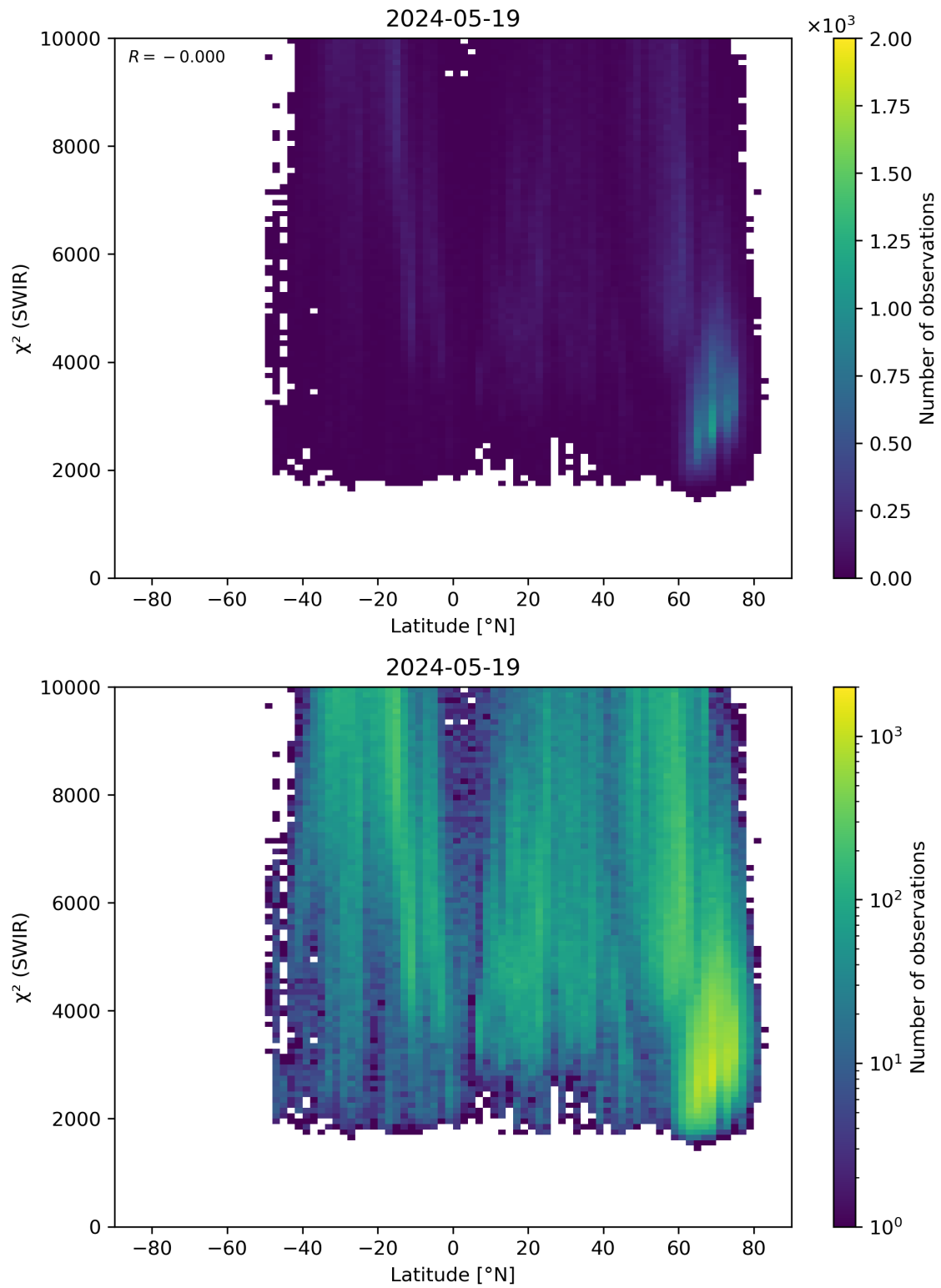
Figure 54: Scatter density plot of “Latitude” against “ \chi^2 (SWIR)” for 2024-05-18 to 2024-05-20.
