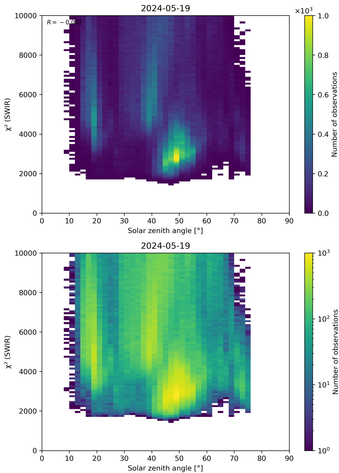
Figure 95: Scatter density plot of “Solar zenith angle” against “ \chi^2 (SWIR)” for 2024-05-18 to 2024-05-20.
