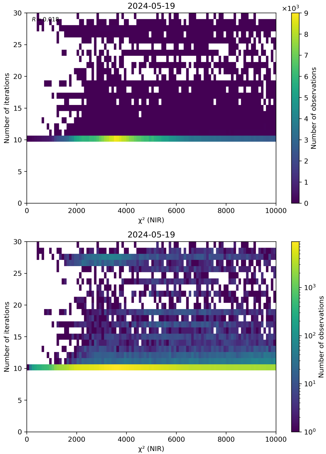
Figure 46: Scatter density plot of “ \chi^2 (NIR)” against “Number of iterations” for 2024-05-18 to 2024-05-20.
