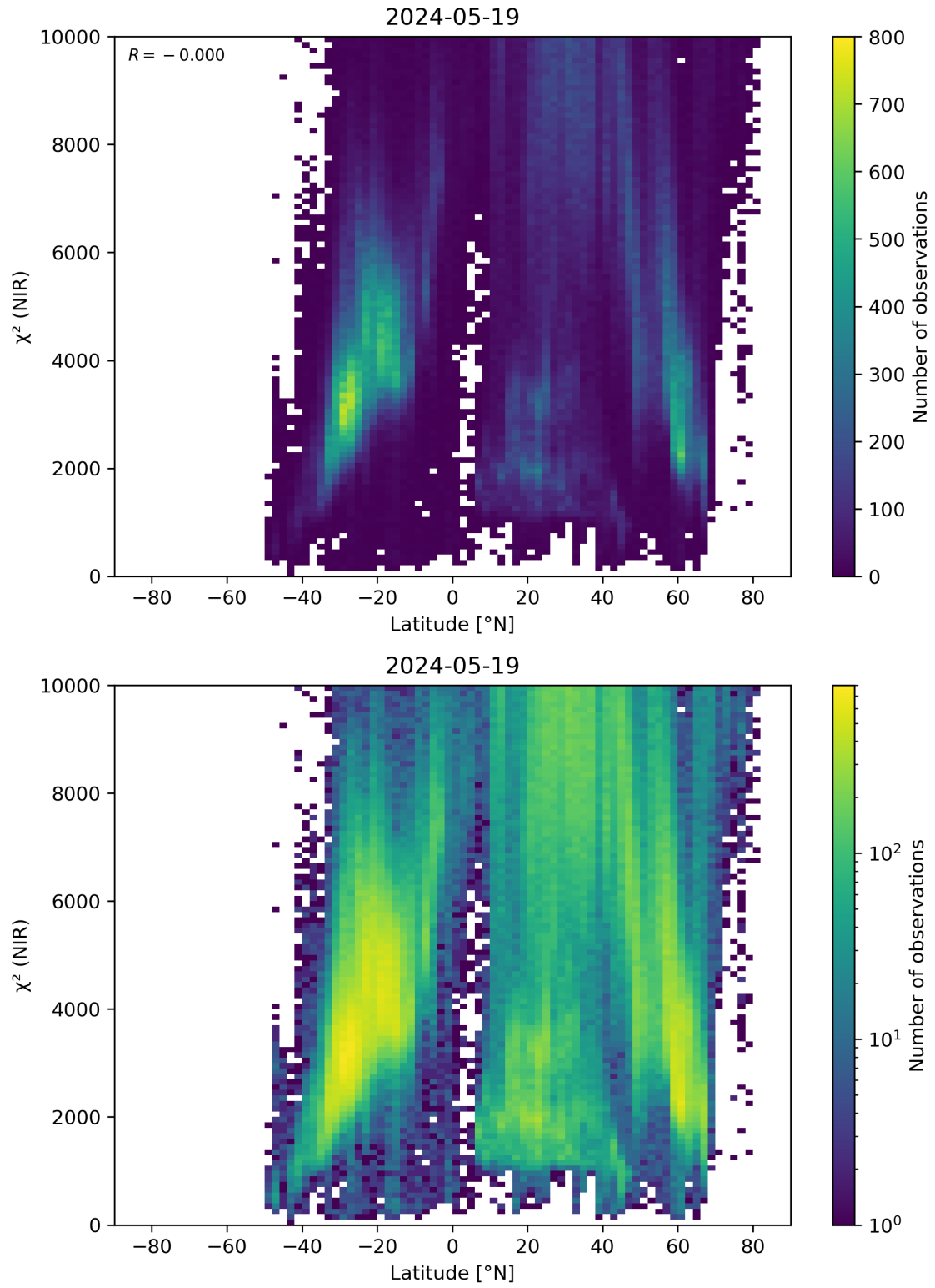
Figure 53: Scatter density plot of “Latitude” against “ \chi^2 (NIR)” for 2024-05-18 to 2024-05-20.
