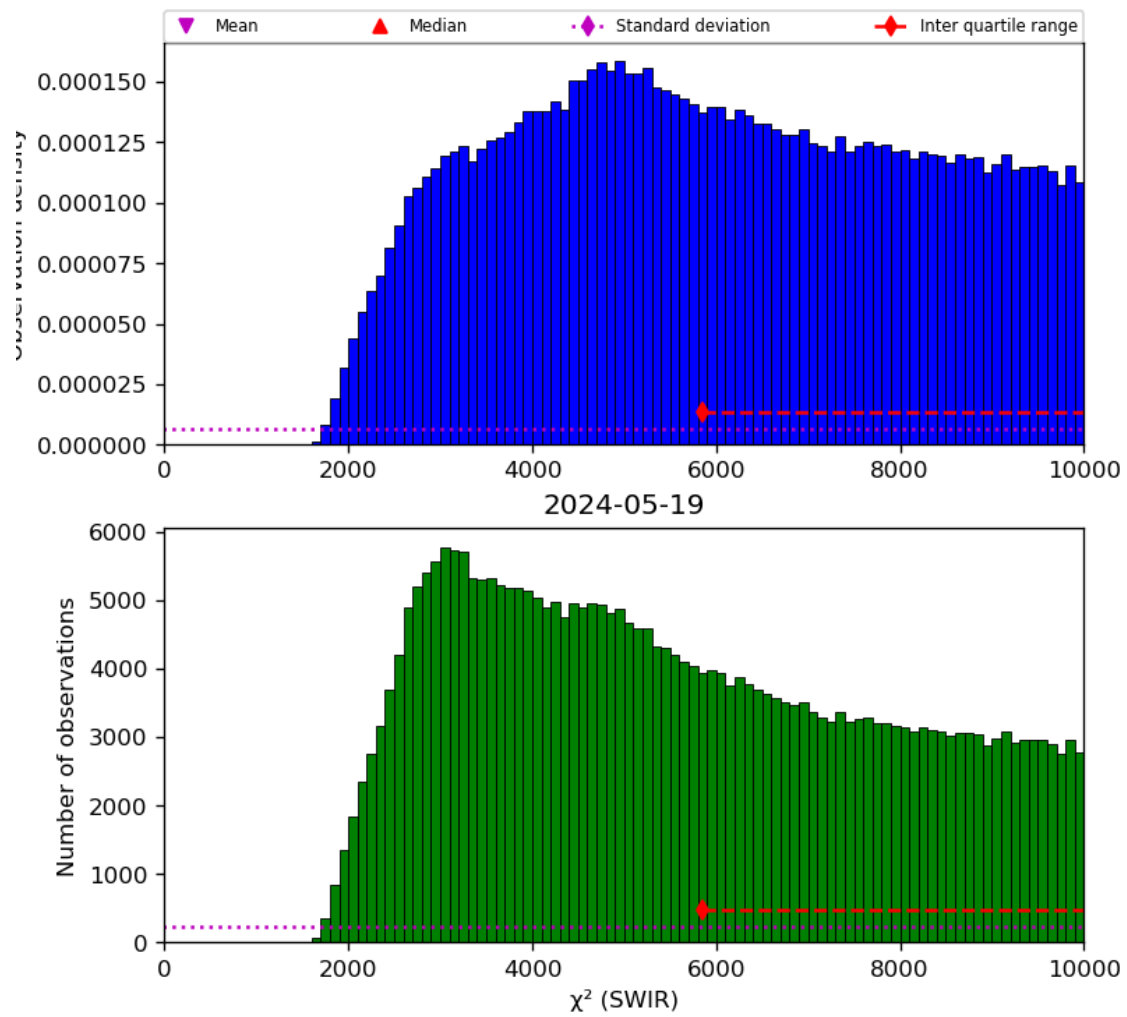
Figure 28: Histogram of “ \chi^2 (SWIR)” for 2024-05-18 to 2024-05-20
