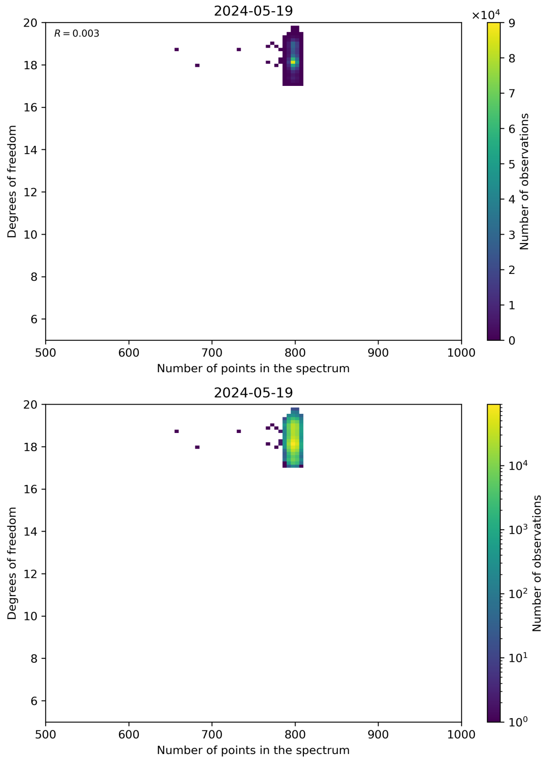
Figure 90: Scatter density plot of “Number of points in the spectrum” against “Degrees of freedom” for 2024-05-18 to 2024-05-20.
