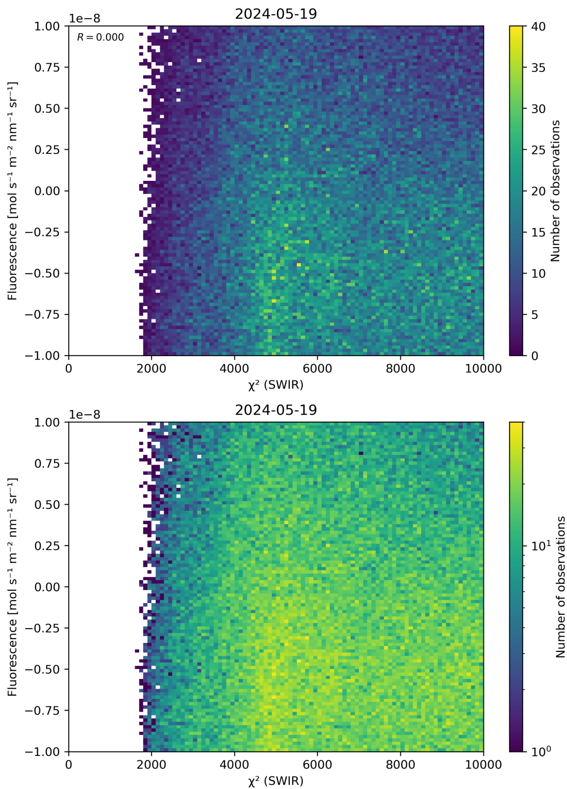
Figure 49: Scatter density plot of “ \chi^2 (SWIR)” against “Fluorescence” for 2024-05-18 to 2024-05-20.
