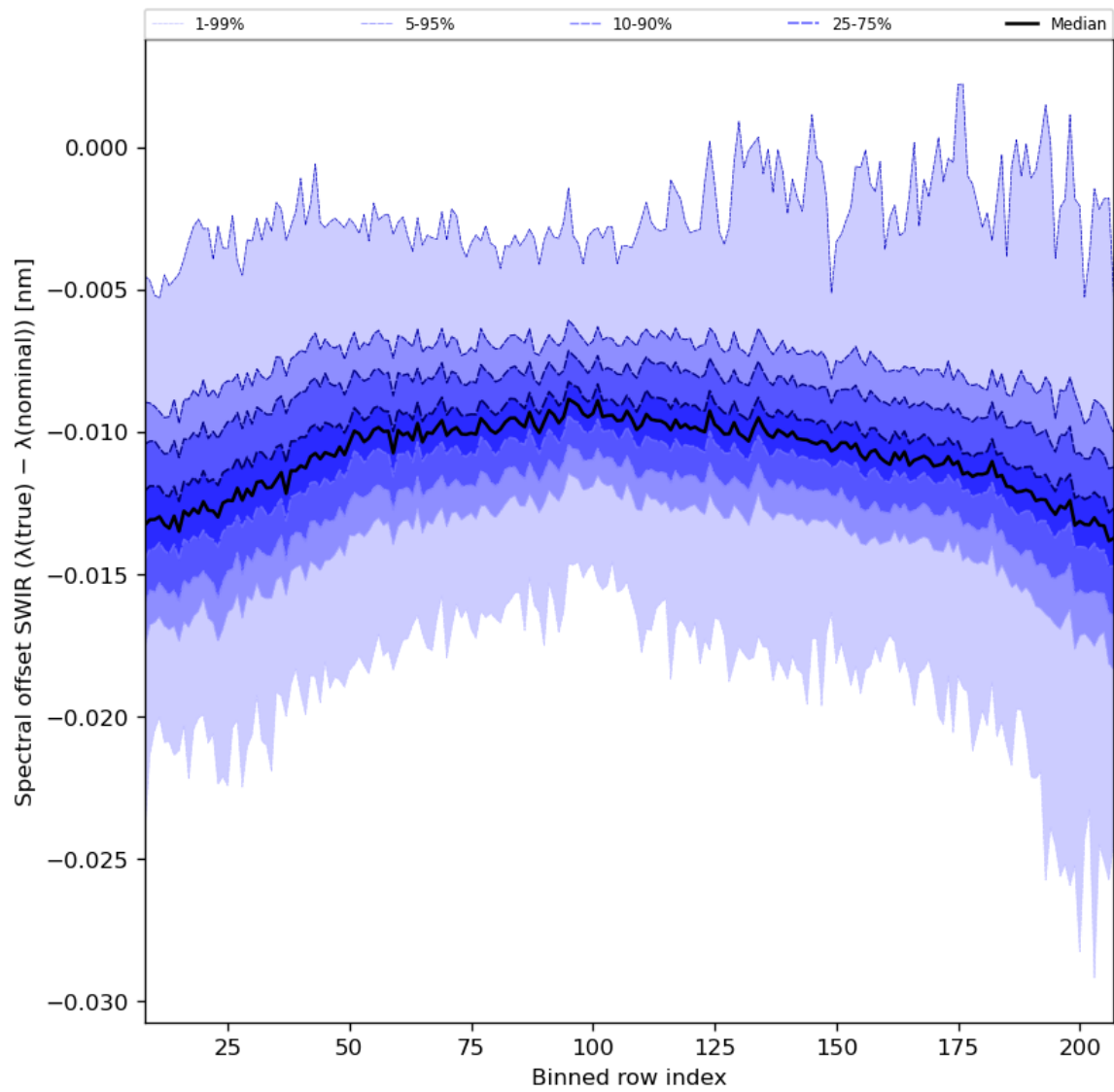
Figure 38: Along track statistics of “Spectral offset SWIR ( \lambda(\text{true}) - \lambda(\text{nominal}) )” for 2024-05-18 to 2024-05-20
