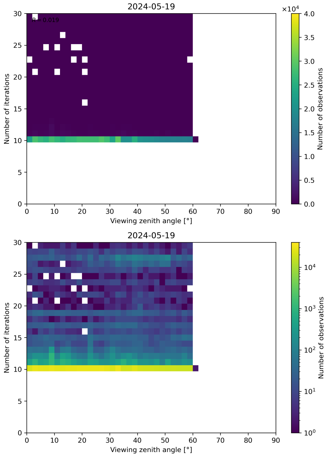
Figure 113: Scatter density plot of “Viewing zenith angle” against “Number of iterations” for 2024-05-18 to 2024-05-20.
