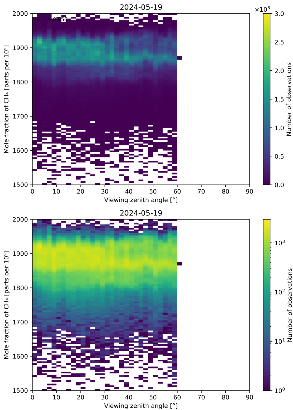
Figure 110: Scatter density plot of “Viewing zenith angle” against “Mole fraction of CH 4 ” for 2024-05-18 to 2024-05-20.
