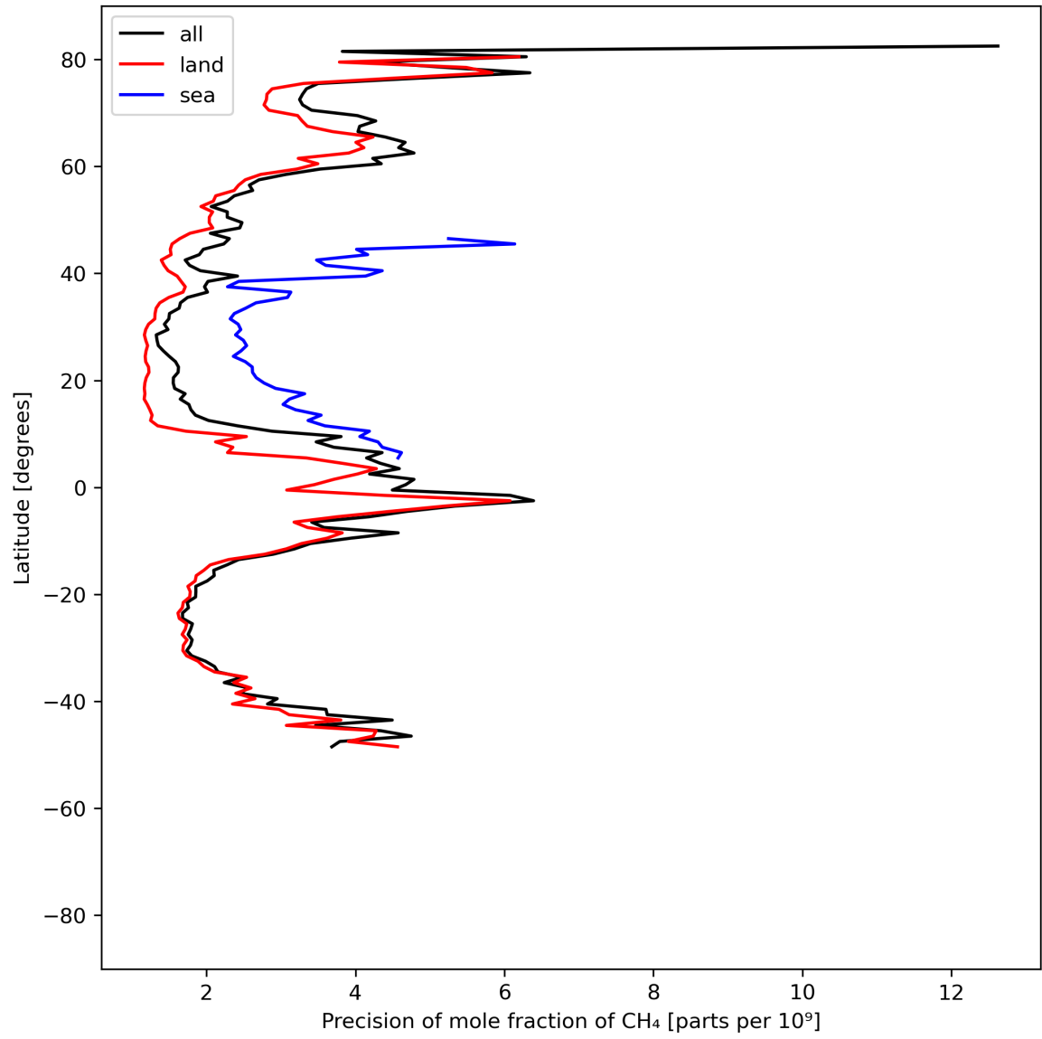
Figure 13: Zonal average of “Precision of mole fraction of \text{CH}_4 ” for 2024-05-18 to 2024-05-20.
