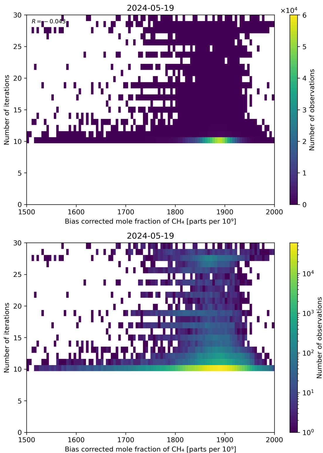
Figure 67: Scatter density plot of “Bias corrected mole fraction of \text{CH}_4 ” against “Number of iterations” for 2024-05-18 to 2024-05-20.
