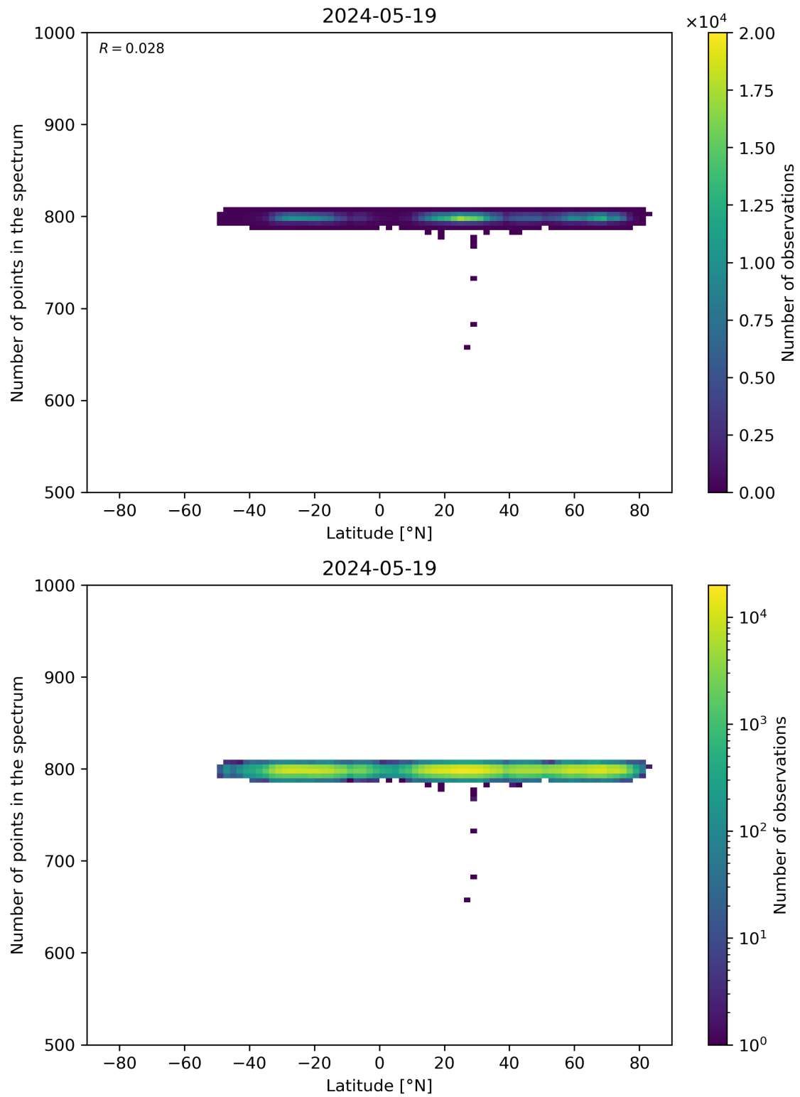
Figure 61: Scatter density plot of “Latitude” against “Number of points in the spectrum” for 2024-05-18 to 2024-05-20.
