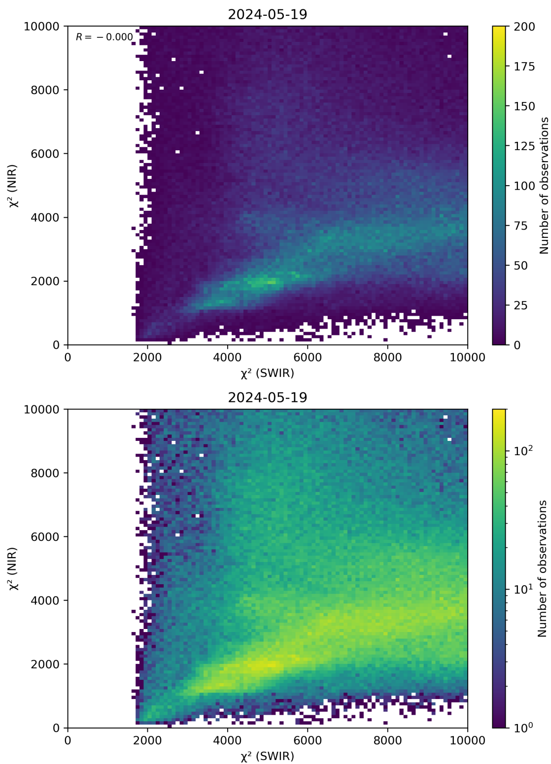
Figure 47: Scatter density plot of “ \chi^2 (SWIR)” against “ \chi^2 (NIR)” for 2024-05-18 to 2024-05-20.
