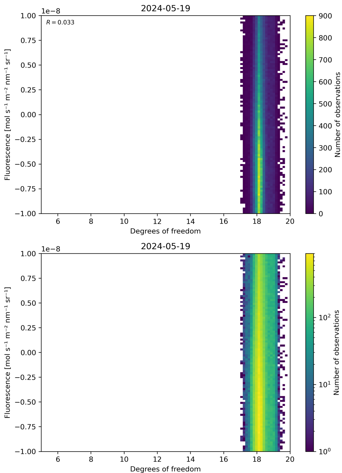
Figure 51: Scatter density plot of “Degrees of freedom” against “Fluorescence” for 2024-05-18 to 2024-05-20.
