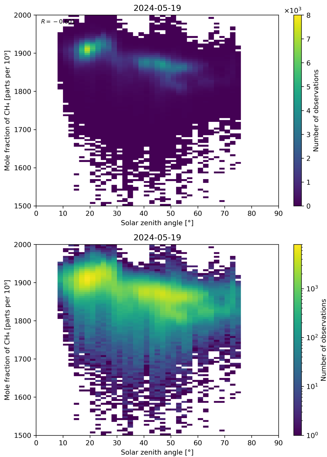
Figure 99: Scatter density plot of “Solar zenith angle” against “Mole fraction of \text{CH}_4 ” for 2024-05-18 to 2024-05-20.
