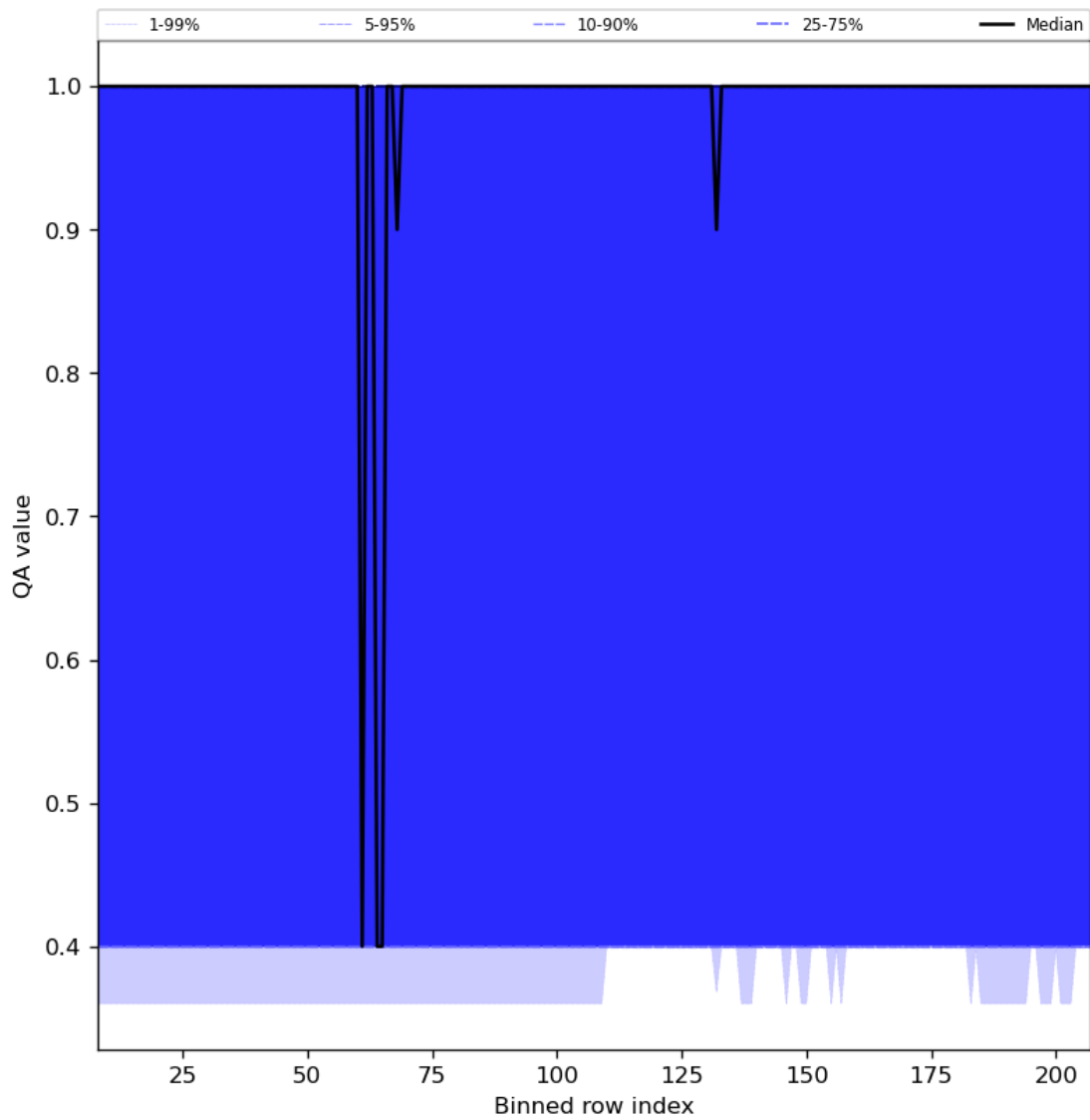
Figure 33: Along track statistics of “QA value” for 2024-05-18 to 2024-05-20
