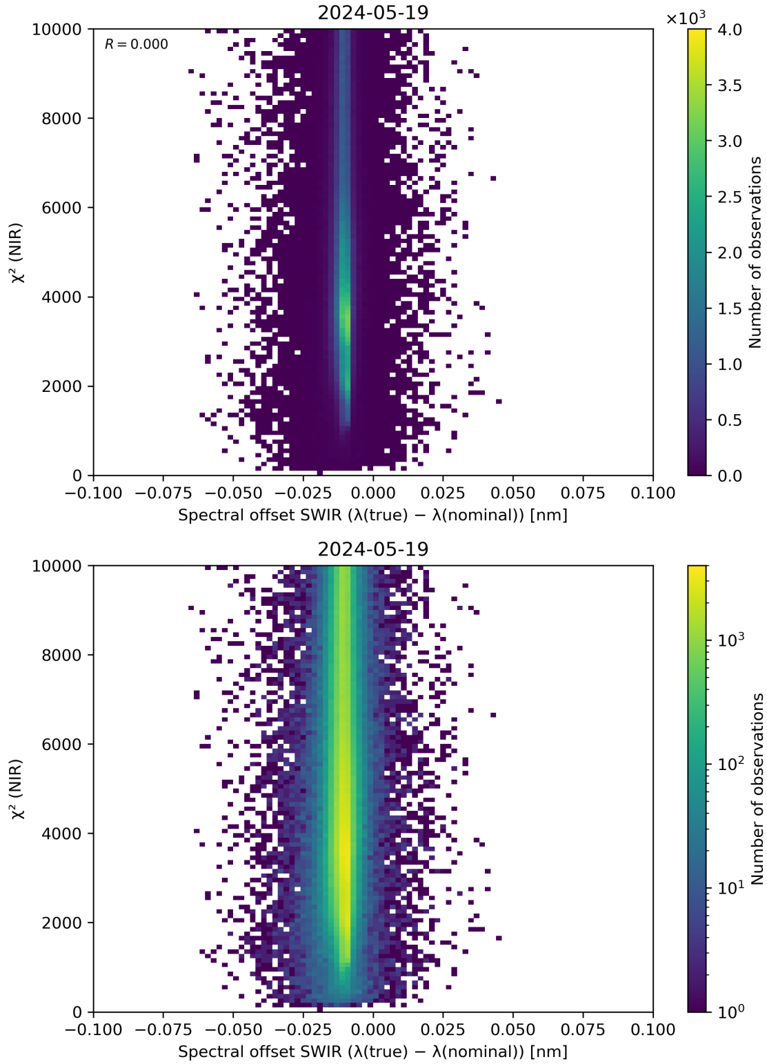
Figure 117: Scatter density plot of “Spectral offset SWIR ( \lambda(\text{true}) - \lambda(\text{nominal}) )” against “ \chi^2 (NIR)” for 2024-05-18 to 2024-05-20.
