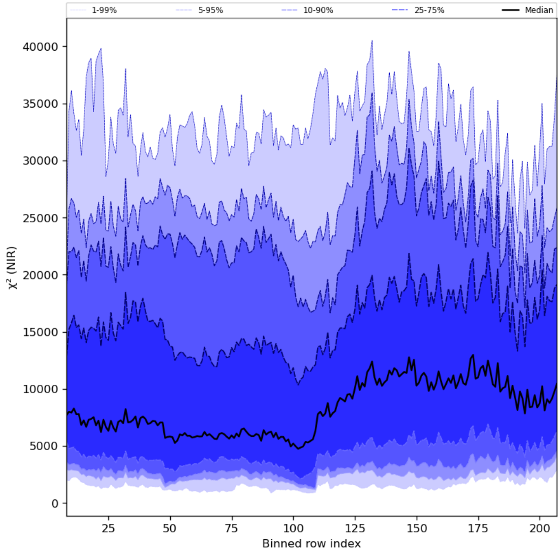
Figure 40: Along track statistics of “ \chi^2 (NIR)” for 2024-05-18 to 2024-05-20
