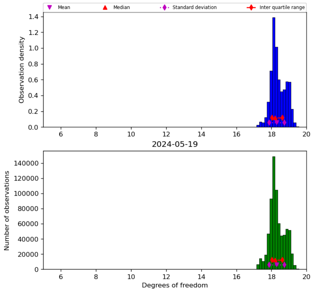
Figure 30: Histogram of “Degrees of freedom” for 2024-05-18 to 2024-05-20
