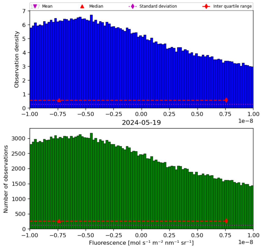
Figure 32: Histogram of “Fluorescence” for 2024-05-18 to 2024-05-20
