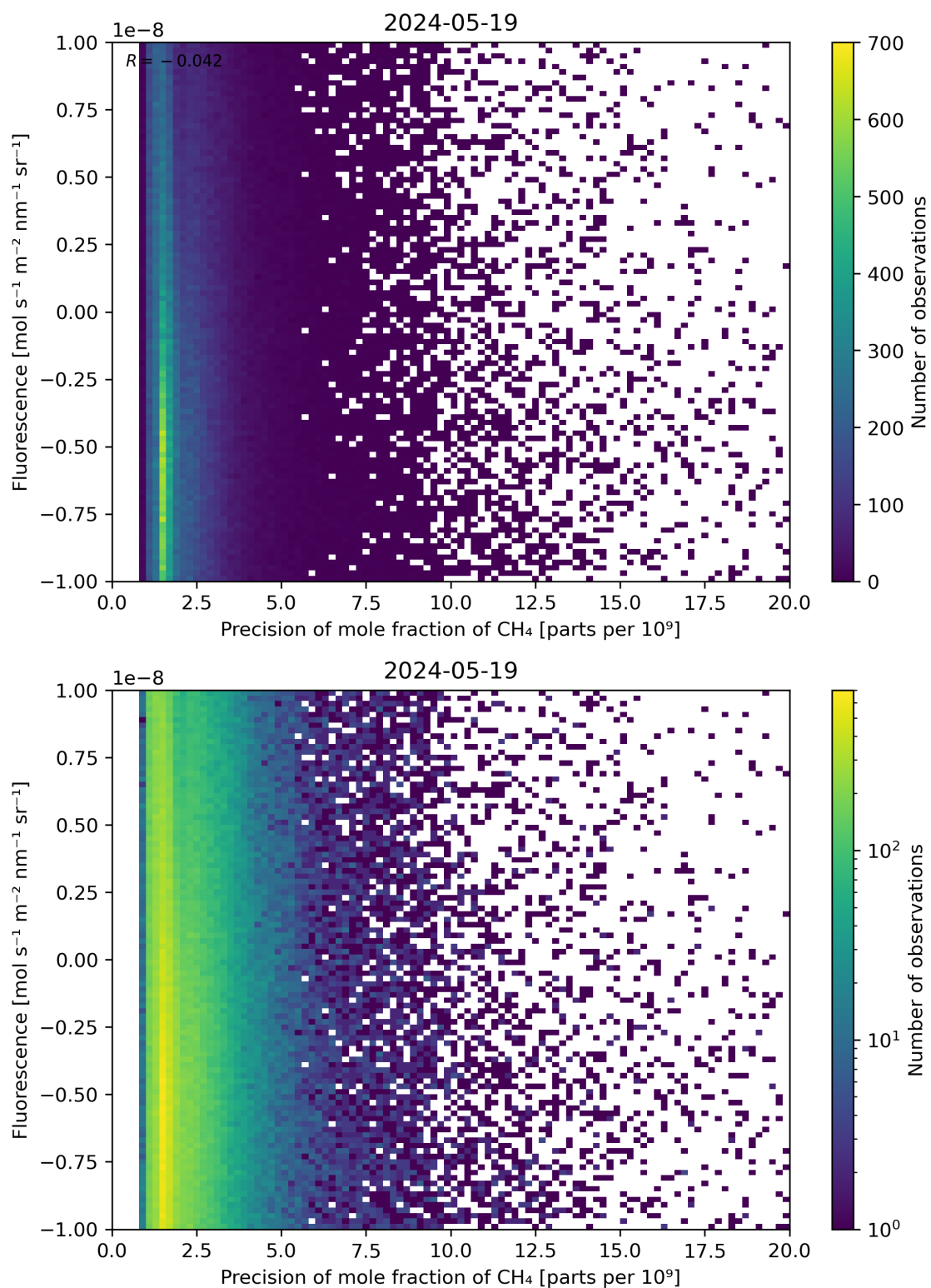
Figure 81: Scatter density plot of “Precision of mole fraction of \text{CH}_4 ” against “Fluorescence” for 2024-05-18 to 2024-05-20.
