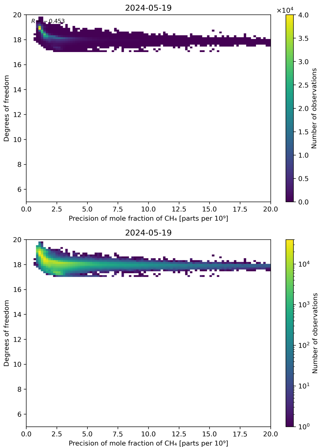
Figure 80: Scatter density plot of “Precision of mole fraction of CH 4 ” against “Degrees of freedom” for 2024-05-18 to 2024-05-20.
