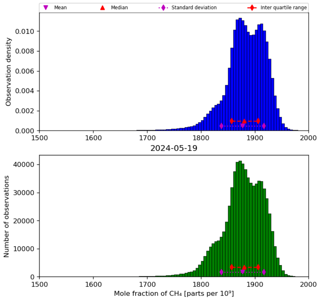
Figure 23: Histogram of “Mole fraction of CH 4 ” for 2024-05-18 to 2024-05-20
