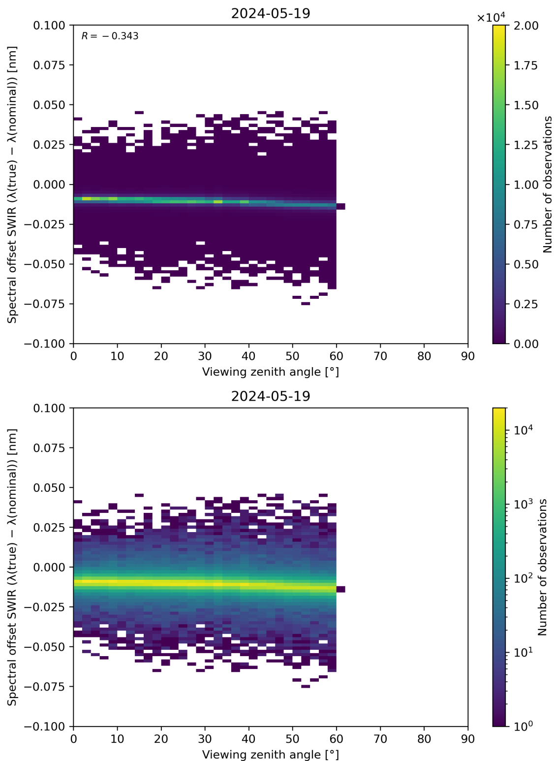
Figure 116: Scatter density plot of “Viewing zenith angle” against “Spectral offset SWIR ( \lambda(\text{true}) - \lambda(\text{nominal}) )” for 2024-05-18 to 2024-05-20.
