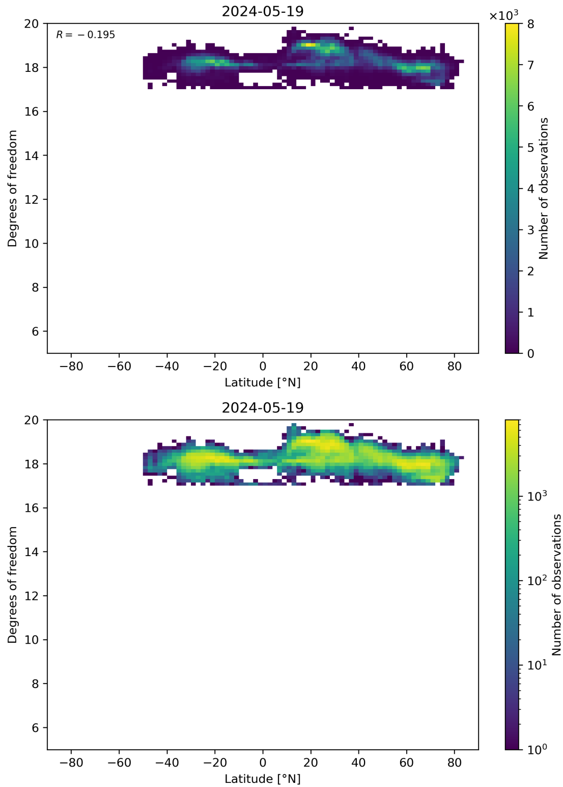
Figure 55: Scatter density plot of “Latitude” against “Degrees of freedom” for 2024-05-18 to 2024-05-20.
