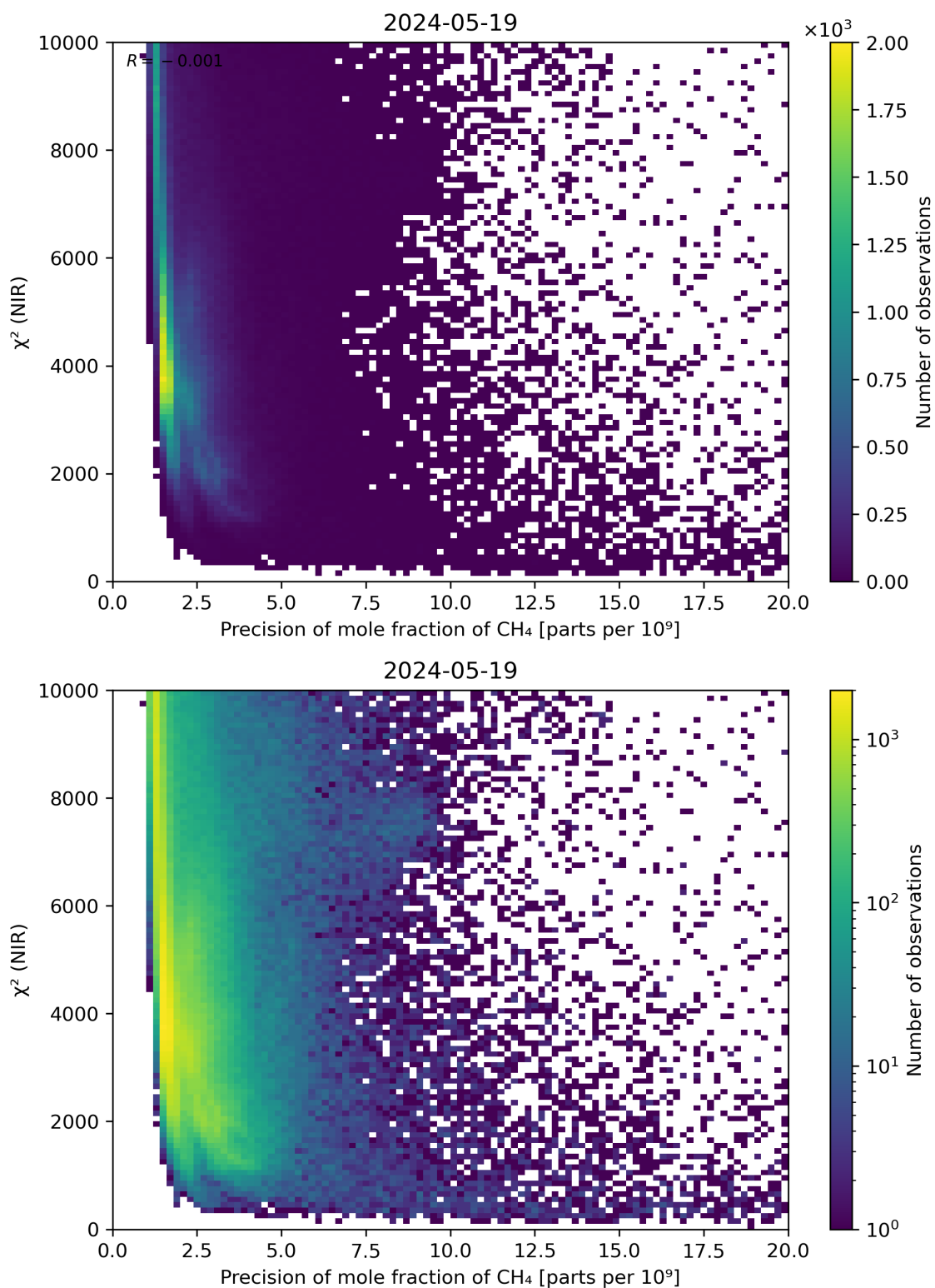
Figure 78: Scatter density plot of “Precision of mole fraction of \text{CH}_4 ” against “ \chi^2 (NIR)” for 2024-05-18 to 2024-05-20.
