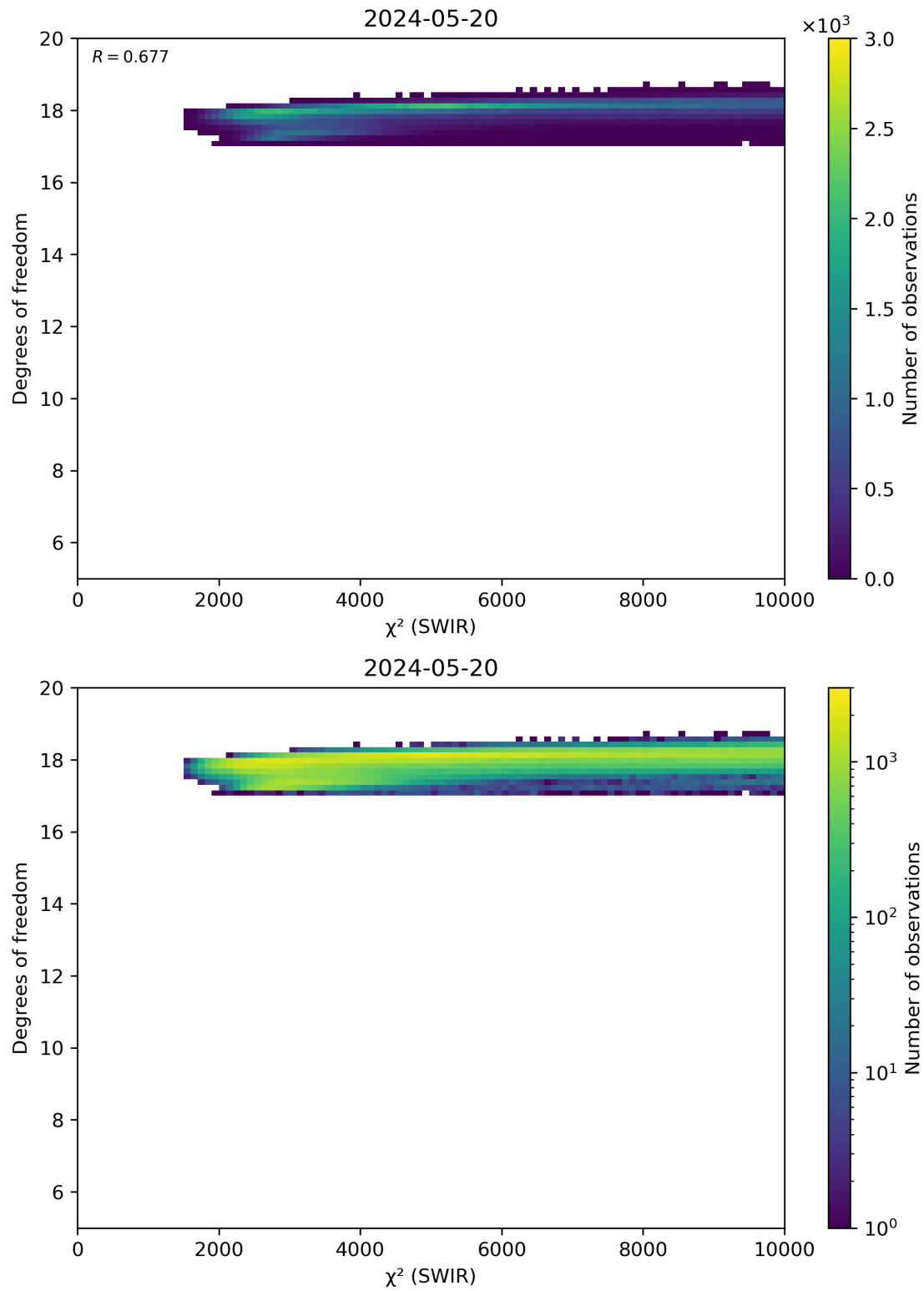
Figure 48: Scatter density plot of “ \chi^2 (SWIR)” against “Degrees of freedom” for 2024-05-19 to 2024-05-21.
