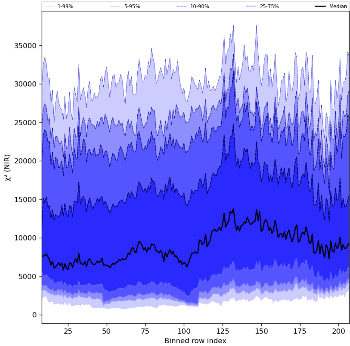
Figure 40: Along track statistics of “ \chi^2 (NIR)” for 2024-05-19 to 2024-05-21
