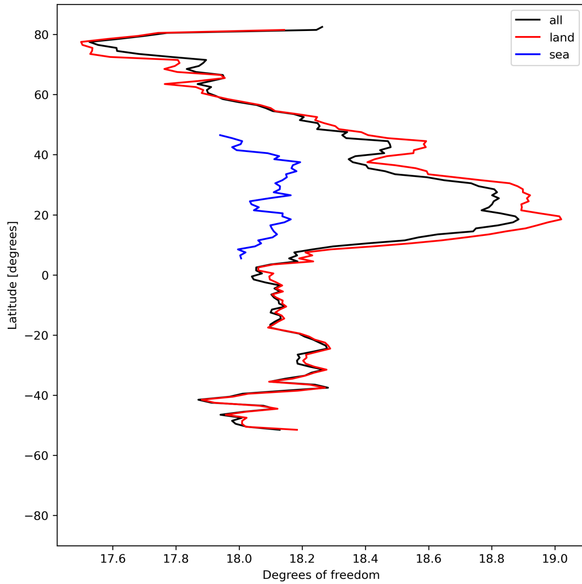
Figure 19: Zonal average of “Degrees of freedom” for 2024-05-19 to 2024-05-21.
