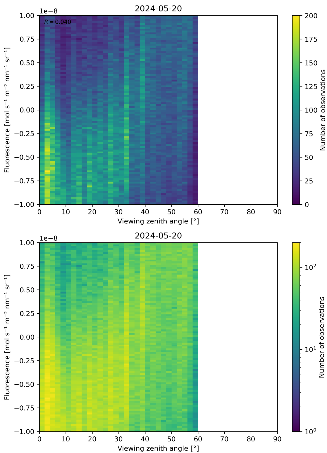
Figure 108: Scatter density plot of “Viewing zenith angle” against “Fluorescence” for 2024-05-19 to 2024-05-21.
