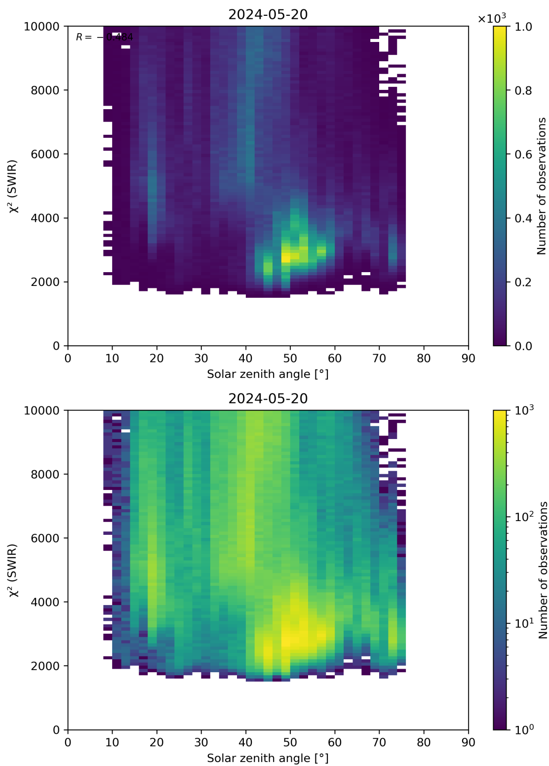
Figure 95: Scatter density plot of “Solar zenith angle” against “ \chi^2 (SWIR)” for 2024-05-19 to 2024-05-21.
