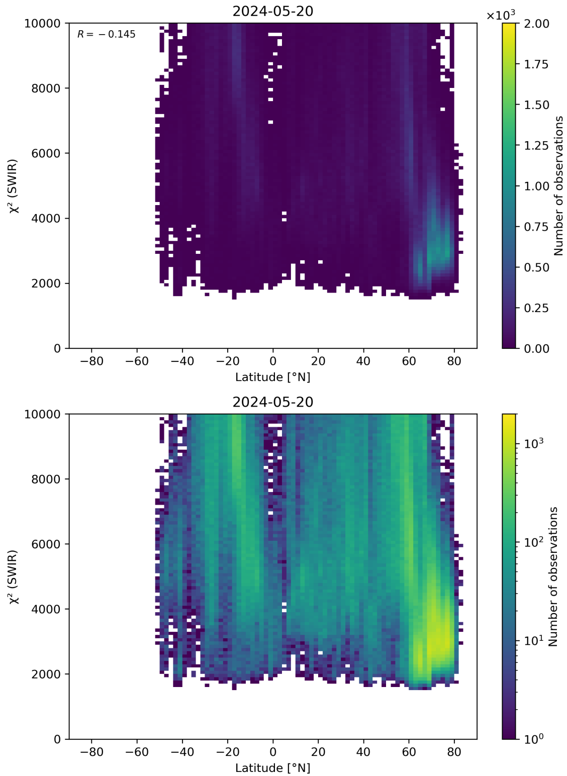
Figure 54: Scatter density plot of “Latitude” against “ \chi^2 (SWIR)” for 2024-05-19 to 2024-05-21.
