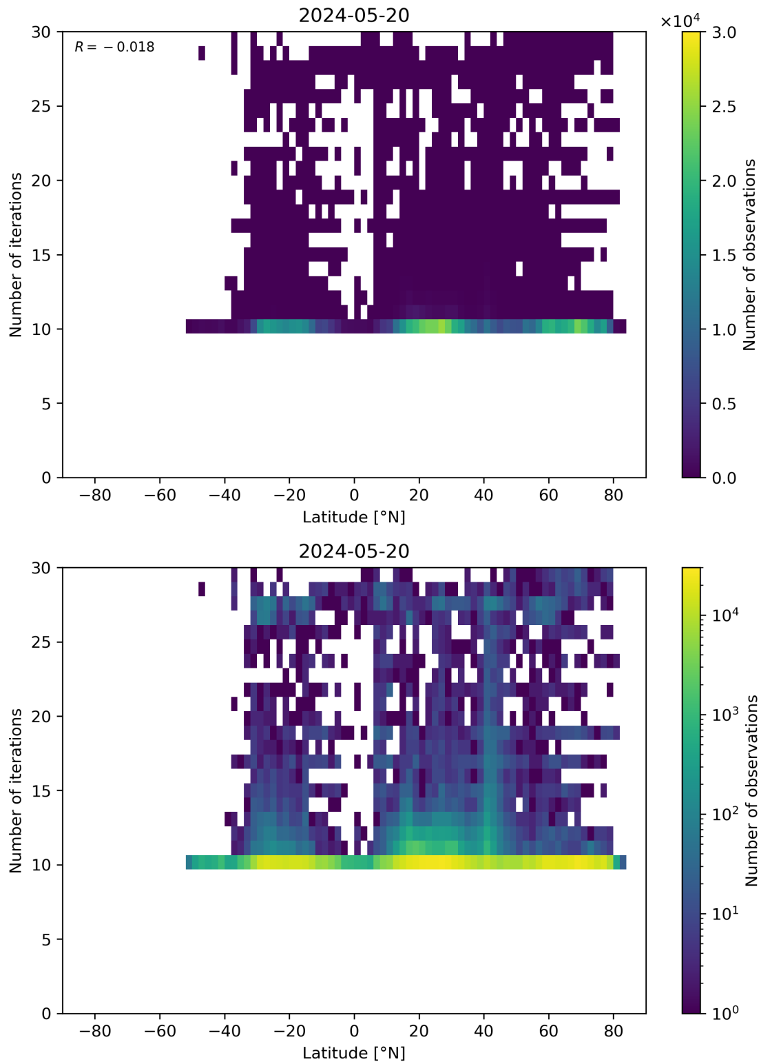
Figure 60: Scatter density plot of “Latitude” against “Number of iterations” for 2024-05-19 to 2024-05-21.
