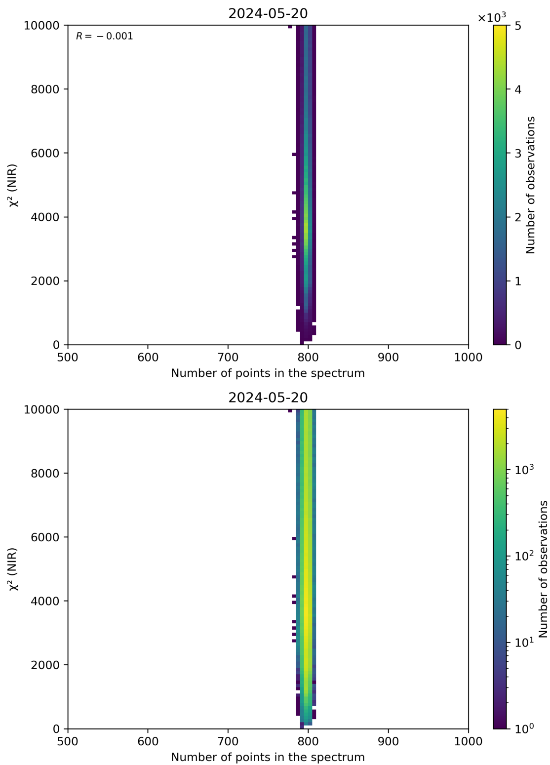
Figure 88: Scatter density plot of “Number of points in the spectrum” against “ \chi^2 (NIR)” for 2024-05-19 to 2024-05-21.
