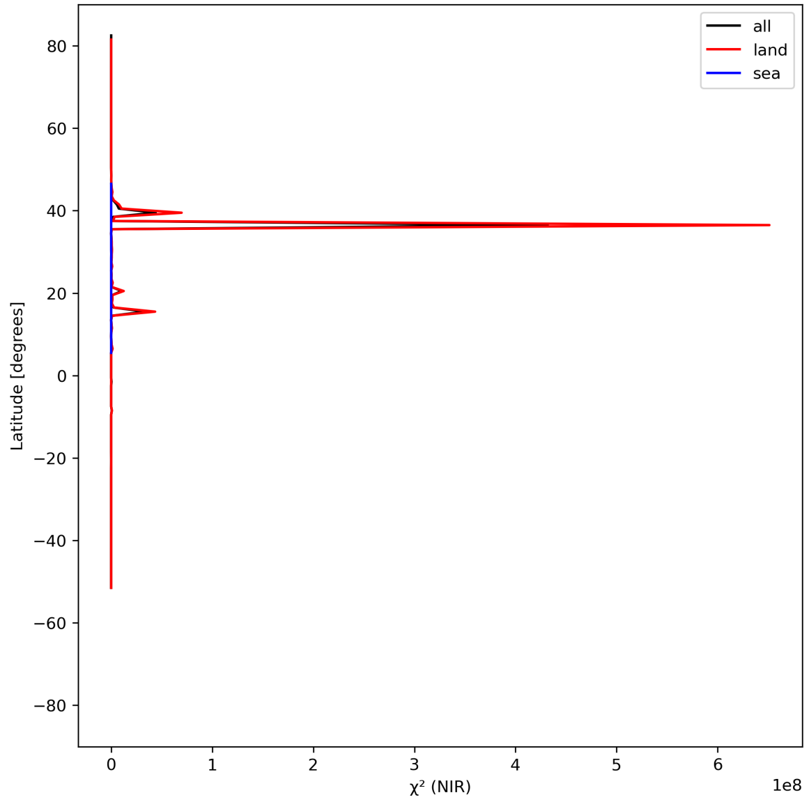
Figure 18: Zonal average of “ \chi^2 (NIR)” for 2024-05-19 to 2024-05-21.
