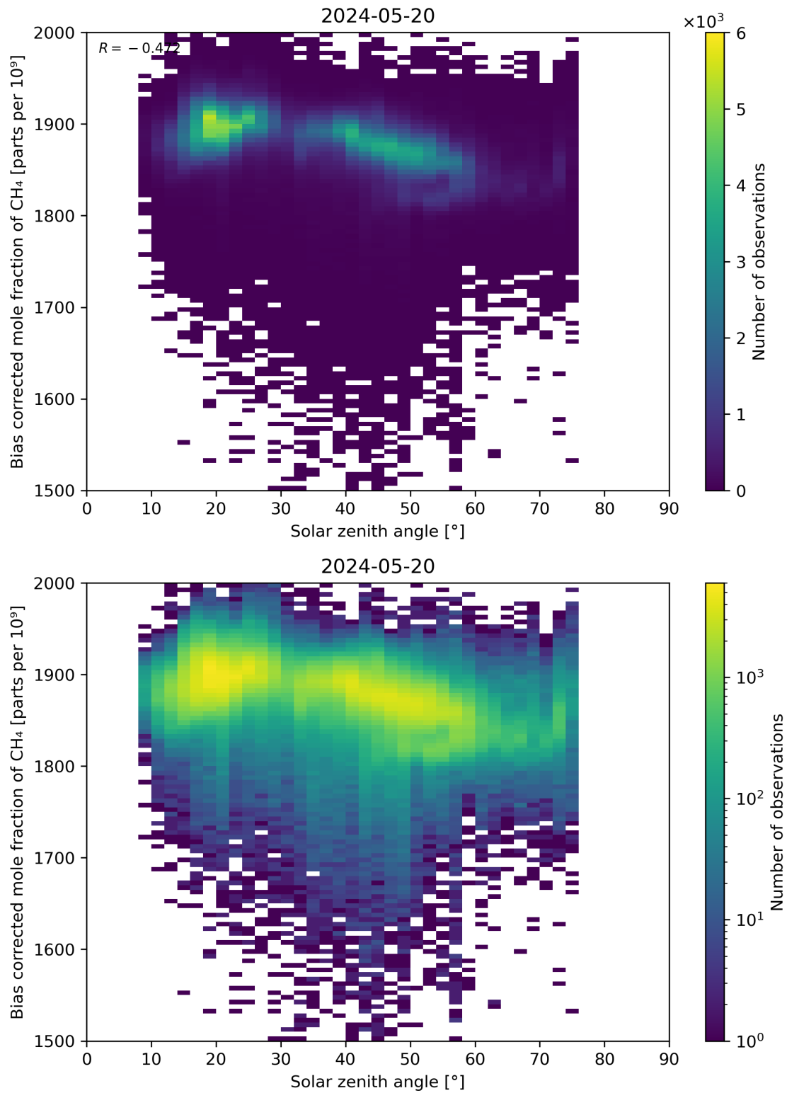
Figure 100: Scatter density plot of “Solar zenith angle” against “Bias corrected mole fraction of CH 4 ” for 2024-05-19 to 2024-05-21.
