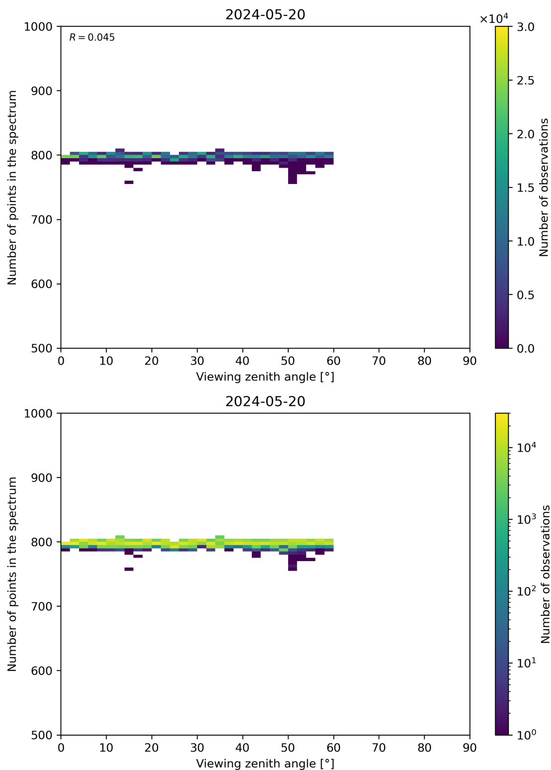
Figure 114: Scatter density plot of “Viewing zenith angle” against “Number of points in the spectrum” for 2024-05-19 to 2024-05-21.
