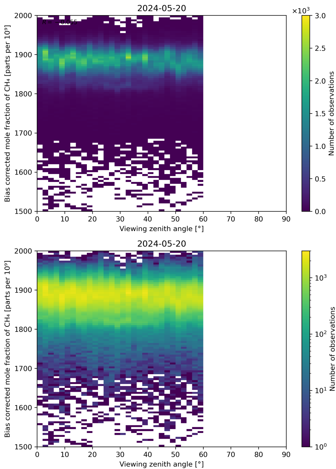
Figure 111: Scatter density plot of “Viewing zenith angle” against “Bias corrected mole fraction of CH 4 ” for 2024-05-19 to 2024-05-21.
