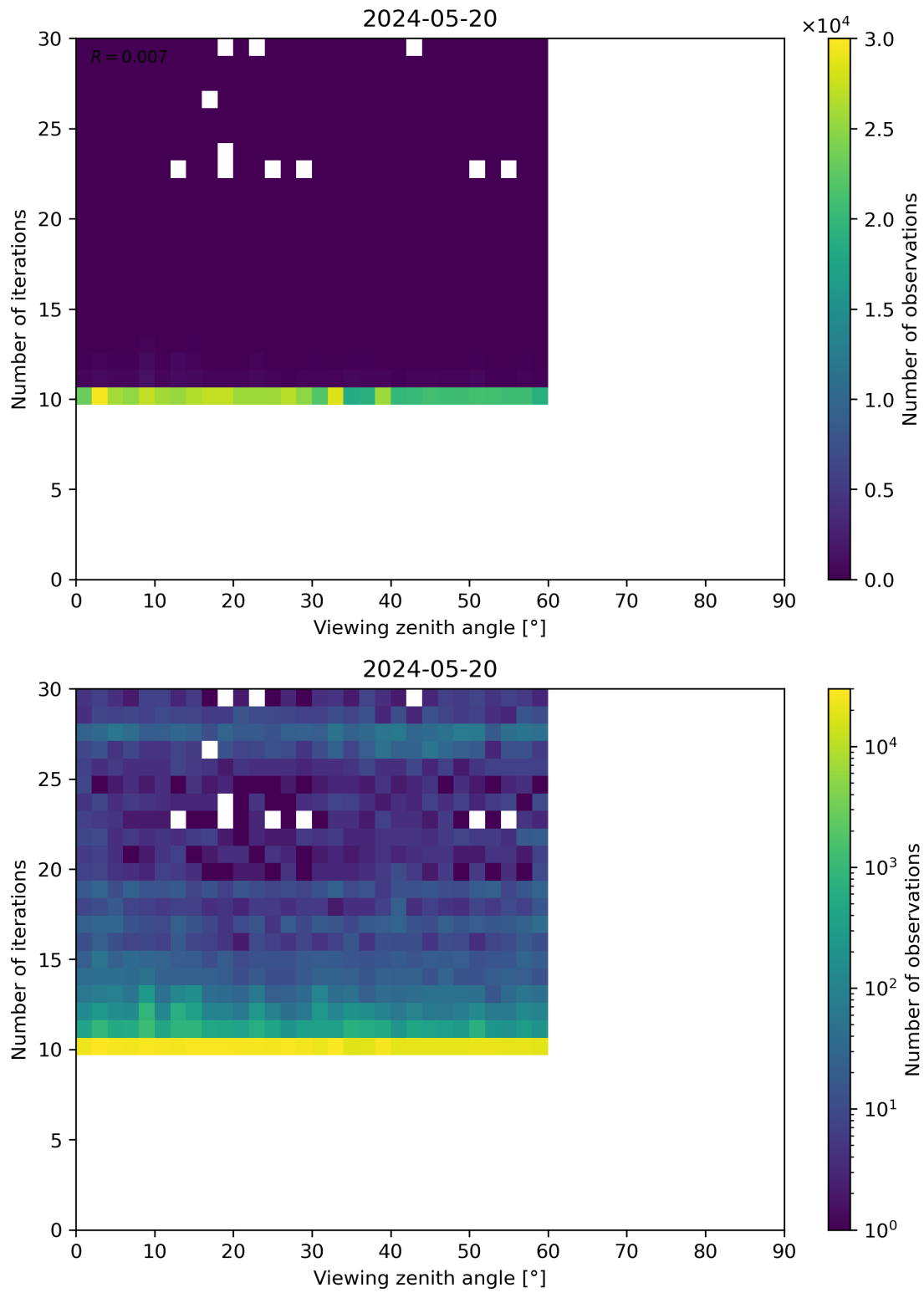
Figure 113: Scatter density plot of “Viewing zenith angle” against “Number of iterations” for 2024-05-19 to 2024-05-21.
