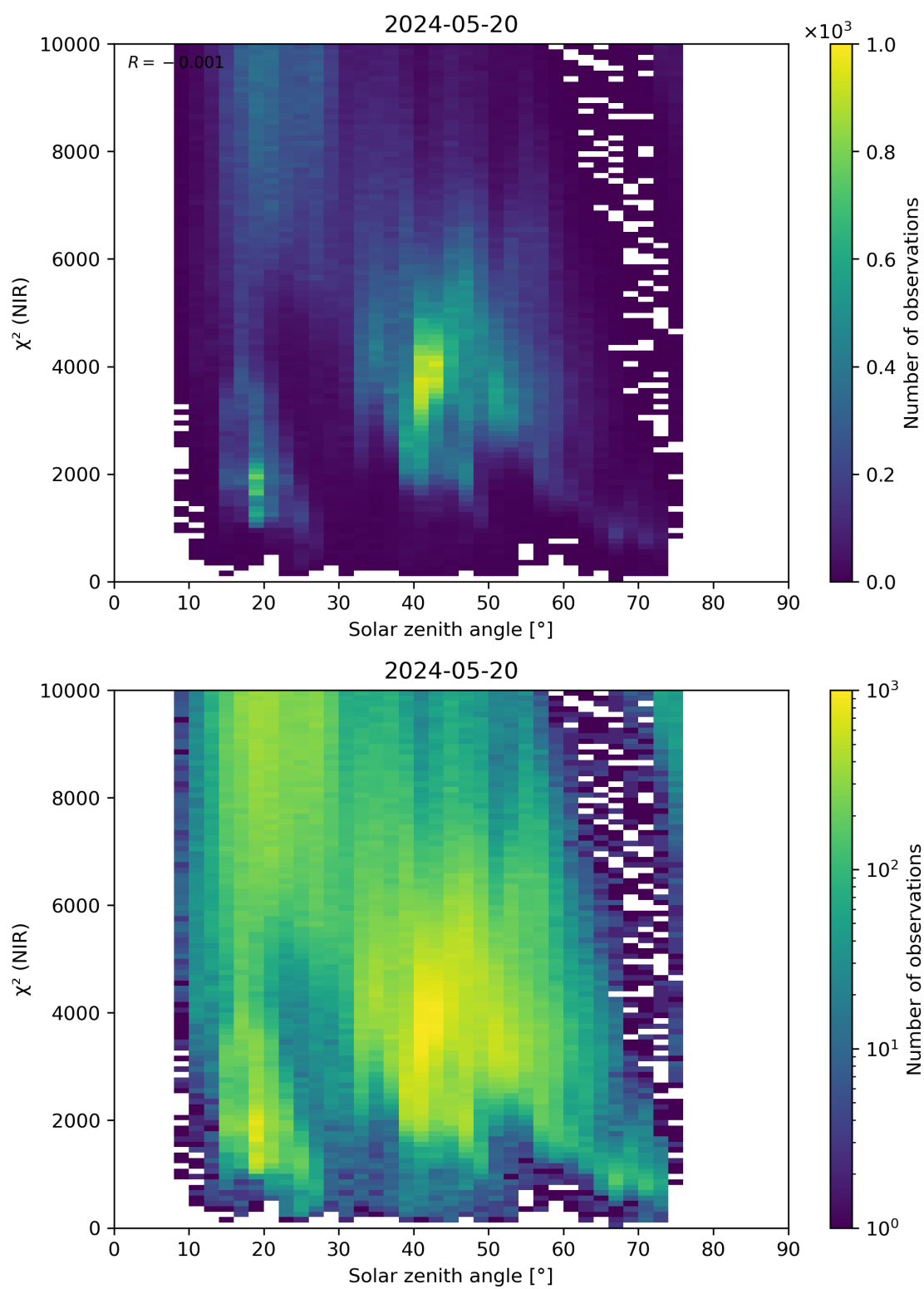
Figure 94: Scatter density plot of “Solar zenith angle” against “ \chi^2 (NIR)” for 2024-05-19 to 2024-05-21.
