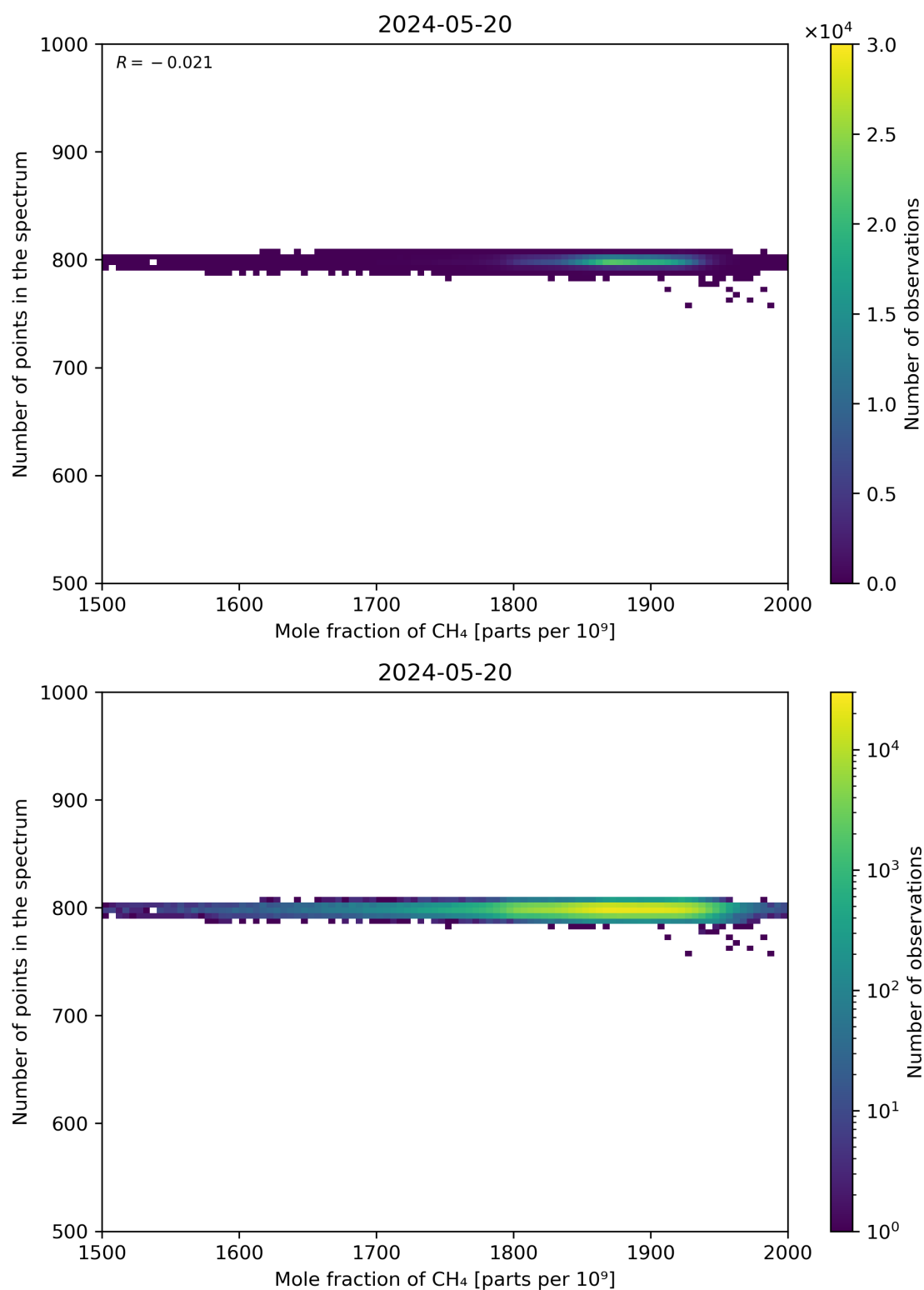
Figure 77: Scatter density plot of “Mole fraction of CH 4 ” against “Number of points in the spectrum” for 2024-05-19 to 2024-05-21.
