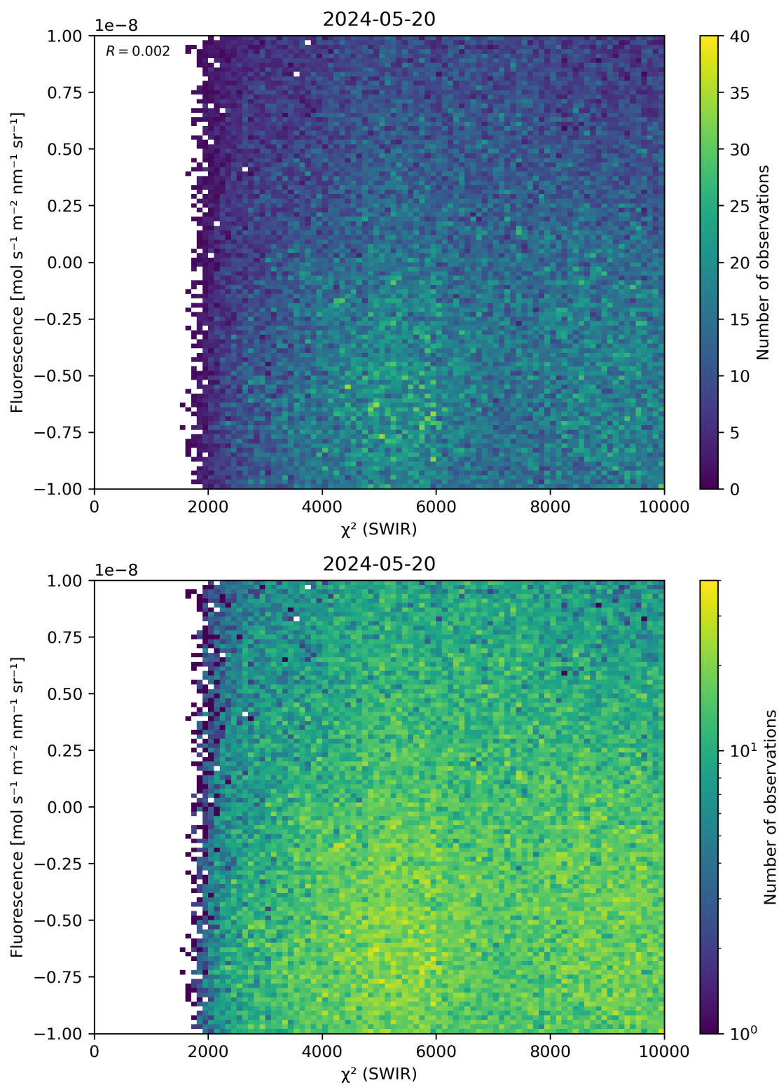
Figure 49: Scatter density plot of “ \chi^2 (SWIR)” against “Fluorescence” for 2024-05-19 to 2024-05-21.
