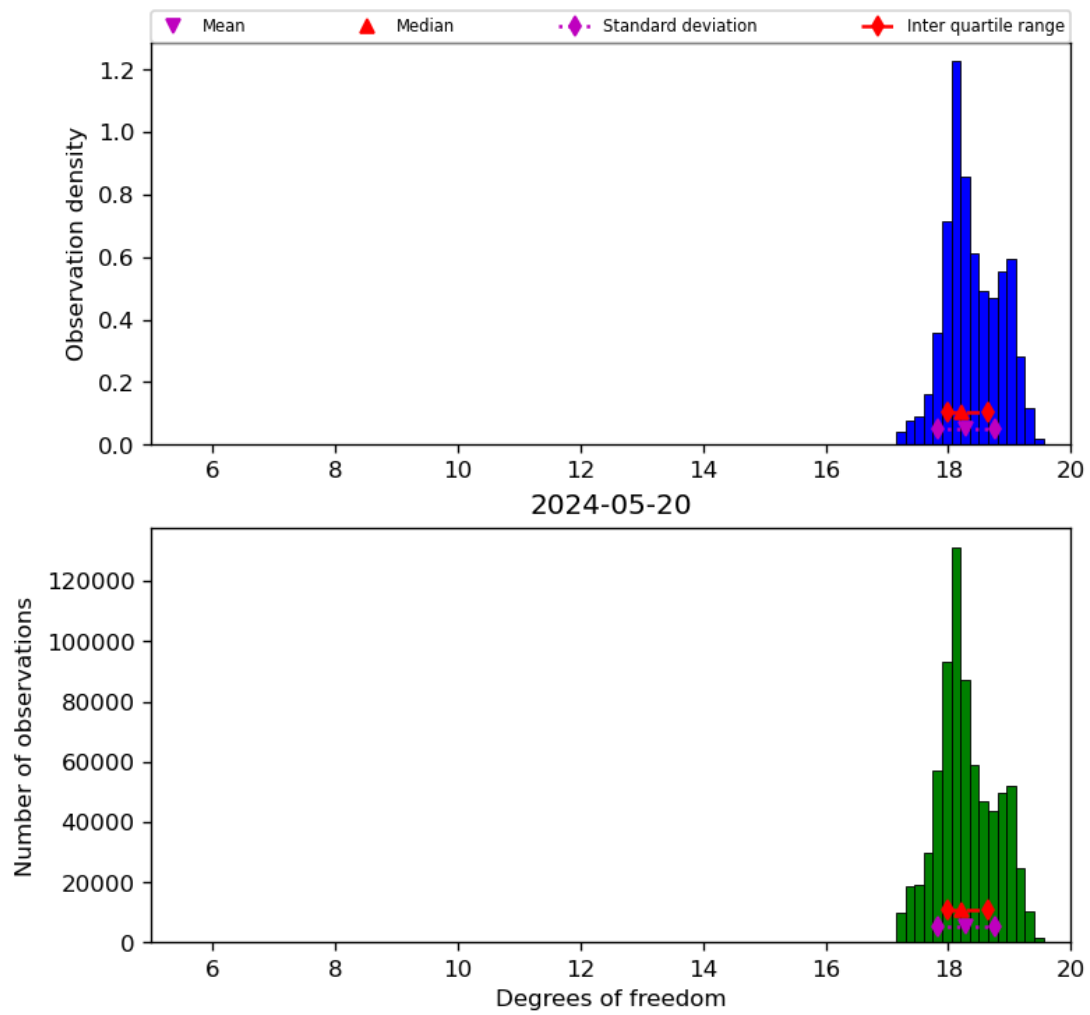
Figure 30: Histogram of “Degrees of freedom” for 2024-05-19 to 2024-05-21
