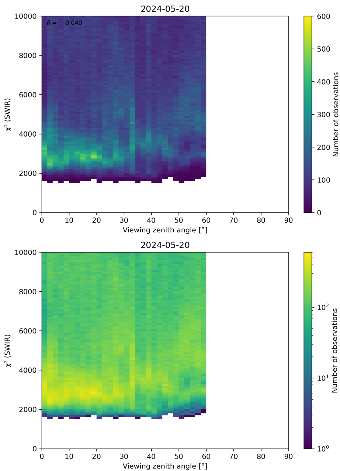
Figure 106: Scatter density plot of “Viewing zenith angle” against “ \chi^2 (SWIR)” for 2024-05-19 to 2024-05-21.
