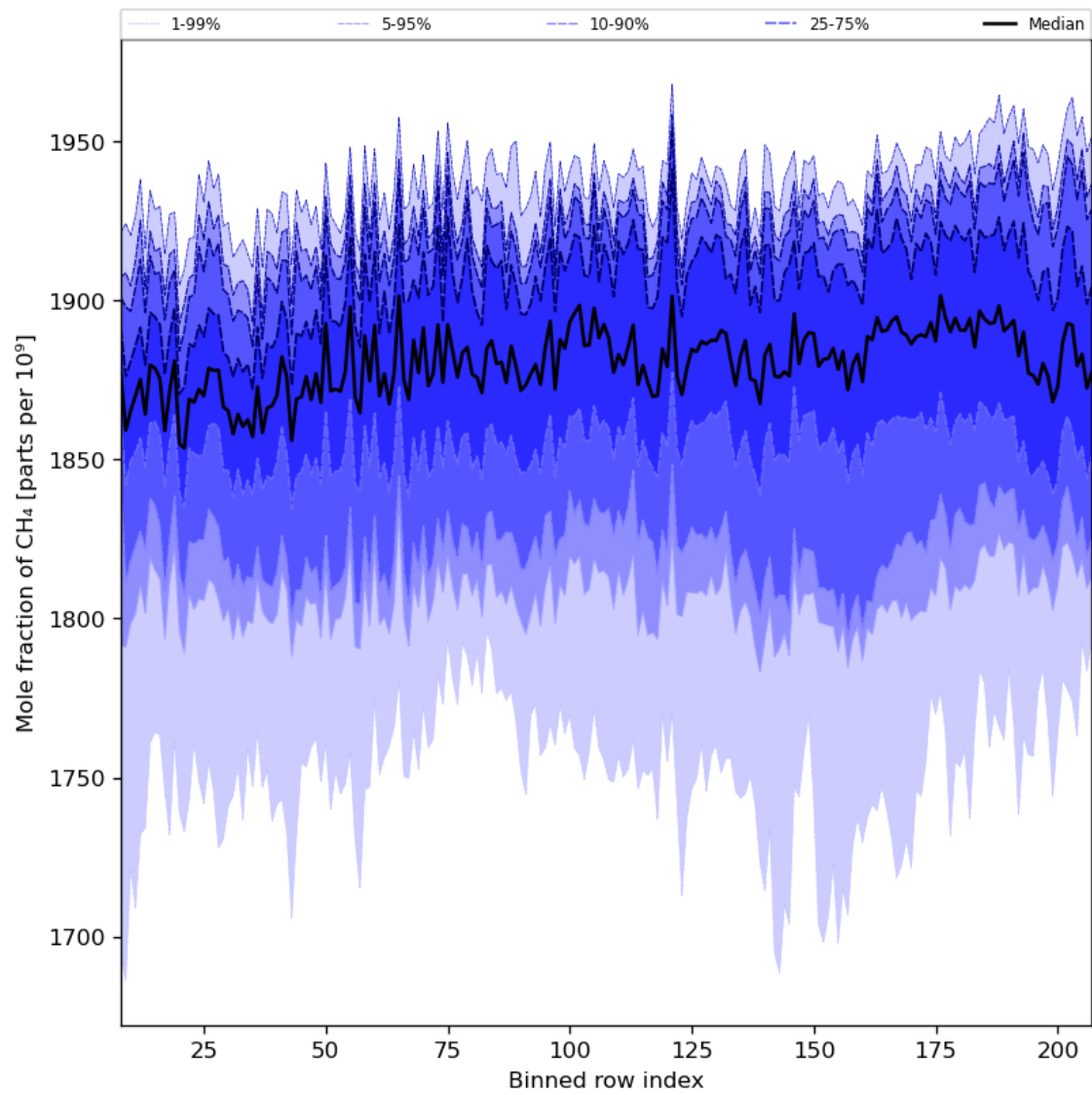
Figure 34: Along track statistics of “Mole fraction of CH 4 ” for 2024-05-19 to 2024-05-21
