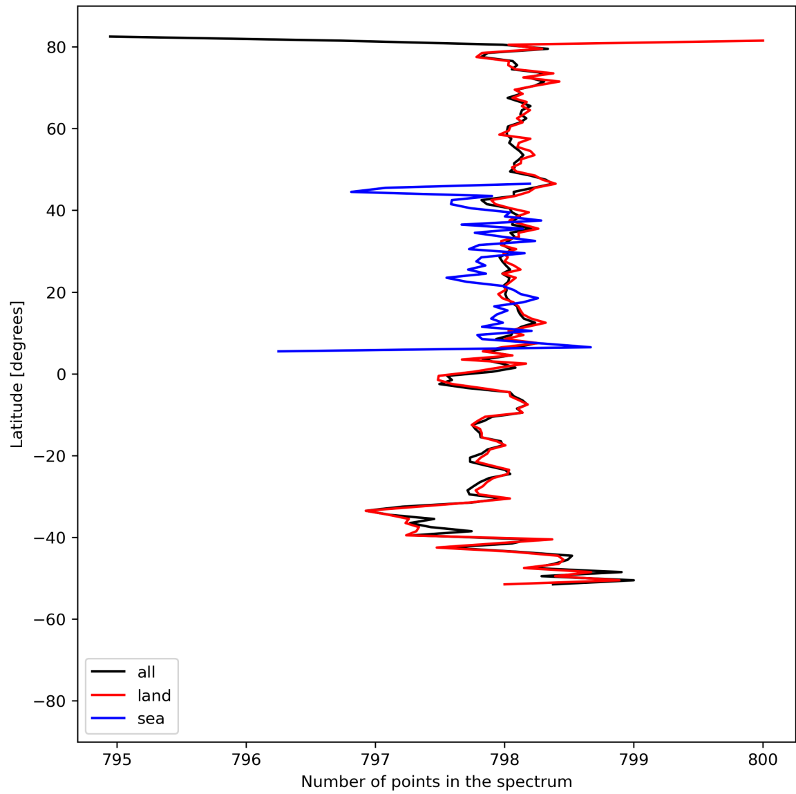
Figure 15: Zonal average of “Number of points in the spectrum” for 2024-05-19 to 2024-05-21.
