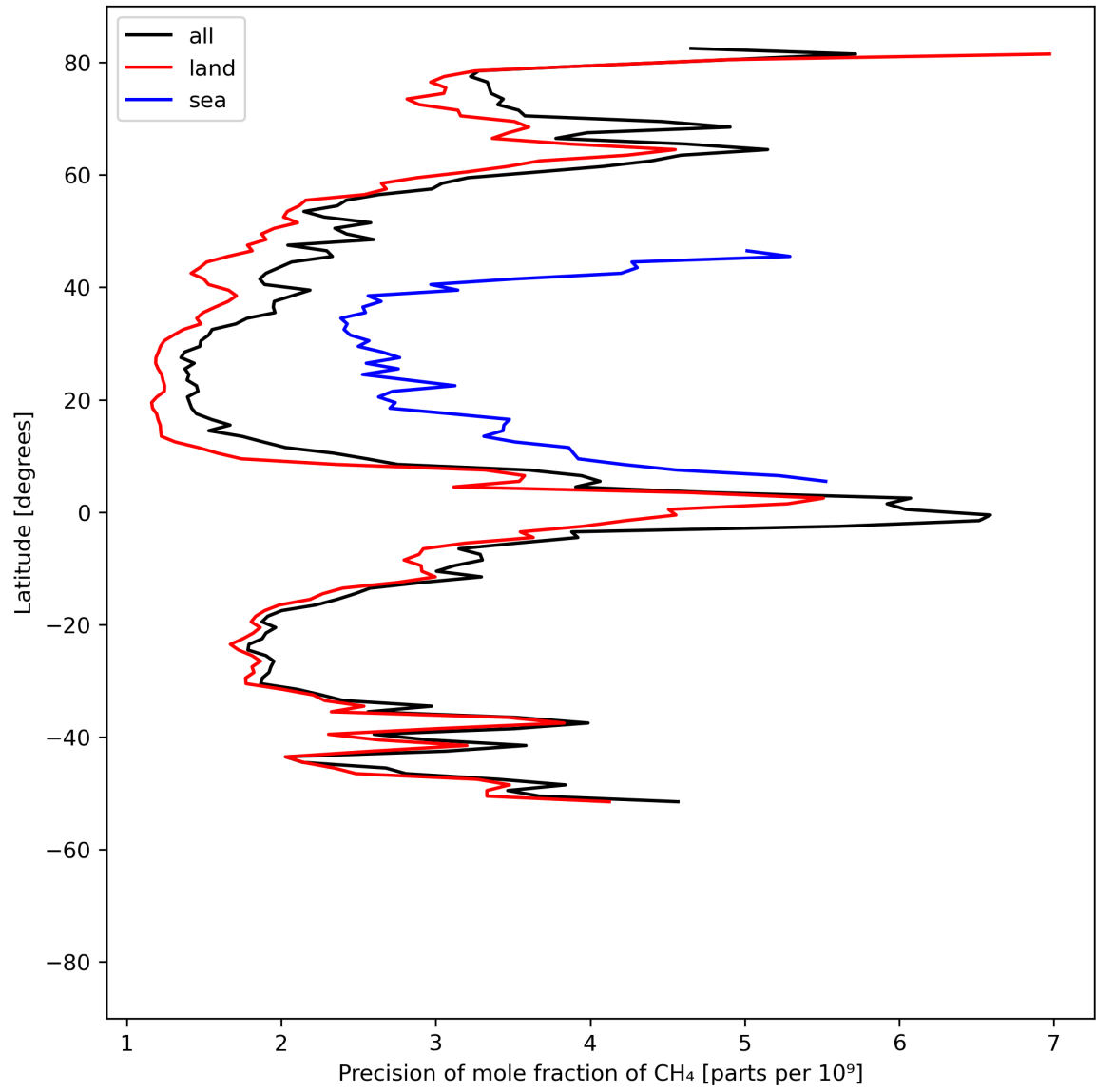
Figure 13: Zonal average of “Precision of mole fraction of CH 4 ” for 2024-05-19 to 2024-05-21.
