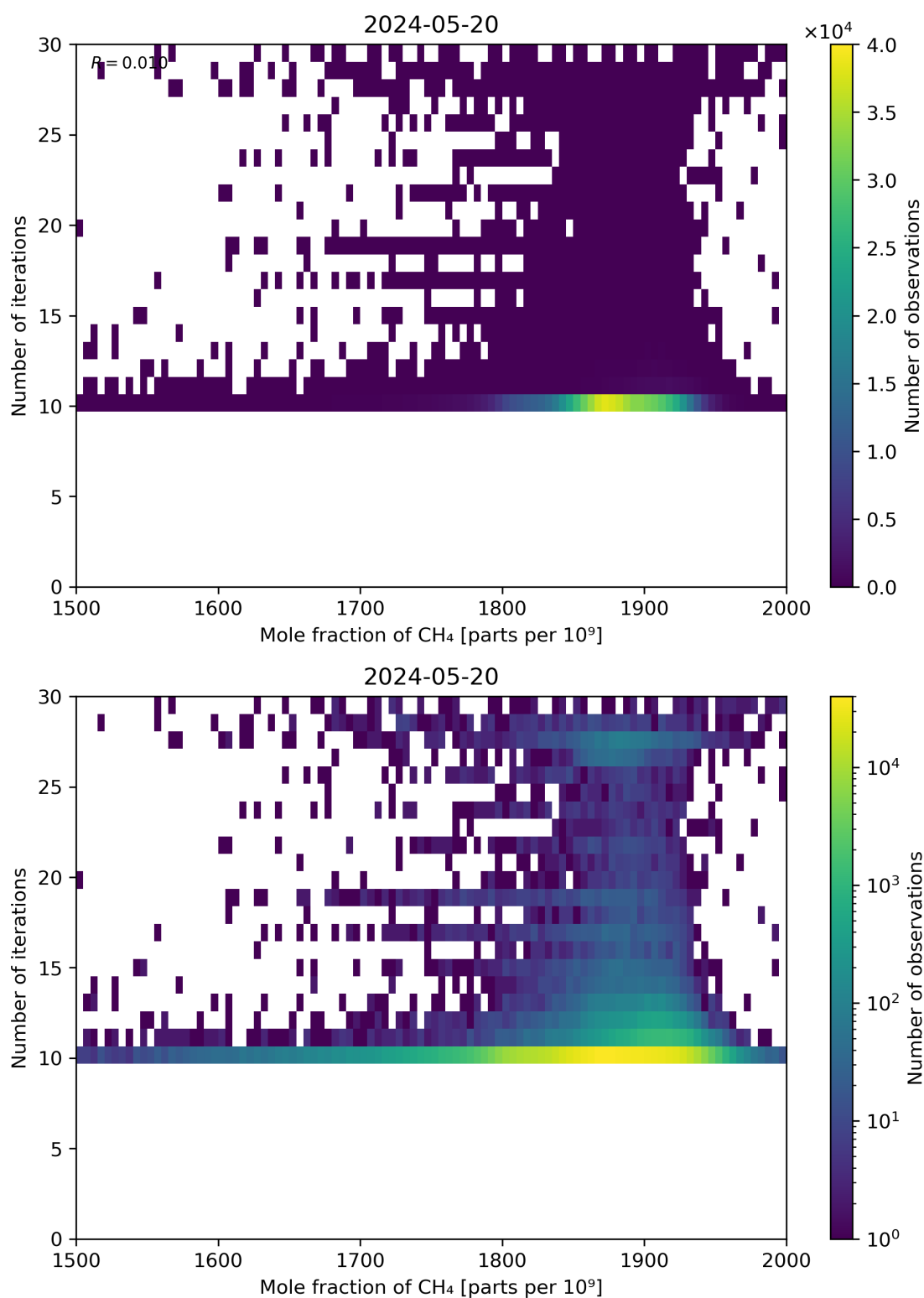
Figure 76: Scatter density plot of “Mole fraction of CH 4 ” against “Number of iterations” for 2024-05-19 to 2024-05-21.
