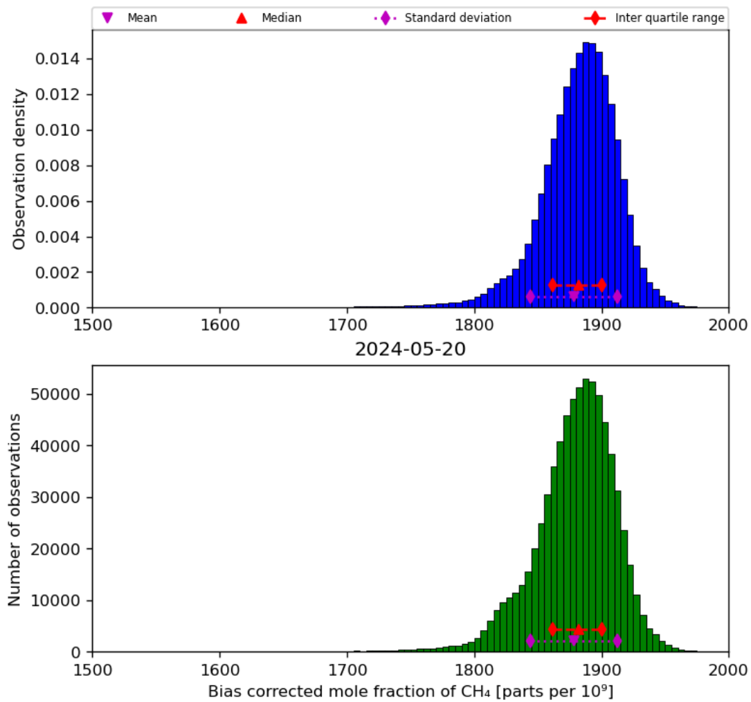
Figure 25: Histogram of “Bias corrected mole fraction of CH 4 ” for 2024-05-19 to 2024-05-21
