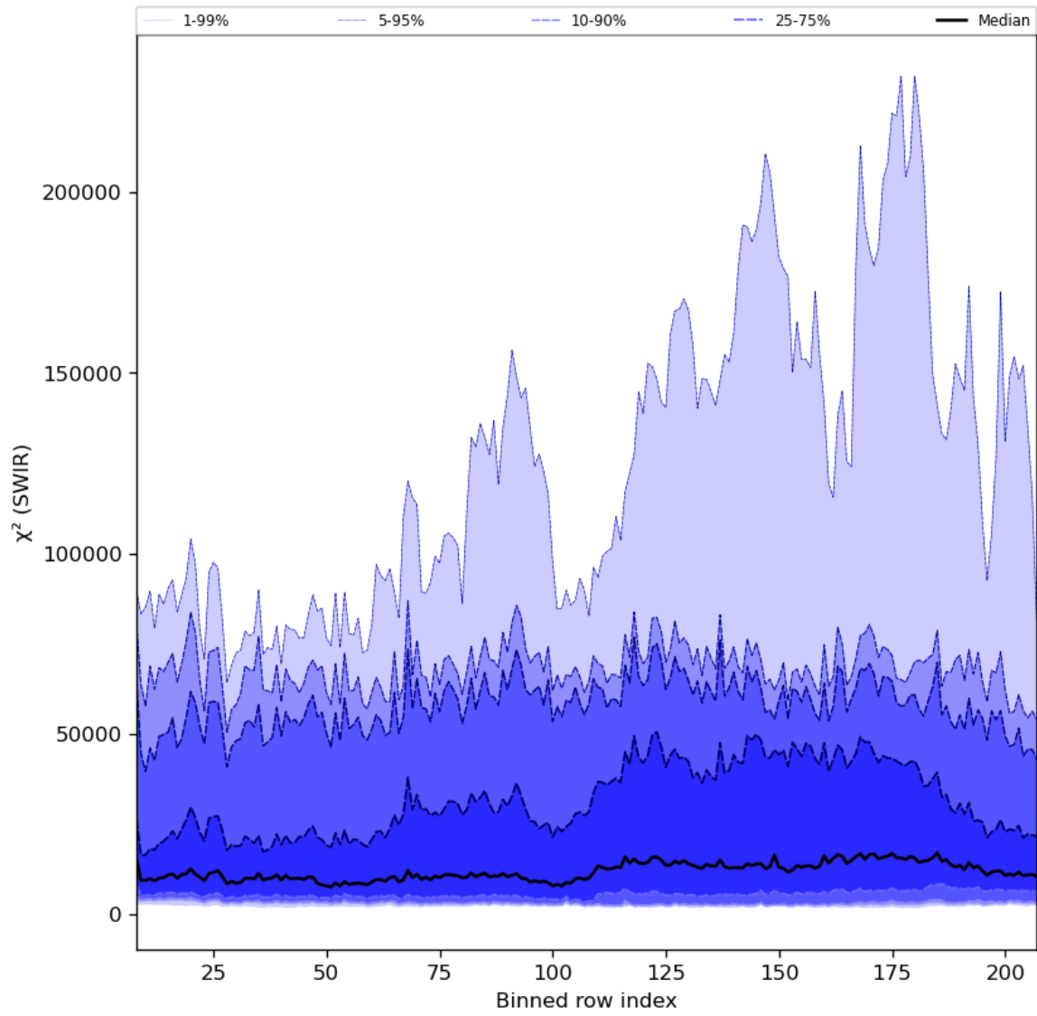
Figure 39: Along track statistics of “ \chi^2 (SWIR)” for 2024-05-19 to 2024-05-21
