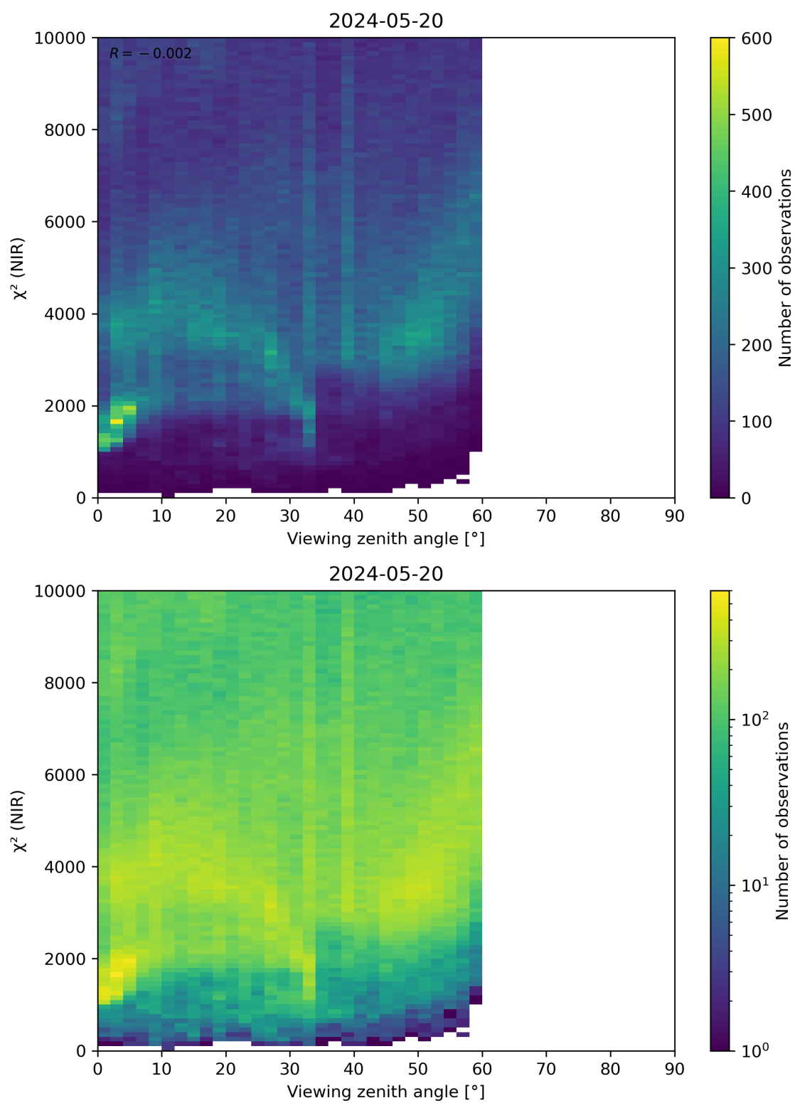
Figure 105: Scatter density plot of “Viewing zenith angle” against “ \chi^2 (NIR)” for 2024-05-19 to 2024-05-21.
