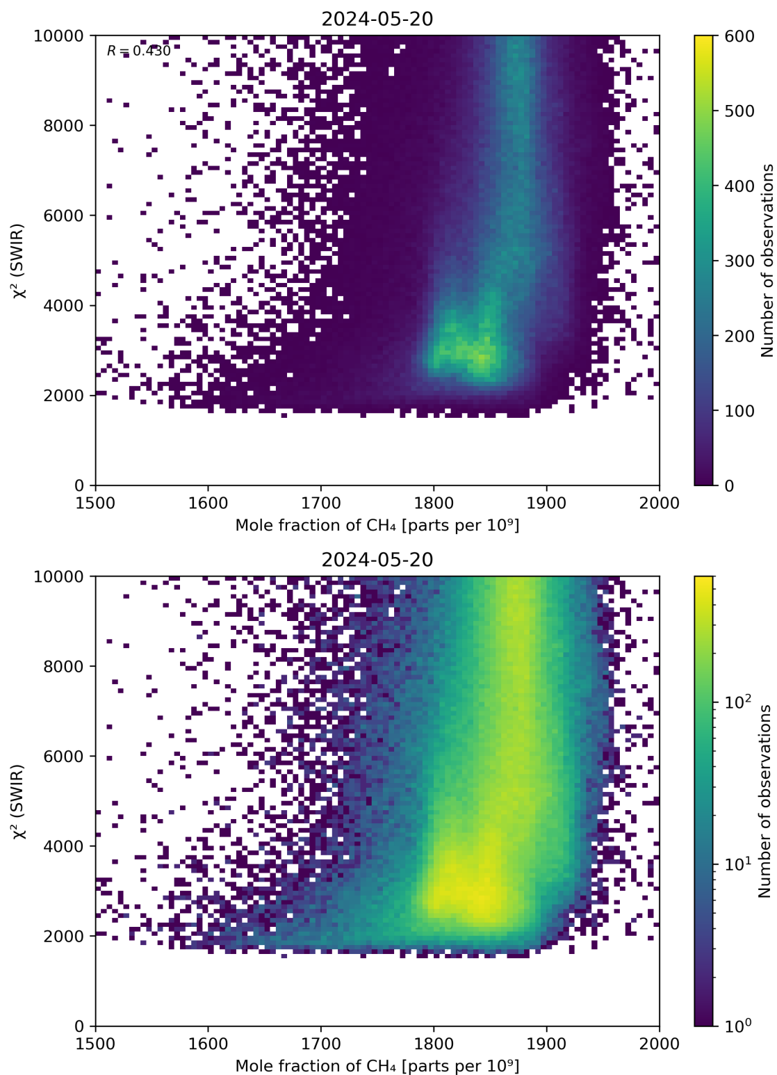
Figure 71: Scatter density plot of “Mole fraction of \text{CH}_4 ” against “ \chi^2 (SWIR)” for 2024-05-19 to 2024-05-21.
