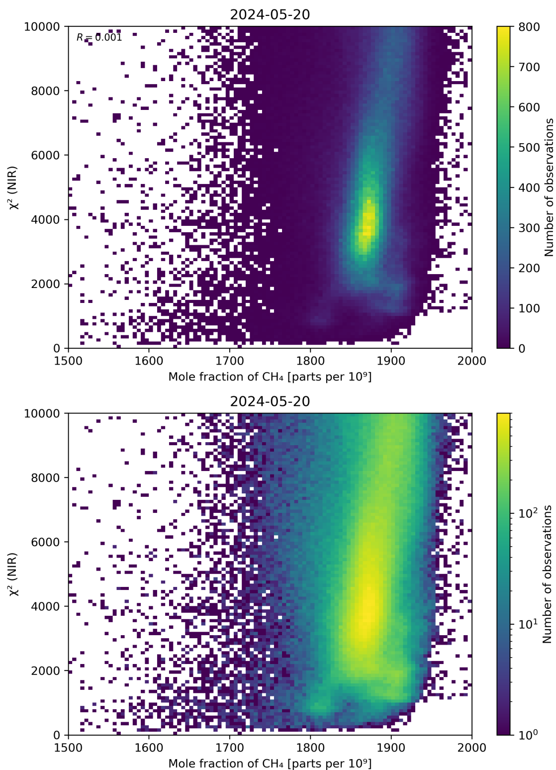
Figure 70: Scatter density plot of “Mole fraction of CH 4 ” against “ \chi^2 (NIR)” for 2024-05-19 to 2024-05-21.
