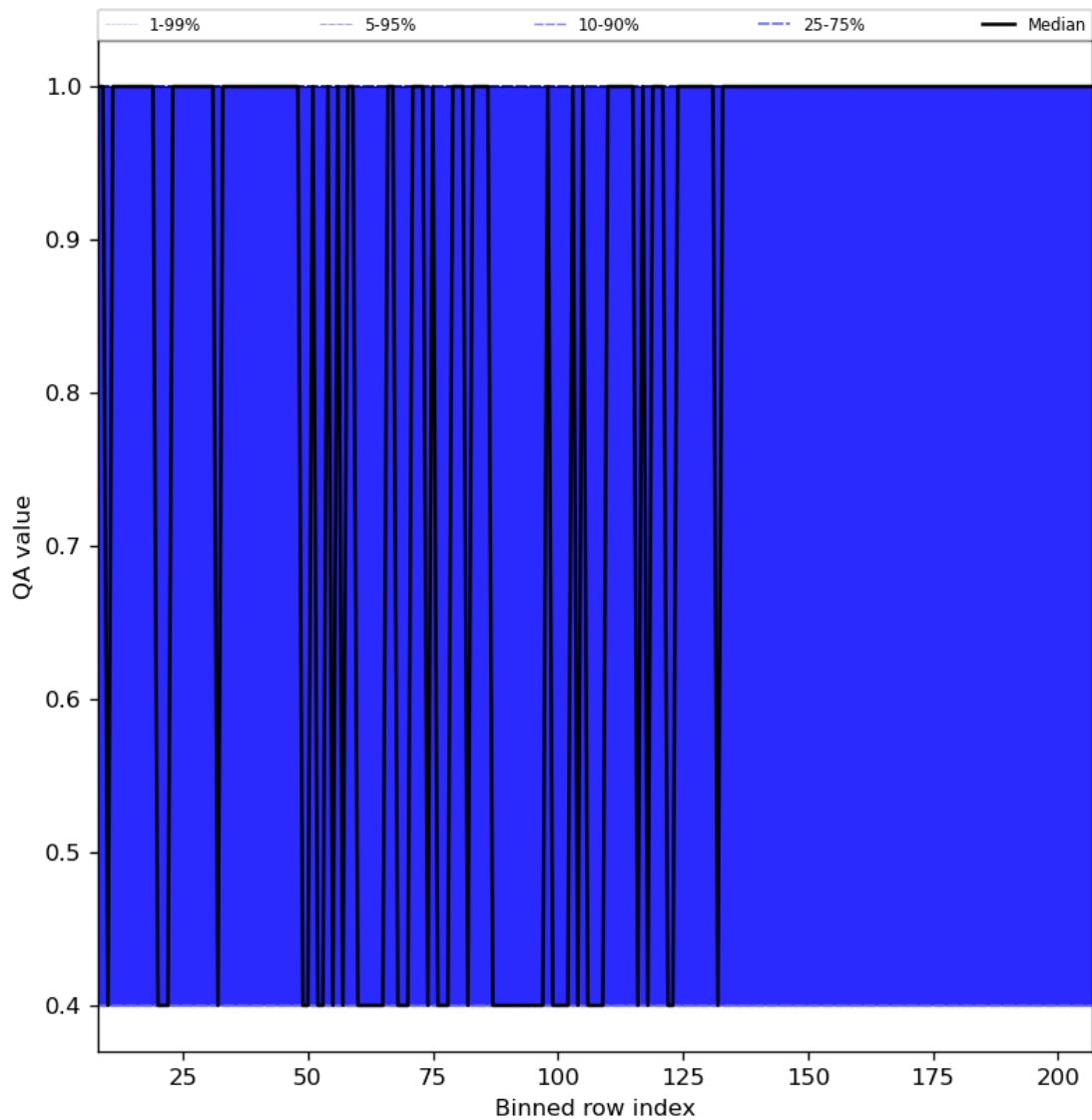
Figure 33: Along track statistics of “QA value” for 2024-05-19 to 2024-05-21
