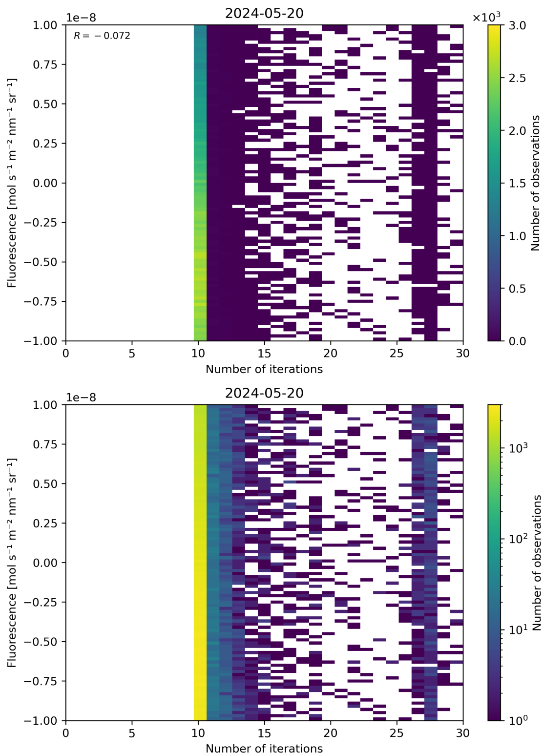
Figure 87: Scatter density plot of “Number of iterations” against “Fluorescence” for 2024-05-19 to 2024-05-21.
