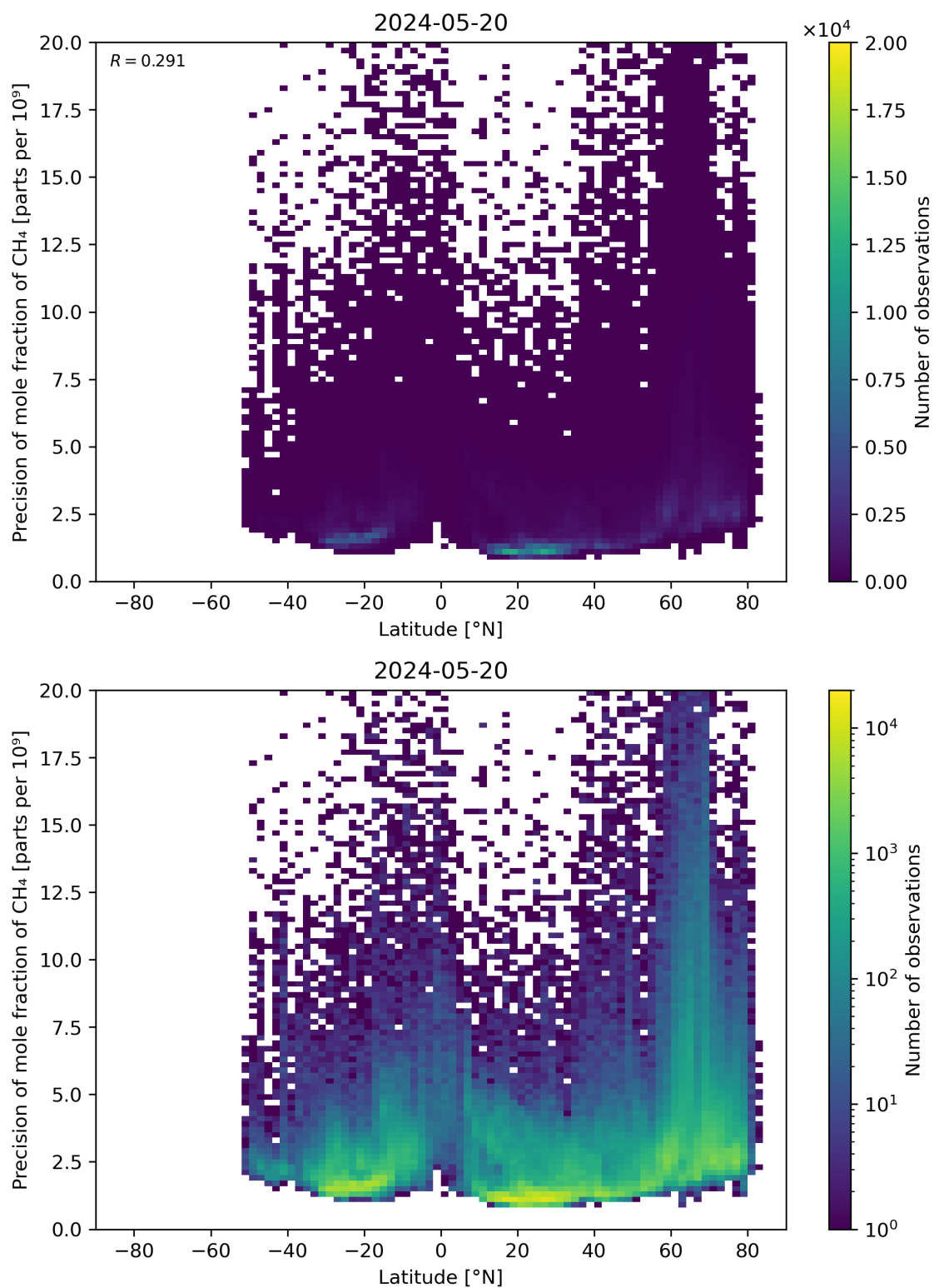
Figure 59: Scatter density plot of “Latitude” against “Precision of mole fraction of \text{CH}_4 ” for 2024-05-19 to 2024-05-21.
