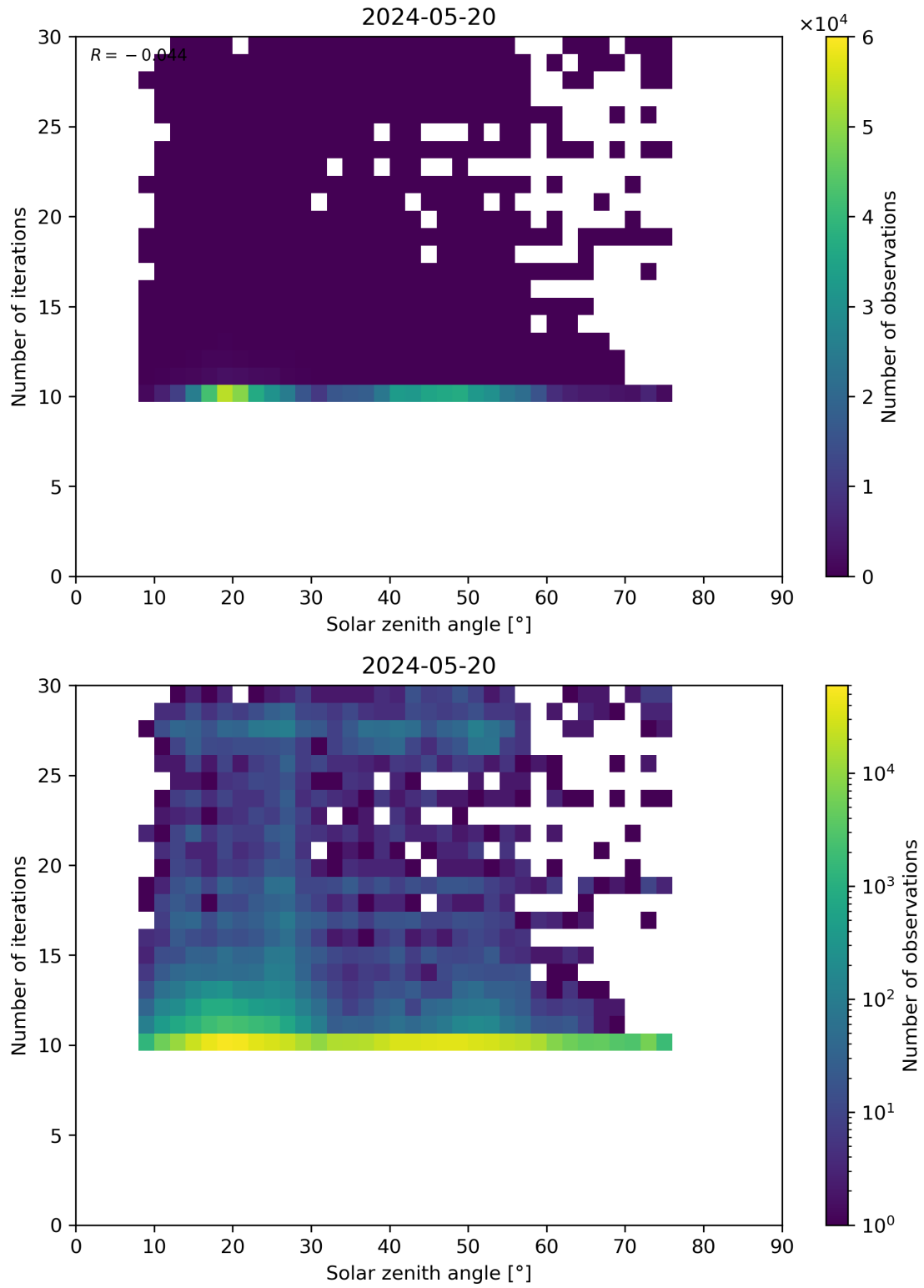
Figure 102: Scatter density plot of “Solar zenith angle” against “Number of iterations” for 2024-05-19 to 2024-05-21.
