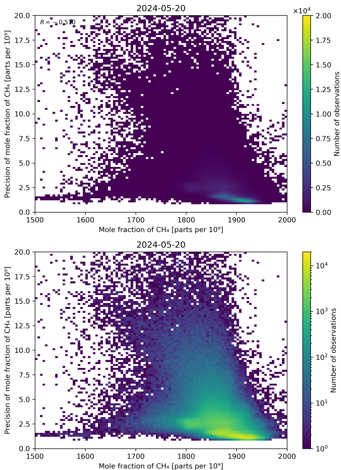
Figure 75: Scatter density plot of “Mole fraction of CH 4 ” against “Precision of mole fraction of CH 4 ” for 2024-05-19 to 2024-05-21.
