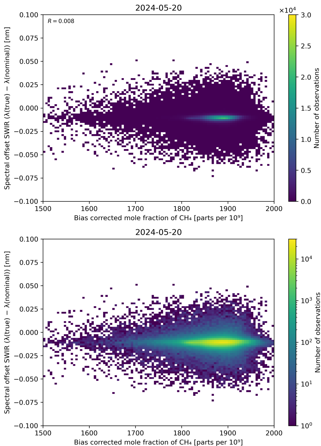
Figure 69: Scatter density plot of “Bias corrected mole fraction of \text{CH}_4 ” against “Spectral offset SWIR ( \lambda(\text{true}) - \lambda(\text{nominal}) )” for 2024-05-19 to 2024-05-21.
