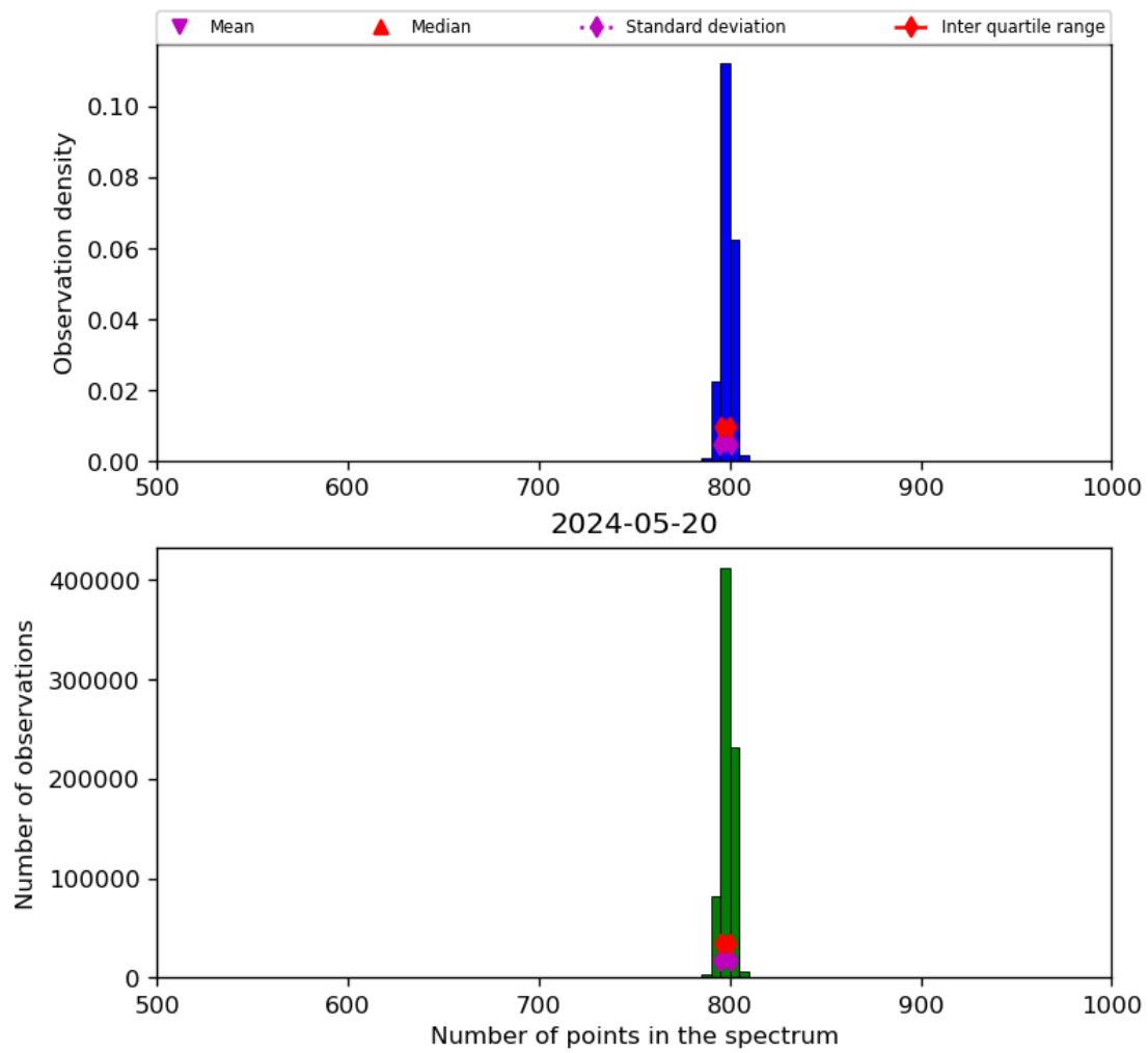
Figure 26: Histogram of “Number of points in the spectrum” for 2024-05-19 to 2024-05-21
