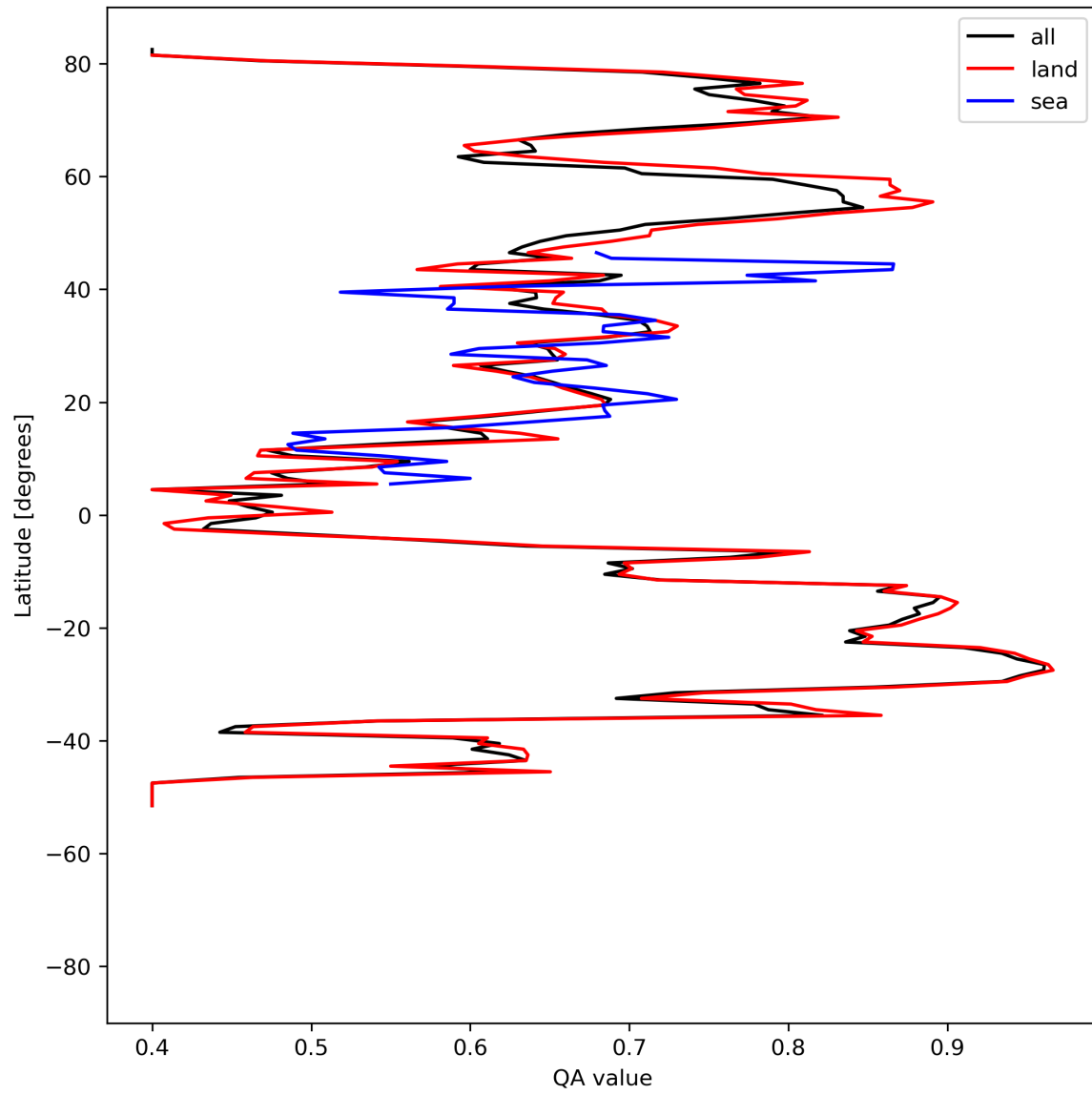
Figure 11: Zonal average of “QA value” for 2024-05-19 to 2024-05-21.
