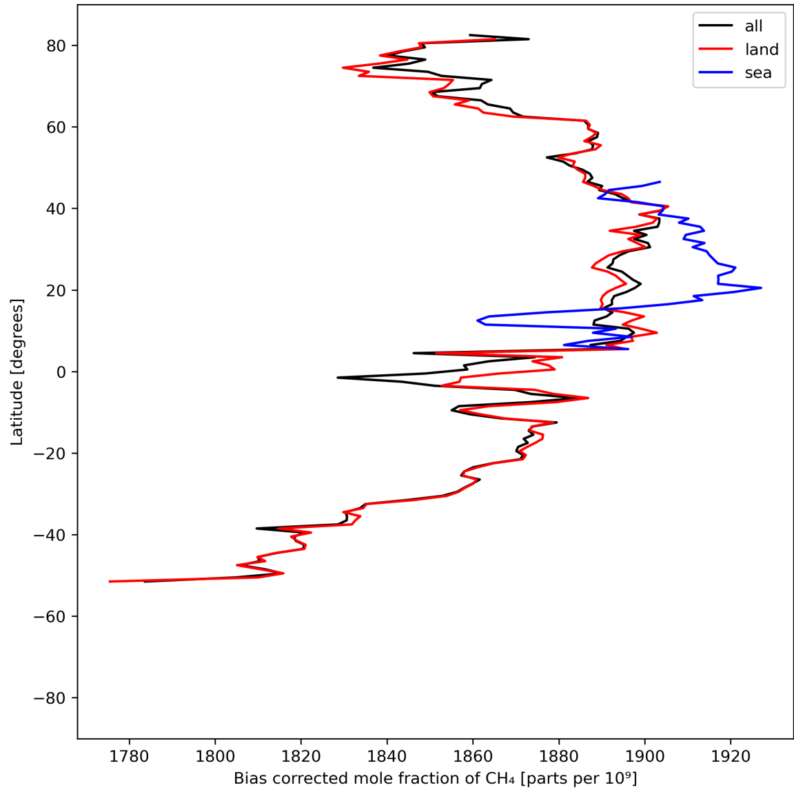
Figure 14: Zonal average of “Bias corrected mole fraction of CH 4 ” for 2024-05-19 to 2024-05-21.
