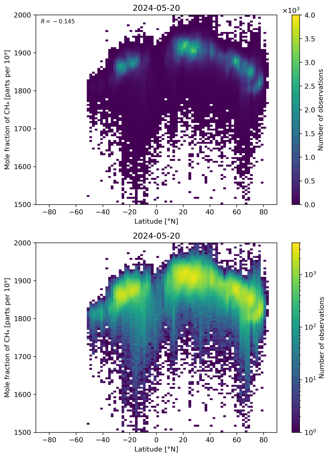
Figure 57: Scatter density plot of “Latitude” against “Mole fraction of \text{CH}_4 ” for 2024-05-19 to 2024-05-21.
