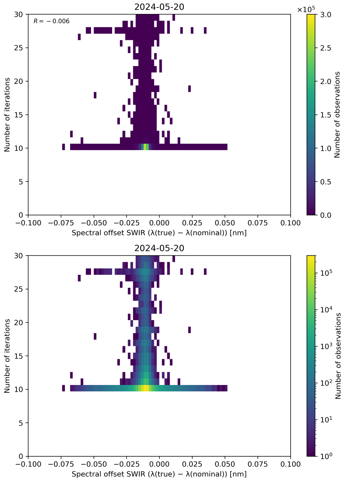
Figure 121: Scatter density plot of “Spectral offset SWIR ( \lambda(\text{true}) - \lambda(\text{nominal}) )” against “Number of iterations” for 2024-05-19 to 2024-05-21.
