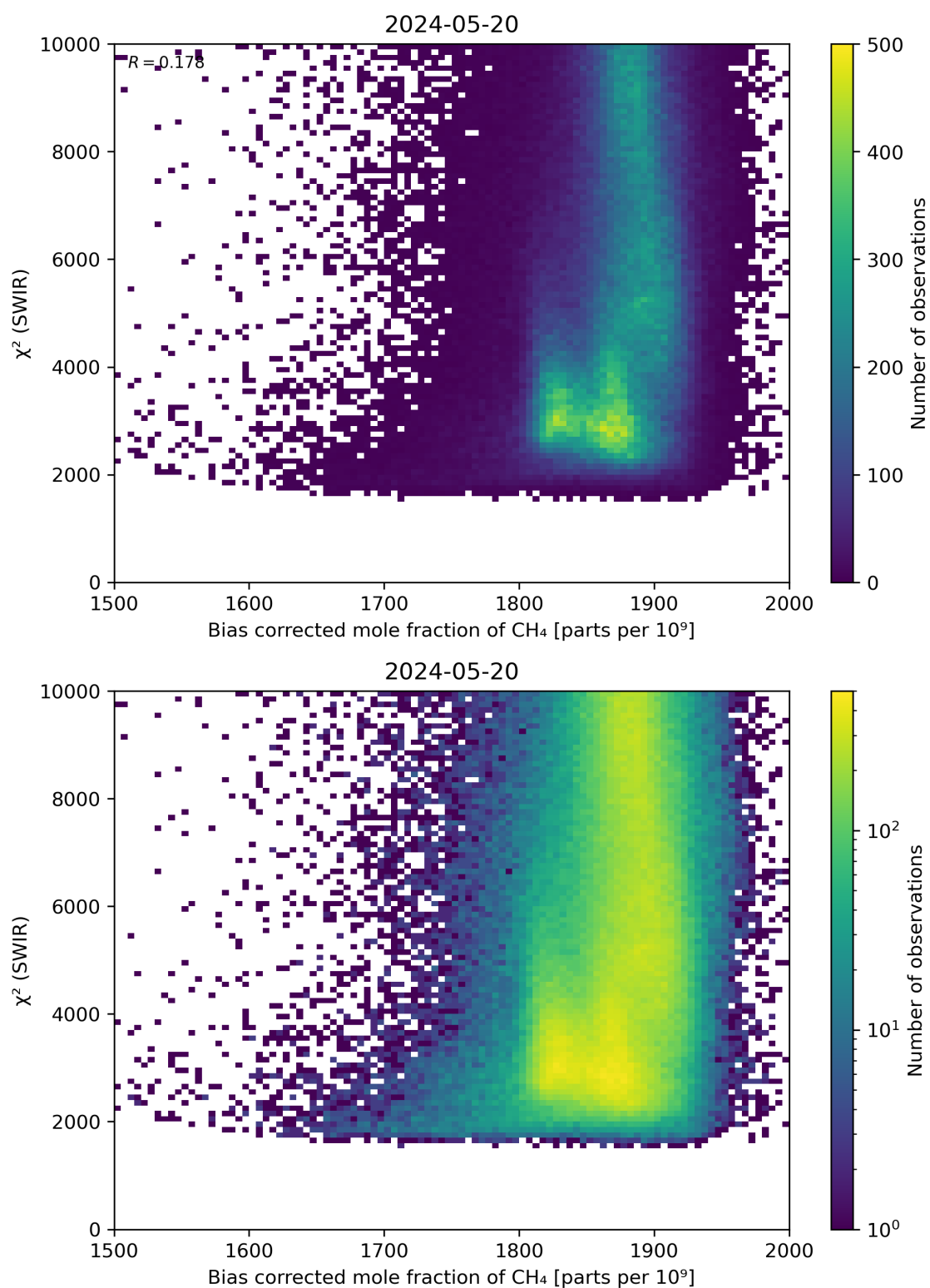
Figure 64: Scatter density plot of “Bias corrected mole fraction of CH 4 ” against “ \chi^2 (SWIR)” for 2024-05-19 to 2024-05-21.
