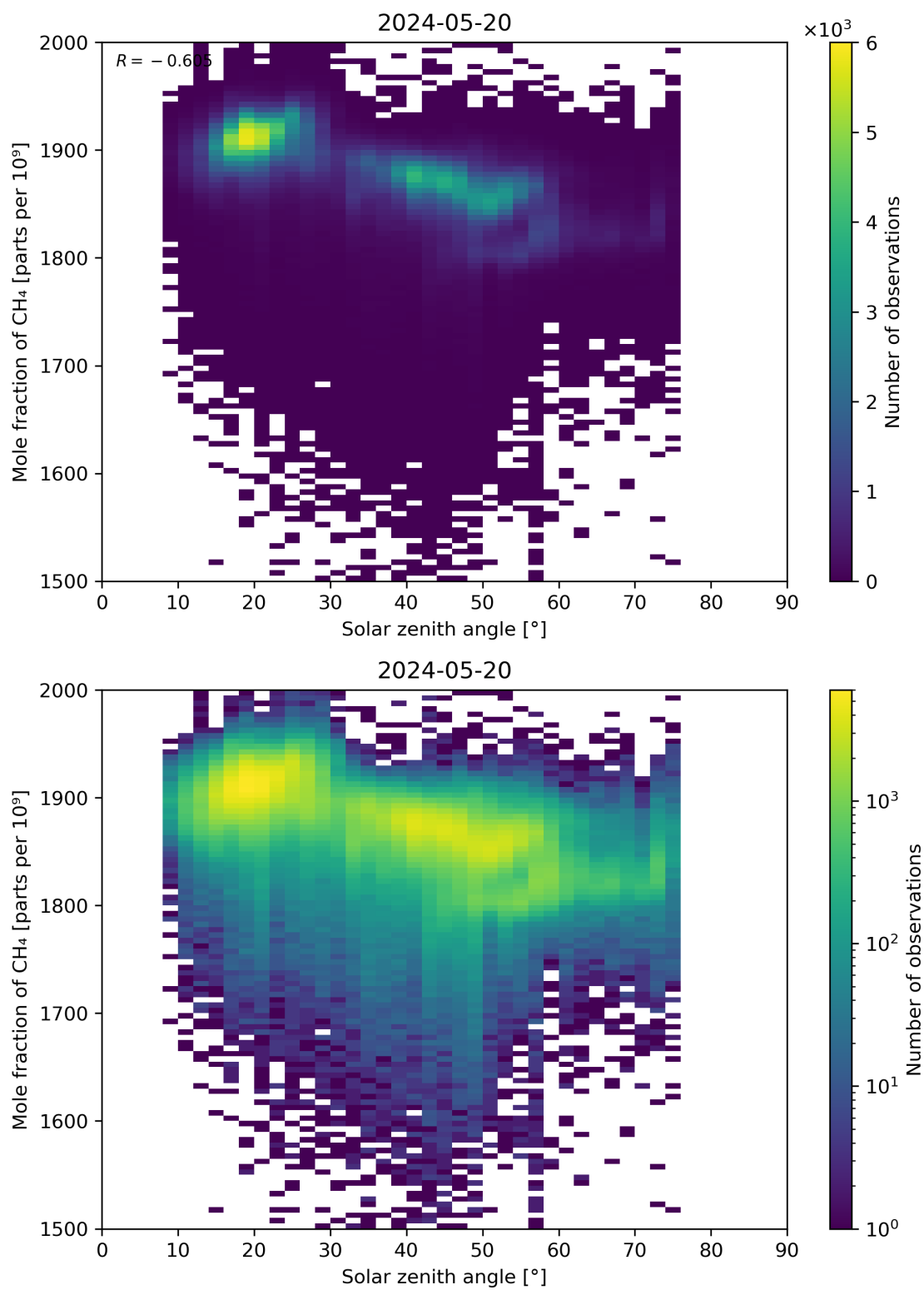
Figure 99: Scatter density plot of “Solar zenith angle” against “Mole fraction of CH 4 ” for 2024-05-19 to 2024-05-21.
