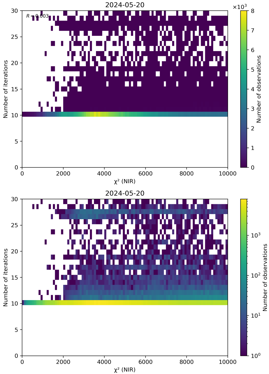
Figure 46: Scatter density plot of “ \chi^2 (NIR)” against “Number of iterations” for 2024-05-19 to 2024-05-21.
