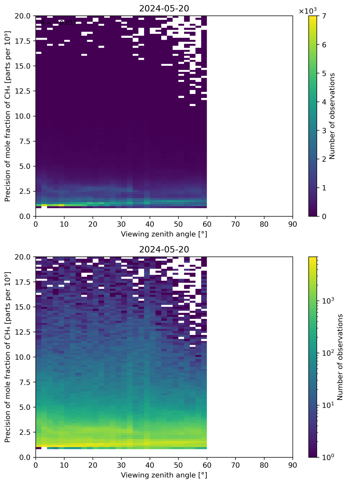
Figure 112: Scatter density plot of “Viewing zenith angle” against “Precision of mole fraction of CH 4 ” for 2024-05-19 to 2024-05-21.
