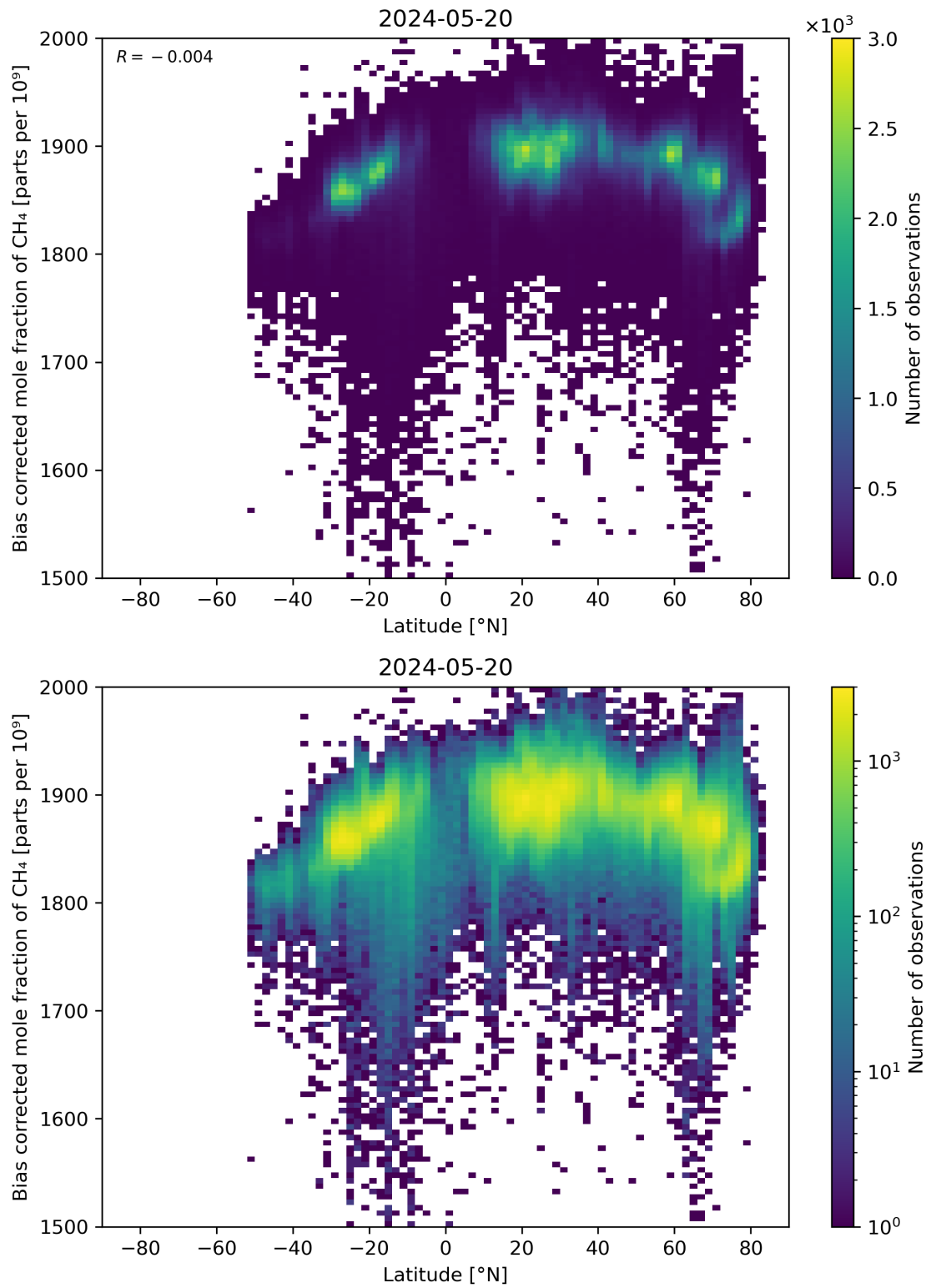
Figure 58: Scatter density plot of “Latitude” against “Bias corrected mole fraction of CH 4 ” for 2024-05-19 to 2024-05-21.
