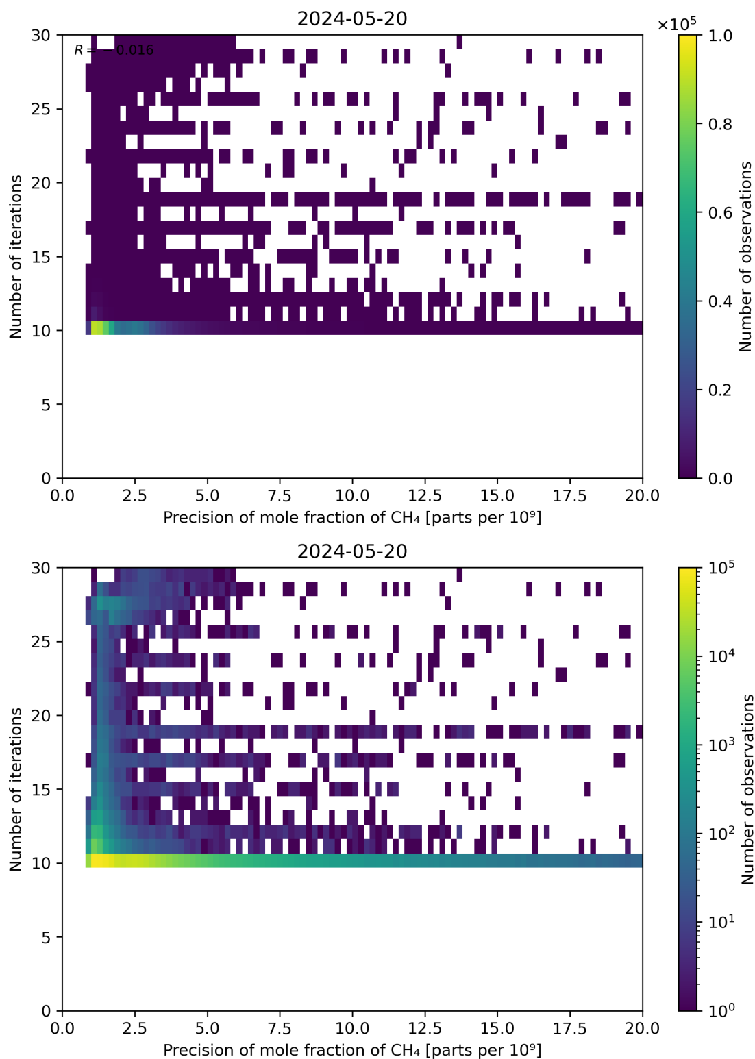
Figure 83: Scatter density plot of “Precision of mole fraction of CH 4 ” against “Number of iterations” for 2024-05-19 to 2024-05-21.
