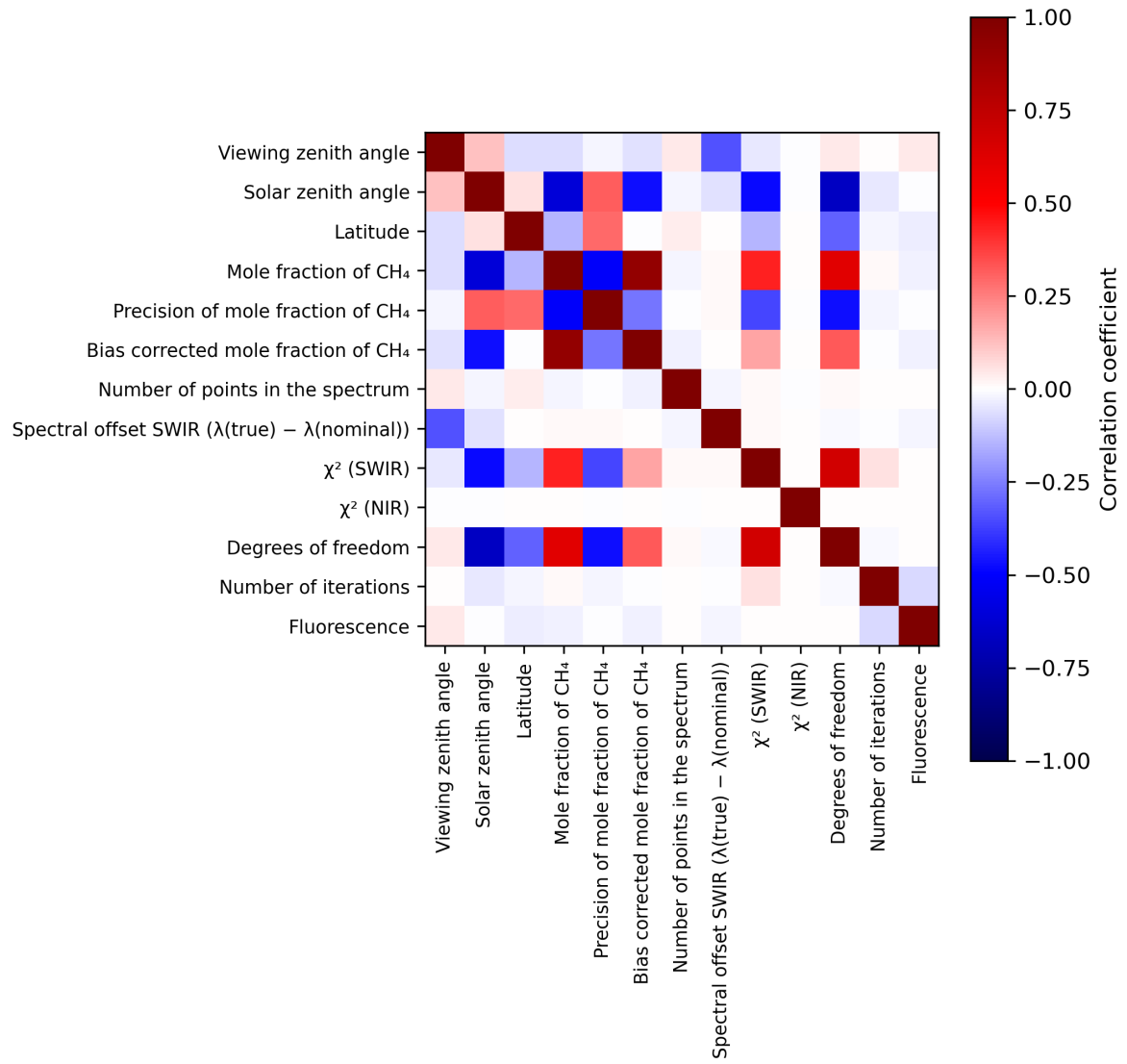
Figure 2: Map of correlation matrix for 2024-05-19 to 2024-05-21.
