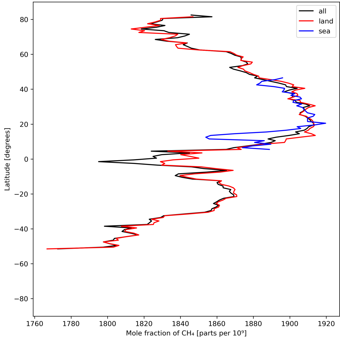
Figure 12: Zonal average of “Mole fraction of \text{CH}_4 ” for 2024-05-19 to 2024-05-21.
