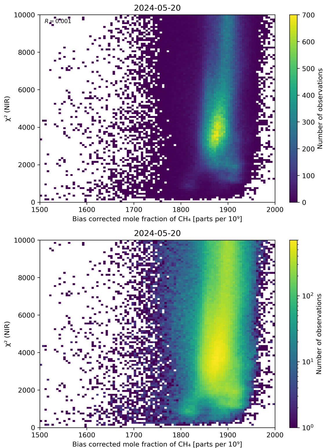
Figure 63: Scatter density plot of “Bias corrected mole fraction of CH 4 ” against “ \chi^2 (NIR)” for 2024-05-19 to 2024-05-21.
