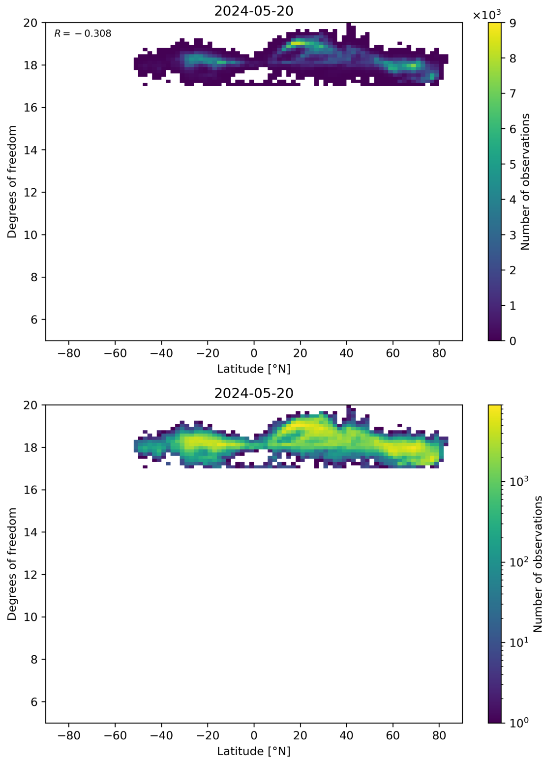
Figure 55: Scatter density plot of “Latitude” against “Degrees of freedom” for 2024-05-19 to 2024-05-21.
