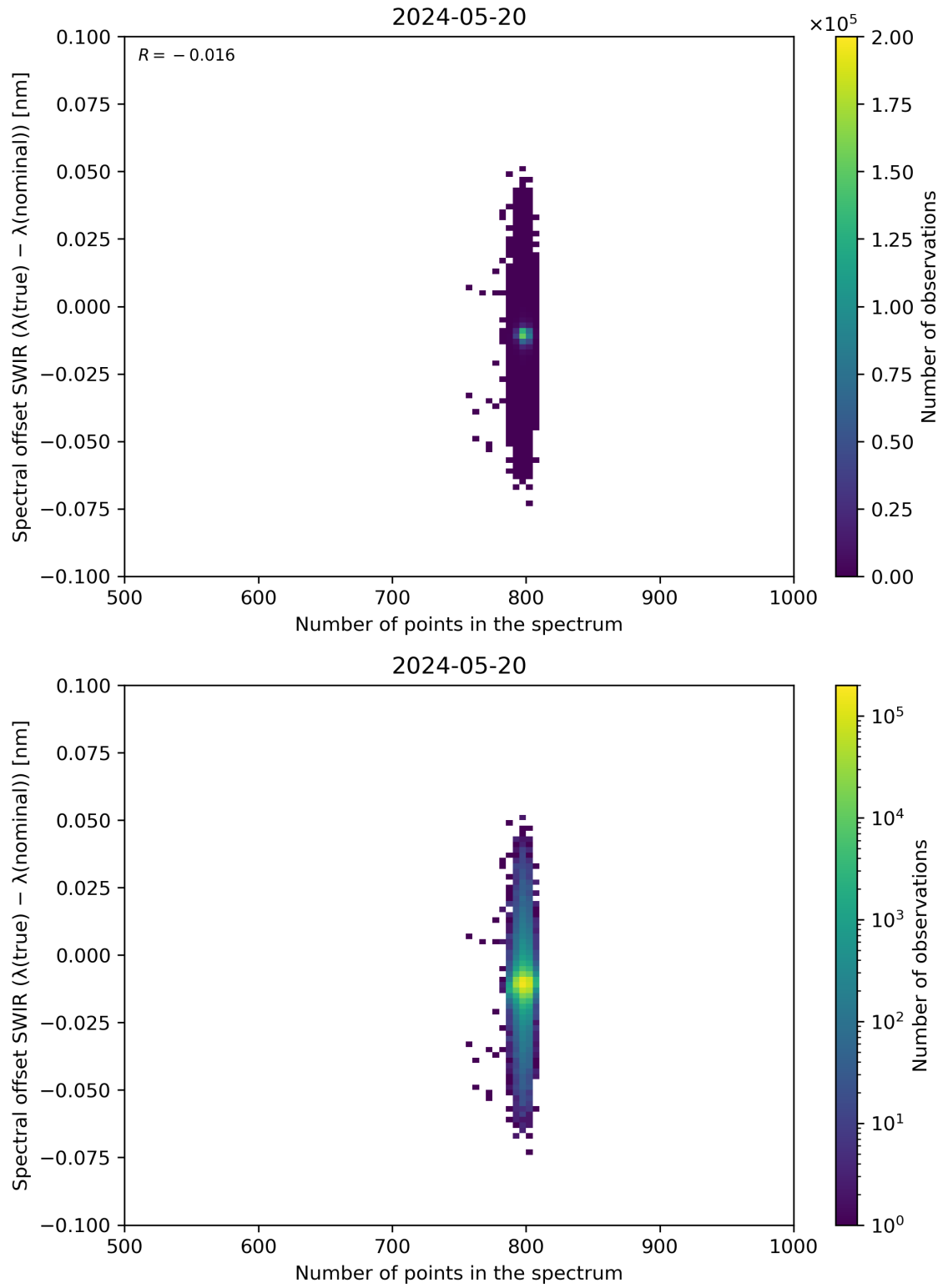
Figure 93: Scatter density plot of “Number of points in the spectrum” against “Spectral offset SWIR ( \lambda(\text{true}) - \lambda(\text{nominal}) )” for 2024-05-19 to 2024-05-21.
