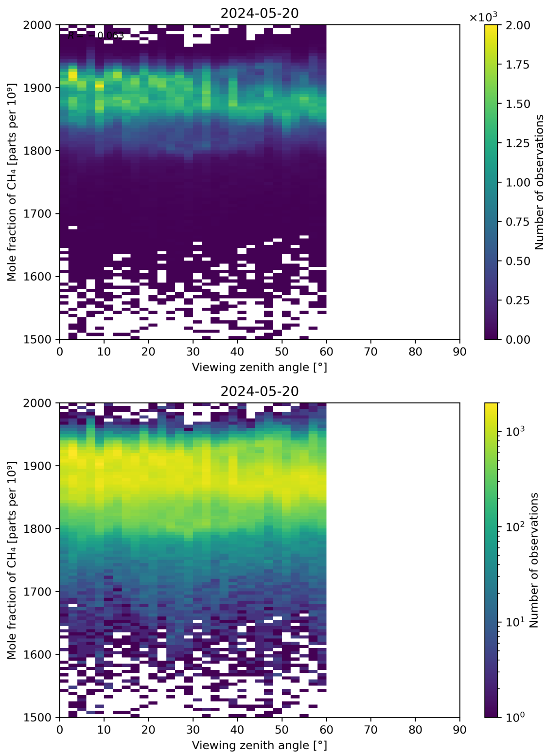
Figure 110: Scatter density plot of “Viewing zenith angle” against “Mole fraction of CH 4 ” for 2024-05-19 to 2024-05-21.
