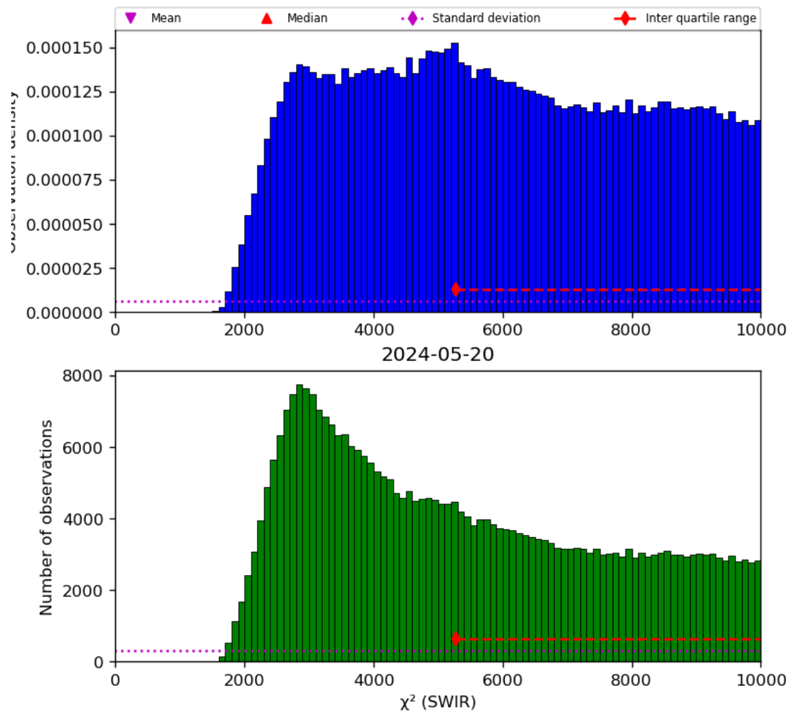
Figure 28: Histogram of “ \chi^2 (SWIR)” for 2024-05-19 to 2024-05-21
