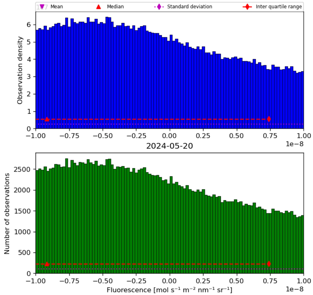
Figure 32: Histogram of “Fluorescence” for 2024-05-19 to 2024-05-21
