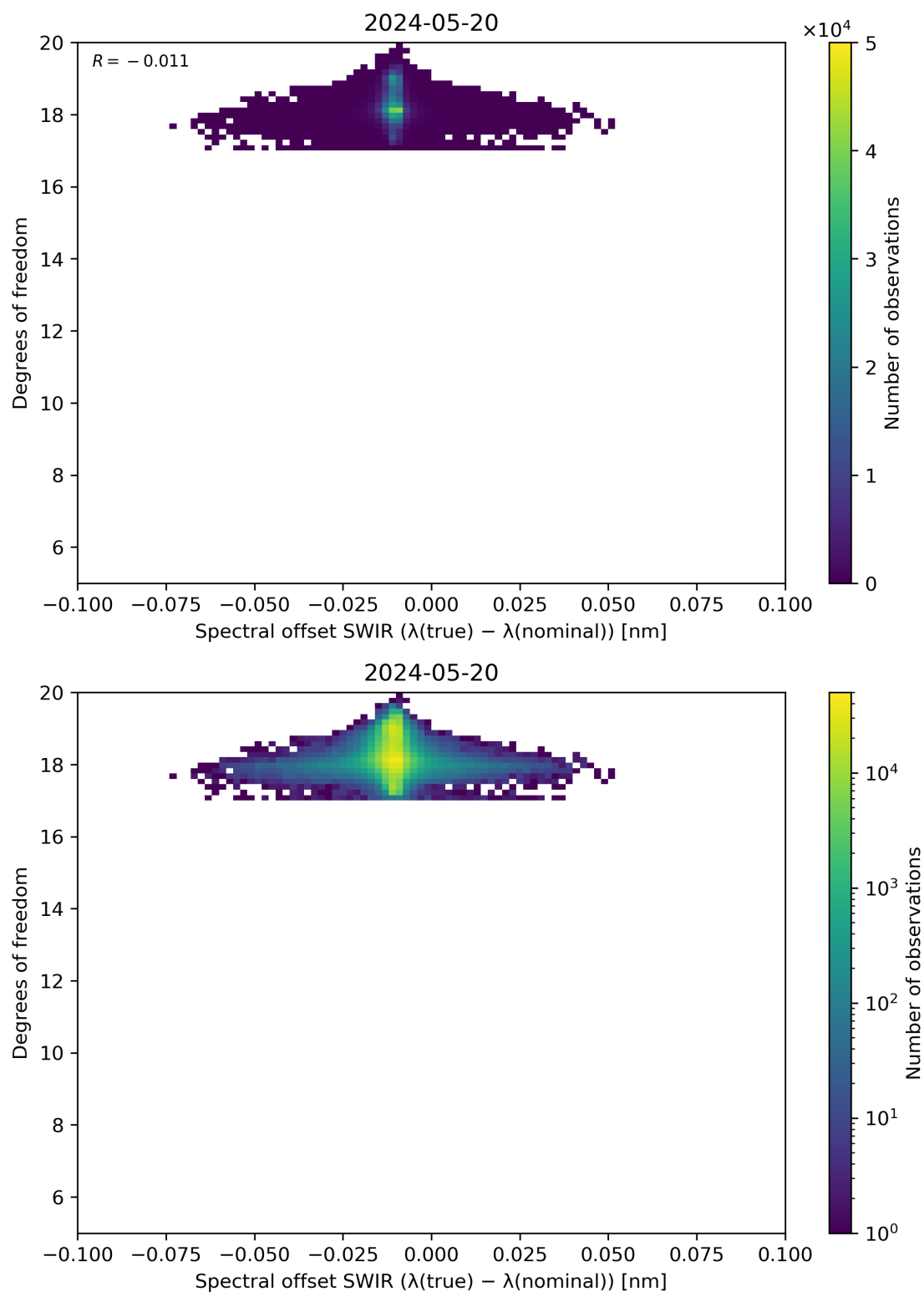
Figure 119: Scatter density plot of “Spectral offset SWIR ( \lambda(\text{true}) - \lambda(\text{nominal}) )” against “Degrees of freedom” for 2024-05-19 to 2024-05-21.
