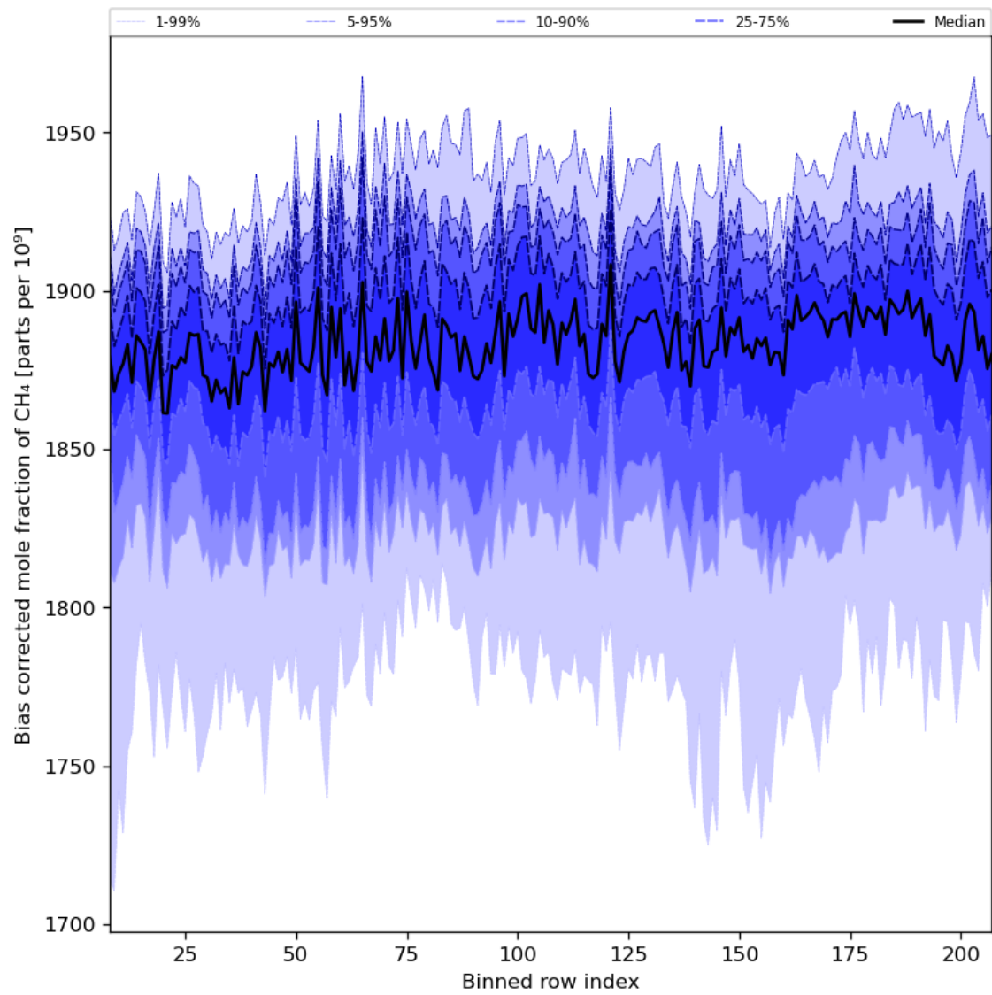
Figure 36: Along track statistics of “Bias corrected mole fraction of CH 4 ” for 2024-05-19 to 2024-05-21
