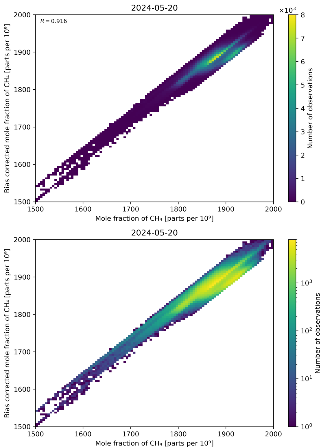
Figure 74: Scatter density plot of “Mole fraction of CH 4 ” against “Bias corrected mole fraction of CH 4 ” for 2024-05-19 to 2024-05-21.
