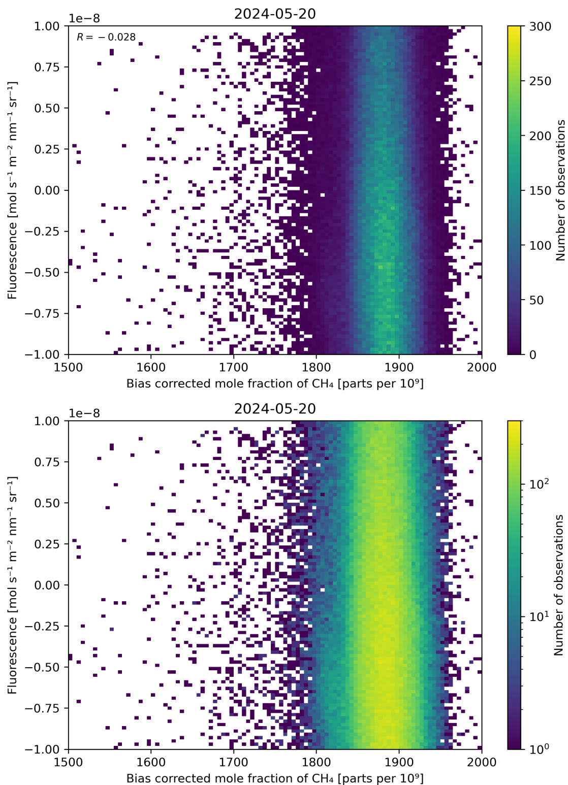
Figure 66: Scatter density plot of “Bias corrected mole fraction of \text{CH}_4 ” against “Fluorescence” for 2024-05-19 to 2024-05-21.
