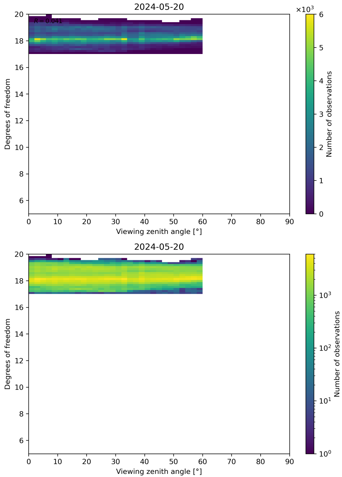
Figure 107: Scatter density plot of “Viewing zenith angle” against “Degrees of freedom” for 2024-05-19 to 2024-05-21.
