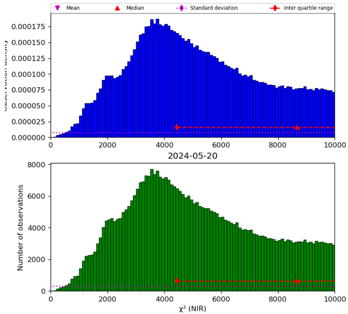
Figure 29: Histogram of “ \chi^2 (NIR)” for 2024-05-19 to 2024-05-21
