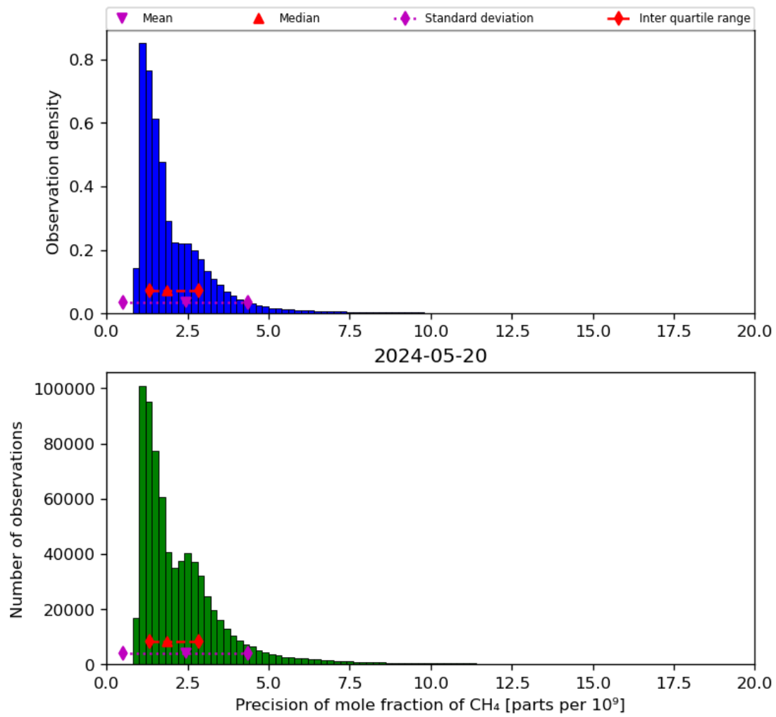
Figure 24: Histogram of “Precision of mole fraction of CH 4 ” for 2024-05-19 to 2024-05-21
