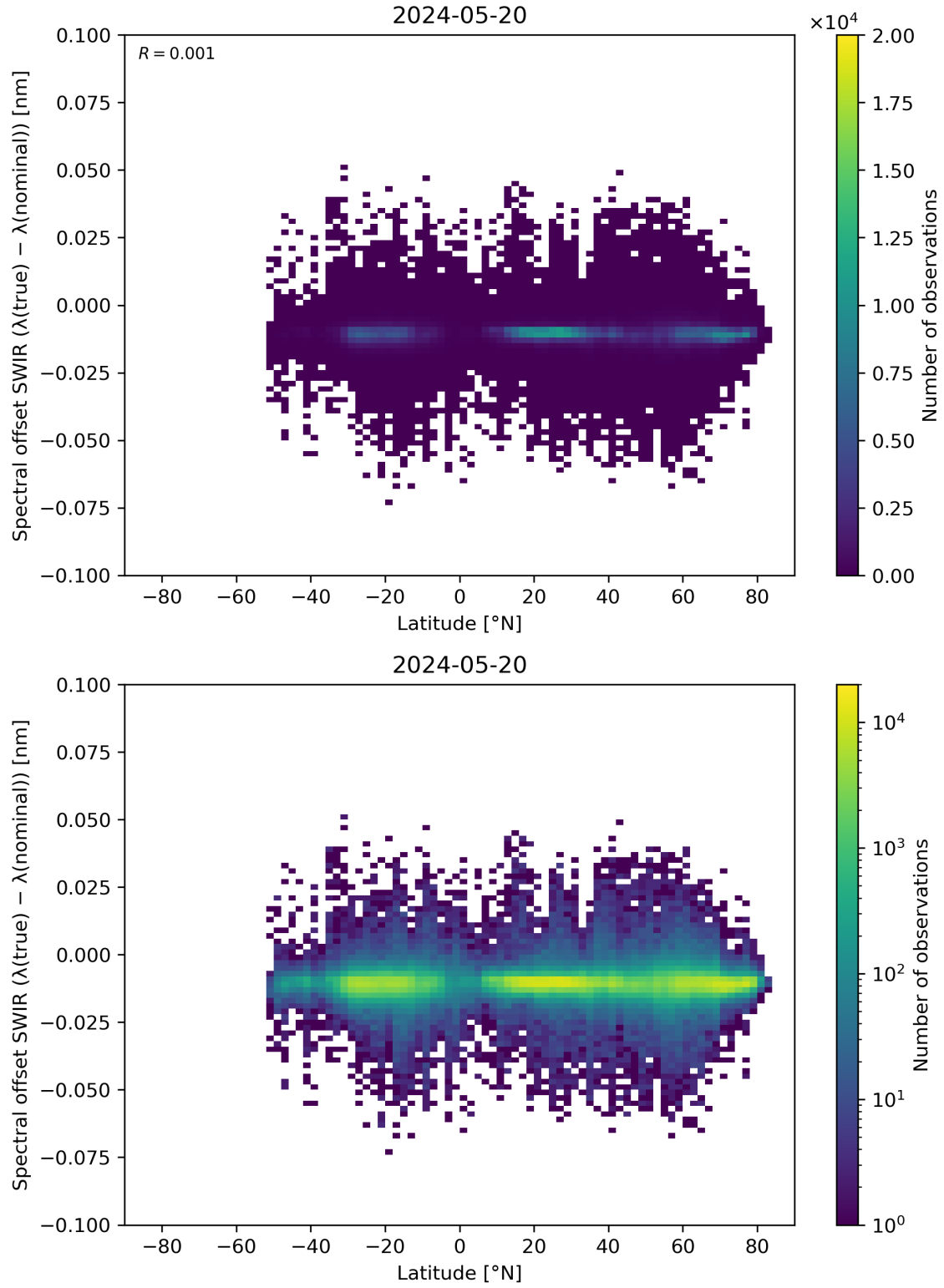
Figure 62: Scatter density plot of “Latitude” against “Spectral offset SWIR ( \lambda(\text{true}) - \lambda(\text{nominal}) )” for 2024-05-19 to 2024-05-21.
