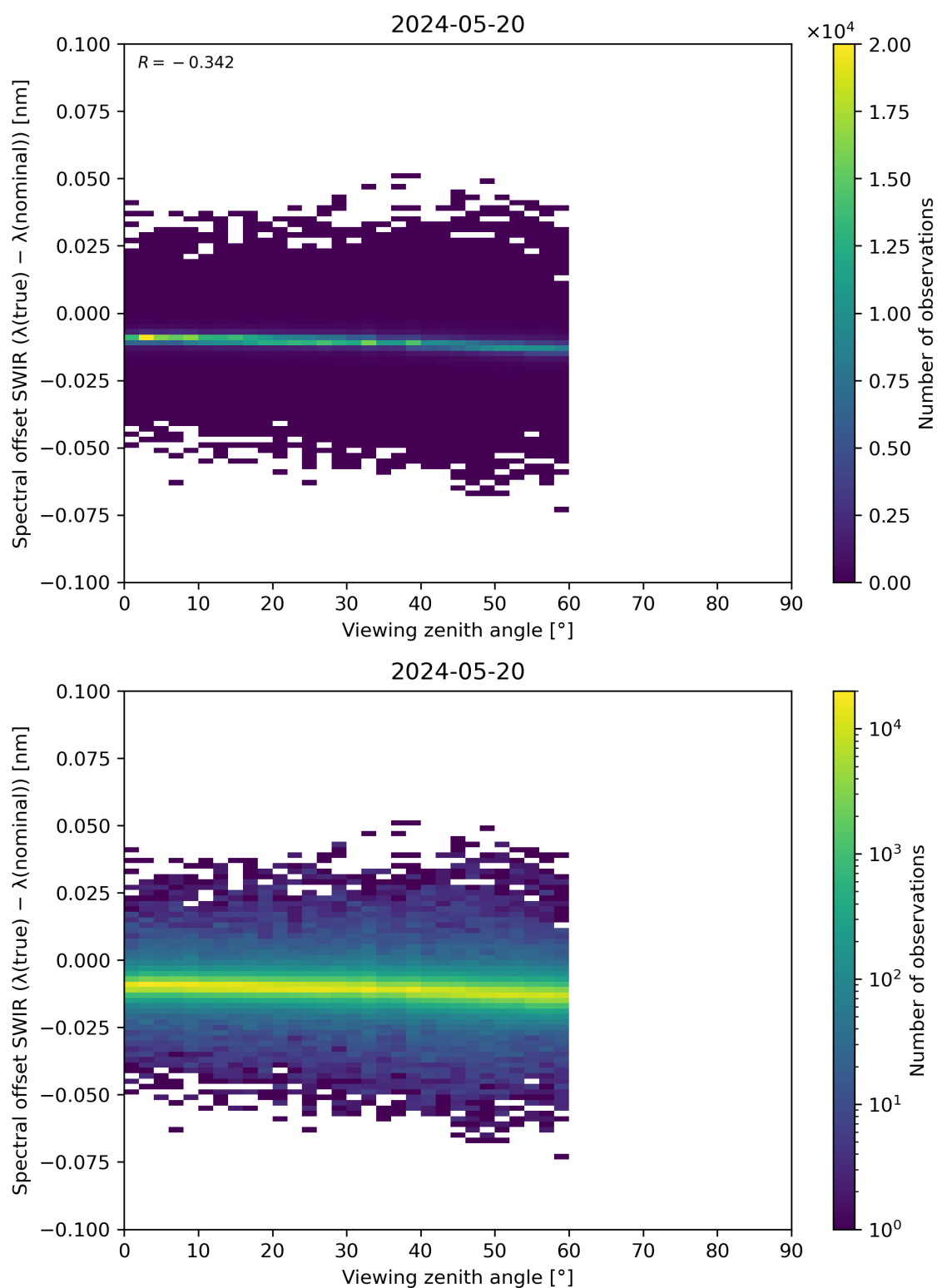
Figure 116: Scatter density plot of “Viewing zenith angle” against “Spectral offset SWIR ( \lambda(\text{true}) - \lambda(\text{nominal}) )” for 2024-05-19 to 2024-05-21.
