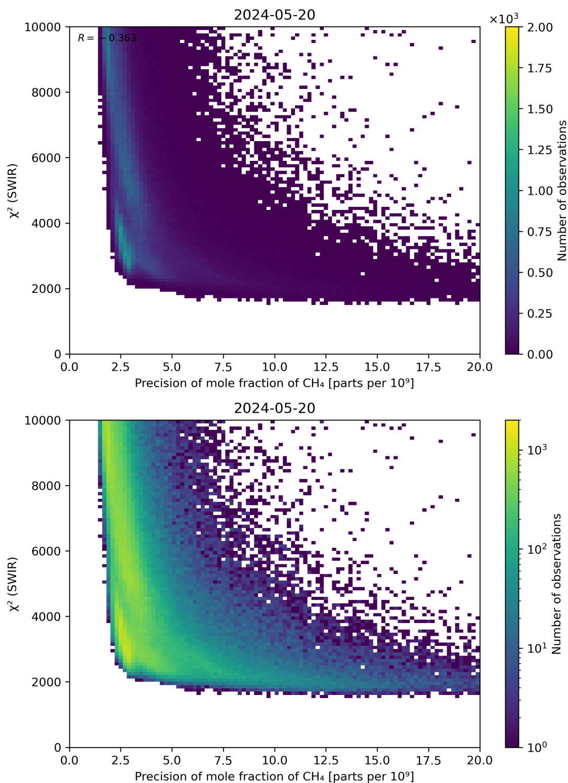
Figure 79: Scatter density plot of “Precision of mole fraction of \text{CH}_4 ” against “ \chi^2 (SWIR)” for 2024-05-19 to 2024-05-21.
