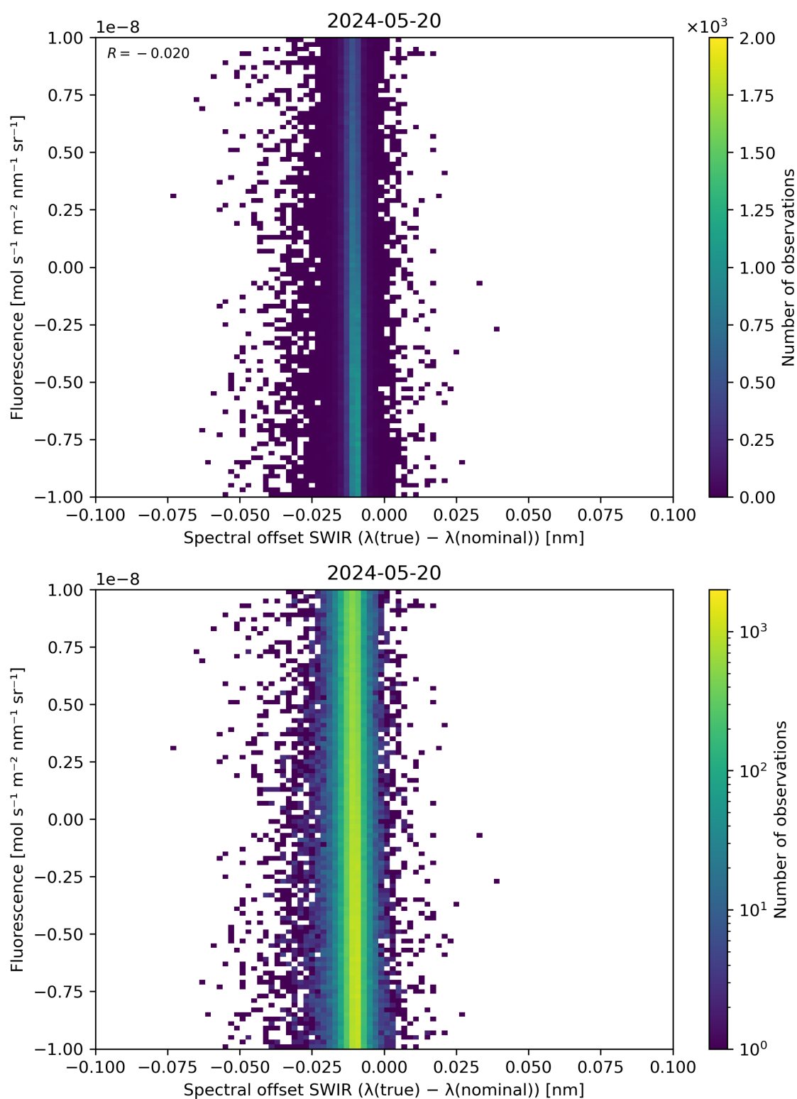
Figure 120: Scatter density plot of “Spectral offset SWIR ( \lambda(\text{true}) - \lambda(\text{nominal}) )” against “Fluorescence” for 2024-05-19 to 2024-05-21.
