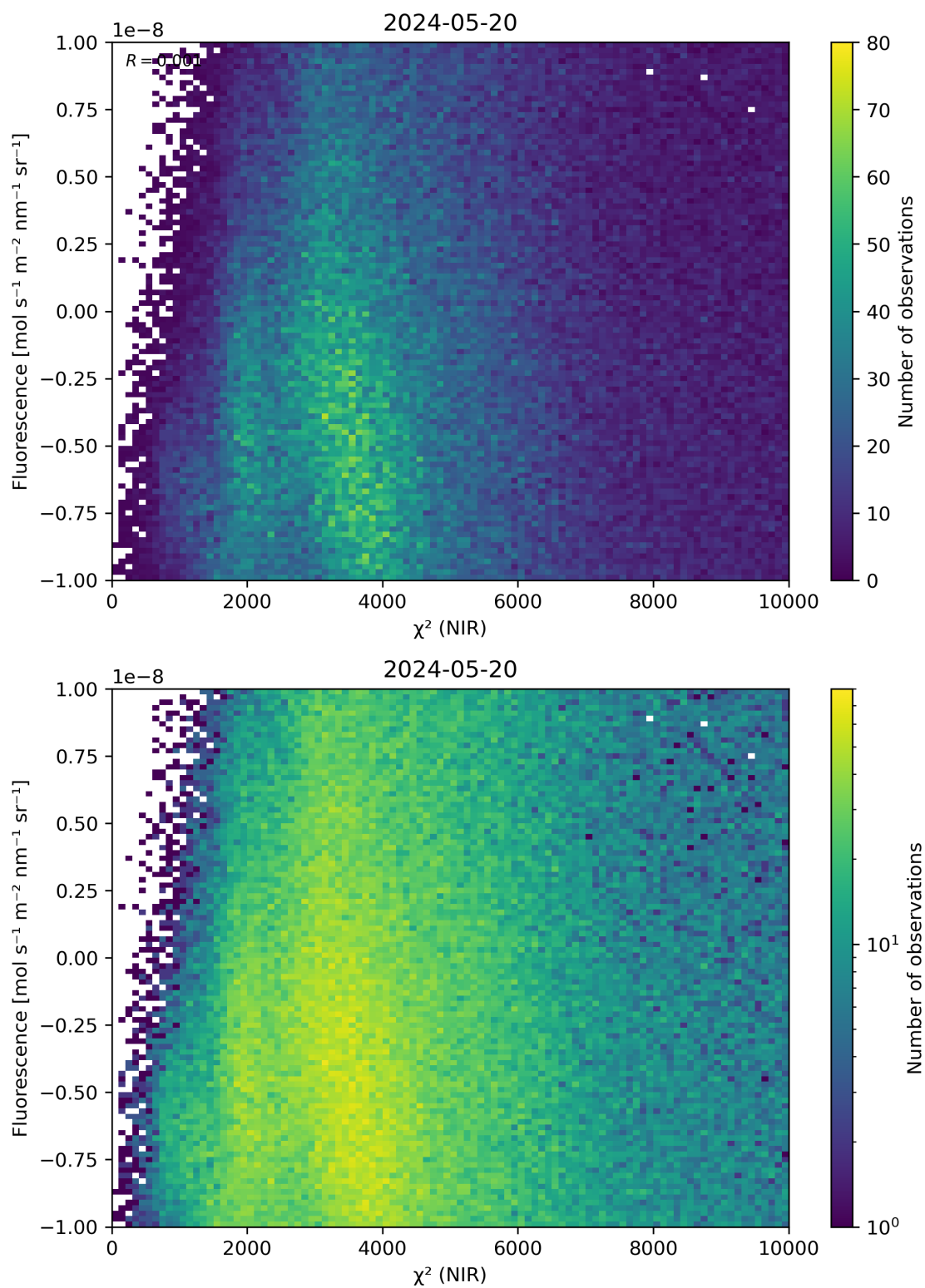
Figure 45: Scatter density plot of “ \chi^2 (NIR)” against “Fluorescence” for 2024-05-19 to 2024-05-21.
