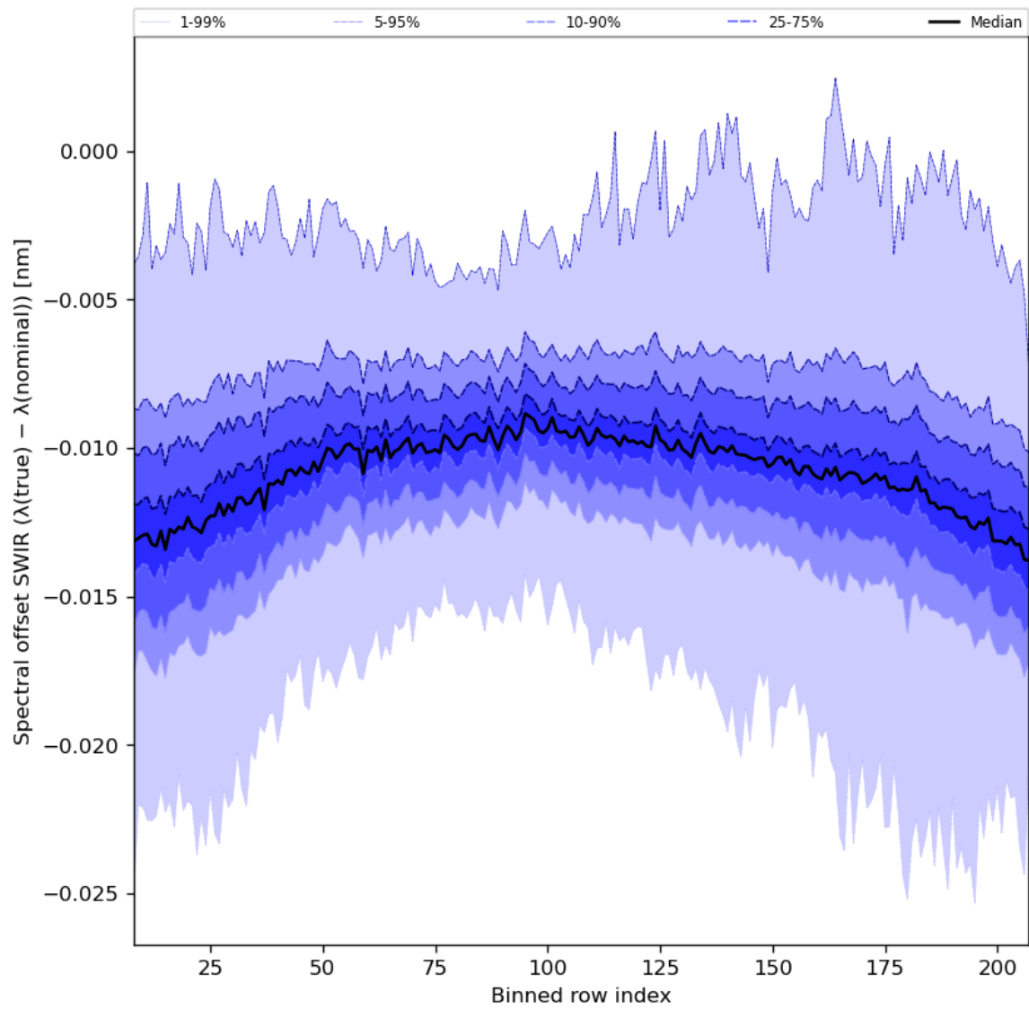
Figure 38: Along track statistics of “Spectral offset SWIR ( \lambda(\text{true}) - \lambda(\text{nominal}) )” for 2024-05-19 to 2024-05-21
