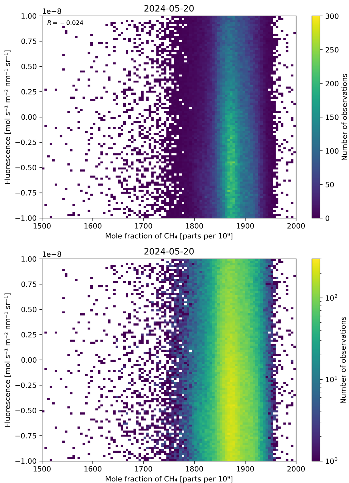
Figure 73: Scatter density plot of “Mole fraction of \text{CH}_4 ” against “Fluorescence” for 2024-05-19 to 2024-05-21.
