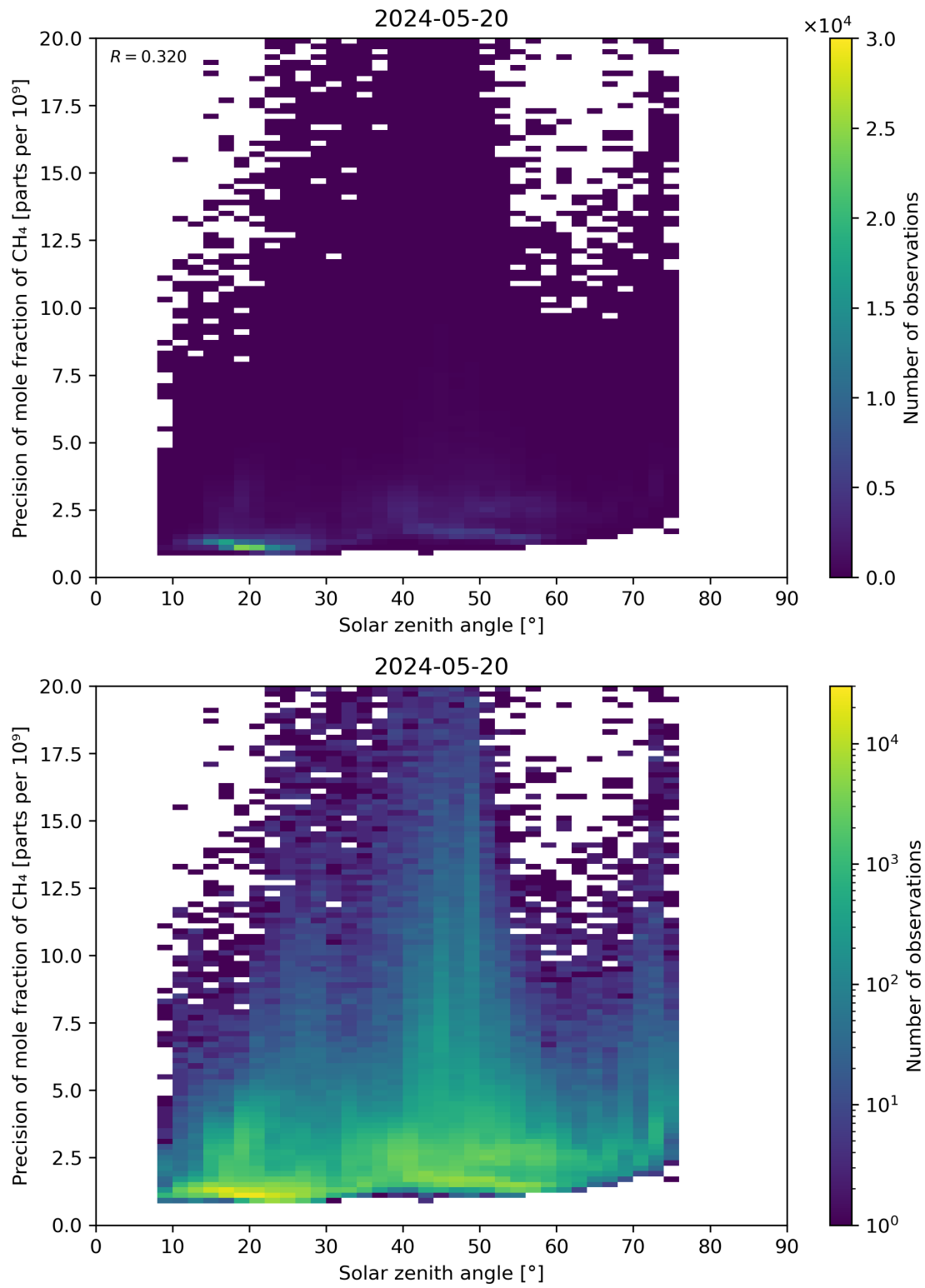
Figure 101: Scatter density plot of “Solar zenith angle” against “Precision of mole fraction of \text{CH}_4 ” for 2024-05-19 to 2024-05-21.
