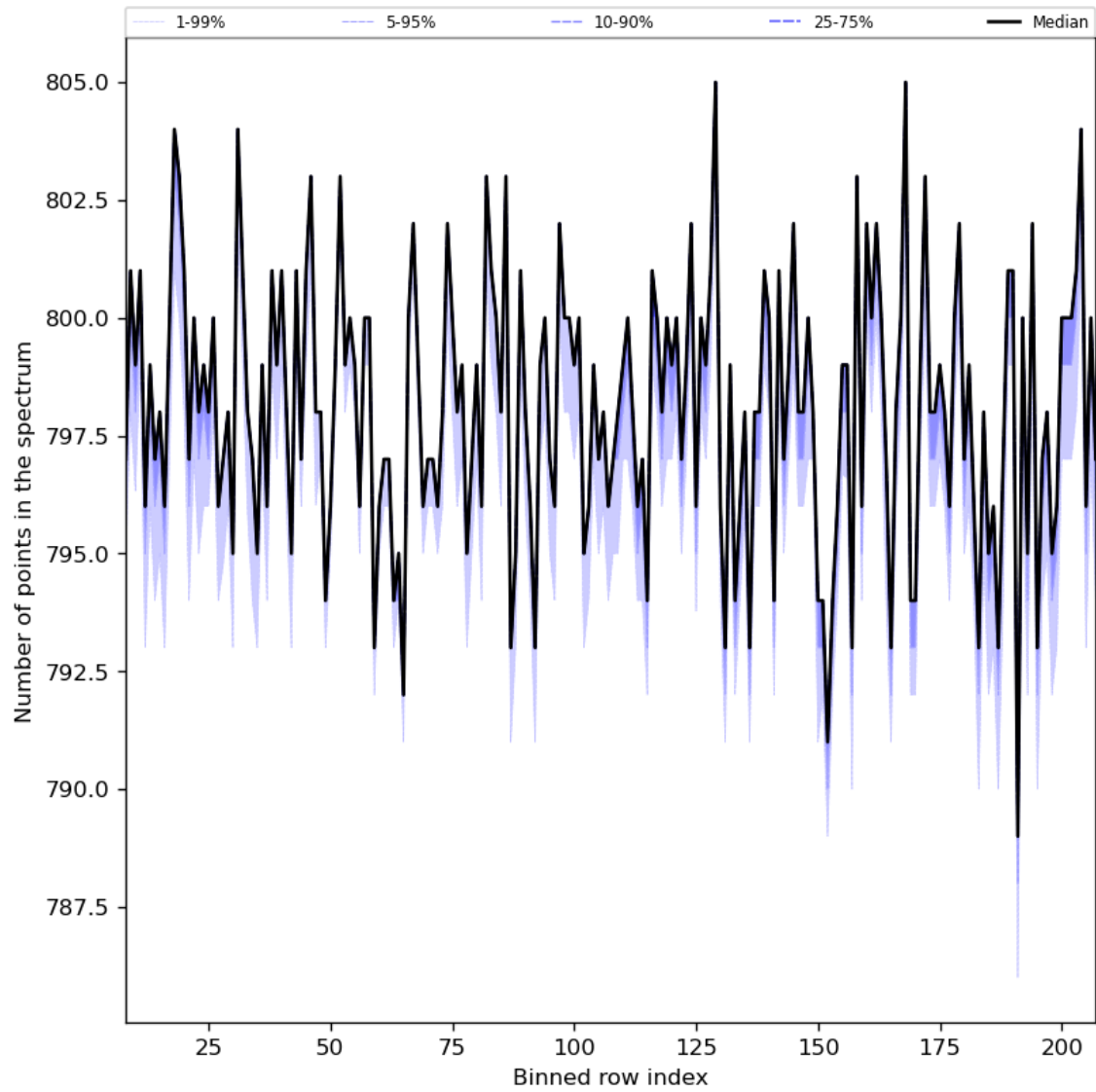
Figure 37: Along track statistics of “Number of points in the spectrum” for 2024-05-19 to 2024-05-21
