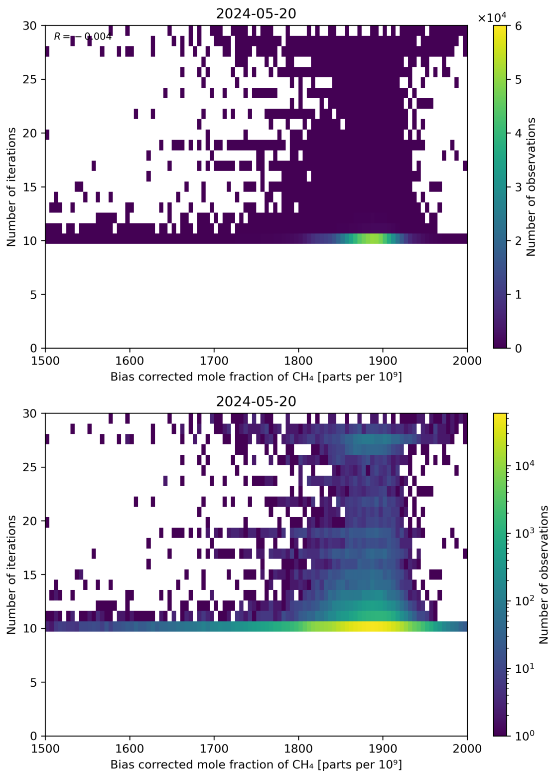
Figure 67: Scatter density plot of “Bias corrected mole fraction of CH 4 ” against “Number of iterations” for 2024-05-19 to 2024-05-21.
