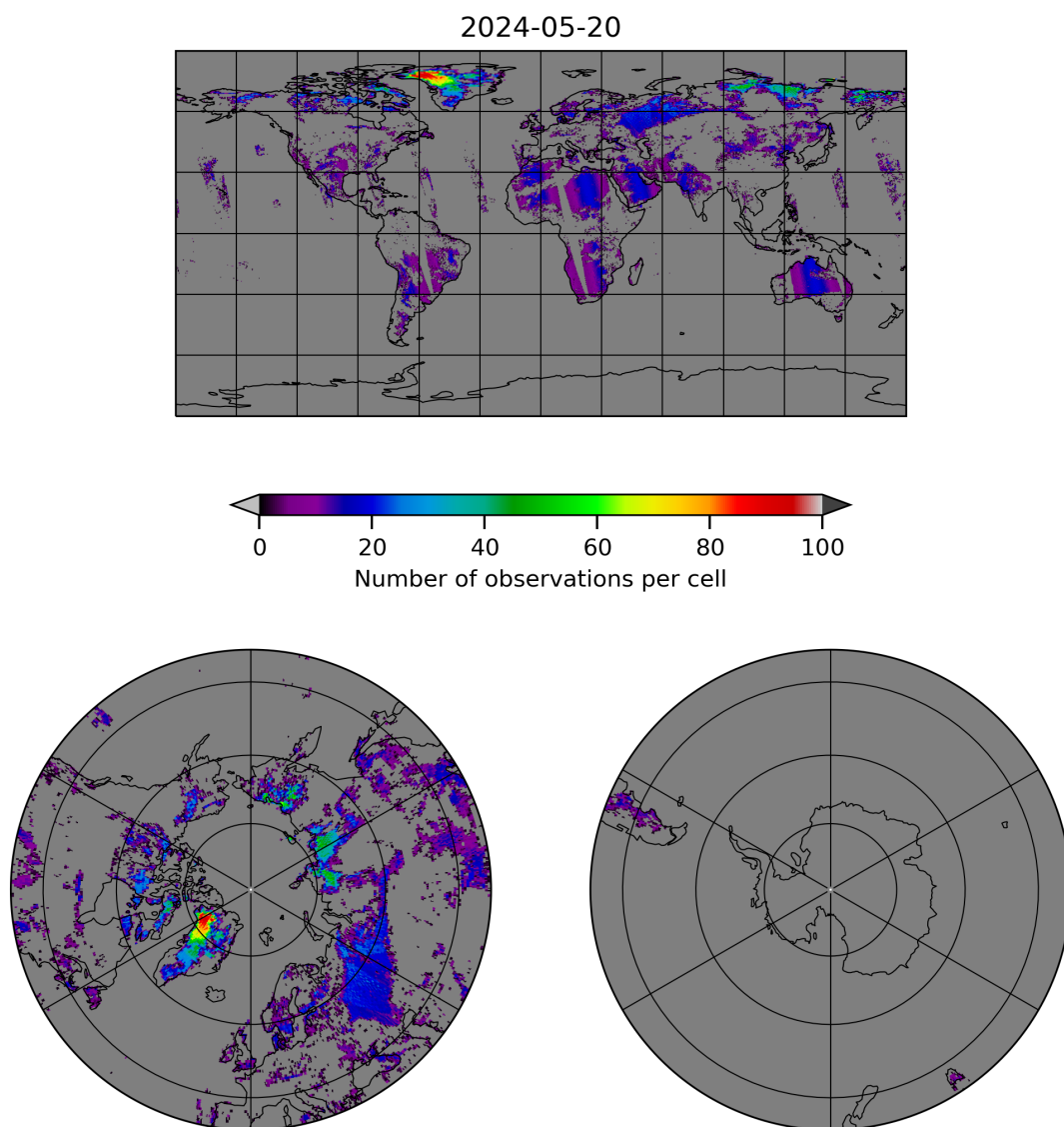
Figure 10: Map of the number of observations for 2024-05-19 to 2024-05-21
