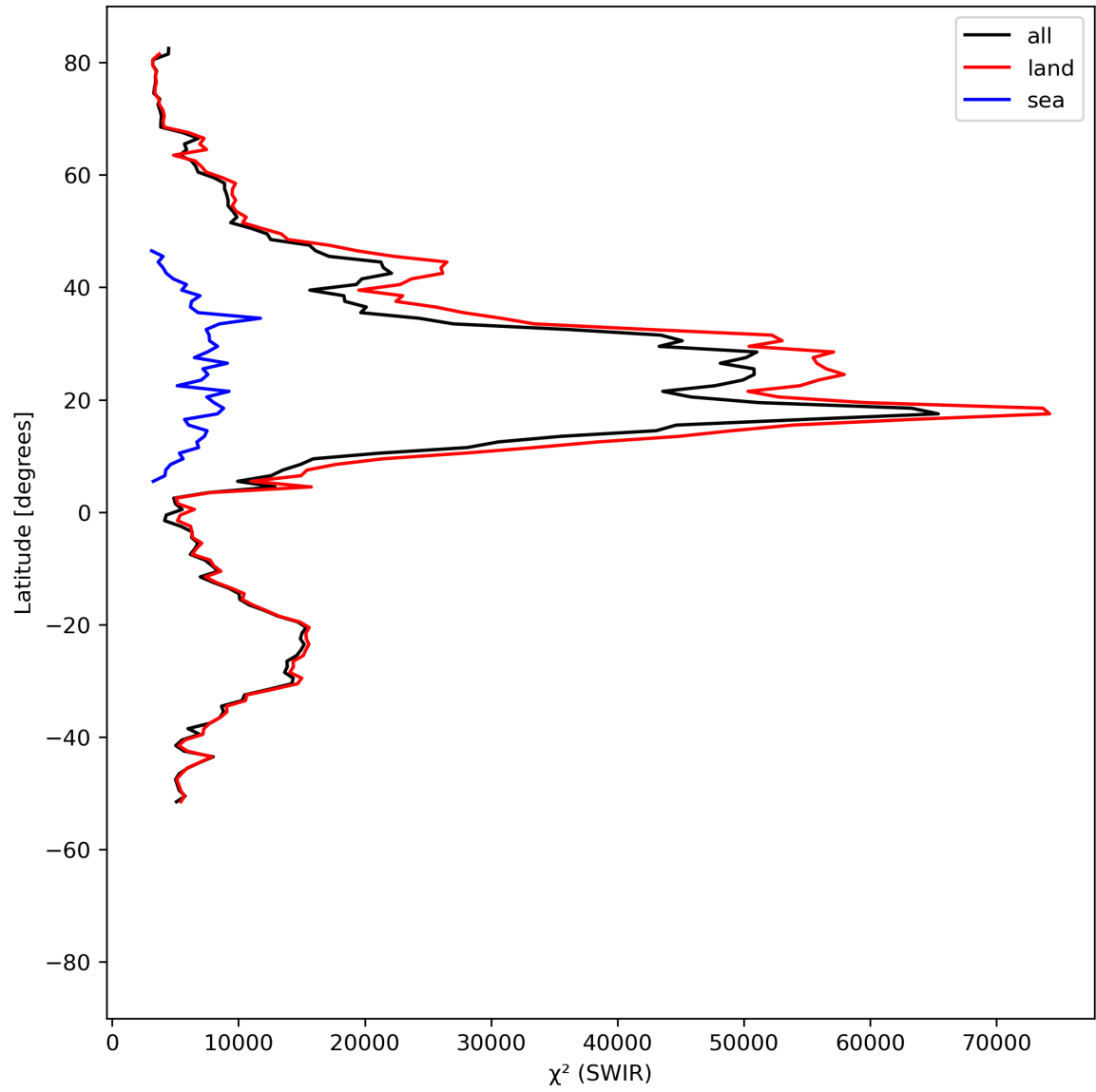
Figure 17: Zonal average of “ \chi^2 (SWIR)” for 2024-05-19 to 2024-05-21.
