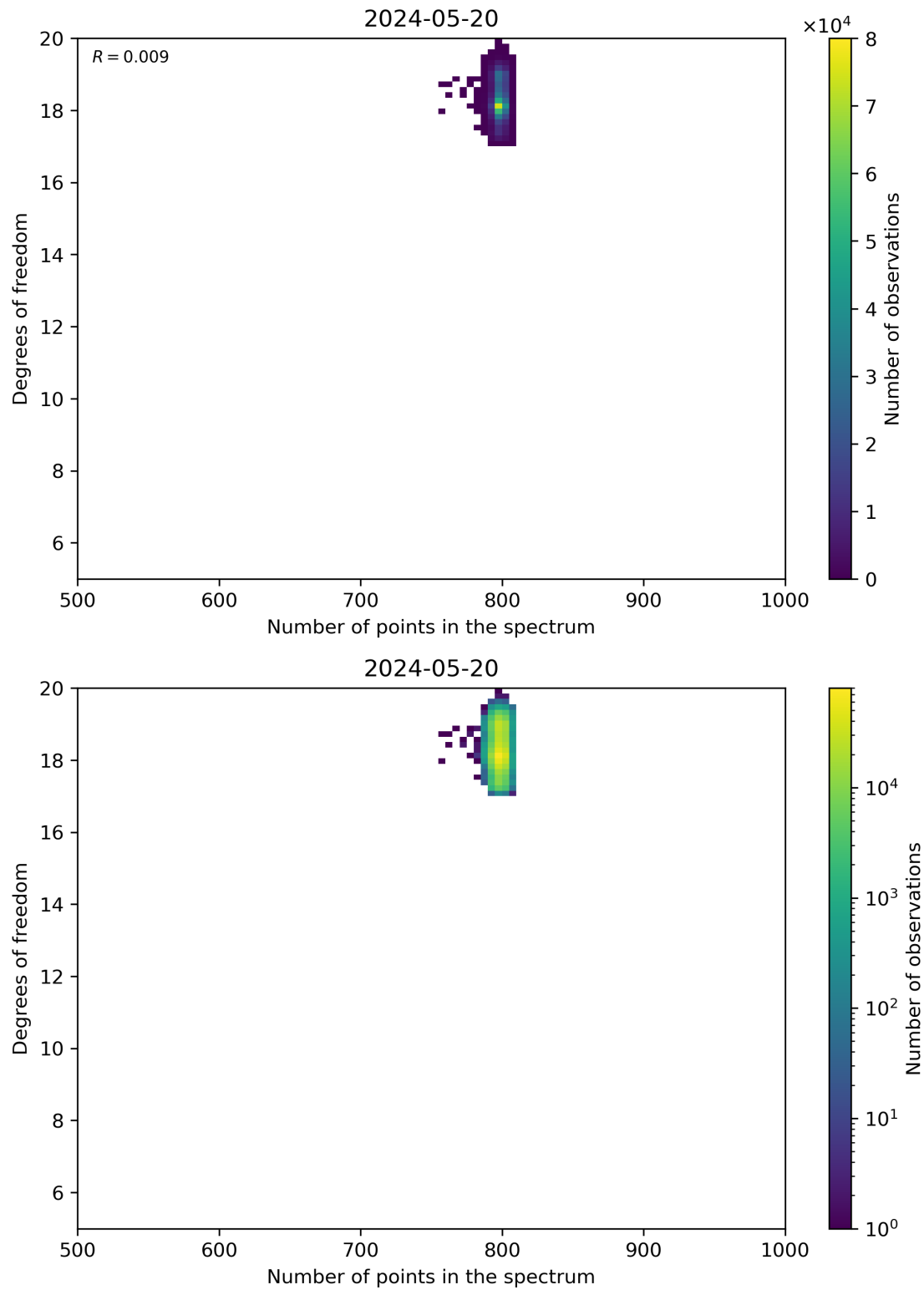
Figure 90: Scatter density plot of “Number of points in the spectrum” against “Degrees of freedom” for 2024-05-19 to 2024-05-21.
