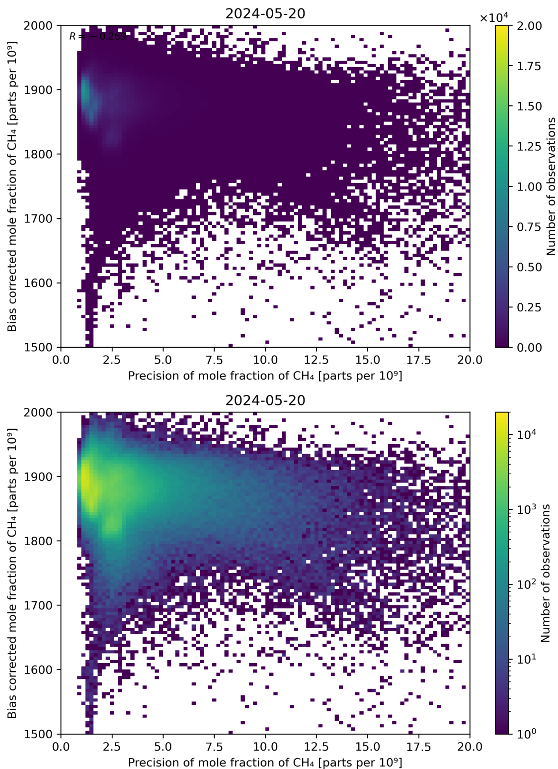
Figure 82: Scatter density plot of “Precision of mole fraction of CH 4 ” against “Bias corrected mole fraction of CH 4 ” for 2024-05-19 to 2024-05-21.
