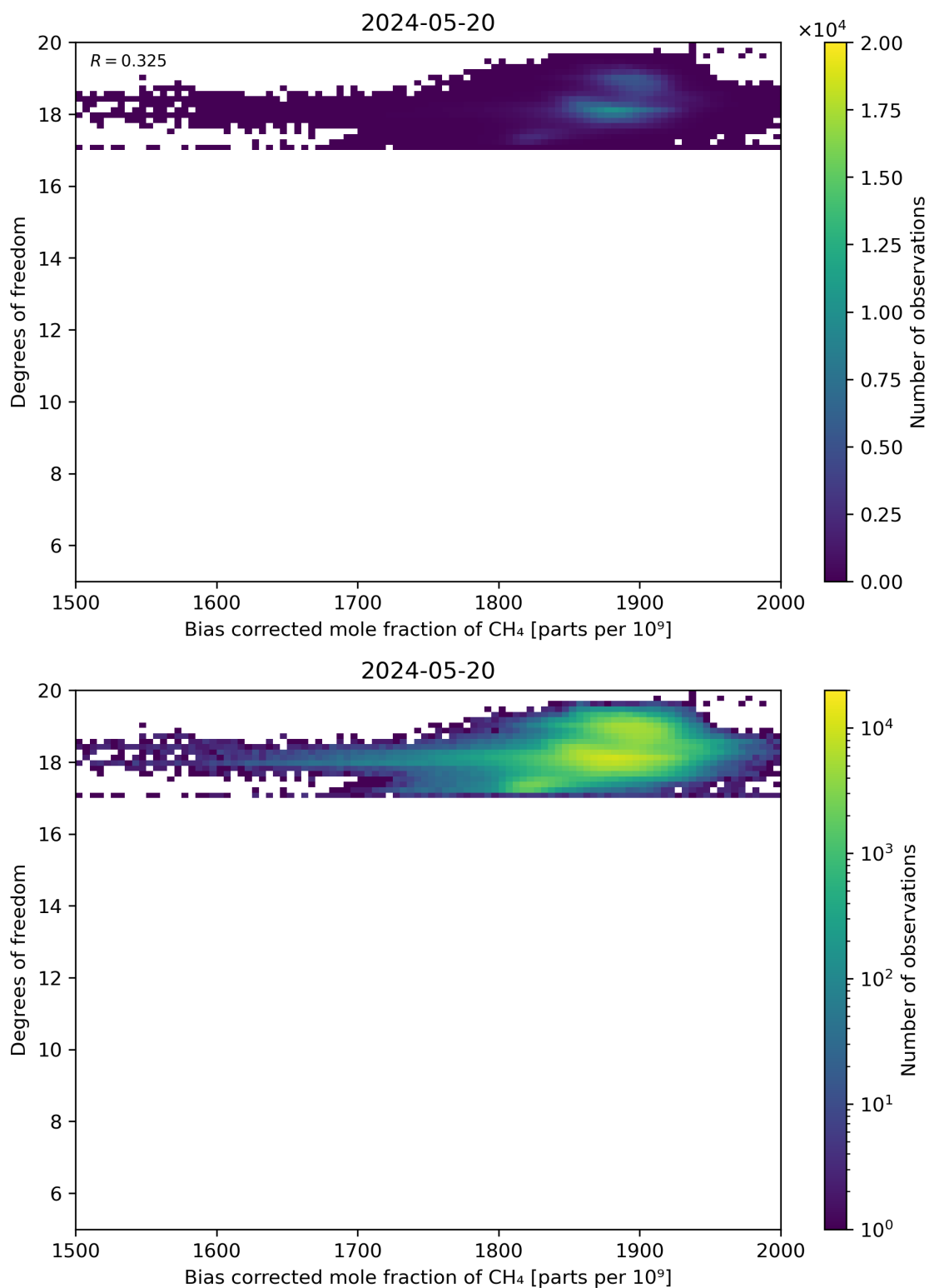
Figure 65: Scatter density plot of “Bias corrected mole fraction of CH 4 ” against “Degrees of freedom” for 2024-05-19 to 2024-05-21.
