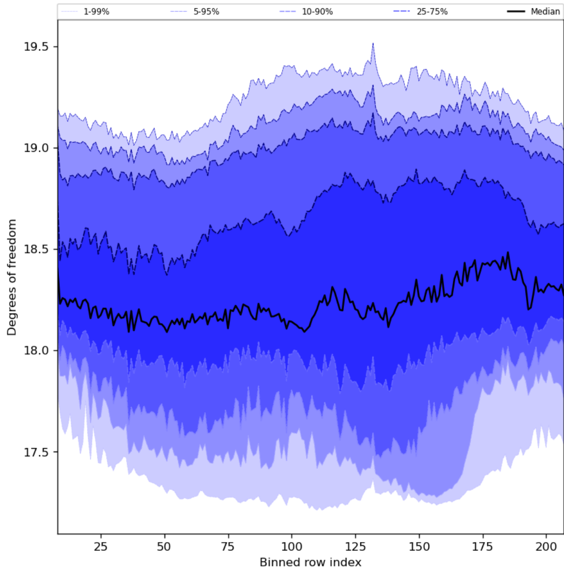
Figure 41: Along track statistics of “Degrees of freedom” for 2024-05-19 to 2024-05-21
