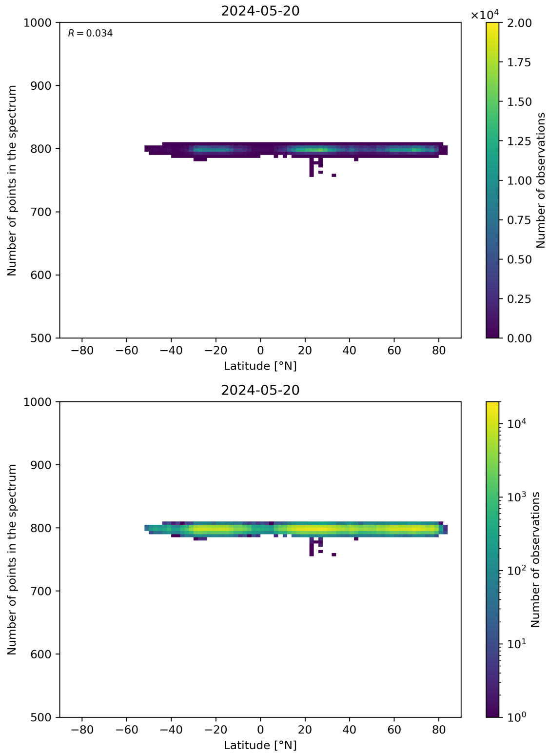
Figure 61: Scatter density plot of “Latitude” against “Number of points in the spectrum” for 2024-05-19 to 2024-05-21.
