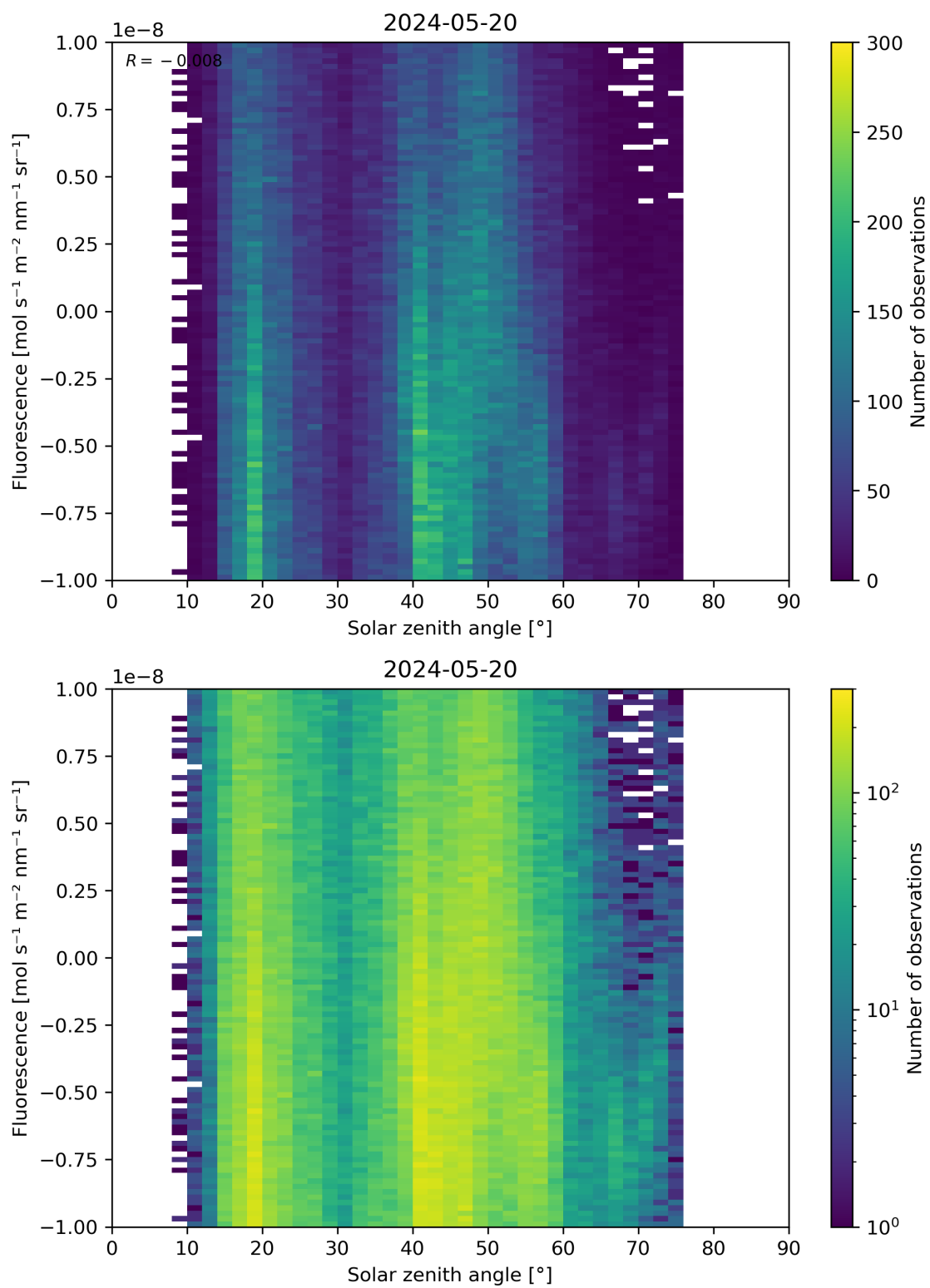
Figure 97: Scatter density plot of “Solar zenith angle” against “Fluorescence” for 2024-05-19 to 2024-05-21.
