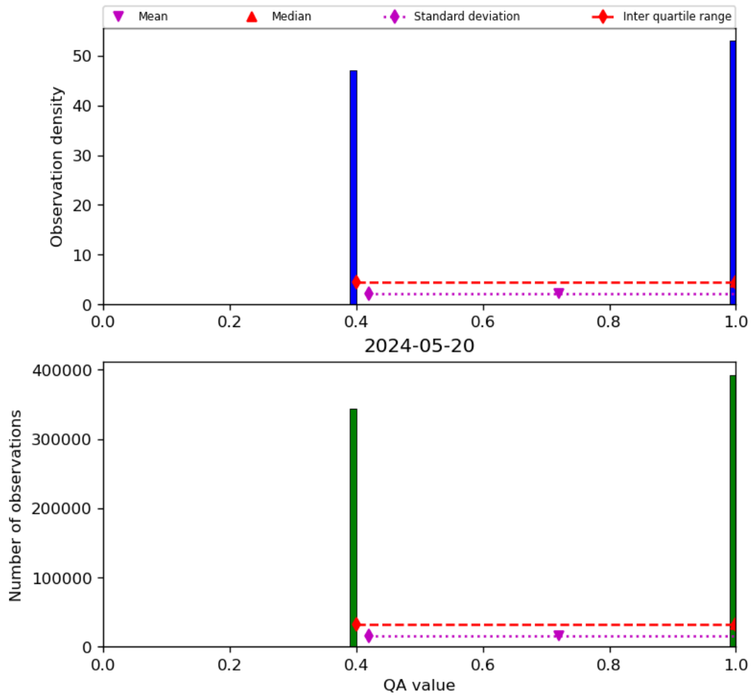
Figure 22: Histogram of “QA value” for 2024-05-19 to 2024-05-21
