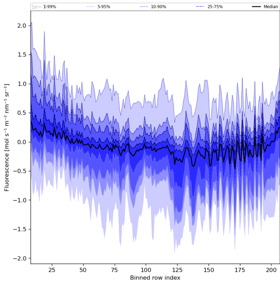
Figure 43: Along track statistics of “Fluorescence” for 2024-05-19 to 2024-05-21
