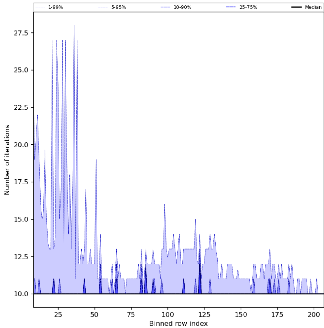
Figure 42: Along track statistics of “Number of iterations” for 2024-05-19 to 2024-05-21
