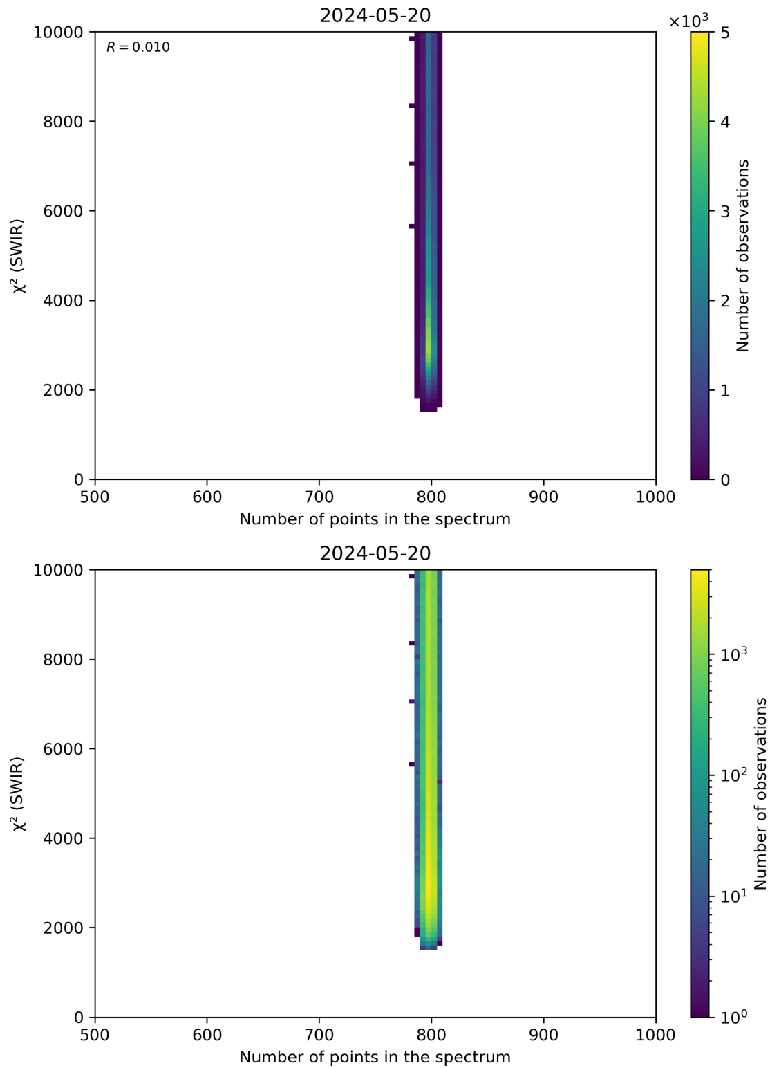
Figure 89: Scatter density plot of “Number of points in the spectrum” against “ \chi^2 (SWIR)” for 2024-05-19 to 2024-05-21.
