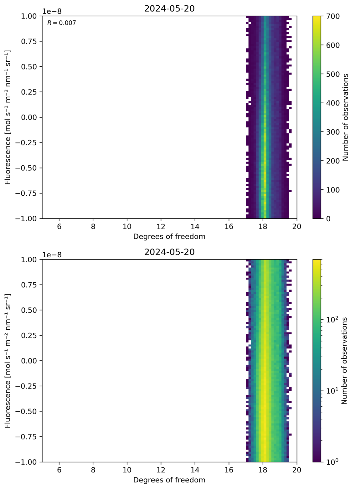
Figure 51: Scatter density plot of “Degrees of freedom” against “Fluorescence” for 2024-05-19 to 2024-05-21.
