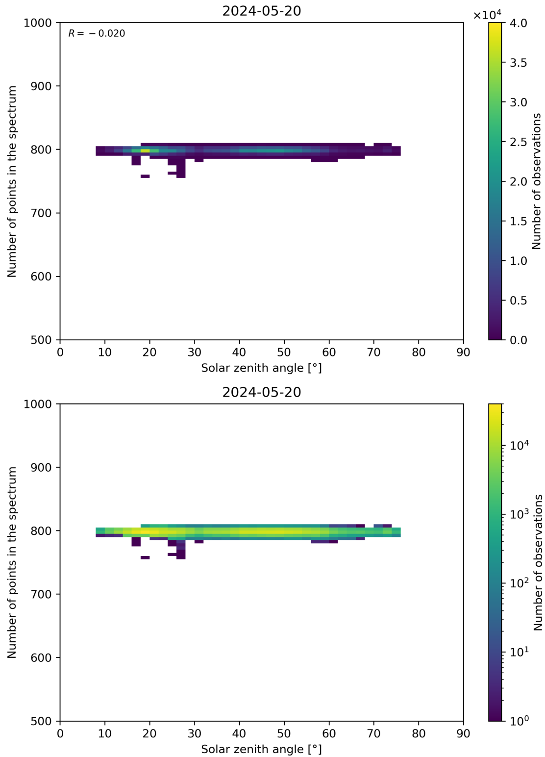
Figure 103: Scatter density plot of “Solar zenith angle” against “Number of points in the spectrum” for 2024-05-19 to 2024-05-21.
