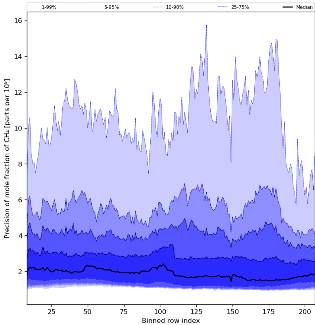
Figure 35: Along track statistics of “Precision of mole fraction of CH 4 ” for 2024-05-19 to 2024-05-21
