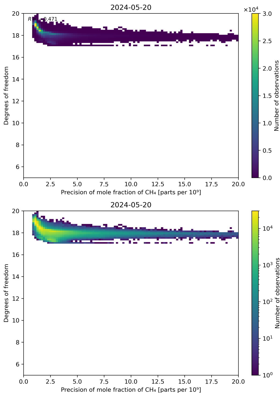
Figure 80: Scatter density plot of “Precision of mole fraction of CH 4 ” against “Degrees of freedom” for 2024-05-19 to 2024-05-21.
