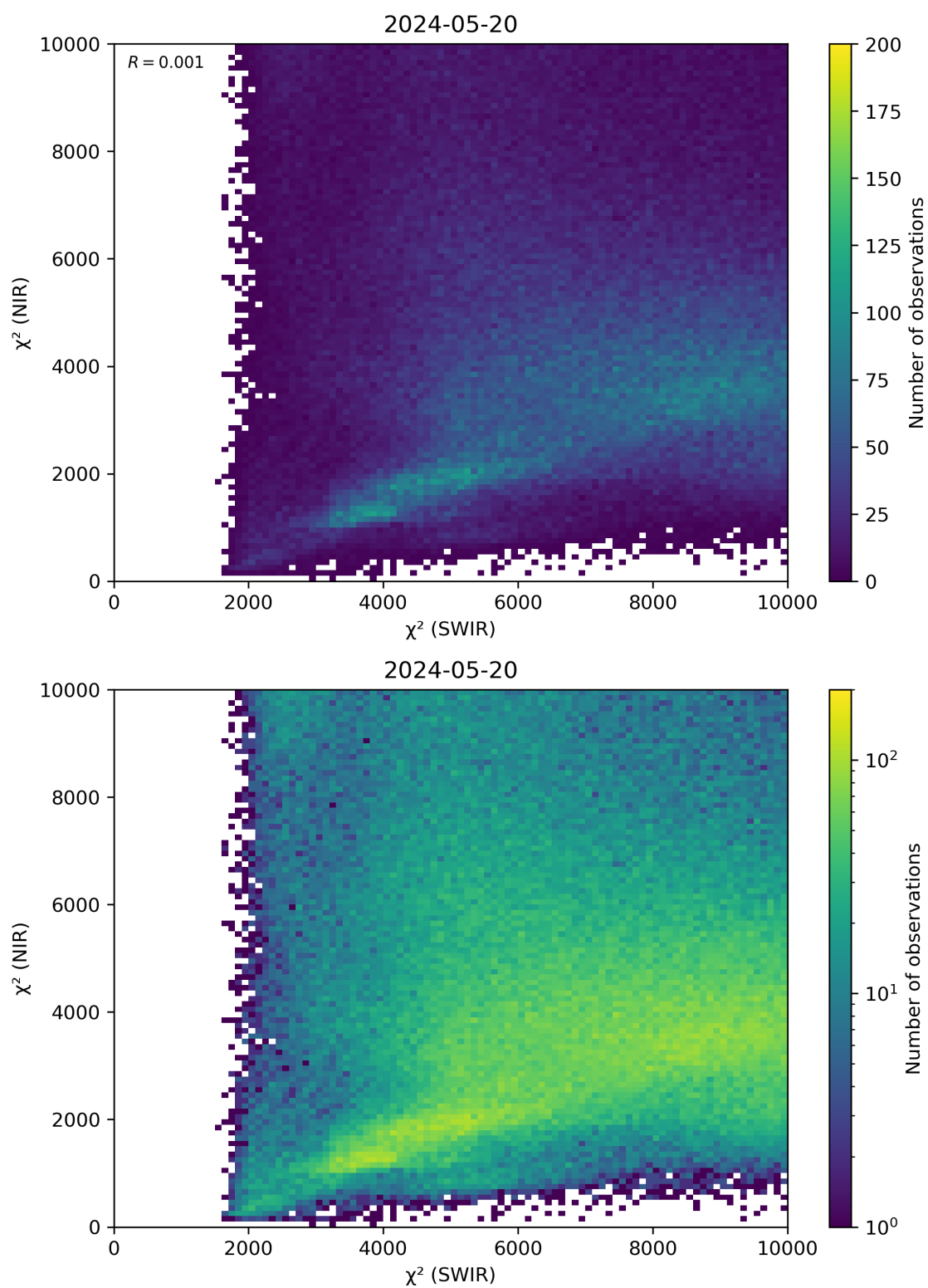
Figure 47: Scatter density plot of “ \chi^2 (SWIR)” against “ \chi^2 (NIR)” for 2024-05-19 to 2024-05-21.
