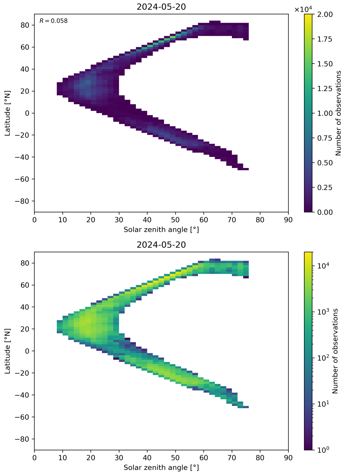
Figure 98: Scatter density plot of “Solar zenith angle” against “Latitude” for 2024-05-19 to 2024-05-21.
