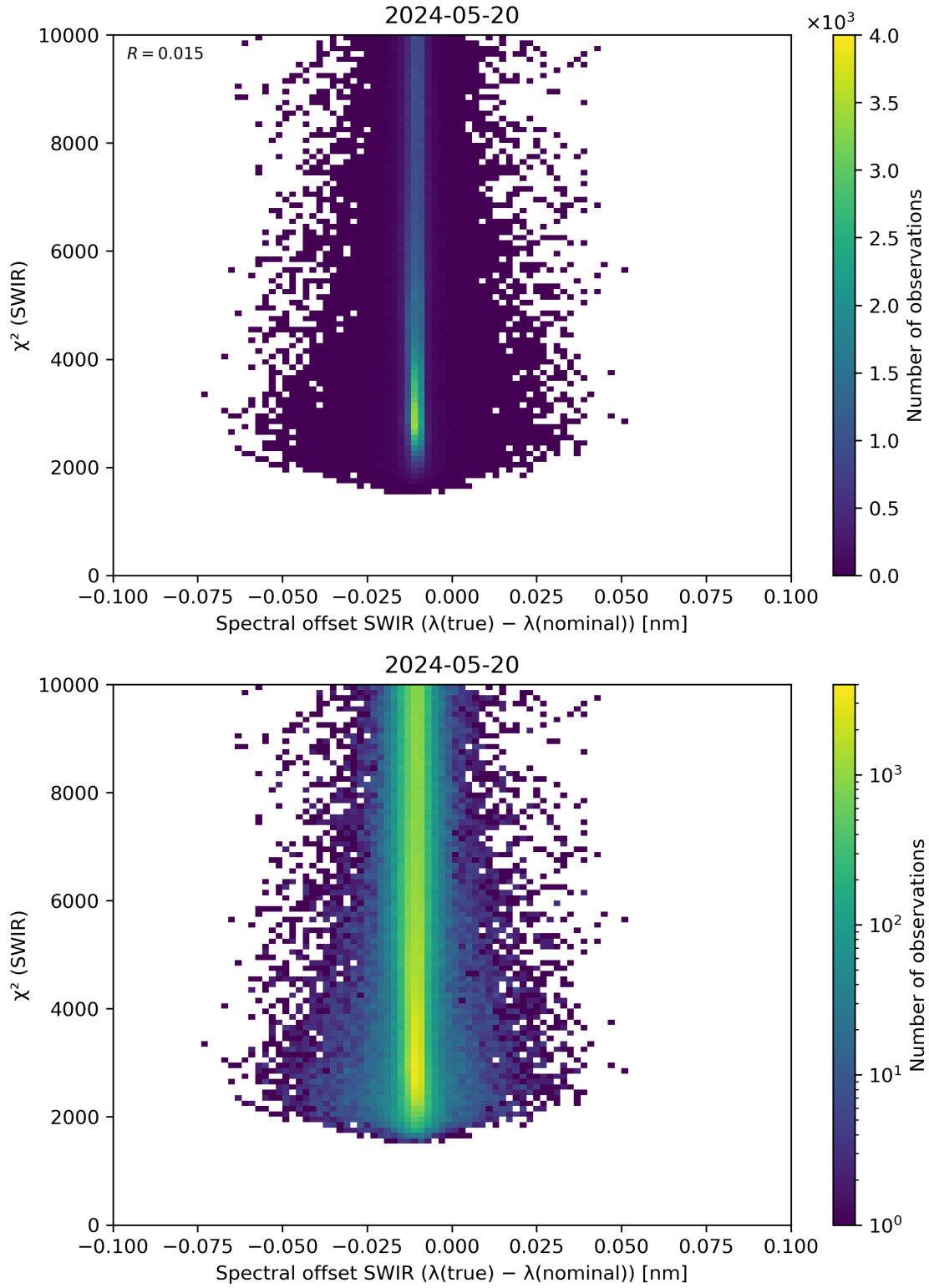
Figure 118: Scatter density plot of “Spectral offset SWIR ( \lambda(\text{true}) - \lambda(\text{nominal}) )” against “ \chi^2 (SWIR)” for 2024-05-19 to 2024-05-21.
