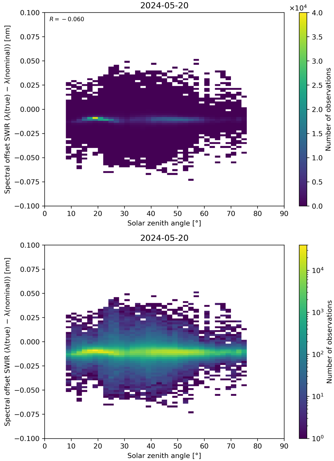
Figure 104: Scatter density plot of “Solar zenith angle” against “Spectral offset SWIR ( \lambda(\text{true}) - \lambda(\text{nominal}) )” for 2024-05-19 to 2024-05-21.
