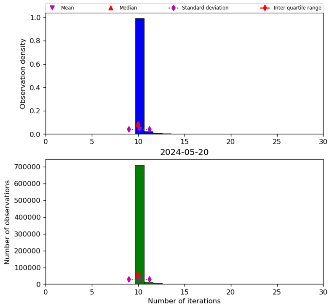
Figure 31: Histogram of “Number of iterations” for 2024-05-19 to 2024-05-21
