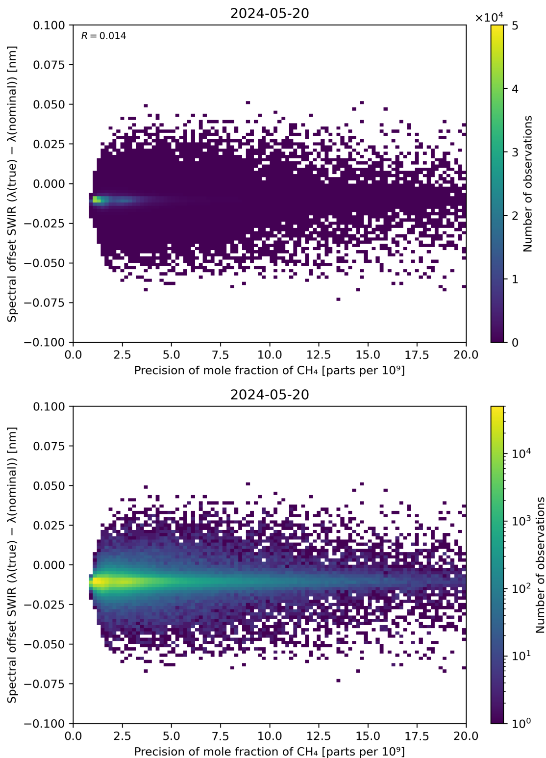
Figure 85: Scatter density plot of “Precision of mole fraction of CH 4 ” against “Spectral offset SWIR ( \lambda(\text{true}) - \lambda(\text{nominal}) )” for 2024-05-19 to 2024-05-21.
