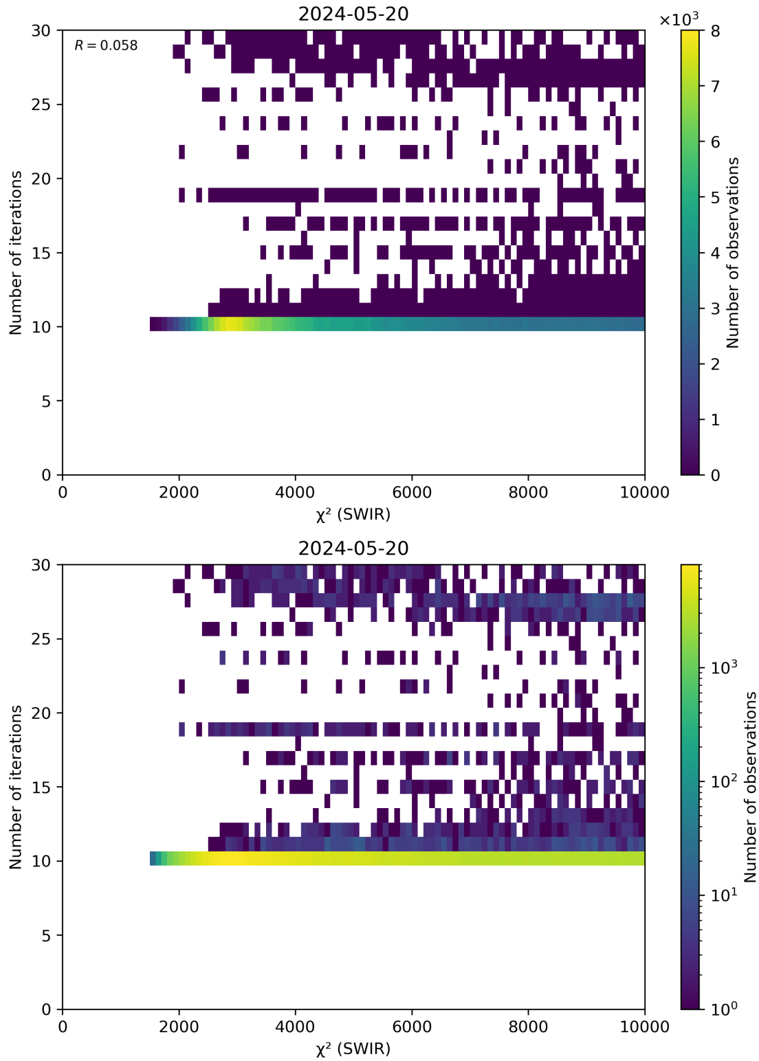
Figure 50: Scatter density plot of “ \chi^2 (SWIR)” against “Number of iterations” for 2024-05-19 to 2024-05-21.
