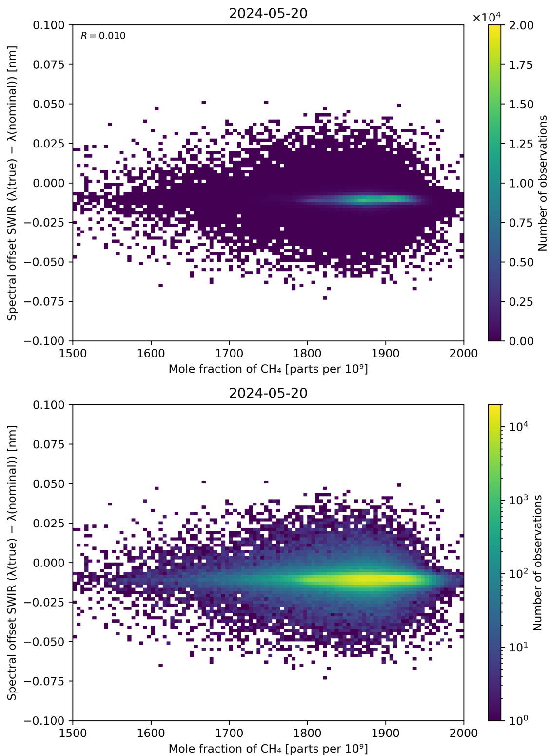
Figure 86: Scatter density plot of “Mole fraction of CH 4 ” against “Spectral offset SWIR ( \lambda(\text{true}) - \lambda(\text{nominal}) )” for 2024-05-19 to 2024-05-21.
