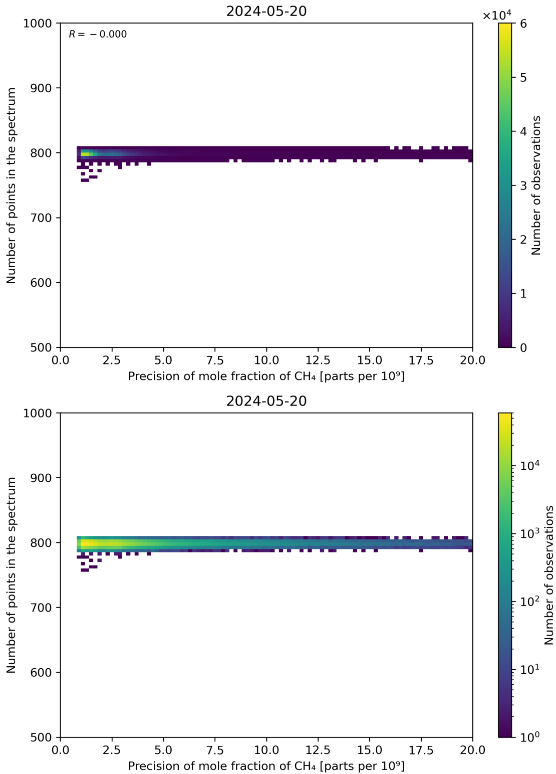
Figure 84: Scatter density plot of “Precision of mole fraction of CH 4 ” against “Number of points in the spectrum” for 2024-05-19 to 2024-05-21.
