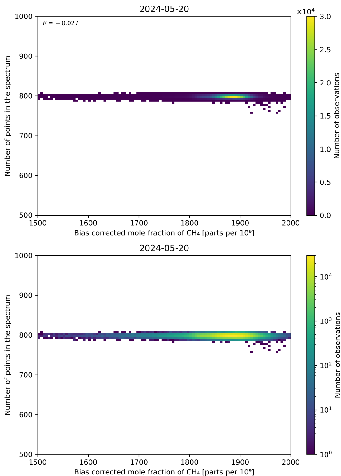
Figure 68: Scatter density plot of “Bias corrected mole fraction of CH 4 ” against “Number of points in the spectrum” for 2024-05-19 to 2024-05-21.
