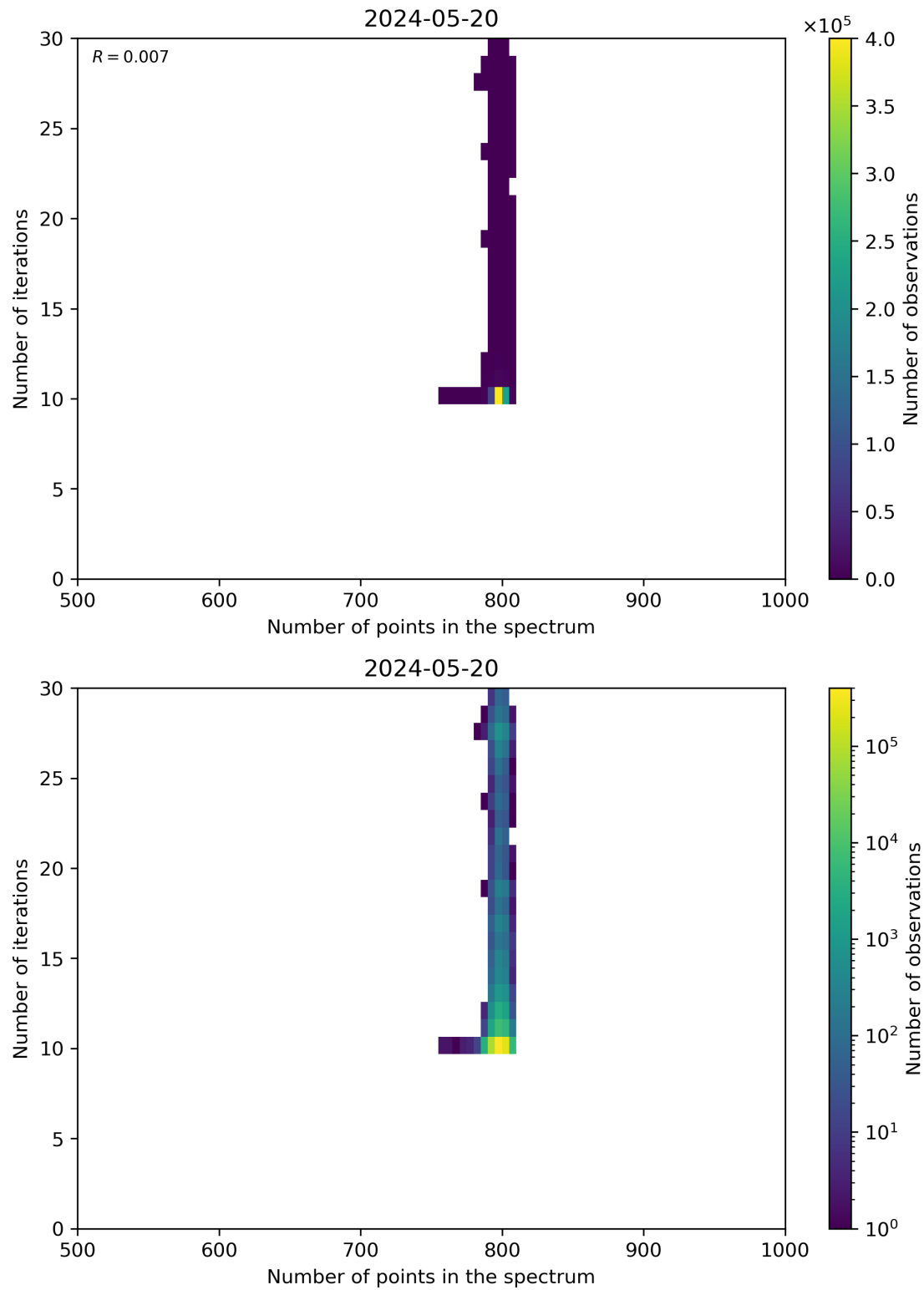
Figure 92: Scatter density plot of “Number of points in the spectrum” against “Number of iterations” for 2024-05-19 to 2024-05-21.
