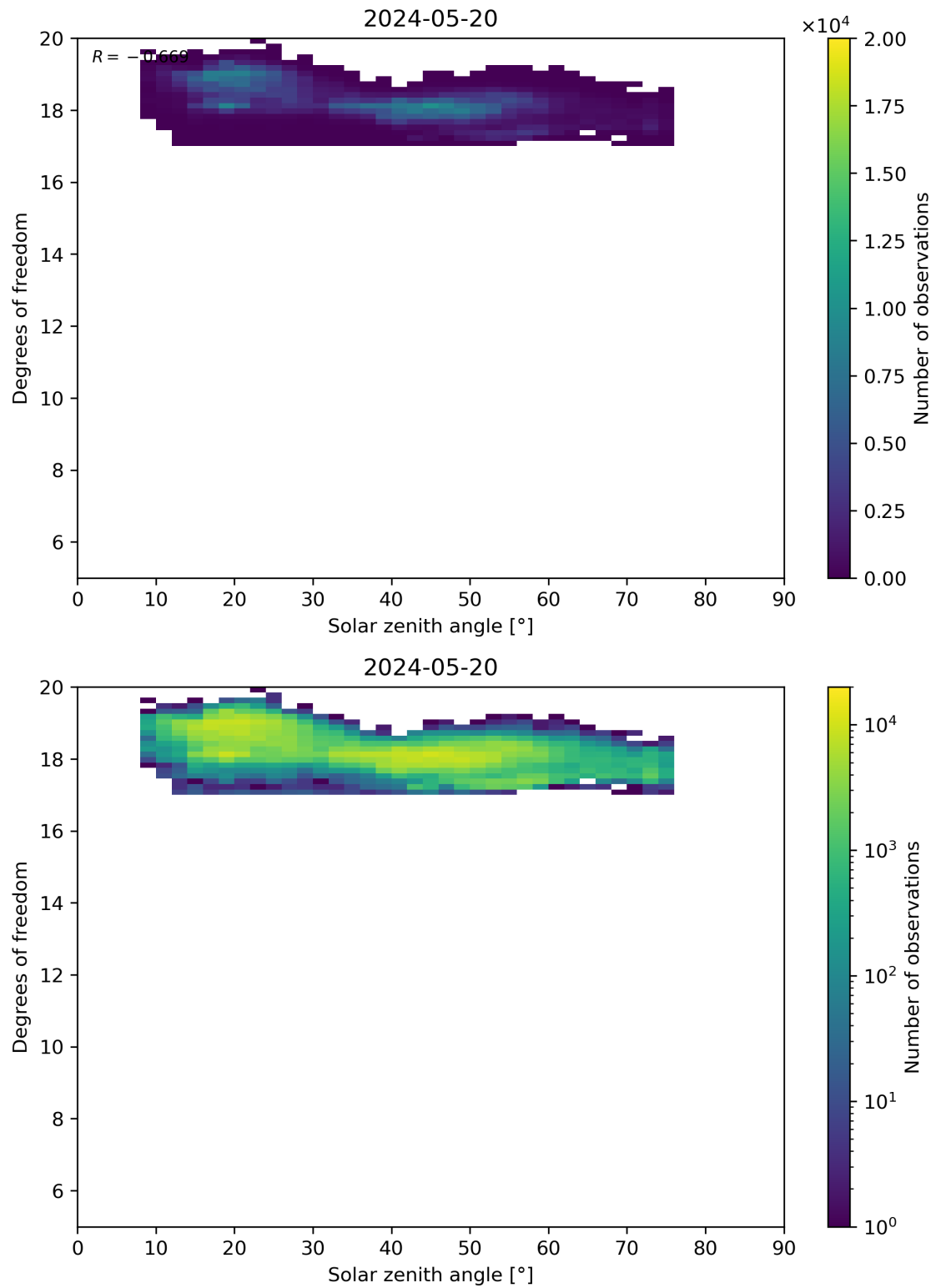
Figure 96: Scatter density plot of “Solar zenith angle” against “Degrees of freedom” for 2024-05-19 to 2024-05-21.
