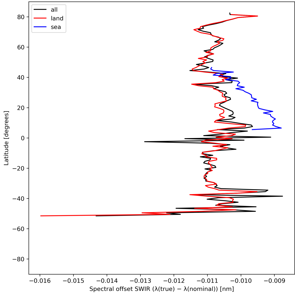
Figure 16: Zonal average of “Spectral offset SWIR ( \lambda(\text{true}) - \lambda(\text{nominal}) )” for 2024-05-19 to 2024-05-21.
