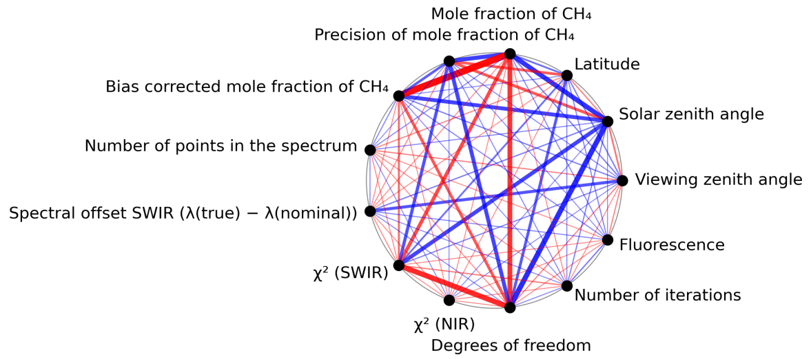
Figure 1: Map of correlation graph for 2024-05-19 to 2024-05-21.
