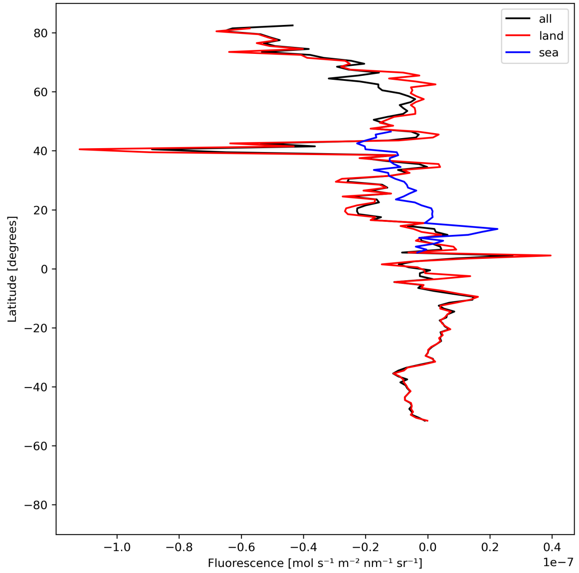
Figure 21: Zonal average of “Fluorescence” for 2024-05-19 to 2024-05-21.
