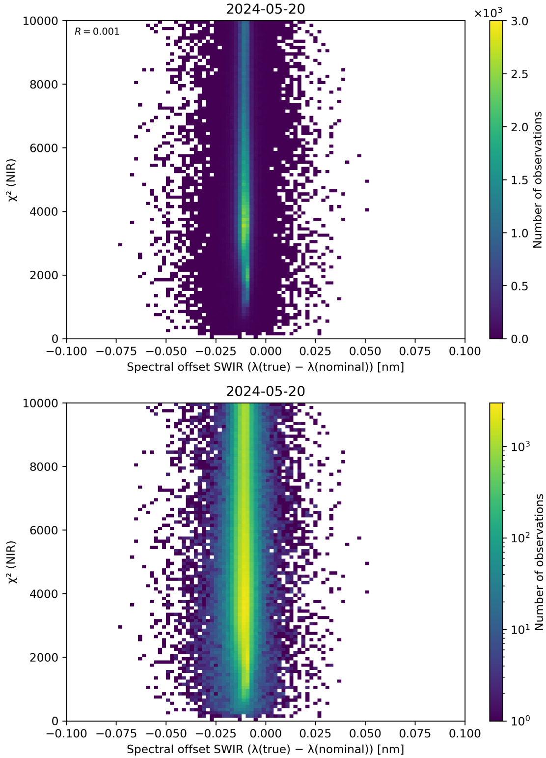
Figure 117: Scatter density plot of “Spectral offset SWIR ( \lambda(\text{true}) - \lambda(\text{nominal}) )” against “ \chi^2 (NIR)” for 2024-05-19 to 2024-05-21.
