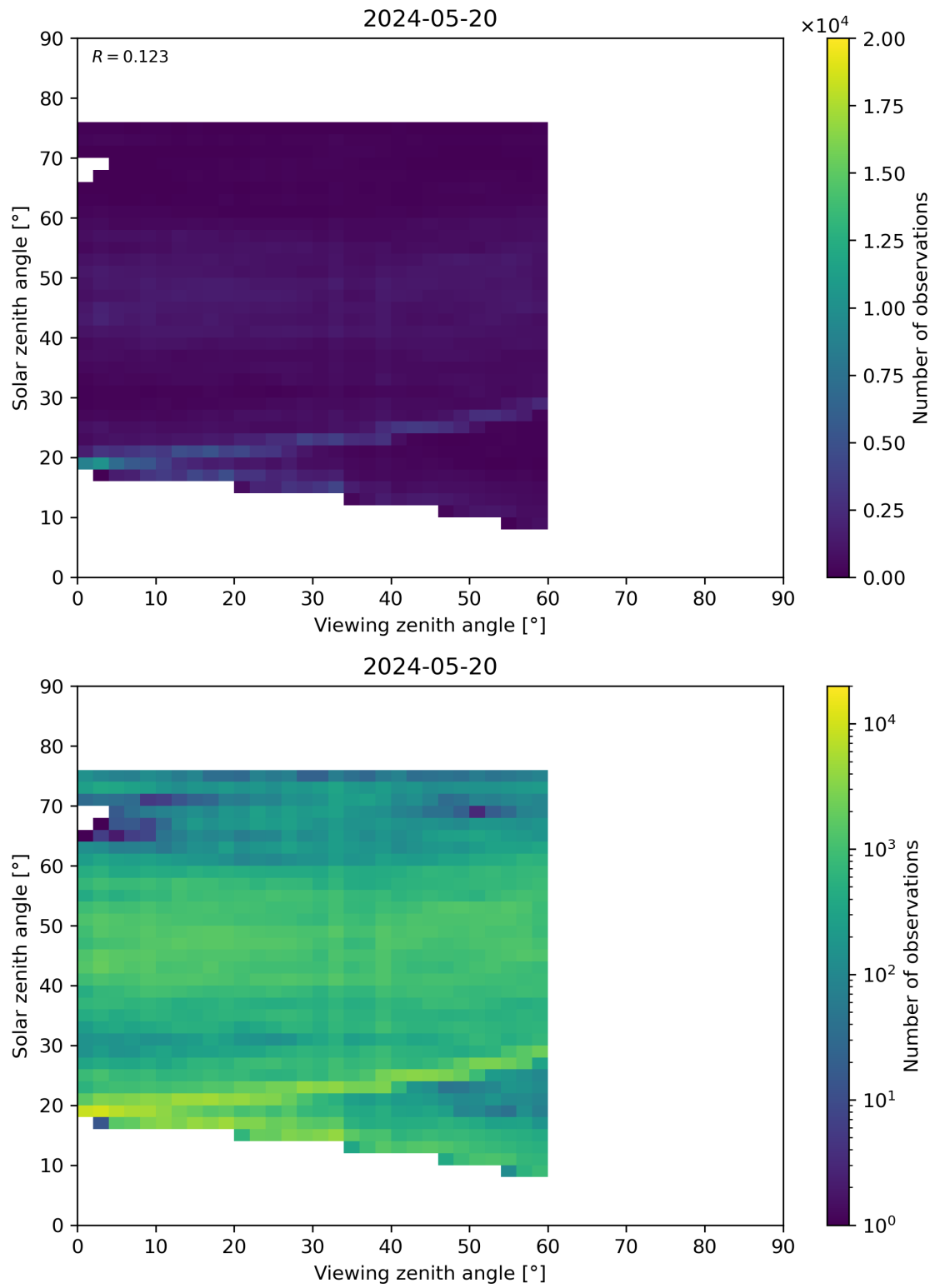
Figure 115: Scatter density plot of “Viewing zenith angle” against “Solar zenith angle” for 2024-05-19 to 2024-05-21.
