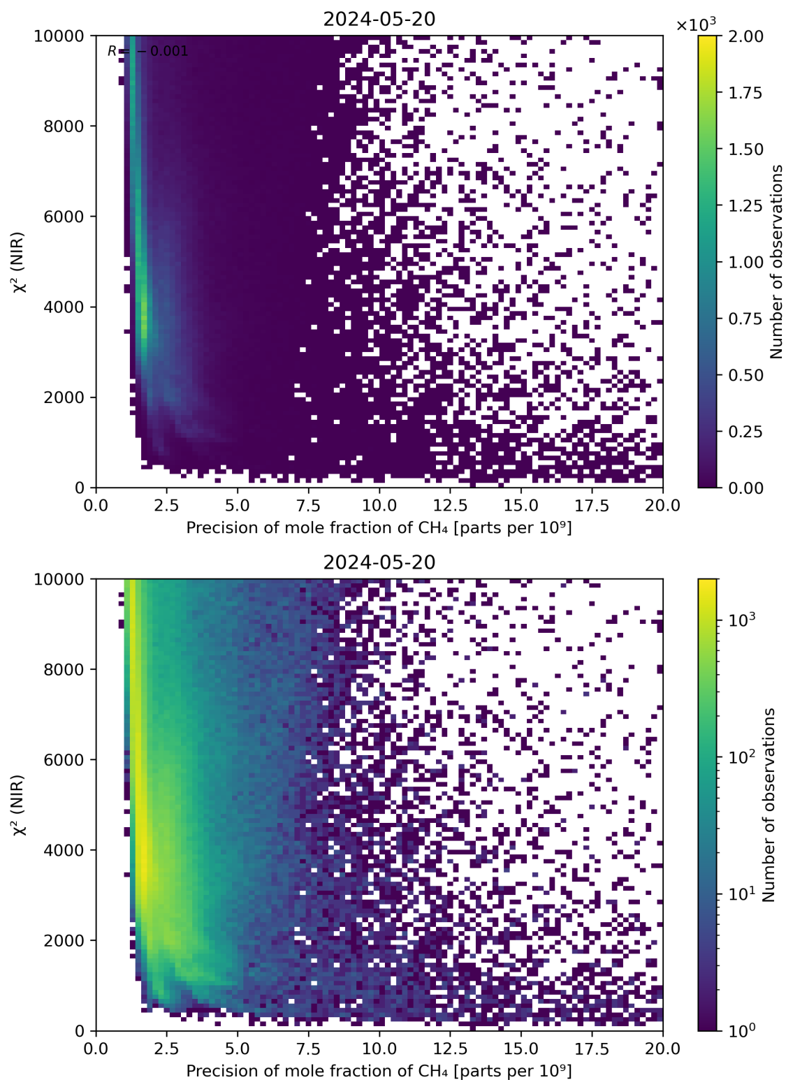
Figure 78: Scatter density plot of “Precision of mole fraction of \text{CH}_4 ” against “ \chi^2 (NIR)” for 2024-05-19 to 2024-05-21.
