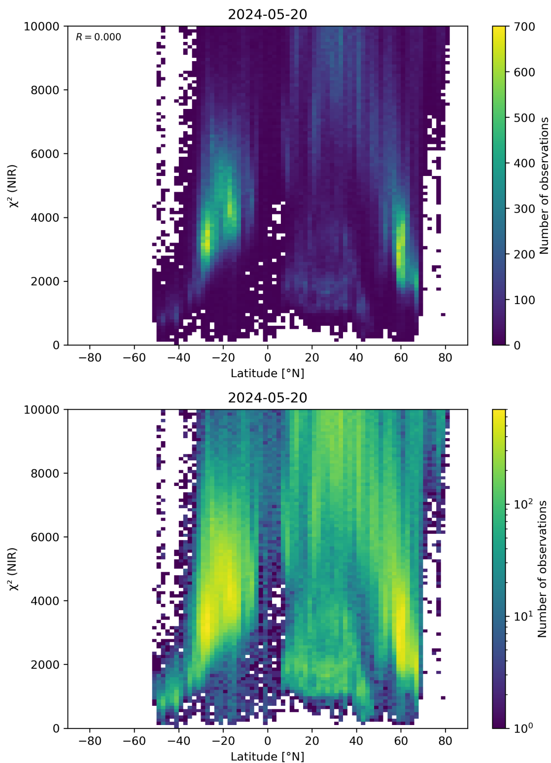
Figure 53: Scatter density plot of “Latitude” against “ \chi^2 (NIR)” for 2024-05-19 to 2024-05-21.
