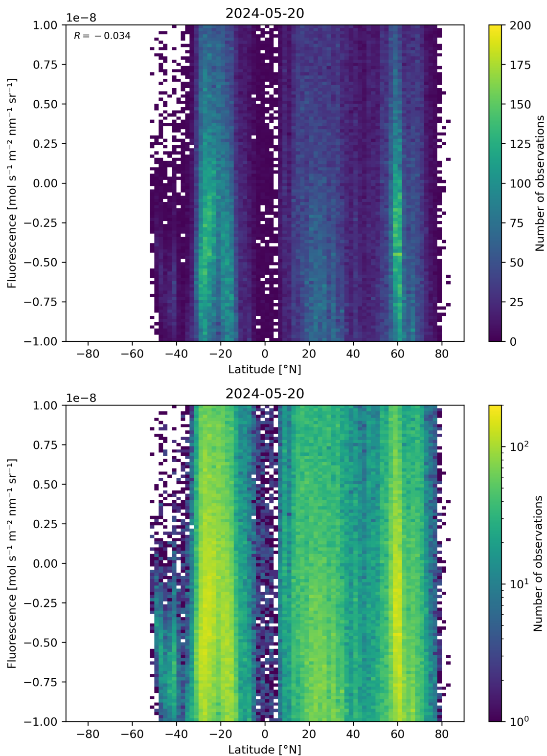
Figure 56: Scatter density plot of “Latitude” against “Fluorescence” for 2024-05-19 to 2024-05-21.
