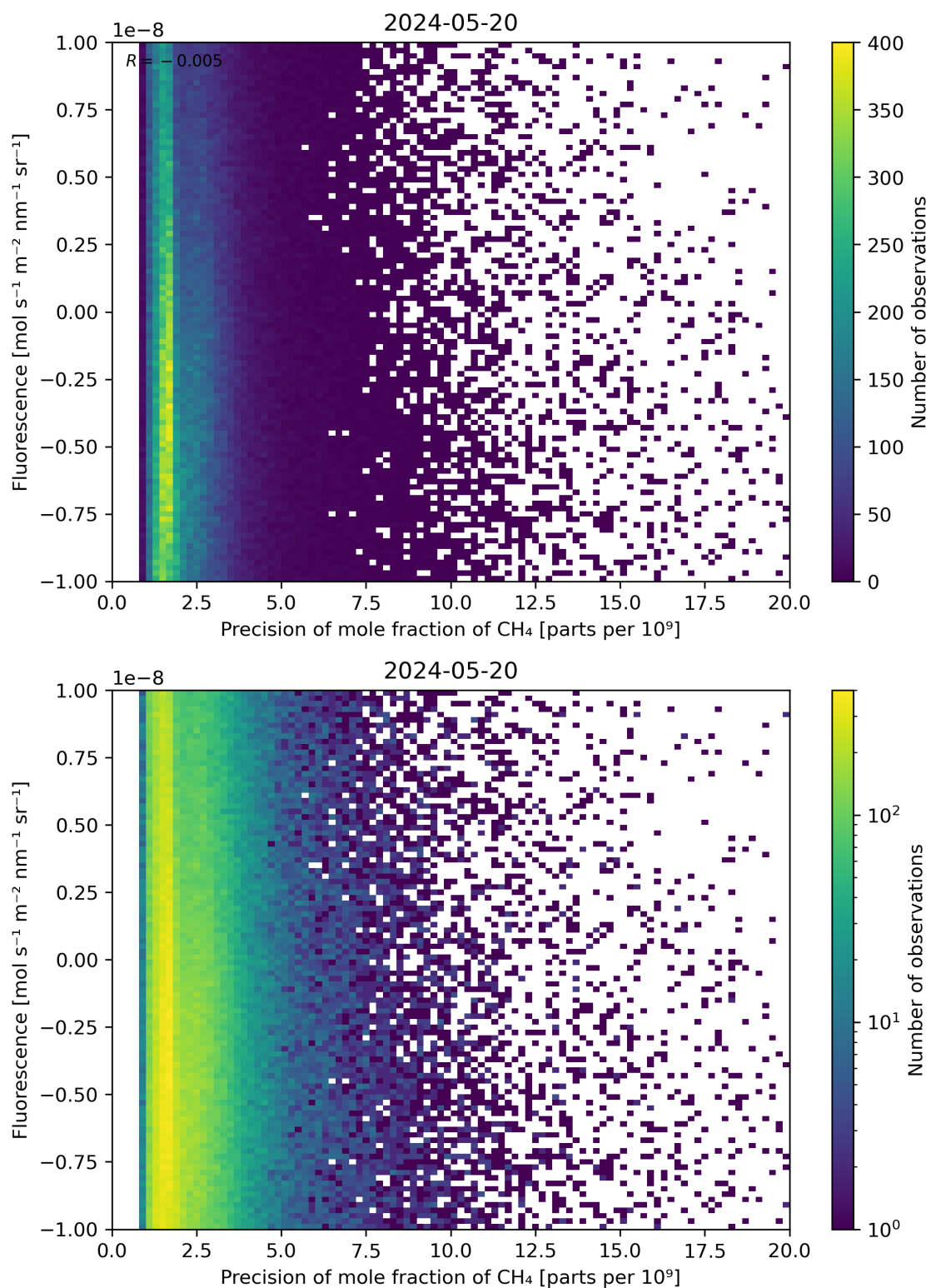
Figure 81: Scatter density plot of “Precision of mole fraction of \text{CH}_4 ” against “Fluorescence” for 2024-05-19 to 2024-05-21.
