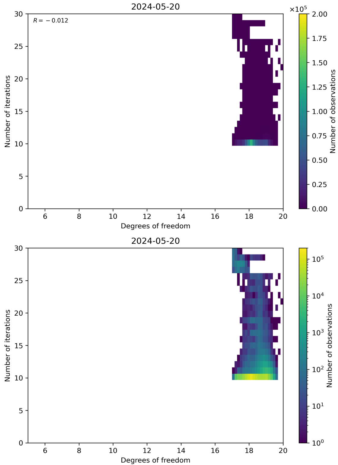
Figure 52: Scatter density plot of “Degrees of freedom” against “Number of iterations” for 2024-05-19 to 2024-05-21.
