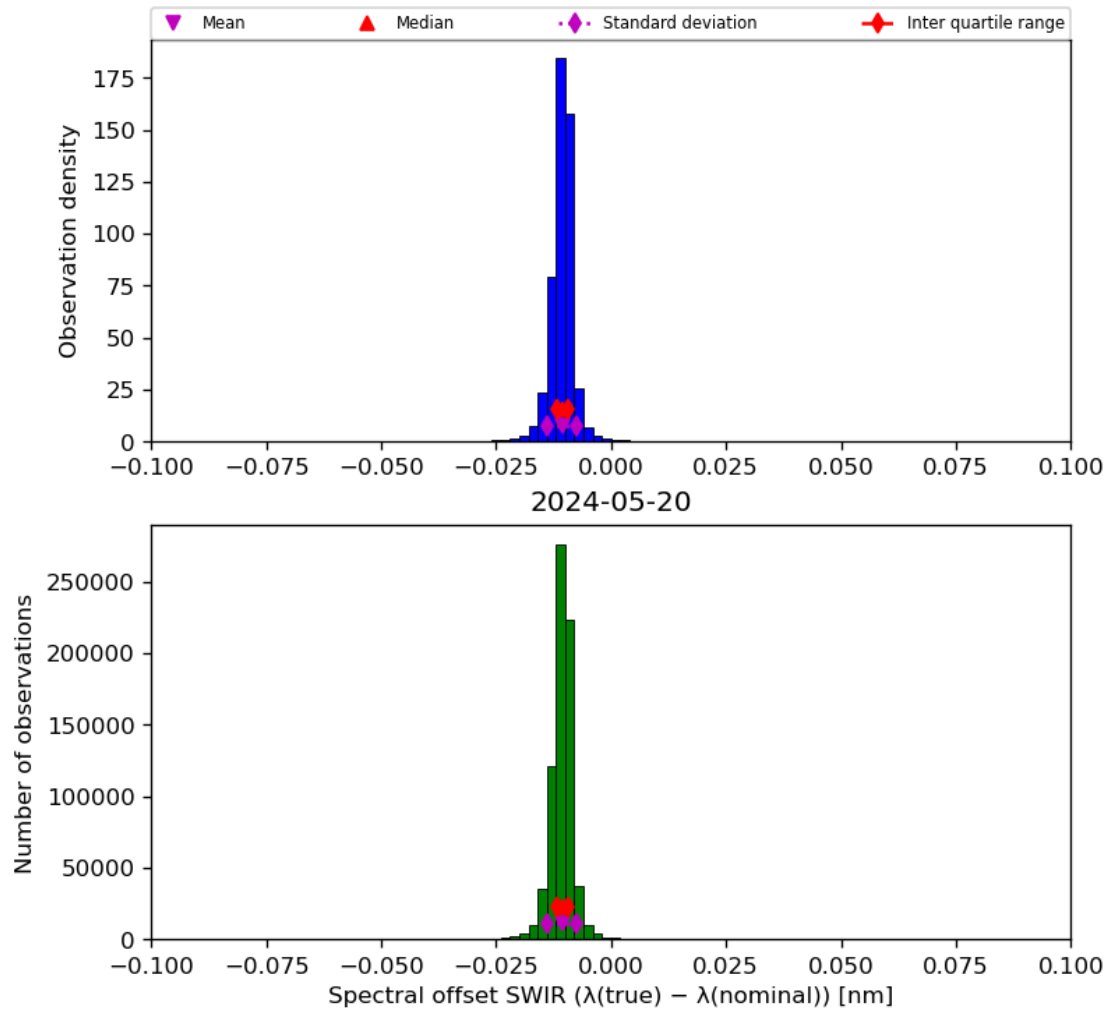
Figure 27: Histogram of “Spectral offset SWIR ( \lambda(\text{true}) - \lambda(\text{nominal}) )” for 2024-05-19 to 2024-05-21
