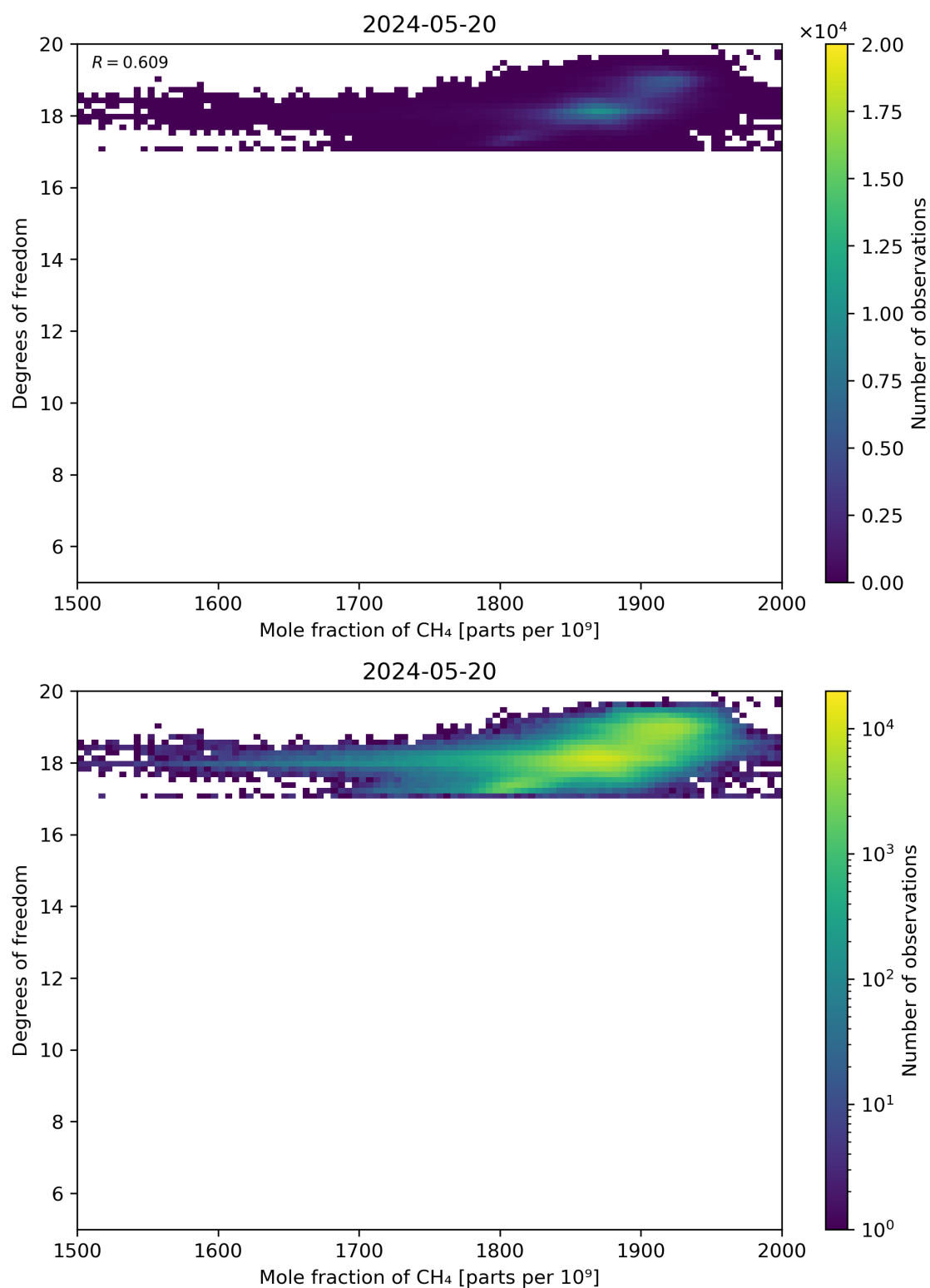
Figure 72: Scatter density plot of “Mole fraction of CH 4 ” against “Degrees of freedom” for 2024-05-19 to 2024-05-21.
