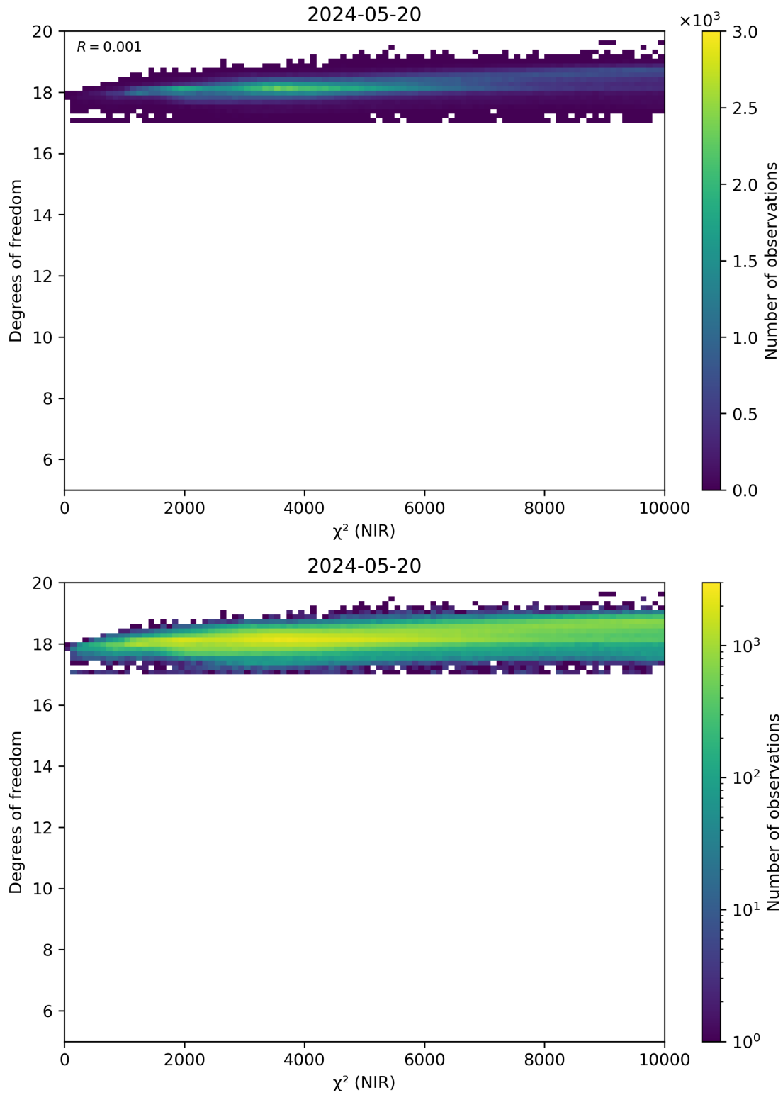
Figure 44: Scatter density plot of “ \chi^2 (NIR)” against “Degrees of freedom” for 2024-05-19 to 2024-05-21.
