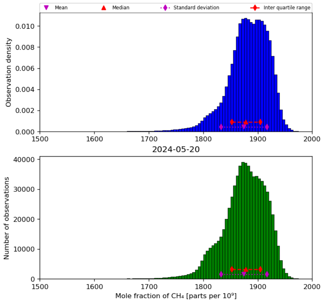
Figure 23: Histogram of “Mole fraction of CH 4 ” for 2024-05-19 to 2024-05-21
