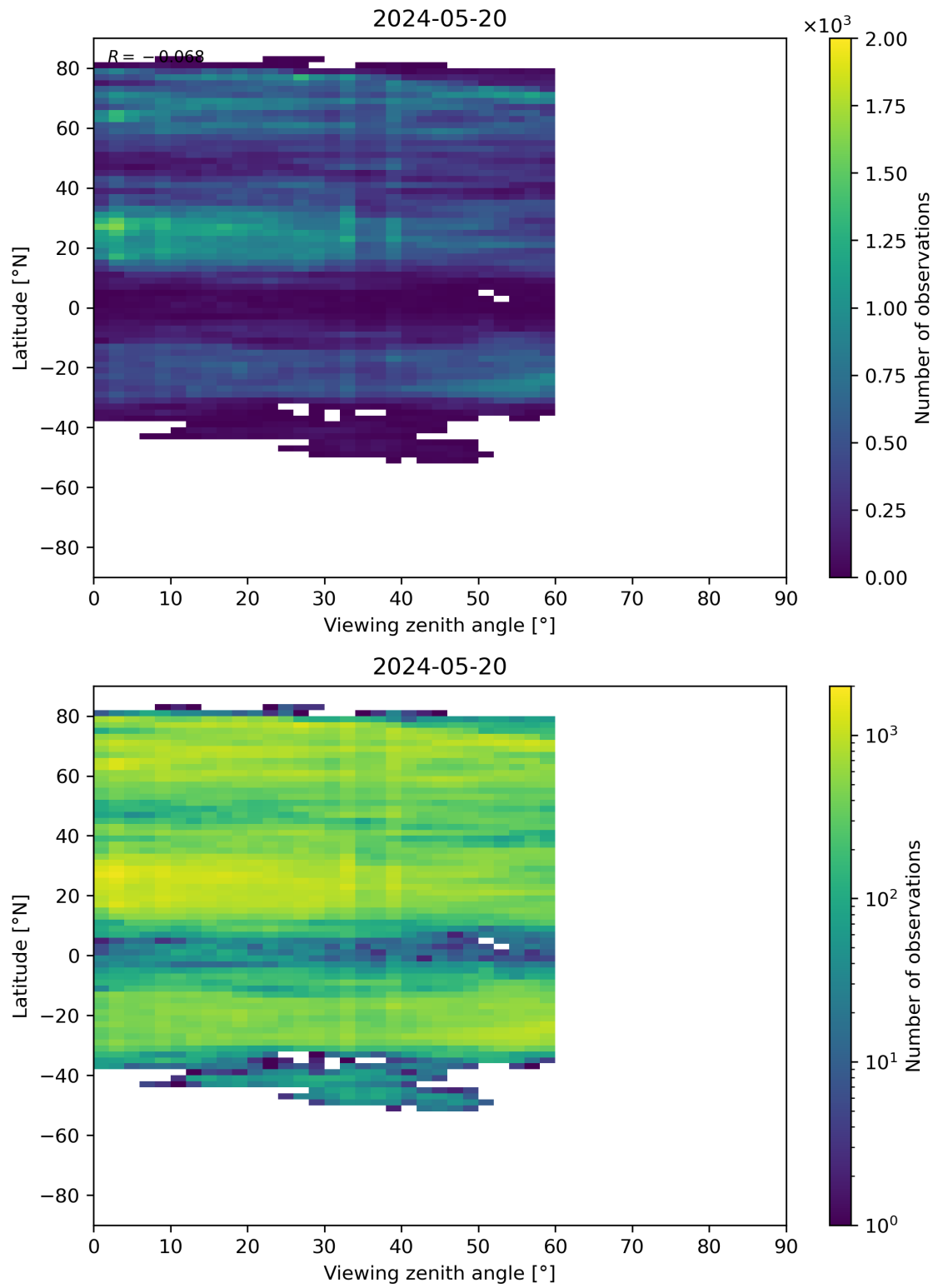
Figure 109: Scatter density plot of “Viewing zenith angle” against “Latitude” for 2024-05-19 to 2024-05-21.
