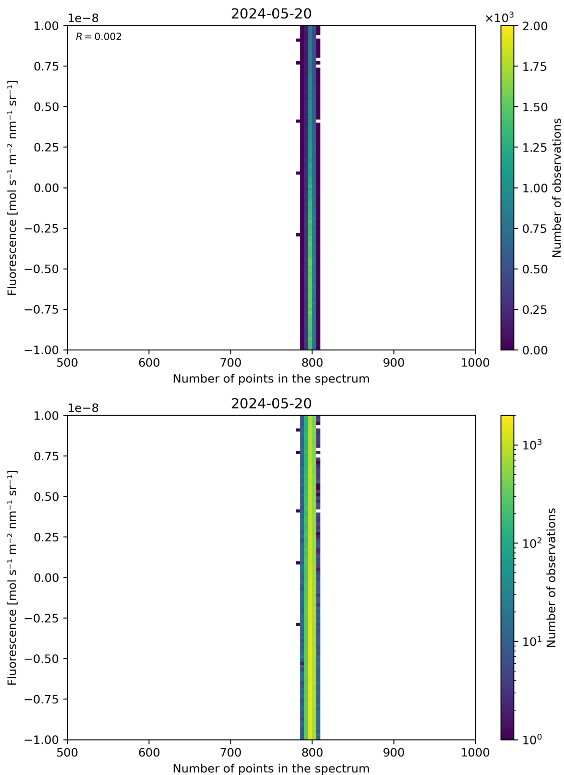
Figure 91: Scatter density plot of “Number of points in the spectrum” against “Fluorescence” for 2024-05-19 to 2024-05-21.
