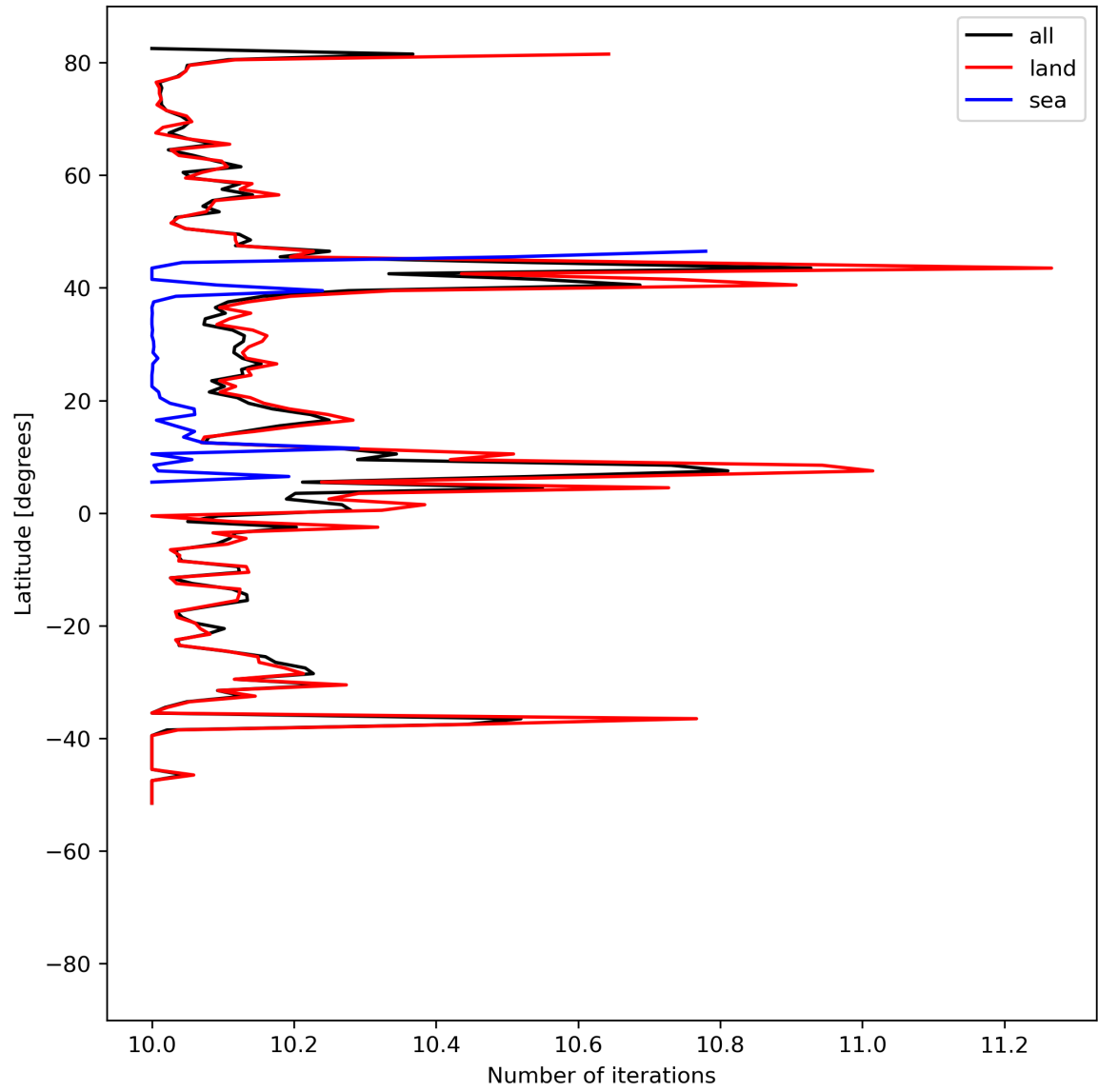
Figure 20: Zonal average of “Number of iterations” for 2024-05-19 to 2024-05-21.
