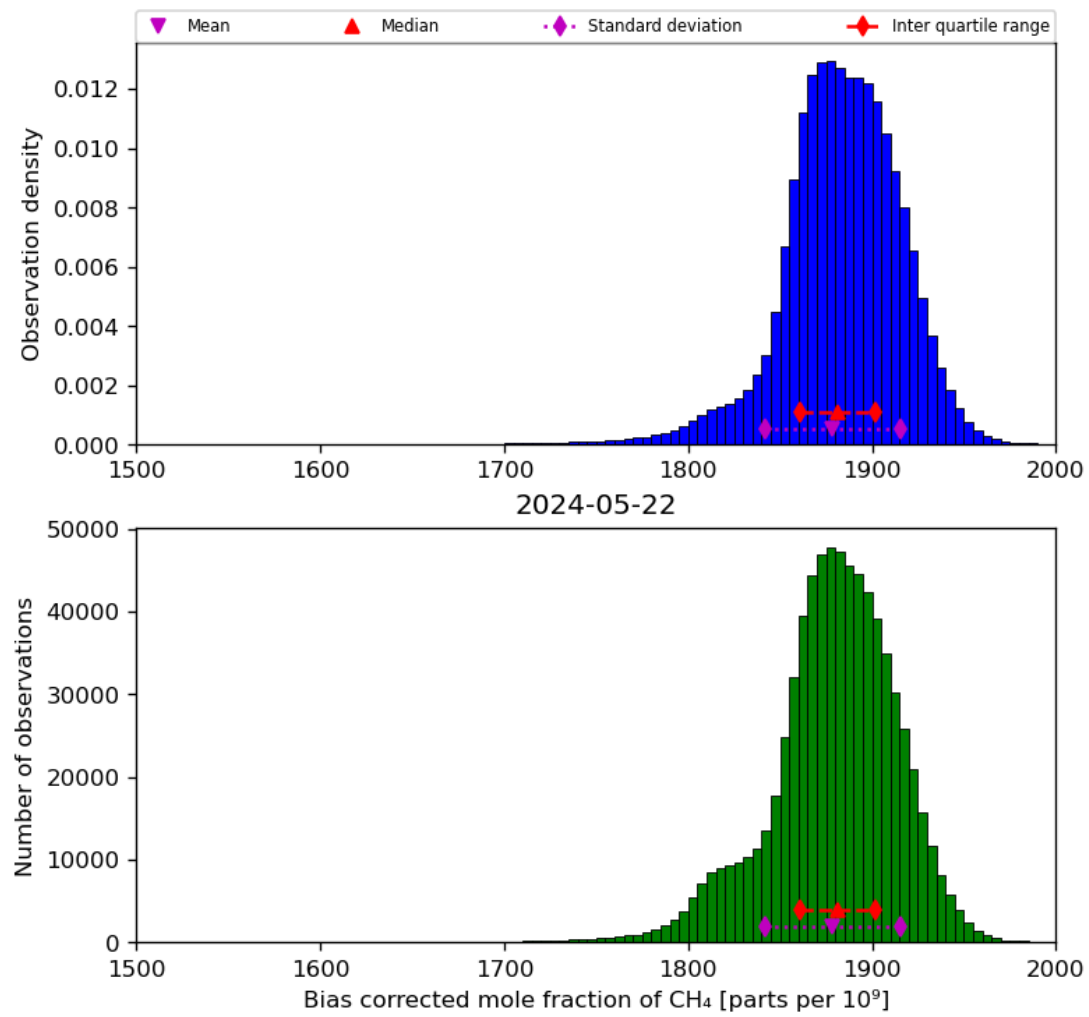
Figure 25: Histogram of “Bias corrected mole fraction of CH 4 ” for 2024-05-21 to 2024-05-23
