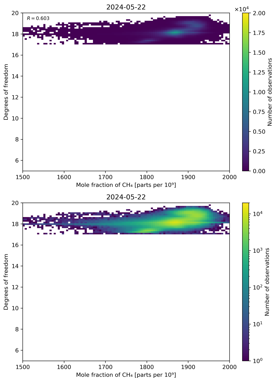
Figure 72: Scatter density plot of “Mole fraction of CH 4 ” against “Degrees of freedom” for 2024-05-21 to 2024-05-23.
