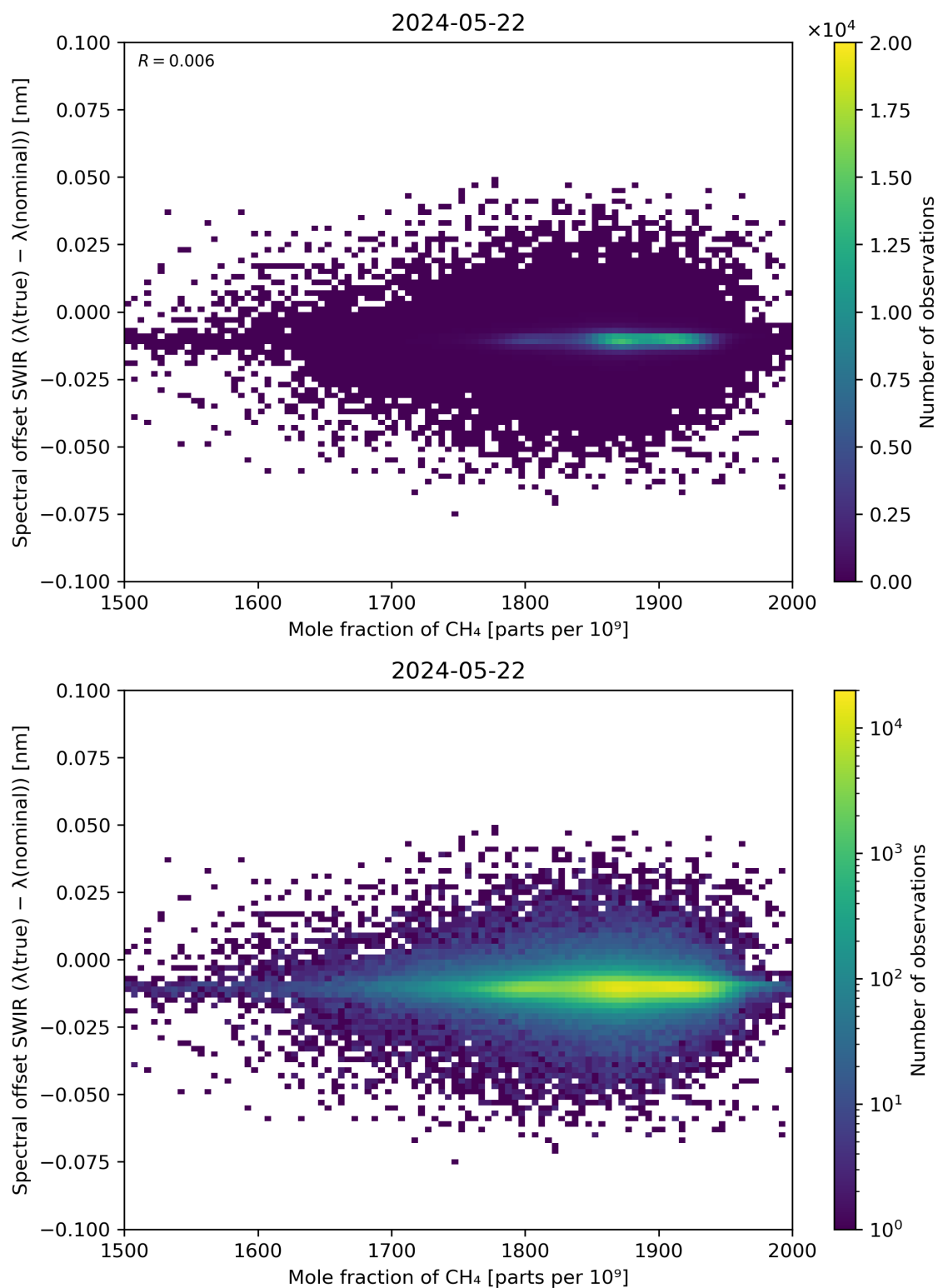
Figure 86: Scatter density plot of “Mole fraction of CH 4 ” against “Spectral offset SWIR ( \lambda(\text{true}) - \lambda(\text{nominal}) )” for 2024-05-21 to 2024-05-23.
