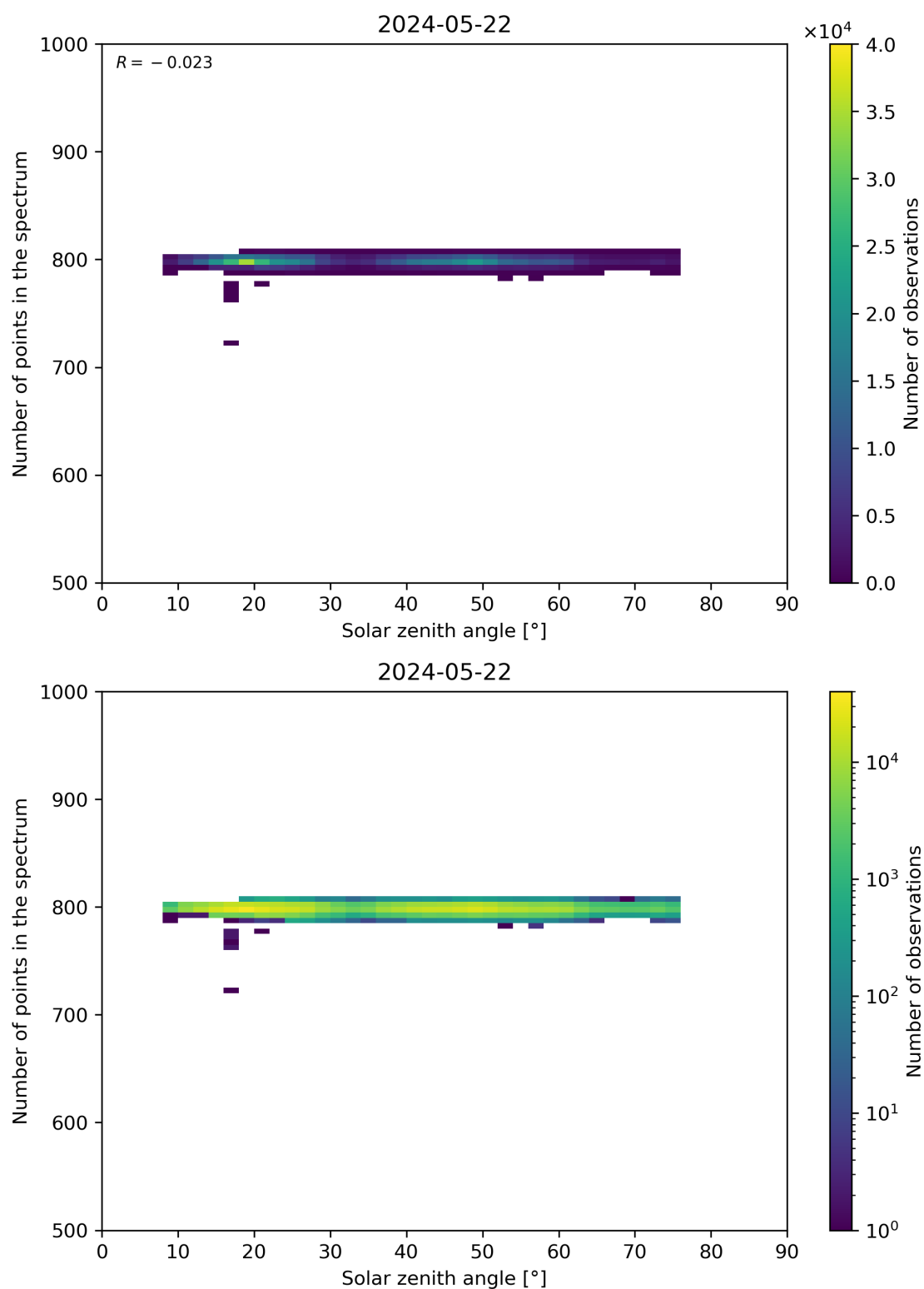
Figure 103: Scatter density plot of “Solar zenith angle” against “Number of points in the spectrum” for 2024-05-21 to 2024-05-23.
