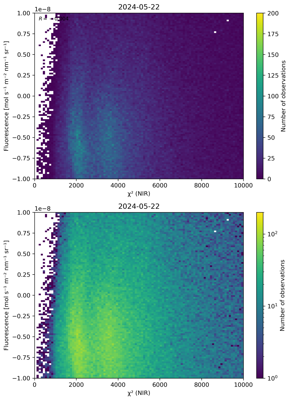
Figure 45: Scatter density plot of “ \chi^2 (NIR)” against “Fluorescence” for 2024-05-21 to 2024-05-23.
