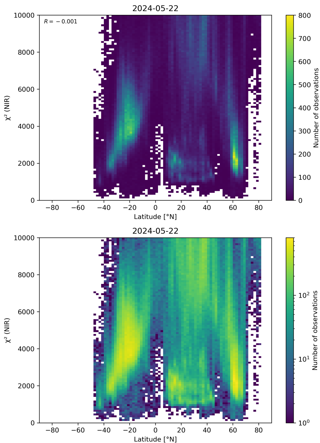
Figure 53: Scatter density plot of “Latitude” against “ \chi^2 (NIR)” for 2024-05-21 to 2024-05-23.
