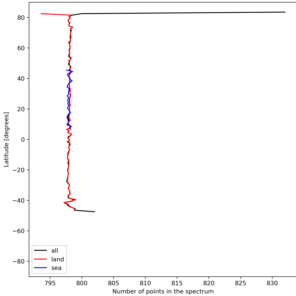
Figure 15: Zonal average of “Number of points in the spectrum” for 2024-05-21 to 2024-05-23.
