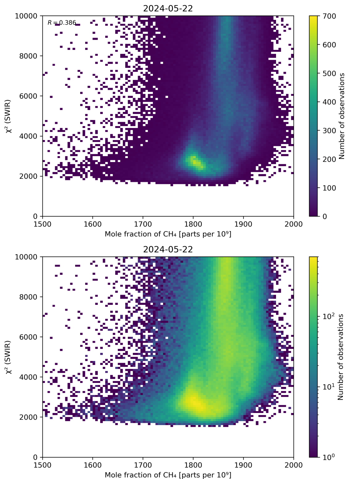
Figure 71: Scatter density plot of “Mole fraction of \text{CH}_4 ” against “ \chi^2 (SWIR)” for 2024-05-21 to 2024-05-23.
