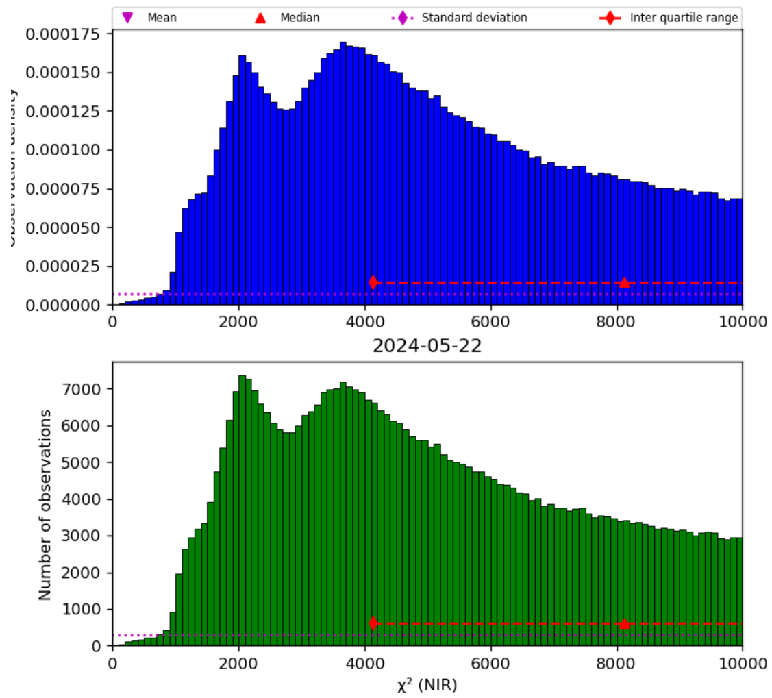
Figure 29: Histogram of “ \chi^2 (NIR)” for 2024-05-21 to 2024-05-23
