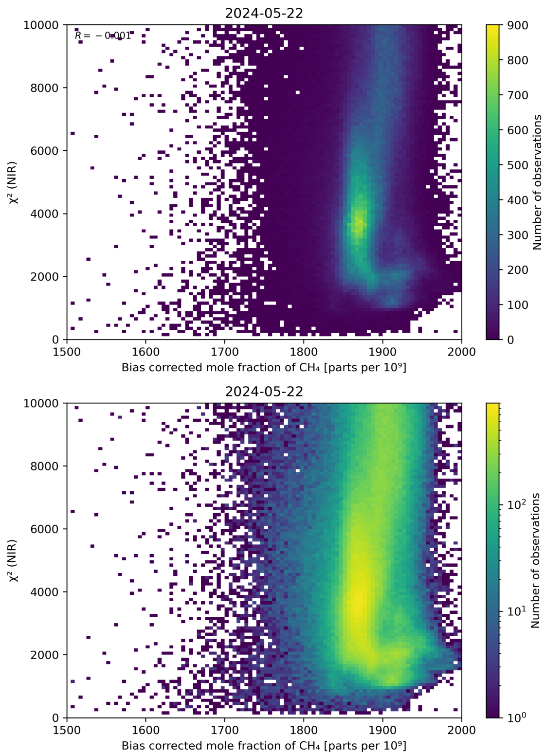
Figure 63: Scatter density plot of “Bias corrected mole fraction of CH 4 ” against “ \chi^2 (NIR)” for 2024-05-21 to 2024-05-23.
