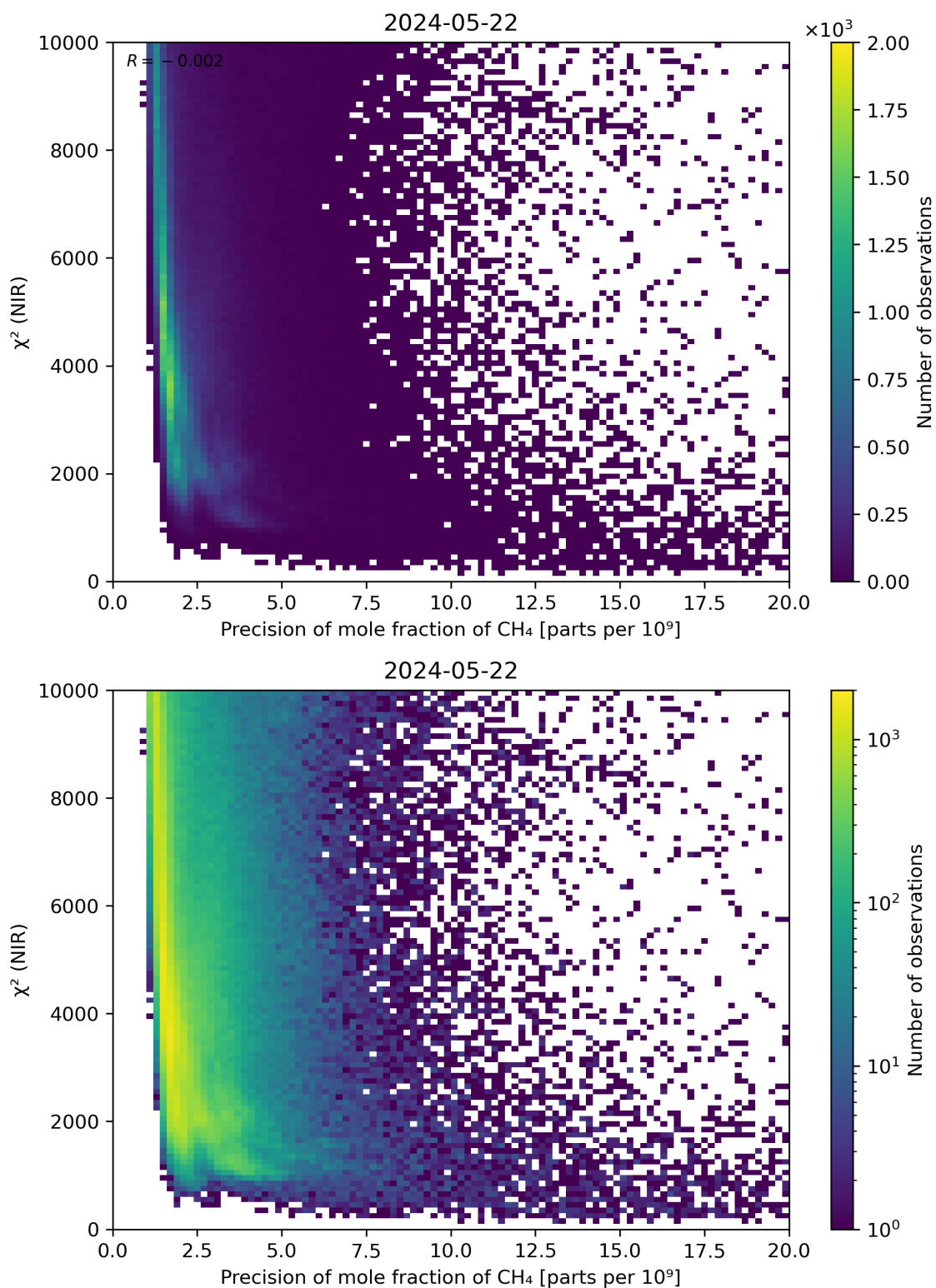
Figure 78: Scatter density plot of “Precision of mole fraction of CH 4 ” against “ \chi^2 (NIR)” for 2024-05-21 to 2024-05-23.
