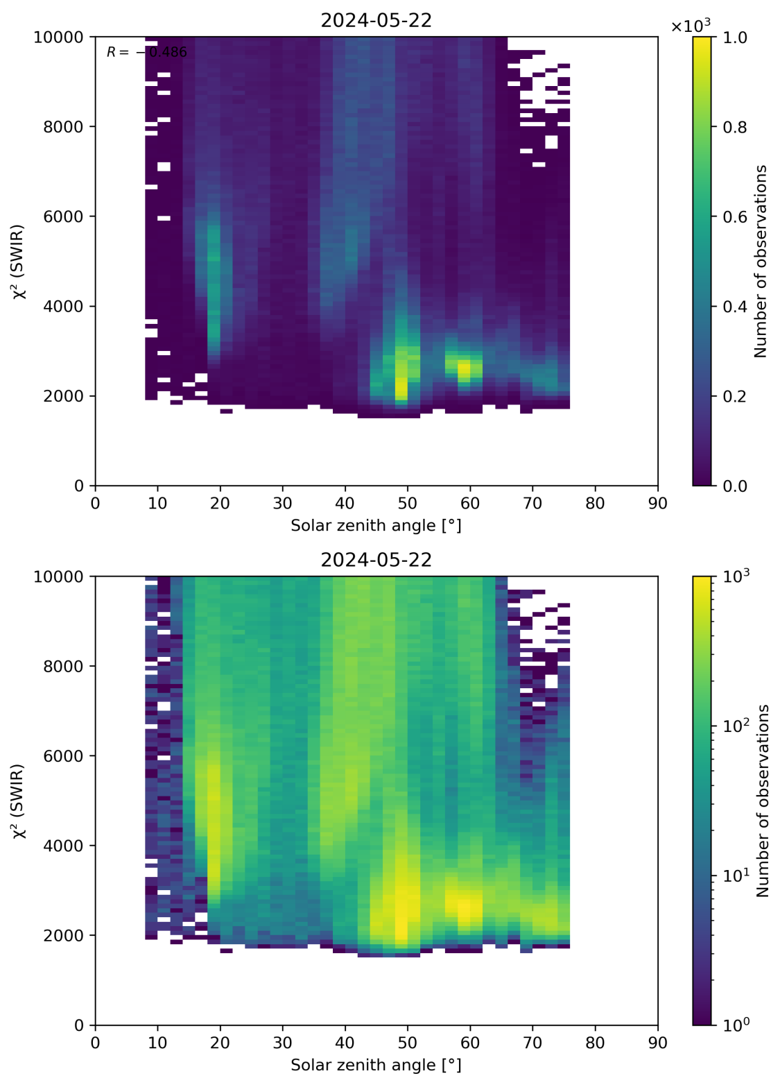
Figure 95: Scatter density plot of “Solar zenith angle” against “ \chi^2 (SWIR)” for 2024-05-21 to 2024-05-23.
