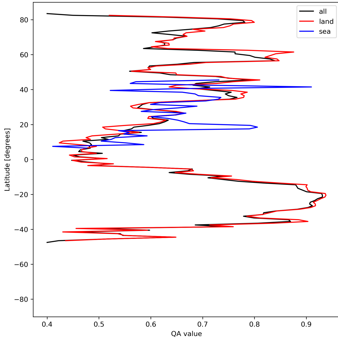
Figure 11: Zonal average of “QA value” for 2024-05-21 to 2024-05-23.
