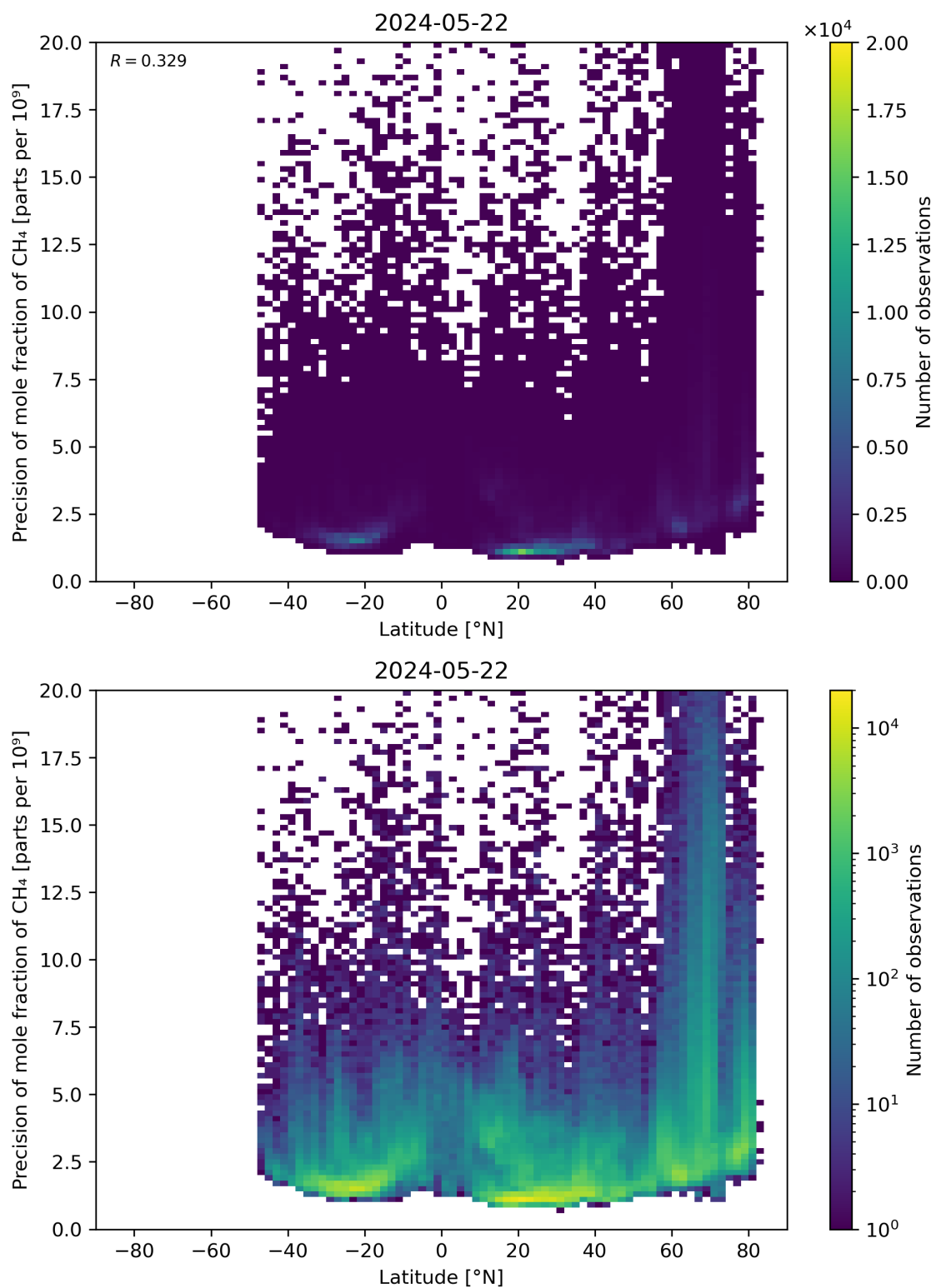
Figure 59: Scatter density plot of “Latitude” against “Precision of mole fraction of \text{CH}_4 ” for 2024-05-21 to 2024-05-23.
