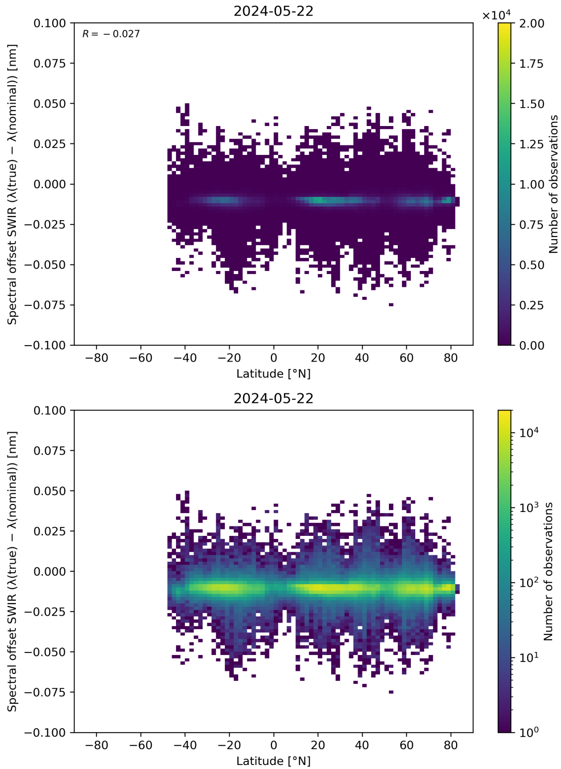
Figure 62: Scatter density plot of “Latitude” against “Spectral offset SWIR ( \lambda(\text{true}) - \lambda(\text{nominal}) )” for 2024-05-21 to 2024-05-23.
