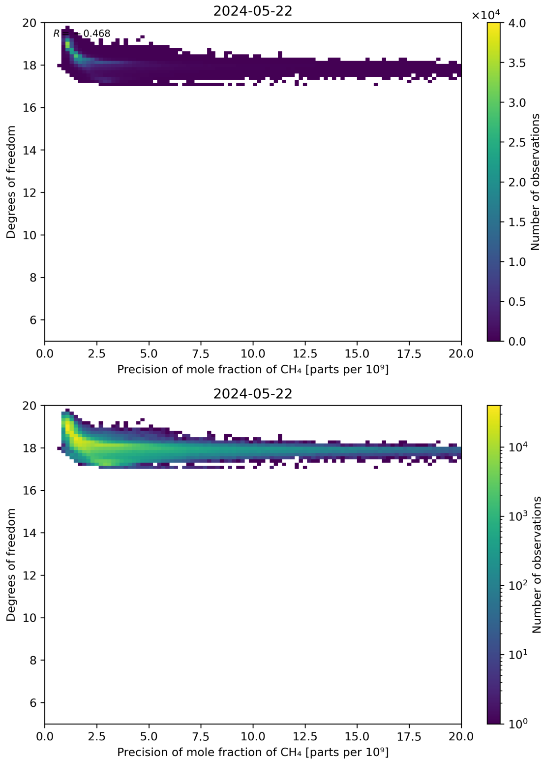
Figure 80: Scatter density plot of “Precision of mole fraction of CH 4 ” against “Degrees of freedom” for 2024-05-21 to 2024-05-23.
