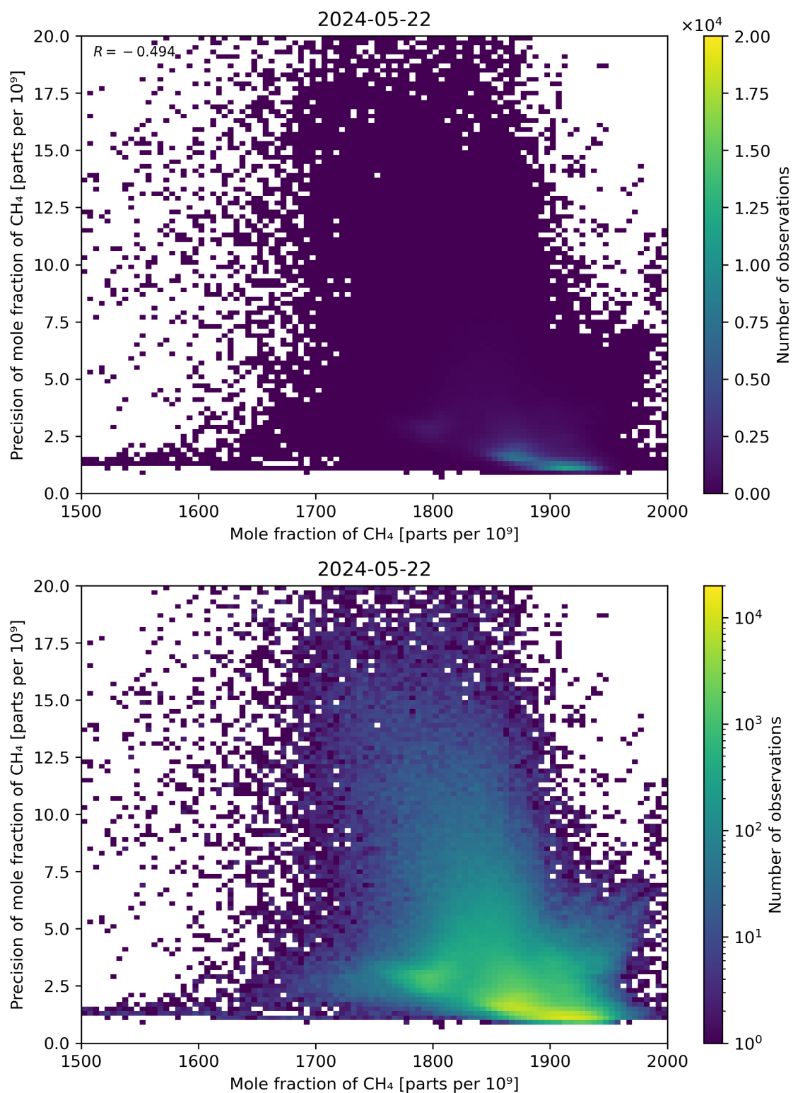
Figure 75: Scatter density plot of “Mole fraction of CH 4 ” against “Precision of mole fraction of CH 4 ” for 2024-05-21 to 2024-05-23.
