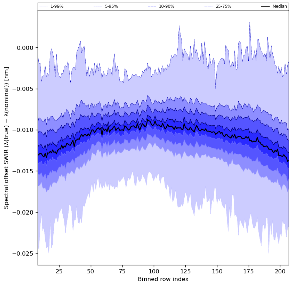
Figure 38: Along track statistics of “Spectral offset SWIR ( \lambda(\text{true}) - \lambda(\text{nominal}) )” for 2024-05-21 to 2024-05-23
