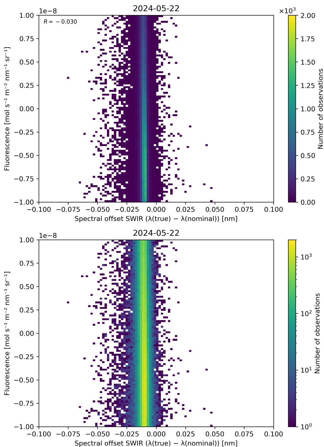
Figure 120: Scatter density plot of “Spectral offset SWIR ( \lambda(\text{true}) - \lambda(\text{nominal}) )” against “Fluorescence” for 2024-05-21 to 2024-05-23.
