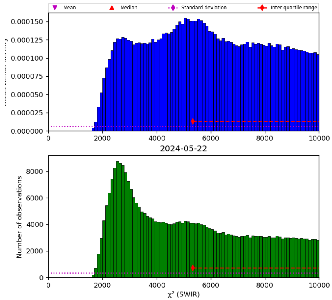
Figure 28: Histogram of “ \chi^2 (SWIR)” for 2024-05-21 to 2024-05-23
