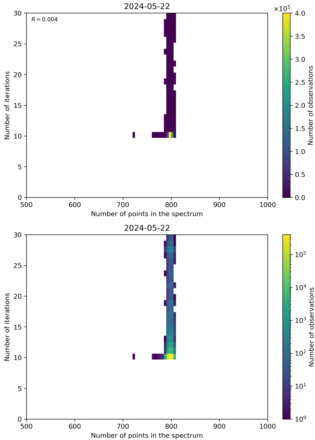
Figure 92: Scatter density plot of “Number of points in the spectrum” against “Number of iterations” for 2024-05-21 to 2024-05-23.
