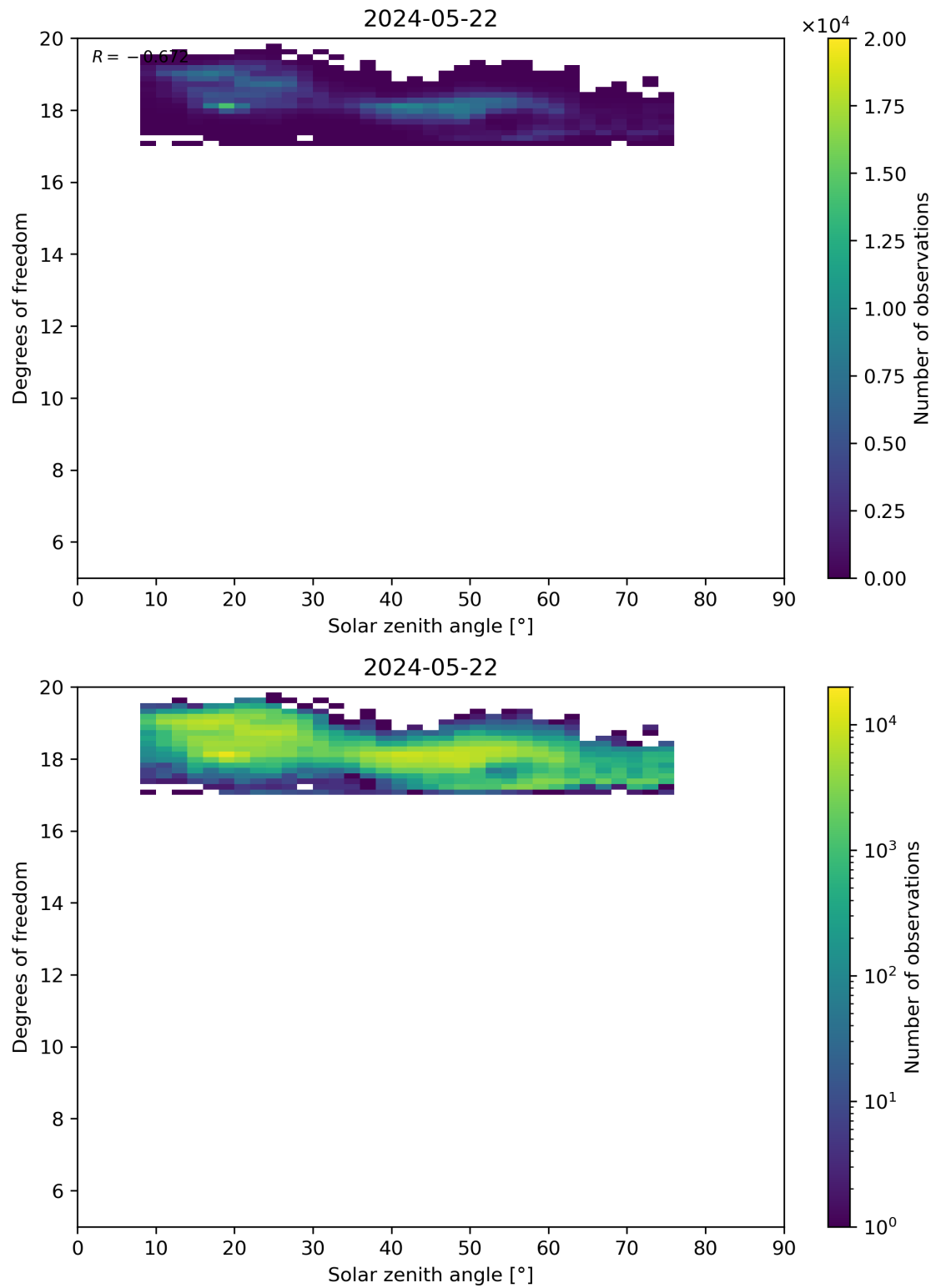
Figure 96: Scatter density plot of “Solar zenith angle” against “Degrees of freedom” for 2024-05-21 to 2024-05-23.
