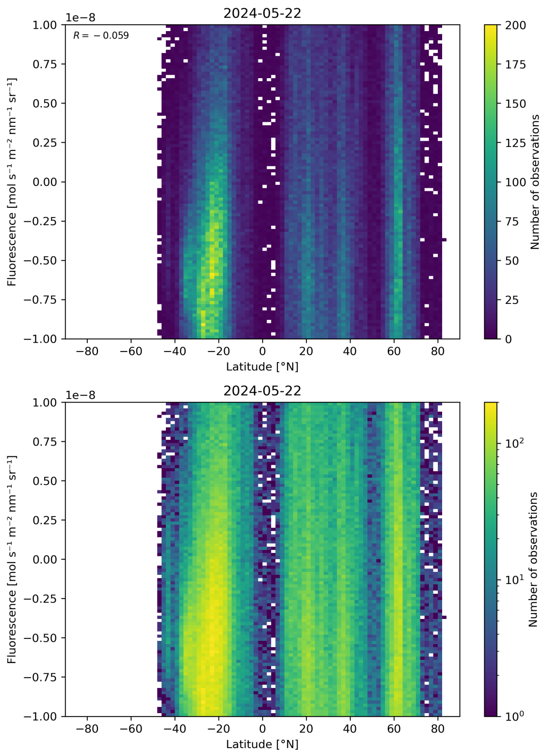
Figure 56: Scatter density plot of “Latitude” against “Fluorescence” for 2024-05-21 to 2024-05-23.
