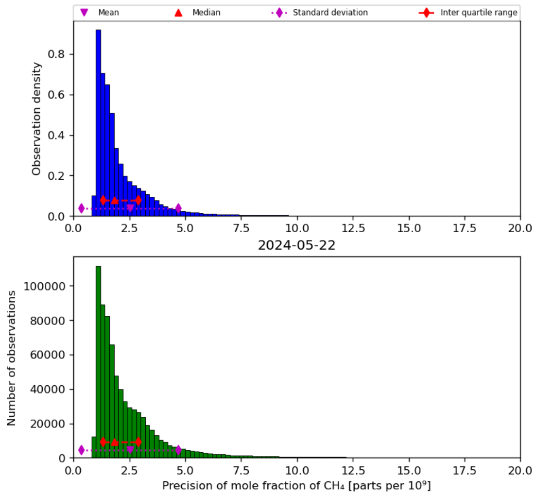
Figure 24: Histogram of “Precision of mole fraction of CH 4 ” for 2024-05-21 to 2024-05-23
