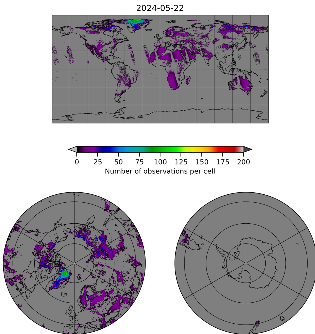
Figure 10: Map of the number of observations for 2024-05-21 to 2024-05-23
