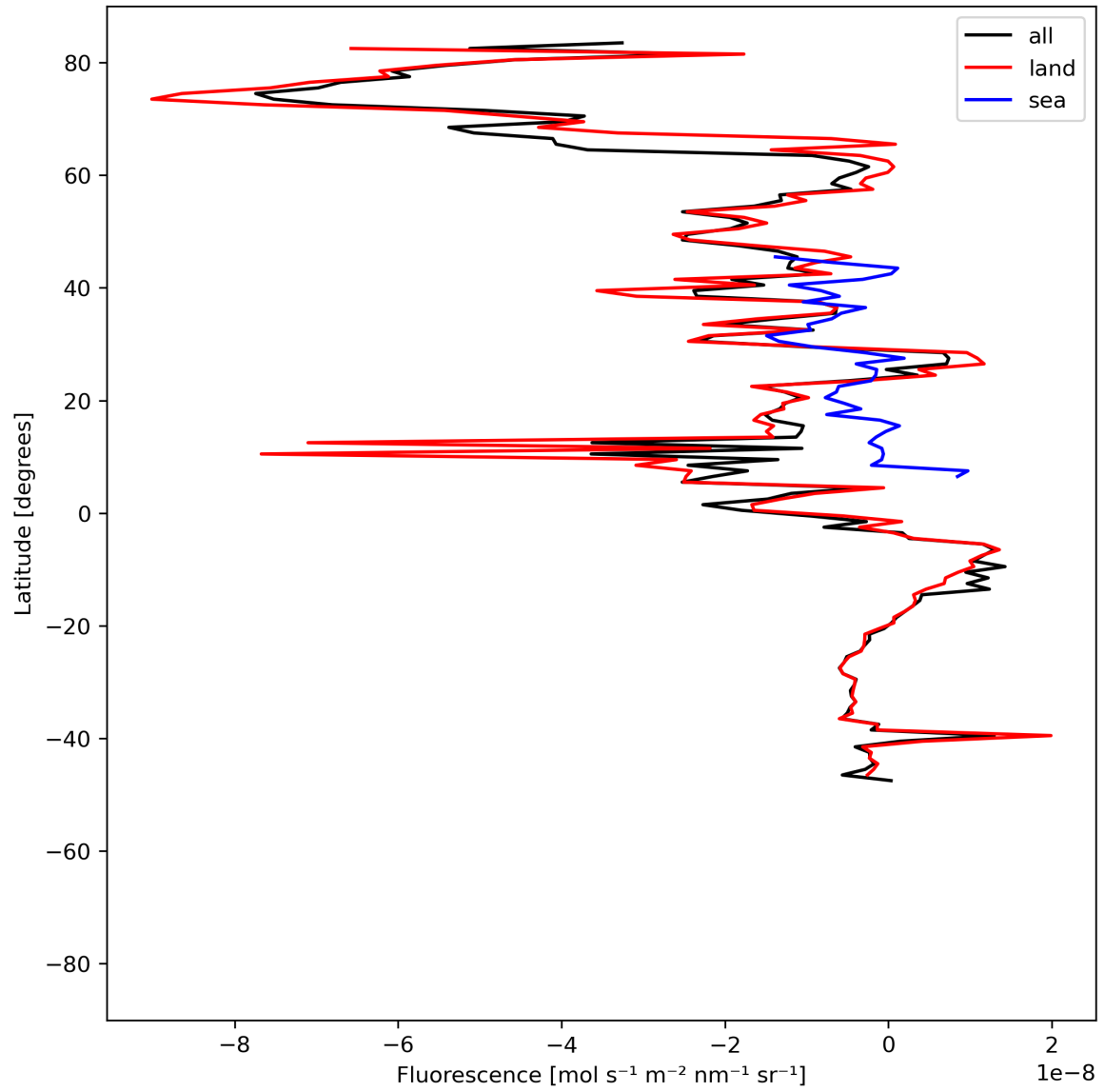
Figure 21: Zonal average of “Fluorescence” for 2024-05-21 to 2024-05-23.
