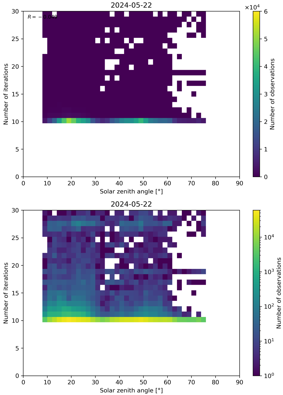
Figure 102: Scatter density plot of “Solar zenith angle” against “Number of iterations” for 2024-05-21 to 2024-05-23.
