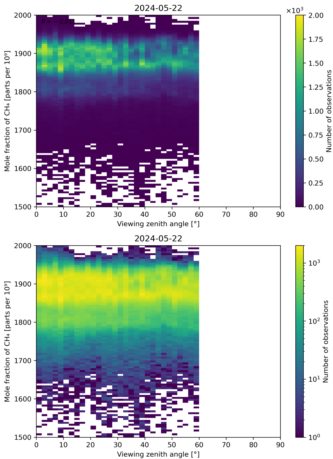
Figure 110: Scatter density plot of “Viewing zenith angle” against “Mole fraction of CH 4 ” for 2024-05-21 to 2024-05-23.
