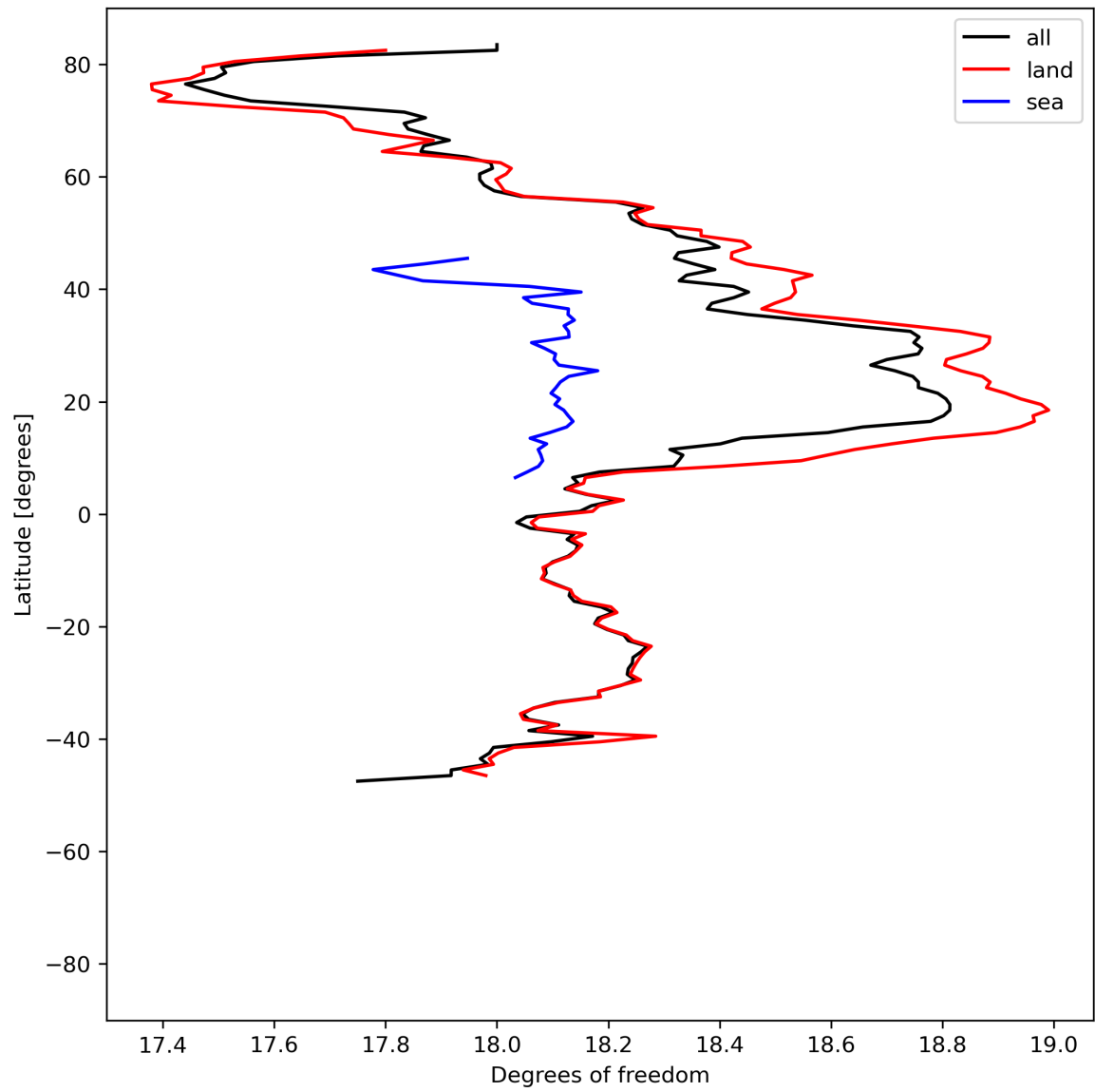
Figure 19: Zonal average of “Degrees of freedom” for 2024-05-21 to 2024-05-23.
