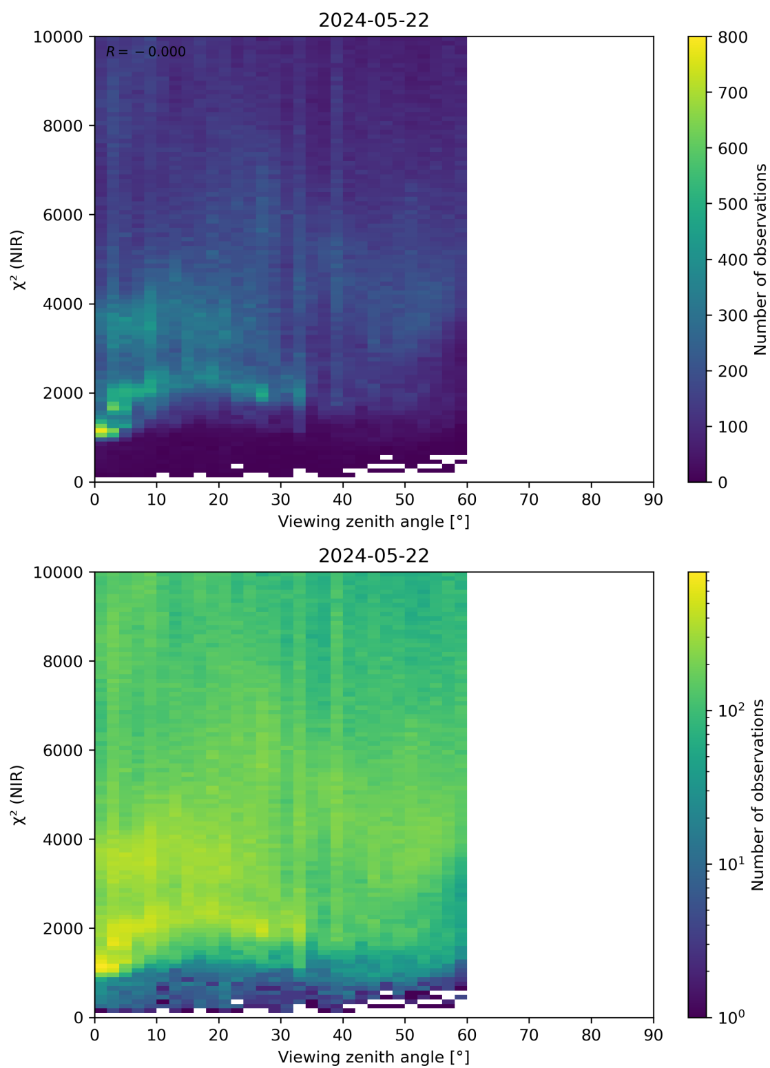
Figure 105: Scatter density plot of “Viewing zenith angle” against “ \chi^2 (NIR)” for 2024-05-21 to 2024-05-23.
