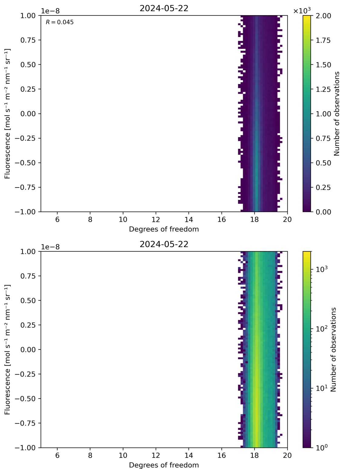
Figure 51: Scatter density plot of “Degrees of freedom” against “Fluorescence” for 2024-05-21 to 2024-05-23.
