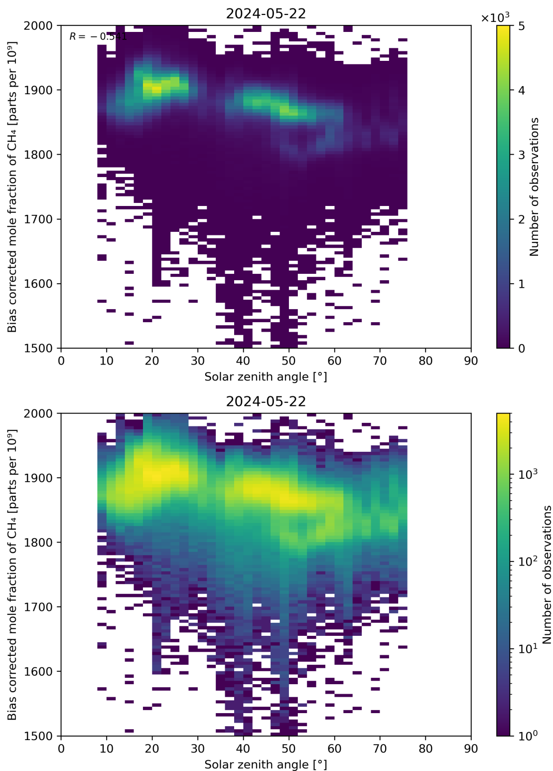
Figure 100: Scatter density plot of “Solar zenith angle” against “Bias corrected mole fraction of CH 4 ” for 2024-05-21 to 2024-05-23.
