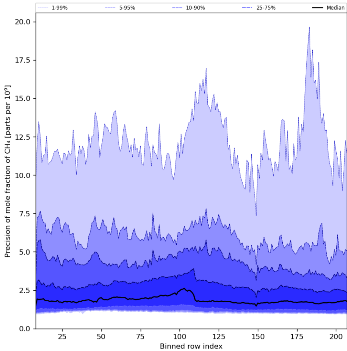
Figure 35: Along track statistics of “Precision of mole fraction of CH 4 ” for 2024-05-21 to 2024-05-23
