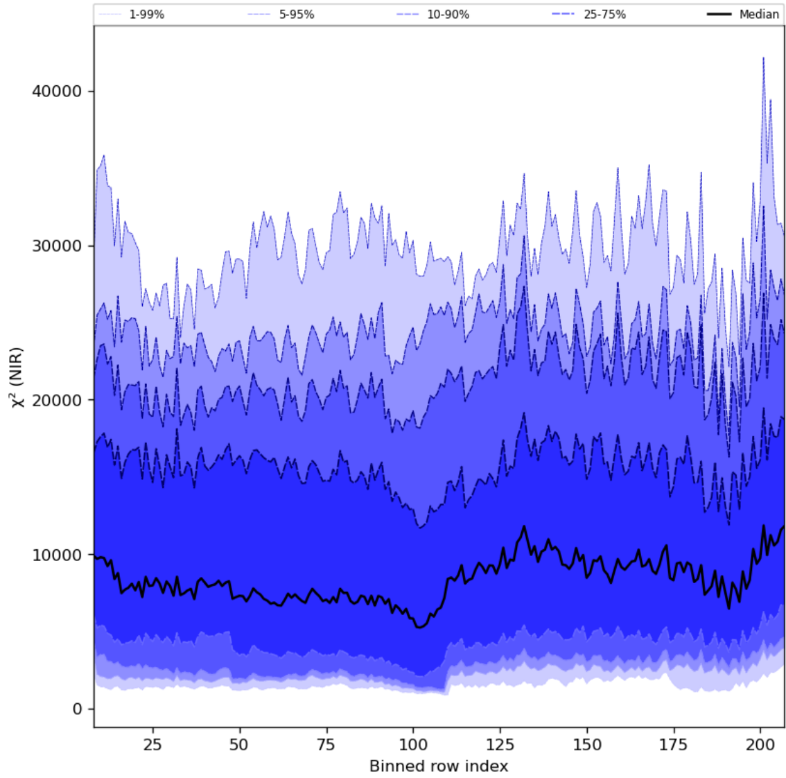
Figure 40: Along track statistics of “ \chi^2 (NIR)” for 2024-05-21 to 2024-05-23
