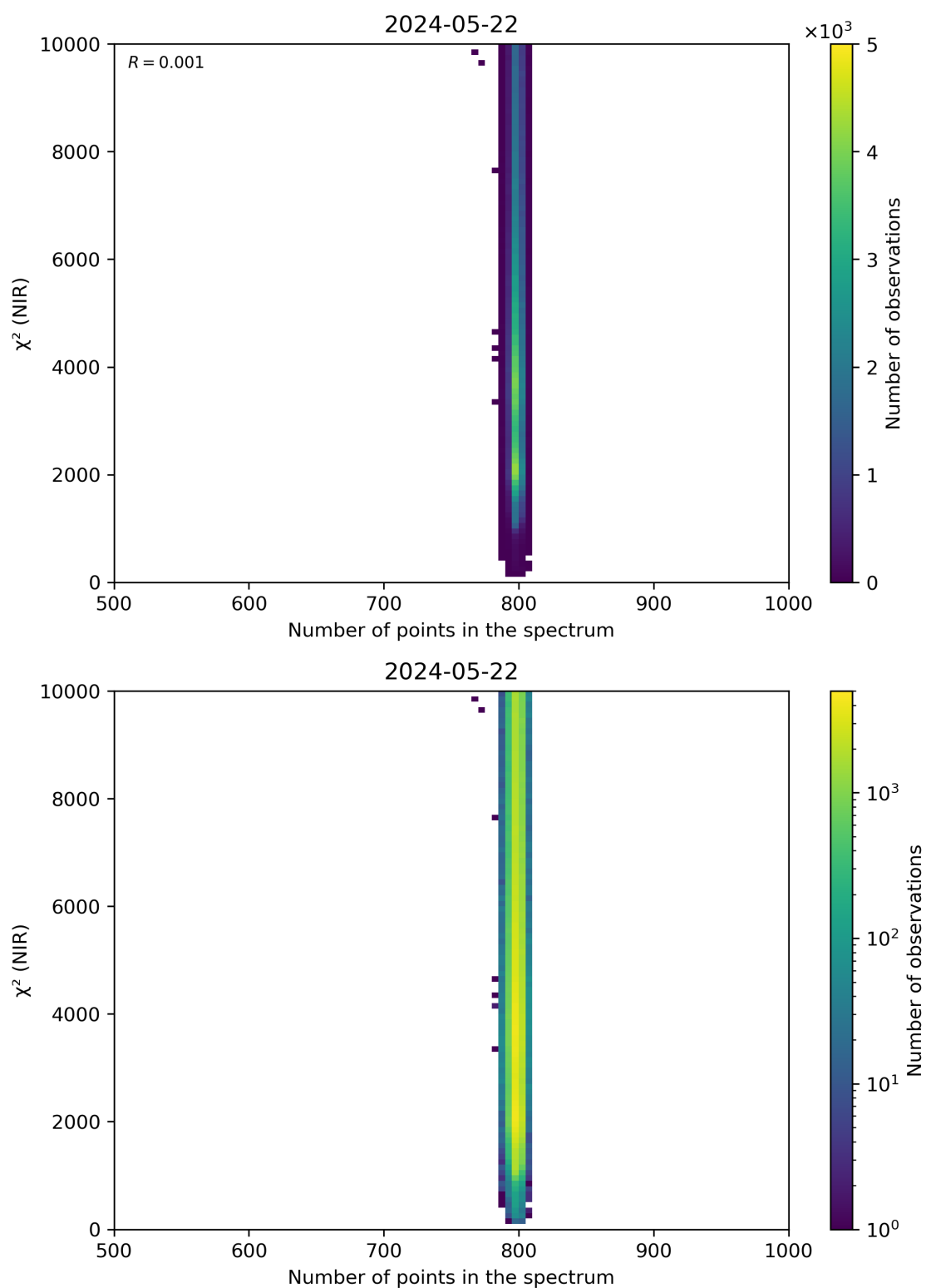
Figure 88: Scatter density plot of “Number of points in the spectrum” against “ \chi^2 (NIR)” for 2024-05-21 to 2024-05-23.
