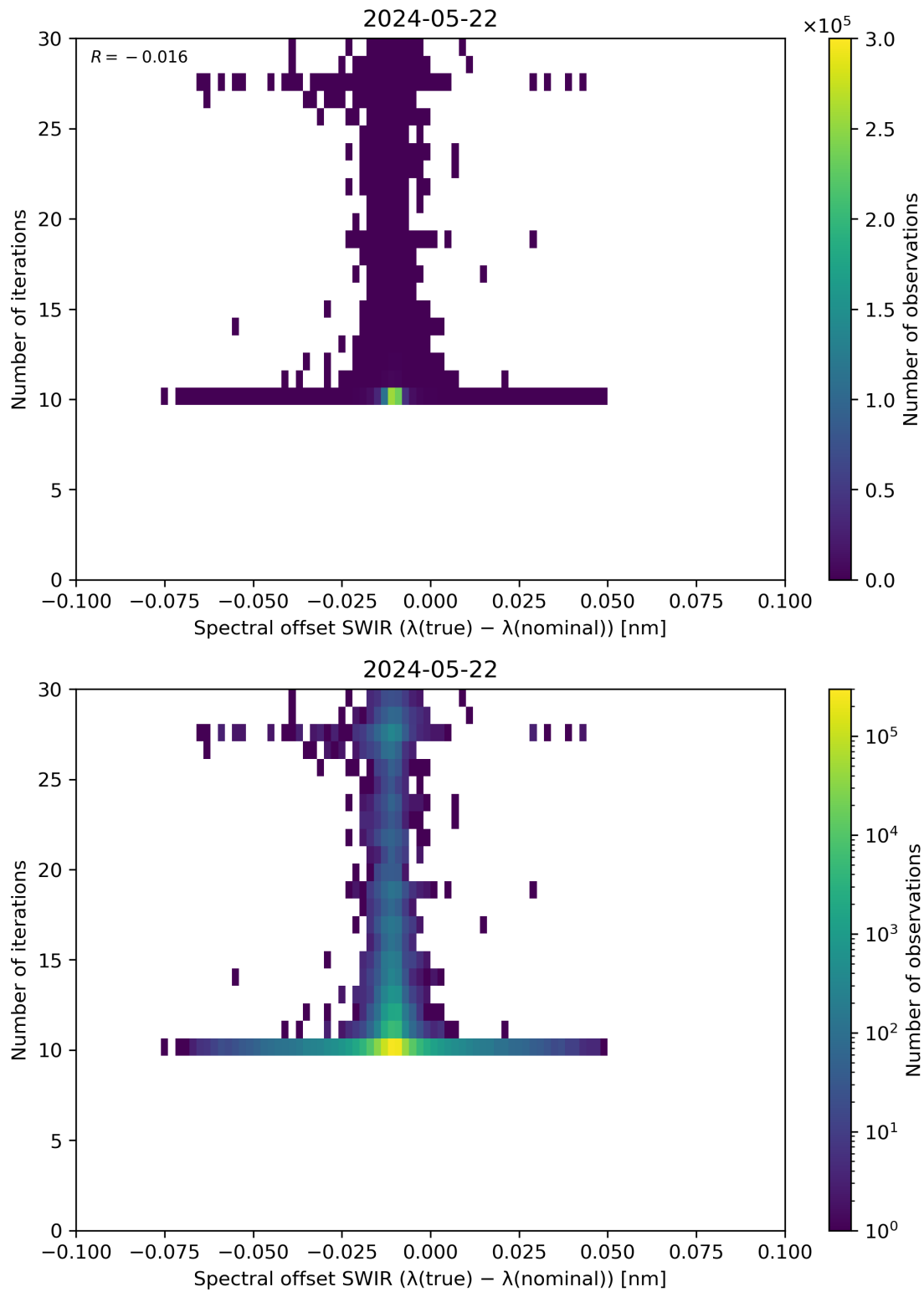
Figure 121: Scatter density plot of “Spectral offset SWIR ( \lambda(\text{true}) - \lambda(\text{nominal}) )” against “Number of iterations” for 2024-05-21 to 2024-05-23.
