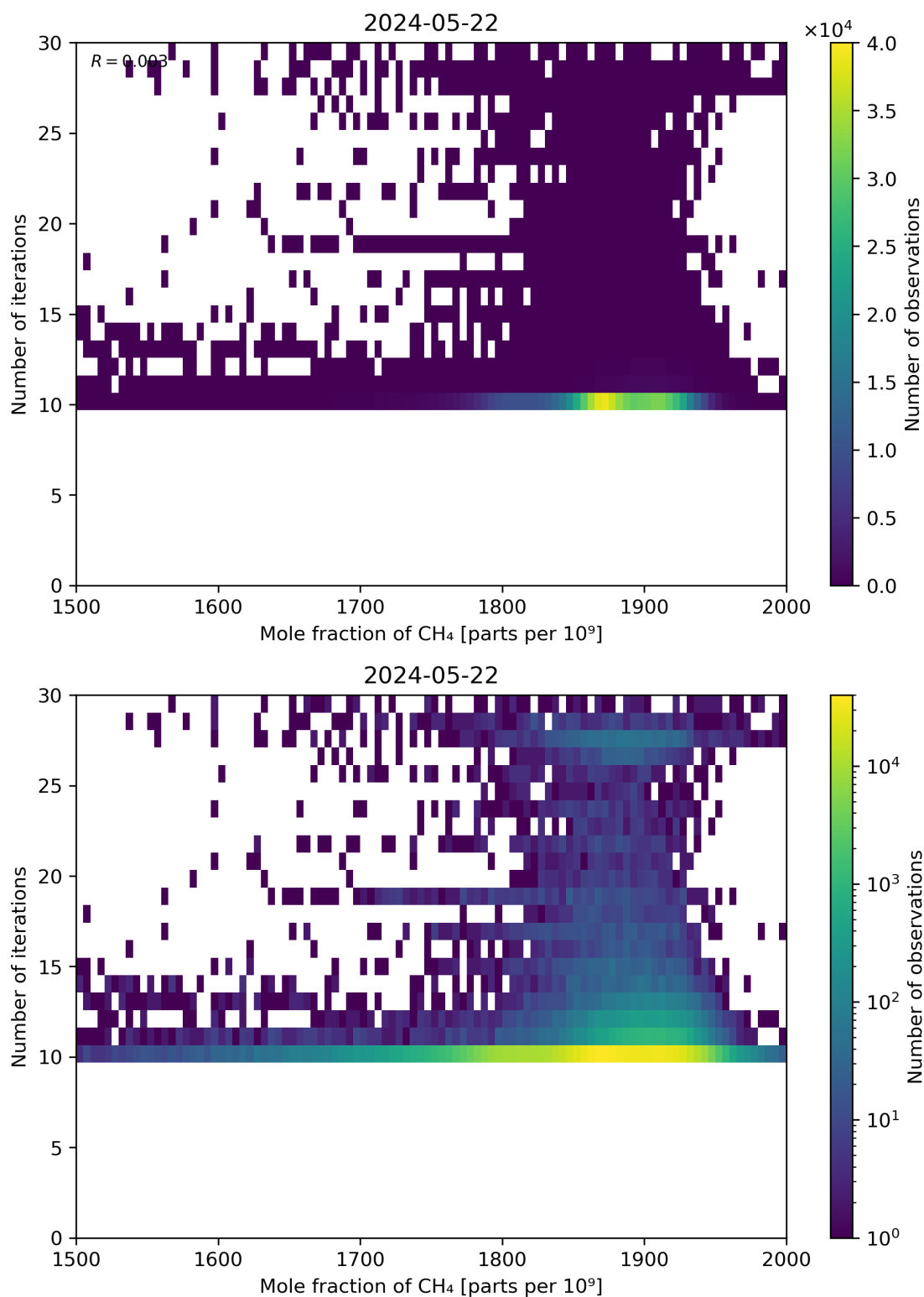
Figure 76: Scatter density plot of “Mole fraction of CH 4 ” against “Number of iterations” for 2024-05-21 to 2024-05-23.
