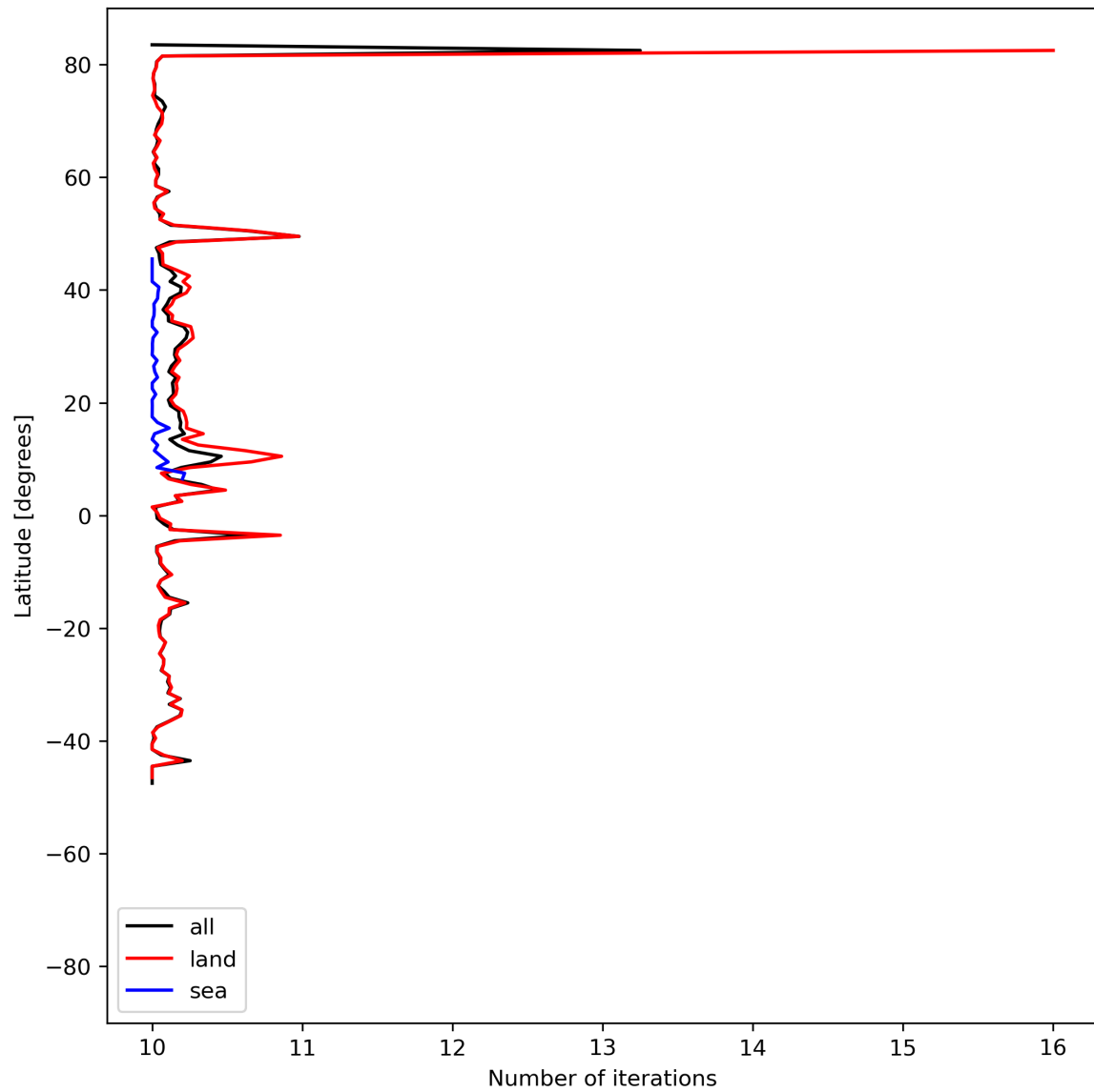
Figure 20: Zonal average of “Number of iterations” for 2024-05-21 to 2024-05-23.
