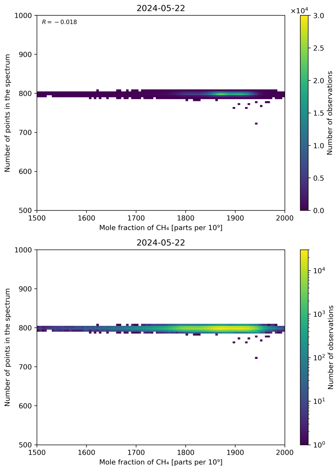
Figure 77: Scatter density plot of “Mole fraction of CH 4 ” against “Number of points in the spectrum” for 2024-05-21 to 2024-05-23.
