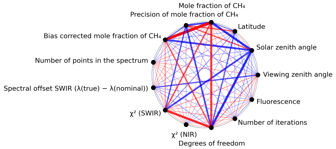
Figure 1: Map of correlation graph for 2024-05-21 to 2024-05-23.
