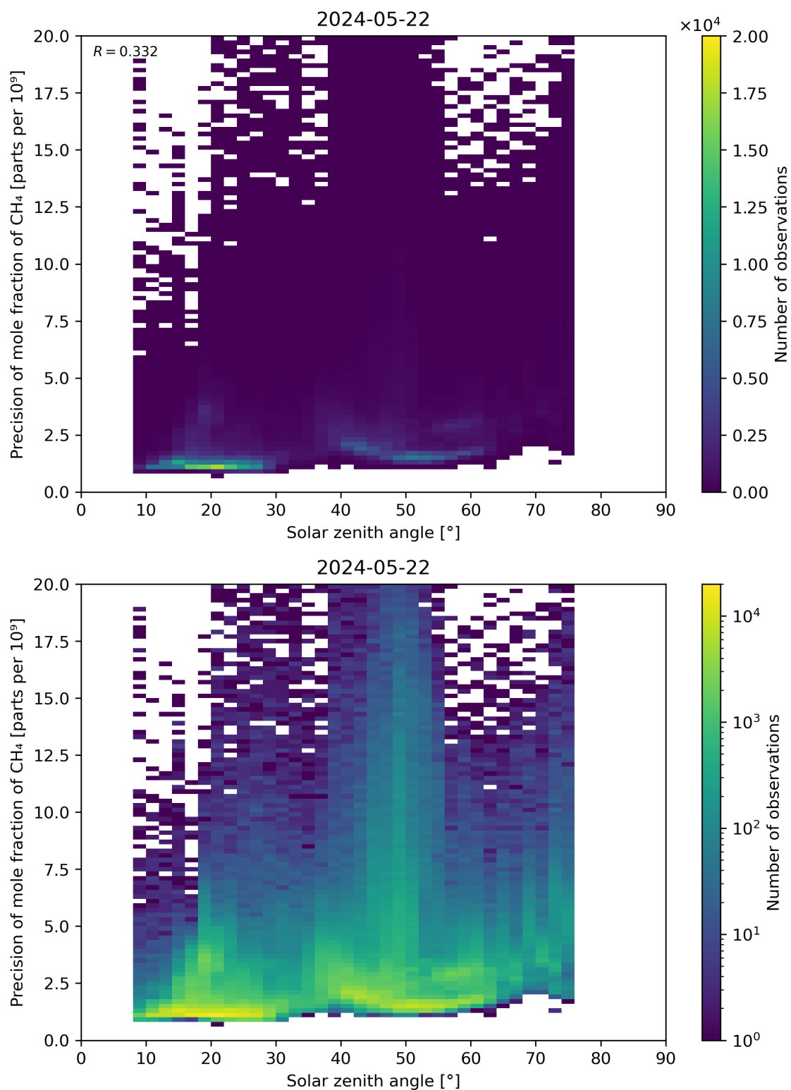
Figure 101: Scatter density plot of “Solar zenith angle” against “Precision of mole fraction of CH 4 ” for 2024-05-21 to 2024-05-23.
