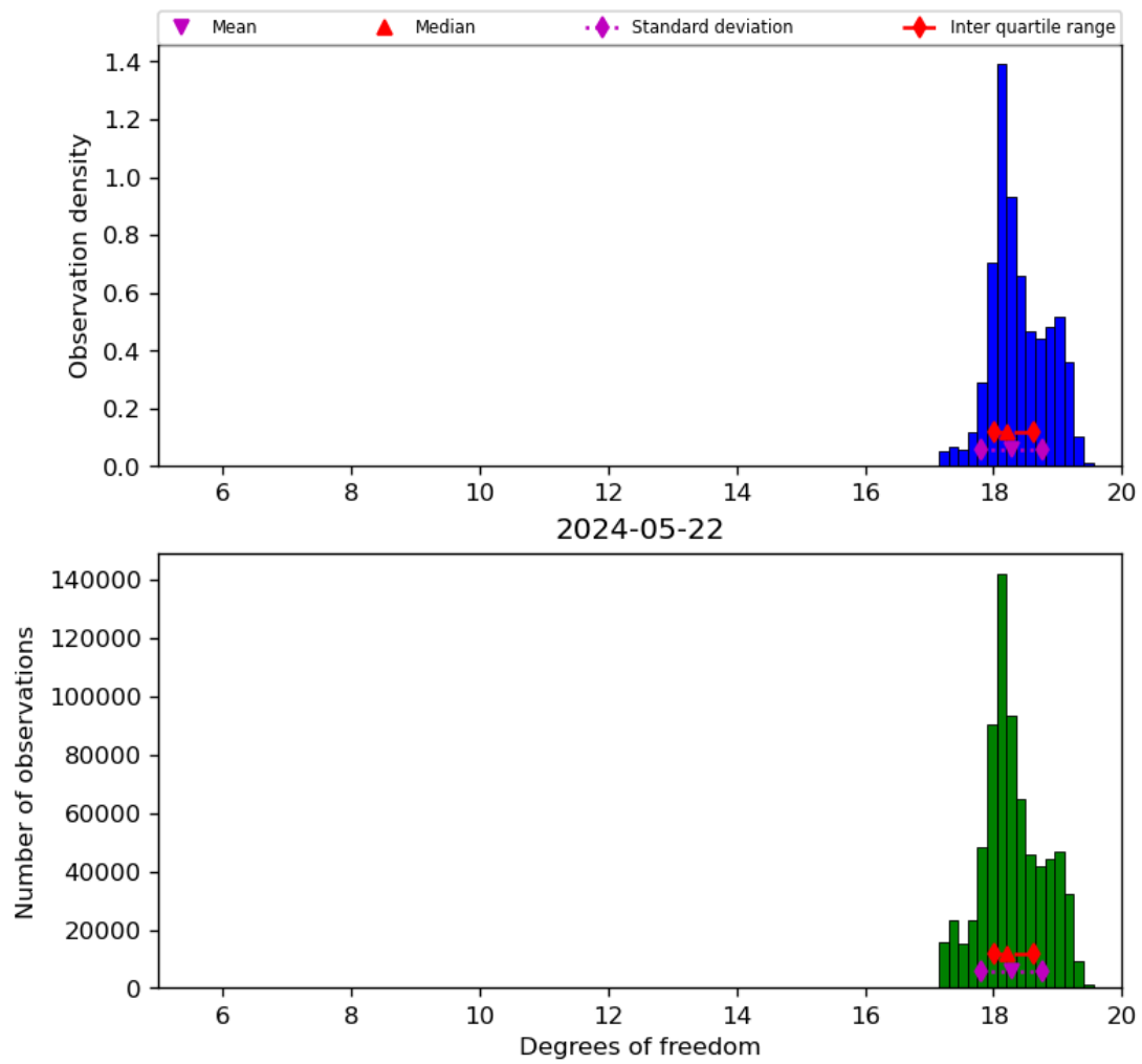
Figure 30: Histogram of “Degrees of freedom” for 2024-05-21 to 2024-05-23
