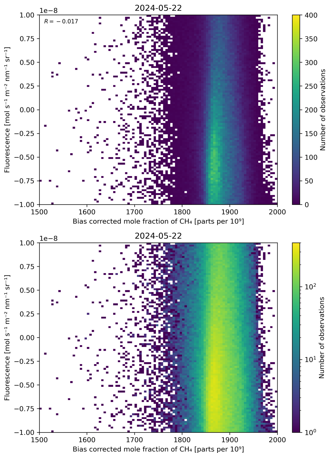
Figure 66: Scatter density plot of “Bias corrected mole fraction of \text{CH}_4 ” against “Fluorescence” for 2024-05-21 to 2024-05-23.
