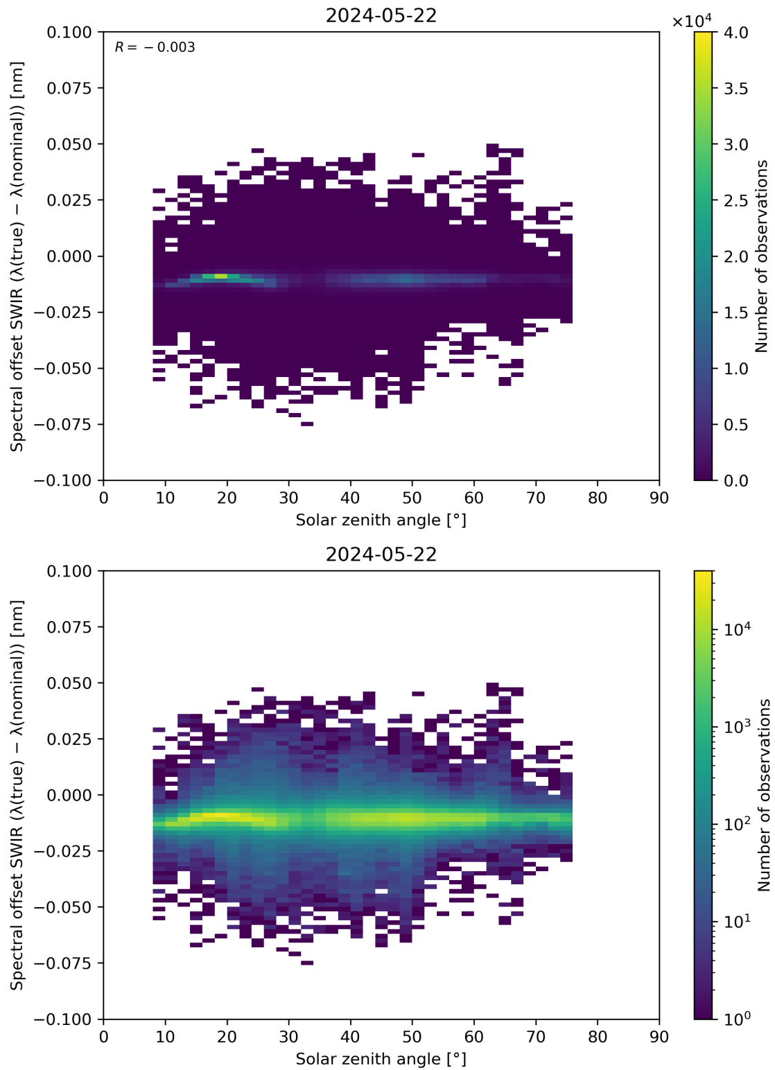
Figure 104: Scatter density plot of “Solar zenith angle” against “Spectral offset SWIR ( \lambda(\text{true}) - \lambda(\text{nominal}) )” for 2024-05-21 to 2024-05-23.
