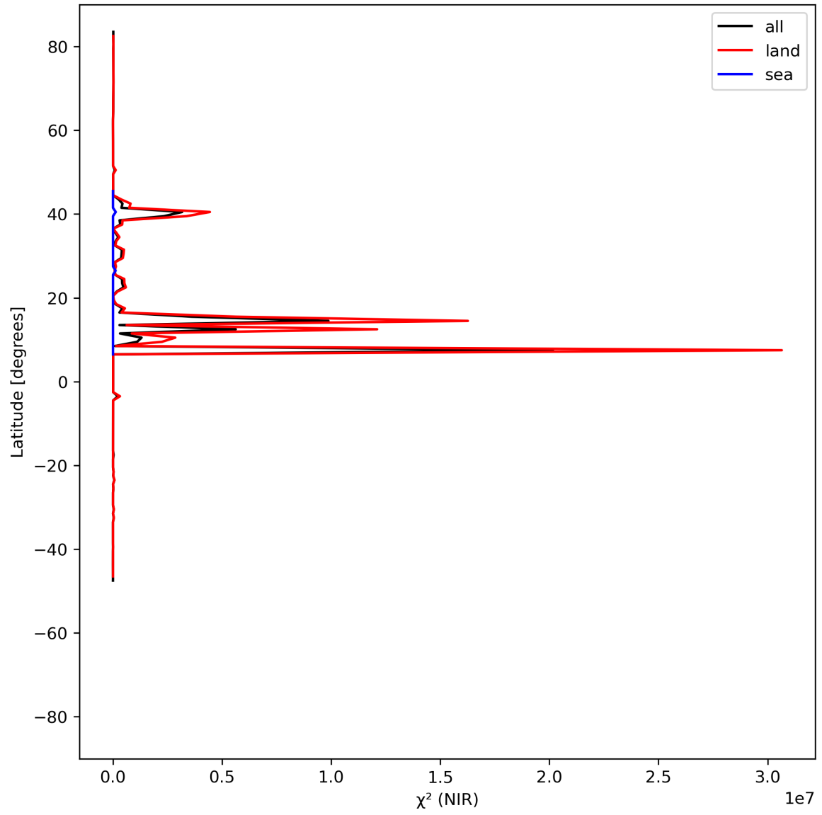
Figure 18: Zonal average of “ \chi^2 (NIR)” for 2024-05-21 to 2024-05-23.
