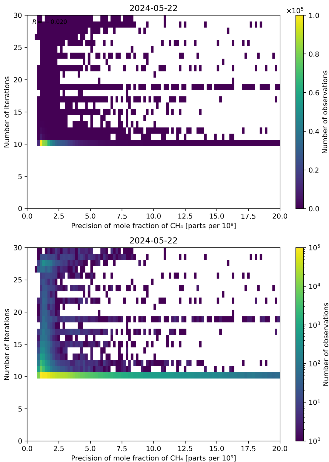
Figure 83: Scatter density plot of “Precision of mole fraction of CH 4 ” against “Number of iterations” for 2024-05-21 to 2024-05-23.
