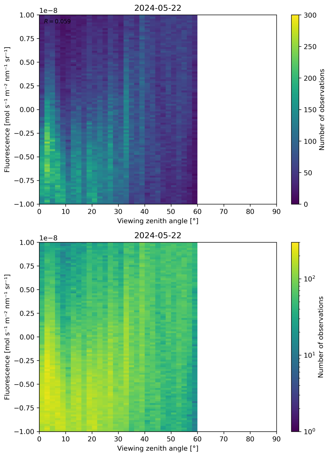
Figure 108: Scatter density plot of “Viewing zenith angle” against “Fluorescence” for 2024-05-21 to 2024-05-23.
