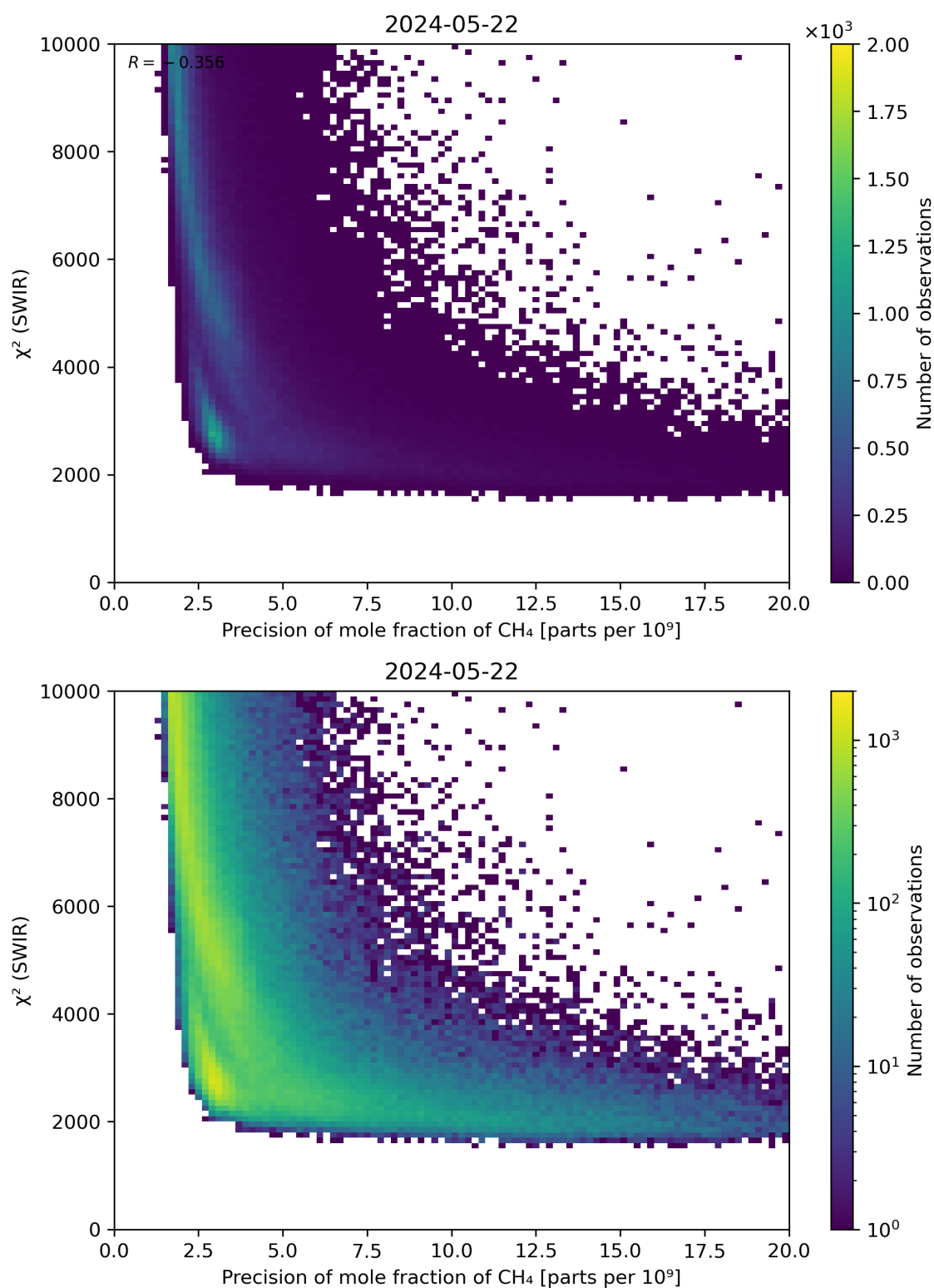
Figure 79: Scatter density plot of “Precision of mole fraction of \text{CH}_4 ” against “ \chi^2 (SWIR)” for 2024-05-21 to 2024-05-23.
