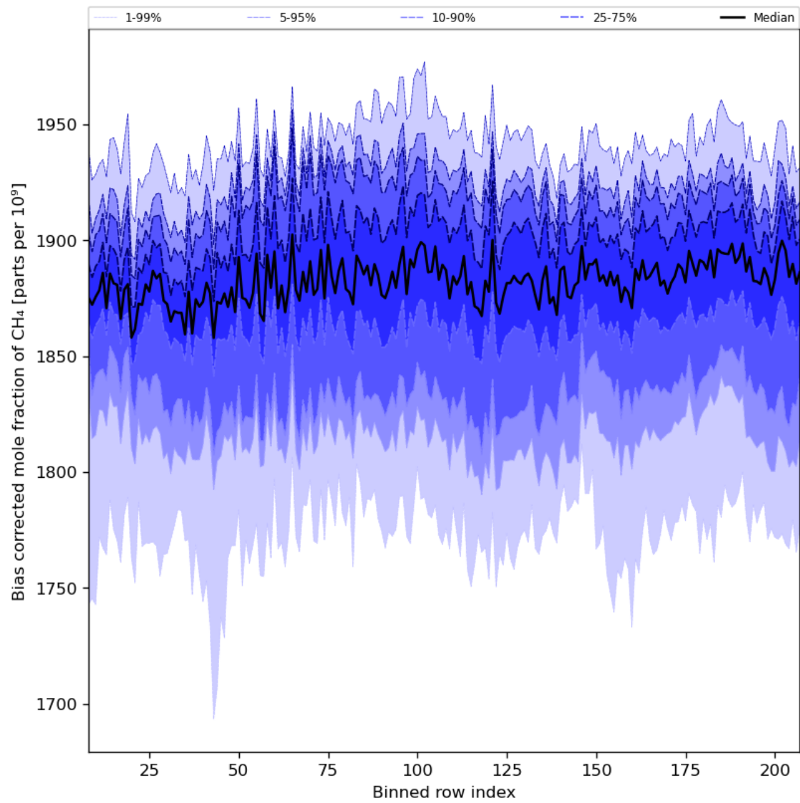
Figure 36: Along track statistics of “Bias corrected mole fraction of CH 4 ” for 2024-05-21 to 2024-05-23
