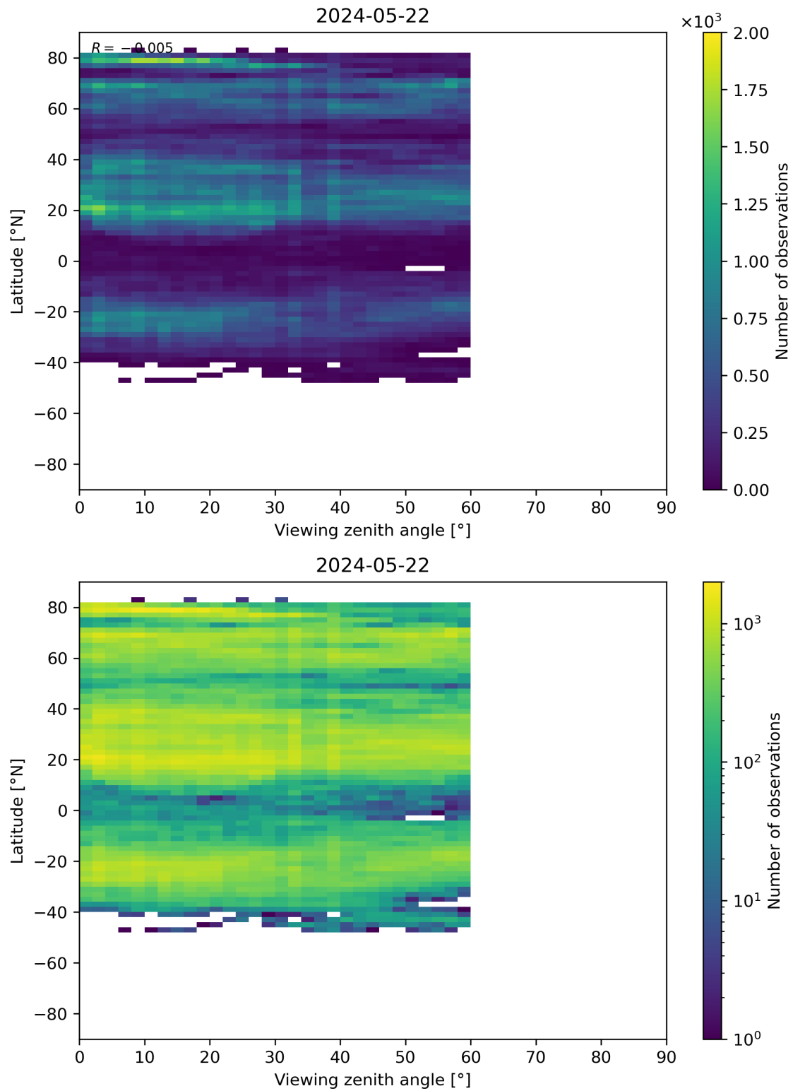
Figure 109: Scatter density plot of “Viewing zenith angle” against “Latitude” for 2024-05-21 to 2024-05-23.
