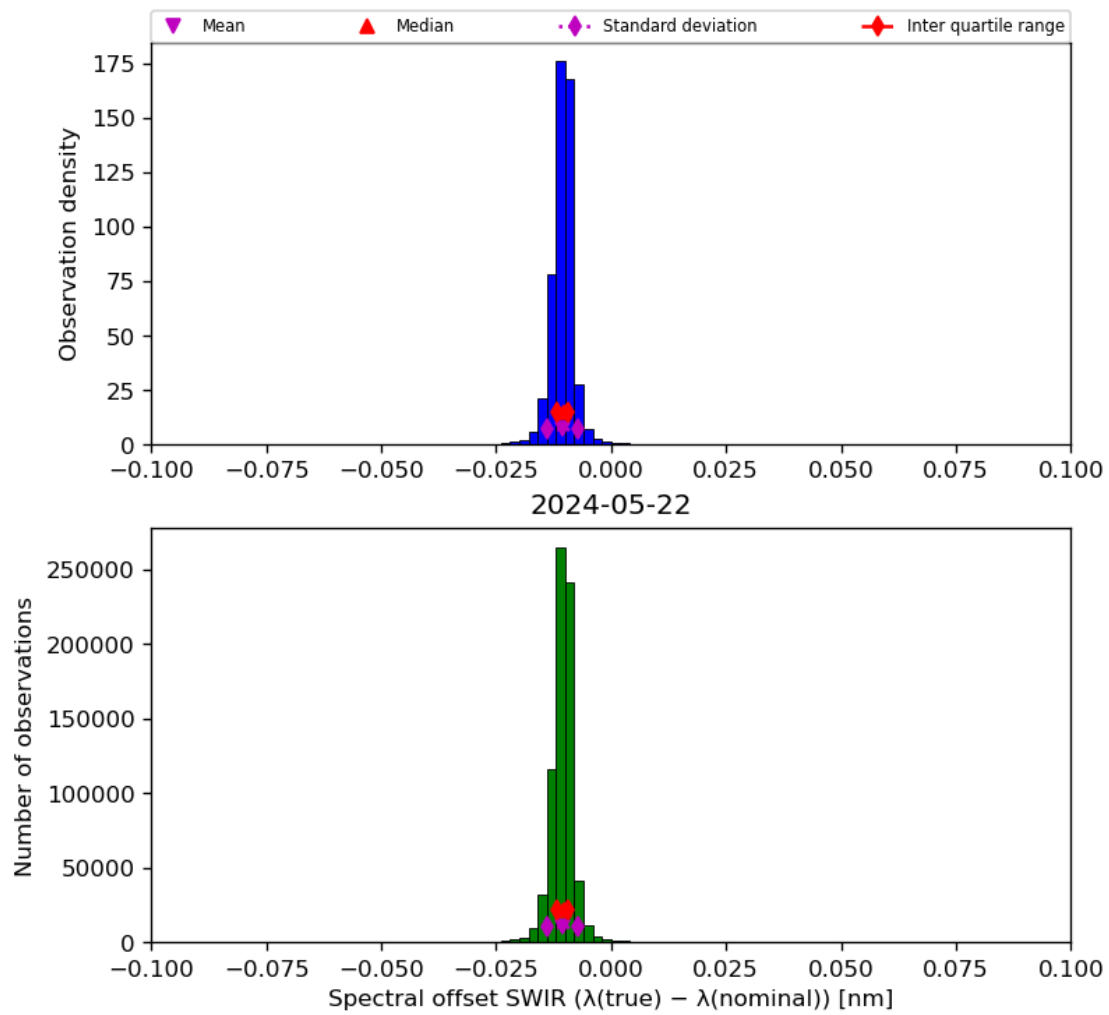
Figure 27: Histogram of “Spectral offset SWIR ( \lambda(\text{true}) - \lambda(\text{nominal}) )” for 2024-05-21 to 2024-05-23
