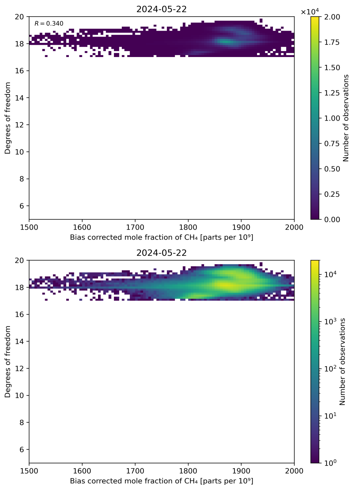
Figure 65: Scatter density plot of “Bias corrected mole fraction of CH 4 ” against “Degrees of freedom” for 2024-05-21 to 2024-05-23.
