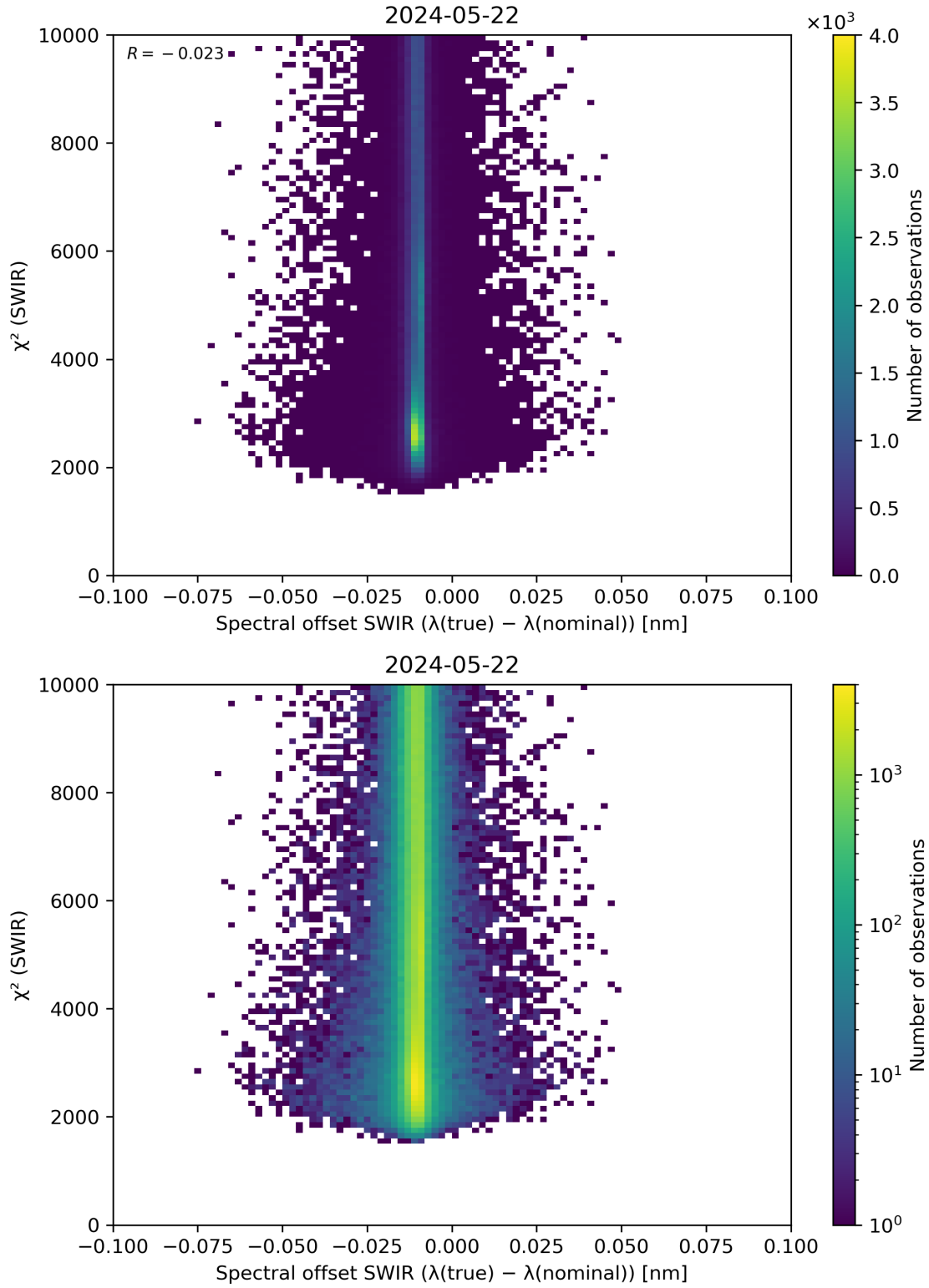
Figure 118: Scatter density plot of “Spectral offset SWIR ( \lambda(\text{true}) - \lambda(\text{nominal}) )” against “ \chi^2 (SWIR)” for 2024-05-21 to 2024-05-23.
