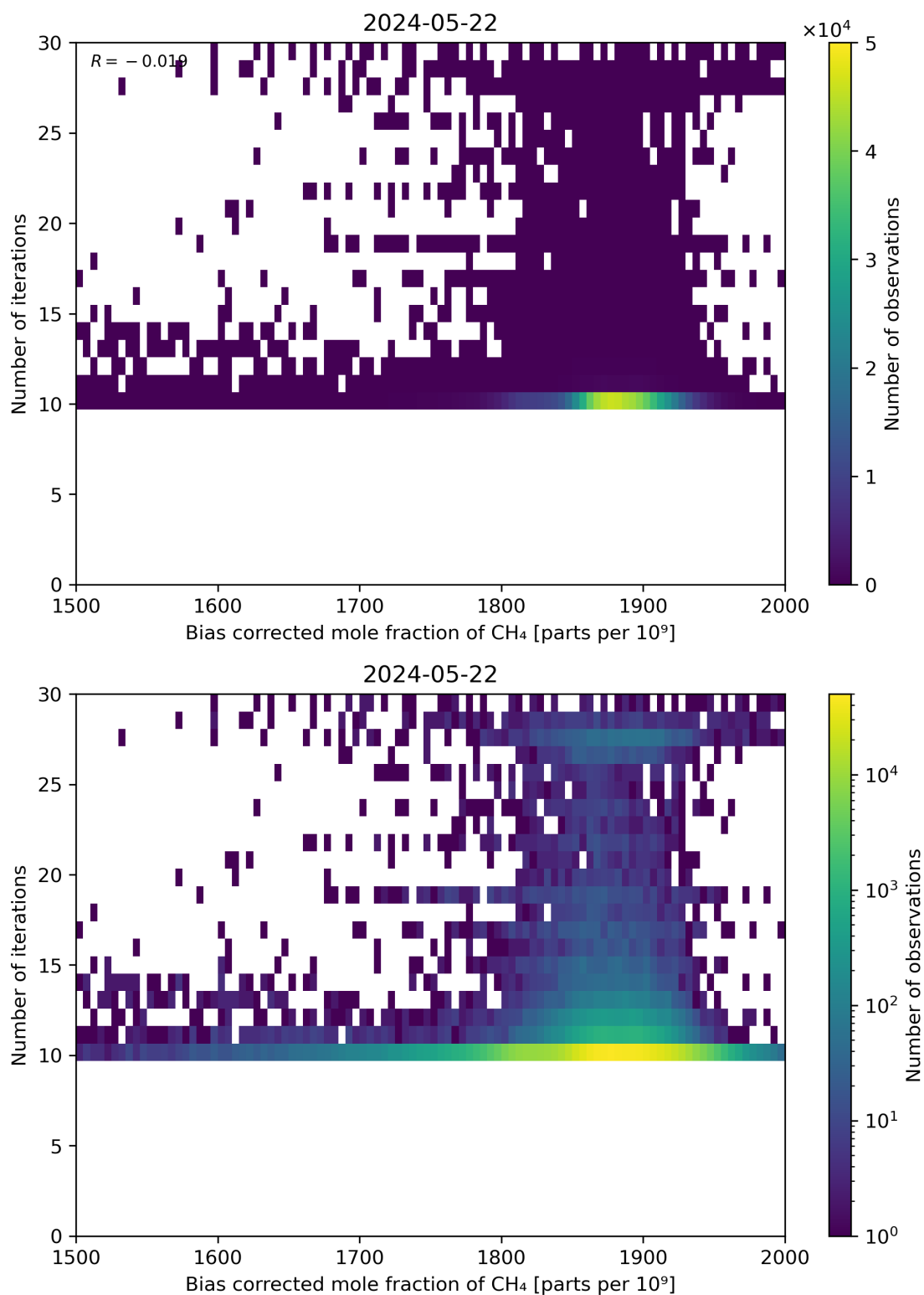
Figure 67: Scatter density plot of “Bias corrected mole fraction of CH 4 ” against “Number of iterations” for 2024-05-21 to 2024-05-23.
