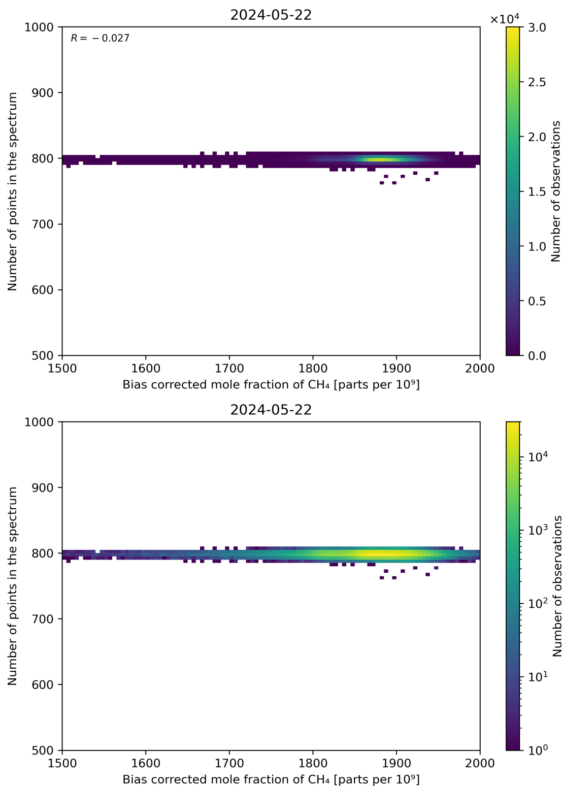
Figure 68: Scatter density plot of “Bias corrected mole fraction of CH 4 ” against “Number of points in the spectrum” for 2024-05-21 to 2024-05-23.
