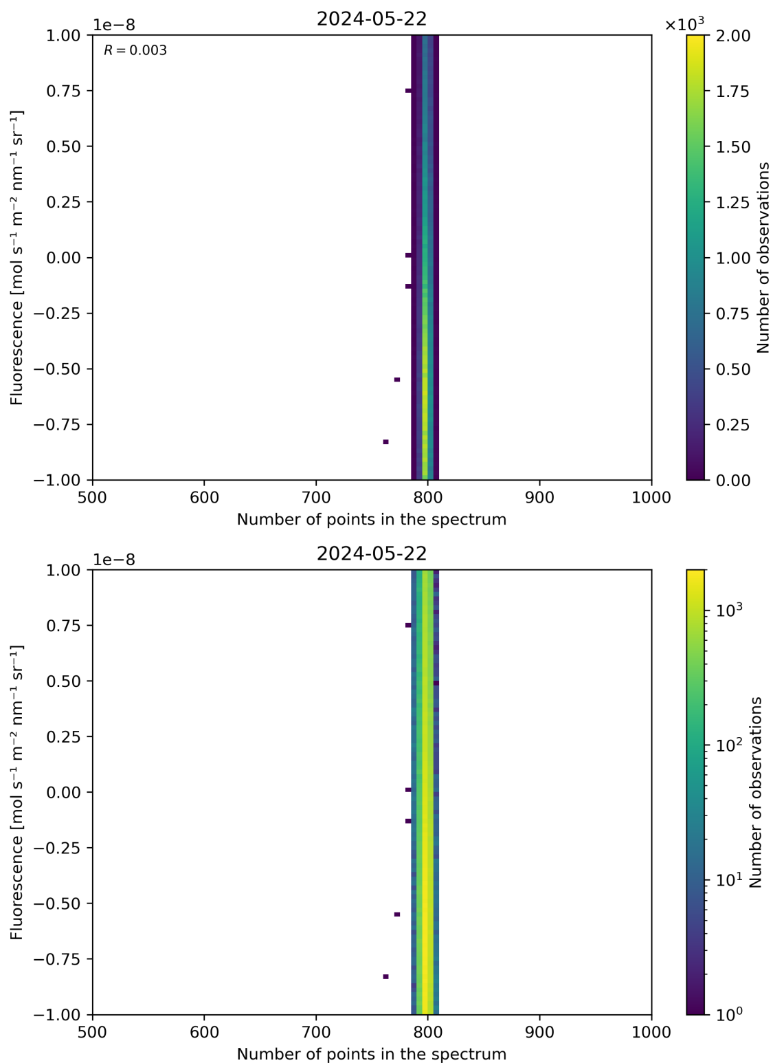
Figure 91: Scatter density plot of “Number of points in the spectrum” against “Fluorescence” for 2024-05-21 to 2024-05-23.
