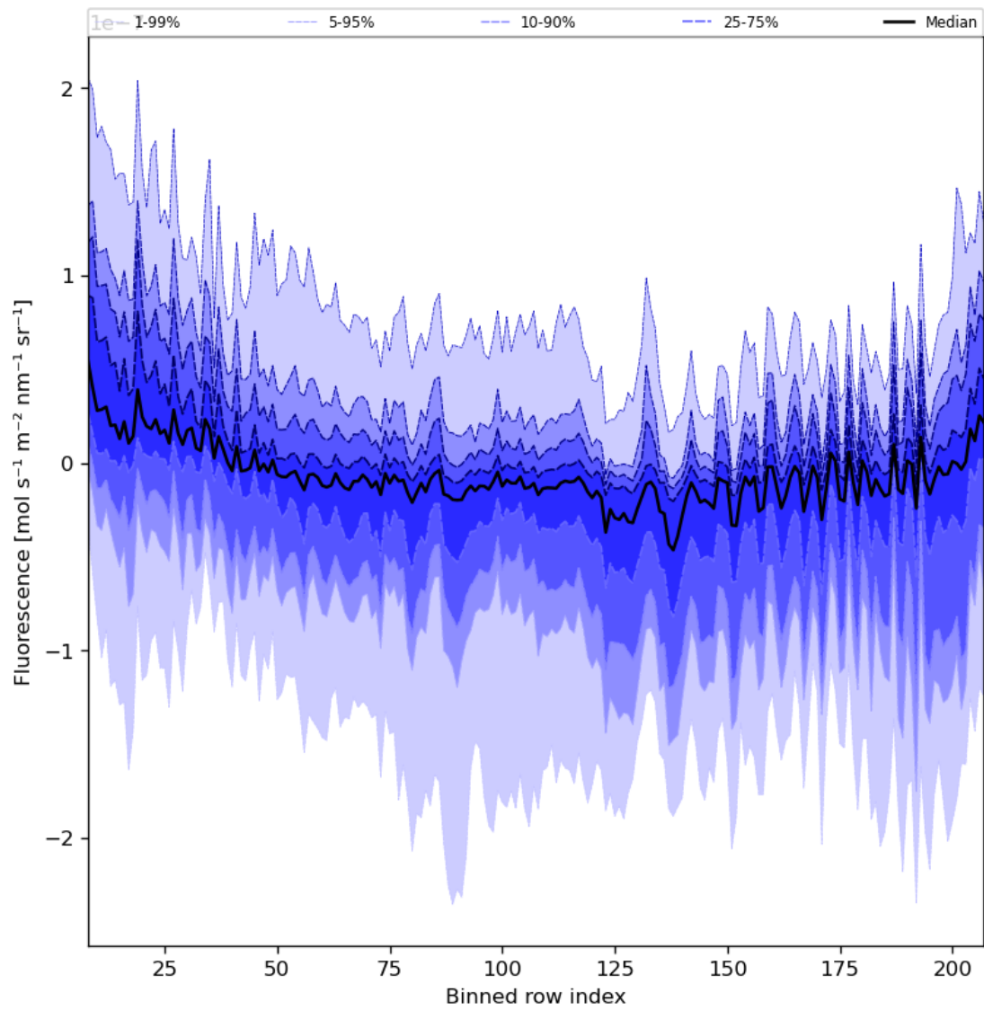
Figure 43: Along track statistics of “Fluorescence” for 2024-05-21 to 2024-05-23
