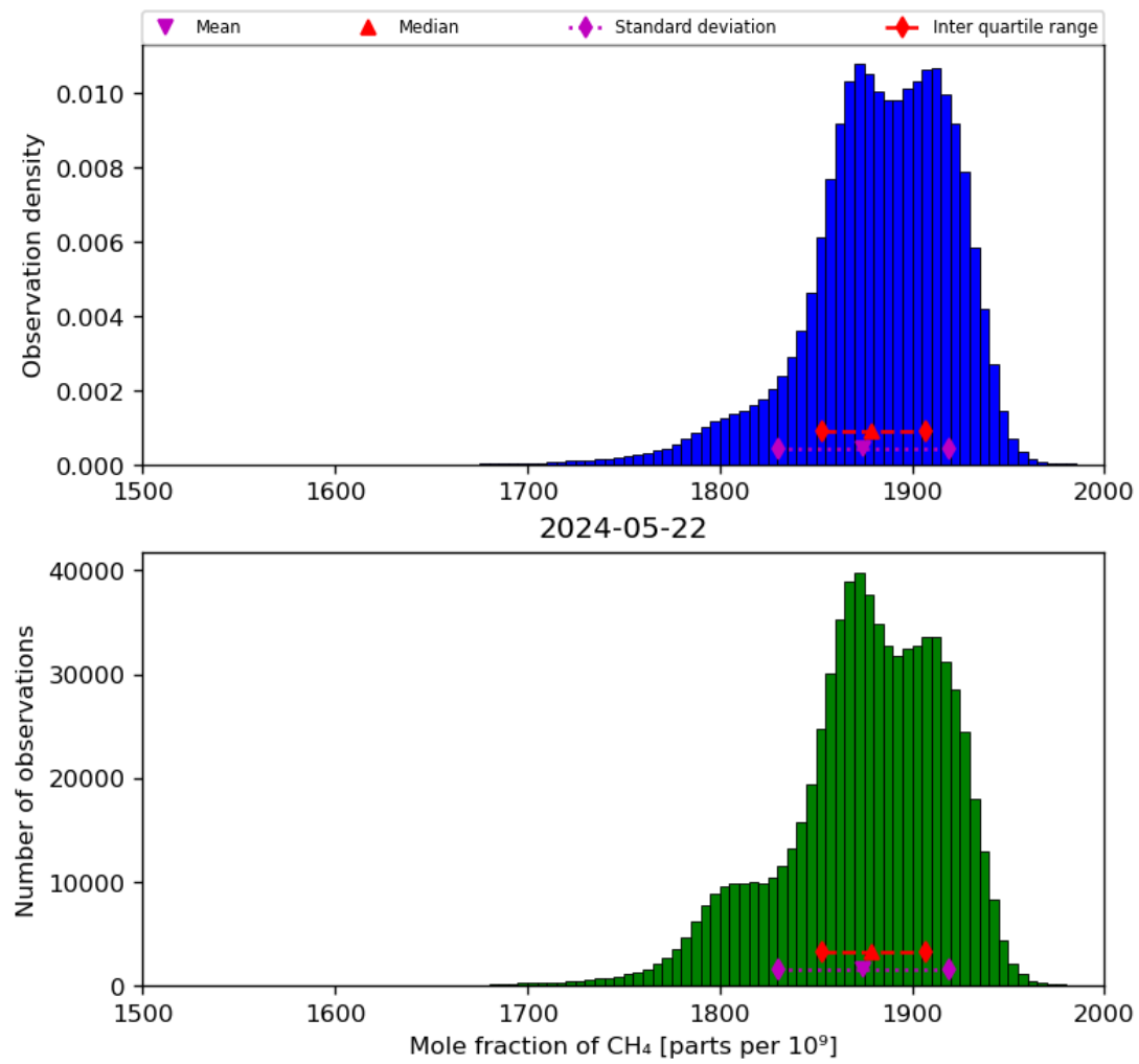
Figure 23: Histogram of “Mole fraction of CH 4 ” for 2024-05-21 to 2024-05-23
