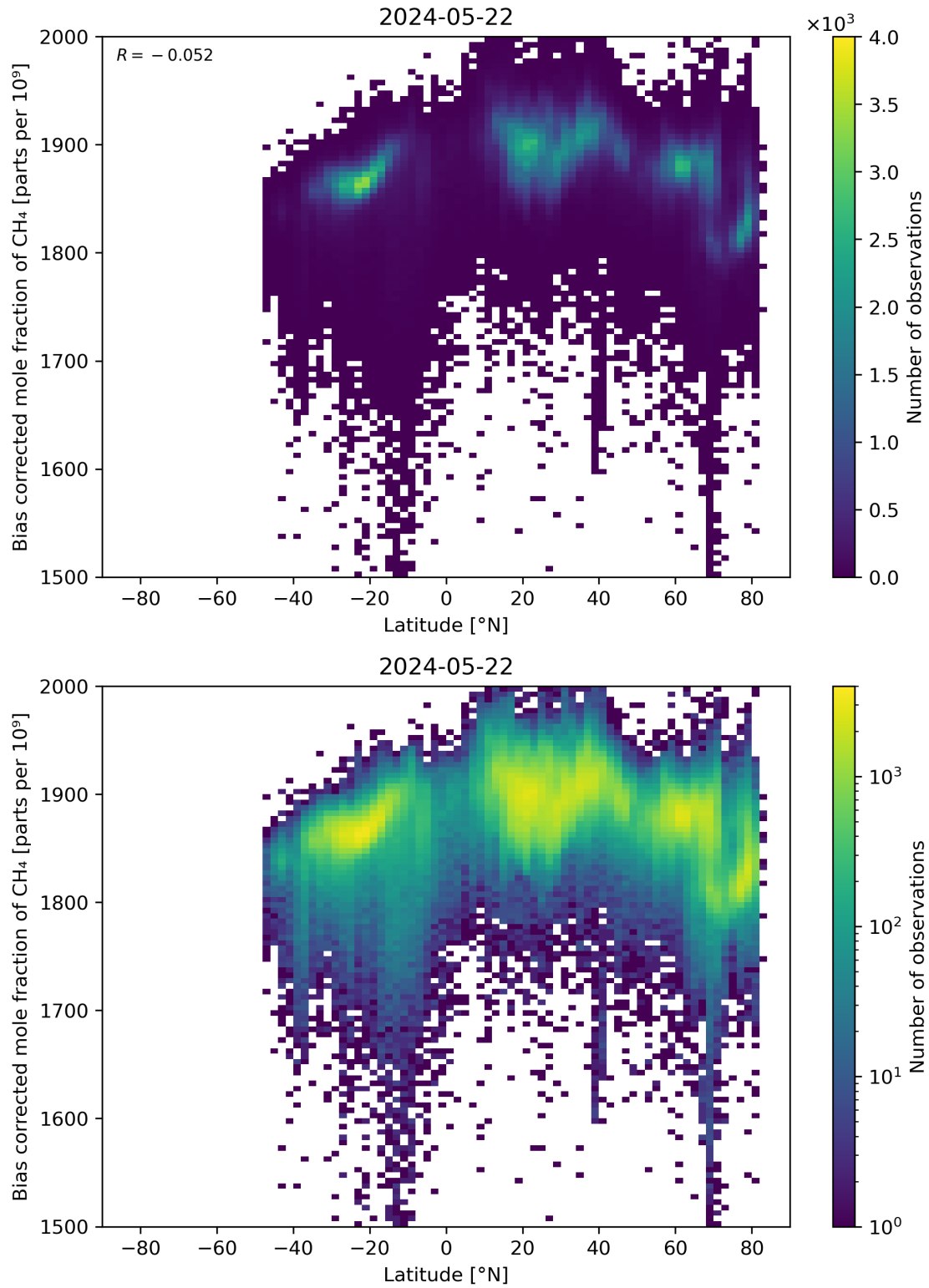
Figure 58: Scatter density plot of “Latitude” against “Bias corrected mole fraction of CH 4 ” for 2024-05-21 to 2024-05-23.
