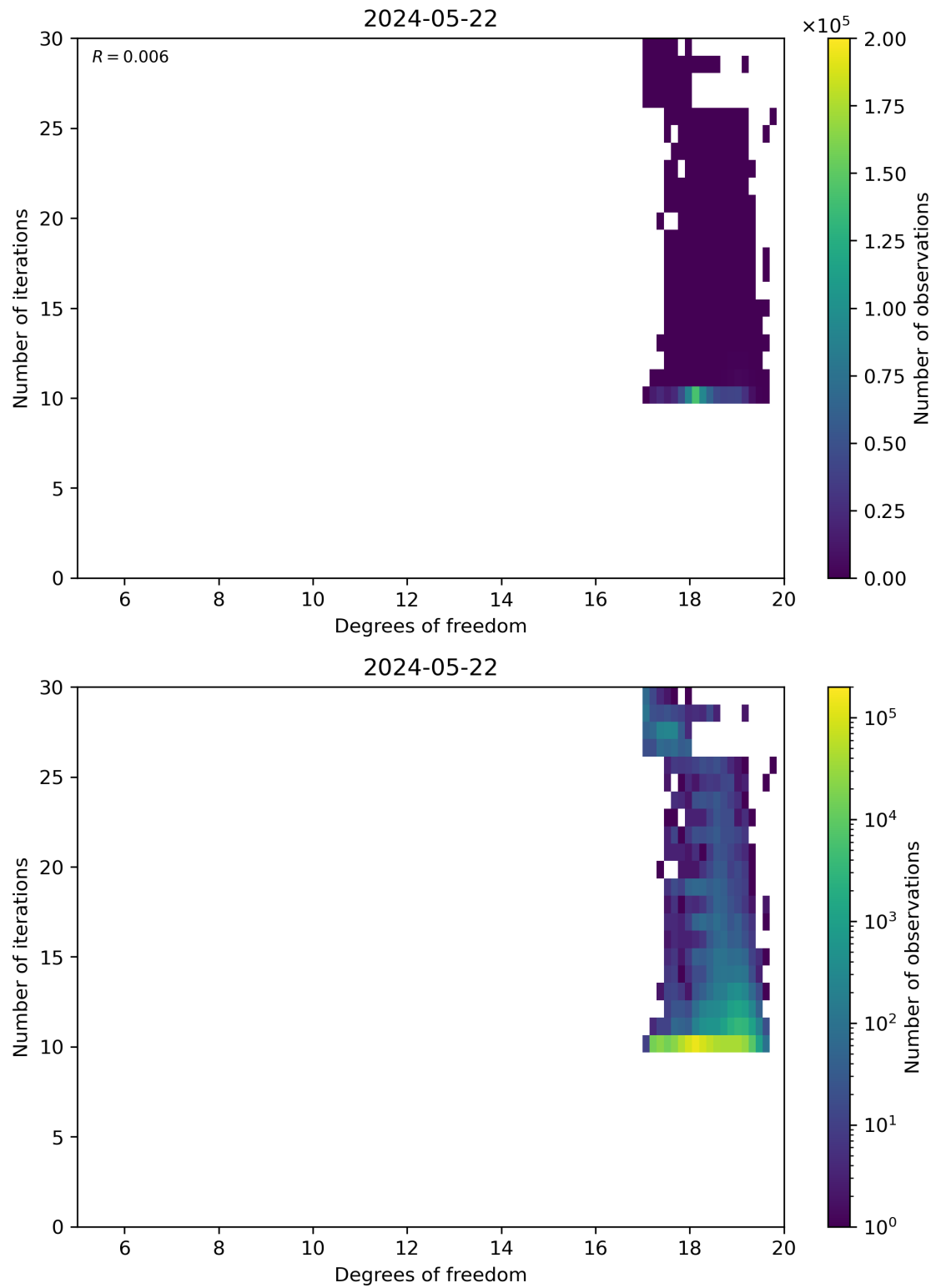
Figure 52: Scatter density plot of “Degrees of freedom” against “Number of iterations” for 2024-05-21 to 2024-05-23.
