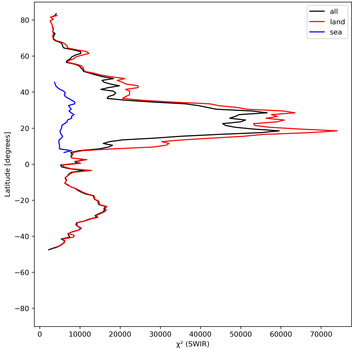
Figure 17: Zonal average of “ \chi^2 (SWIR)” for 2024-05-21 to 2024-05-23.
