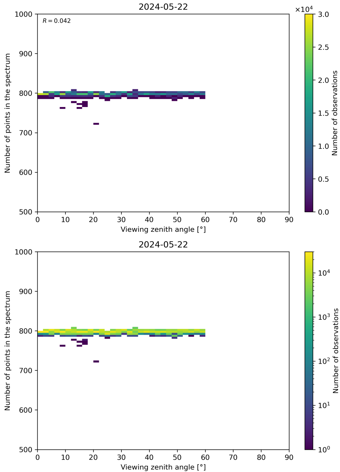
Figure 114: Scatter density plot of “Viewing zenith angle” against “Number of points in the spectrum” for 2024-05-21 to 2024-05-23.
