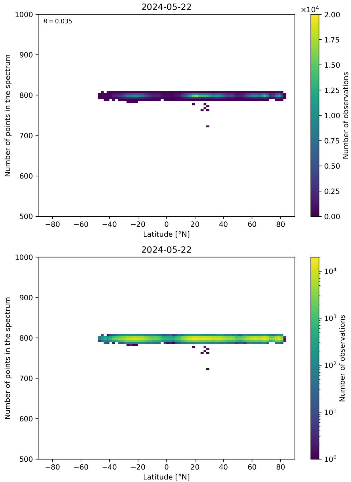
Figure 61: Scatter density plot of “Latitude” against “Number of points in the spectrum” for 2024-05-21 to 2024-05-23.
