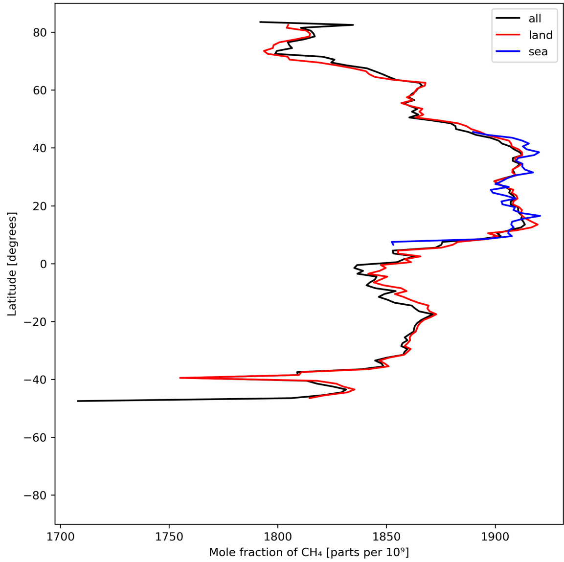
Figure 12: Zonal average of “Mole fraction of \text{CH}_4 ” for 2024-05-21 to 2024-05-23.
