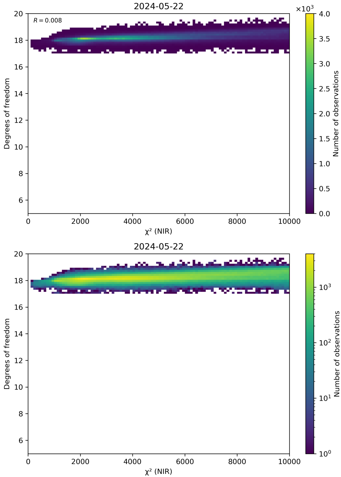
Figure 44: Scatter density plot of “ \chi^2 (NIR)” against “Degrees of freedom” for 2024-05-21 to 2024-05-23.
