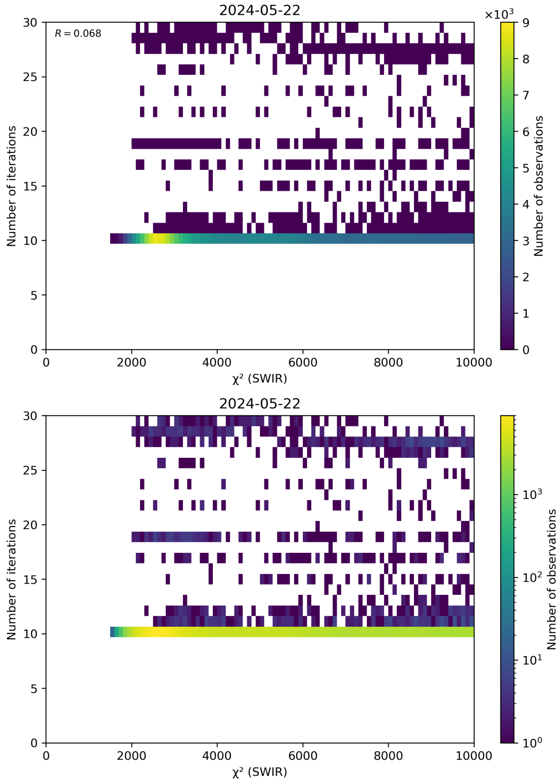
Figure 50: Scatter density plot of “ \chi^2 (SWIR)” against “Number of iterations” for 2024-05-21 to 2024-05-23.
