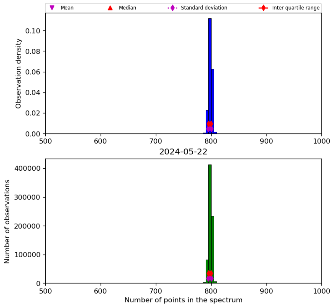
Figure 26: Histogram of “Number of points in the spectrum” for 2024-05-21 to 2024-05-23
