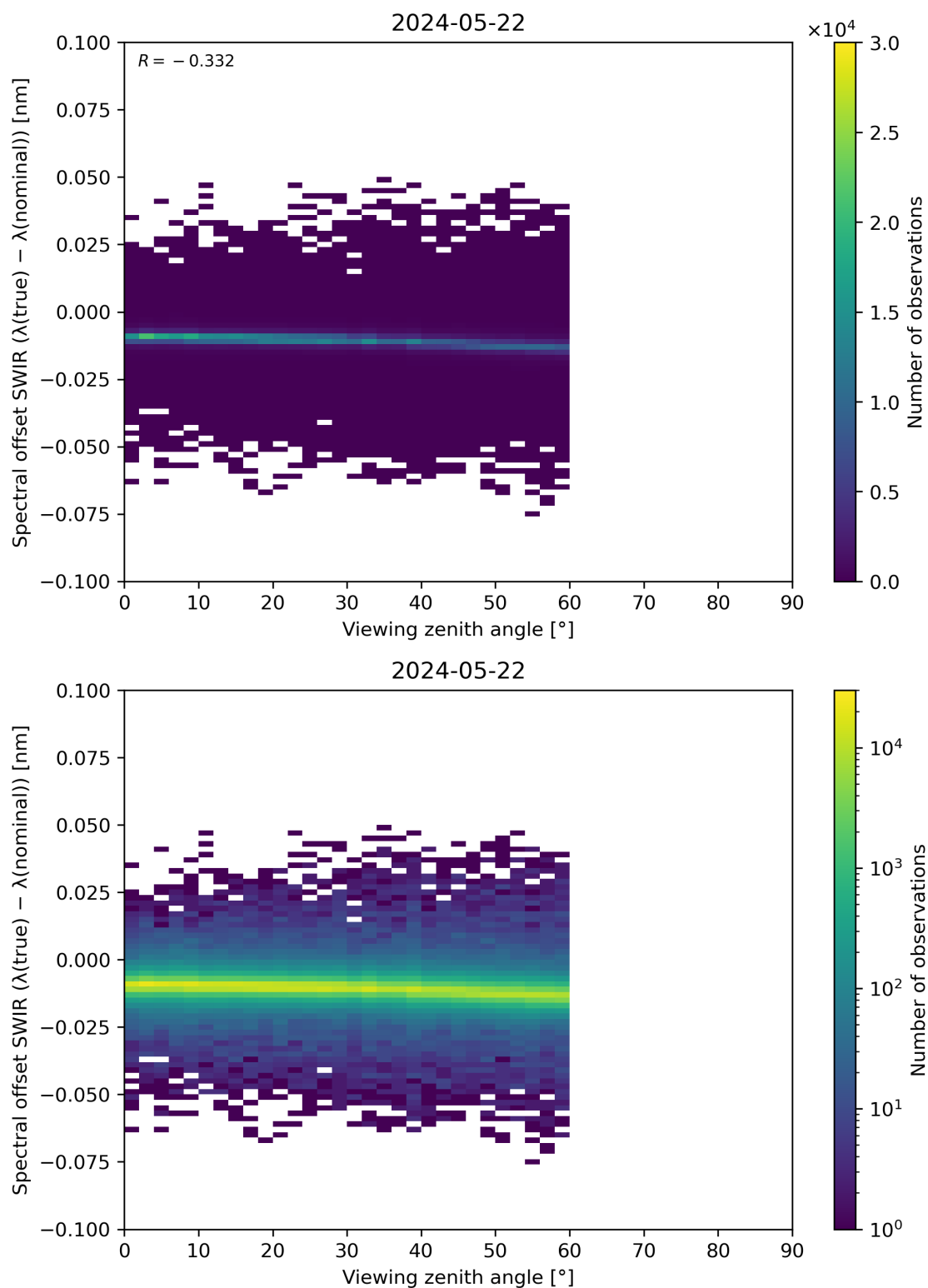
Figure 116: Scatter density plot of “Viewing zenith angle” against “Spectral offset SWIR ( \lambda(\text{true}) - \lambda(\text{nominal}) )” for 2024-05-21 to 2024-05-23.
