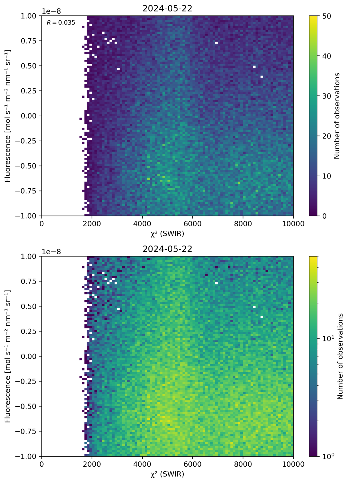
Figure 49: Scatter density plot of “ \chi^2 (SWIR)” against “Fluorescence” for 2024-05-21 to 2024-05-23.
