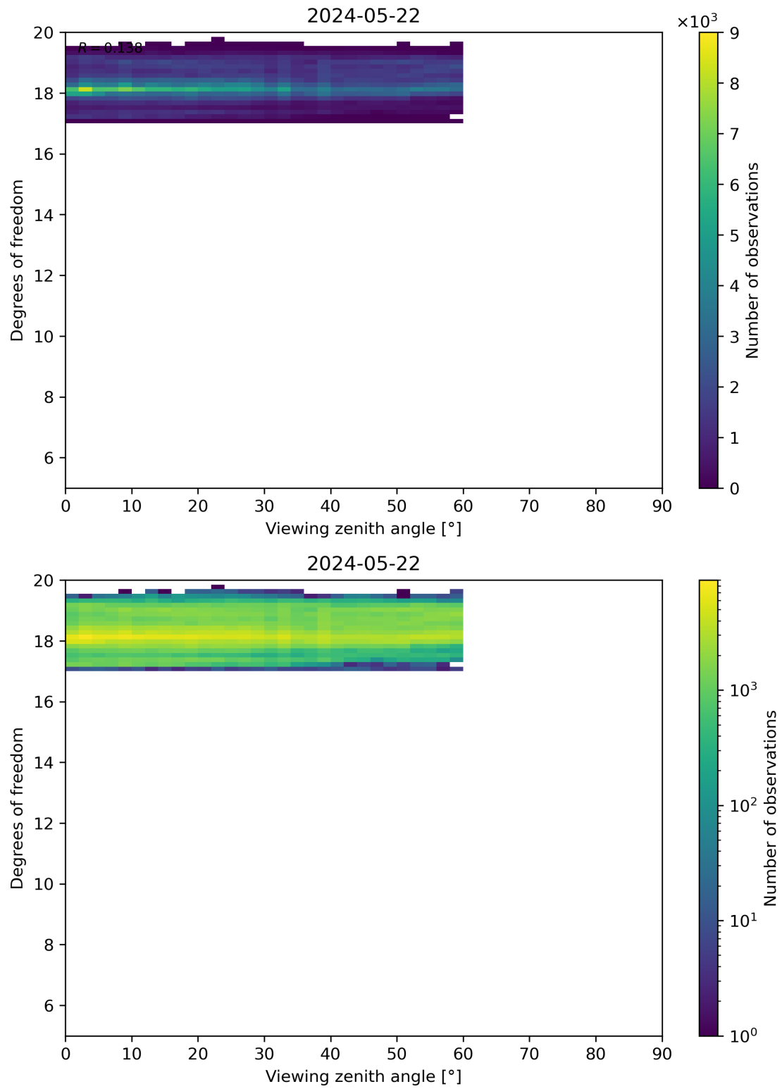
Figure 107: Scatter density plot of “Viewing zenith angle” against “Degrees of freedom” for 2024-05-21 to 2024-05-23.
