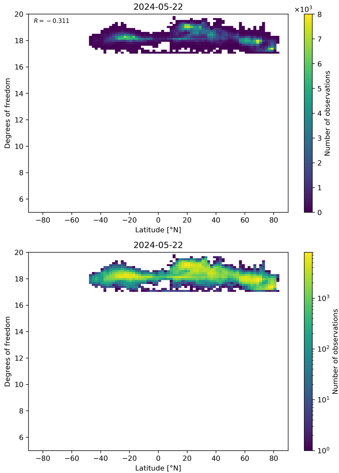
Figure 55: Scatter density plot of “Latitude” against “Degrees of freedom” for 2024-05-21 to 2024-05-23.
