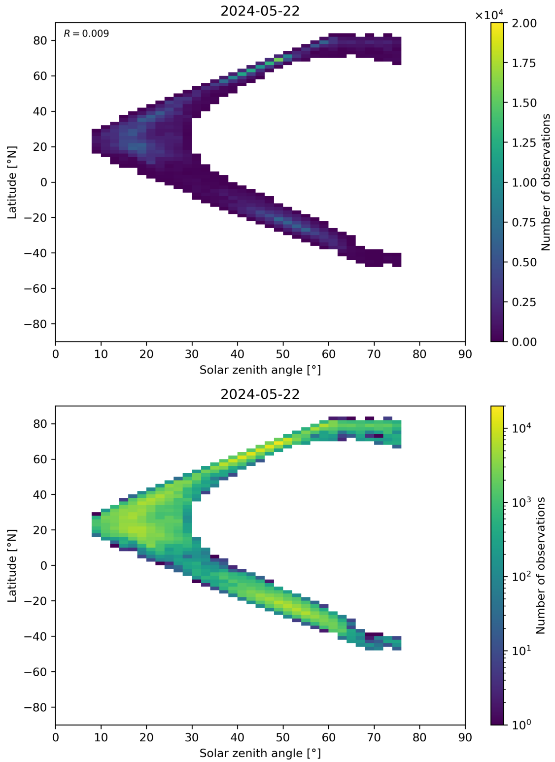
Figure 98: Scatter density plot of “Solar zenith angle” against “Latitude” for 2024-05-21 to 2024-05-23.
