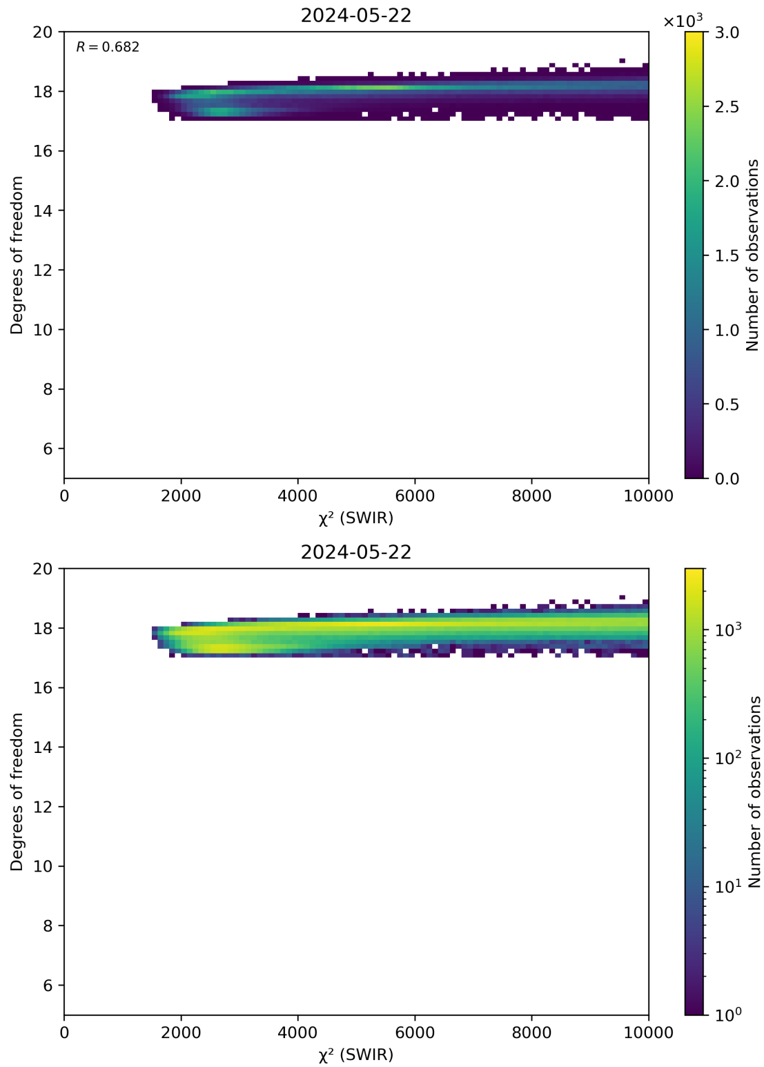
Figure 48: Scatter density plot of “ \chi^2 (SWIR)” against “Degrees of freedom” for 2024-05-21 to 2024-05-23.
