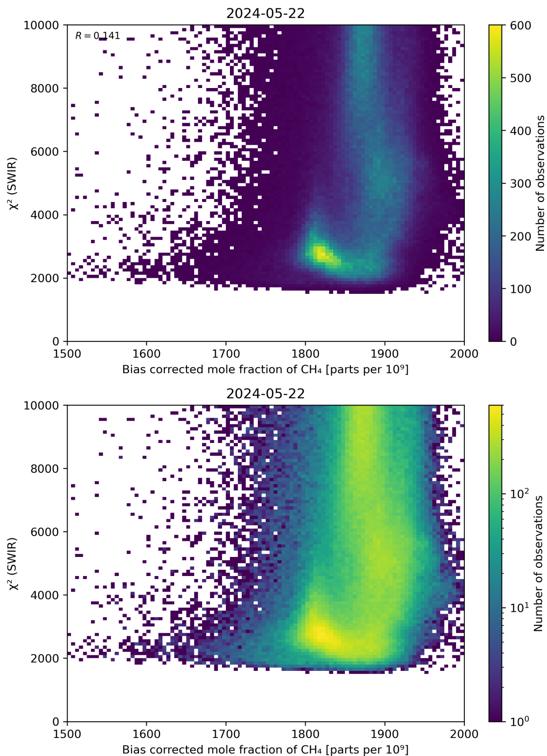
Figure 64: Scatter density plot of “Bias corrected mole fraction of CH 4 ” against “ \chi^2 (SWIR)” for 2024-05-21 to 2024-05-23.
