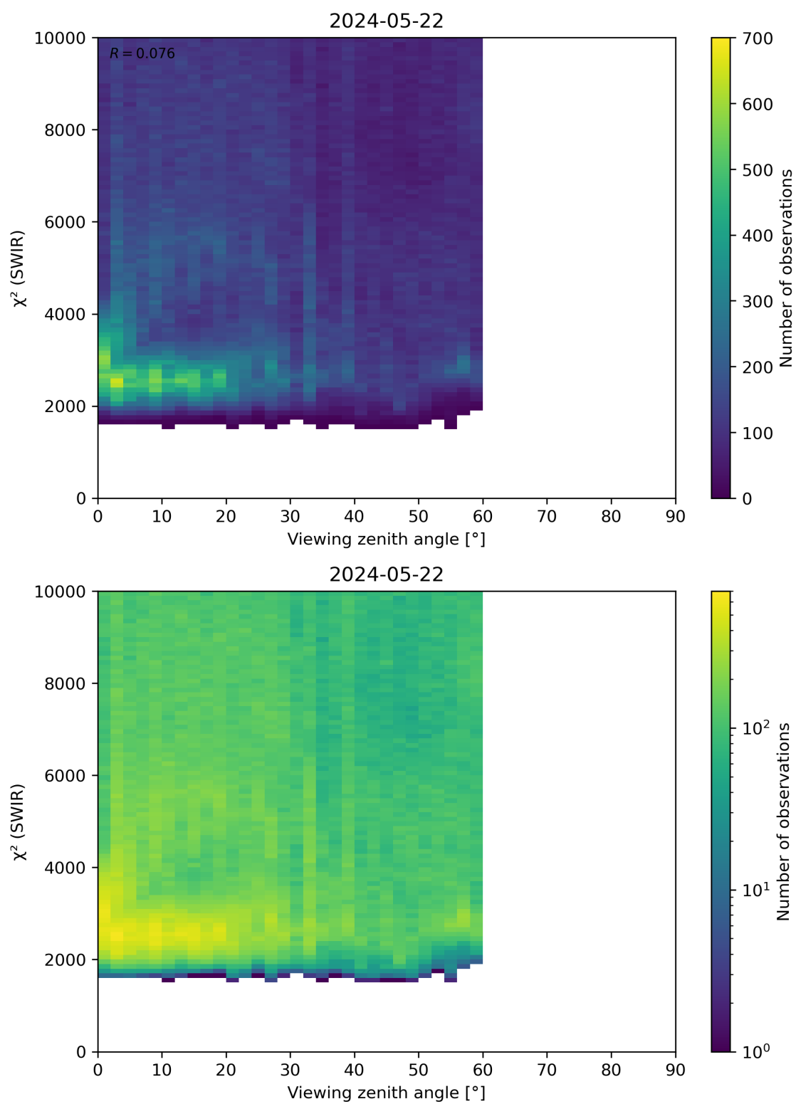
Figure 106: Scatter density plot of “Viewing zenith angle” against “ \chi^2 (SWIR)” for 2024-05-21 to 2024-05-23.
