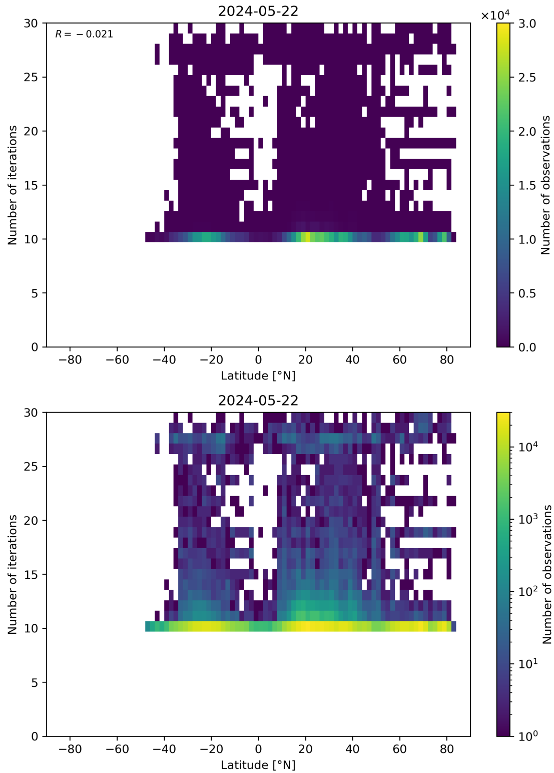
Figure 60: Scatter density plot of “Latitude” against “Number of iterations” for 2024-05-21 to 2024-05-23.
