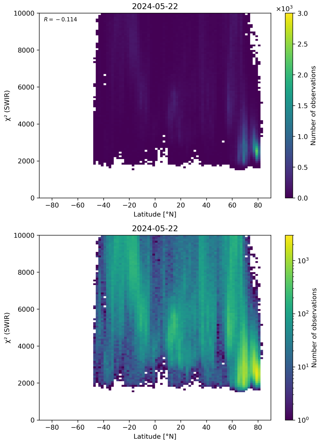
Figure 54: Scatter density plot of “Latitude” against “ \chi^2 (SWIR)” for 2024-05-21 to 2024-05-23.
