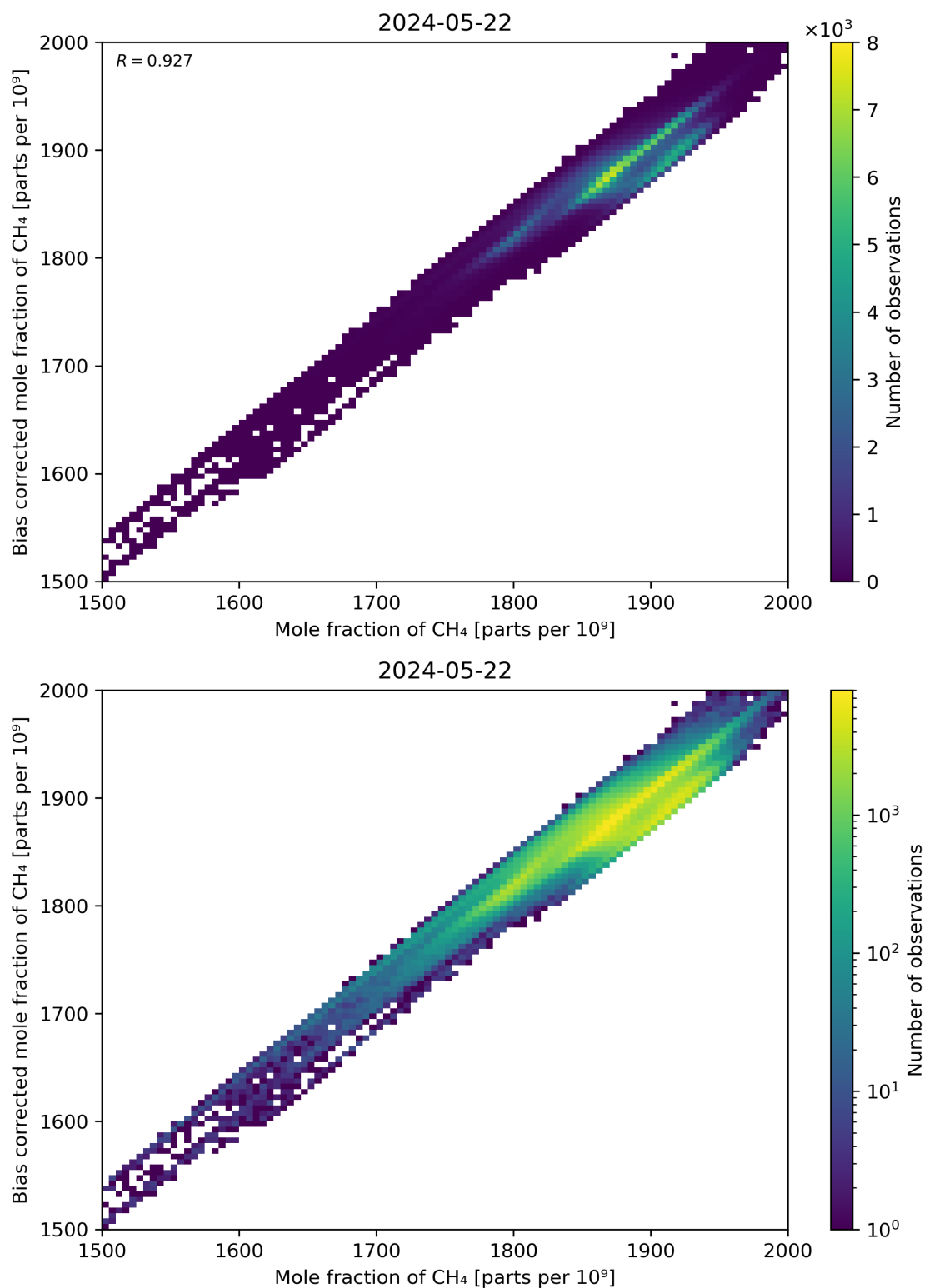
Figure 74: Scatter density plot of “Mole fraction of CH 4 ” against “Bias corrected mole fraction of CH 4 ” for 2024-05-21 to 2024-05-23.
