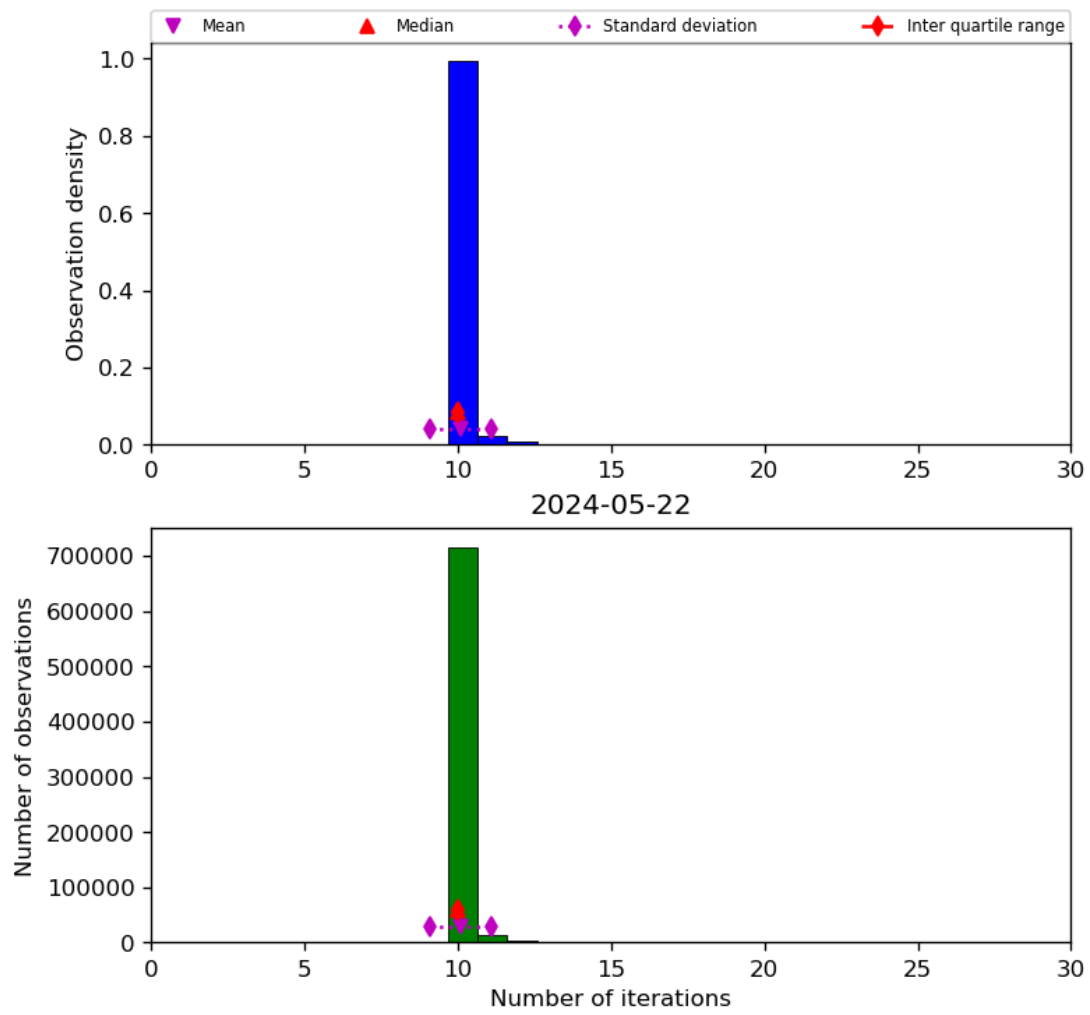
Figure 31: Histogram of “Number of iterations” for 2024-05-21 to 2024-05-23
