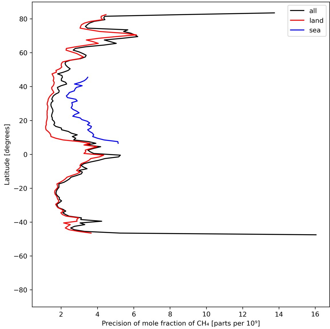
Figure 13: Zonal average of “Precision of mole fraction of CH 4 ” for 2024-05-21 to 2024-05-23.
