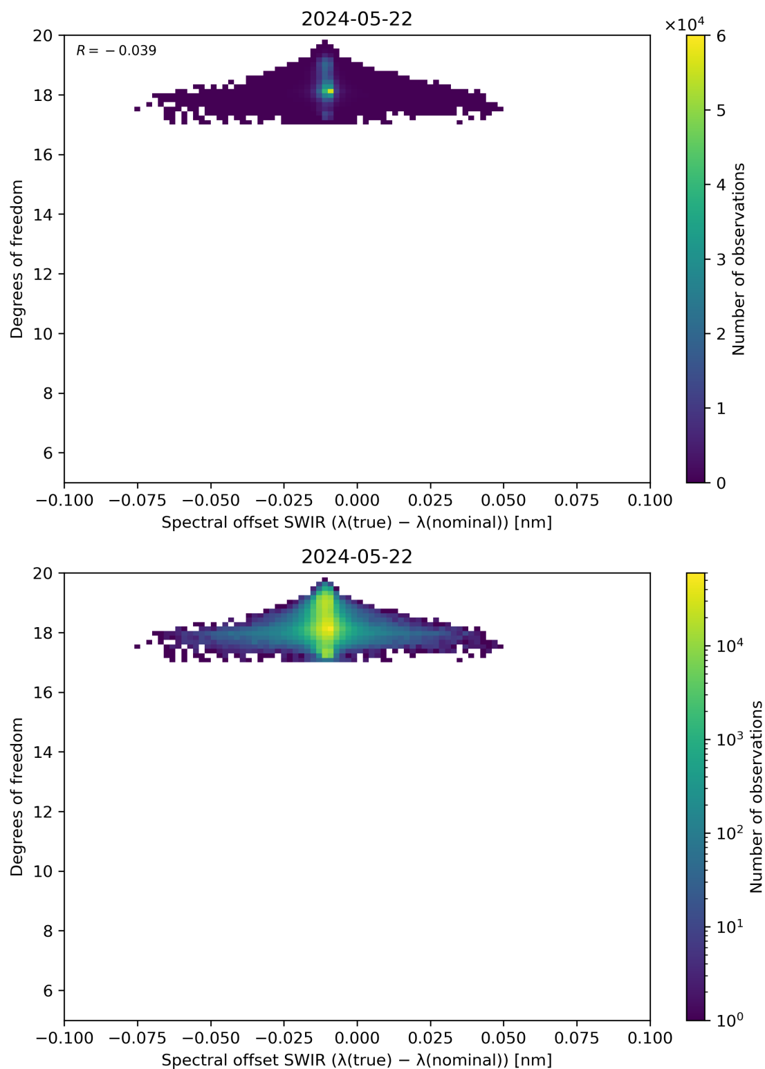
Figure 119: Scatter density plot of “Spectral offset SWIR ( \lambda(\text{true}) - \lambda(\text{nominal}) )” against “Degrees of freedom” for 2024-05-21 to 2024-05-23.
