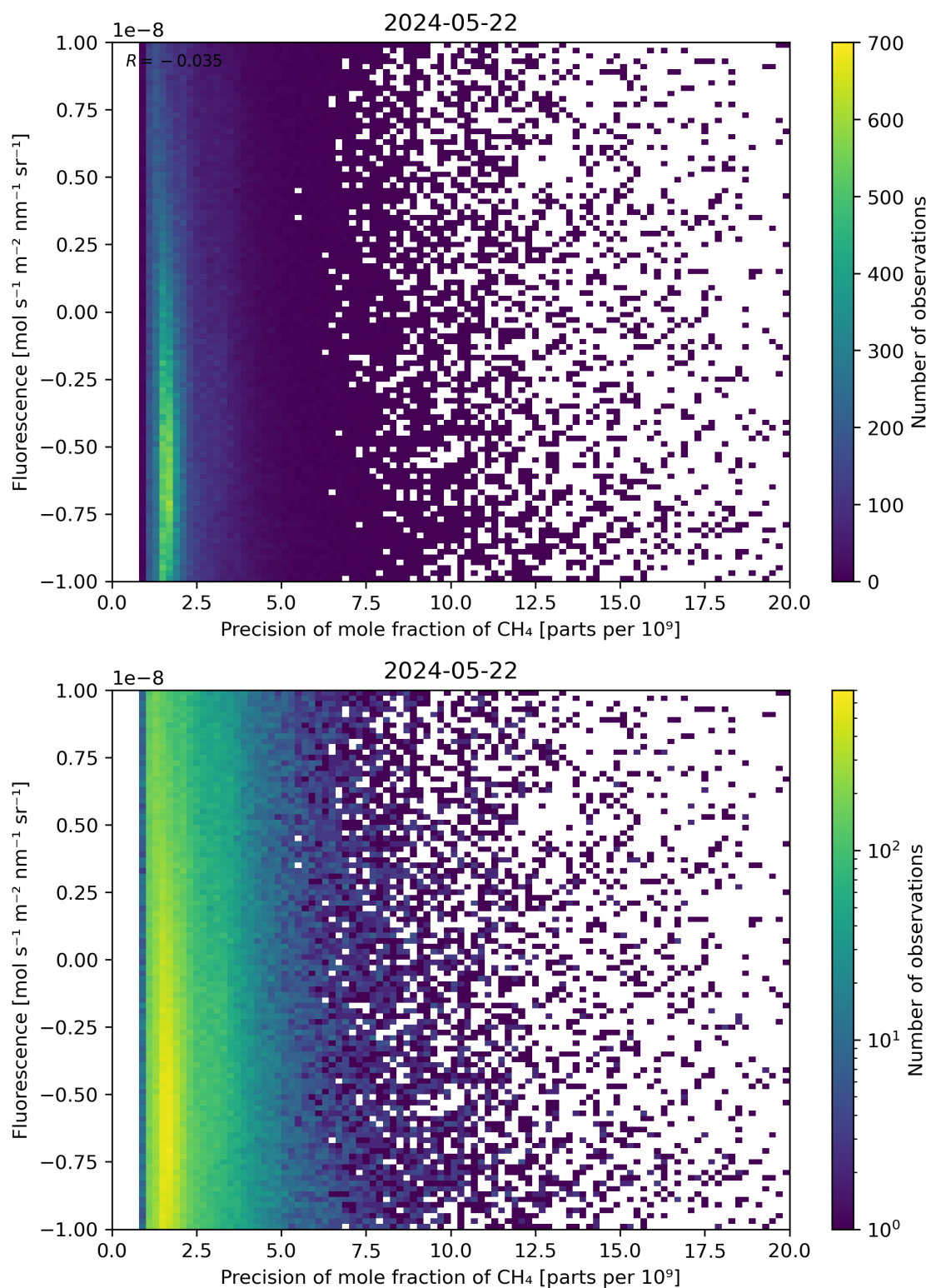
Figure 81: Scatter density plot of “Precision of mole fraction of \text{CH}_4 ” against “Fluorescence” for 2024-05-21 to 2024-05-23.
