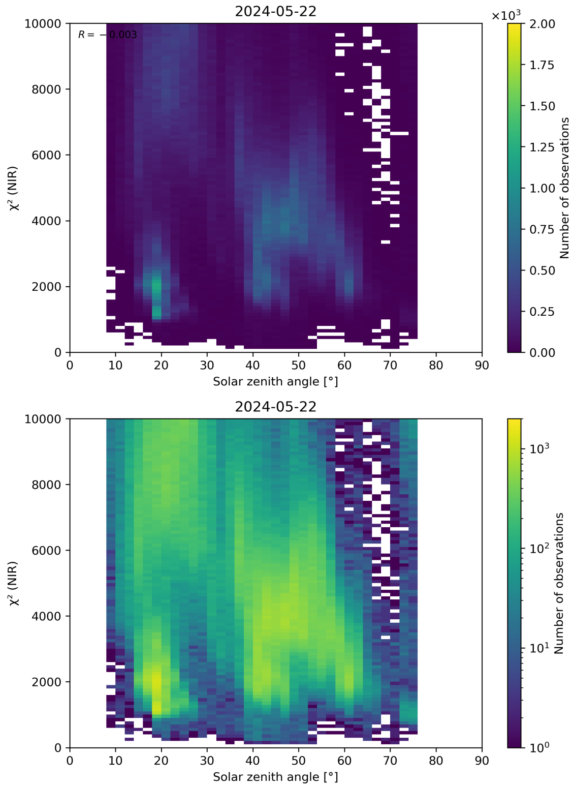
Figure 94: Scatter density plot of “Solar zenith angle” against “ \chi^2 (NIR)” for 2024-05-21 to 2024-05-23.
