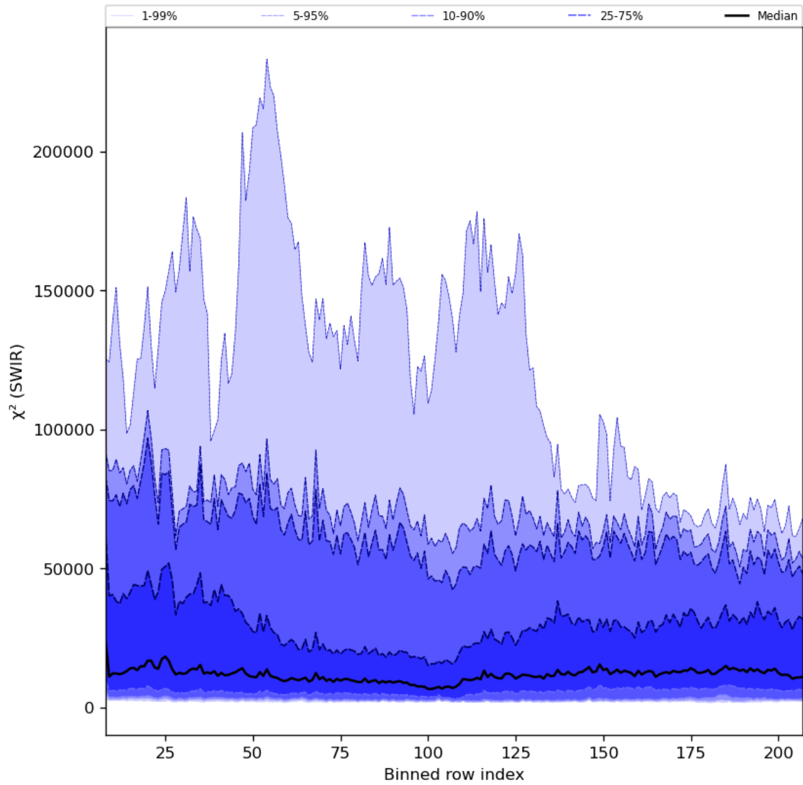
Figure 39: Along track statistics of “ \chi^2 (SWIR)” for 2024-05-21 to 2024-05-23
