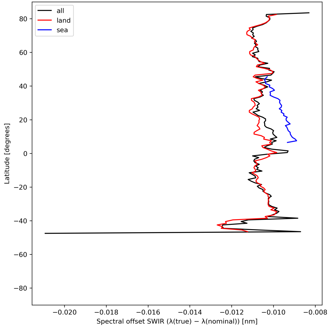
Figure 16: Zonal average of “Spectral offset SWIR ( \lambda(\text{true}) - \lambda(\text{nominal}) )” for 2024-05-21 to 2024-05-23.
