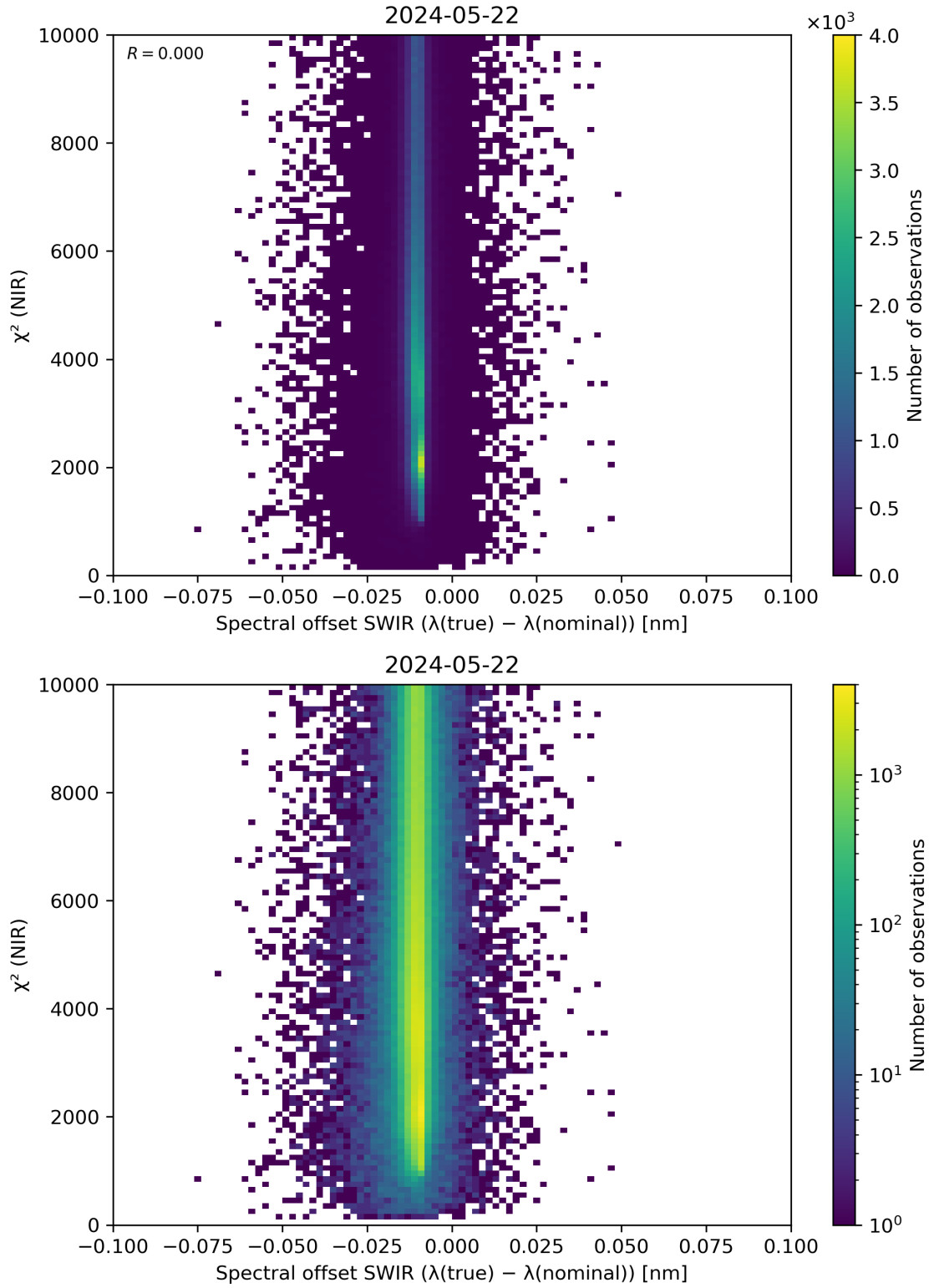
Figure 117: Scatter density plot of “Spectral offset SWIR ( \lambda(\text{true}) - \lambda(\text{nominal}) )” against “ \chi^2 (NIR)” for 2024-05-21 to 2024-05-23.
