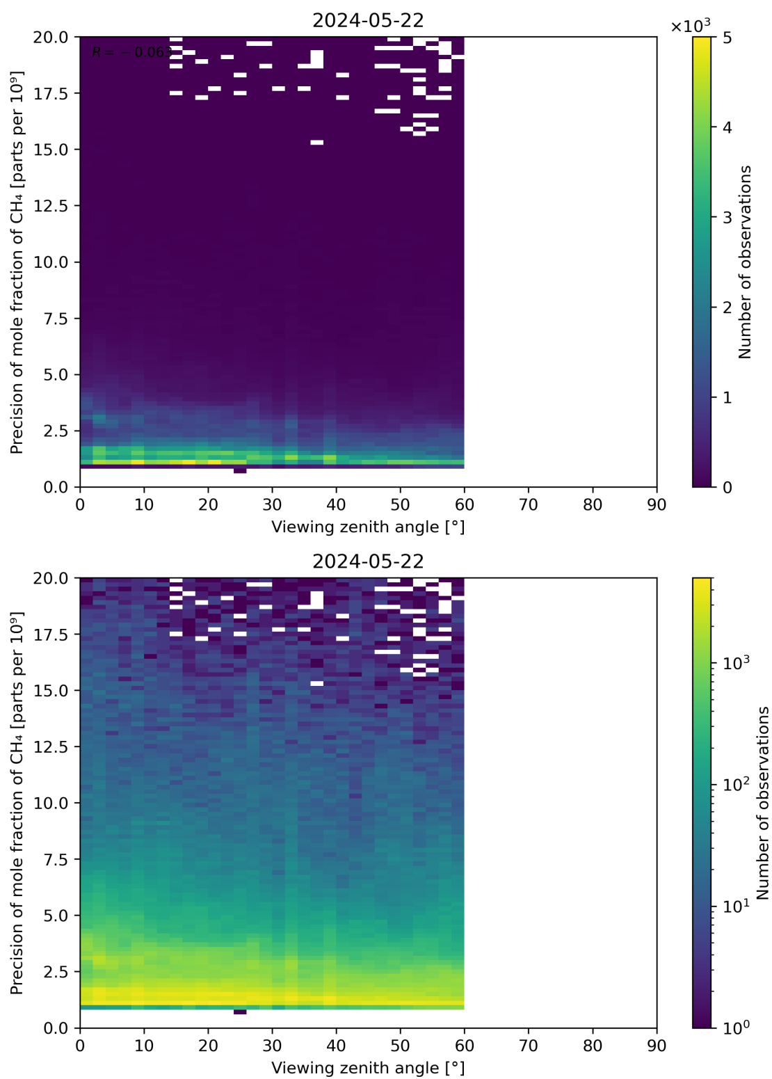
Figure 112: Scatter density plot of “Viewing zenith angle” against “Precision of mole fraction of CH 4 ” for 2024-05-21 to 2024-05-23.
