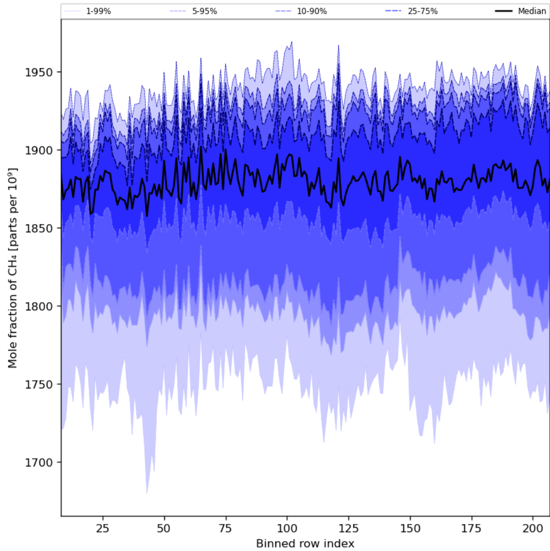
Figure 34: Along track statistics of “Mole fraction of CH 4 ” for 2024-05-21 to 2024-05-23
