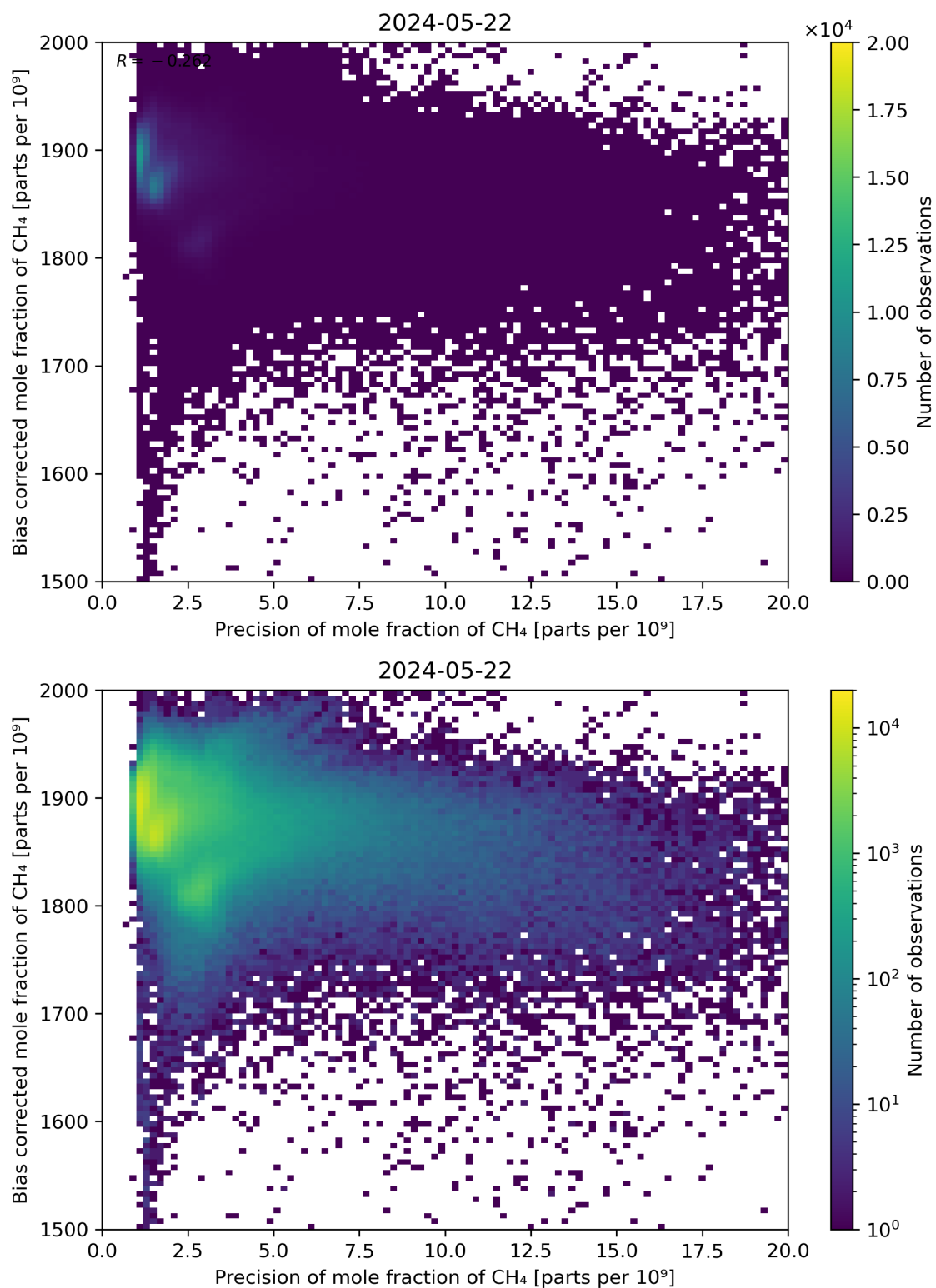
Figure 82: Scatter density plot of “Precision of mole fraction of \text{CH}_4 ” against “Bias corrected mole fraction of \text{CH}_4 ” for 2024-05-21 to 2024-05-23.
