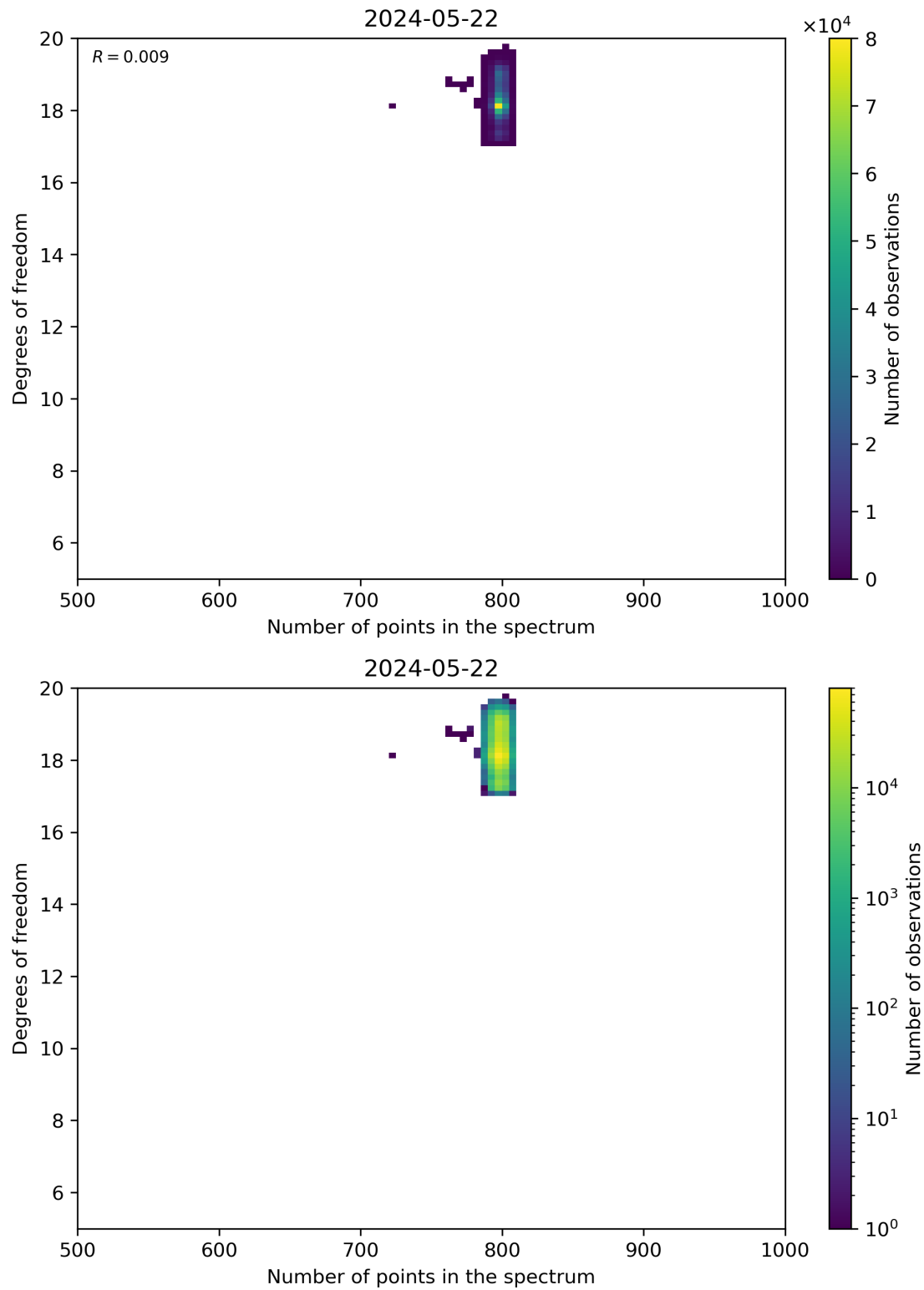
Figure 90: Scatter density plot of “Number of points in the spectrum” against “Degrees of freedom” for 2024-05-21 to 2024-05-23.
