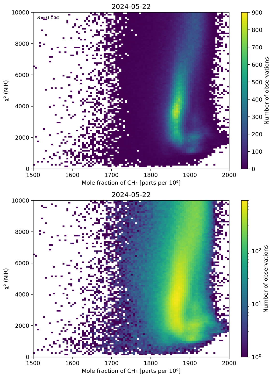
Figure 70: Scatter density plot of “Mole fraction of \text{CH}_4 ” against “ \chi^2 (NIR)” for 2024-05-21 to 2024-05-23.
