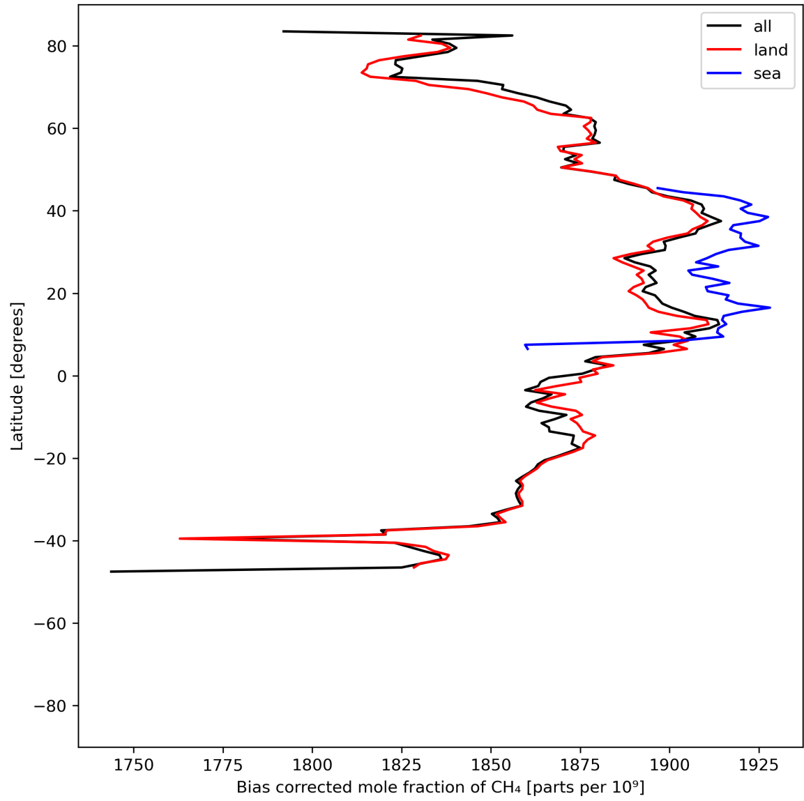
Figure 14: Zonal average of “Bias corrected mole fraction of CH 4 ” for 2024-05-21 to 2024-05-23.
