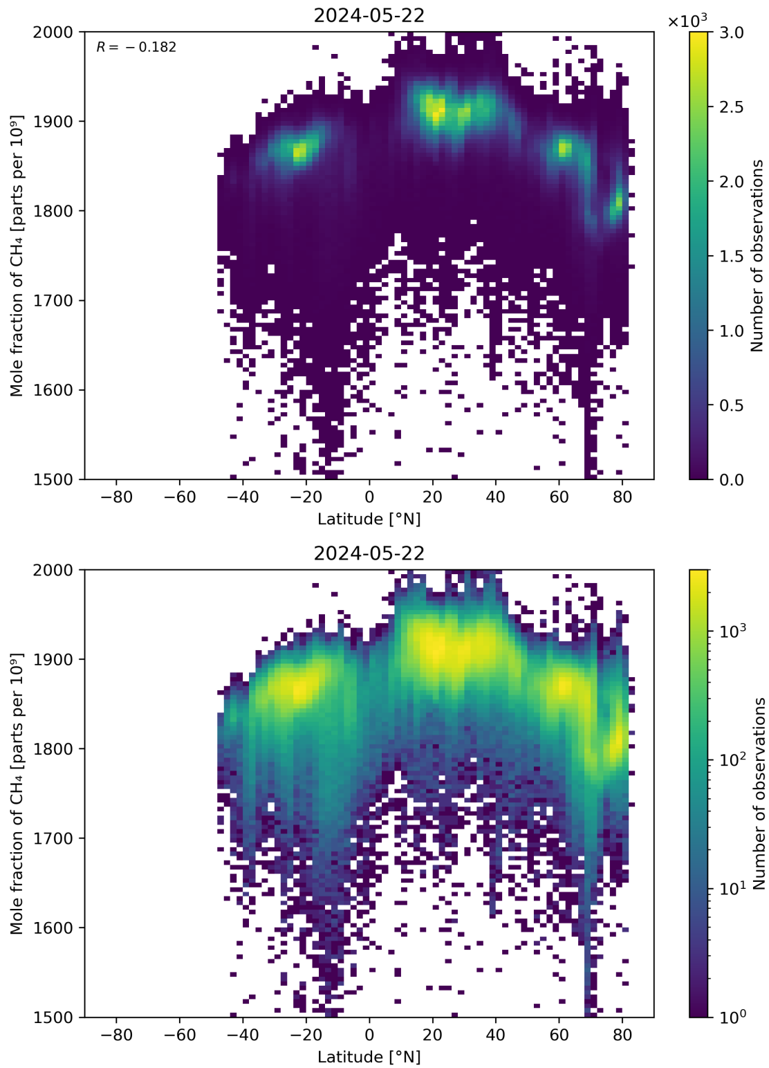
Figure 57: Scatter density plot of “Latitude” against “Mole fraction of CH 4 ” for 2024-05-21 to 2024-05-23.
