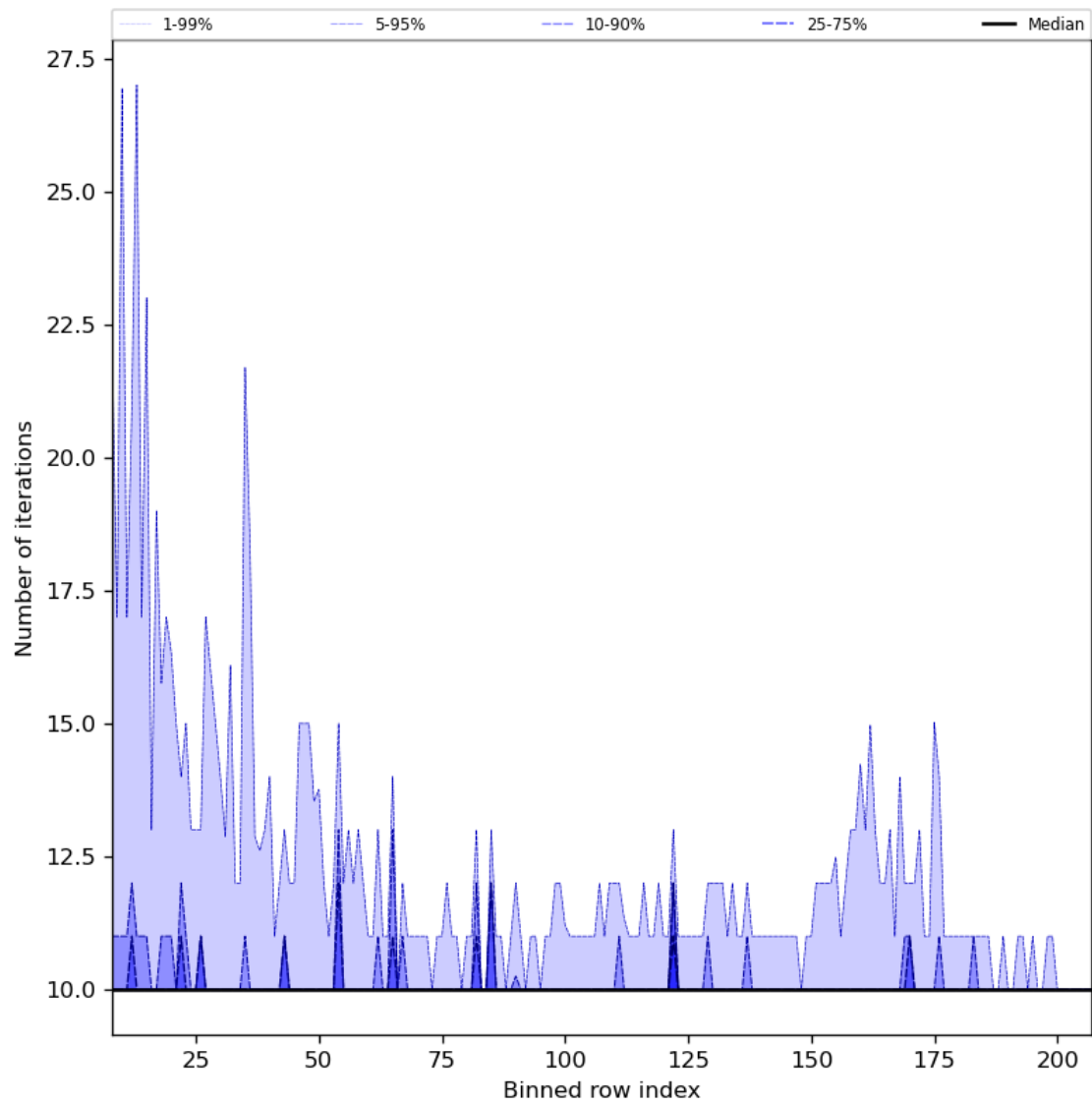
Figure 42: Along track statistics of “Number of iterations” for 2024-05-21 to 2024-05-23
