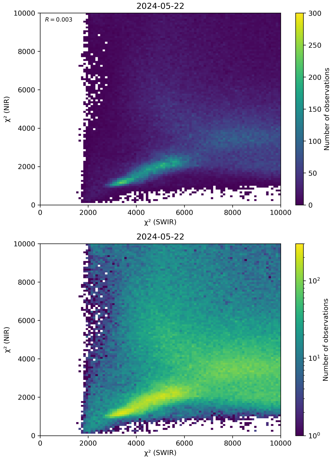
Figure 47: Scatter density plot of “ \chi^2 (SWIR)” against “ \chi^2 (NIR)” for 2024-05-21 to 2024-05-23.
