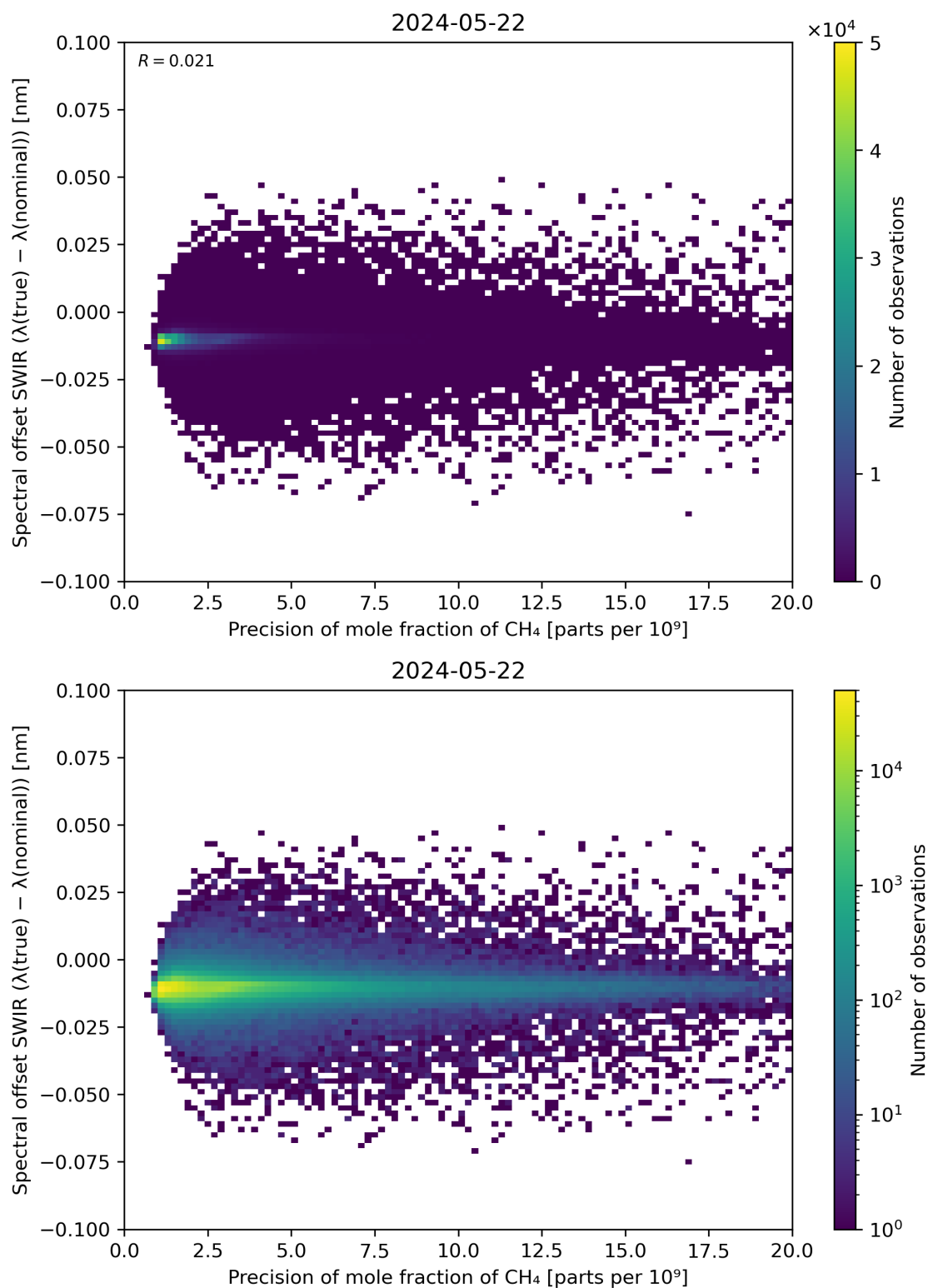
Figure 85: Scatter density plot of “Precision of mole fraction of CH 4 ” against “Spectral offset SWIR ( \lambda(\text{true}) - \lambda(\text{nominal}) )” for 2024-05-21 to 2024-05-23.
