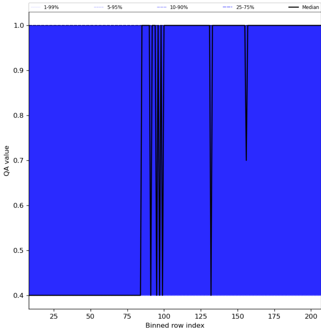
Figure 33: Along track statistics of “QA value” for 2024-05-21 to 2024-05-23
