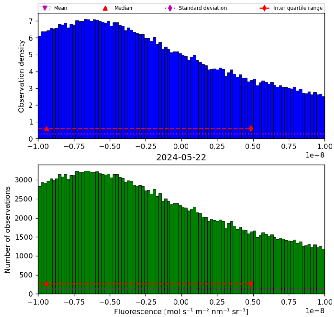
Figure 32: Histogram of “Fluorescence” for 2024-05-21 to 2024-05-23
