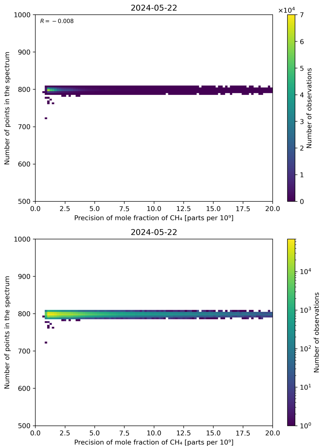
Figure 84: Scatter density plot of “Precision of mole fraction of CH 4 ” against “Number of points in the spectrum” for 2024-05-21 to 2024-05-23.
