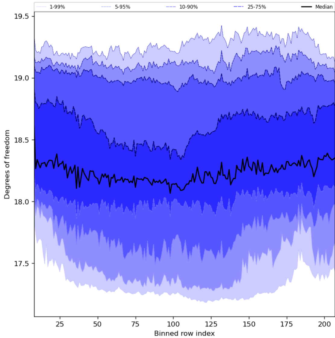
Figure 41: Along track statistics of “Degrees of freedom” for 2024-05-21 to 2024-05-23
