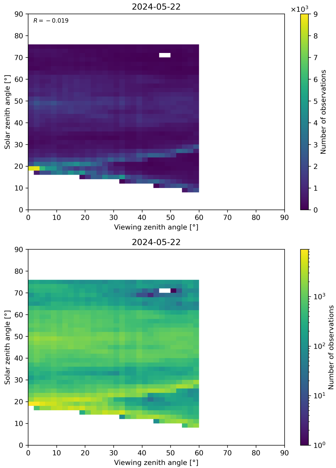
Figure 115: Scatter density plot of “Viewing zenith angle” against “Solar zenith angle” for 2024-05-21 to 2024-05-23.
