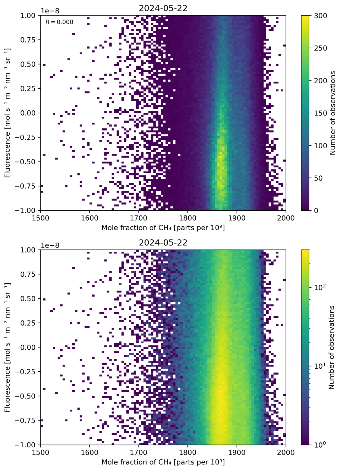
Figure 73: Scatter density plot of “Mole fraction of \text{CH}_4 ” against “Fluorescence” for 2024-05-21 to 2024-05-23.
