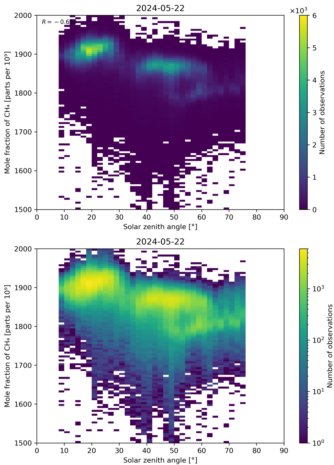
Figure 99: Scatter density plot of “Solar zenith angle” against “Mole fraction of CH 4 ” for 2024-05-21 to 2024-05-23.
