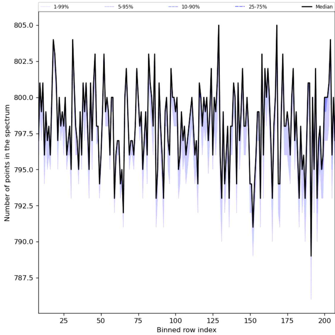
Figure 37: Along track statistics of “Number of points in the spectrum” for 2024-05-21 to 2024-05-23
