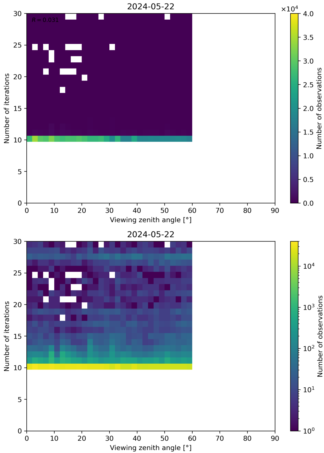
Figure 113: Scatter density plot of “Viewing zenith angle” against “Number of iterations” for 2024-05-21 to 2024-05-23.
