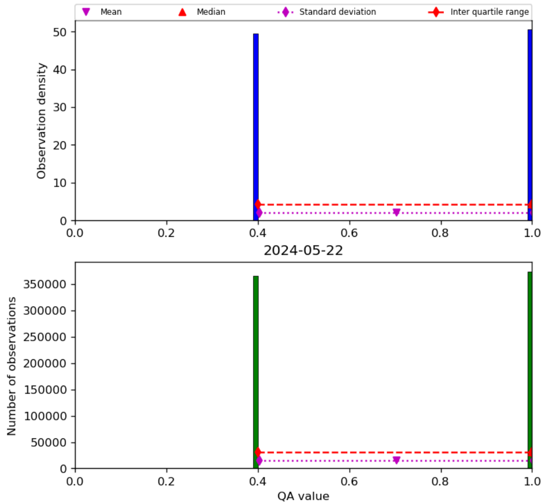
Figure 22: Histogram of "QA value" for 2024-05-21 to 2024-05-23
