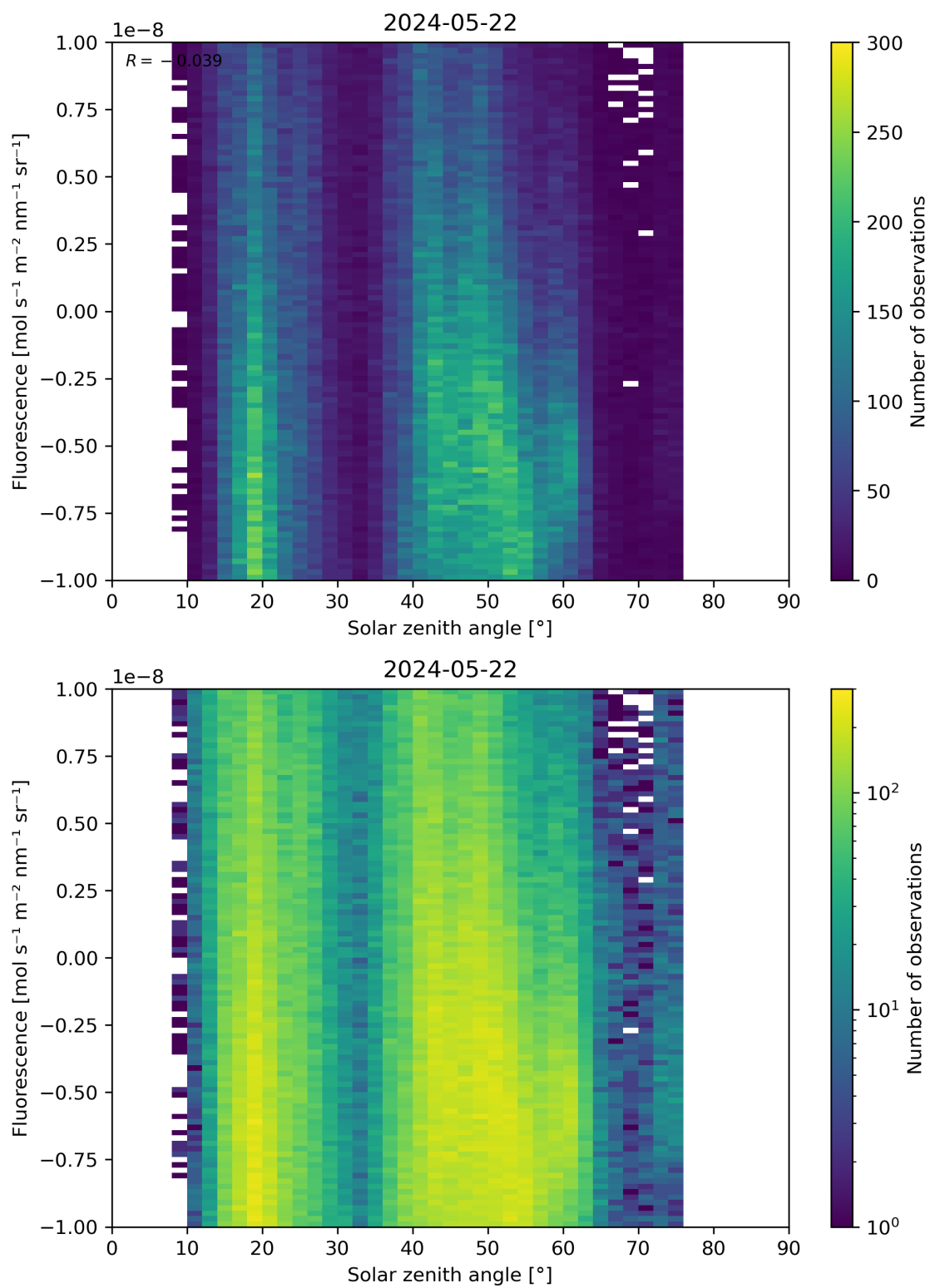
Figure 97: Scatter density plot of “Solar zenith angle” against “Fluorescence” for 2024-05-21 to 2024-05-23.
