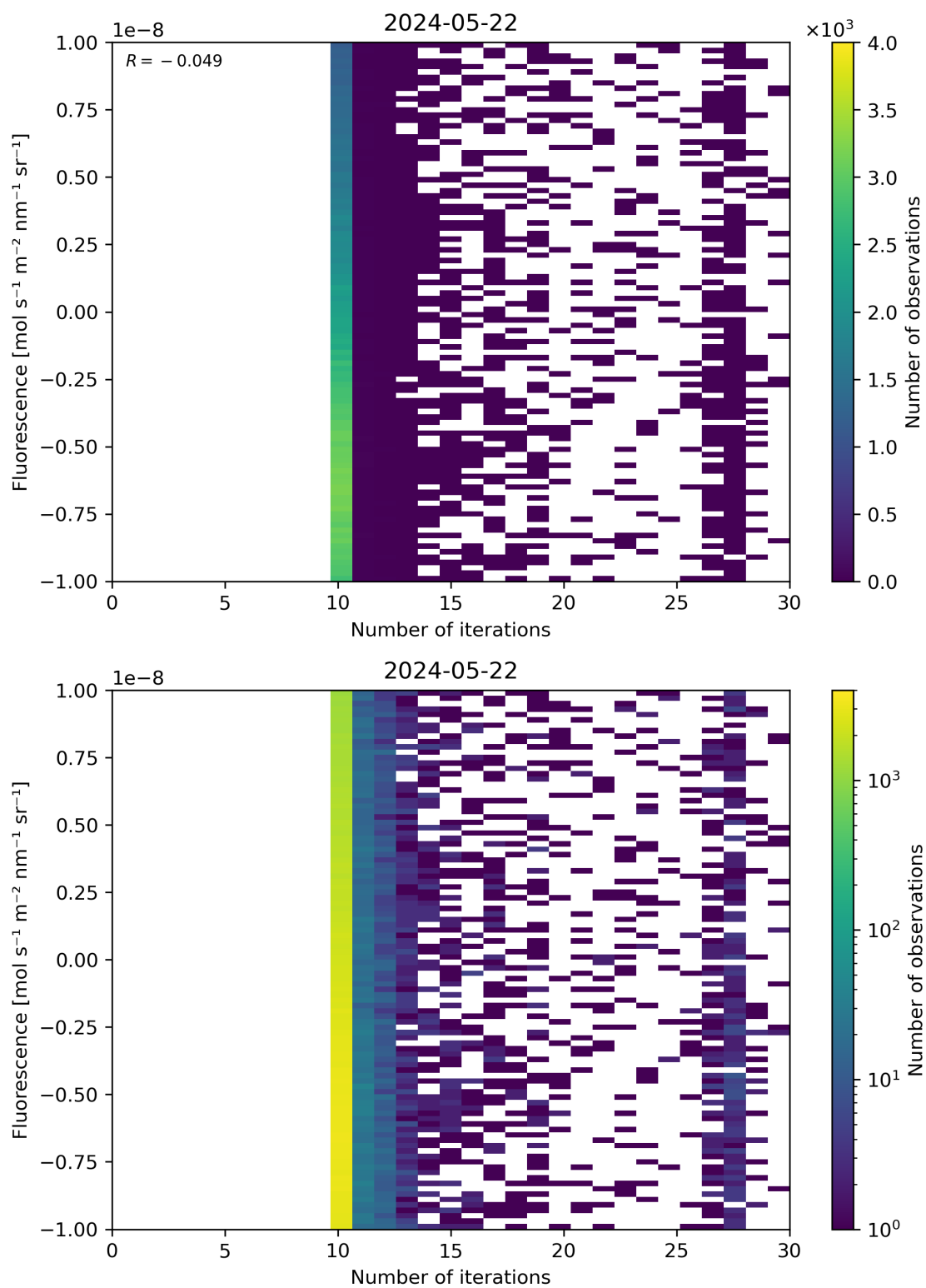
Figure 87: Scatter density plot of “Number of iterations” against “Fluorescence” for 2024-05-21 to 2024-05-23.
