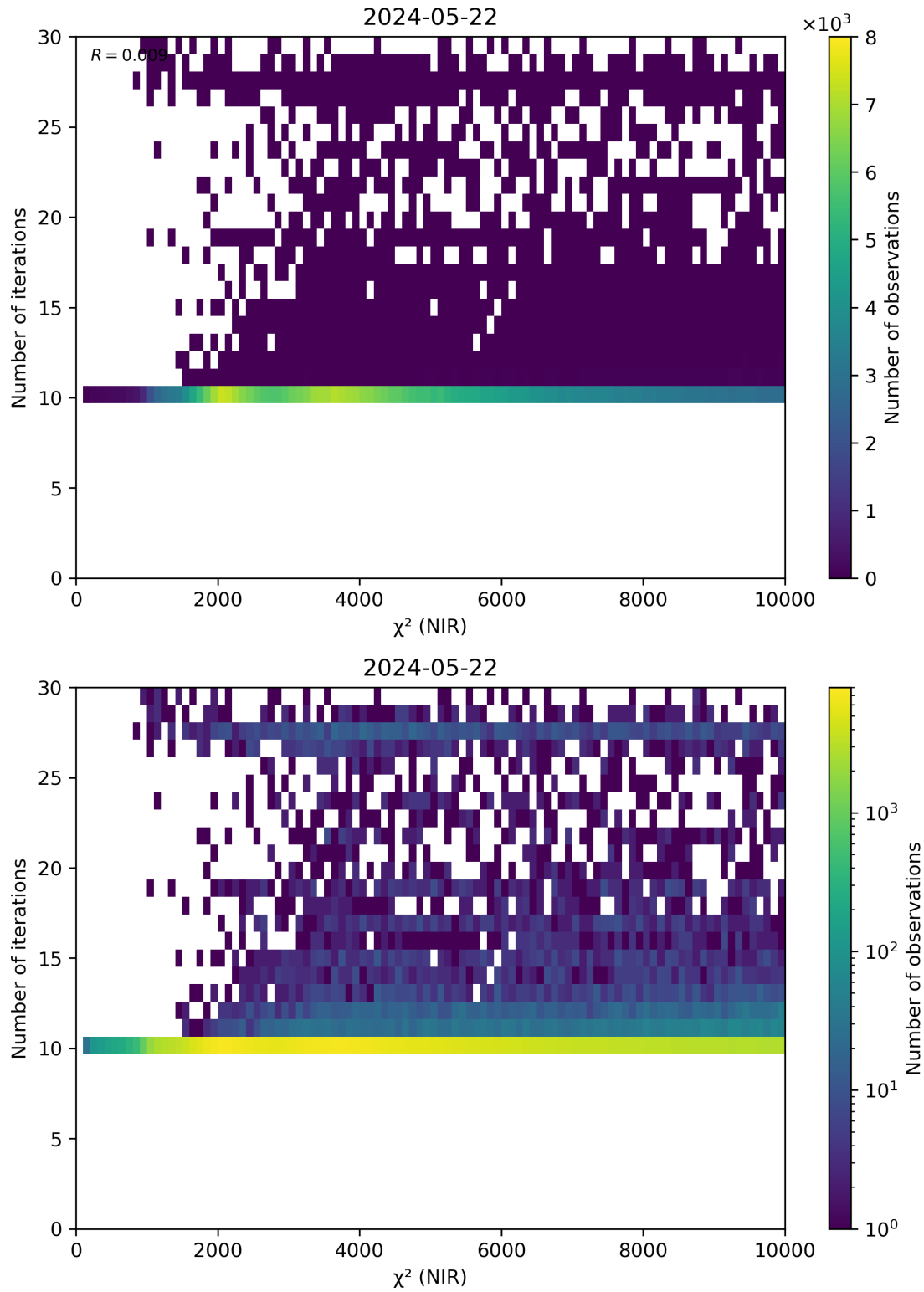
Figure 46: Scatter density plot of “ \chi^2 (NIR)” against “Number of iterations” for 2024-05-21 to 2024-05-23.
