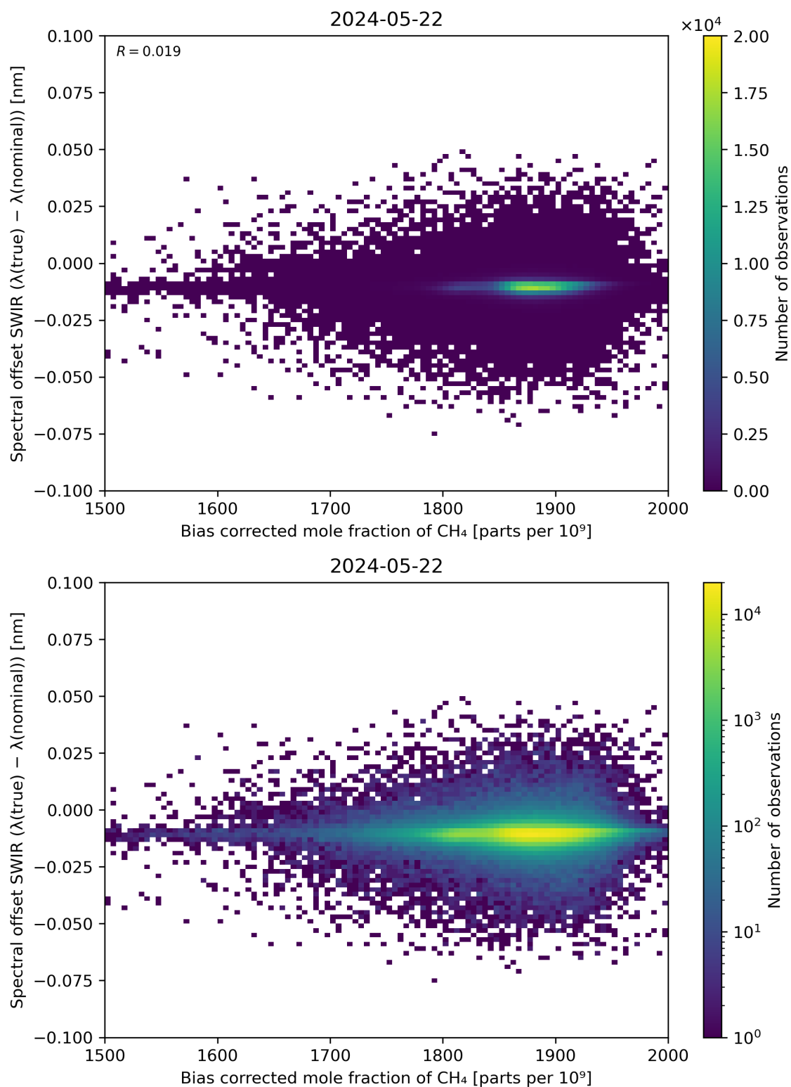
Figure 69: Scatter density plot of “Bias corrected mole fraction of \text{CH}_4 ” against “Spectral offset SWIR ( \lambda(\text{true}) - \lambda(\text{nominal}) )” for 2024-05-21 to 2024-05-23.
