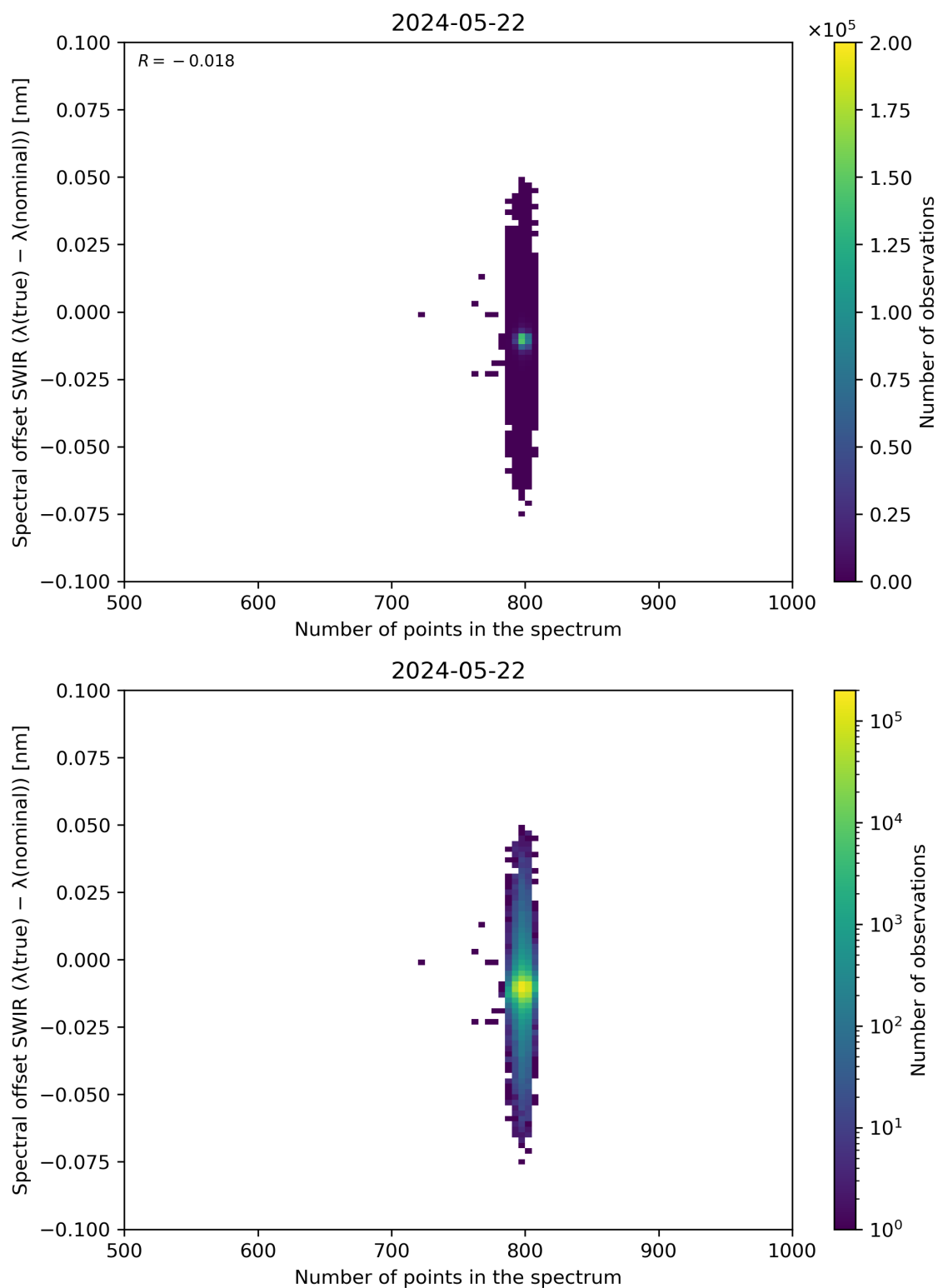
Figure 93: Scatter density plot of “Number of points in the spectrum” against “Spectral offset SWIR ( \lambda(\text{true}) - \lambda(\text{nominal}) )” for 2024-05-21 to 2024-05-23.
