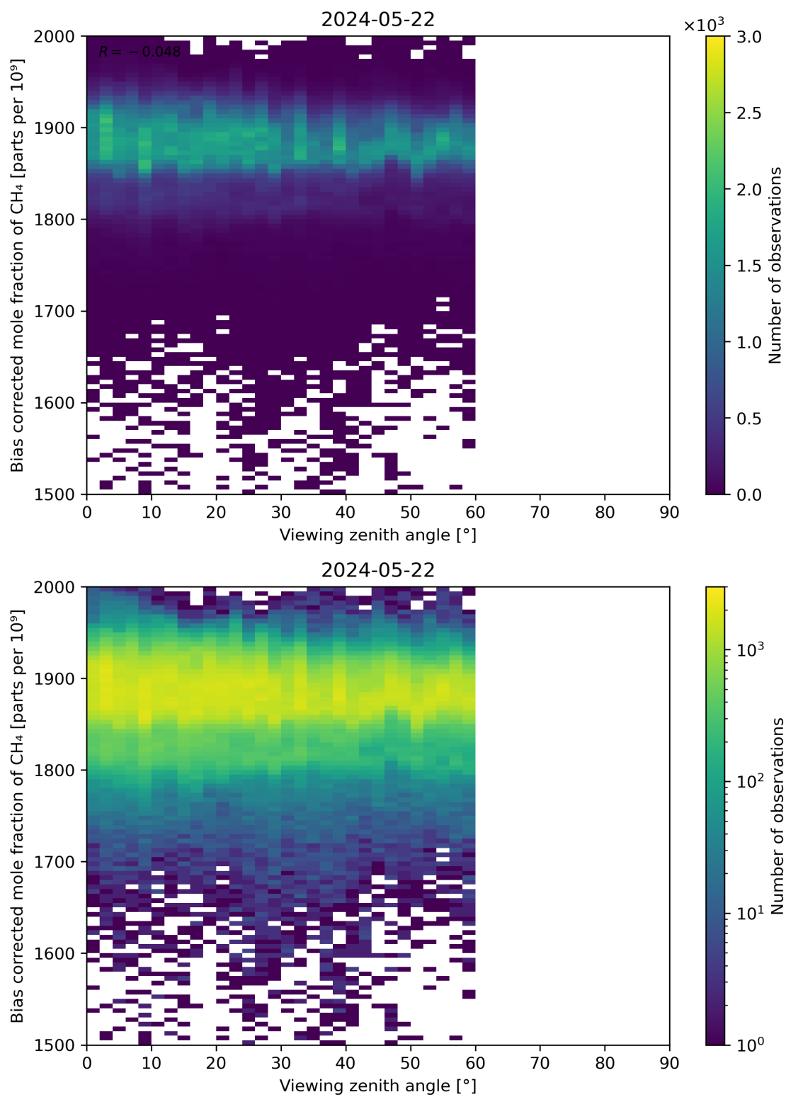
Figure 111: Scatter density plot of “Viewing zenith angle” against “Bias corrected mole fraction of CH 4 ” for 2024-05-21 to 2024-05-23.
