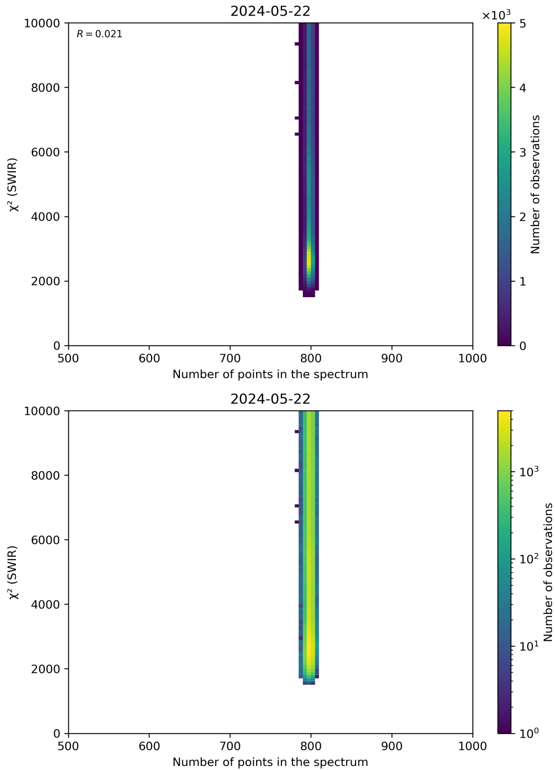
Figure 89: Scatter density plot of “Number of points in the spectrum” against “ \chi^2 (SWIR)” for 2024-05-21 to 2024-05-23.
