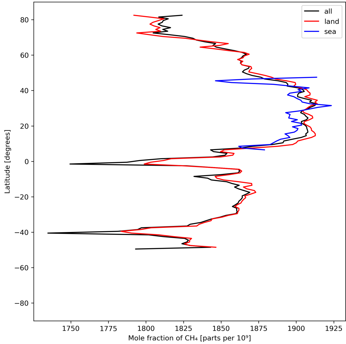
Figure 12: Zonal average of “Mole fraction of \text{CH}_4 ” for 2024-05-23 to 2024-05-24.
