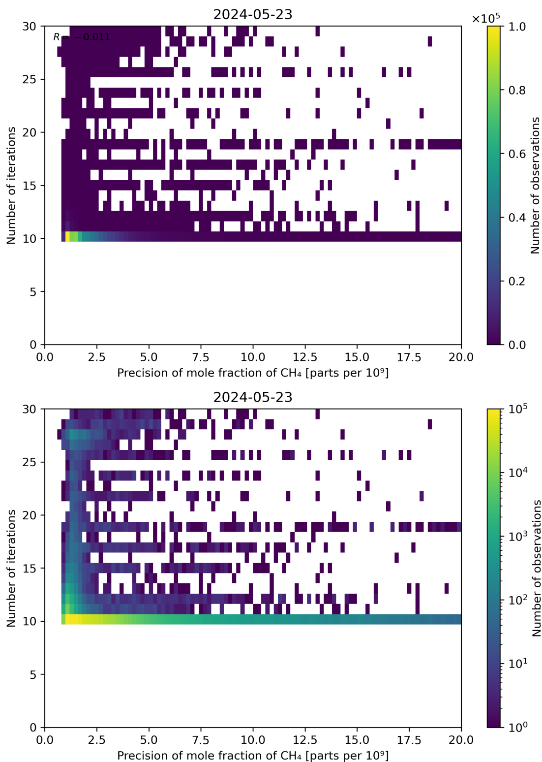
Figure 83: Scatter density plot of “Precision of mole fraction of CH 4 ” against “Number of iterations” for 2024-05-23 to 2024-05-24.
