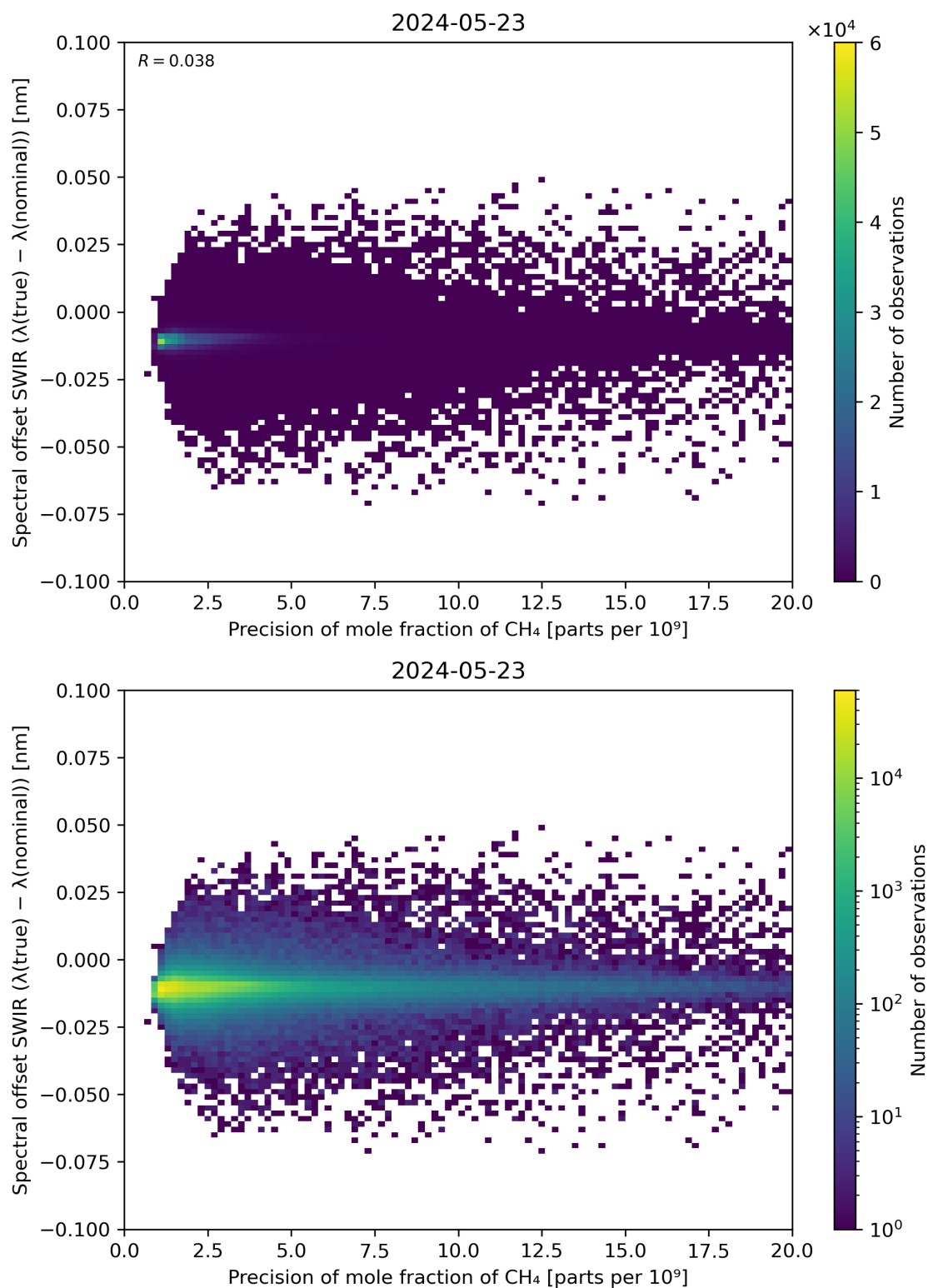
Figure 85: Scatter density plot of “Precision of mole fraction of \text{CH}_4 ” against “Spectral offset SWIR ( \lambda(\text{true}) - \lambda(\text{nominal}) )” for 2024-05-23 to 2024-05-24.
