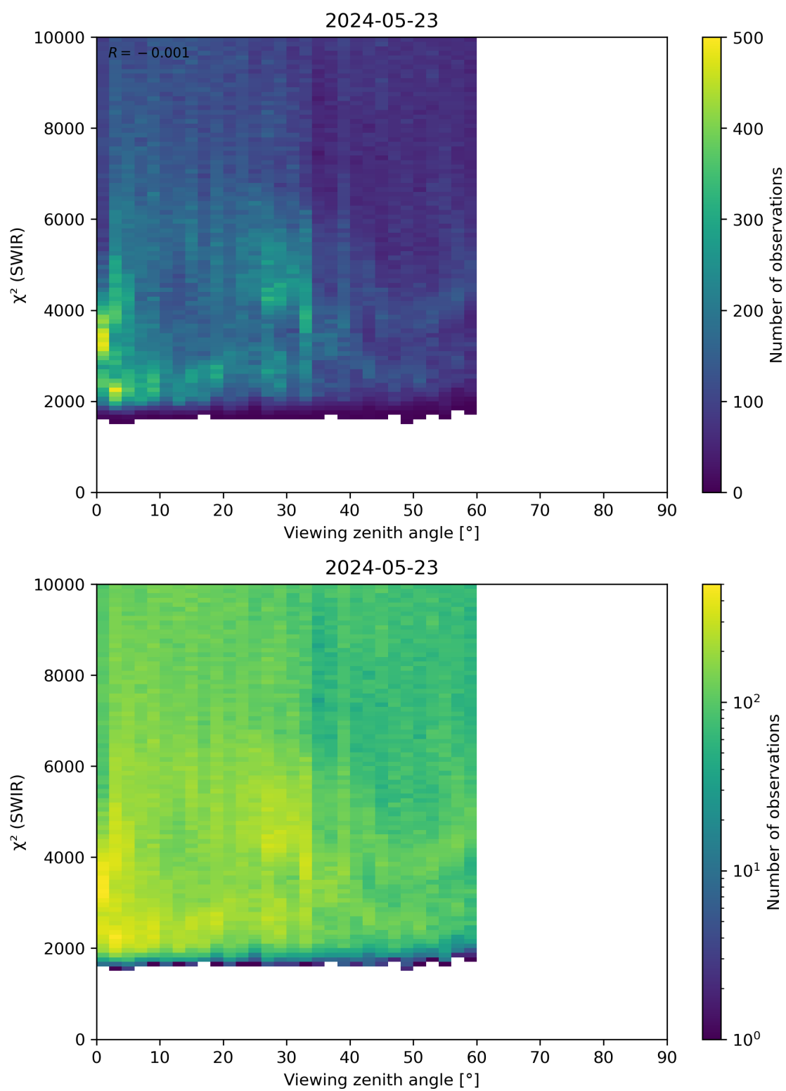
Figure 106: Scatter density plot of “Viewing zenith angle” against “ \chi^2 (SWIR)” for 2024-05-23 to 2024-05-24.
