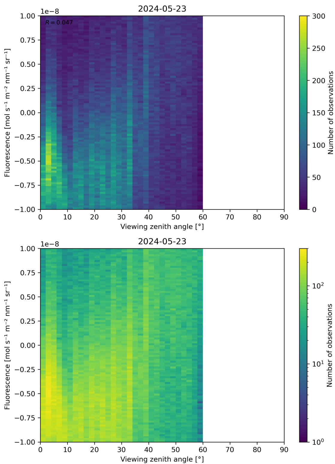
Figure 108: Scatter density plot of “Viewing zenith angle” against “Fluorescence” for 2024-05-23 to 2024-05-24.
