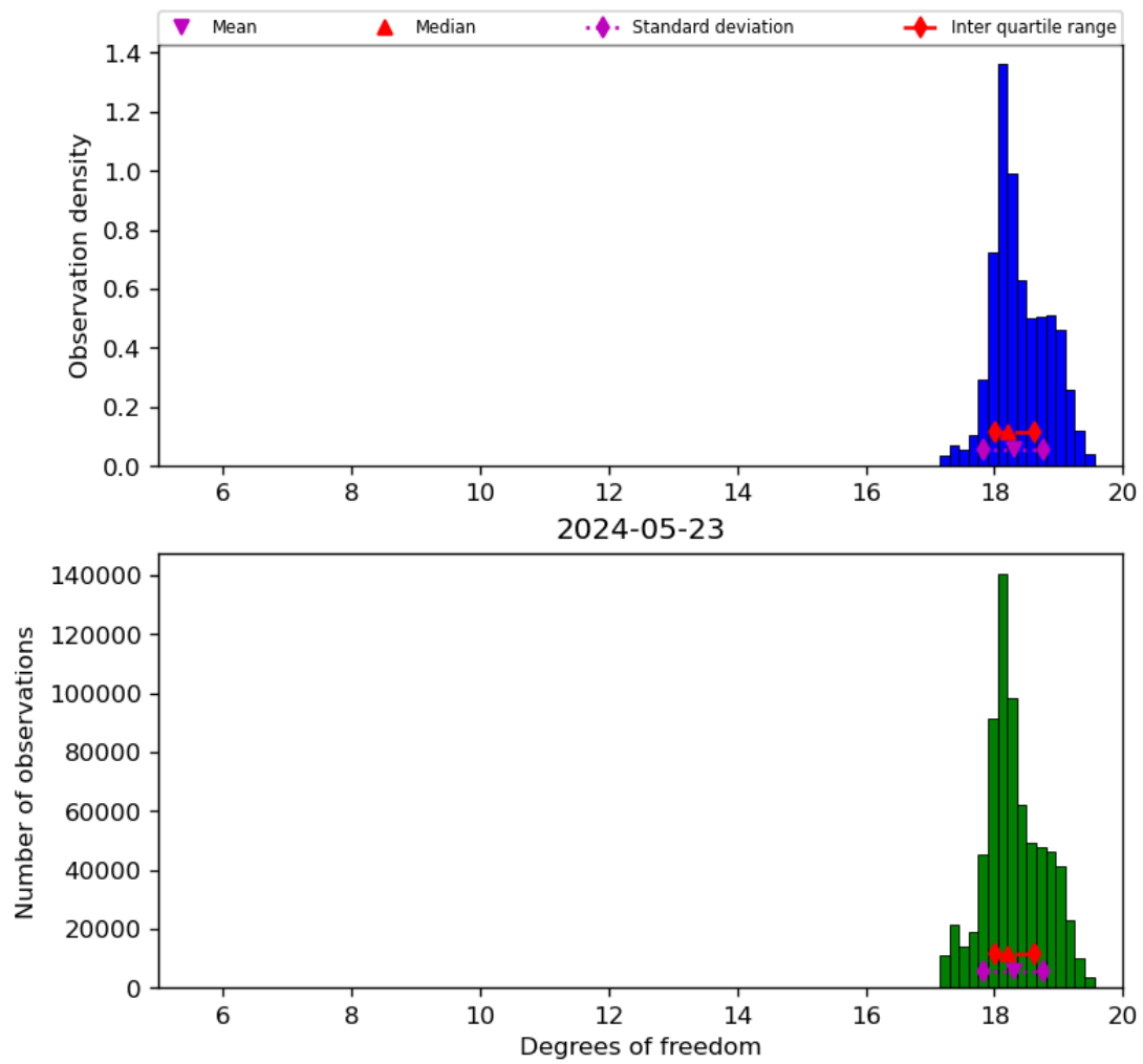
Figure 30: Histogram of “Degrees of freedom” for 2024-05-23 to 2024-05-24
