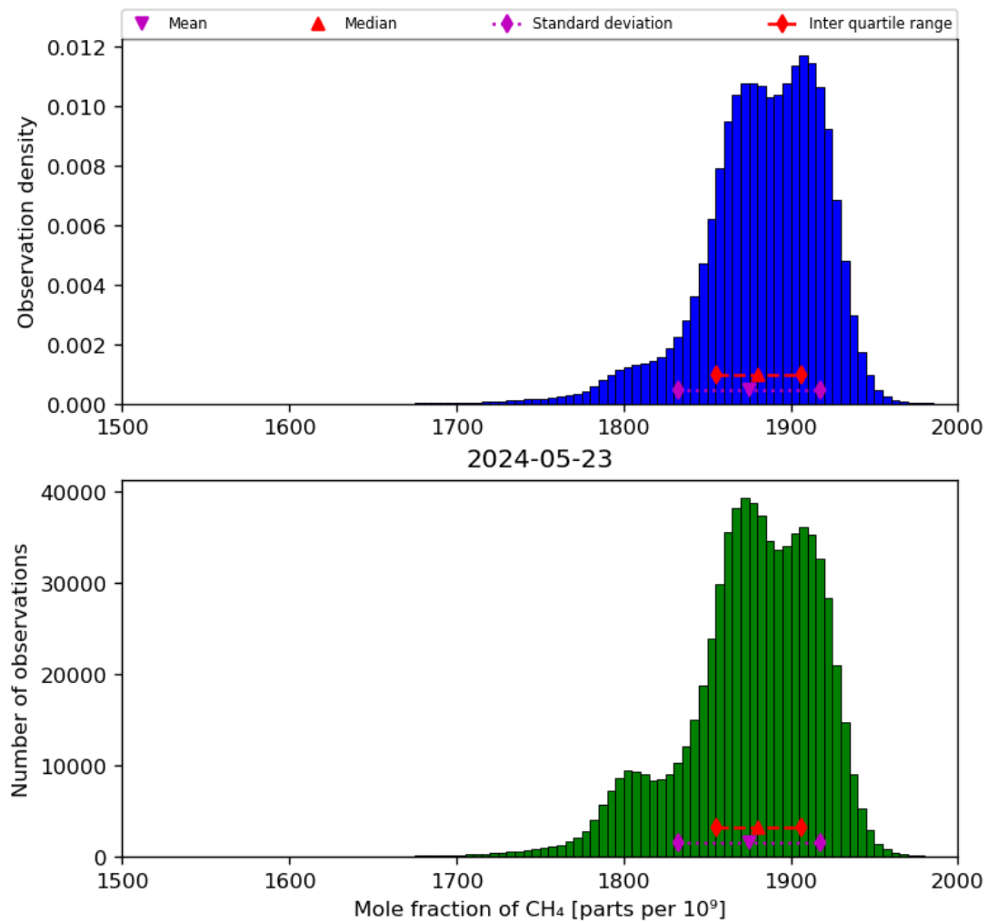
Figure 23: Histogram of “Mole fraction of CH 4 ” for 2024-05-23 to 2024-05-24
