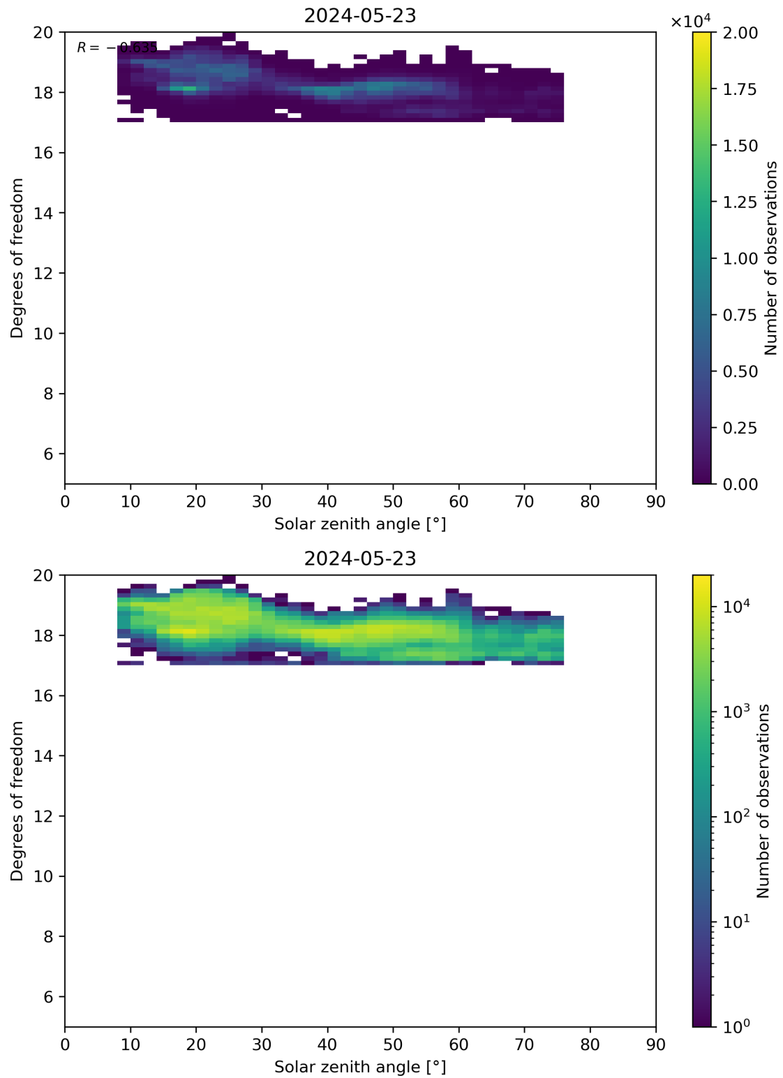
Figure 96: Scatter density plot of “Solar zenith angle” against “Degrees of freedom” for 2024-05-23 to 2024-05-24.
