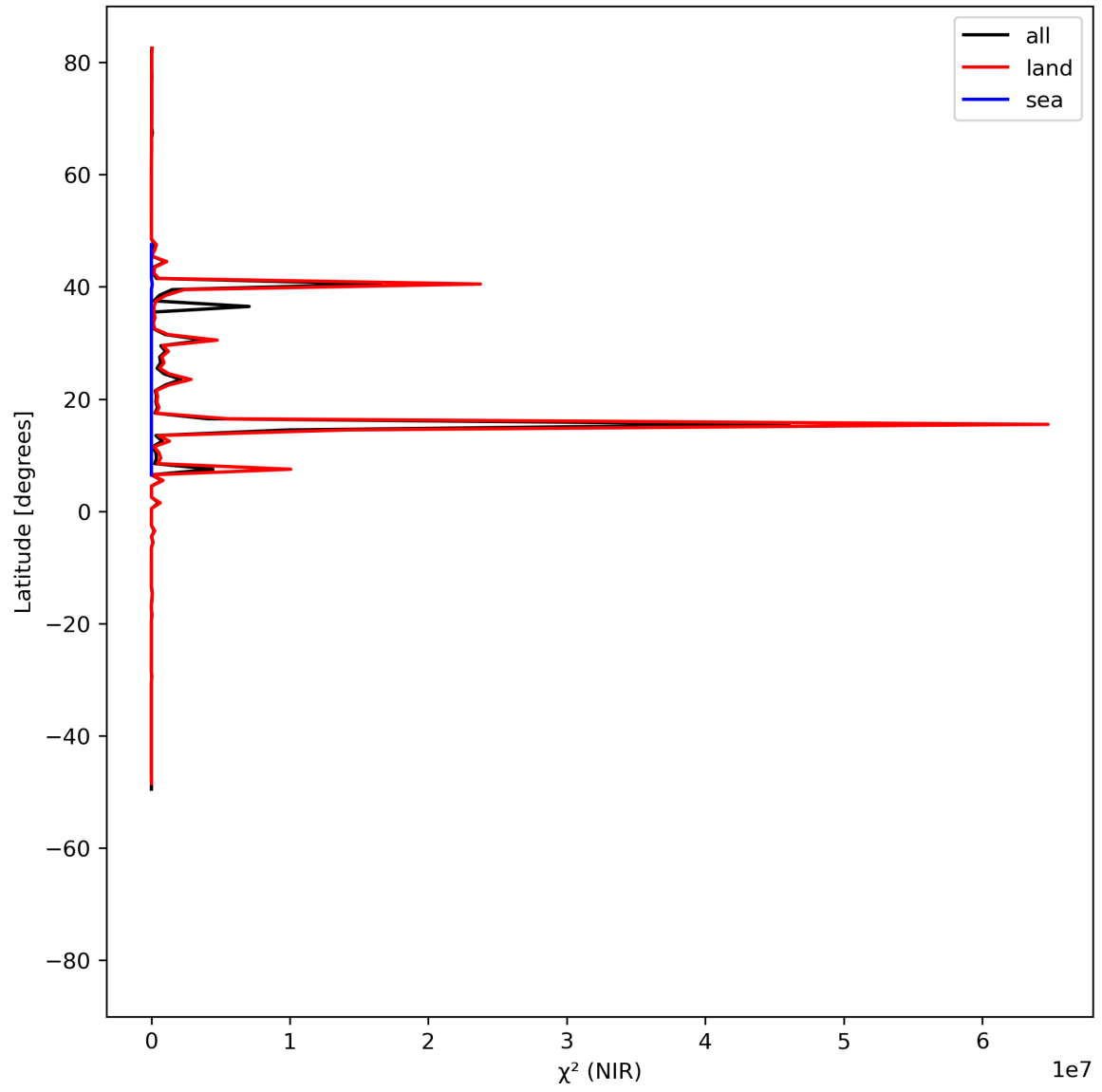
Figure 18: Zonal average of “ \chi^2 (NIR)” for 2024-05-23 to 2024-05-24.
