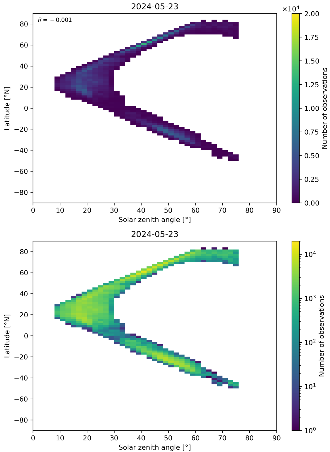
Figure 98: Scatter density plot of “Solar zenith angle” against “Latitude” for 2024-05-23 to 2024-05-24.
