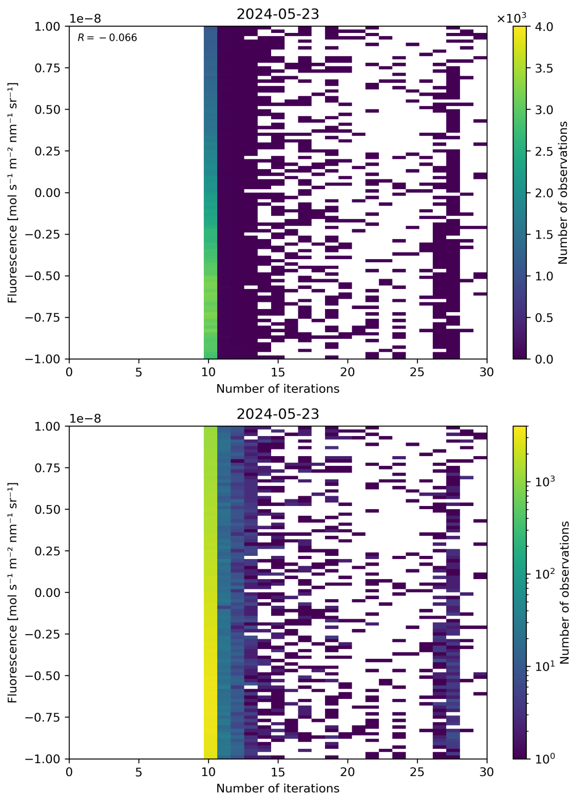
Figure 87: Scatter density plot of “Number of iterations” against “Fluorescence” for 2024-05-23 to 2024-05-24.
