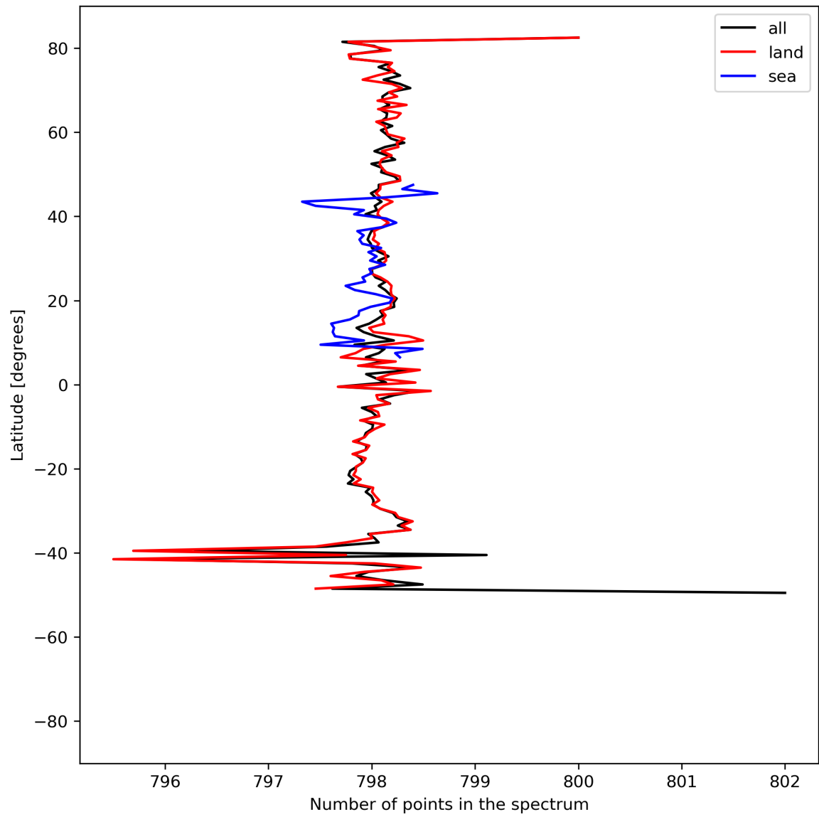
Figure 15: Zonal average of “Number of points in the spectrum” for 2024-05-23 to 2024-05-24.
