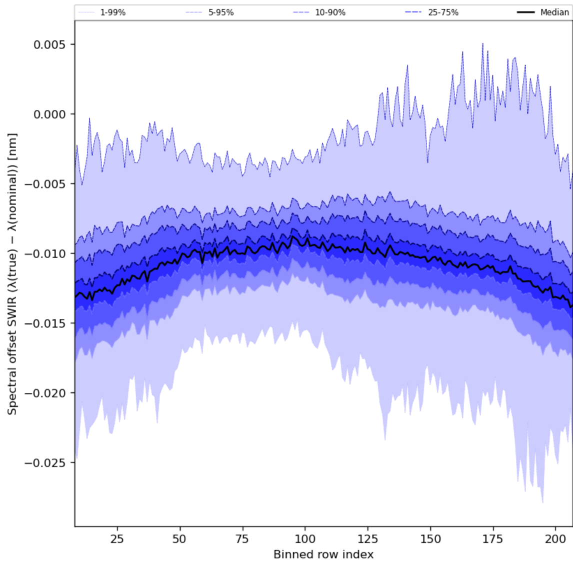
Figure 38: Along track statistics of “Spectral offset SWIR ( \lambda(\text{true}) - \lambda(\text{nominal}) )” for 2024-05-23 to 2024-05-24
