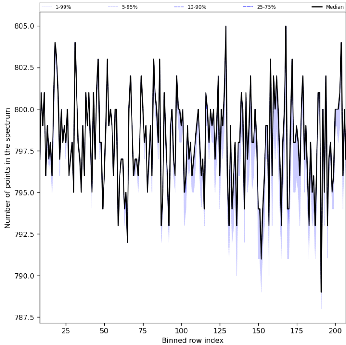
Figure 37: Along track statistics of “Number of points in the spectrum” for 2024-05-23 to 2024-05-24
