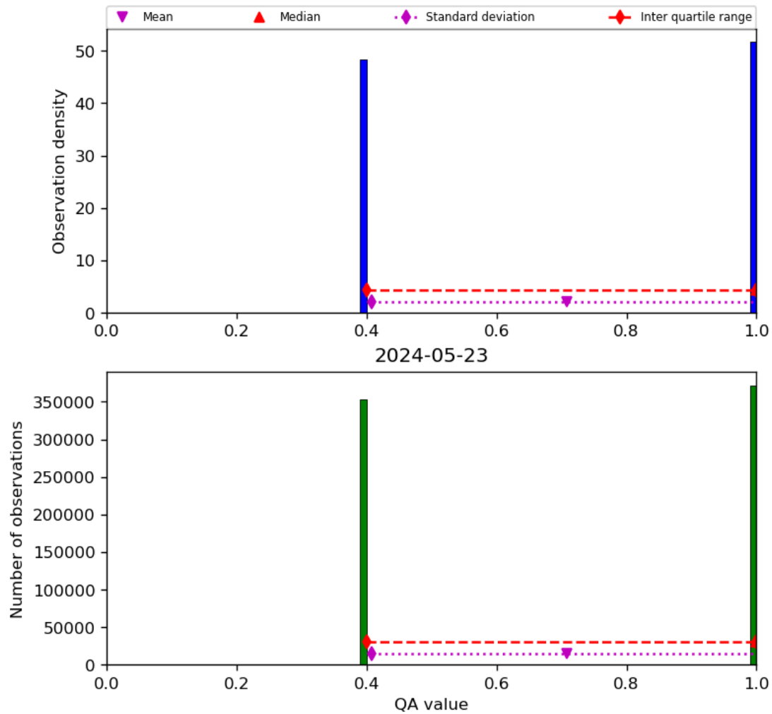
Figure 22: Histogram of “QA value” for 2024-05-23 to 2024-05-24
