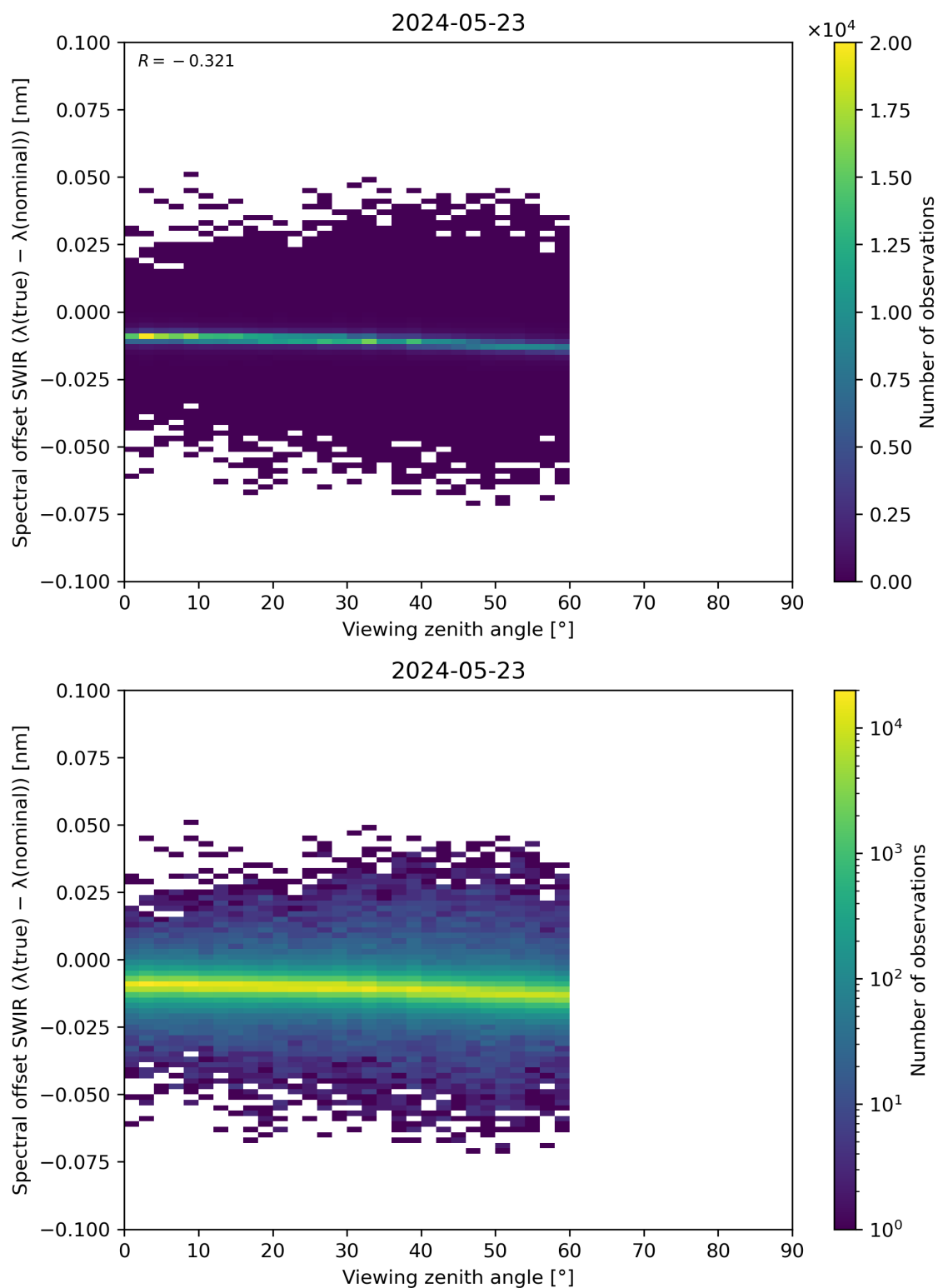
Figure 116: Scatter density plot of “Viewing zenith angle” against “Spectral offset SWIR ( \lambda(\text{true}) - \lambda(\text{nominal}) )” for 2024-05-23 to 2024-05-24.
