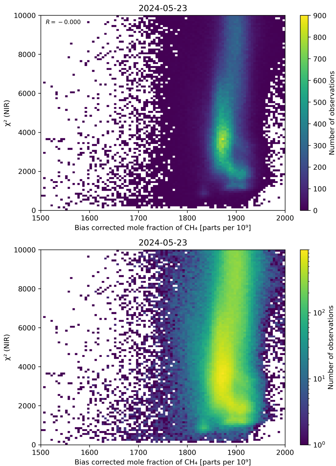
Figure 63: Scatter density plot of “Bias corrected mole fraction of CH 4 ” against “ \chi^2 (NIR)” for 2024-05-23 to 2024-05-24.
