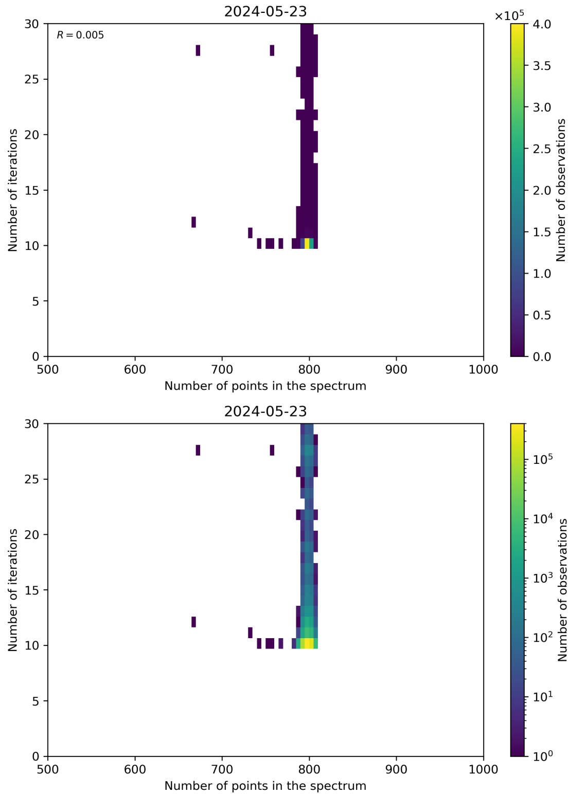
Figure 92: Scatter density plot of “Number of points in the spectrum” against “Number of iterations” for 2024-05-23 to 2024-05-24.
