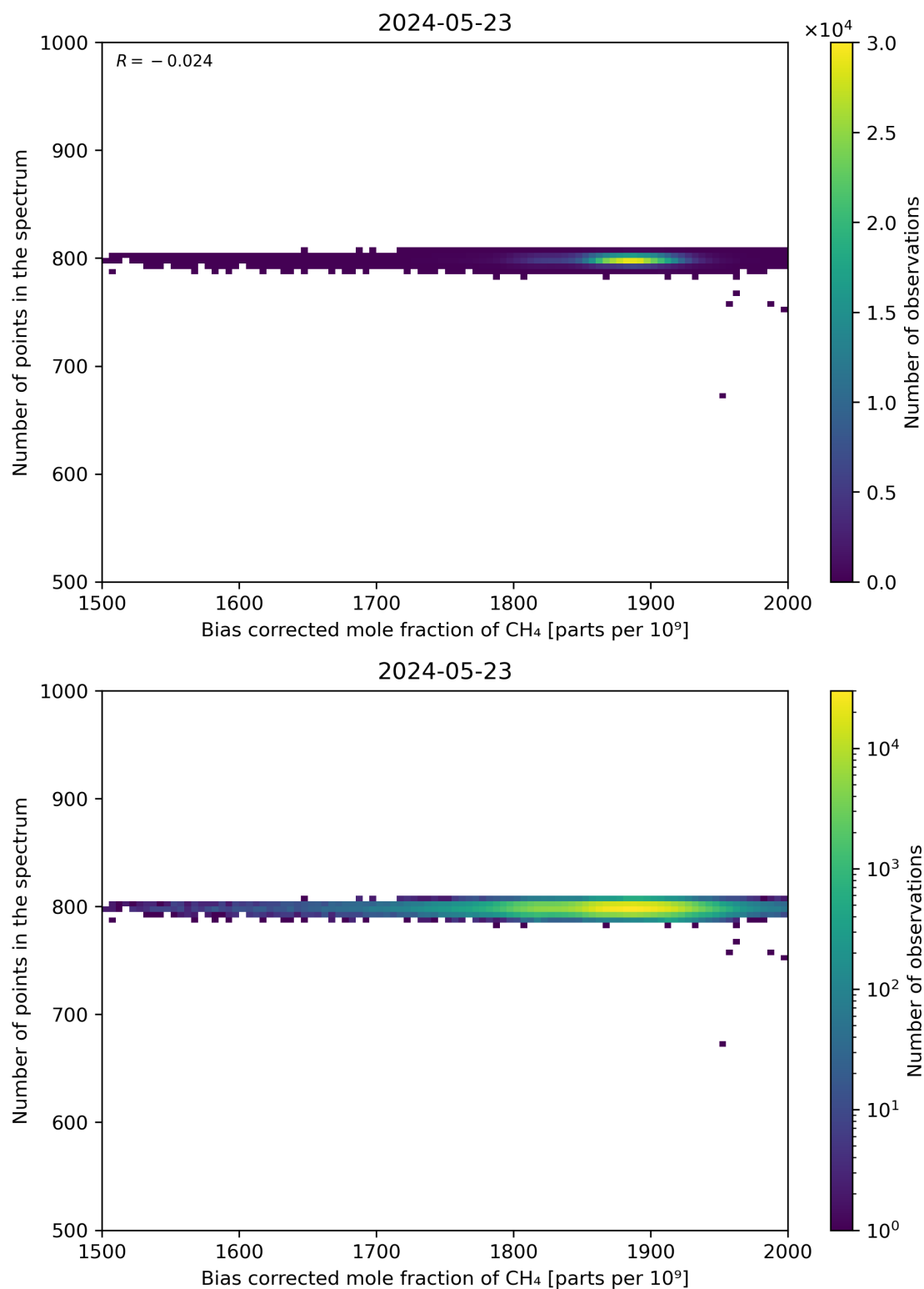
Figure 68: Scatter density plot of “Bias corrected mole fraction of CH 4 ” against “Number of points in the spectrum” for 2024-05-23 to 2024-05-24.
