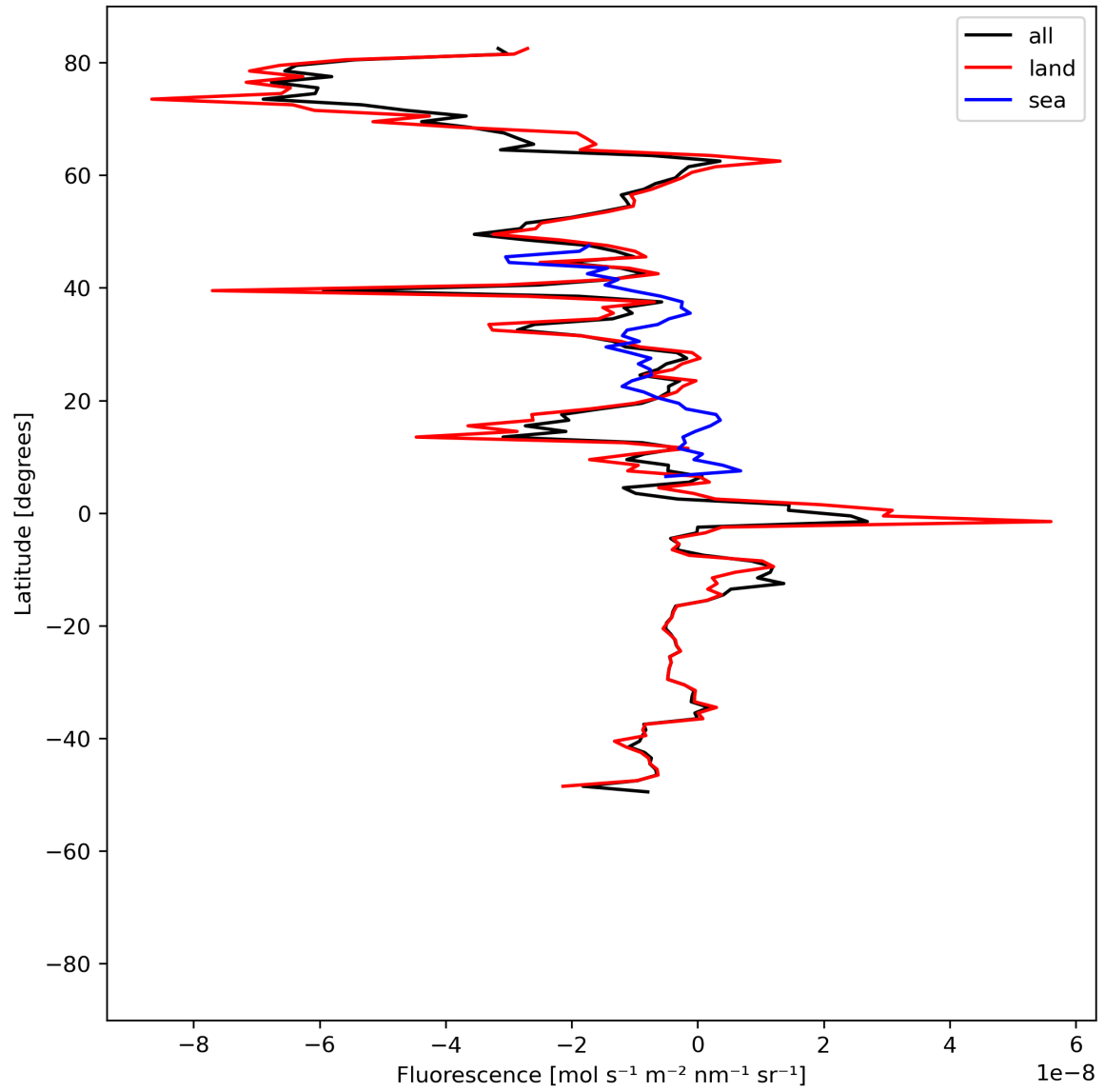
Figure 21: Zonal average of “Fluorescence” for 2024-05-23 to 2024-05-24.
