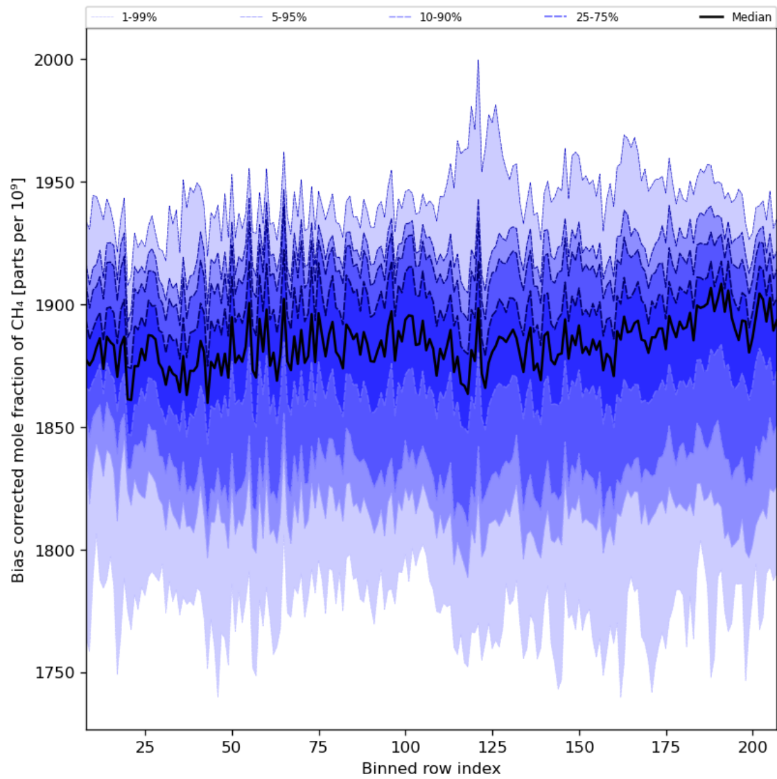
Figure 36: Along track statistics of “Bias corrected mole fraction of CH 4 ” for 2024-05-23 to 2024-05-24
