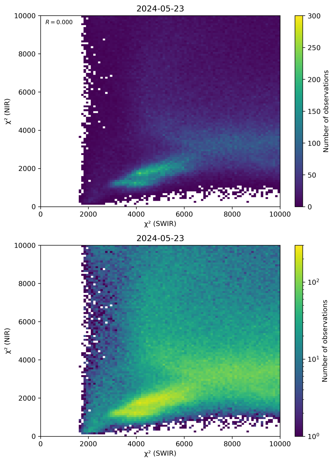
Figure 47: Scatter density plot of “ \chi^2 (SWIR)” against “ \chi^2 (NIR)” for 2024-05-23 to 2024-05-24.
