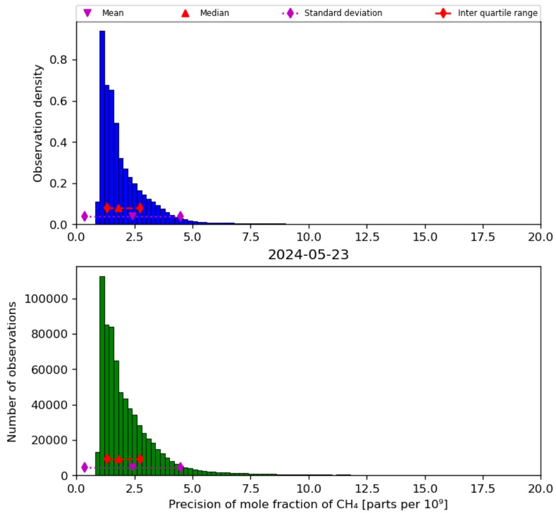
Figure 24: Histogram of “Precision of mole fraction of CH 4 ” for 2024-05-23 to 2024-05-24
