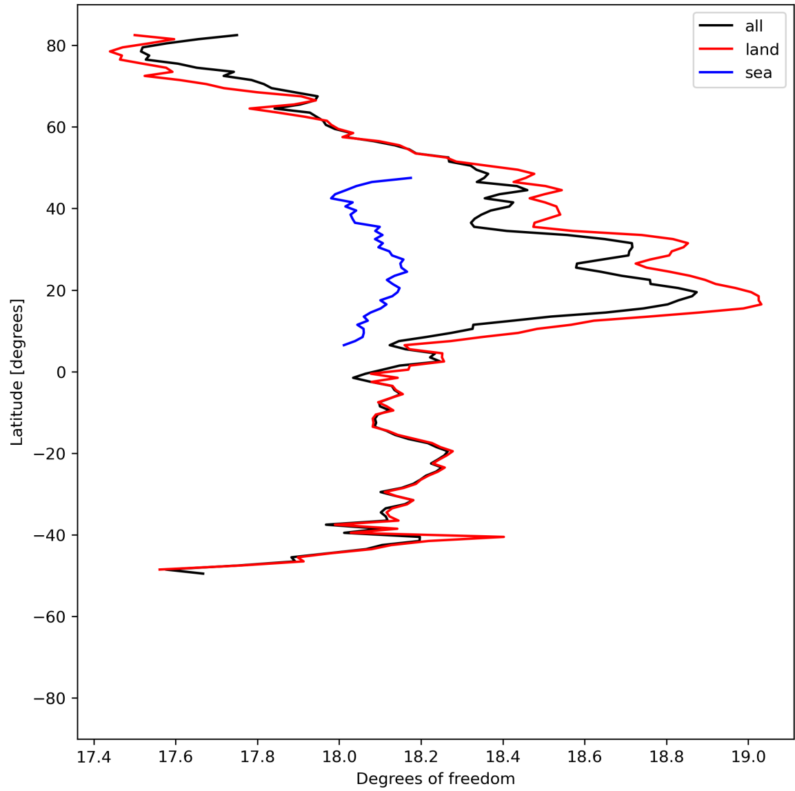
Figure 19: Zonal average of “Degrees of freedom” for 2024-05-23 to 2024-05-24.
