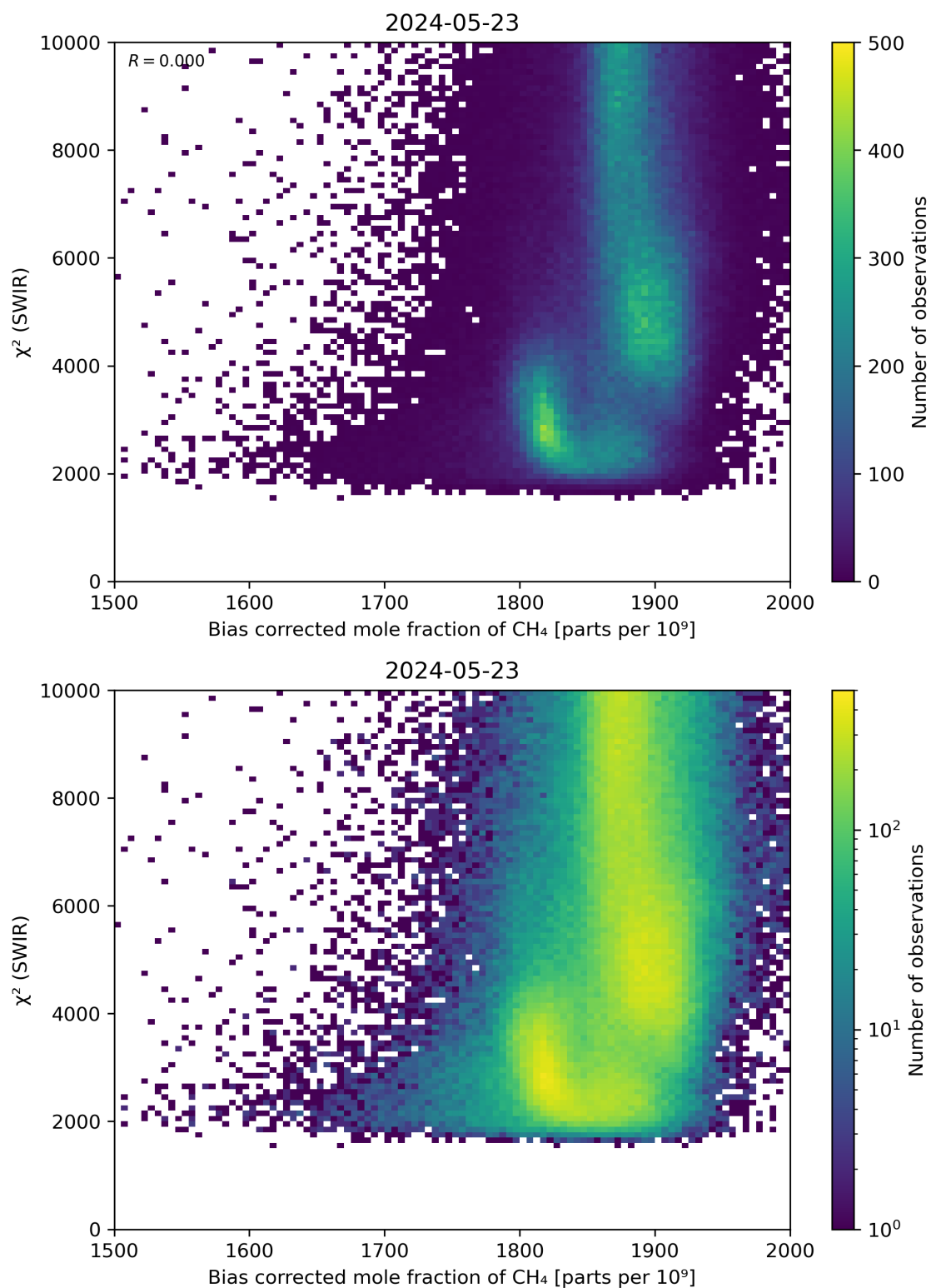
Figure 64: Scatter density plot of “Bias corrected mole fraction of CH 4 ” against “ \chi^2 (SWIR)” for 2024-05-23 to 2024-05-24.
