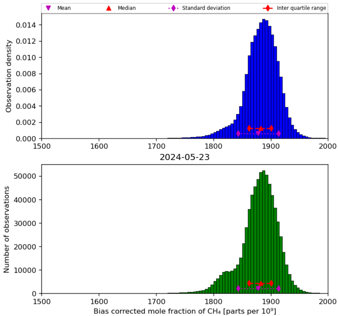
Figure 25: Histogram of “Bias corrected mole fraction of CH 4 ” for 2024-05-23 to 2024-05-24
