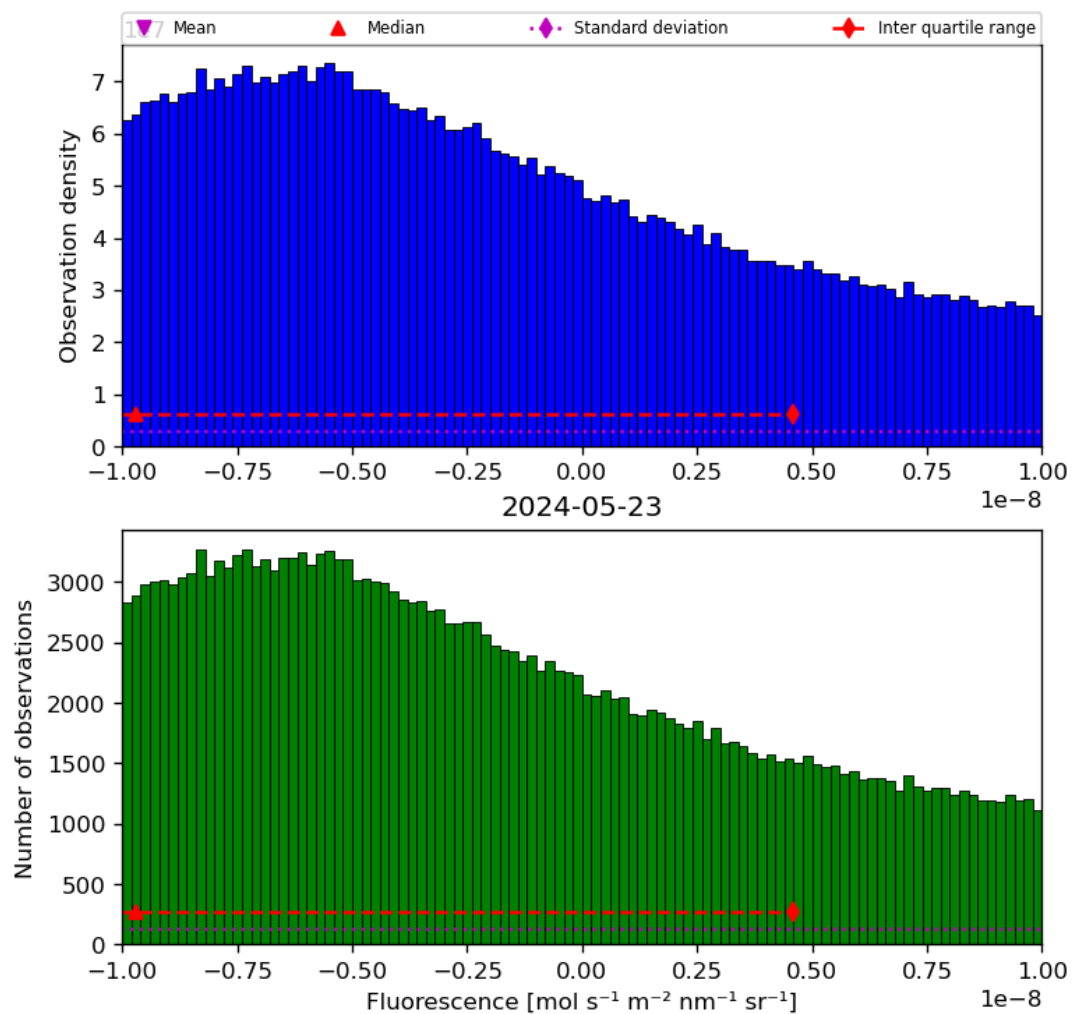
Figure 32: Histogram of “Fluorescence” for 2024-05-23 to 2024-05-24
