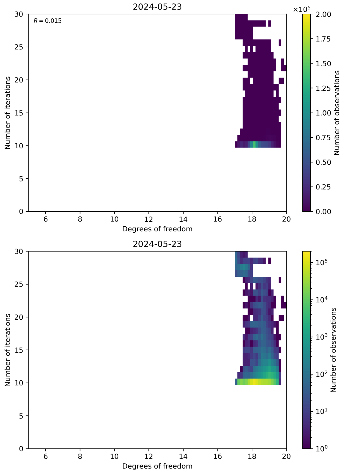
Figure 52: Scatter density plot of “Degrees of freedom” against “Number of iterations” for 2024-05-23 to 2024-05-24.
