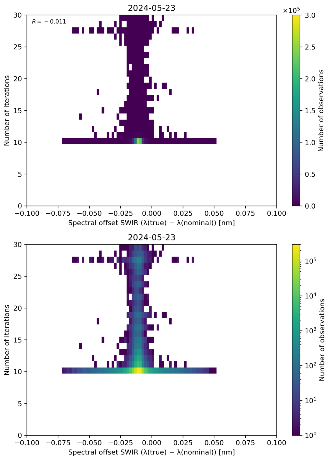
Figure 121: Scatter density plot of “Spectral offset SWIR ( \lambda(\text{true}) - \lambda(\text{nominal}) )” against “Number of iterations” for 2024-05-23 to 2024-05-24.
