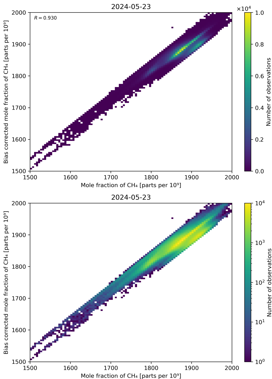
Figure 74: Scatter density plot of “Mole fraction of CH 4 ” against “Bias corrected mole fraction of CH 4 ” for 2024-05-23 to 2024-05-24.
