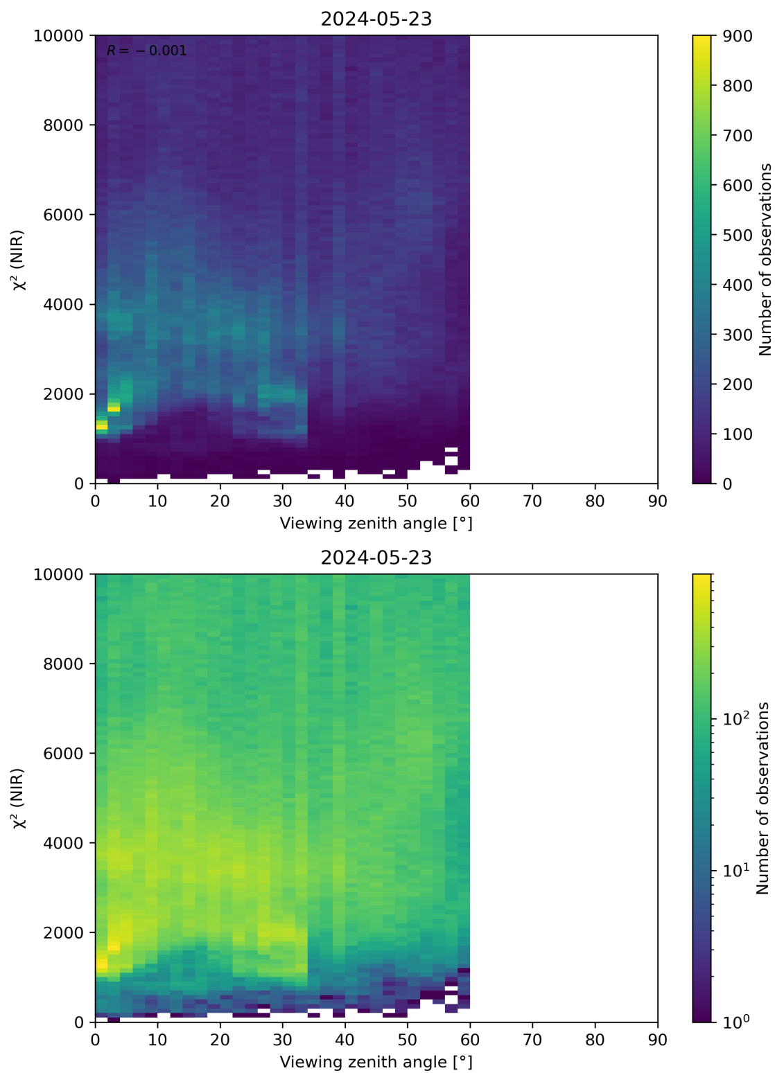
Figure 105: Scatter density plot of “Viewing zenith angle” against “ \chi^2 (NIR)” for 2024-05-23 to 2024-05-24.
