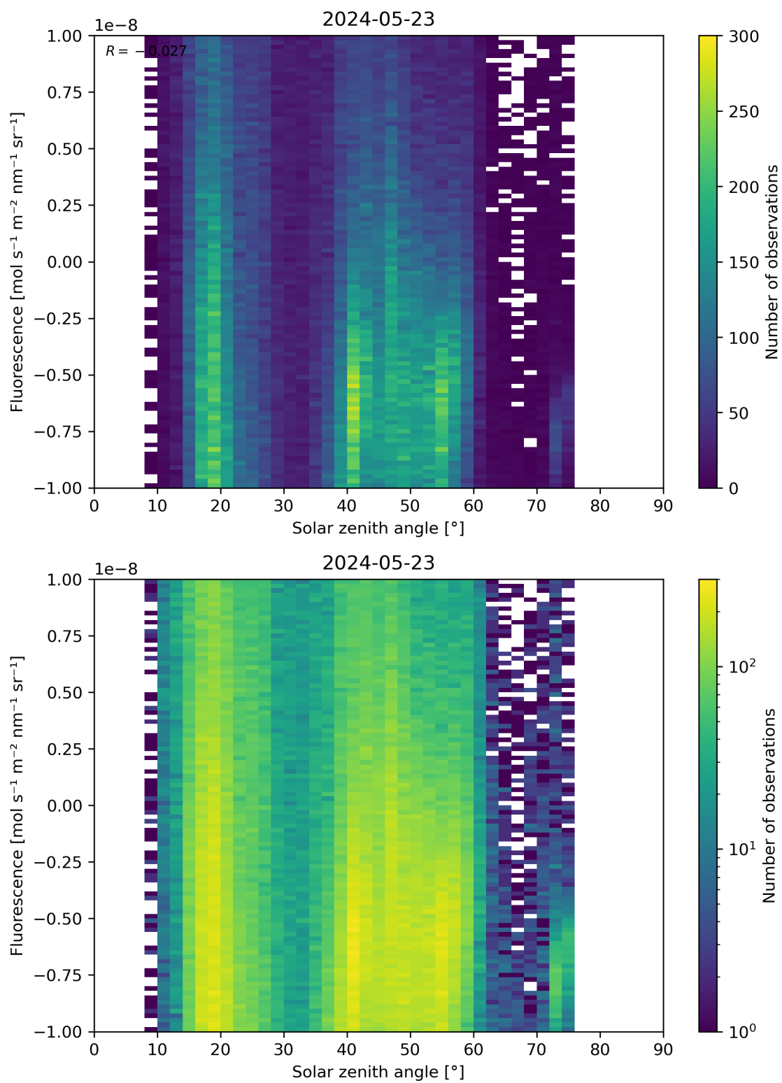
Figure 97: Scatter density plot of “Solar zenith angle” against “Fluorescence” for 2024-05-23 to 2024-05-24.
