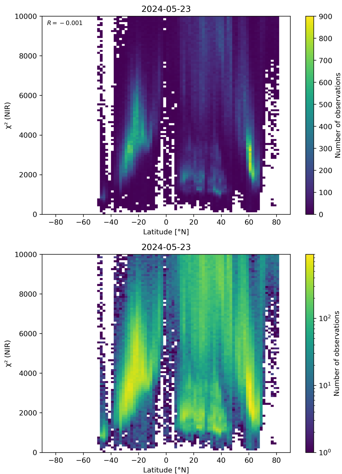
Figure 53: Scatter density plot of “Latitude” against “ \chi^2 (NIR)” for 2024-05-23 to 2024-05-24.
