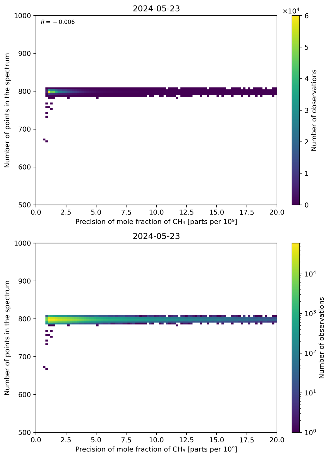
Figure 84: Scatter density plot of “Precision of mole fraction of CH 4 ” against “Number of points in the spectrum” for 2024-05-23 to 2024-05-24.
