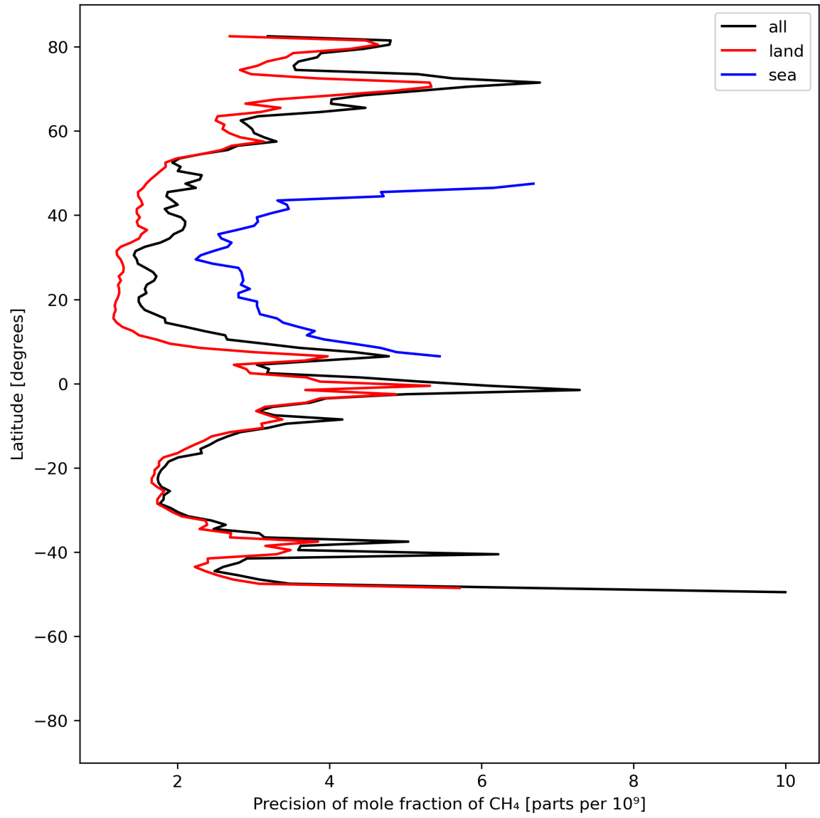
Figure 13: Zonal average of “Precision of mole fraction of CH 4 ” for 2024-05-23 to 2024-05-24.
