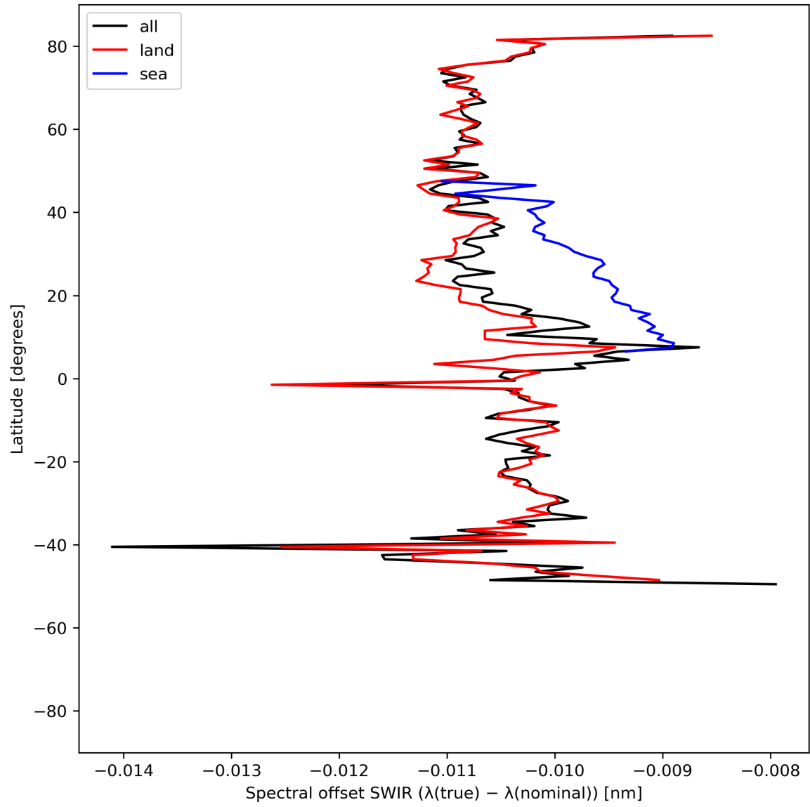
Figure 16: Zonal average of “Spectral offset SWIR ( \lambda(\text{true}) - \lambda(\text{nominal}) )” for 2024-05-23 to 2024-05-24.
