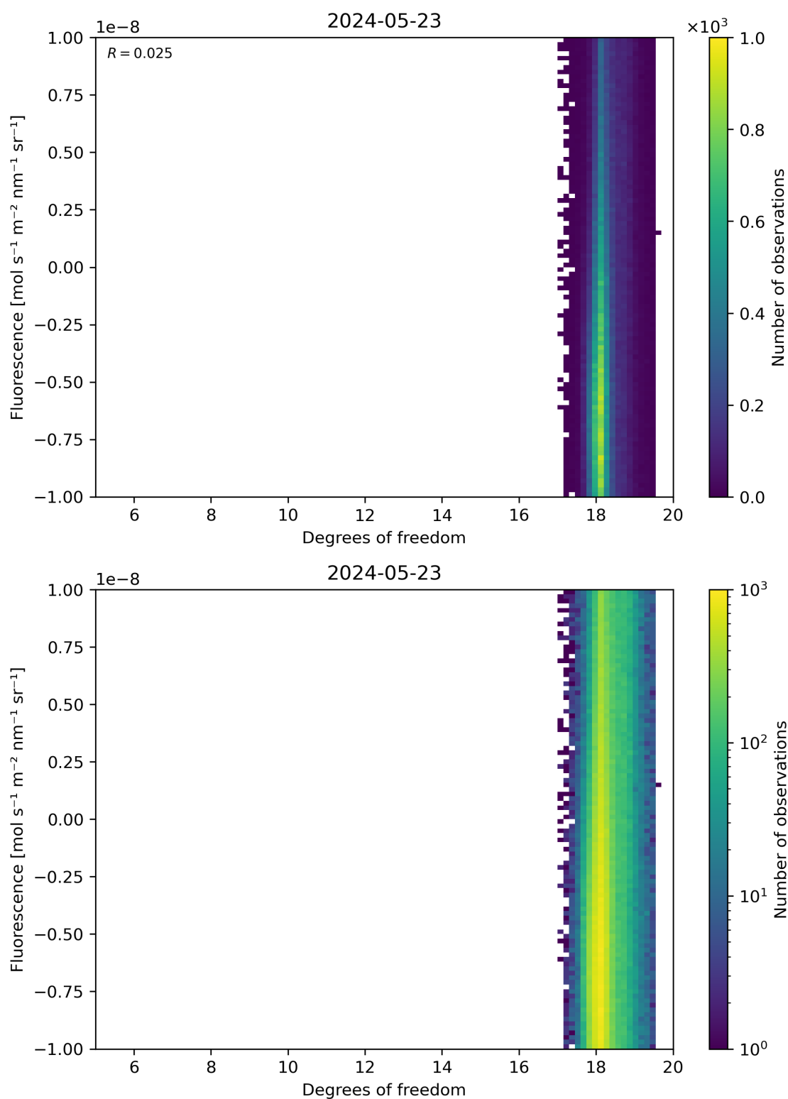
Figure 51: Scatter density plot of “Degrees of freedom” against “Fluorescence” for 2024-05-23 to 2024-05-24.
