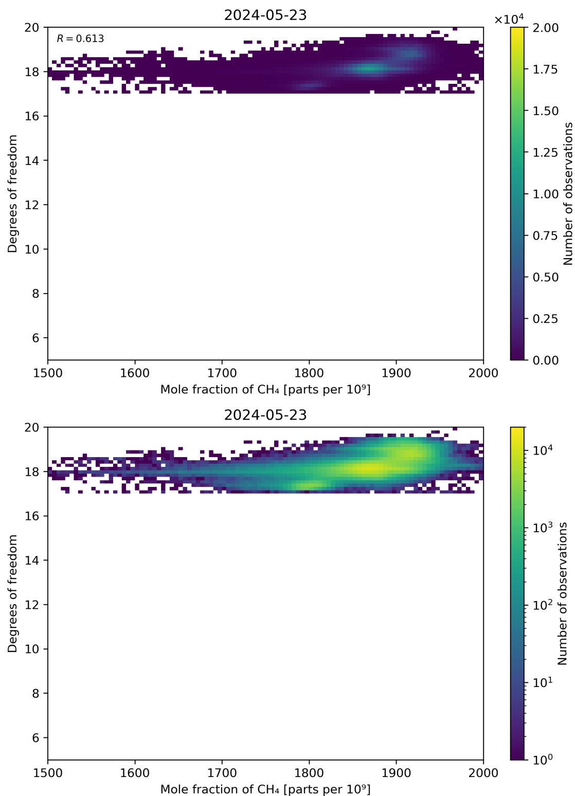
Figure 72: Scatter density plot of “Mole fraction of CH 4 ” against “Degrees of freedom” for 2024-05-23 to 2024-05-24.
