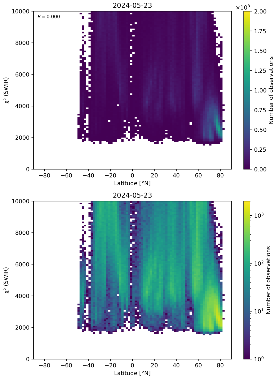
Figure 54: Scatter density plot of “Latitude” against “ \chi^2 (SWIR)” for 2024-05-23 to 2024-05-24.
