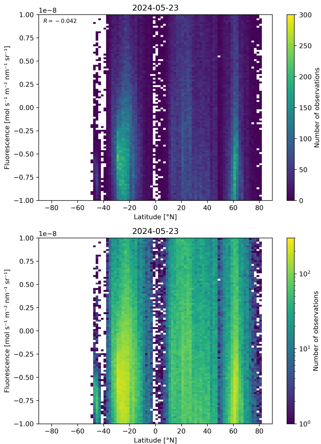
Figure 56: Scatter density plot of “Latitude” against “Fluorescence” for 2024-05-23 to 2024-05-24.
