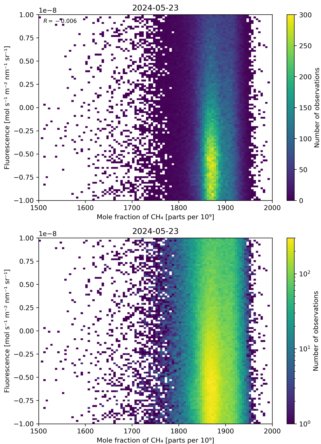
Figure 73: Scatter density plot of “Mole fraction of \text{CH}_4 ” against “Fluorescence” for 2024-05-23 to 2024-05-24.
