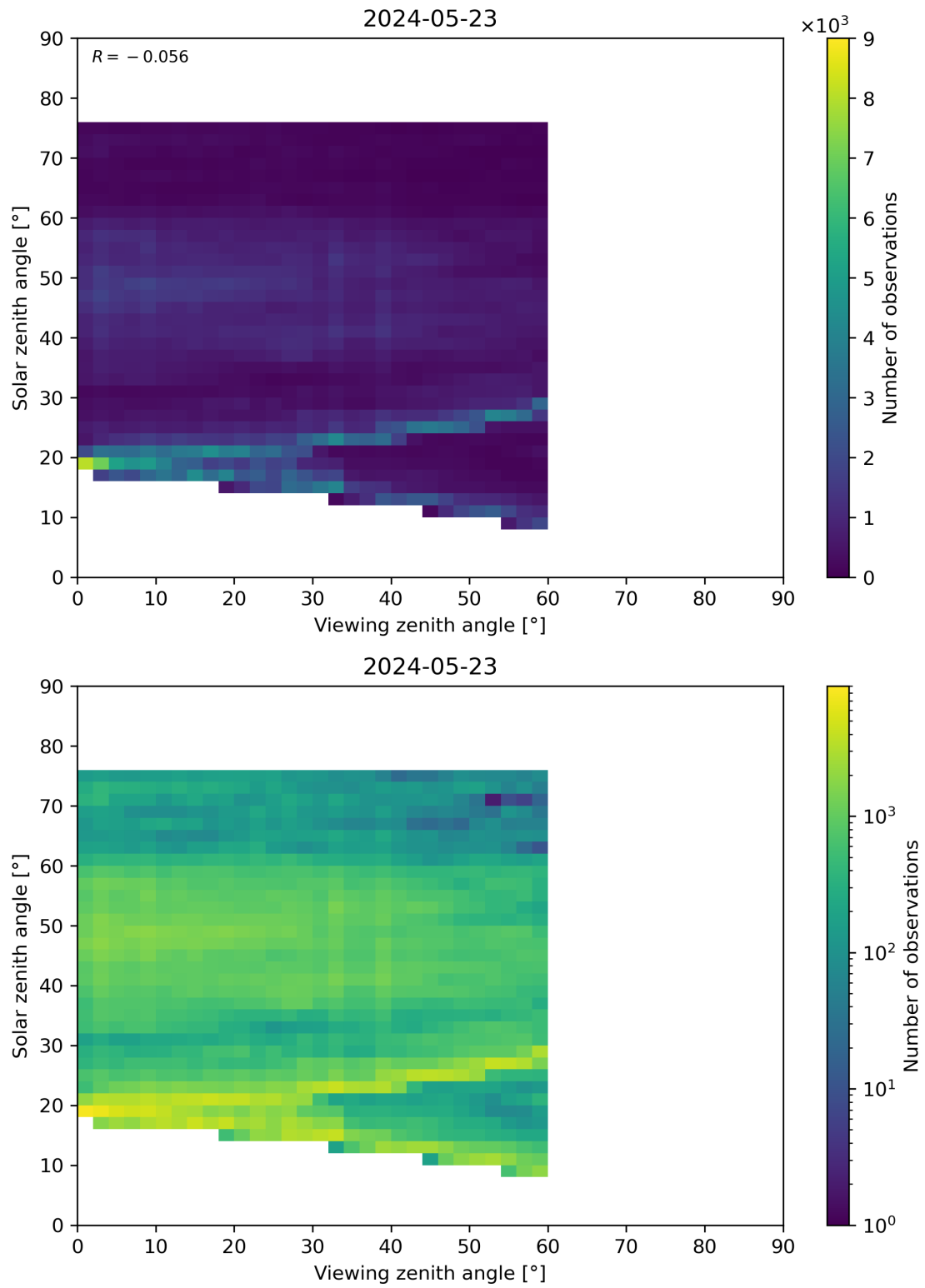
Figure 115: Scatter density plot of “Viewing zenith angle” against “Solar zenith angle” for 2024-05-23 to 2024-05-24.
