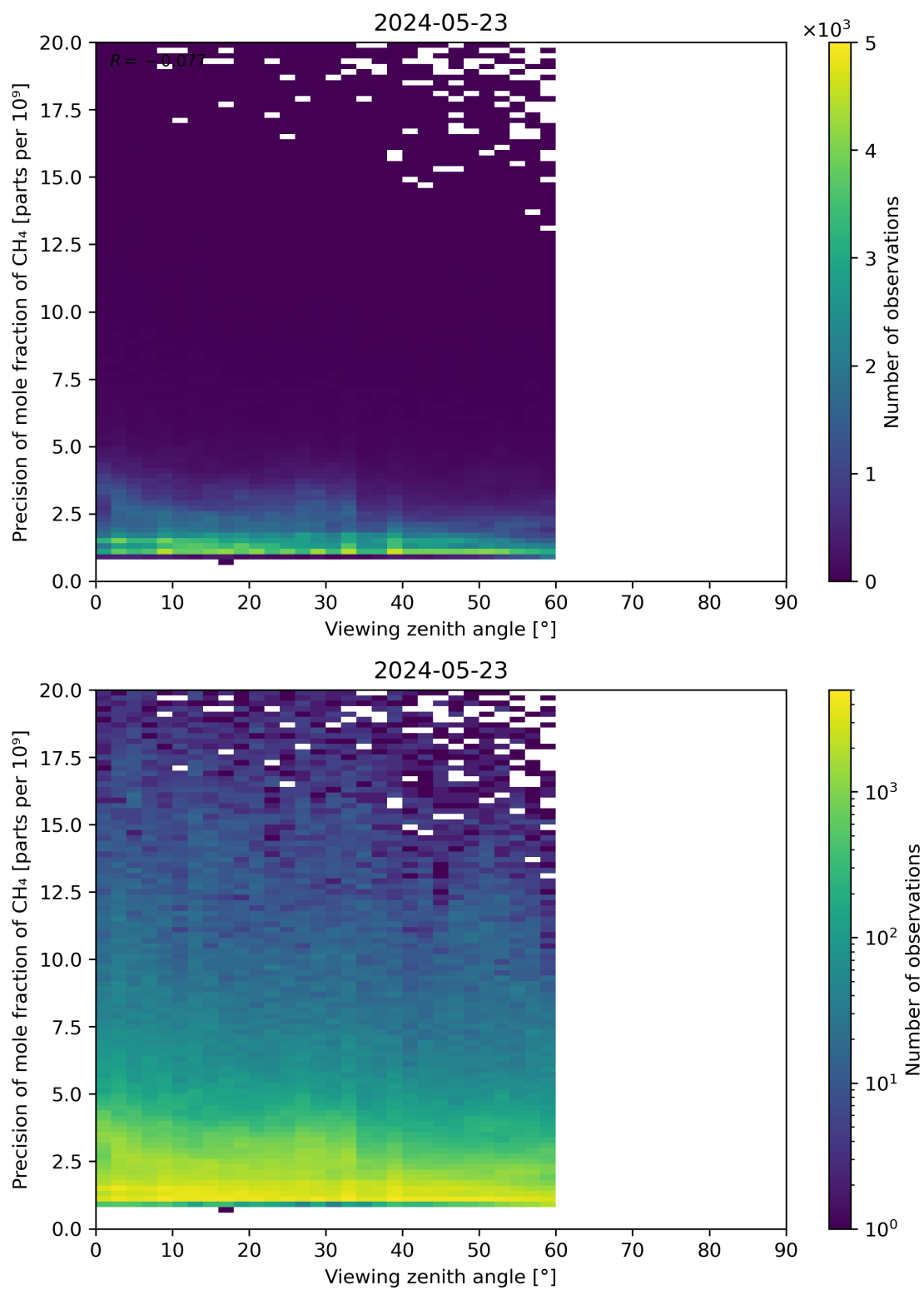
Figure 112: Scatter density plot of “Viewing zenith angle” against “Precision of mole fraction of CH 4 ” for 2024-05-23 to 2024-05-24.
