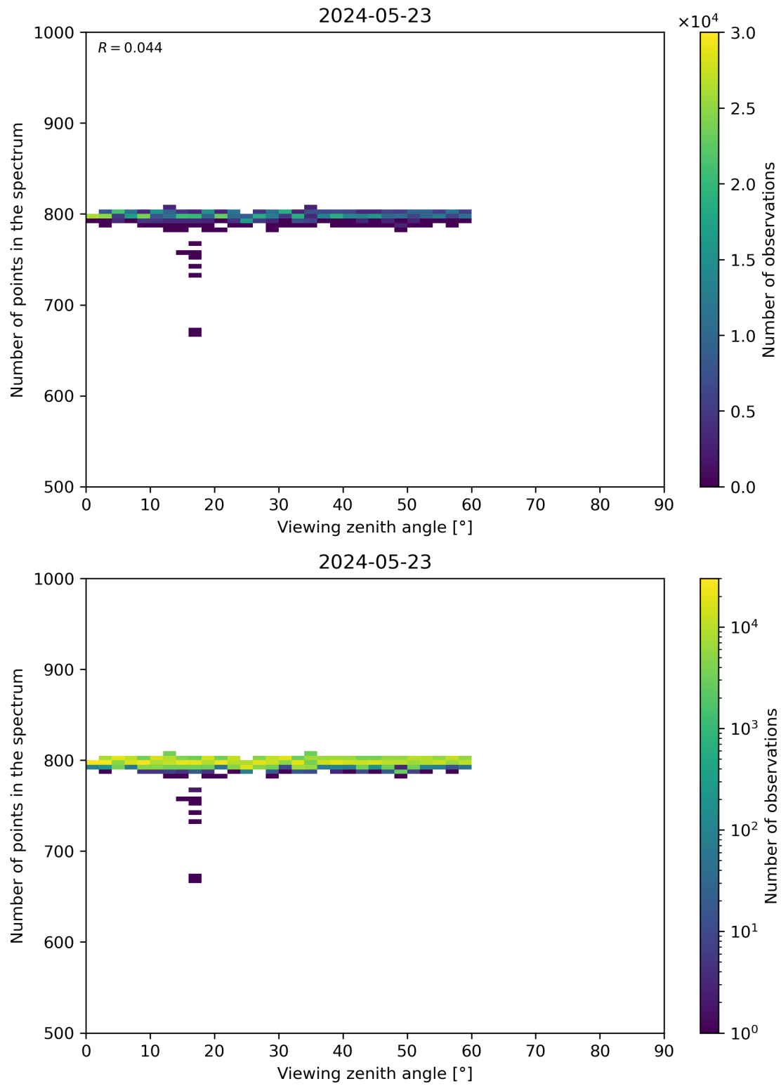
Figure 114: Scatter density plot of “Viewing zenith angle” against “Number of points in the spectrum” for 2024-05-23 to 2024-05-24.
