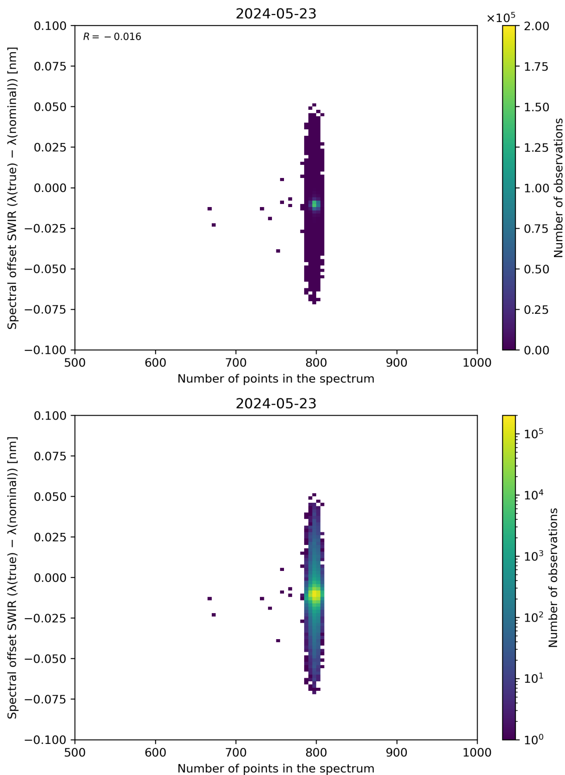
Figure 93: Scatter density plot of “Number of points in the spectrum” against “Spectral offset SWIR ( \lambda(\text{true}) - \lambda(\text{nominal}) )” for 2024-05-23 to 2024-05-24.
