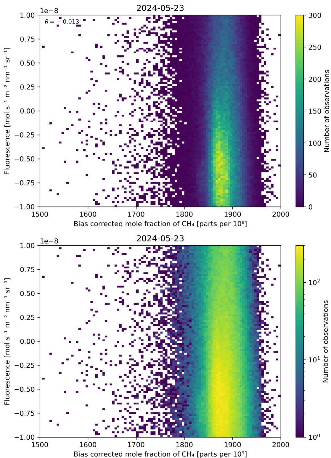
Figure 66: Scatter density plot of “Bias corrected mole fraction of \text{CH}_4 ” against “Fluorescence” for 2024-05-23 to 2024-05-24.
