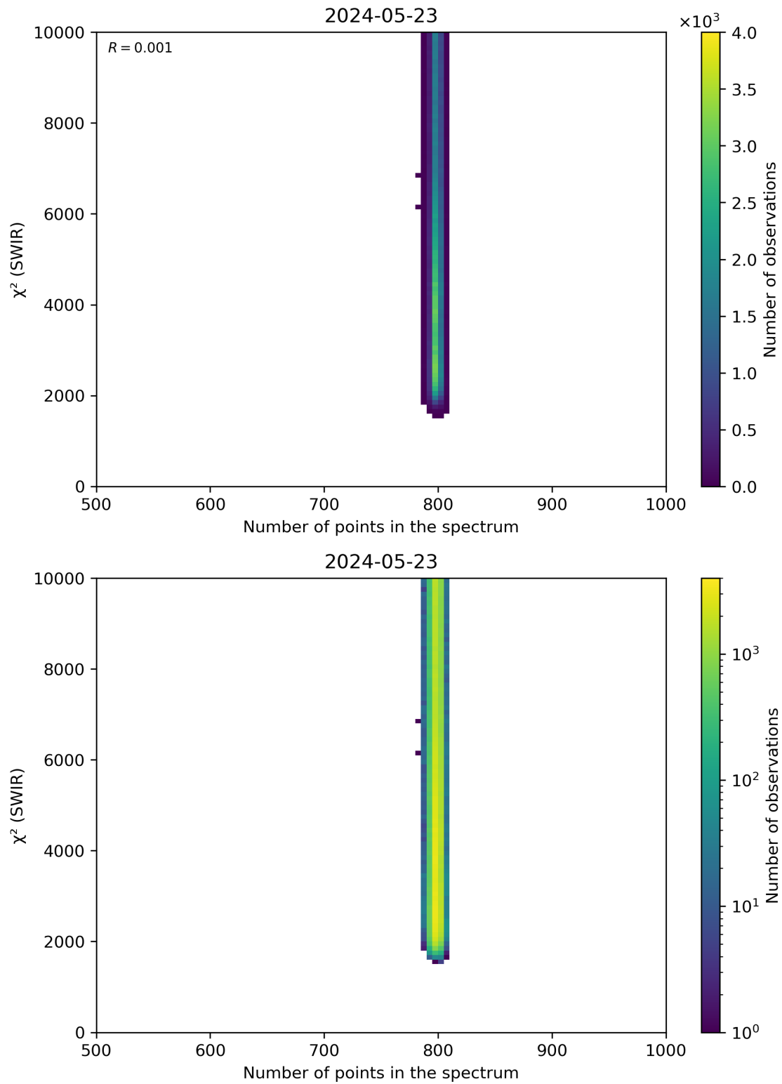
Figure 89: Scatter density plot of “Number of points in the spectrum” against “ \chi^2 (SWIR)” for 2024-05-23 to 2024-05-24.
