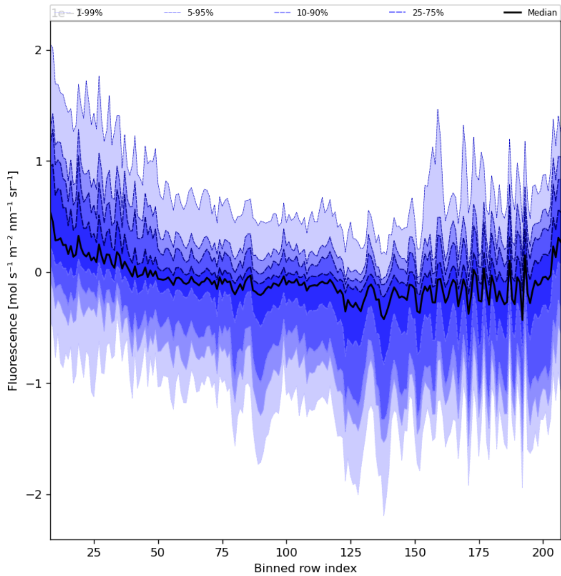
Figure 43: Along track statistics of “Fluorescence” for 2024-05-23 to 2024-05-24
