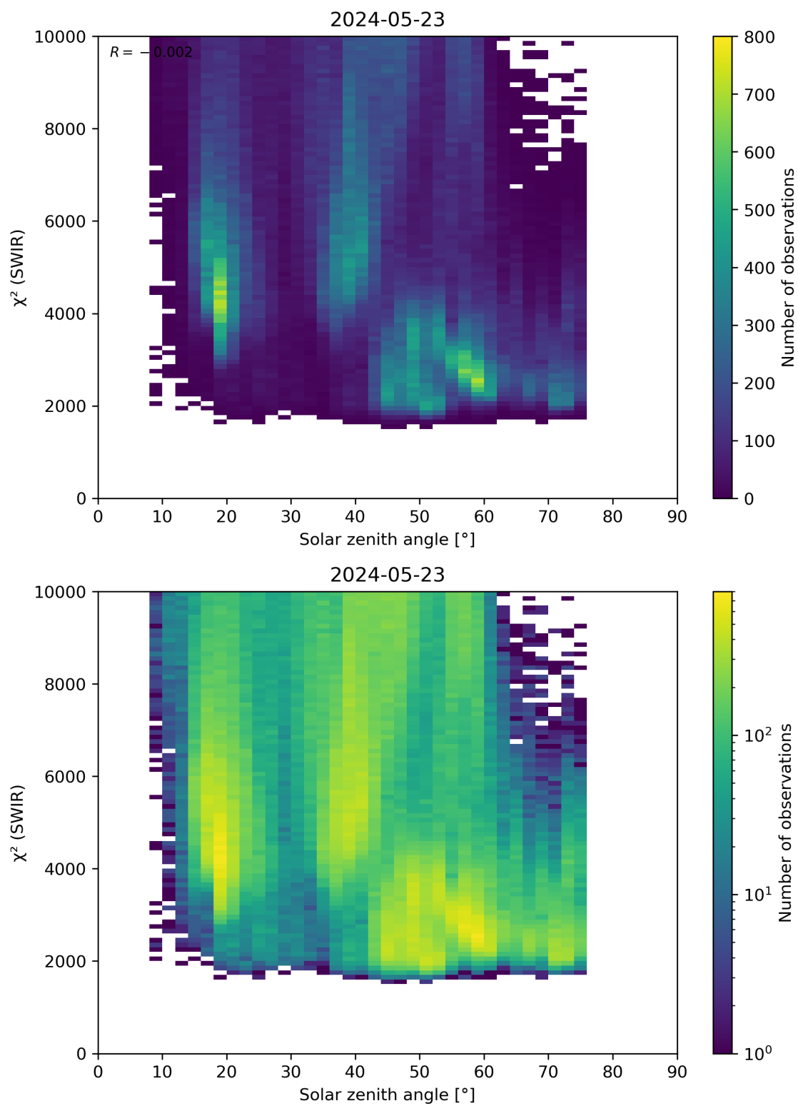
Figure 95: Scatter density plot of “Solar zenith angle” against “ \chi^2 (SWIR)” for 2024-05-23 to 2024-05-24.
