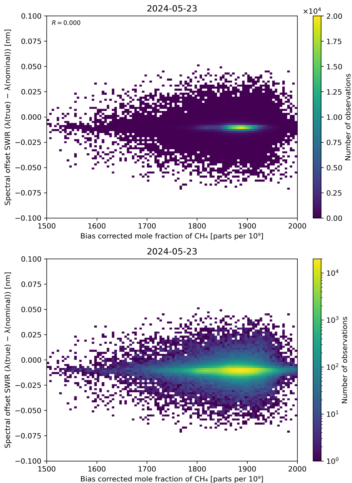
Figure 69: Scatter density plot of “Bias corrected mole fraction of \text{CH}_4 ” against “Spectral offset SWIR ( \lambda(\text{true}) - \lambda(\text{nominal}) )” for 2024-05-23 to 2024-05-24.
