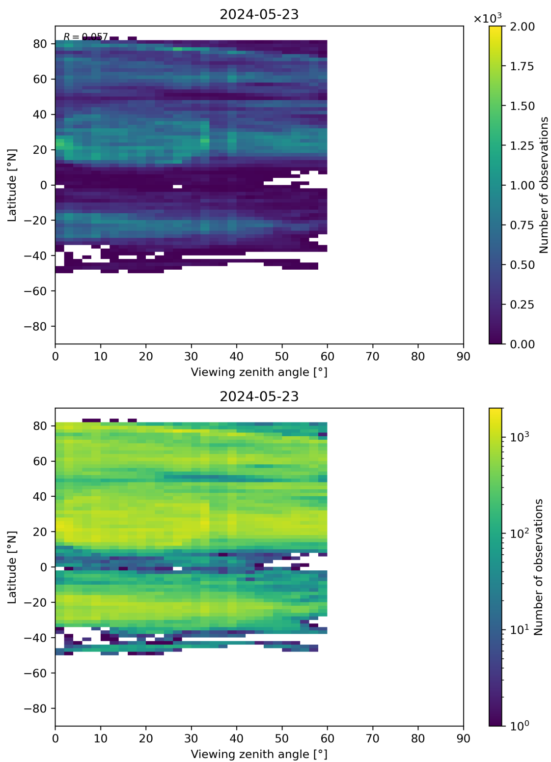
Figure 109: Scatter density plot of “Viewing zenith angle” against “Latitude” for 2024-05-23 to 2024-05-24.
