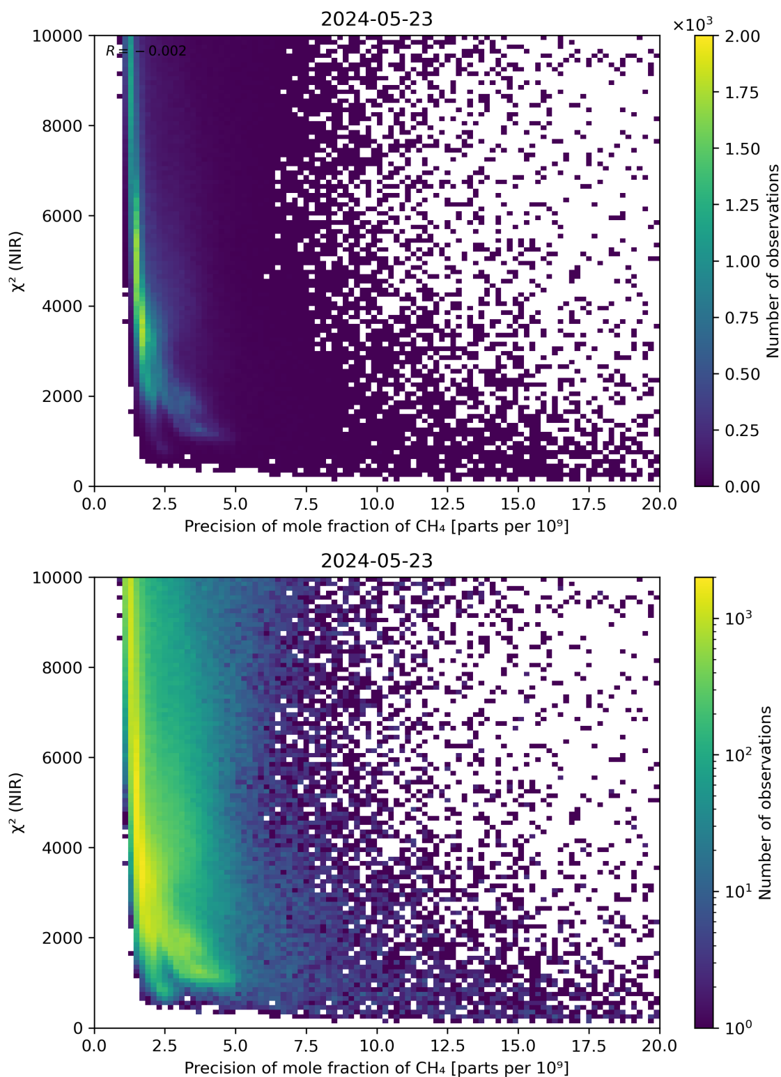
Figure 78: Scatter density plot of “Precision of mole fraction of CH 4 ” against “ \chi^2 (NIR)” for 2024-05-23 to 2024-05-24.
