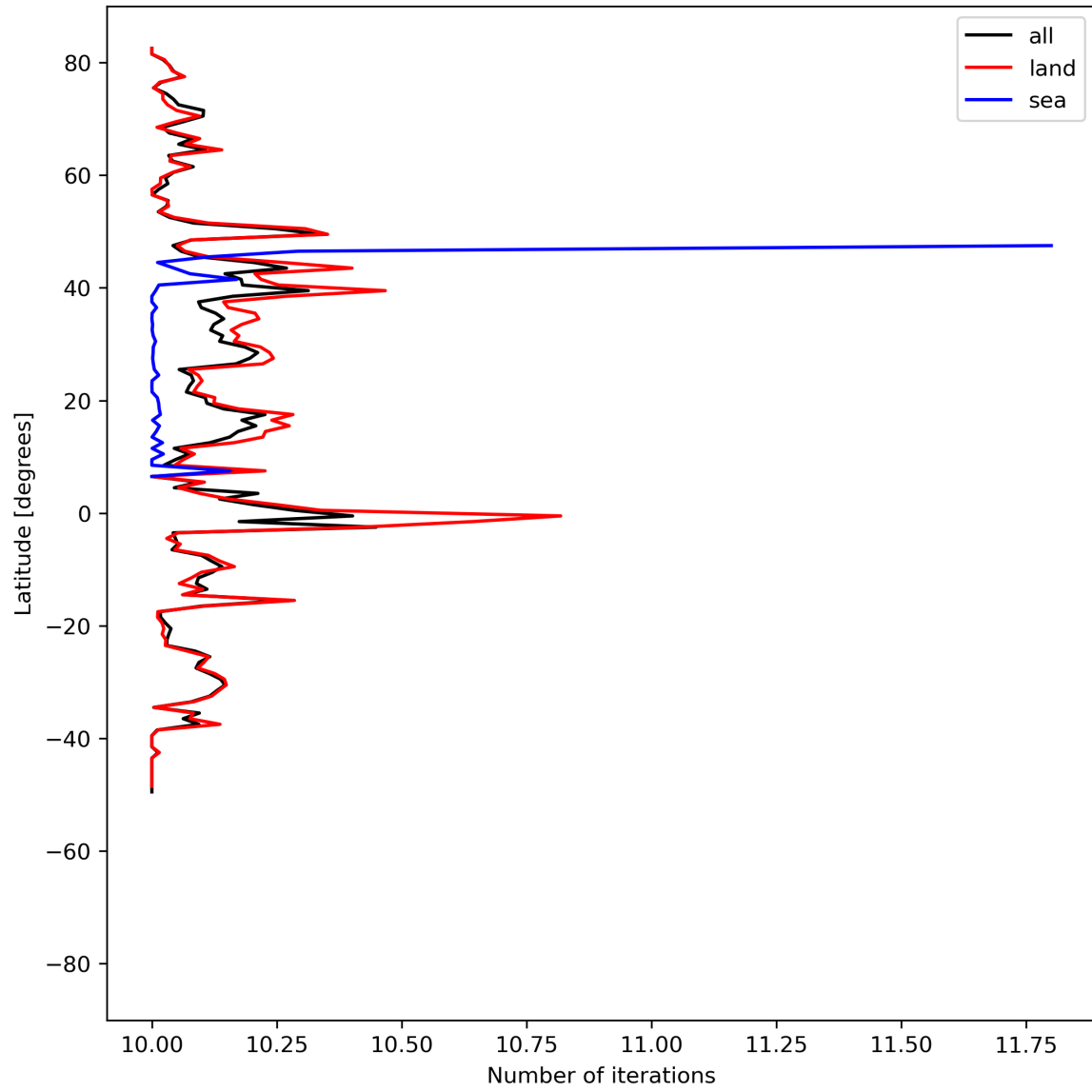
Figure 20: Zonal average of “Number of iterations” for 2024-05-23 to 2024-05-24.
