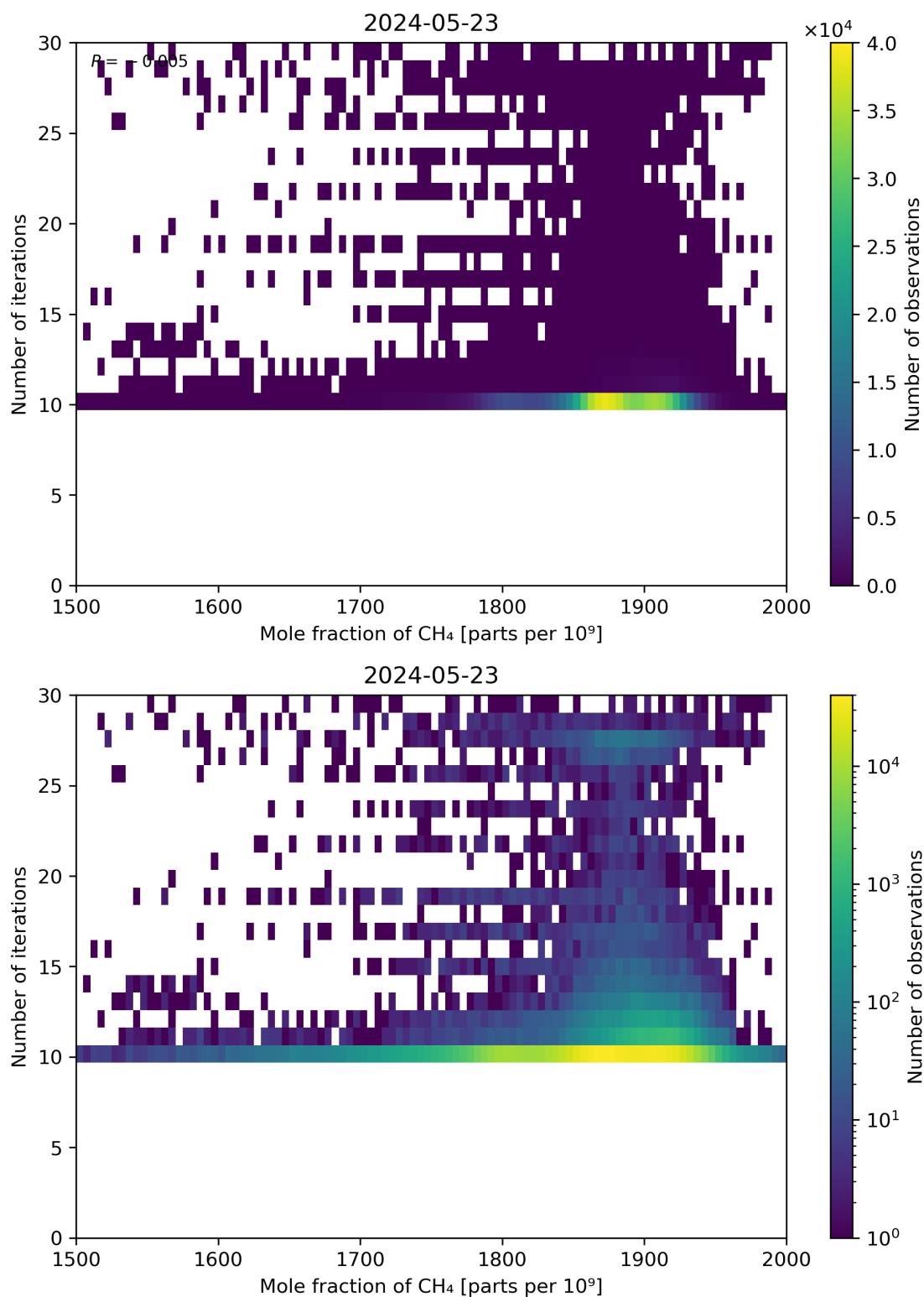
Figure 76: Scatter density plot of “Mole fraction of CH 4 ” against “Number of iterations” for 2024-05-23 to 2024-05-24.
