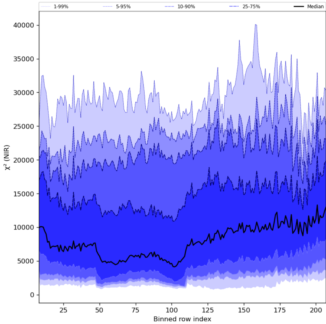
Figure 40: Along track statistics of “ \chi^2 (NIR)” for 2024-05-23 to 2024-05-24
