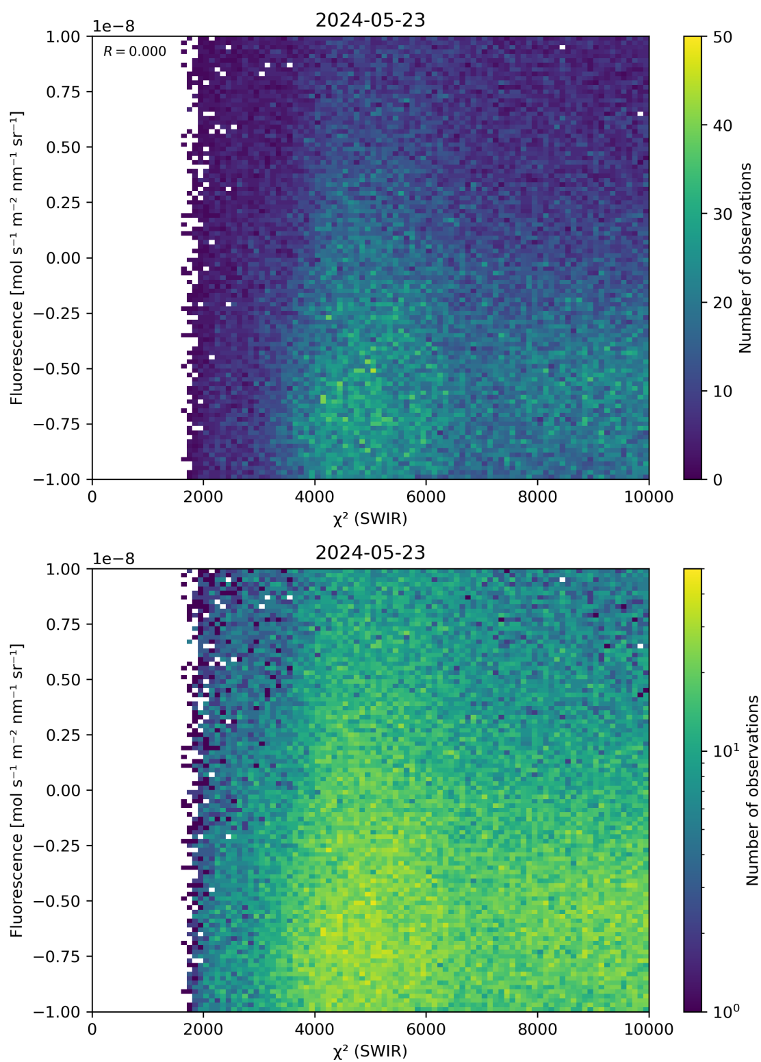
Figure 49: Scatter density plot of “ \chi^2 (SWIR)” against “Fluorescence” for 2024-05-23 to 2024-05-24.
