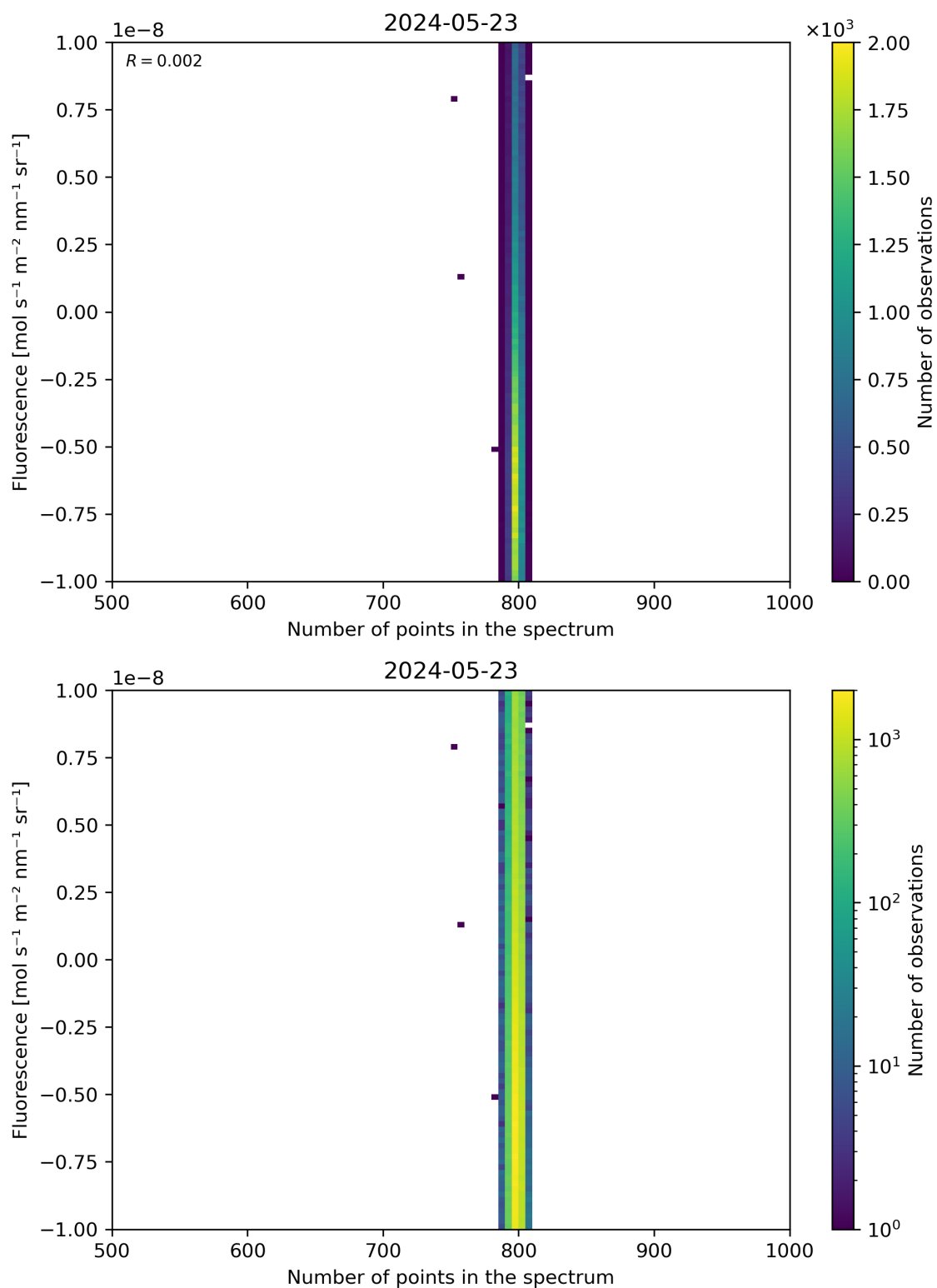
Figure 91: Scatter density plot of “Number of points in the spectrum” against “Fluorescence” for 2024-05-23 to 2024-05-24.
