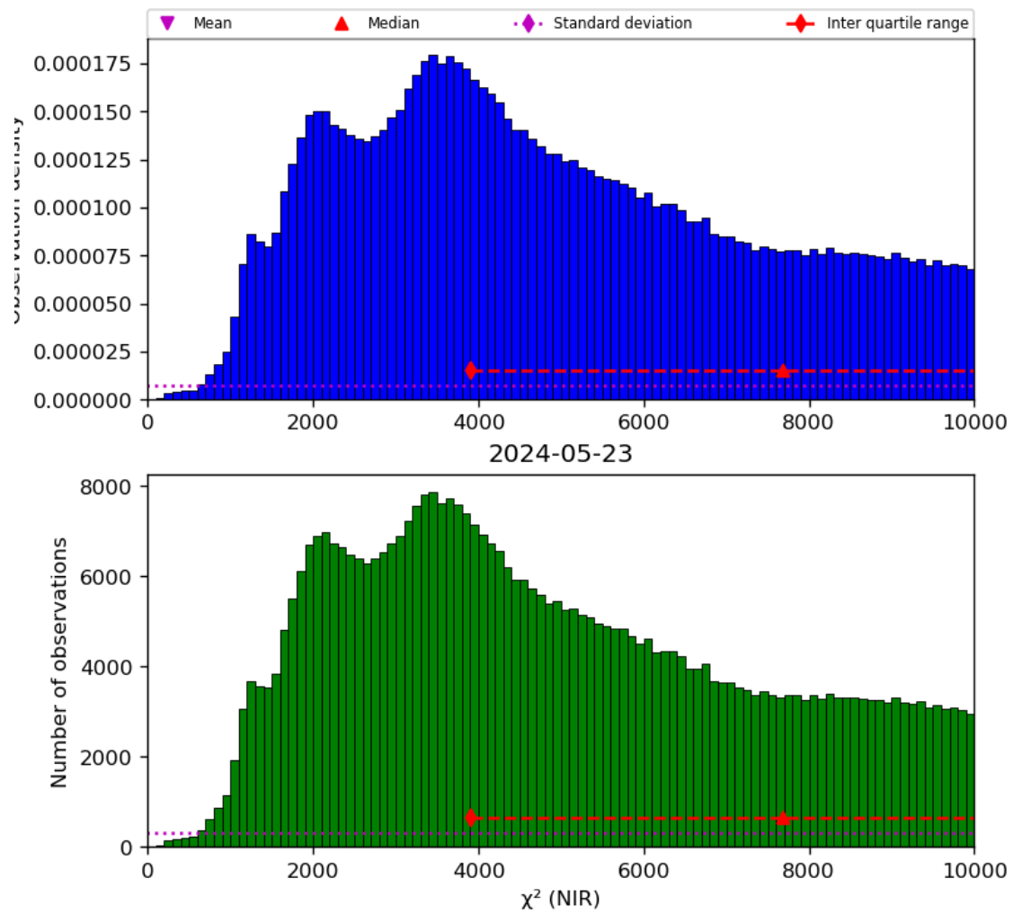
Figure 29: Histogram of “ \chi^2 (NIR)” for 2024-05-23 to 2024-05-24
