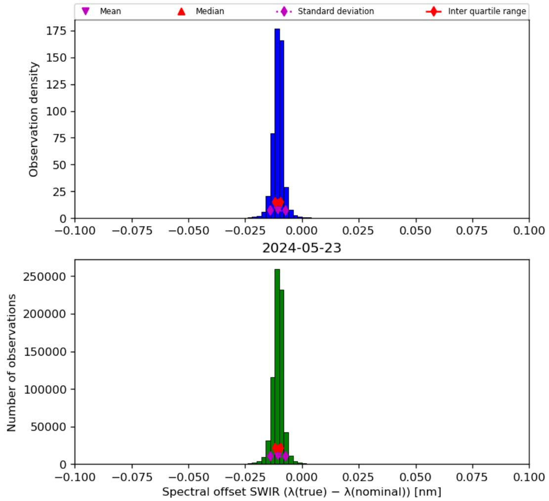
Figure 27: Histogram of “Spectral offset SWIR ( \lambda(\text{true}) - \lambda(\text{nominal}) )” for 2024-05-23 to 2024-05-24
