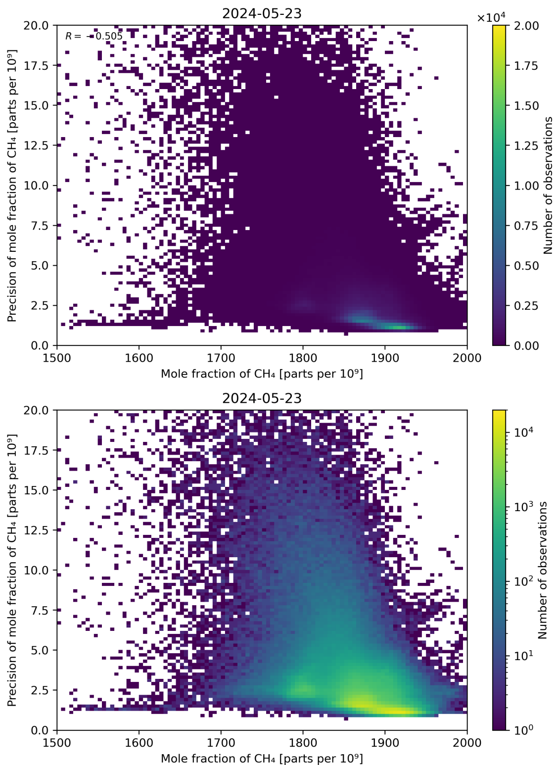
Figure 75: Scatter density plot of “Mole fraction of CH 4 ” against “Precision of mole fraction of CH 4 ” for 2024-05-23 to 2024-05-24.
