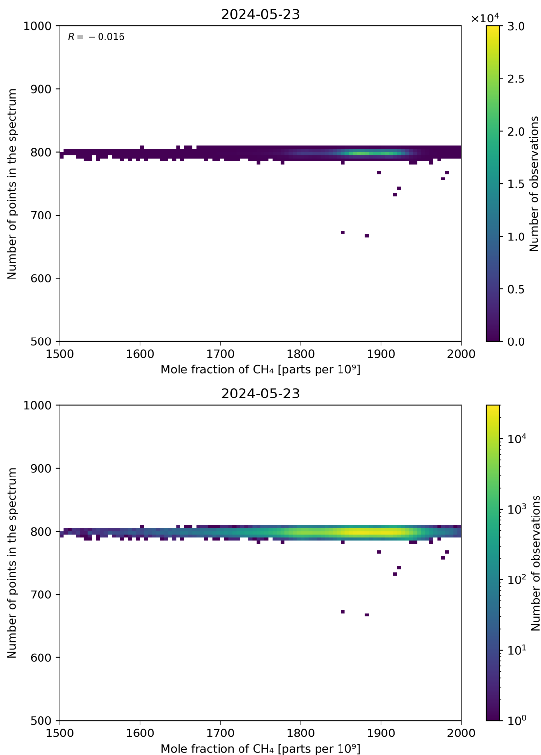
Figure 77: Scatter density plot of “Mole fraction of CH 4 ” against “Number of points in the spectrum” for 2024-05-23 to 2024-05-24.
