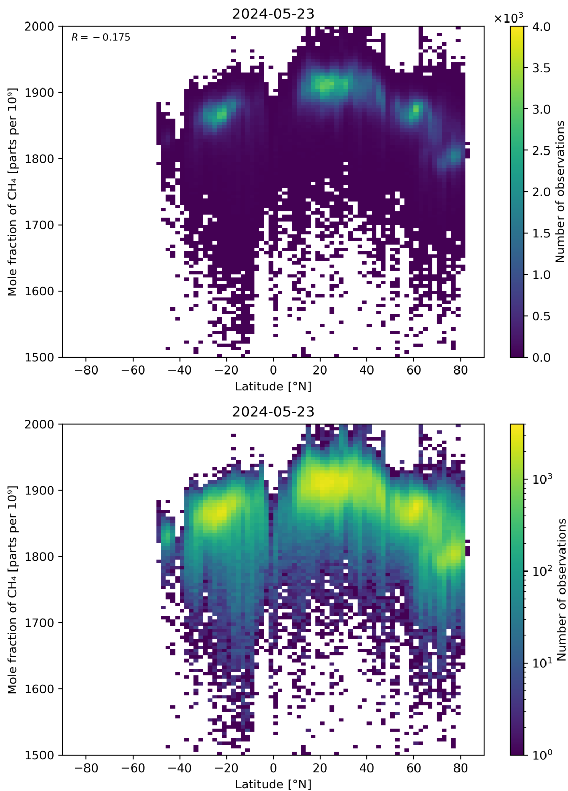
Figure 57: Scatter density plot of “Latitude” against “Mole fraction of \text{CH}_4 ” for 2024-05-23 to 2024-05-24.
