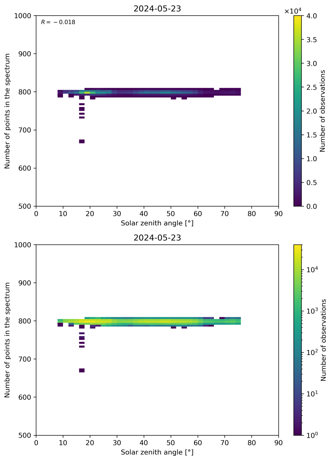
Figure 103: Scatter density plot of “Solar zenith angle” against “Number of points in the spectrum” for 2024-05-23 to 2024-05-24.
