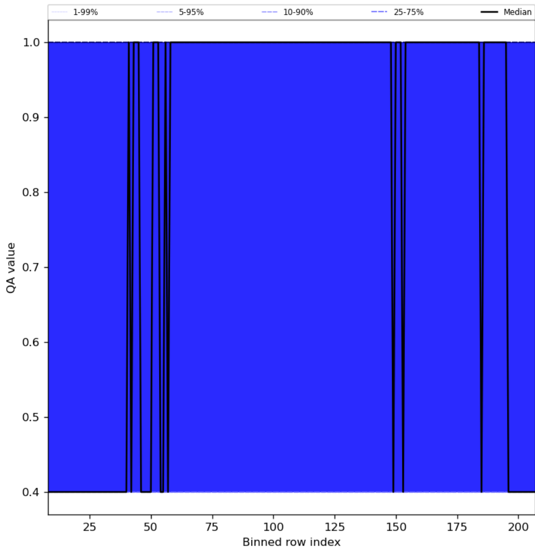
Figure 33: Along track statistics of “QA value” for 2024-05-23 to 2024-05-24
