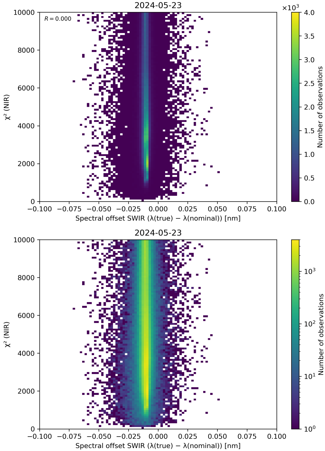
Figure 117: Scatter density plot of “Spectral offset SWIR ( \lambda(\text{true}) - \lambda(\text{nominal}) )” against “ \chi^2 (NIR)” for 2024-05-23 to 2024-05-24.
