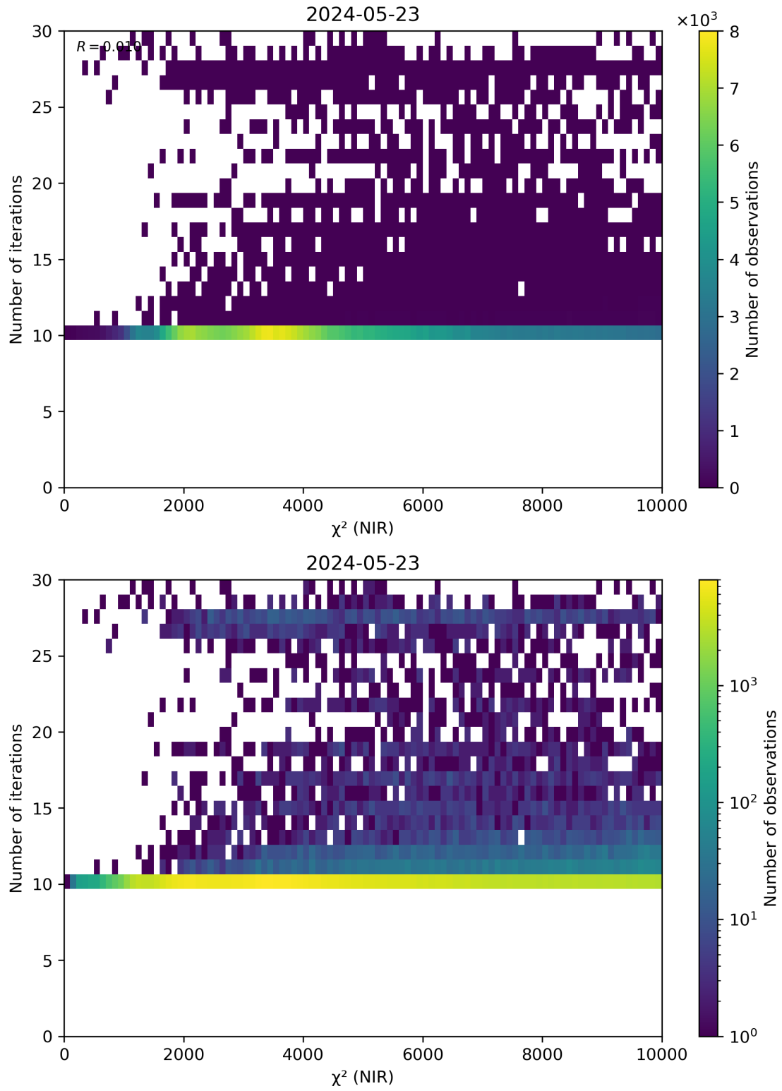
Figure 46: Scatter density plot of “ \chi^2 (NIR)” against “Number of iterations” for 2024-05-23 to 2024-05-24.
