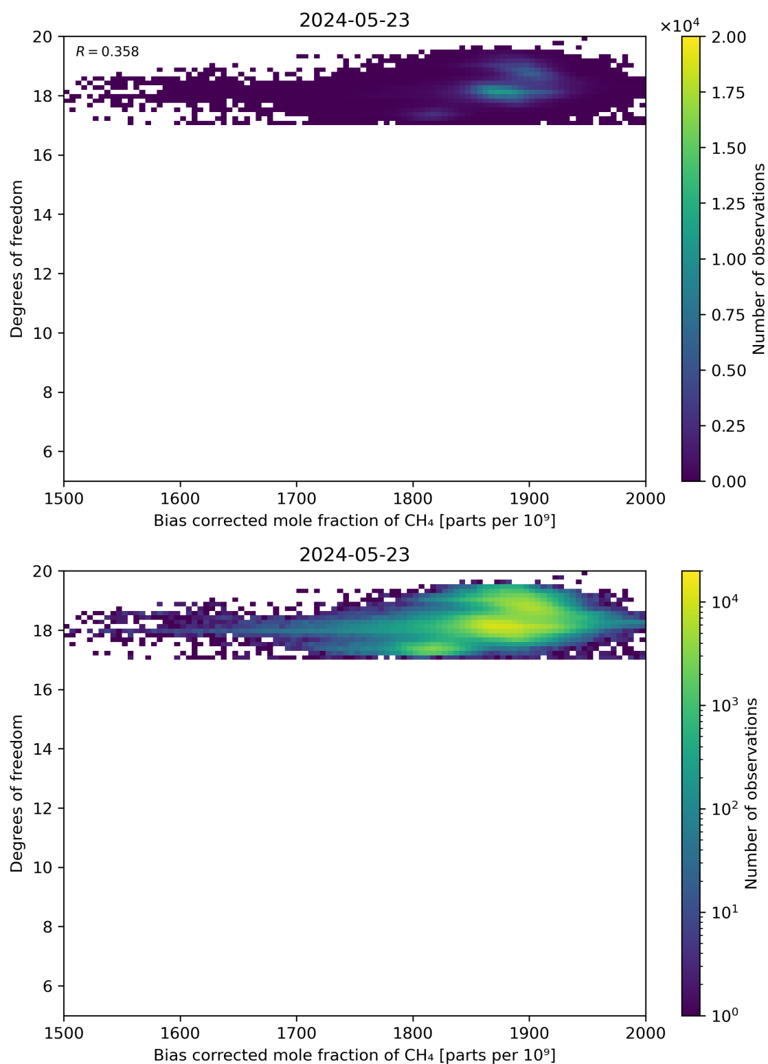
Figure 65: Scatter density plot of “Bias corrected mole fraction of CH 4 ” against “Degrees of freedom” for 2024-05-23 to 2024-05-24.
