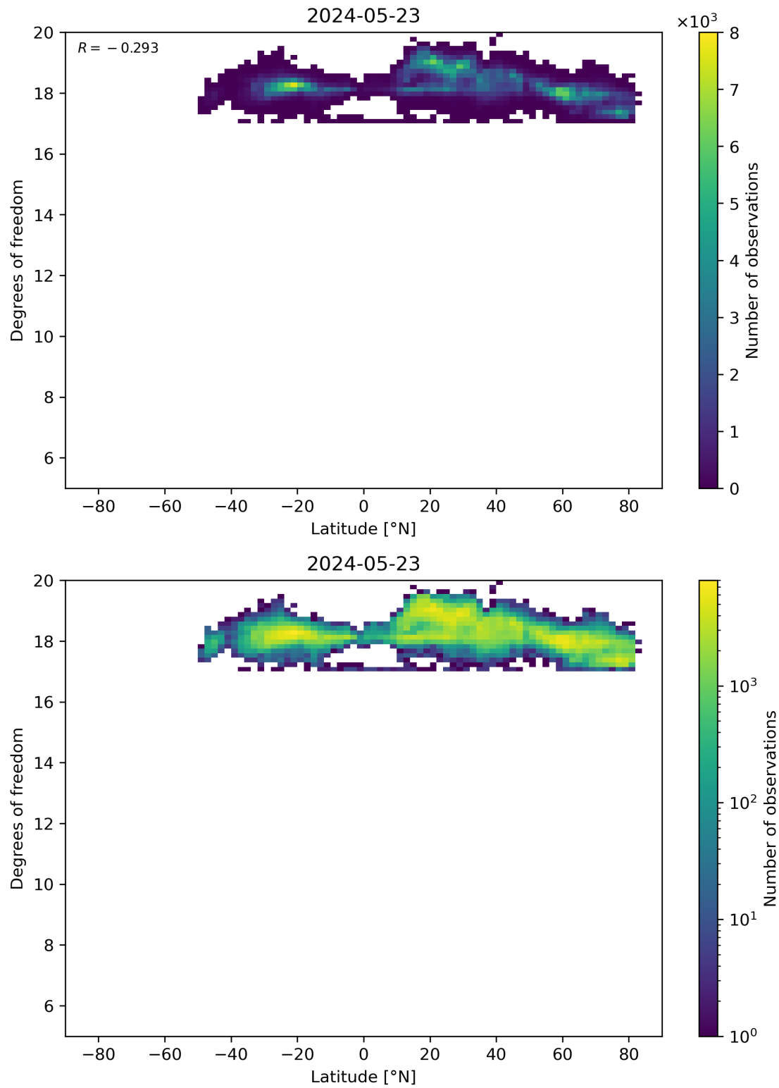
Figure 55: Scatter density plot of “Latitude” against “Degrees of freedom” for 2024-05-23 to 2024-05-24.
