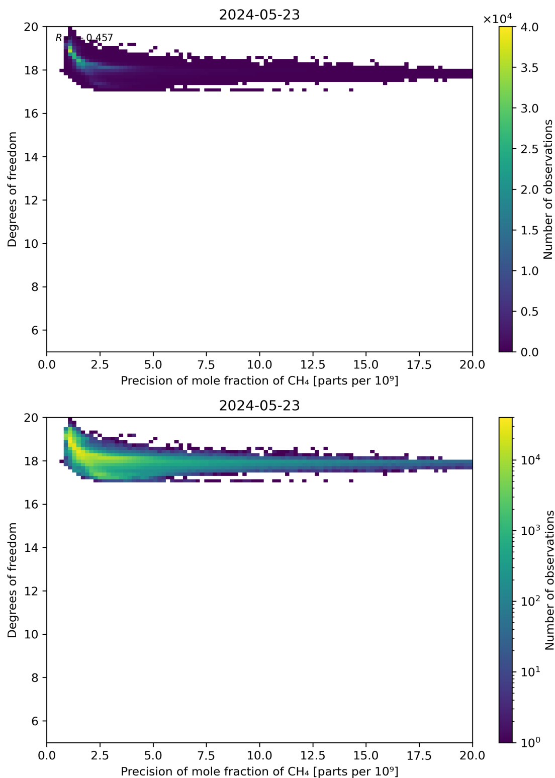
Figure 80: Scatter density plot of “Precision of mole fraction of CH 4 ” against “Degrees of freedom” for 2024-05-23 to 2024-05-24.
