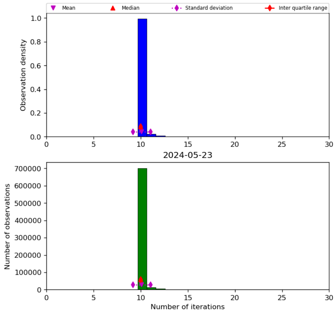
Figure 31: Histogram of “Number of iterations” for 2024-05-23 to 2024-05-24
