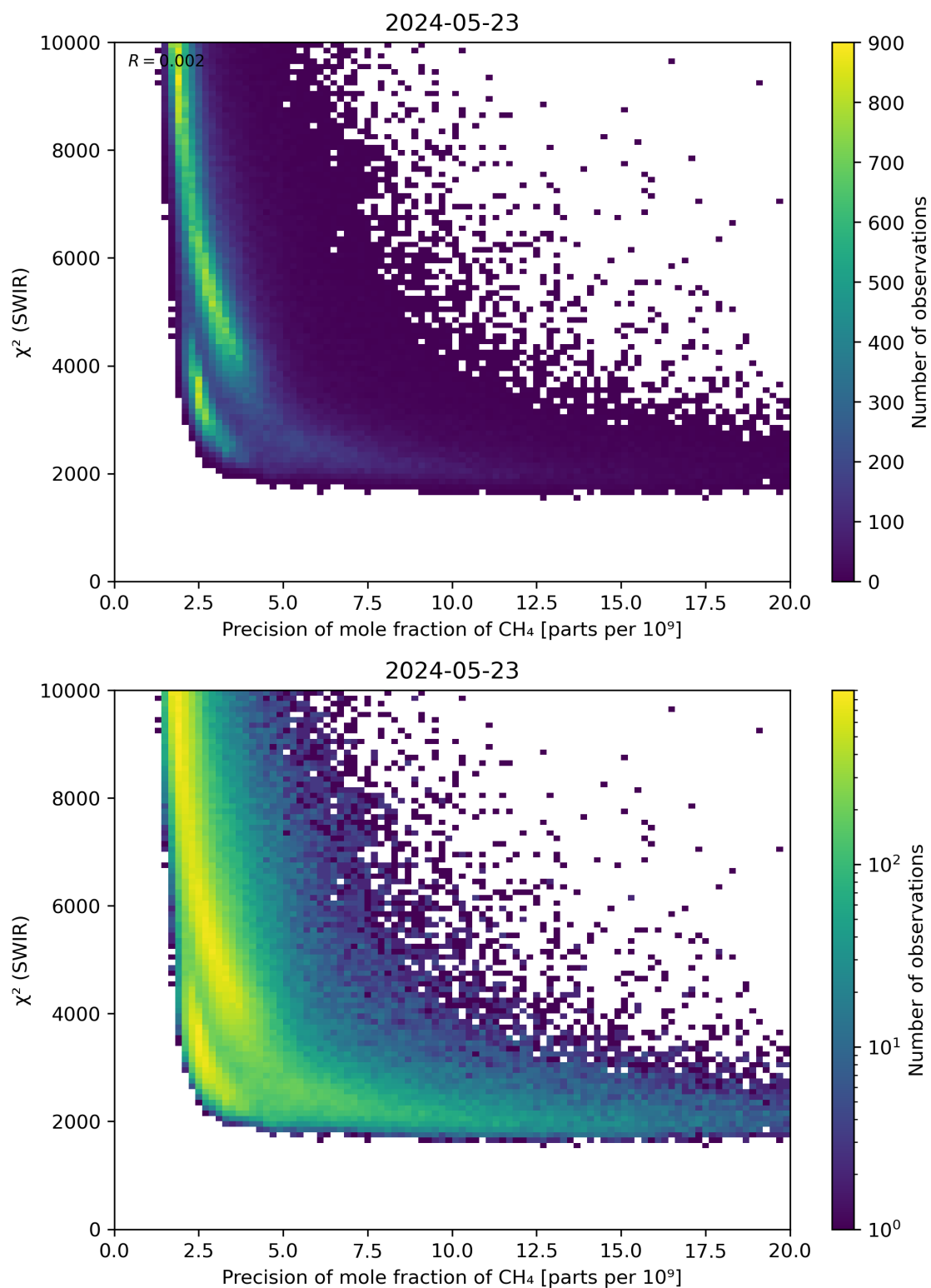
Figure 79: Scatter density plot of “Precision of mole fraction of CH 4 ” against “ \chi^2 (SWIR)” for 2024-05-23 to 2024-05-24.
