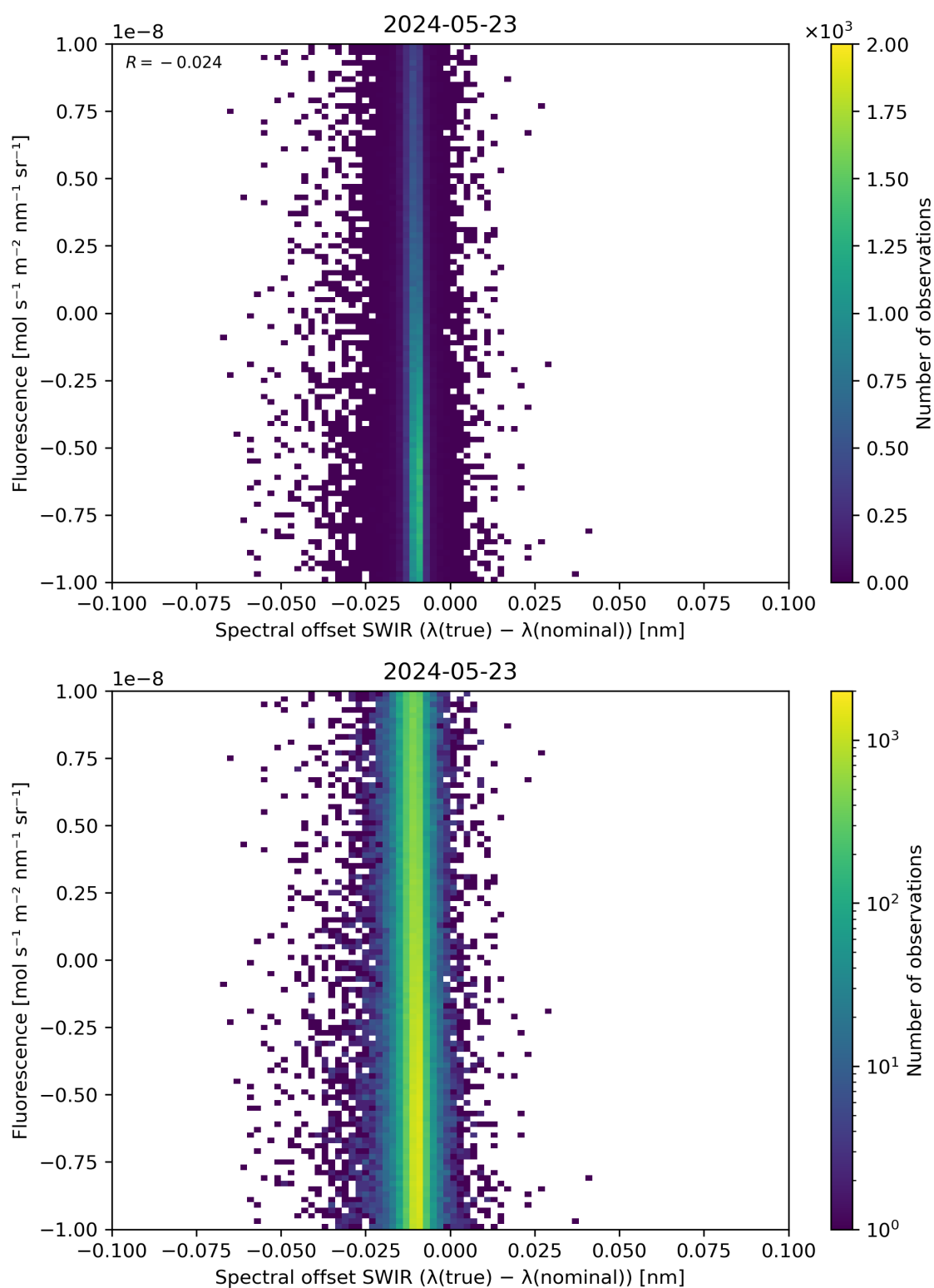
Figure 120: Scatter density plot of “Spectral offset SWIR ( \lambda(\text{true}) - \lambda(\text{nominal}) )” against “Fluorescence” for 2024-05-23 to 2024-05-24.
