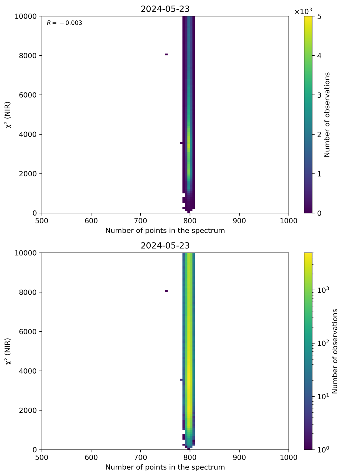
Figure 88: Scatter density plot of “Number of points in the spectrum” against “ \chi^2 (NIR)” for 2024-05-23 to 2024-05-24.
