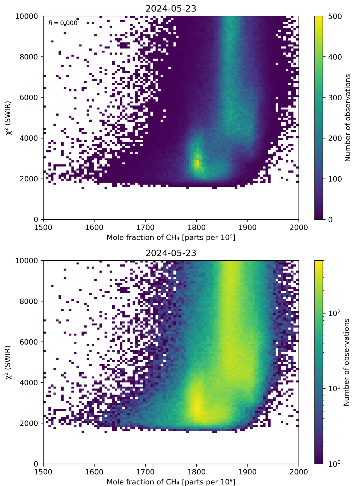
Figure 71: Scatter density plot of “Mole fraction of \text{CH}_4 ” against “ \chi^2 (SWIR)” for 2024-05-23 to 2024-05-24.
