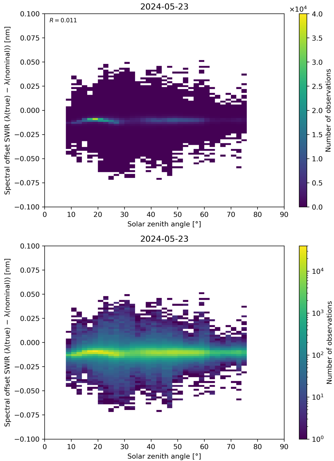
Figure 104: Scatter density plot of “Solar zenith angle” against “Spectral offset SWIR ( \lambda(\text{true}) - \lambda(\text{nominal}) )” for 2024-05-23 to 2024-05-24.
