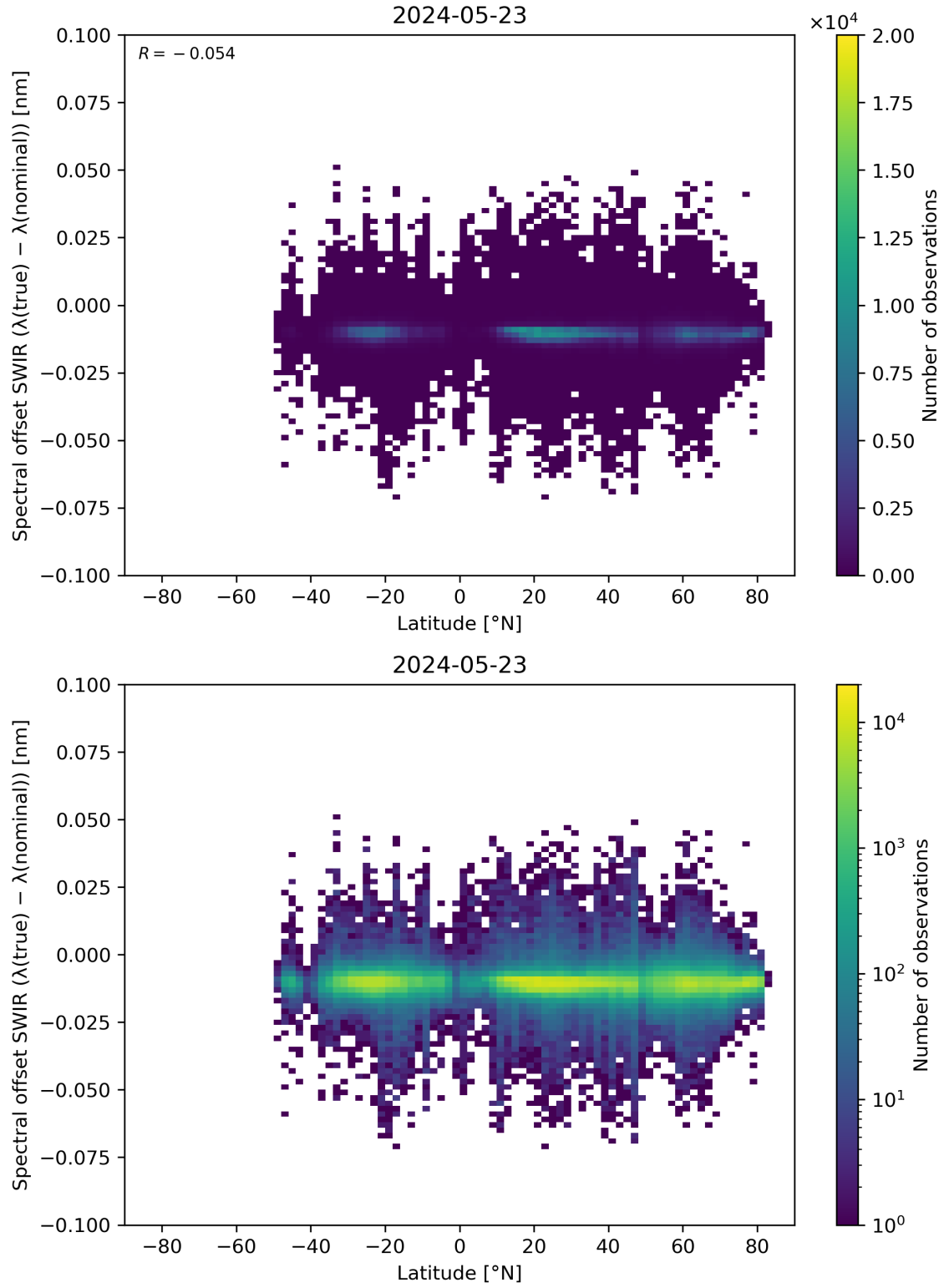
Figure 62: Scatter density plot of “Latitude” against “Spectral offset SWIR ( \lambda(\text{true}) - \lambda(\text{nominal}) )” for 2024-05-23 to 2024-05-24.
