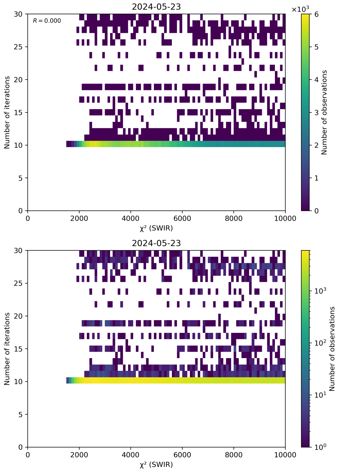
Figure 50: Scatter density plot of “ \chi^2 (SWIR)” against “Number of iterations” for 2024-05-23 to 2024-05-24.
