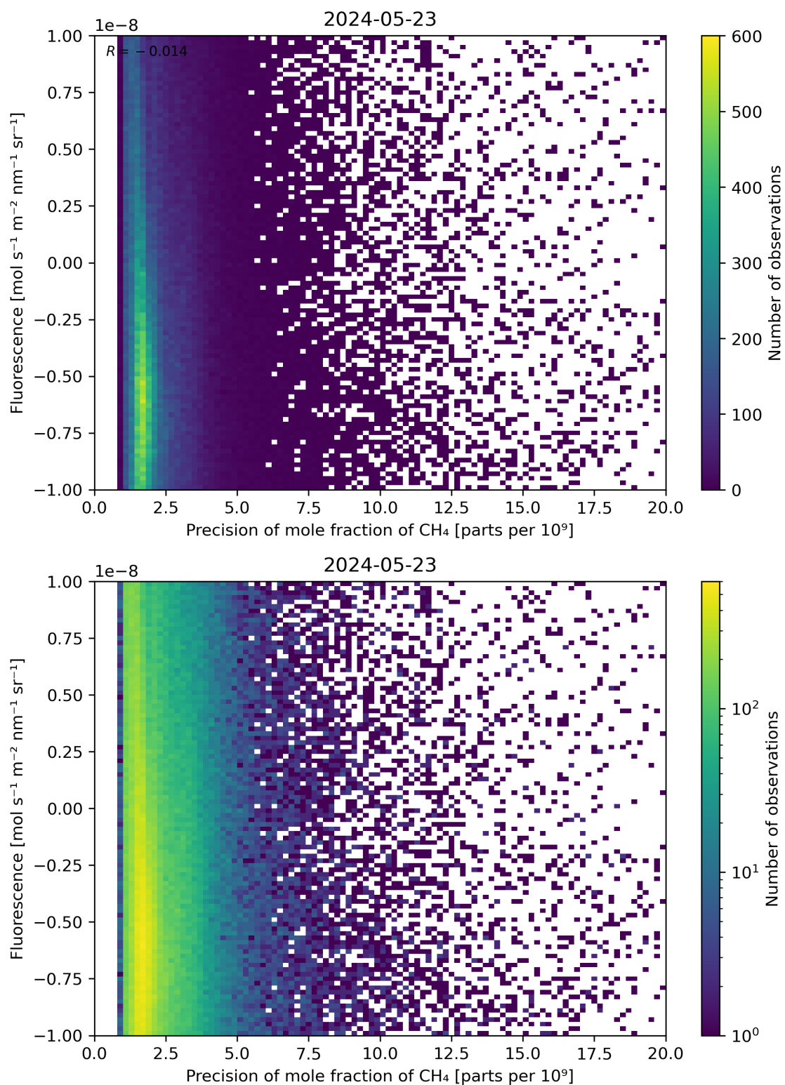
Figure 81: Scatter density plot of “Precision of mole fraction of \text{CH}_4 ” against “Fluorescence” for 2024-05-23 to 2024-05-24.
