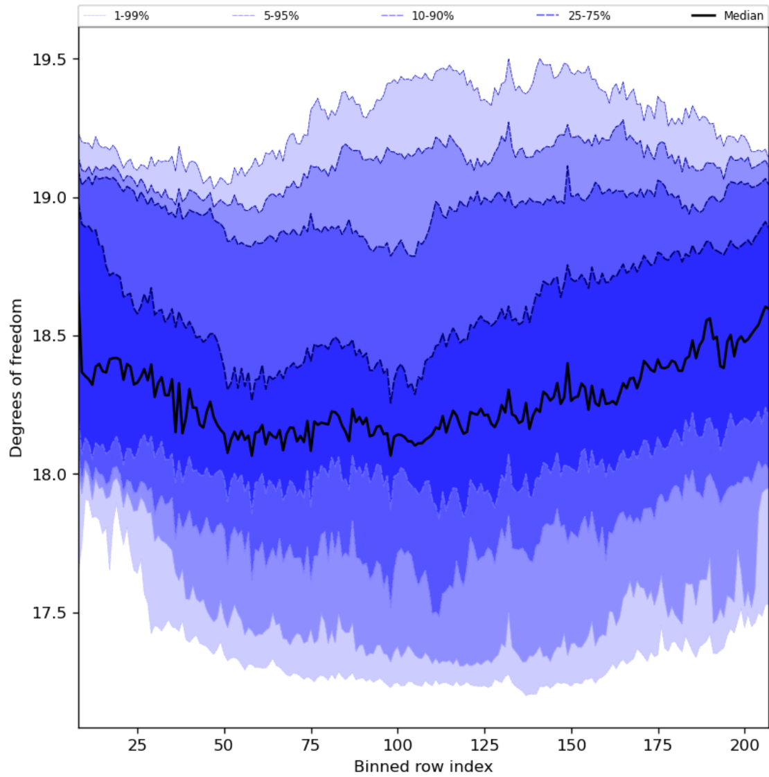
Figure 41: Along track statistics of “Degrees of freedom” for 2024-05-23 to 2024-05-24
