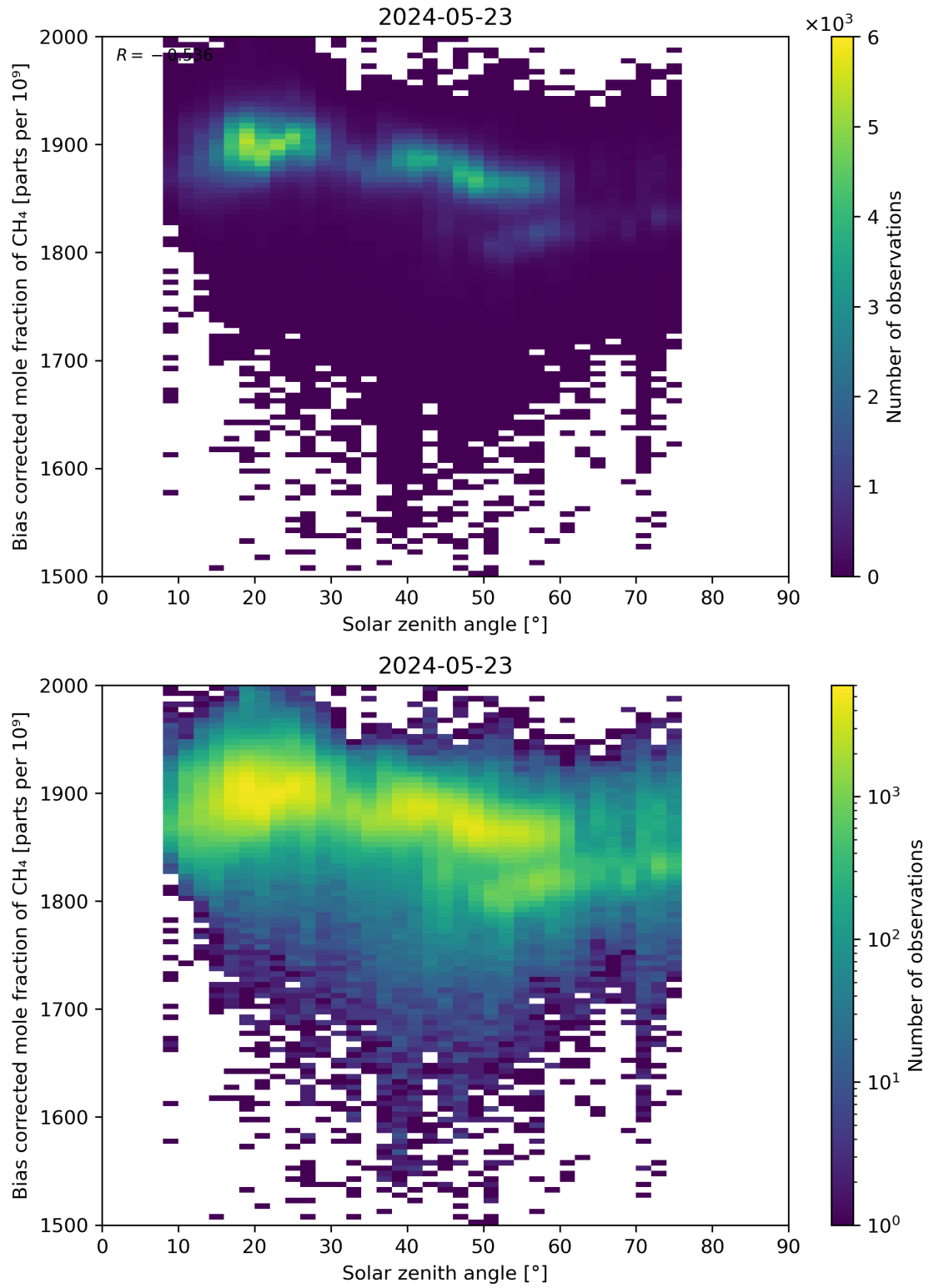
Figure 100: Scatter density plot of “Solar zenith angle” against “Bias corrected mole fraction of CH 4 ” for 2024-05-23 to 2024-05-24.
