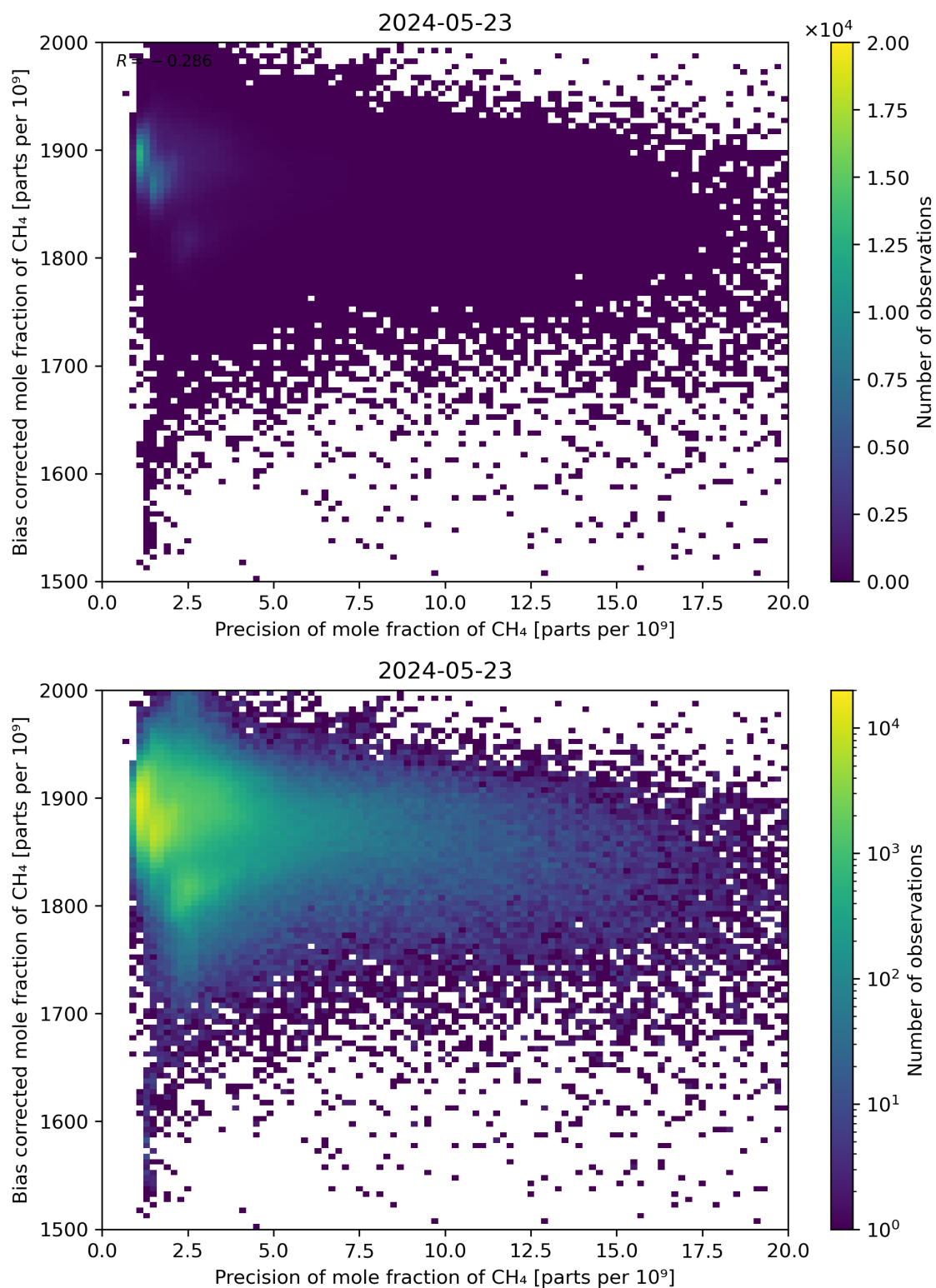
Figure 82: Scatter density plot of “Precision of mole fraction of CH 4 ” against “Bias corrected mole fraction of CH 4 ” for 2024-05-23 to 2024-05-24.
