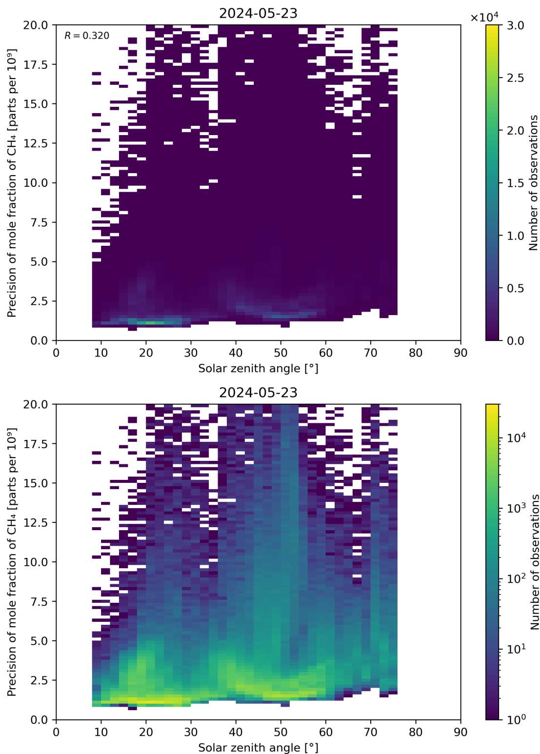
Figure 101: Scatter density plot of “Solar zenith angle” against “Precision of mole fraction of \text{CH}_4 ” for 2024-05-23 to 2024-05-24.
