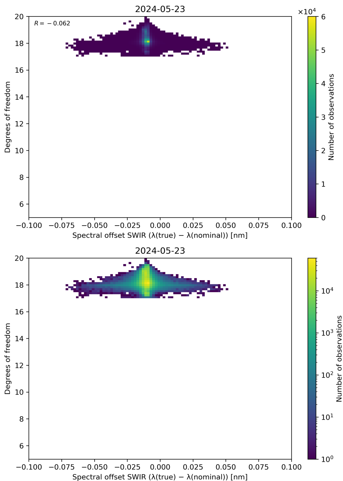
Figure 119: Scatter density plot of “Spectral offset SWIR ( \lambda(\text{true}) - \lambda(\text{nominal}) )” against “Degrees of freedom” for 2024-05-23 to 2024-05-24.
