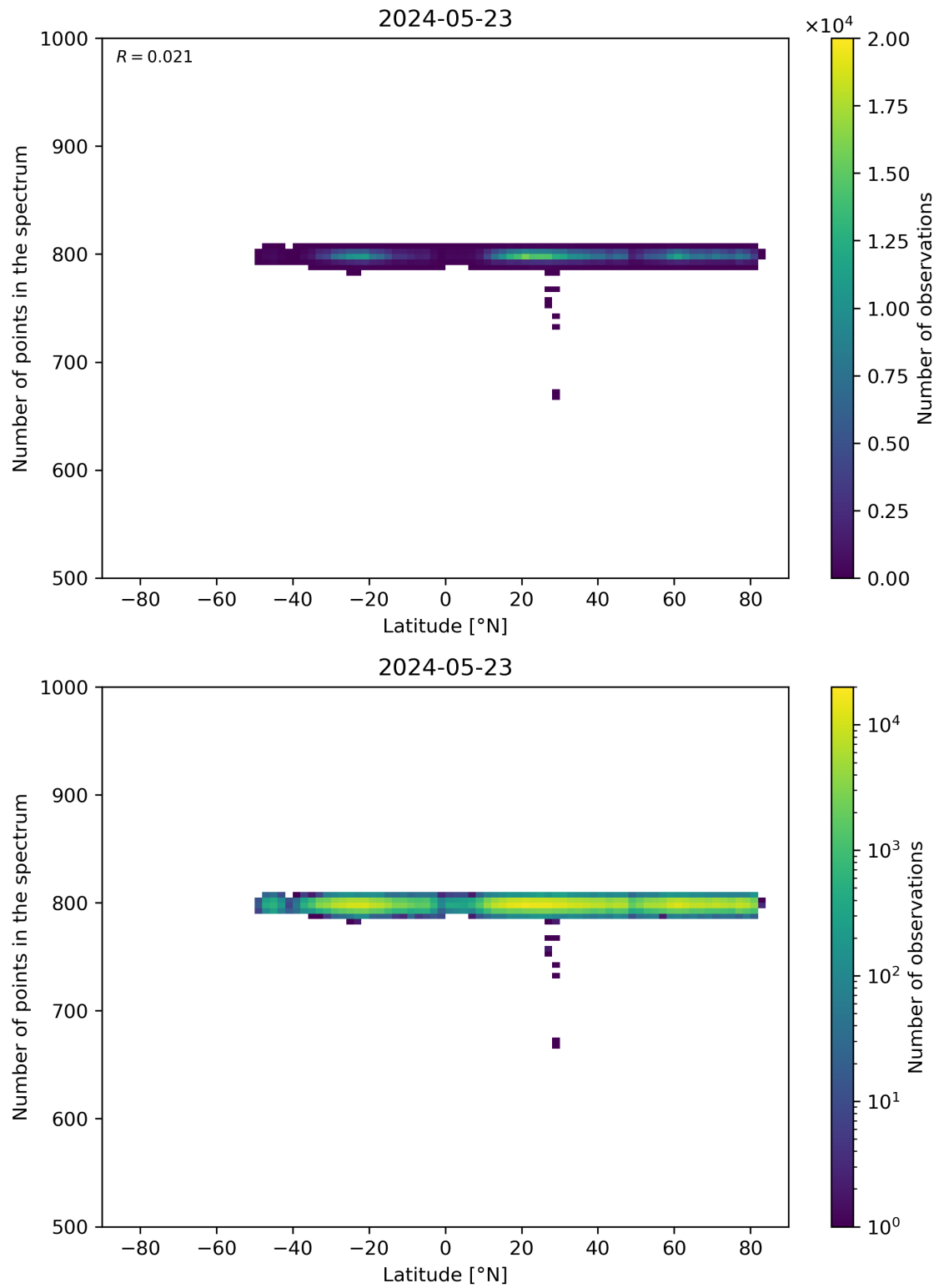
Figure 61: Scatter density plot of “Latitude” against “Number of points in the spectrum” for 2024-05-23 to 2024-05-24.
