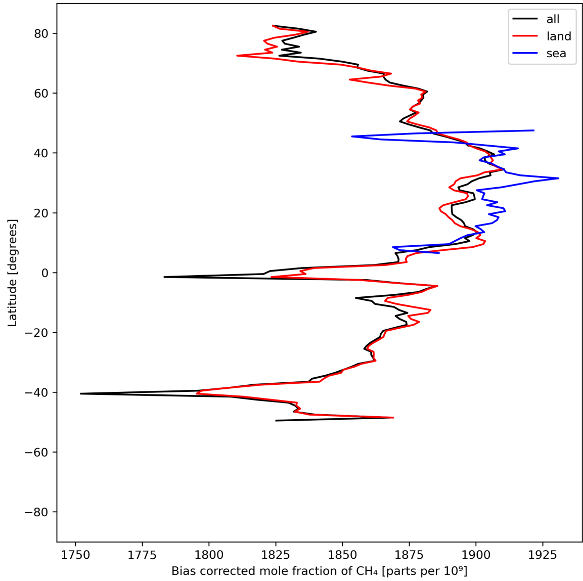
Figure 14: Zonal average of “Bias corrected mole fraction of CH 4 ” for 2024-05-23 to 2024-05-24.
