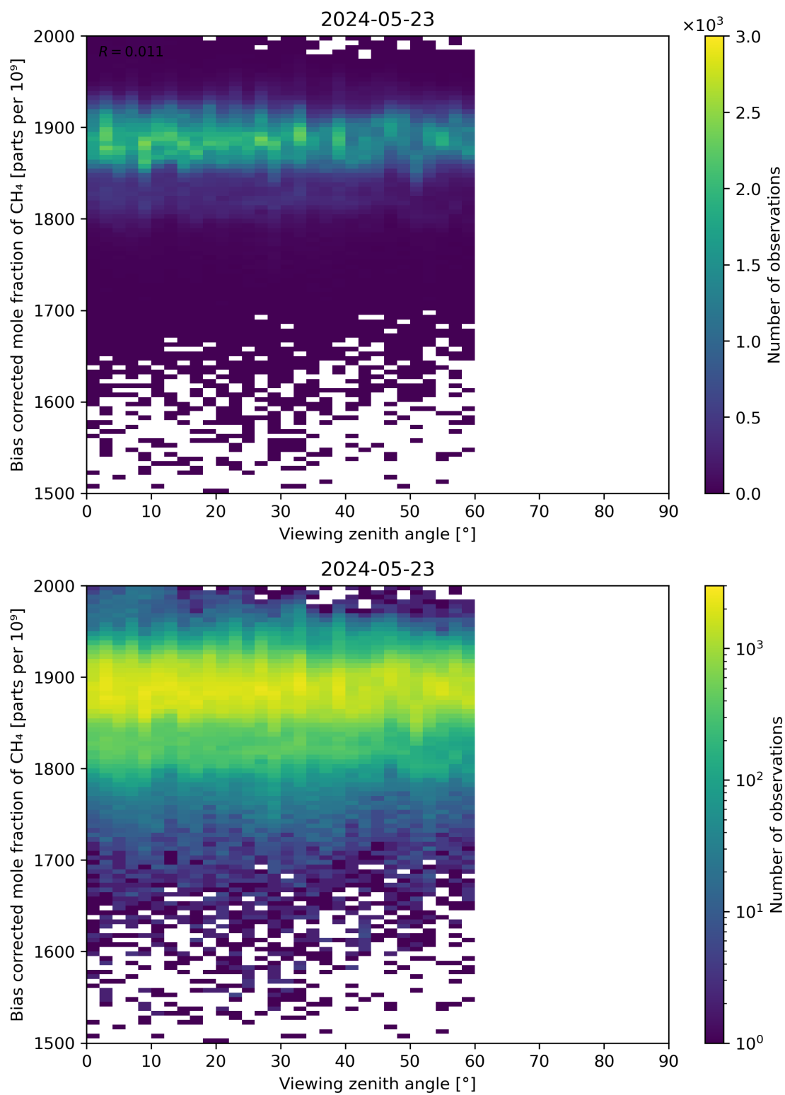
Figure 111: Scatter density plot of “Viewing zenith angle” against “Bias corrected mole fraction of CH 4 ” for 2024-05-23 to 2024-05-24.
