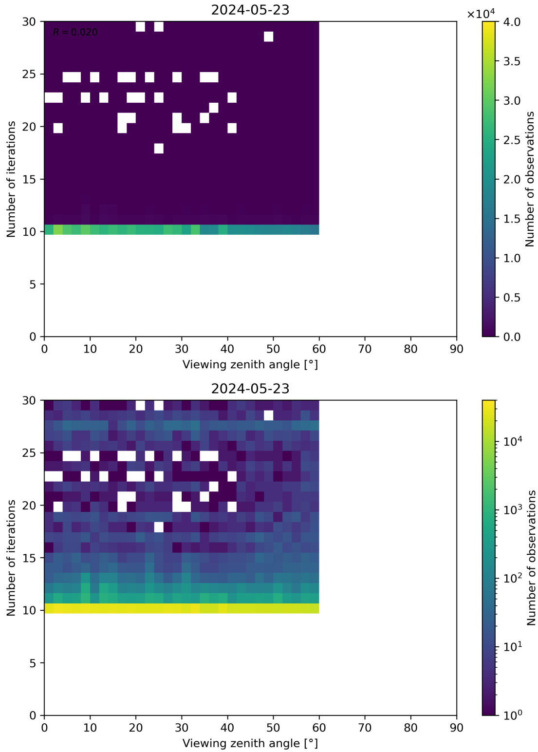
Figure 113: Scatter density plot of “Viewing zenith angle” against “Number of iterations” for 2024-05-23 to 2024-05-24.
