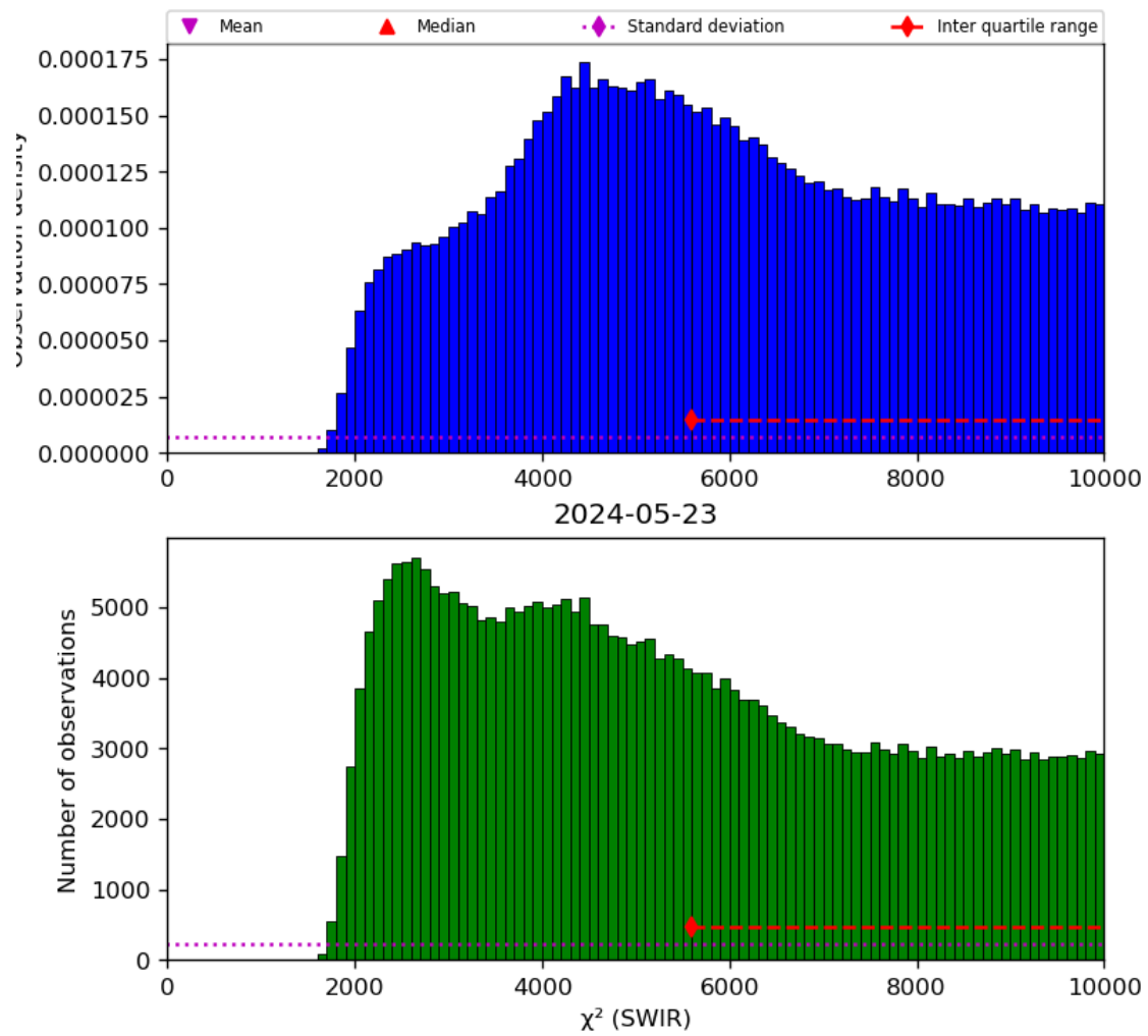
Figure 28: Histogram of “ \chi^2 (SWIR)” for 2024-05-23 to 2024-05-24
