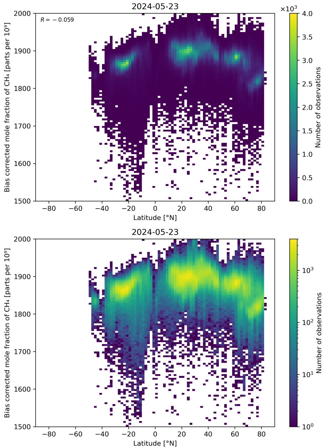
Figure 58: Scatter density plot of “Latitude” against “Bias corrected mole fraction of \text{CH}_4 ” for 2024-05-23 to 2024-05-24.
