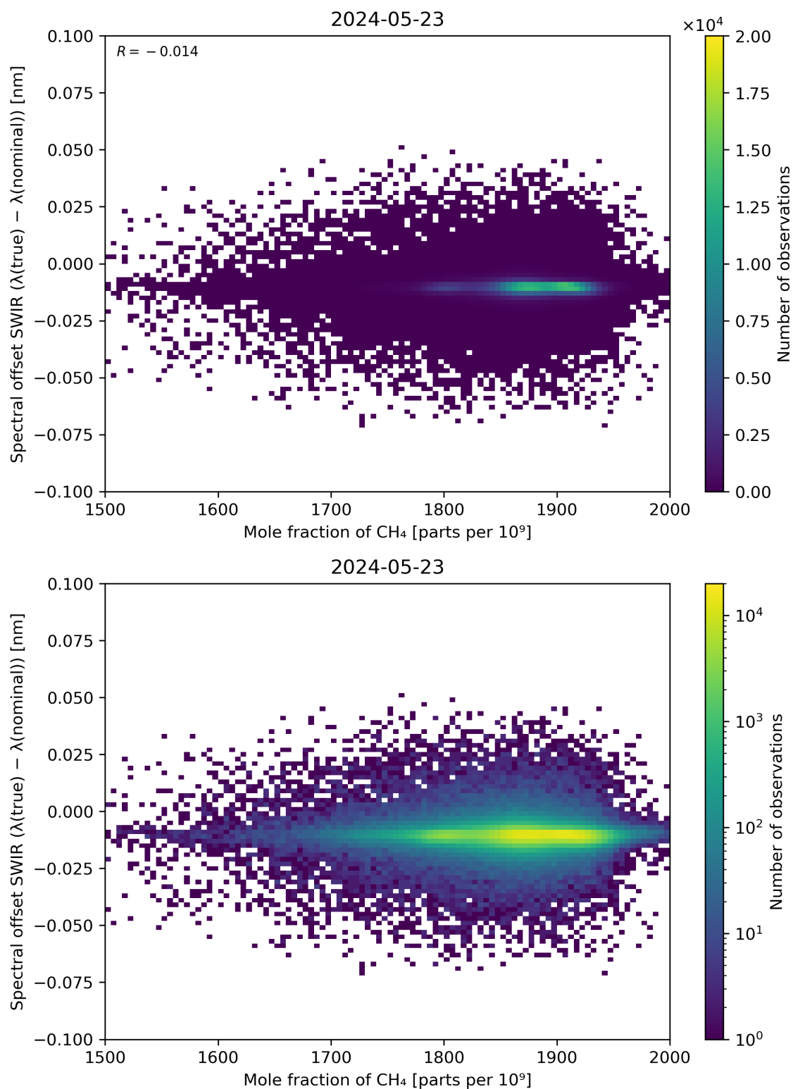
Figure 86: Scatter density plot of “Mole fraction of CH 4 ” against “Spectral offset SWIR ( \lambda(\text{true}) - \lambda(\text{nominal}) )” for 2024-05-23 to 2024-05-24.
