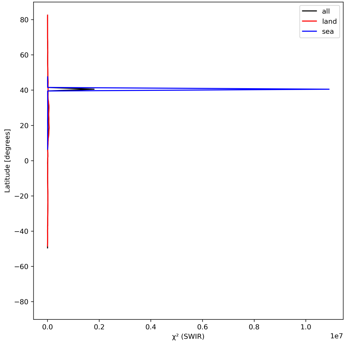
Figure 17: Zonal average of “ \chi^2 (SWIR)” for 2024-05-23 to 2024-05-24.
