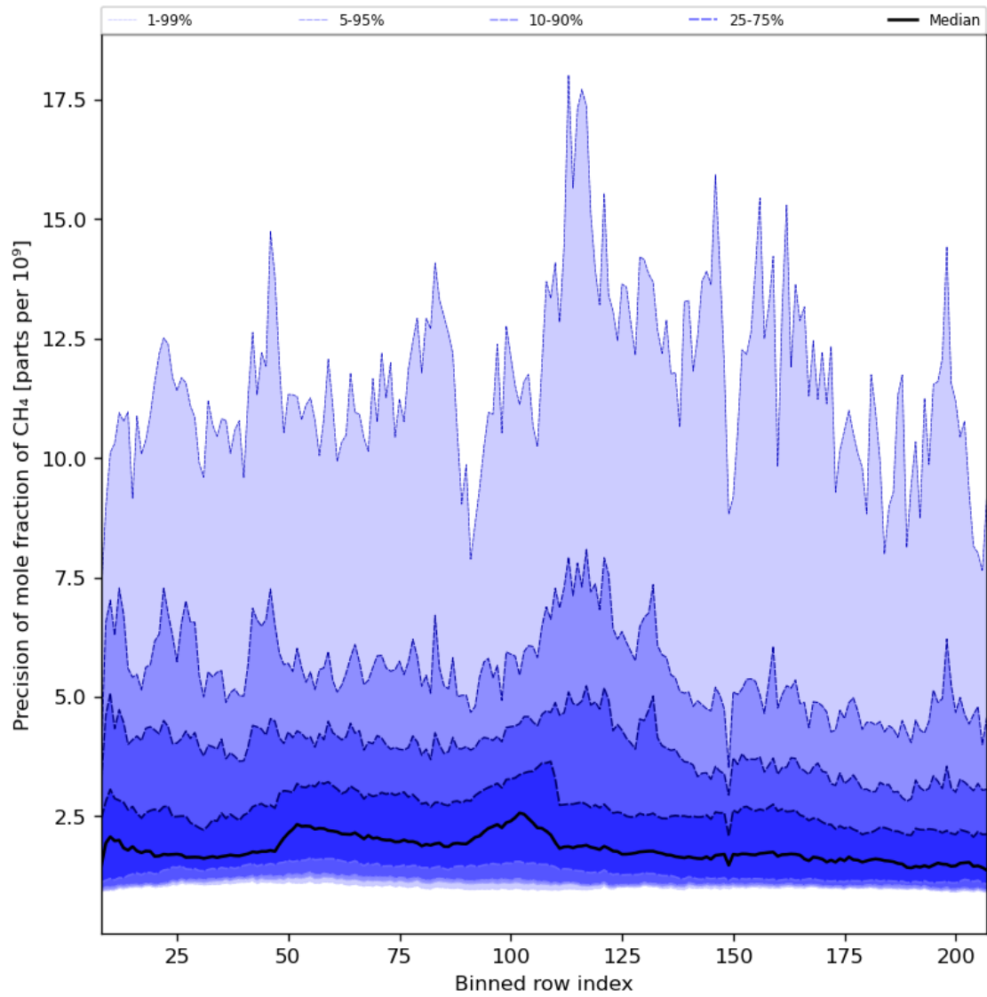
Figure 35: Along track statistics of “Precision of mole fraction of CH 4 ” for 2024-05-23 to 2024-05-24
