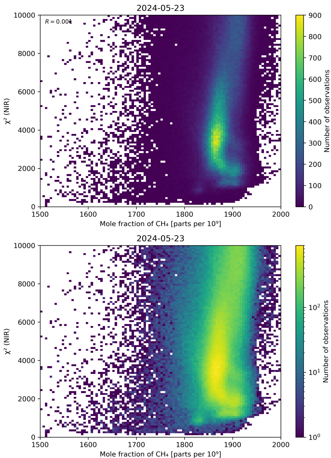
Figure 70: Scatter density plot of “Mole fraction of CH 4 ” against “ \chi^2 (NIR)” for 2024-05-23 to 2024-05-24.
