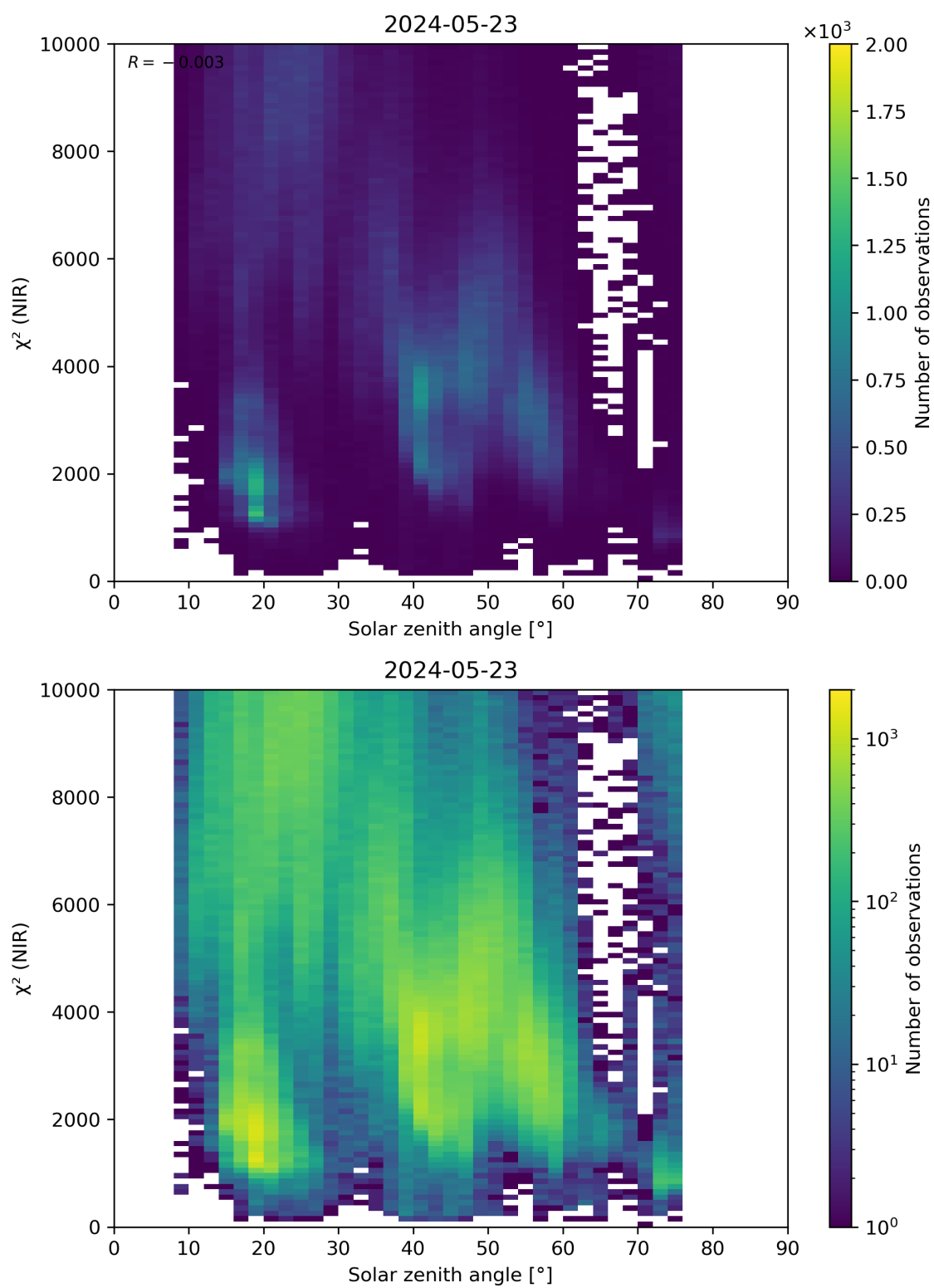
Figure 94: Scatter density plot of “Solar zenith angle” against “ \chi^2 (NIR)” for 2024-05-23 to 2024-05-24.
