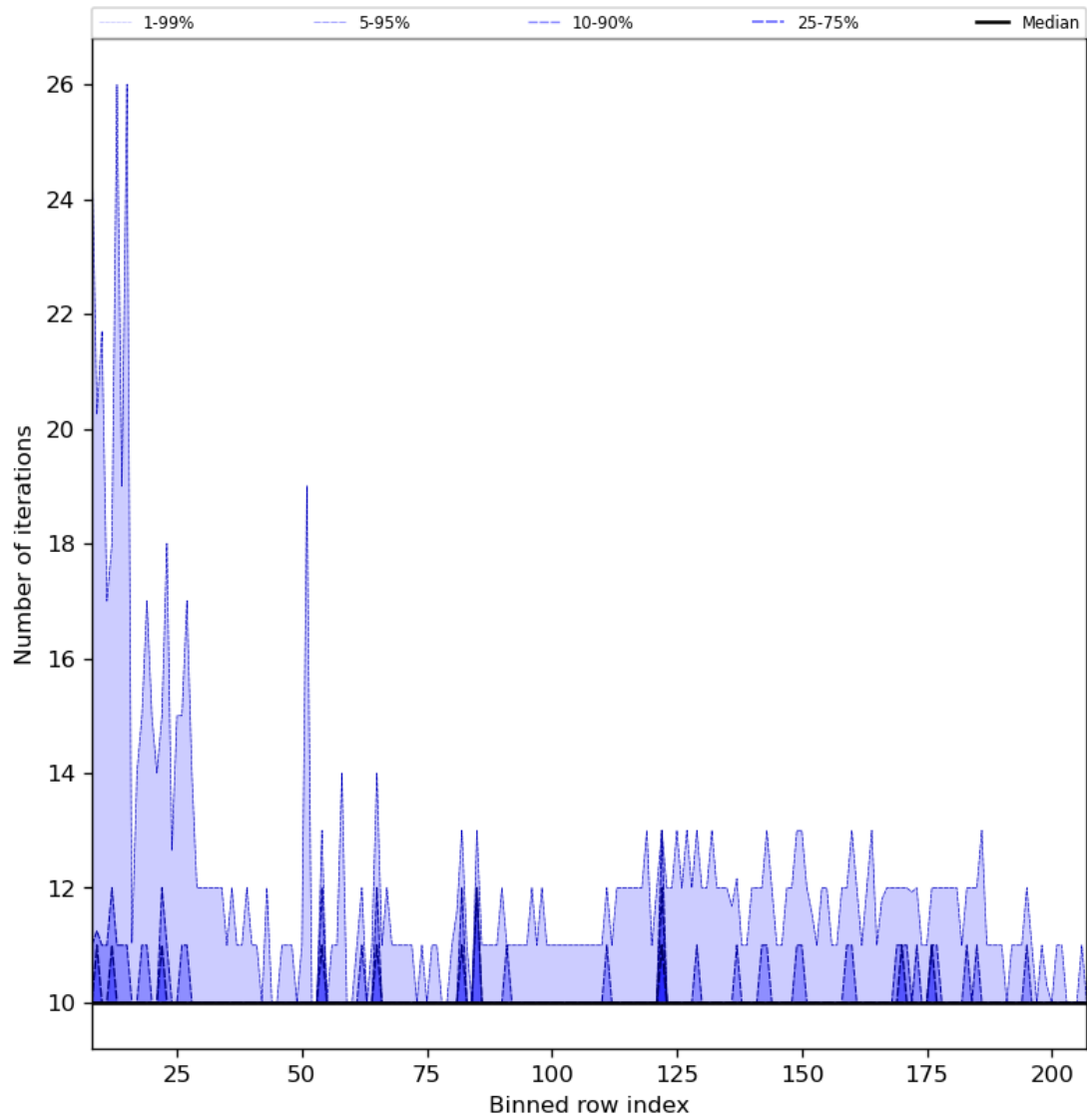
Figure 42: Along track statistics of “Number of iterations” for 2024-05-23 to 2024-05-24
