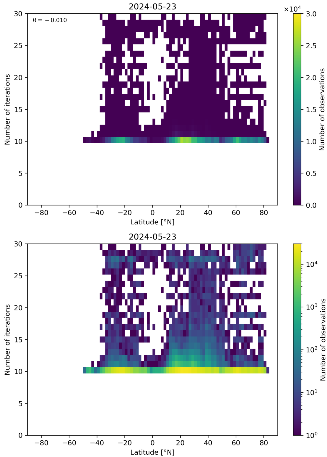
Figure 60: Scatter density plot of “Latitude” against “Number of iterations” for 2024-05-23 to 2024-05-24.
