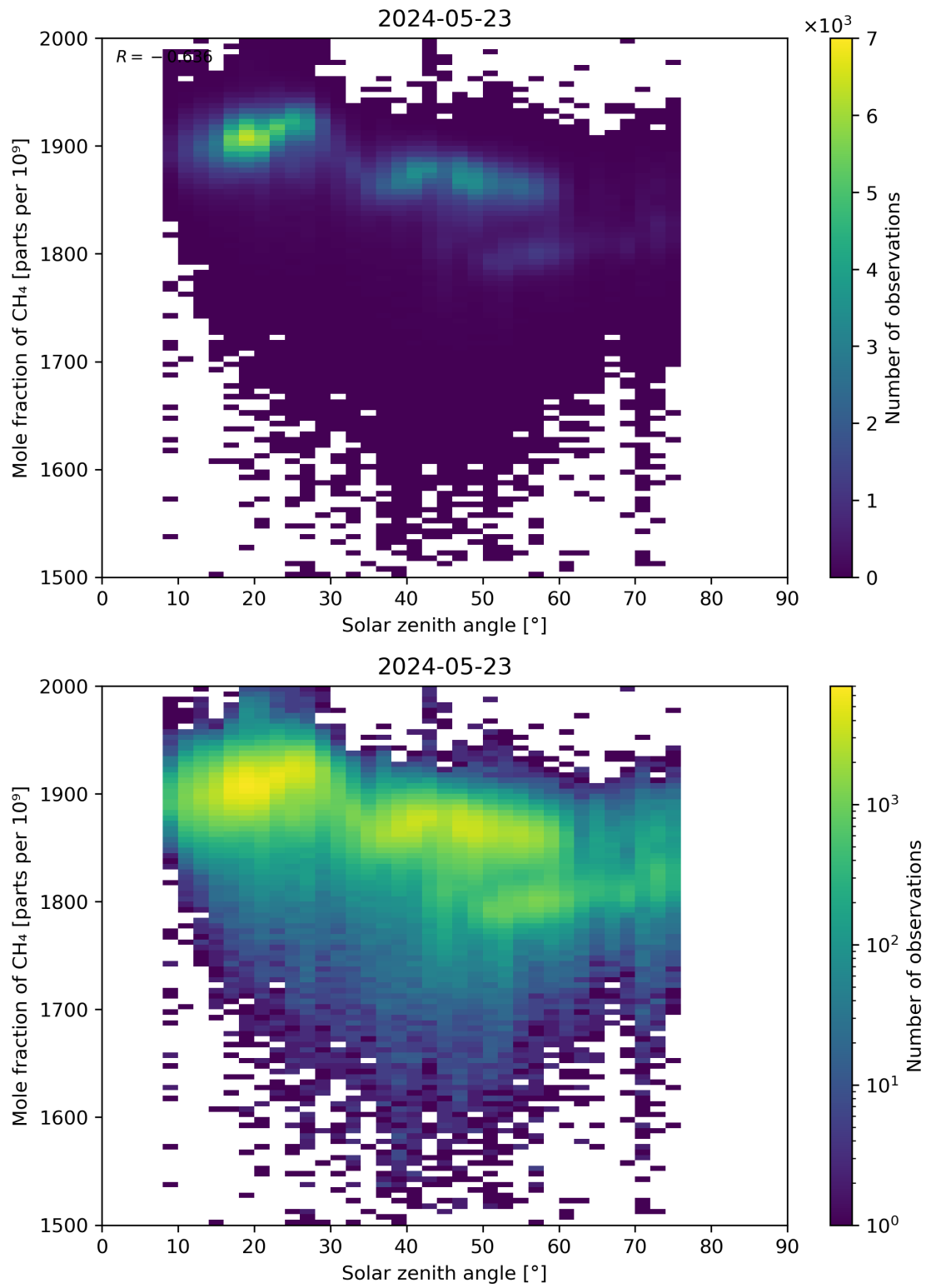
Figure 99: Scatter density plot of “Solar zenith angle” against “Mole fraction of CH 4 ” for 2024-05-23 to 2024-05-24.
