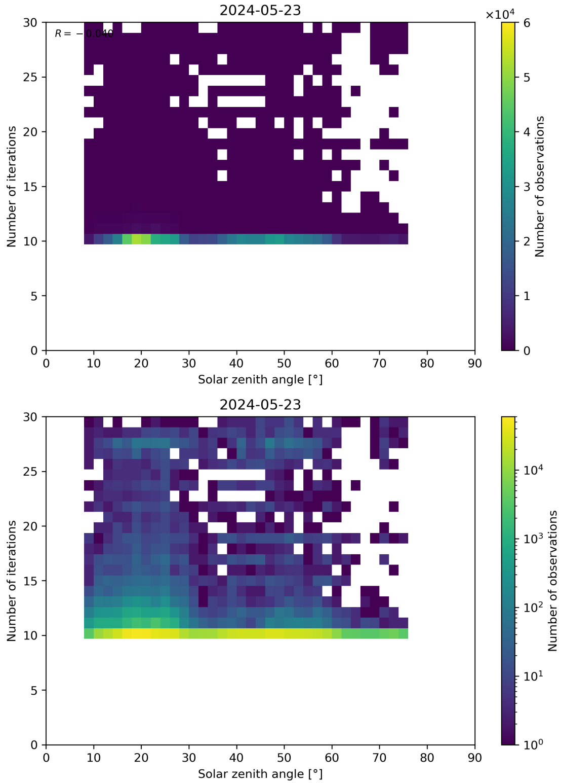
Figure 102: Scatter density plot of “Solar zenith angle” against “Number of iterations” for 2024-05-23 to 2024-05-24.
