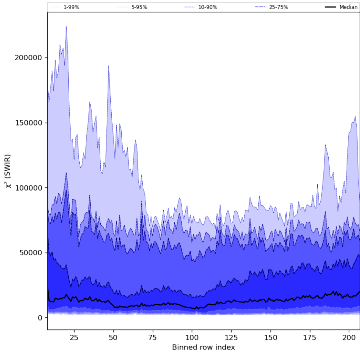
Figure 39: Along track statistics of " \chi^2 (SWIR)" for 2024-05-23 to 2024-05-24
