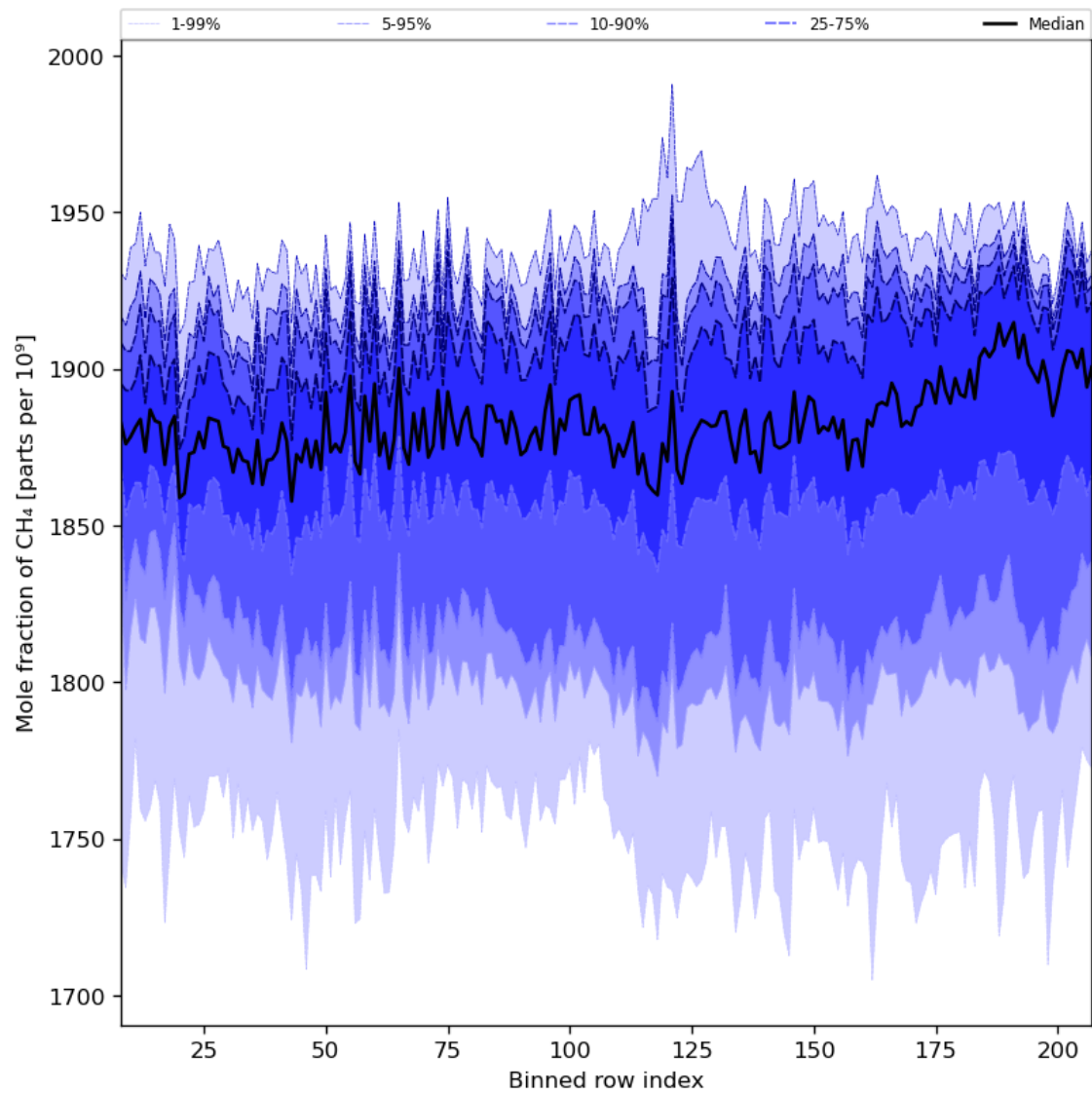
Figure 34: Along track statistics of “Mole fraction of CH 4 ” for 2024-05-23 to 2024-05-24
