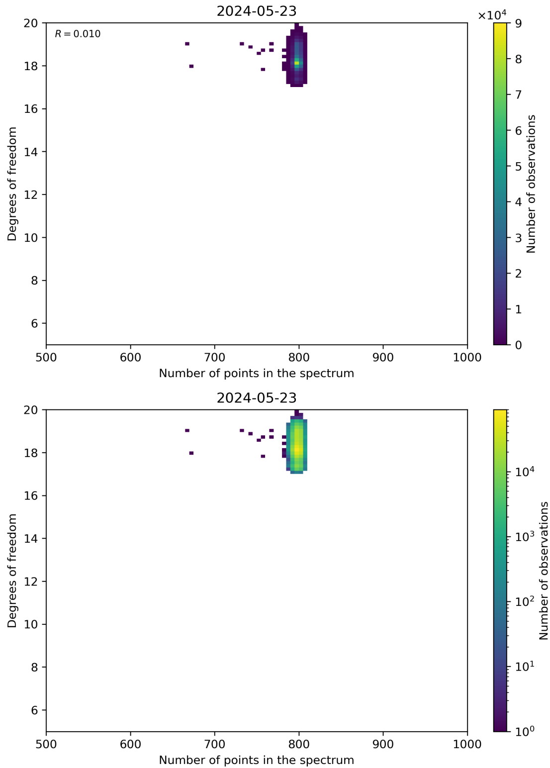
Figure 90: Scatter density plot of “Number of points in the spectrum” against “Degrees of freedom” for 2024-05-23 to 2024-05-24.
