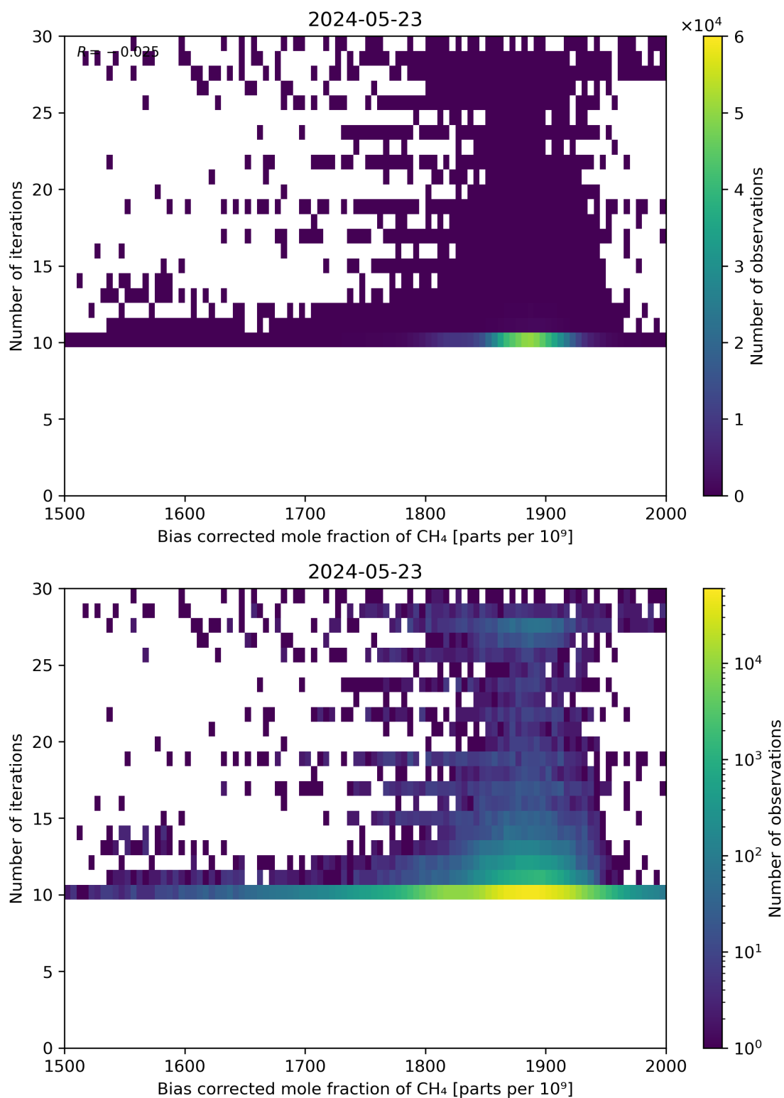
Figure 67: Scatter density plot of “Bias corrected mole fraction of CH 4 ” against “Number of iterations” for 2024-05-23 to 2024-05-24.
