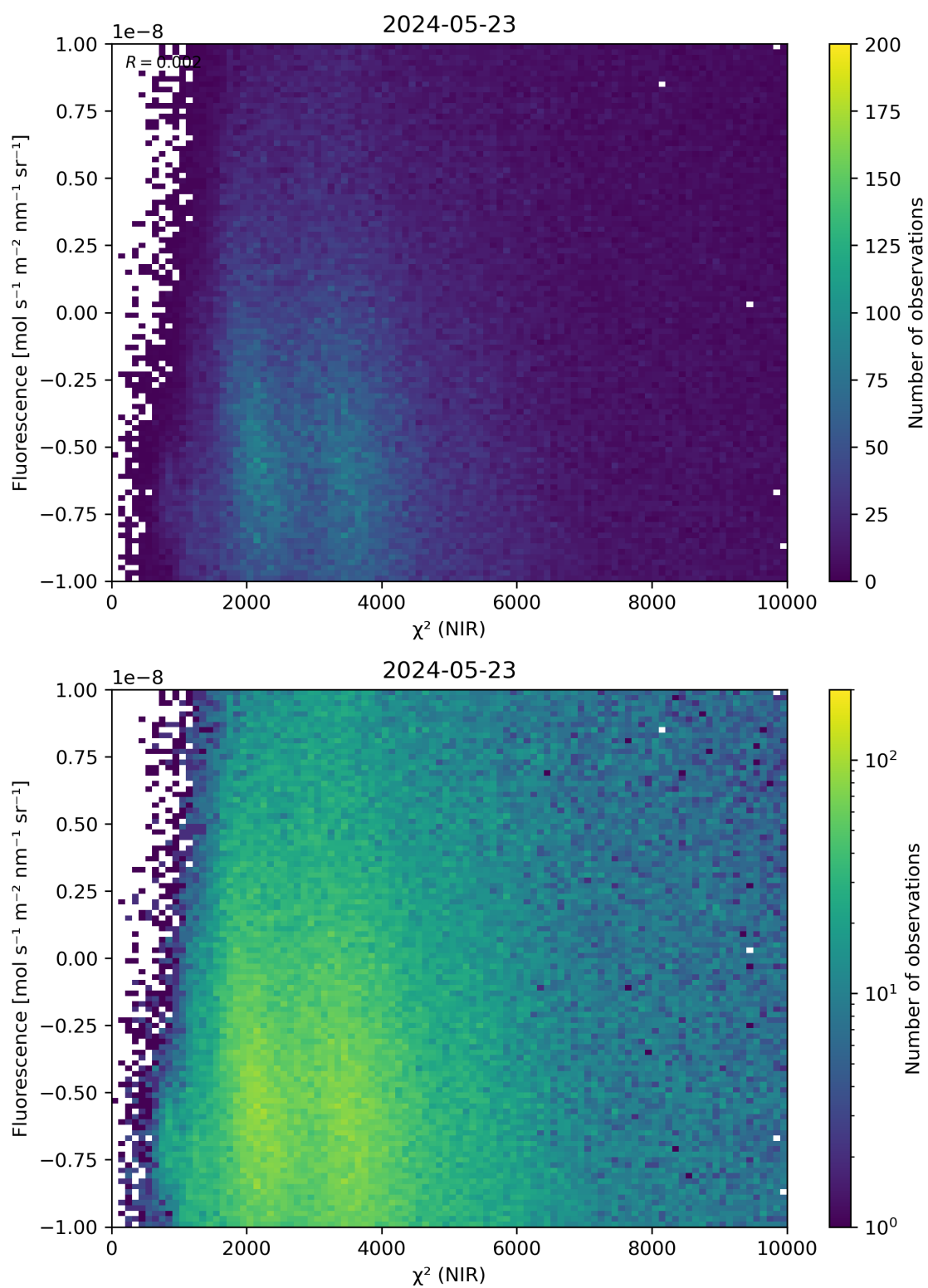
Figure 45: Scatter density plot of “ \chi^2 (NIR)” against “Fluorescence” for 2024-05-23 to 2024-05-24.
