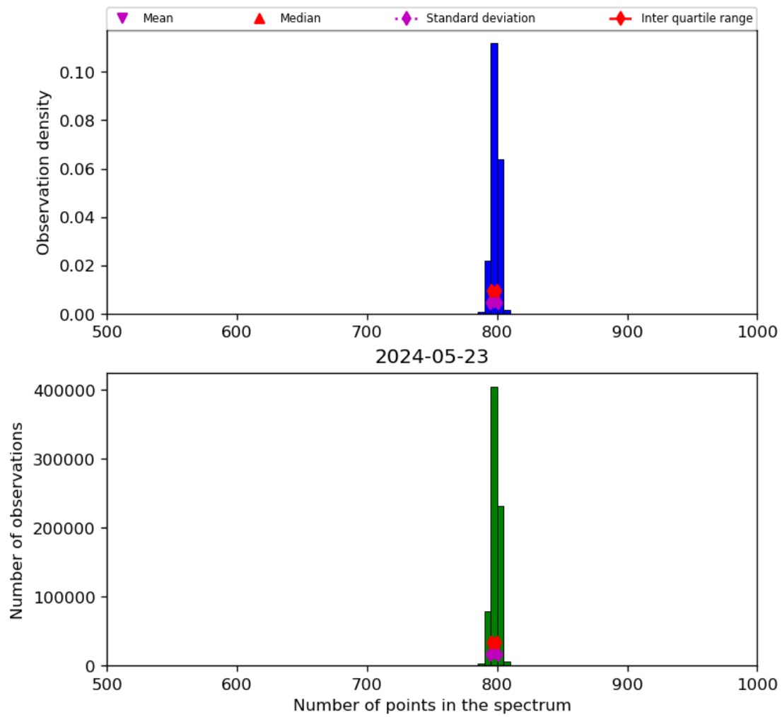
Figure 26: Histogram of “Number of points in the spectrum” for 2024-05-23 to 2024-05-24
