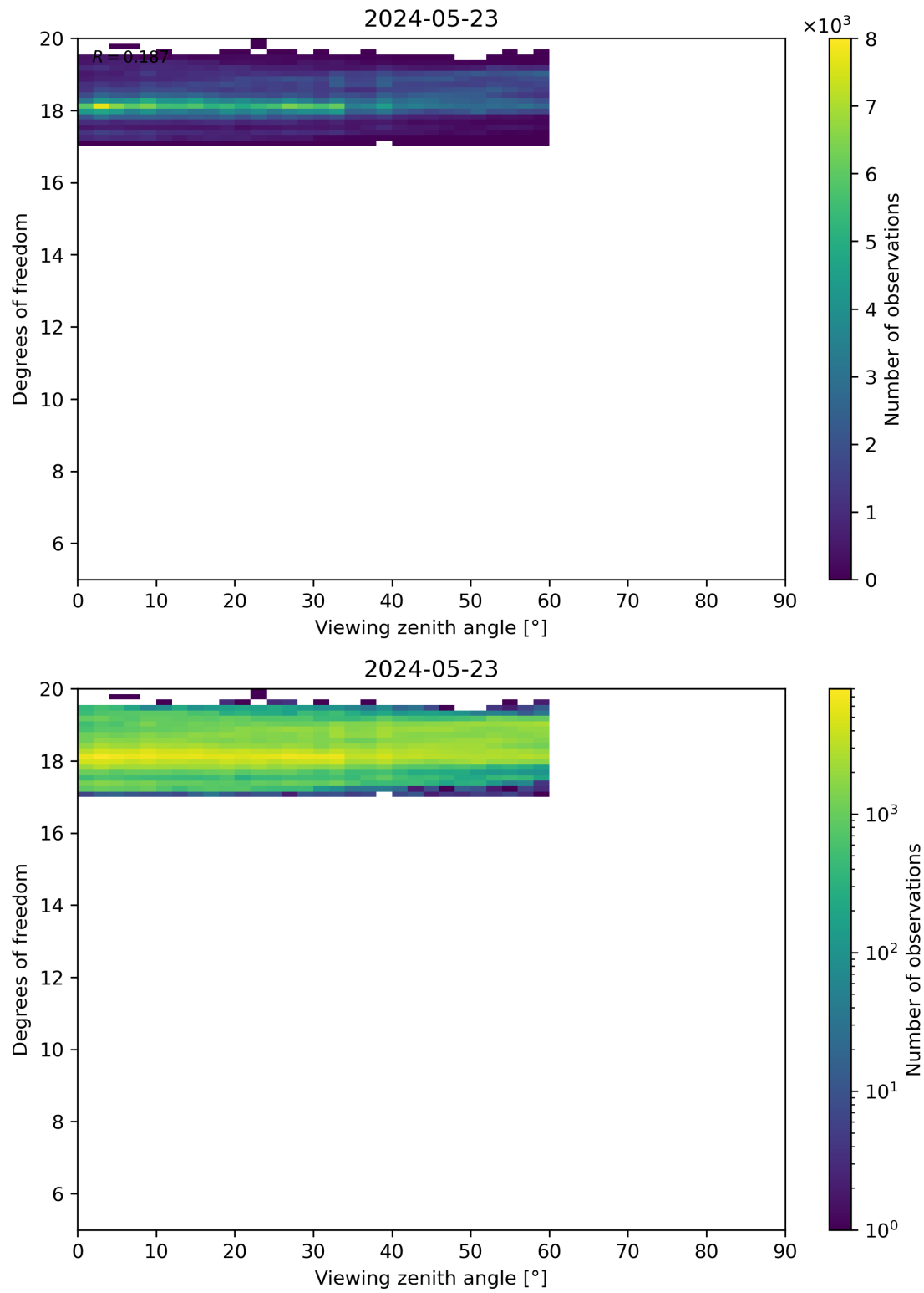
Figure 107: Scatter density plot of “Viewing zenith angle” against “Degrees of freedom” for 2024-05-23 to 2024-05-24.
