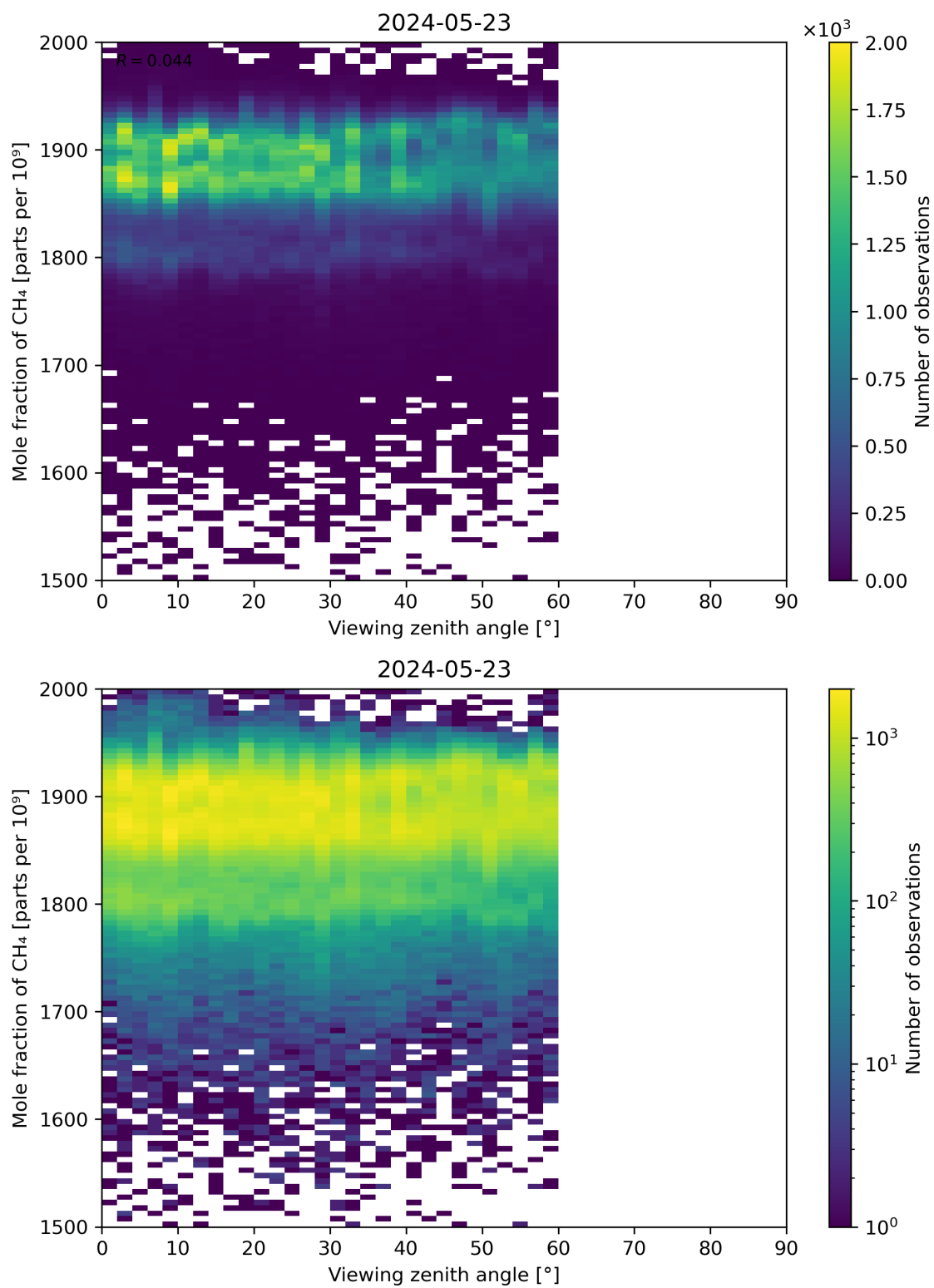
Figure 110: Scatter density plot of “Viewing zenith angle” against “Mole fraction of CH 4 ” for 2024-05-23 to 2024-05-24.
