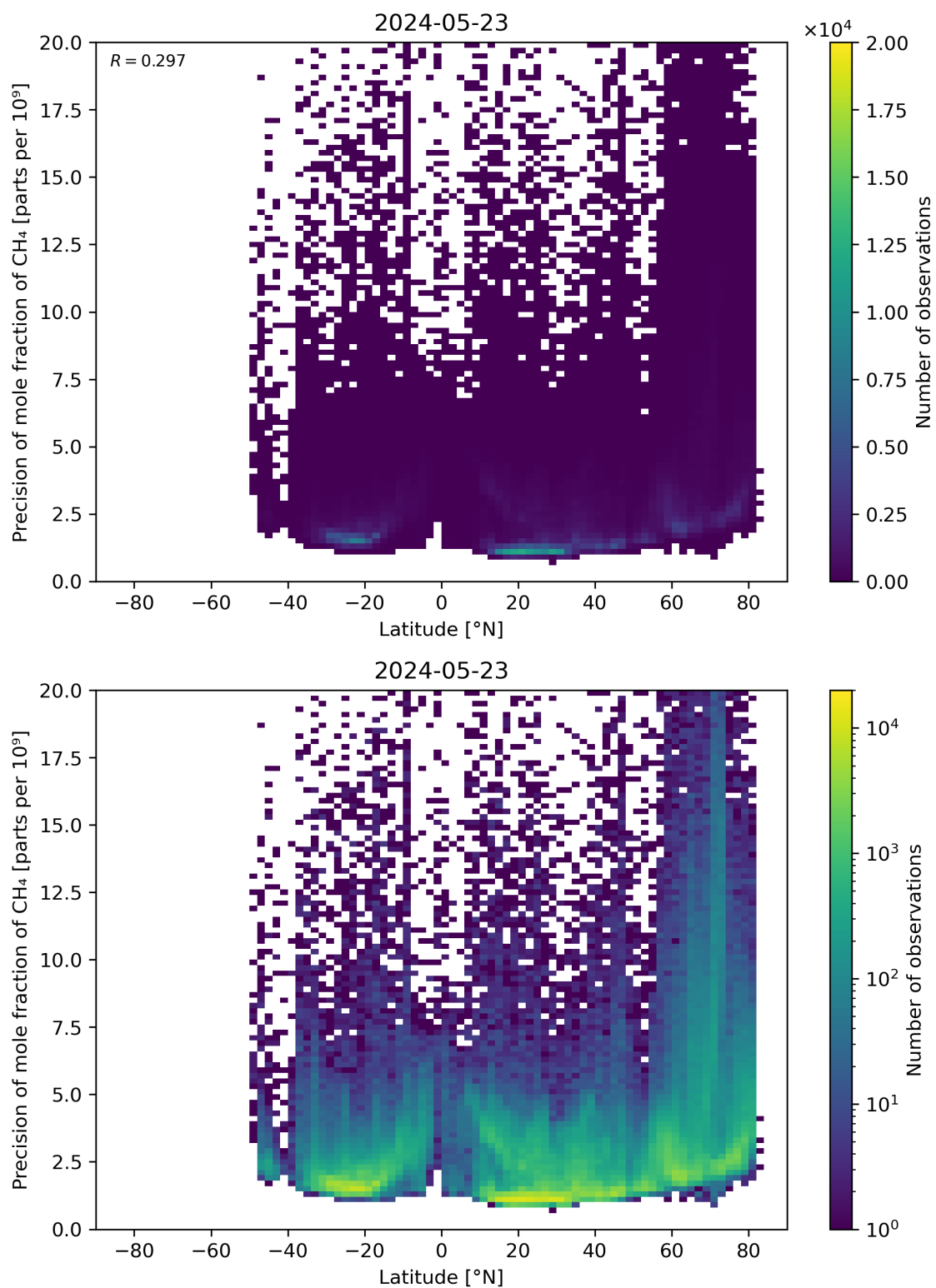
Figure 59: Scatter density plot of “Latitude” against “Precision of mole fraction of \text{CH}_4 ” for 2024-05-23 to 2024-05-24.
