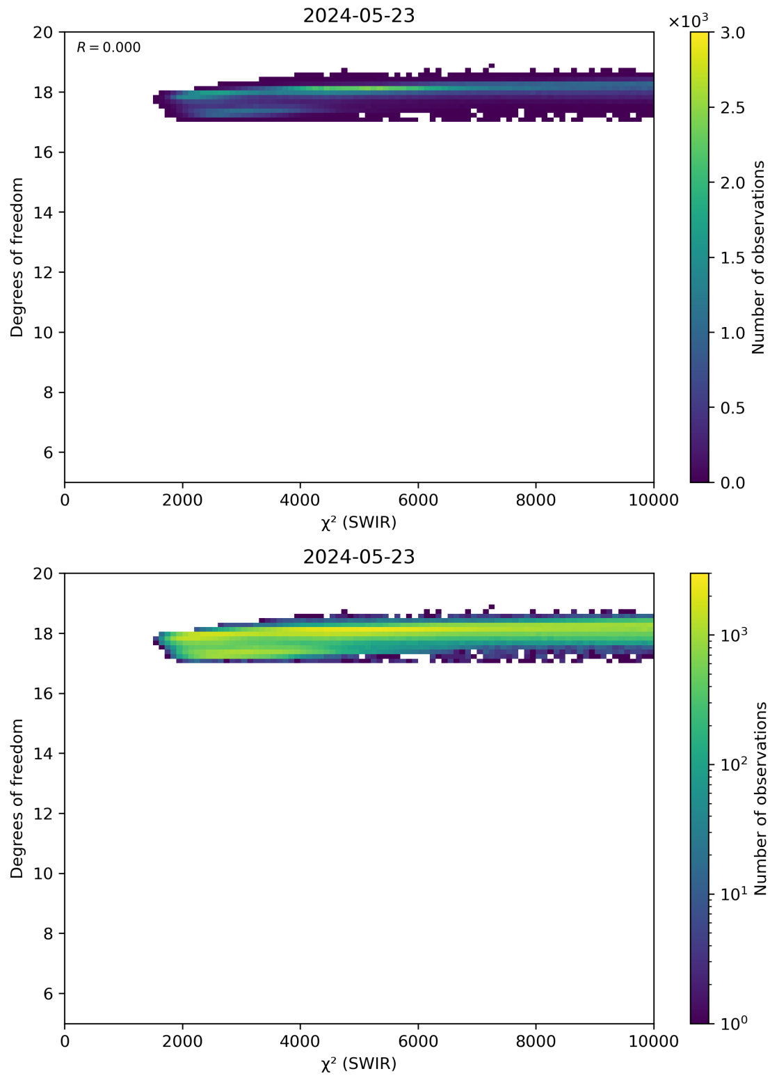
Figure 48: Scatter density plot of “ \chi^2 (SWIR)” against “Degrees of freedom” for 2024-05-23 to 2024-05-24.
