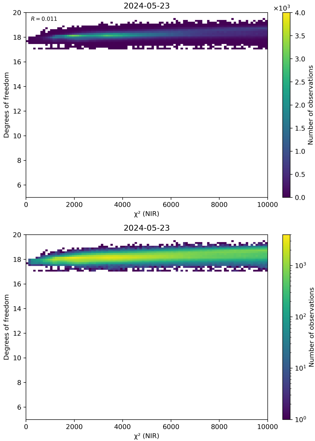
Figure 44: Scatter density plot of “ \chi^2 (NIR)” against “Degrees of freedom” for 2024-05-23 to 2024-05-24.
