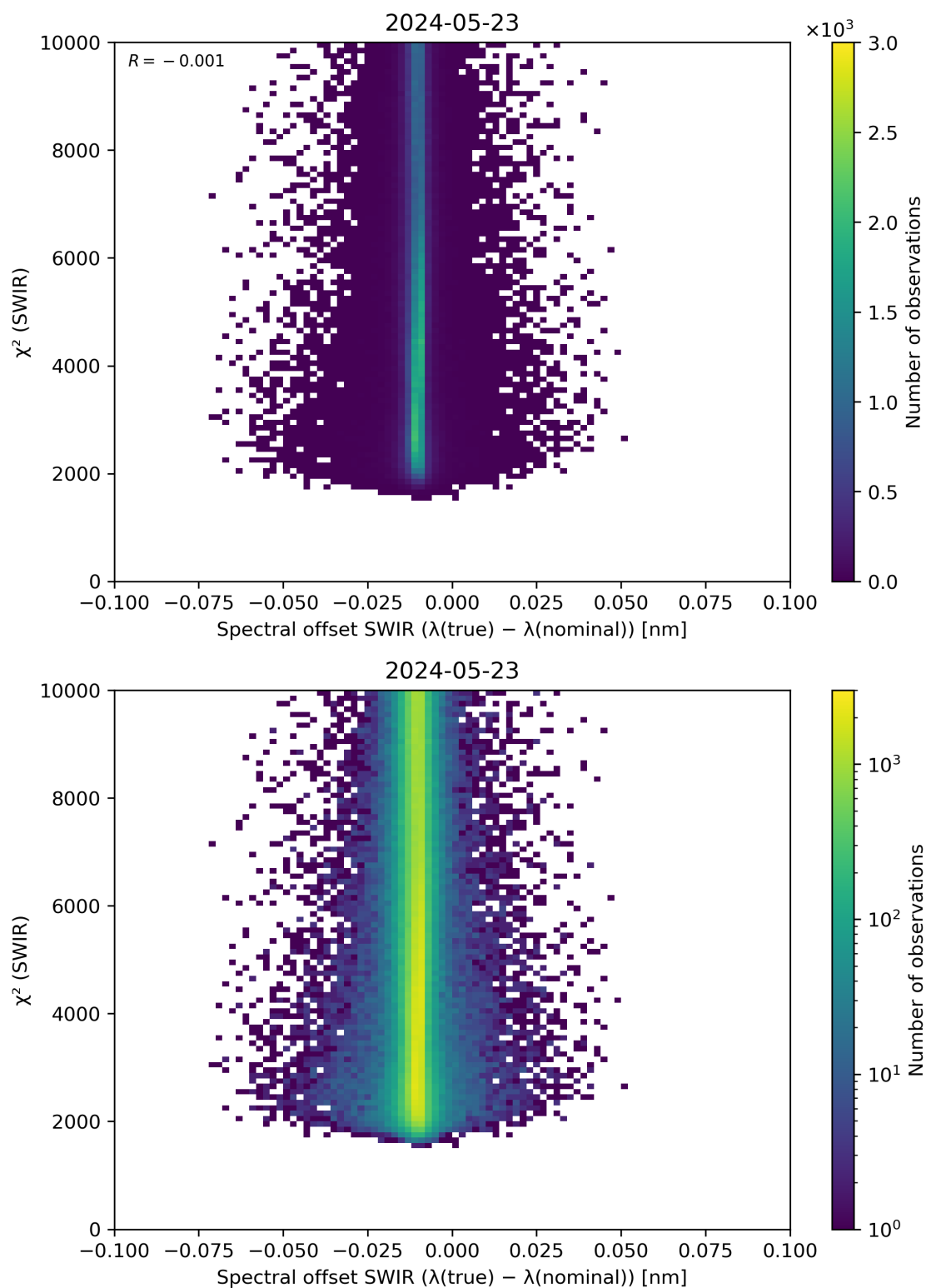
Figure 118: Scatter density plot of “Spectral offset SWIR ( \lambda(\text{true}) - \lambda(\text{nominal}) )” against “ \chi^2 (SWIR)” for 2024-05-23 to 2024-05-24.
